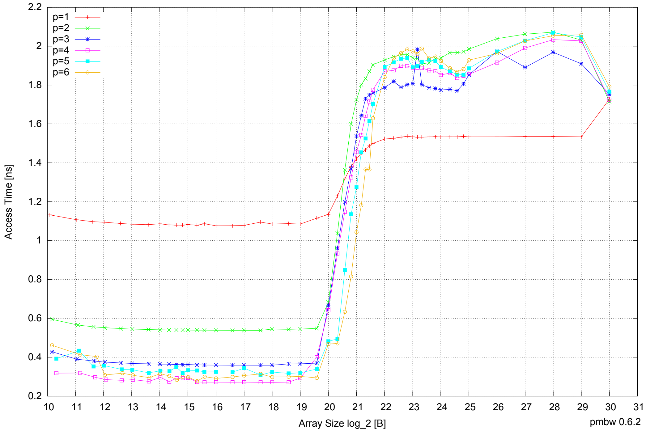
Samsung Galaxy Note 10.1 GT-N8010: Exynos 4412 Quad-Core 2GB - Parallel Memory Access Time - ScanWrite32PtrSimpleLoop
