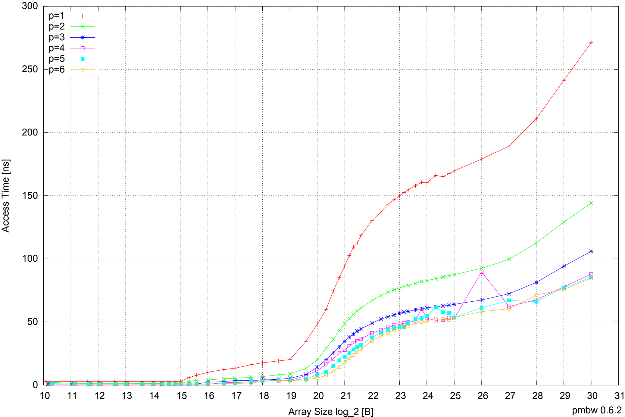
Samsung Galaxy Note 10.1 GT-N8010: Exynos 4412 Quad-Core 2GB - Parallel Memory Access Time - PermRead32SimpleLoop
