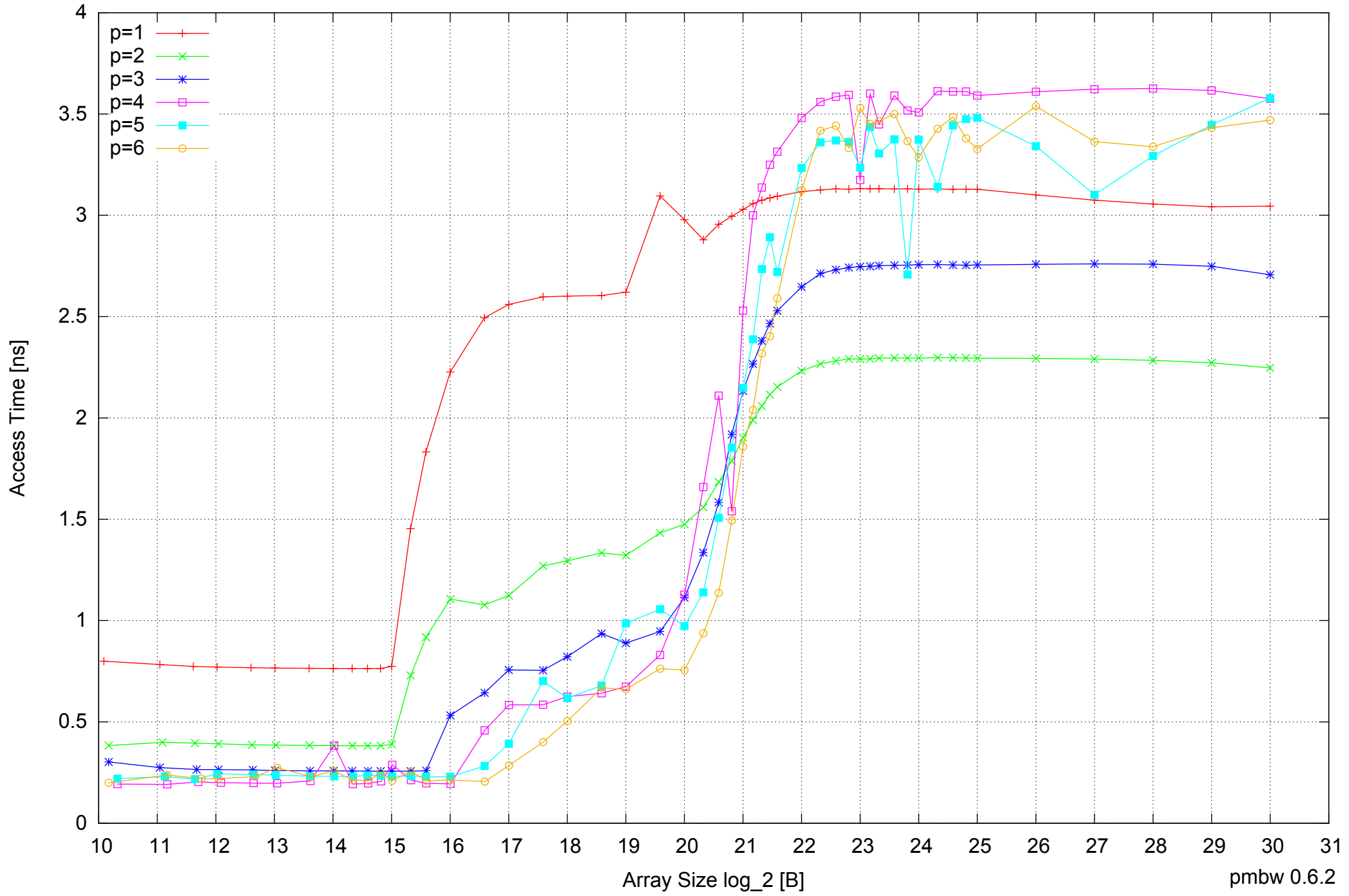
Samsung Galaxy Note 10.1 GT-N8010: Exynos 4412 Quad-Core 2GB - Parallel Memory Access Time - ScanRead32PtrUnrollLoop
