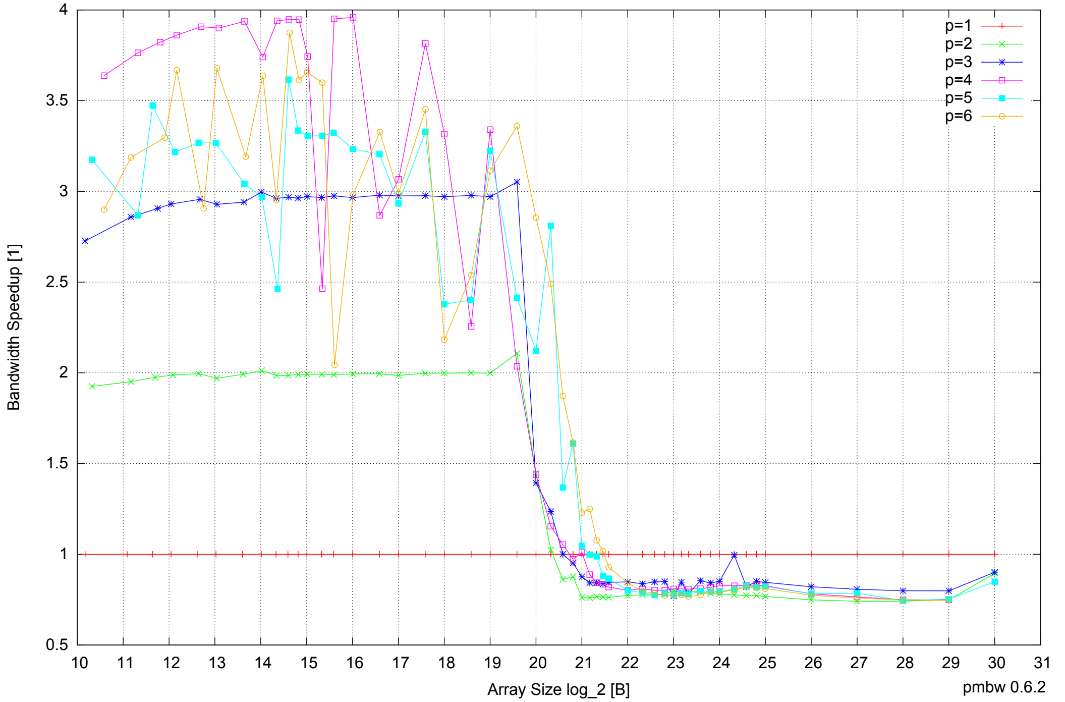
Samsung Galaxy Note 10.1 GT-N8010: Exynos 4412 Quad-Core 2GB - Speedup of Parallel Memory Bandwidth - ScanWrite64PtrSimpleLoop
