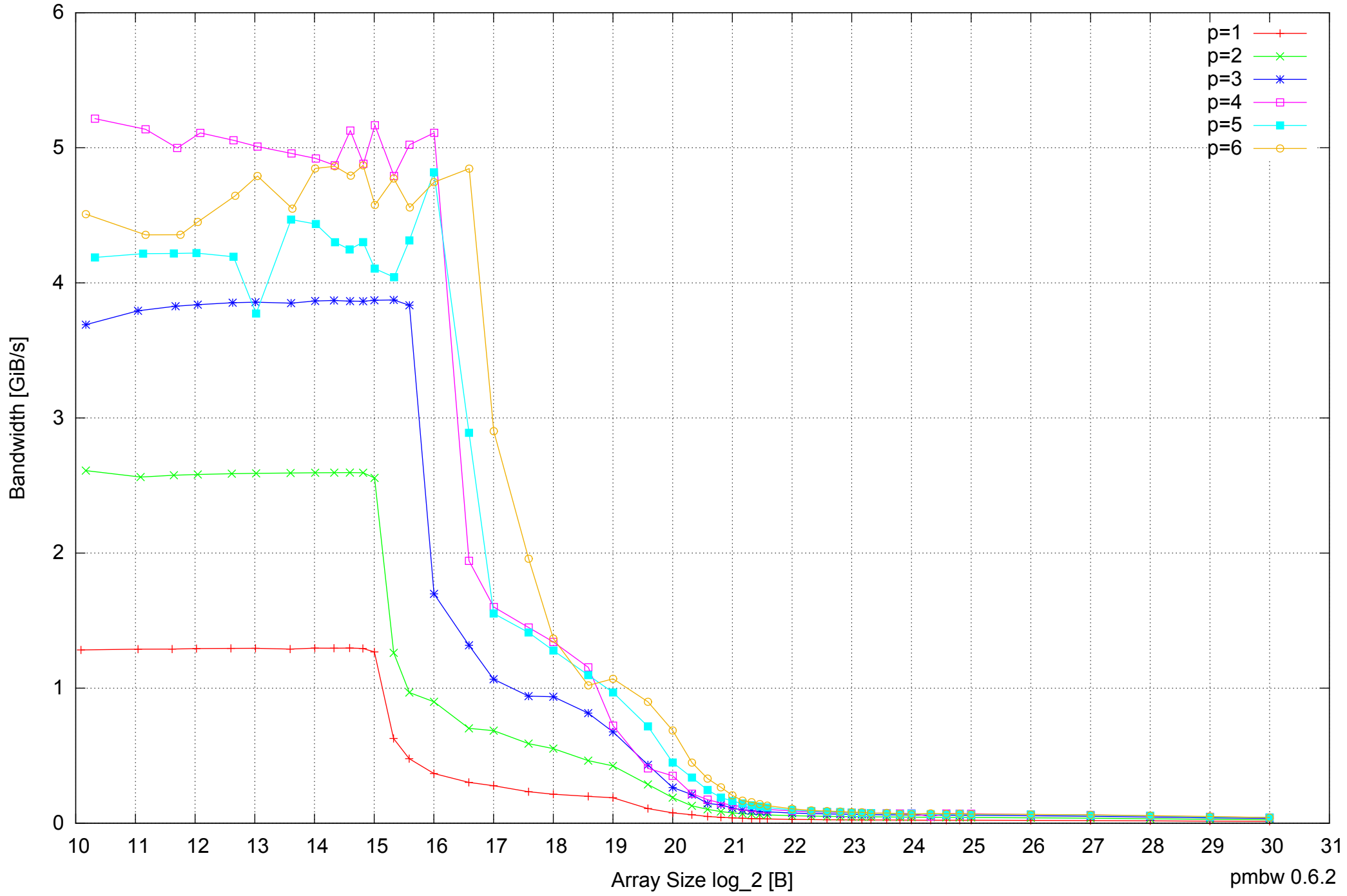
Samsung Galaxy Note 10.1 GT-N8010: Exynos 4412 Quad-Core 2GB - Parallel Memory Bandwidth - PermRead32UnrollLoop
