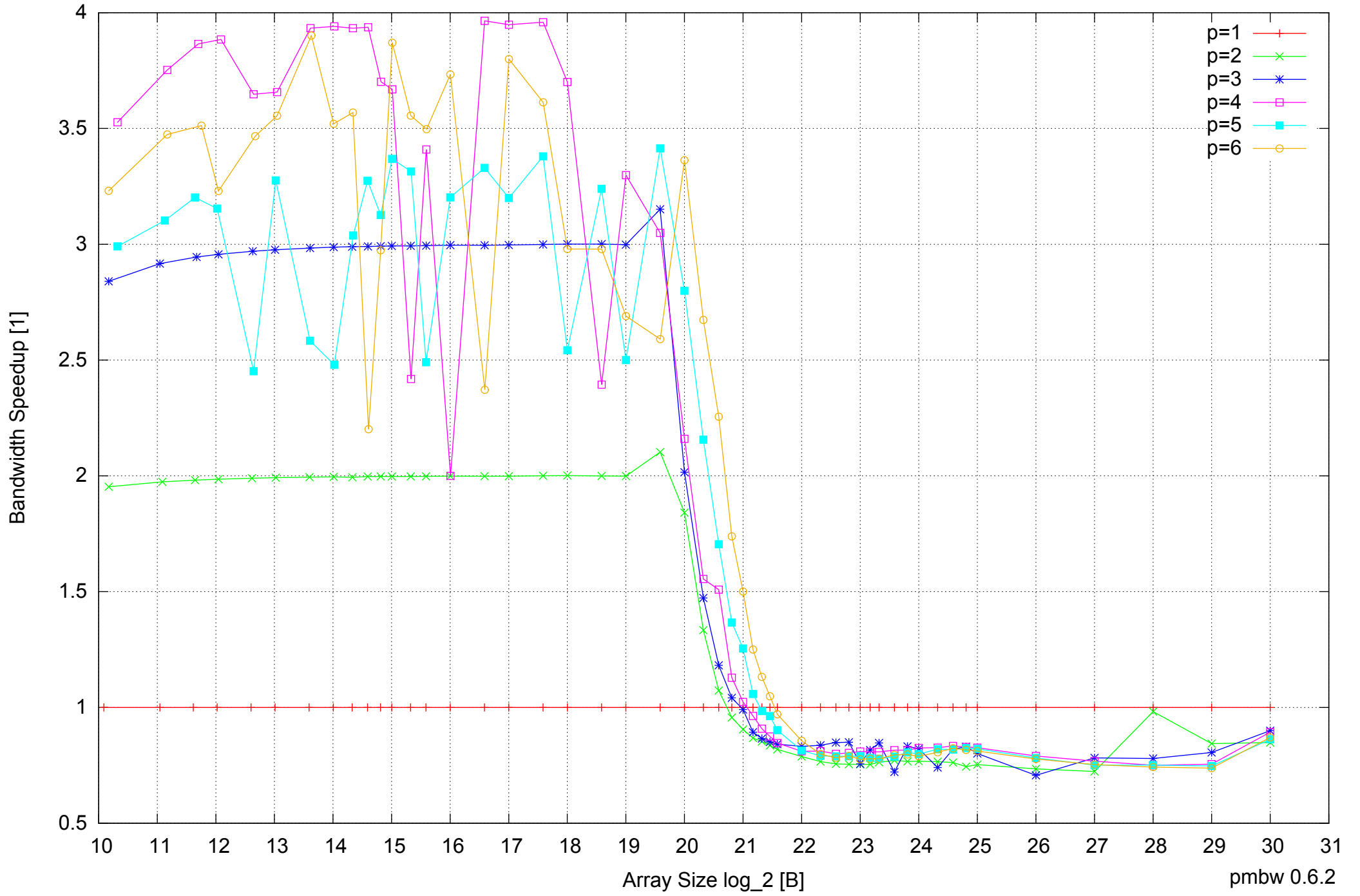
Samsung Galaxy Note 10.1 GT-N8010: Exynos 4412 Quad-Core 2GB - Speedup of Parallel Memory Bandwidth - ScanWrite32IndexSimpleLoop
