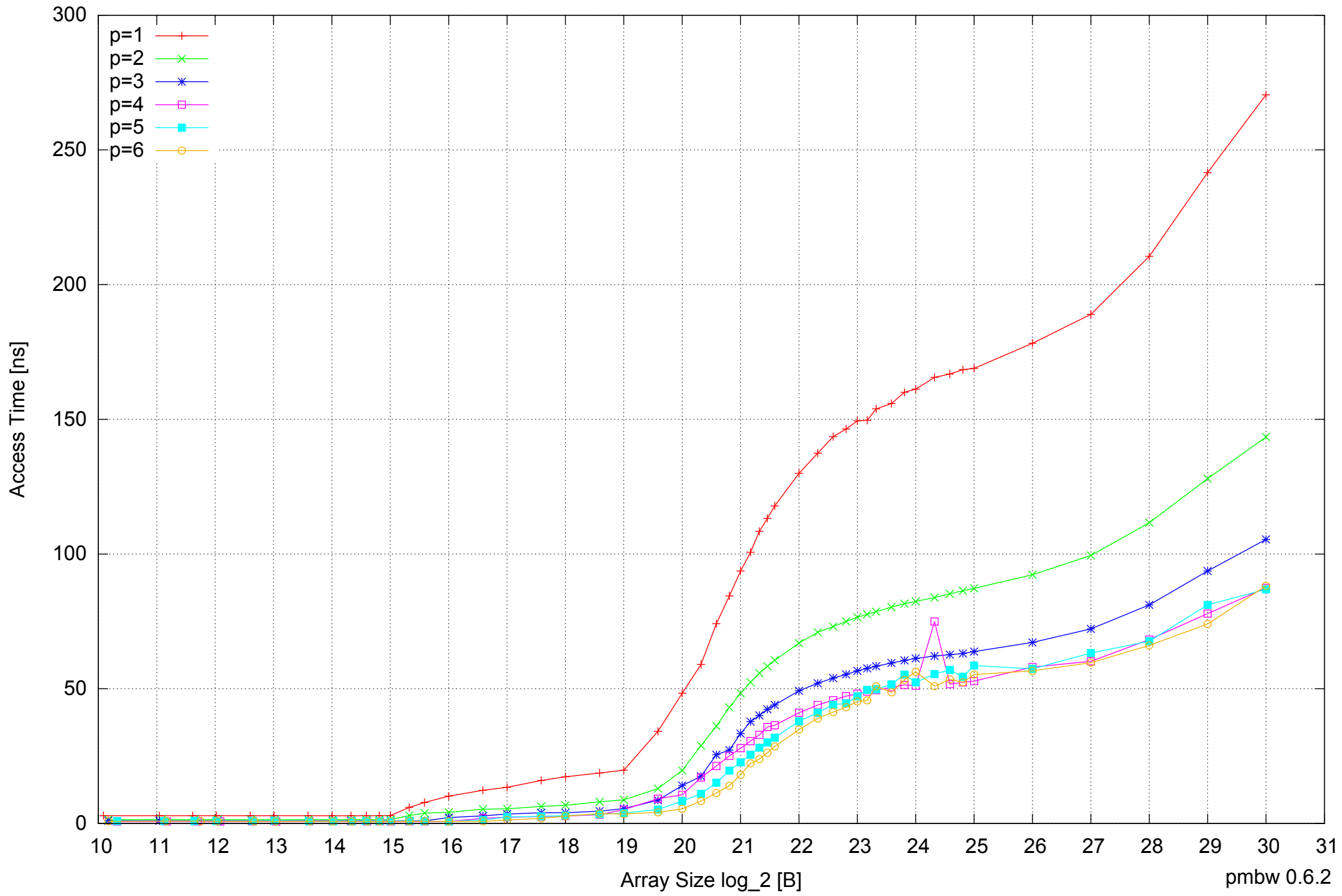
Samsung Galaxy Note 10.1 GT-N8010: Exynos 4412 Quad-Core 2GB - Parallel Memory Access Time - PermRead32UnrollLoop
