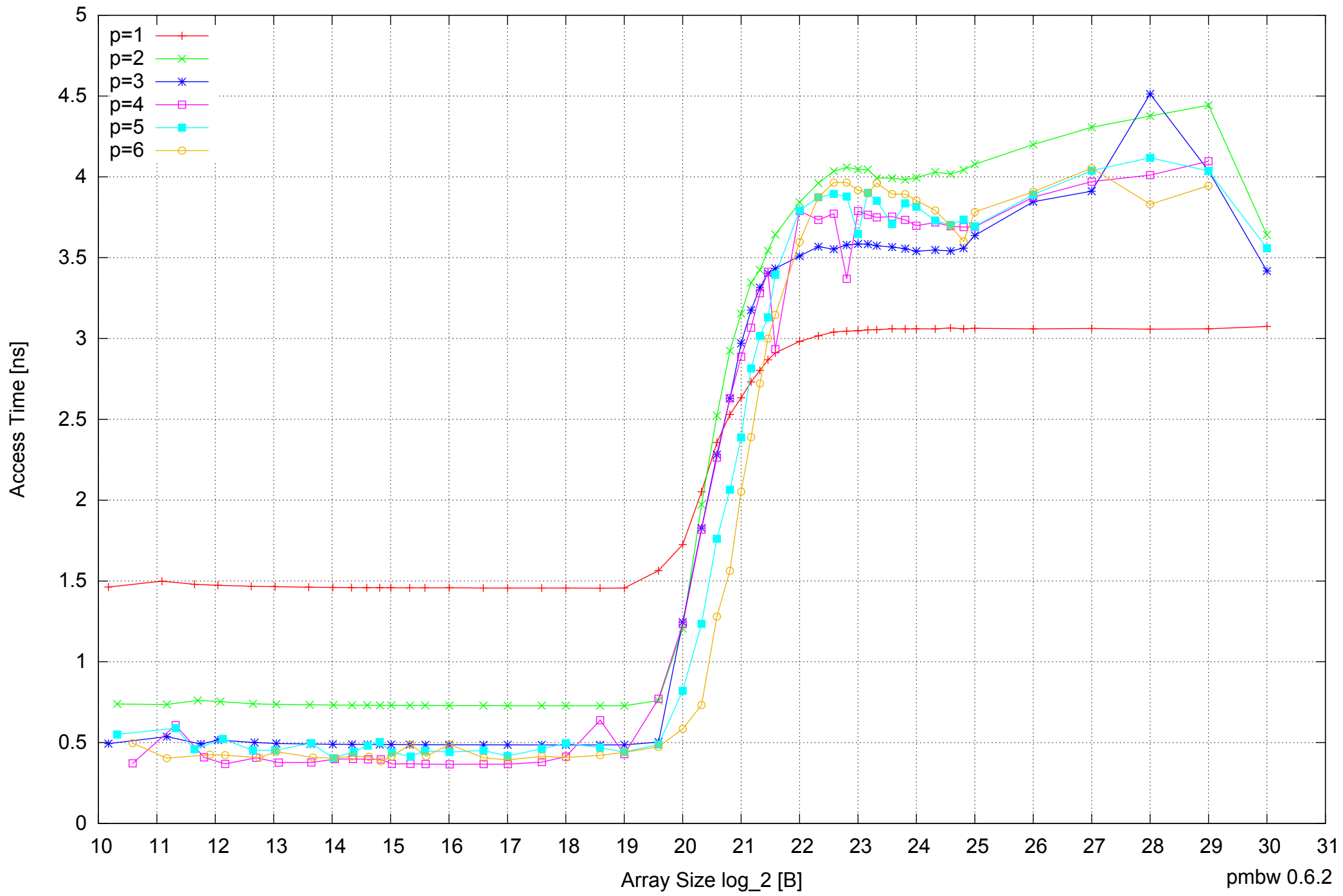
Samsung Galaxy Note 10.1 GT-N8010: Exynos 4412 Quad-Core 2GB - Parallel Memory Access Time - ScanWrite64PtrUnrollLoop
