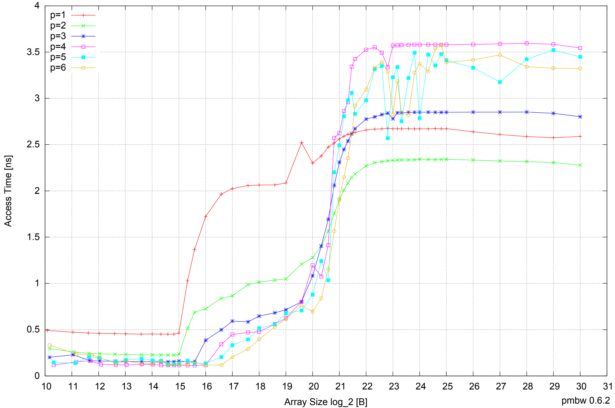
Samsung Galaxy Note 10.1 GT-N8010: Exynos 4412 Quad-Core 2GB - Parallel Memory Access Time - ScanRead32PtrMultiLoop
