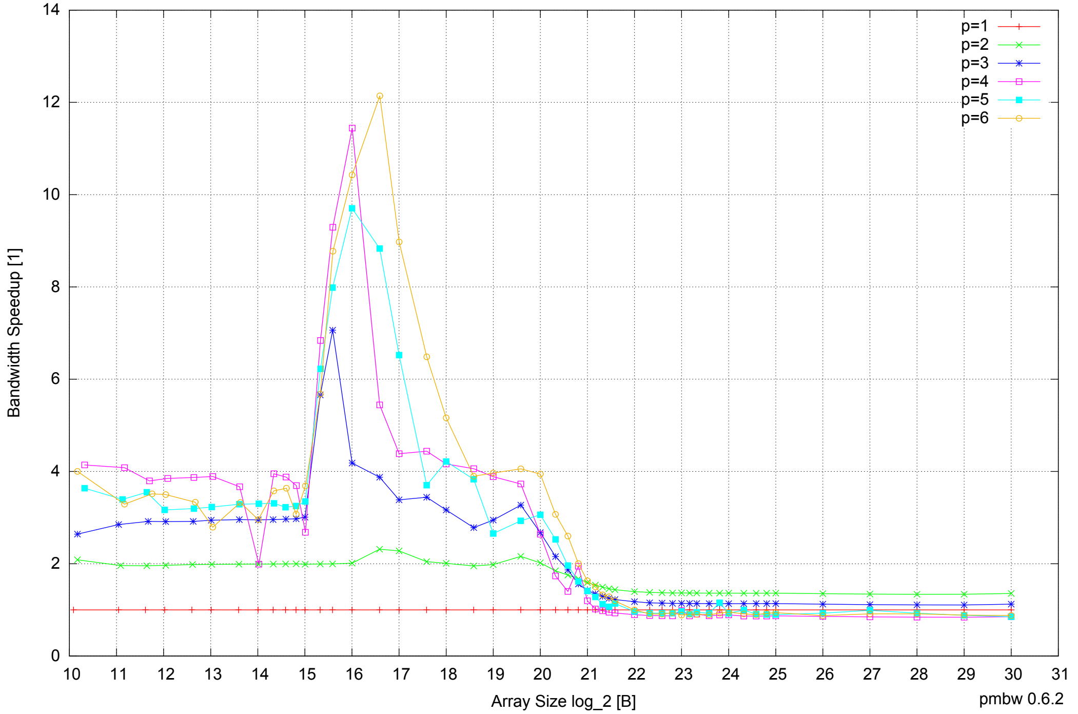
Samsung Galaxy Note 10.1 GT-N8010: Exynos 4412 Quad-Core 2GB - Speedup of Parallel Memory Bandwidth - ScanRead32PtrUnrollLoop
