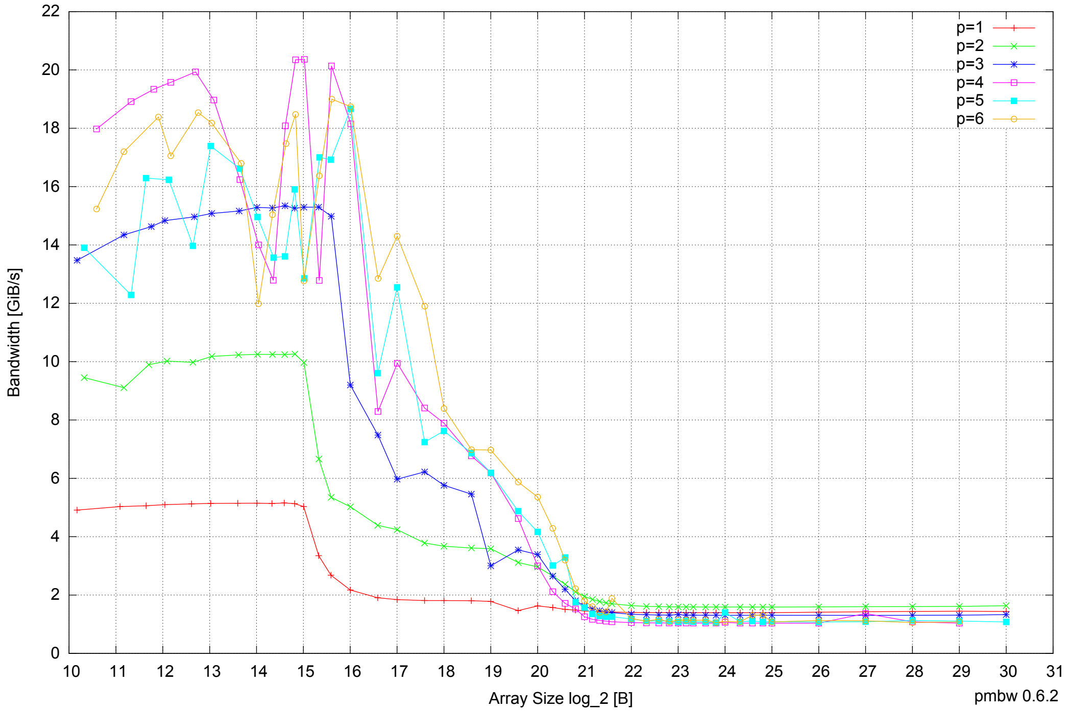
Samsung Galaxy Note 10.1 GT-N8010: Exynos 4412 Quad-Core 2GB - Parallel Memory Bandwidth - ScanRead64PtrSimpleLoop
