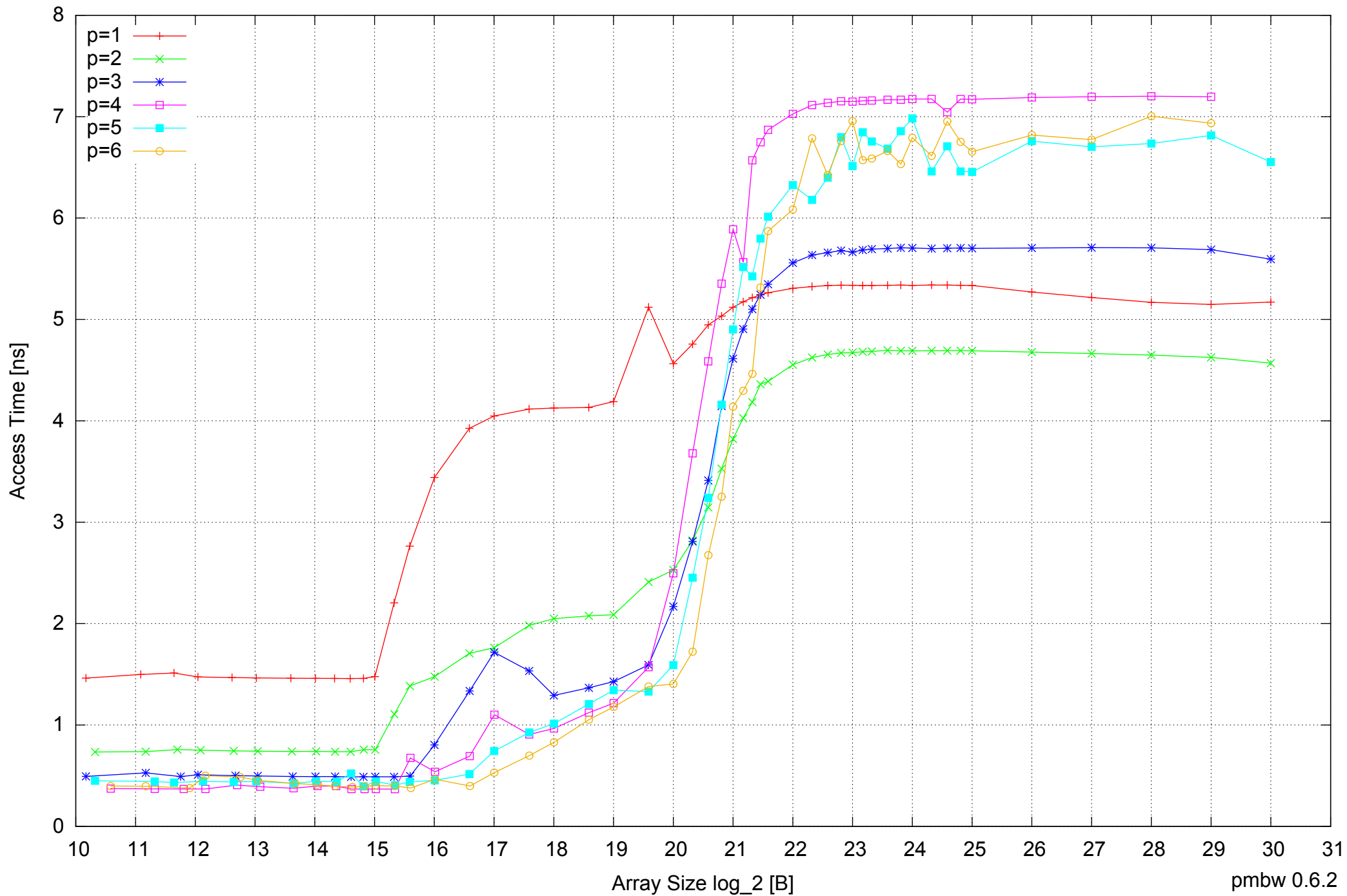
Samsung Galaxy Note 10.1 GT-N8010: Exynos 4412 Quad-Core 2GB - Parallel Memory Access Time - ScanRead64PtrUnrollLoop
