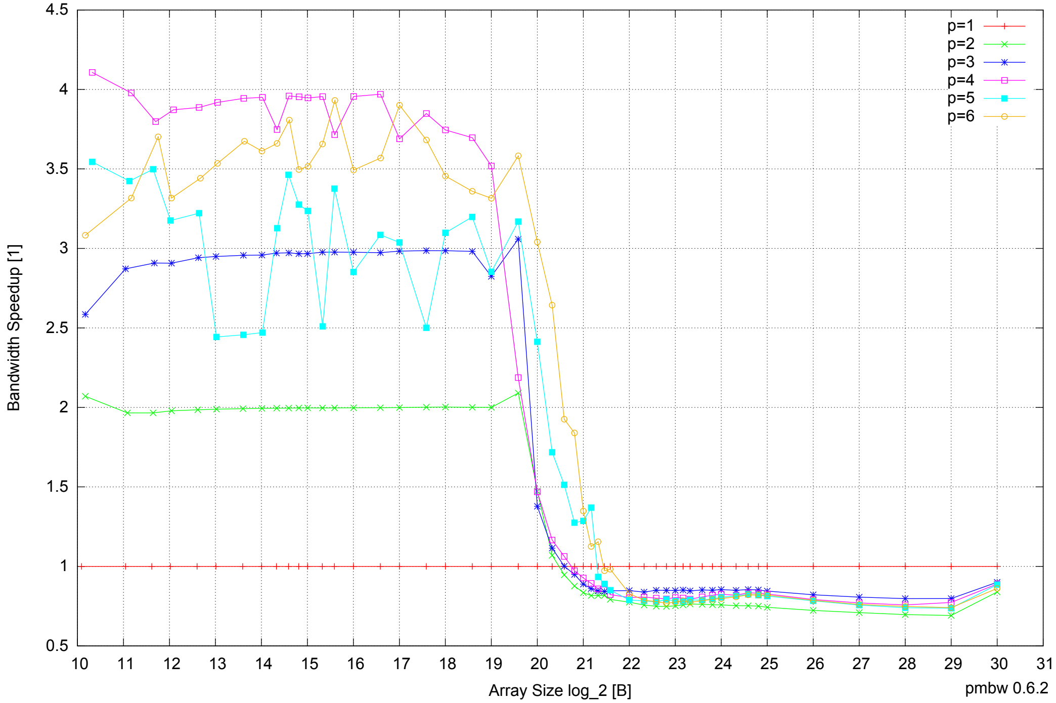
Samsung Galaxy Note 10.1 GT-N8010: Exynos 4412 Quad-Core 2GB - Speedup of Parallel Memory Bandwidth - ScanWrite32PtrUnrollLoop
