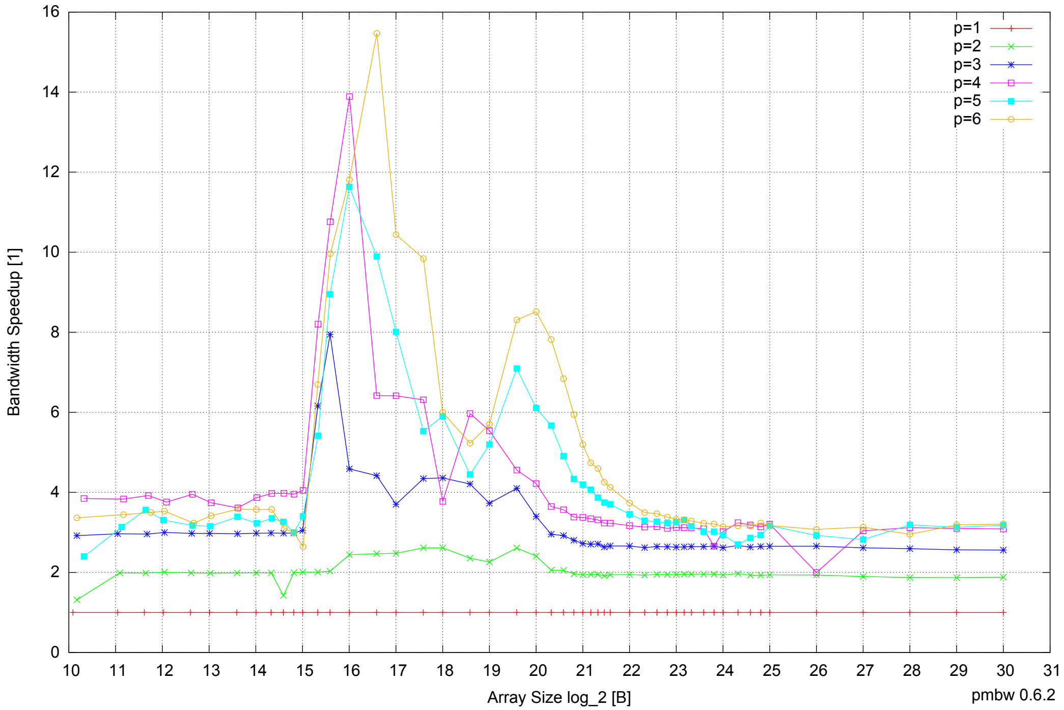
Samsung Galaxy Note 10.1 GT-N8010: Exynos 4412 Quad-Core 2GB - Speedup of Parallel Memory Bandwidth - PermRead32SimpleLoop
