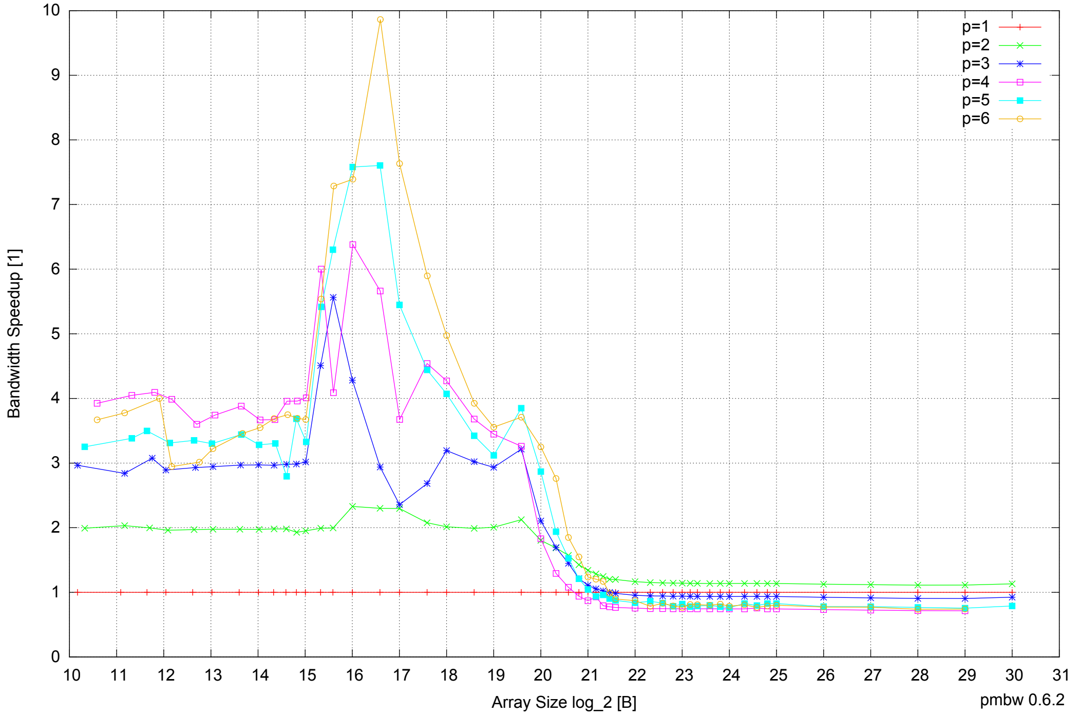
Samsung Galaxy Note 10.1 GT-N8010: Exynos 4412 Quad-Core 2GB - Speedup of Parallel Memory Bandwidth - ScanRead64PtrUnrollLoop
