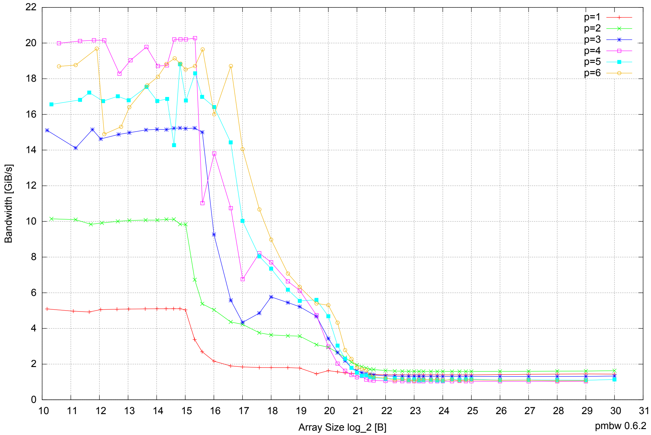
Samsung Galaxy Note 10.1 GT-N8010: Exynos 4412 Quad-Core 2GB - Parallel Memory Bandwidth - ScanRead64PtrUnrollLoop
