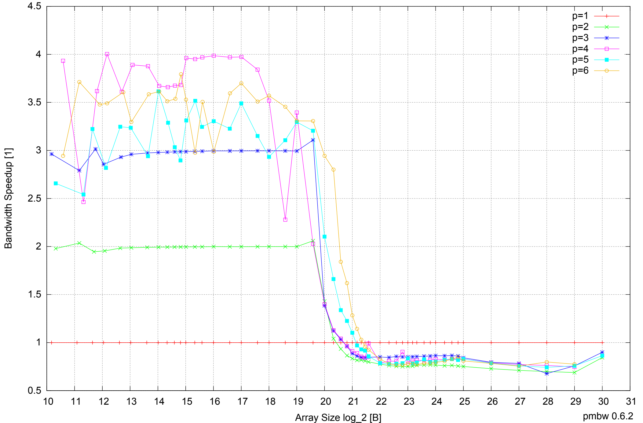
Samsung Galaxy Note 10.1 GT-N8010: Exynos 4412 Quad-Core 2GB - Speedup of Parallel Memory Bandwidth - ScanWrite64PtrUnrollLoop
