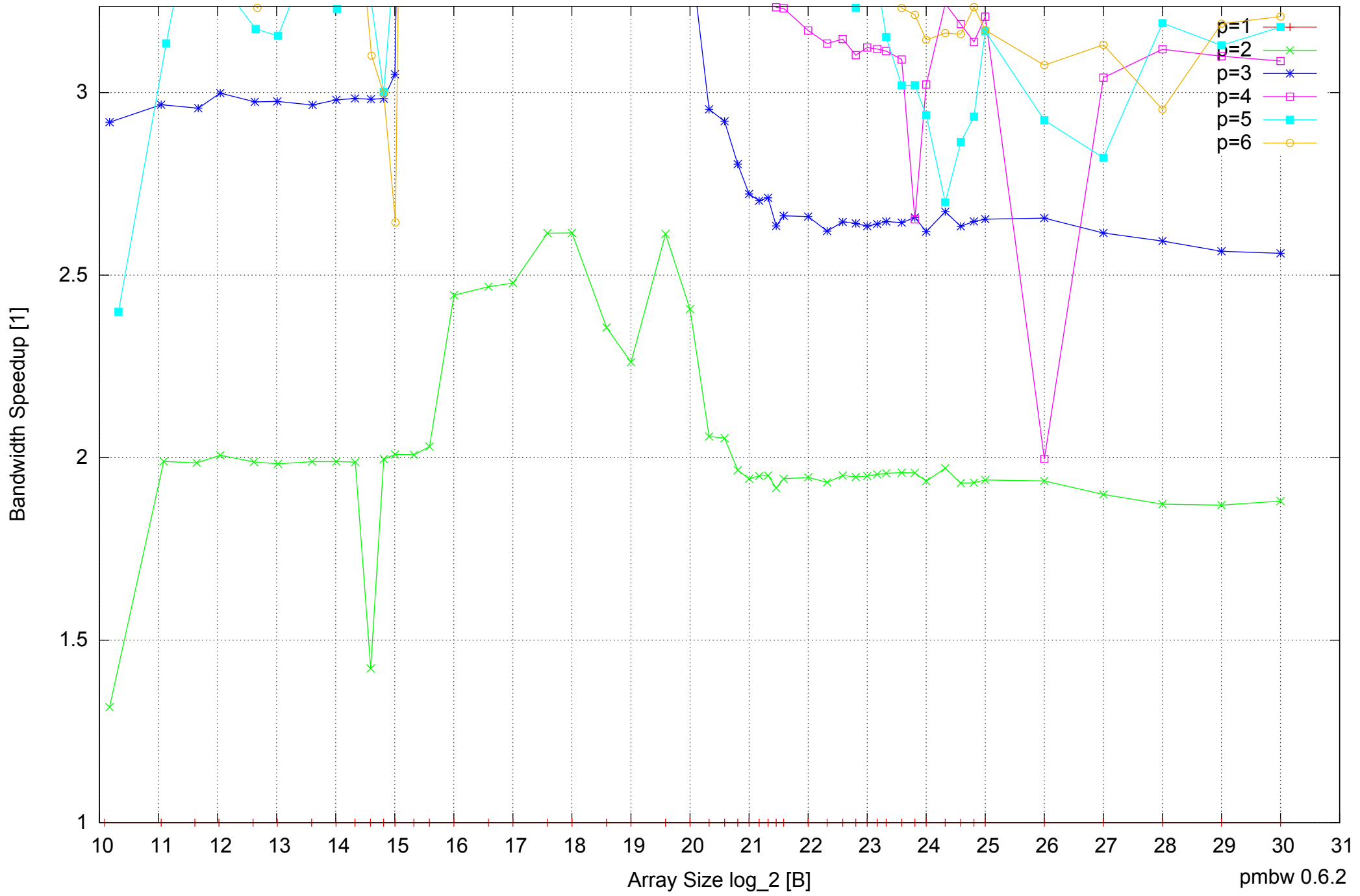
Samsung Galaxy Note 10.1 GT-N8010: Exynos 4412 Quad-Core 2GB - Speedup of Parallel Memory Bandwidth (enlarged) - PermRead32SimpleL
