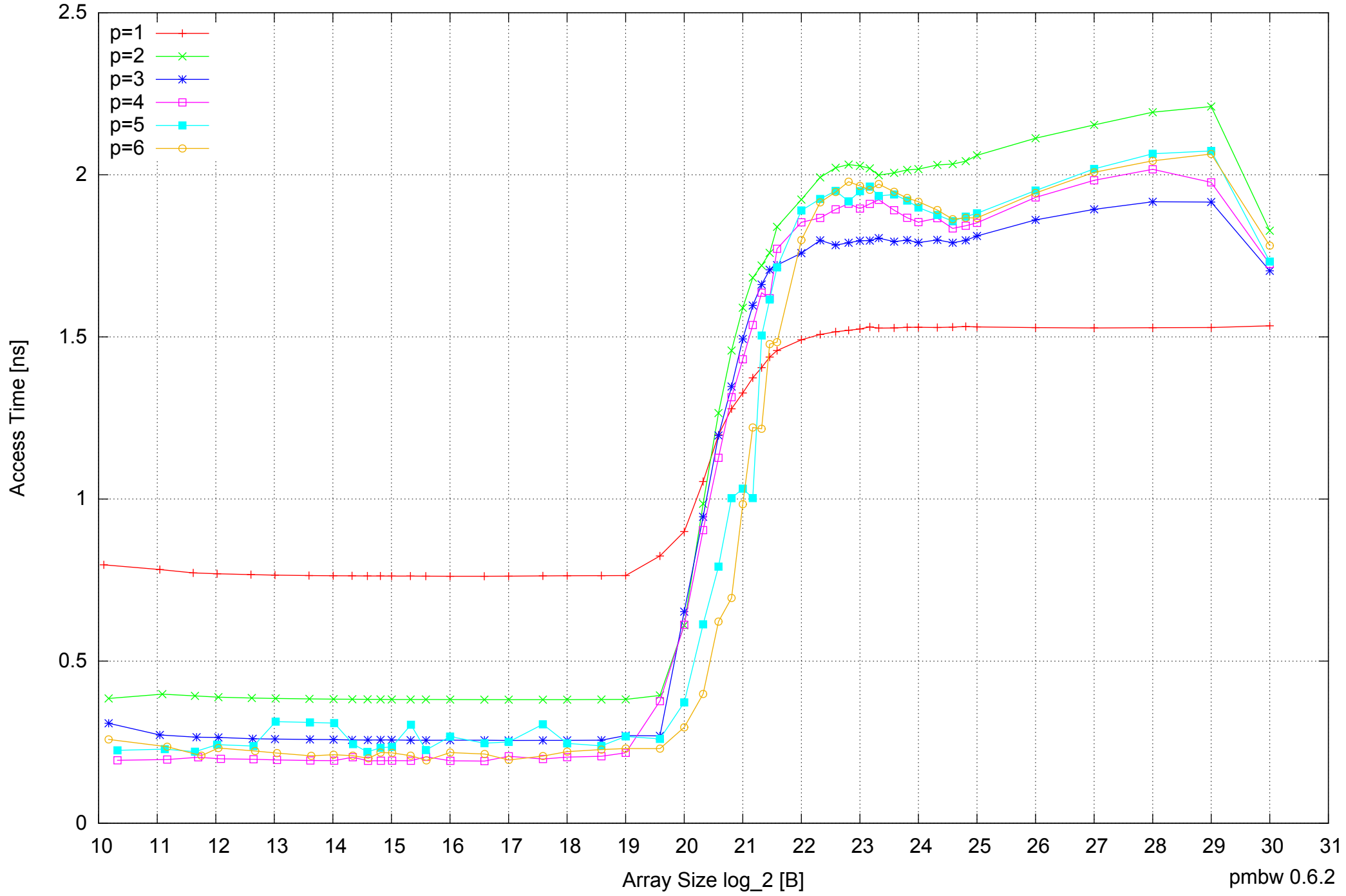
Samsung Galaxy Note 10.1 GT-N8010: Exynos 4412 Quad-Core 2GB - Parallel Memory Access Time - ScanWrite32PtrUnrollLoop
