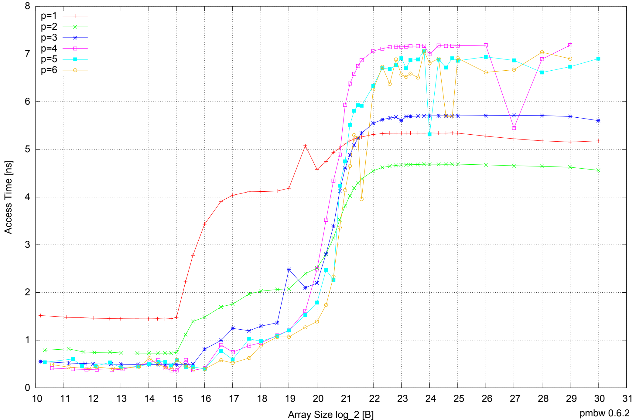
Samsung Galaxy Note 10.1 GT-N8010: Exynos 4412 Quad-Core 2GB - Parallel Memory Access Time - ScanRead64PtrSimpleLoop
