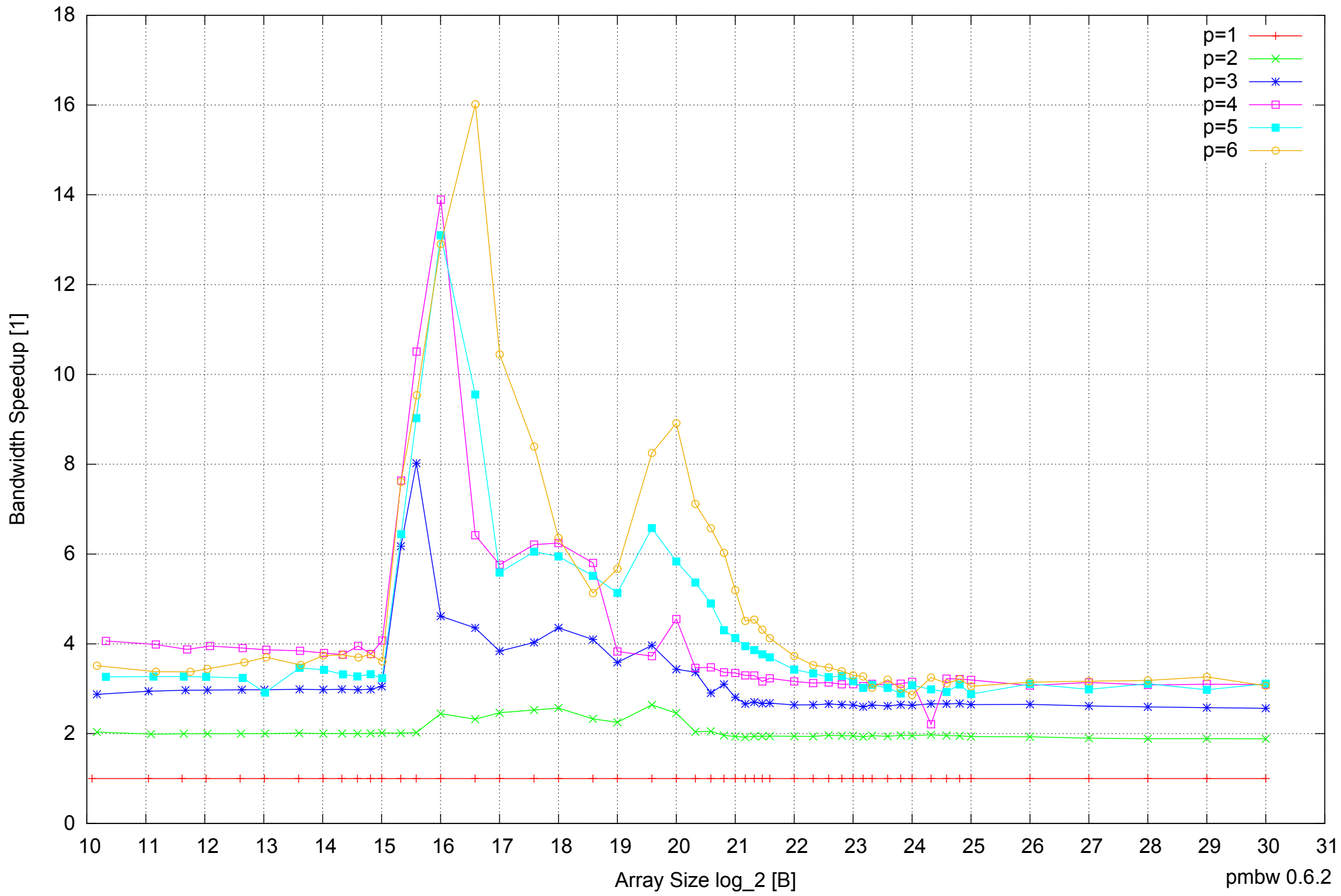
Samsung Galaxy Note 10.1 GT-N8010: Exynos 4412 Quad-Core 2GB - Speedup of Parallel Memory Bandwidth - PermRead32UnrollLoop
