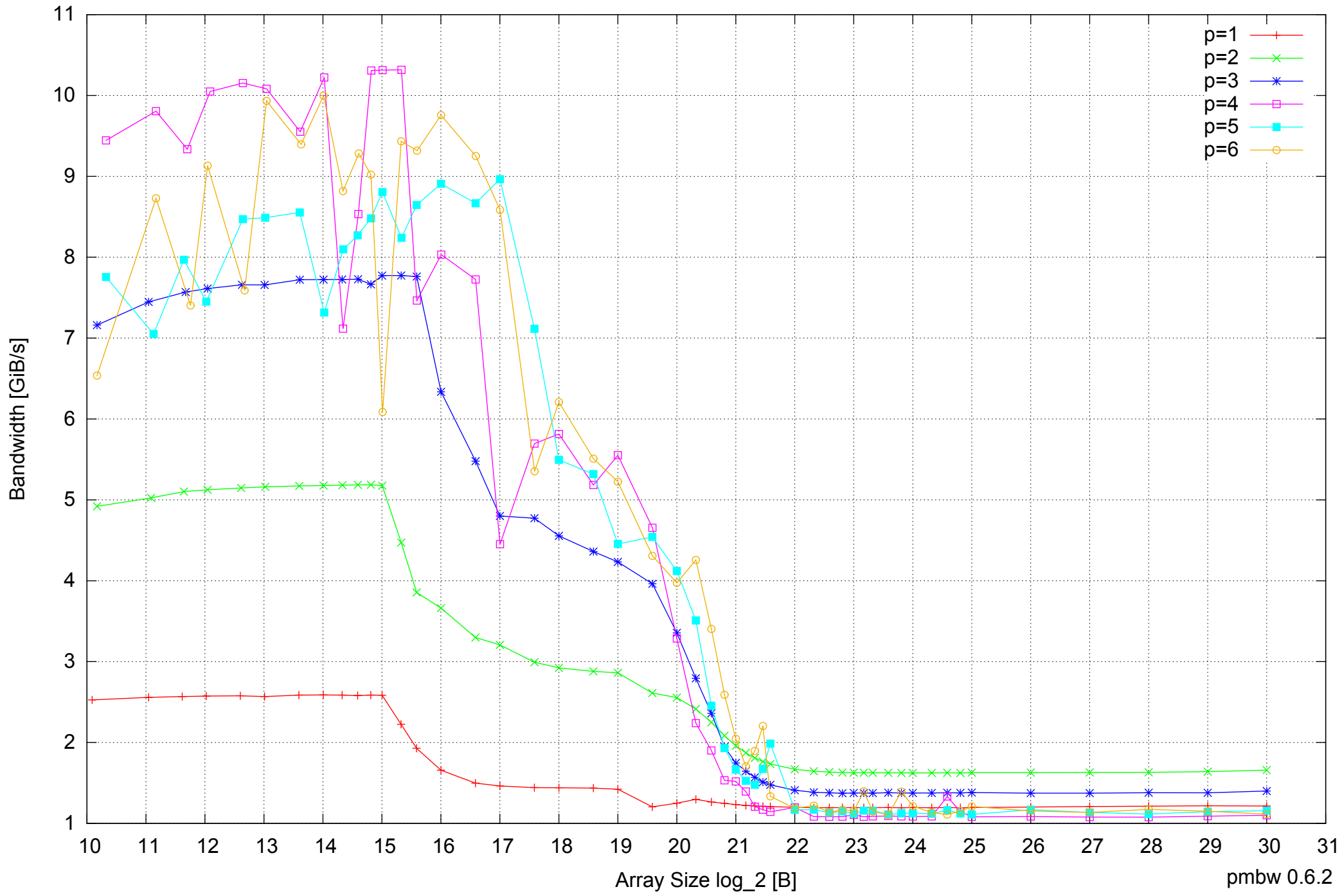
Samsung Galaxy Note 10.1 GT-N8010: Exynos 4412 Quad-Core 2GB - Parallel Memory Bandwidth - ScanRead32PtrSimpleLoop
