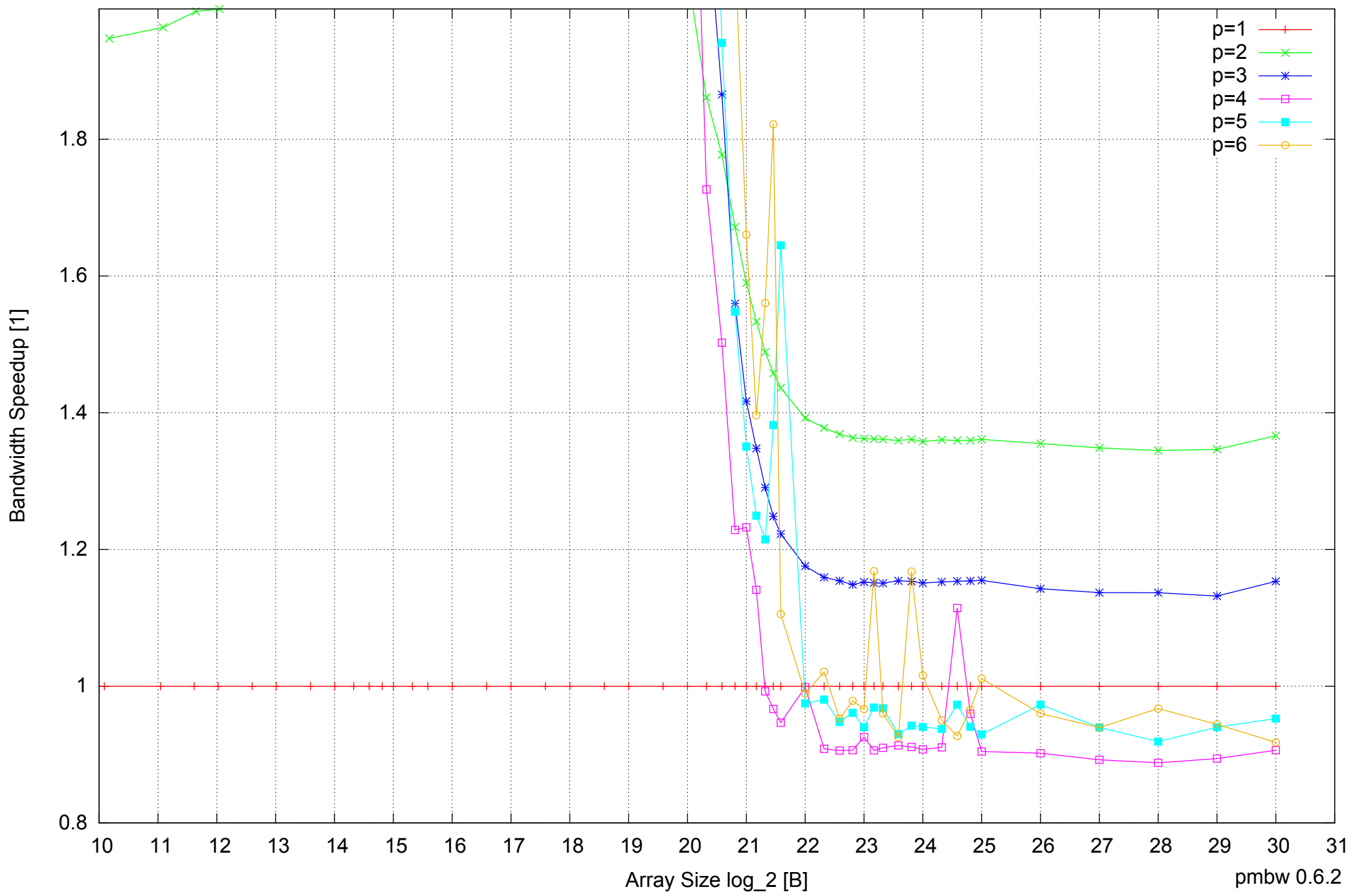
Samsung Galaxy Note 10.1 GT-N8010: Exynos 4412 Quad-Core 2GB - Speedup of Parallel Memory Bandwidth (enlarged) - ScanRead32PtrSimple
