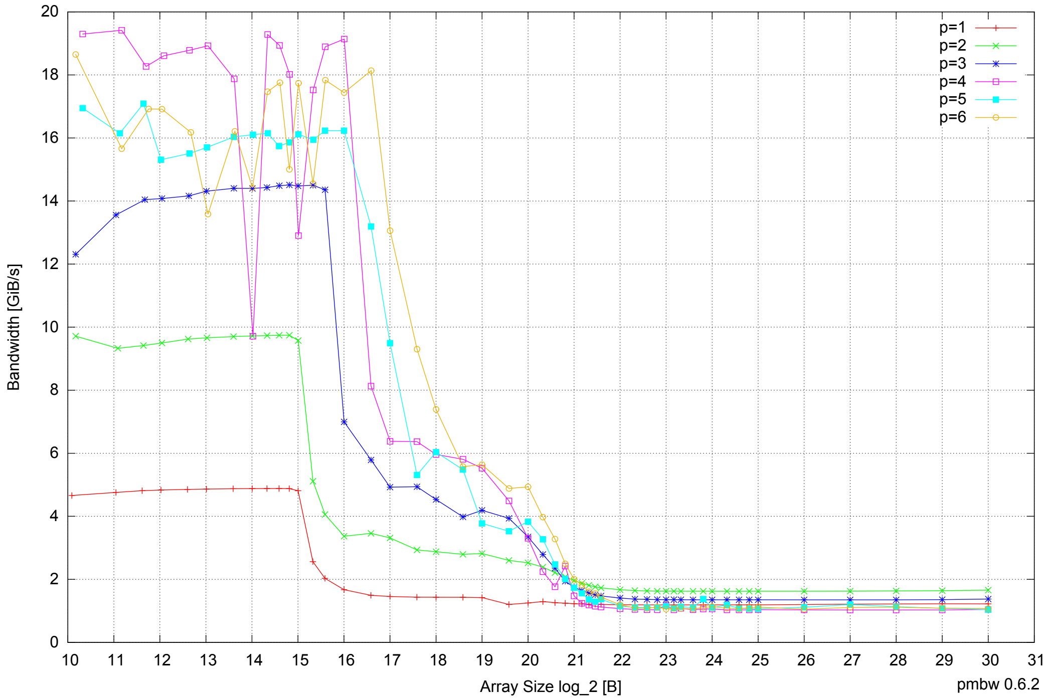
Samsung Galaxy Note 10.1 GT-N8010: Exynos 4412 Quad-Core 2GB - Parallel Memory Bandwidth - ScanRead32PtrUnrollLoop
