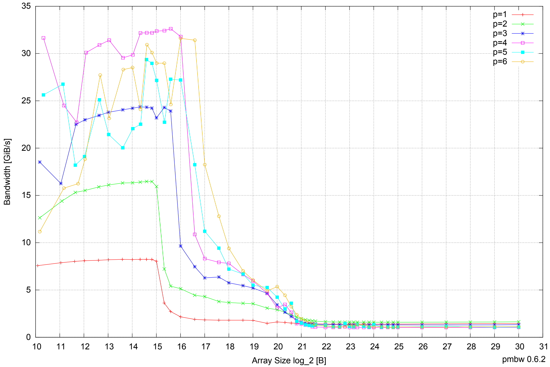
Samsung Galaxy Note 10.1 GT-N8010: Exynos 4412 Quad-Core 2GB - Parallel Memory Bandwidth - ScanRead32PtrMultiLoop
