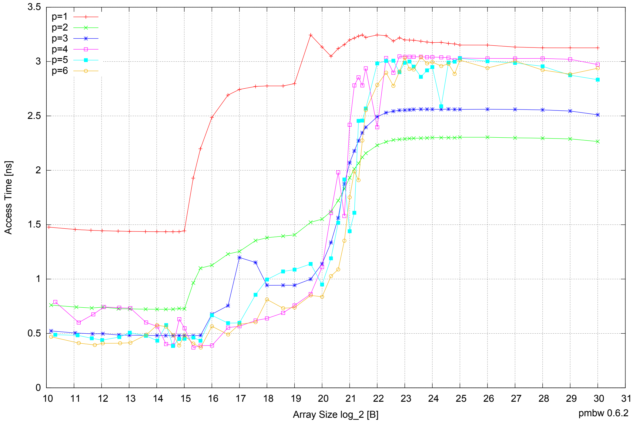
Samsung Galaxy Note 10.1 GT-N8010: Exynos 4412 Quad-Core 2GB - Parallel Memory Access Time - ScanRead32IndexSimpleLoop
