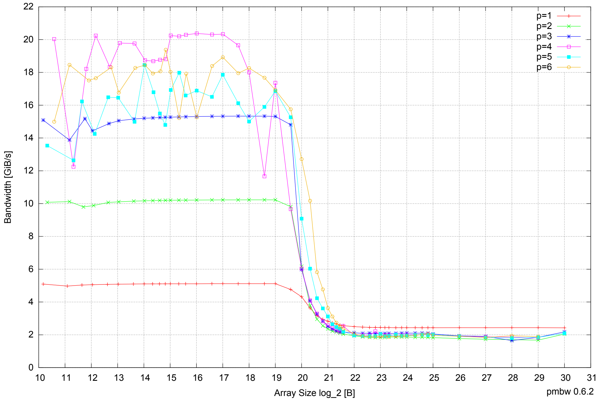
Samsung Galaxy Note 10.1 GT-N8010: Exynos 4412 Quad-Core 2GB - Parallel Memory Bandwidth - ScanWrite64PtrUnrollLoop
