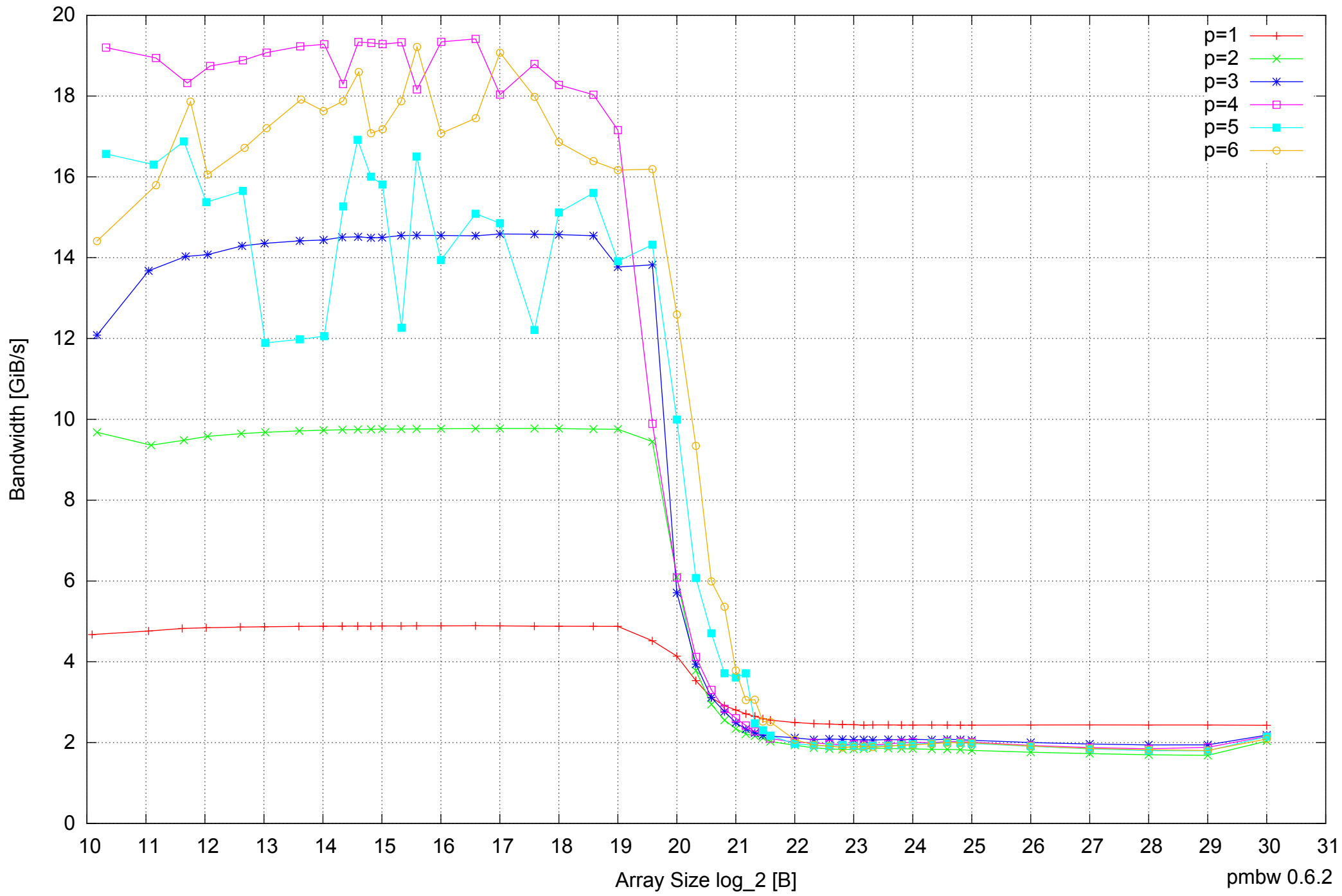
Samsung Galaxy Note 10.1 GT-N8010: Exynos 4412 Quad-Core 2GB - Parallel Memory Bandwidth - ScanWrite32PtrUnrollLoop
