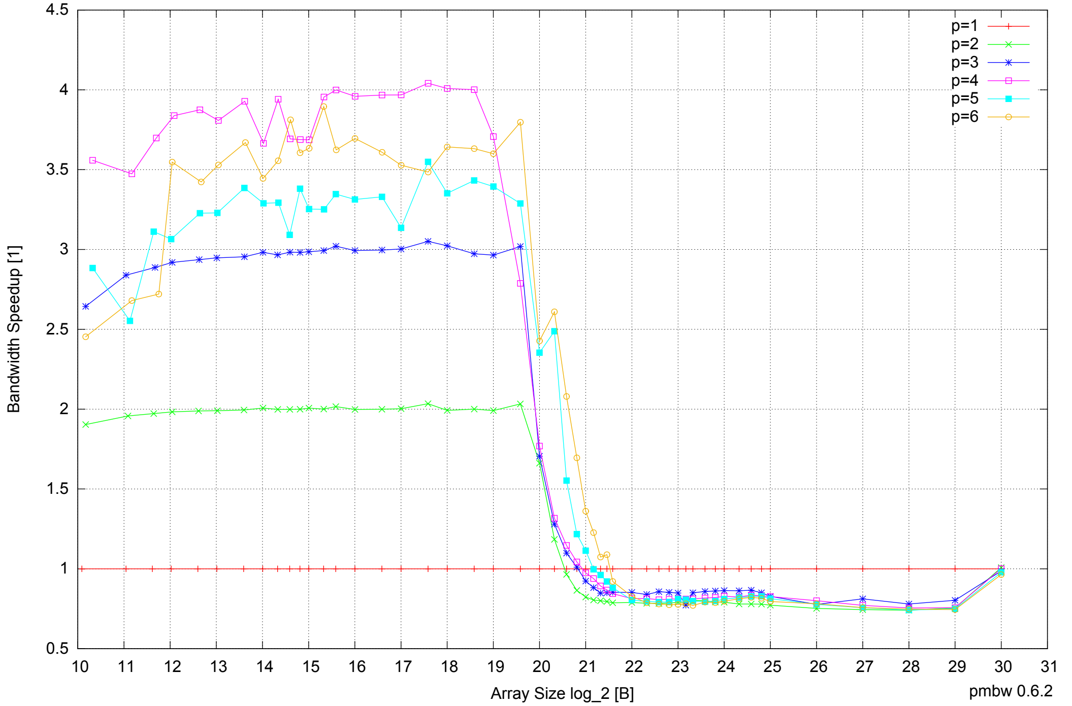
Samsung Galaxy Note 10.1 GT-N8010: Exynos 4412 Quad-Core 2GB - Speedup of Parallel Memory Bandwidth - ScanWrite32PtrSimpleLoop
