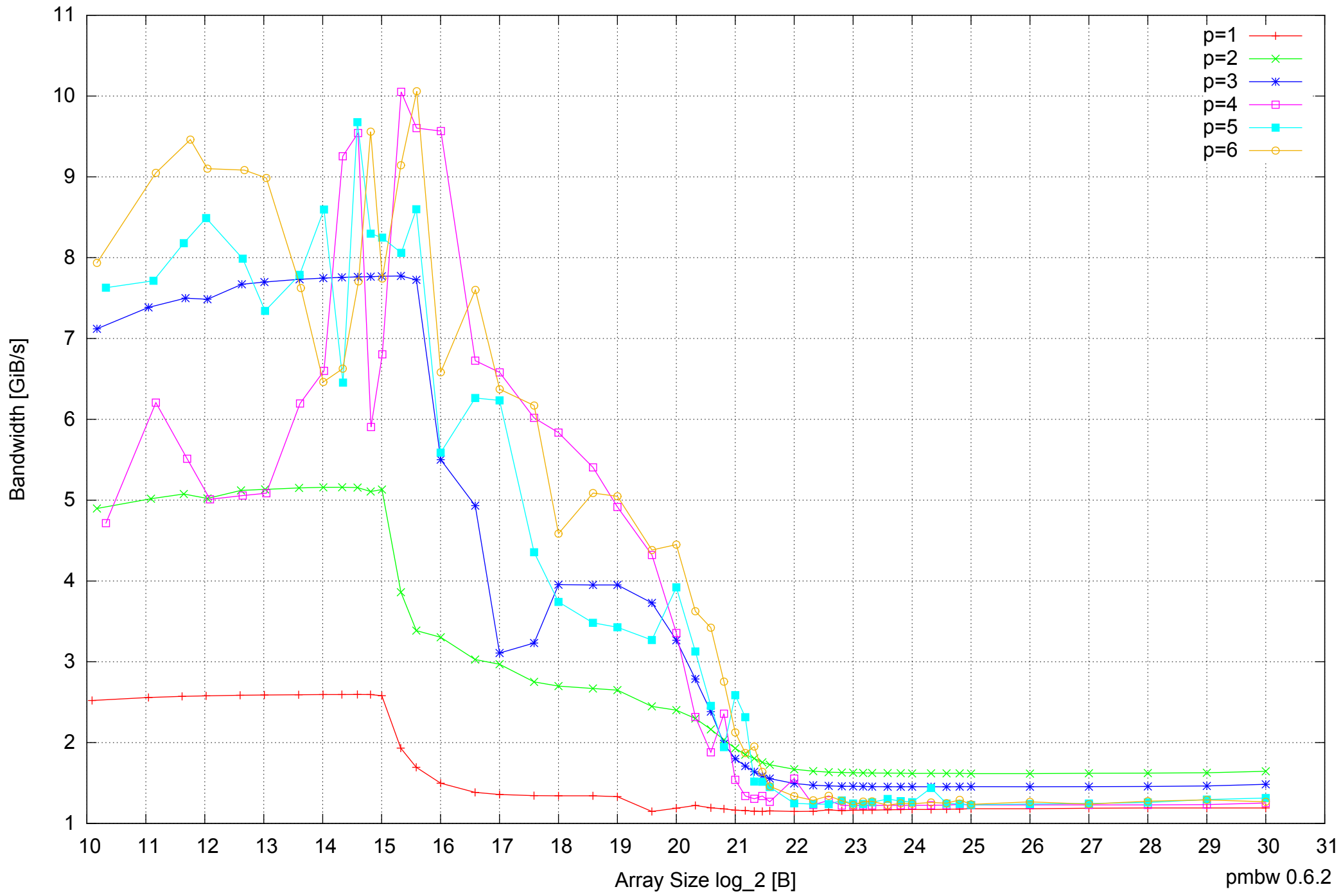
Samsung Galaxy Note 10.1 GT-N8010: Exynos 4412 Quad-Core 2GB - Parallel Memory Bandwidth - ScanRead32IndexSimpleLoop
