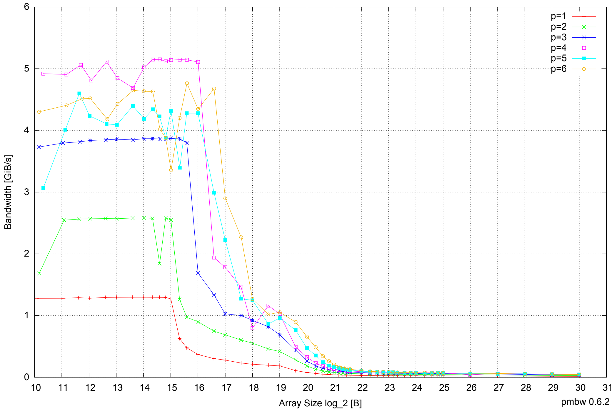
Samsung Galaxy Note 10.1 GT-N8010: Exynos 4412 Quad-Core 2GB - Parallel Memory Bandwidth - PermRead32SimpleLoop
