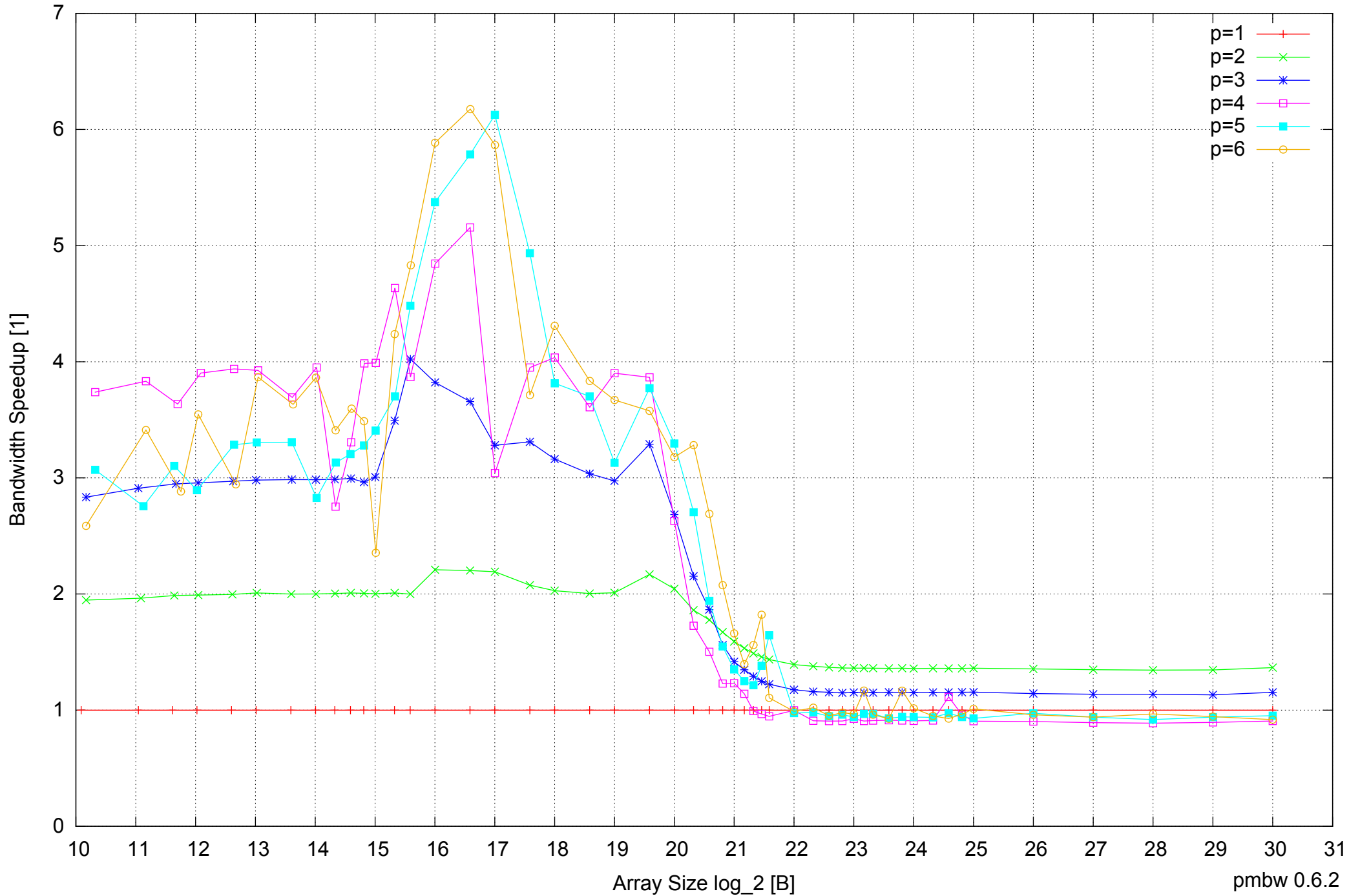
Samsung Galaxy Note 10.1 GT-N8010: Exynos 4412 Quad-Core 2GB - Speedup of Parallel Memory Bandwidth - ScanRead32PtrSimpleLoop
