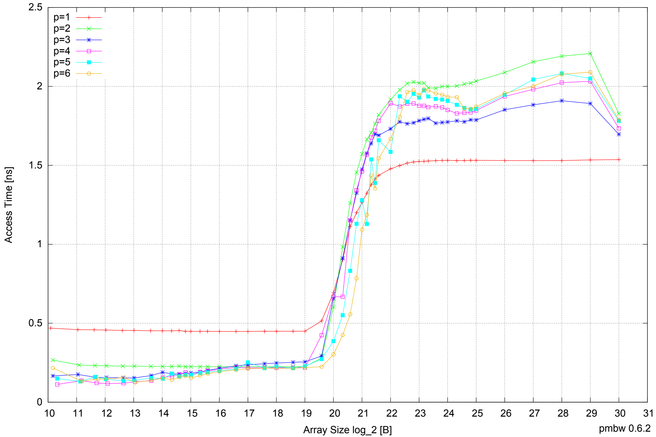
Samsung Galaxy Note 10.1 GT-N8010: Exynos 4412 Quad-Core 2GB - Parallel Memory Access Time - ScanWrite32PtrMultiLoop
