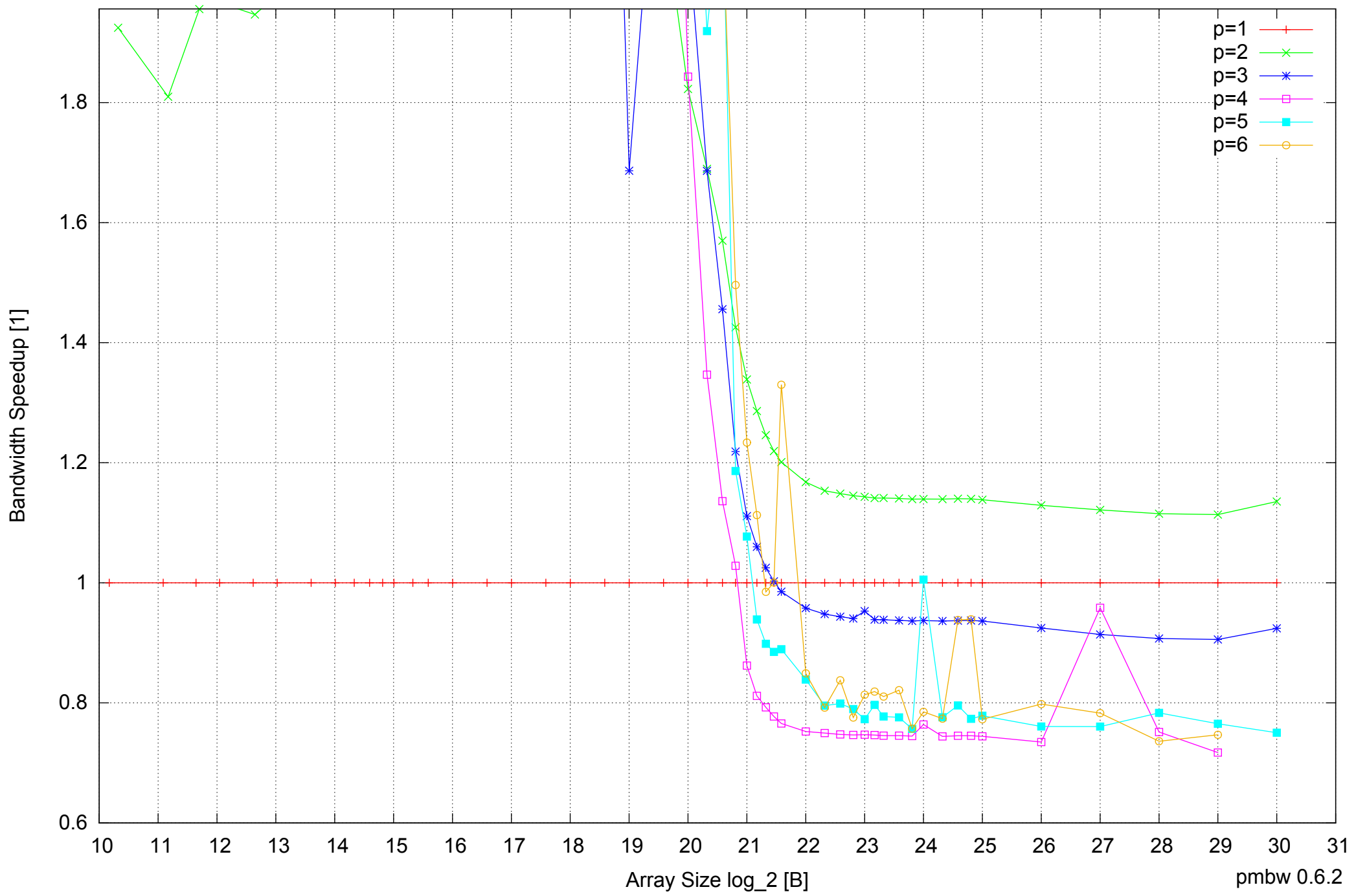
Samsung Galaxy Note 10.1 GT-N8010: Exynos 4412 Quad-Core 2GB - Speedup of Parallel Memory Bandwidth (enlarged) - ScanRead64PtrSimple
