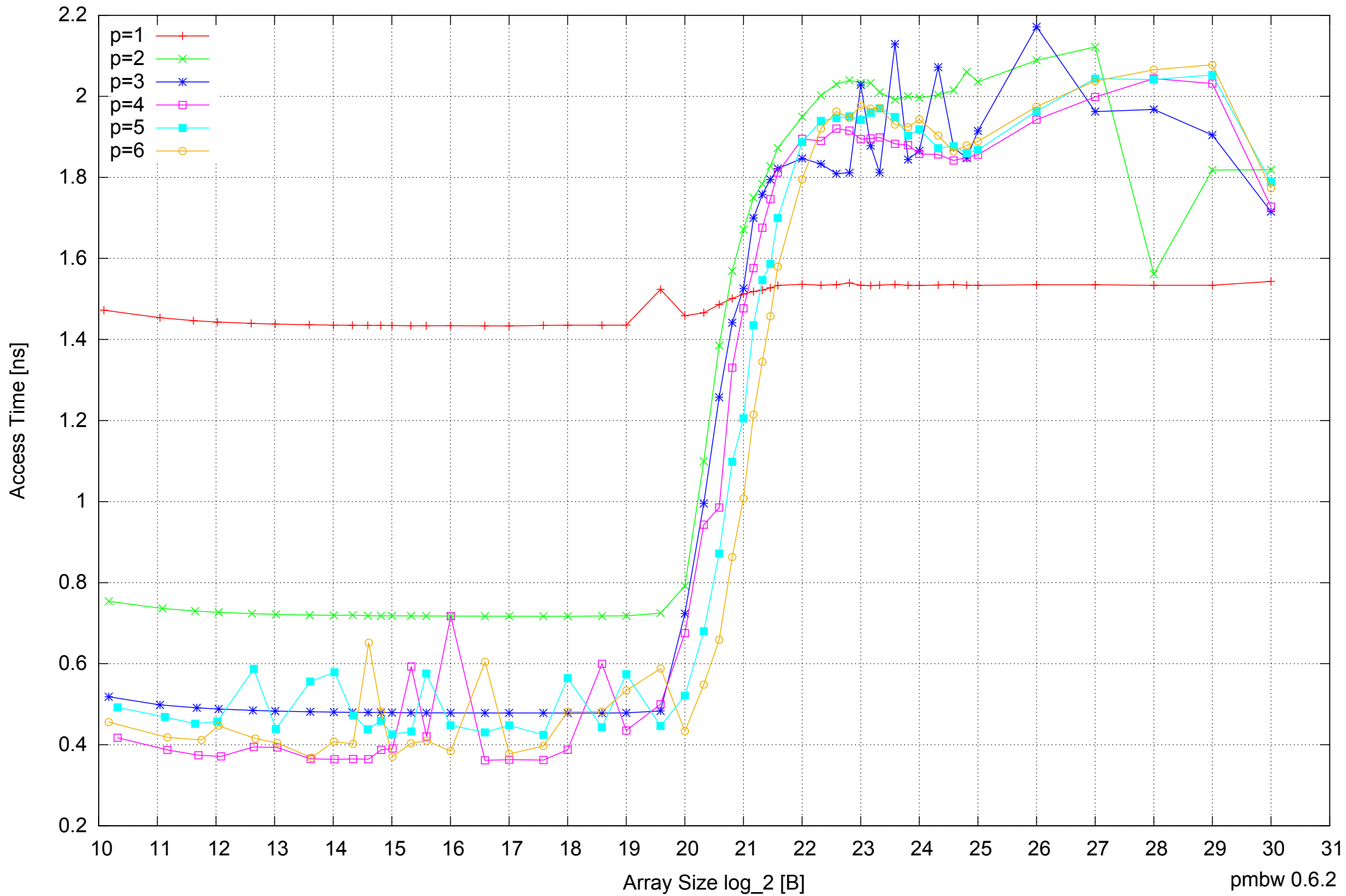
Samsung Galaxy Note 10.1 GT-N8010: Exynos 4412 Quad-Core 2GB - Parallel Memory Access Time - ScanWrite32IndexSimpleLoop
