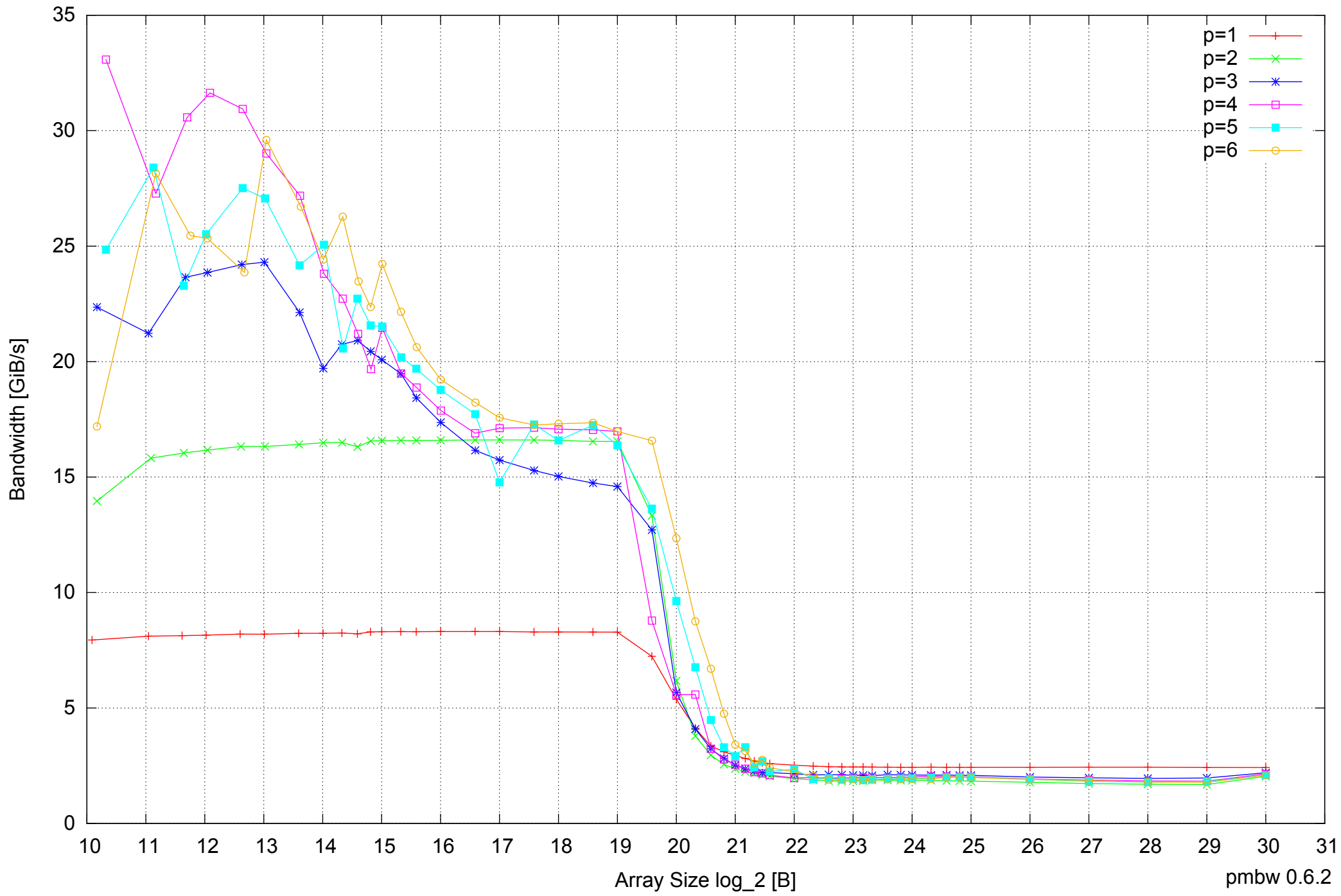
Samsung Galaxy Note 10.1 GT-N8010: Exynos 4412 Quad-Core 2GB - Parallel Memory Bandwidth - ScanWrite32PtrMultiLoop
