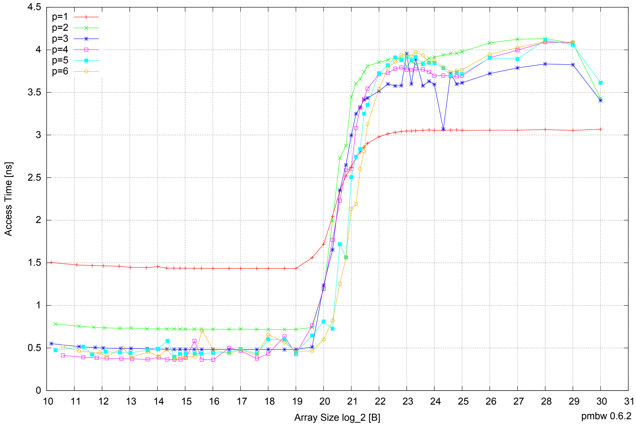
Samsung Galaxy Note 10.1 GT-N8010: Exynos 4412 Quad-Core 2GB - Parallel Memory Access Time - ScanWrite64PtrSimpleLoop
