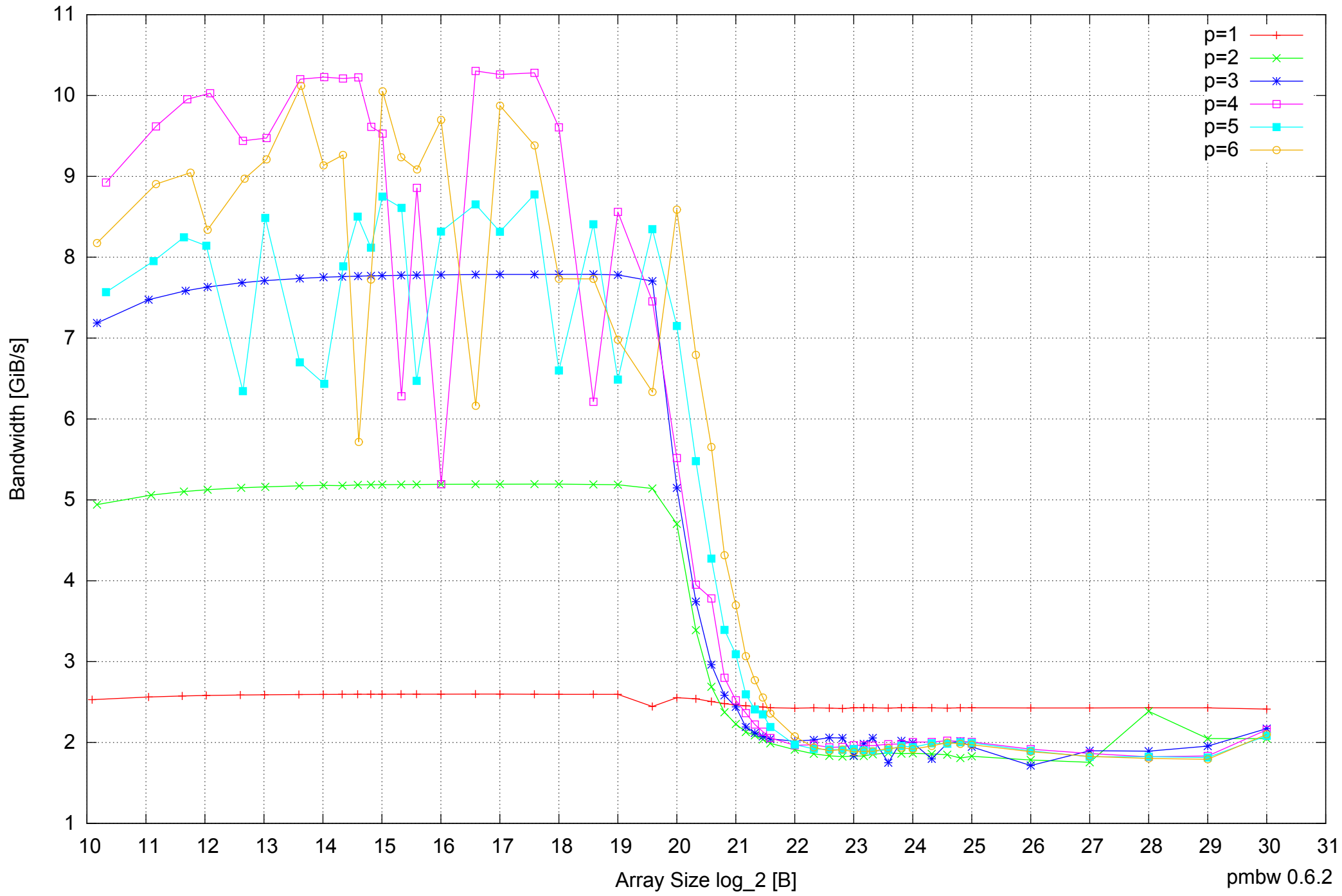
Samsung Galaxy Note 10.1 GT-N8010: Exynos 4412 Quad-Core 2GB - Parallel Memory Bandwidth - ScanWrite32IndexSimpleLoop
