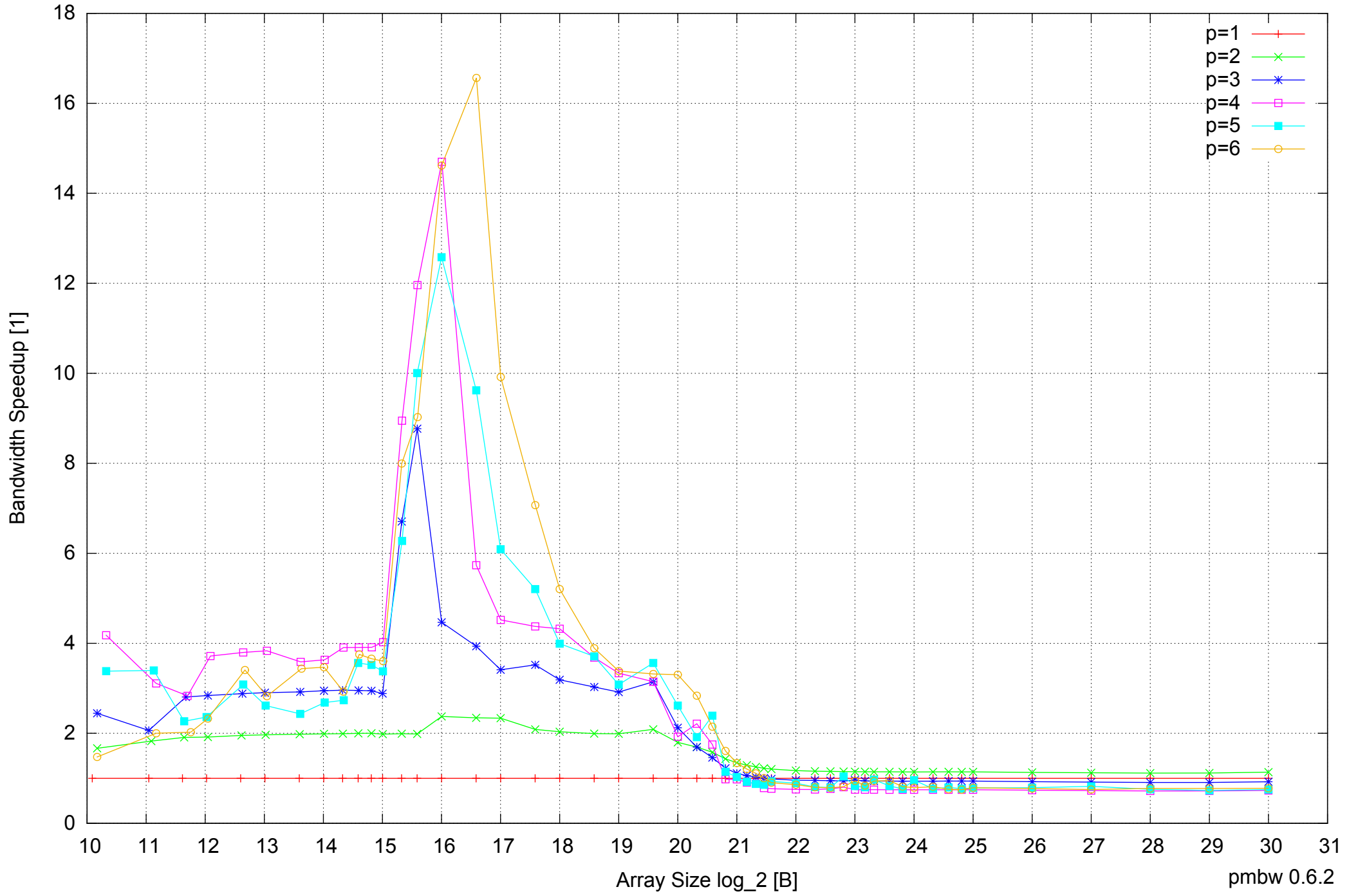
Samsung Galaxy Note 10.1 GT-N8010: Exynos 4412 Quad-Core 2GB - Speedup of Parallel Memory Bandwidth - ScanRead32PtrMultiLoop
