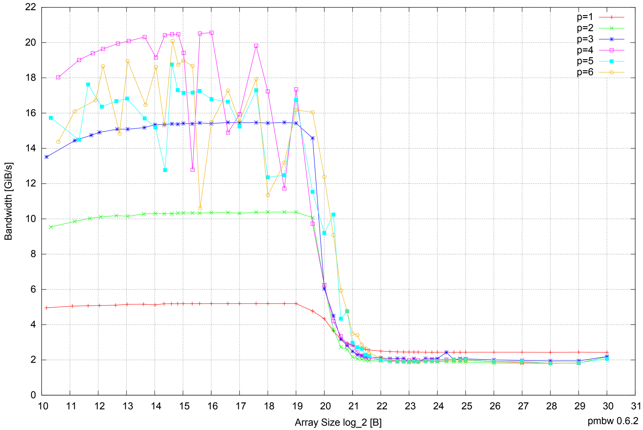
Samsung Galaxy Note 10.1 GT-N8010: Exynos 4412 Quad-Core 2GB - Parallel Memory Bandwidth - ScanWrite64PtrSimpleLoop
