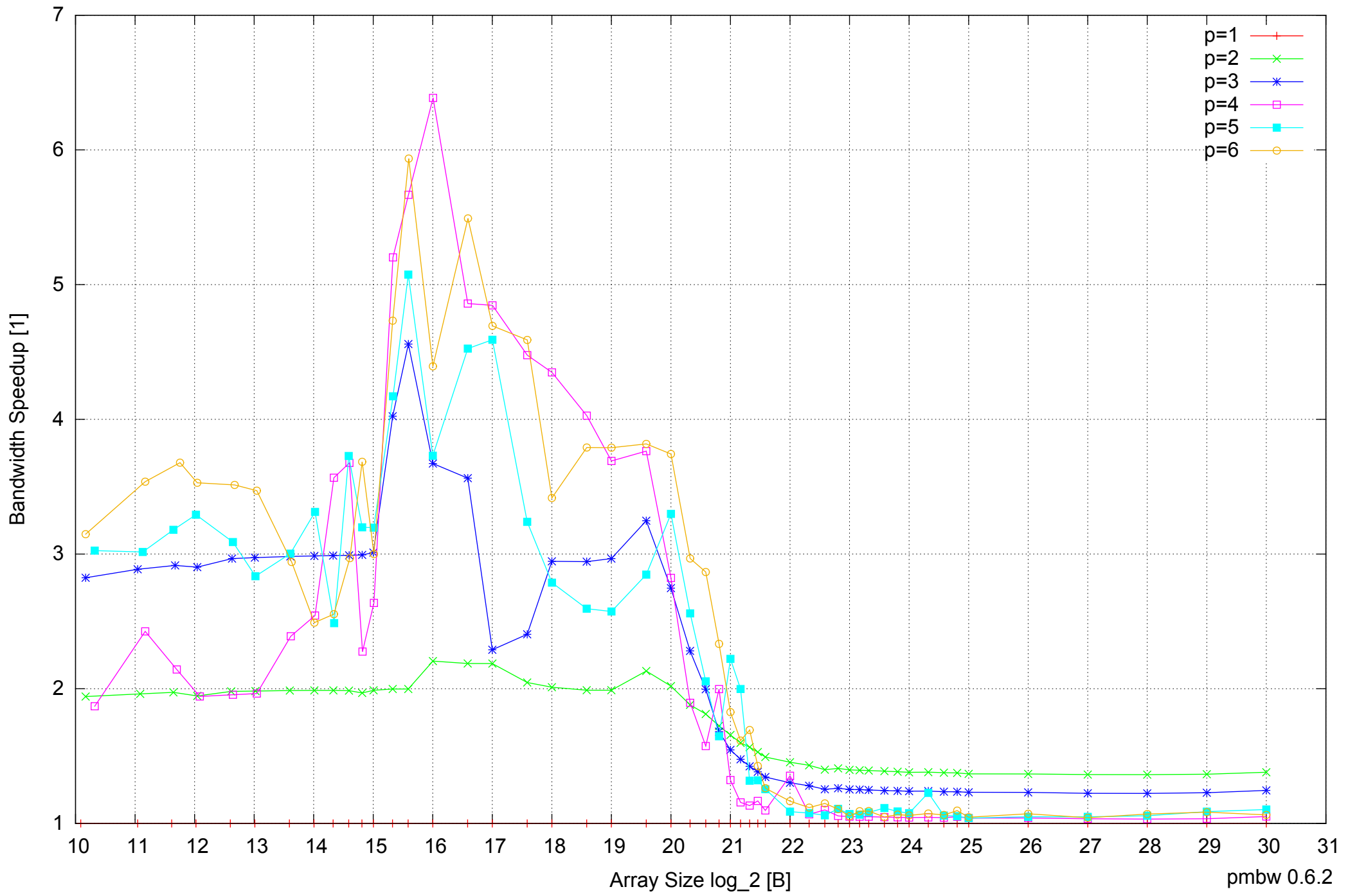
Samsung Galaxy Note 10.1 GT-N8010: Exynos 4412 Quad-Core 2GB - Speedup of Parallel Memory Bandwidth - ScanRead32IndexSimpleLoop
