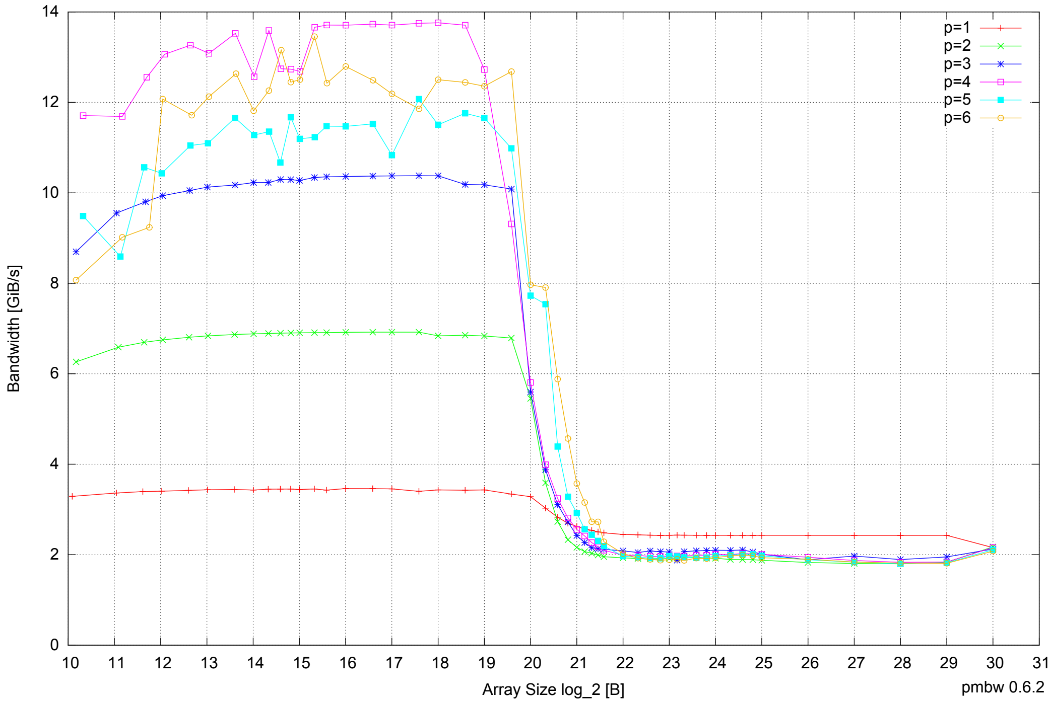
Samsung Galaxy Note 10.1 GT-N8010: Exynos 4412 Quad-Core 2GB - Parallel Memory Bandwidth - ScanWrite32PtrSimpleLoop
