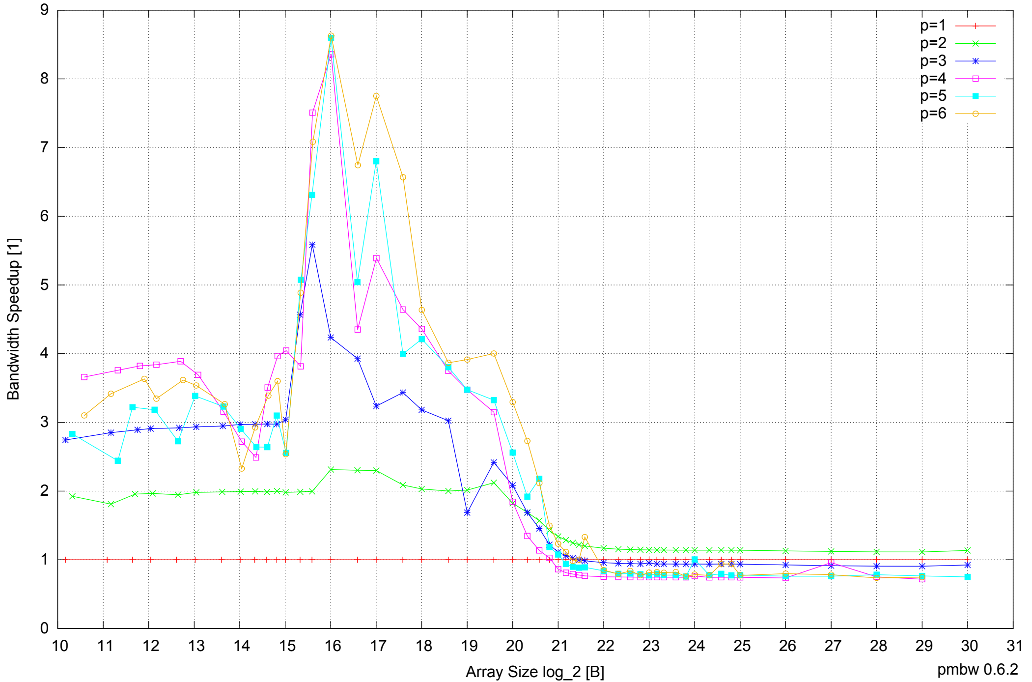
Samsung Galaxy Note 10.1 GT-N8010: Exynos 4412 Quad-Core 2GB - Speedup of Parallel Memory Bandwidth - ScanRead64PtrSimpleLoop
