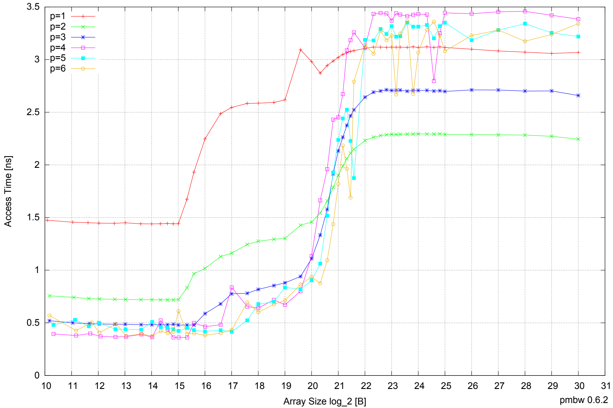
Samsung Galaxy Note 10.1 GT-N8010: Exynos 4412 Quad-Core 2GB - Parallel Memory Access Time - ScanRead32PtrSimpleLoop
