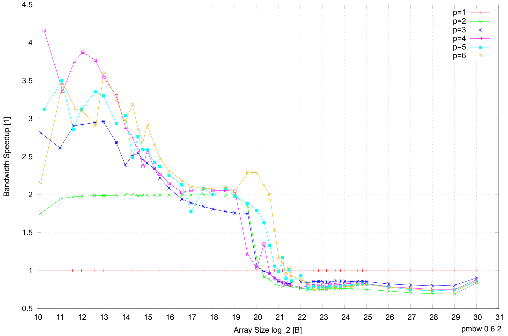
Samsung Galaxy Note 10.1 GT-N8010: Exynos 4412 Quad-Core 2GB - Speedup of Parallel Memory Bandwidth - ScanWrite32PtrMultiLoop
