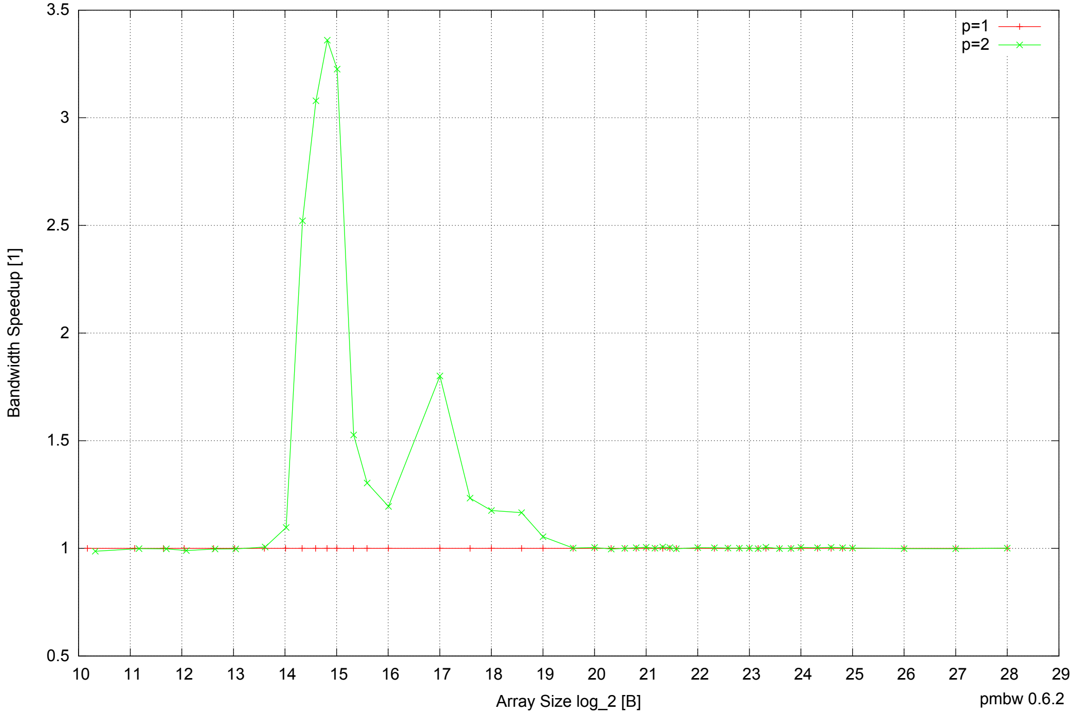
Raspberry Pi Model B: ARM1176JZF-S 512MB - Speedup of Parallel Memory Bandwidth - ScanRead64PtrUnrollLoop
