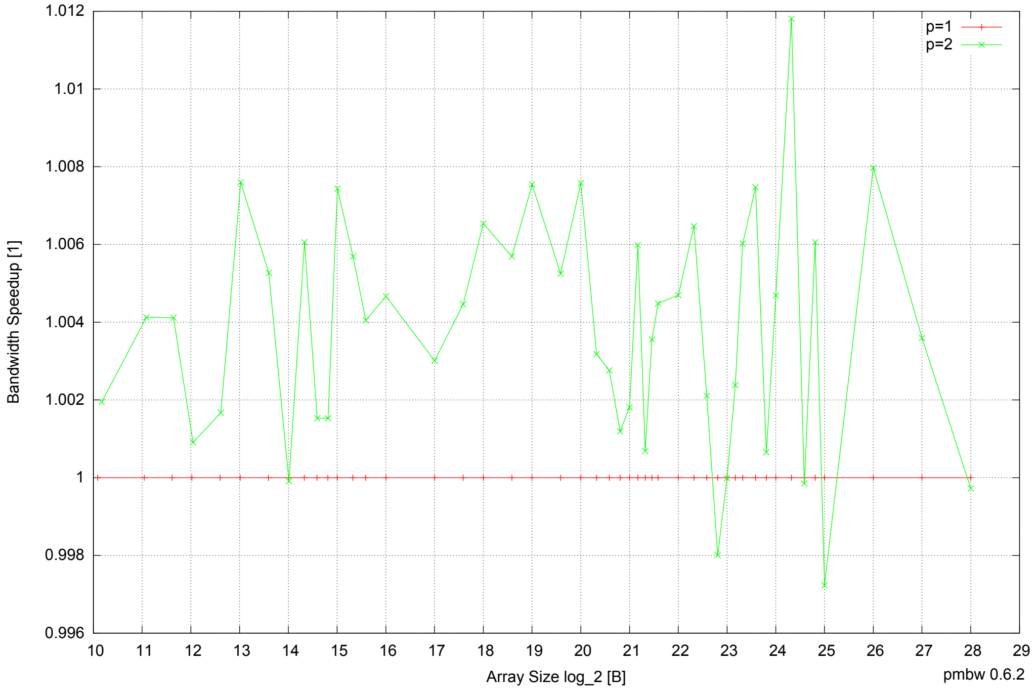
Raspberry Pi Model B: ARM1176JZF-S 512MB - Speedup of Parallel Memory Bandwidth - ScanWrite32PtrUnrollLoop
