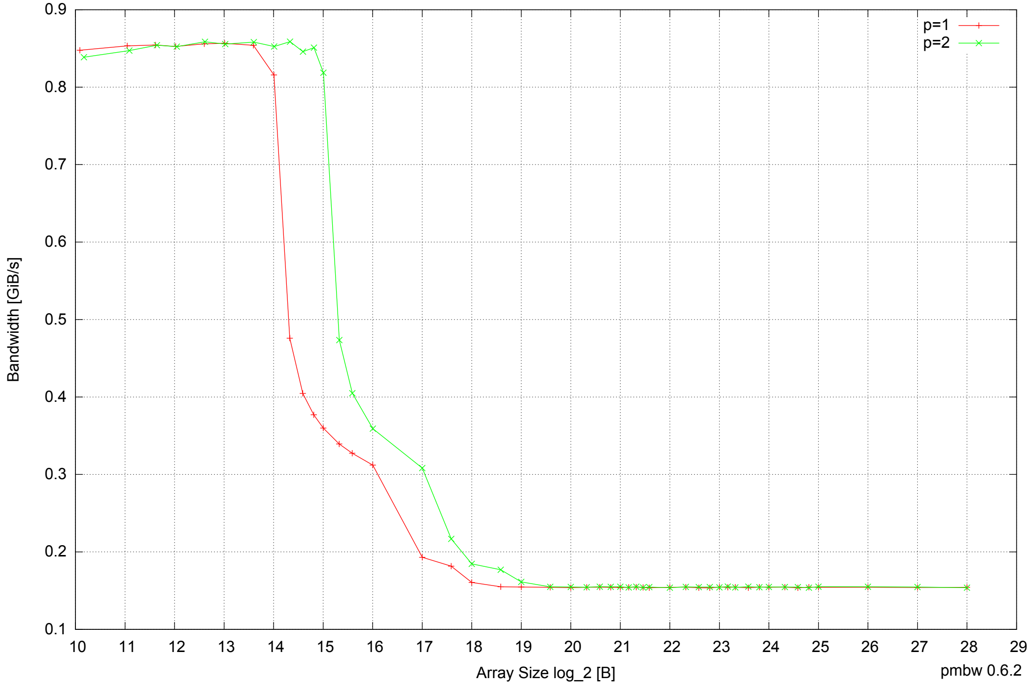
Raspberry Pi Model B: ARM1176JZF-S 512MB - Parallel Memory Bandwidth - ScanRead32PtrSimpleLoop
