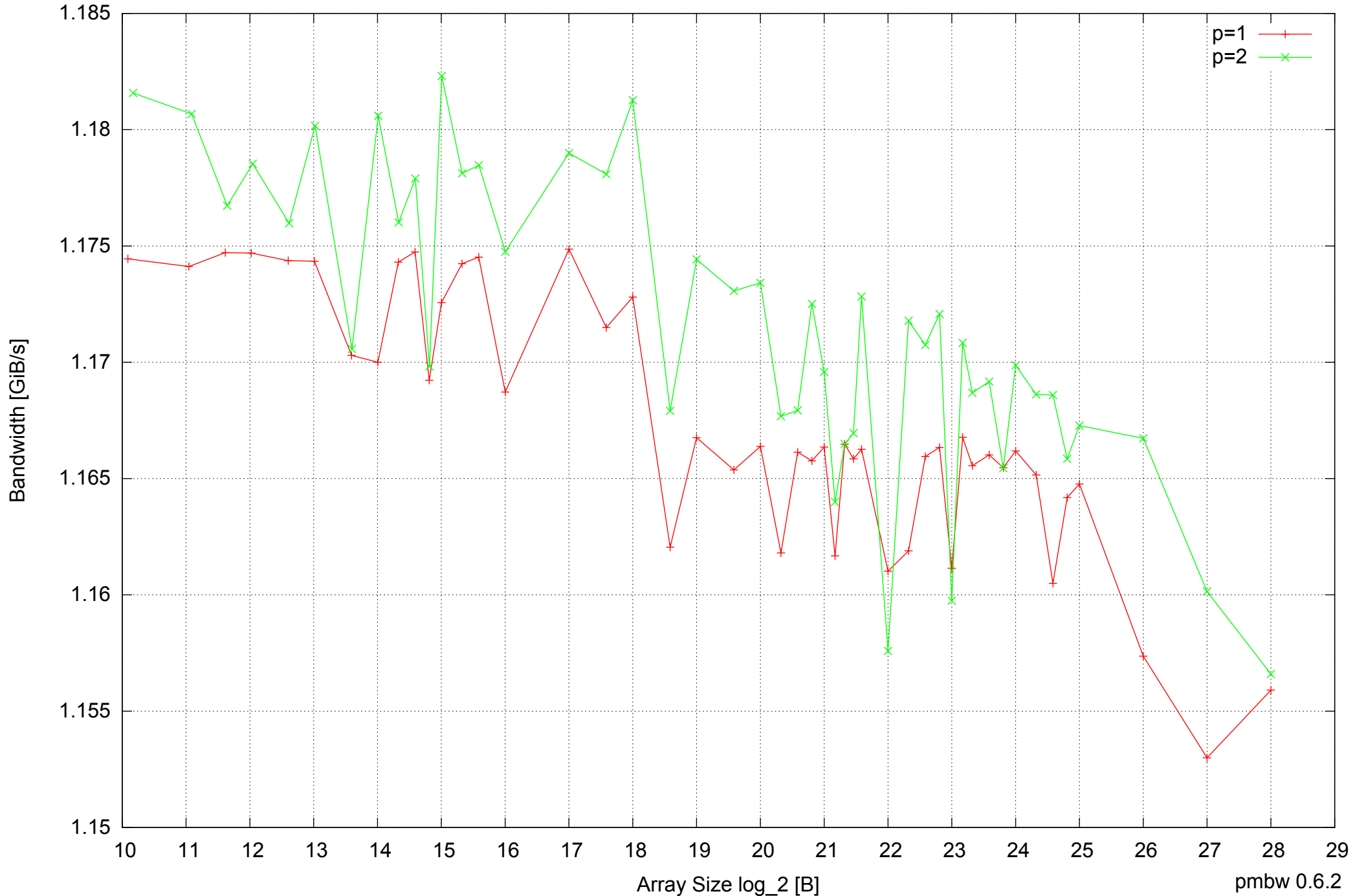
Raspberry Pi Model B: ARM1176JZF-S 512MB - Parallel Memory Bandwidth - ScanWrite32PtrMultiLoop
