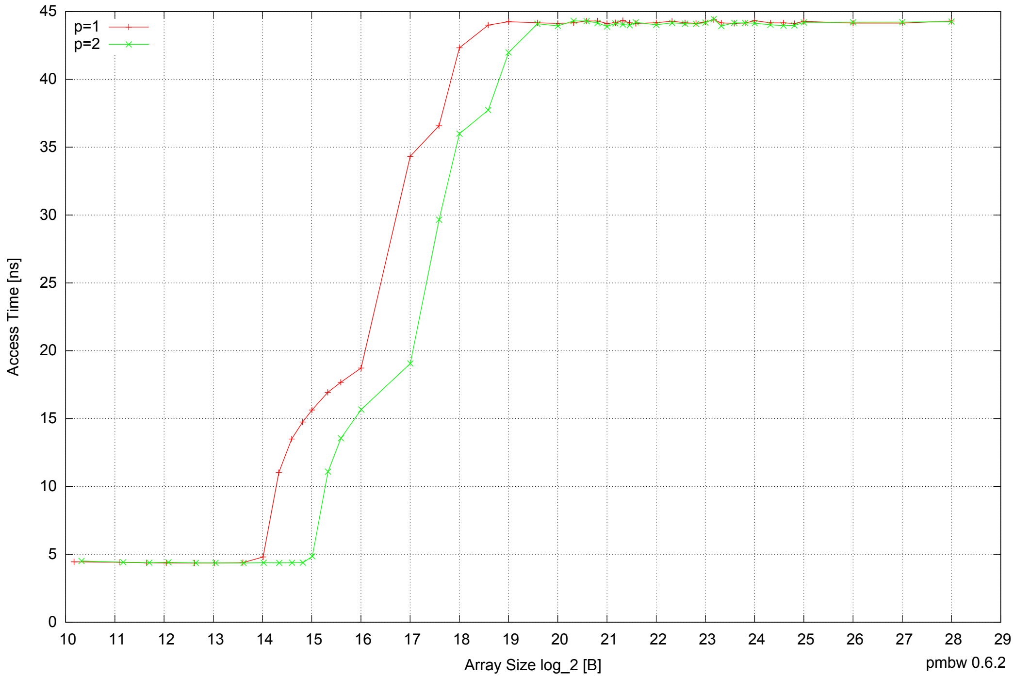
Raspberry Pi Model B: ARM1176JZF-S 512MB - Parallel Memory Access Time - ScanRead64PtrUnrollLoop
