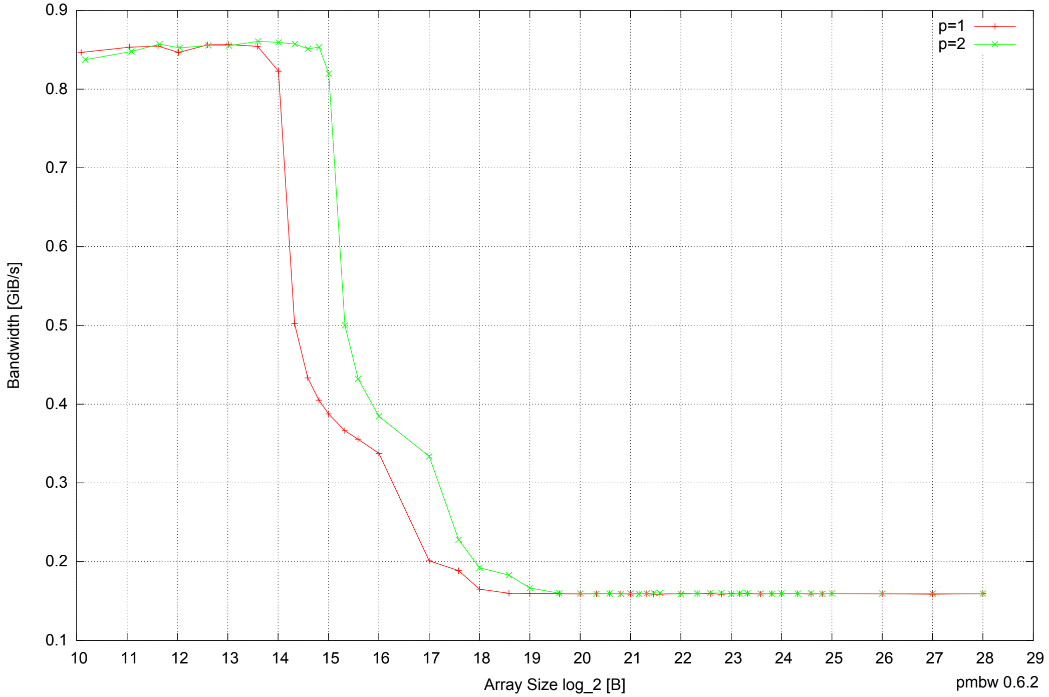
Raspberry Pi Model B: ARM1176JZF-S 512MB - Parallel Memory Bandwidth - ScanRead32PtrUnrollLoop
