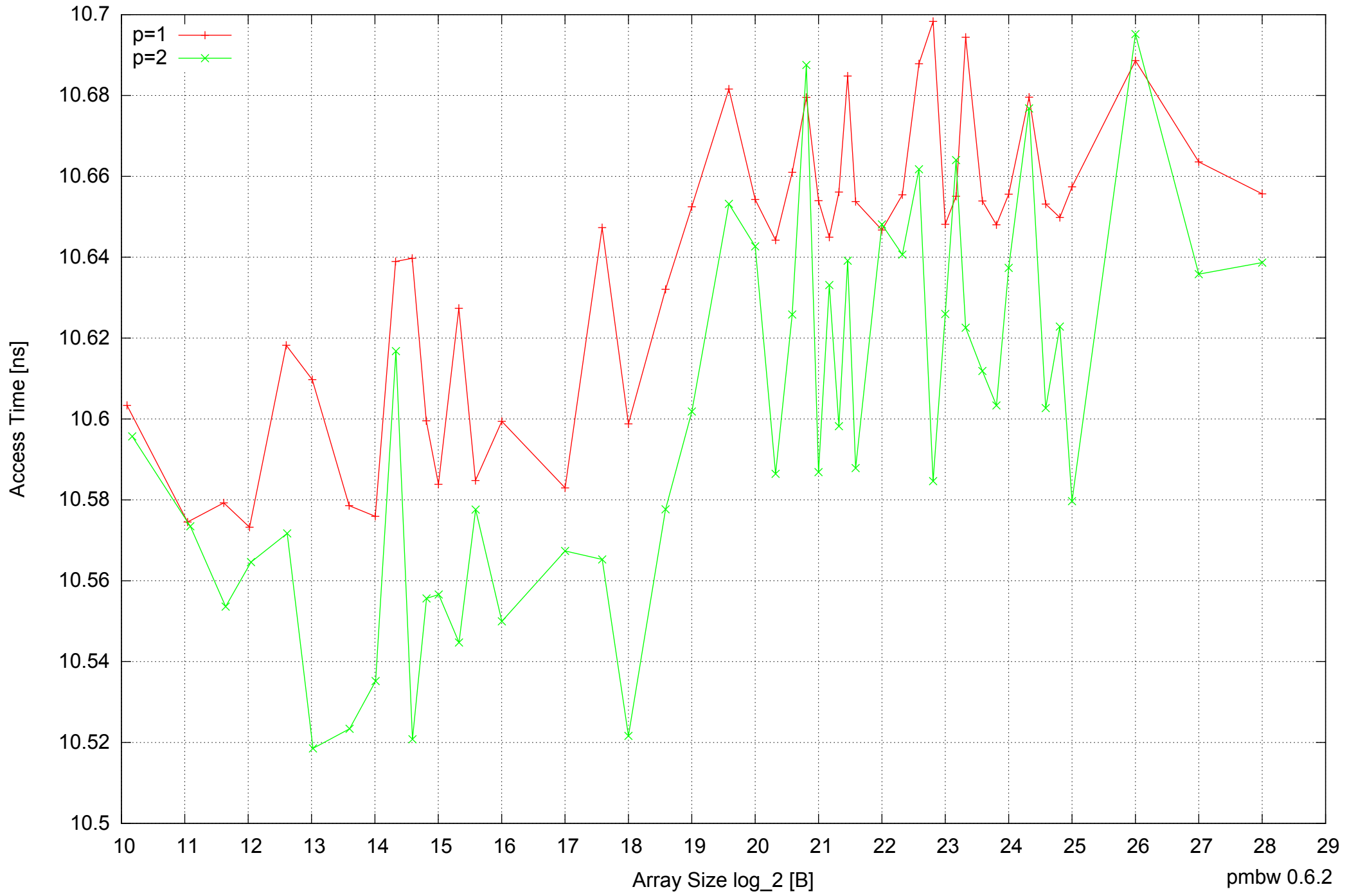
Raspberry Pi Model B: ARM1176JZF-S 512MB - Parallel Memory Access Time - ScanWrite32IndexSimpleLoop
