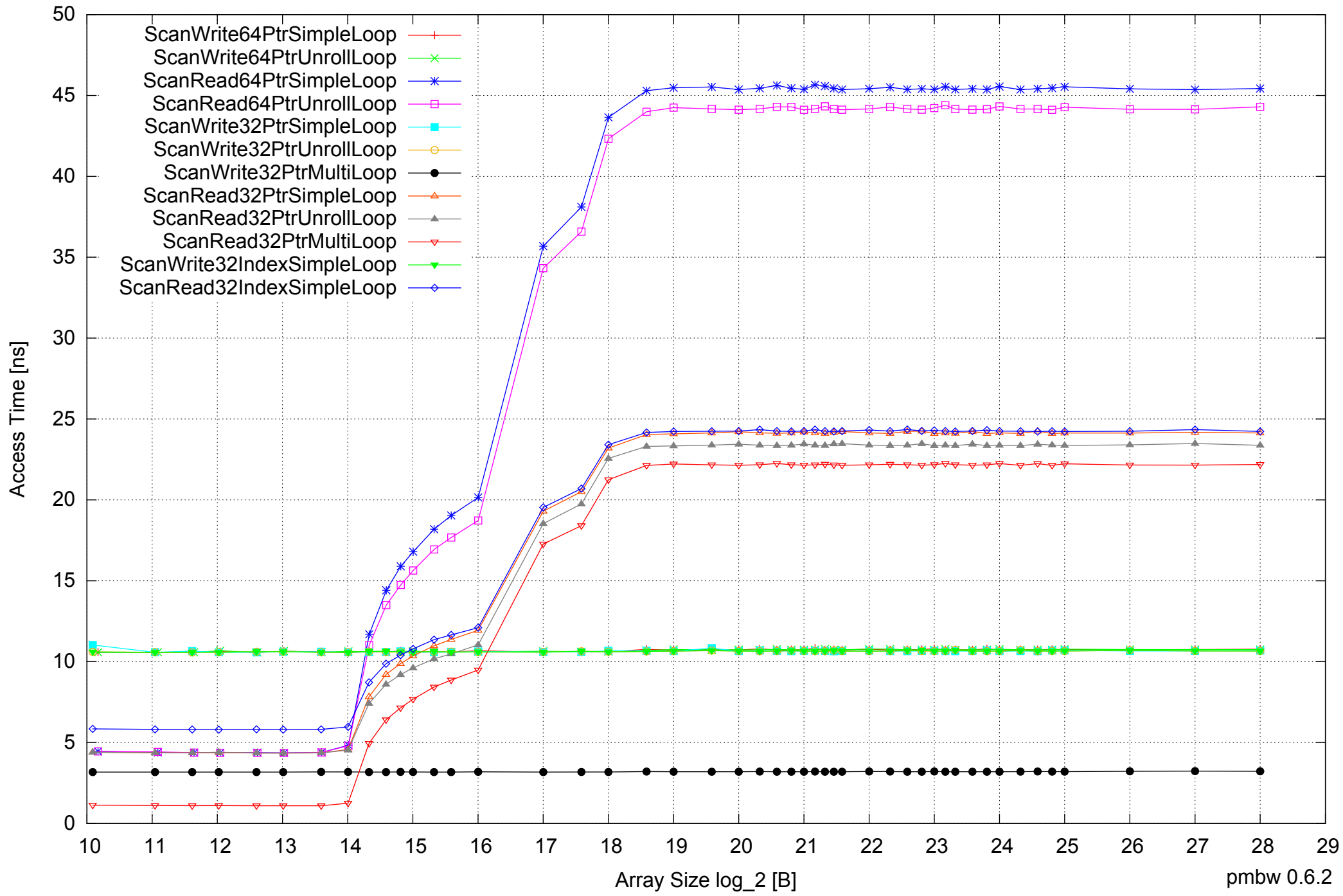
Raspberry Pi Model B: ARM1176JZF-S 512MB - One Thread Memory Latency (excluding Permutation)
