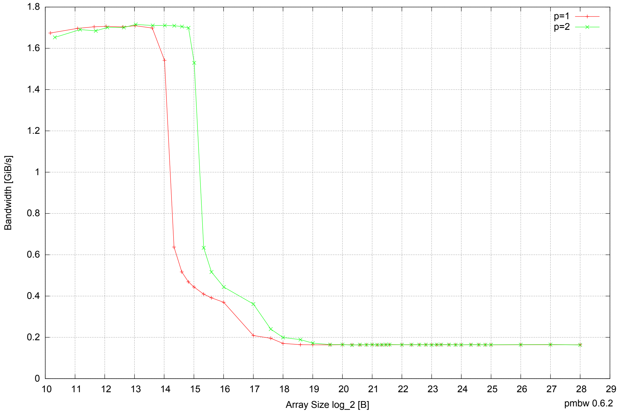
Raspberry Pi Model B: ARM1176JZF-S 512MB - Parallel Memory Bandwidth - ScanRead64PtrSimpleLoop
