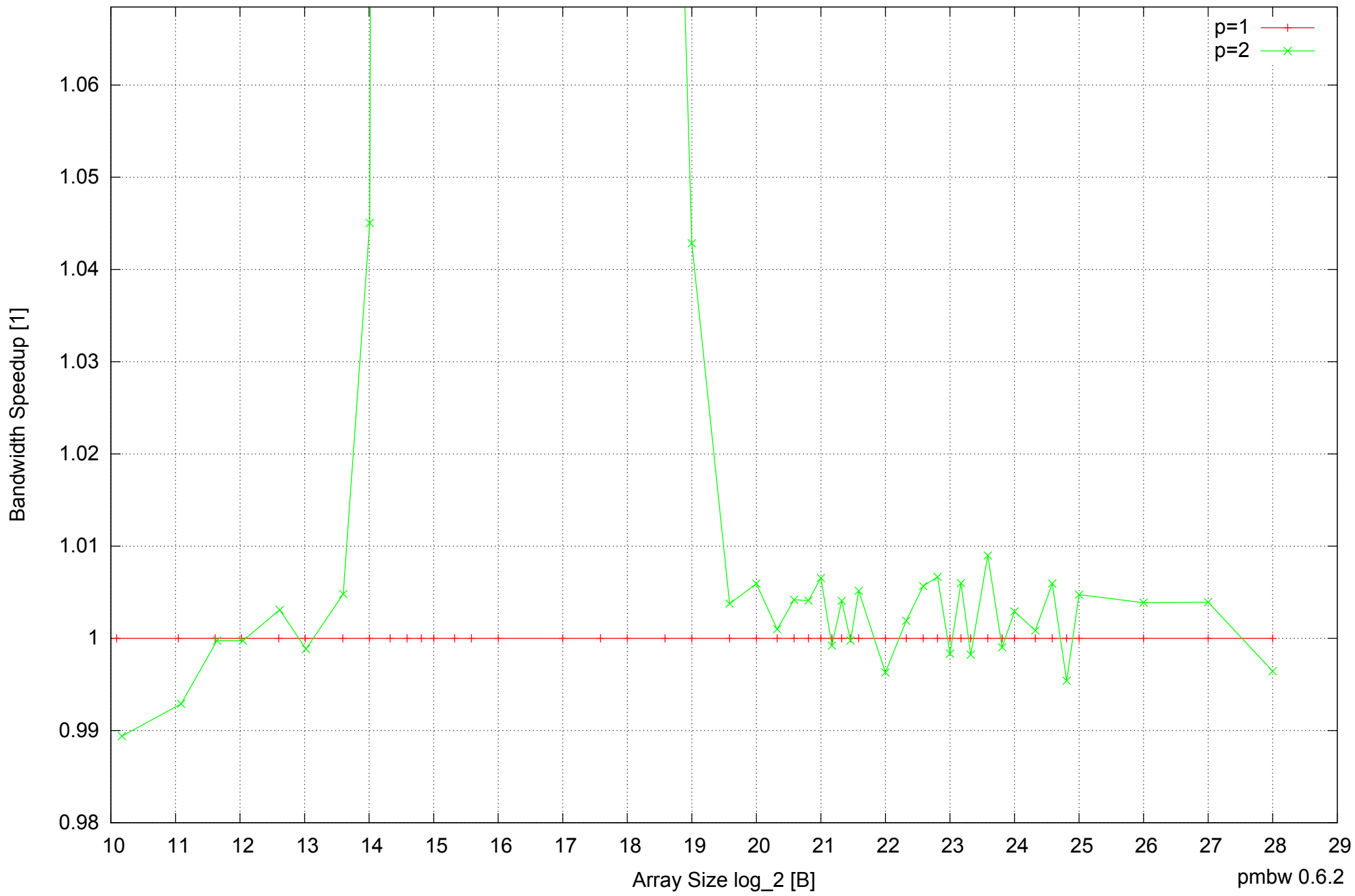
Raspberry Pi Model B: ARM1176JZF-S 512MB - Speedup of Parallel Memory Bandwidth (enlarged) - ScanRead32PtrSimpleLoop
