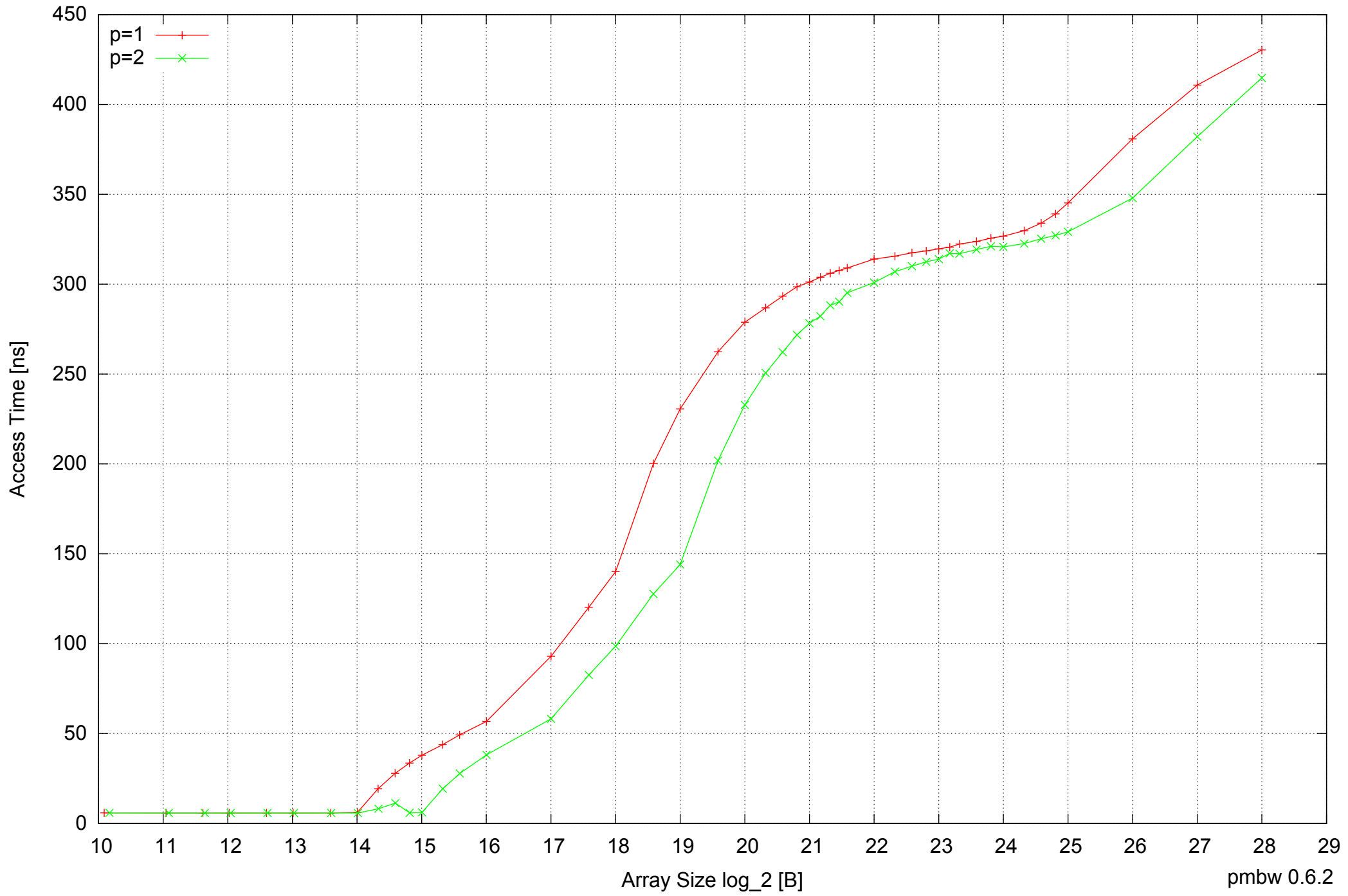
Raspberry Pi Model B: ARM1176JZF-S 512MB - Parallel Memory Access Time - PermRead32UnrollLoop
