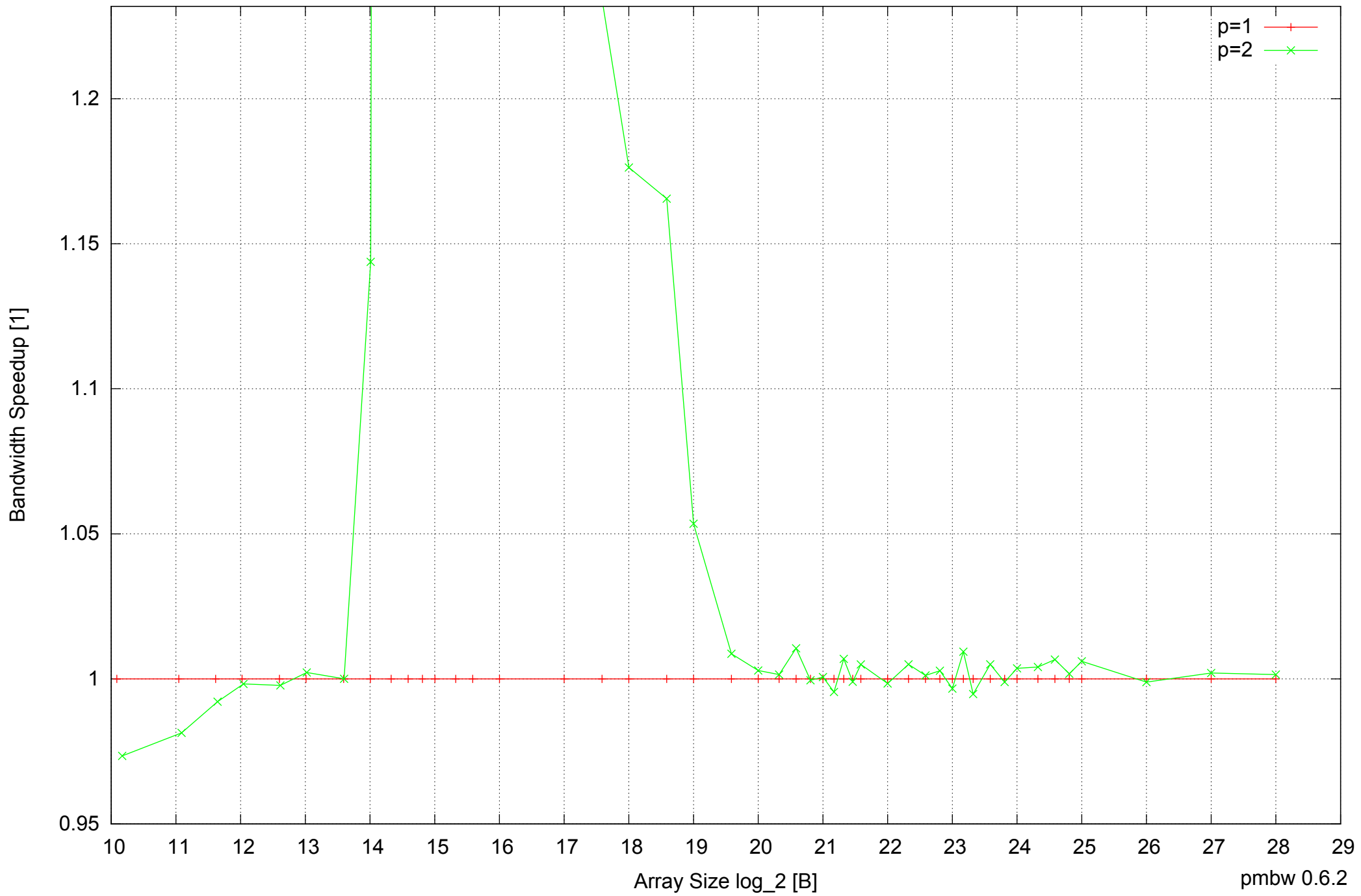
Raspberry Pi Model B: ARM1176JZF-S 512MB - Speedup of Parallel Memory Bandwidth (enlarged) - ScanRead32PtrMultiLoop
