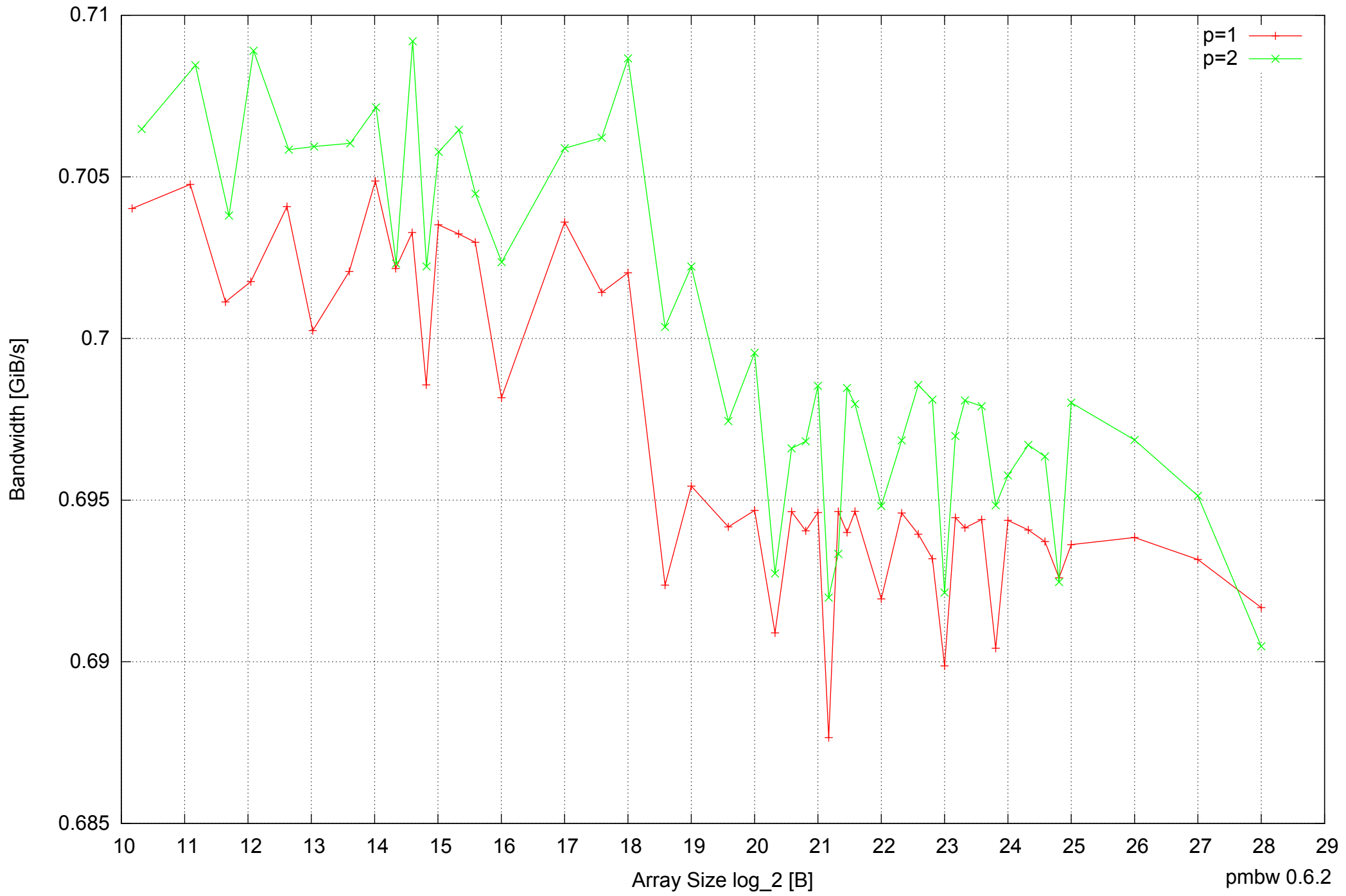
Raspberry Pi Model B: ARM1176JZF-S 512MB - Parallel Memory Bandwidth - ScanWrite64PtrSimpleLoop
