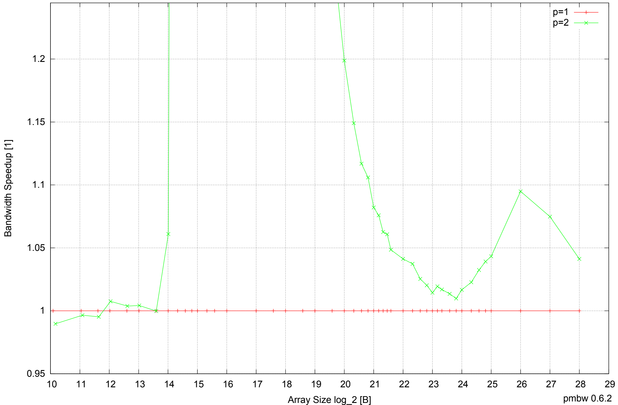
Raspberry Pi Model B: ARM1176JZF-S 512MB - Speedup of Parallel Memory Bandwidth (enlarged) - PermRead32SimpleLoop
