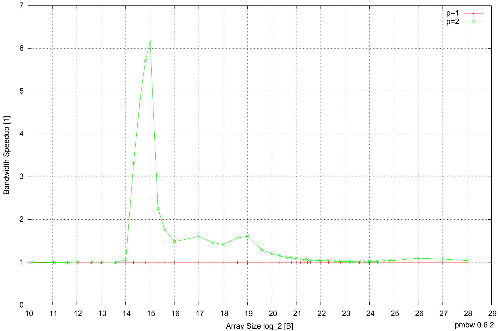
Raspberry Pi Model B: ARM1176JZF-S 512MB - Speedup of Parallel Memory Bandwidth - PermRead32SimpleLoop
