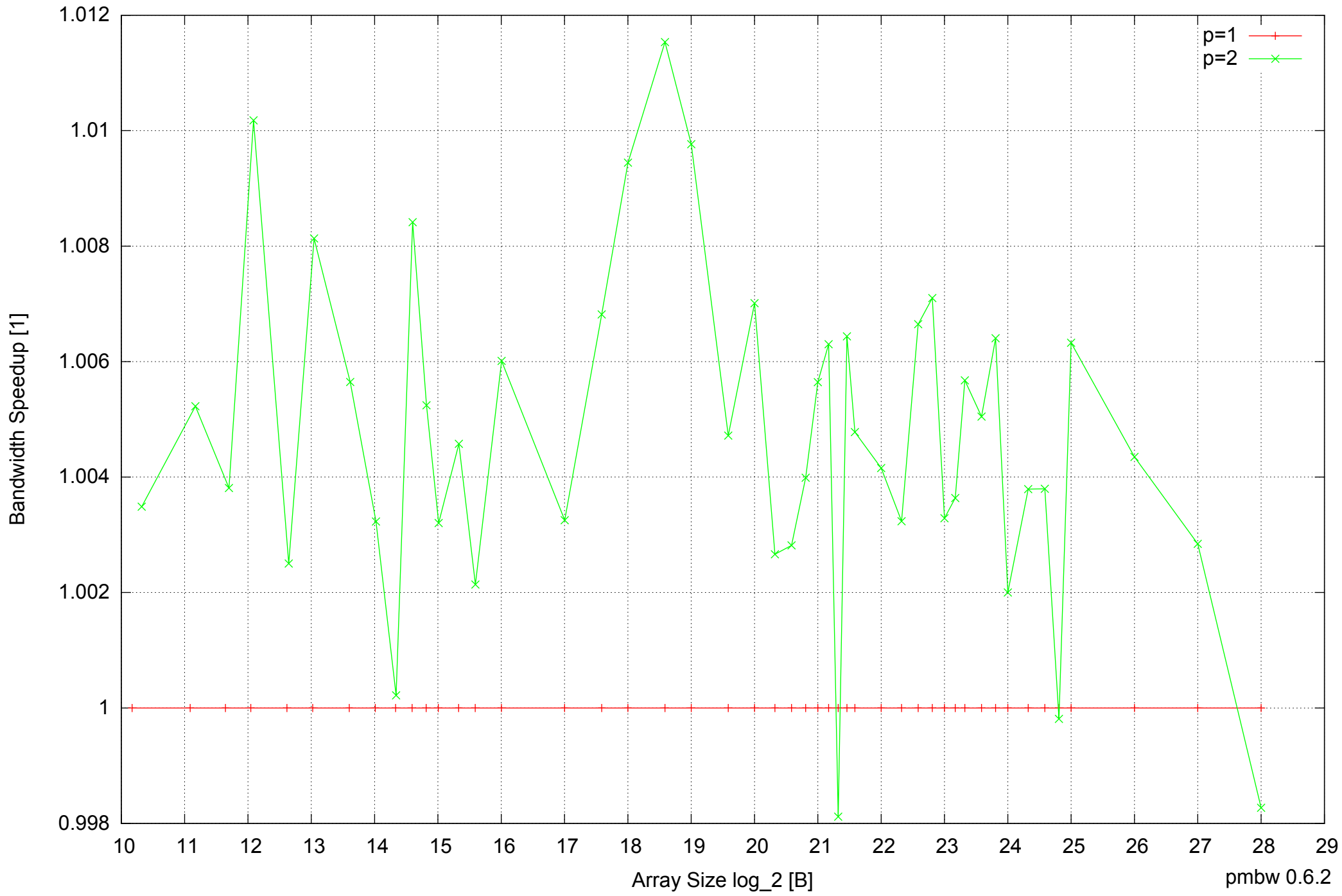
Raspberry Pi Model B: ARM1176JZF-S 512MB - Speedup of Parallel Memory Bandwidth - ScanWrite64PtrSimpleLoop
