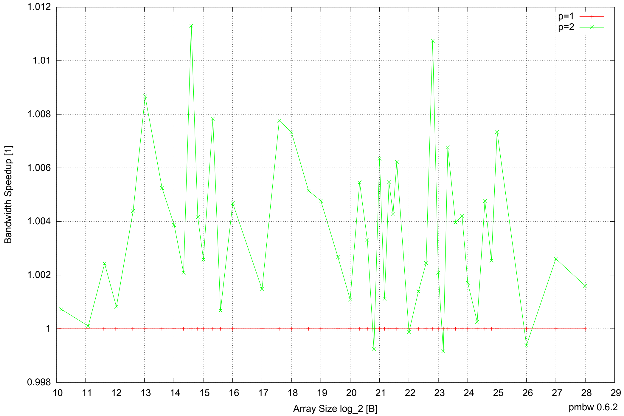
Raspberry Pi Model B: ARM1176JZF-S 512MB - Speedup of Parallel Memory Bandwidth - ScanWrite32IndexSimpleLoop
