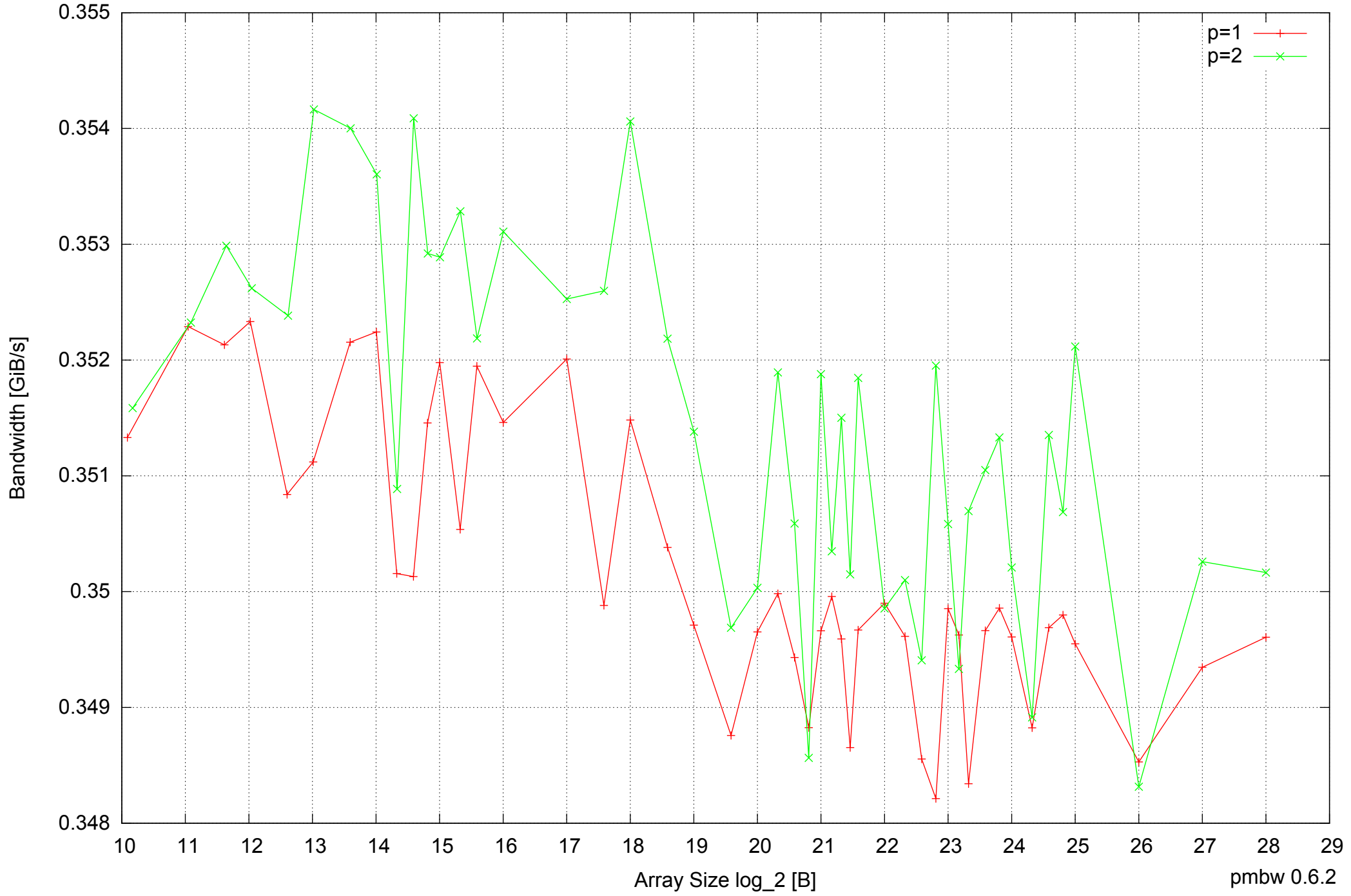
Raspberry Pi Model B: ARM1176JZF-S 512MB - Parallel Memory Bandwidth - ScanWrite32IndexSimpleLoop
