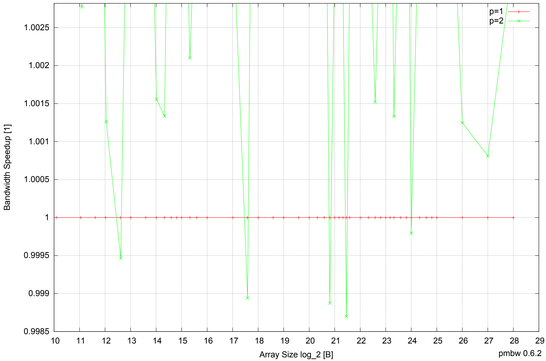
Raspberry Pi Model B: ARM1176JZF-S 512MB - Speedup of Parallel Memory Bandwidth (enlarged) - ScanWrite32PtrSimpleLoop
