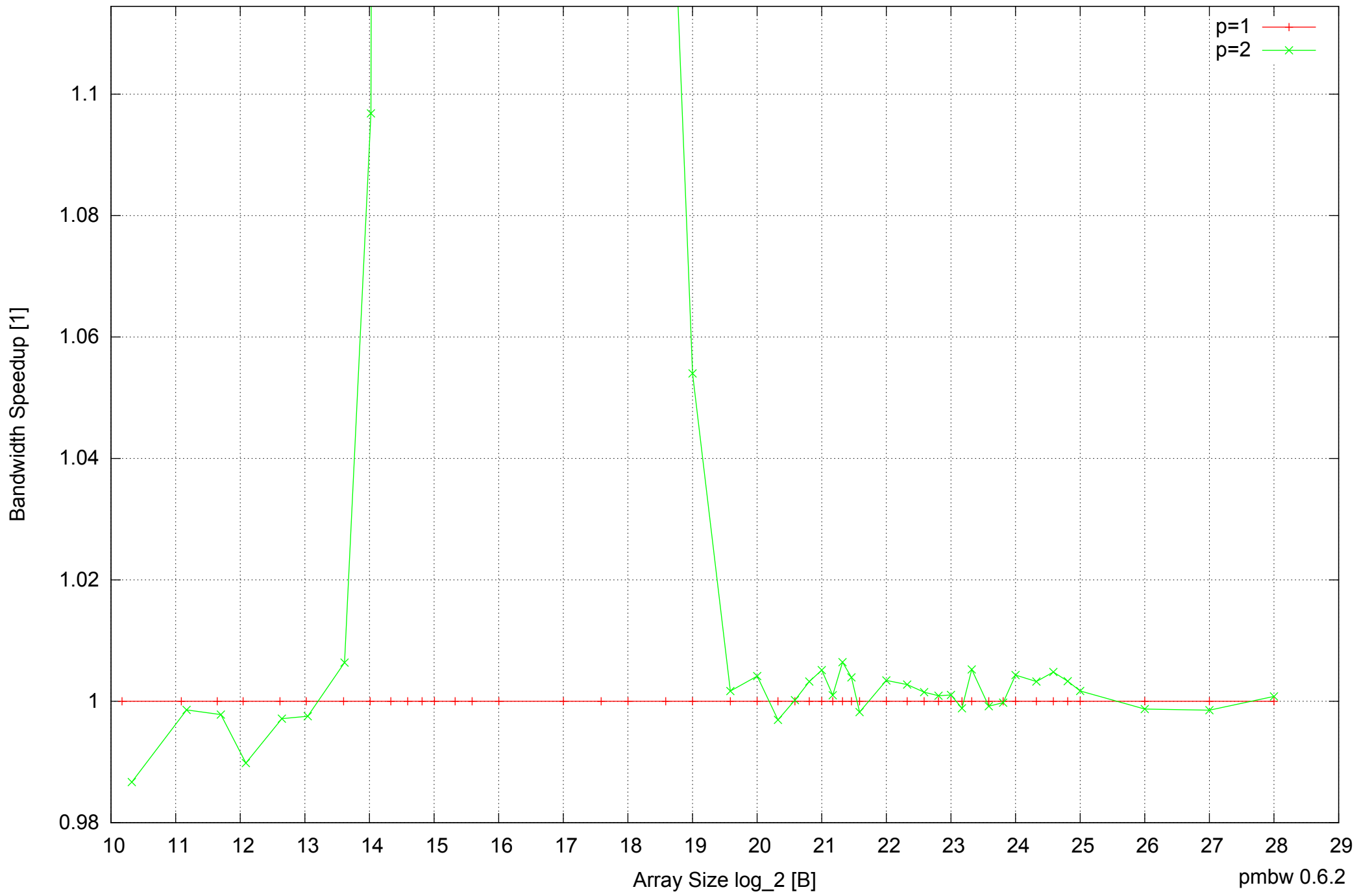
Raspberry Pi Model B: ARM1176JZF-S 512MB - Speedup of Parallel Memory Bandwidth (enlarged) - ScanRead64PtrUnrollLoop
