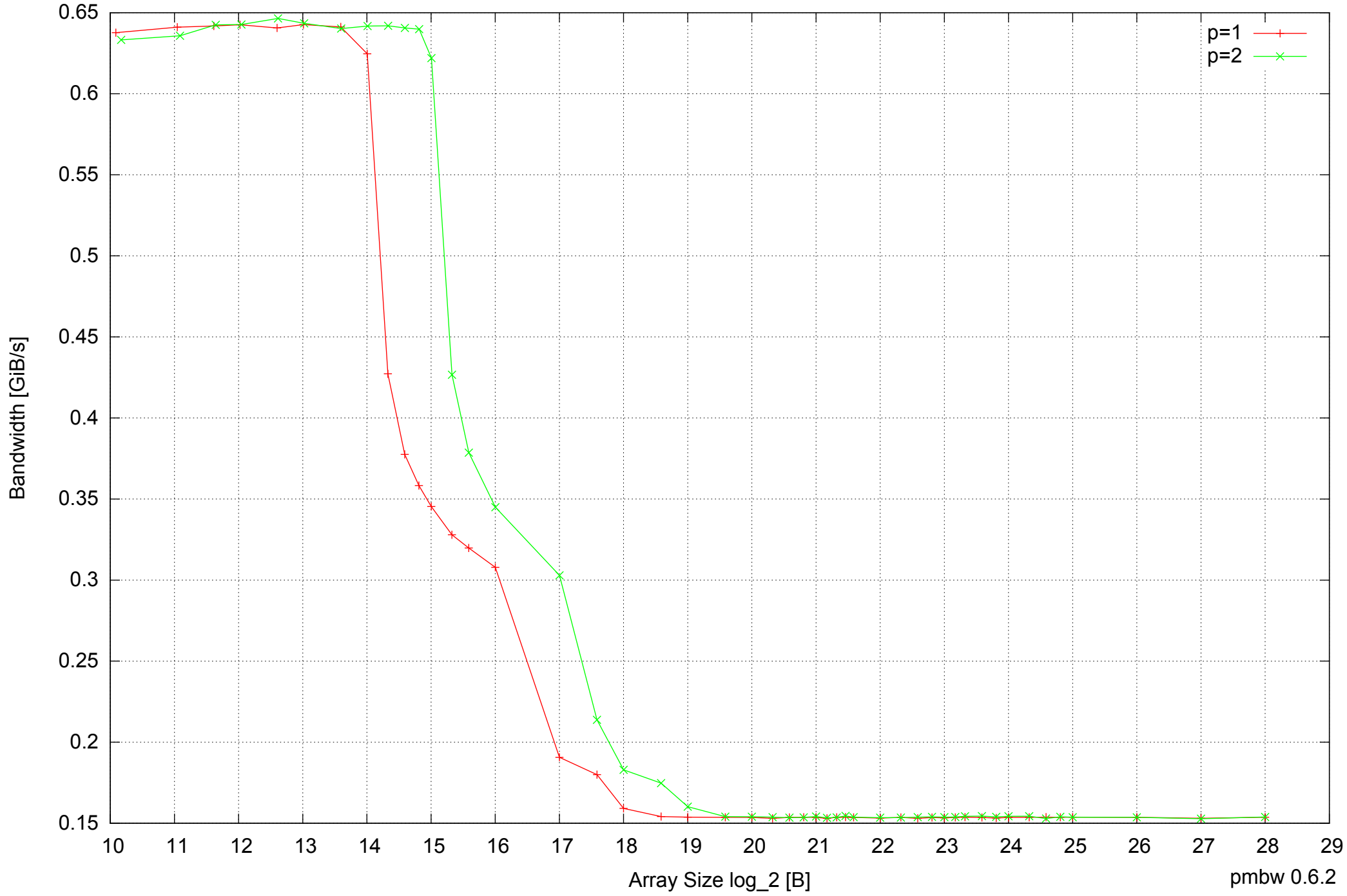
Raspberry Pi Model B: ARM1176JZF-S 512MB - Parallel Memory Bandwidth - ScanRead32IndexSimpleLoop
