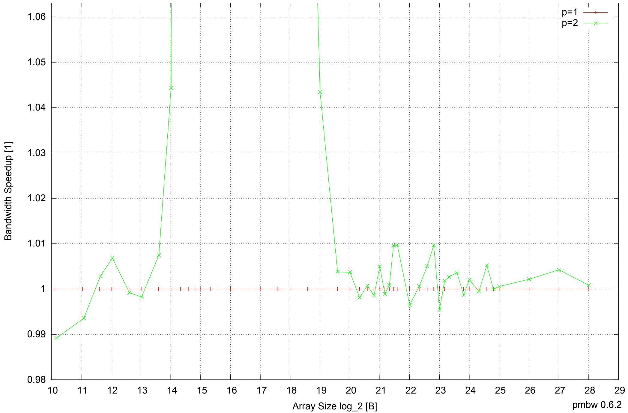
Raspberry Pi Model B: ARM1176JZF-S 512MB - Speedup of Parallel Memory Bandwidth (enlarged) - ScanRead32PtrUnrollLoop
