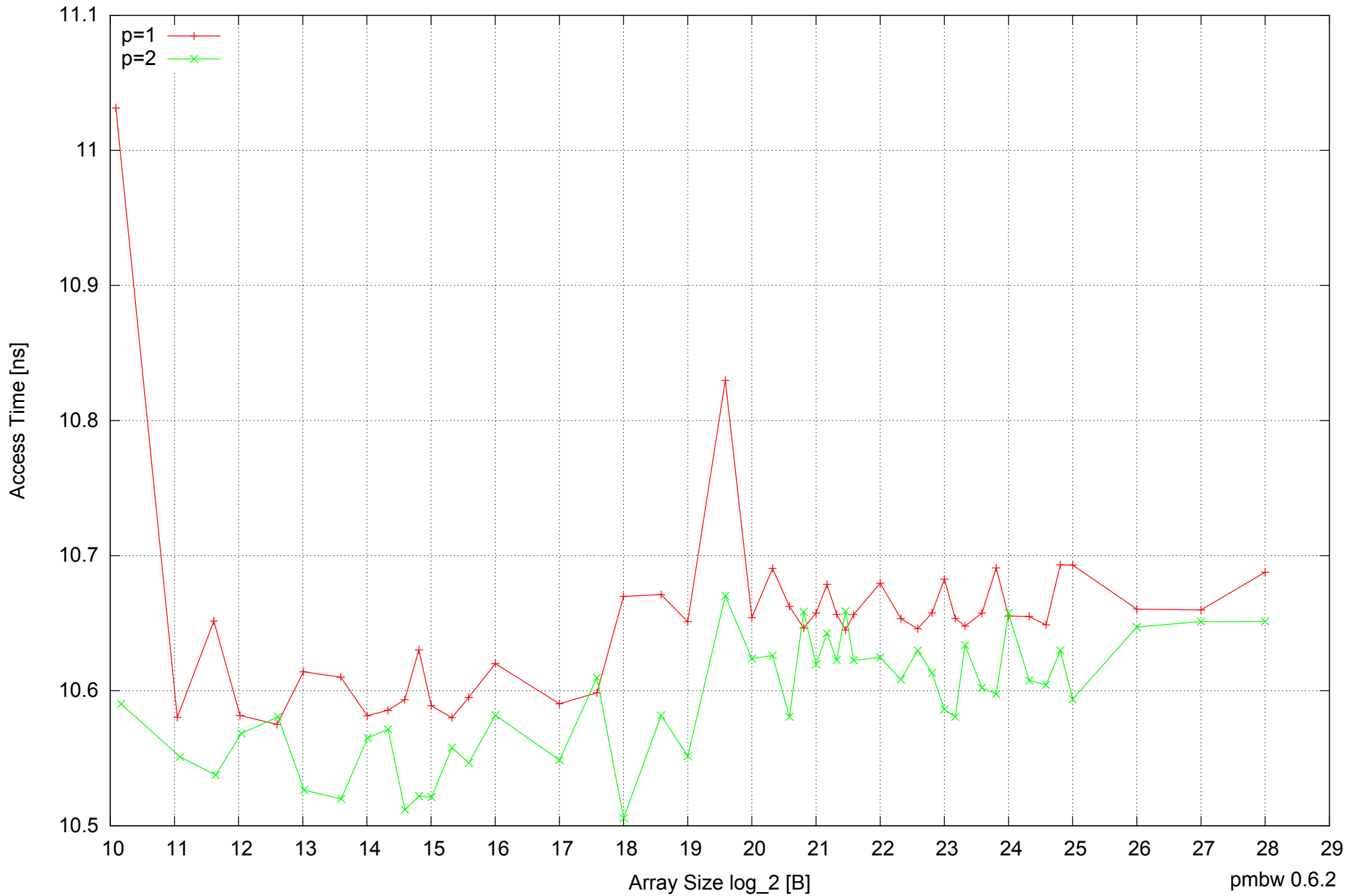
Raspberry Pi Model B: ARM1176JZF-S 512MB - Parallel Memory Access Time - ScanWrite32PtrSimpleLoop
