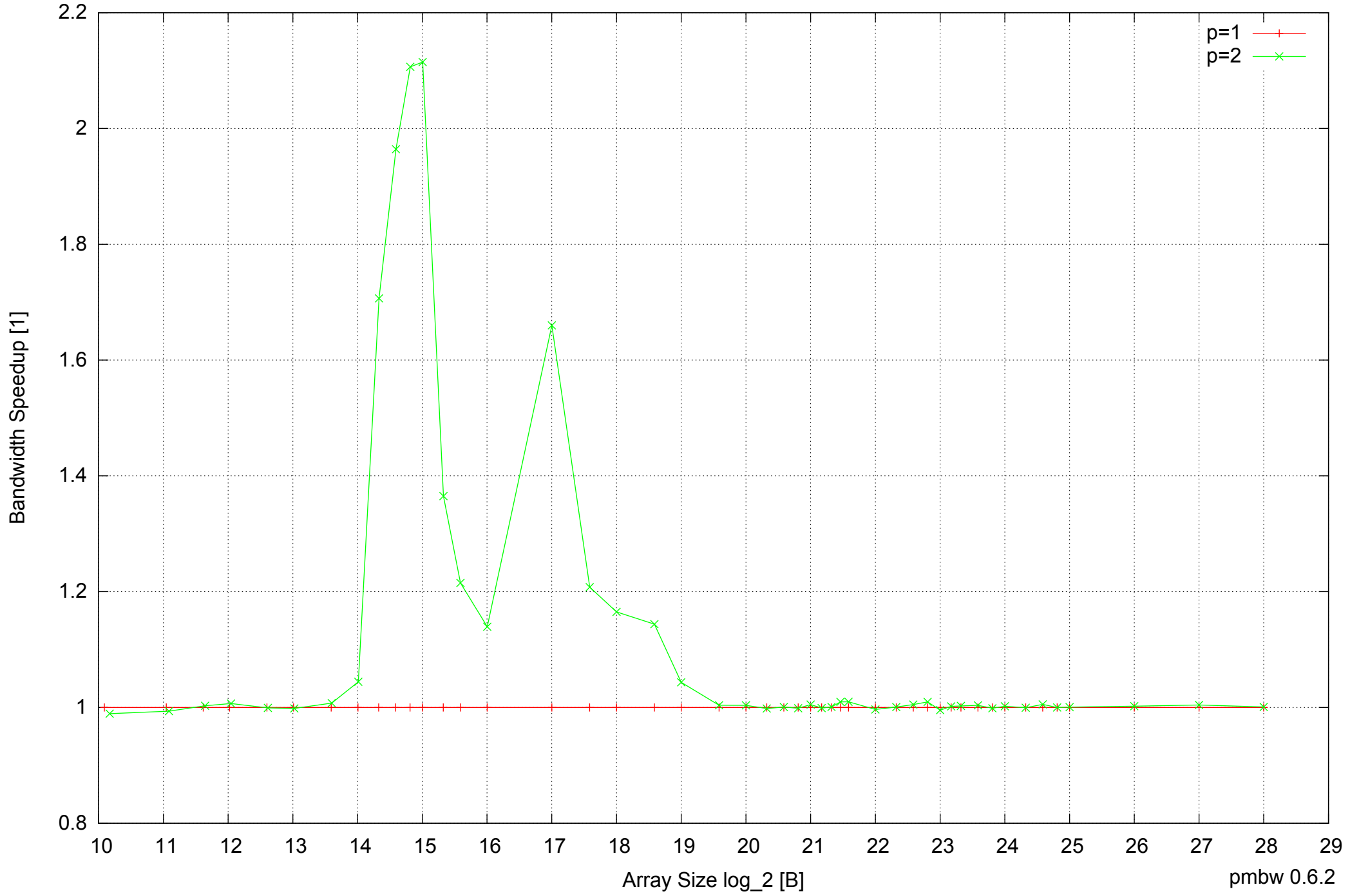
Raspberry Pi Model B: ARM1176JZF-S 512MB - Speedup of Parallel Memory Bandwidth - ScanRead32PtrUnrollLoop
