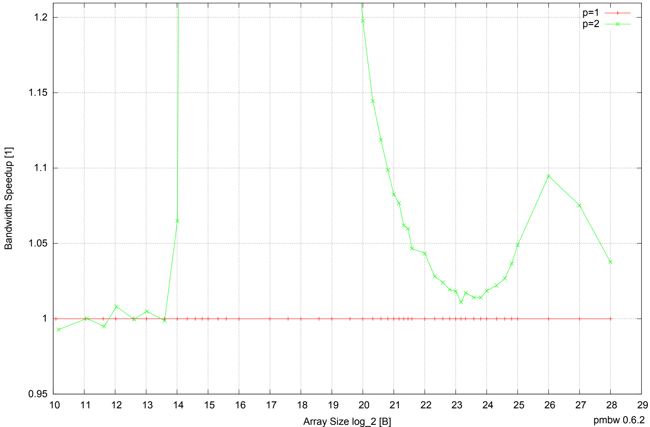
Raspberry Pi Model B: ARM1176JZF-S 512MB - Speedup of Parallel Memory Bandwidth (enlarged) - PermRead32UnrollLoop
