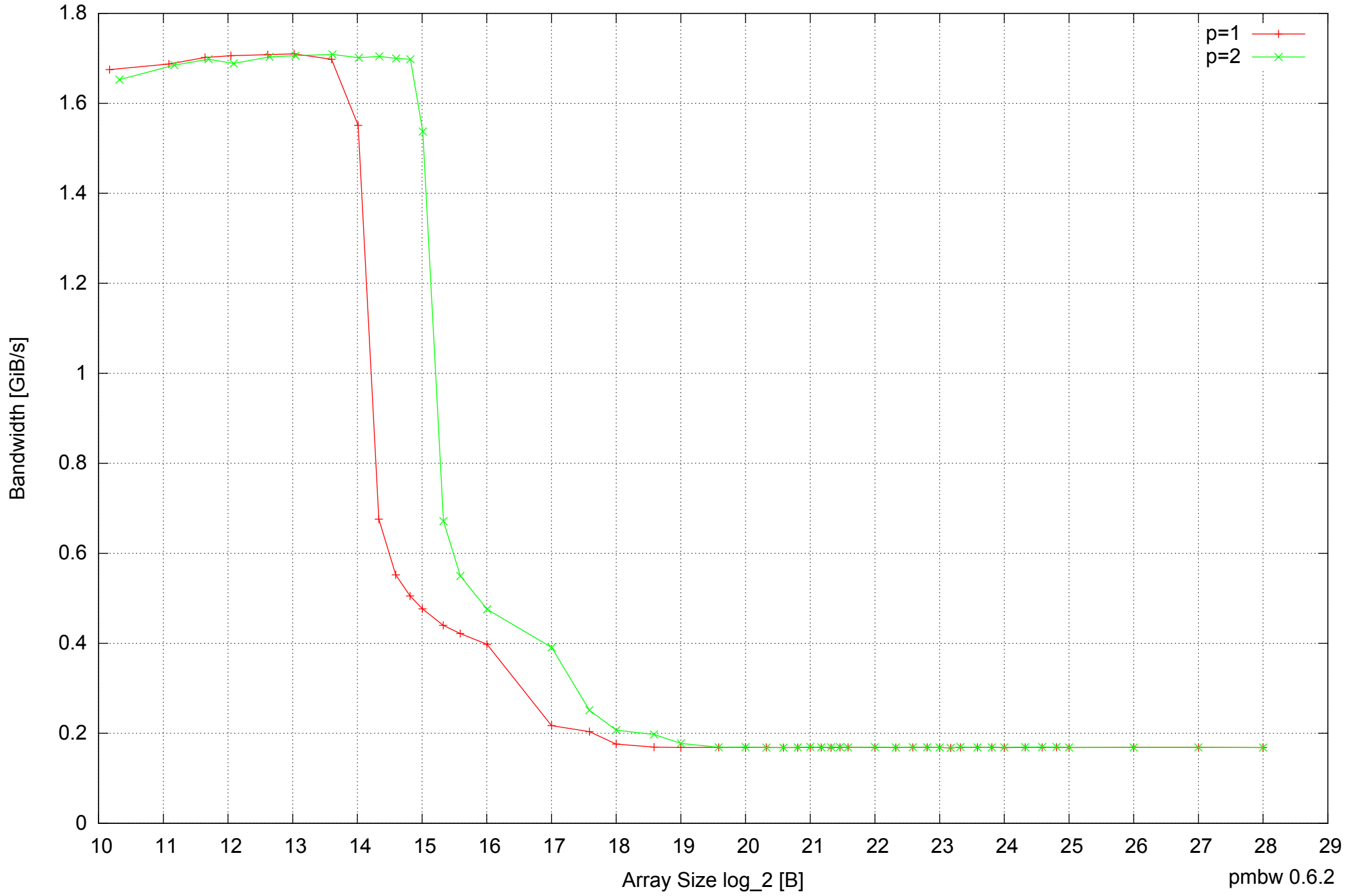
Raspberry Pi Model B: ARM1176JZF-S 512MB - Parallel Memory Bandwidth - ScanRead64PtrUnrollLoop
