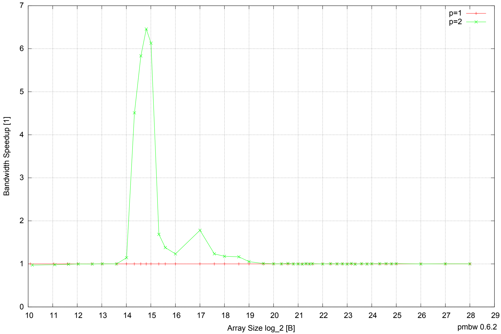
Raspberry Pi Model B: ARM1176JZF-S 512MB - Speedup of Parallel Memory Bandwidth - ScanRead32PtrMultiLoop
