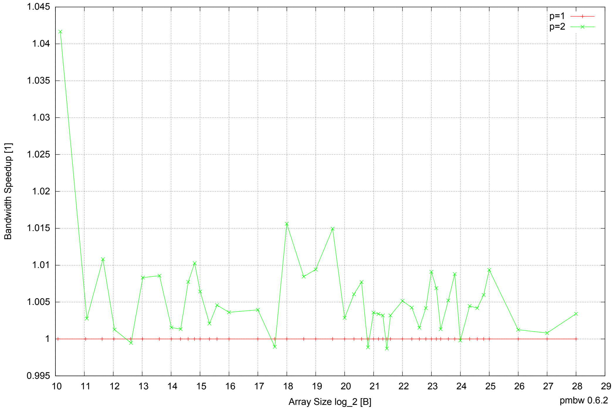
Raspberry Pi Model B: ARM1176JZF-S 512MB - Speedup of Parallel Memory Bandwidth - ScanWrite32PtrSimpleLoop
