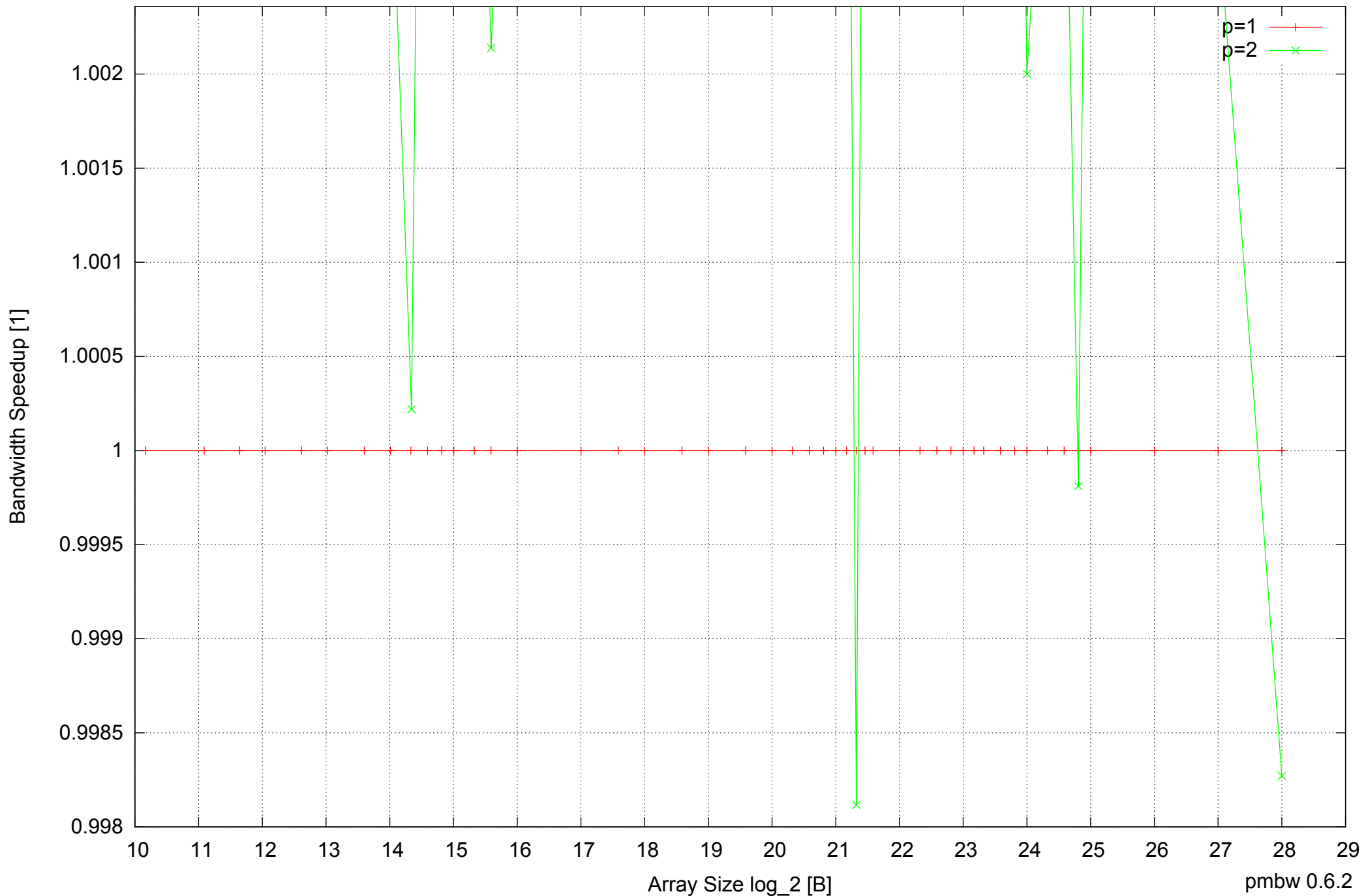
Raspberry Pi Model B: ARM1176JZF-S 512MB - Speedup of Parallel Memory Bandwidth (enlarged) - ScanWrite64PtrSimpleLoop
