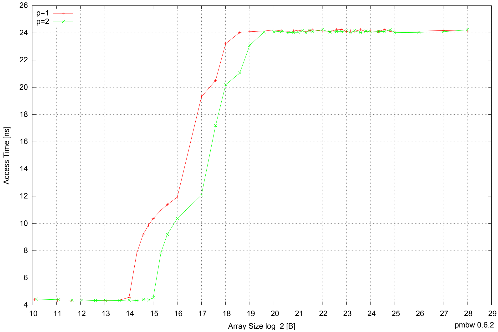
Raspberry Pi Model B: ARM1176JZF-S 512MB - Parallel Memory Access Time - ScanRead32PtrSimpleLoop
