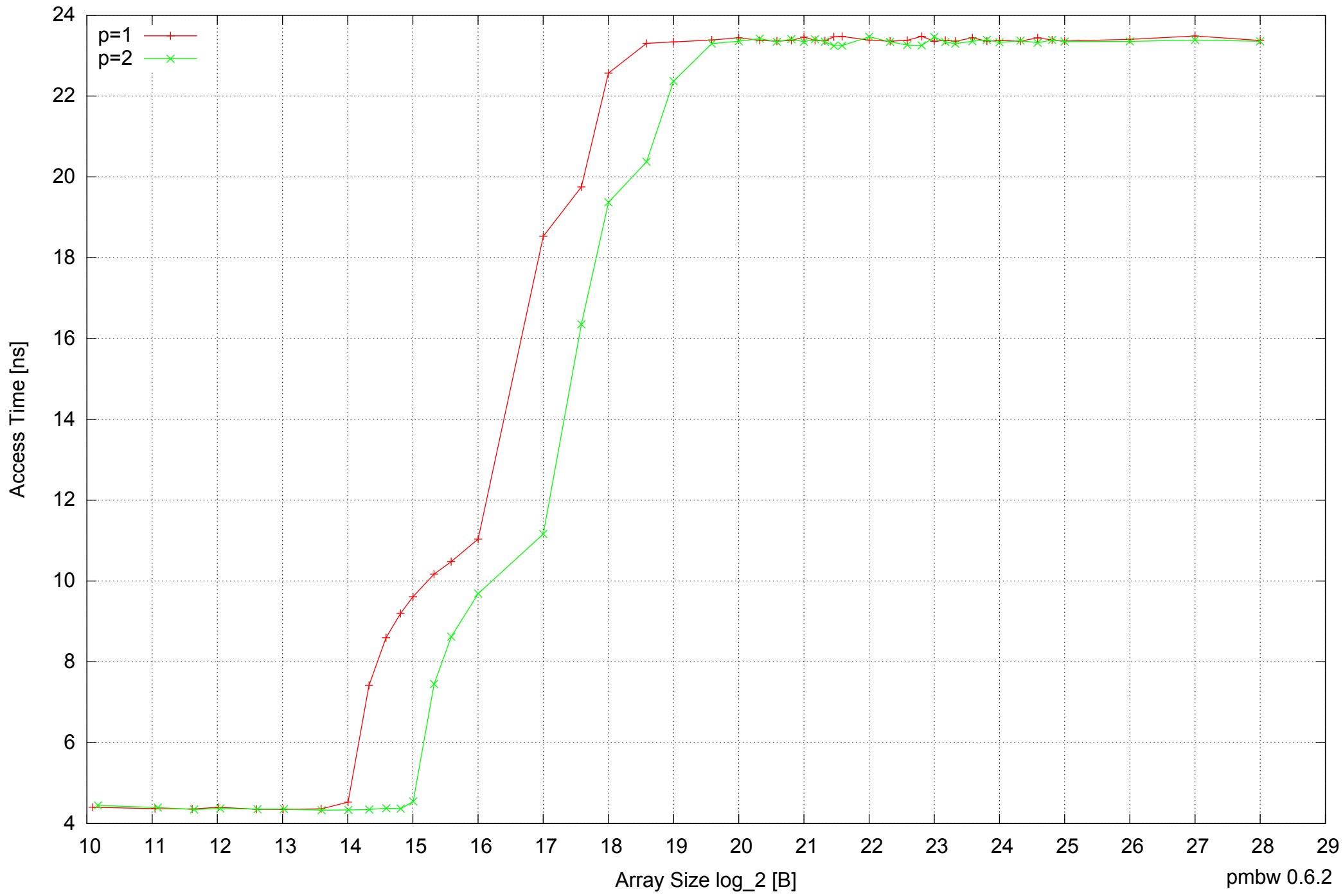
Raspberry Pi Model B: ARM1176JZF-S 512MB - Parallel Memory Access Time - ScanRead32PtrUnrollLoop
