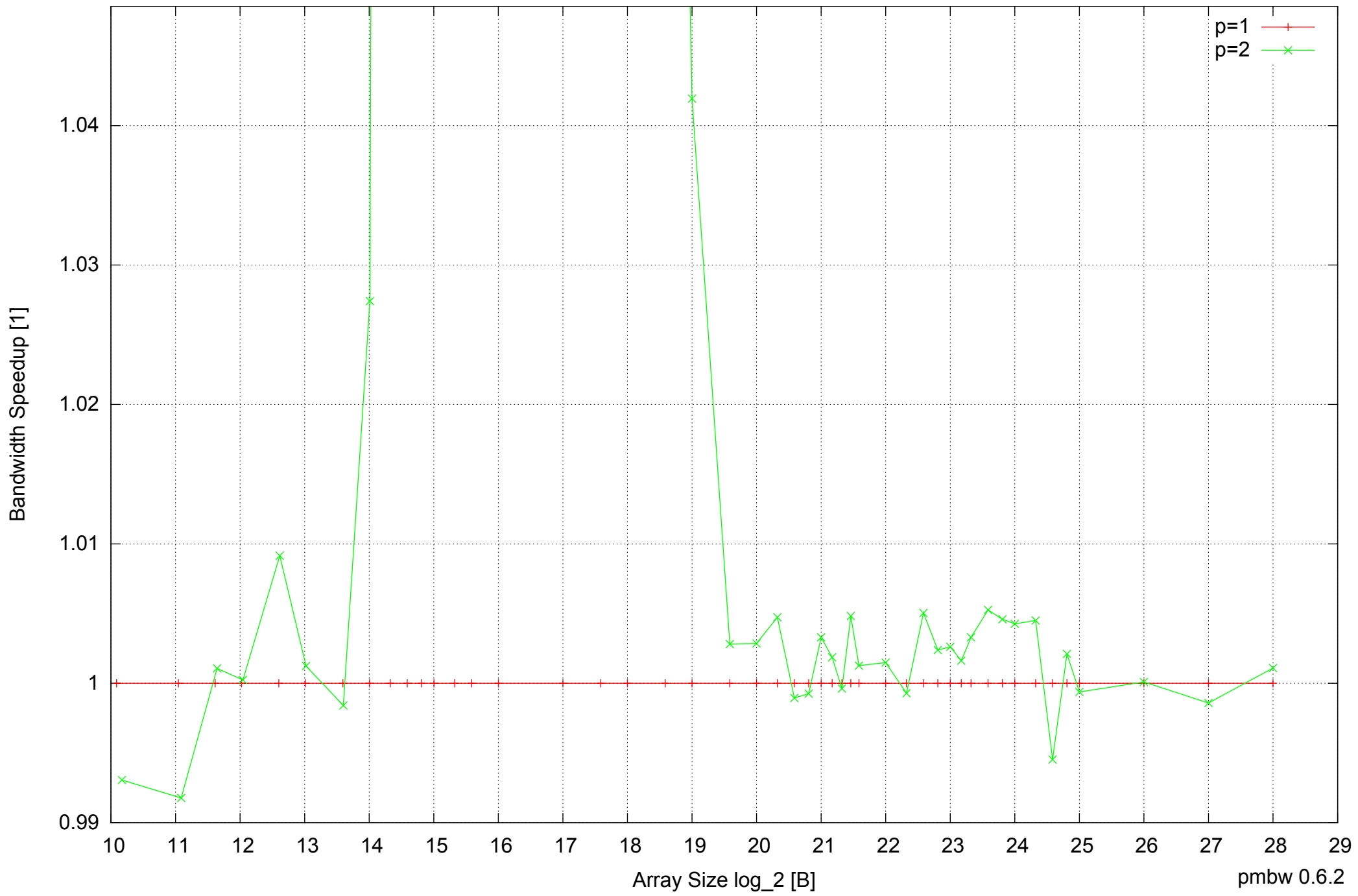
Raspberry Pi Model B: ARM1176JZF-S 512MB - Speedup of Parallel Memory Bandwidth (enlarged) - ScanRead32IndexSimpleLoop
