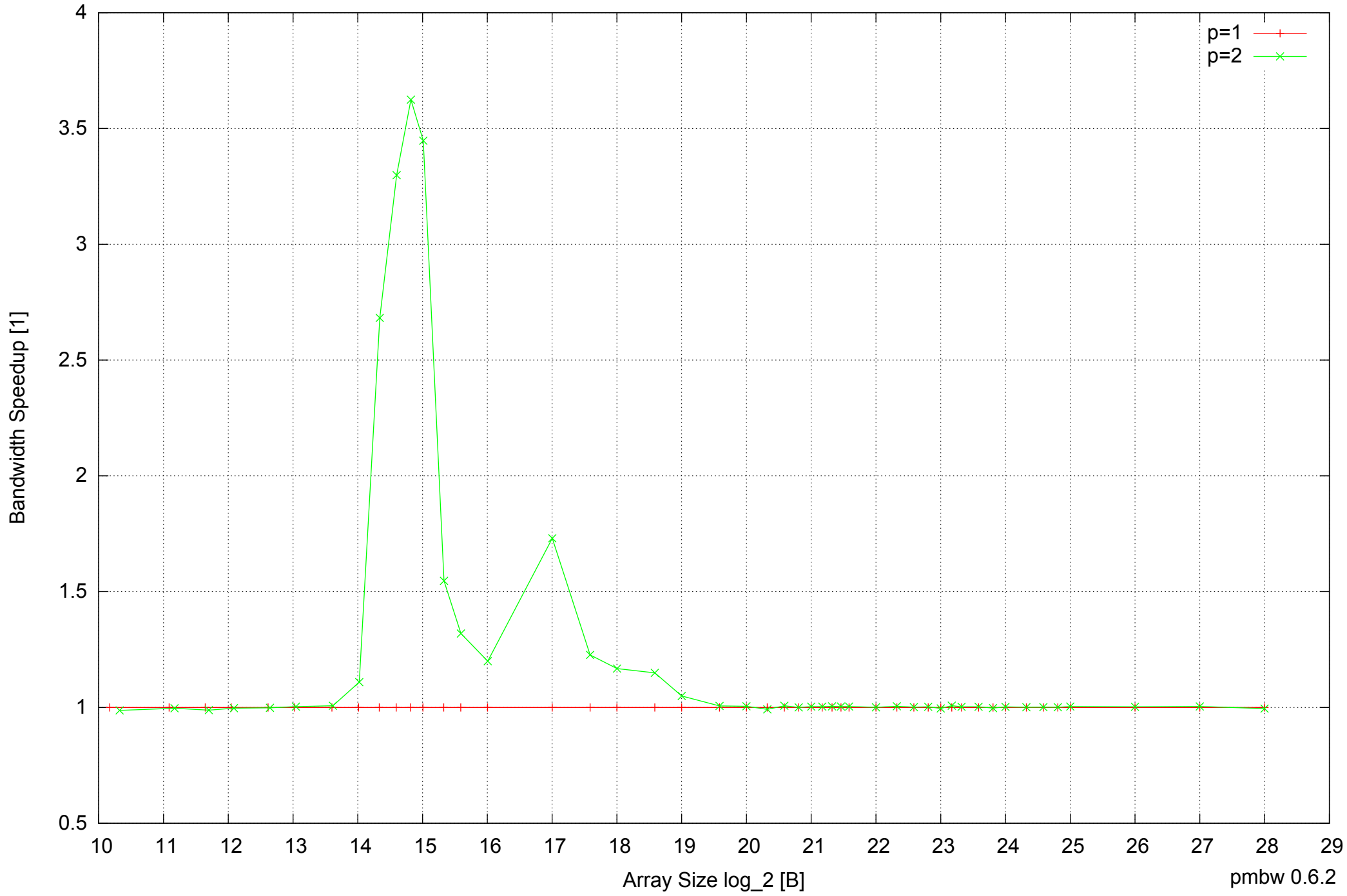
Raspberry Pi Model B: ARM1176JZF-S 512MB - Speedup of Parallel Memory Bandwidth - ScanRead64PtrSimpleLoop
