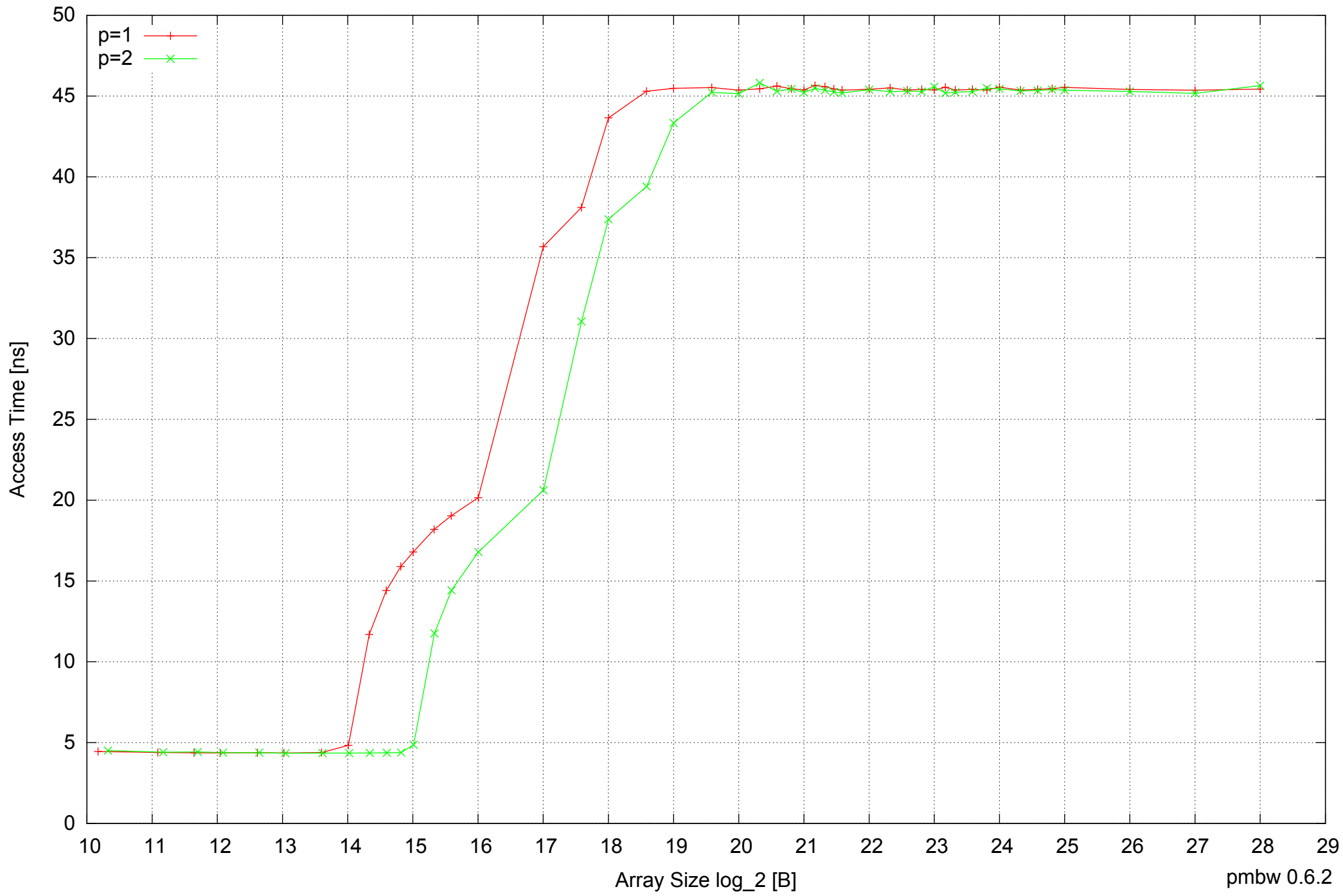
Raspberry Pi Model B: ARM1176JZF-S 512MB - Parallel Memory Access Time - ScanRead64PtrSimpleLoop
