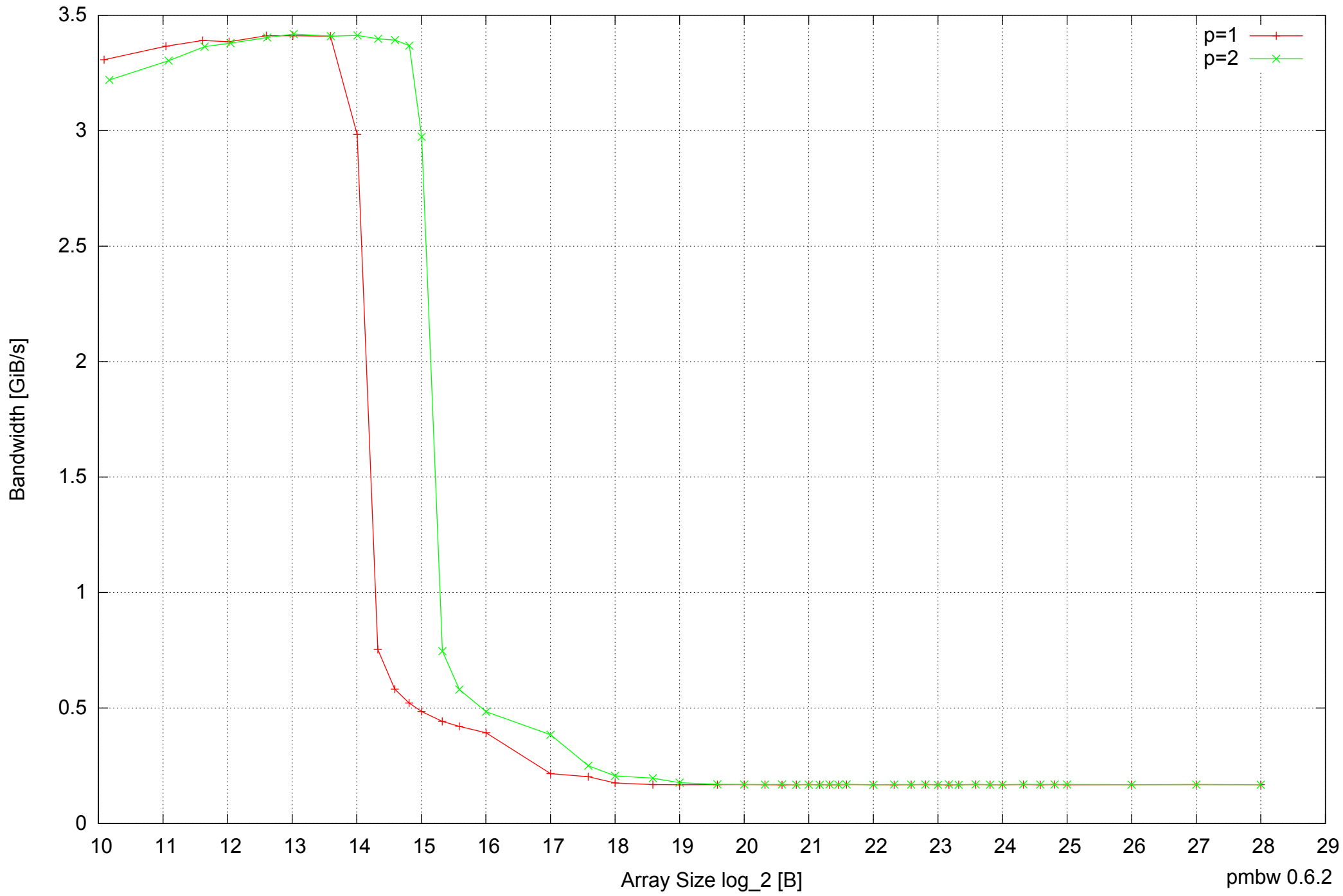
Raspberry Pi Model B: ARM1176JZF-S 512MB - Parallel Memory Bandwidth - ScanRead32PtrMultiLoop
