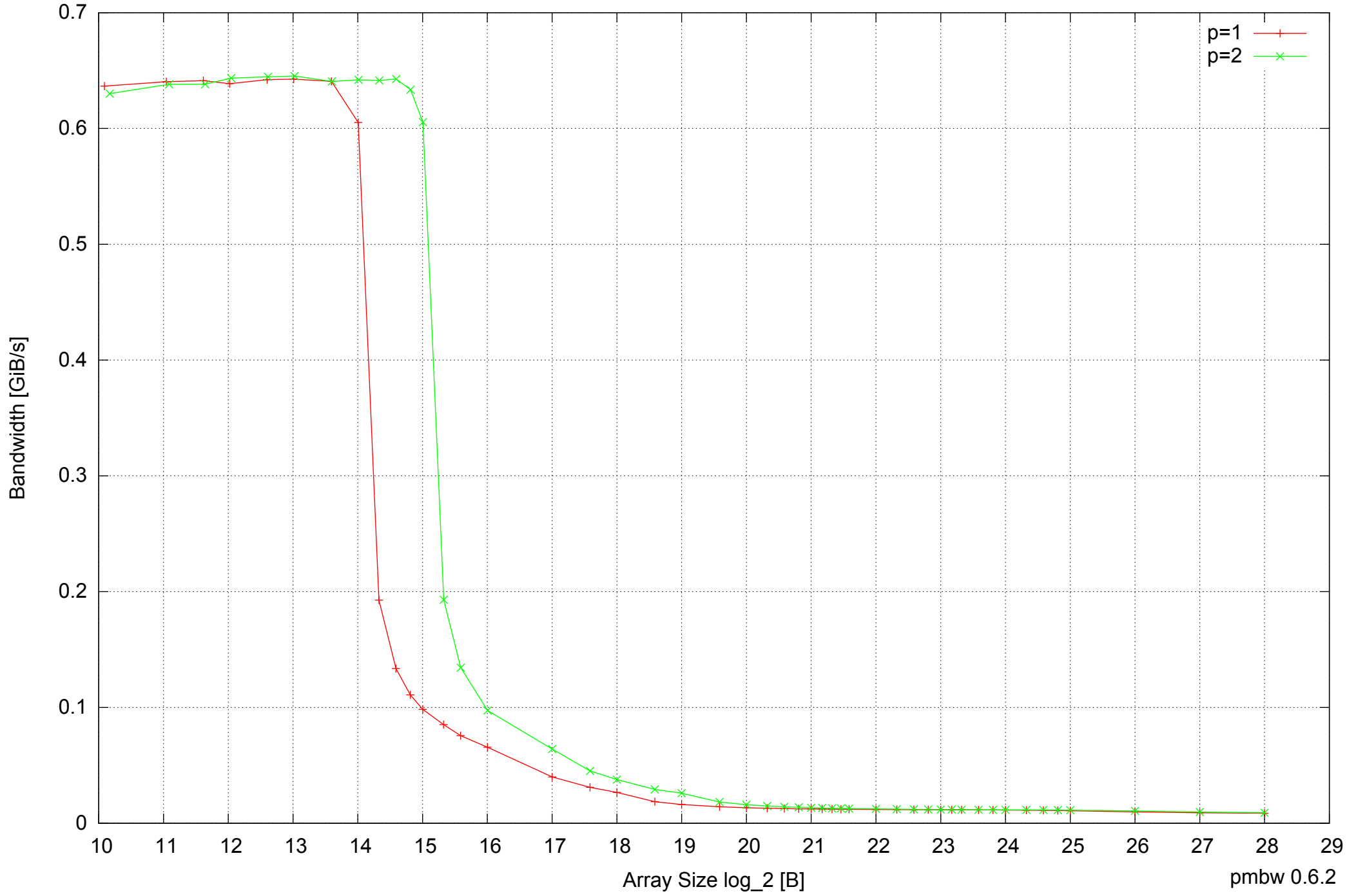
Raspberry Pi Model B: ARM1176JZF-S 512MB - Parallel Memory Bandwidth - PermRead32SimpleLoop
