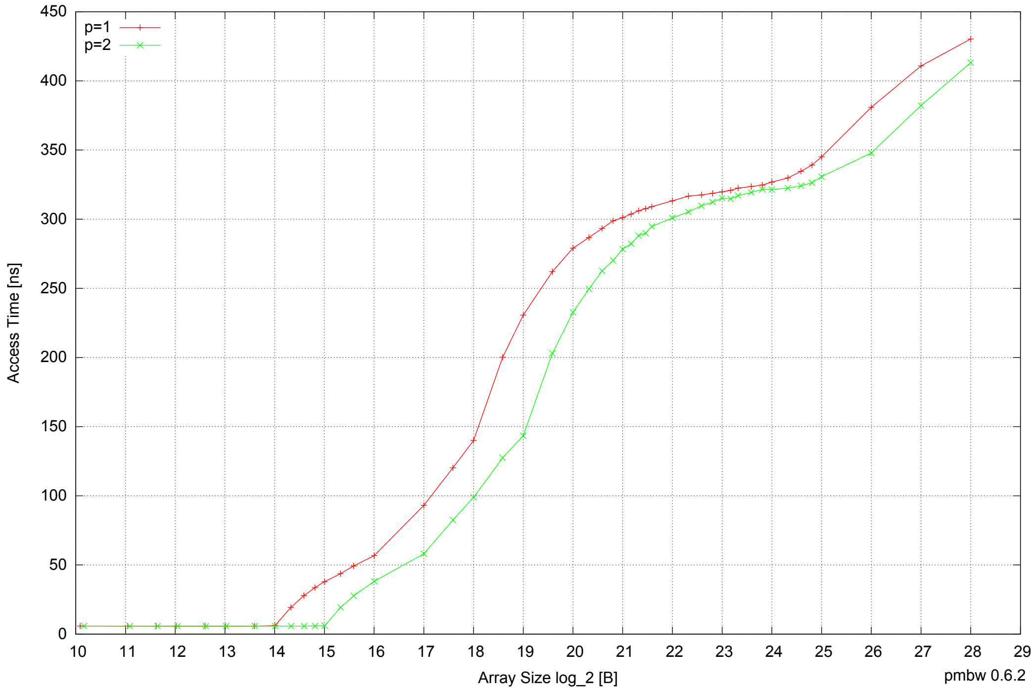
Raspberry Pi Model B: ARM1176JZF-S 512MB - Parallel Memory Access Time - PermRead32SimpleLoop
