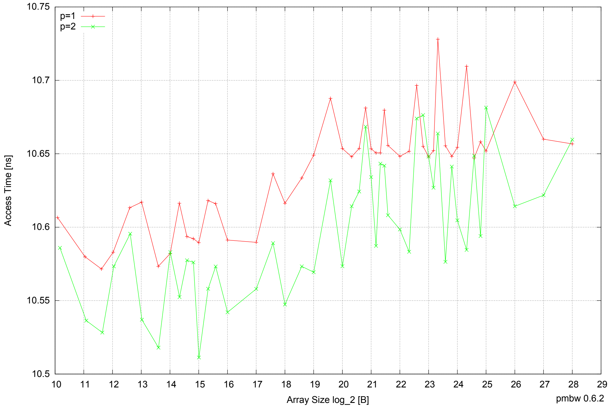
Raspberry Pi Model B: ARM1176JZF-S 512MB - Parallel Memory Access Time - ScanWrite32PtrUnrollLoop
