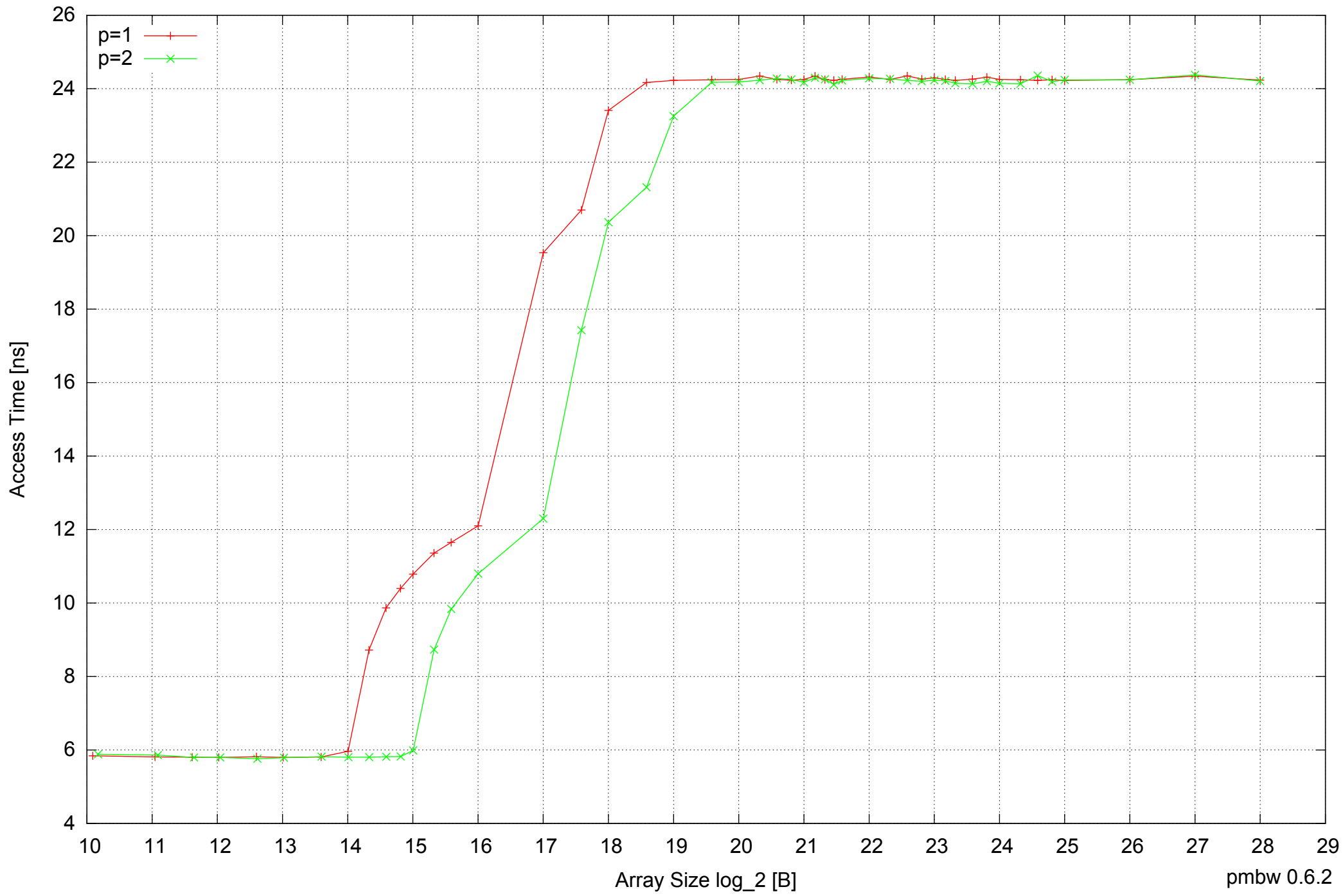
Raspberry Pi Model B: ARM1176JZF-S 512MB - Parallel Memory Access Time - ScanRead32IndexSimpleLoop
