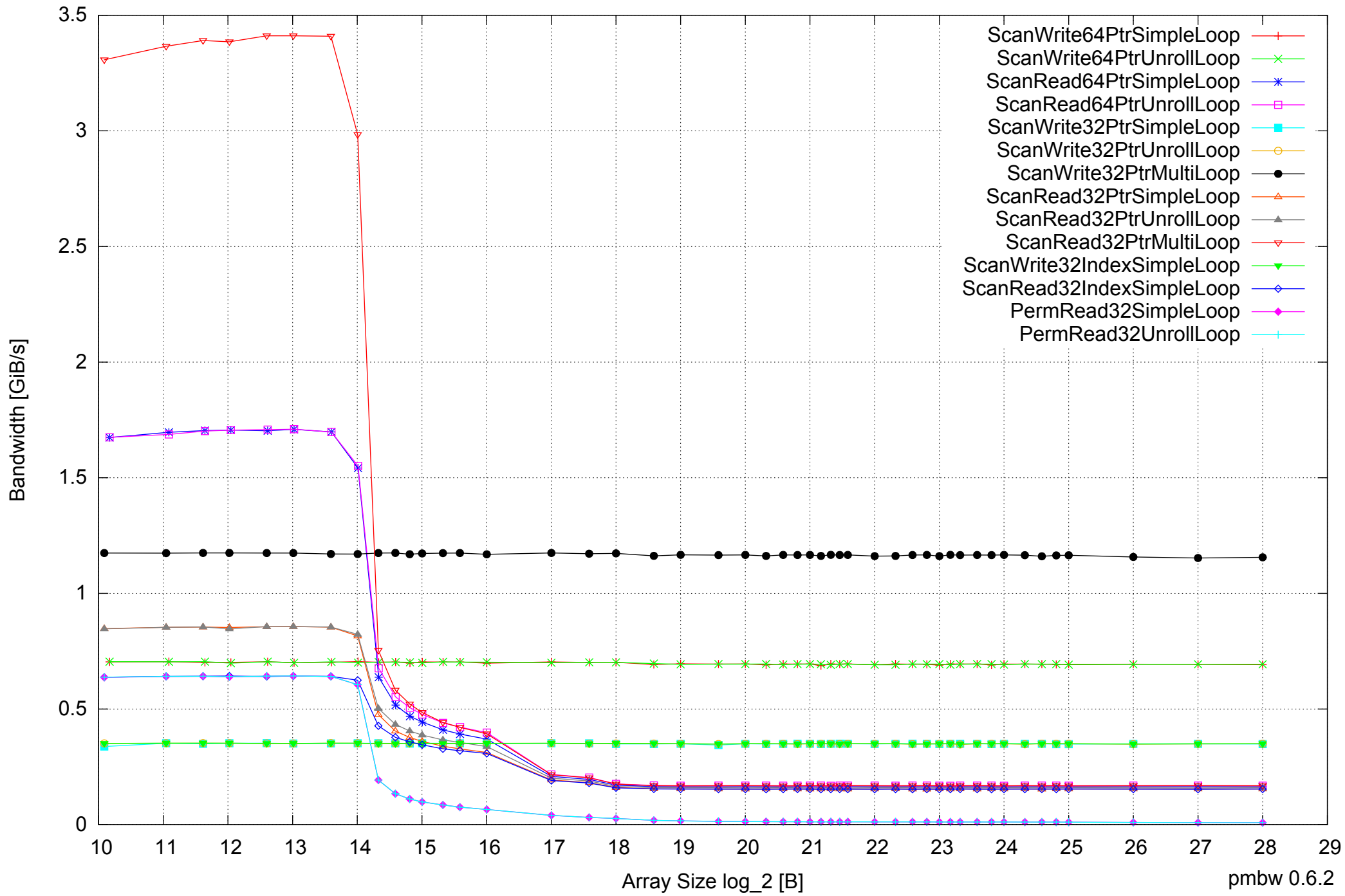
Raspberry Pi Model B: ARM1176JZF-S 512MB - One Thread Memory Bandwidth
