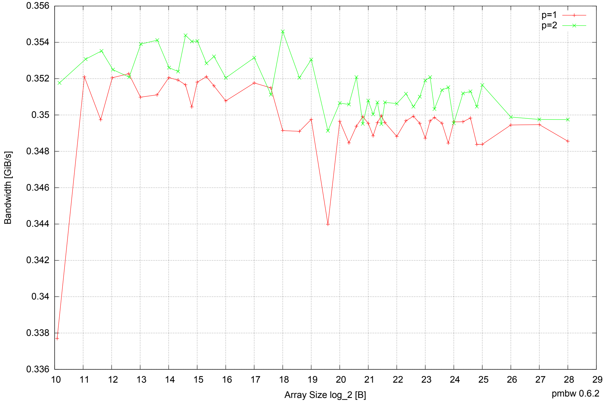
Raspberry Pi Model B: ARM1176JZF-S 512MB - Parallel Memory Bandwidth - ScanWrite32PtrSimpleLoop
