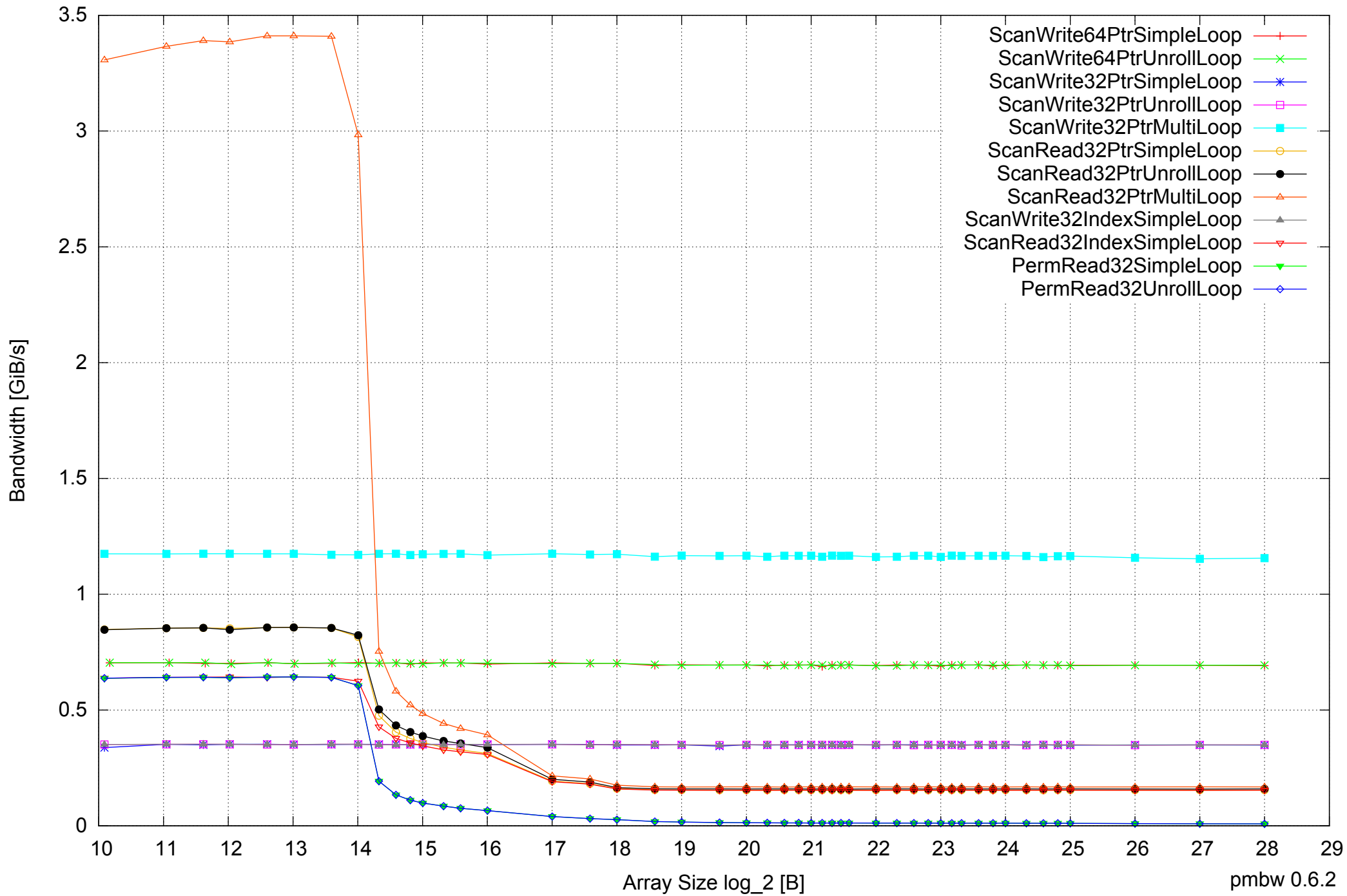
Raspberry Pi Model B: ARM1176JZF-S 512MB - One Thread Memory Bandwidth (only 64-bit Reads)
