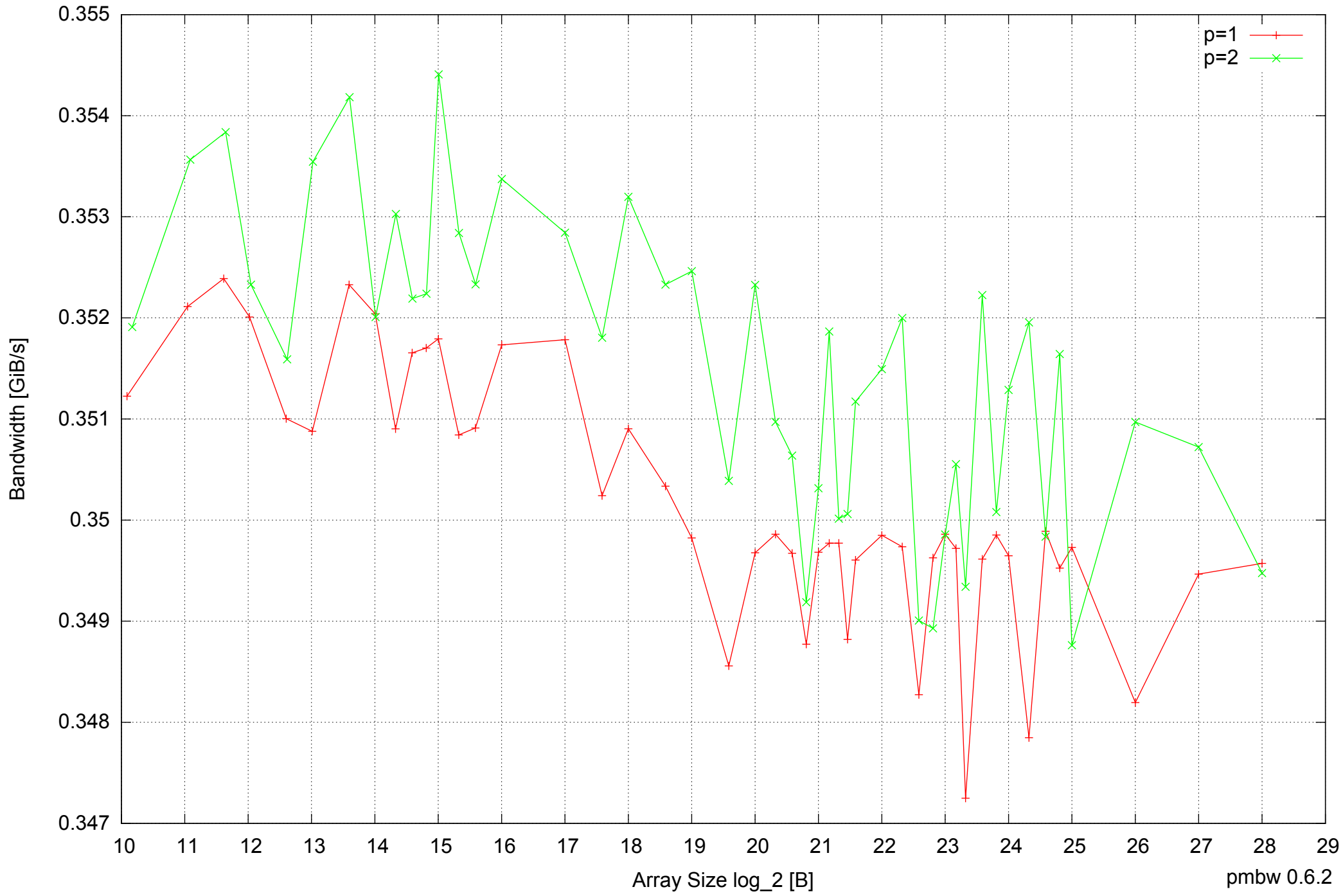
Raspberry Pi Model B: ARM1176JZF-S 512MB - Parallel Memory Bandwidth - ScanWrite32PtrUnrollLoop
