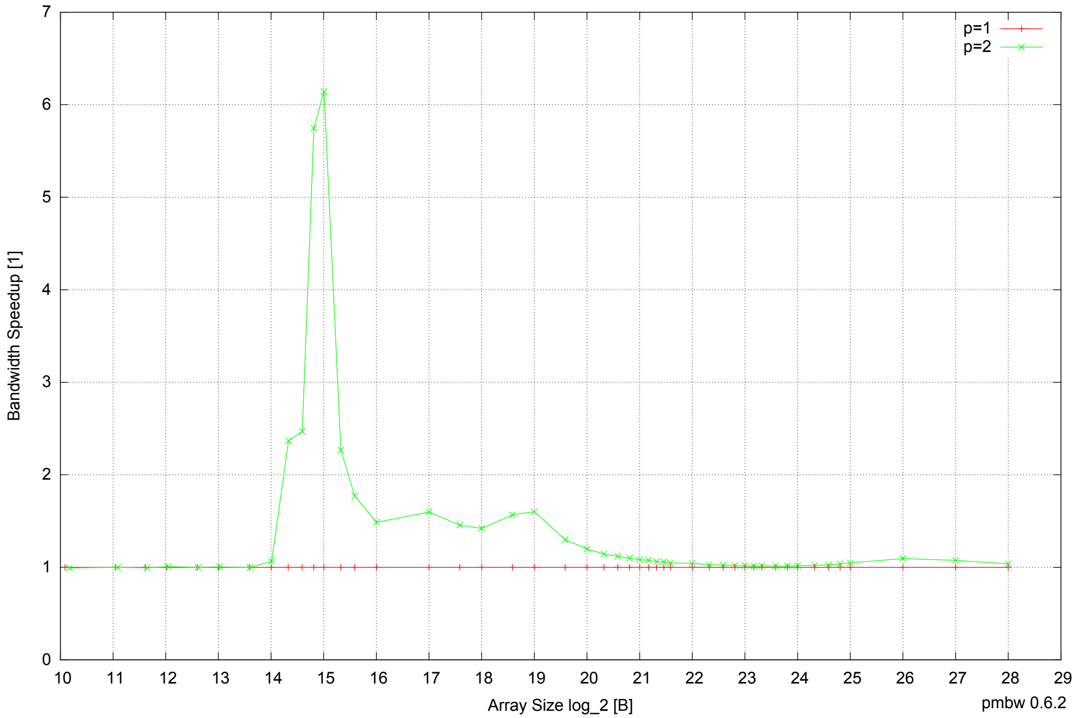
Raspberry Pi Model B: ARM1176JZF-S 512MB - Speedup of Parallel Memory Bandwidth - PermRead32UnrollLoop
