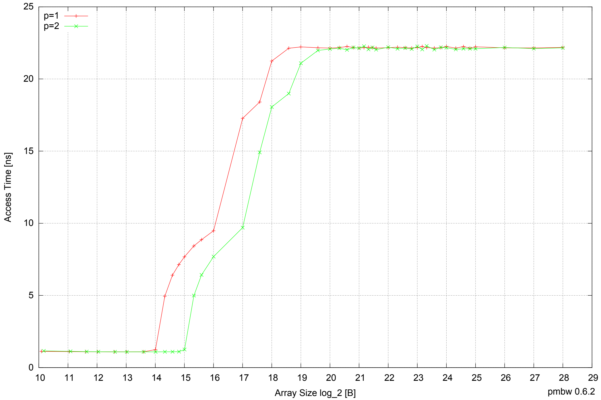
Raspberry Pi Model B: ARM1176JZF-S 512MB - Parallel Memory Access Time - ScanRead32PtrMultiLoop
