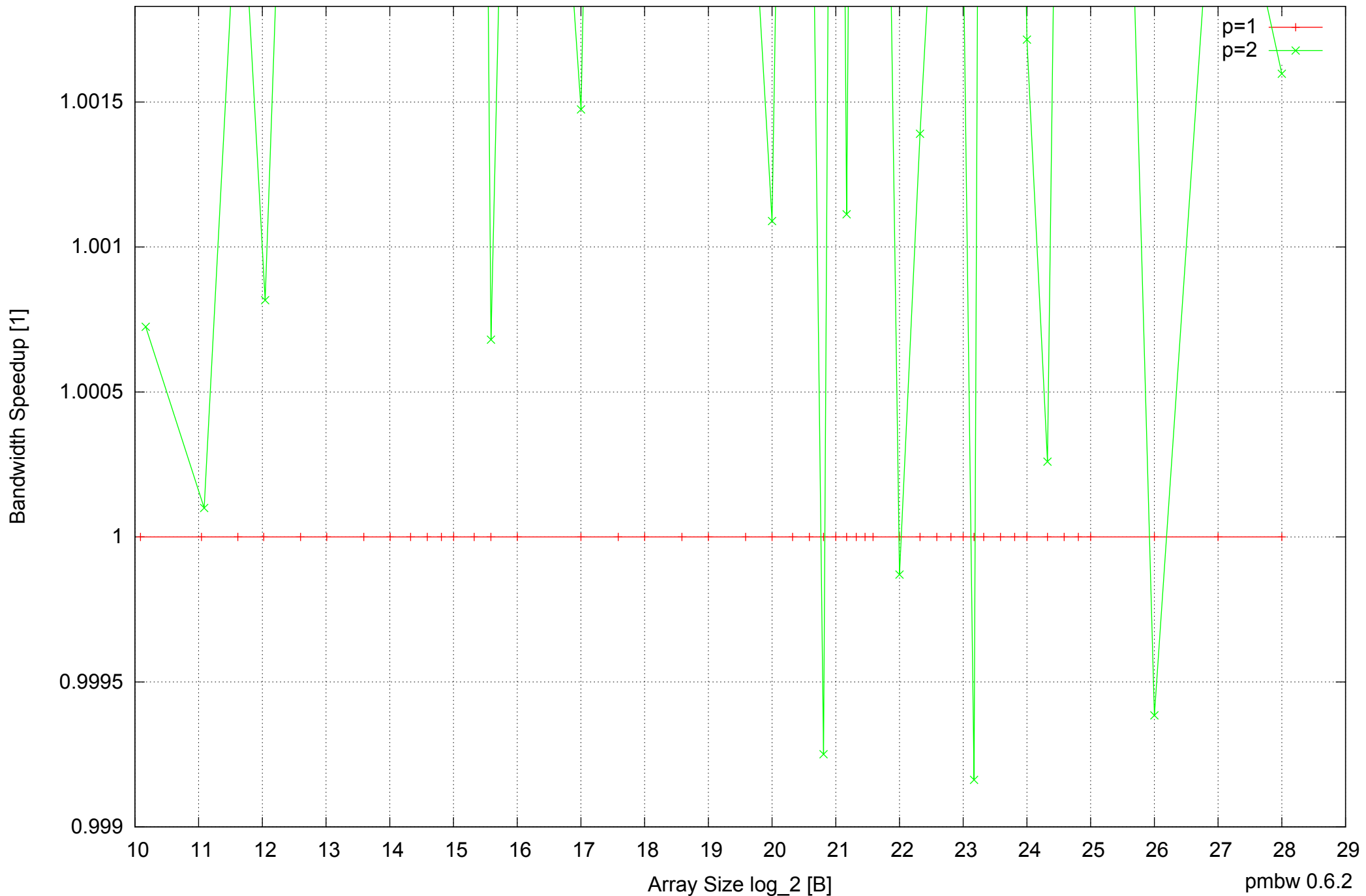
Raspberry Pi Model B: ARM1176JZF-S 512MB - Speedup of Parallel Memory Bandwidth (enlarged) - ScanWrite32IndexSimpleLoop
