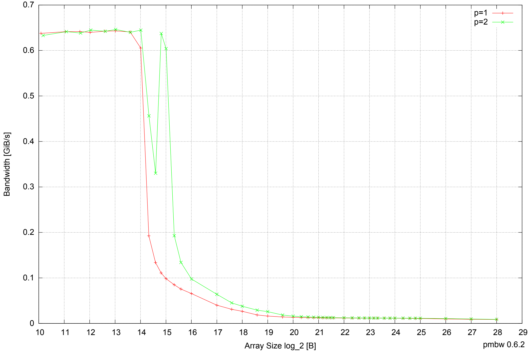
Raspberry Pi Model B: ARM1176JZF-S 512MB - Parallel Memory Bandwidth - PermRead32UnrollLoop
