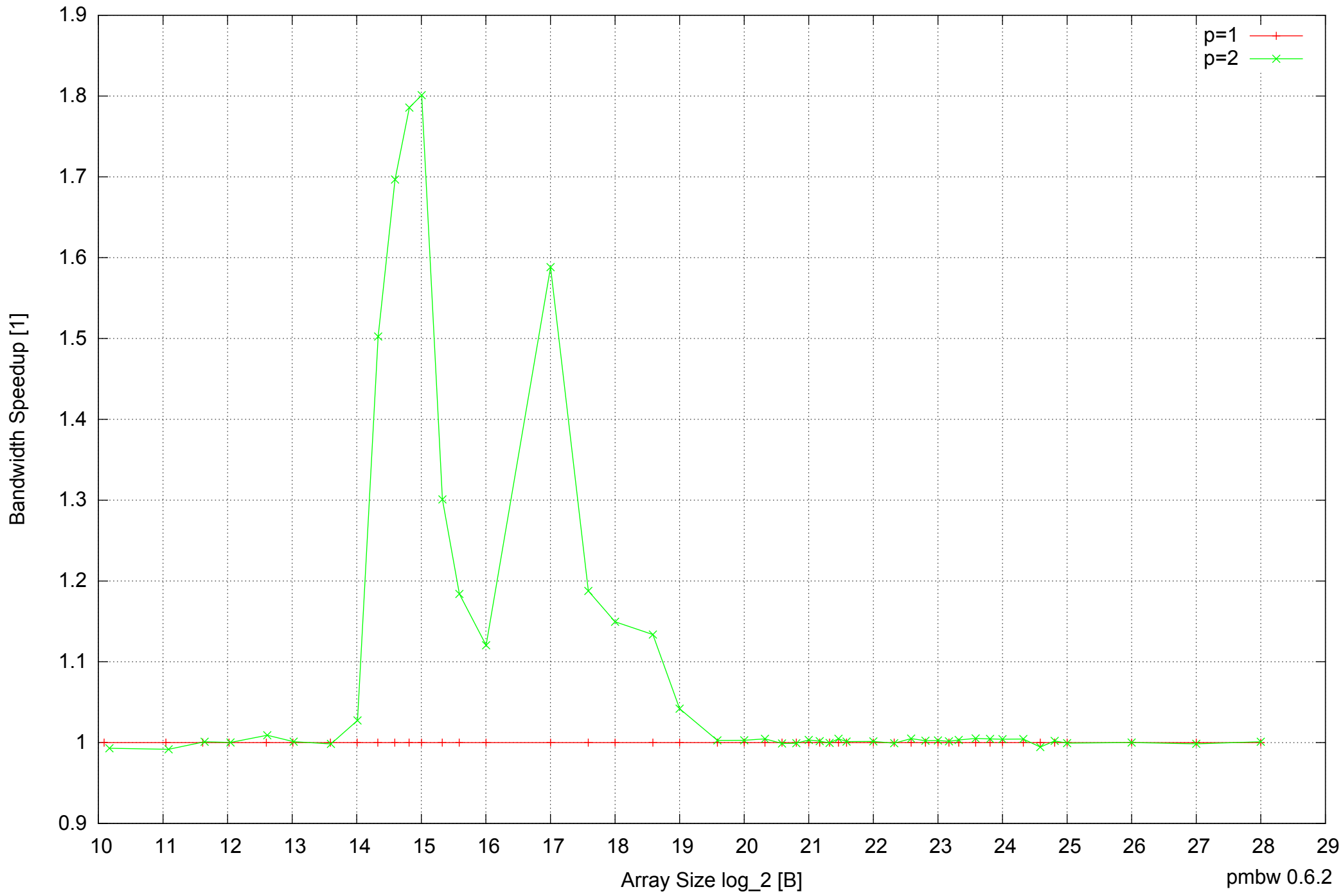
Raspberry Pi Model B: ARM1176JZF-S 512MB - Speedup of Parallel Memory Bandwidth - ScanRead32IndexSimpleLoop
