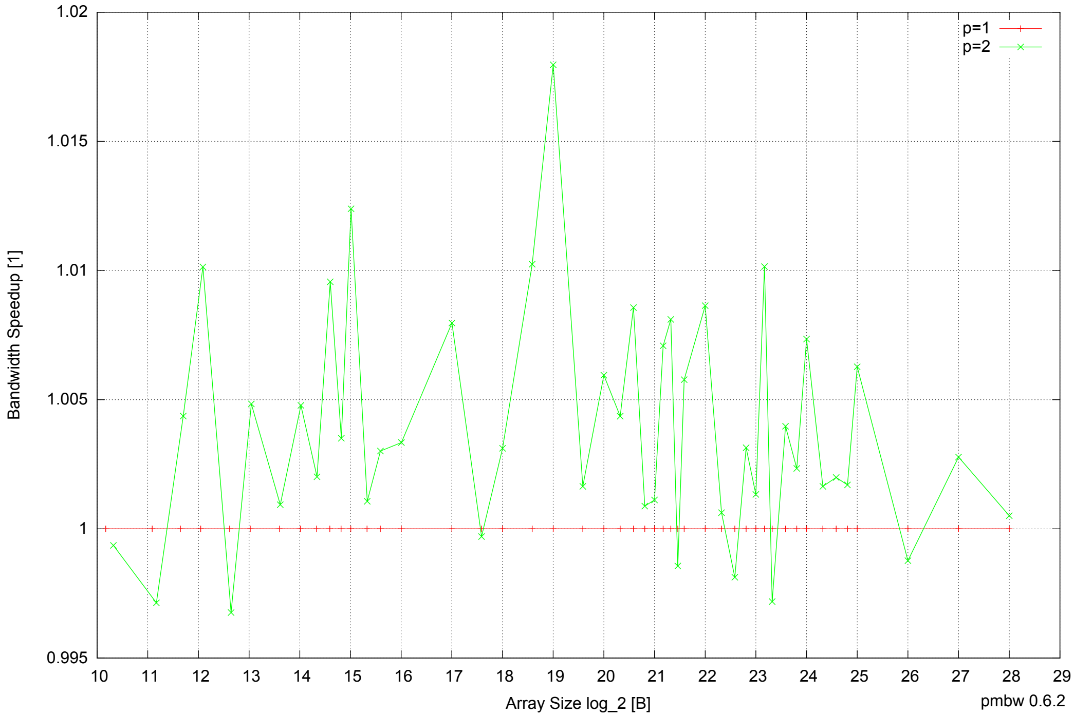
Raspberry Pi Model B: ARM1176JZF-S 512MB - Speedup of Parallel Memory Bandwidth - ScanWrite64PtrUnrollLoop
