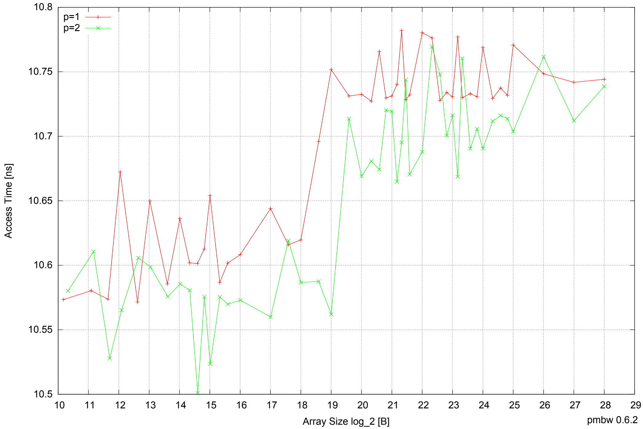
Raspberry Pi Model B: ARM1176JZF-S 512MB - Parallel Memory Access Time - ScanWrite64PtrUnrollLoop
