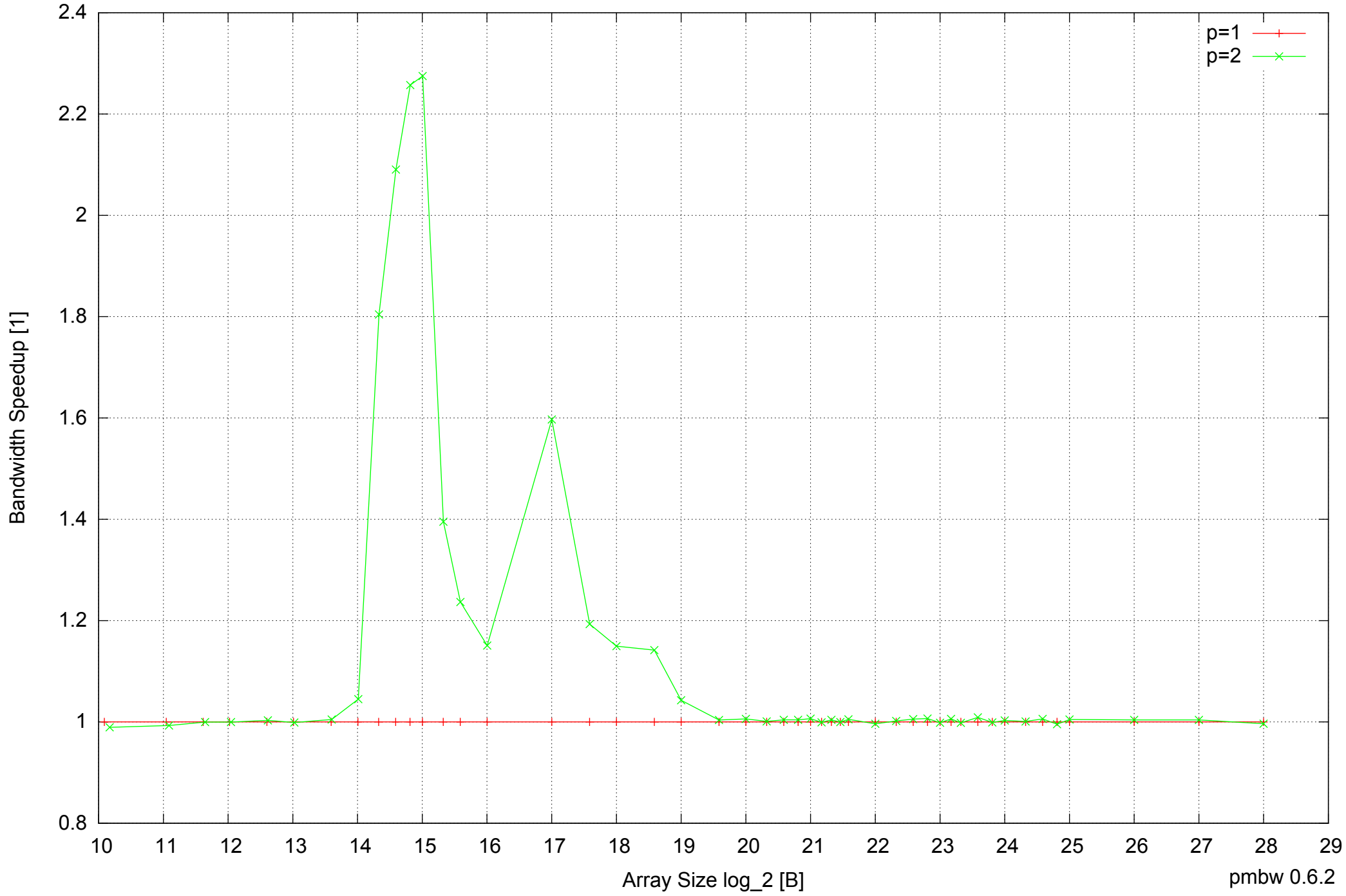
Raspberry Pi Model B: ARM1176JZF-S 512MB - Speedup of Parallel Memory Bandwidth - ScanRead32PtrSimpleLoop
