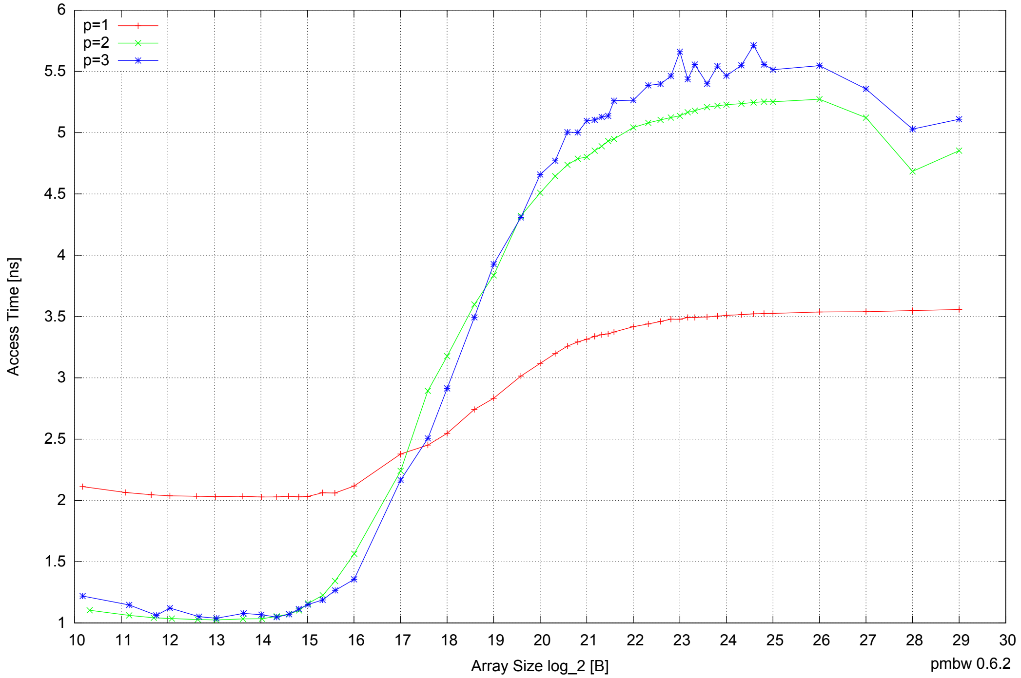
Motorola Atrix: ARM Cortex A9 1GB - Parallel Memory Access Time - ScanWrite64PtrSimpleLoop
