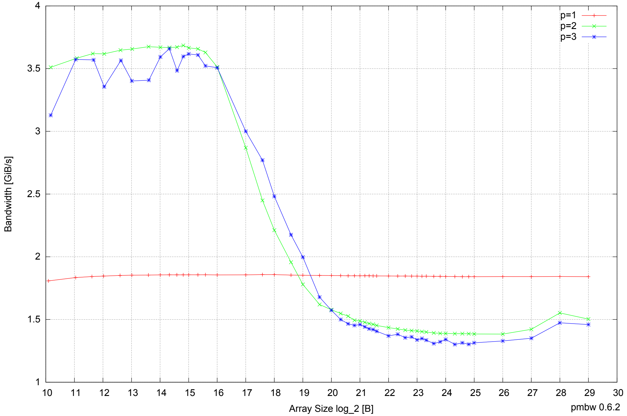
Motorola Atrix: ARM Cortex A9 1GB - Parallel Memory Bandwidth - ScanWrite32IndexSimpleLoop
