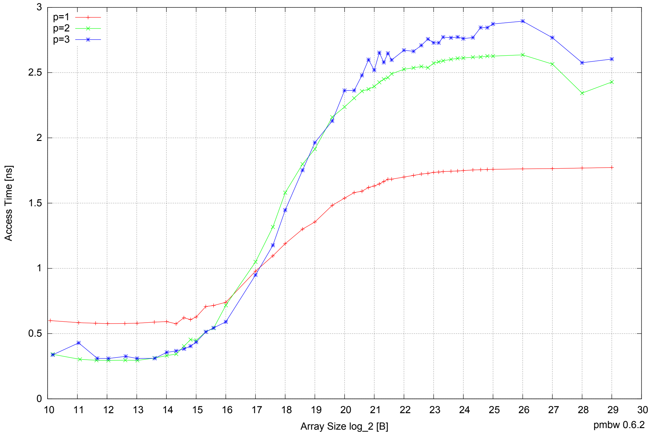
Motorola Atrix: ARM Cortex A9 1GB - Parallel Memory Access Time - ScanWrite32PtrMultiLoop
