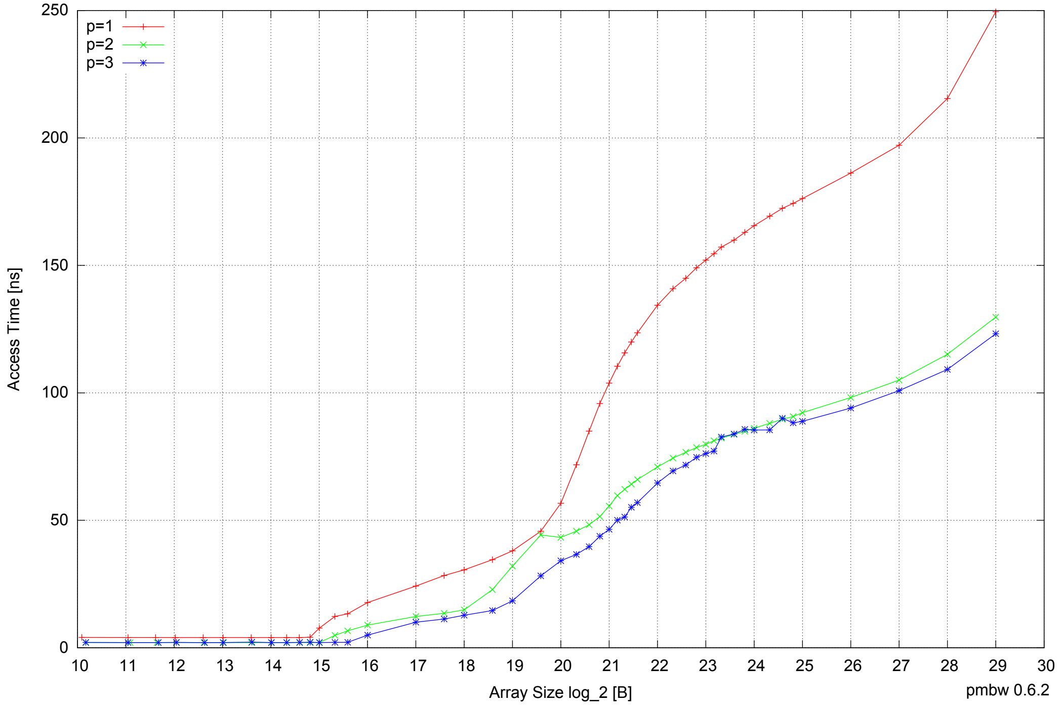
Motorola Atrix: ARM Cortex A9 1GB - Parallel Memory Access Time - PermRead32UnrollLoop
