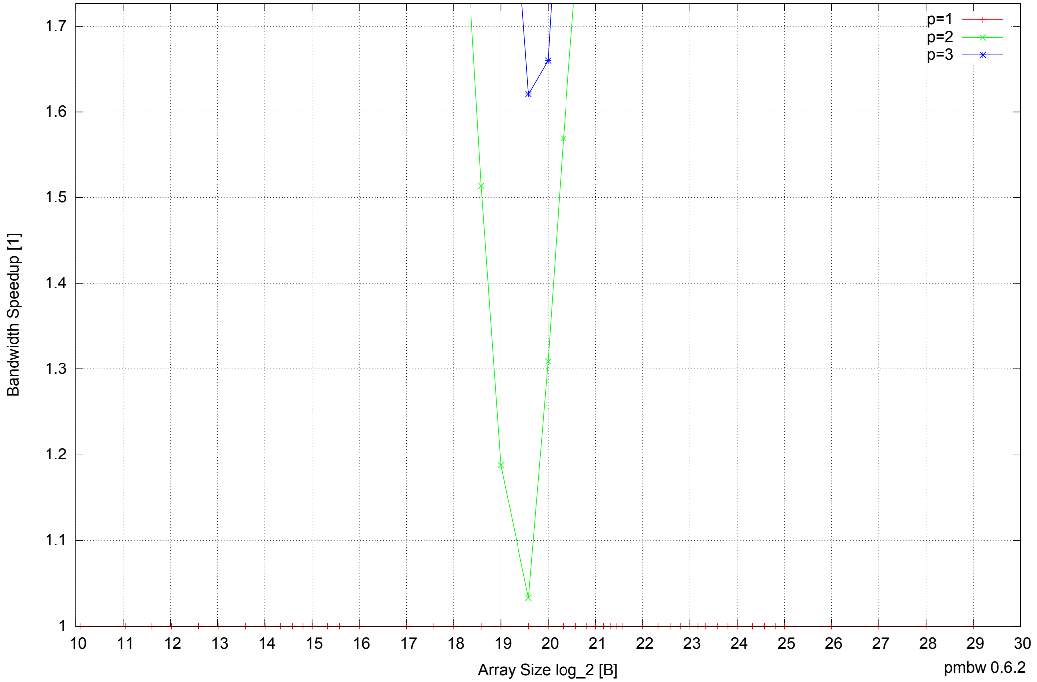
Motorola Atrix: ARM Cortex A9 1GB - Speedup of Parallel Memory Bandwidth (enlarged) - PermRead32UnrollLoop
