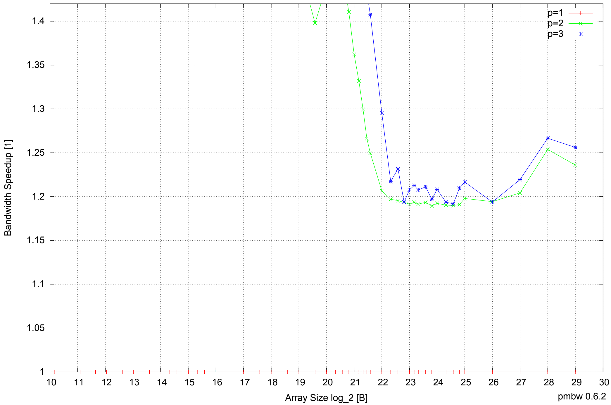
Motorola Atrix: ARM Cortex A9 1GB - Speedup of Parallel Memory Bandwidth (enlarged) - ScanRead64PtrUnrollLoop
