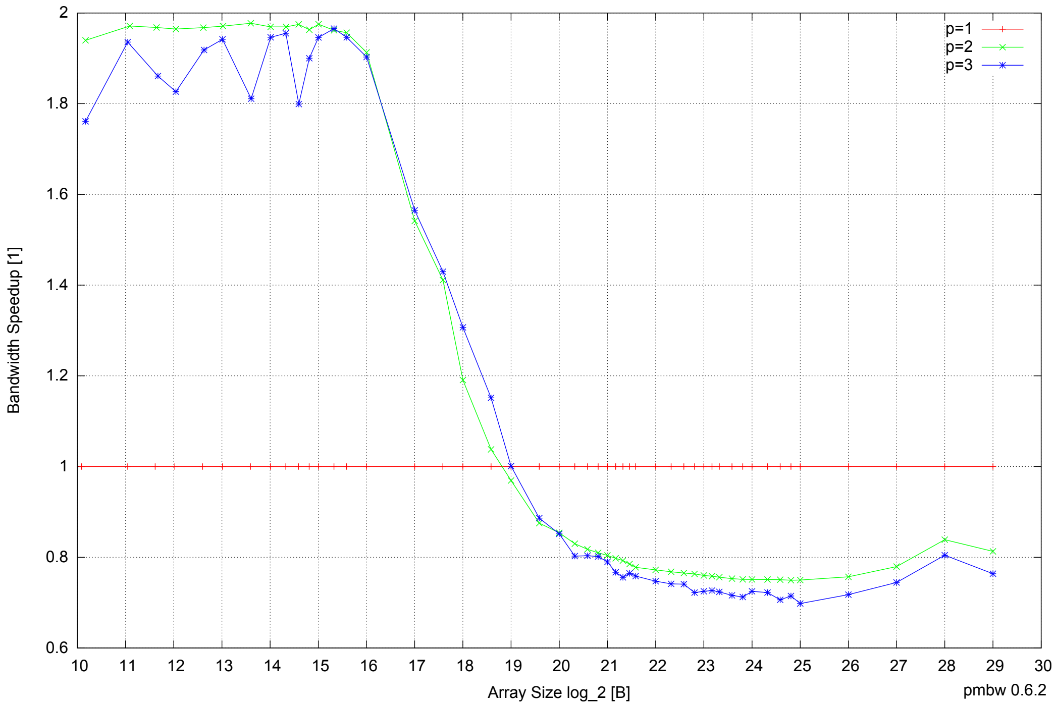
Motorola Atrix: ARM Cortex A9 1GB - Speedup of Parallel Memory Bandwidth - ScanWrite32PtrSimpleLoop
