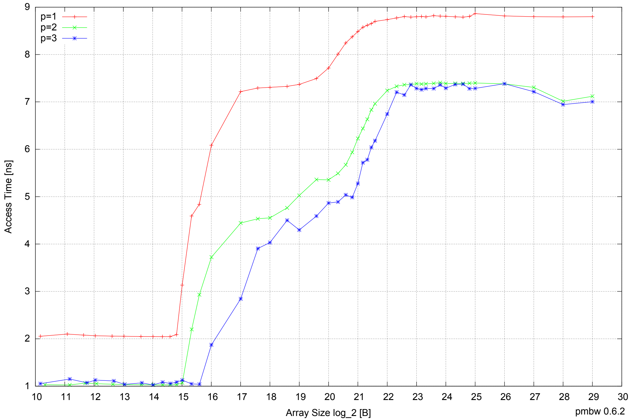
Motorola Atrix: ARM Cortex A9 1GB - Parallel Memory Access Time - ScanRead64PtrUnrollLoop
