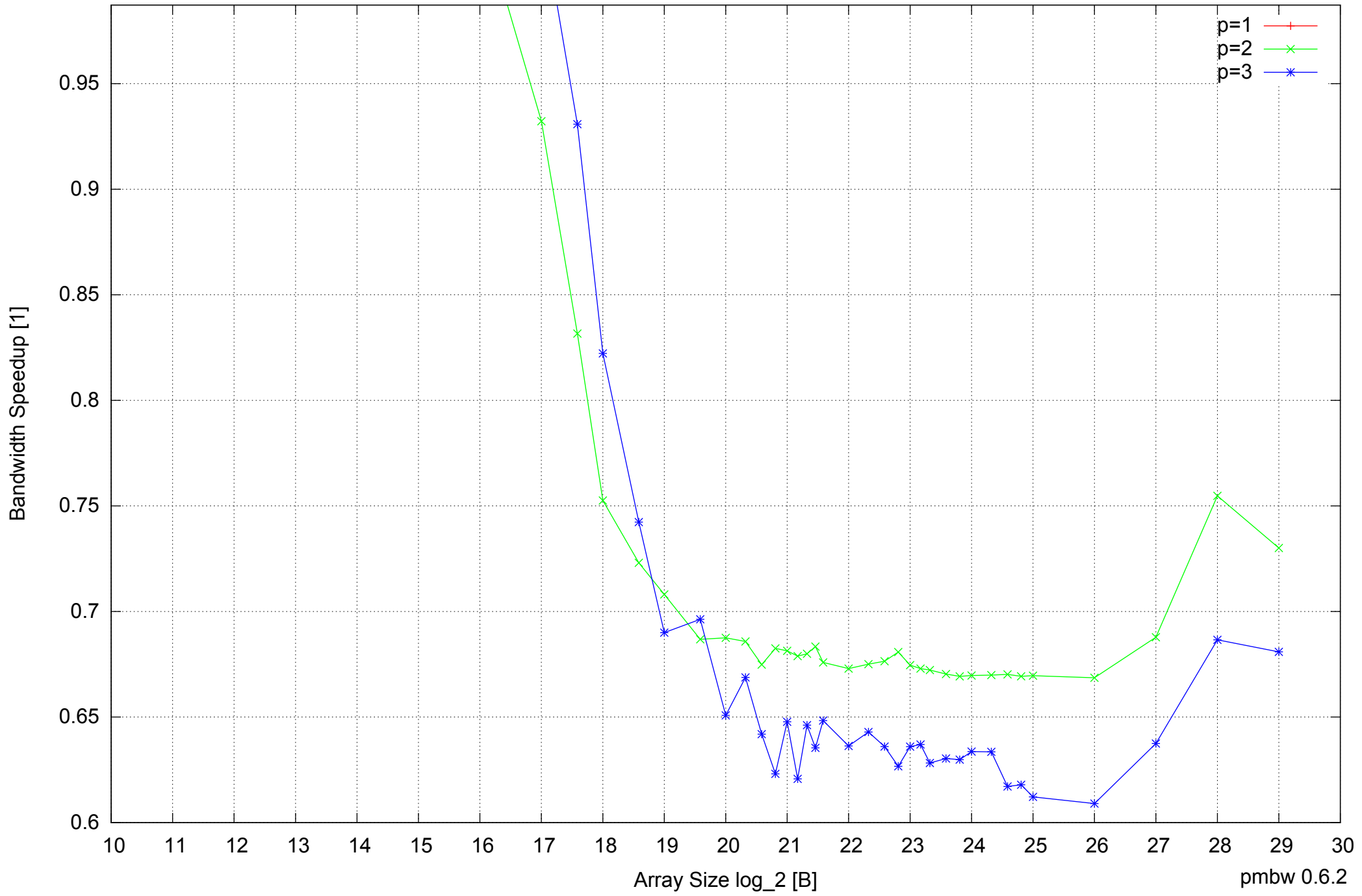
Motorola Atrix: ARM Cortex A9 1GB - Speedup of Parallel Memory Bandwidth (enlarged) - ScanWrite32PtrMultiLoop
