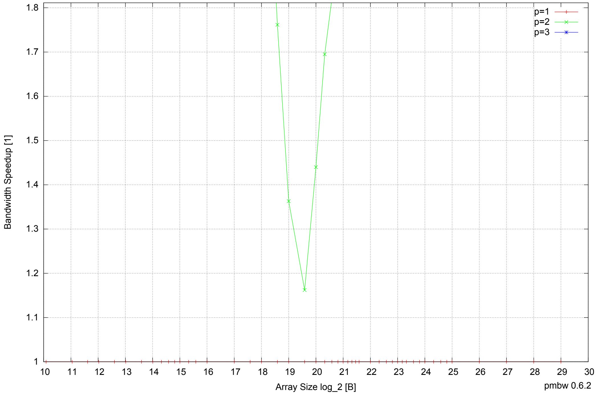
Motorola Atrix: ARM Cortex A9 1GB - Speedup of Parallel Memory Bandwidth (enlarged) - PermRead32SimpleLoop
