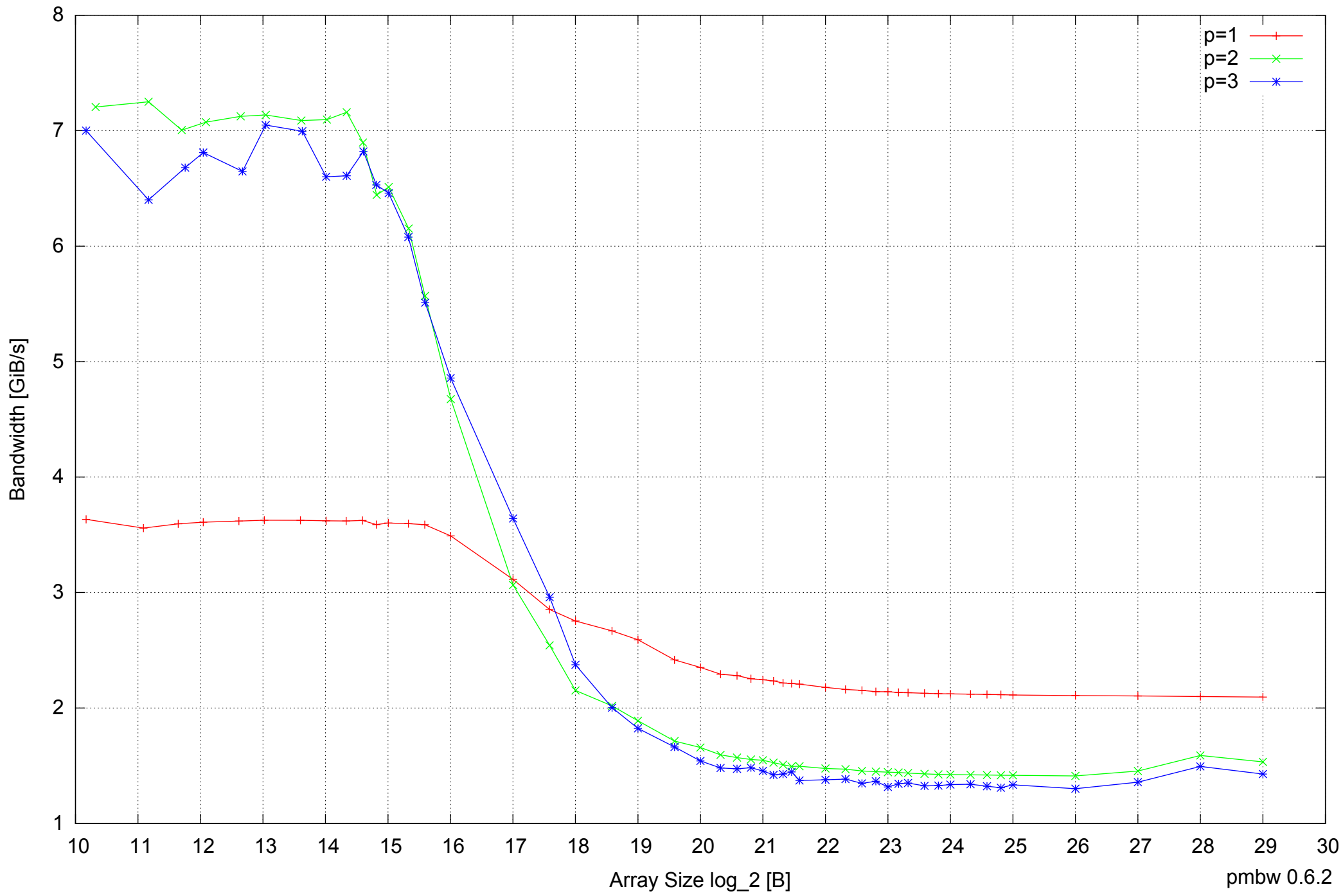
Motorola Atrix: ARM Cortex A9 1GB - Parallel Memory Bandwidth - ScanWrite64PtrUnrollLoop
