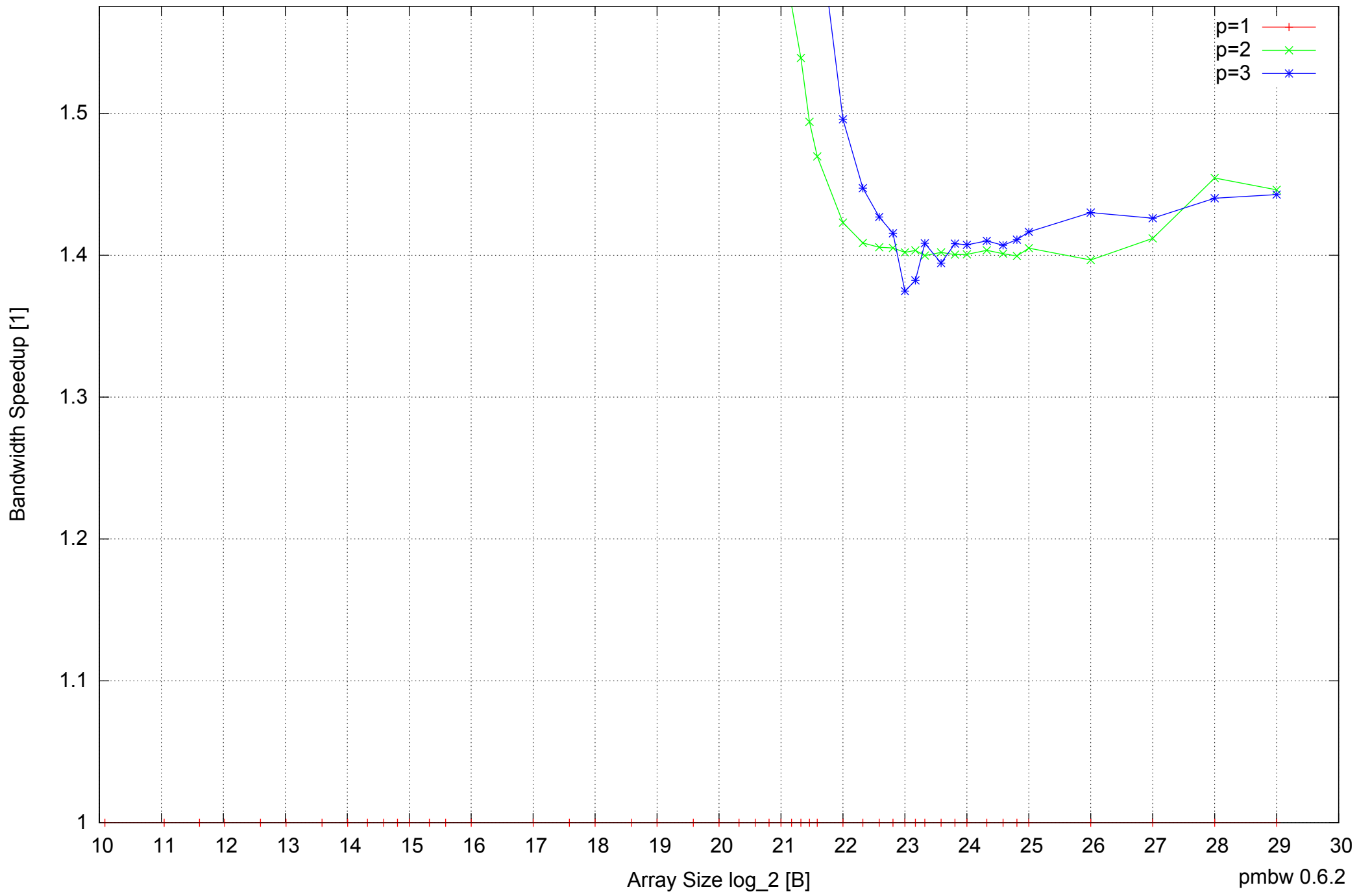
Motorola Atrix: ARM Cortex A9 1GB - Speedup of Parallel Memory Bandwidth (enlarged) - ScanRead32PtrUnrollLoop
