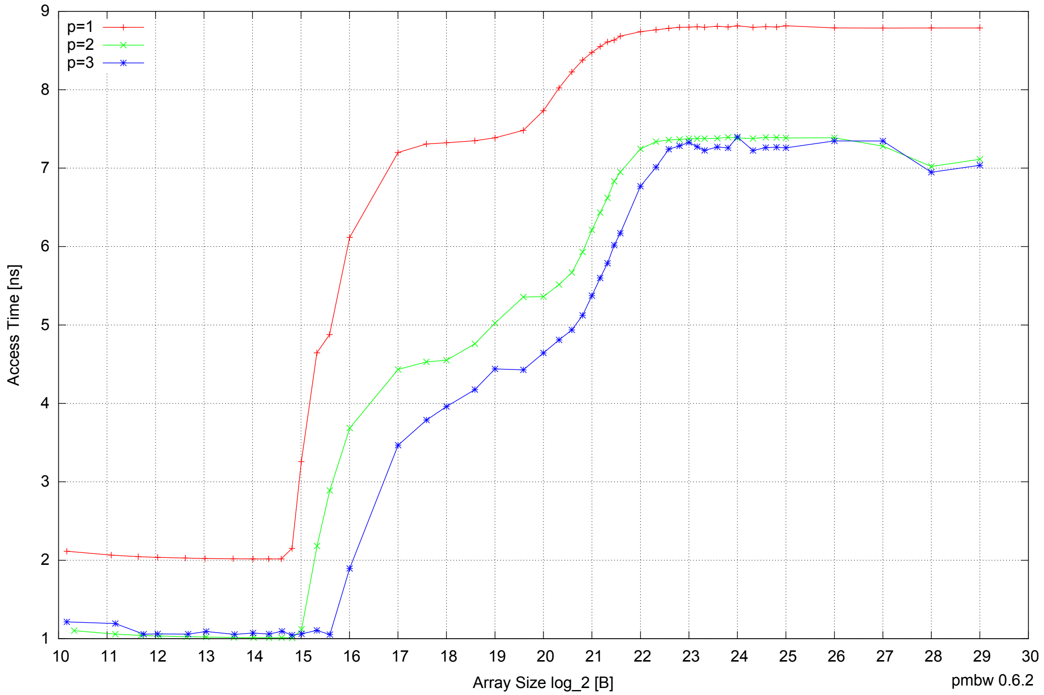
Motorola Atrix: ARM Cortex A9 1GB - Parallel Memory Access Time - ScanRead64PtrSimpleLoop
