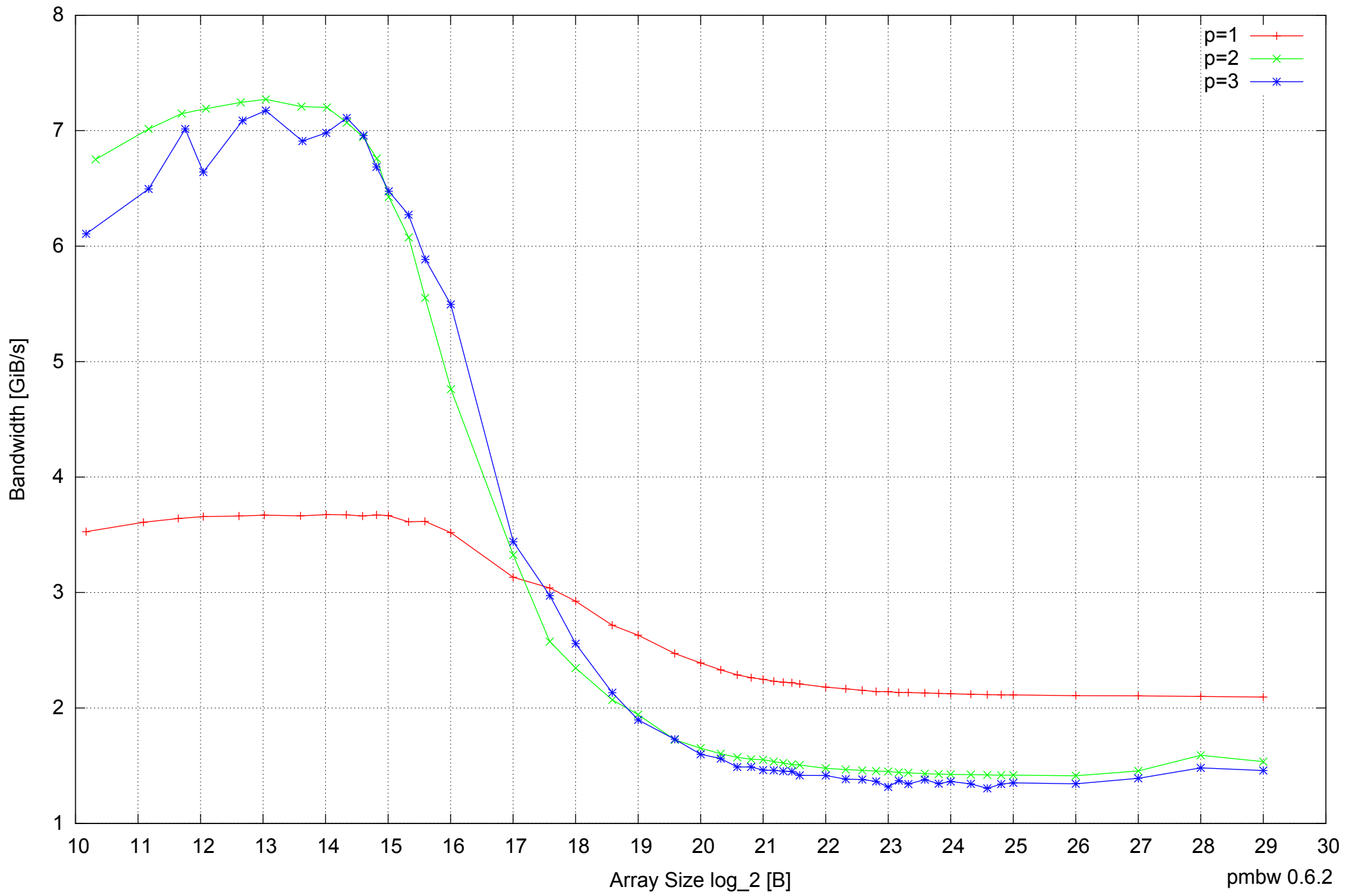
Motorola Atrix: ARM Cortex A9 1GB - Parallel Memory Bandwidth - ScanWrite64PtrSimpleLoop
