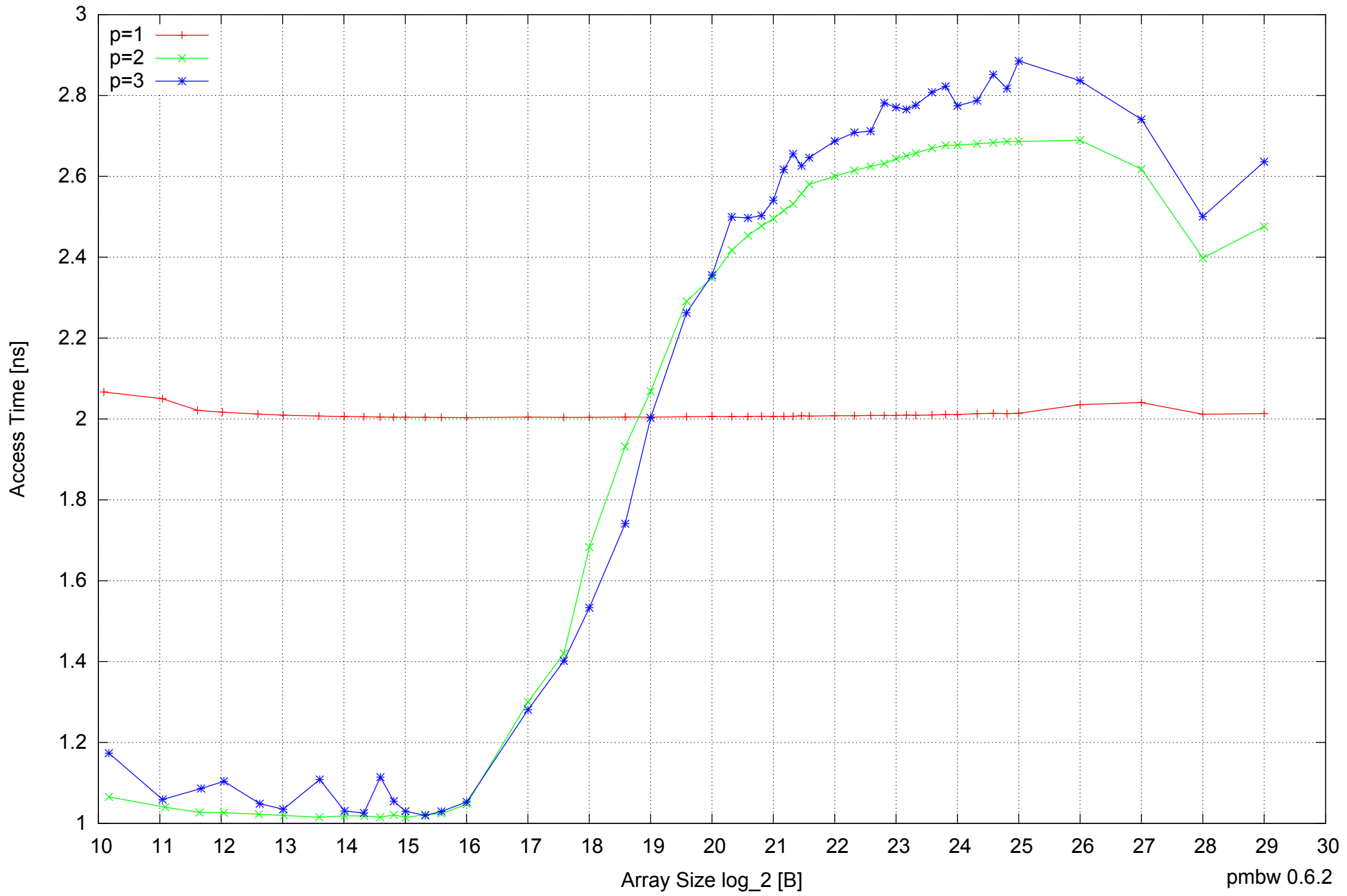
Motorola Atrix: ARM Cortex A9 1GB - Parallel Memory Access Time - ScanWrite32PtrSimpleLoop
