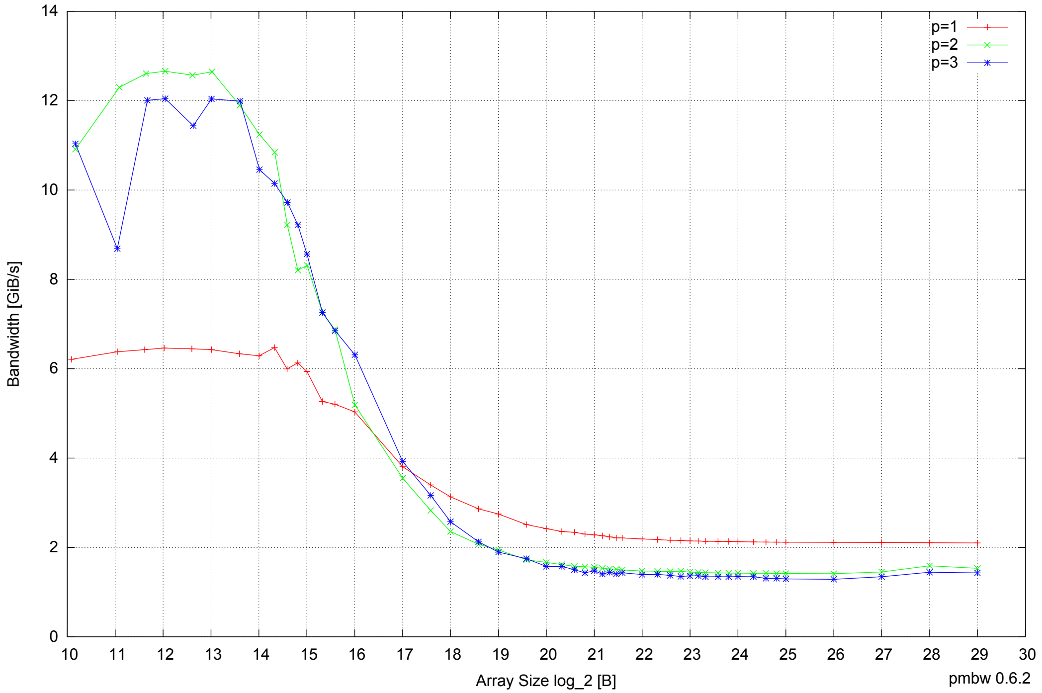
Motorola Atrix: ARM Cortex A9 1GB - Parallel Memory Bandwidth - ScanWrite32PtrMultiLoop
