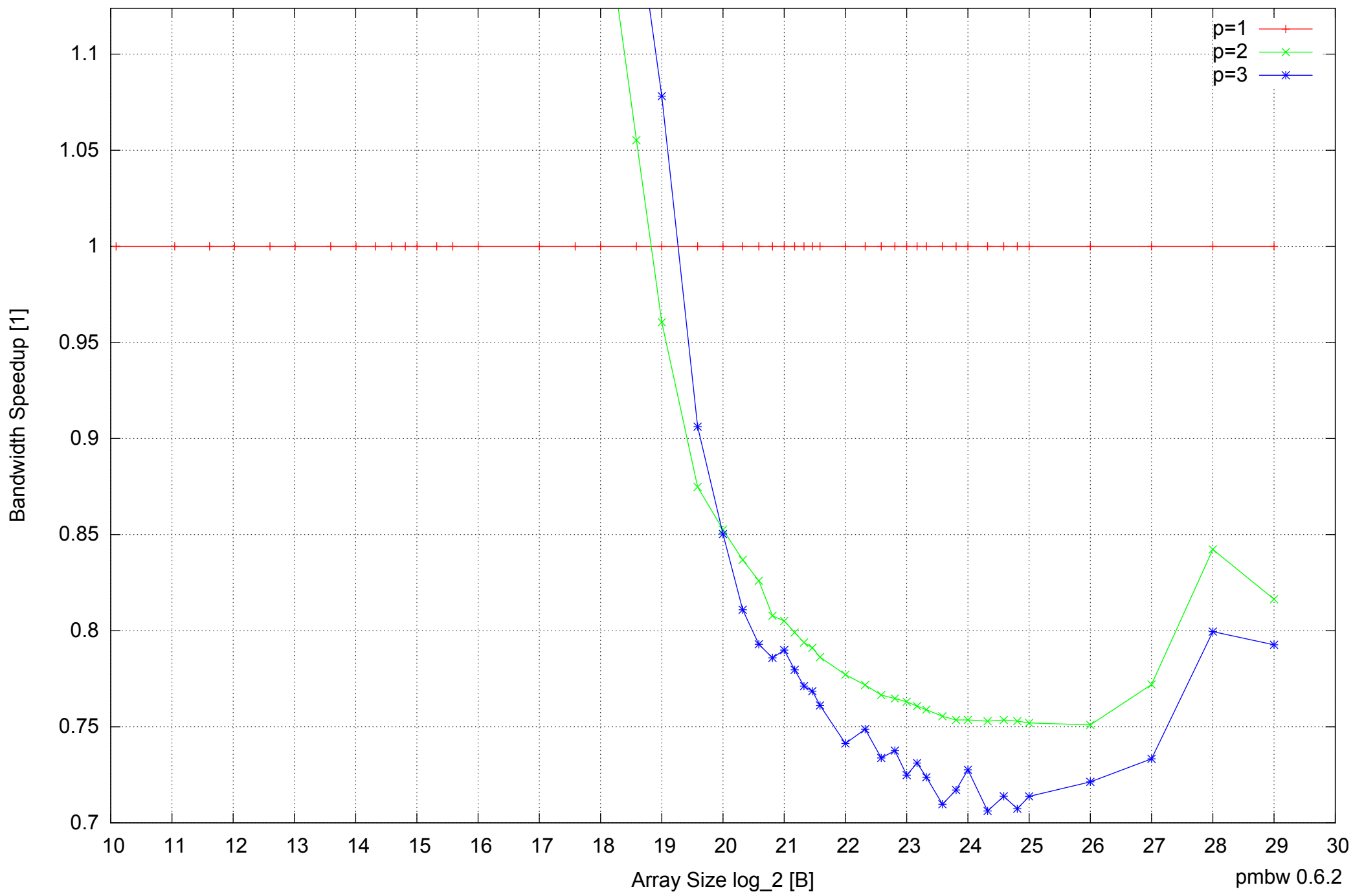
Motorola Atrix: ARM Cortex A9 1GB - Speedup of Parallel Memory Bandwidth (enlarged) - ScanWrite32IndexSimpleLoop
