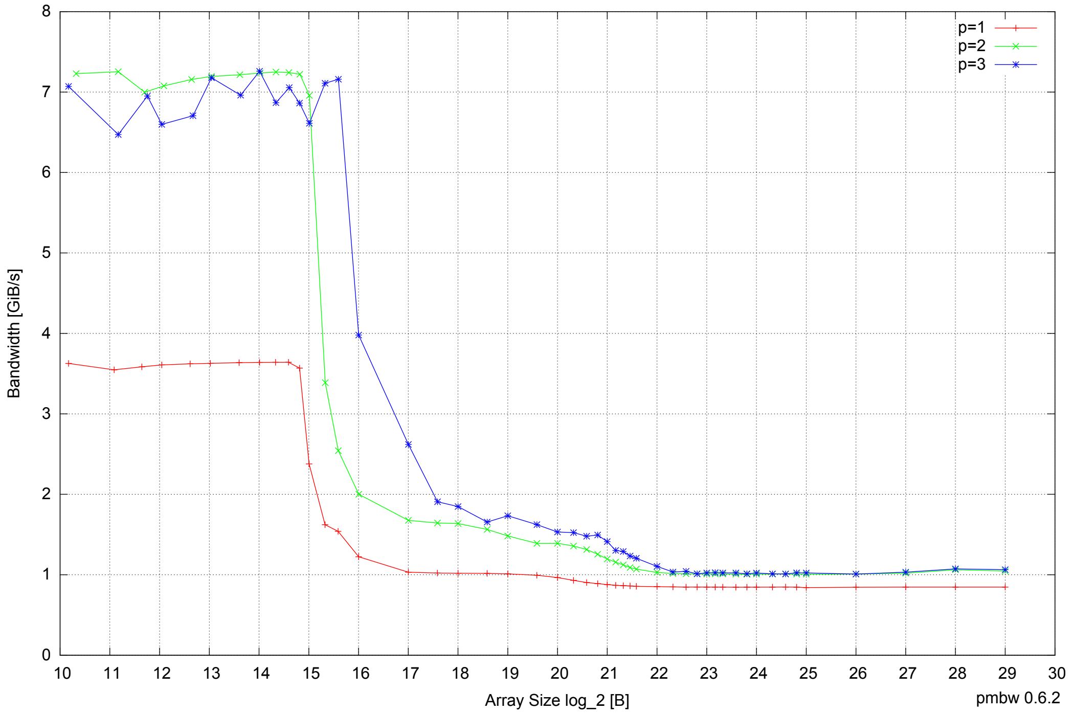
Motorola Atrix: ARM Cortex A9 1GB - Parallel Memory Bandwidth - ScanRead64PtrUnrollLoop
