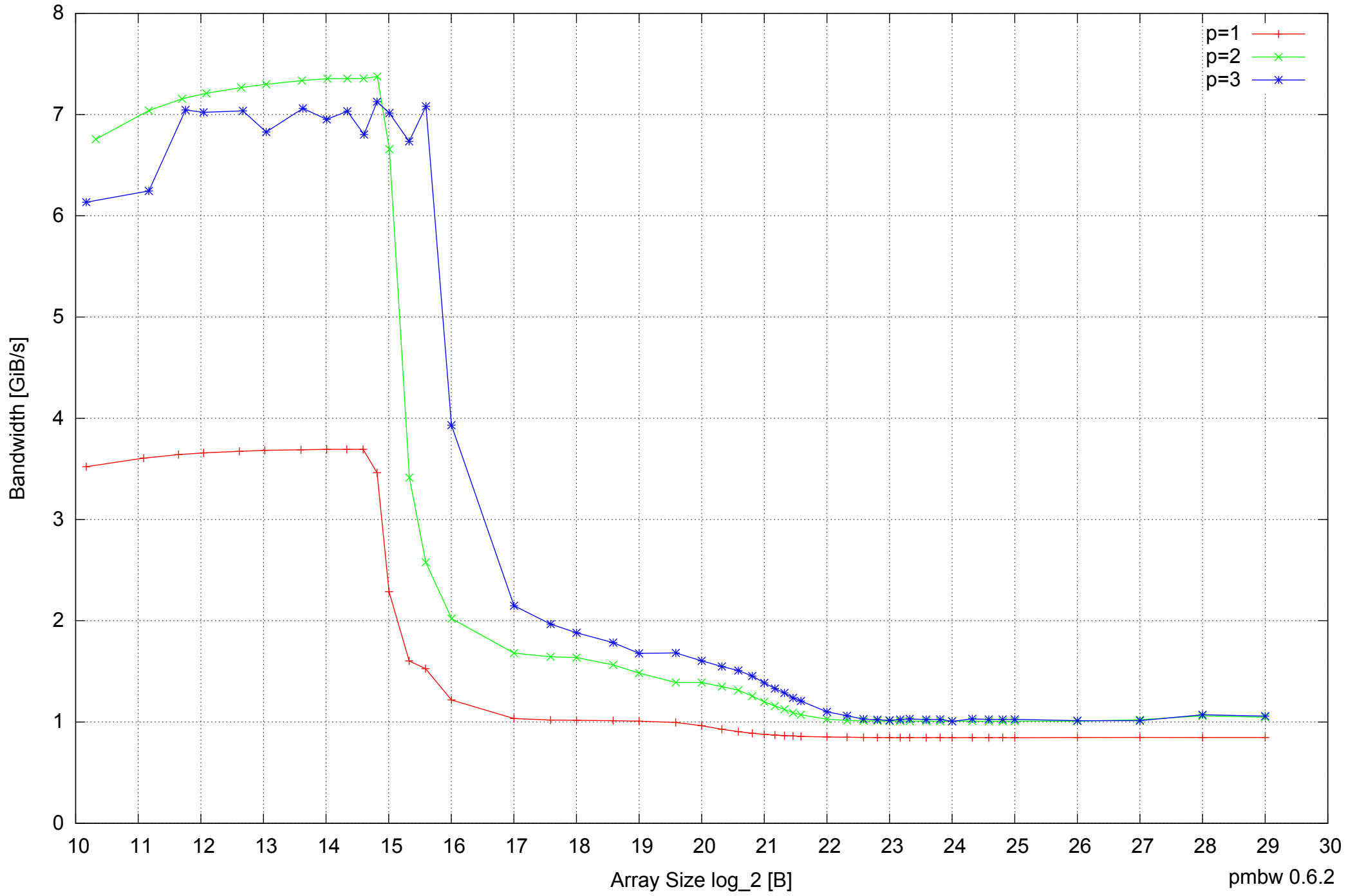
Motorola Atrix: ARM Cortex A9 1GB - Parallel Memory Bandwidth - ScanRead64PtrSimpleLoop
