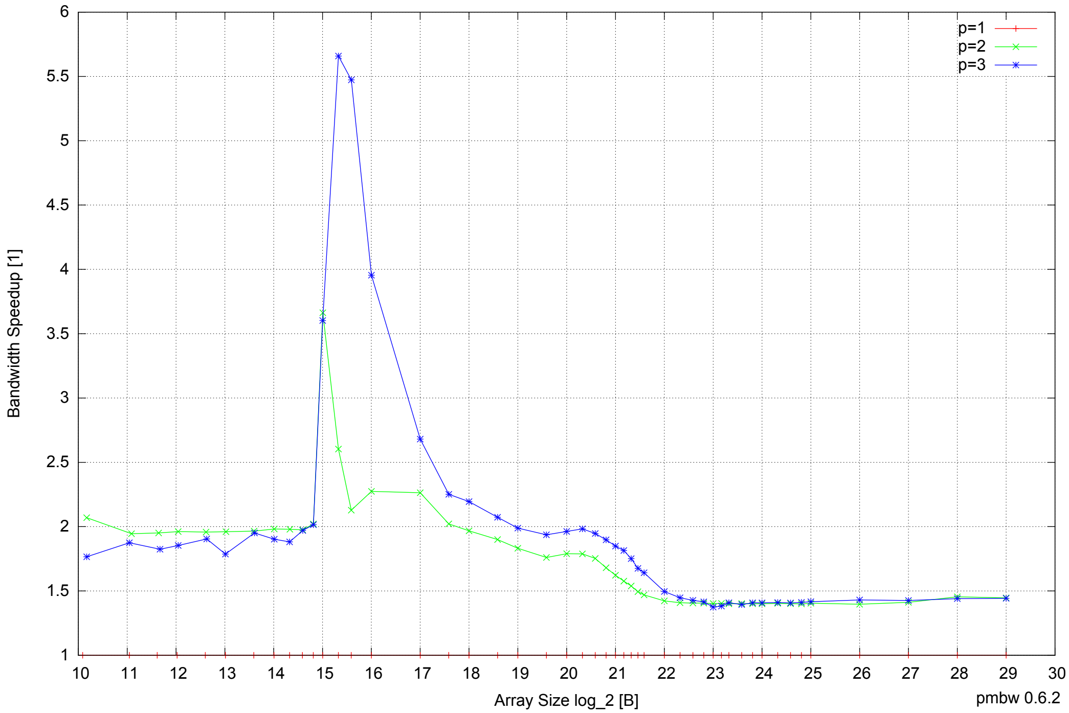
Motorola Atrix: ARM Cortex A9 1GB - Speedup of Parallel Memory Bandwidth - ScanRead32PtrUnrollLoop
