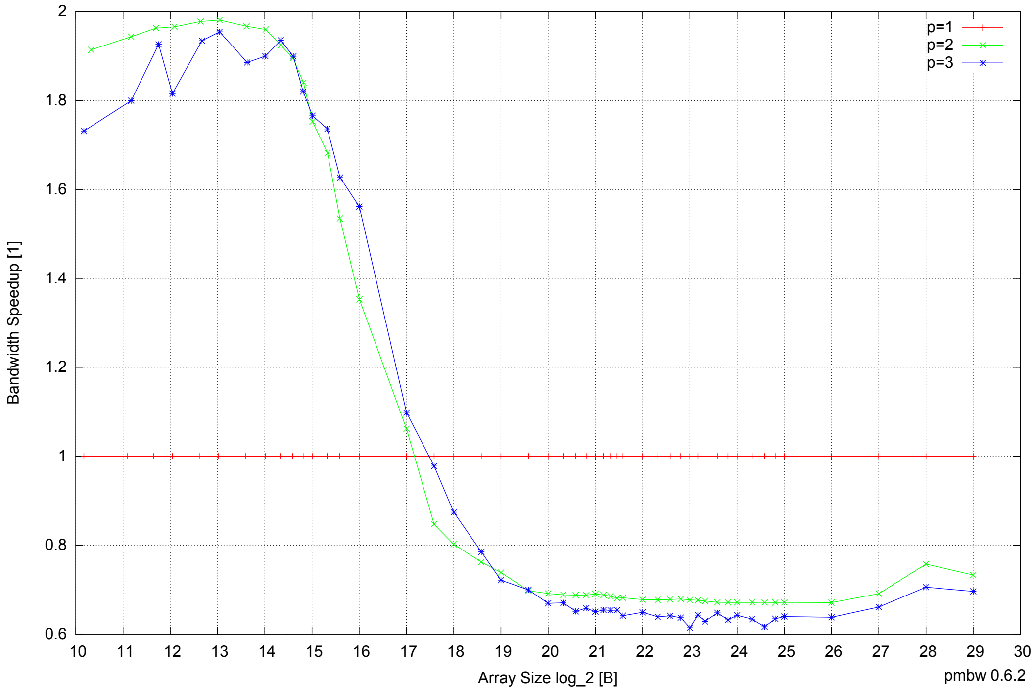
Motorola Atrix: ARM Cortex A9 1GB - Speedup of Parallel Memory Bandwidth - ScanWrite64PtrSimpleLoop
