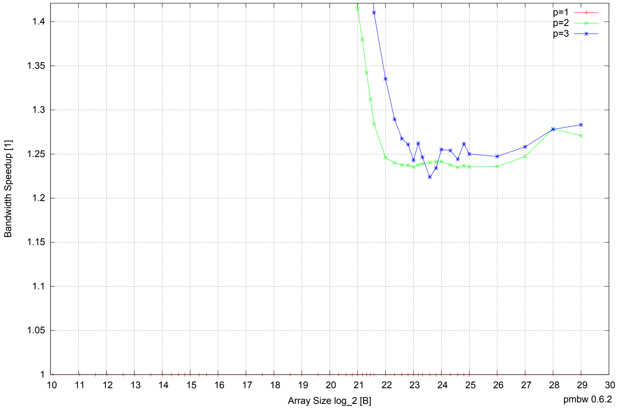
Motorola Atrix: ARM Cortex A9 1GB - Speedup of Parallel Memory Bandwidth (enlarged) - ScanRead32PtrSimpleLoop
