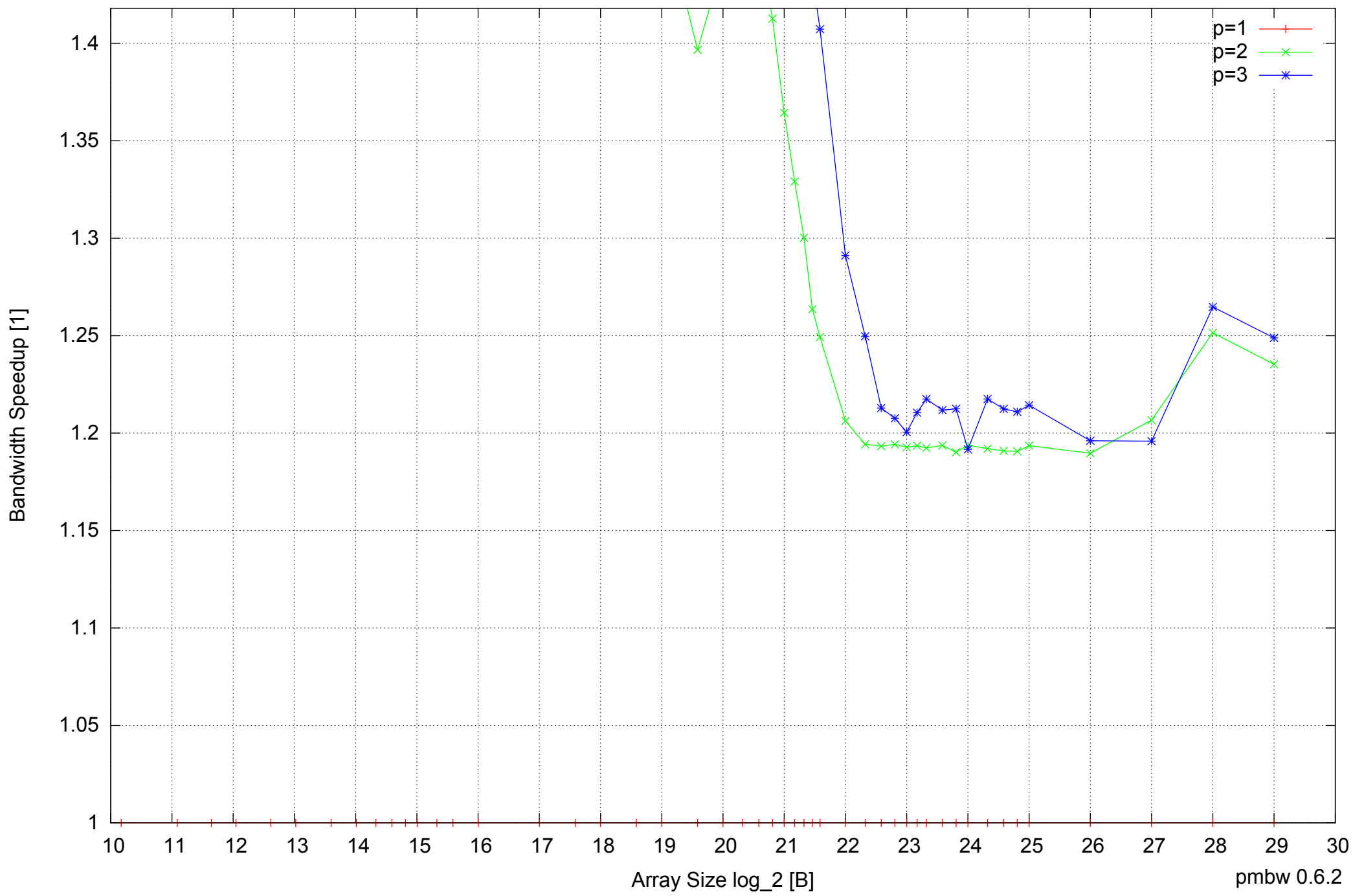
Motorola Atrix: ARM Cortex A9 1GB - Speedup of Parallel Memory Bandwidth (enlarged) - ScanRead64PtrSimpleLoop
