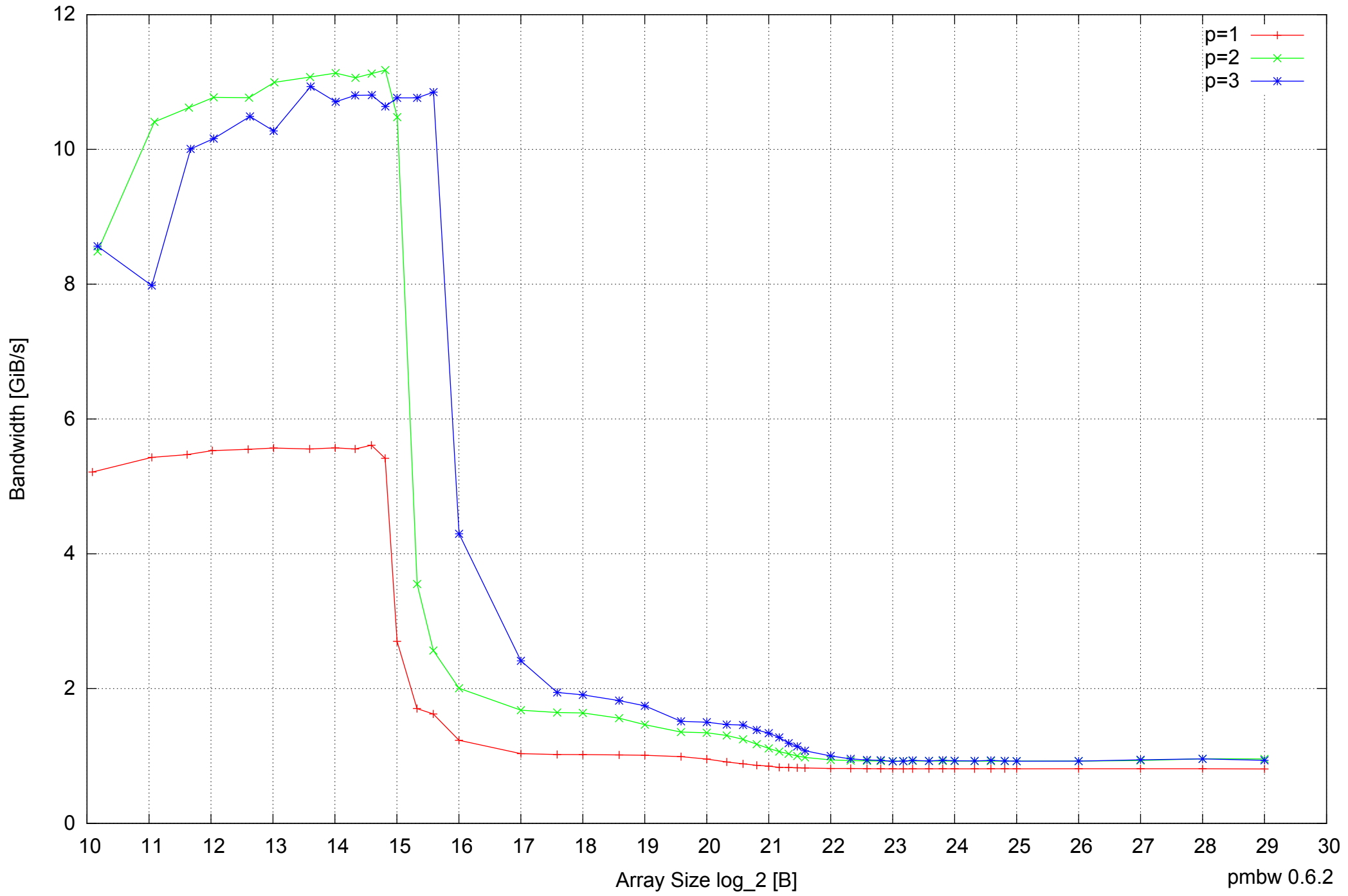
Motorola Atrix: ARM Cortex A9 1GB - Parallel Memory Bandwidth - ScanRead32PtrMultiLoop
