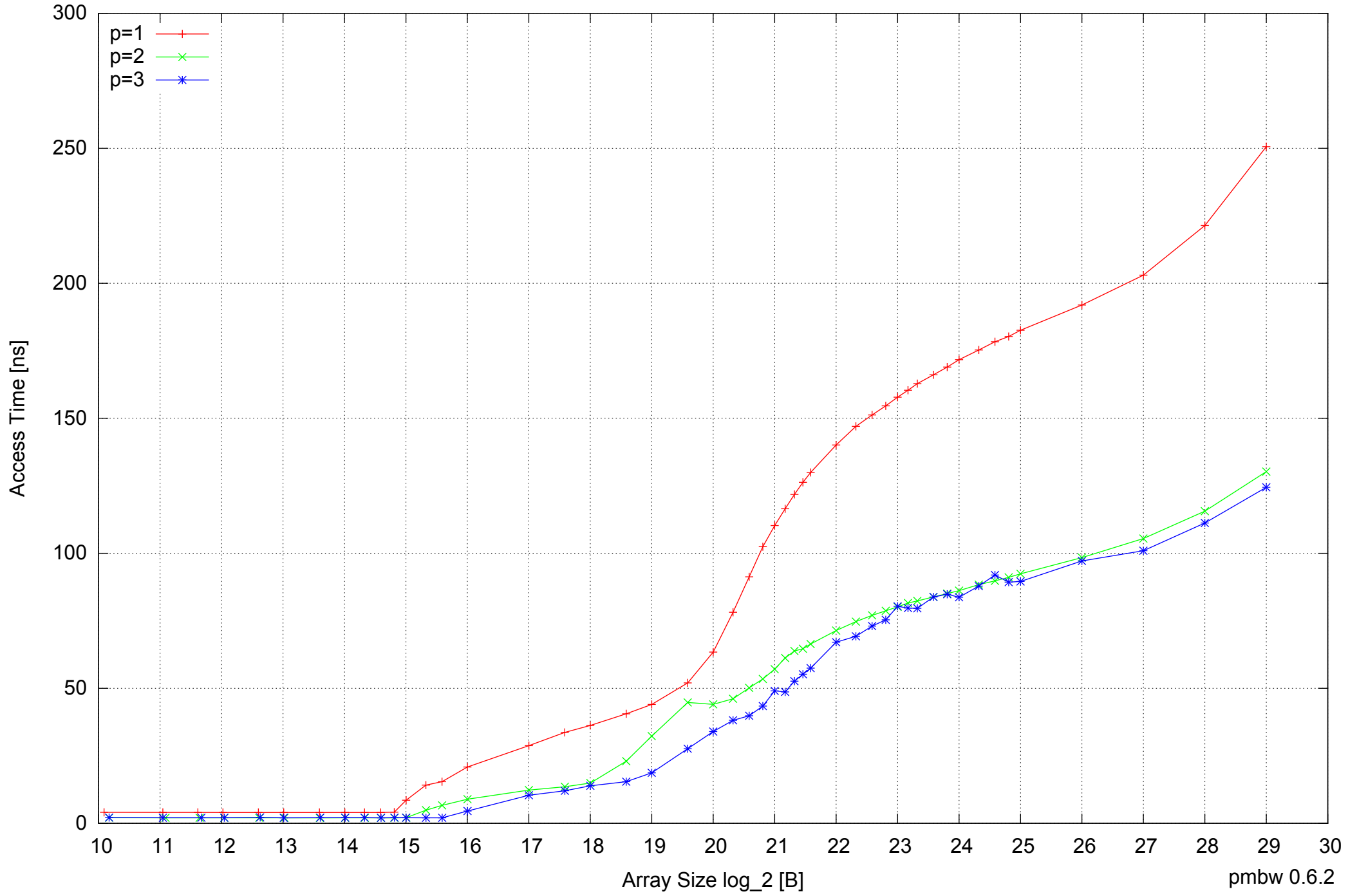
Motorola Atrix: ARM Cortex A9 1GB - Parallel Memory Access Time - PermRead32SimpleLoop
