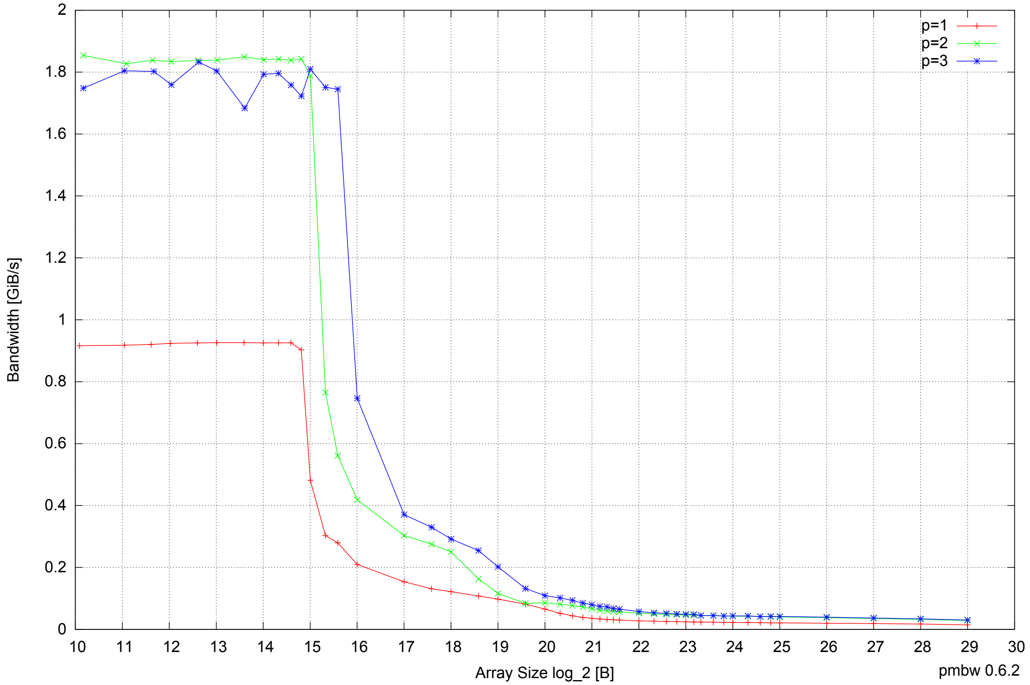
Motorola Atrix: ARM Cortex A9 1GB - Parallel Memory Bandwidth - PermRead32UnrollLoop
