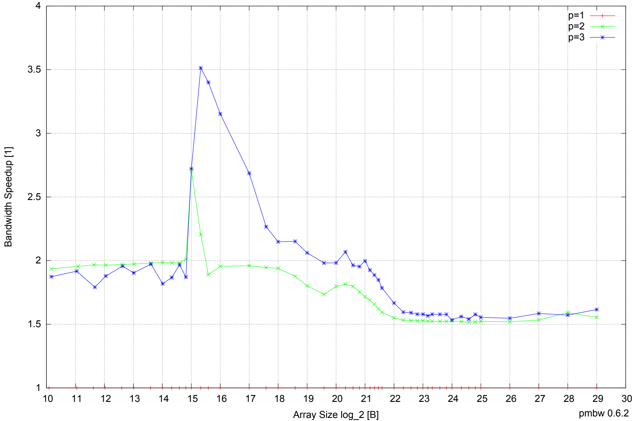
Motorola Atrix: ARM Cortex A9 1GB - Speedup of Parallel Memory Bandwidth - ScanRead32IndexSimpleLoop
