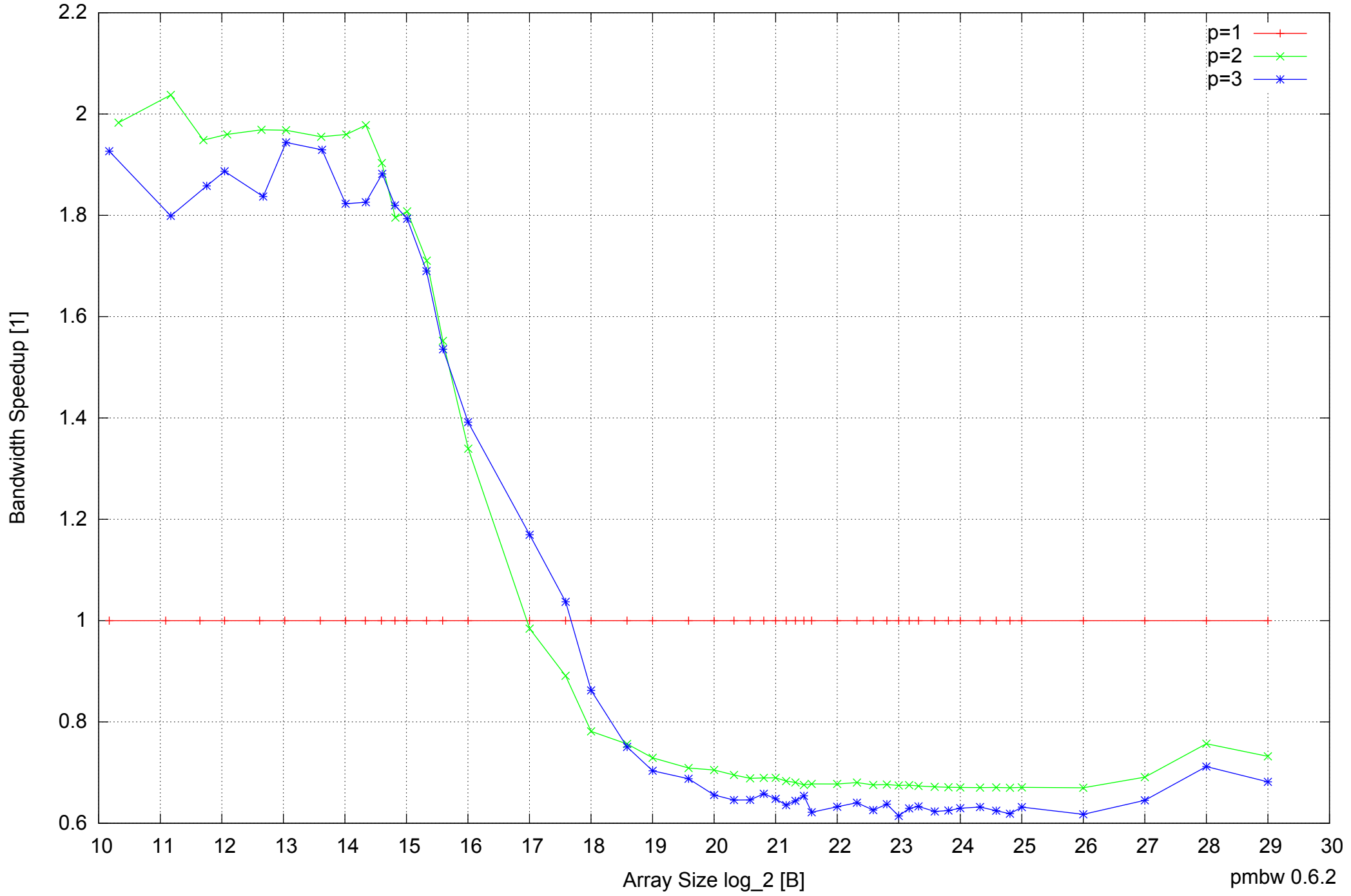
Motorola Atrix: ARM Cortex A9 1GB - Speedup of Parallel Memory Bandwidth - ScanWrite64PtrUnrollLoop
