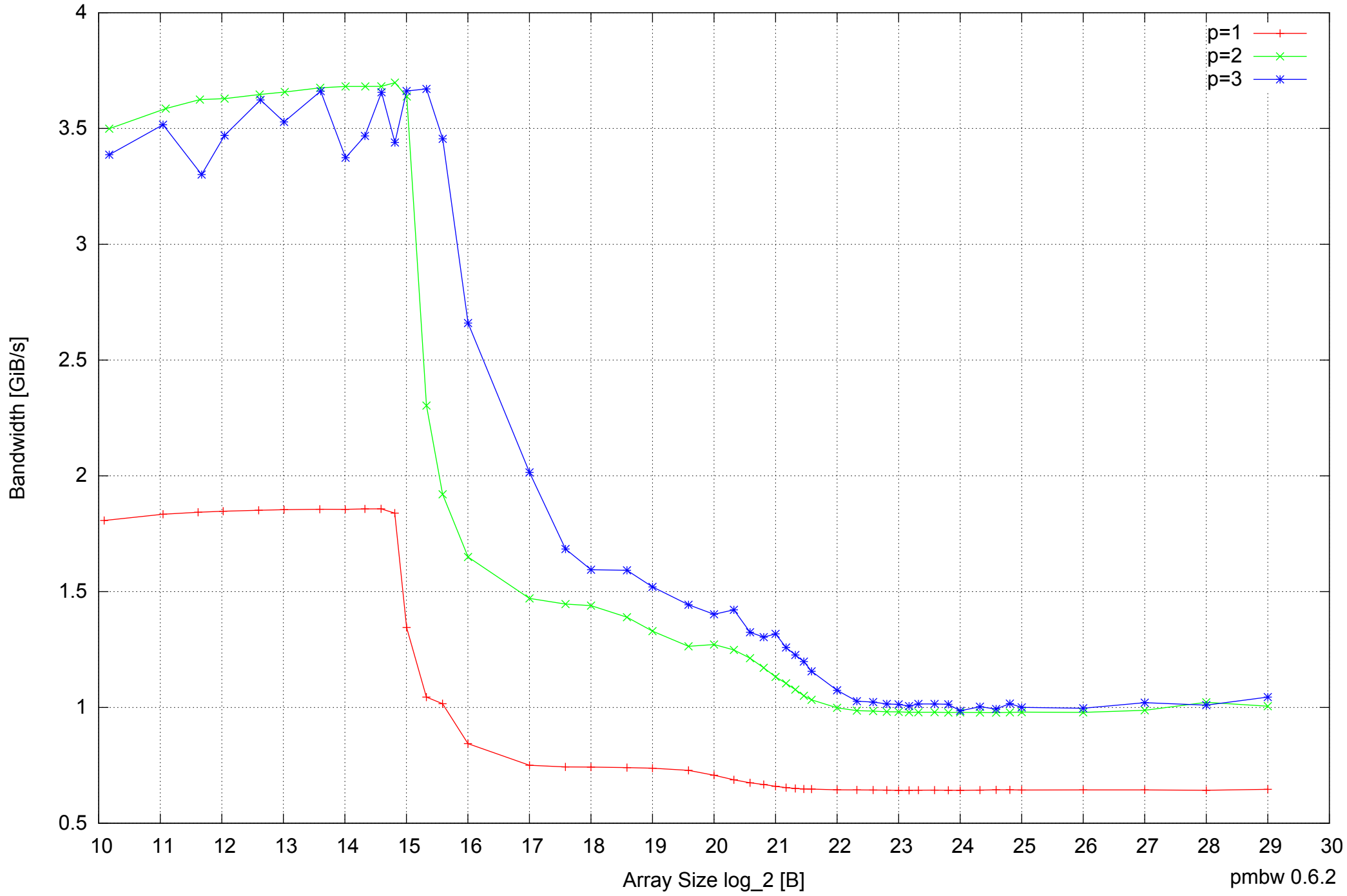
Motorola Atrix: ARM Cortex A9 1GB - Parallel Memory Bandwidth - ScanRead32IndexSimpleLoop
