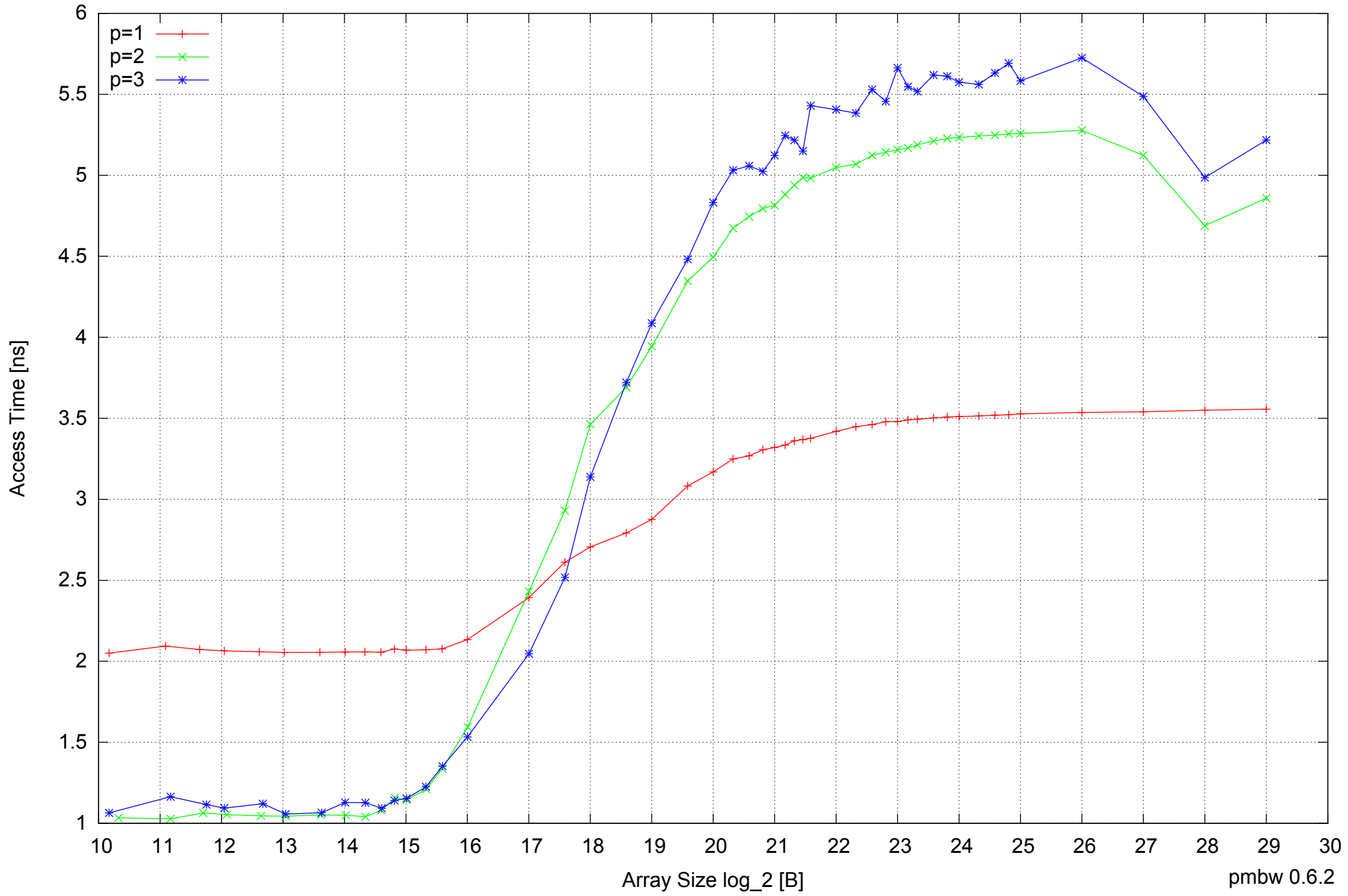
Motorola Atrix: ARM Cortex A9 1GB - Parallel Memory Access Time - ScanWrite64PtrUnrollLoop
