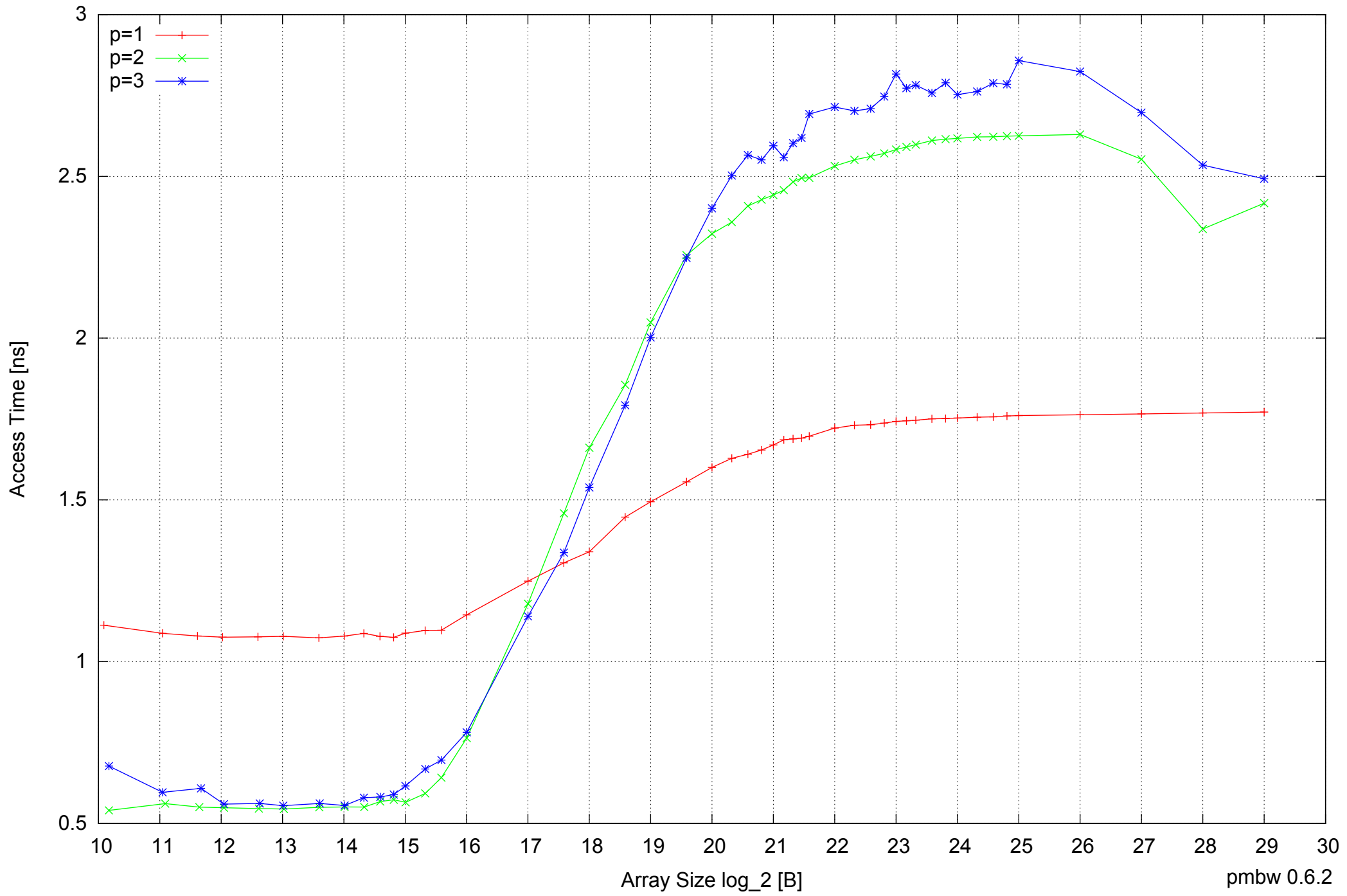
Motorola Atrix: ARM Cortex A9 1GB - Parallel Memory Access Time - ScanWrite32PtrUnrollLoop
