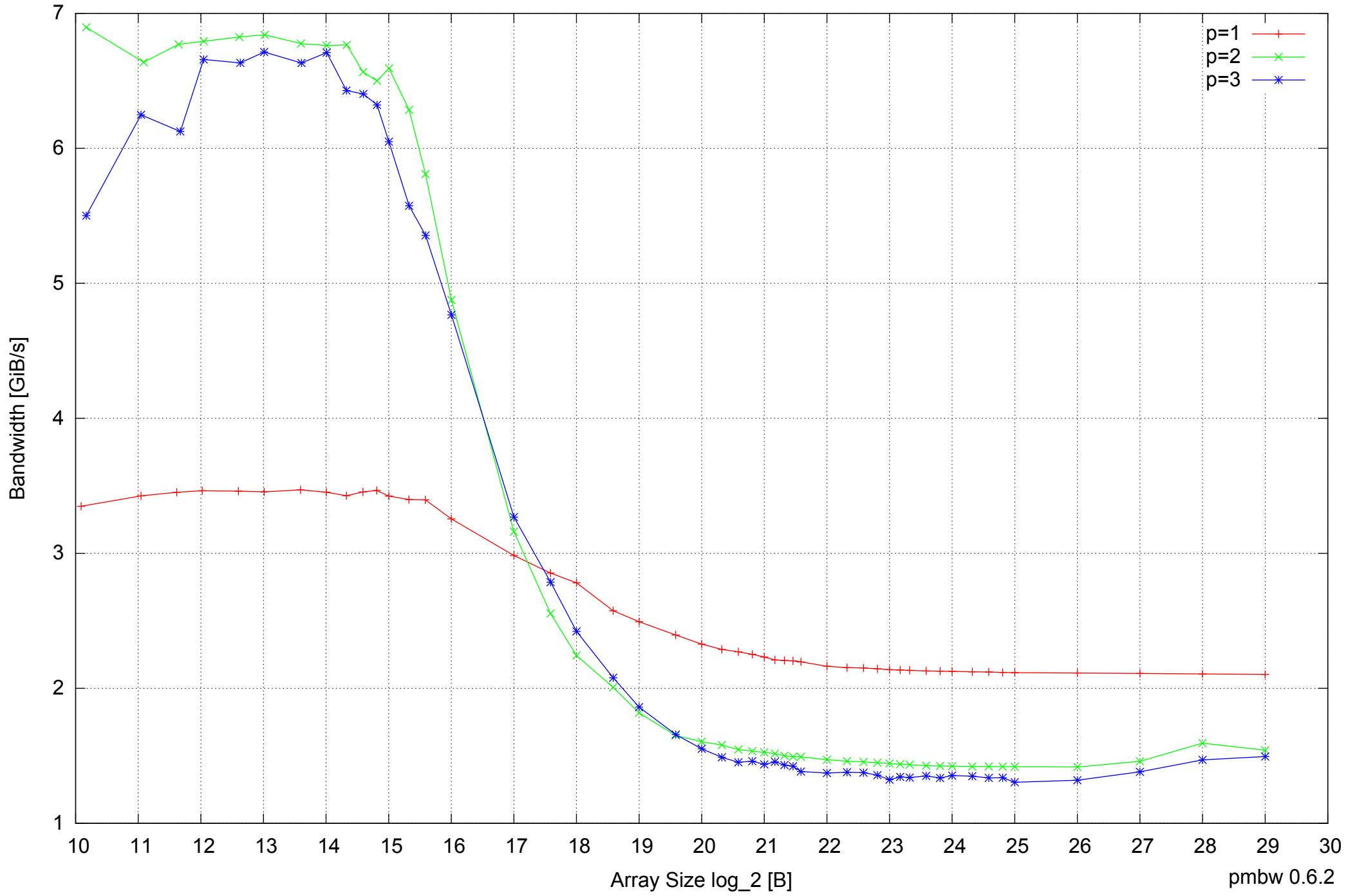
Motorola Atrix: ARM Cortex A9 1GB - Parallel Memory Bandwidth - ScanWrite32PtrUnrollLoop
