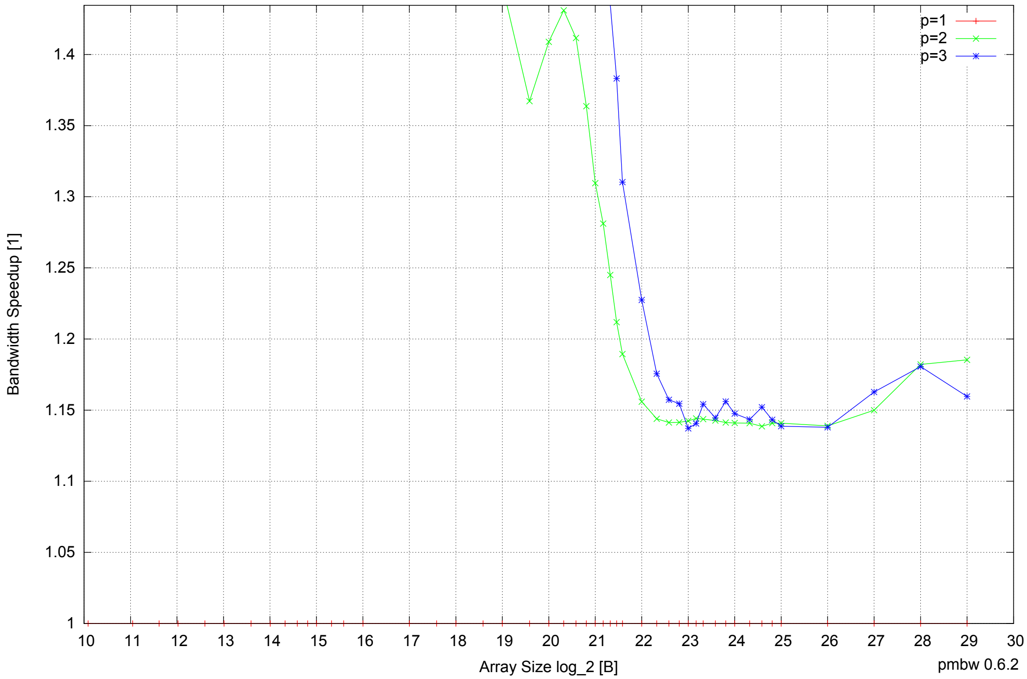
Motorola Atrix: ARM Cortex A9 1GB - Speedup of Parallel Memory Bandwidth (enlarged) - ScanRead32PtrMultiLoop
