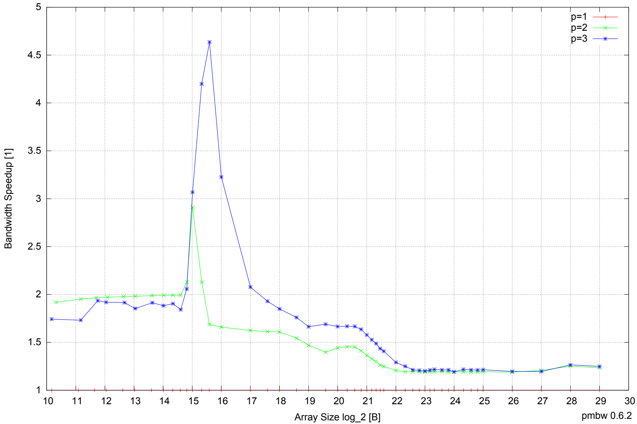
Motorola Atrix: ARM Cortex A9 1GB - Speedup of Parallel Memory Bandwidth - ScanRead64PtrSimpleLoop
