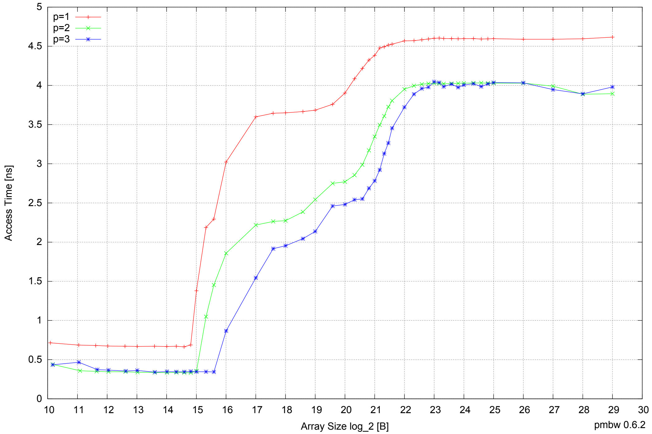
Motorola Atrix: ARM Cortex A9 1GB - Parallel Memory Access Time - ScanRead32PtrMultiLoop
