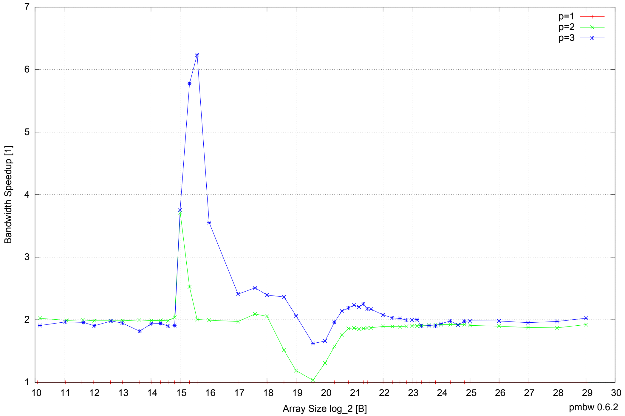
Motorola Atrix: ARM Cortex A9 1GB - Speedup of Parallel Memory Bandwidth - PermRead32UnrollLoop
