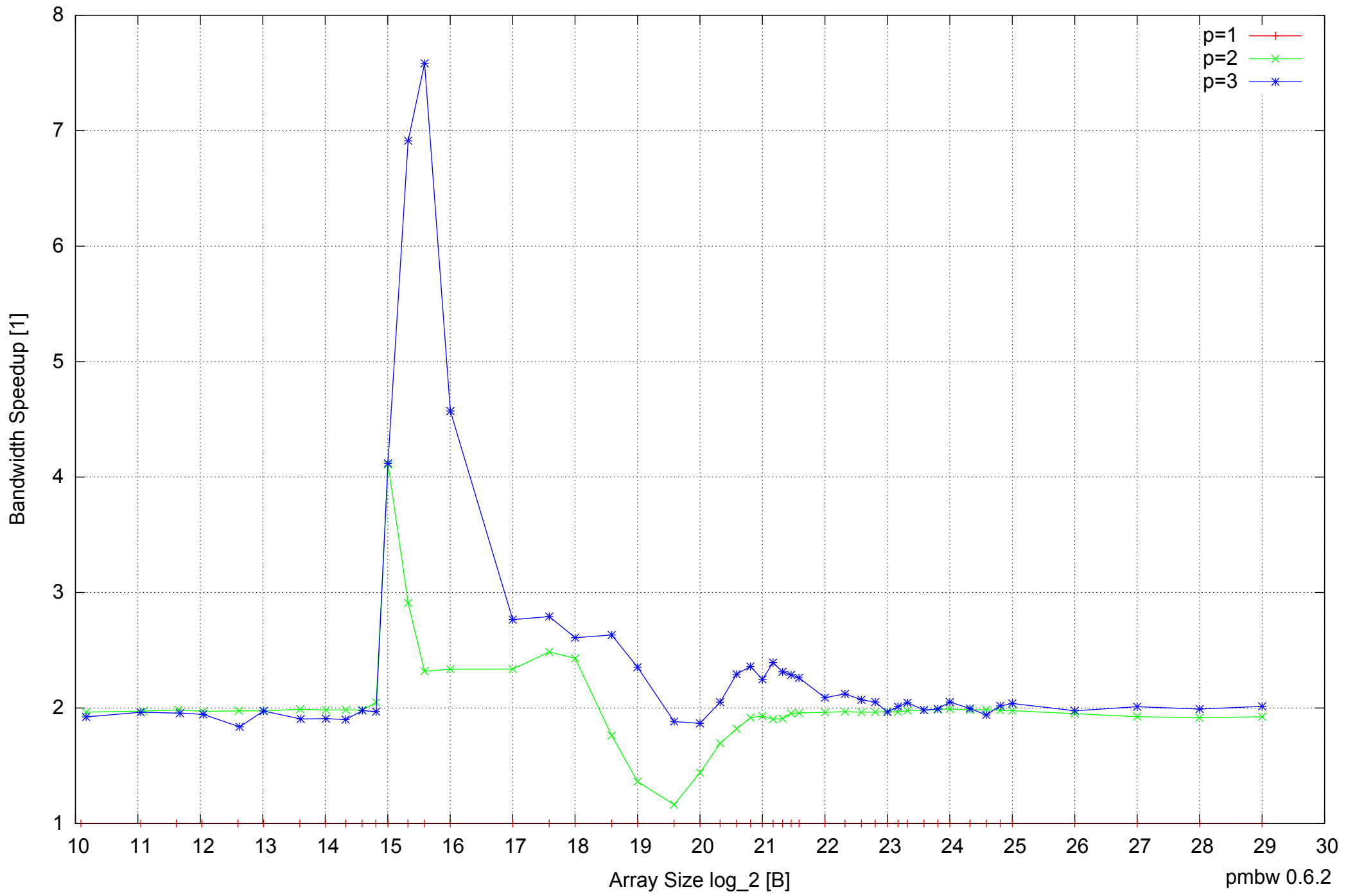
Motorola Atrix: ARM Cortex A9 1GB - Speedup of Parallel Memory Bandwidth - PermRead32SimpleLoop
