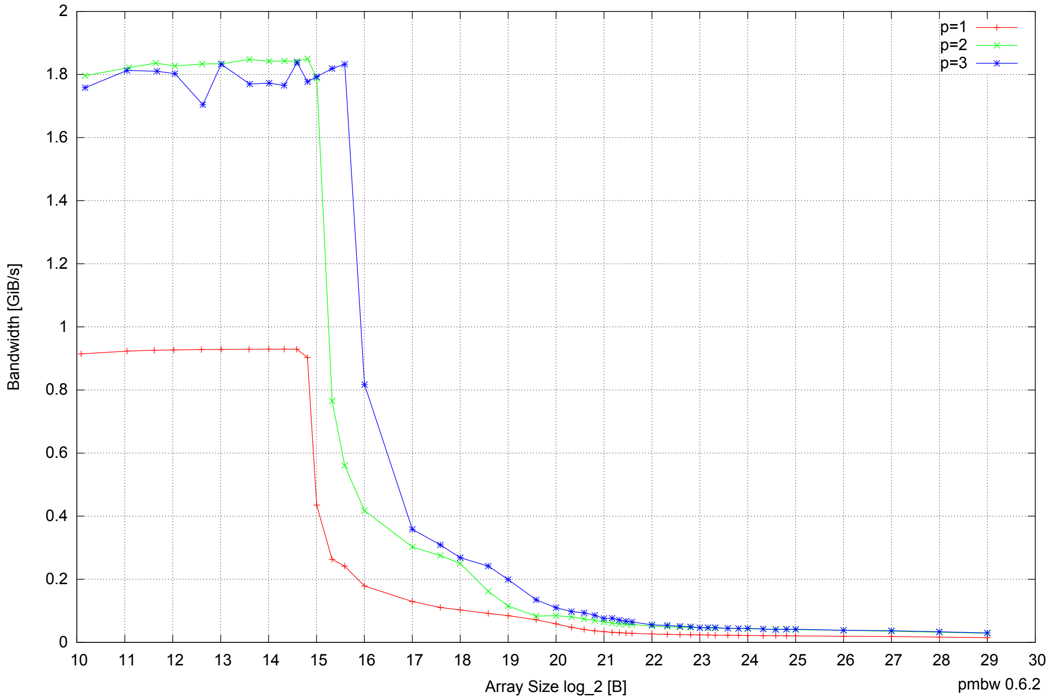
Motorola Atrix: ARM Cortex A9 1GB - Parallel Memory Bandwidth - PermRead32SimpleLoop
