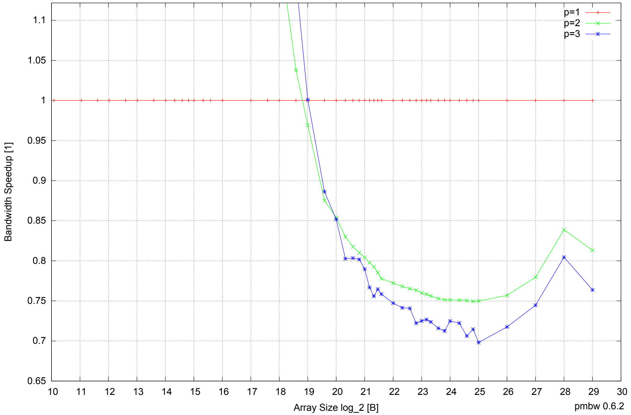
Motorola Atrix: ARM Cortex A9 1GB - Speedup of Parallel Memory Bandwidth (enlarged) - ScanWrite32PtrSimpleLoop
