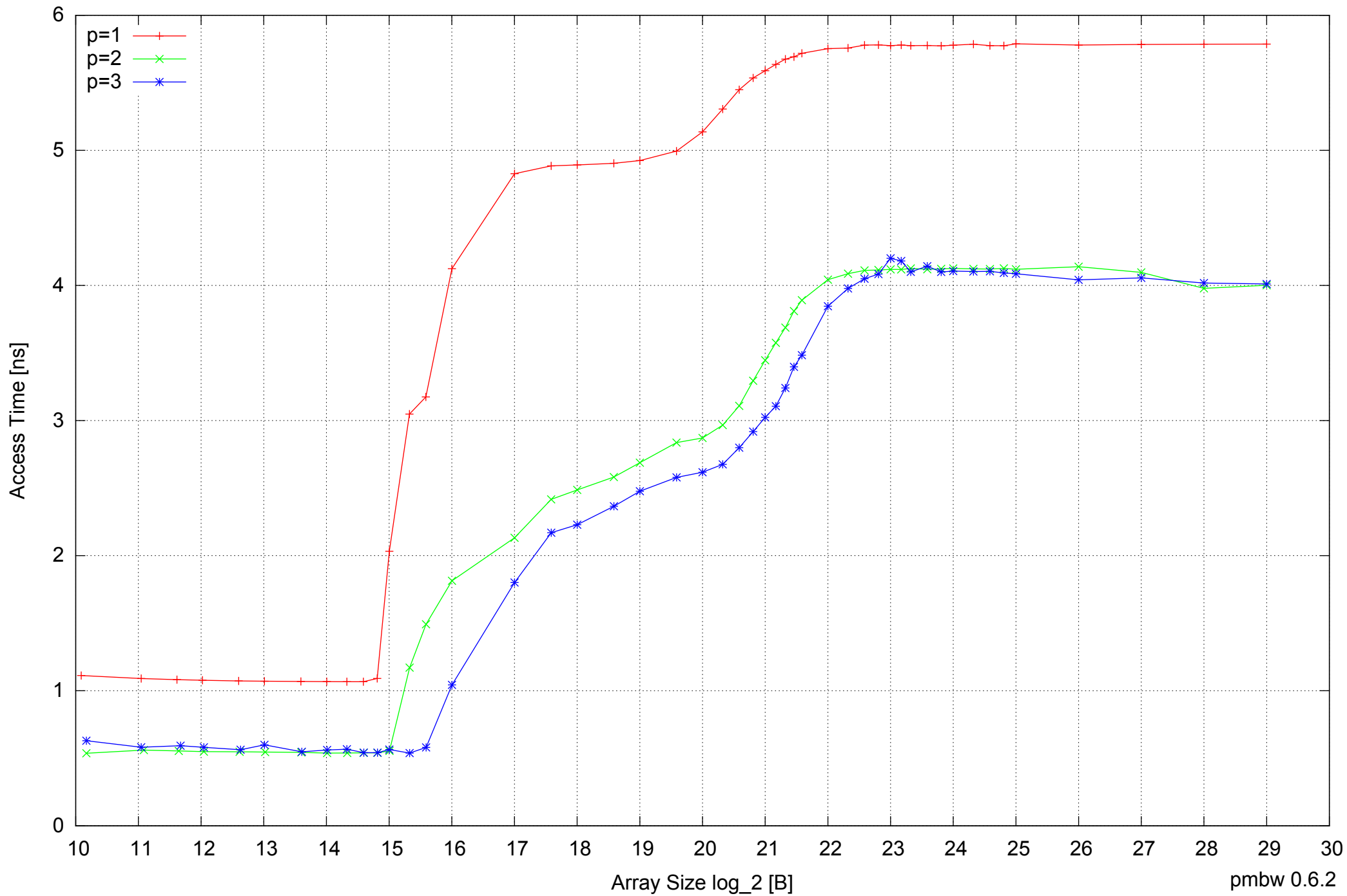
Motorola Atrix: ARM Cortex A9 1GB - Parallel Memory Access Time - ScanRead32PtrUnrollLoop
