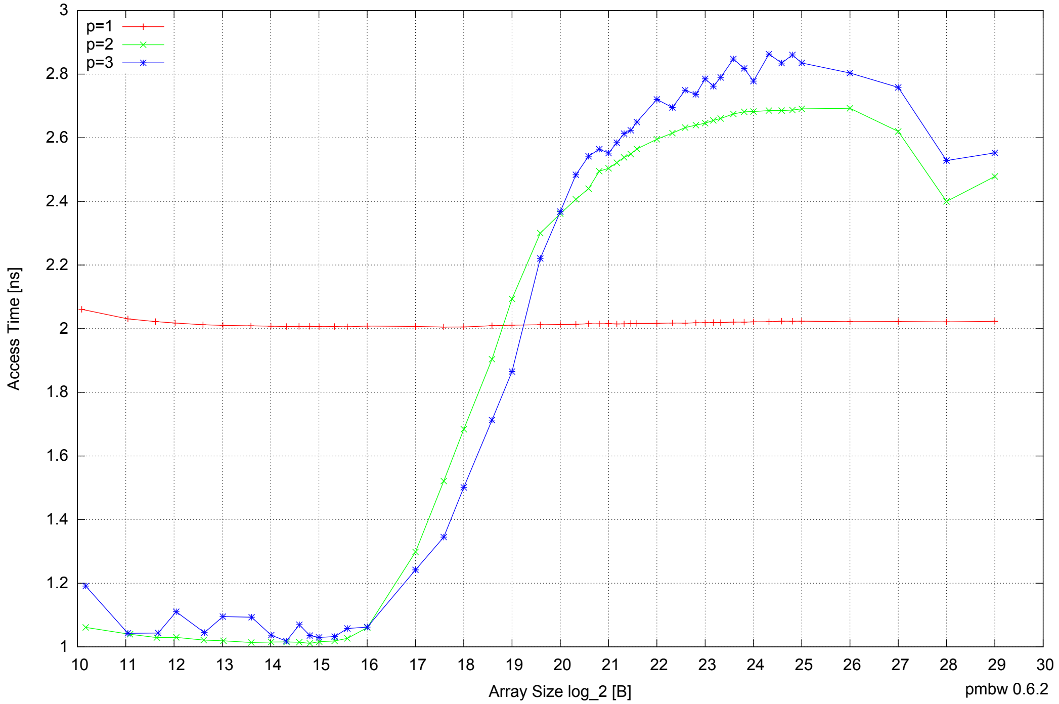
Motorola Atrix: ARM Cortex A9 1GB - Parallel Memory Access Time - ScanWrite32IndexSimpleLoop
