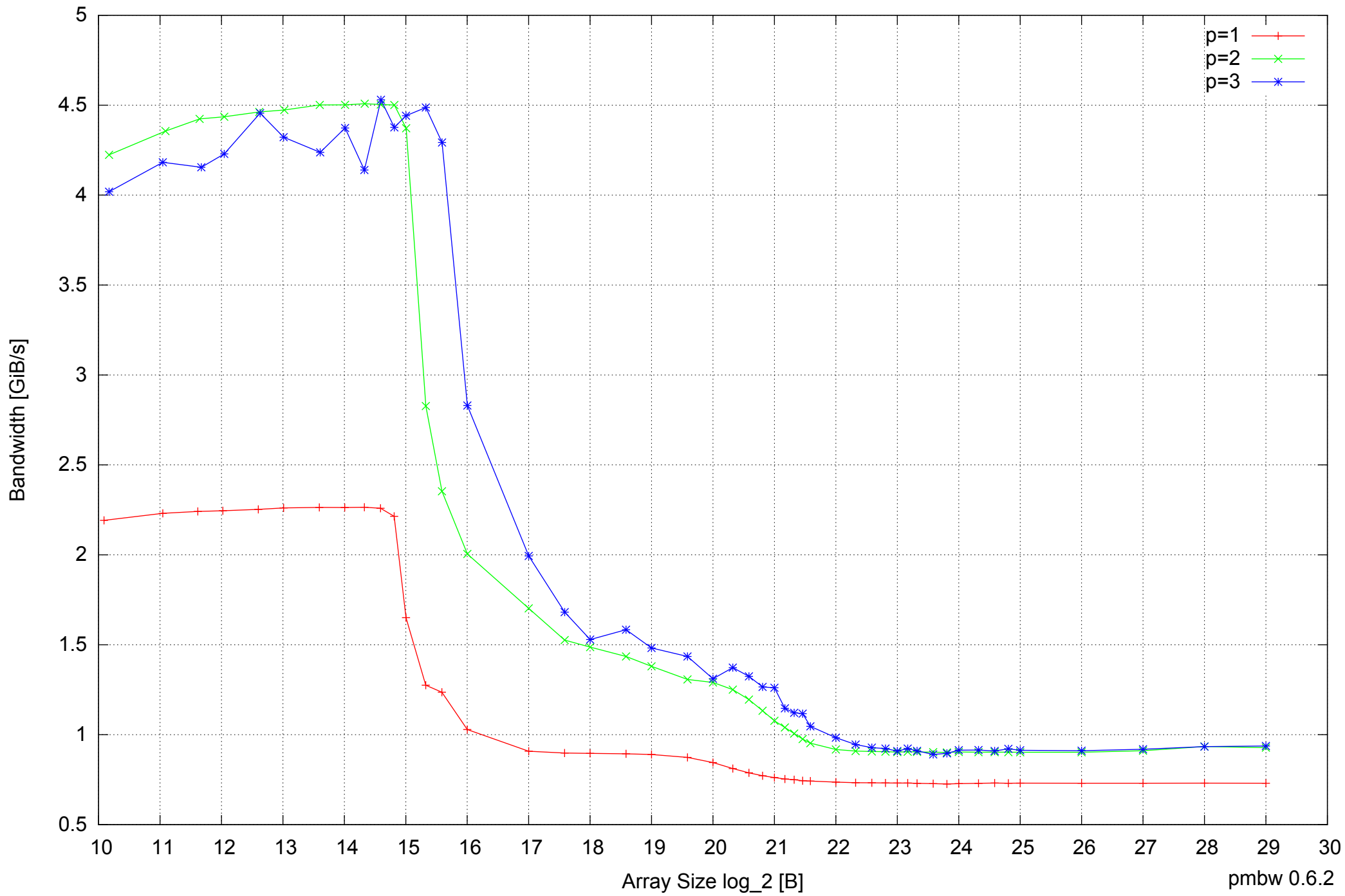
Motorola Atrix: ARM Cortex A9 1GB - Parallel Memory Bandwidth - ScanRead32PtrSimpleLoop
