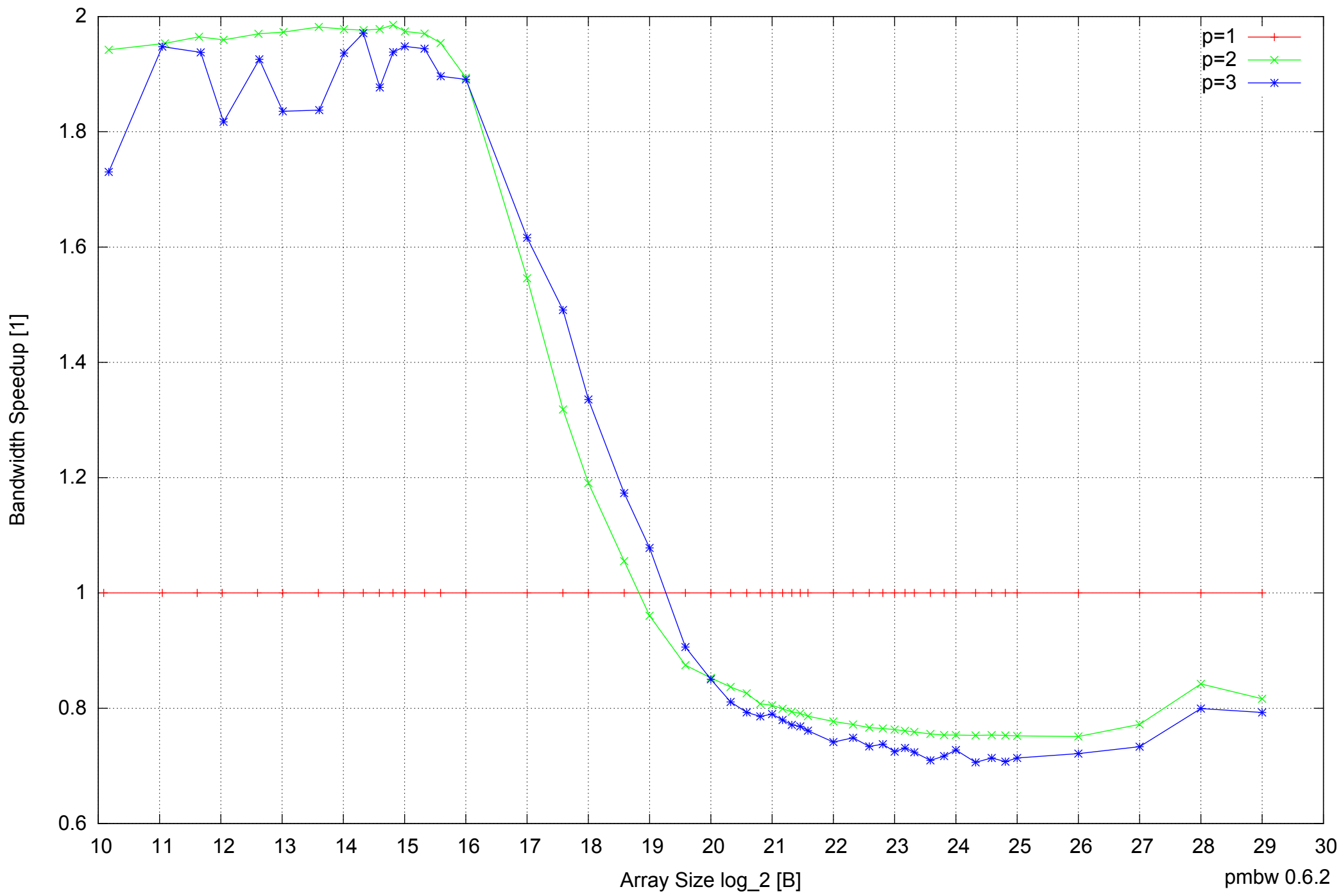
Motorola Atrix: ARM Cortex A9 1GB - Speedup of Parallel Memory Bandwidth - ScanWrite32IndexSimpleLoop
