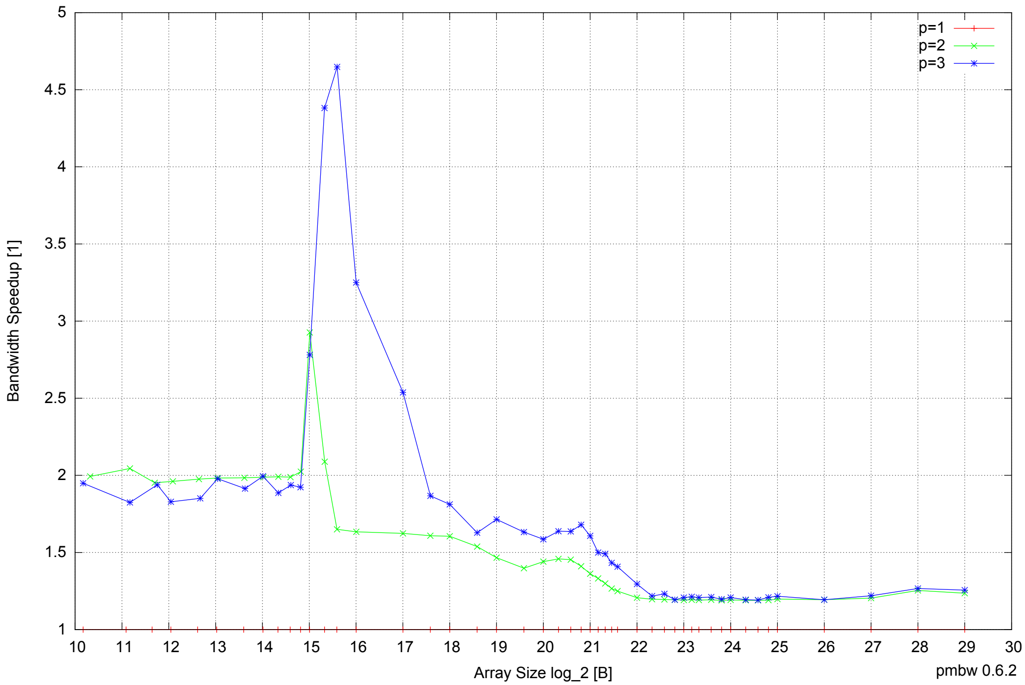
Motorola Atrix: ARM Cortex A9 1GB - Speedup of Parallel Memory Bandwidth - ScanRead64PtrUnrollLoop
