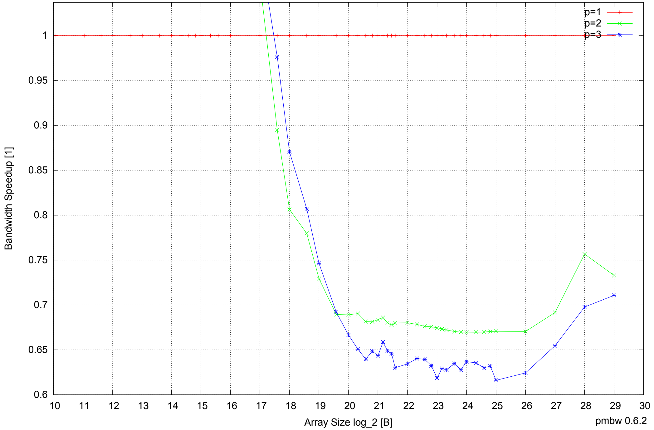
Motorola Atrix: ARM Cortex A9 1GB - Speedup of Parallel Memory Bandwidth (enlarged) - ScanWrite32PtrUnrollLoop
