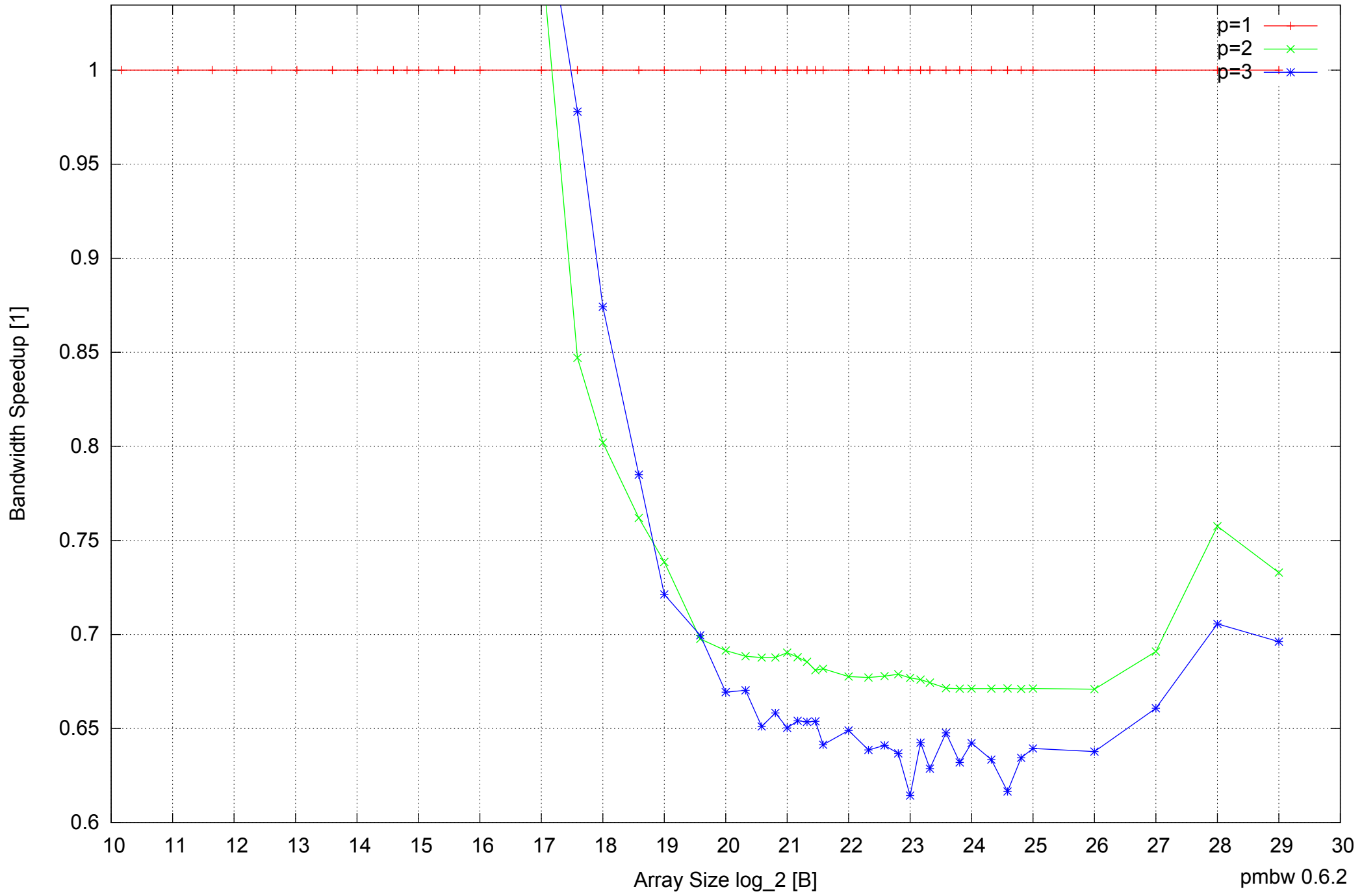
Motorola Atrix: ARM Cortex A9 1GB - Speedup of Parallel Memory Bandwidth (enlarged) - ScanWrite64PtrSimpleLoop
