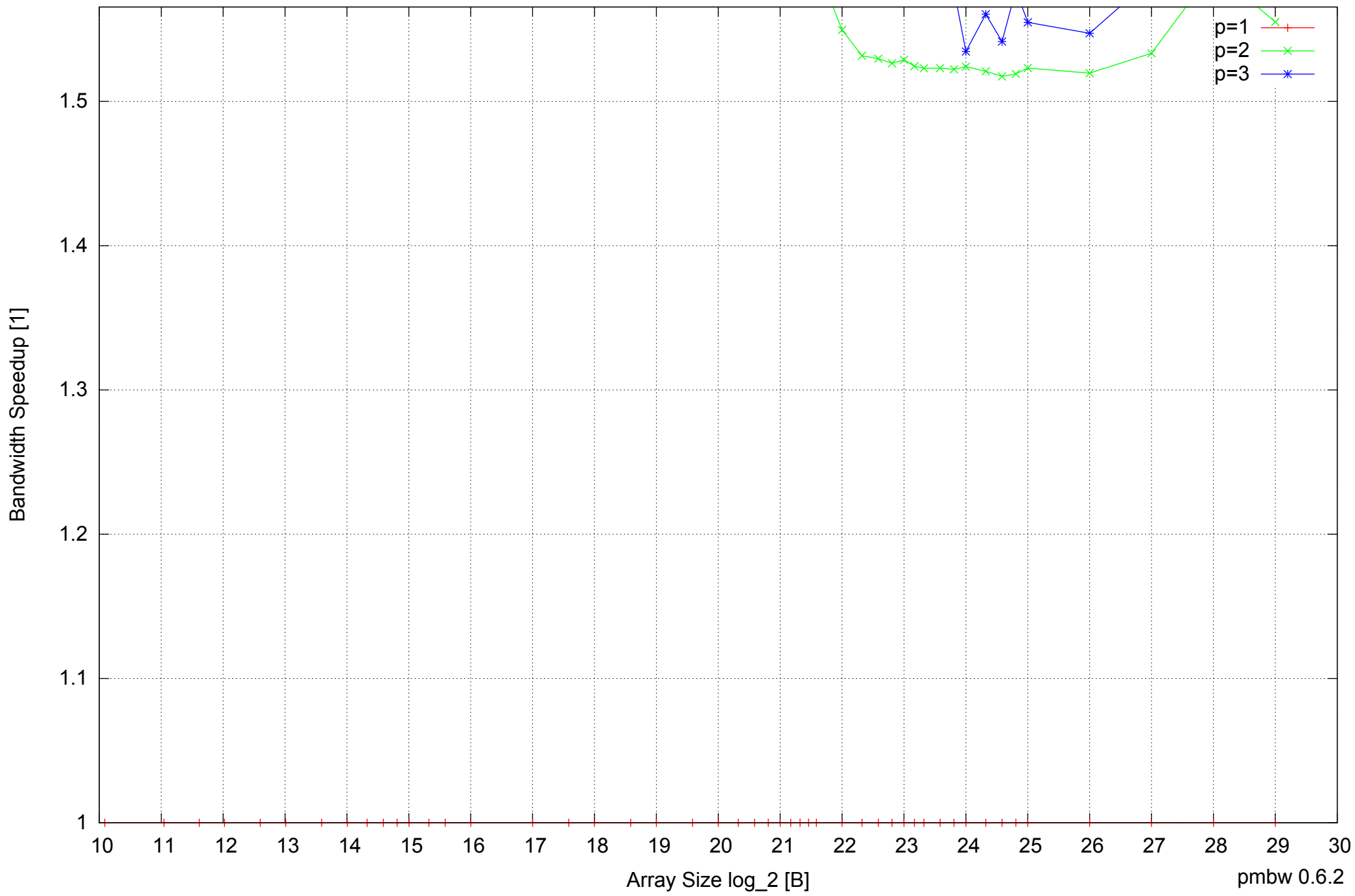
Motorola Atrix: ARM Cortex A9 1GB - Speedup of Parallel Memory Bandwidth (enlarged) - ScanRead32IndexSimpleLoop
