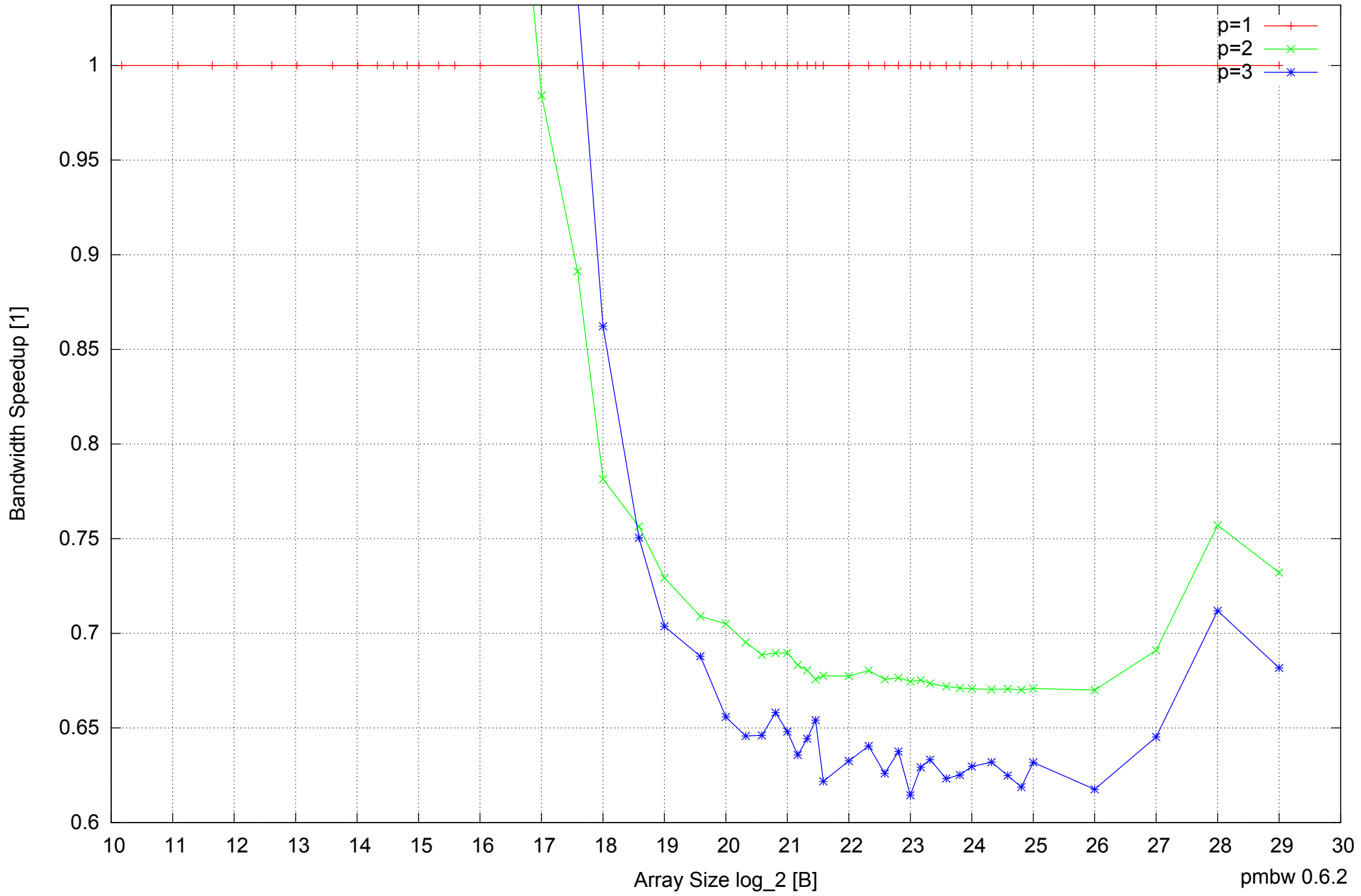
Motorola Atrix: ARM Cortex A9 1GB - Speedup of Parallel Memory Bandwidth (enlarged) - ScanWrite64PtrUnrollLoop
