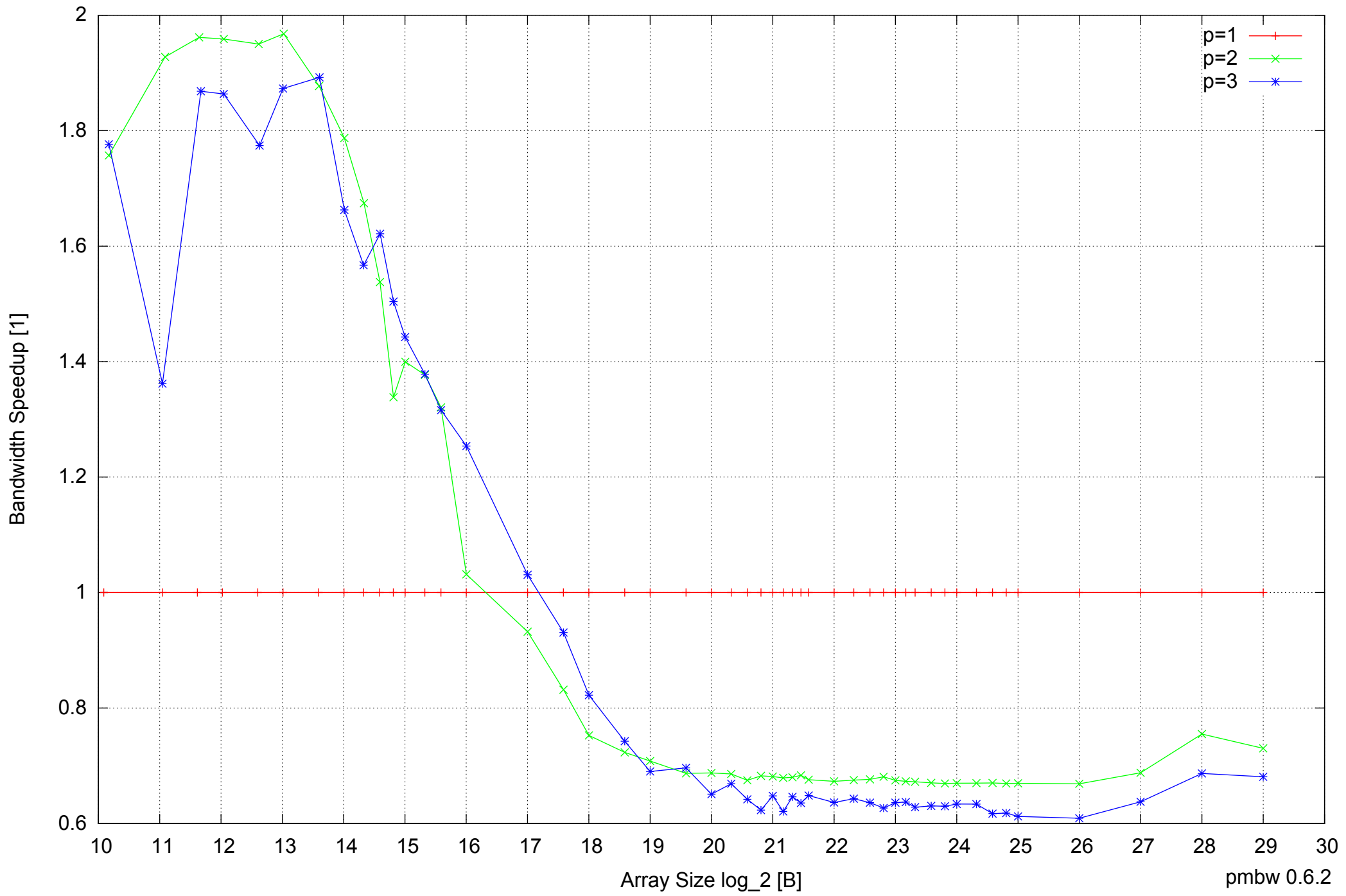
Motorola Atrix: ARM Cortex A9 1GB - Speedup of Parallel Memory Bandwidth - ScanWrite32PtrMultiLoop
