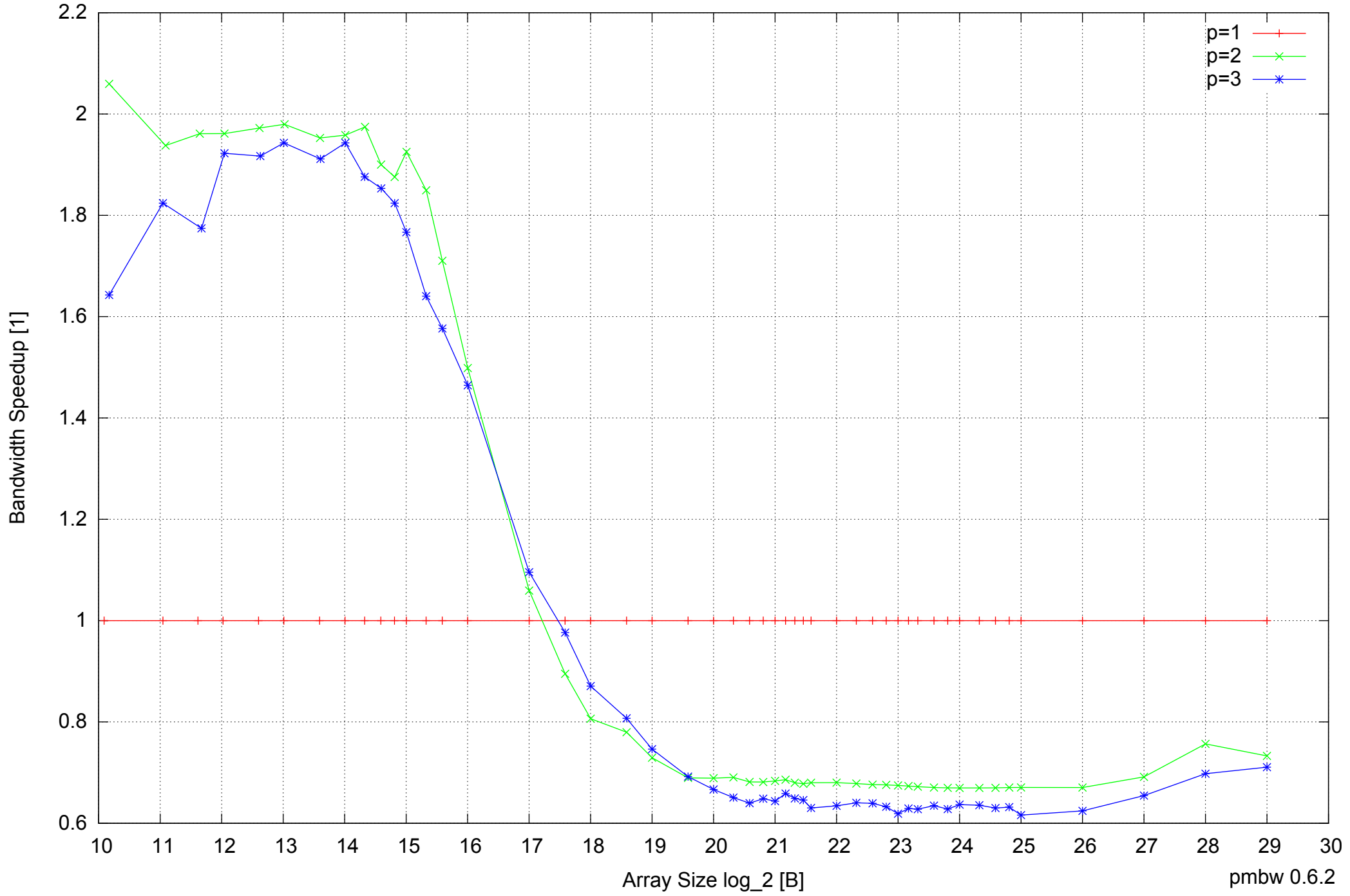
Motorola Atrix: ARM Cortex A9 1GB - Speedup of Parallel Memory Bandwidth - ScanWrite32PtrUnrollLoop
