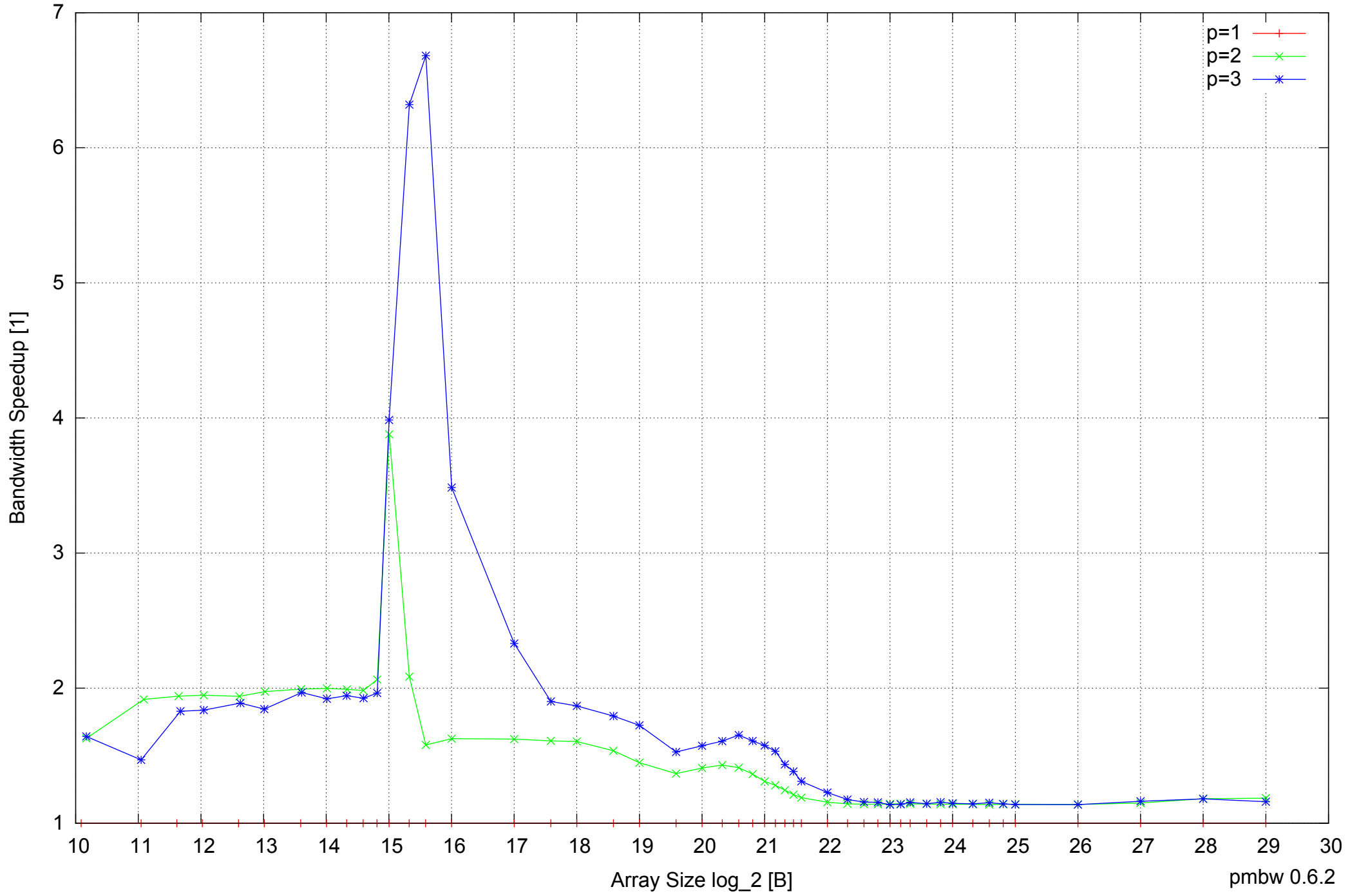
Motorola Atrix: ARM Cortex A9 1GB - Speedup of Parallel Memory Bandwidth - ScanRead32PtrMultiLoop
