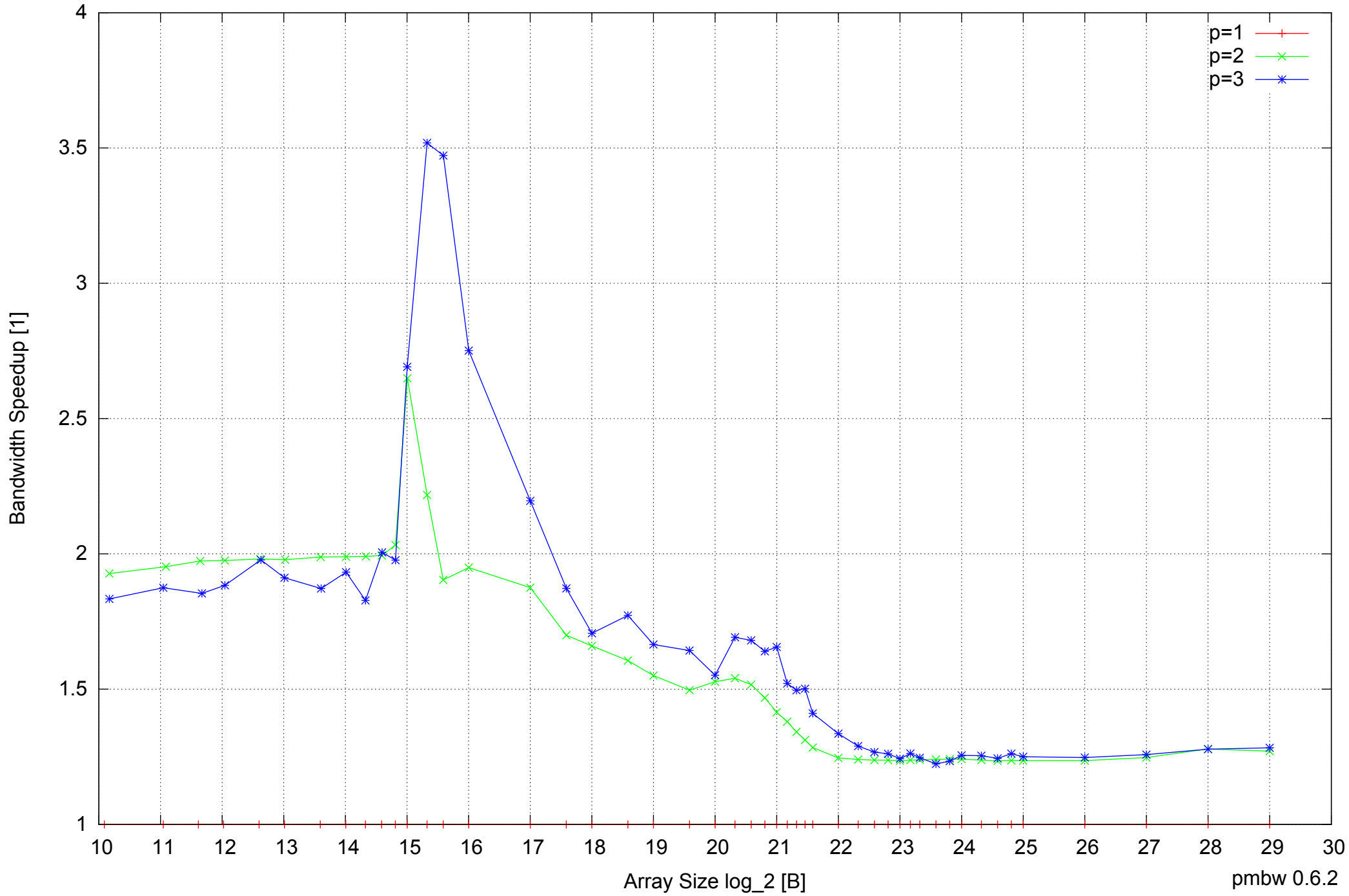
Motorola Atrix: ARM Cortex A9 1GB - Speedup of Parallel Memory Bandwidth - ScanRead32PtrSimpleLoop
