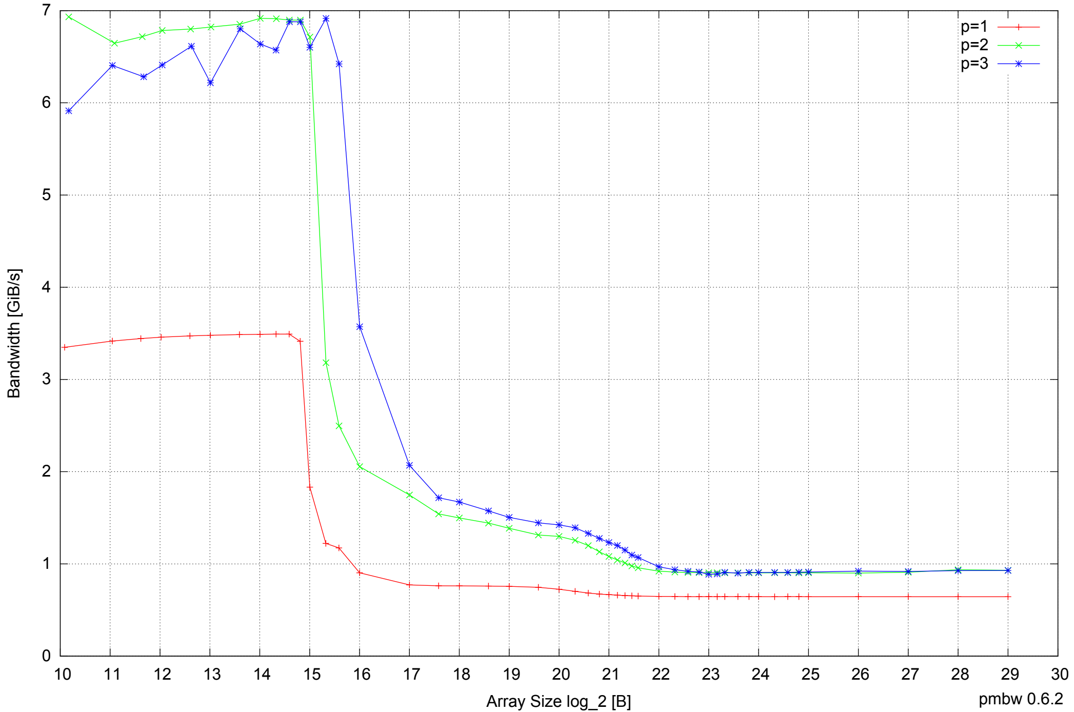
Motorola Atrix: ARM Cortex A9 1GB - Parallel Memory Bandwidth - ScanRead32PtrUnrollLoop
