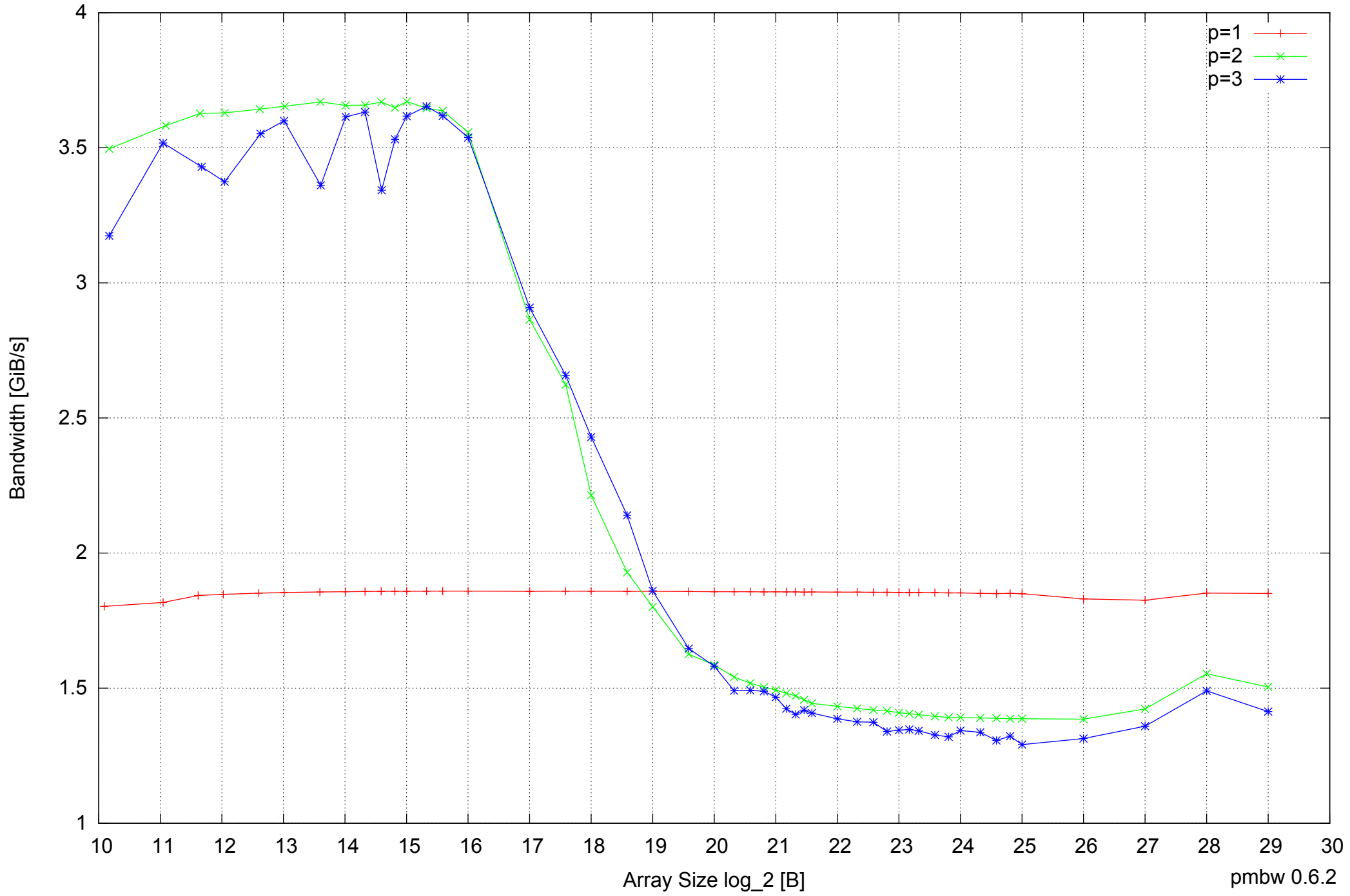
Motorola Atrix: ARM Cortex A9 1GB - Parallel Memory Bandwidth - ScanWrite32PtrSimpleLoop
