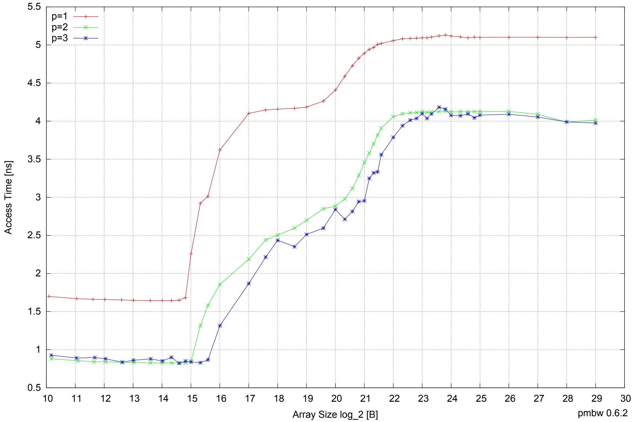
Motorola Atrix: ARM Cortex A9 1GB - Parallel Memory Access Time - ScanRead32PtrSimpleLoop
