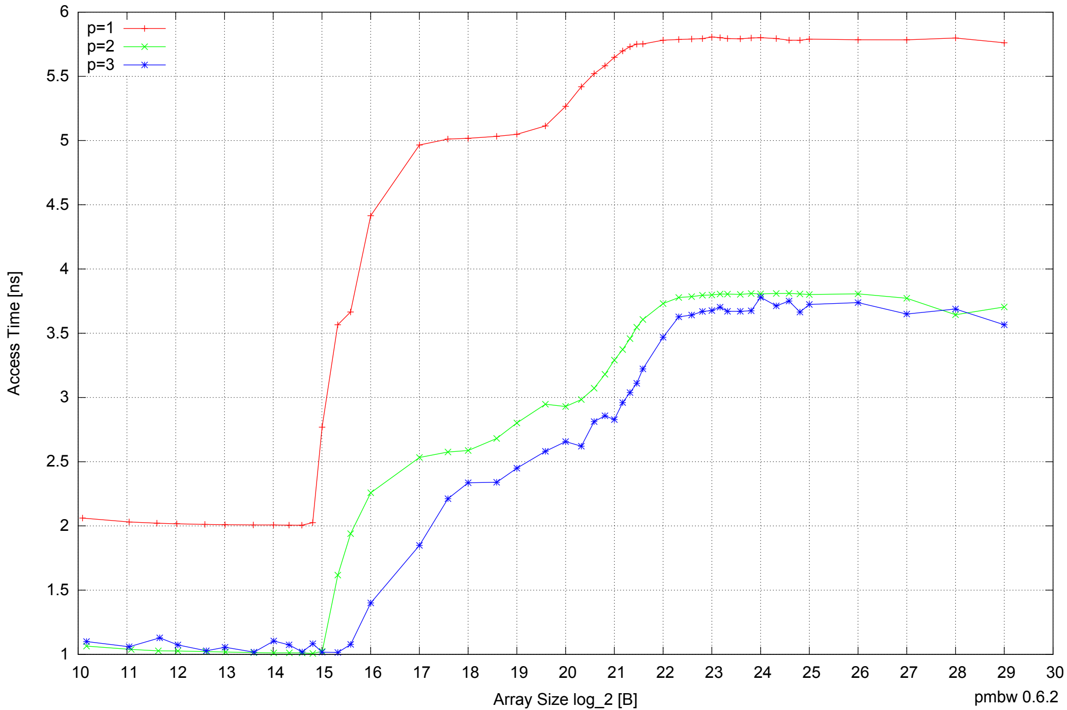
Motorola Atrix: ARM Cortex A9 1GB - Parallel Memory Access Time - ScanRead32IndexSimpleLoop
