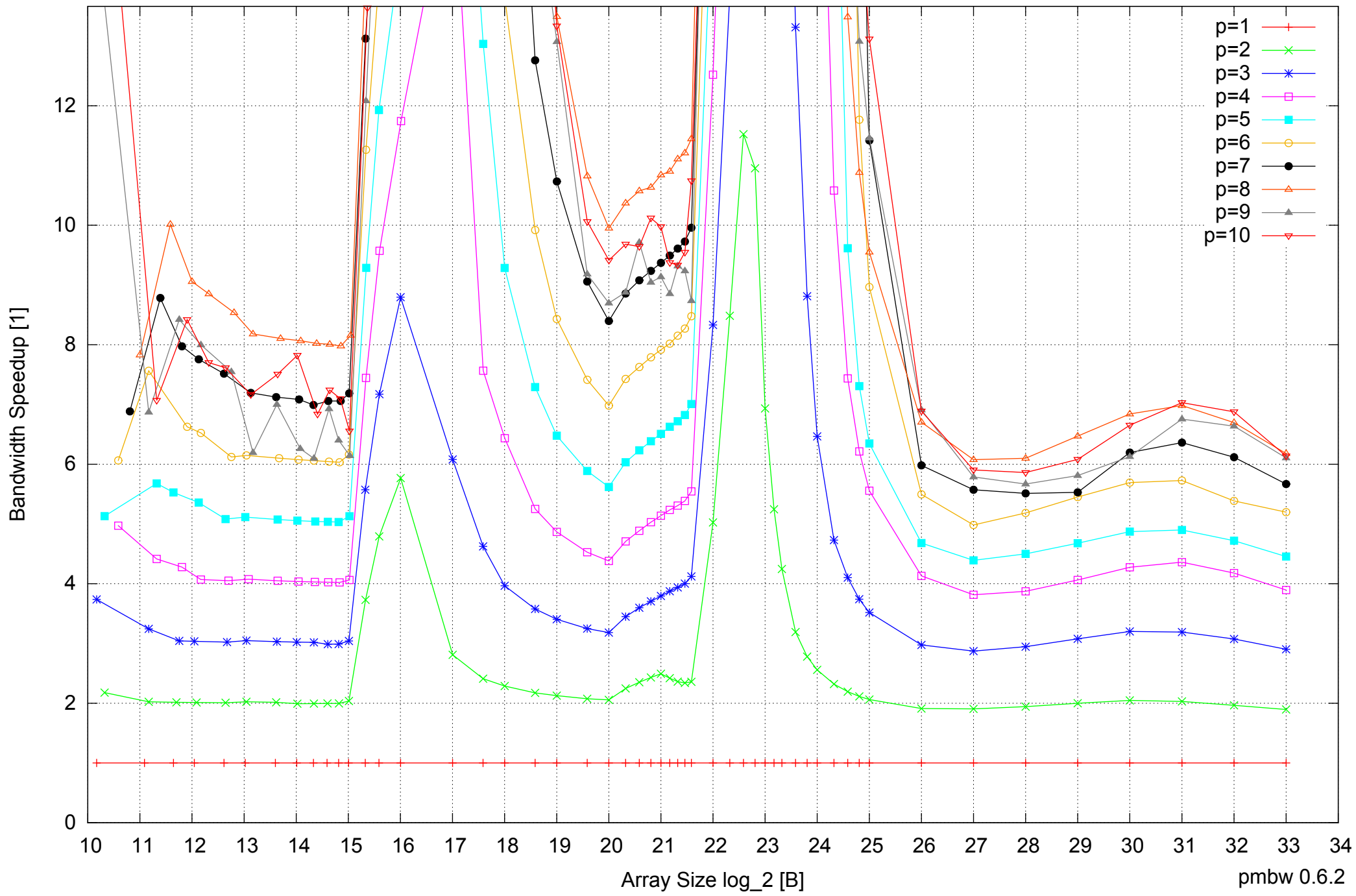
Intel Xeon X5355 16GB - Speedup of Parallel Memory Bandwidth (enlarged) - PermRead64UnrollLoop
