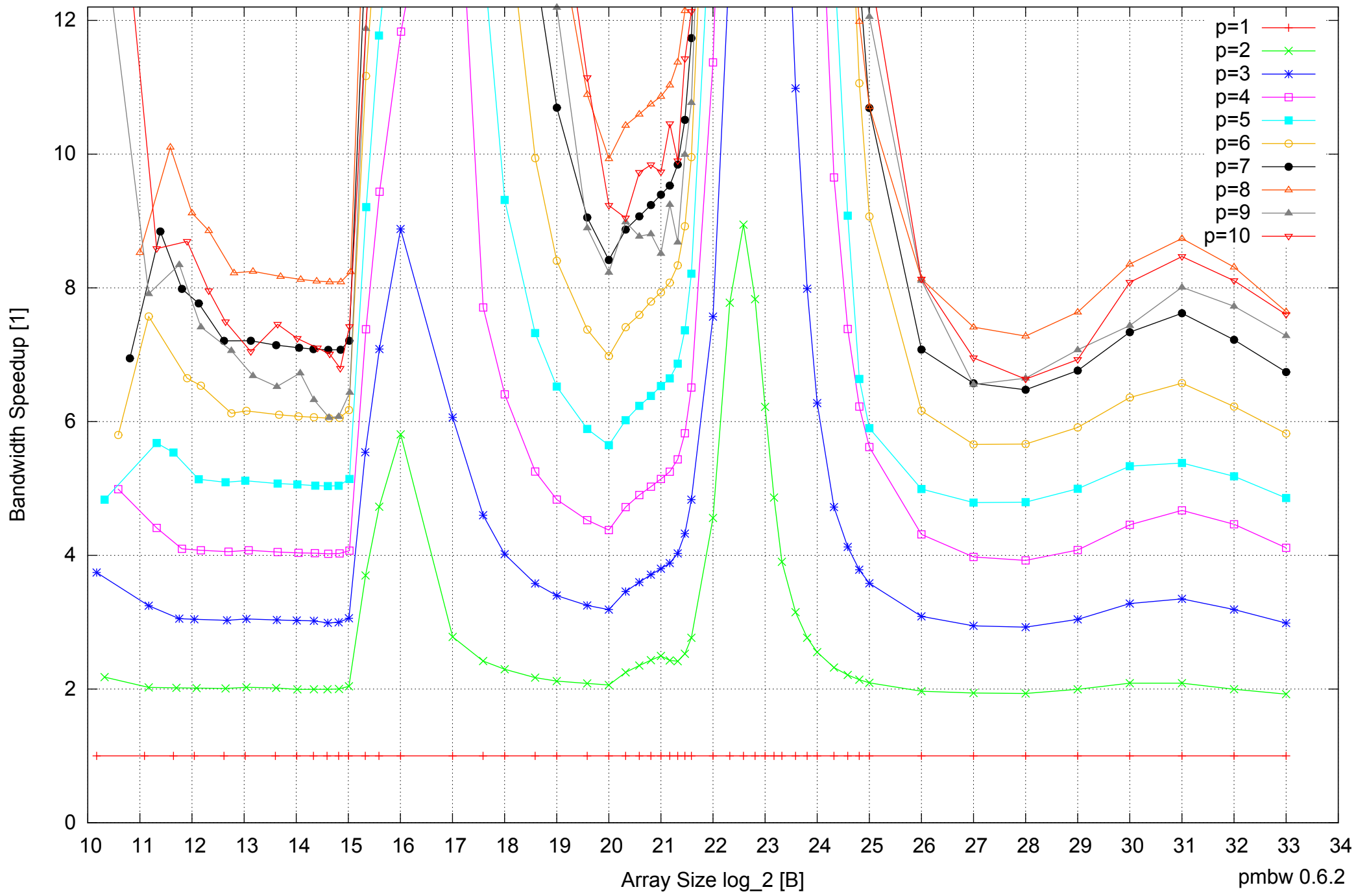
Intel Xeon E5345 16GB - Speedup of Parallel Memory Bandwidth (enlarged) - PermRead64UnrollLoop
