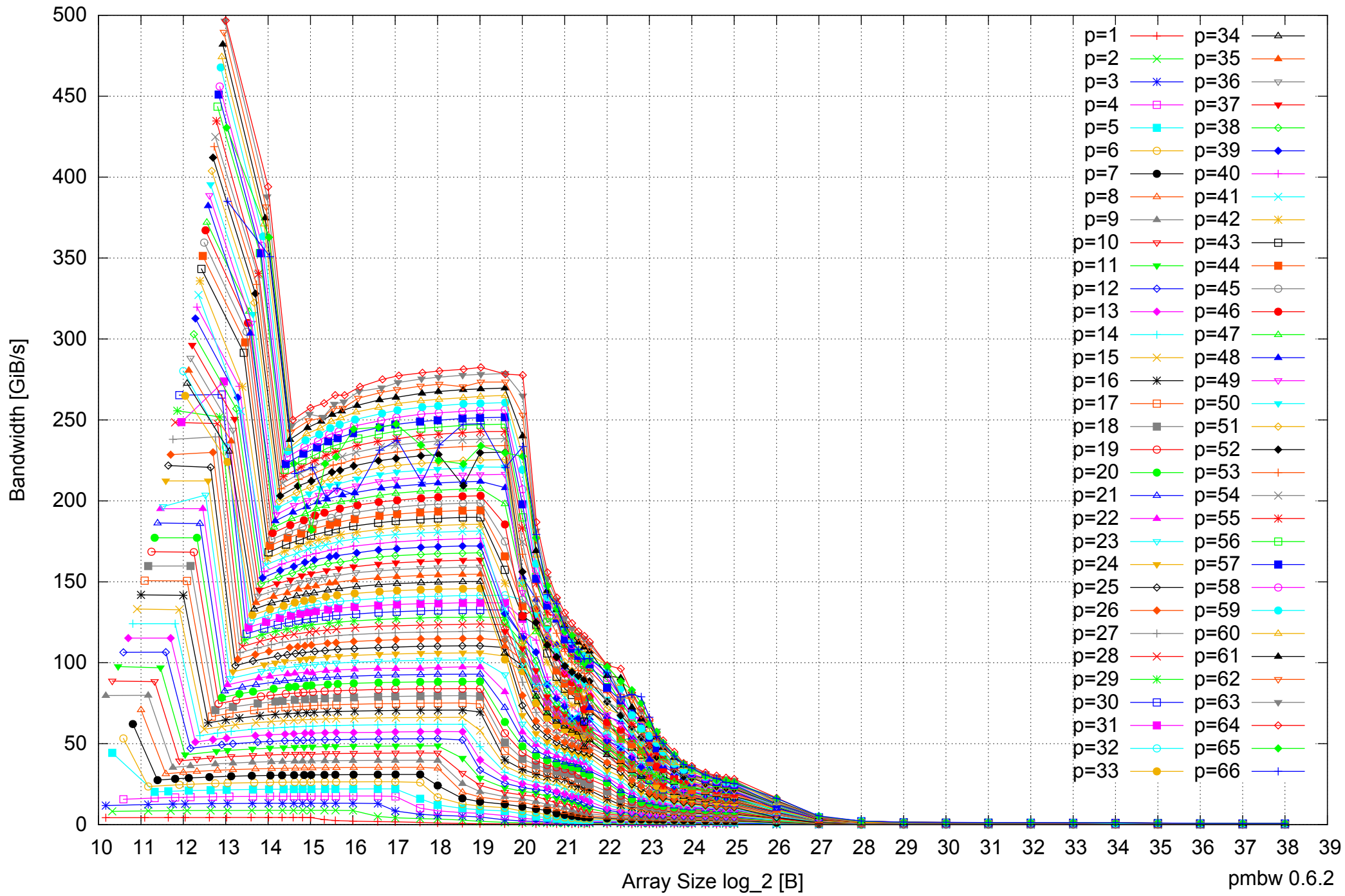
Intel Xeon E5-4640 512GB - Parallel Memory Bandwidth - PermRead64SimpleLoop
