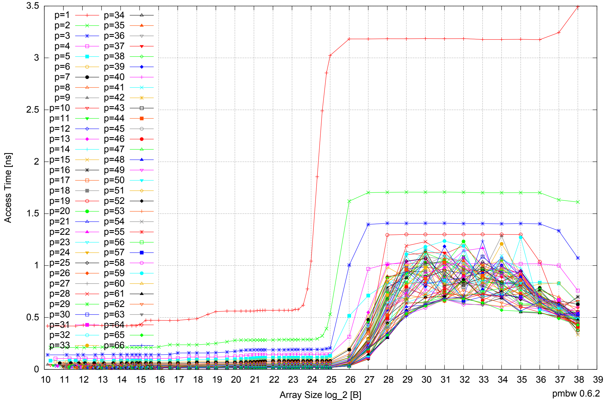
Intel Xeon E5-4640 512GB - Parallel Memory Access Time - ScanWrite64IndexUnrollLoop
