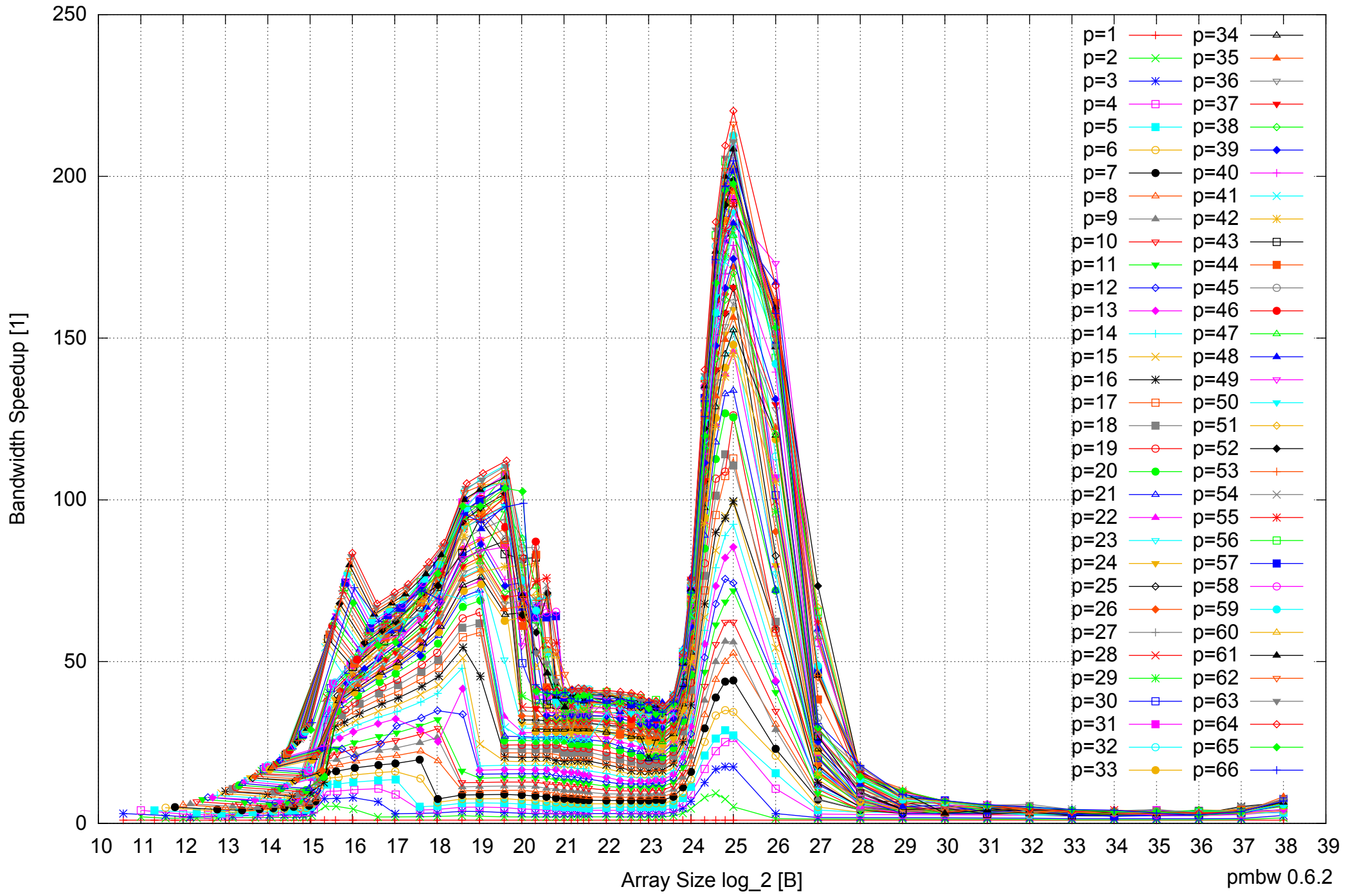
Intel Xeon E5-4640 512GB - Speedup of Parallel Memory Bandwidth - ScanRead256PtrSimpleLoop
