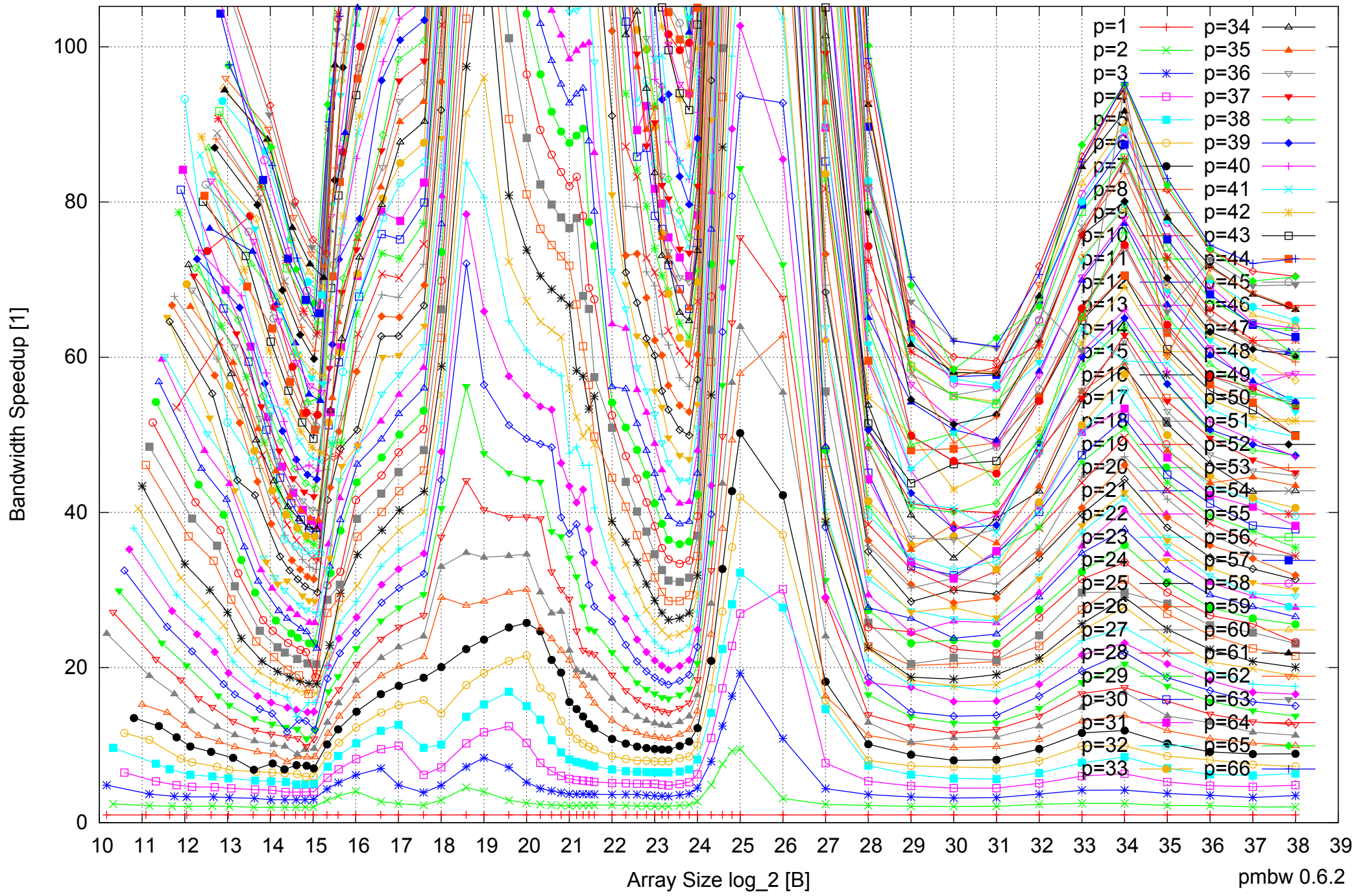
Intel Xeon E5-4640 512GB - Speedup of Parallel Memory Bandwidth (enlarged) - PermRead64UnrollLoop
