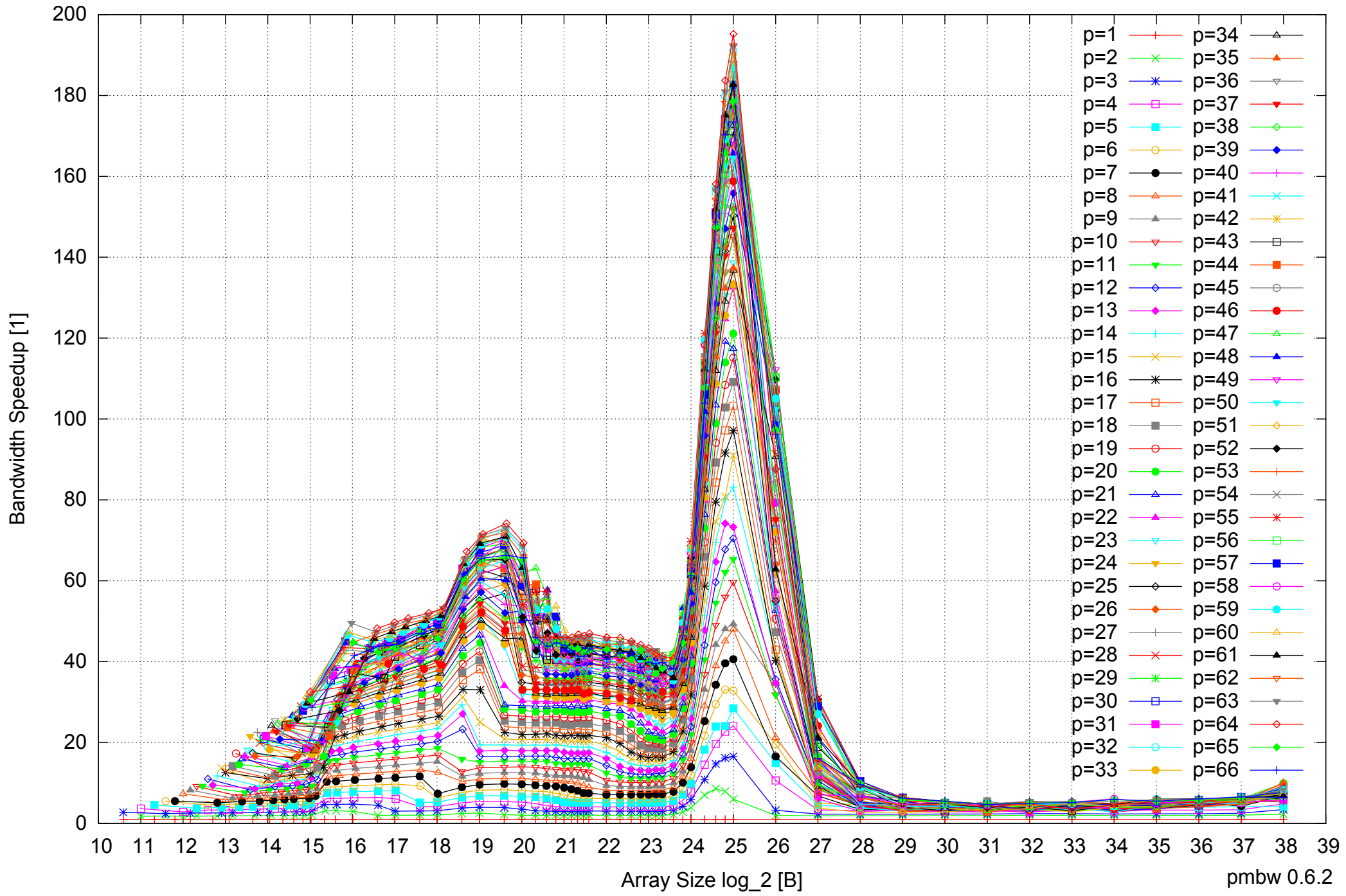
Intel Xeon E5-4640 512GB - Speedup of Parallel Memory Bandwidth - ScanWrite256PtrSimpleLoop
