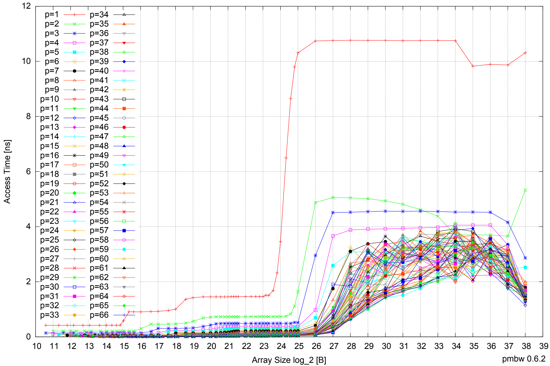
Intel Xeon E5-4640 512GB - Parallel Memory Access Time - ScanRead256PtrUnrollLoop
