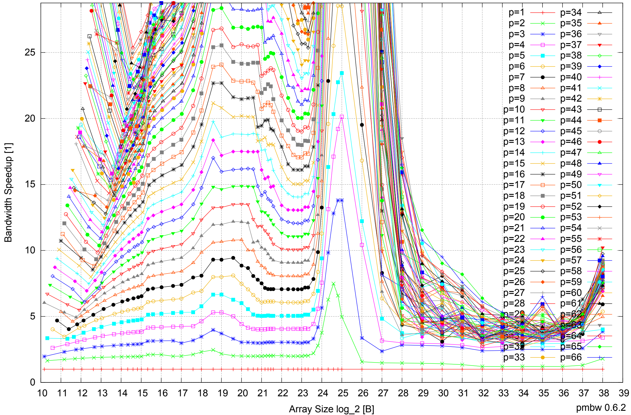
Intel Xeon E5-4640 512GB - Speedup of Parallel Memory Bandwidth (enlarged) - ScanRead64IndexSimpleLoop
