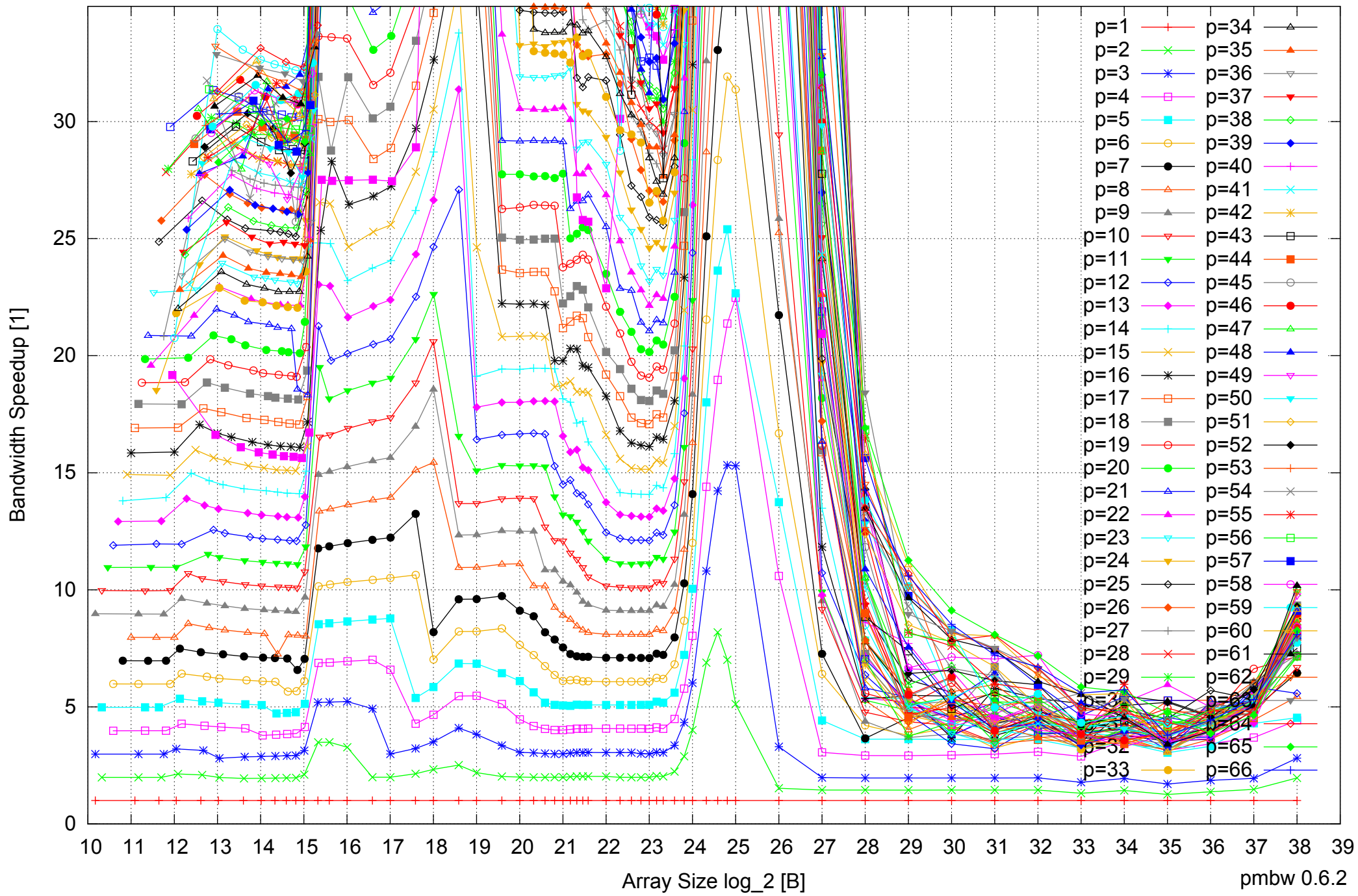
Intel Xeon E5-4640 512GB - Speedup of Parallel Memory Bandwidth (enlarged) - ScanRead64PtrUnrollLoop
