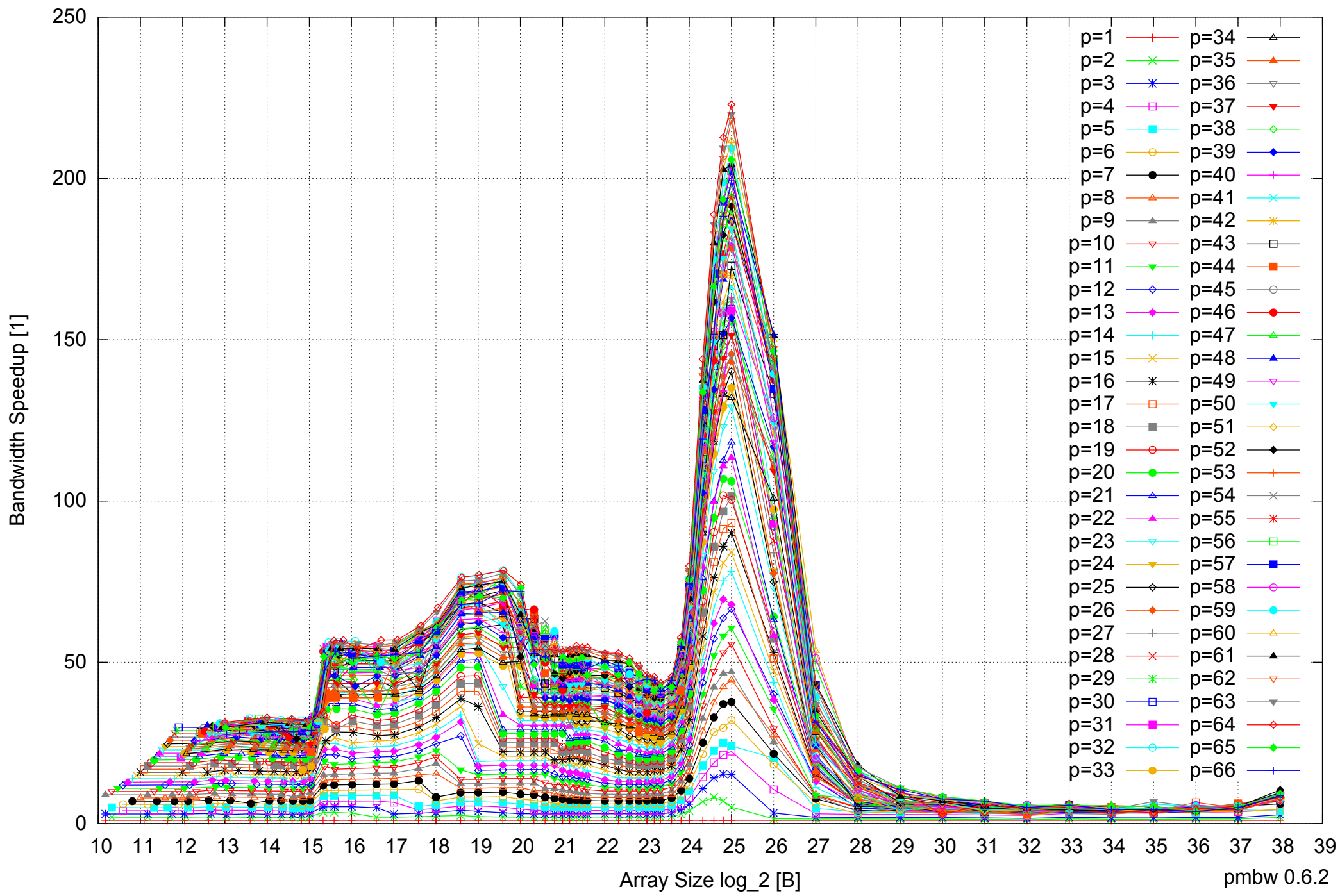
Intel Xeon E5-4640 512GB - Speedup of Parallel Memory Bandwidth - ScanRead64IndexUnrollLoop
