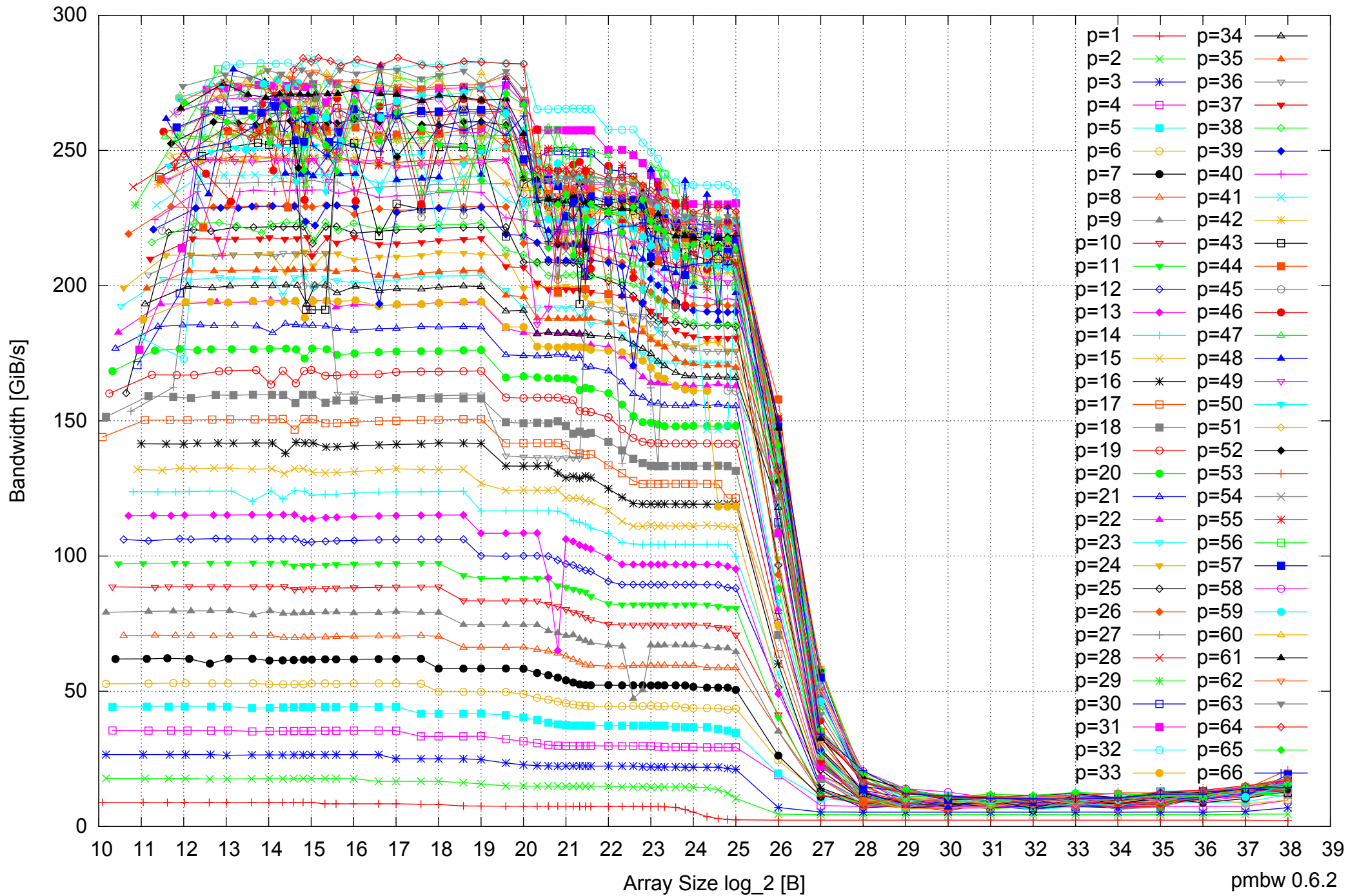
Intel Xeon E5-4640 512GB - Parallel Memory Bandwidth - ScanWrite32PtrUnrollLoop
