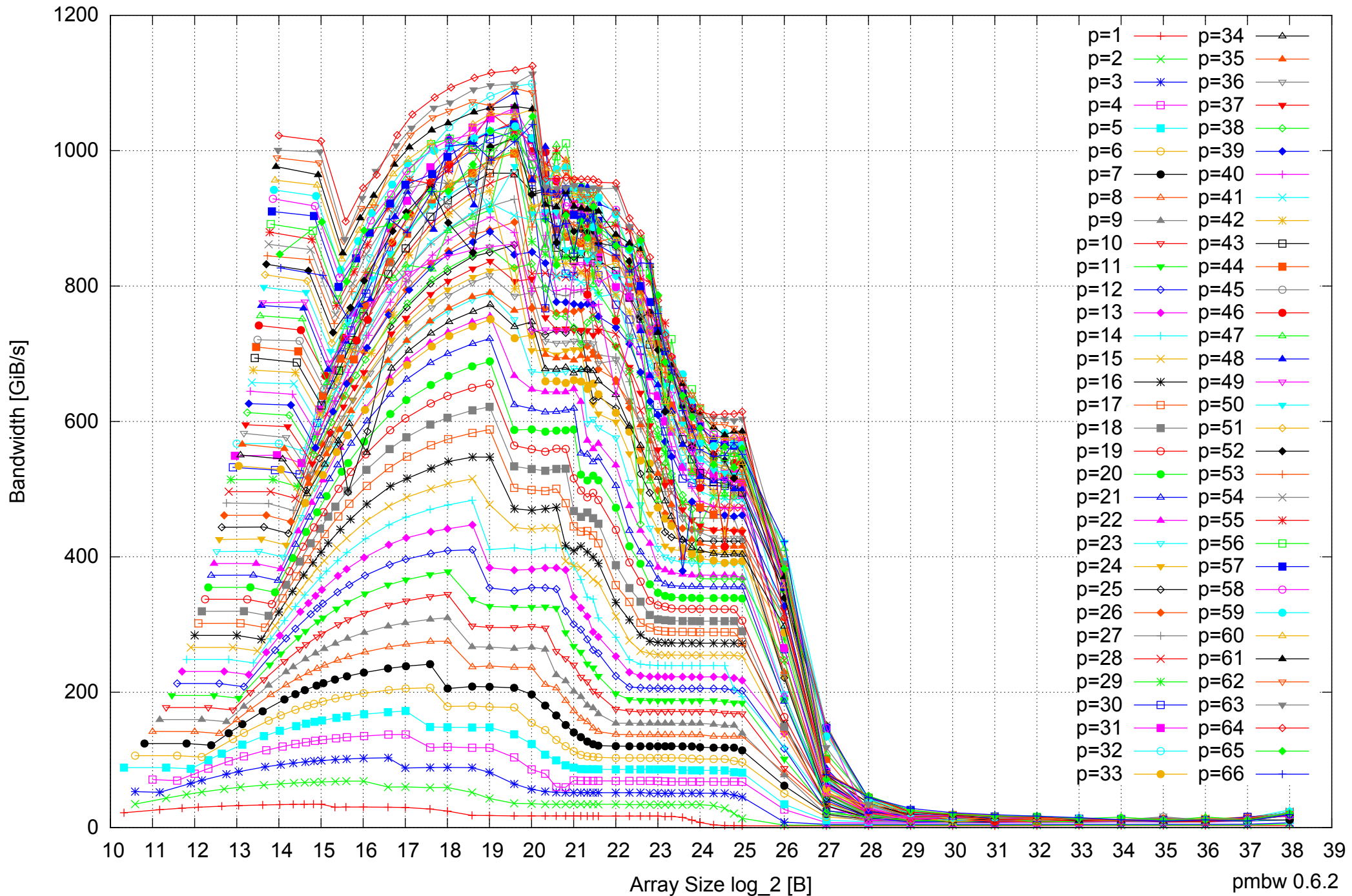
Intel Xeon E5-4640 512GB - Parallel Memory Bandwidth - ScanRead128PtrSimpleLoop
