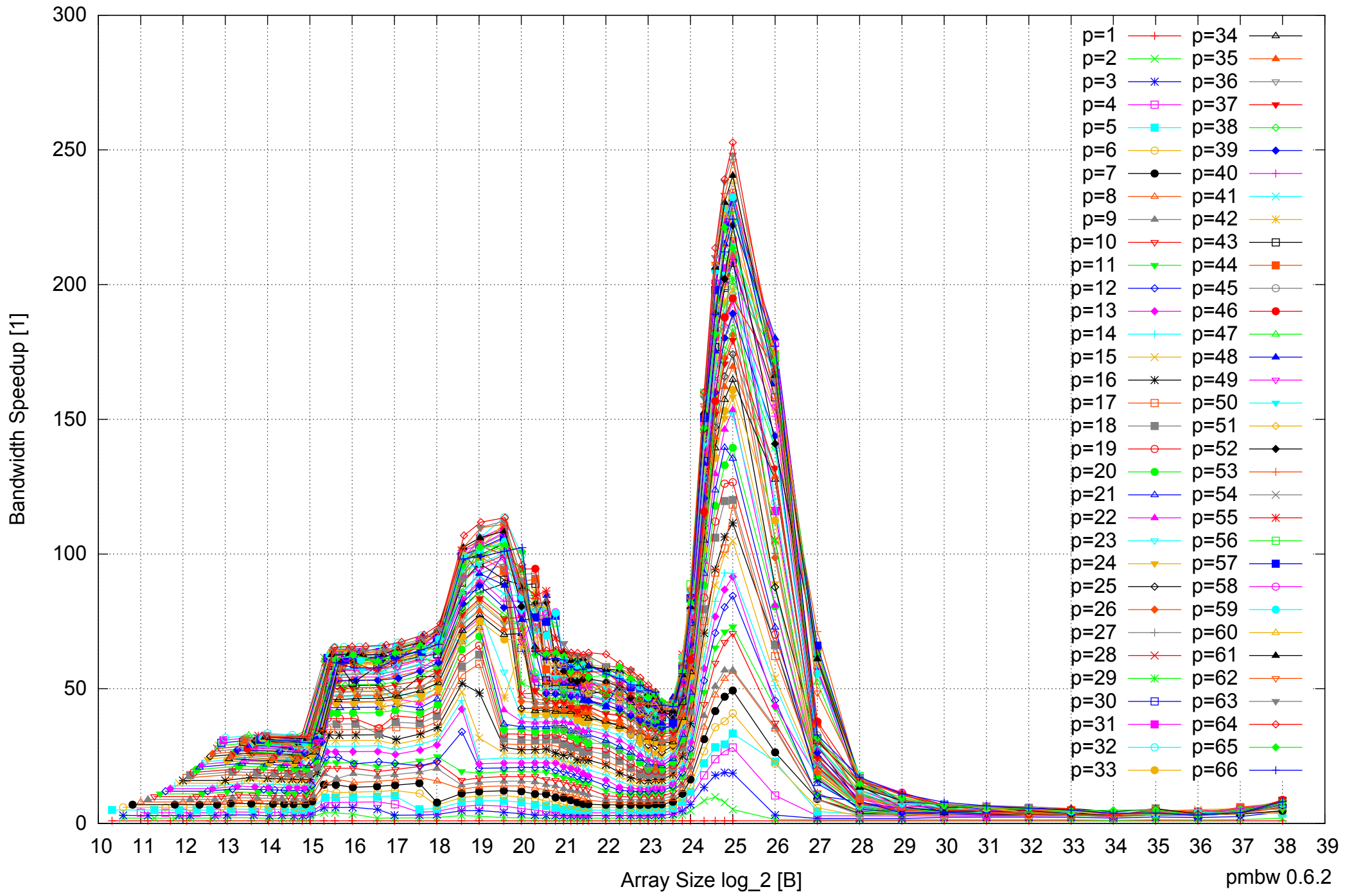
Intel Xeon E5-4640 512GB - Speedup of Parallel Memory Bandwidth - ScanRead128PtrUnrollLoop
