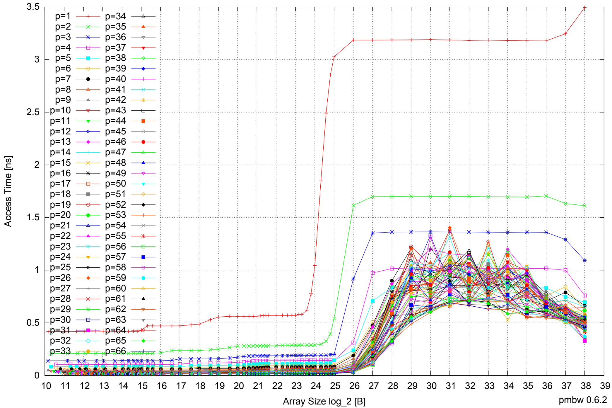
Intel Xeon E5-4640 512GB - Parallel Memory Access Time - ScanWrite64PtrUnrollLoop
