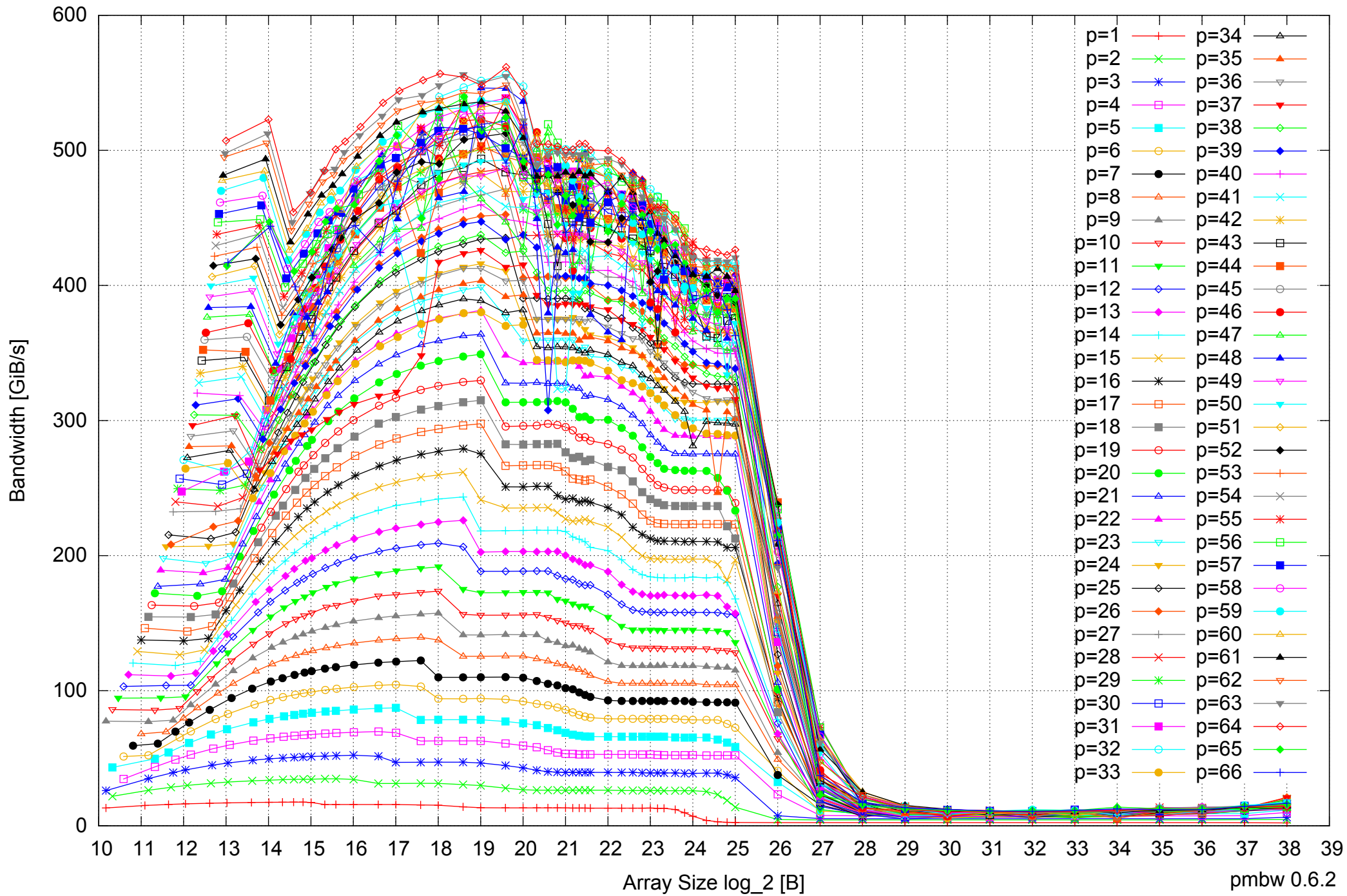
Intel Xeon E5-4640 512GB - Parallel Memory Bandwidth - ScanWrite64PtrSimpleLoop
