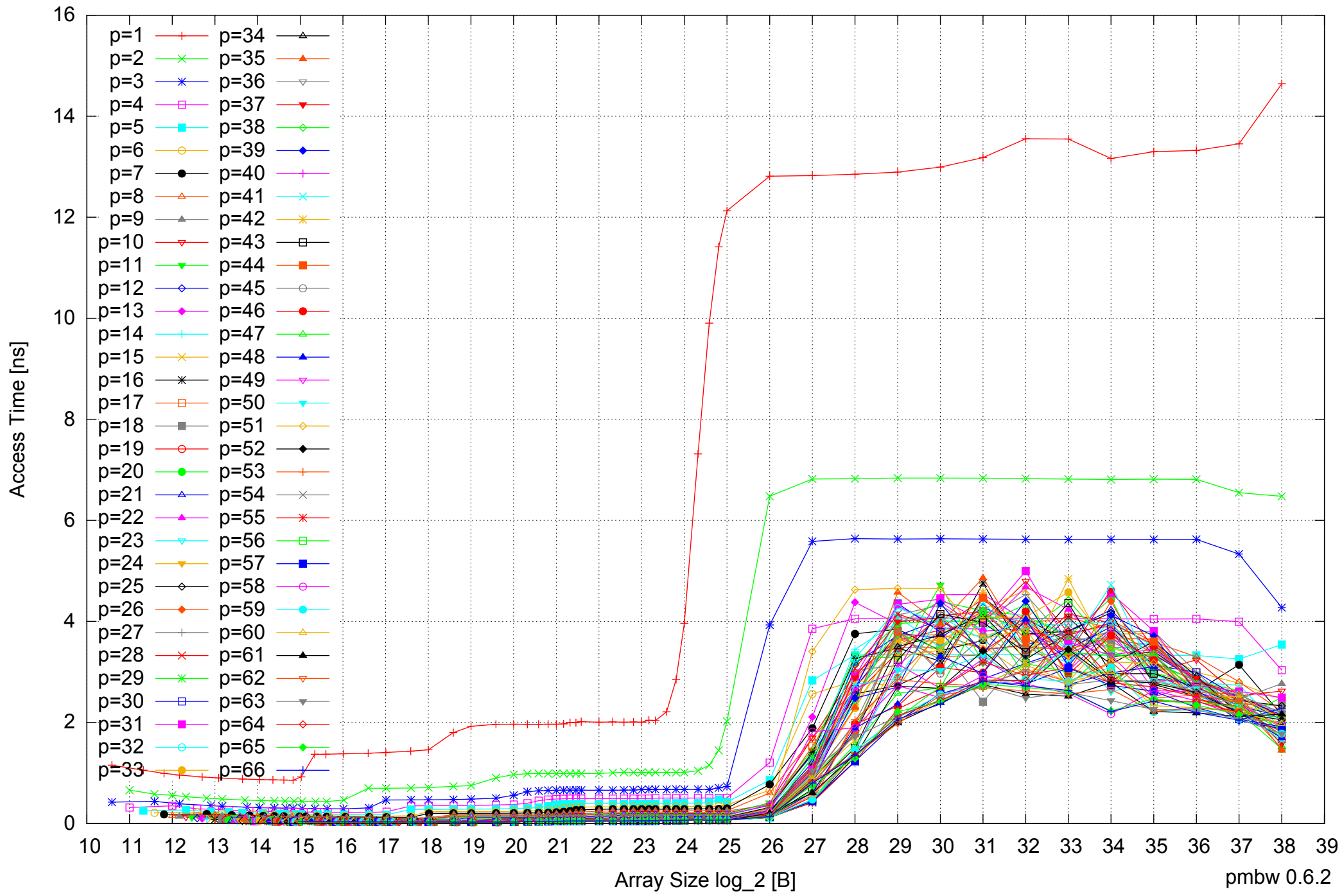
Intel Xeon E5-4640 512GB - Parallel Memory Access Time - ScanWrite256PtrSimpleLoop
