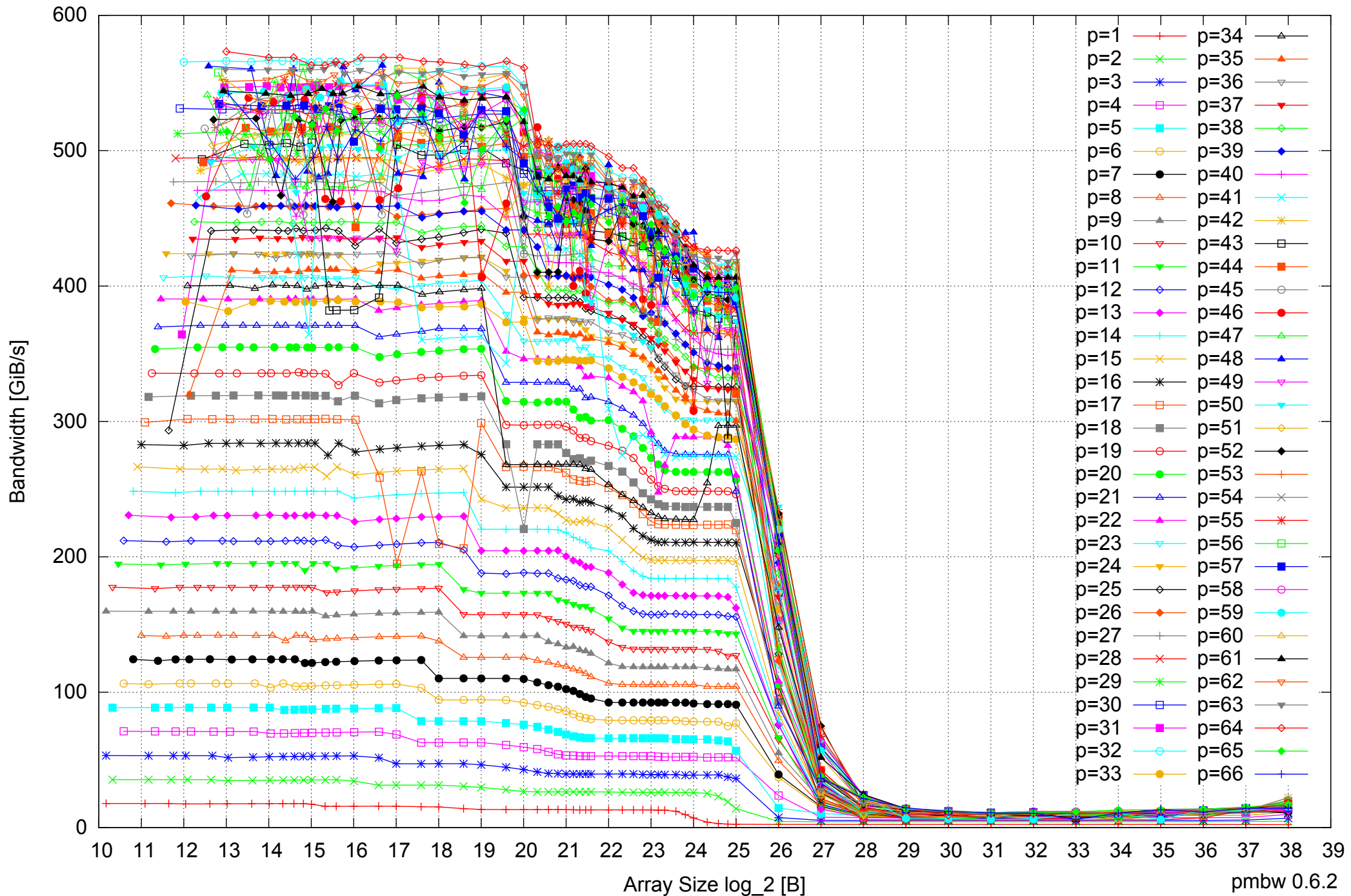
Intel Xeon E5-4640 512GB - Parallel Memory Bandwidth - ScanWrite64IndexUnrollLoop
