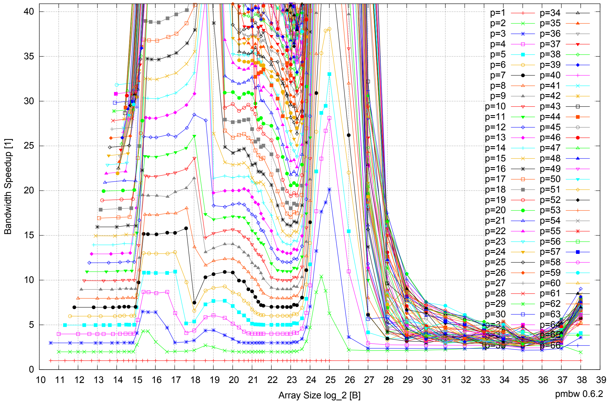
Intel Xeon E5-4640 512GB - Speedup of Parallel Memory Bandwidth (enlarged) - ScanRead256PtrUnrollLoop
