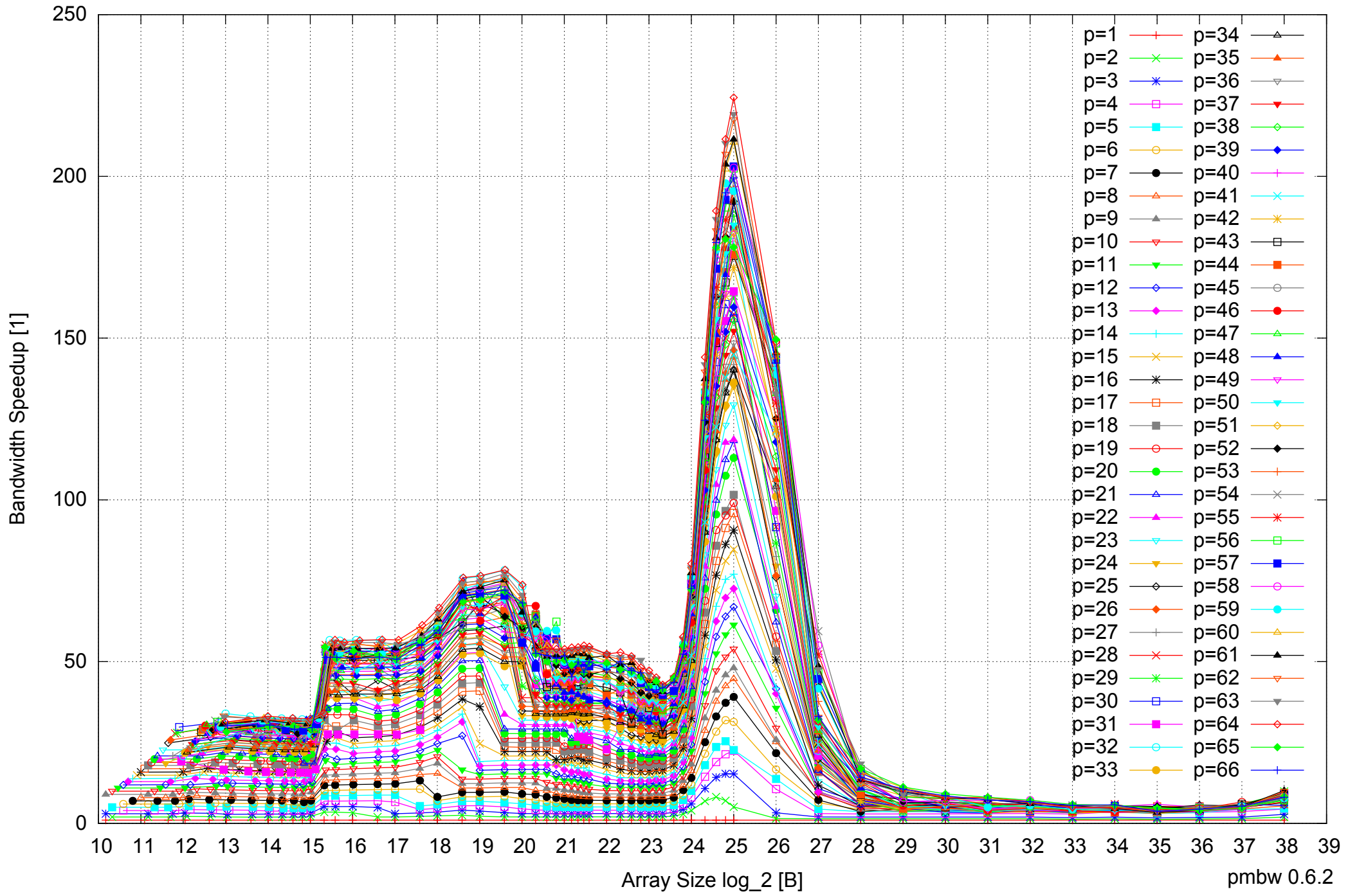
Intel Xeon E5-4640 512GB - Speedup of Parallel Memory Bandwidth - ScanRead64PtrUnrollLoop
