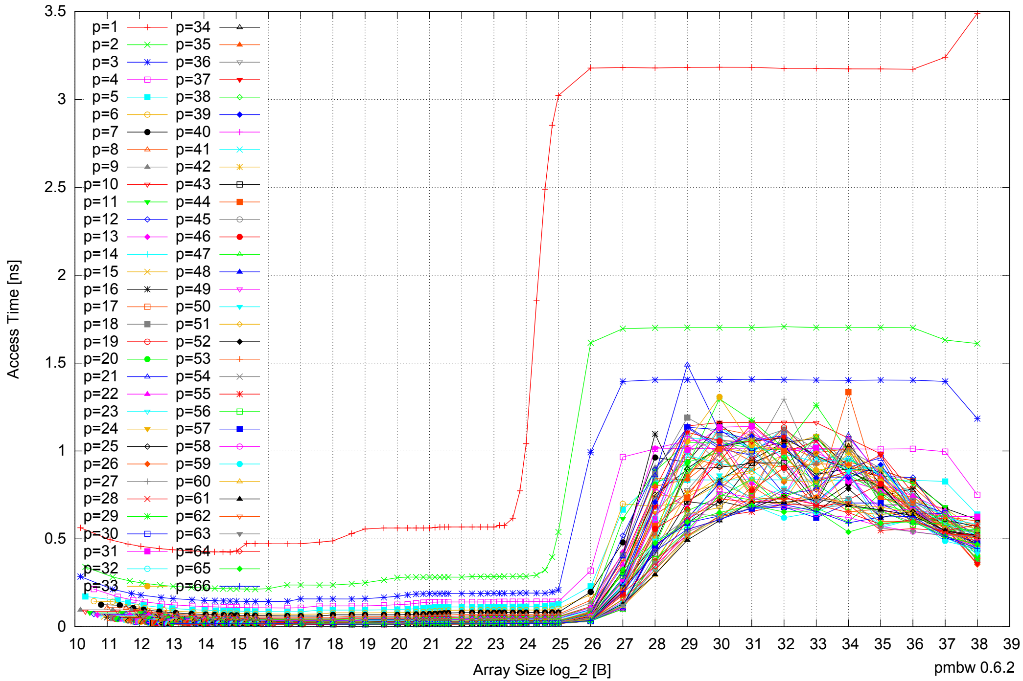
Intel Xeon E5-4640 512GB - Parallel Memory Access Time - ScanWrite64PtrSimpleLoop
