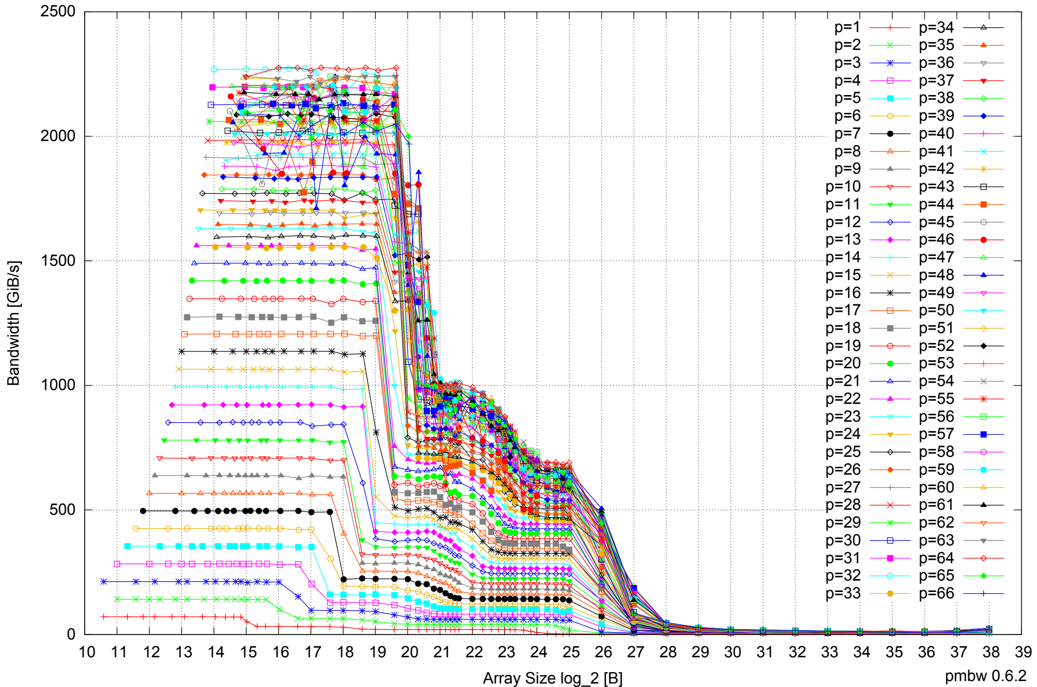
Intel Xeon E5-4640 512GB - Parallel Memory Bandwidth - ScanRead256PtrUnrollLoop
