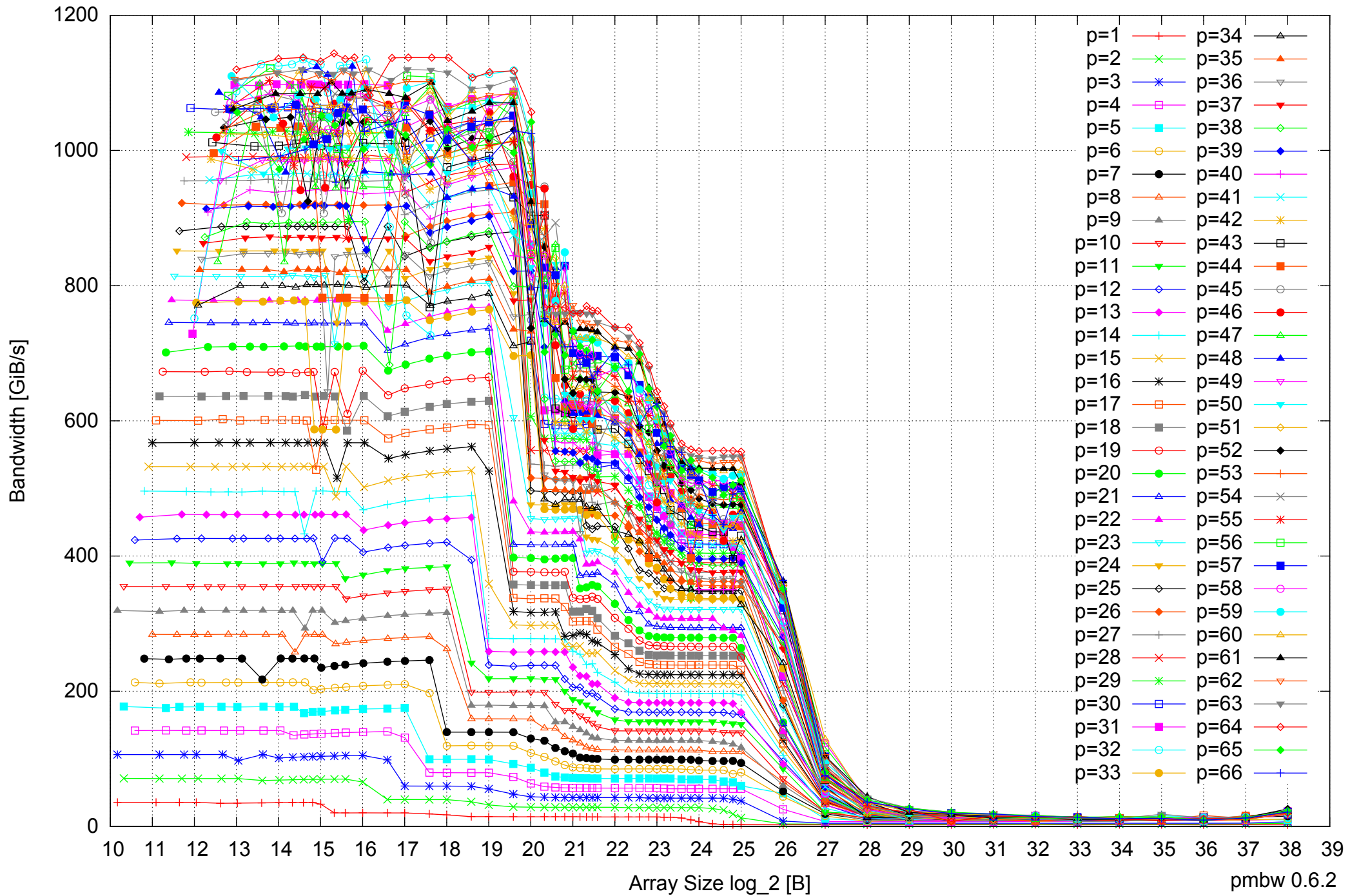
Intel Xeon E5-4640 512GB - Parallel Memory Bandwidth - ScanRead64IndexUnrollLoop
