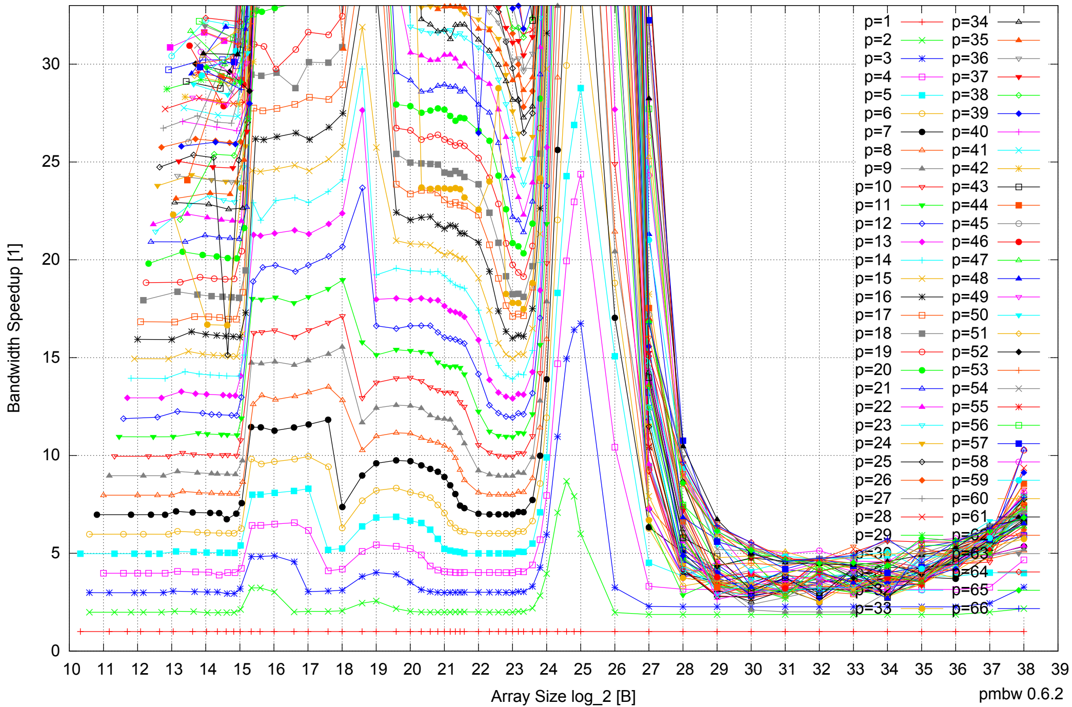
Intel Xeon E5-4640 512GB - Speedup of Parallel Memory Bandwidth (enlarged) - ScanWrite128PtrUnrollLoop
