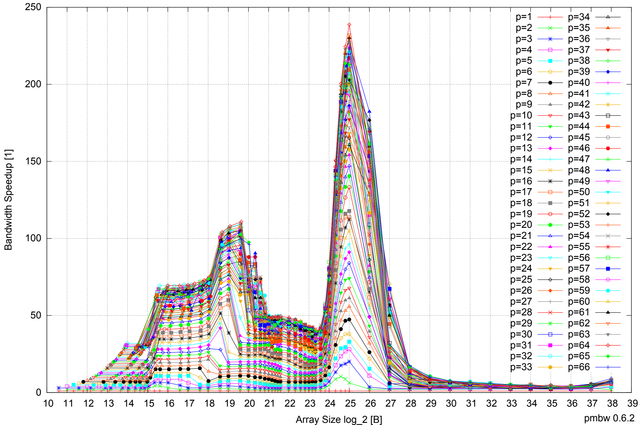
Intel Xeon E5-4640 512GB - Speedup of Parallel Memory Bandwidth - ScanRead256PtrUnrollLoop
