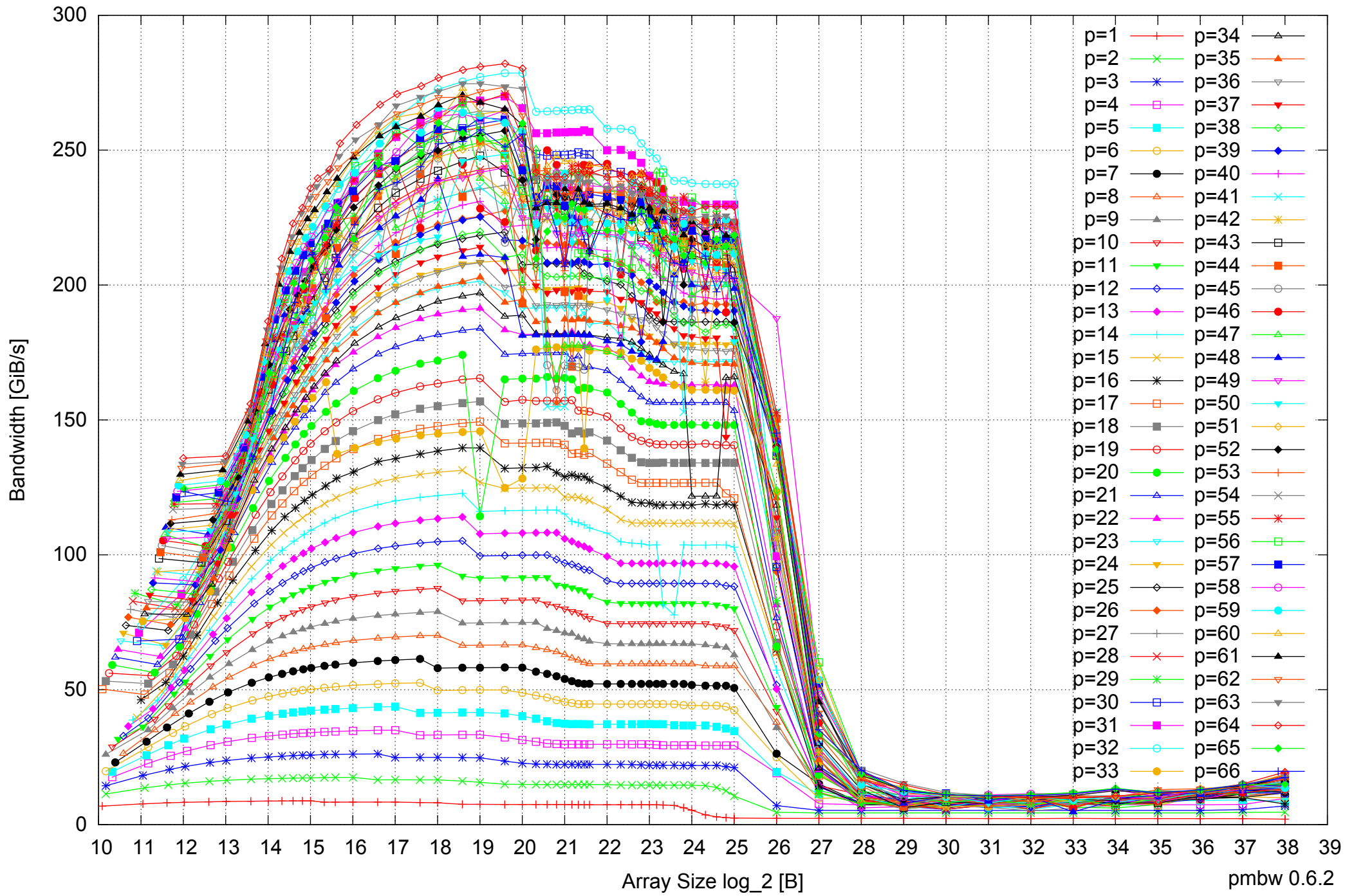
Intel Xeon E5-4640 512GB - Parallel Memory Bandwidth - ScanWrite32PtrSimpleLoop
