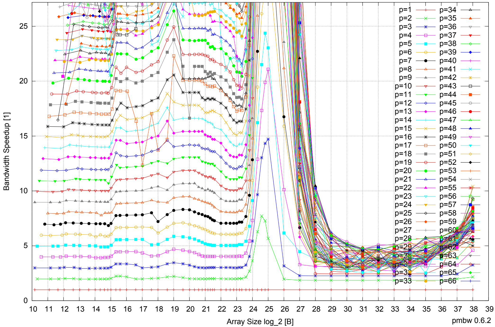
Intel Xeon E5-4640 512GB - Speedup of Parallel Memory Bandwidth (enlarged) - ScanWrite64IndexUnrollLoop
