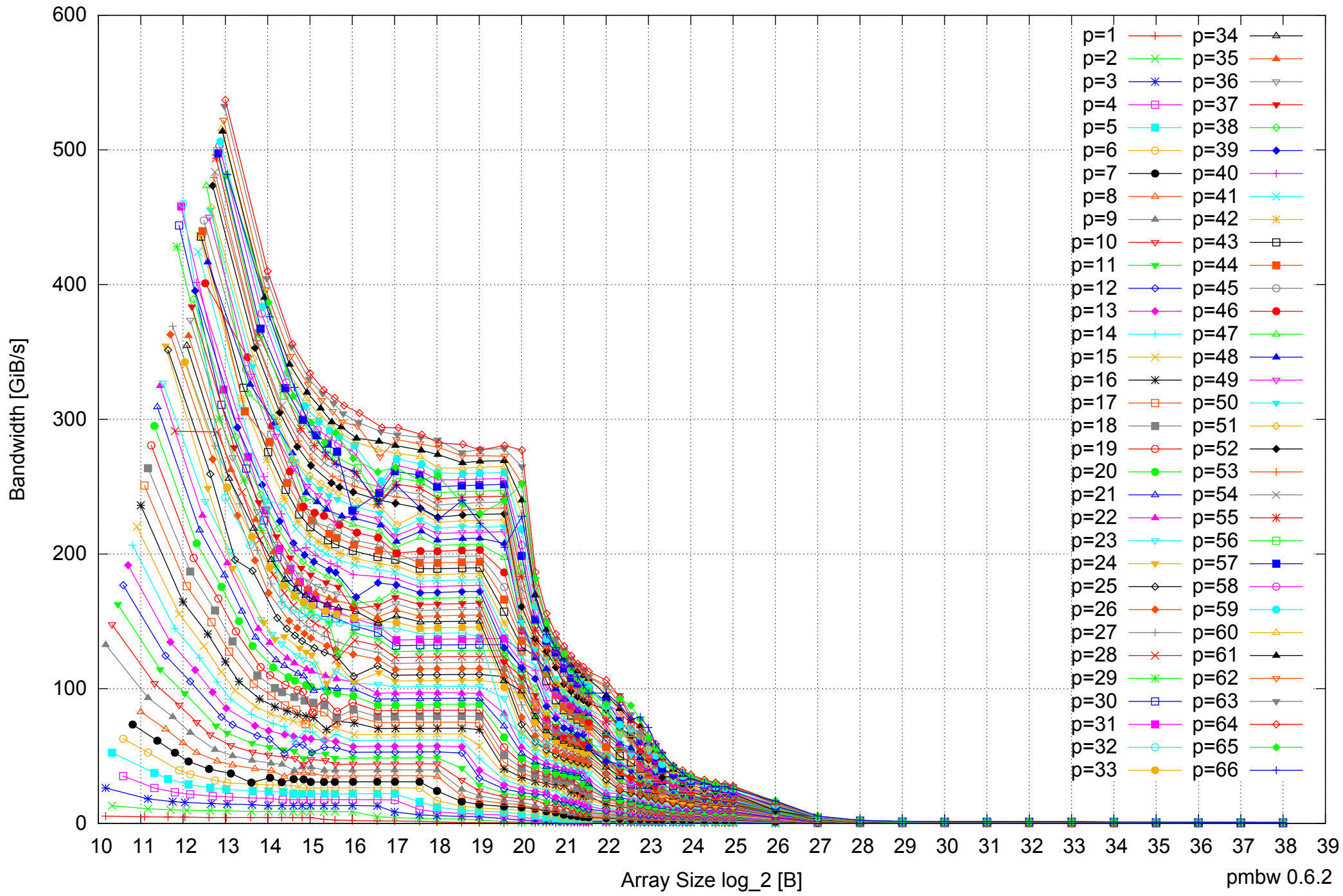
Intel Xeon E5-4640 512GB - Parallel Memory Bandwidth - PermRead64UnrollLoop
