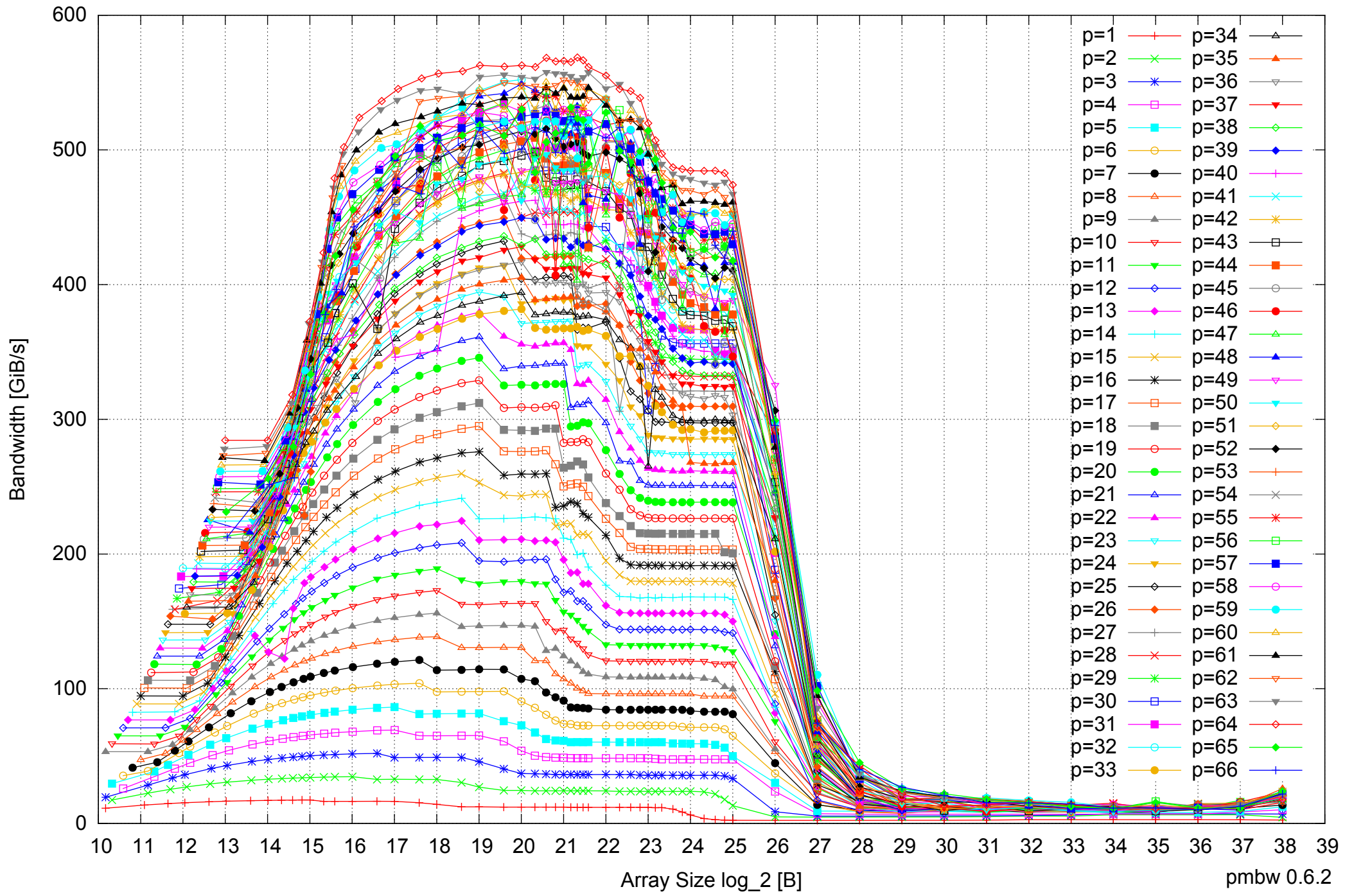
Intel Xeon E5-4640 512GB - Parallel Memory Bandwidth - ScanRead64PtrSimpleLoop
