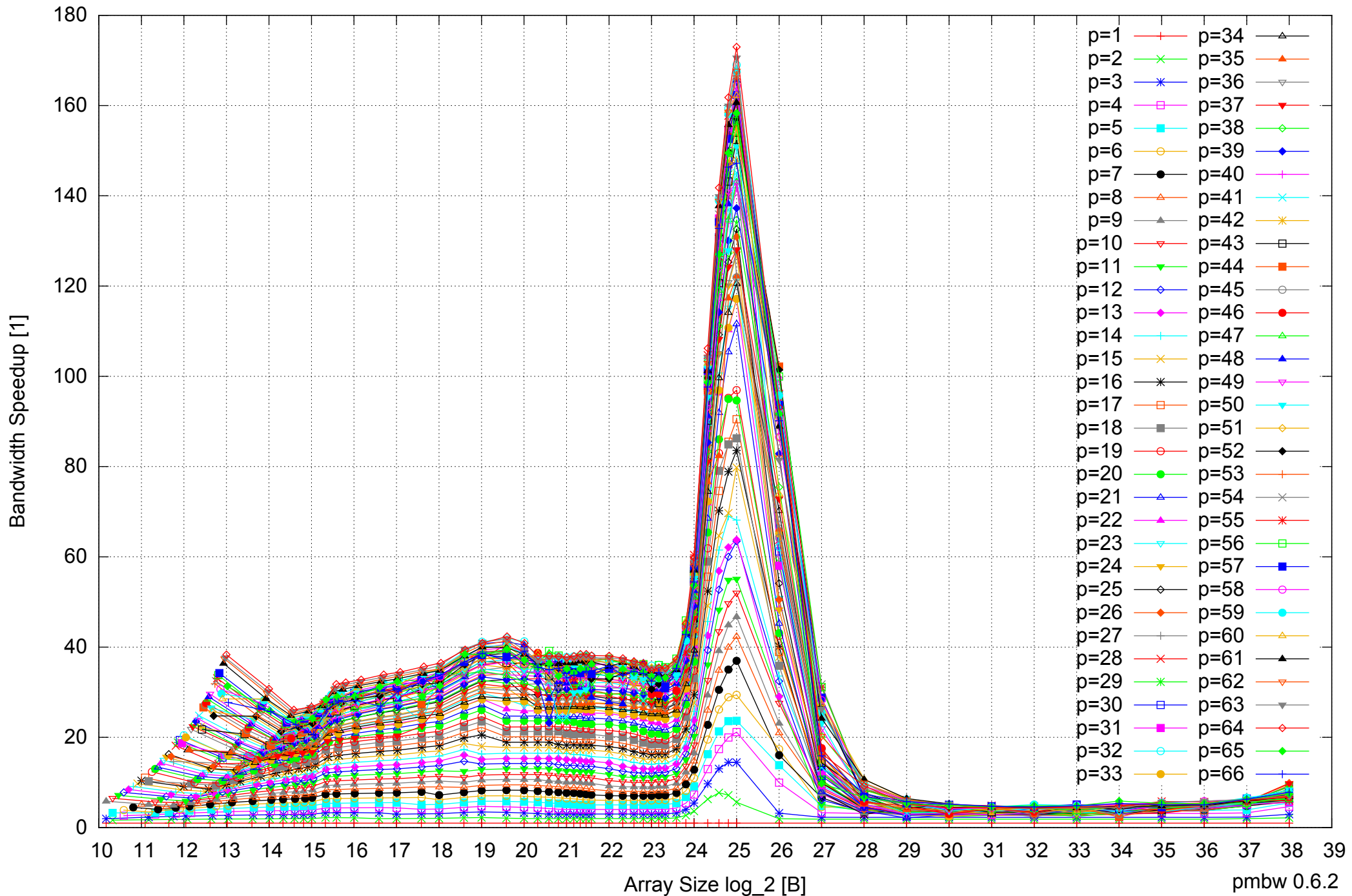
Intel Xeon E5-4640 512GB - Speedup of Parallel Memory Bandwidth - ScanWrite64PtrSimpleLoop
