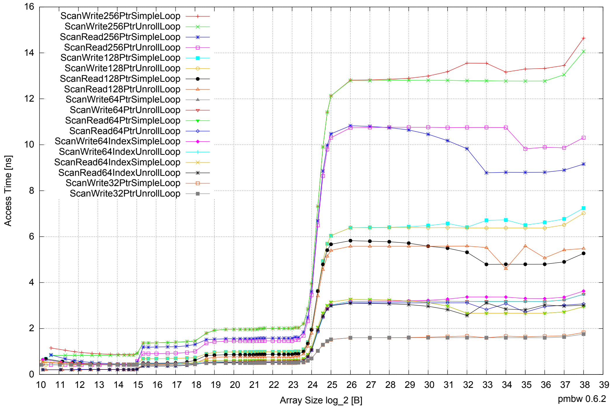
Intel Xeon E5-4640 512GB - One Thread Memory Latency (excluding Permutation)
