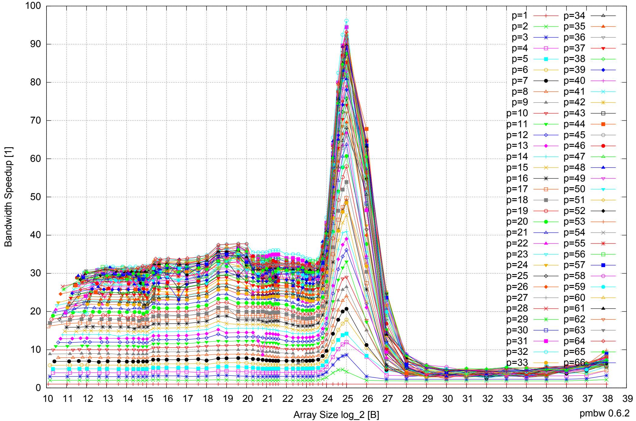
Intel Xeon E5-4640 512GB - Speedup of Parallel Memory Bandwidth - ScanWrite32PtrUnrollLoop
