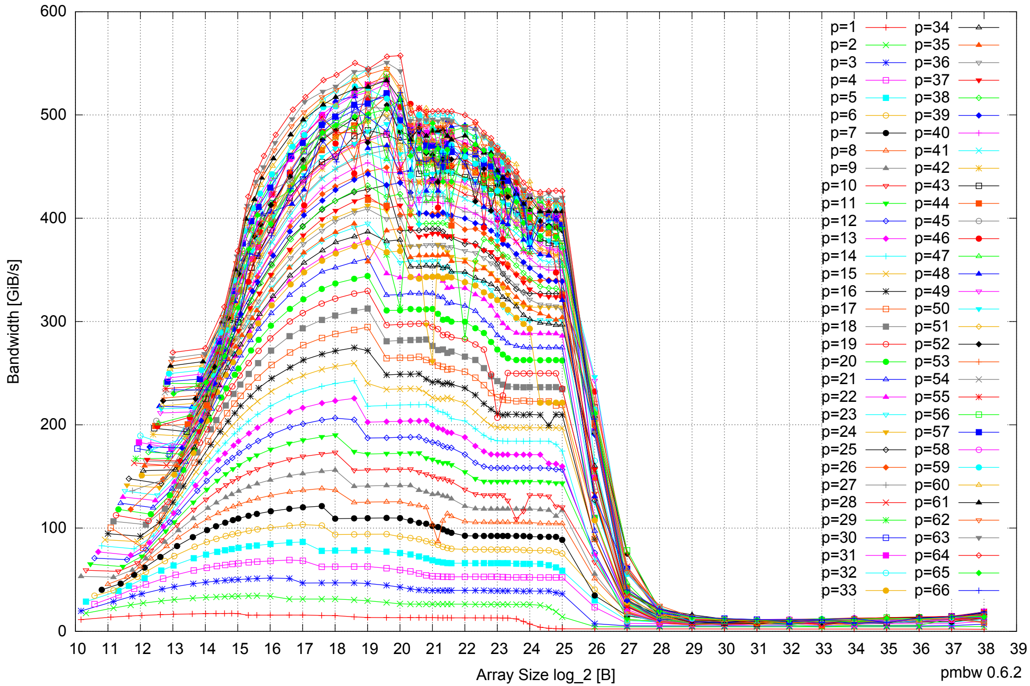
Intel Xeon E5-4640 512GB - Parallel Memory Bandwidth - ScanWrite64IndexSimpleLoop
