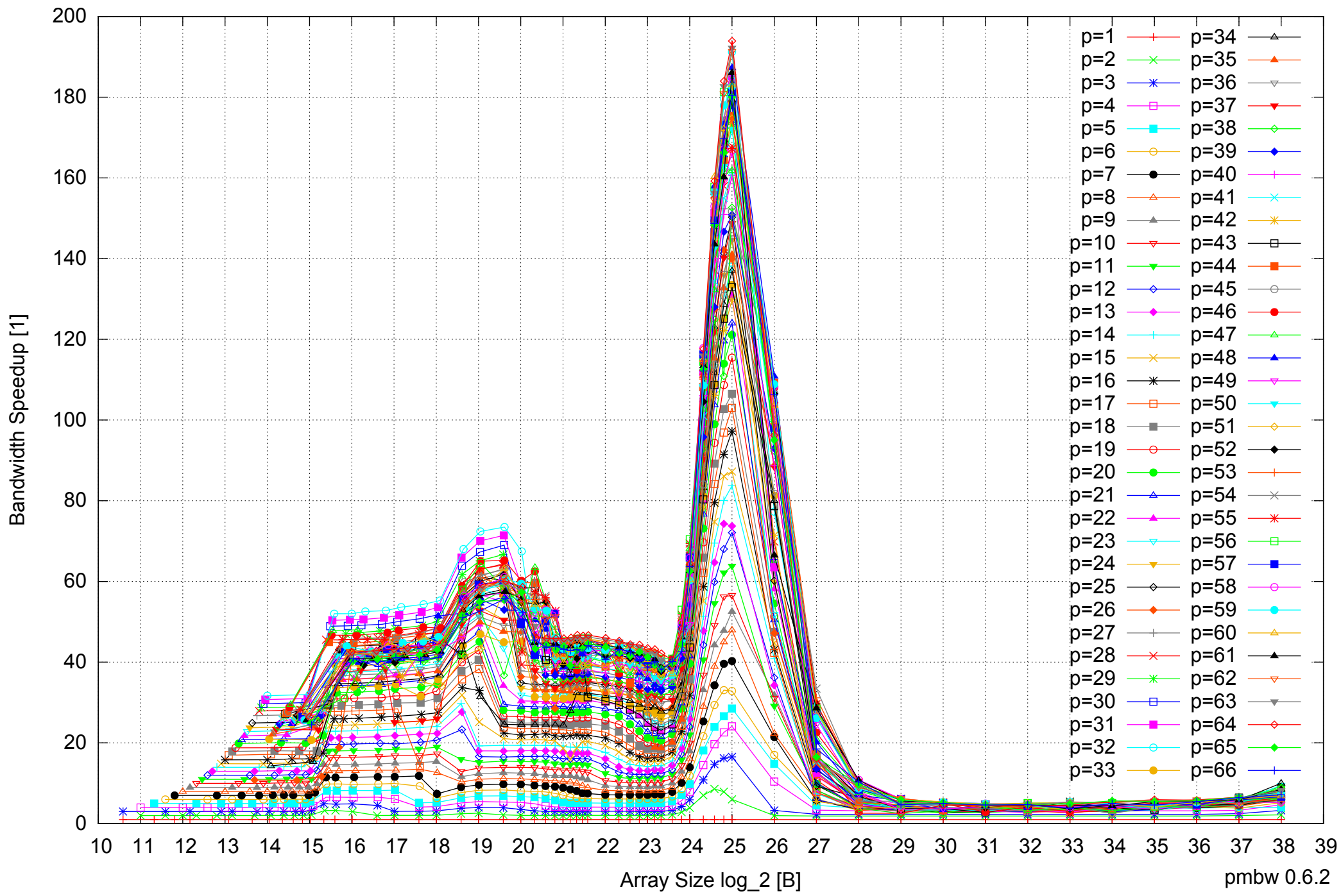
Intel Xeon E5-4640 512GB - Speedup of Parallel Memory Bandwidth - ScanWrite256PtrUnrollLoop
