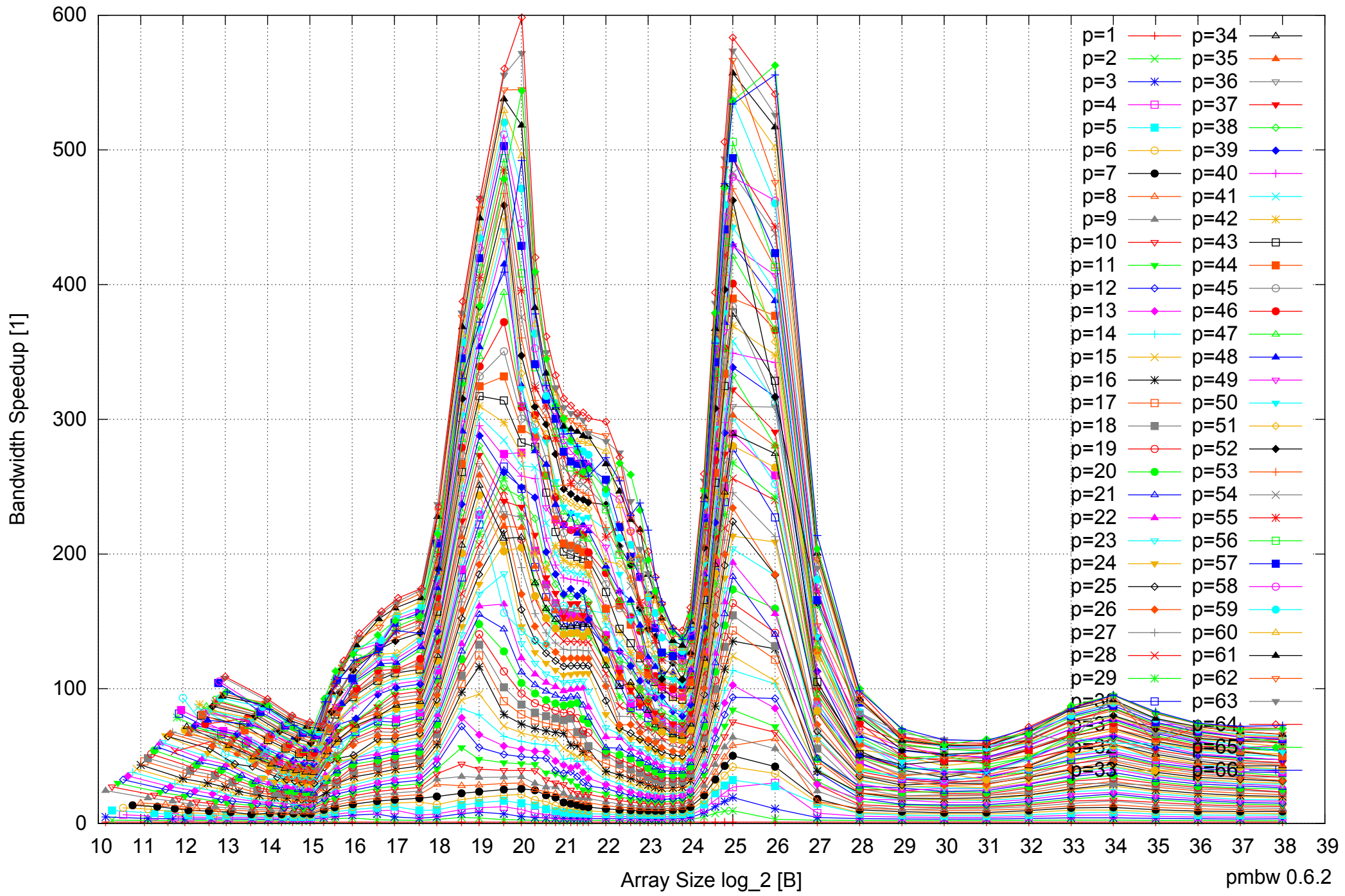
Intel Xeon E5-4640 512GB - Speedup of Parallel Memory Bandwidth - PermRead64UnrollLoop
