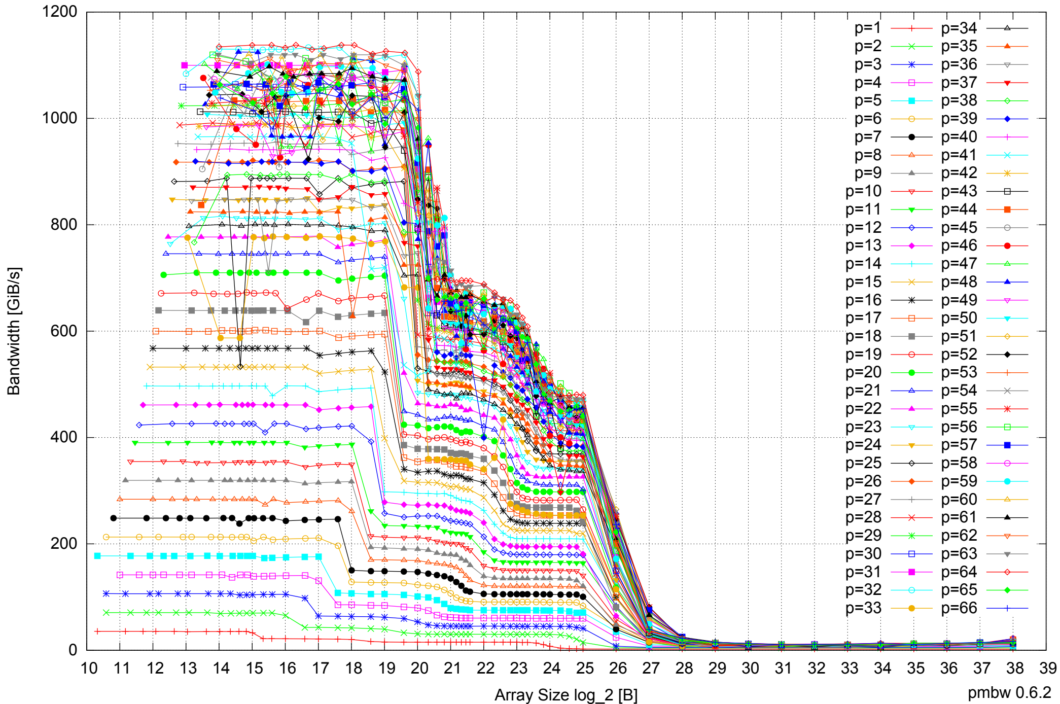
Intel Xeon E5-4640 512GB - Parallel Memory Bandwidth - ScanWrite128PtrUnrollLoop
