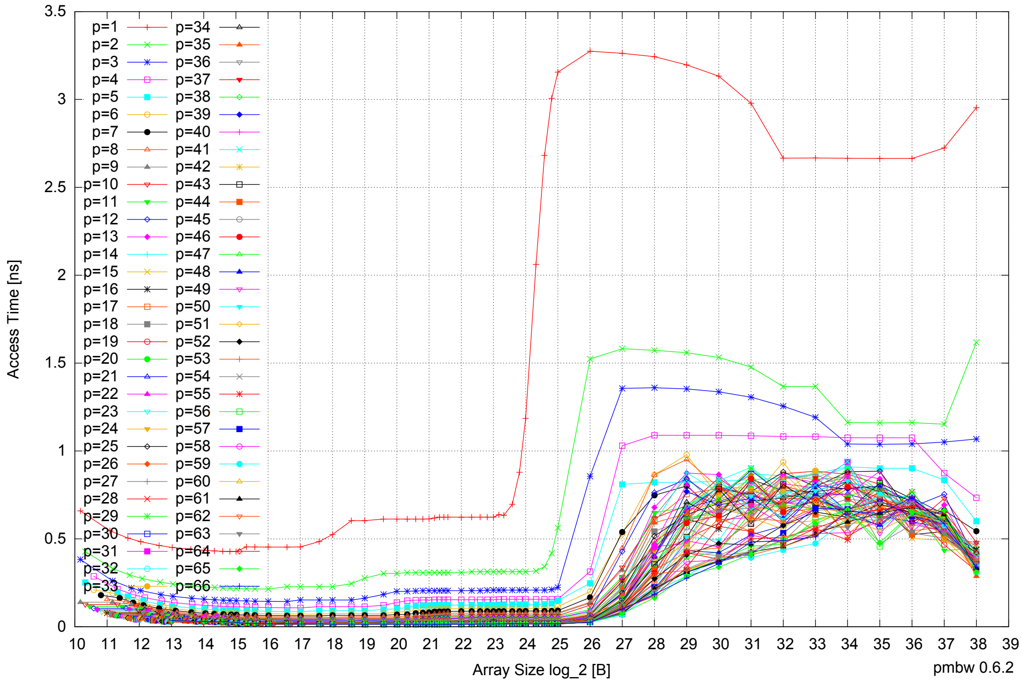
Intel Xeon E5-4640 512GB - Parallel Memory Access Time - ScanRead64PtrSimpleLoop
