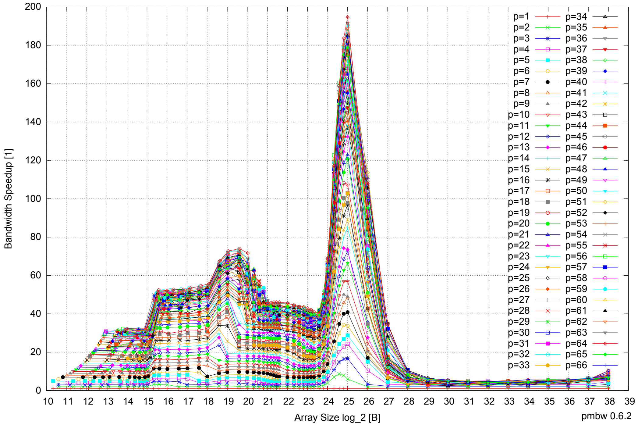
Intel Xeon E5-4640 512GB - Speedup of Parallel Memory Bandwidth - ScanWrite128PtrUnrollLoop
