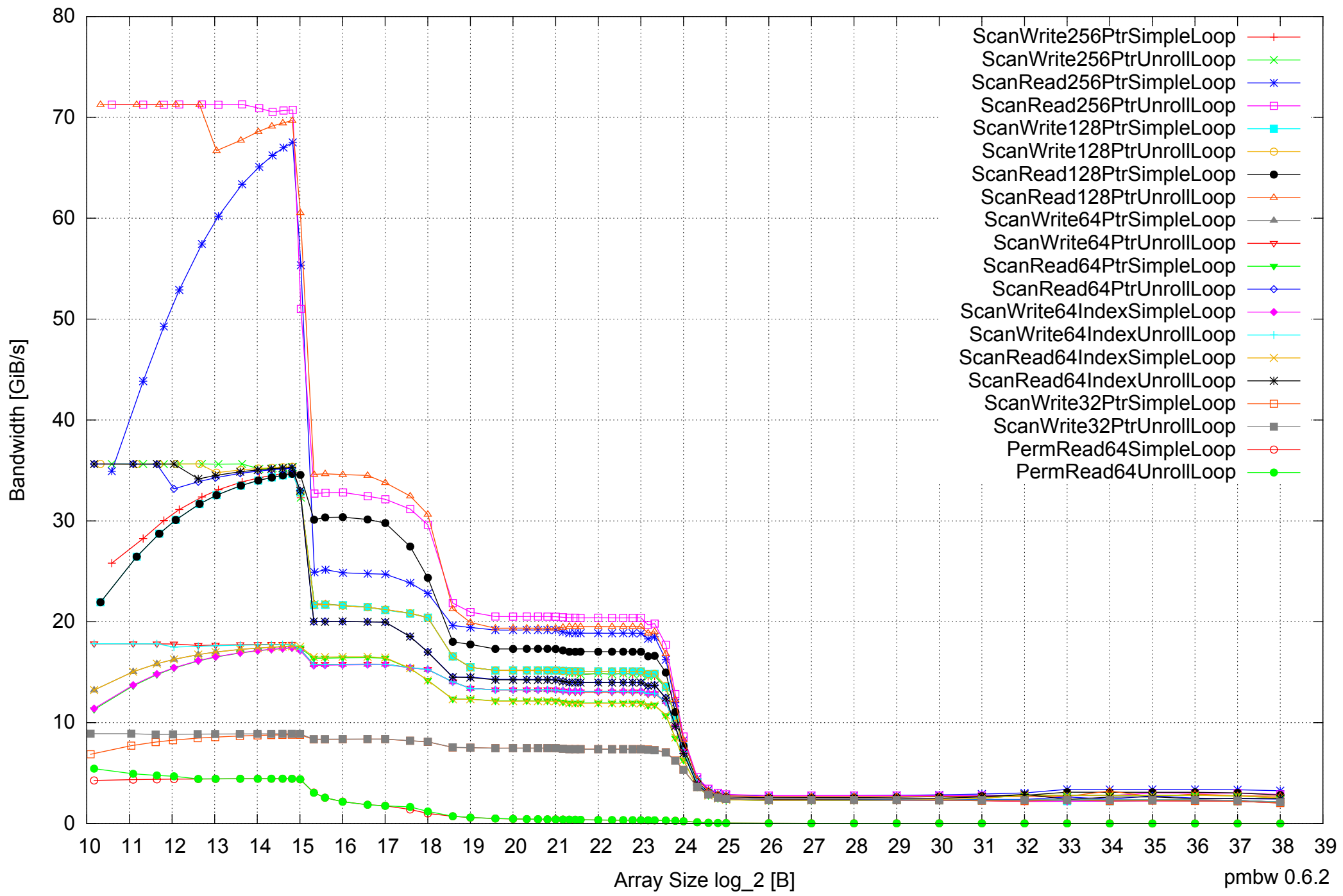
Intel Xeon E5-4640 512GB - One Thread Memory Bandwidth
