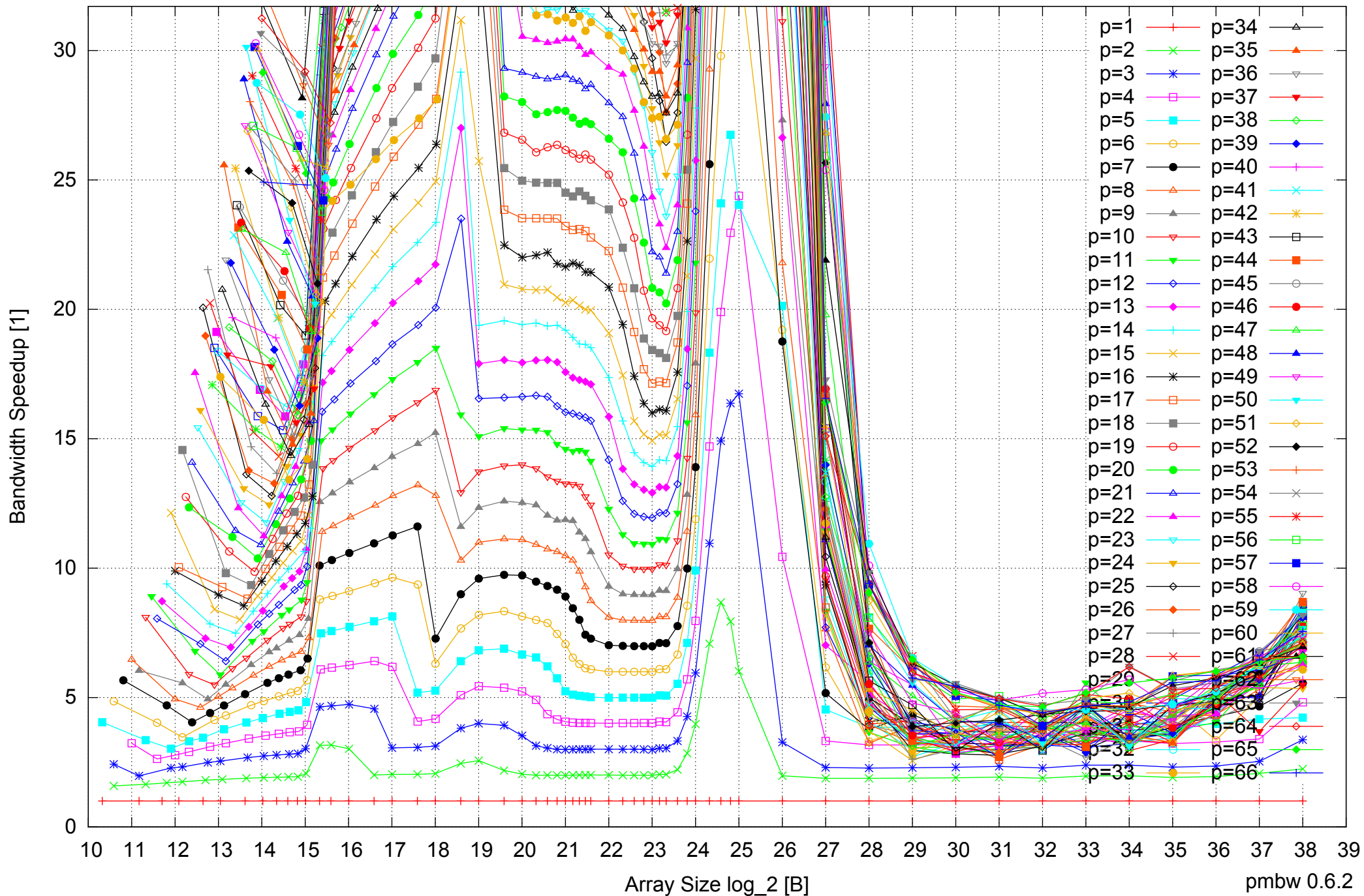
Intel Xeon E5-4640 512GB - Speedup of Parallel Memory Bandwidth (enlarged) - ScanWrite128PtrSimpleLoop
