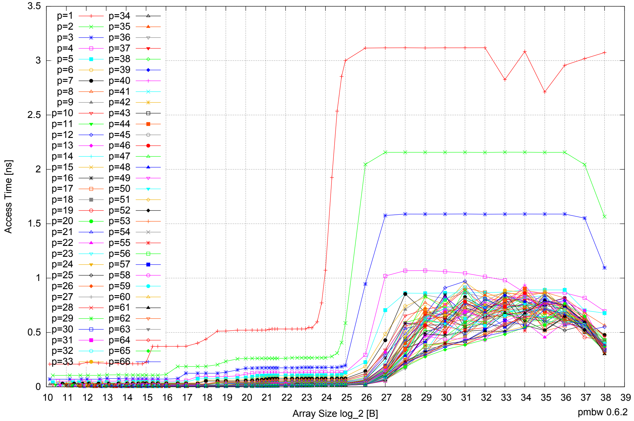
Intel Xeon E5-4640 512GB - Parallel Memory Access Time - ScanRead64PtrUnrollLoop
