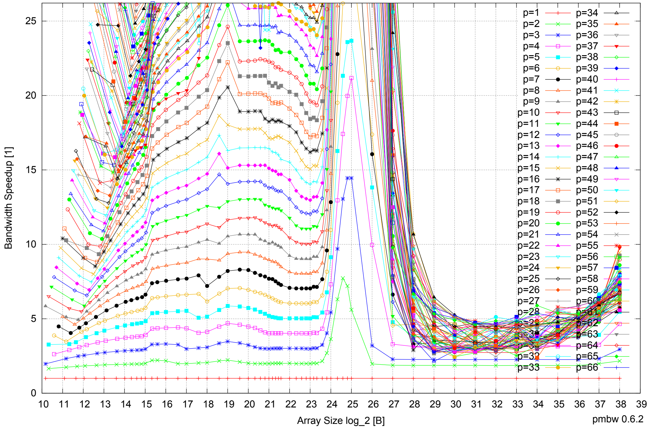
Intel Xeon E5-4640 512GB - Speedup of Parallel Memory Bandwidth (enlarged) - ScanWrite64PtrSimpleLoop
