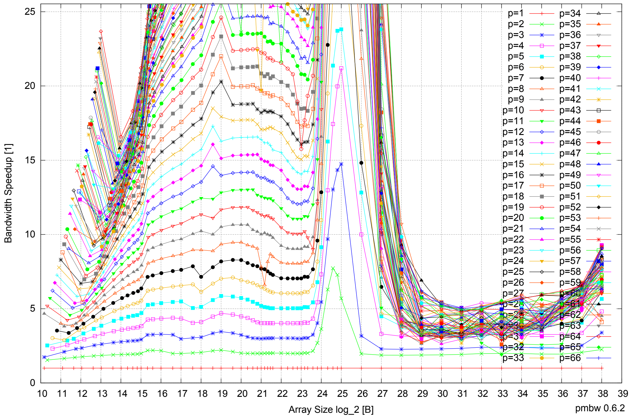
Intel Xeon E5-4640 512GB - Speedup of Parallel Memory Bandwidth (enlarged) - ScanWrite64IndexSimpleLoop
