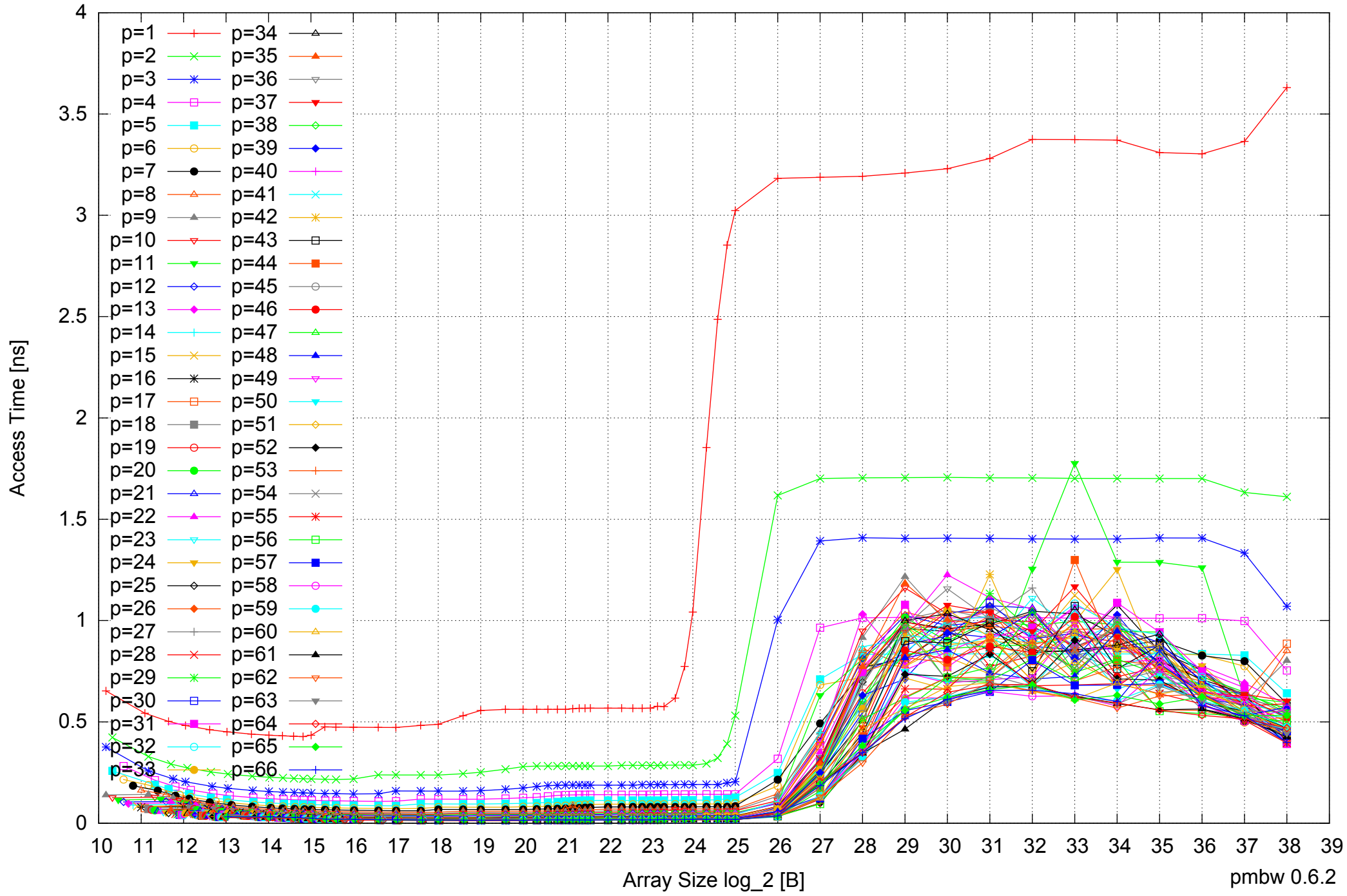
Intel Xeon E5-4640 512GB - Parallel Memory Access Time - ScanWrite64IndexSimpleLoop
