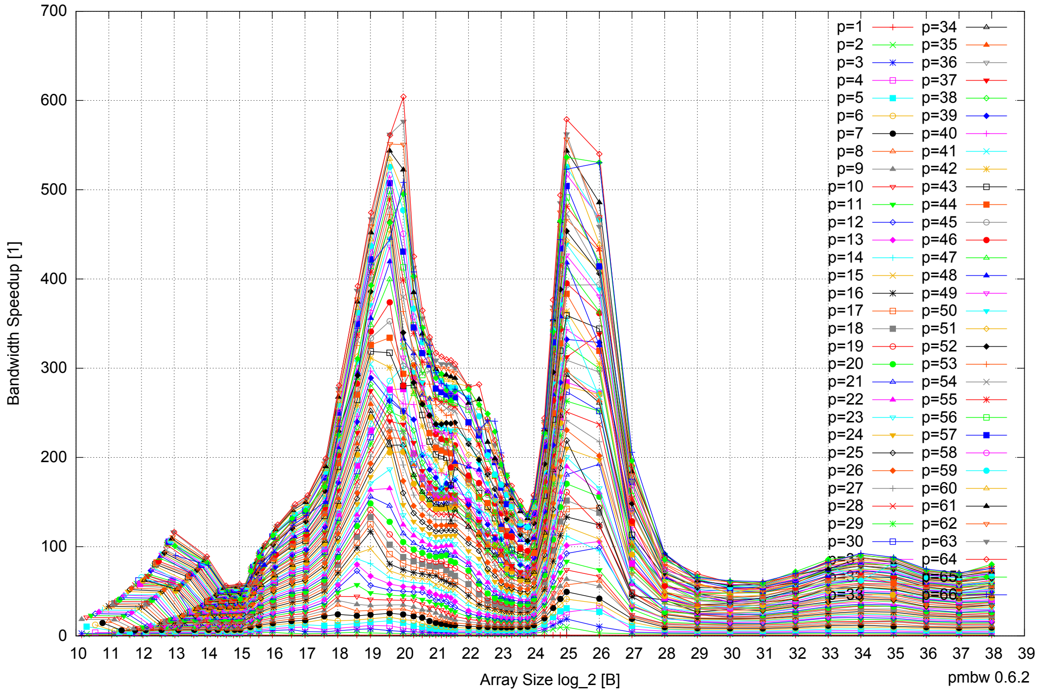
Intel Xeon E5-4640 512GB - Speedup of Parallel Memory Bandwidth - PermRead64SimpleLoop
