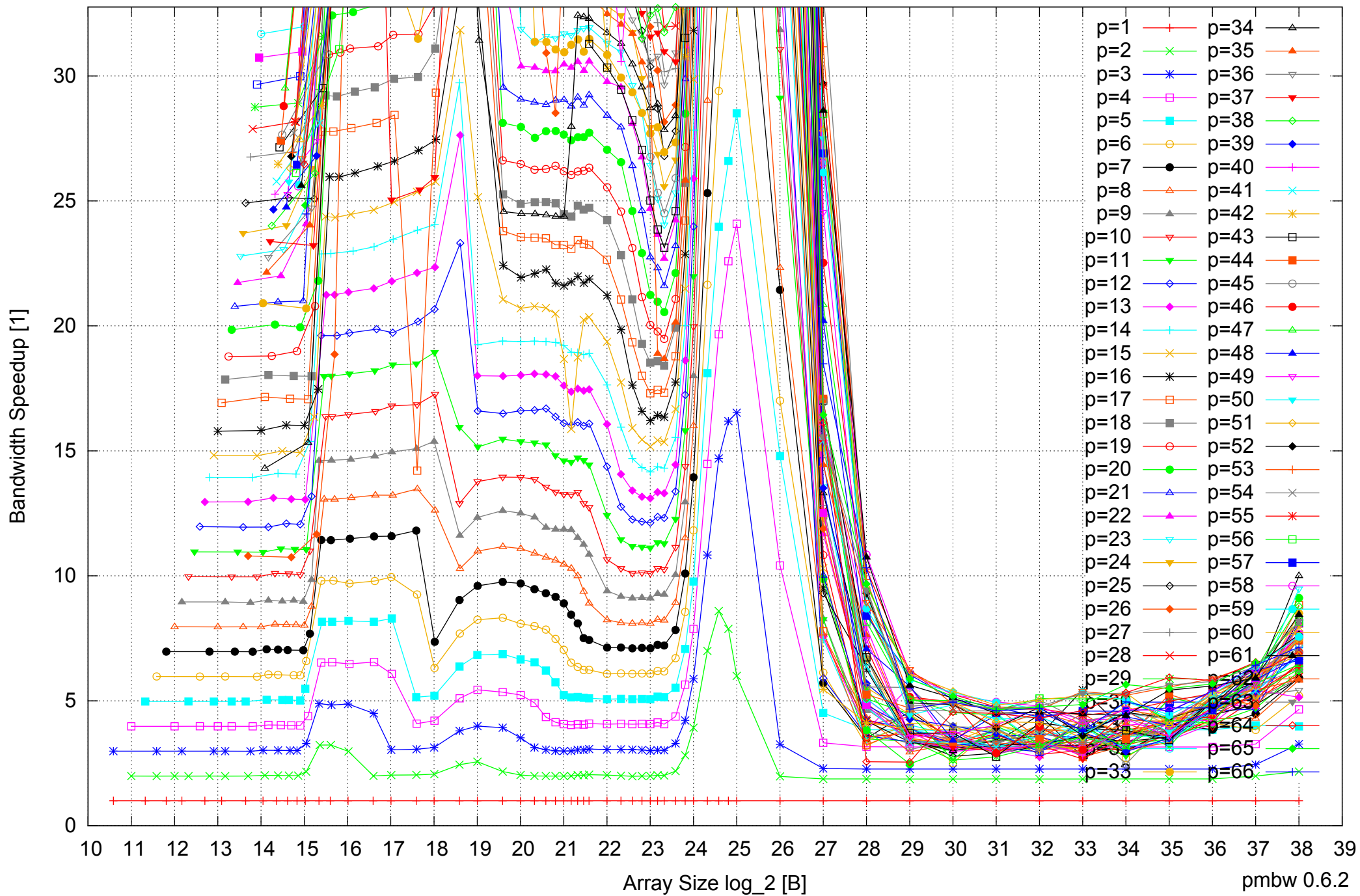
Intel Xeon E5-4640 512GB - Speedup of Parallel Memory Bandwidth (enlarged) - ScanWrite256PtrUnrollLoop
