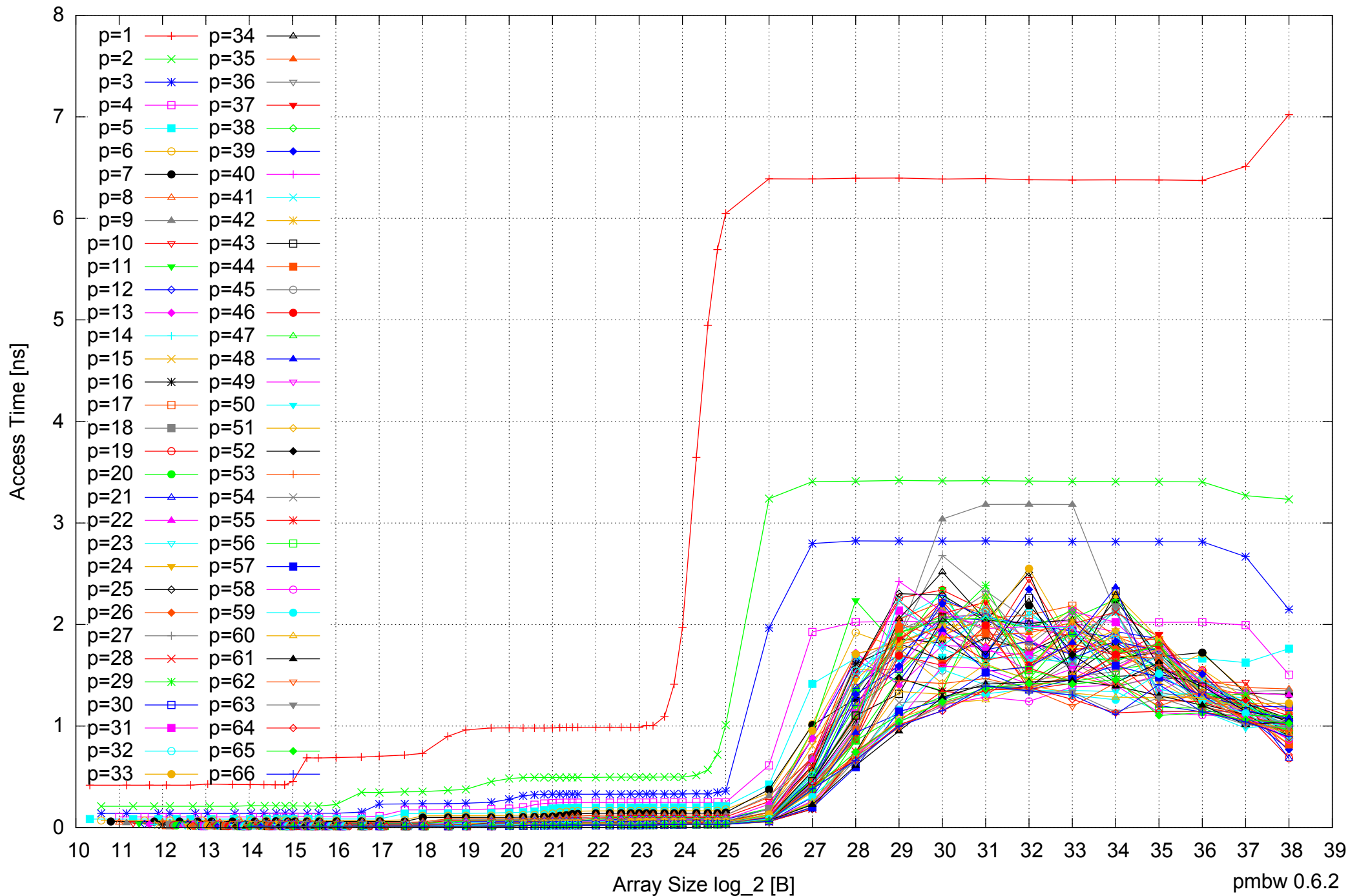
Intel Xeon E5-4640 512GB - Parallel Memory Access Time - ScanWrite128PtrUnrollLoop
