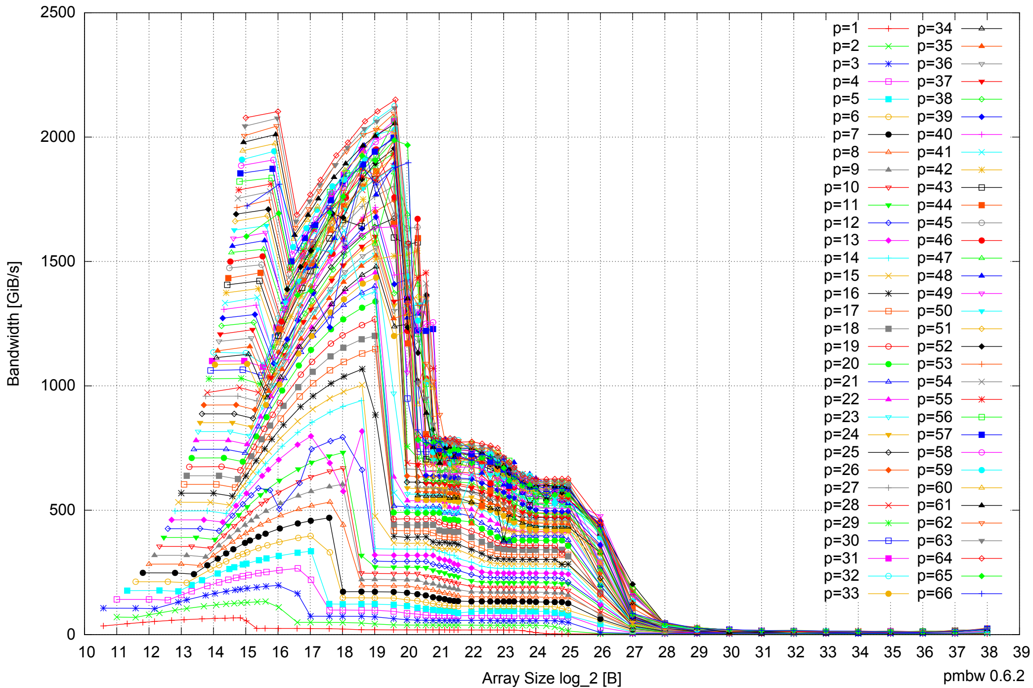
Intel Xeon E5-4640 512GB - Parallel Memory Bandwidth - ScanRead256PtrSimpleLoop
