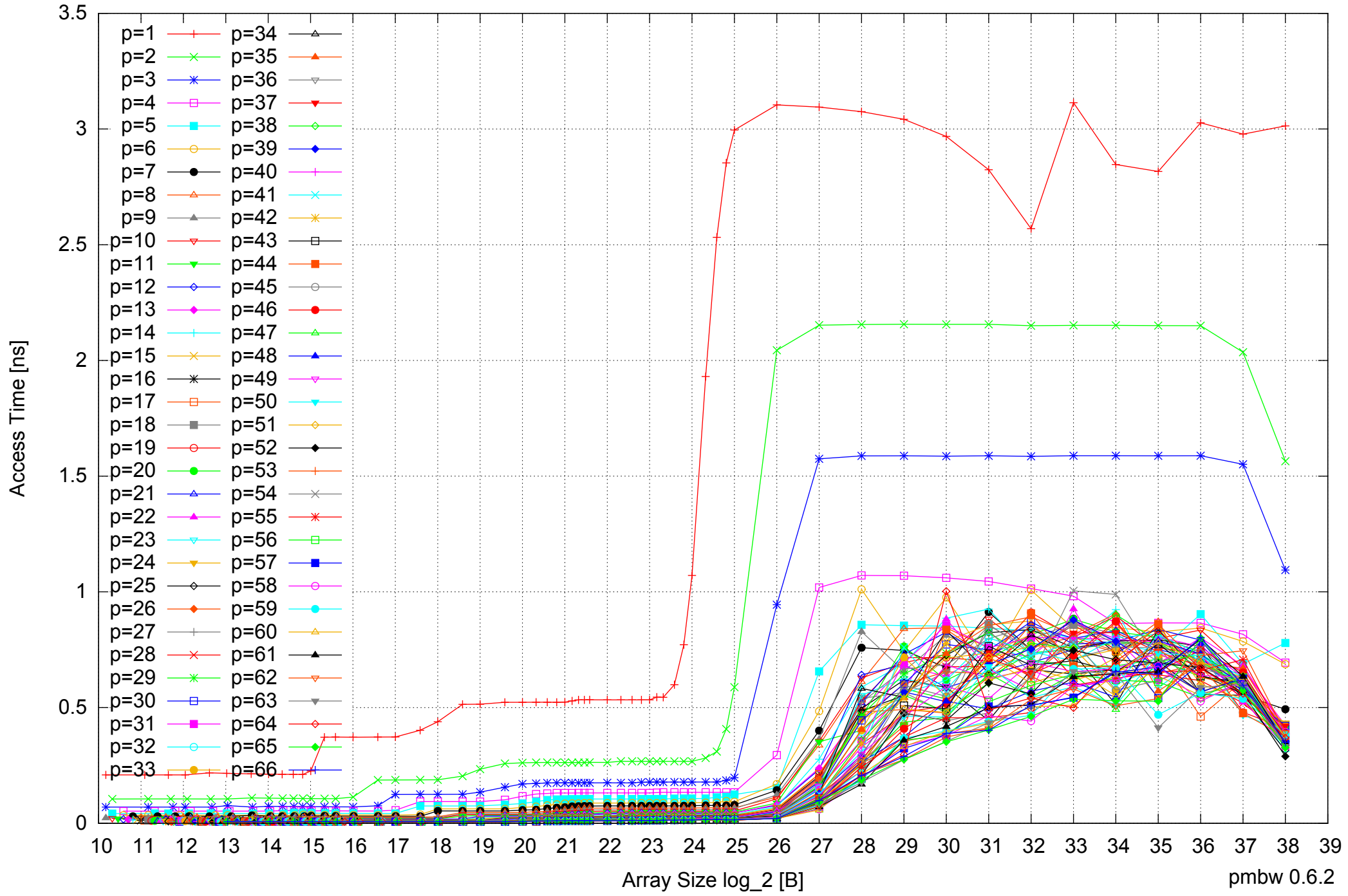
Intel Xeon E5-4640 512GB - Parallel Memory Access Time - ScanRead64IndexUnrollLoop
