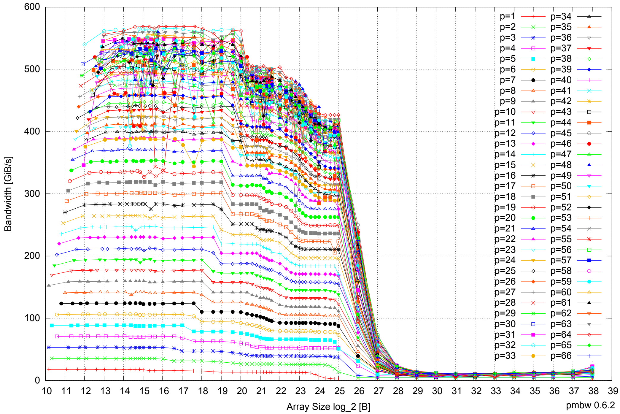
Intel Xeon E5-4640 512GB - Parallel Memory Bandwidth - ScanWrite64PtrUnrollLoop
