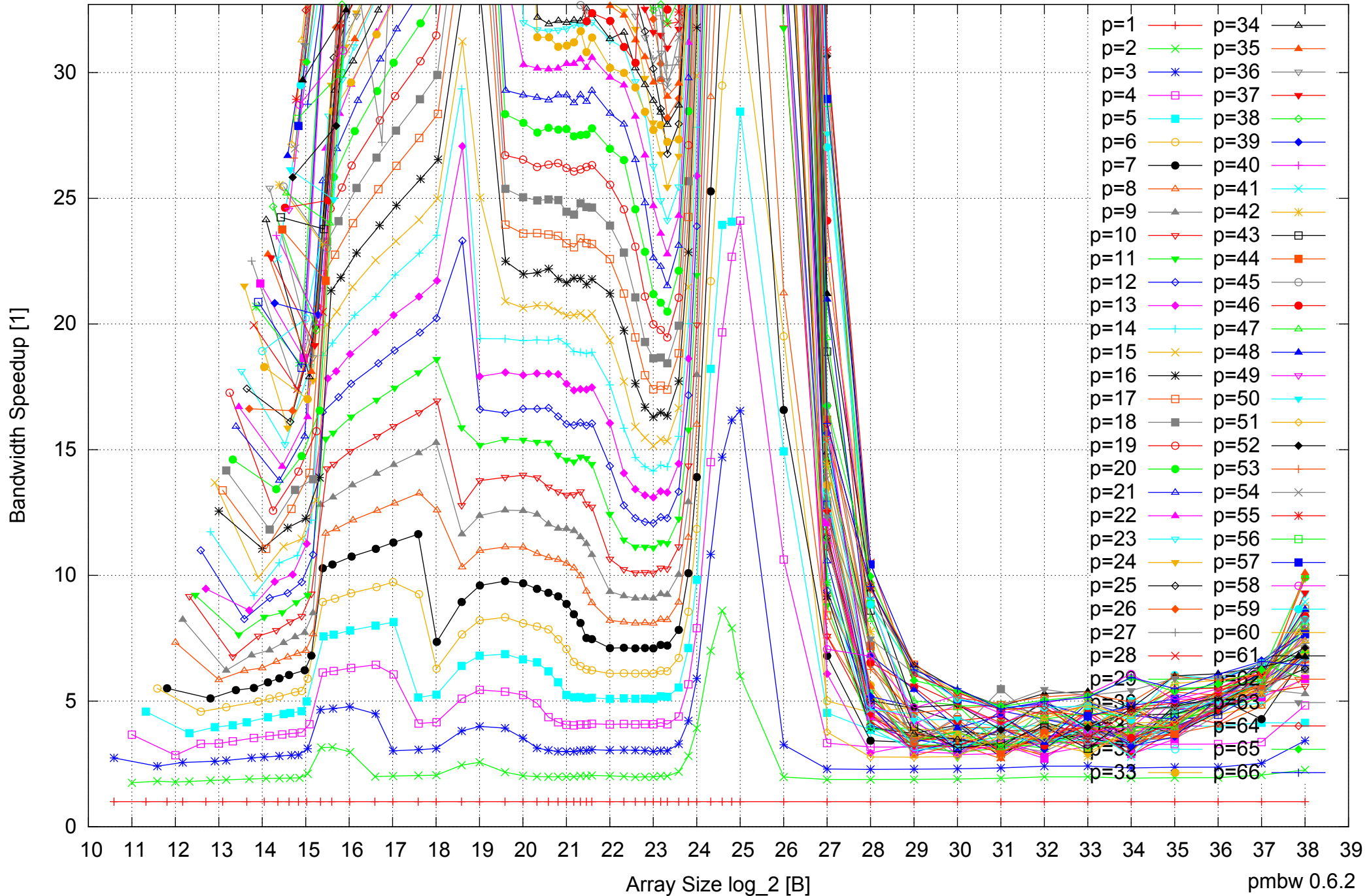
Intel Xeon E5-4640 512GB - Speedup of Parallel Memory Bandwidth (enlarged) - ScanWrite256PtrSimpleLoop
