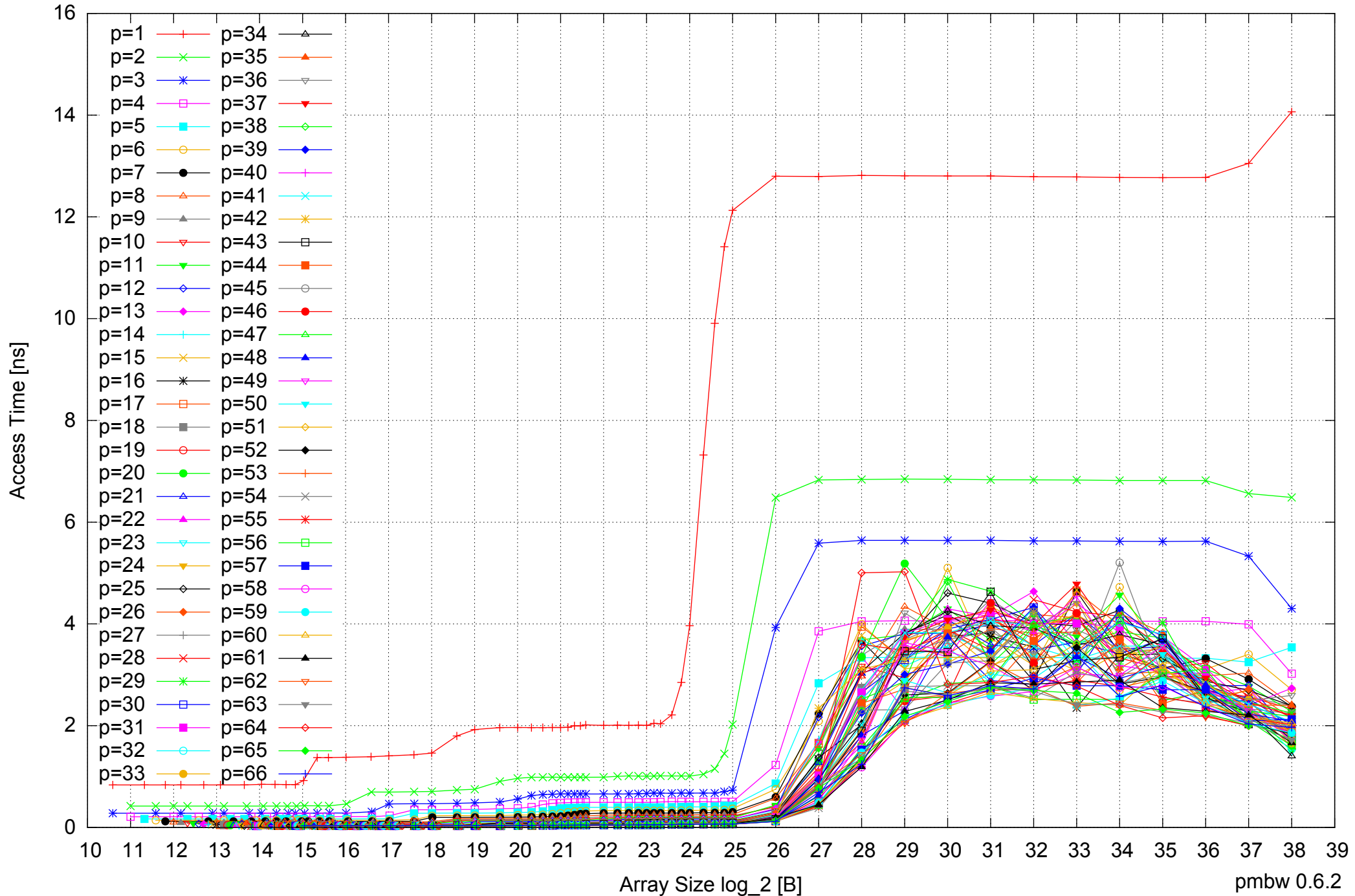
Intel Xeon E5-4640 512GB - Parallel Memory Access Time - ScanWrite256PtrUnrollLoop
