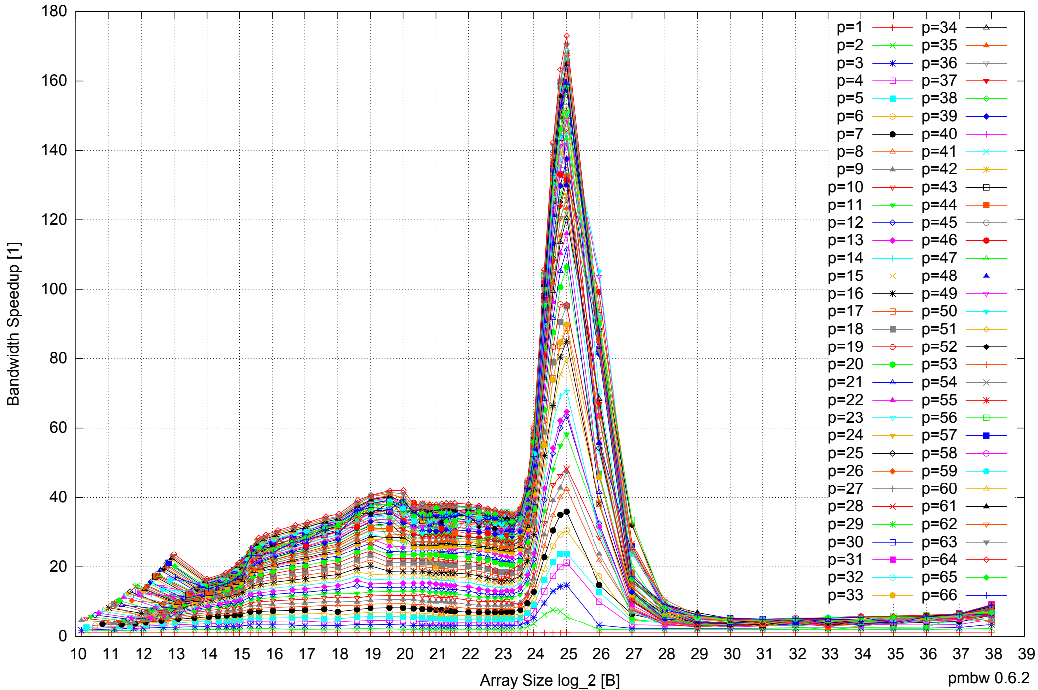
Intel Xeon E5-4640 512GB - Speedup of Parallel Memory Bandwidth - ScanWrite64IndexSimpleLoop
