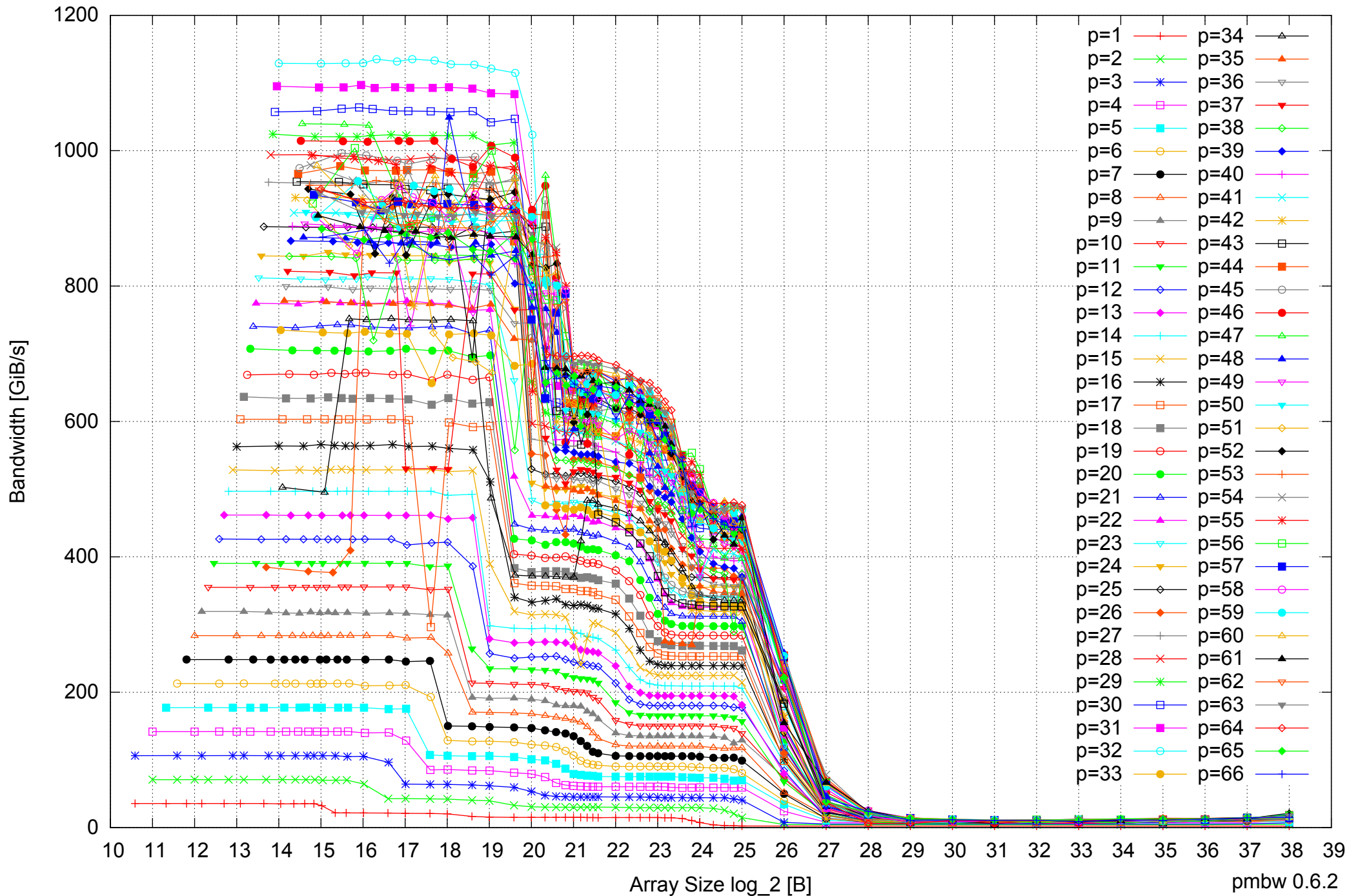
Intel Xeon E5-4640 512GB - Parallel Memory Bandwidth - ScanWrite256PtrUnrollLoop
