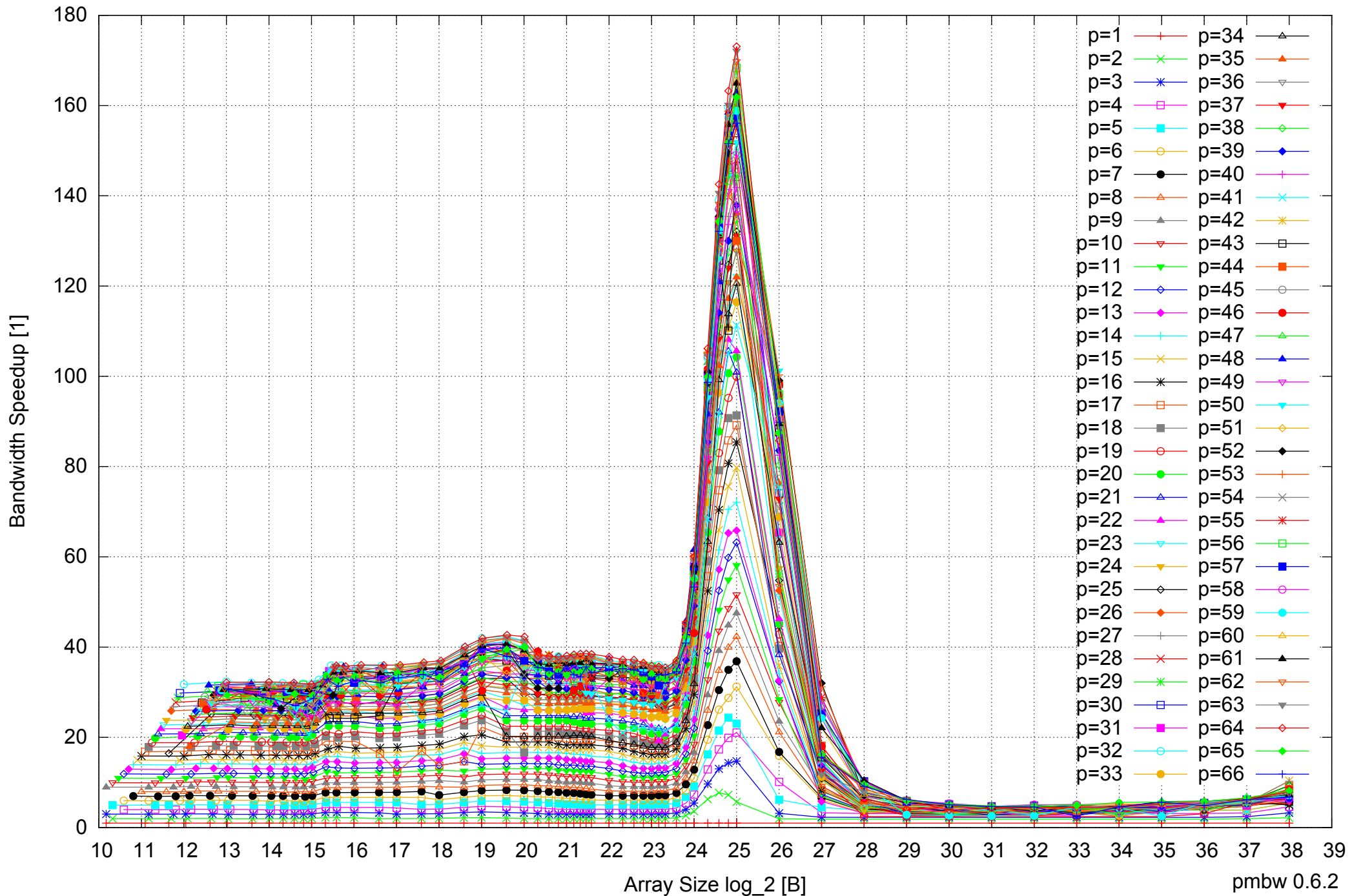
Intel Xeon E5-4640 512GB - Speedup of Parallel Memory Bandwidth - ScanWrite64IndexUnrollLoop
