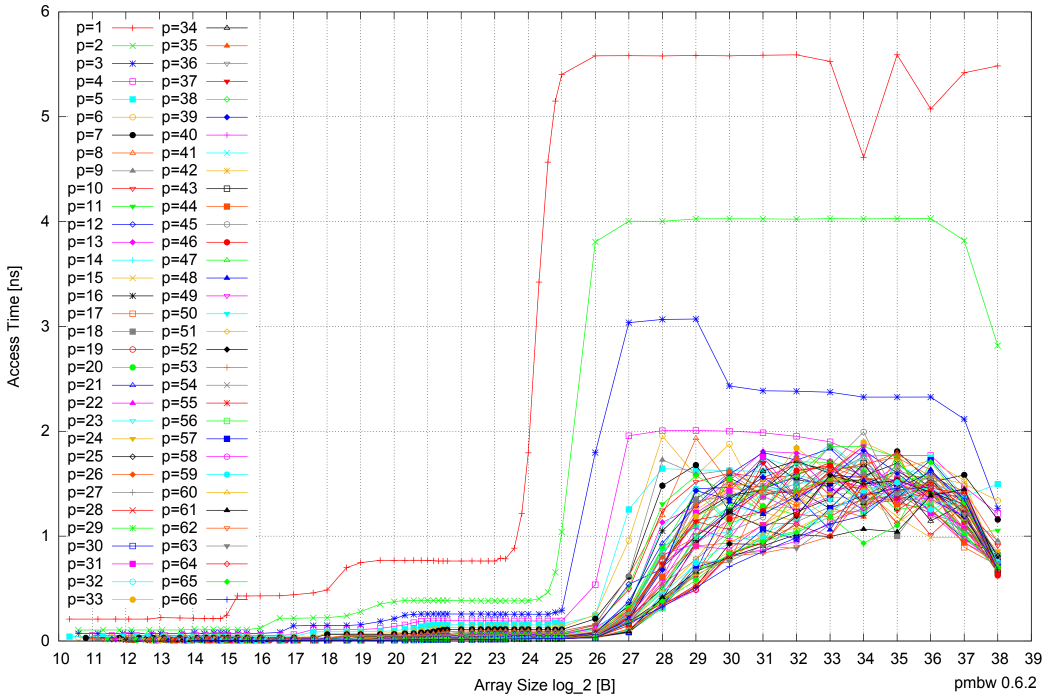
Intel Xeon E5-4640 512GB - Parallel Memory Access Time - ScanRead128PtrUnrollLoop
