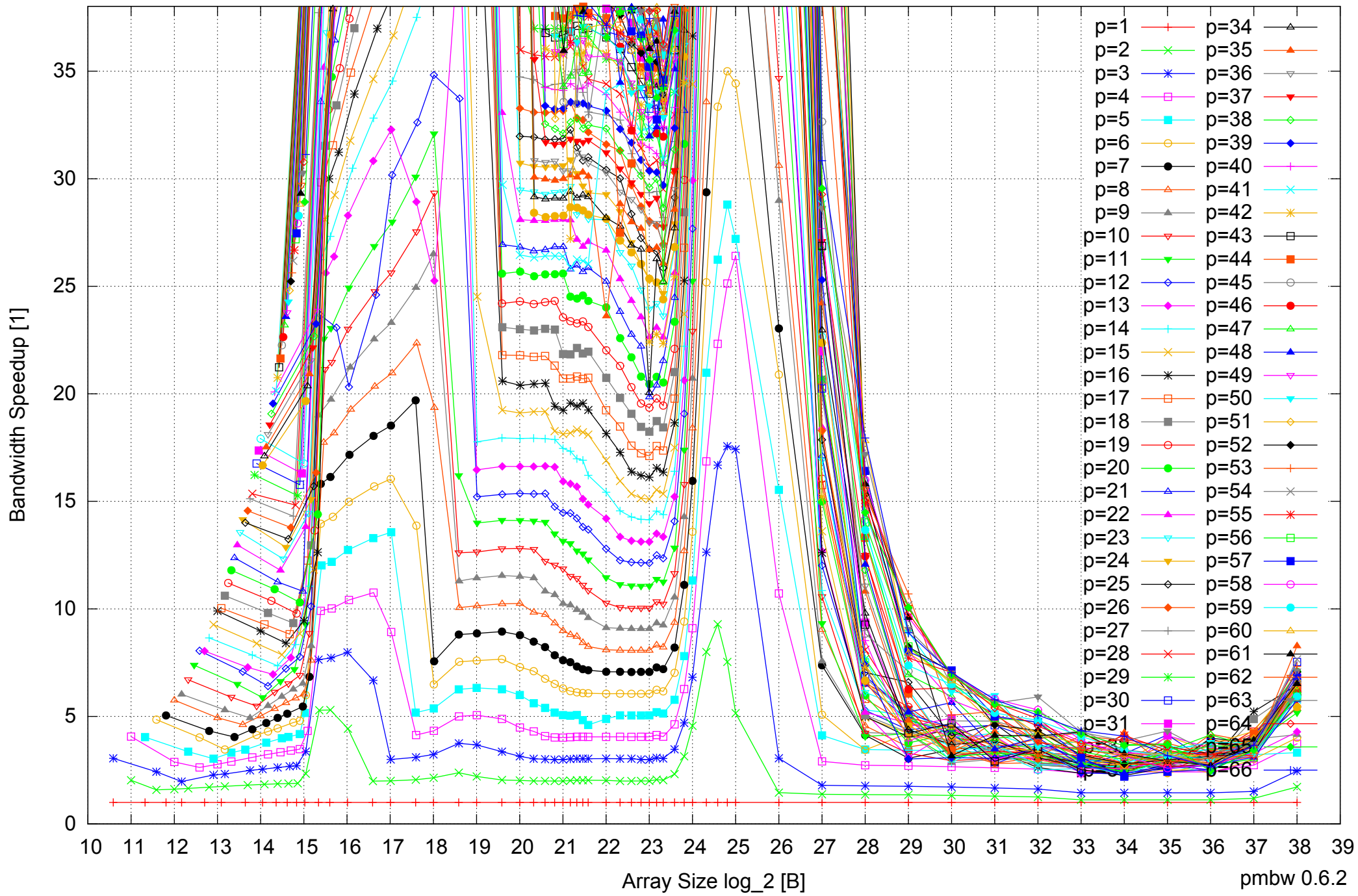
Intel Xeon E5-4640 512GB - Speedup of Parallel Memory Bandwidth (enlarged) - ScanRead256PtrSimpleLoop
