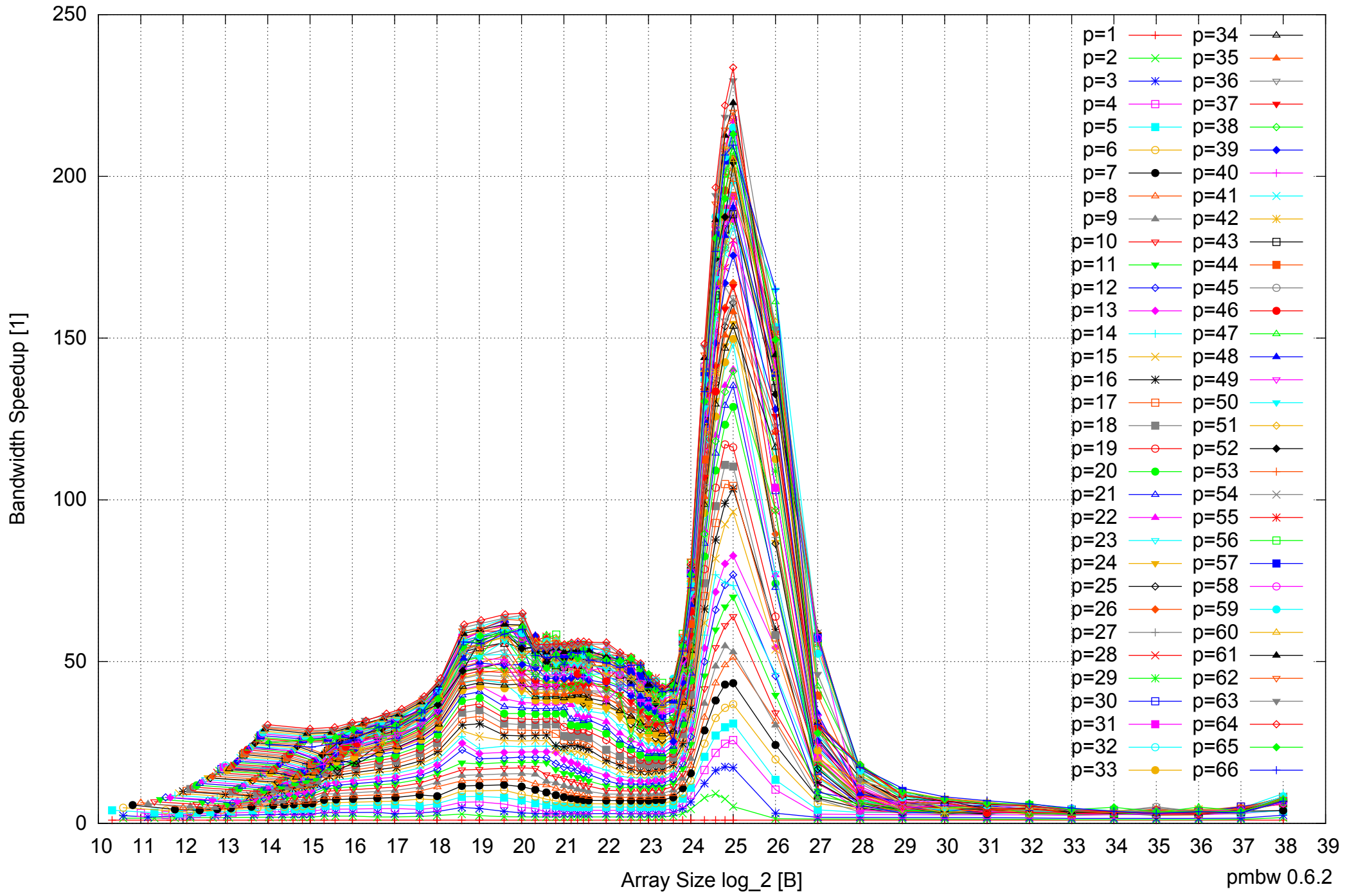
Intel Xeon E5-4640 512GB - Speedup of Parallel Memory Bandwidth - ScanRead128PtrSimpleLoop
