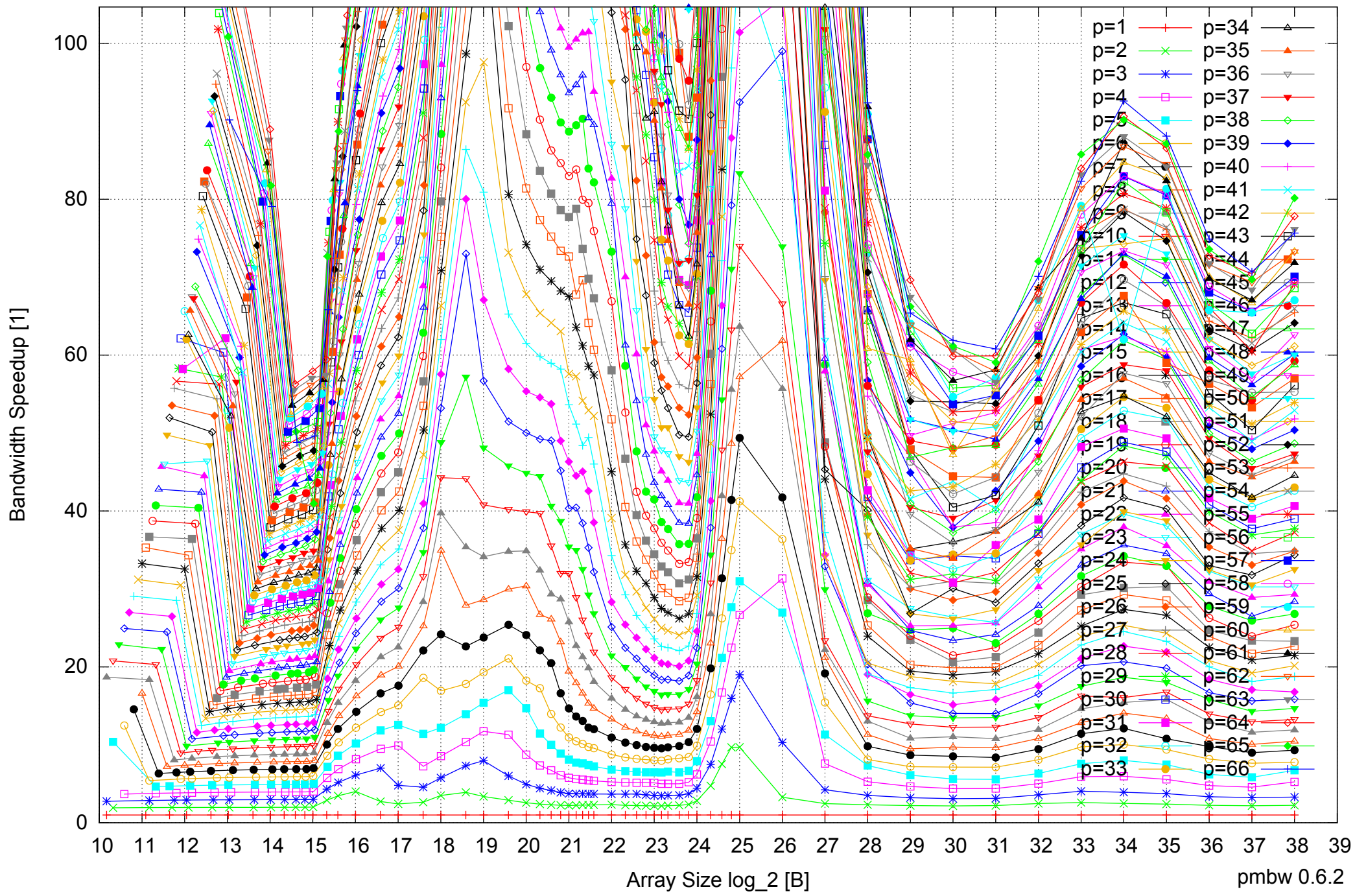
Intel Xeon E5-4640 512GB - Speedup of Parallel Memory Bandwidth (enlarged) - PermRead64SimpleLoop
