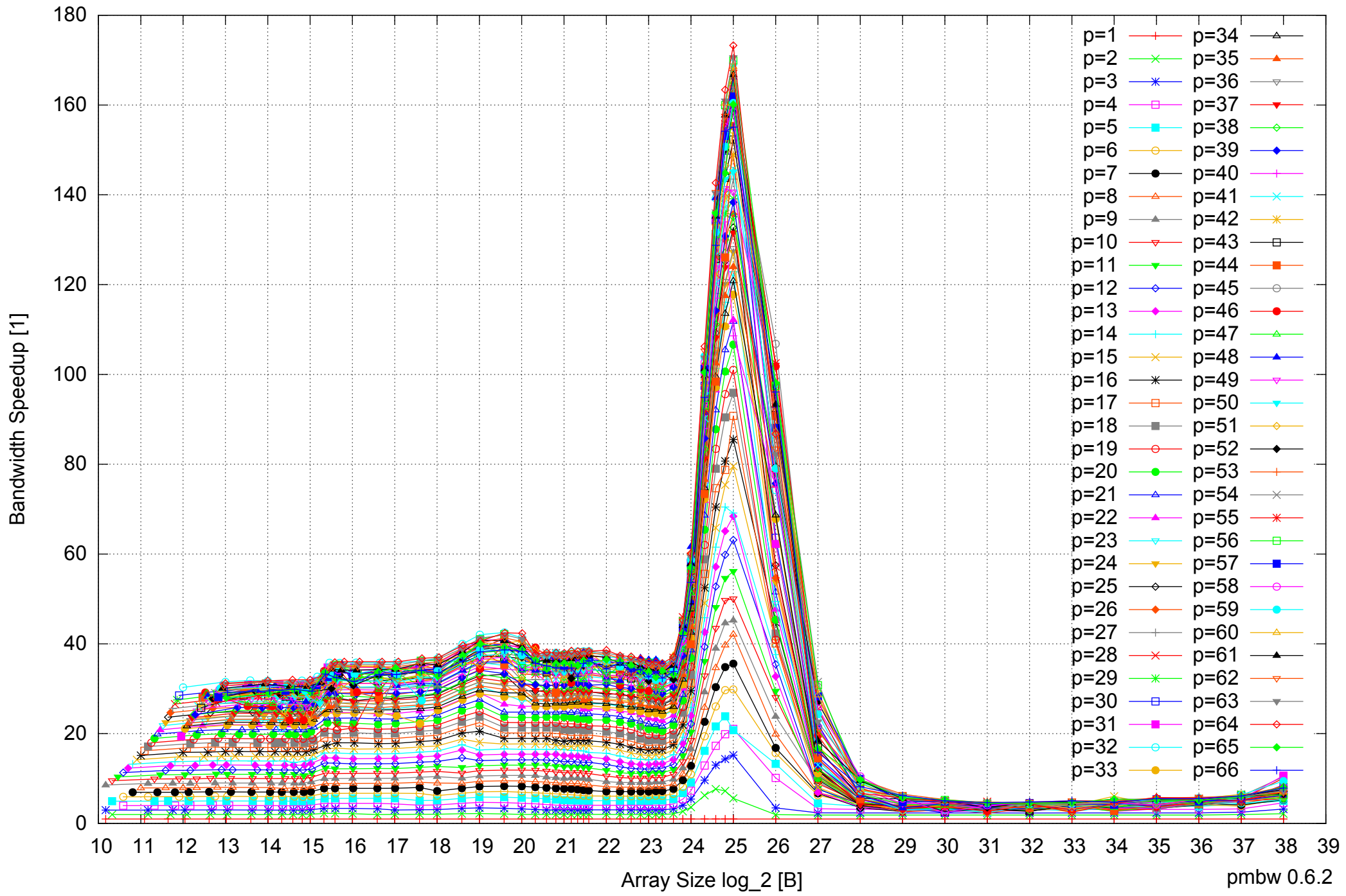
Intel Xeon E5-4640 512GB - Speedup of Parallel Memory Bandwidth - ScanWrite64PtrUnrollLoop
