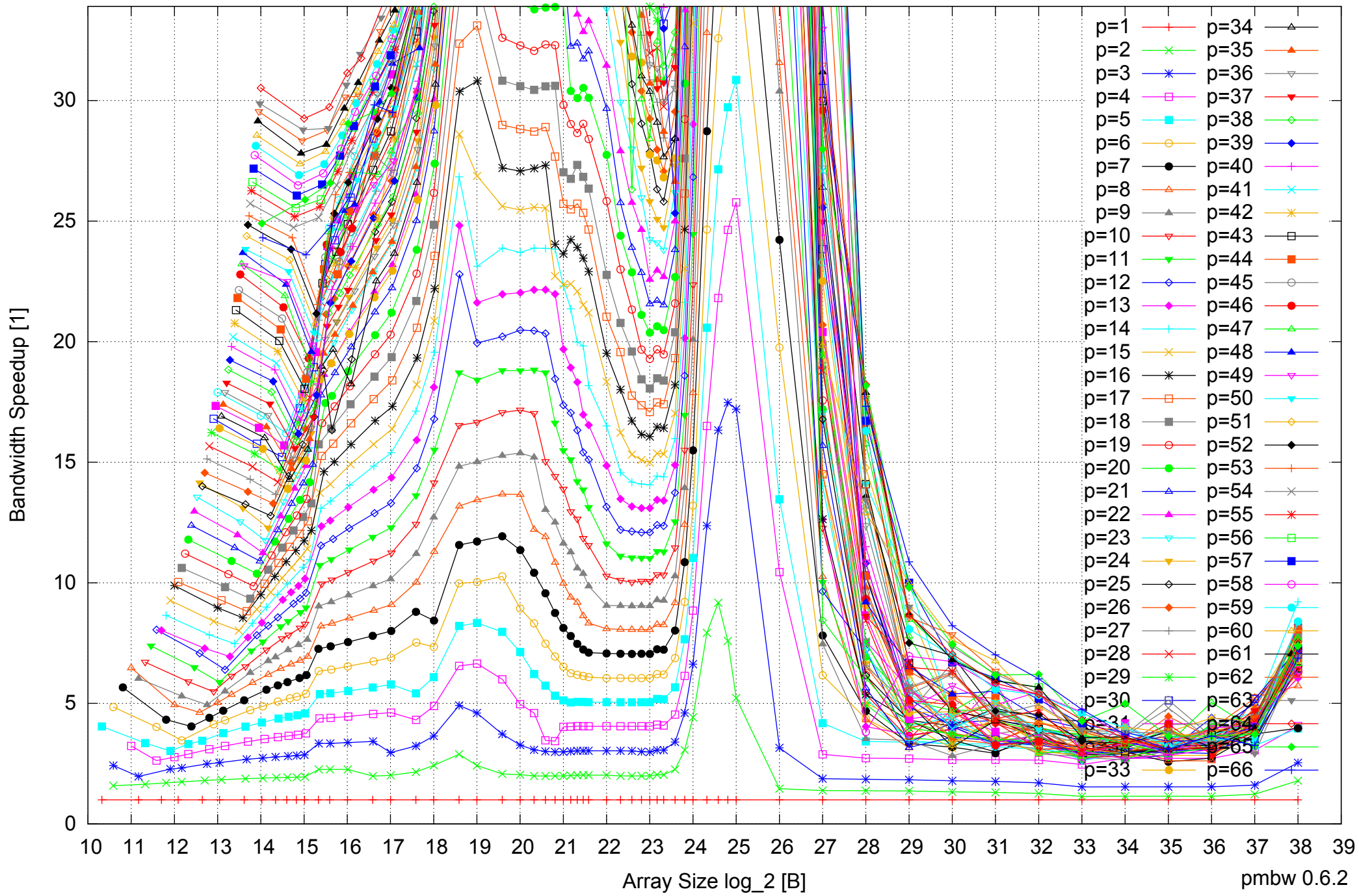
Intel Xeon E5-4640 512GB - Speedup of Parallel Memory Bandwidth (enlarged) - ScanRead128PtrSimpleLoop
