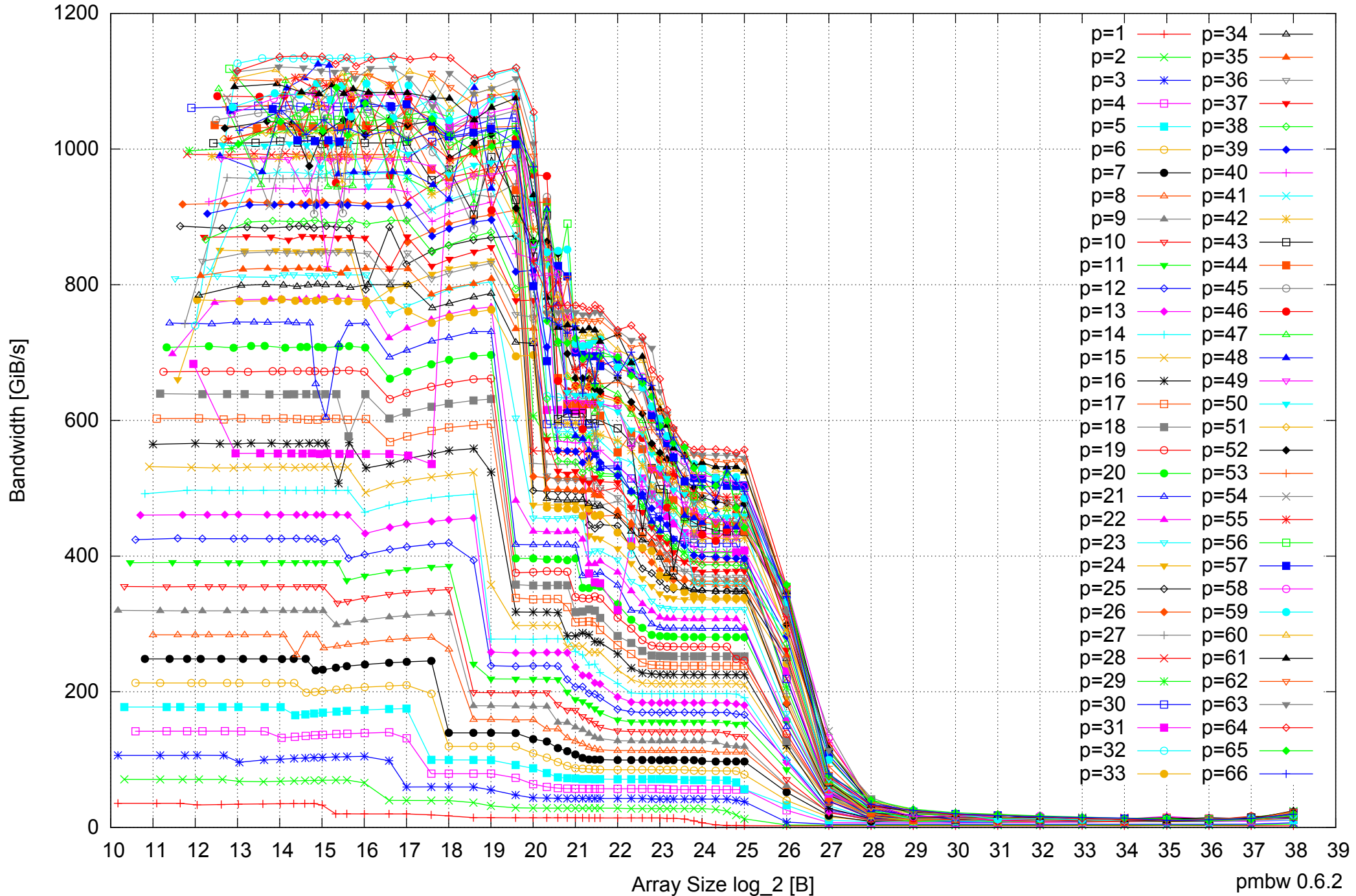
Intel Xeon E5-4640 512GB - Parallel Memory Bandwidth - ScanRead64PtrUnrollLoop
