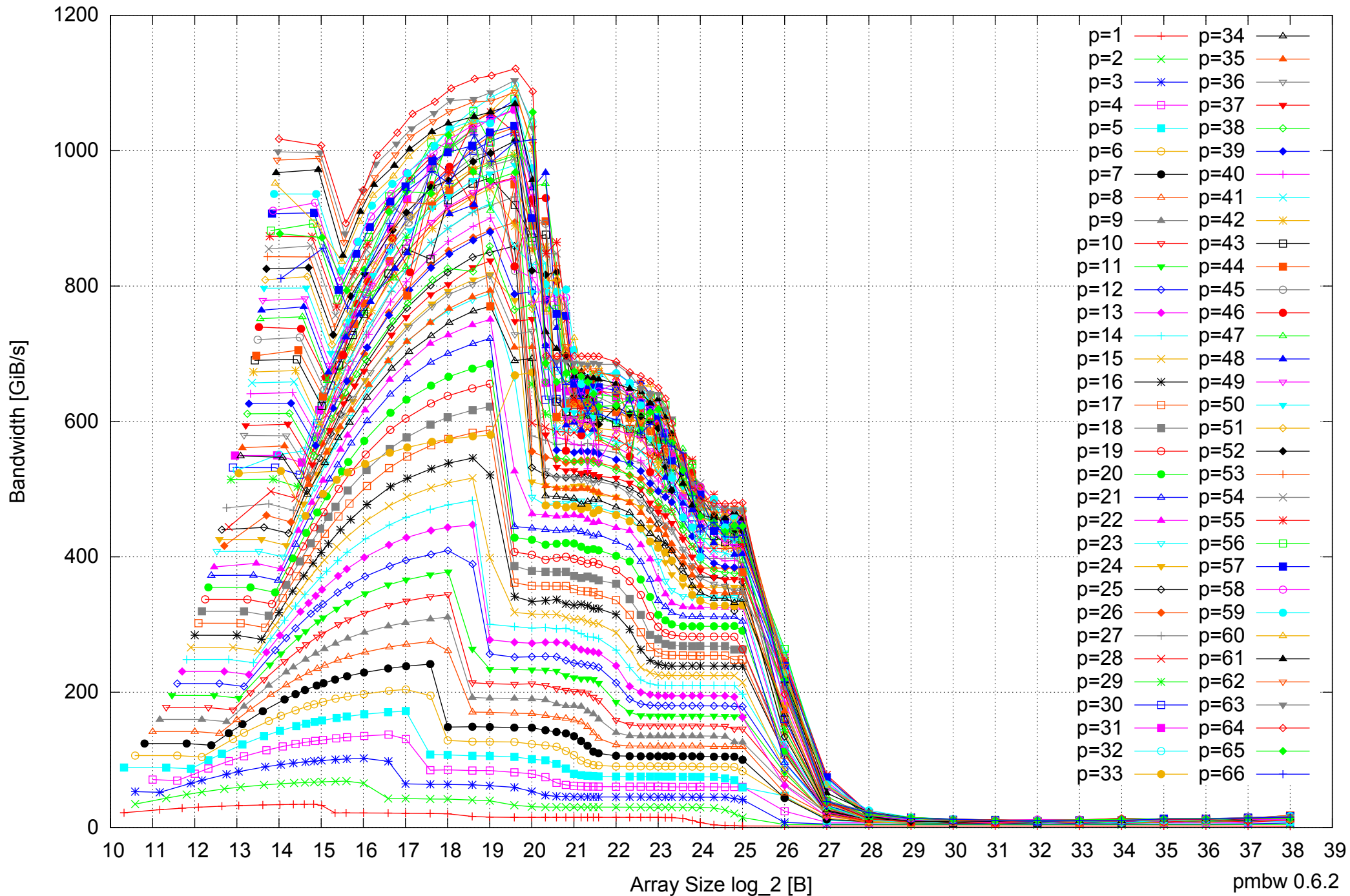
Intel Xeon E5-4640 512GB - Parallel Memory Bandwidth - ScanWrite128PtrSimpleLoop
