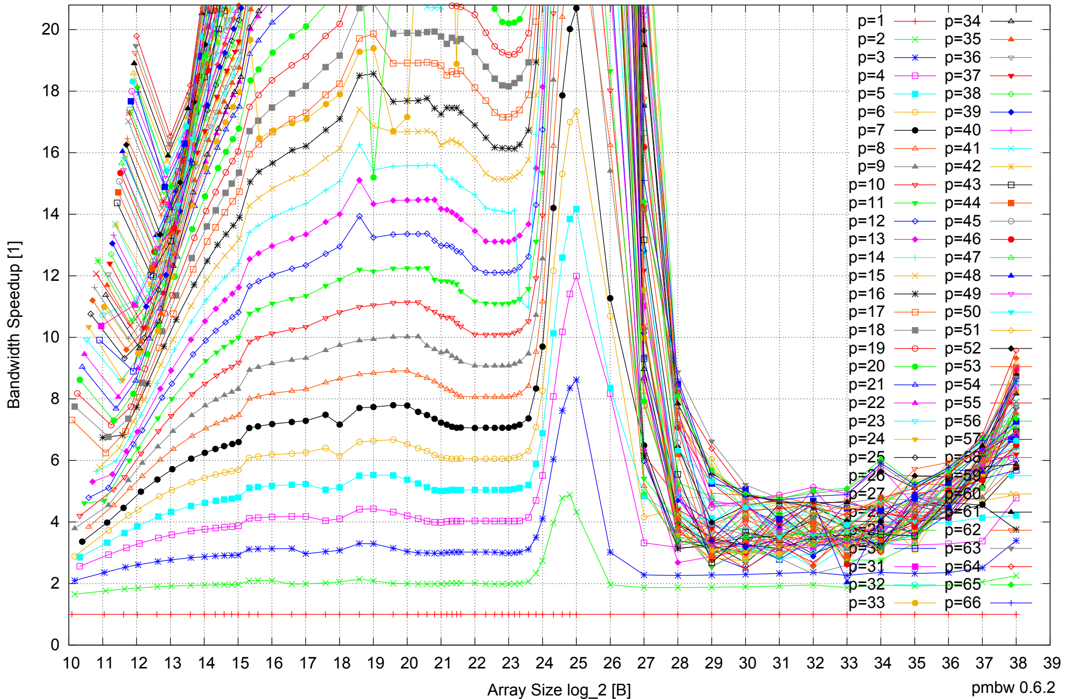
Intel Xeon E5-4640 512GB - Speedup of Parallel Memory Bandwidth (enlarged) - ScanWrite32PtrSimpleLoop
