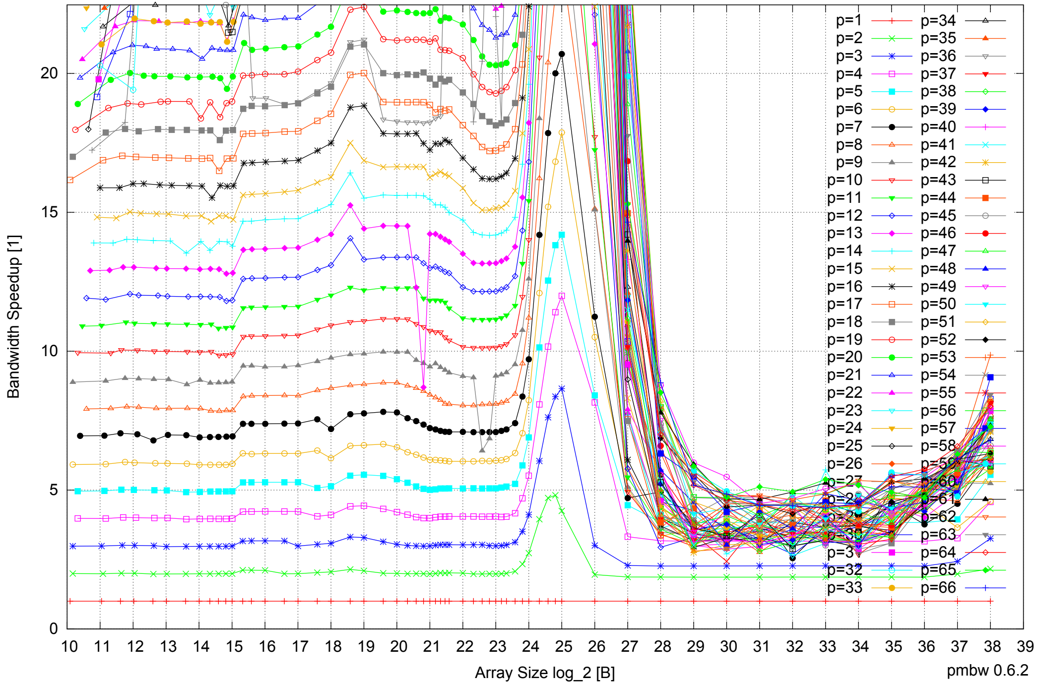
Intel Xeon E5-4640 512GB - Speedup of Parallel Memory Bandwidth (enlarged) - ScanWrite32PtrUnrollLoop
