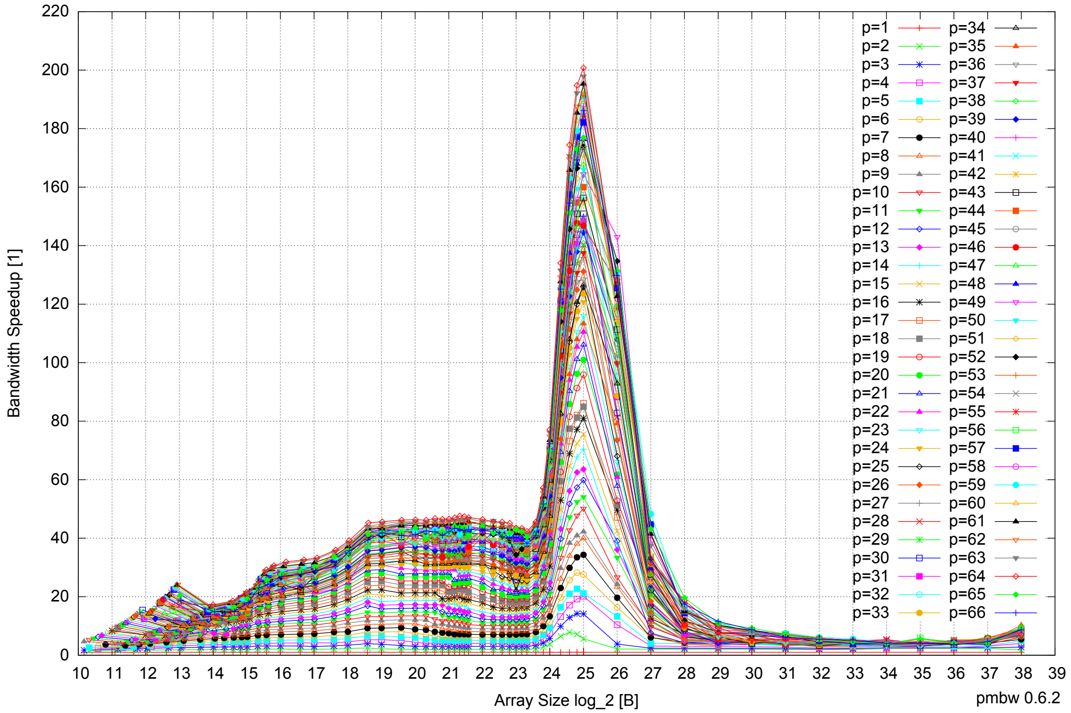
Intel Xeon E5-4640 512GB - Speedup of Parallel Memory Bandwidth - ScanRead64PtrSimpleLoop
