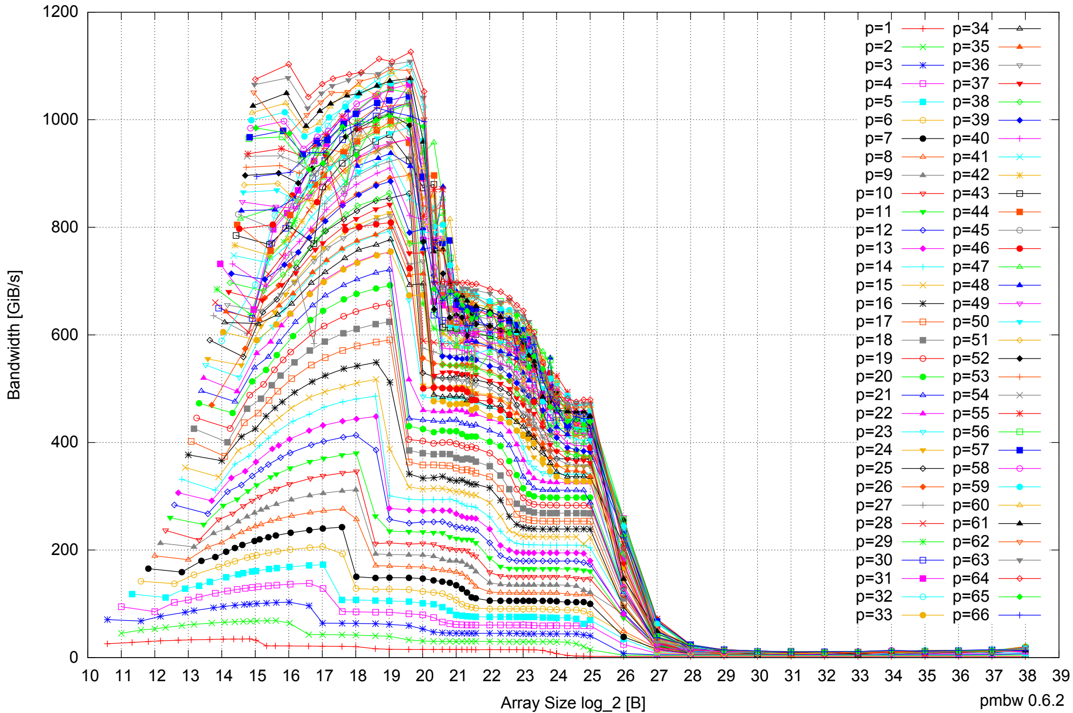
Intel Xeon E5-4640 512GB - Parallel Memory Bandwidth - ScanWrite256PtrSimpleLoop
