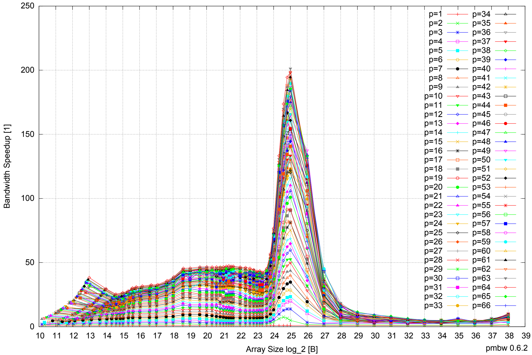
Intel Xeon E5-4640 512GB - Speedup of Parallel Memory Bandwidth - ScanRead64IndexSimpleLoop
