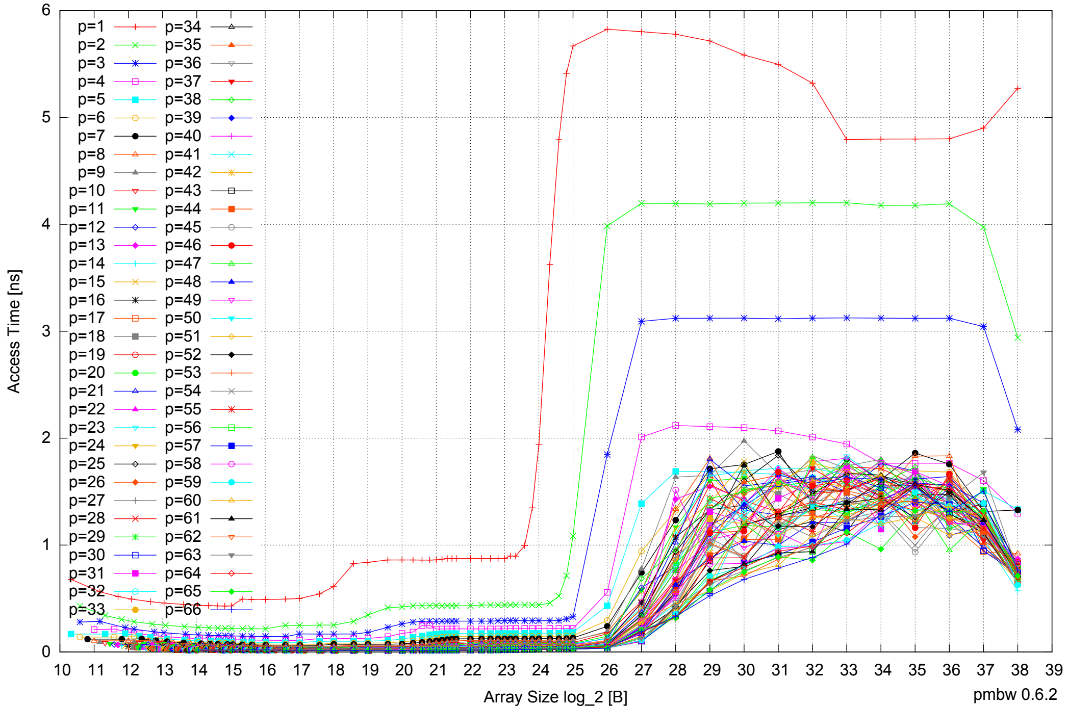
Intel Xeon E5-4640 512GB - Parallel Memory Access Time - ScanRead128PtrSimpleLoop
