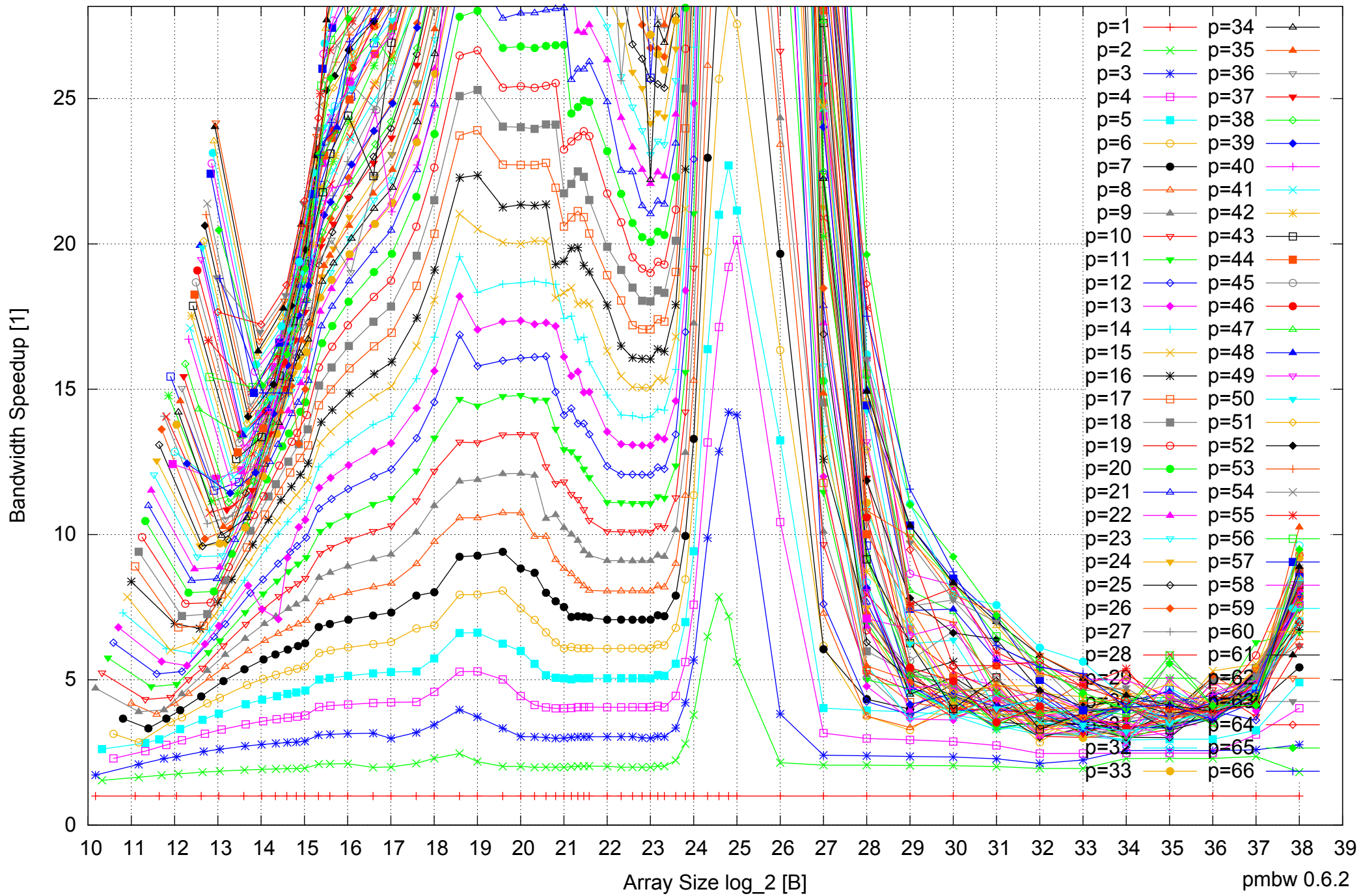
Intel Xeon E5-4640 512GB - Speedup of Parallel Memory Bandwidth (enlarged) - ScanRead64PtrSimpleLoop
