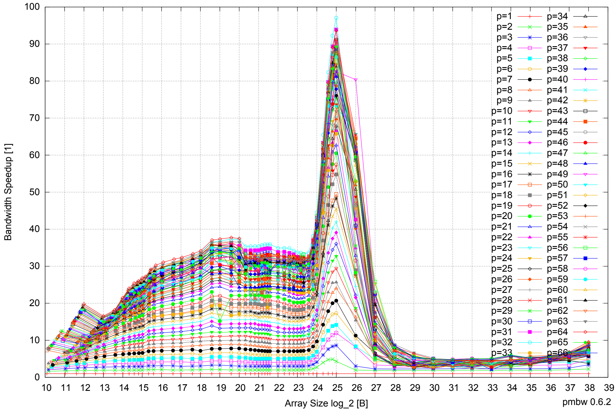
Intel Xeon E5-4640 512GB - Speedup of Parallel Memory Bandwidth - ScanWrite32PtrSimpleLoop
