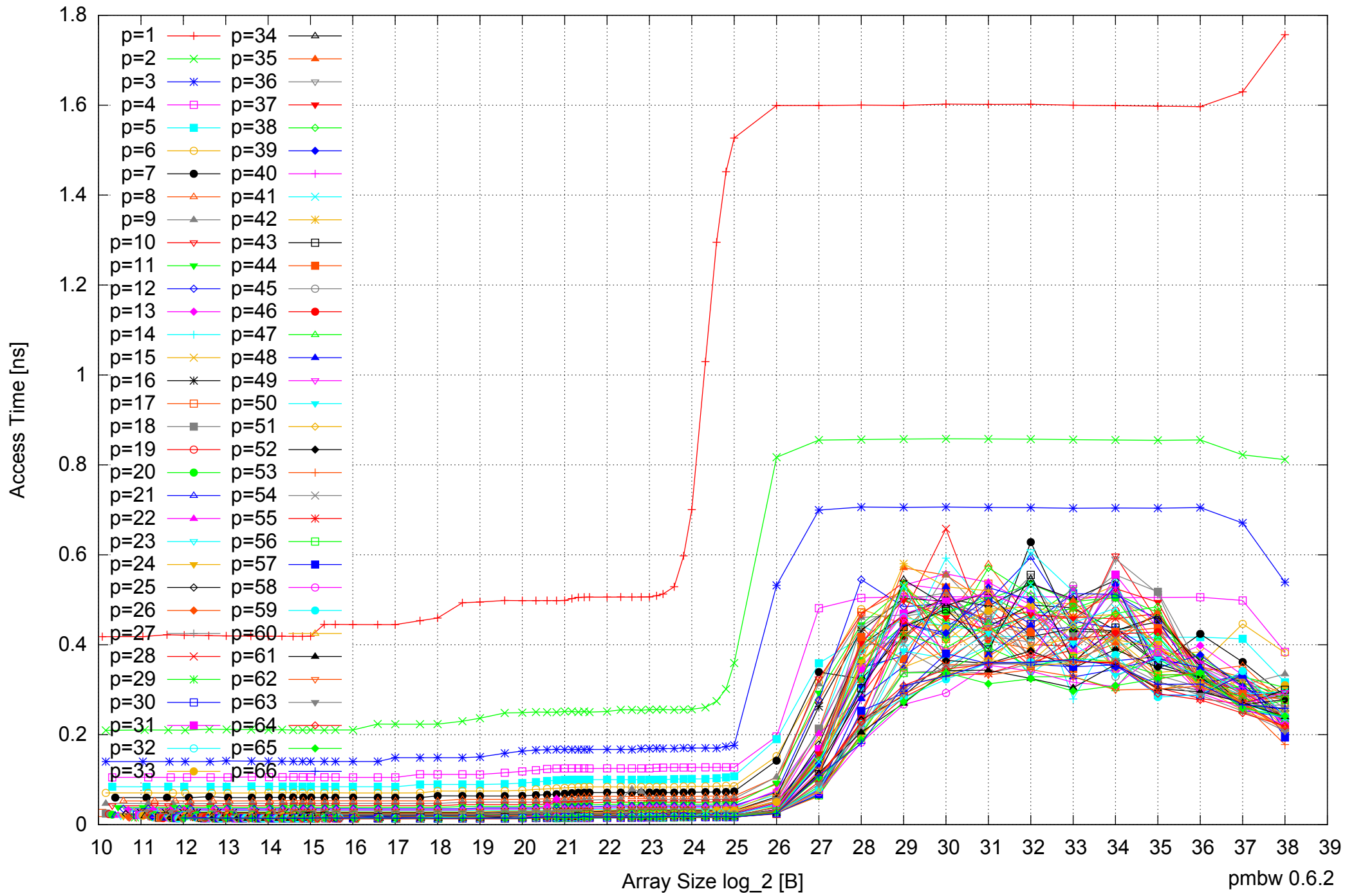
Intel Xeon E5-4640 512GB - Parallel Memory Access Time - ScanWrite32PtrUnrollLoop
