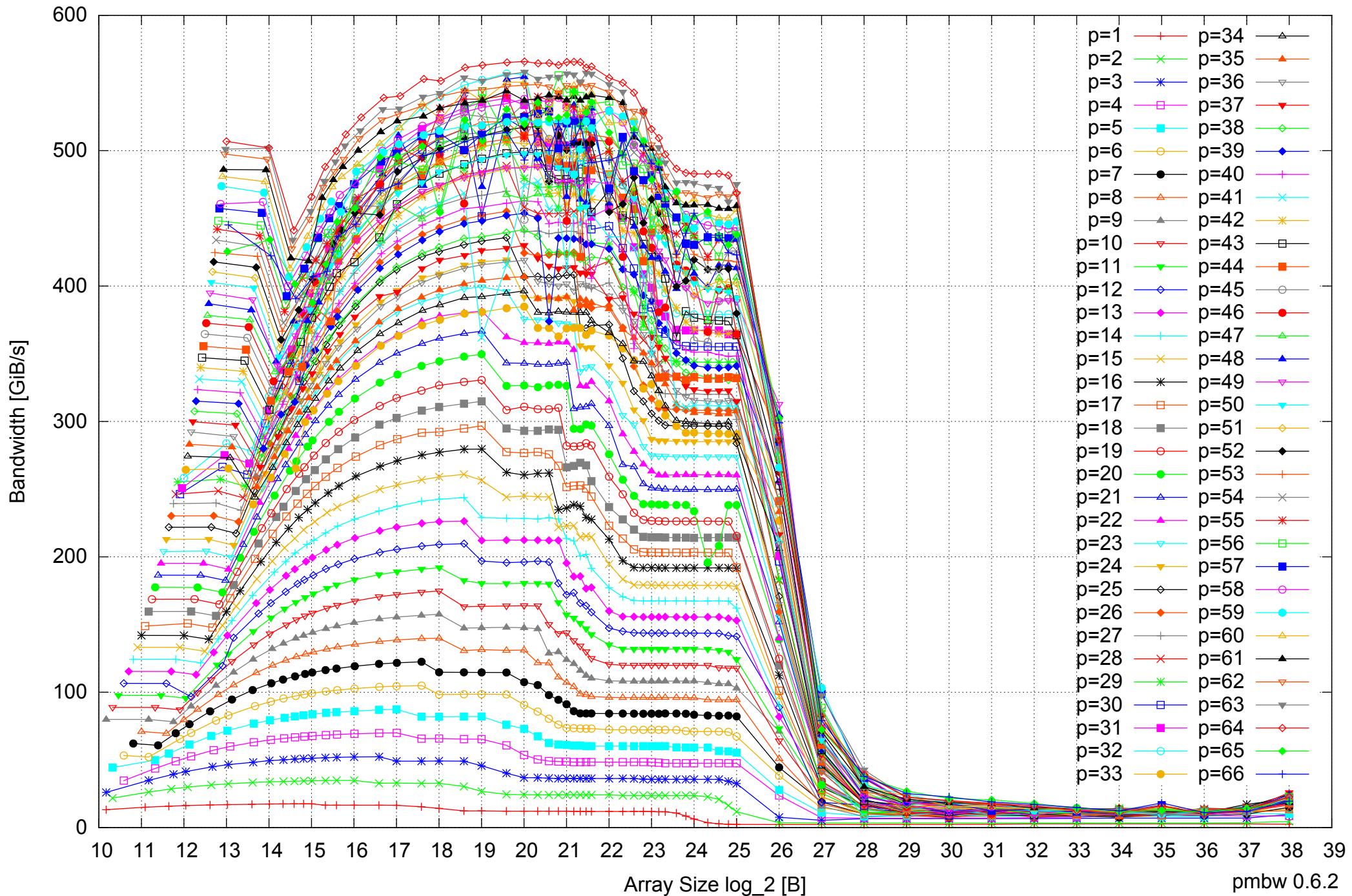
Intel Xeon E5-4640 512GB - Parallel Memory Bandwidth - ScanRead64IndexSimpleLoop
