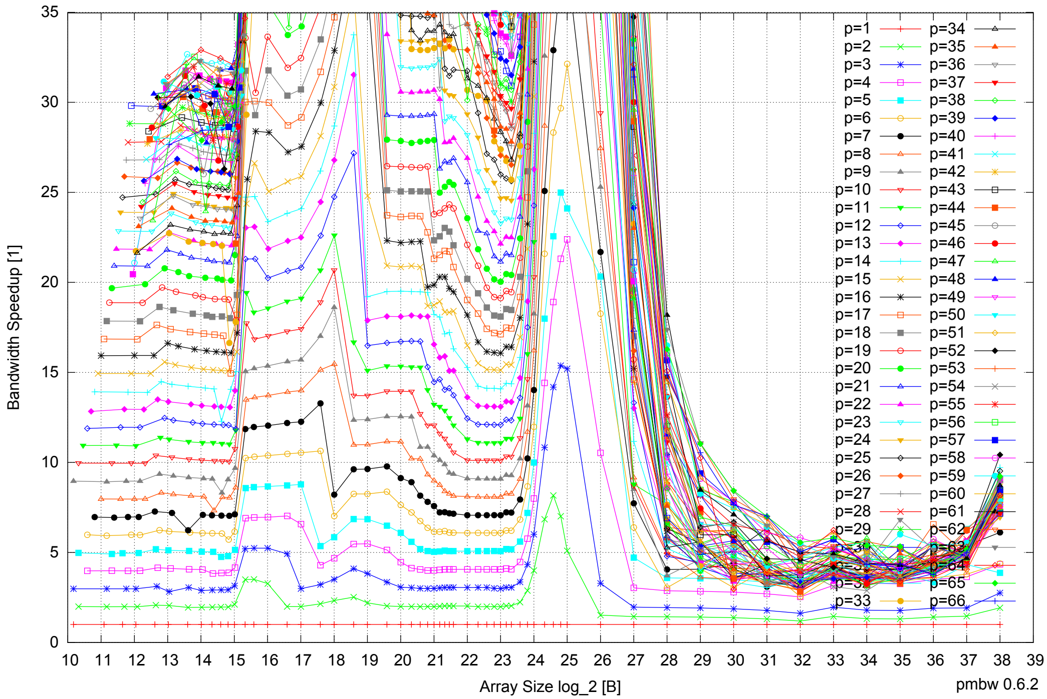
Intel Xeon E5-4640 512GB - Speedup of Parallel Memory Bandwidth (enlarged) - ScanRead64IndexUnrollLoop
