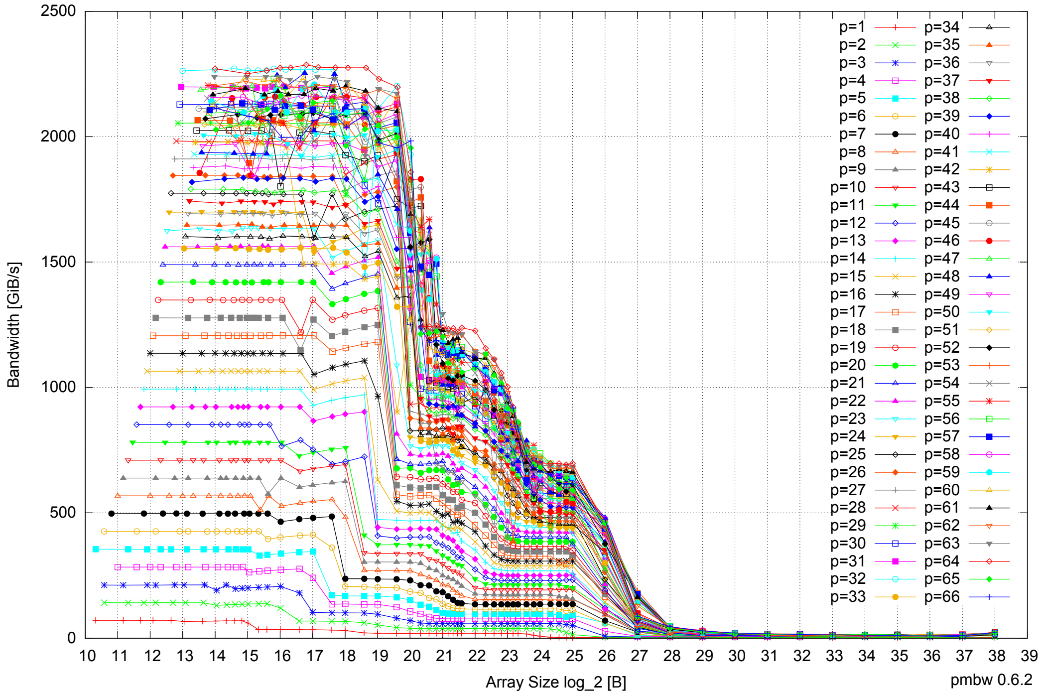
Intel Xeon E5-4640 512GB - Parallel Memory Bandwidth - ScanRead128PtrUnrollLoop
