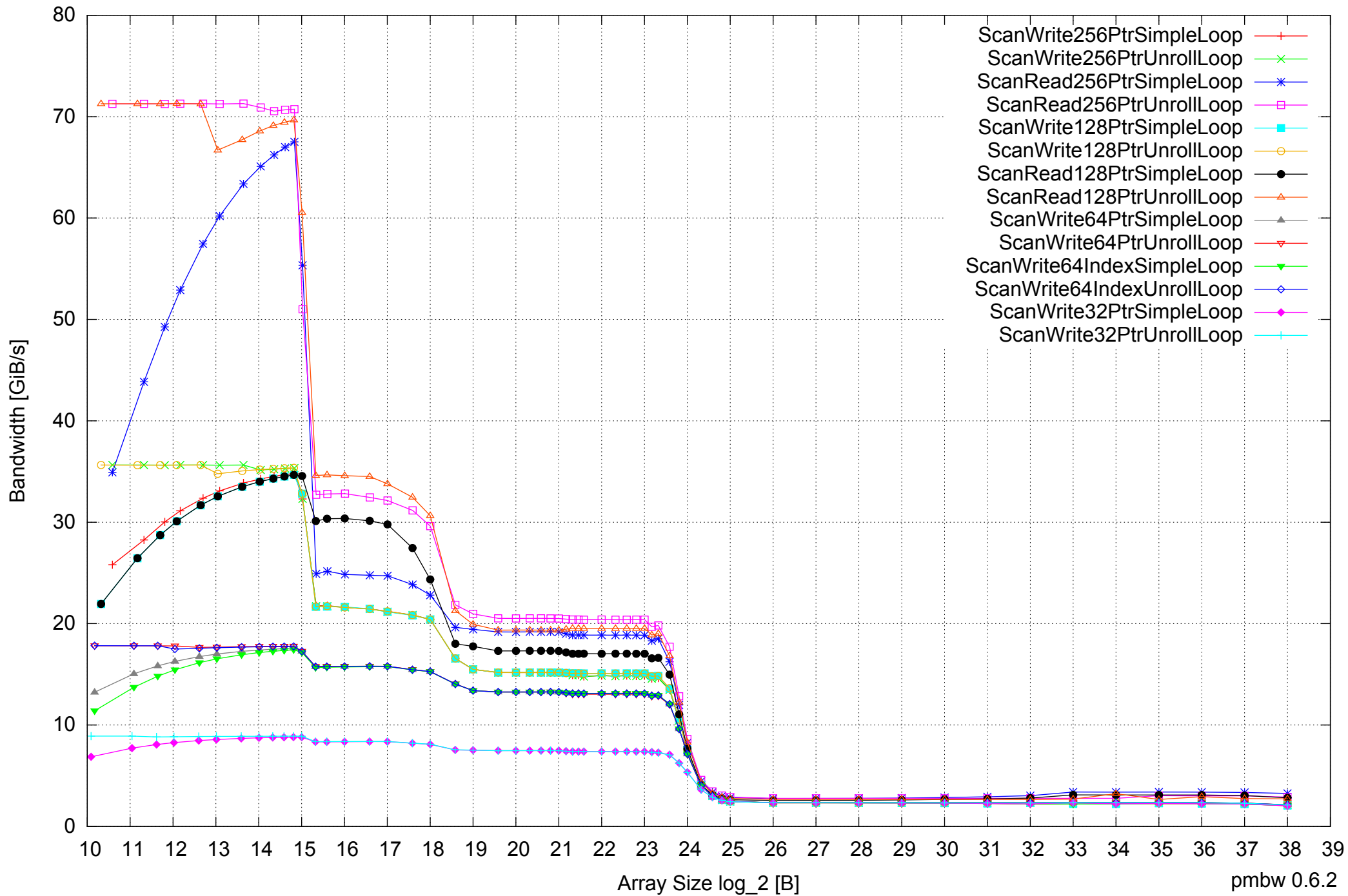
Intel Xeon E5-4640 512GB - One Thread Memory Bandwidth (only 64-bit Reads)
