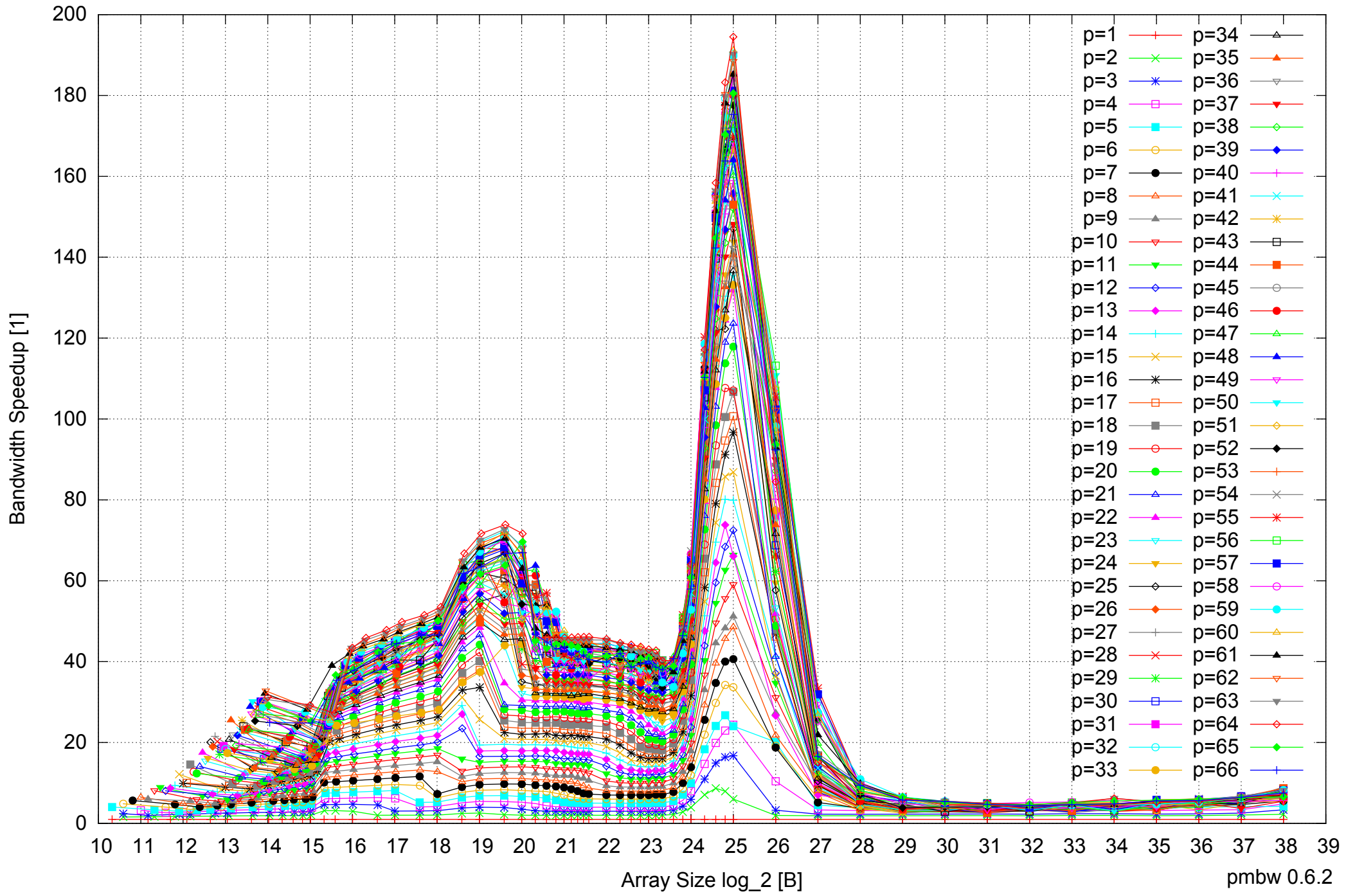
Intel Xeon E5-4640 512GB - Speedup of Parallel Memory Bandwidth - ScanWrite128PtrSimpleLoop
