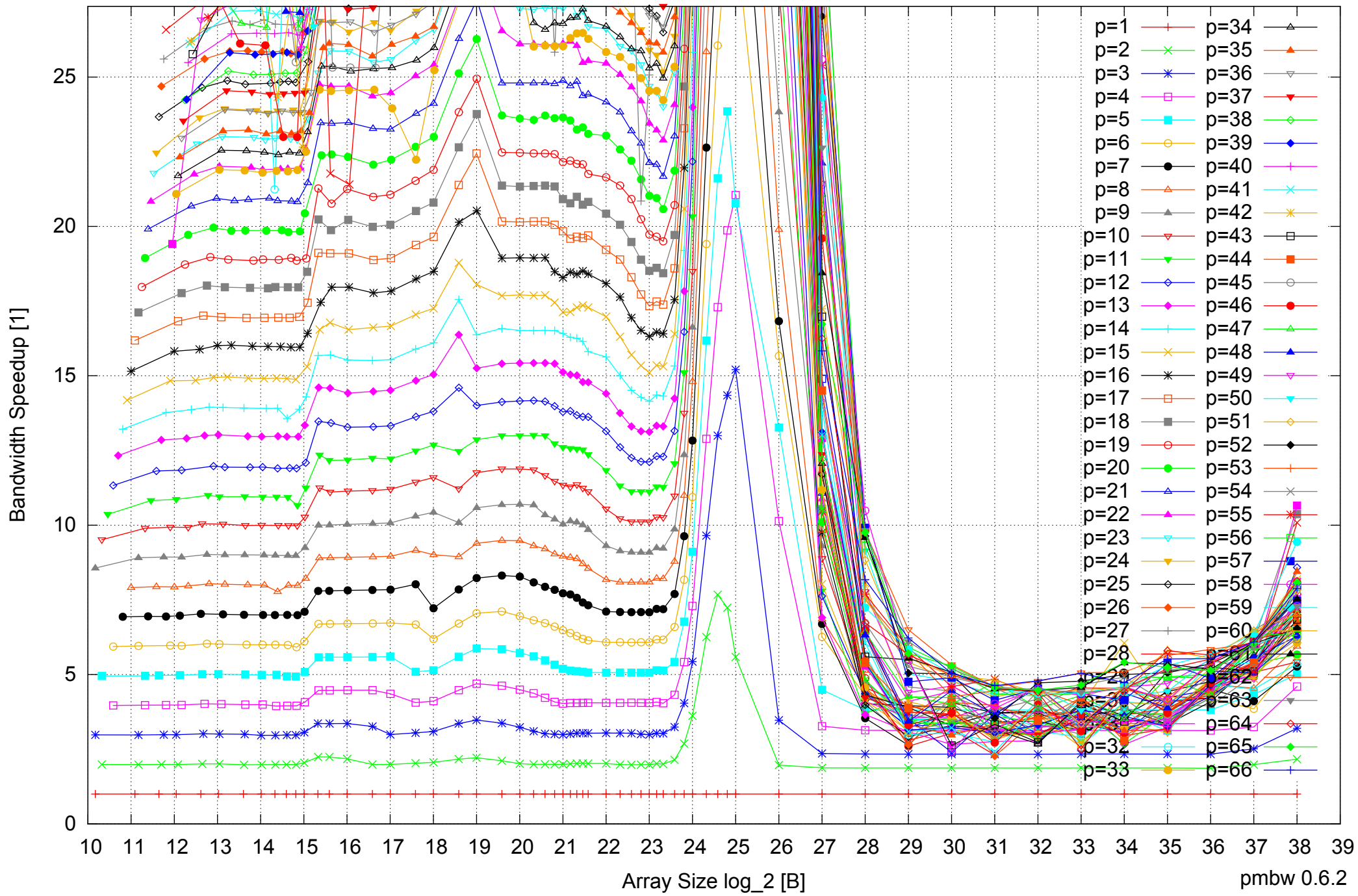
Intel Xeon E5-4640 512GB - Speedup of Parallel Memory Bandwidth (enlarged) - ScanWrite64PtrUnrollLoop
