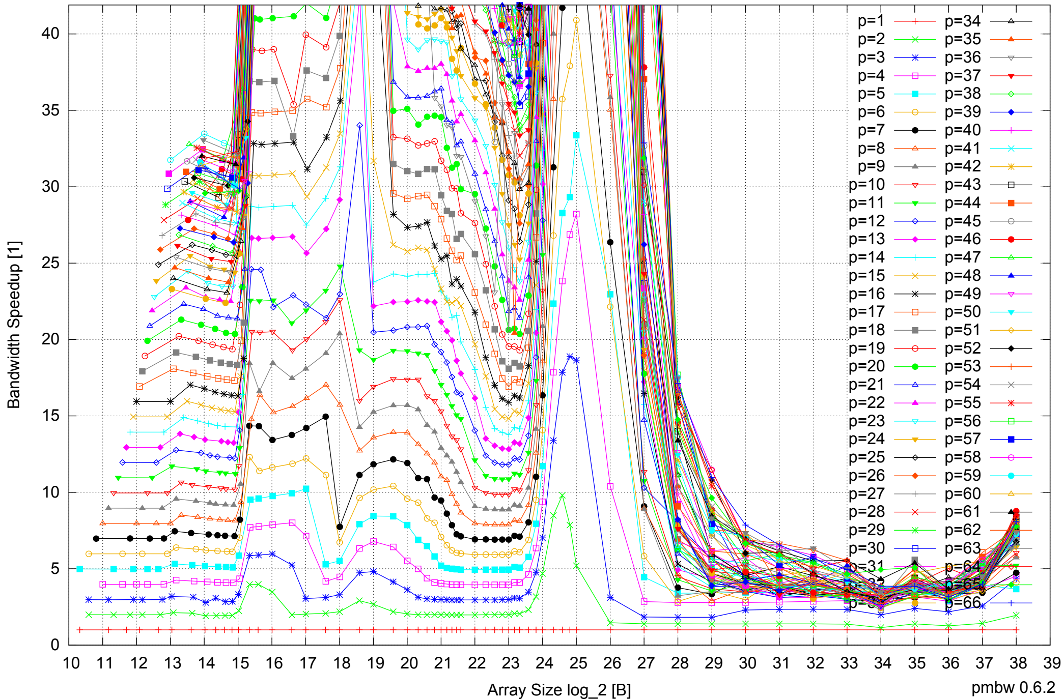
Intel Xeon E5-4640 512GB - Speedup of Parallel Memory Bandwidth (enlarged) - ScanRead128PtrUnrollLoop
