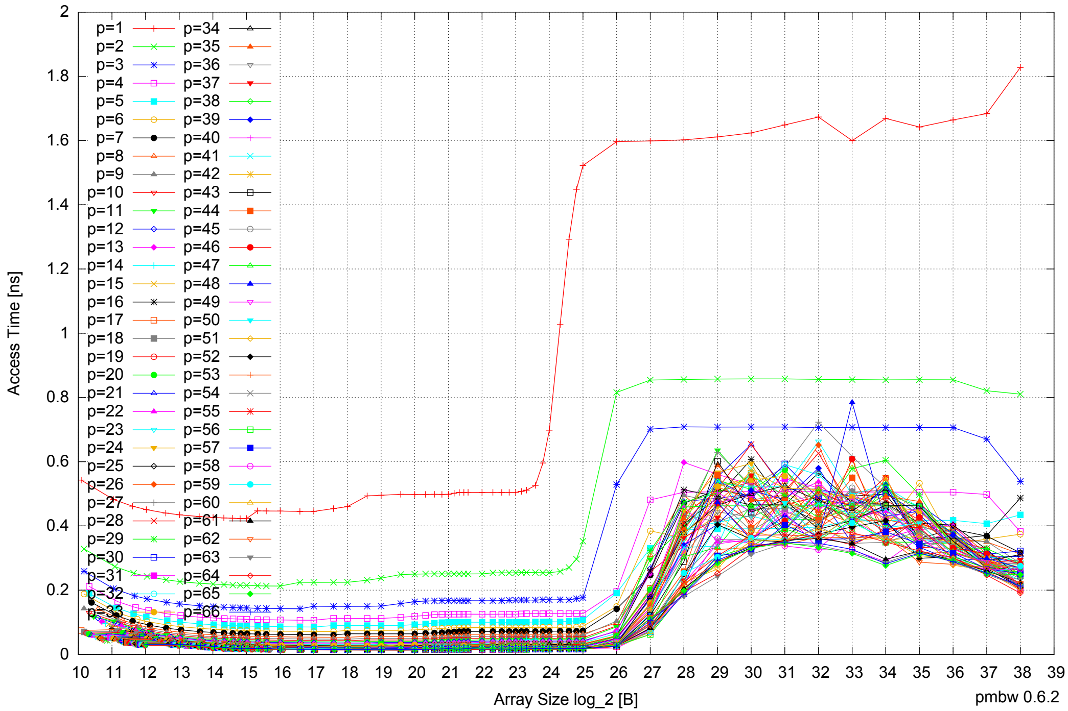
Intel Xeon E5-4640 512GB - Parallel Memory Access Time - ScanWrite32PtrSimpleLoop
