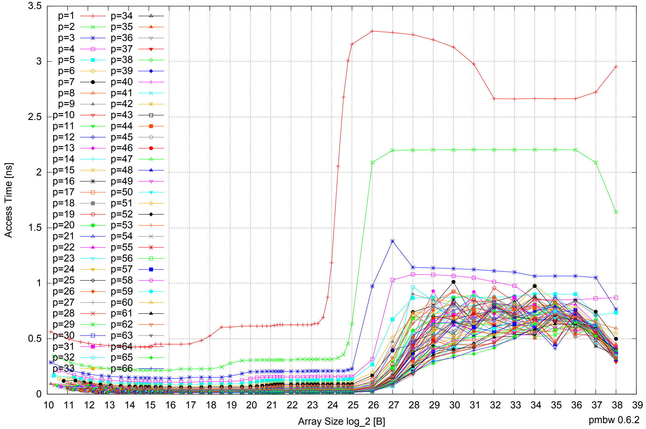
Intel Xeon E5-4640 512GB - Parallel Memory Access Time - ScanRead64IndexSimpleLoop
