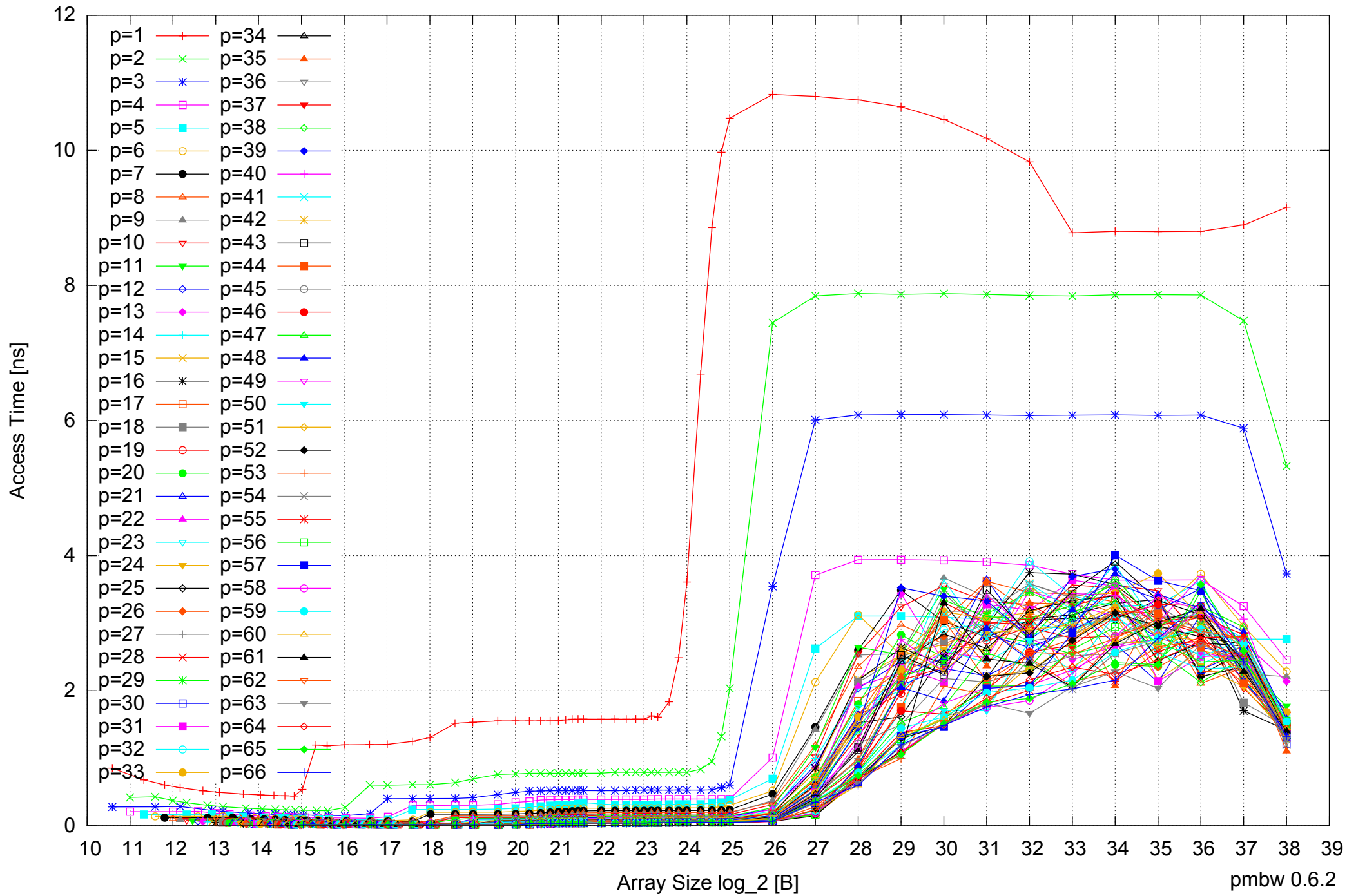
Intel Xeon E5-4640 512GB - Parallel Memory Access Time - ScanRead256PtrSimpleLoop
