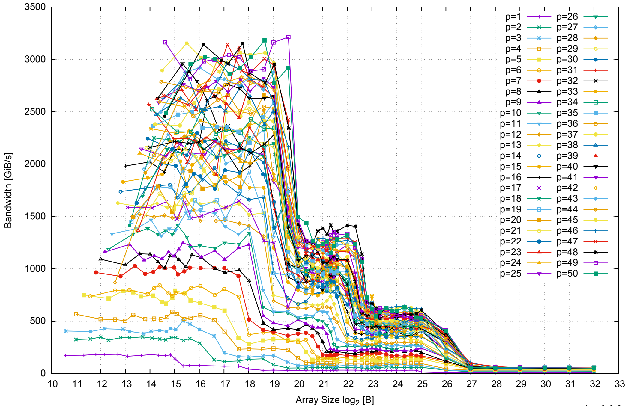
Intel Xeon E5-2670v3 256GB - Parallel Memory Bandwidth - ScanRead256PtrUnrollLoop
