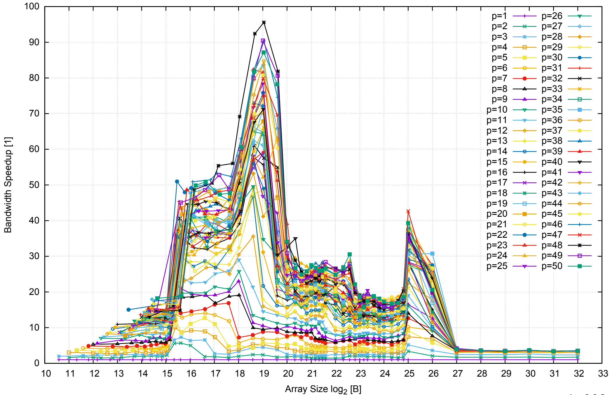
Intel Xeon E5-2670v3 256GB - Speedup of Parallel Memory Bandwidth - ScanWrite256PtrUnrollLoop
