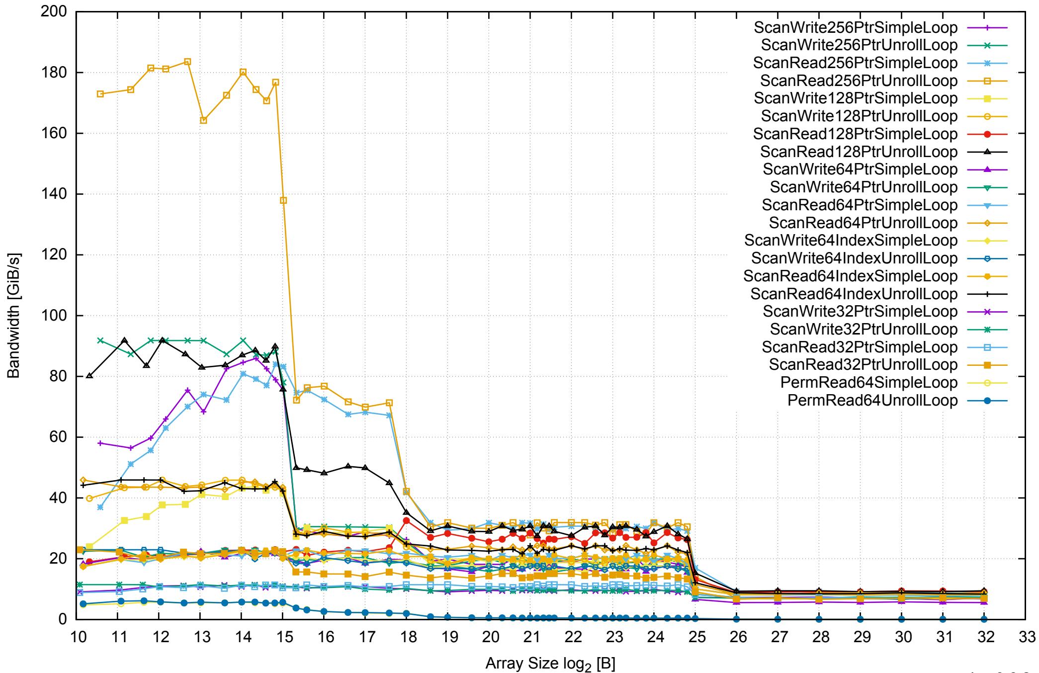
Intel Xeon E5-2670v3 256GB - One Thread Memory Bandwidth
