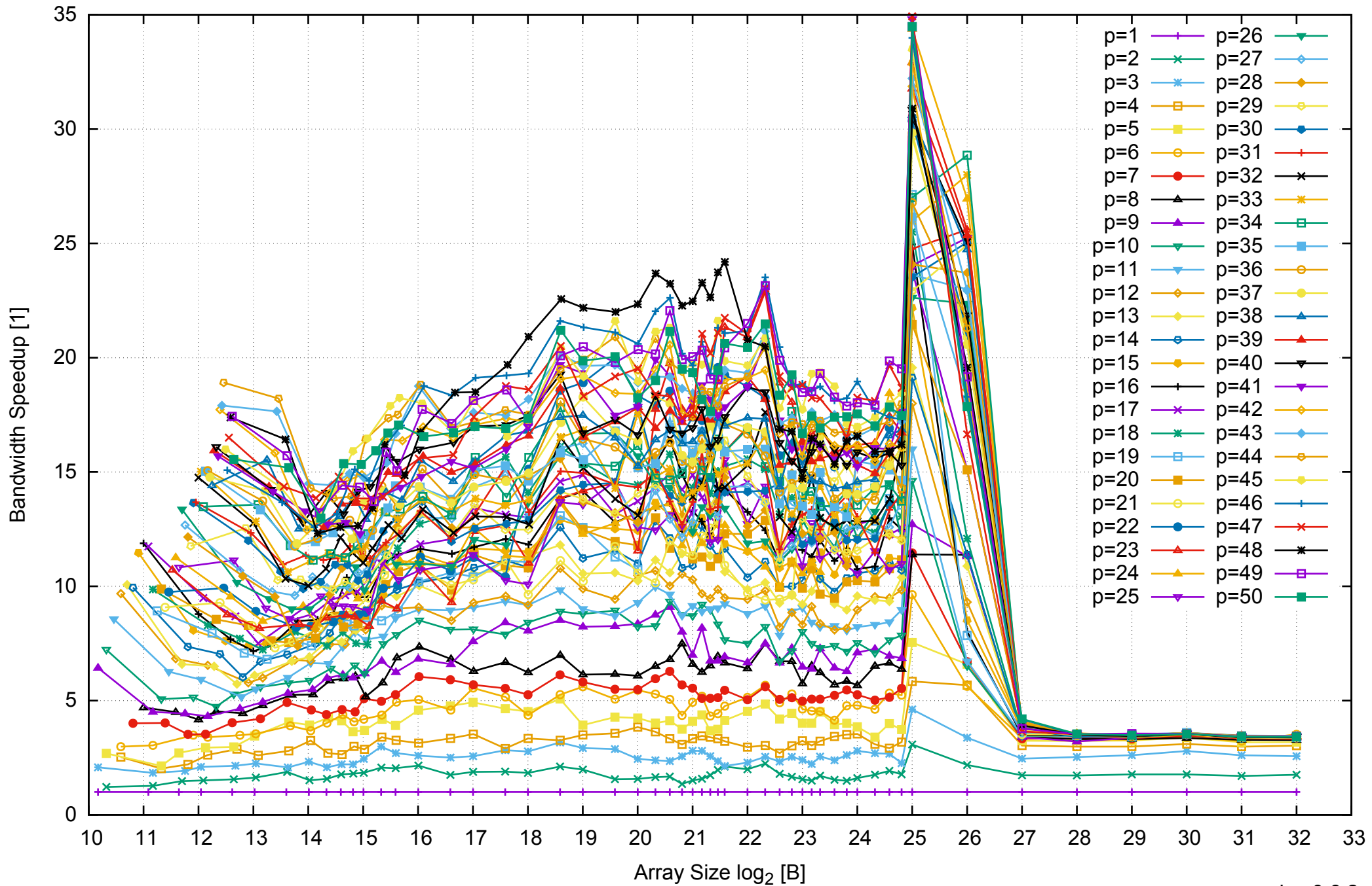
Intel Xeon E5-2670v3 256GB - Speedup of Parallel Memory Bandwidth - ScanWrite64IndexSimpleLoop
