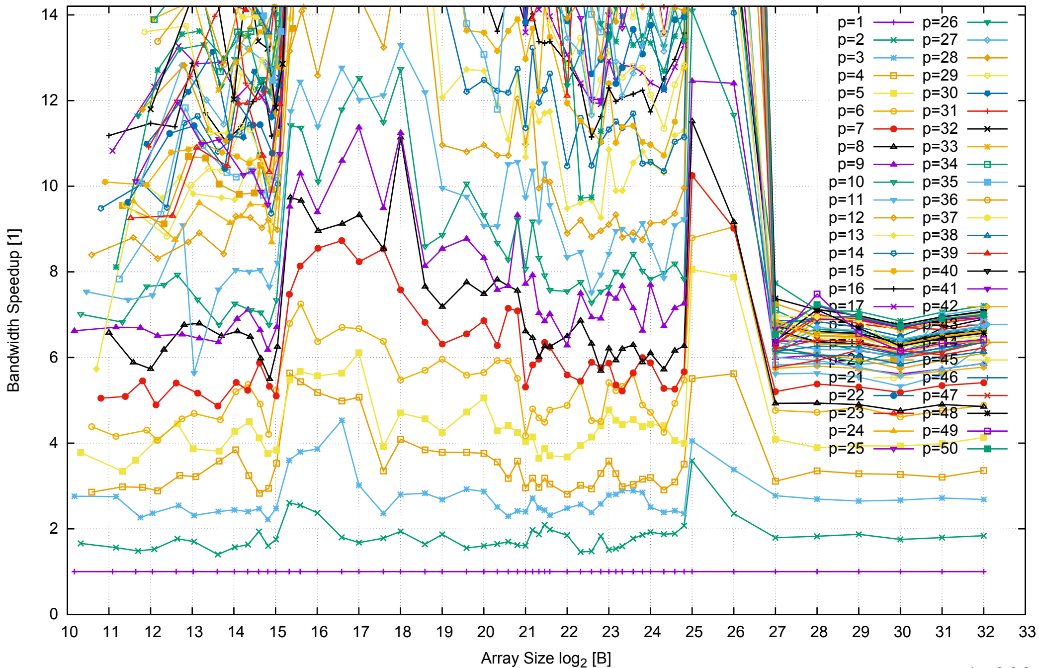
Intel Xeon E5-2670v3 256GB - Speedup of Parallel Memory Bandwidth (enlarged) - ScanRead64IndexUnrollLoop
