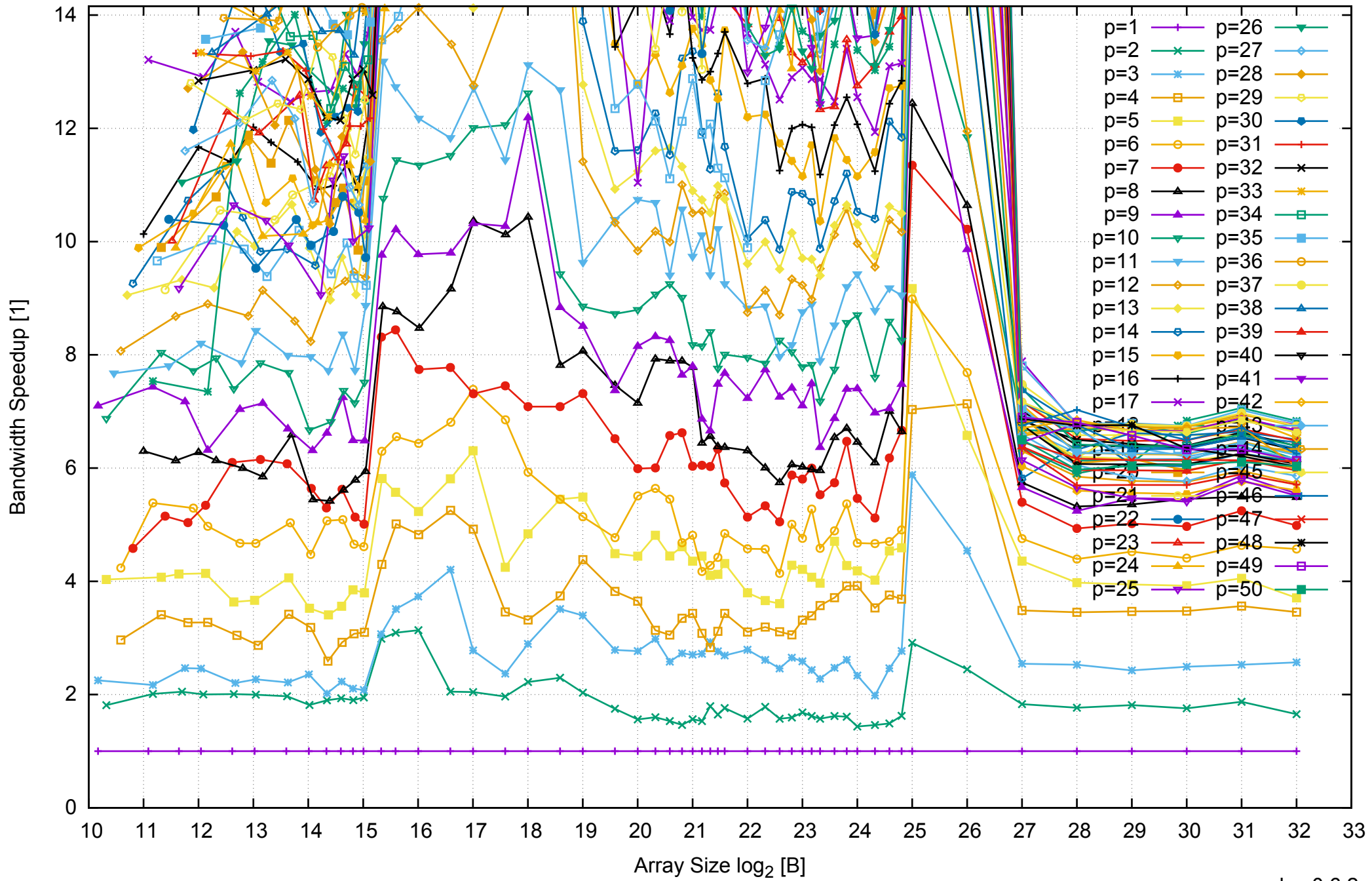
Intel Xeon E5-2670v3 256GB - Speedup of Parallel Memory Bandwidth (enlarged) - ScanRead64PtrUnrollLoop
