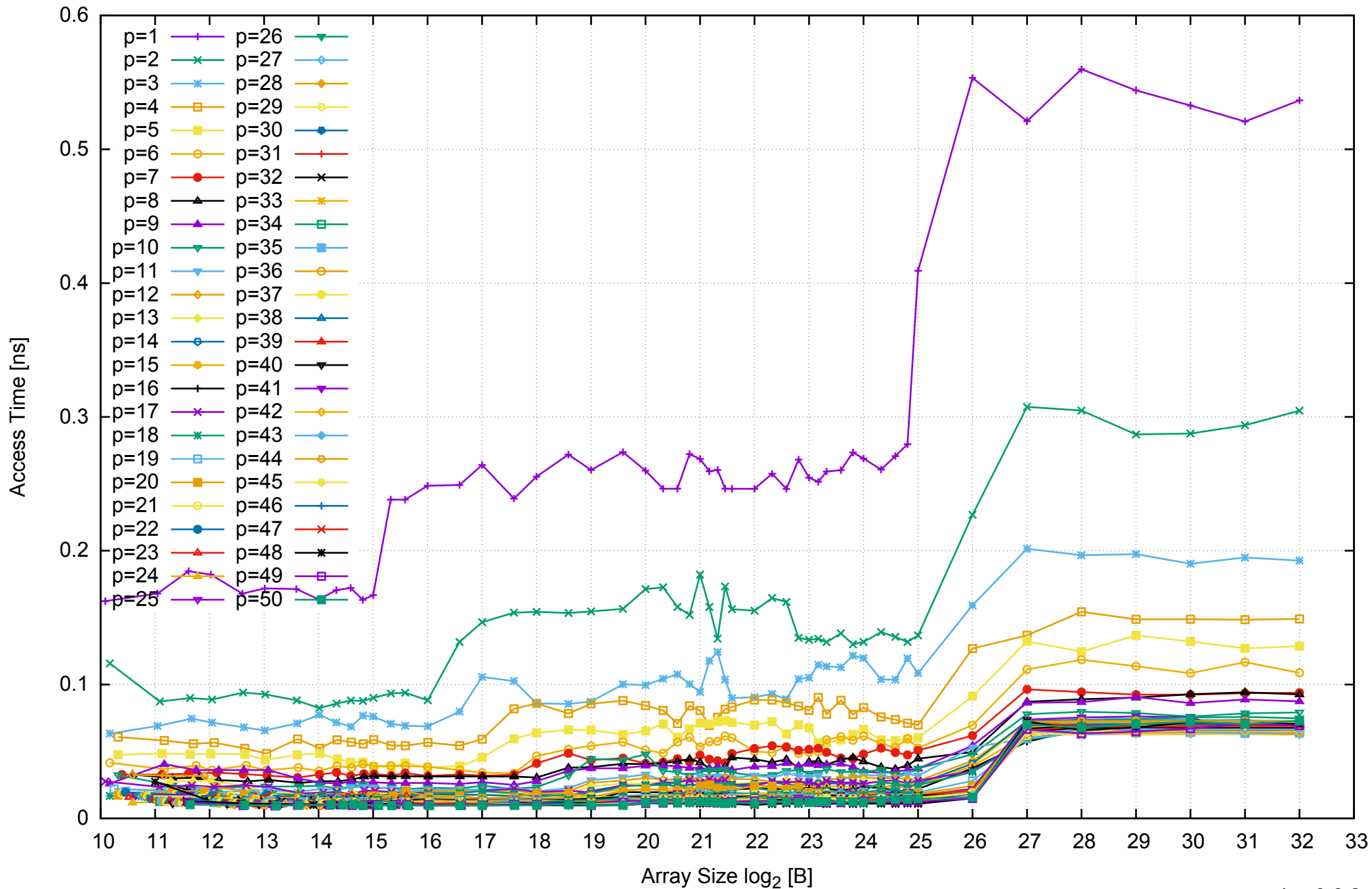
Intel Xeon E5-2670v3 256GB - Parallel Memory Access Time - ScanRead32PtrUnrollLoop
