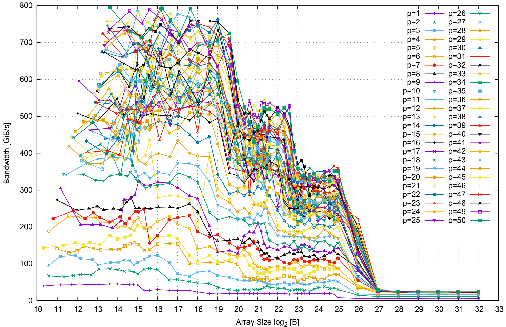
Intel Xeon E5-2670v3 256GB - Parallel Memory Bandwidth - ScanWrite128PtrUnrollLoop
