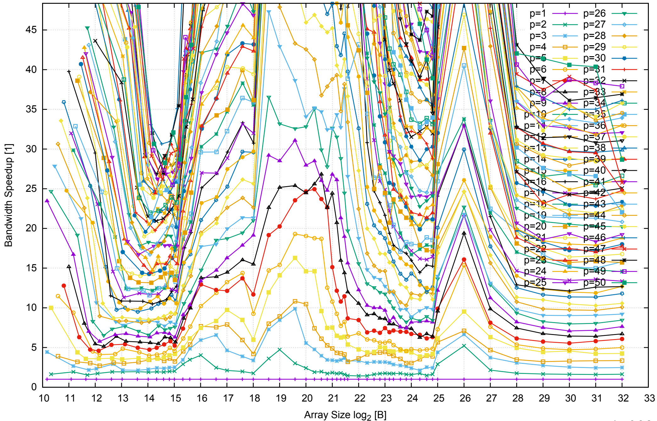
Intel Xeon E5-2670v3 256GB - Speedup of Parallel Memory Bandwidth (enlarged) - PermRead64SimpleLoop
