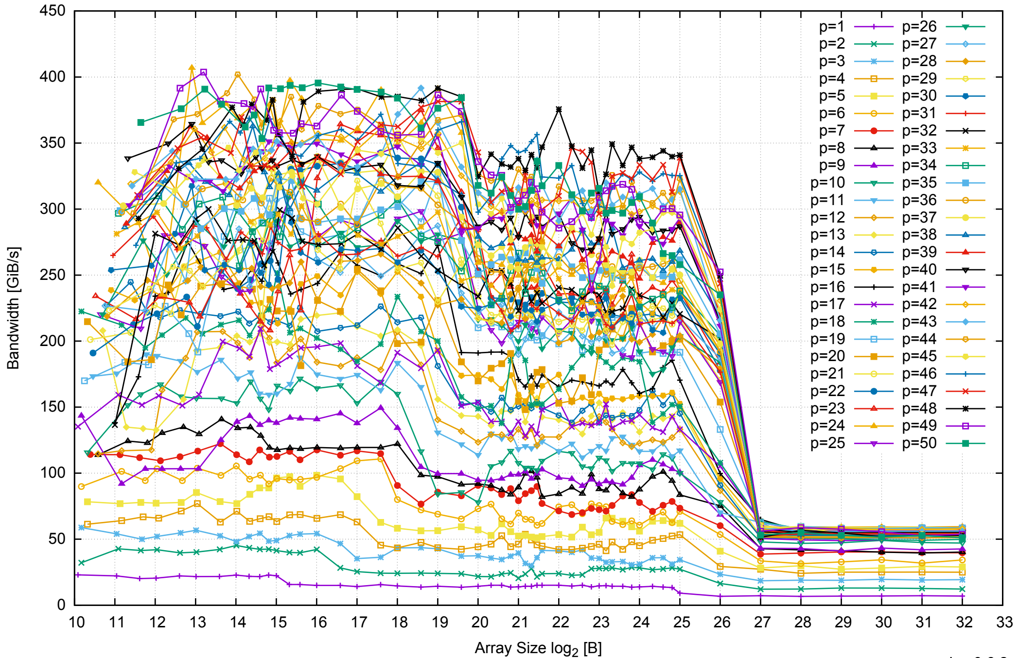
Intel Xeon E5-2670v3 256GB - Parallel Memory Bandwidth - ScanRead32PtrUnrollLoop
