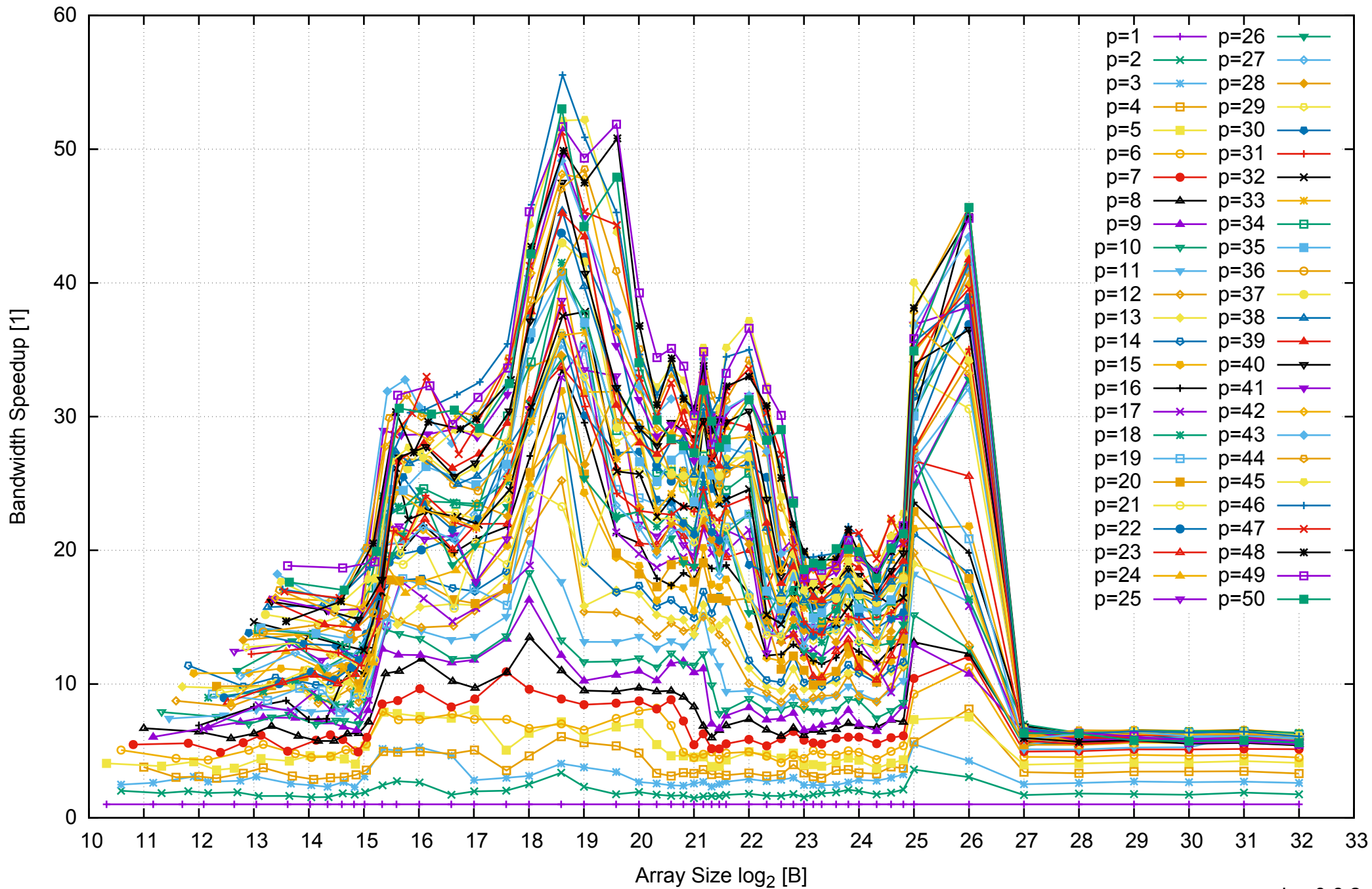
Intel Xeon E5-2670v3 256GB - Speedup of Parallel Memory Bandwidth - ScanRead128PtrUnrollLoop
