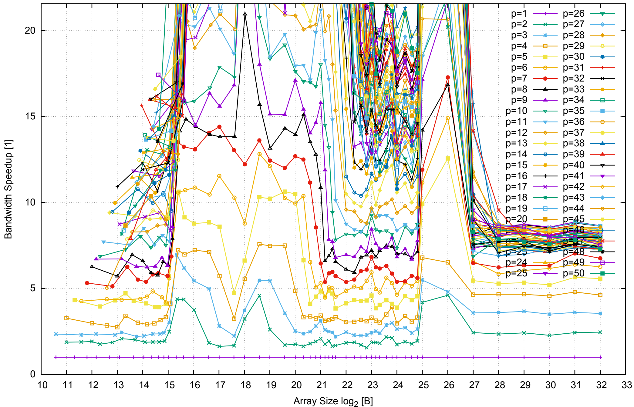
Intel Xeon E5-2670v3 256GB - Speedup of Parallel Memory Bandwidth (enlarged) - ScanRead256PtrUnrollLoop
