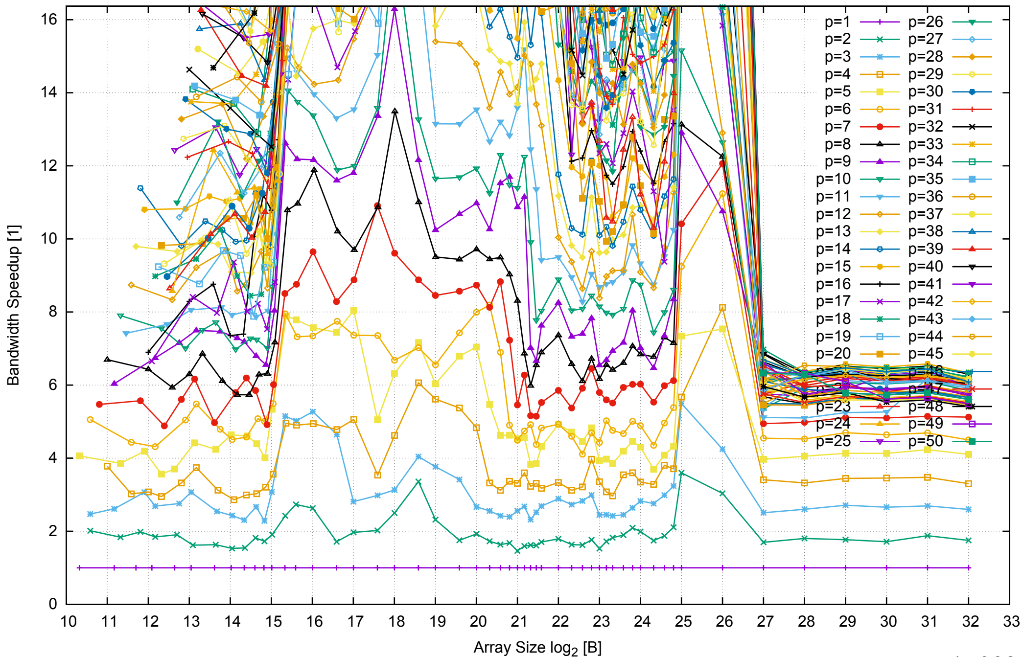
Intel Xeon E5-2670v3 256GB - Speedup of Parallel Memory Bandwidth (enlarged) - ScanRead128PtrUnrollLoop
