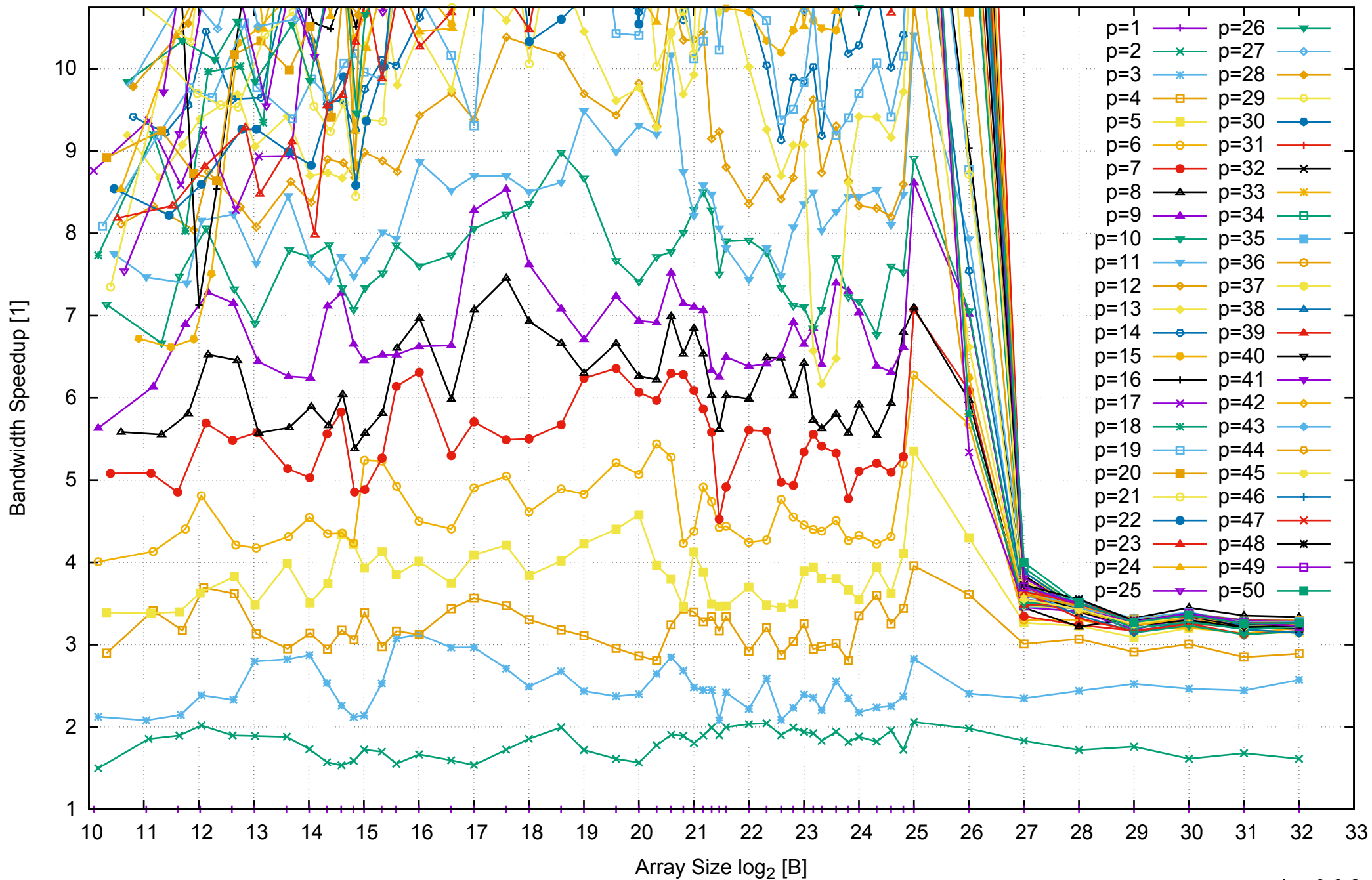
Intel Xeon E5-2670v3 256GB - Speedup of Parallel Memory Bandwidth (enlarged) - ScanWrite32PtrUnrollLoop
