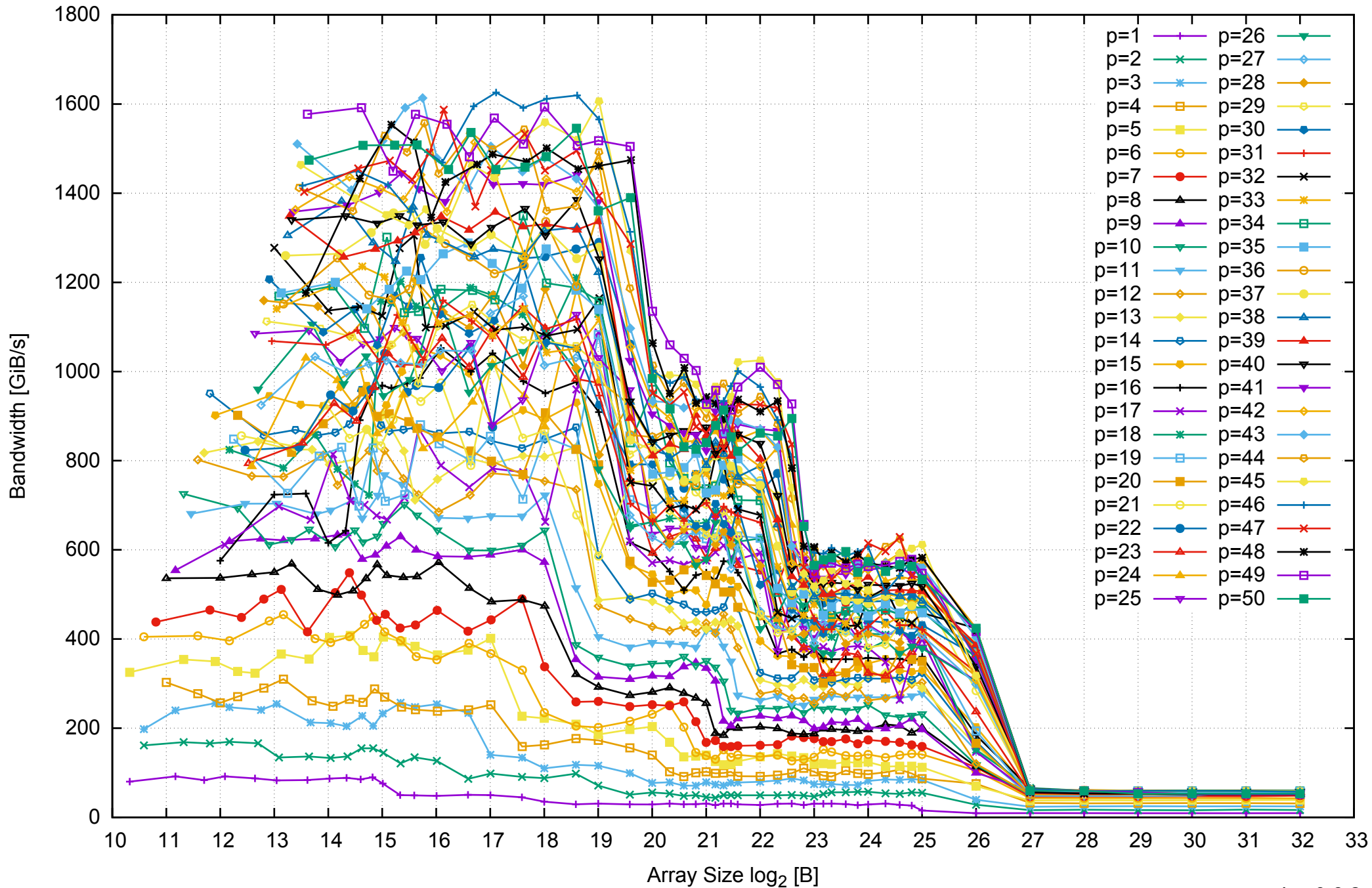
Intel Xeon E5-2670v3 256GB - Parallel Memory Bandwidth - ScanRead128PtrUnrollLoop
