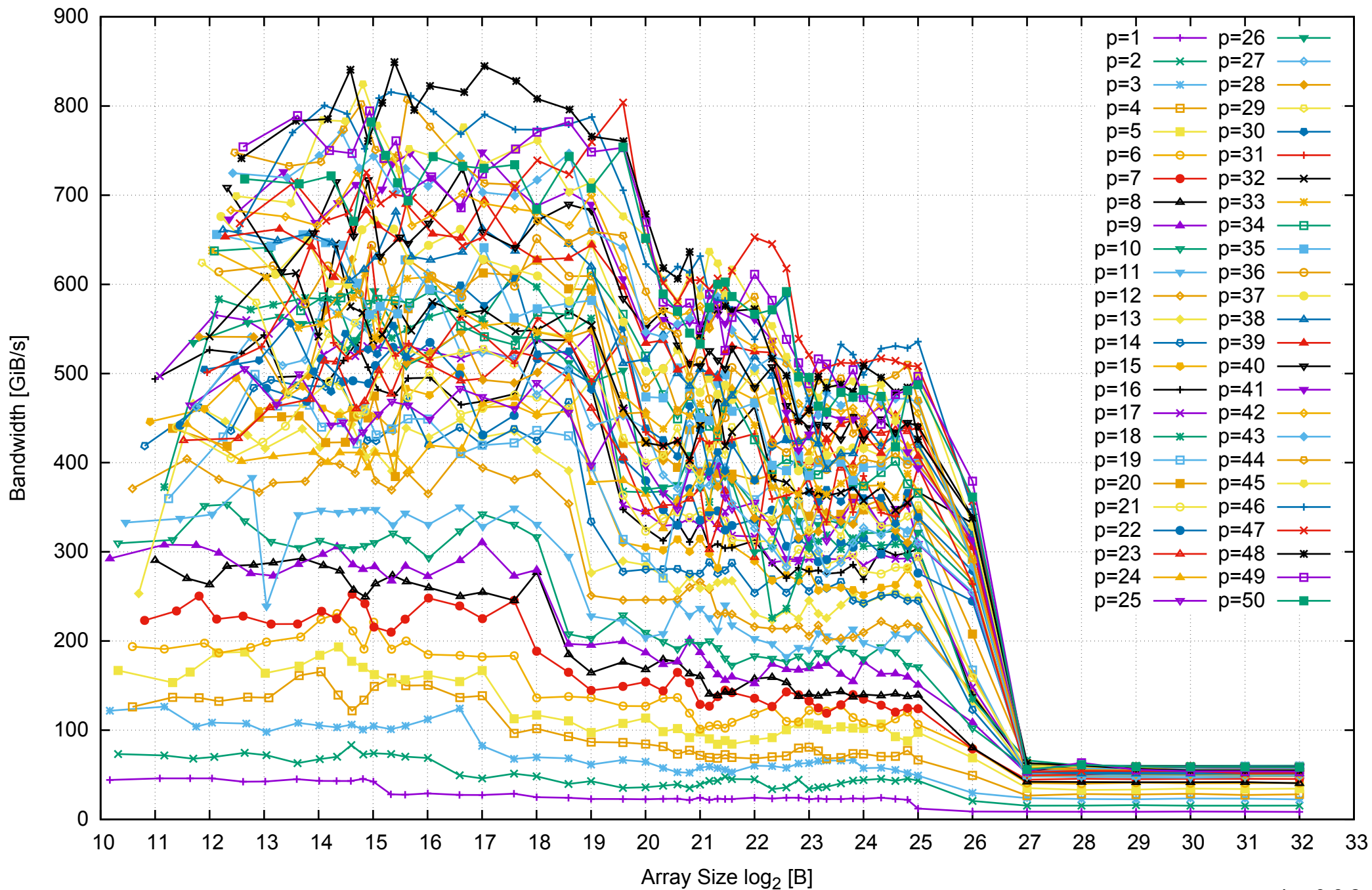
Intel Xeon E5-2670v3 256GB - Parallel Memory Bandwidth - ScanRead64IndexUnrollLoop
