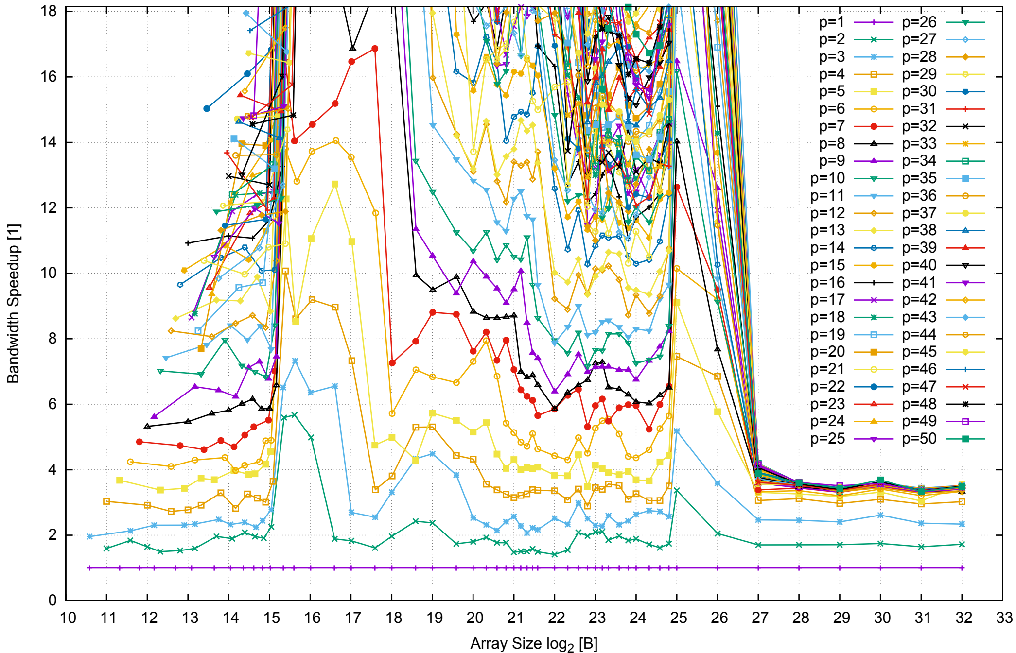
Intel Xeon E5-2670v3 256GB - Speedup of Parallel Memory Bandwidth (enlarged) - ScanWrite256PtrUnrollLoop
