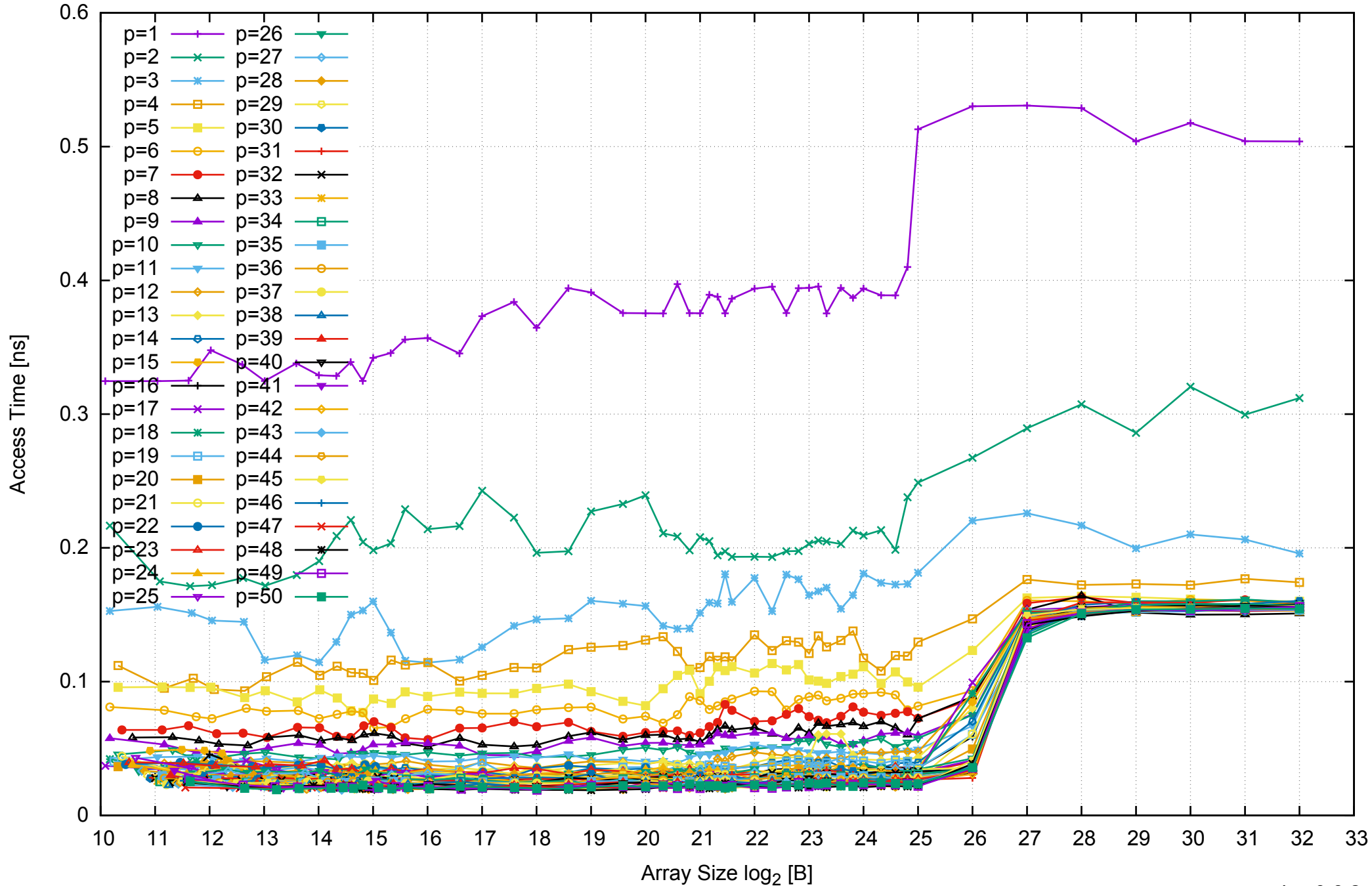
Intel Xeon E5-2670v3 256GB - Parallel Memory Access Time - ScanWrite32PtrUnrollLoop
