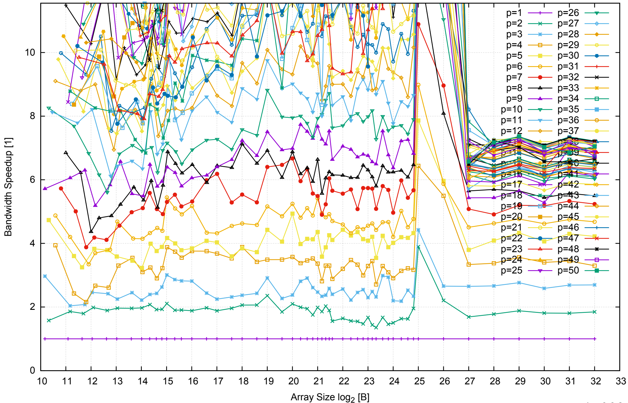
Intel Xeon E5-2670v3 256GB - Speedup of Parallel Memory Bandwidth (enlarged) - ScanRead64IndexSimpleLoop
