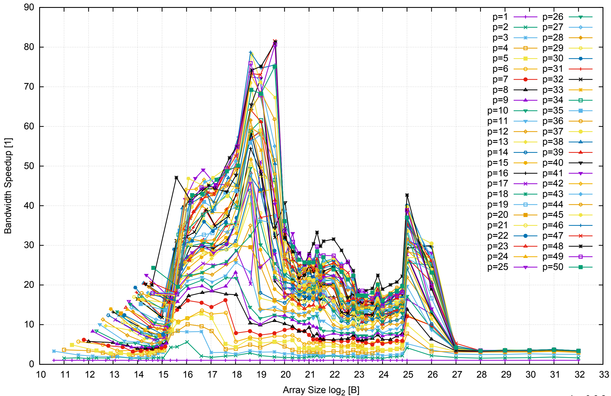
Intel Xeon E5-2670v3 256GB - Speedup of Parallel Memory Bandwidth - ScanWrite256PtrSimpleLoop
