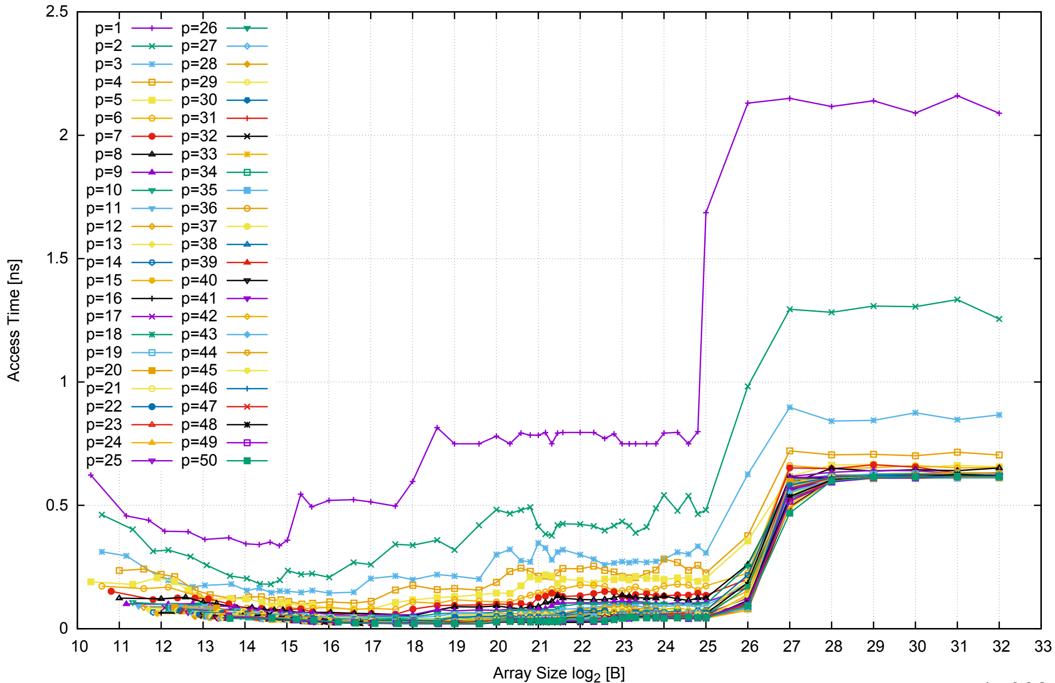
Intel Xeon E5-2670v3 256GB - Parallel Memory Access Time - ScanWrite128PtrSimpleLoop
