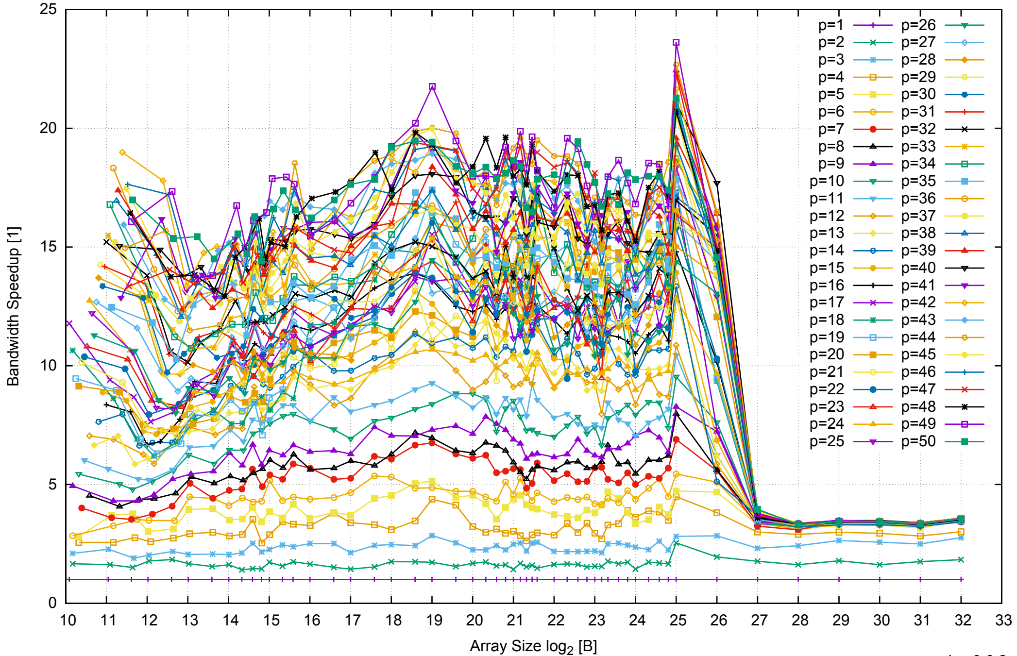
Intel Xeon E5-2670v3 256GB - Speedup of Parallel Memory Bandwidth - ScanWrite32PtrSimpleLoop
