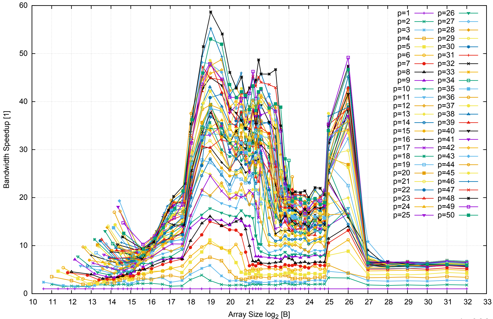
Intel Xeon E5-2670v3 256GB - Speedup of Parallel Memory Bandwidth - ScanRead256PtrSimpleLoop
