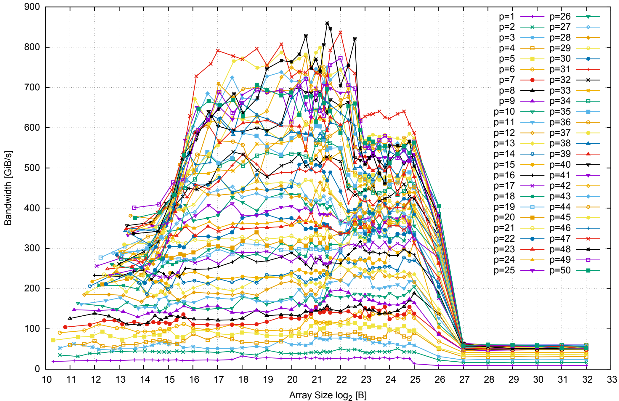
Intel Xeon E5-2670v3 256GB - Parallel Memory Bandwidth - ScanRead128PtrSimpleLoop
