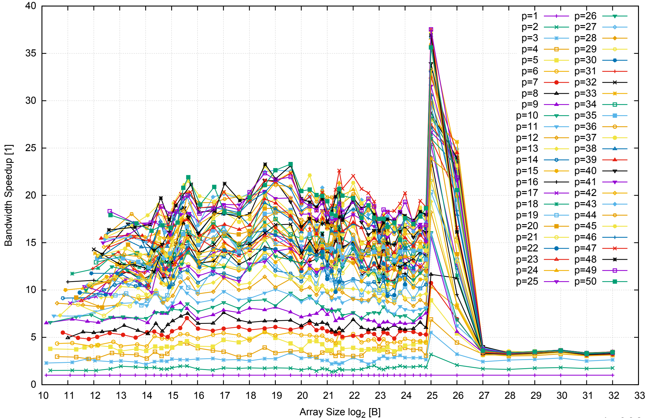
Intel Xeon E5-2670v3 256GB - Speedup of Parallel Memory Bandwidth - ScanWrite64IndexUnrollLoop
