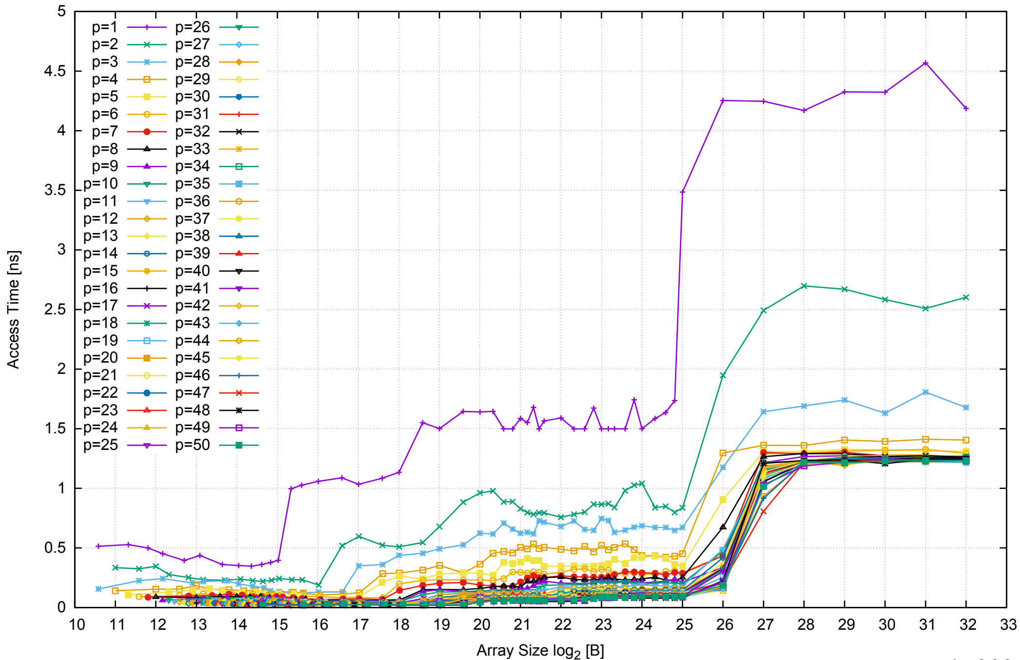
Intel Xeon E5-2670v3 256GB - Parallel Memory Access Time - ScanWrite256PtrSimpleLoop
