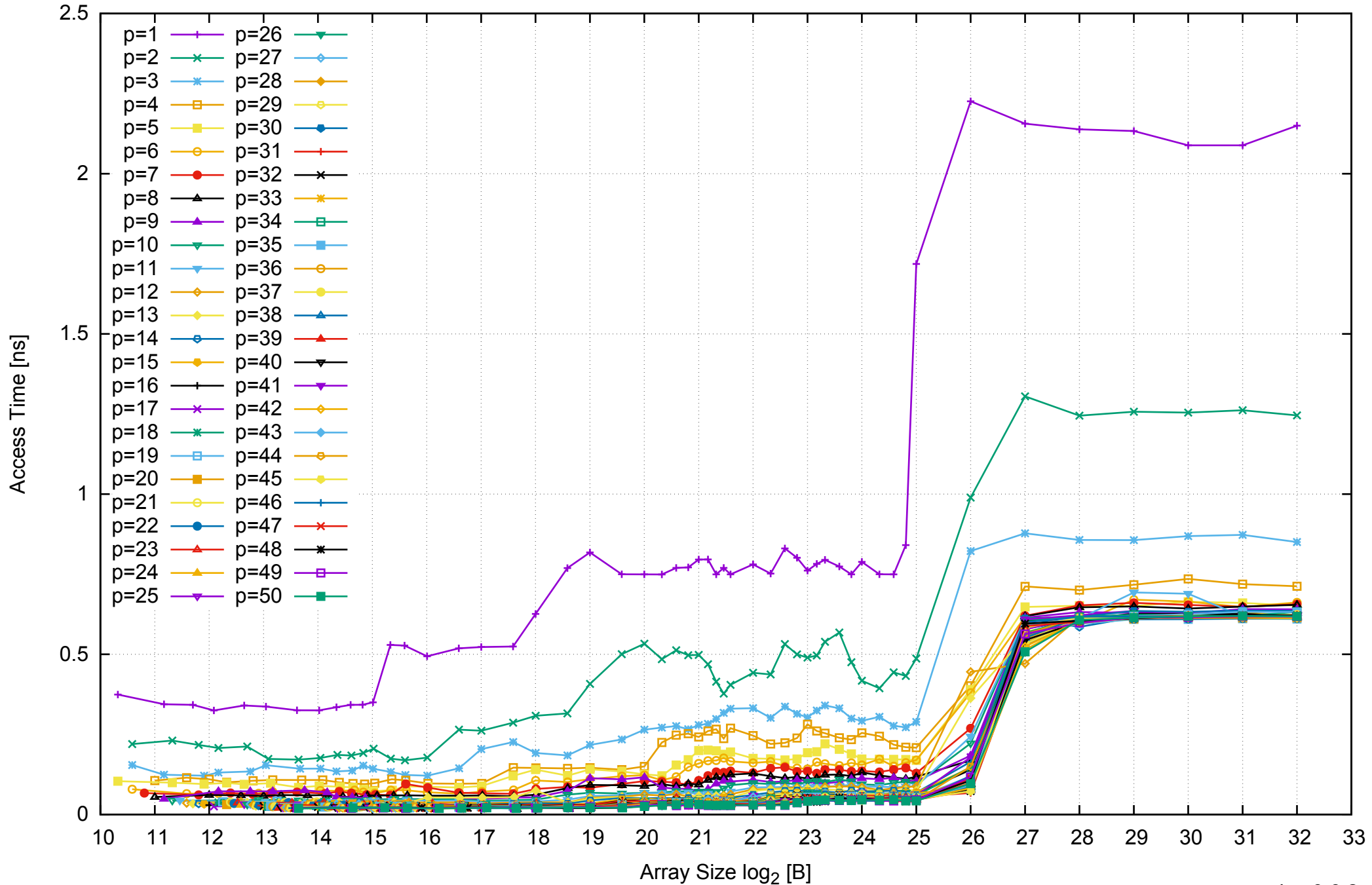
Intel Xeon E5-2670v3 256GB - Parallel Memory Access Time - ScanWrite128PtrUnrollLoop
