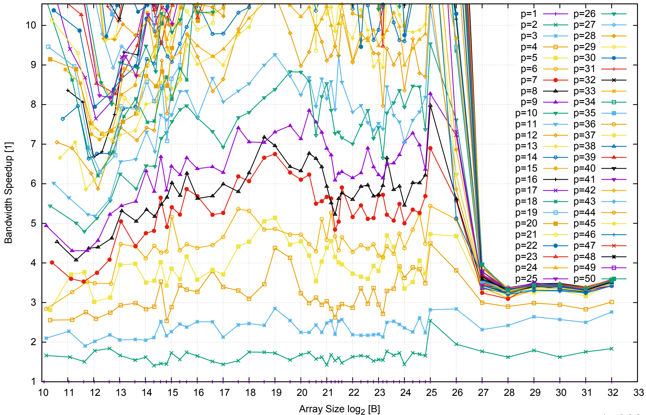
Intel Xeon E5-2670v3 256GB - Speedup of Parallel Memory Bandwidth (enlarged) - ScanWrite32PtrSimpleLoop
