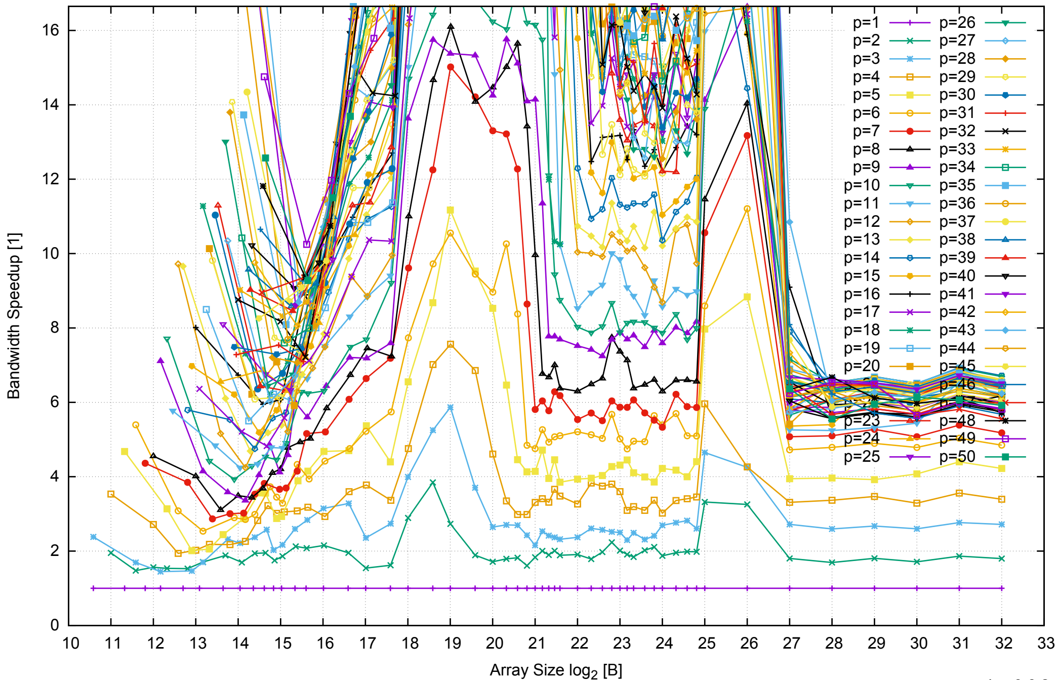
Intel Xeon E5-2670v3 256GB - Speedup of Parallel Memory Bandwidth (enlarged) - ScanRead256PtrSimpleLoop
