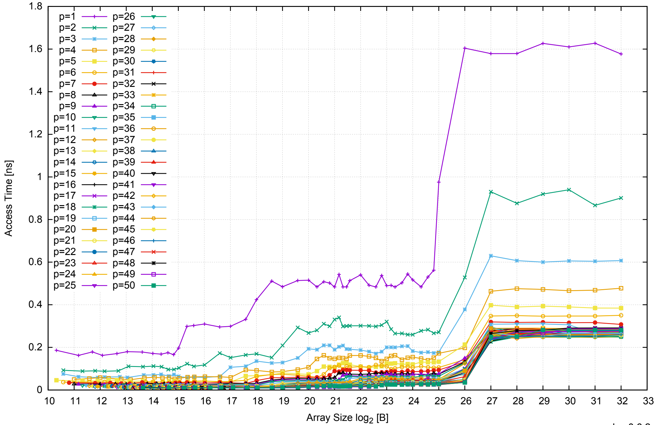
Intel Xeon E5-2670v3 256GB - Parallel Memory Access Time - ScanRead128PtrUnrollLoop
