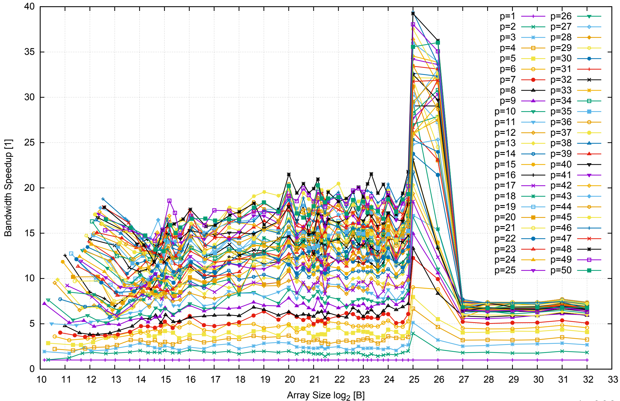
Intel Xeon E5-2670v3 256GB - Speedup of Parallel Memory Bandwidth - ScanRead64PtrSimpleLoop
