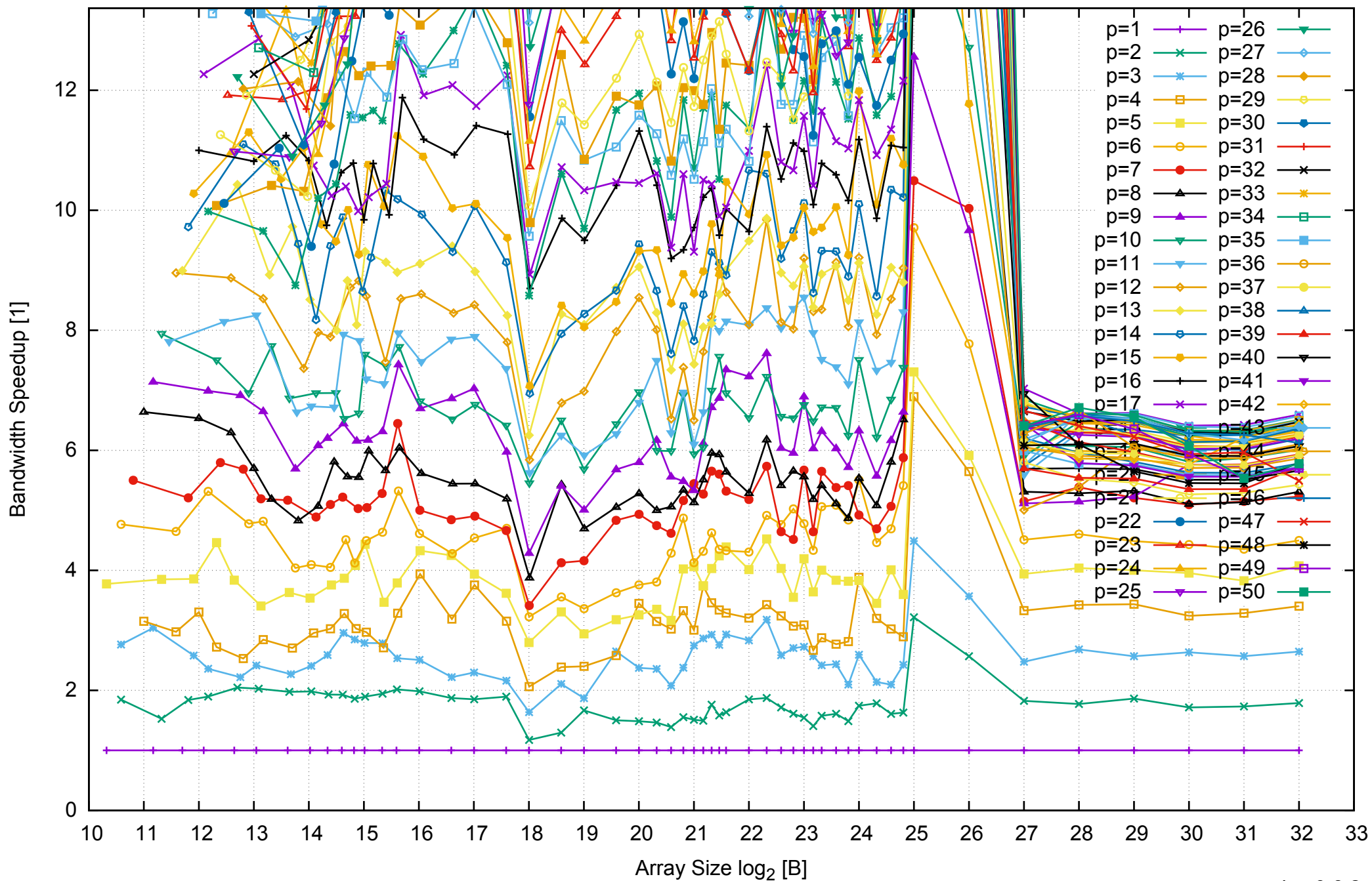
Intel Xeon E5-2670v3 256GB - Speedup of Parallel Memory Bandwidth (enlarged) - ScanRead128PtrSimpleLoop
