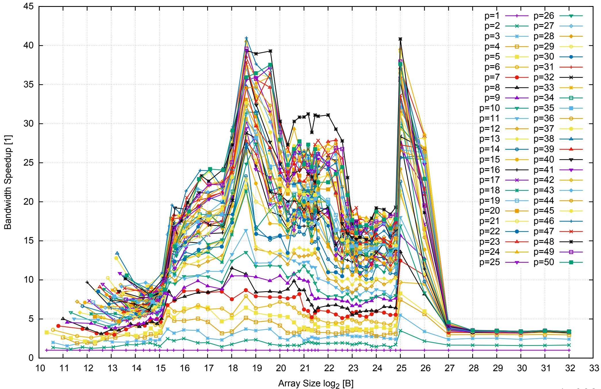
Intel Xeon E5-2670v3 256GB - Speedup of Parallel Memory Bandwidth - ScanWrite128PtrSimpleLoop
