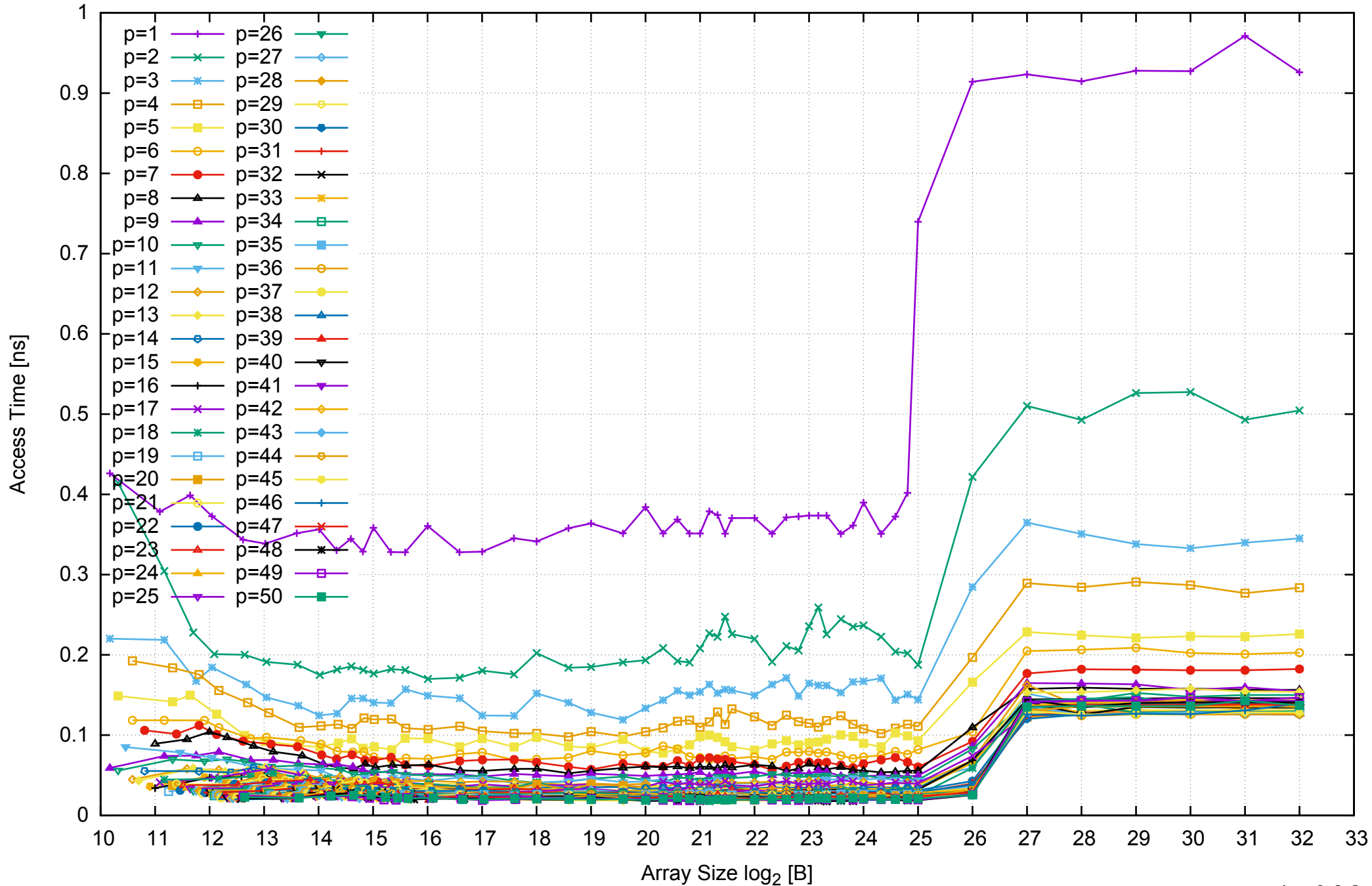
Intel Xeon E5-2670v3 256GB - Parallel Memory Access Time - ScanRead64PtrSimpleLoop
