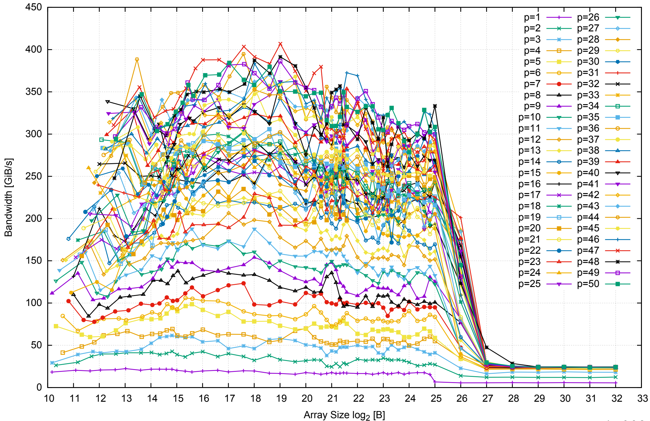
Intel Xeon E5-2670v3 256GB - Parallel Memory Bandwidth - ScanWrite64PtrSimpleLoop
