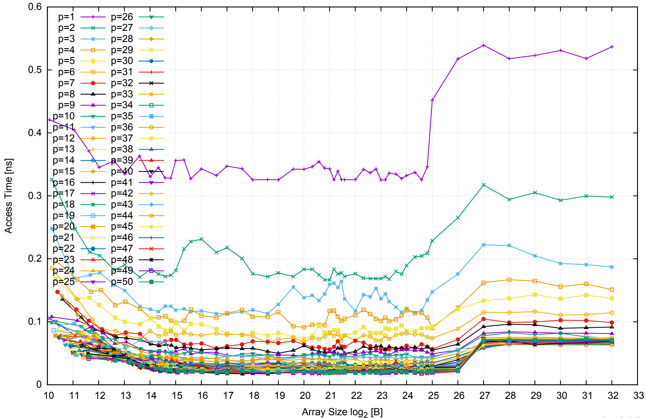
Intel Xeon E5-2670v3 256GB - Parallel Memory Access Time - ScanRead32PtrSimpleLoop
