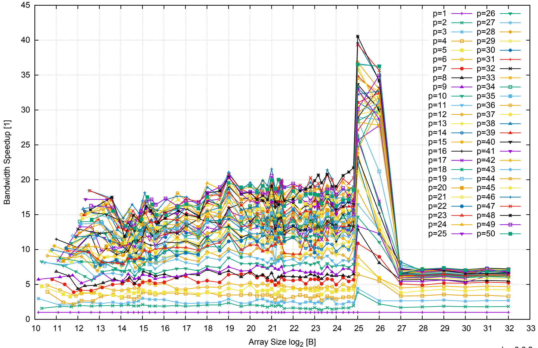
Intel Xeon E5-2670v3 256GB - Speedup of Parallel Memory Bandwidth - ScanRead64IndexSimpleLoop
