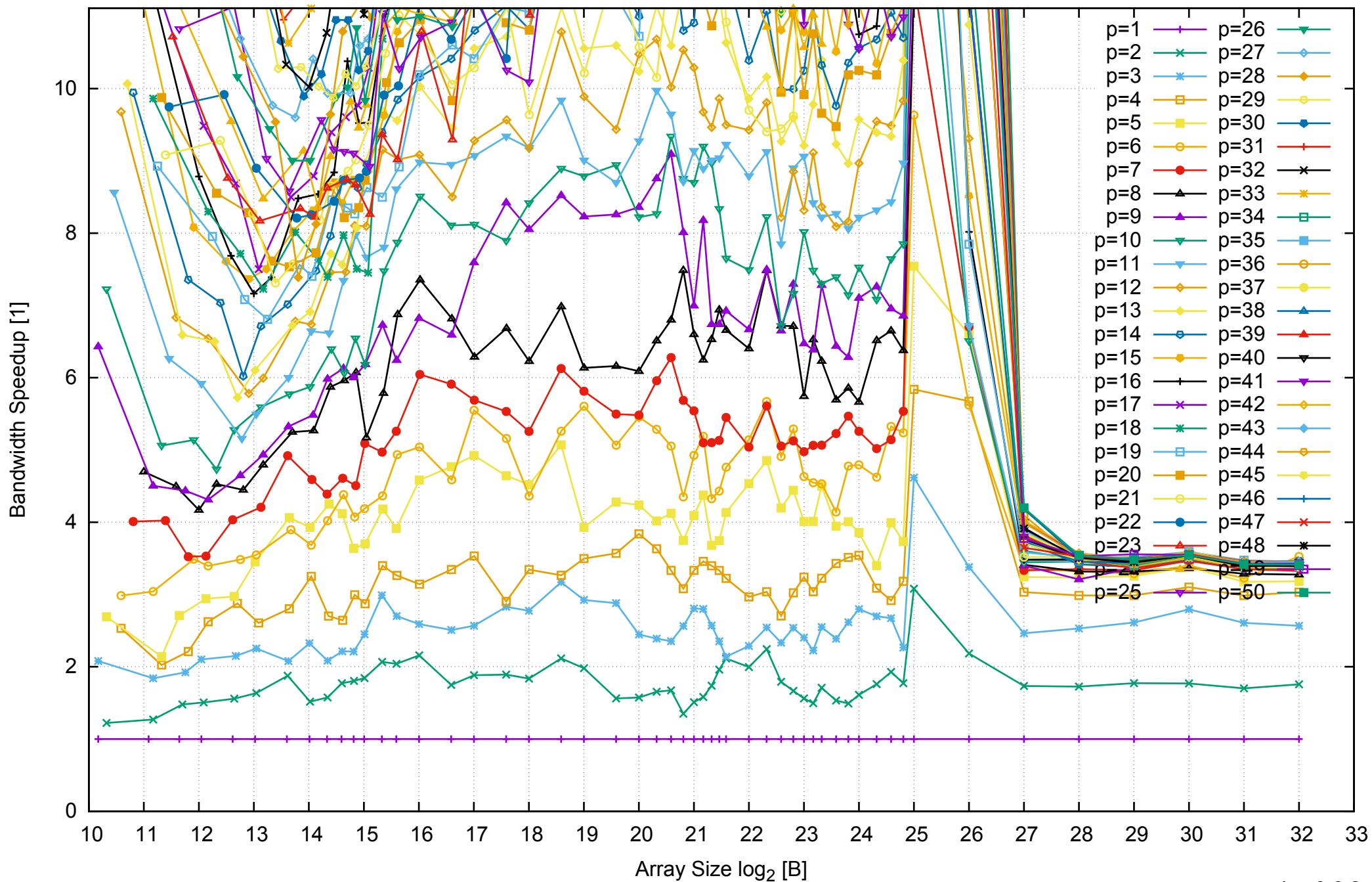
Intel Xeon E5-2670v3 256GB - Speedup of Parallel Memory Bandwidth (enlarged) - ScanWrite64IndexSimpleLoop
