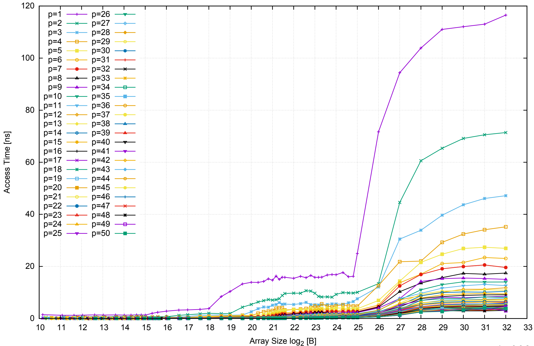
Intel Xeon E5-2670v3 256GB - Parallel Memory Access Time - PermRead64UnrollLoop
