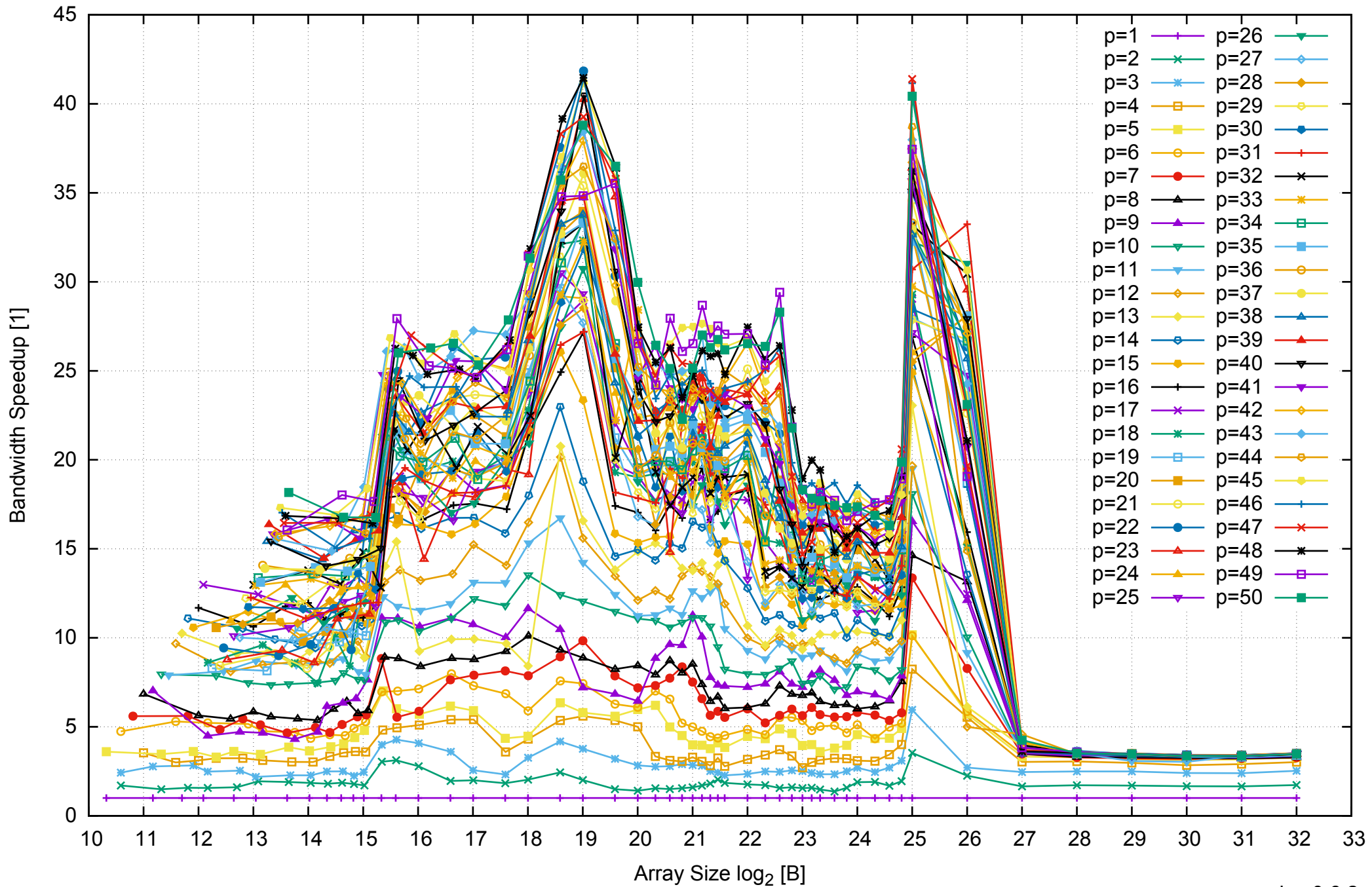
Intel Xeon E5-2670v3 256GB - Speedup of Parallel Memory Bandwidth - ScanWrite128PtrUnrollLoop
