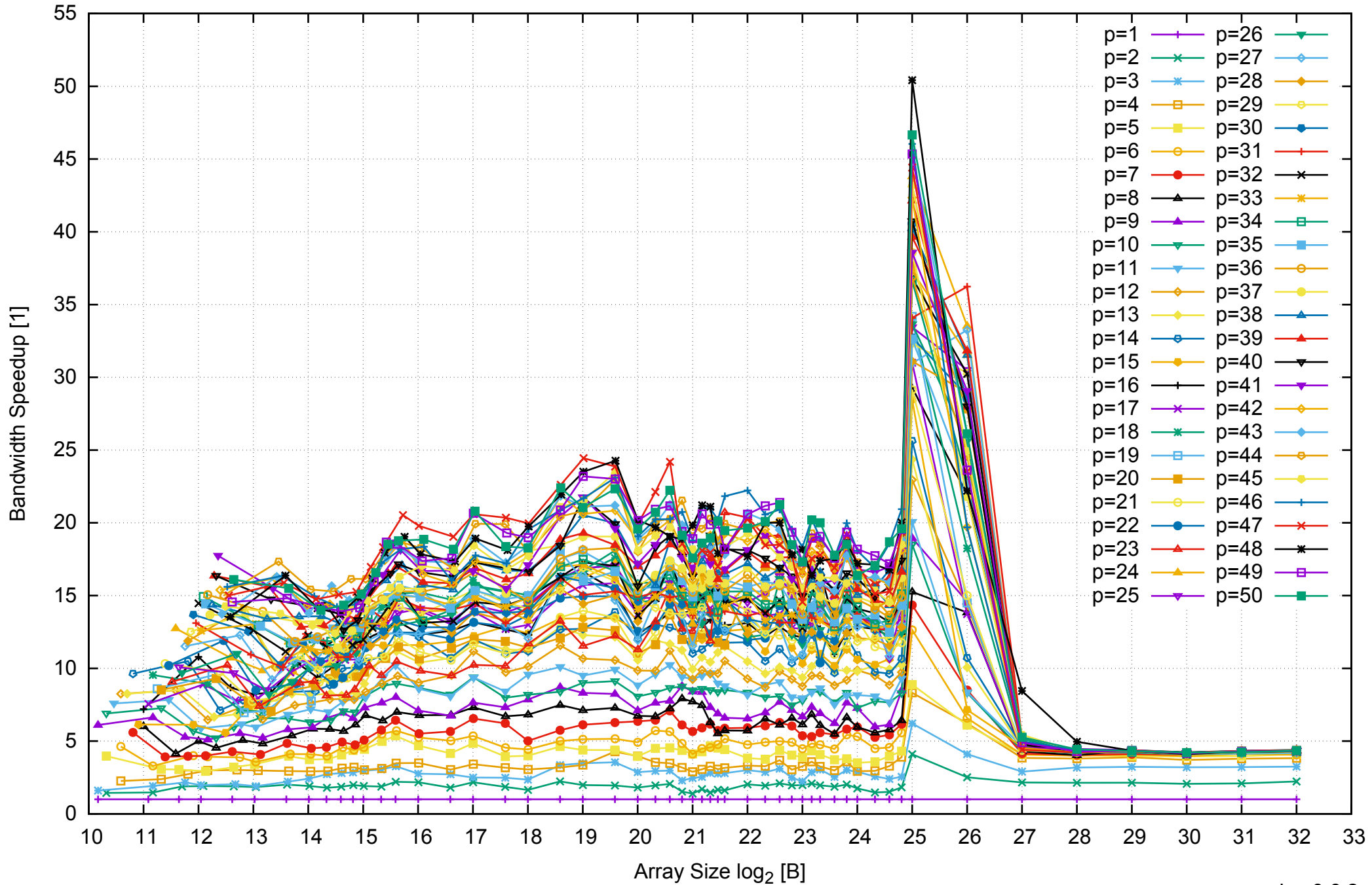
Intel Xeon E5-2670v3 256GB - Speedup of Parallel Memory Bandwidth - ScanWrite64PtrSimpleLoop
