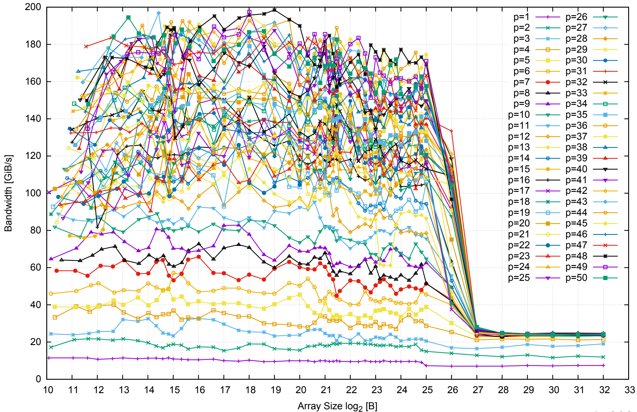
Intel Xeon E5-2670v3 256GB - Parallel Memory Bandwidth - ScanWrite32PtrUnrollLoop
