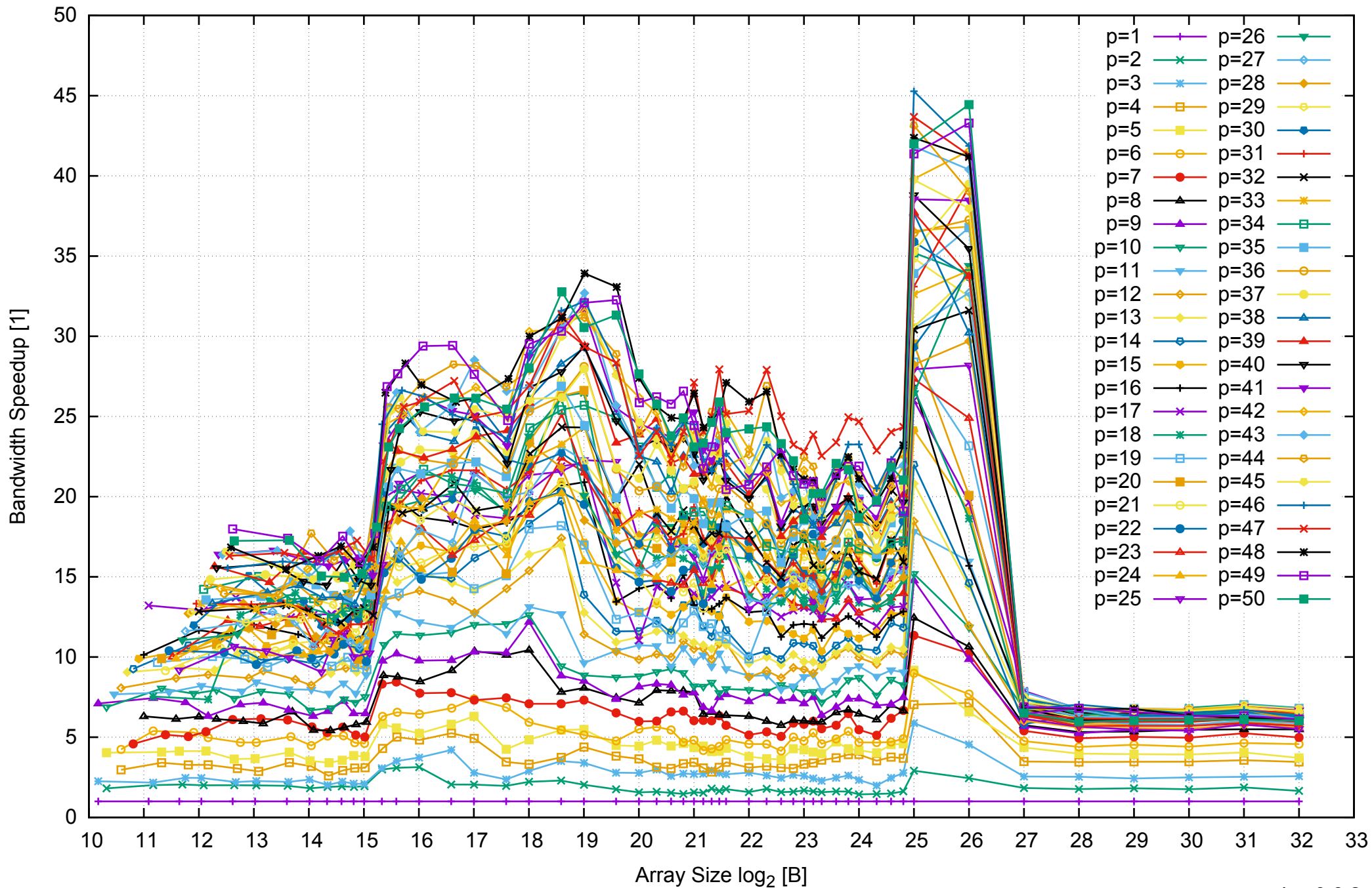
Intel Xeon E5-2670v3 256GB - Speedup of Parallel Memory Bandwidth - ScanRead64PtrUnrollLoop
