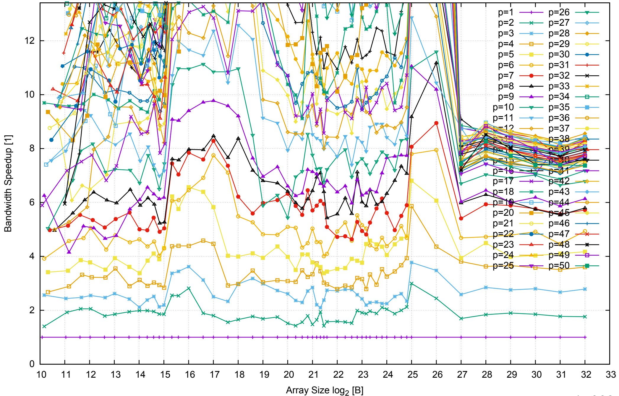
Intel Xeon E5-2670v3 256GB - Speedup of Parallel Memory Bandwidth (enlarged) - ScanRead32PtrUnrollLoop
