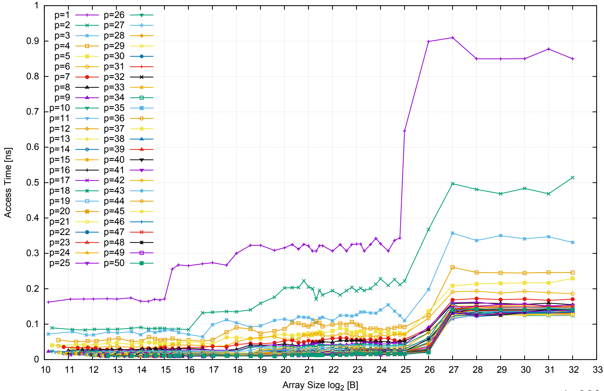
Intel Xeon E5-2670v3 256GB - Parallel Memory Access Time - ScanRead64PtrUnrollLoop
