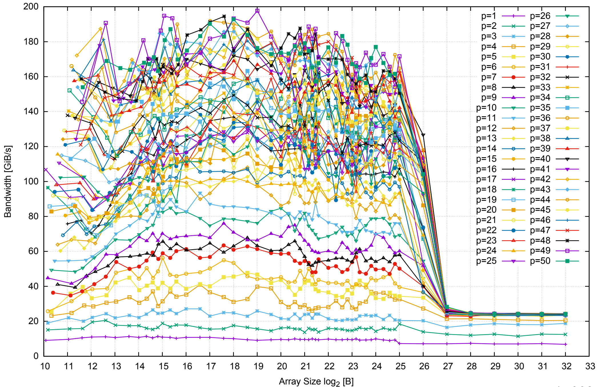
Intel Xeon E5-2670v3 256GB - Parallel Memory Bandwidth - ScanWrite32PtrSimpleLoop
