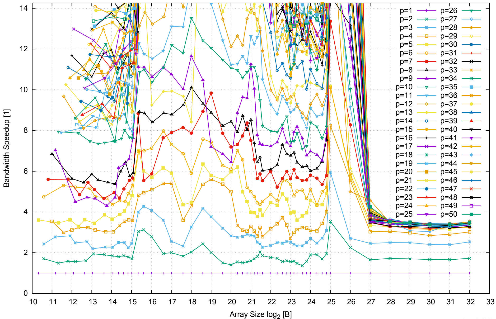
Intel Xeon E5-2670v3 256GB - Speedup of Parallel Memory Bandwidth (enlarged) - ScanWrite128PtrUnrollLoop
