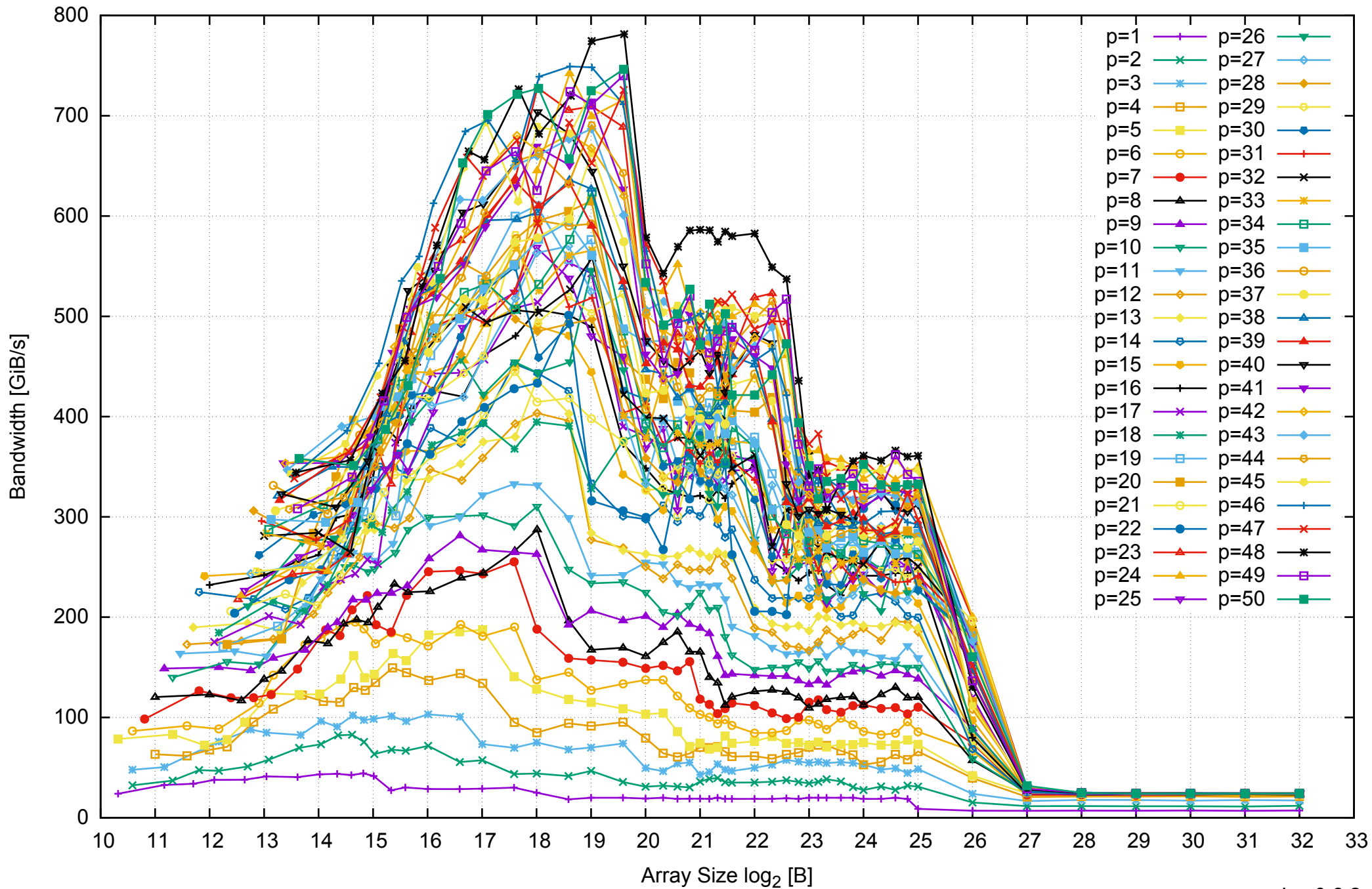
Intel Xeon E5-2670v3 256GB - Parallel Memory Bandwidth - ScanWrite128PtrSimpleLoop
