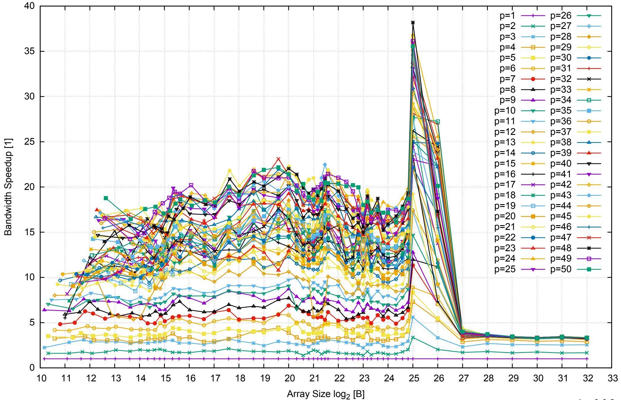
Intel Xeon E5-2670v3 256GB - Speedup of Parallel Memory Bandwidth - ScanWrite64PtrUnrollLoop
