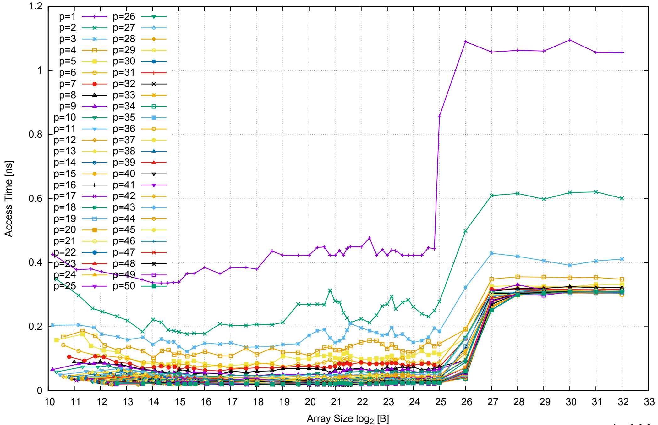
Intel Xeon E5-2670v3 256GB - Parallel Memory Access Time - ScanWrite64IndexSimpleLoop
