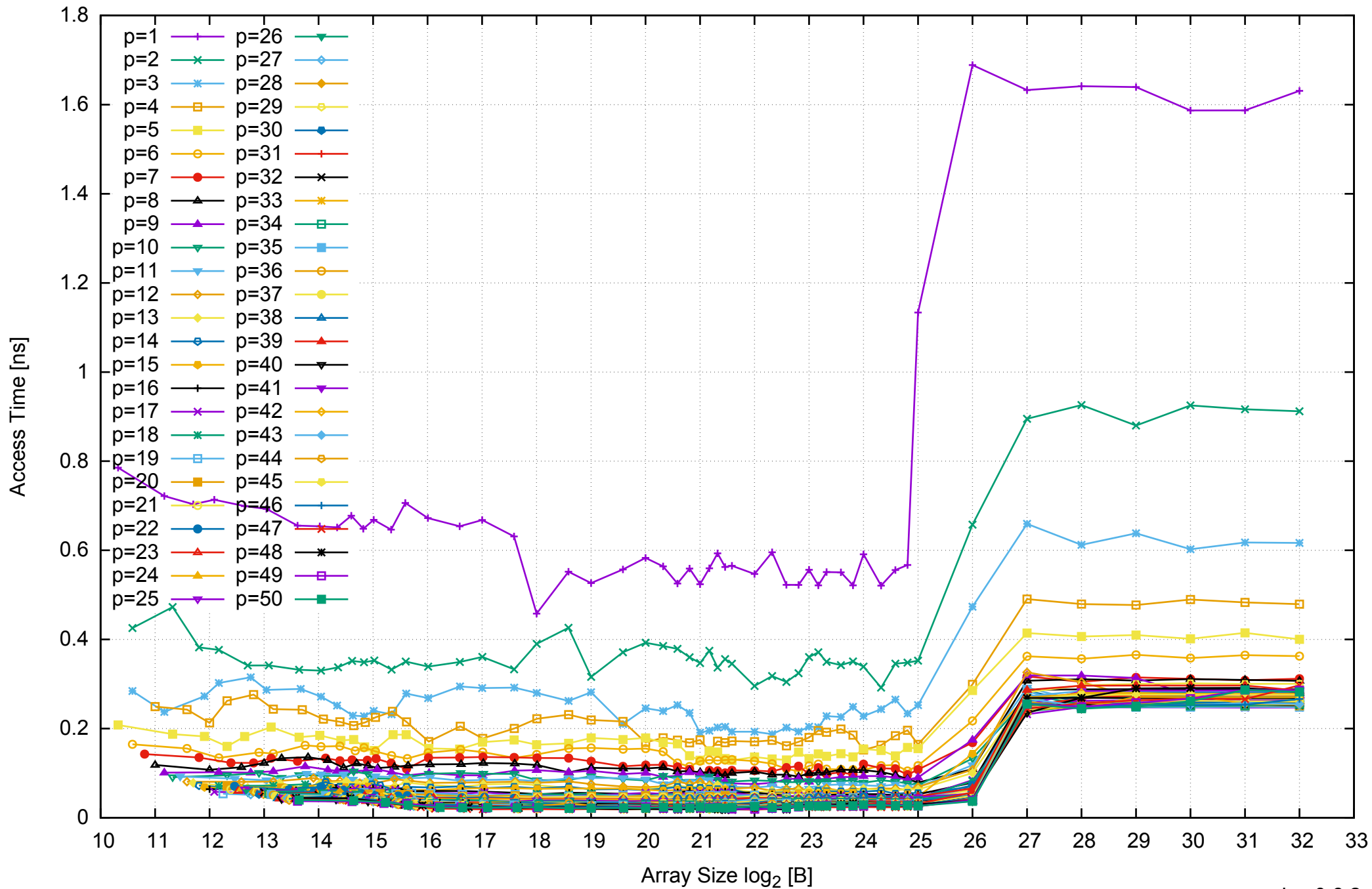
Intel Xeon E5-2670v3 256GB - Parallel Memory Access Time - ScanRead128PtrSimpleLoop
