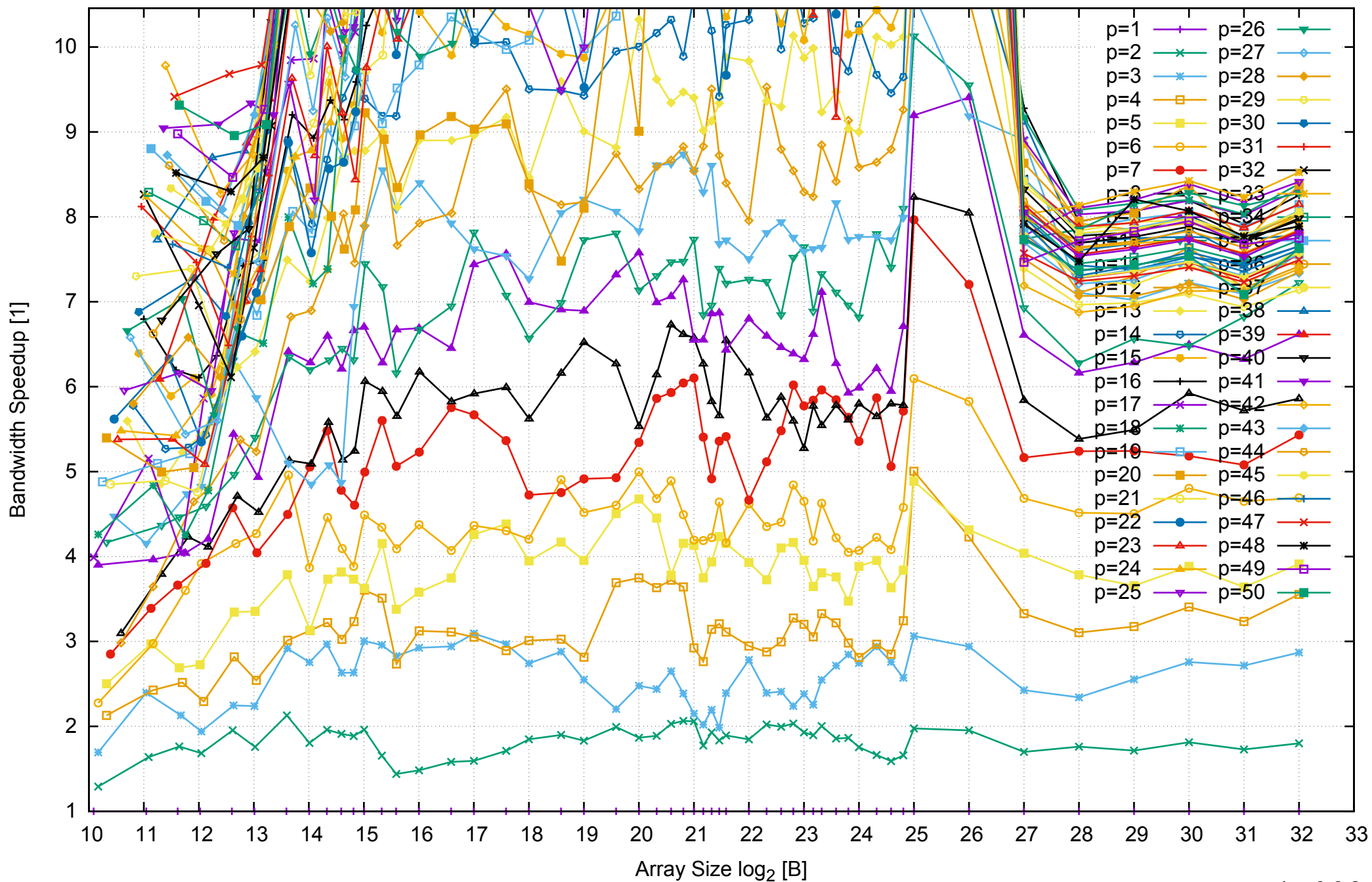
Intel Xeon E5-2670v3 256GB - Speedup of Parallel Memory Bandwidth (enlarged) - ScanRead32PtrSimpleLoop
