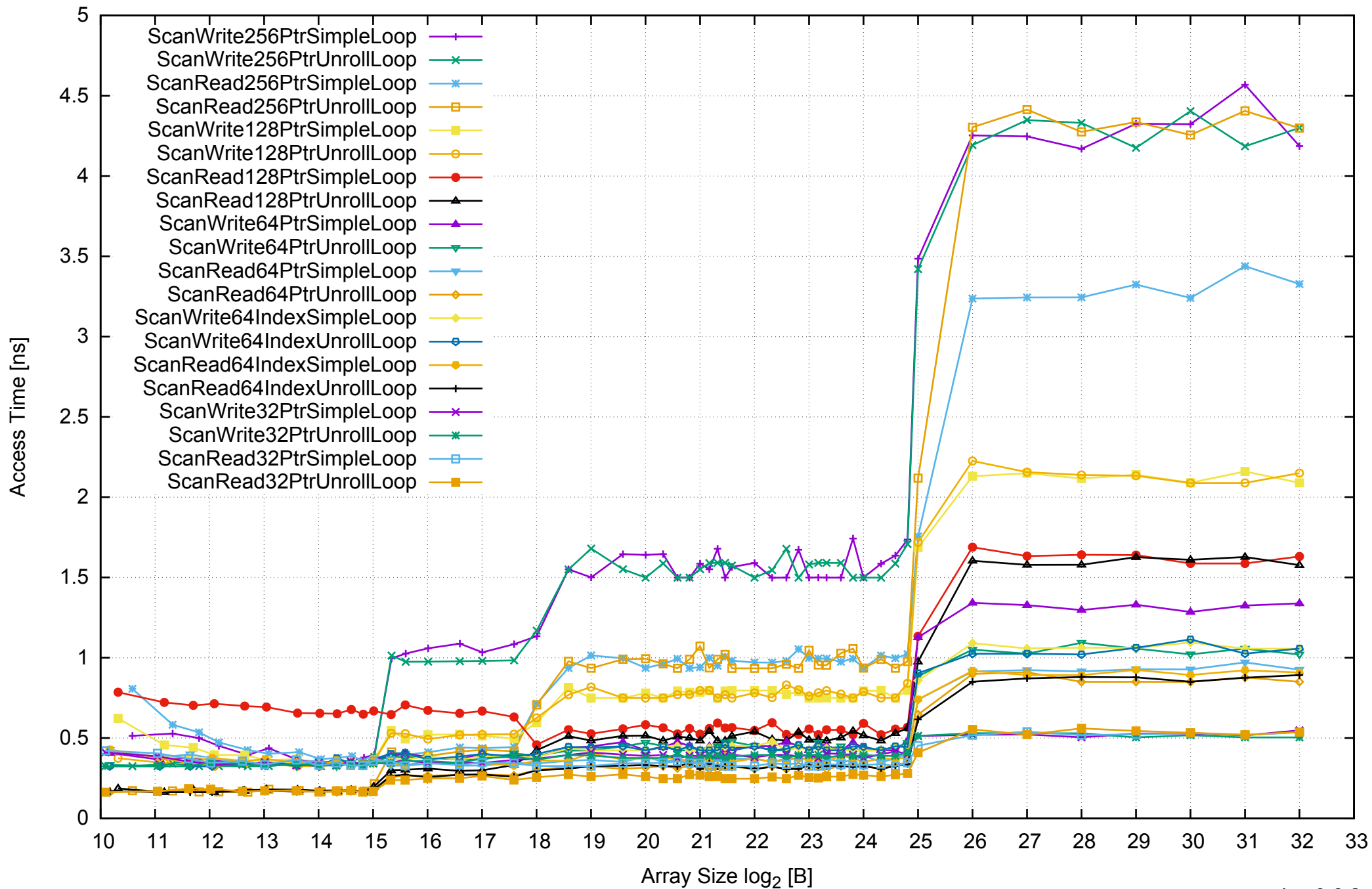
Intel Xeon E5-2670v3 256GB - One Thread Memory Latency (excluding Permutation)
