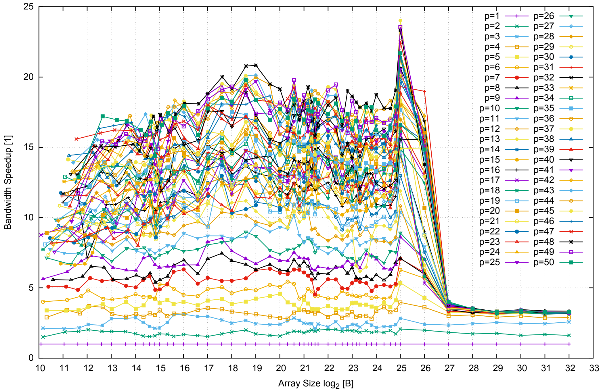
Intel Xeon E5-2670v3 256GB - Speedup of Parallel Memory Bandwidth - ScanWrite32PtrUnrollLoop
