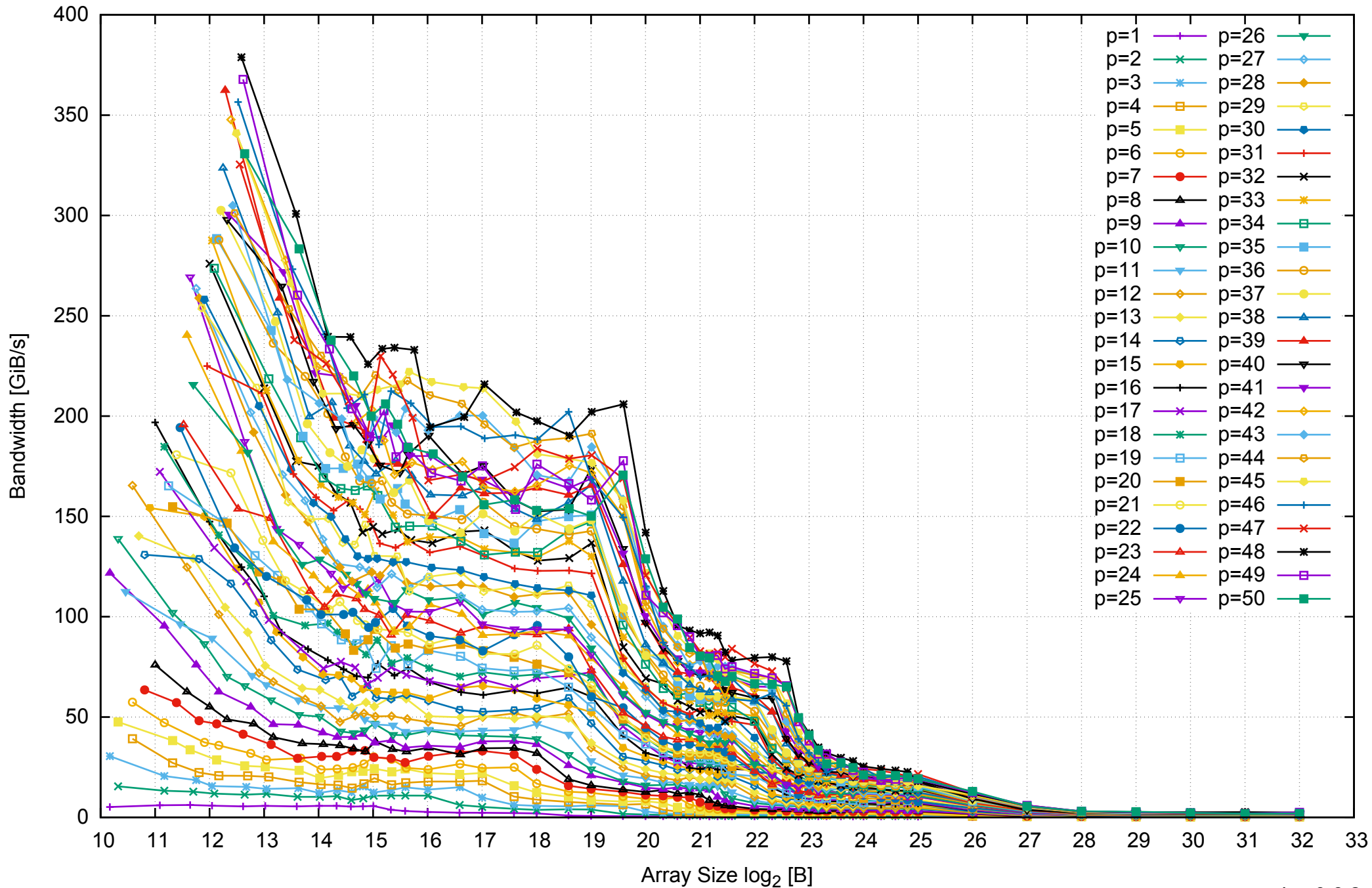
Intel Xeon E5-2670v3 256GB - Parallel Memory Bandwidth - PermRead64UnrollLoop
