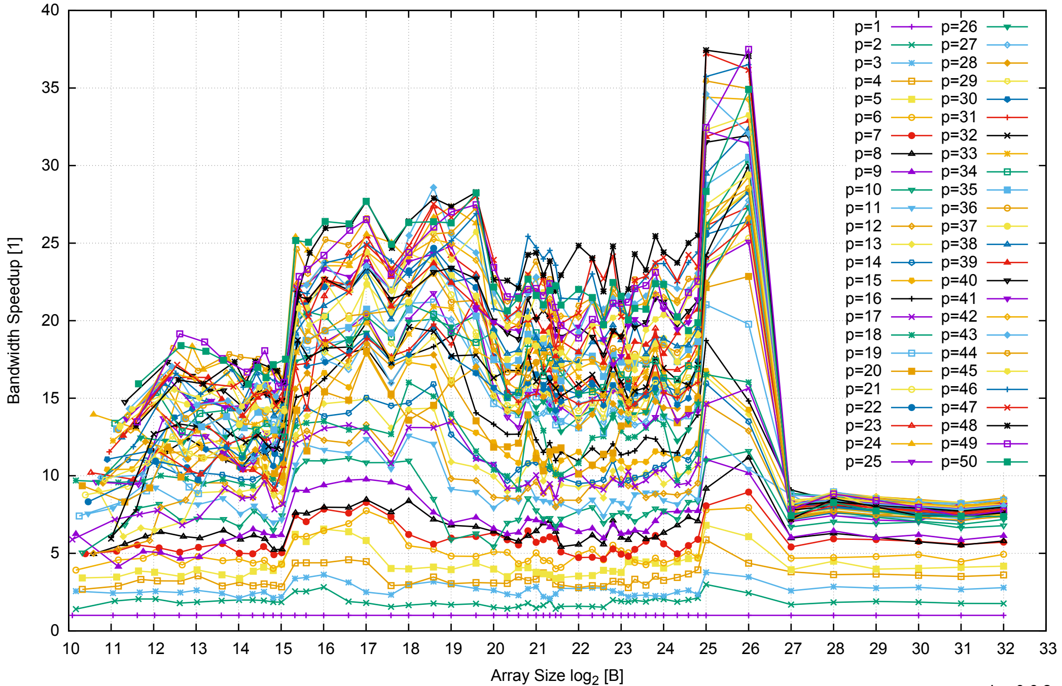
Intel Xeon E5-2670v3 256GB - Speedup of Parallel Memory Bandwidth - ScanRead32PtrUnrollLoop
