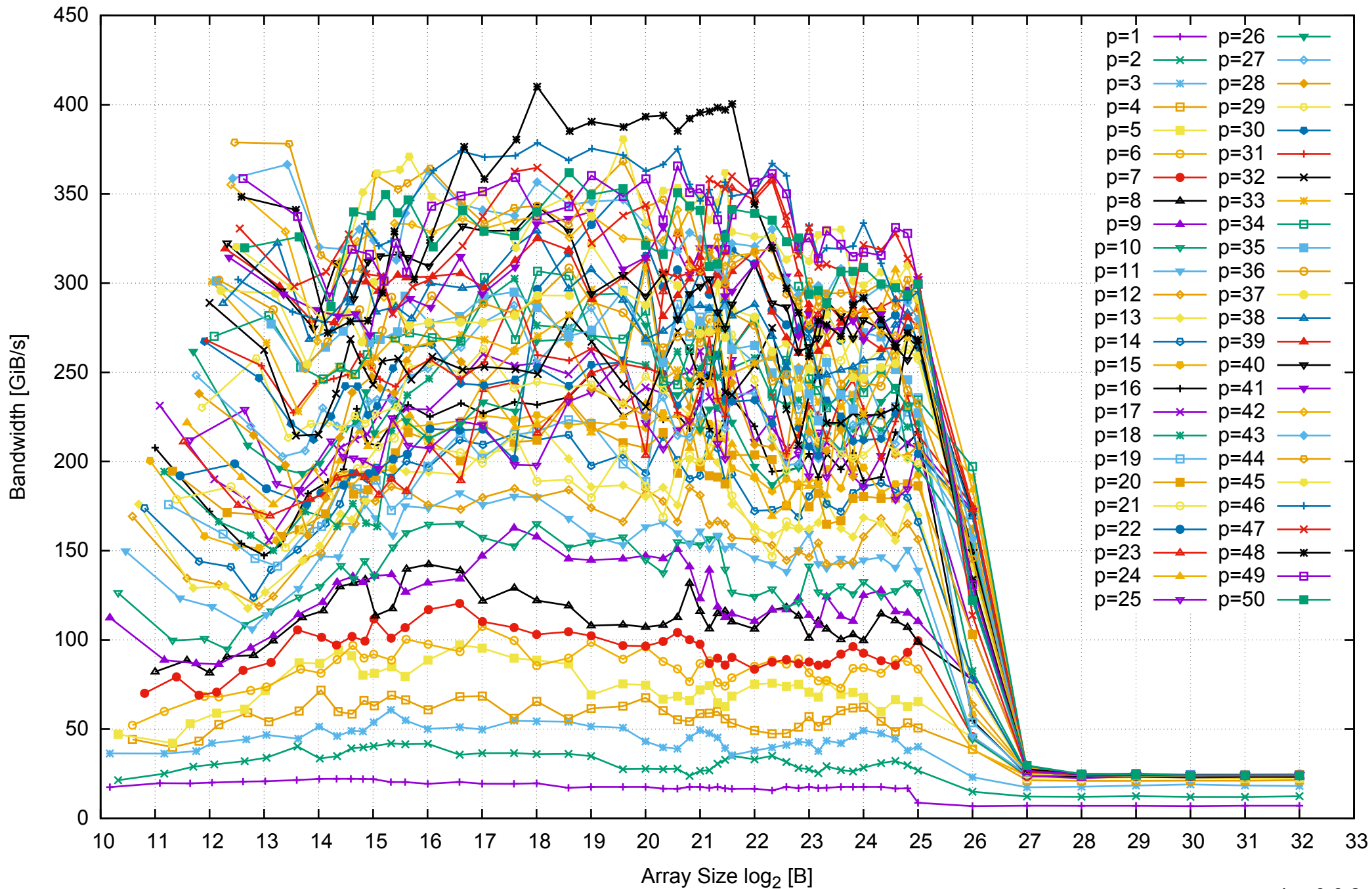
Intel Xeon E5-2670v3 256GB - Parallel Memory Bandwidth - ScanWrite64IndexSimpleLoop
