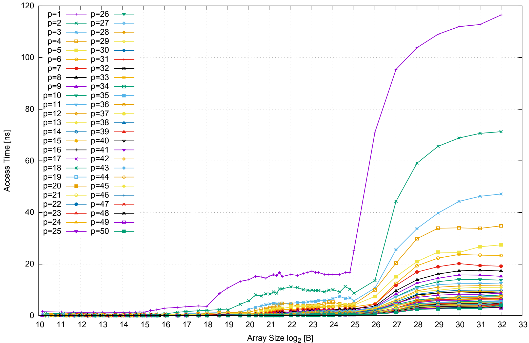
Intel Xeon E5-2670v3 256GB - Parallel Memory Access Time - PermRead64SimpleLoop
