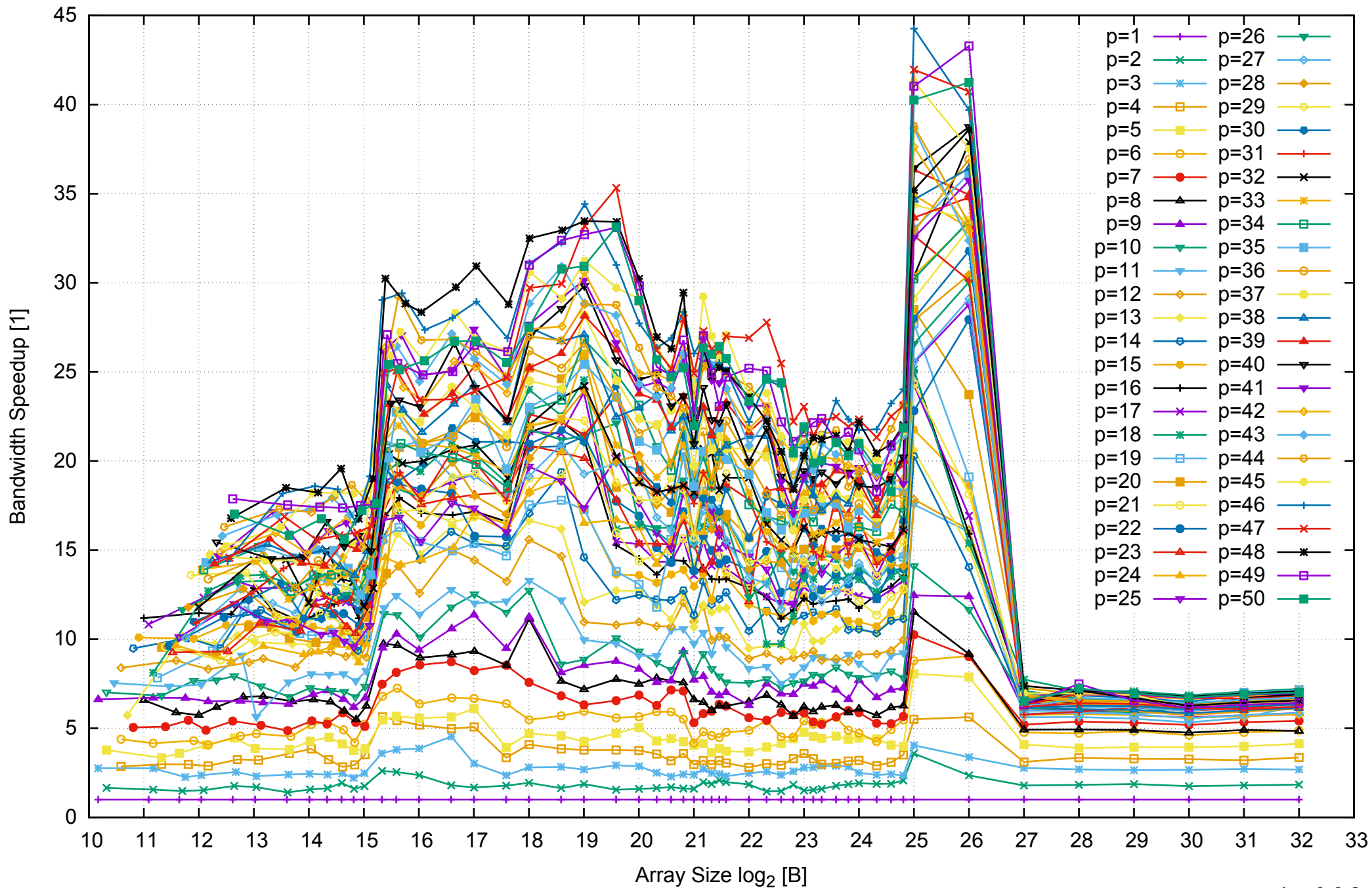
Intel Xeon E5-2670v3 256GB - Speedup of Parallel Memory Bandwidth - ScanRead64IndexUnrollLoop
