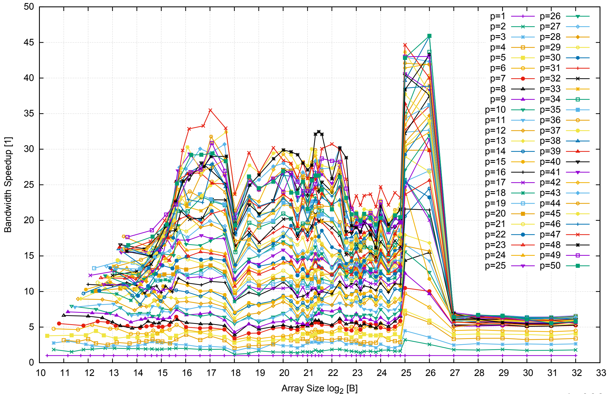
Intel Xeon E5-2670v3 256GB - Speedup of Parallel Memory Bandwidth - ScanRead128PtrSimpleLoop
