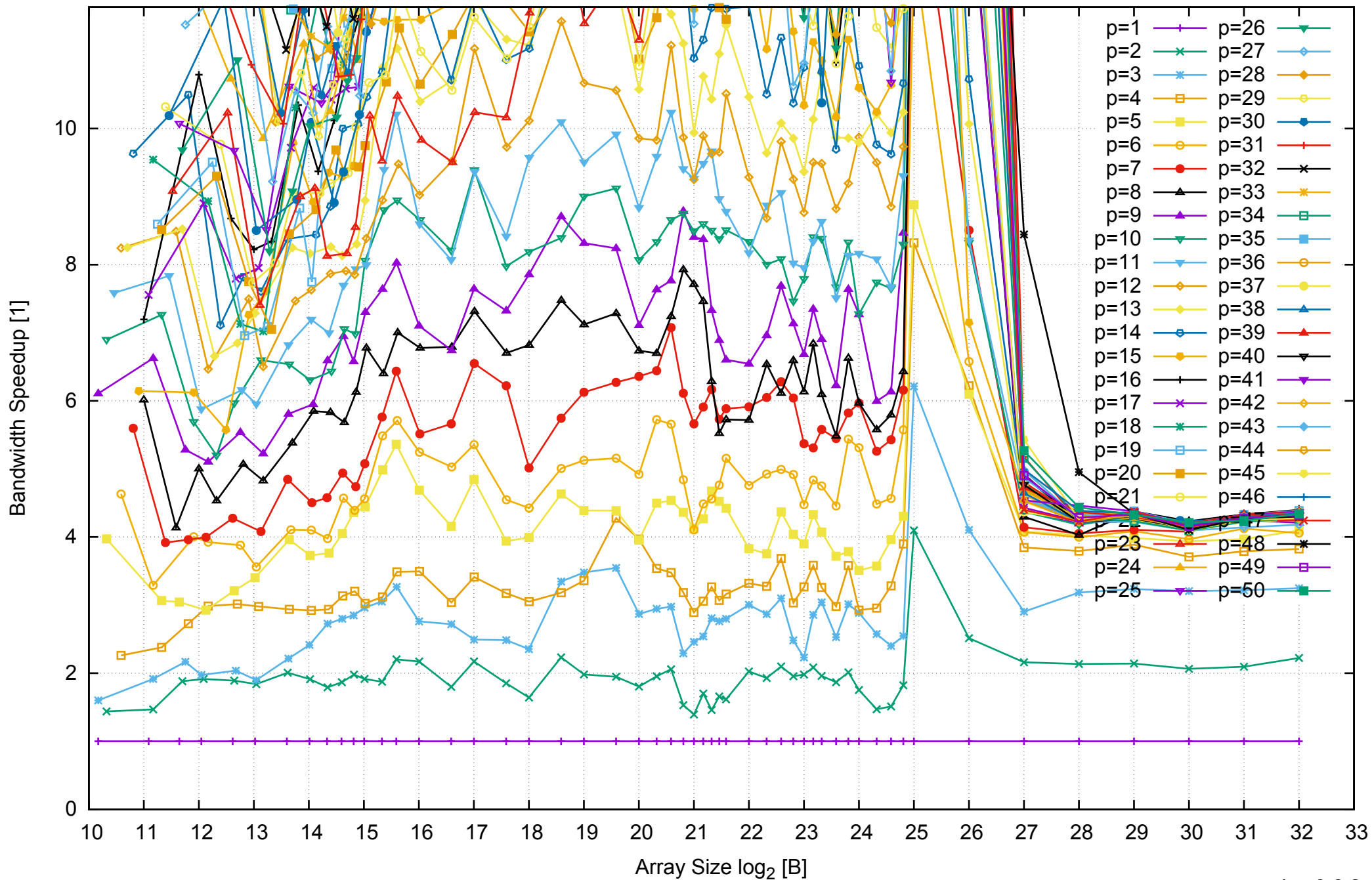
Intel Xeon E5-2670v3 256GB - Speedup of Parallel Memory Bandwidth (enlarged) - ScanWrite64PtrSimpleLoop
