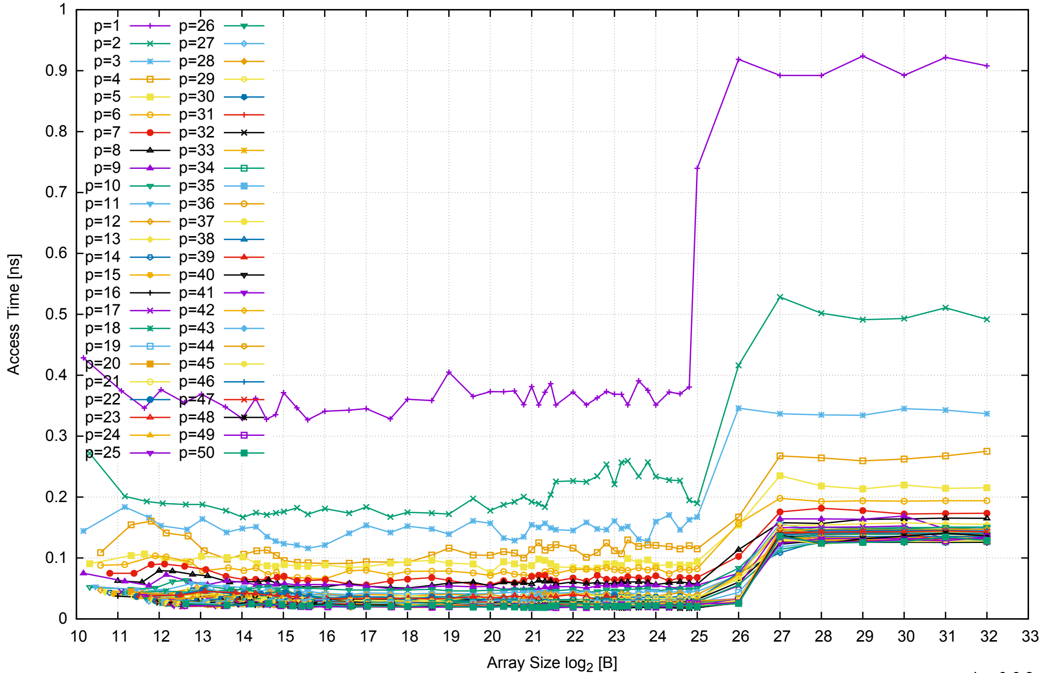
Intel Xeon E5-2670v3 256GB - Parallel Memory Access Time - ScanRead64IndexSimpleLoop
