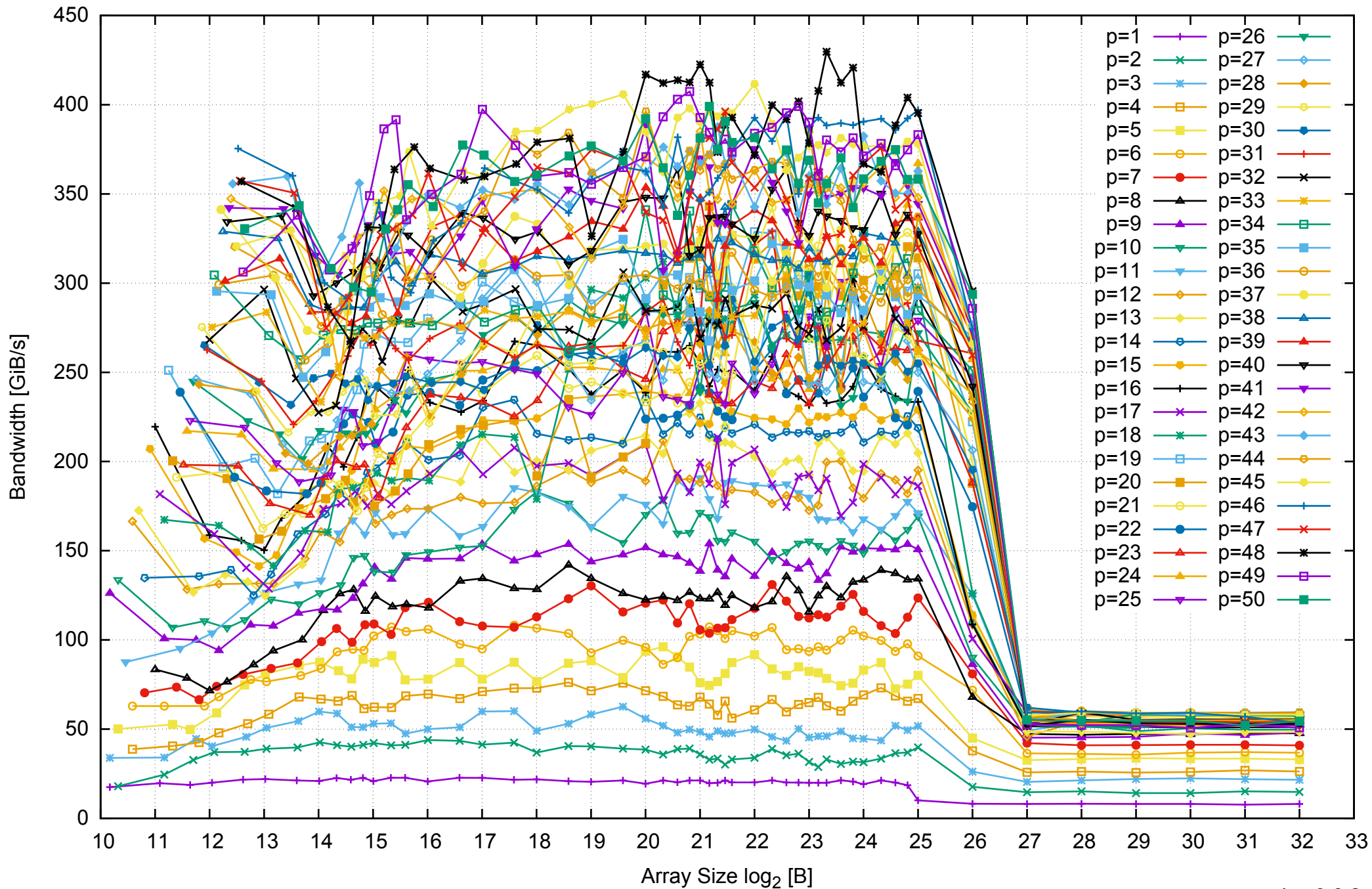
Intel Xeon E5-2670v3 256GB - Parallel Memory Bandwidth - ScanRead64PtrSimpleLoop
