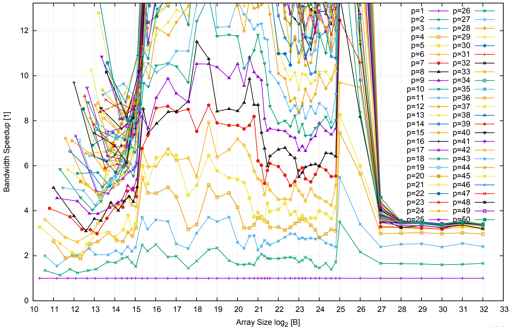
Intel Xeon E5-2670v3 256GB - Speedup of Parallel Memory Bandwidth (enlarged) - ScanWrite128PtrSimpleLoop
