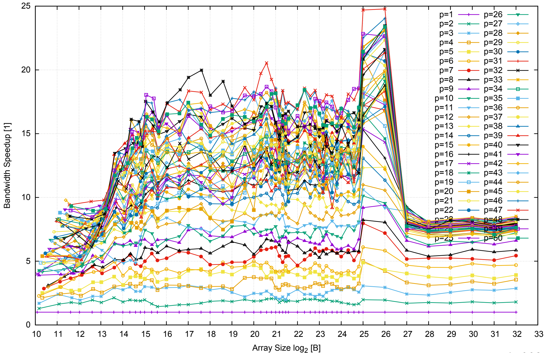
Intel Xeon E5-2670v3 256GB - Speedup of Parallel Memory Bandwidth - ScanRead32PtrSimpleLoop
