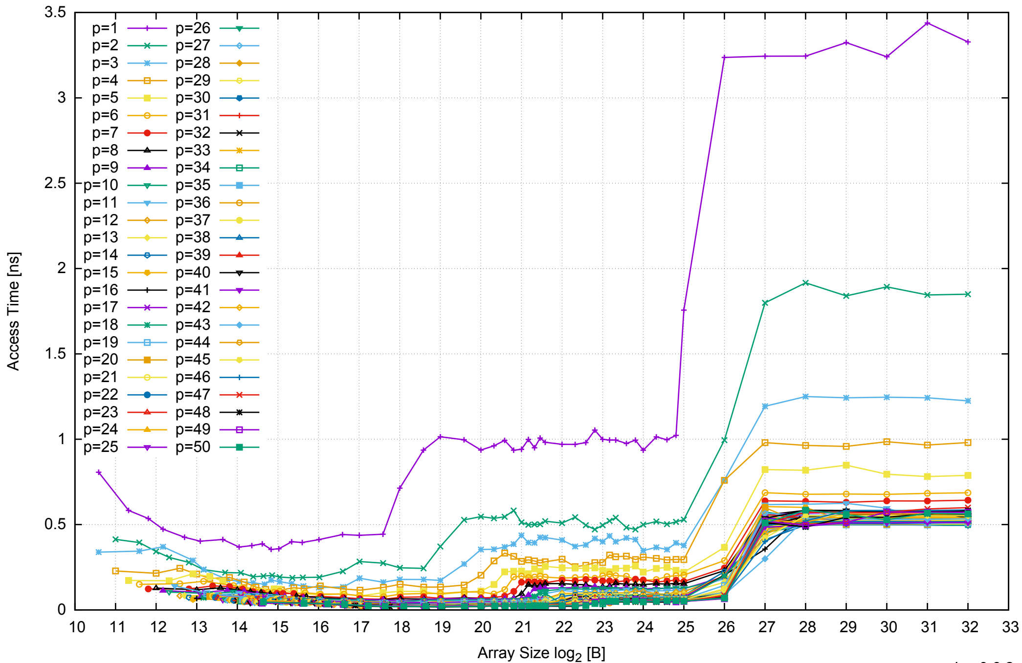
Intel Xeon E5-2670v3 256GB - Parallel Memory Access Time - ScanRead256PtrSimpleLoop
