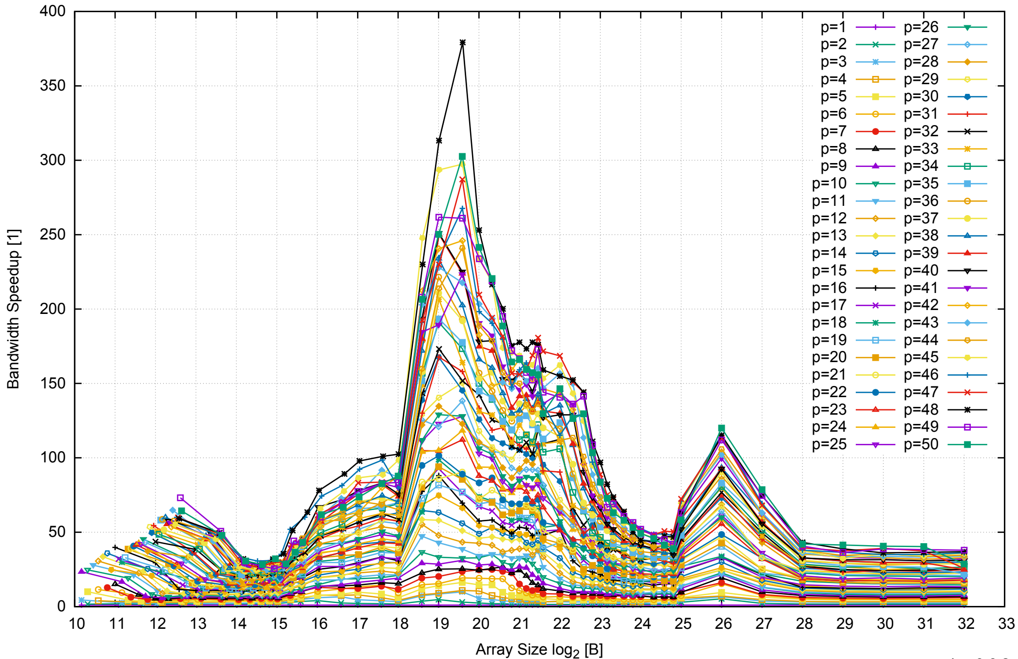
Intel Xeon E5-2670v3 256GB - Speedup of Parallel Memory Bandwidth - PermRead64SimpleLoop
