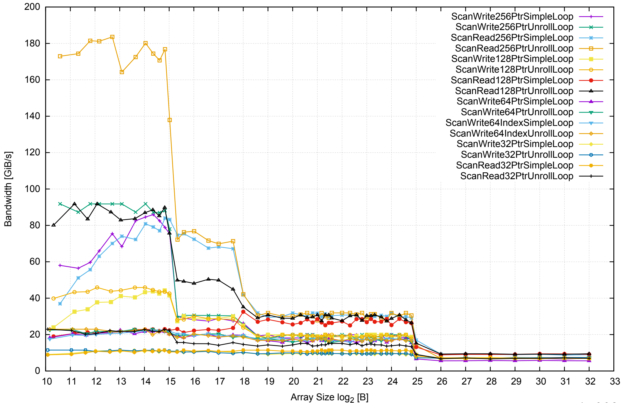
Intel Xeon E5-2670v3 256GB - One Thread Memory Bandwidth (only 64-bit Reads)
