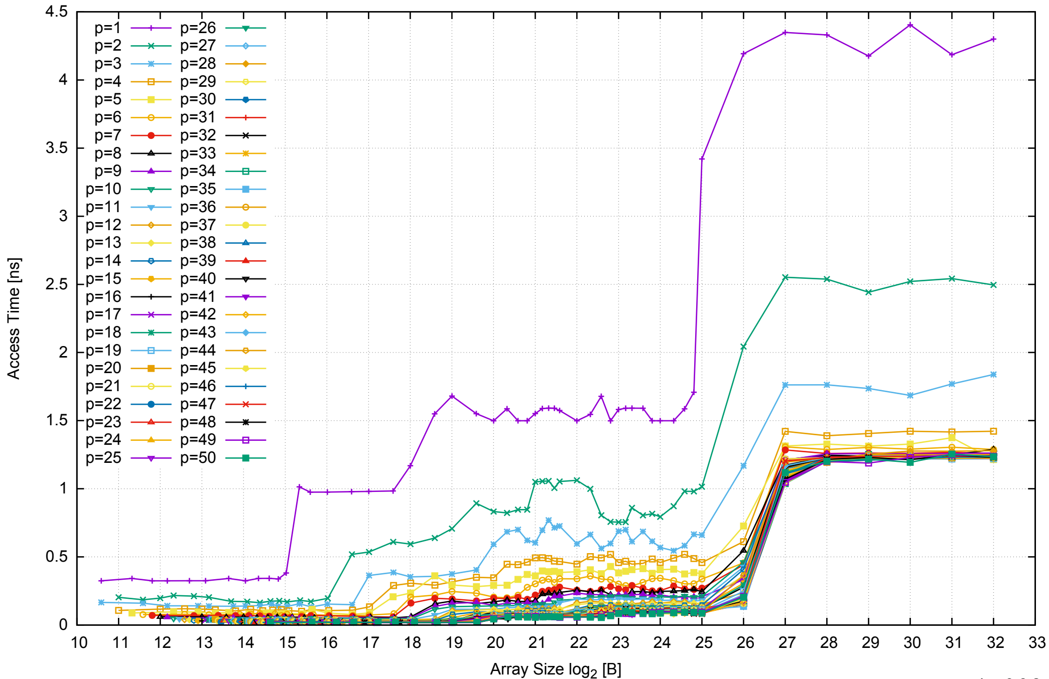
Intel Xeon E5-2670v3 256GB - Parallel Memory Access Time - ScanWrite256PtrUnrollLoop
