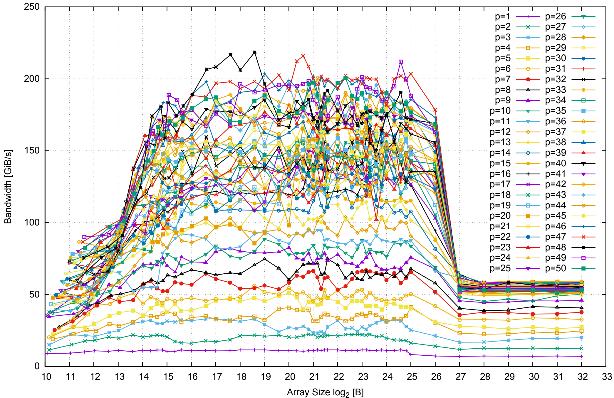
Intel Xeon E5-2670v3 256GB - Parallel Memory Bandwidth - ScanRead32PtrSimpleLoop
