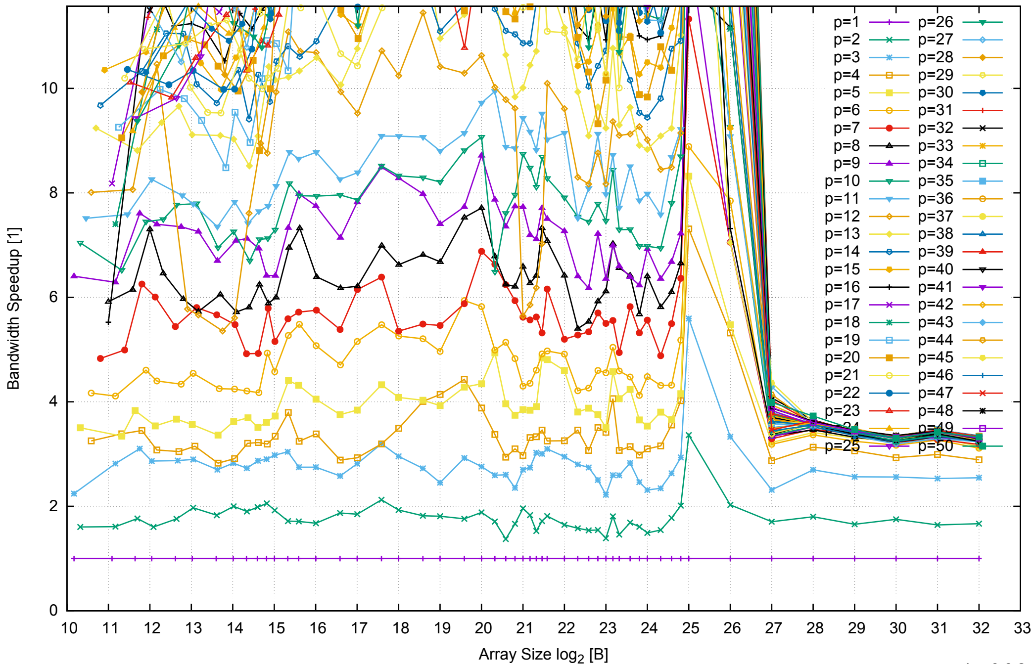
Intel Xeon E5-2670v3 256GB - Speedup of Parallel Memory Bandwidth (enlarged) - ScanWrite64PtrUnrollLoop
