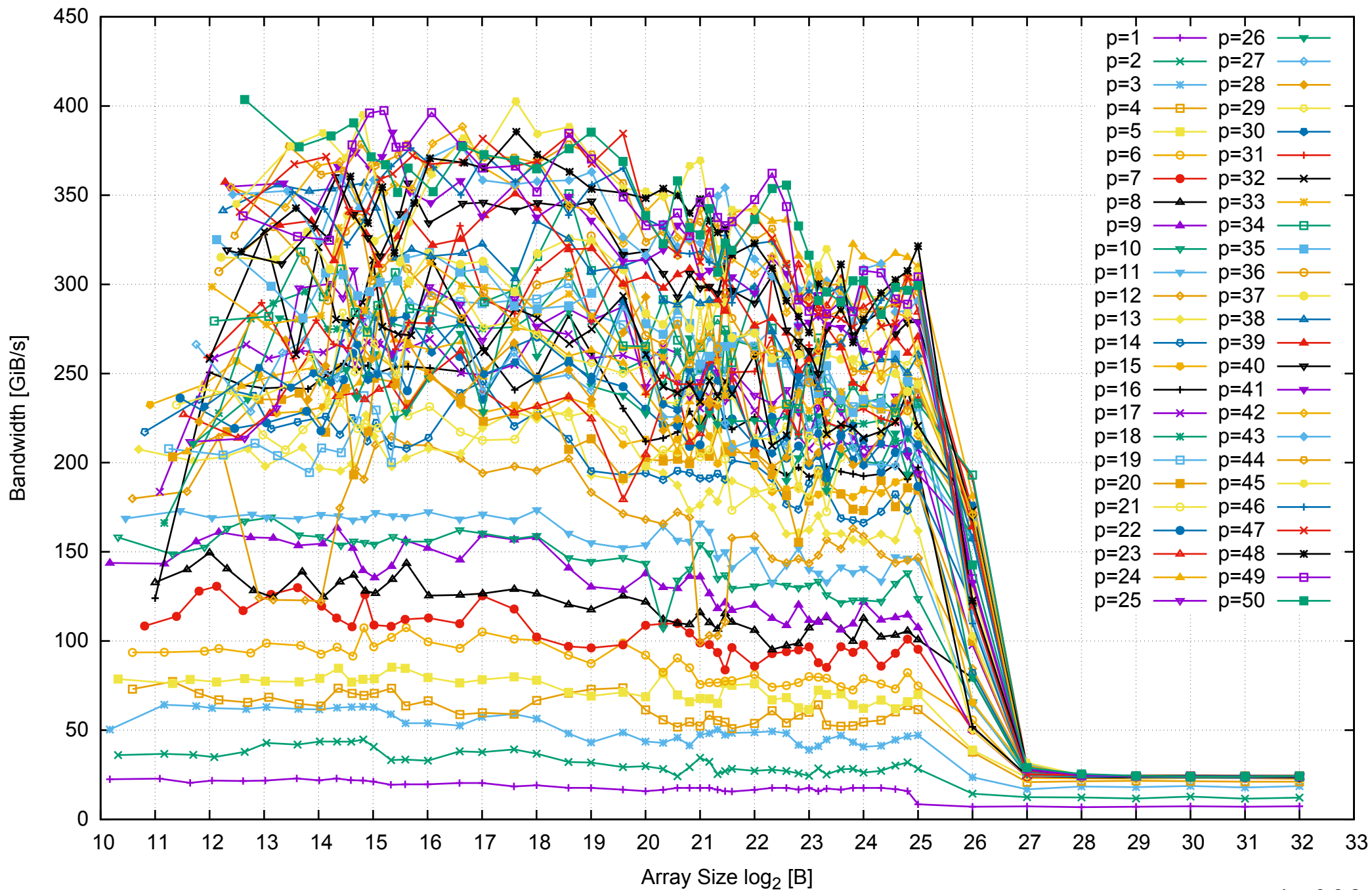
Intel Xeon E5-2670v3 256GB - Parallel Memory Bandwidth - ScanWrite64PtrUnrollLoop
