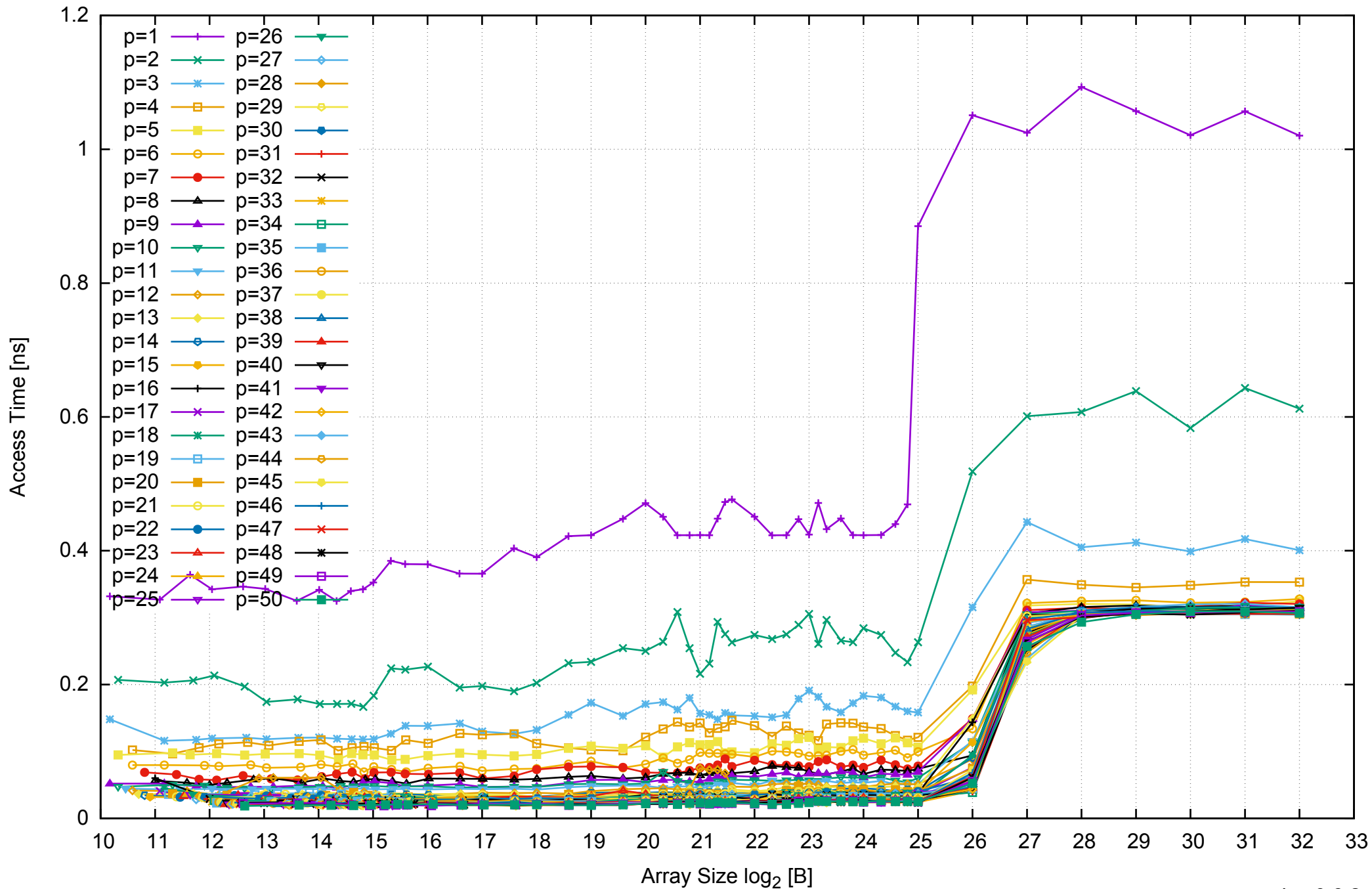
Intel Xeon E5-2670v3 256GB - Parallel Memory Access Time - ScanWrite64PtrUnrollLoop
