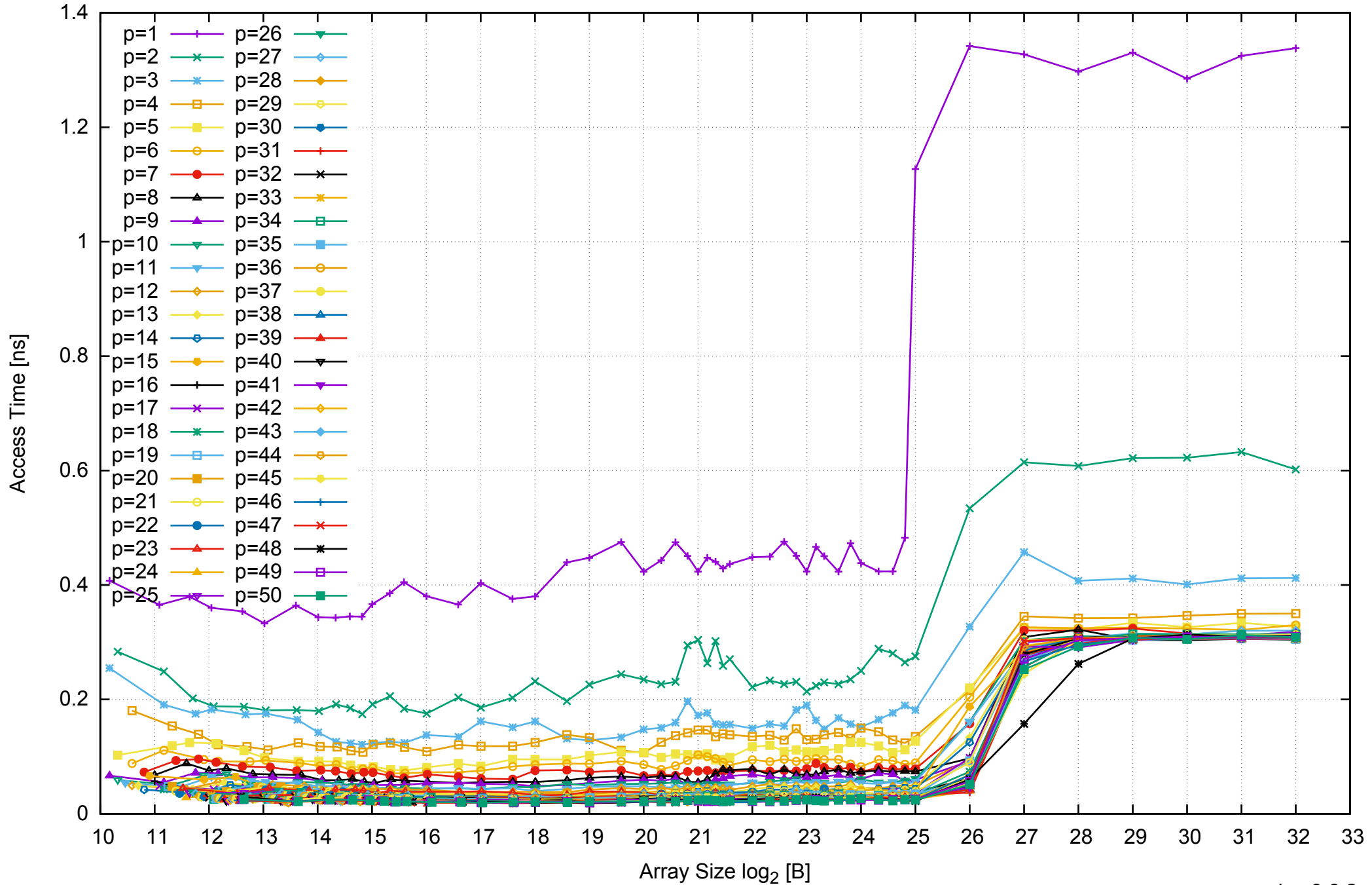
Intel Xeon E5-2670v3 256GB - Parallel Memory Access Time - ScanWrite64PtrSimpleLoop
