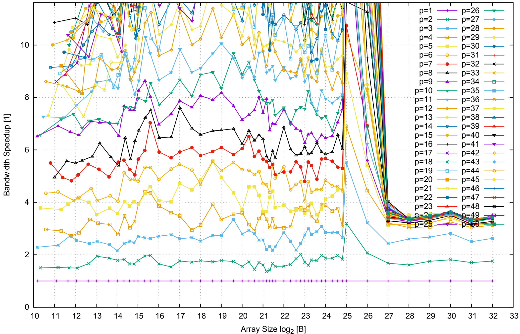
Intel Xeon E5-2670v3 256GB - Speedup of Parallel Memory Bandwidth (enlarged) - ScanWrite64IndexUnrollLoop
