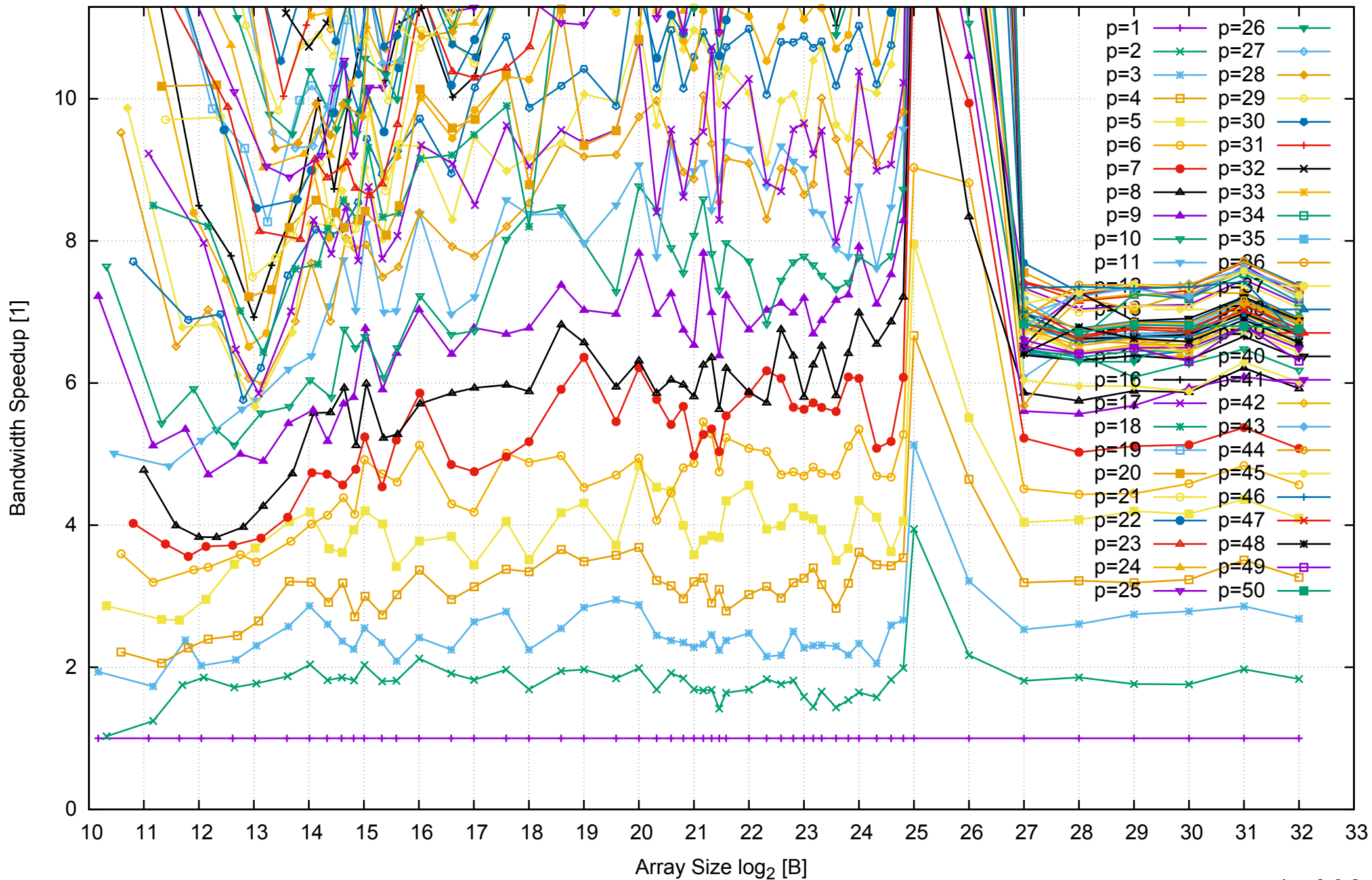
Intel Xeon E5-2670v3 256GB - Speedup of Parallel Memory Bandwidth (enlarged) - ScanRead64PtrSimpleLoop
