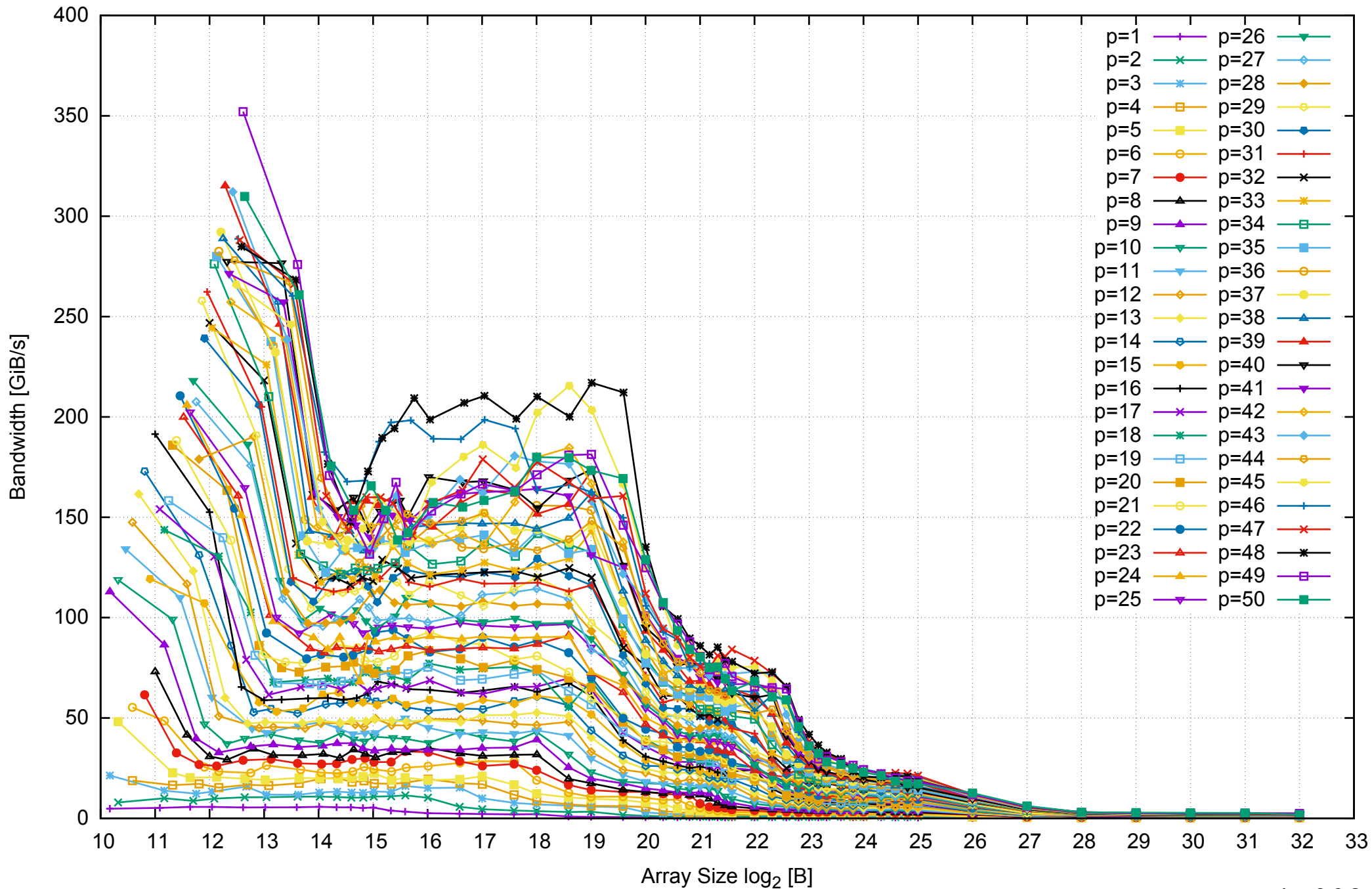
Intel Xeon E5-2670v3 256GB - Parallel Memory Bandwidth - PermRead64SimpleLoop
