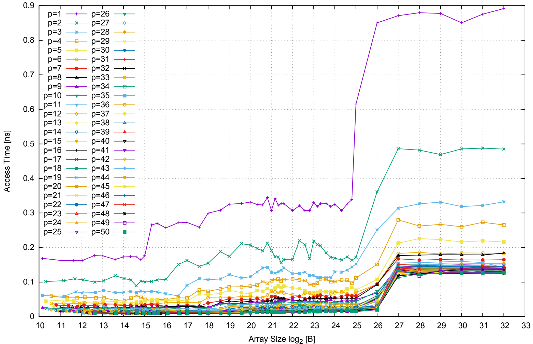
Intel Xeon E5-2670v3 256GB - Parallel Memory Access Time - ScanRead64IndexUnrollLoop
