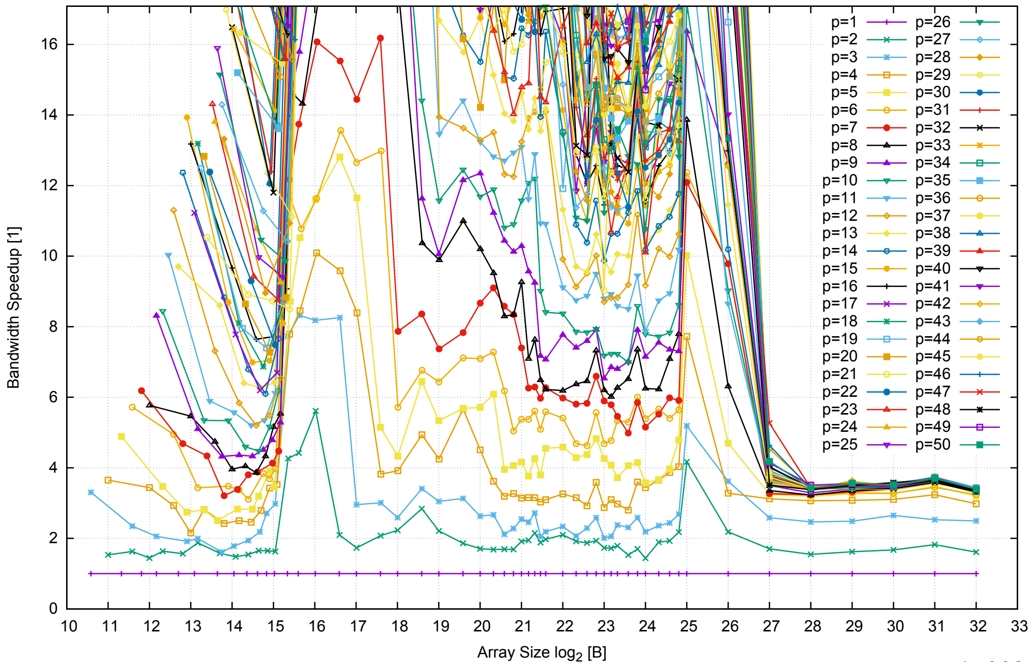
Intel Xeon E5-2670v3 256GB - Speedup of Parallel Memory Bandwidth (enlarged) - ScanWrite256PtrSimpleLoop
