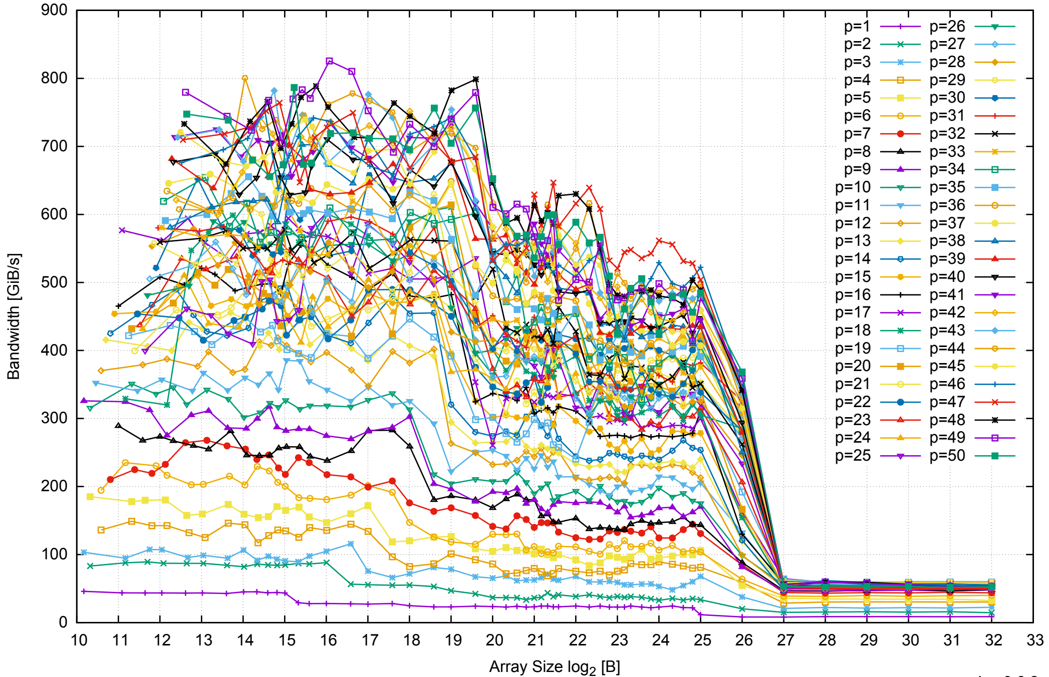
Intel Xeon E5-2670v3 256GB - Parallel Memory Bandwidth - ScanRead64PtrUnrollLoop
