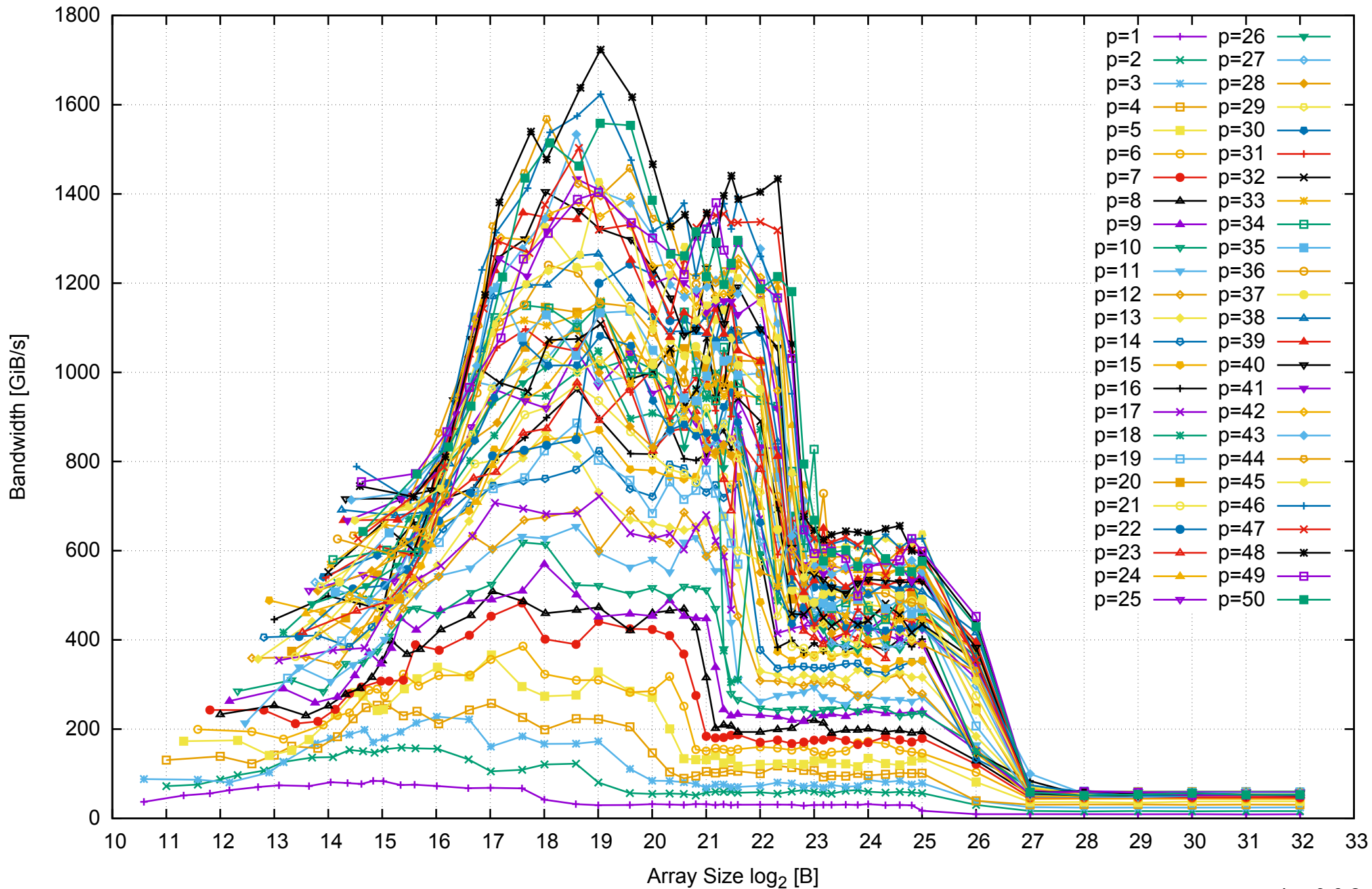
Intel Xeon E5-2670v3 256GB - Parallel Memory Bandwidth - ScanRead256PtrSimpleLoop
