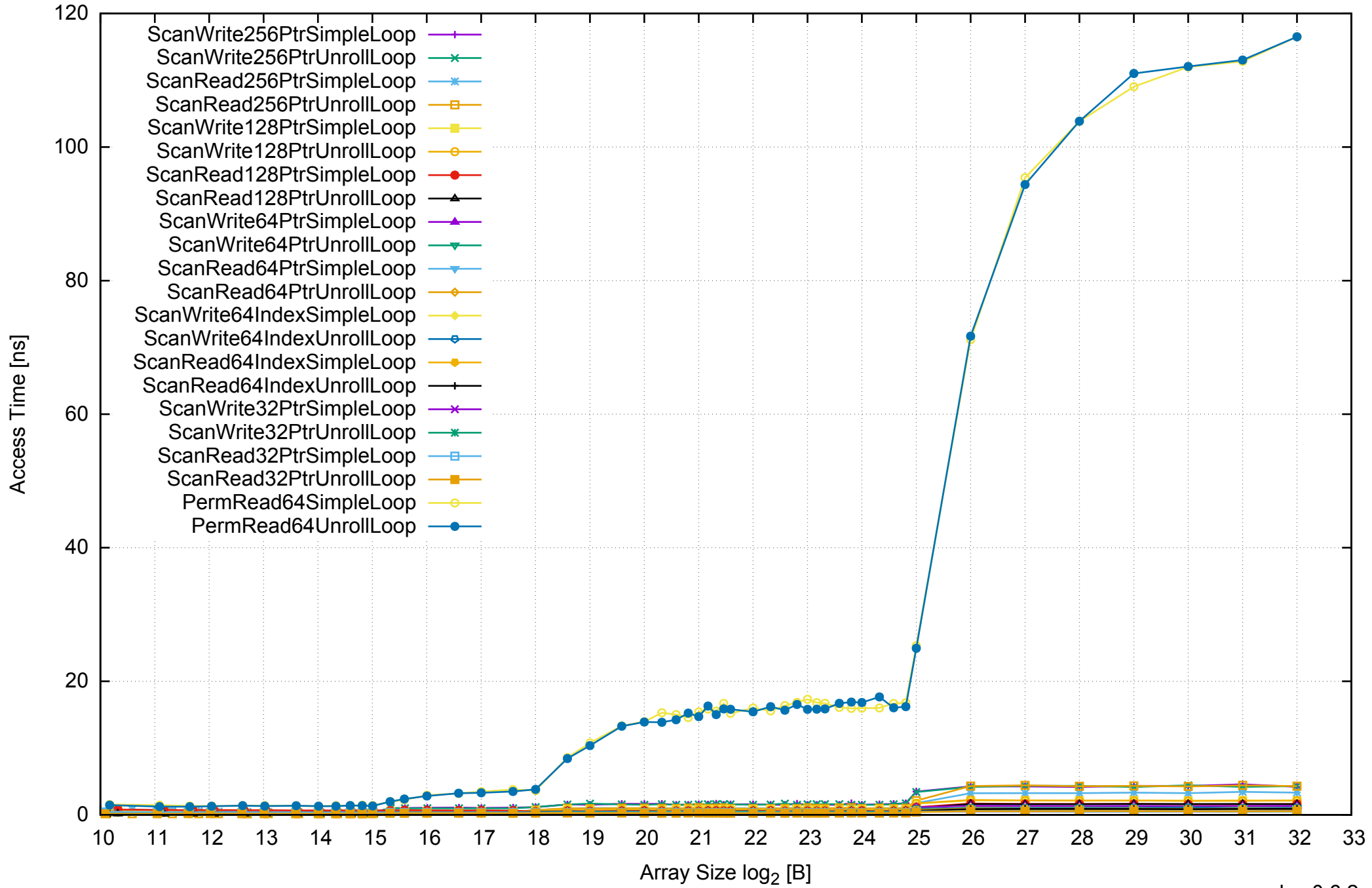
Intel Xeon E5-2670v3 256GB - One Thread Memory Latency (Access Time)
