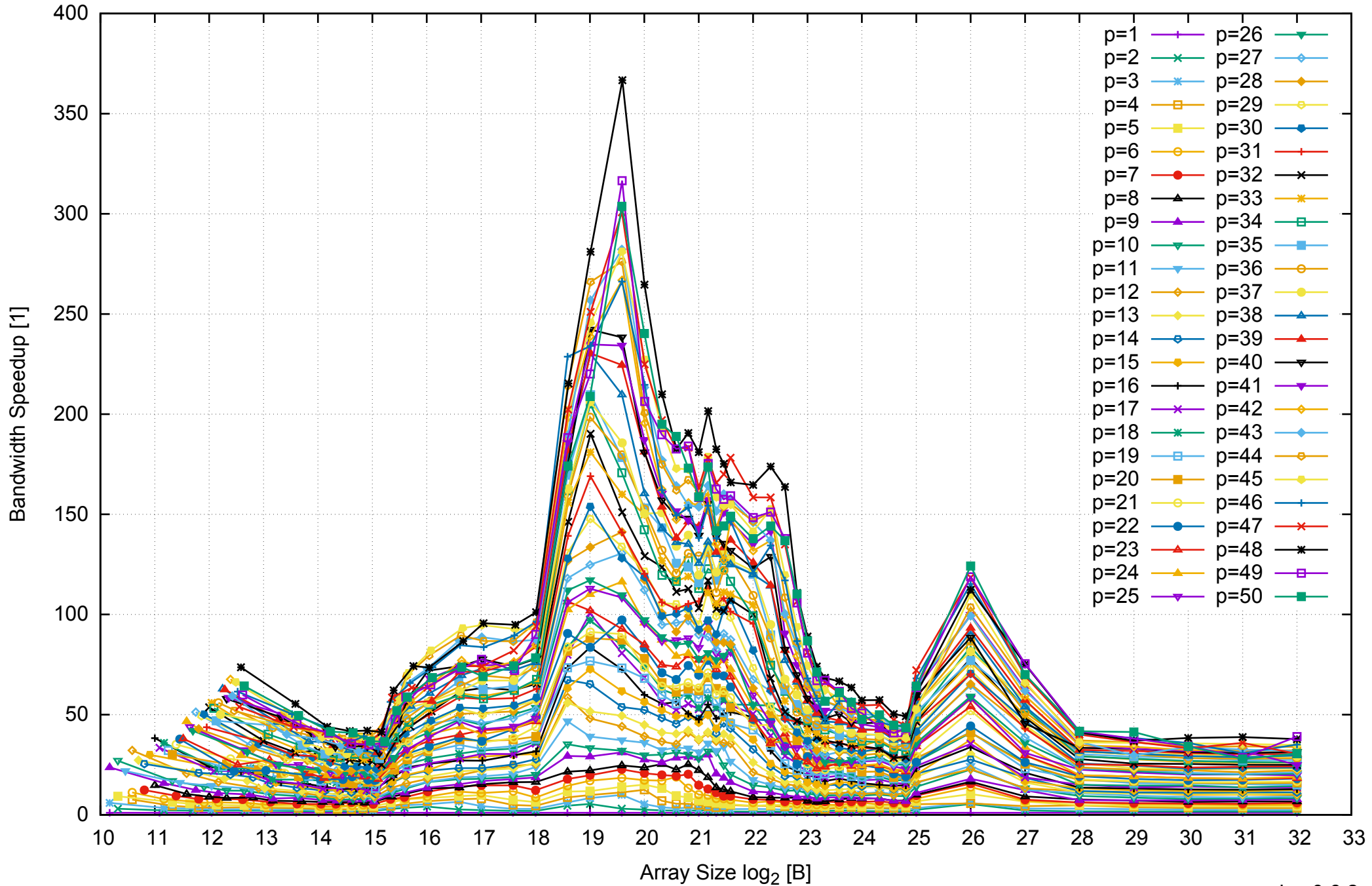
Intel Xeon E5-2670v3 256GB - Speedup of Parallel Memory Bandwidth - PermRead64UnrollLoop
