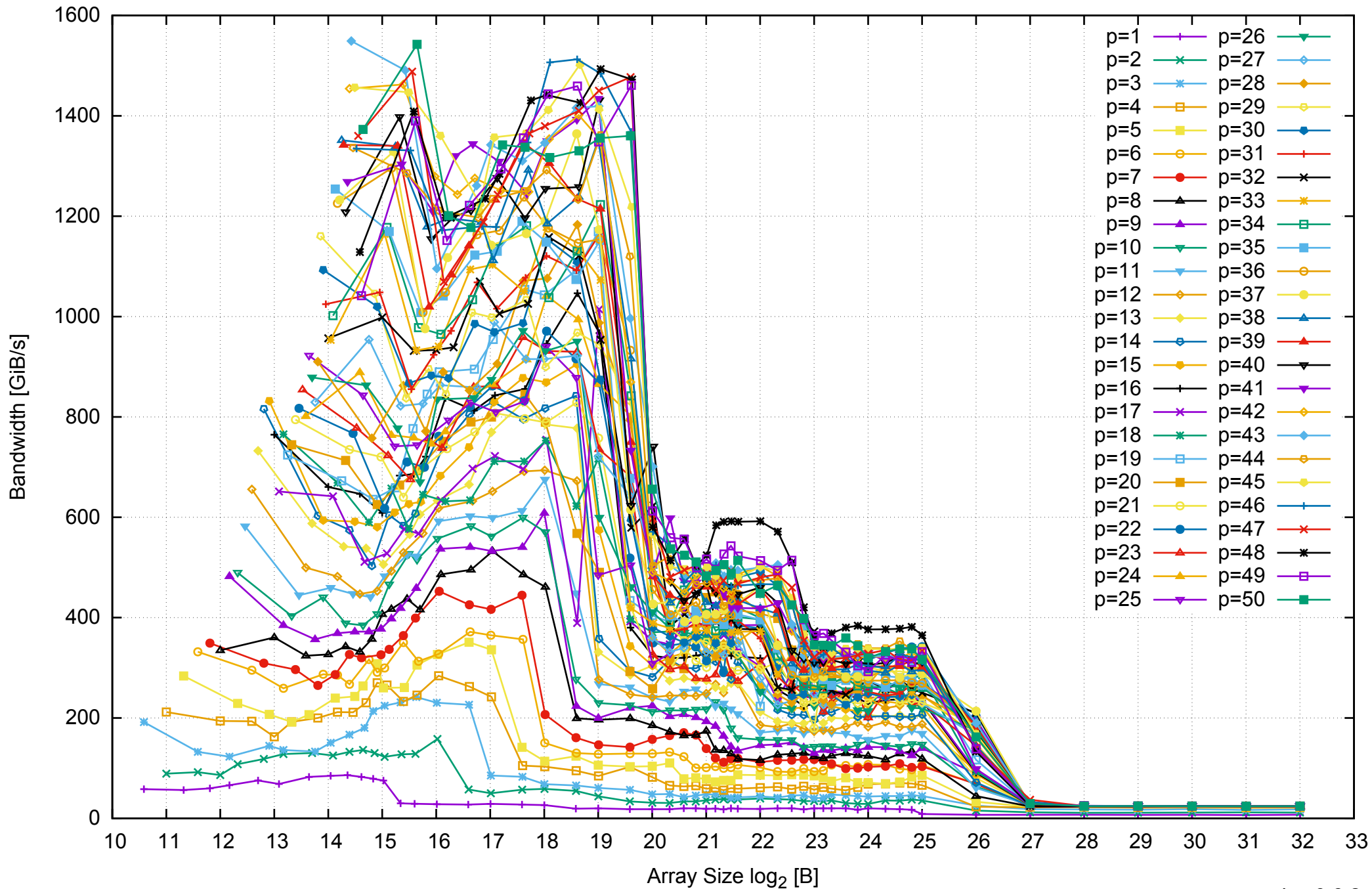
Intel Xeon E5-2670v3 256GB - Parallel Memory Bandwidth - ScanWrite256PtrSimpleLoop
