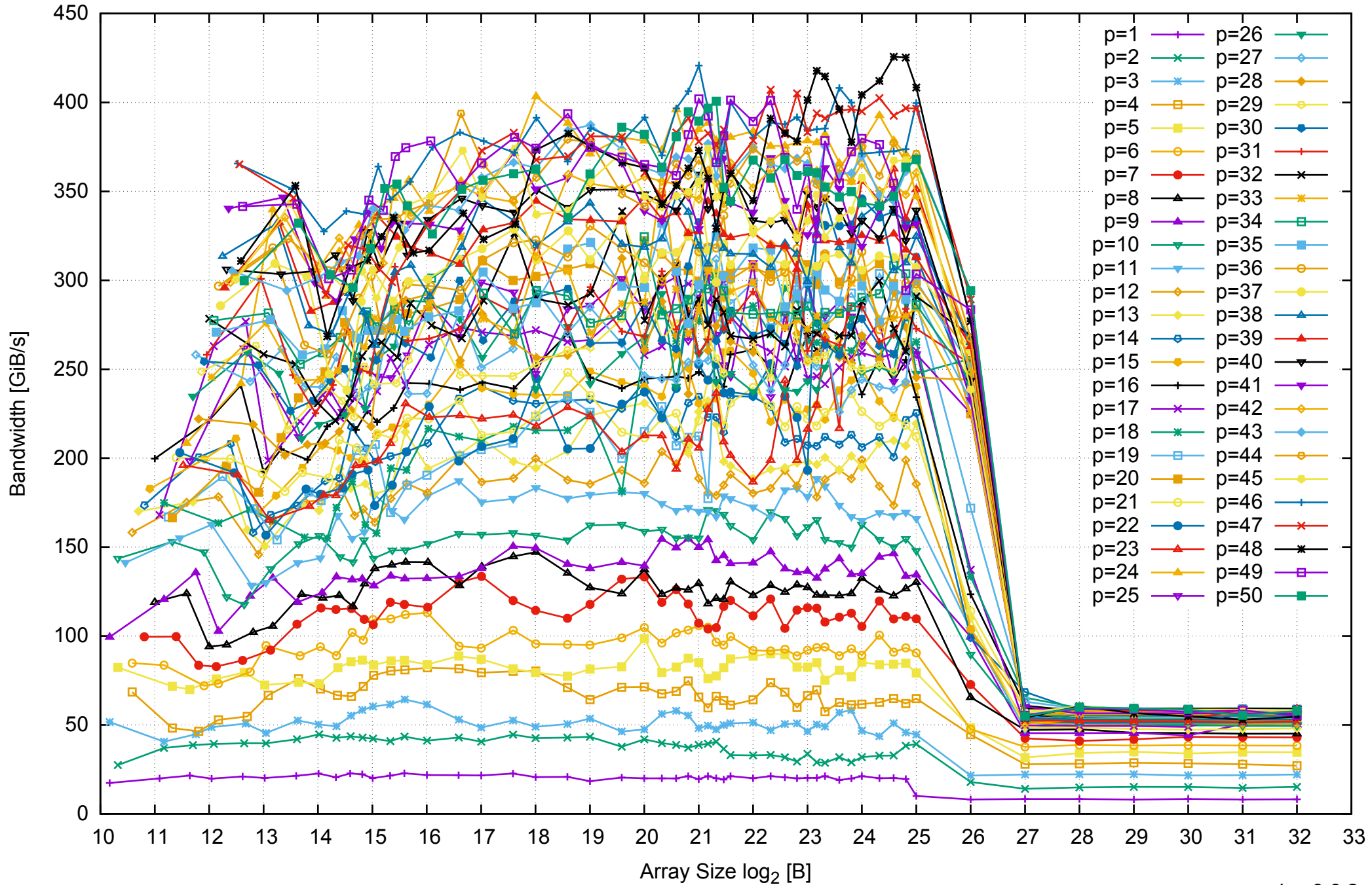
Intel Xeon E5-2670v3 256GB - Parallel Memory Bandwidth - ScanRead64IndexSimpleLoop
