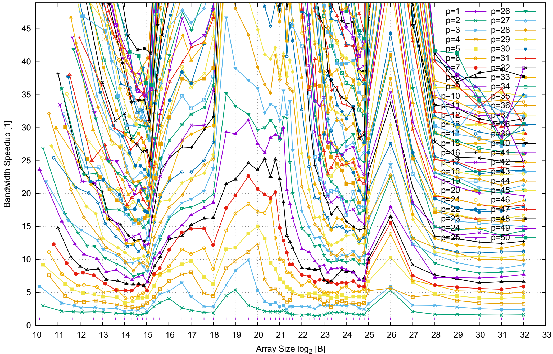
Intel Xeon E5-2670v3 256GB - Speedup of Parallel Memory Bandwidth (enlarged) - PermRead64UnrollLoop
