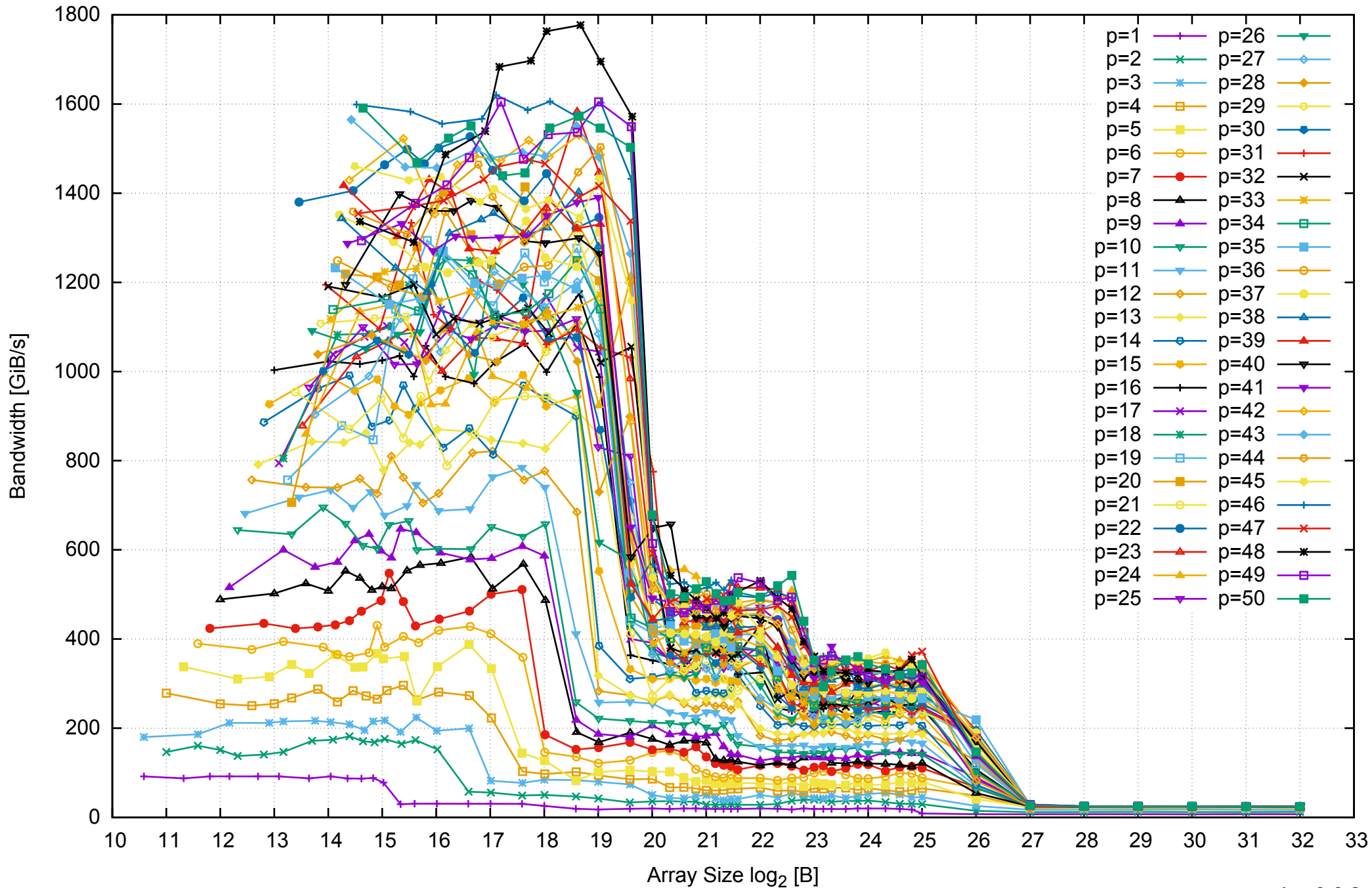
Intel Xeon E5-2670v3 256GB - Parallel Memory Bandwidth - ScanWrite256PtrUnrollLoop
