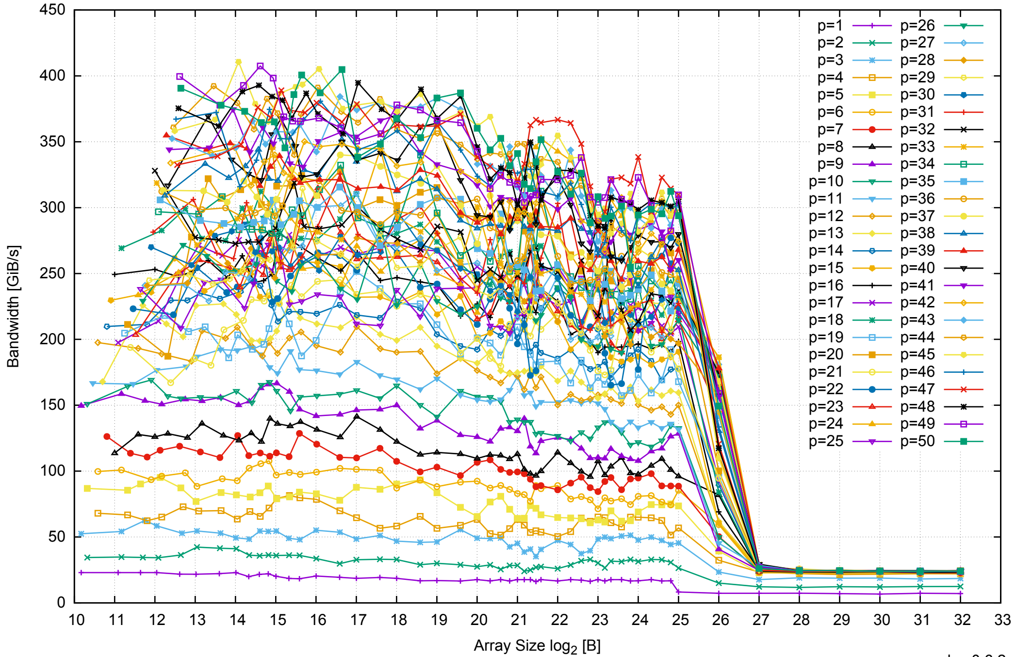
Intel Xeon E5-2670v3 256GB - Parallel Memory Bandwidth - ScanWrite64IndexUnrollLoop
