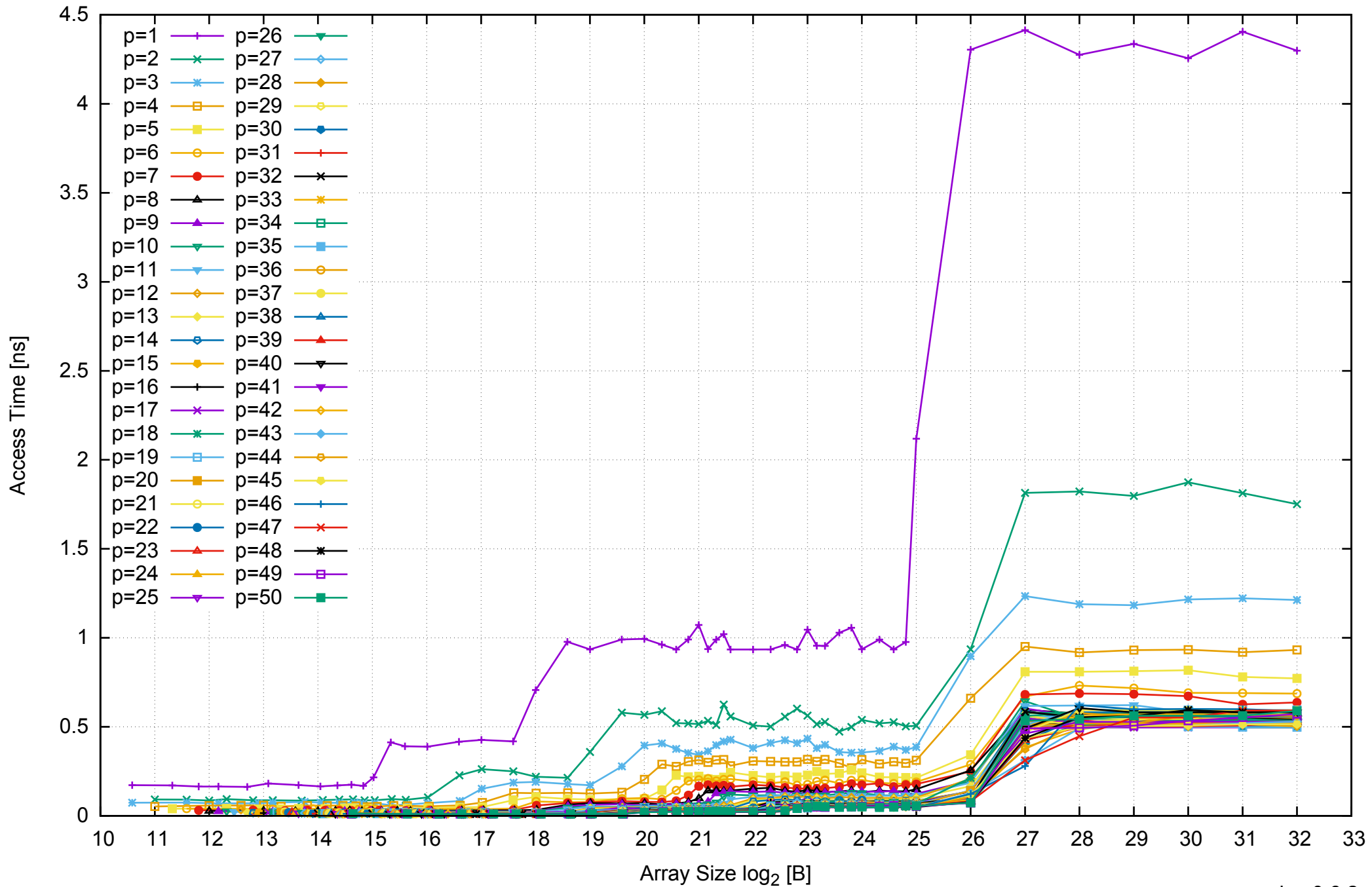
Intel Xeon E5-2670v3 256GB - Parallel Memory Access Time - ScanRead256PtrUnrollLoop
