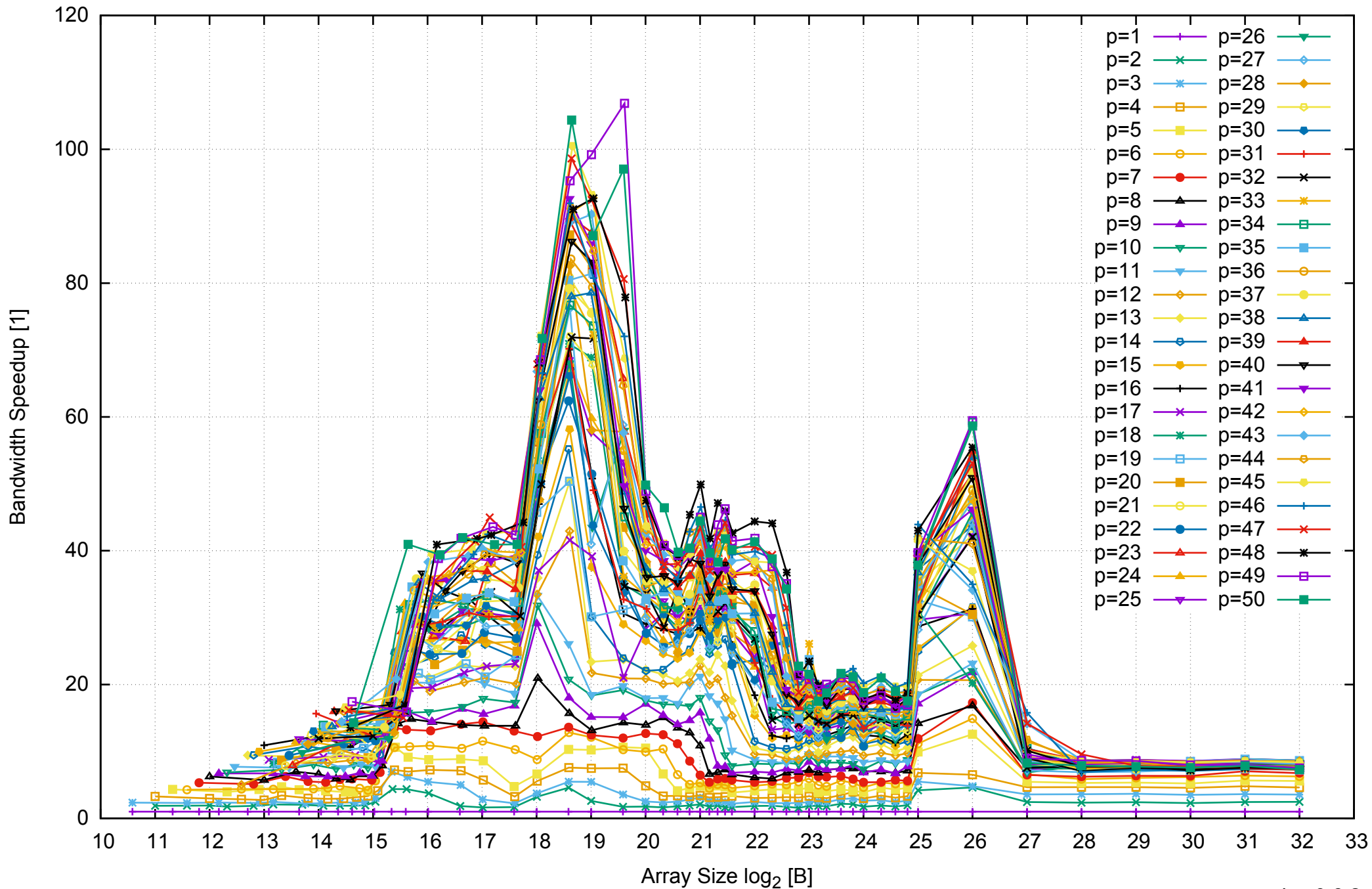
Intel Xeon E5-2670v3 256GB - Speedup of Parallel Memory Bandwidth - ScanRead256PtrUnrollLoop
