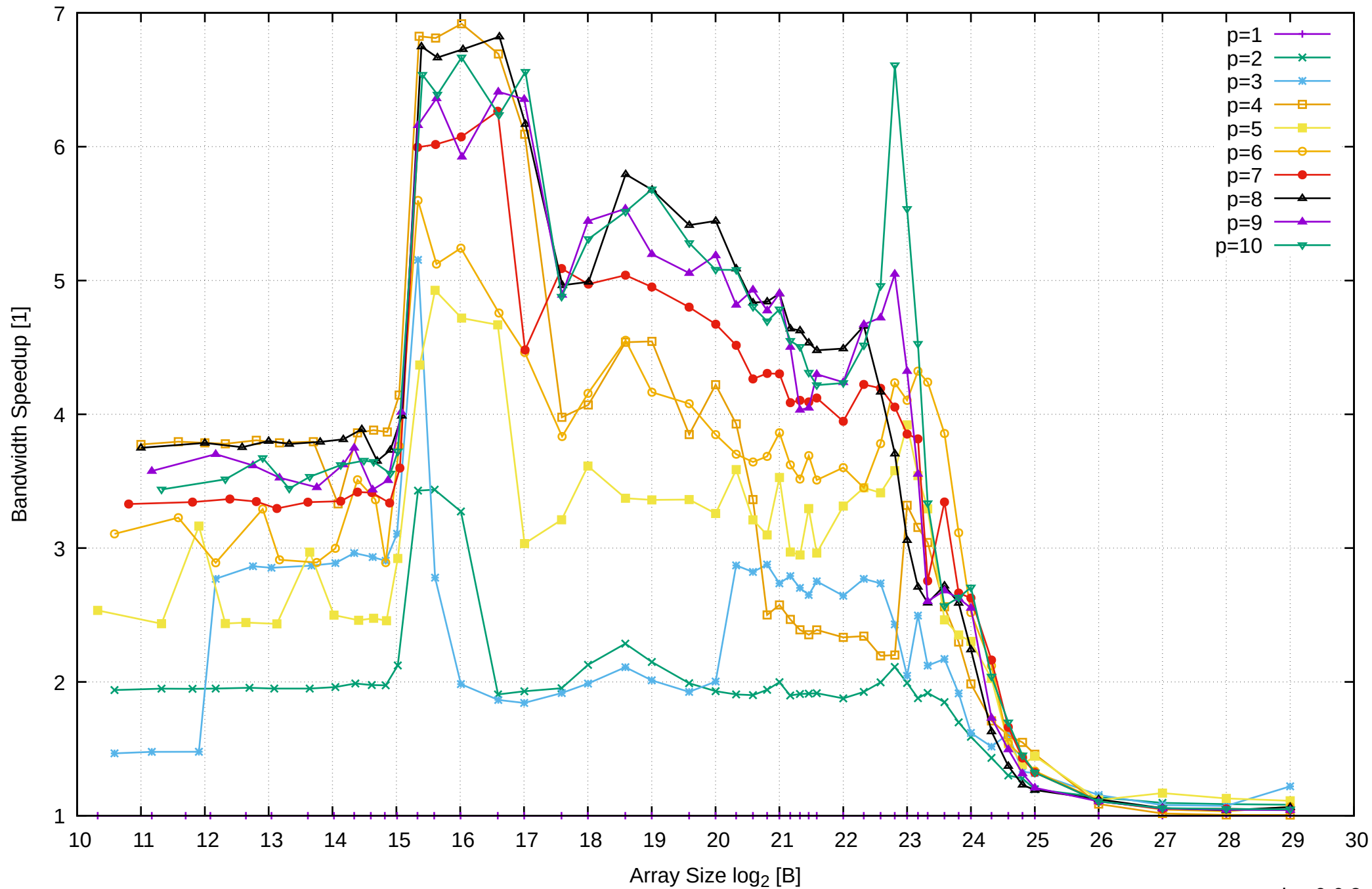
Intel Xeon E3-1260L v5 64GB - Speedup of Parallel Memory Bandwidth - ScanRead128PtrUnrollLoop
