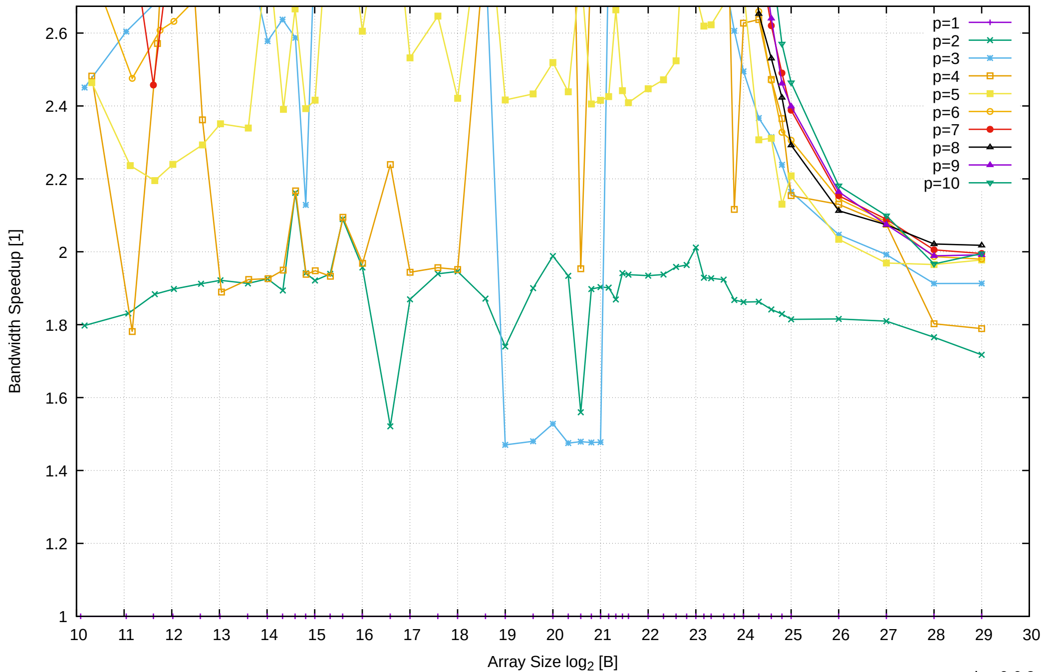
Intel Xeon E3-1260L v5 64GB - Speedup of Parallel Memory Bandwidth (enlarged) - ScanRead32PtrSimpleLoop
