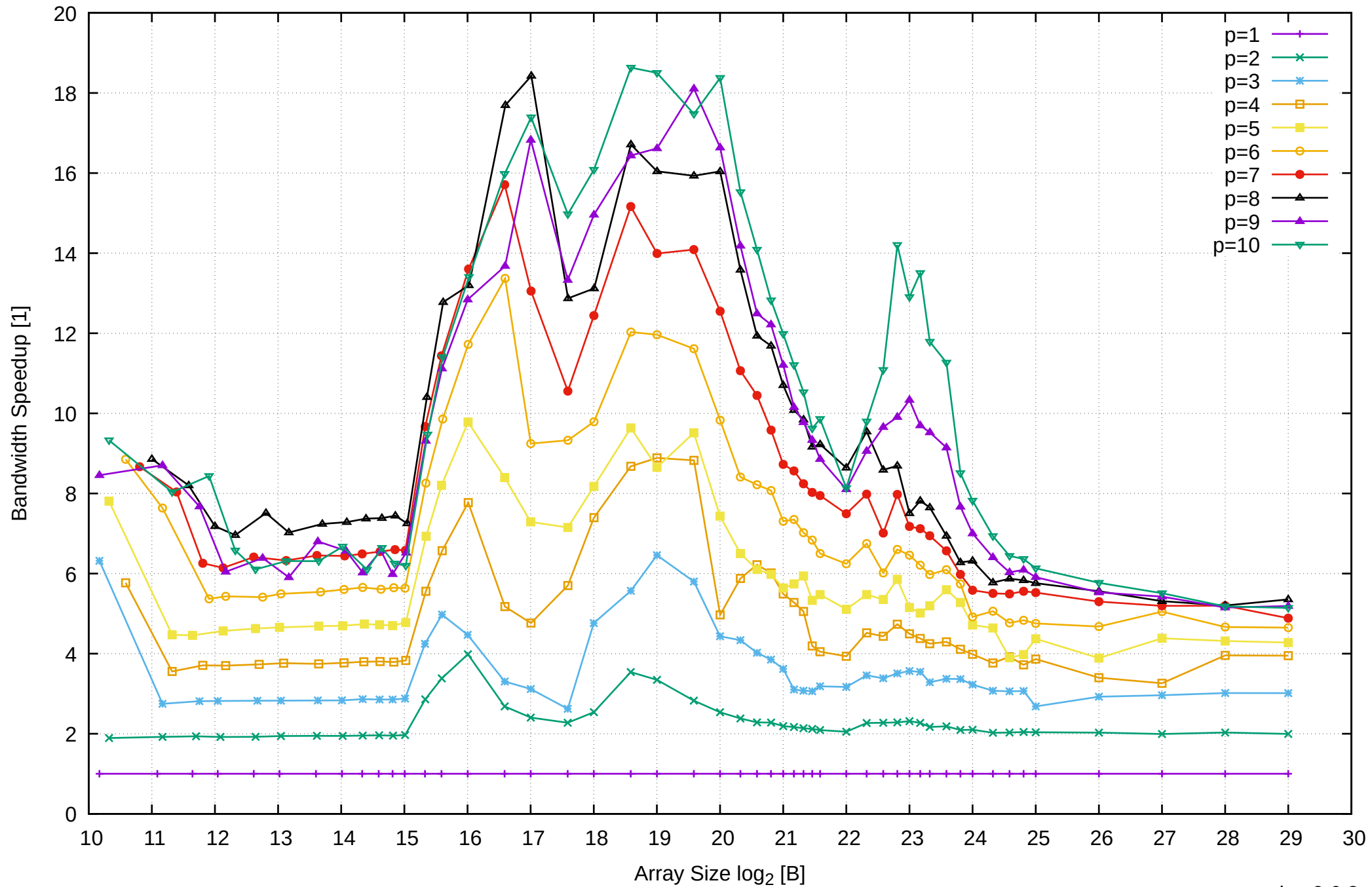
Intel Xeon E3-1260L v5 64GB - Speedup of Parallel Memory Bandwidth - PermRead64SimpleLoop
