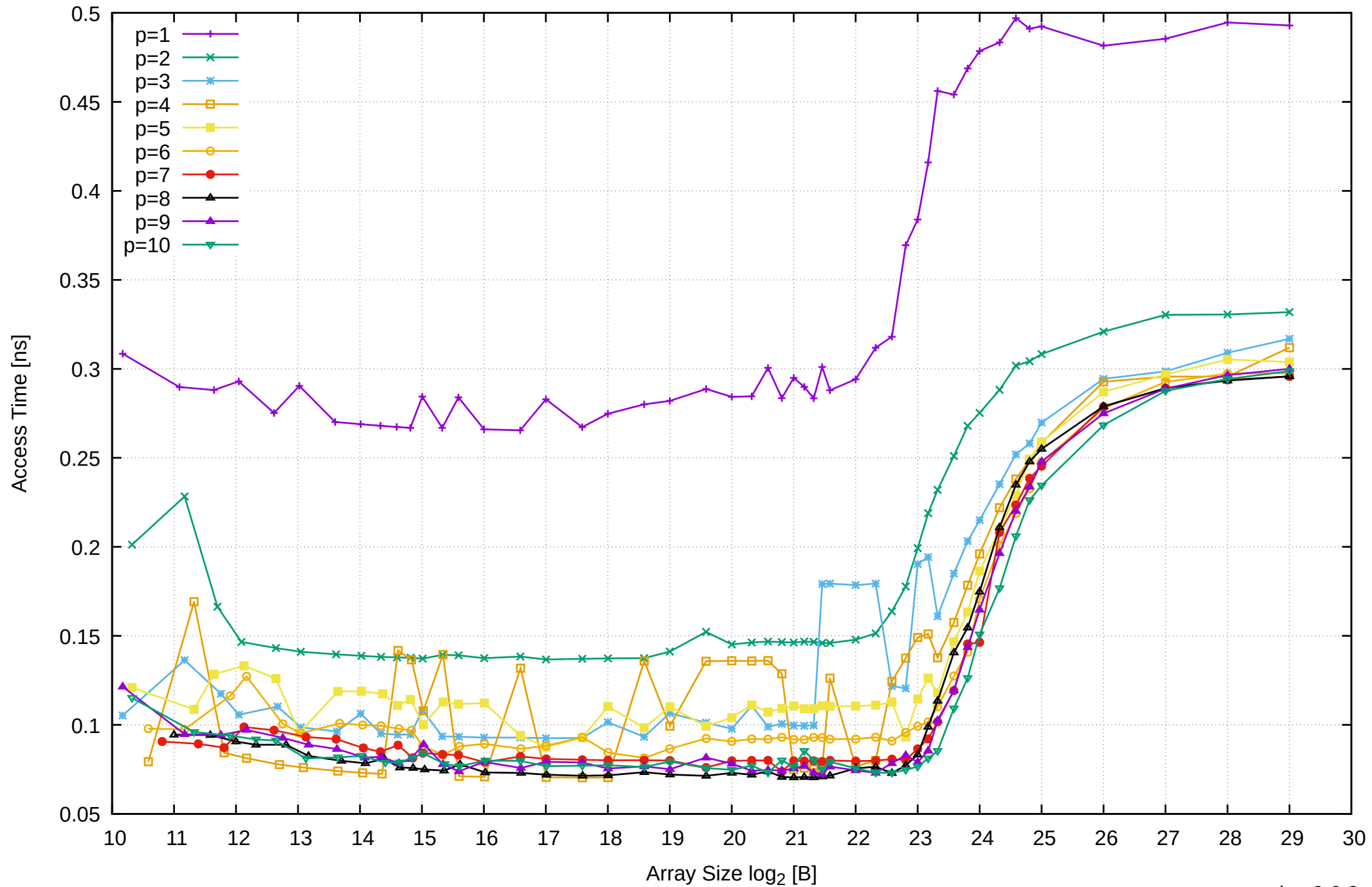
Intel Xeon E3-1260L v5 64GB - Parallel Memory Access Time - ScanRead64IndexSimpleLoop
