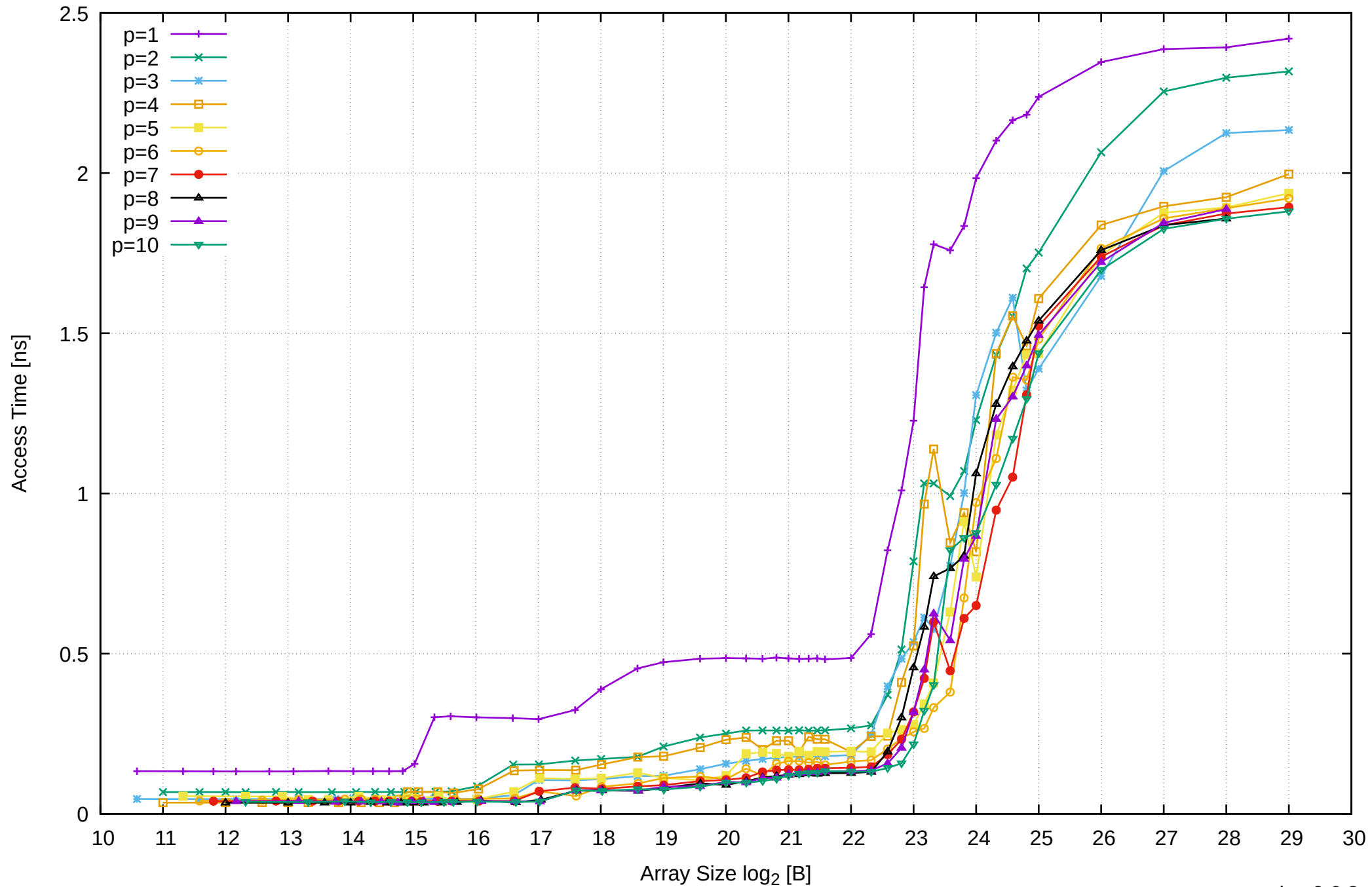
Intel Xeon E3-1260L v5 64GB - Parallel Memory Access Time - ScanRead256PtrUnrollLoop
