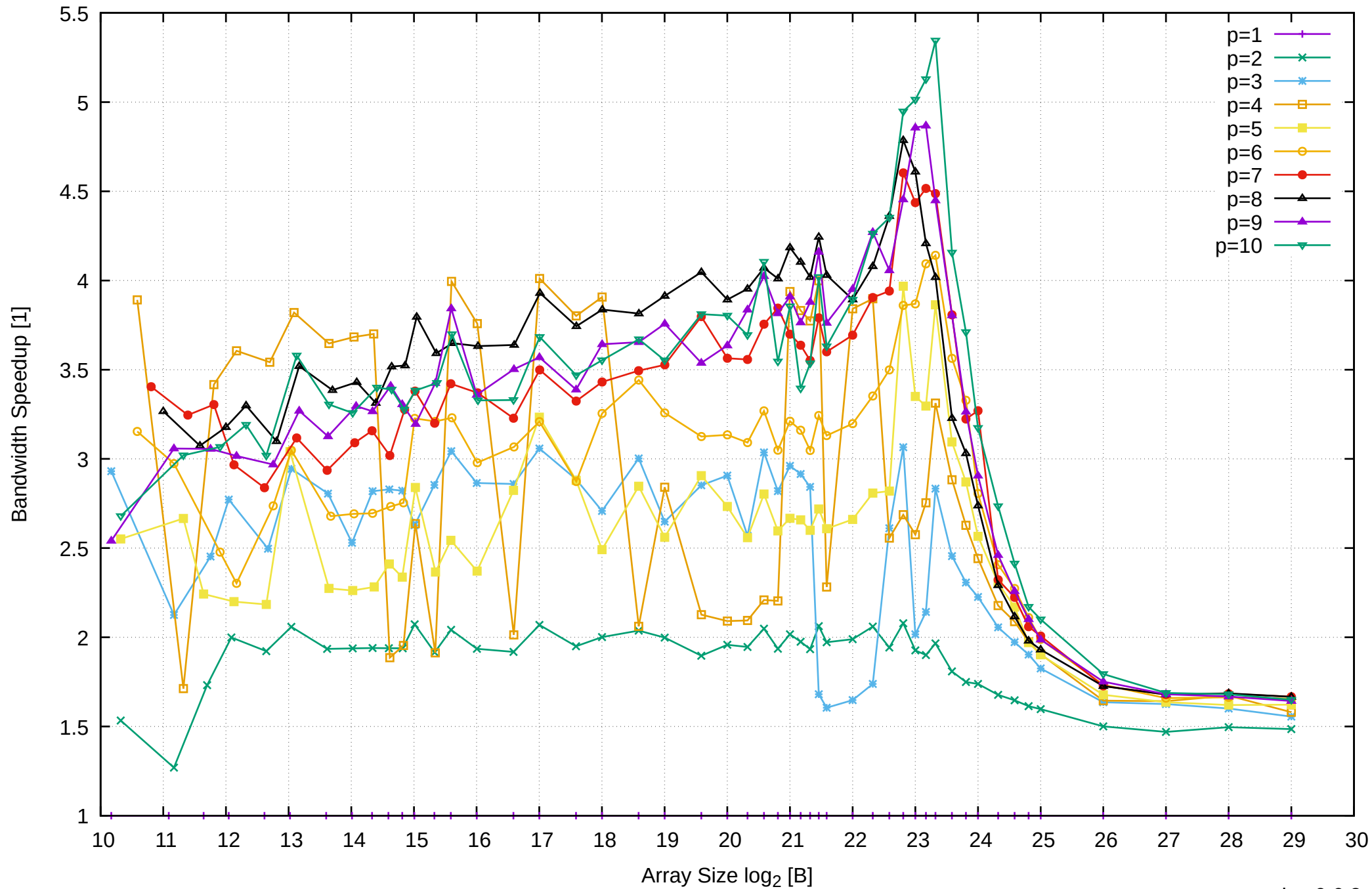
Intel Xeon E3-1260L v5 64GB - Speedup of Parallel Memory Bandwidth - ScanRead64IndexSimpleLoop
