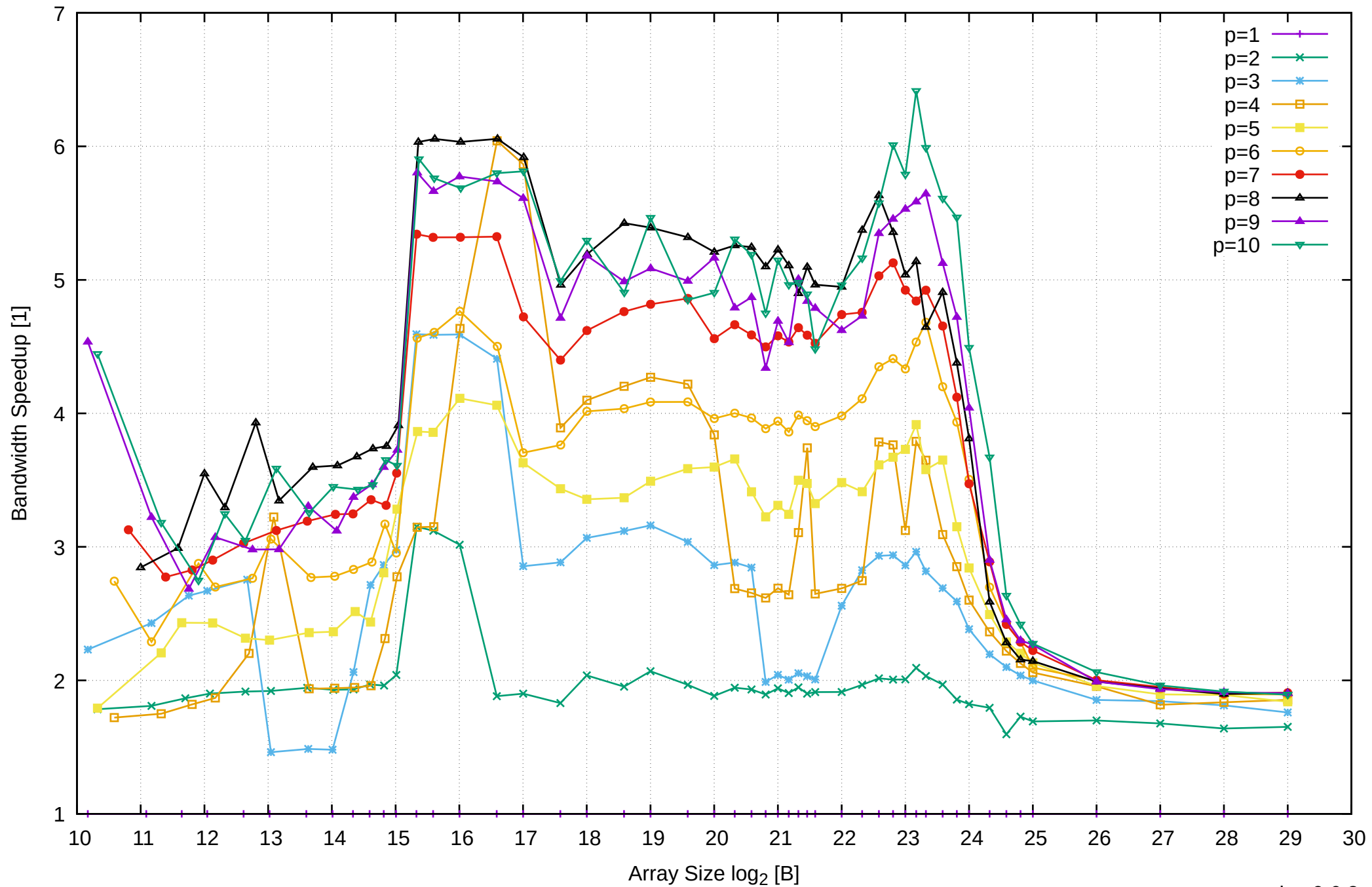
Intel Xeon E3-1260L v5 64GB - Speedup of Parallel Memory Bandwidth - ScanRead64IndexUnrollLoop
