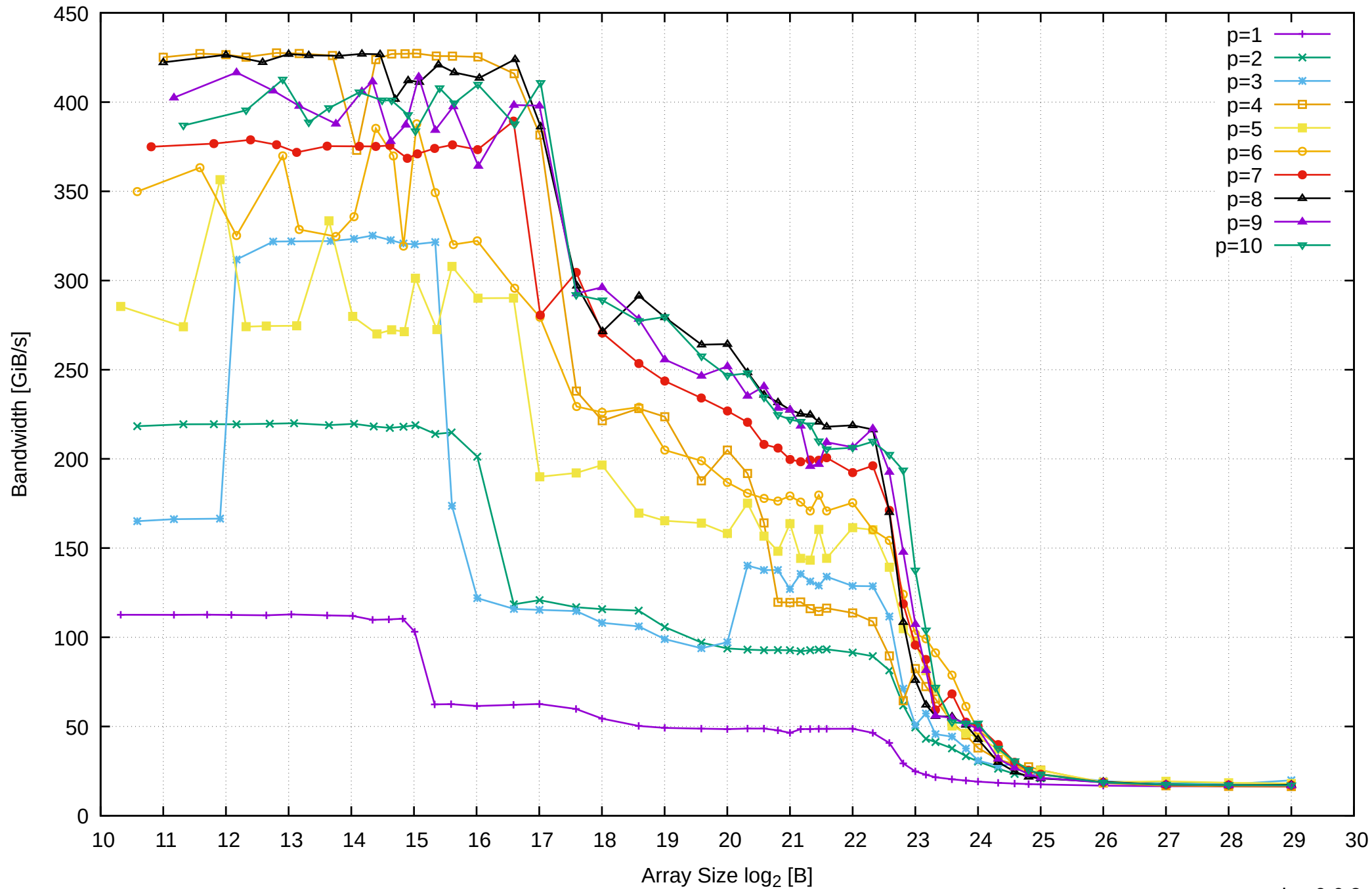
Intel Xeon E3-1260L v5 64GB - Parallel Memory Bandwidth - ScanRead128PtrUnrollLoop
