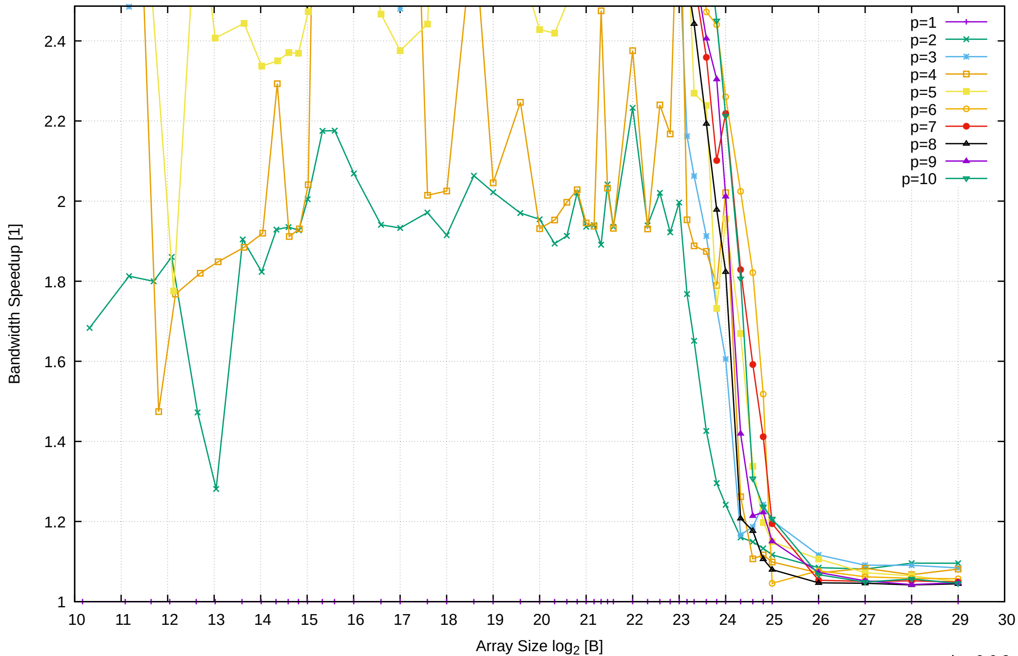
Intel Xeon E3-1260L v5 64GB - Speedup of Parallel Memory Bandwidth (enlarged) - ScanWrite64IndexSimpleLoop
