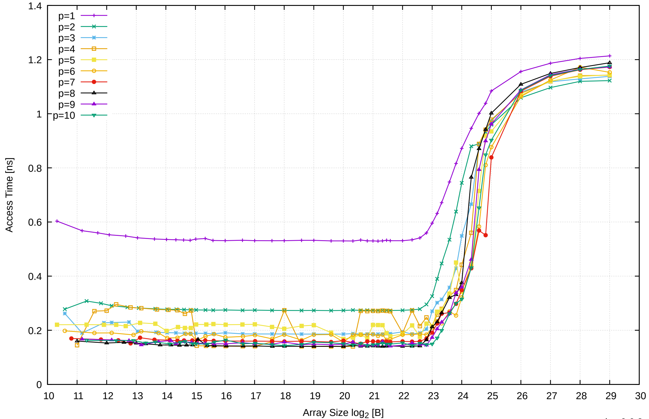
Intel Xeon E3-1260L v5 64GB - Parallel Memory Access Time - ScanWrite128PtrSimpleLoop
