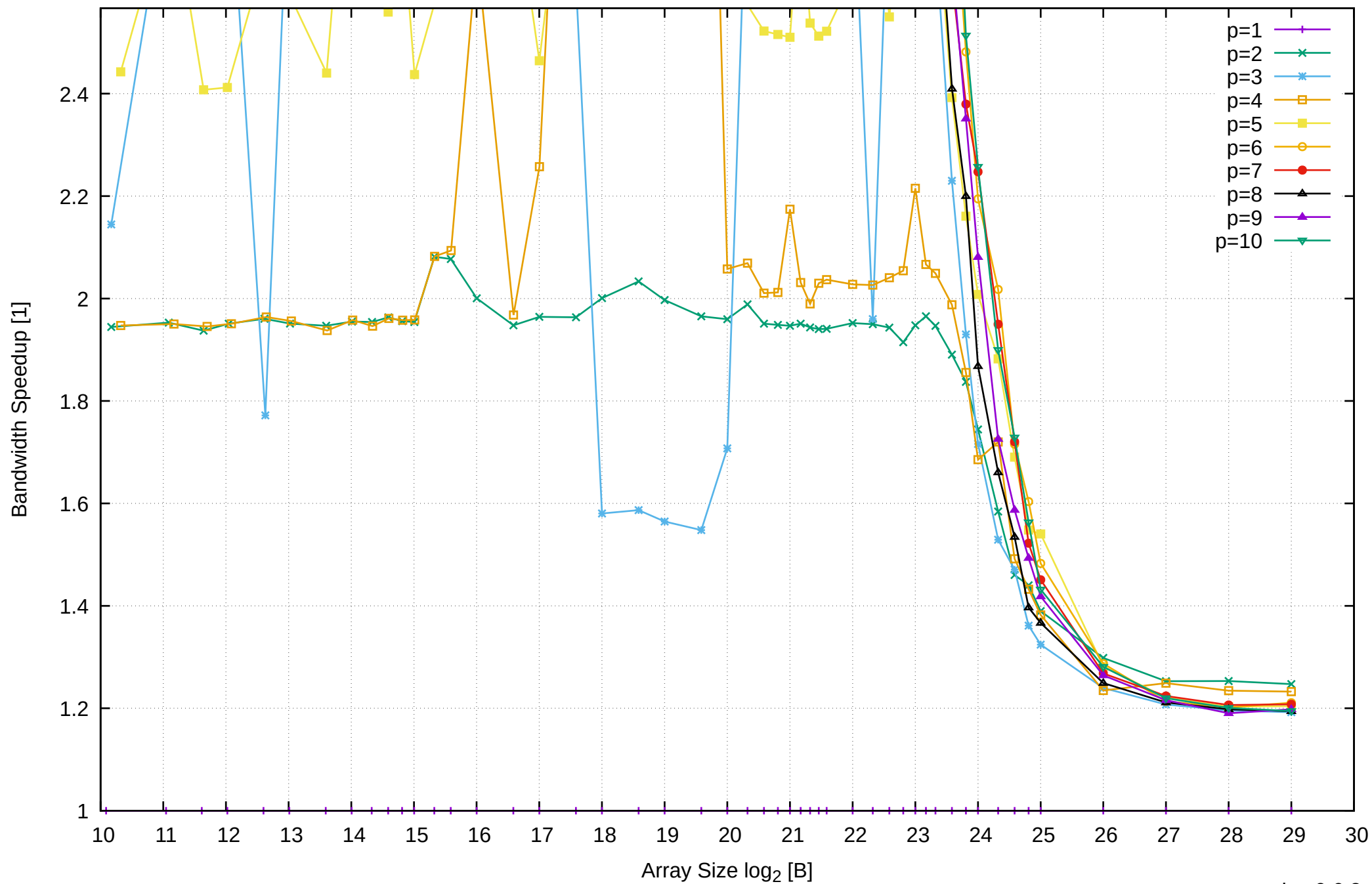
Intel Xeon E3-1260L v5 64GB - Speedup of Parallel Memory Bandwidth (enlarged) - ScanWrite32PtrUnrollLoop
