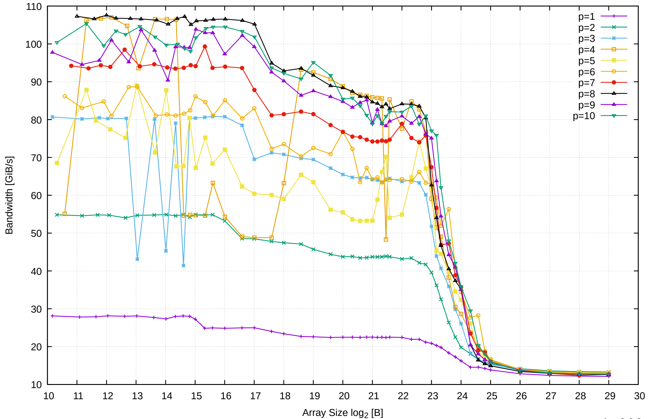
Intel Xeon E3-1260L v5 64GB - Parallel Memory Bandwidth - ScanWrite64PtrUnrollLoop
