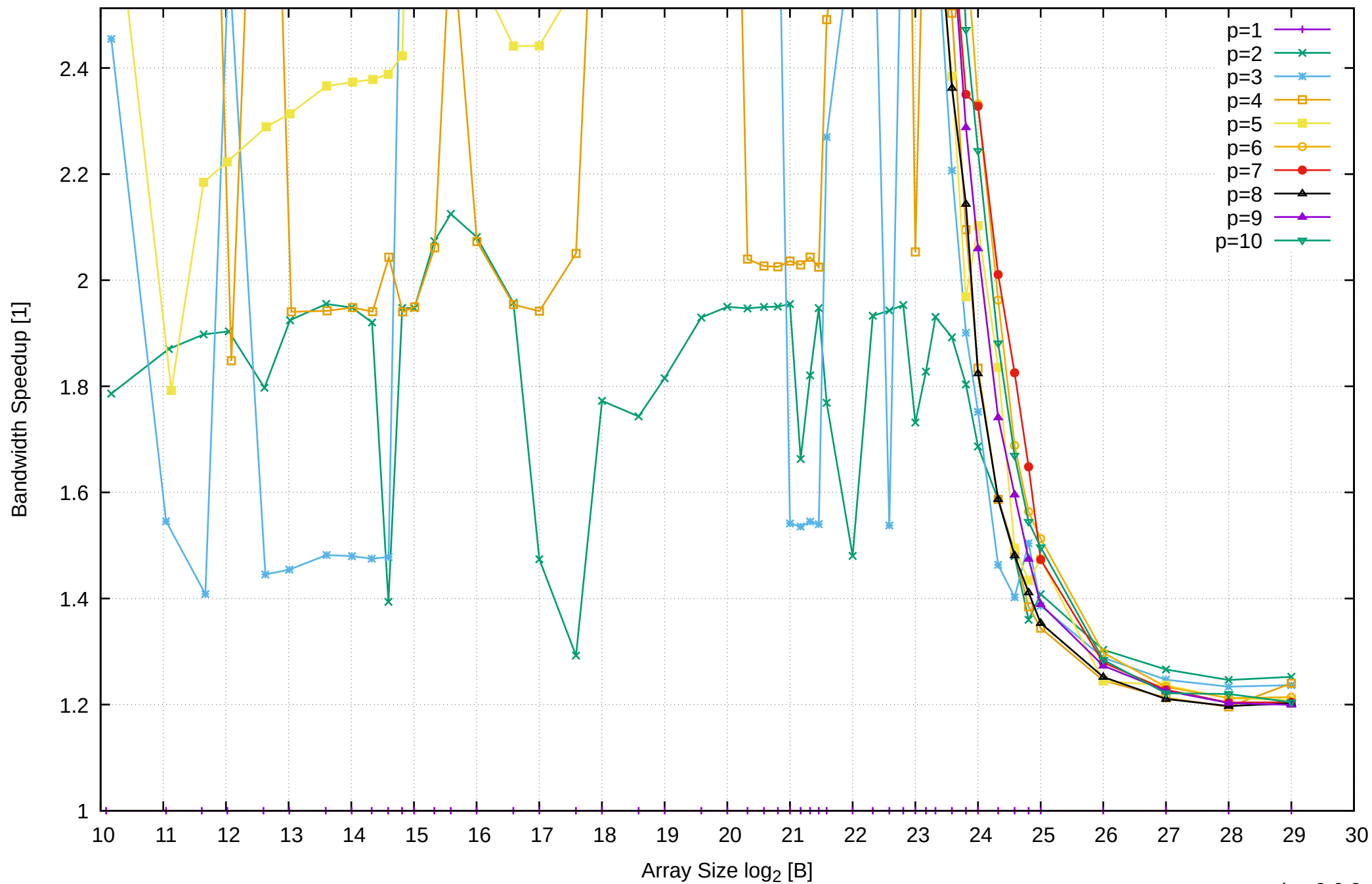
Intel Xeon E3-1260L v5 64GB - Speedup of Parallel Memory Bandwidth (enlarged) - ScanWrite32PtrSimpleLoop
