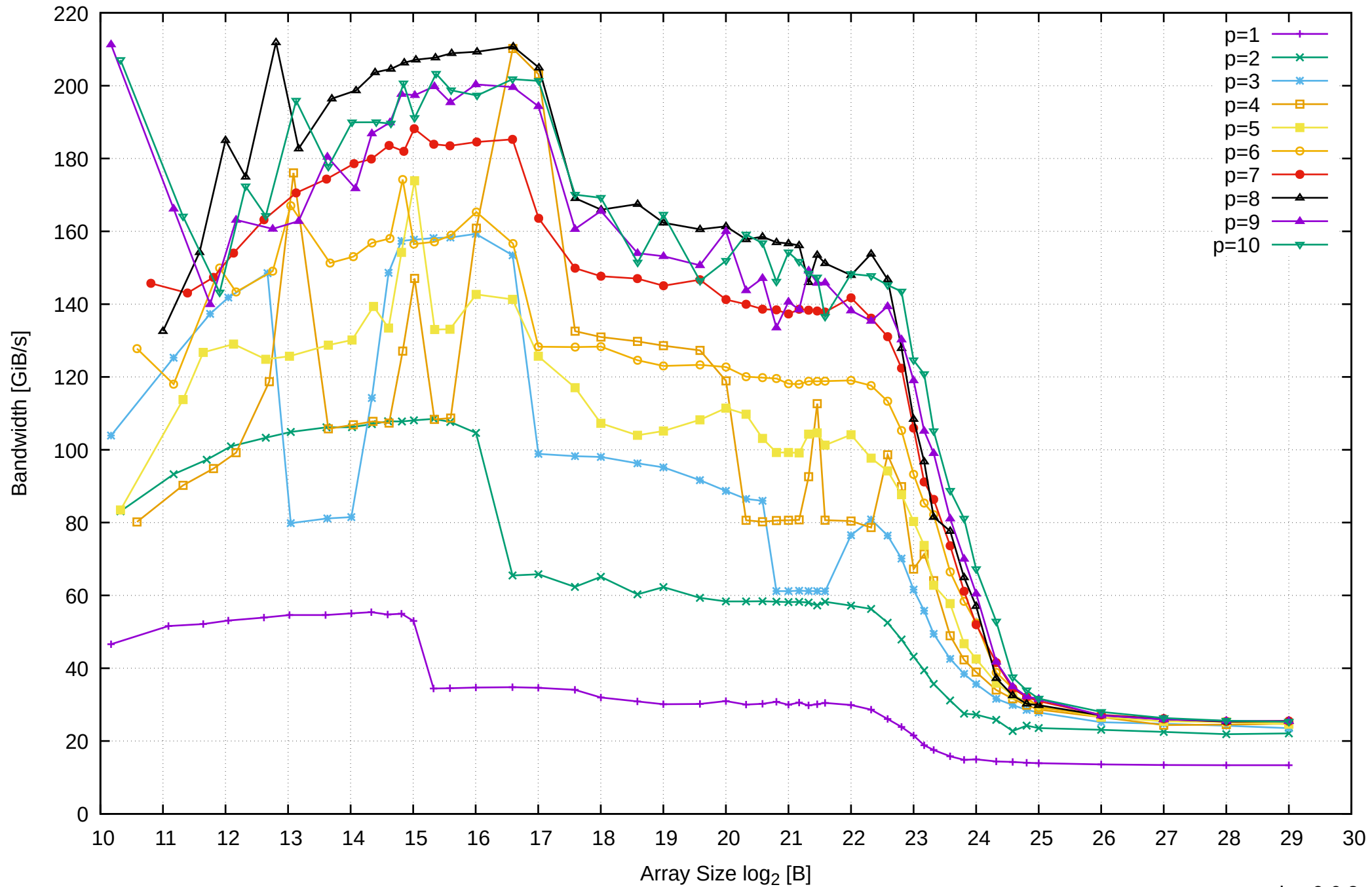
Intel Xeon E3-1260L v5 64GB - Parallel Memory Bandwidth - ScanRead64IndexUnrollLoop
