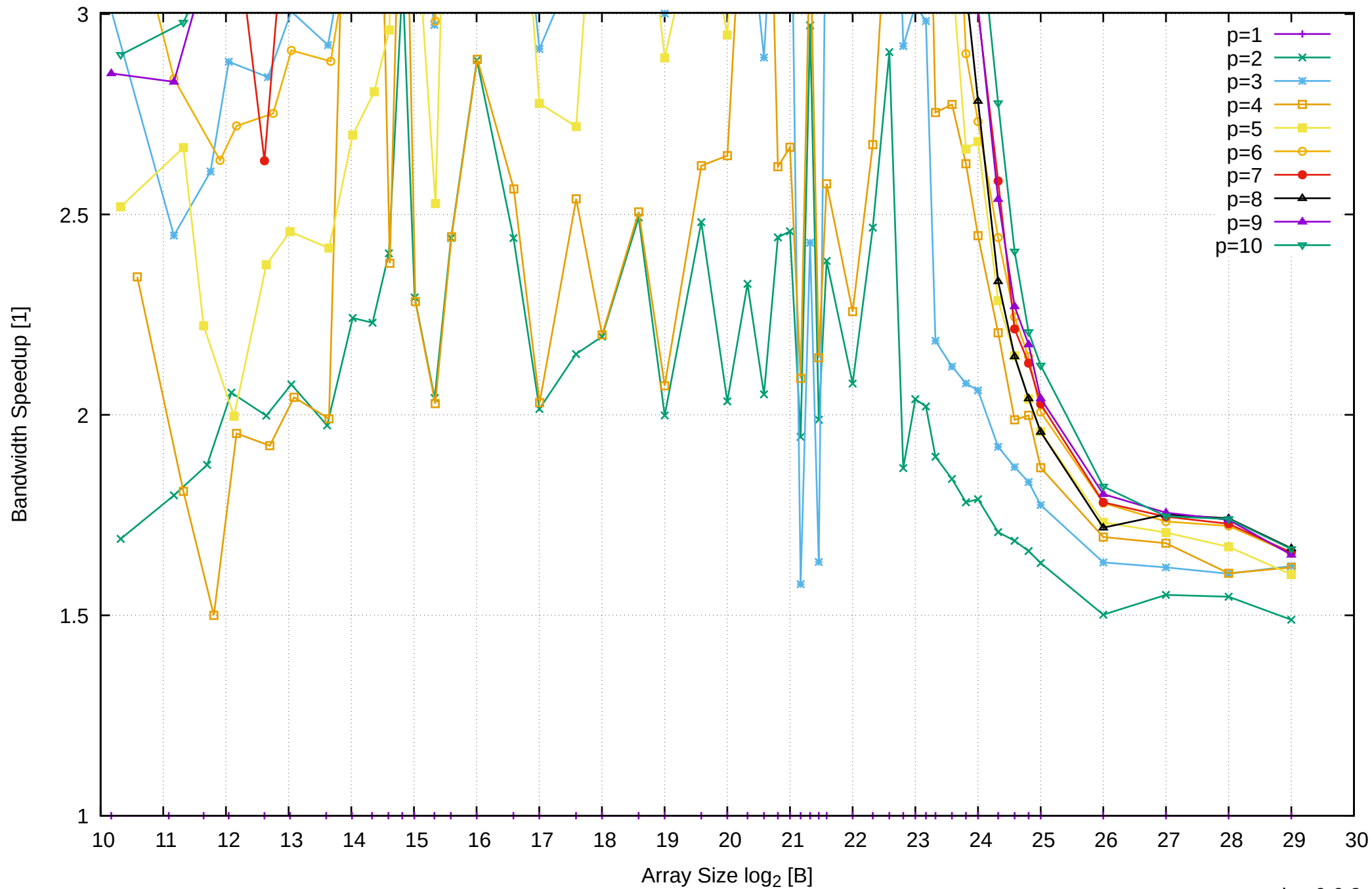
Intel Xeon E3-1260L v5 64GB - Speedup of Parallel Memory Bandwidth (enlarged) - ScanRead64PtrSimpleLoop
