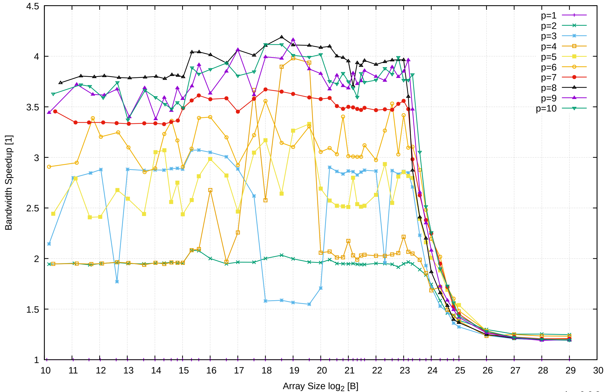
Intel Xeon E3-1260L v5 64GB - Speedup of Parallel Memory Bandwidth - ScanWrite32PtrUnrollLoop
