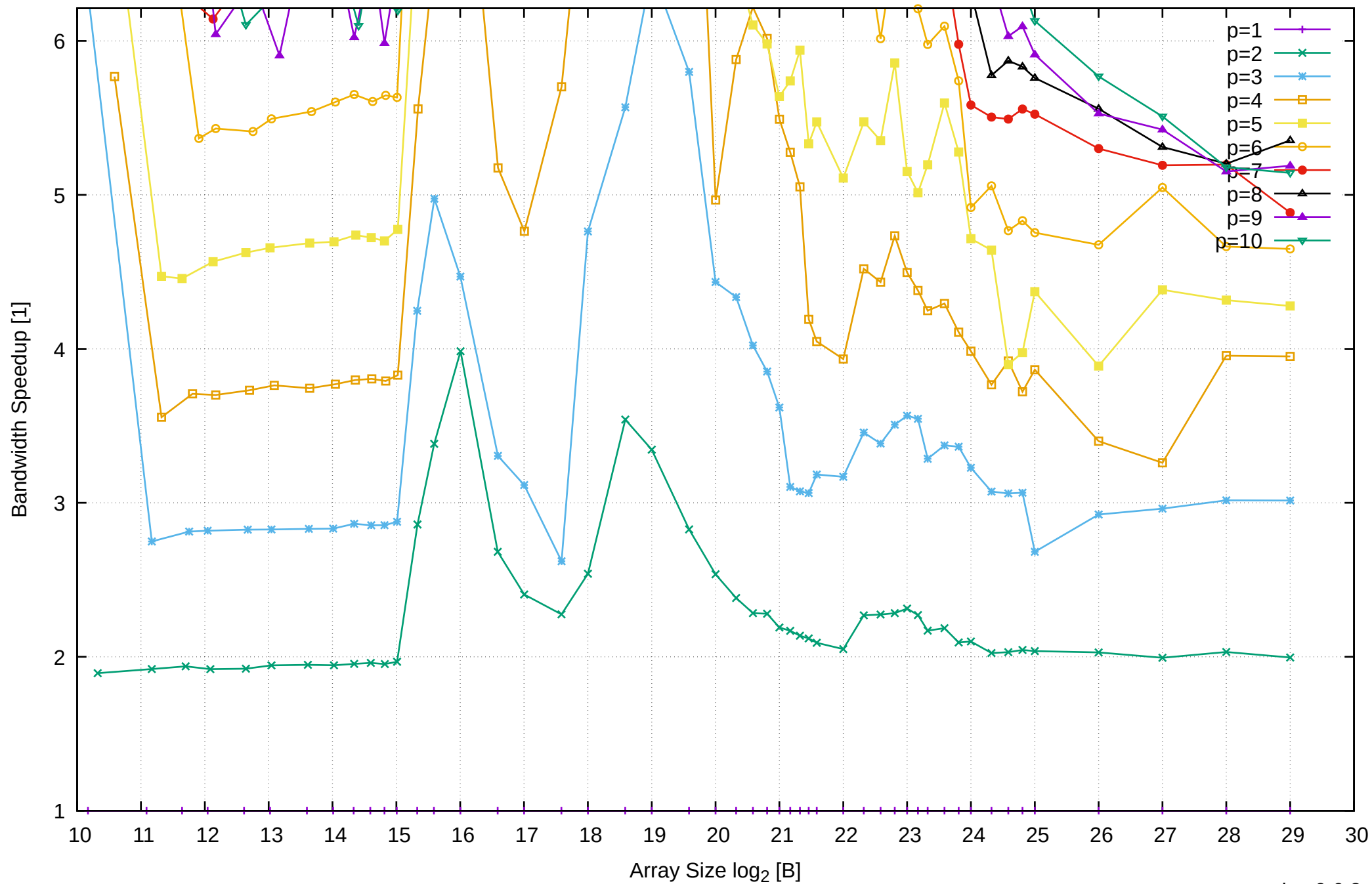
Intel Xeon E3-1260L v5 64GB - Speedup of Parallel Memory Bandwidth (enlarged) - PermRead64SimpleLoop
