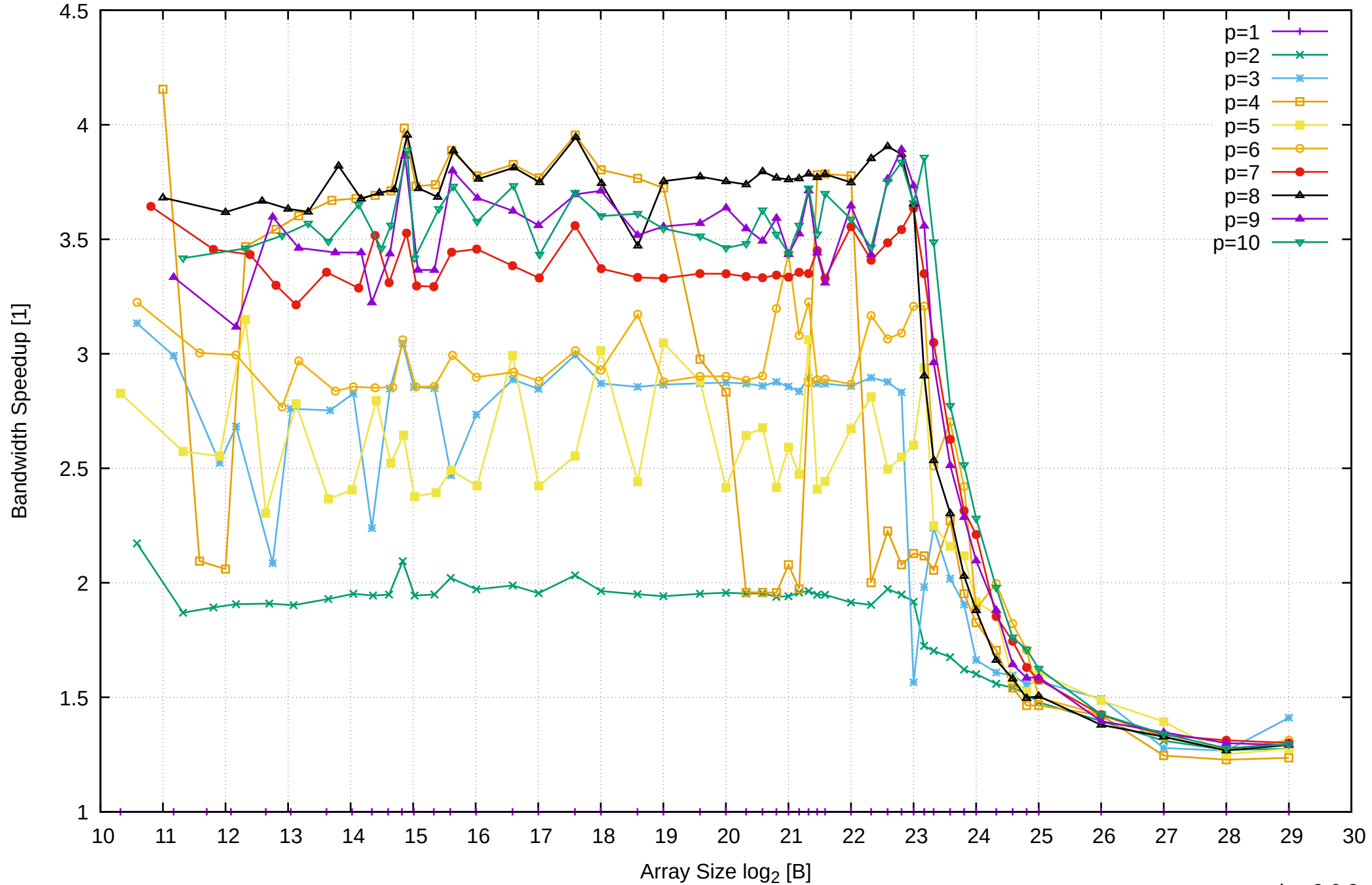
Intel Xeon E3-1260L v5 64GB - Speedup of Parallel Memory Bandwidth - ScanRead128PtrSimpleLoop
