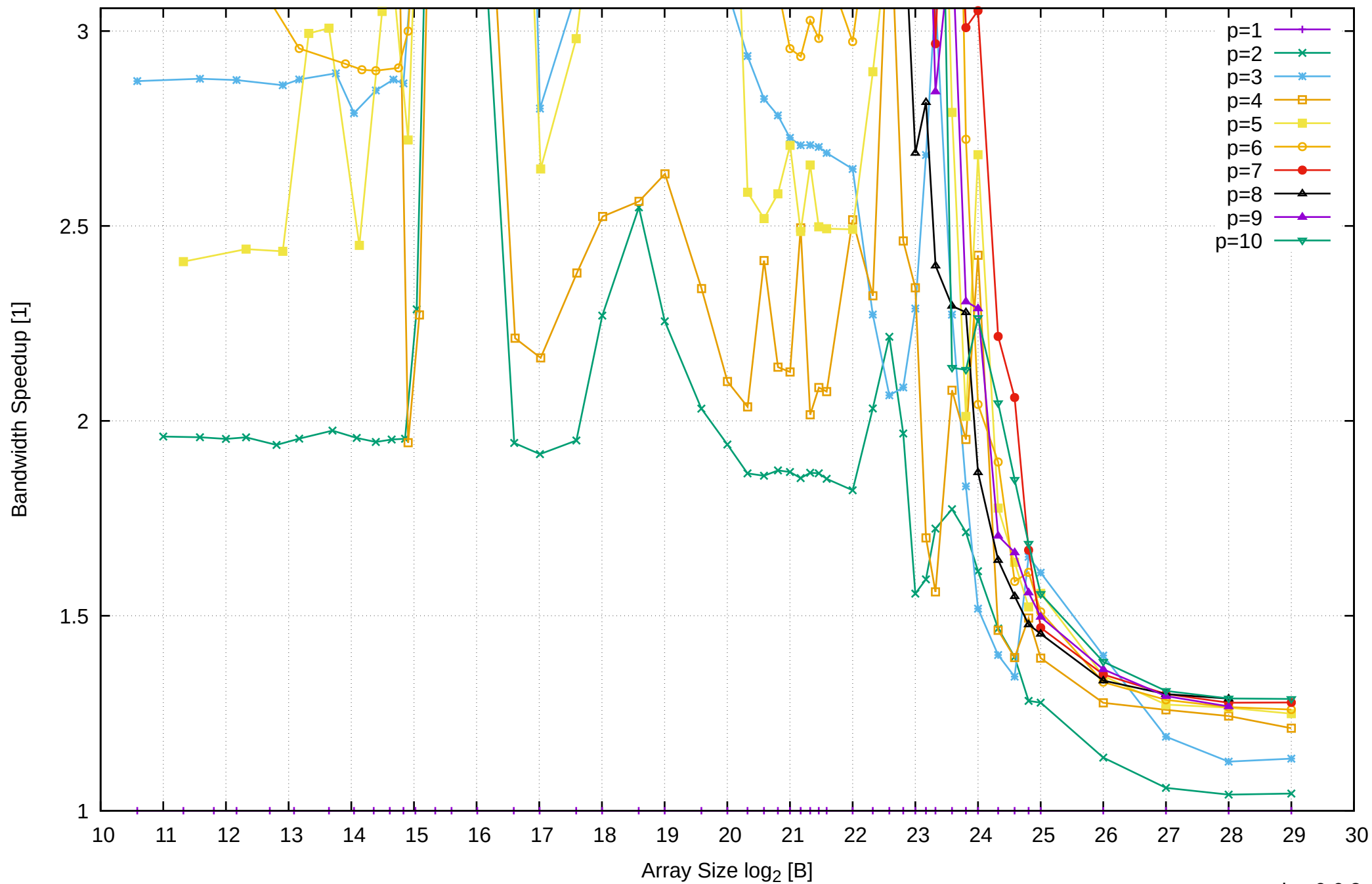
Intel Xeon E3-1260L v5 64GB - Speedup of Parallel Memory Bandwidth (enlarged) - ScanRead256PtrUnrollLoop
