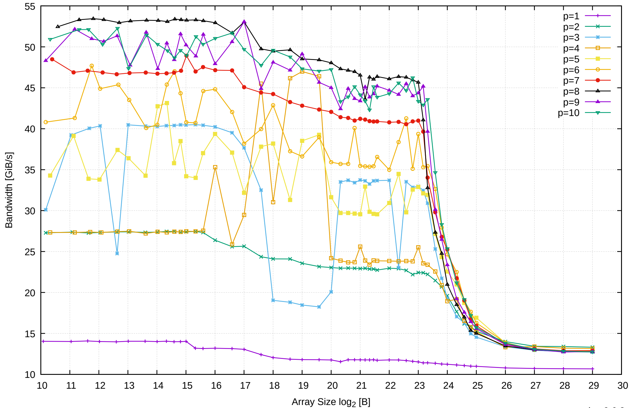
Intel Xeon E3-1260L v5 64GB - Parallel Memory Bandwidth - ScanWrite32PtrUnrollLoop
