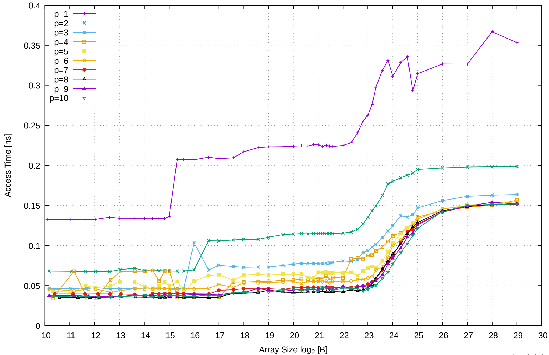
Intel Xeon E3-1260L v5 64GB - Parallel Memory Access Time - ScanRead32PtrUnrollLoop
