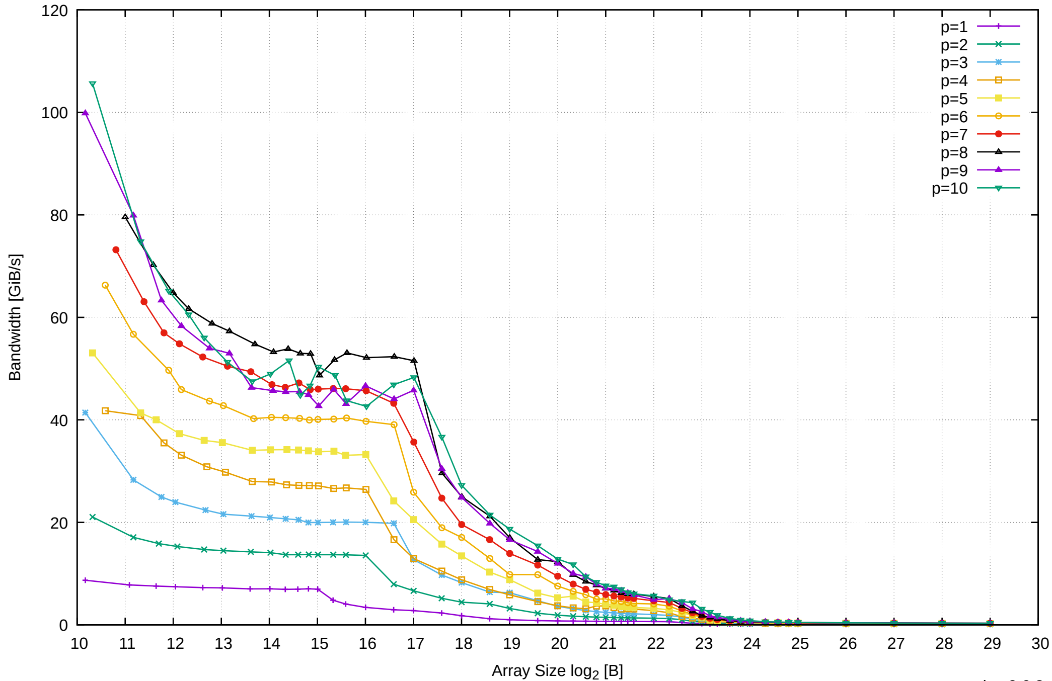
Intel Xeon E3-1260L v5 64GB - Parallel Memory Bandwidth - PermRead64UnrollLoop
