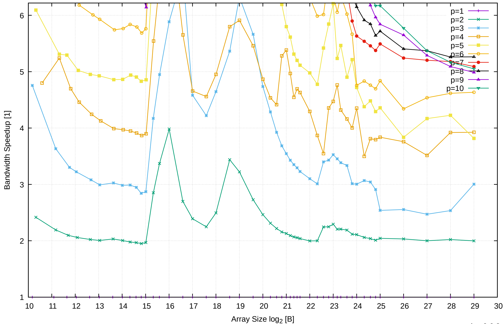
Intel Xeon E3-1260L v5 64GB - Speedup of Parallel Memory Bandwidth (enlarged) - PermRead64UnrollLoop
