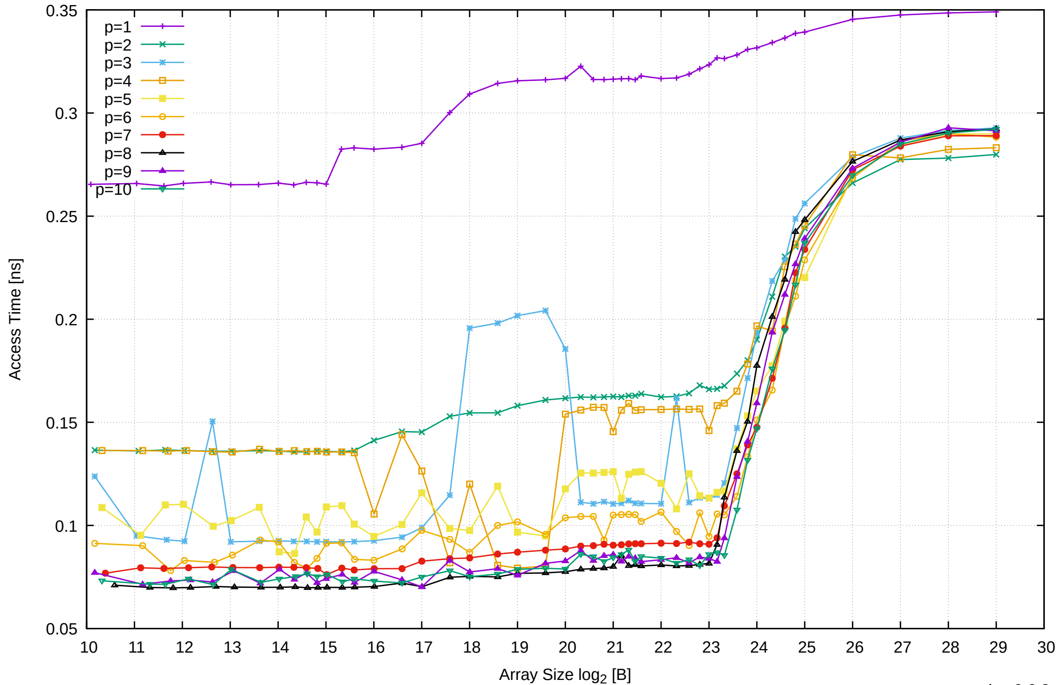
Intel Xeon E3-1260L v5 64GB - Parallel Memory Access Time - ScanWrite32PtrUnrollLoop
