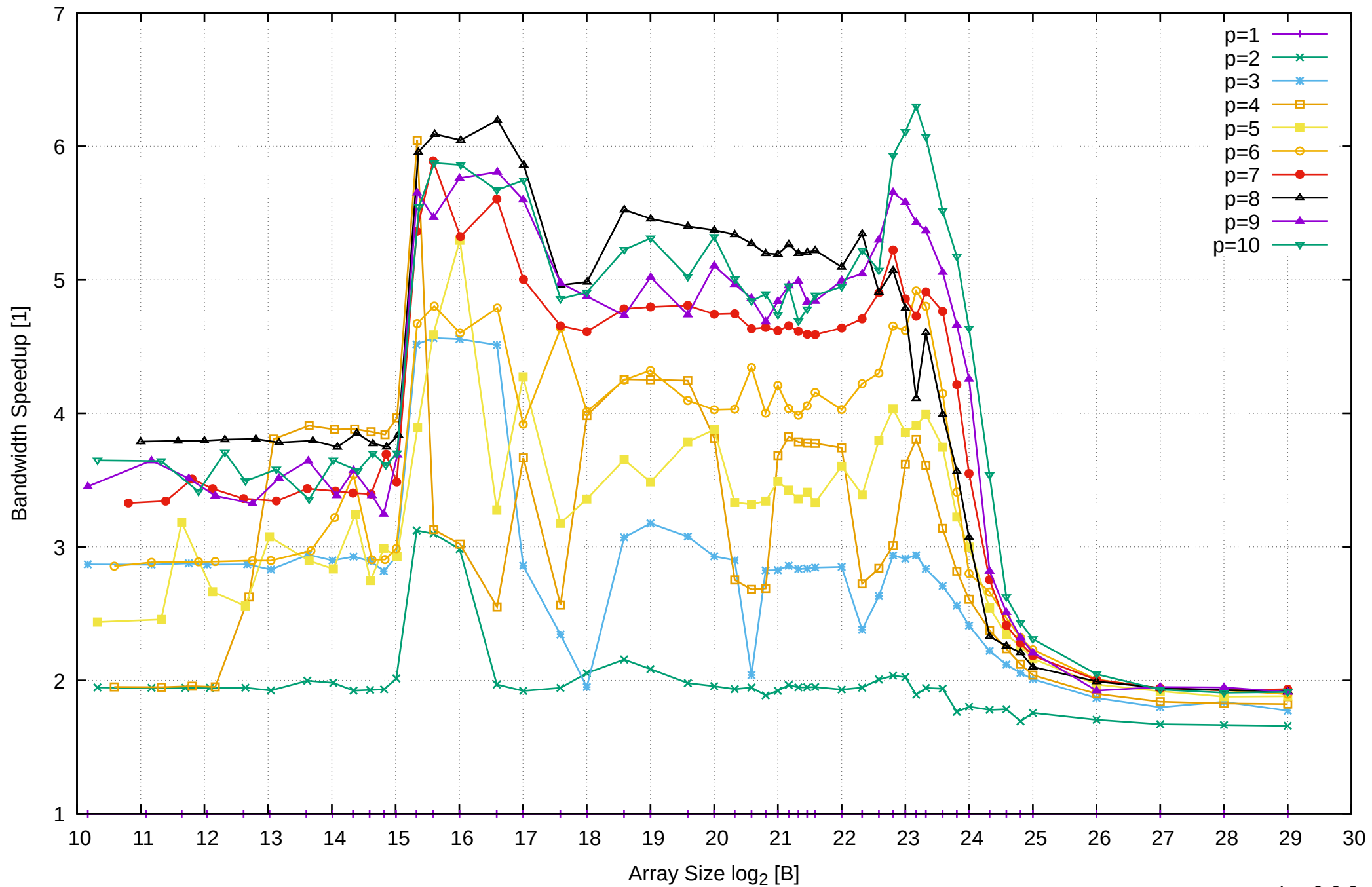
Intel Xeon E3-1260L v5 64GB - Speedup of Parallel Memory Bandwidth - ScanRead64PtrUnrollLoop
