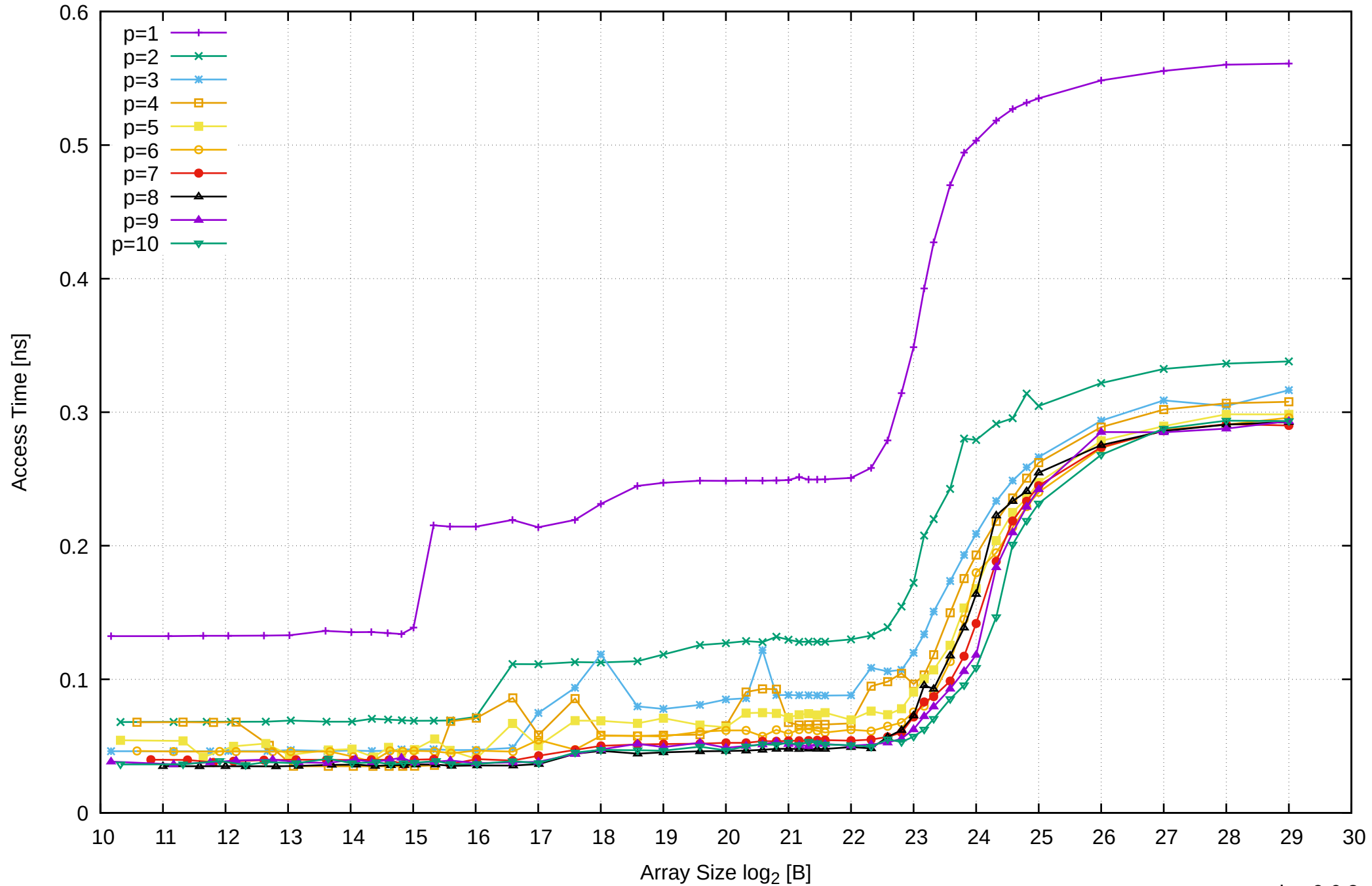
Intel Xeon E3-1260L v5 64GB - Parallel Memory Access Time - ScanRead64PtrUnrollLoop
