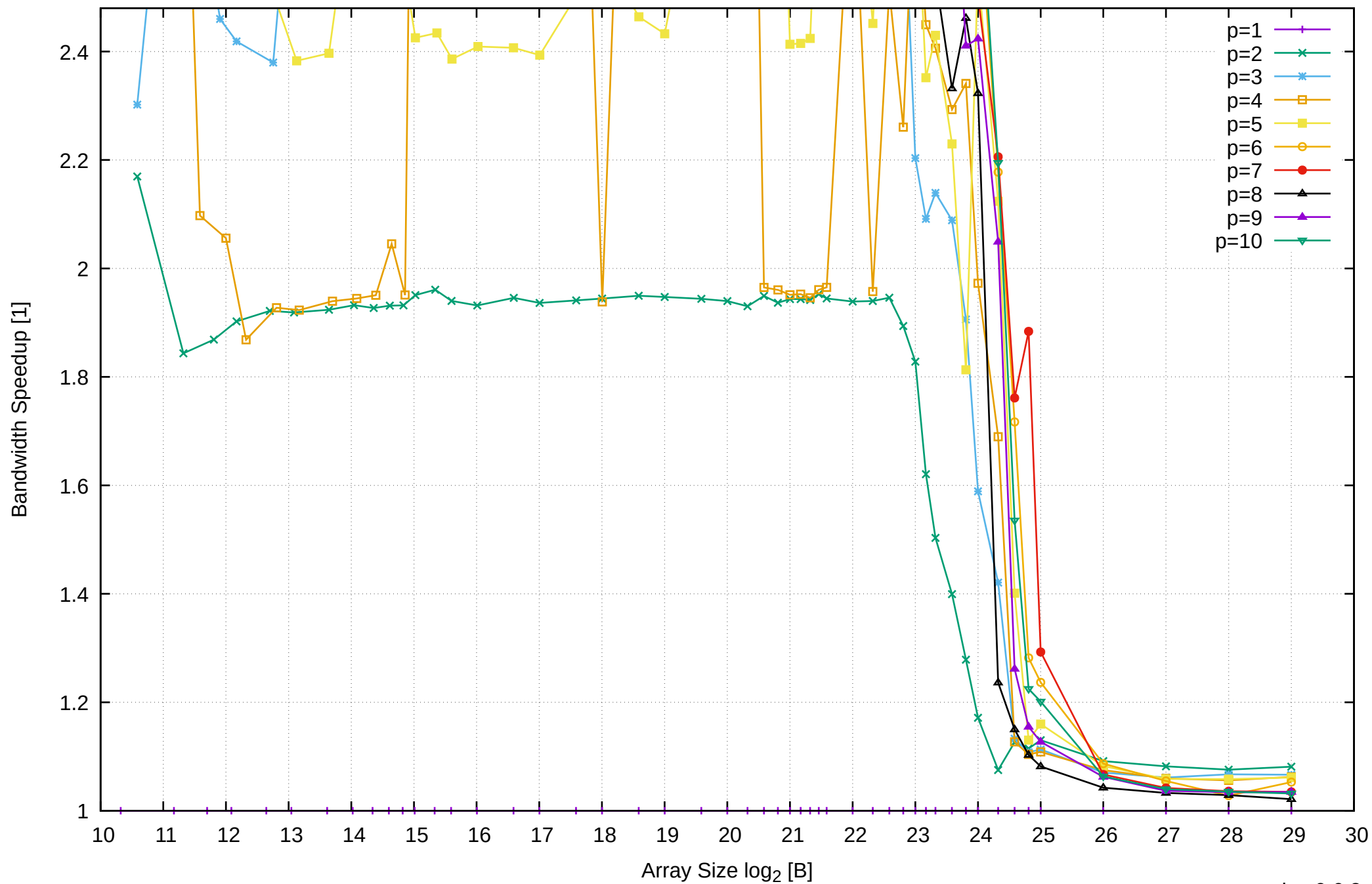
Intel Xeon E3-1260L v5 64GB - Speedup of Parallel Memory Bandwidth (enlarged) - ScanWrite128PtrSimpleLoop
