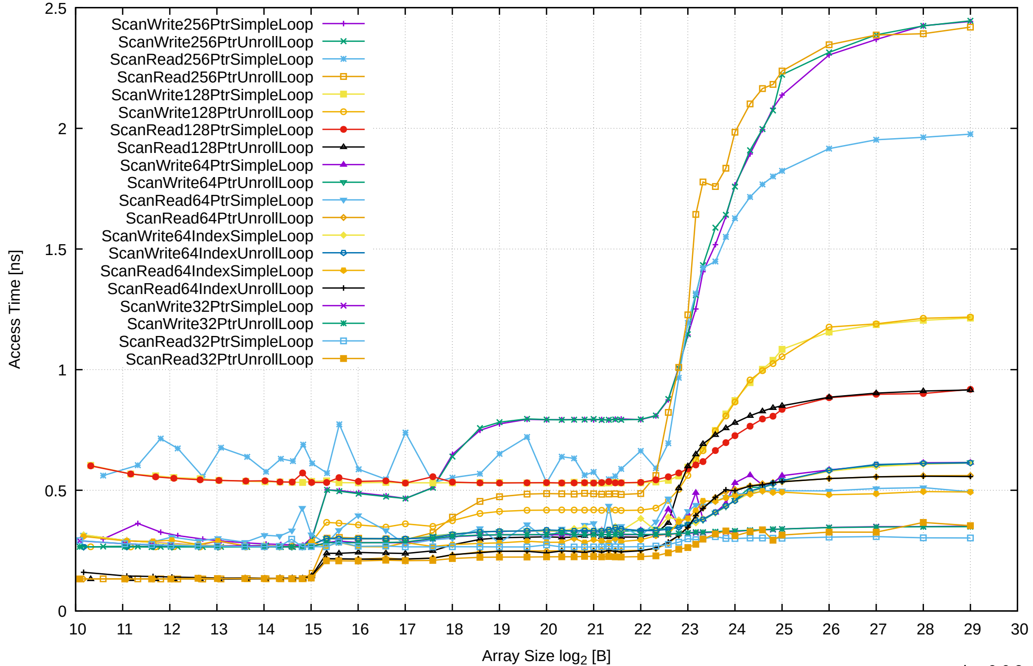
Intel Xeon E3-1260L v5 64GB - One Thread Memory Latency (excluding Permutation)
