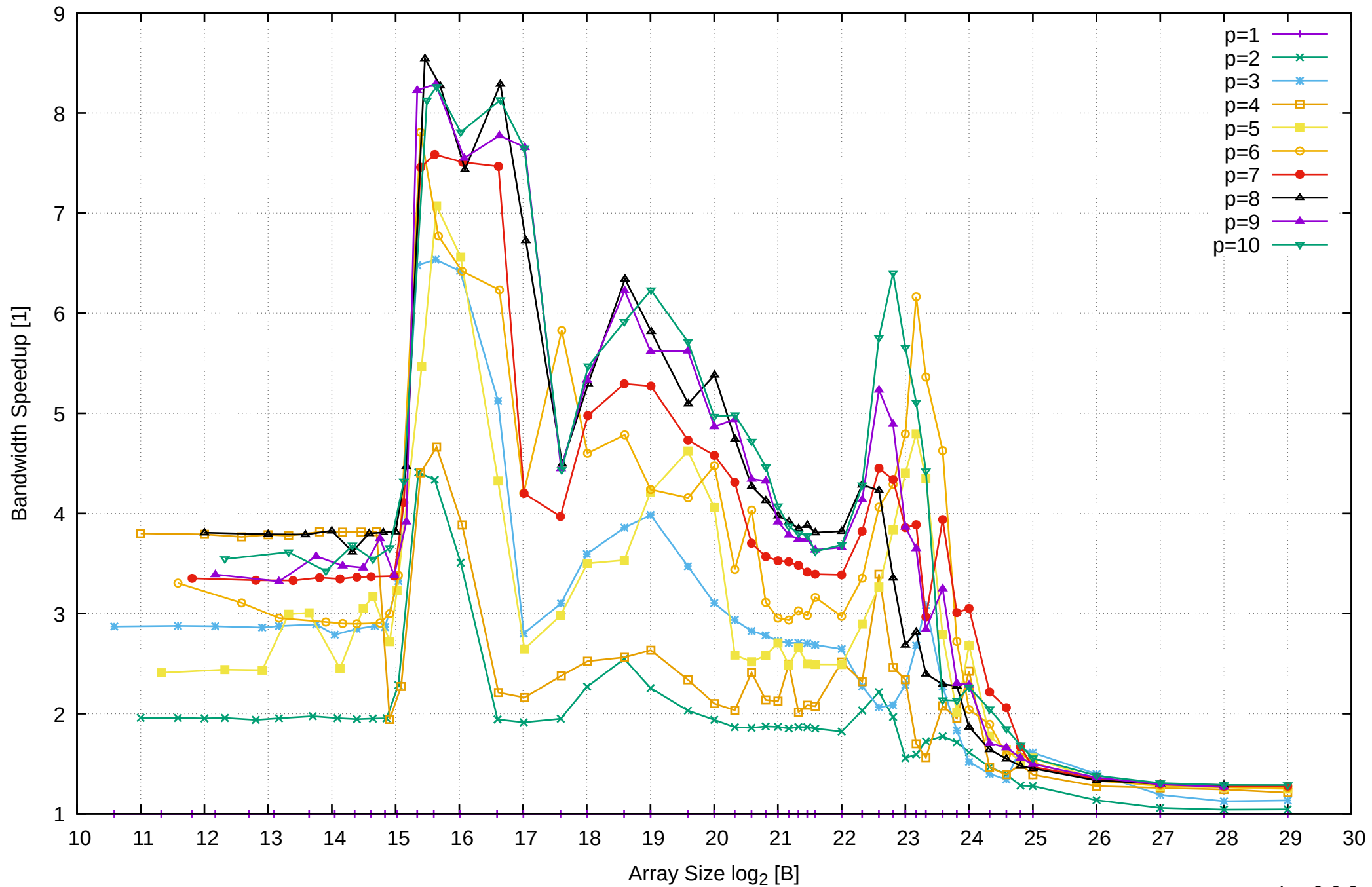
Intel Xeon E3-1260L v5 64GB - Speedup of Parallel Memory Bandwidth - ScanRead256PtrUnrollLoop
