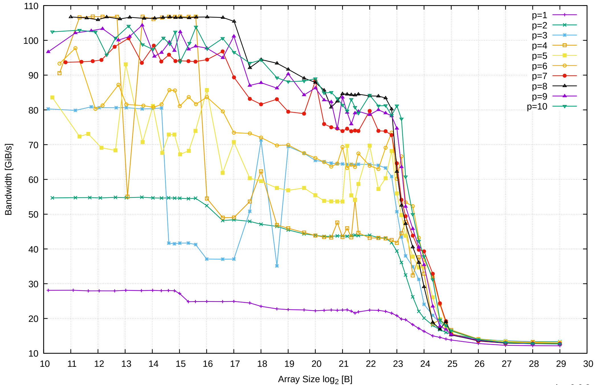
Intel Xeon E3-1260L v5 64GB - Parallel Memory Bandwidth - ScanWrite64IndexUnrollLoop
