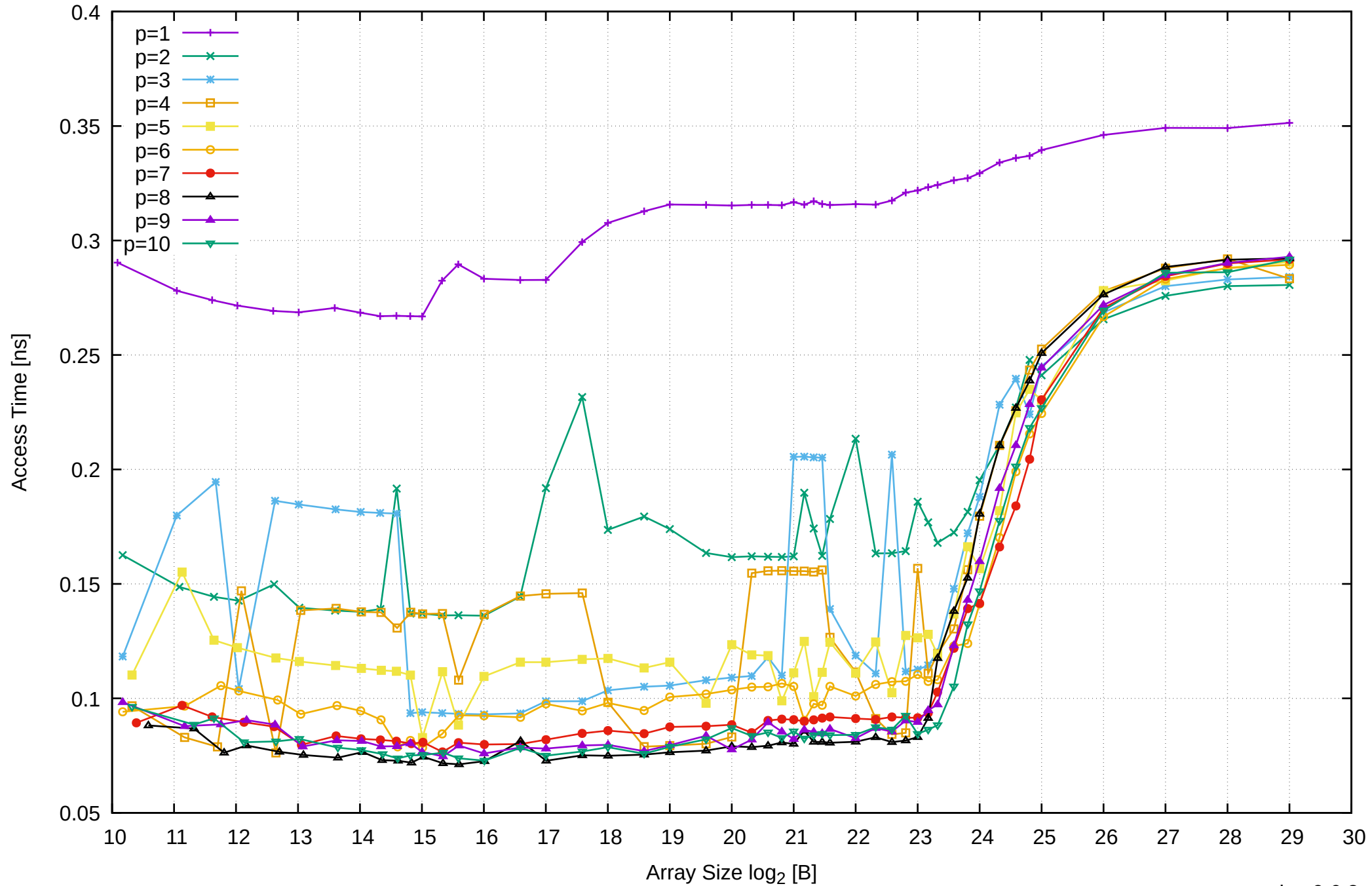
Intel Xeon E3-1260L v5 64GB - Parallel Memory Access Time - ScanWrite32PtrSimpleLoop
