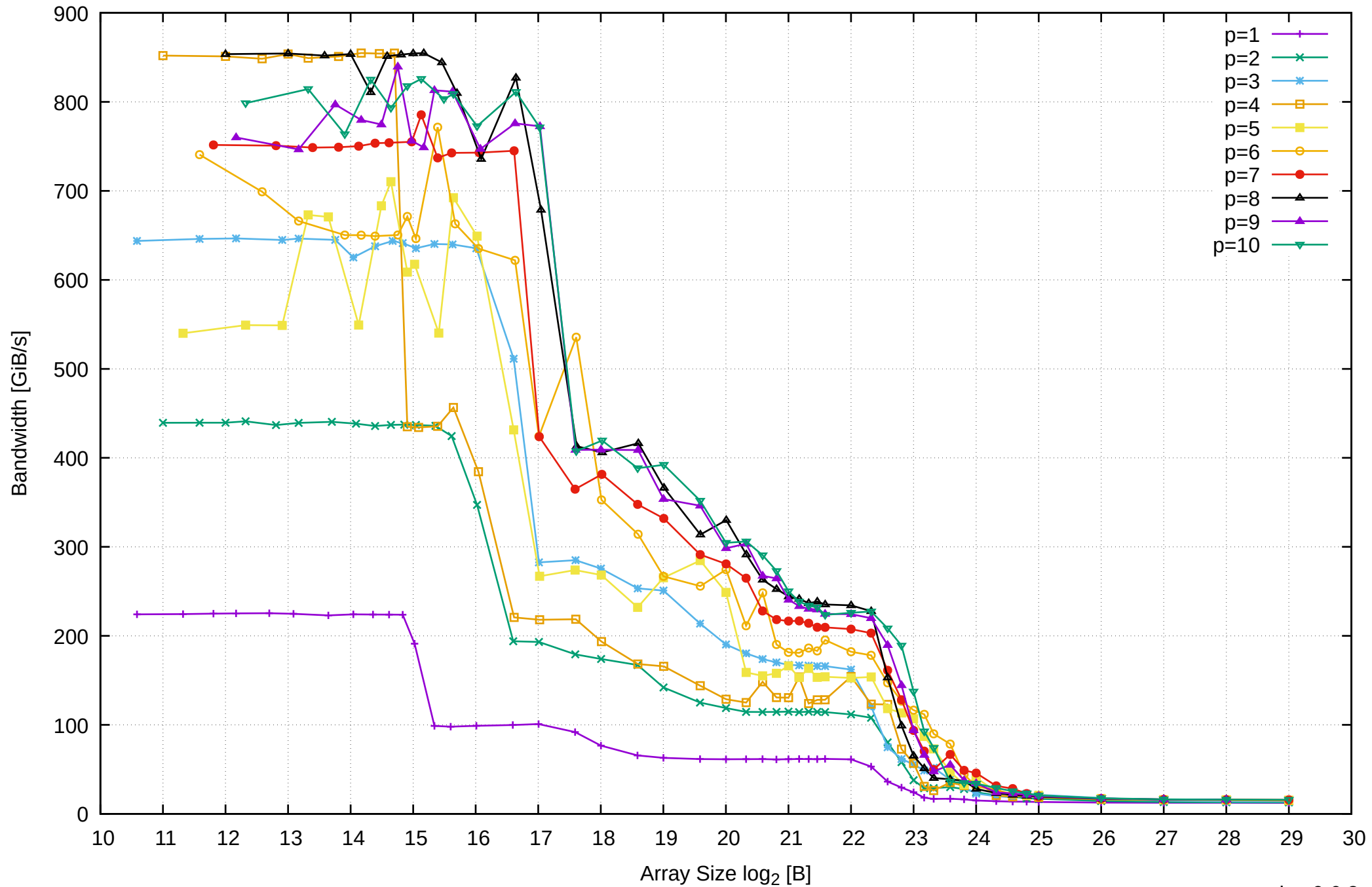
Intel Xeon E3-1260L v5 64GB - Parallel Memory Bandwidth - ScanRead256PtrUnrollLoop
