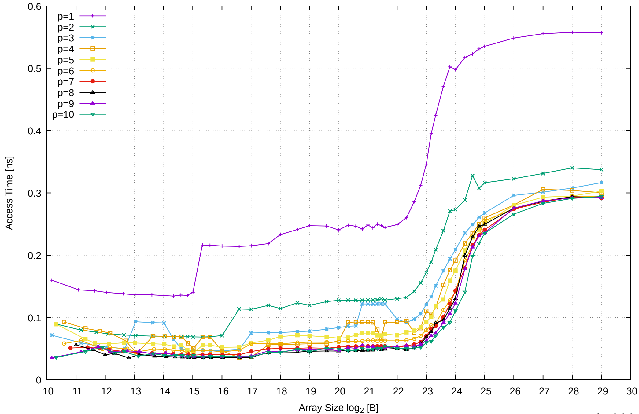
Intel Xeon E3-1260L v5 64GB - Parallel Memory Access Time - ScanRead64IndexUnrollLoop
