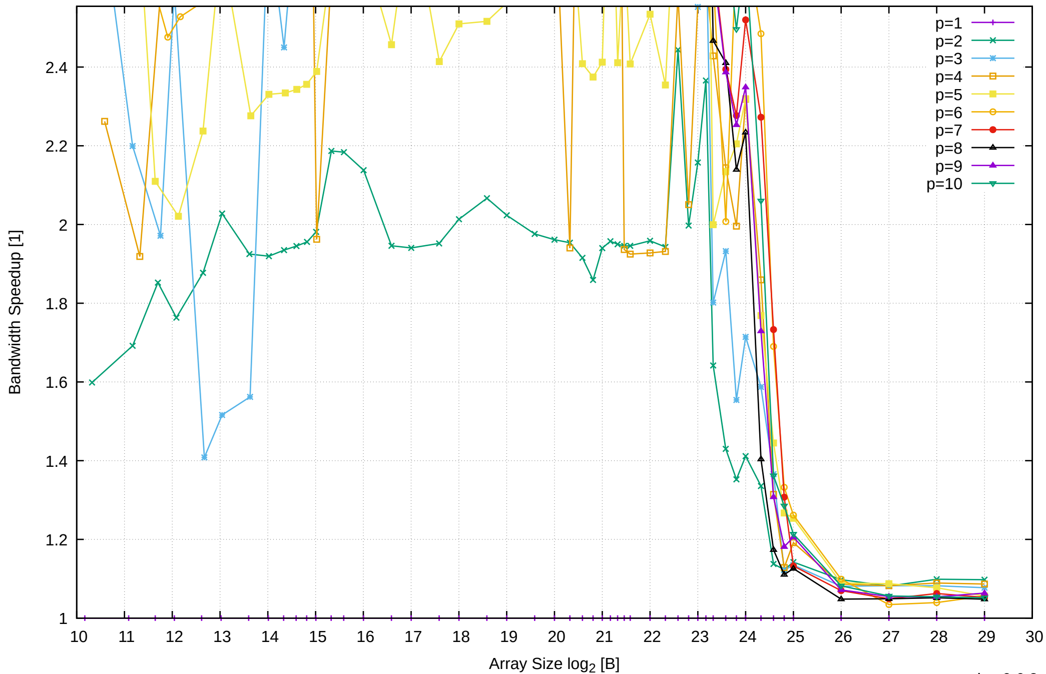
Intel Xeon E3-1260L v5 64GB - Speedup of Parallel Memory Bandwidth (enlarged) - ScanWrite64PtrSimpleLoop
