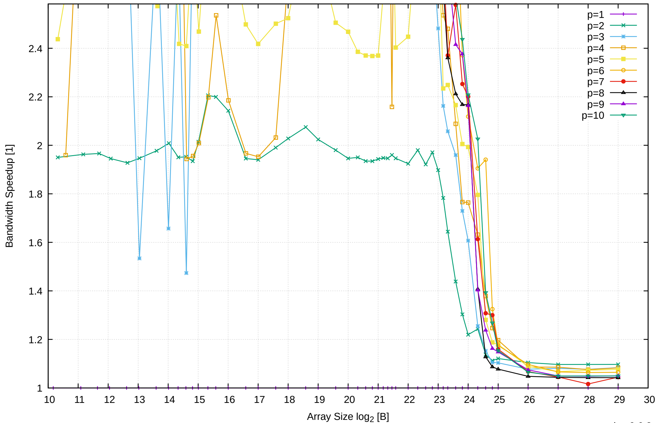
Intel Xeon E3-1260L v5 64GB - Speedup of Parallel Memory Bandwidth (enlarged) - ScanWrite64PtrUnrollLoop
