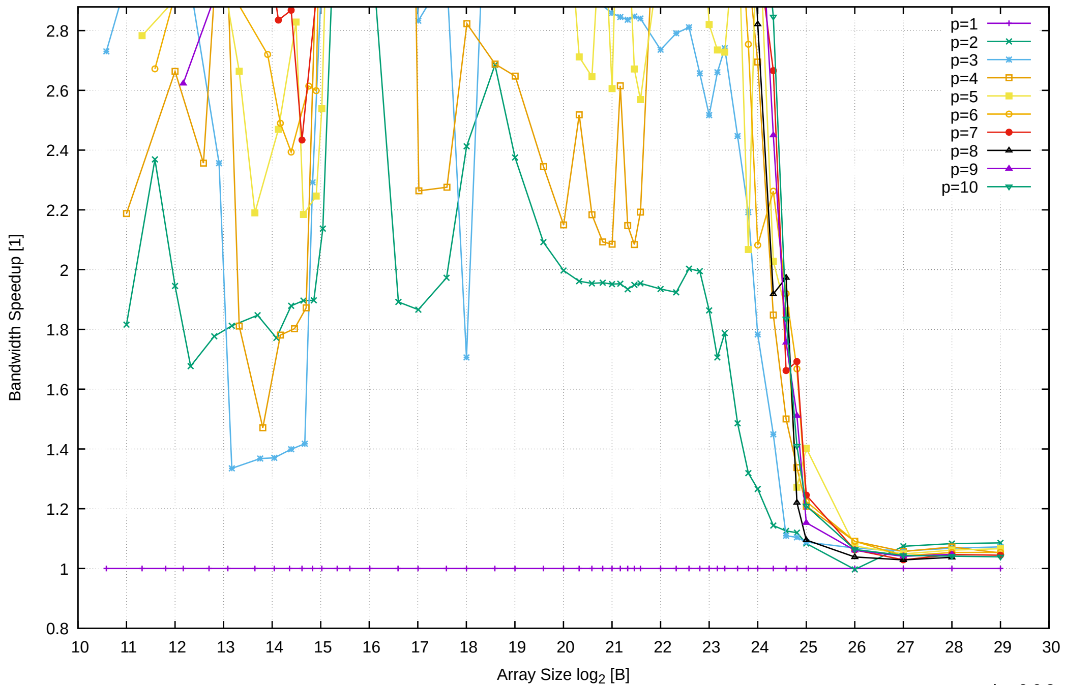
Intel Xeon E3-1260L v5 64GB - Speedup of Parallel Memory Bandwidth (enlarged) - ScanWrite256PtrSimpleLoop
