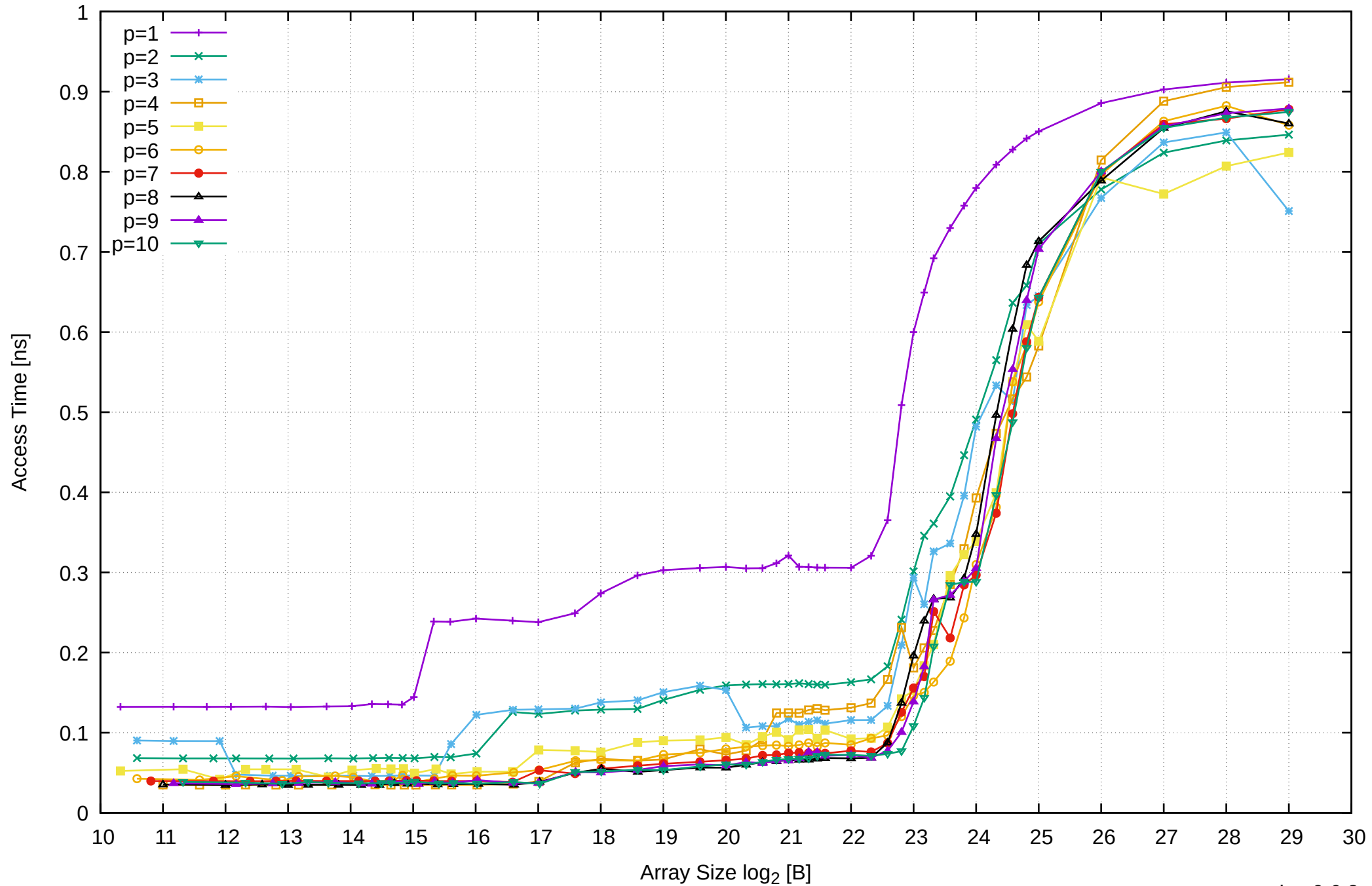
Intel Xeon E3-1260L v5 64GB - Parallel Memory Access Time - ScanRead128PtrUnrollLoop
