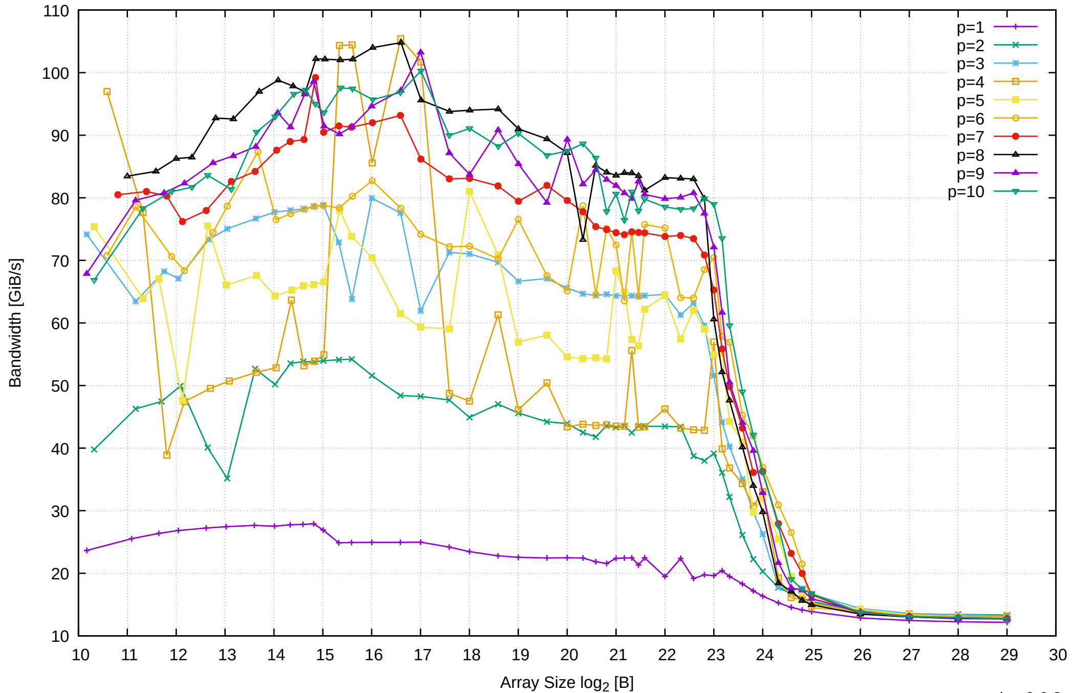
Intel Xeon E3-1260L v5 64GB - Parallel Memory Bandwidth - ScanWrite64IndexSimpleLoop
