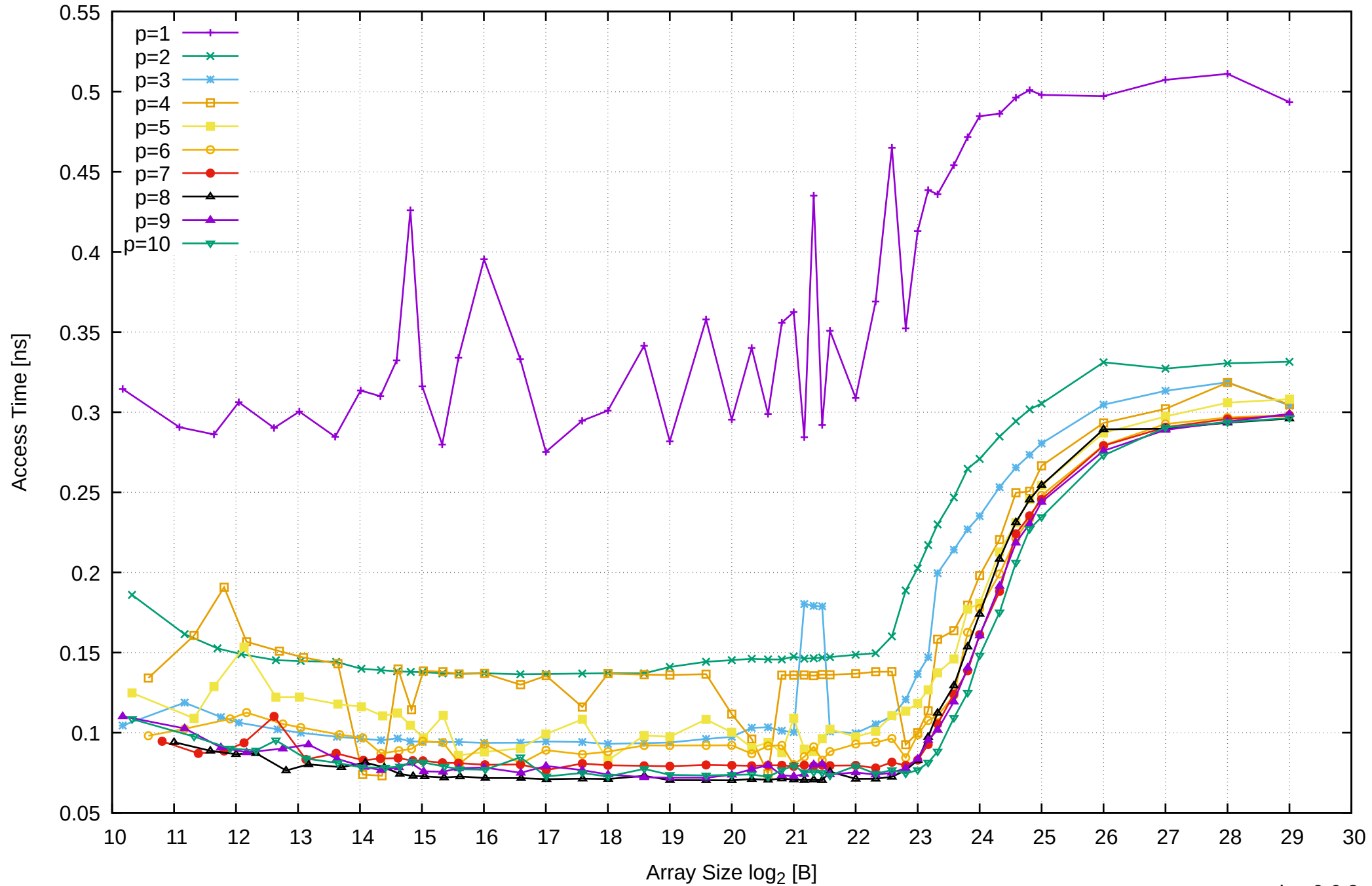
Intel Xeon E3-1260L v5 64GB - Parallel Memory Access Time - ScanRead64PtrSimpleLoop
