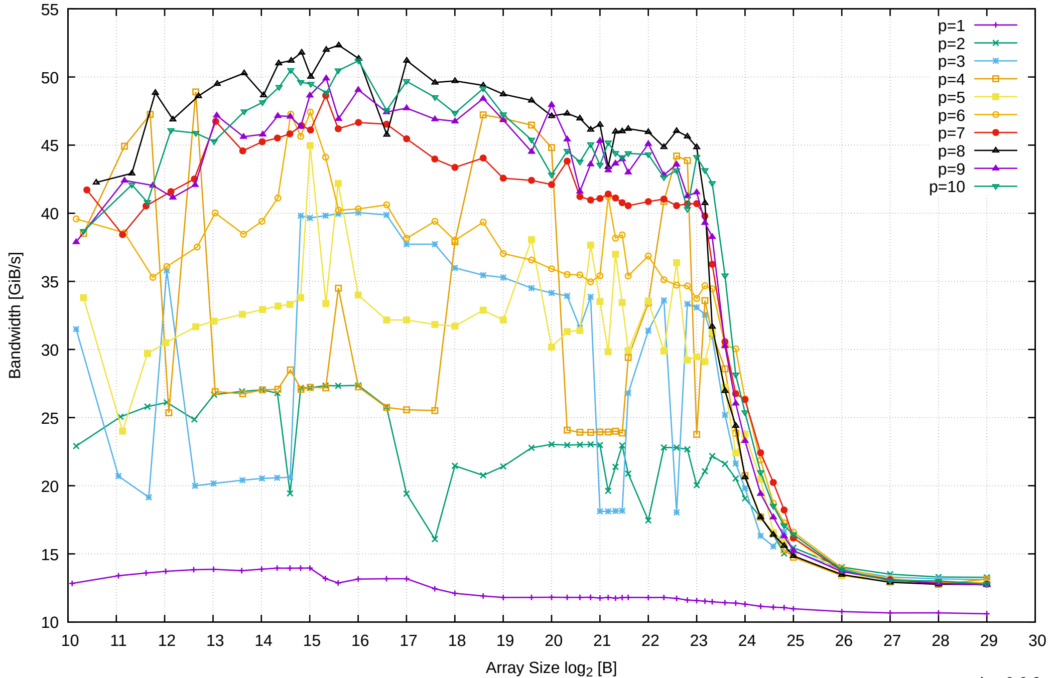
Intel Xeon E3-1260L v5 64GB - Parallel Memory Bandwidth - ScanWrite32PtrSimpleLoop
