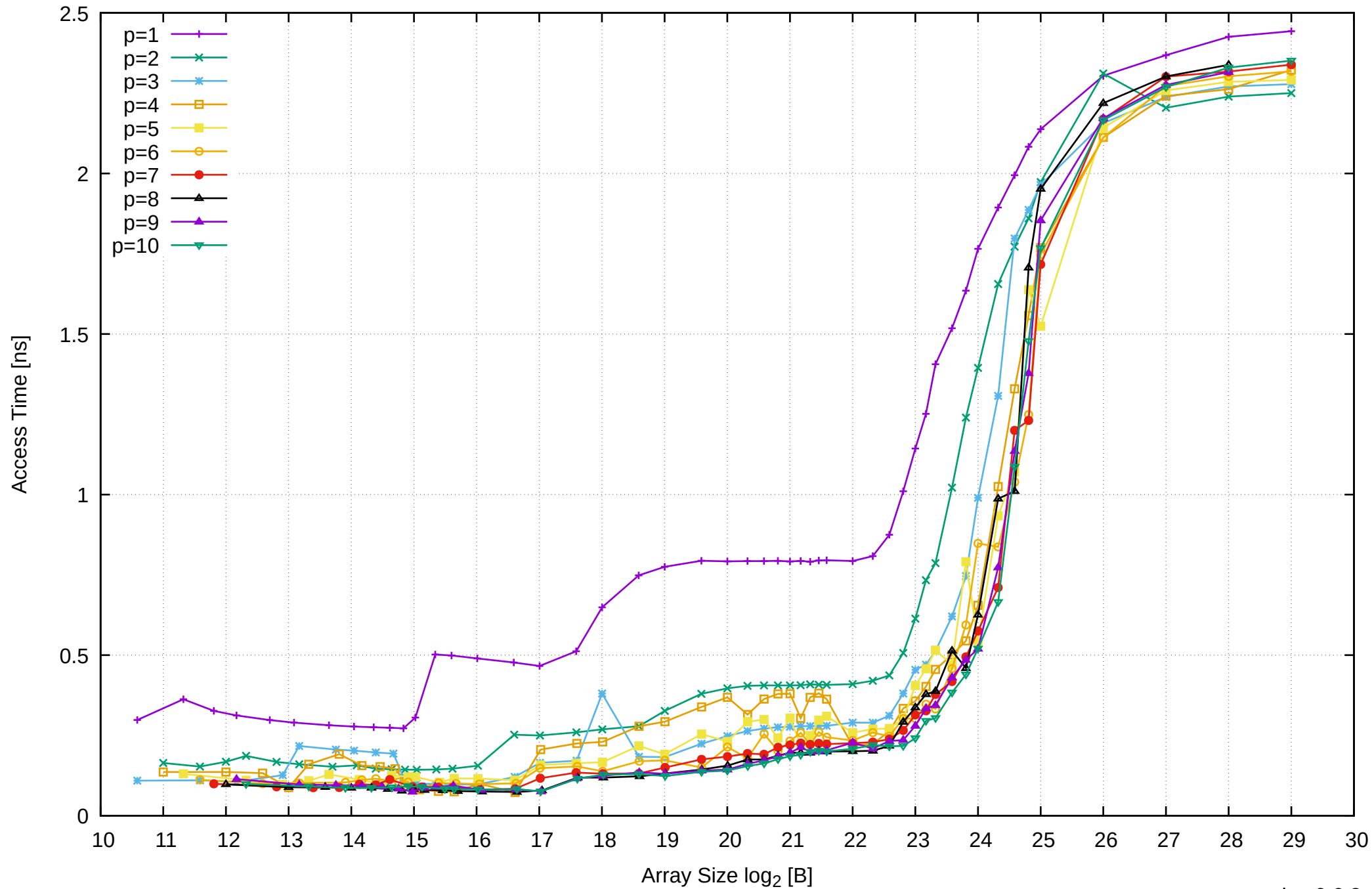
Intel Xeon E3-1260L v5 64GB - Parallel Memory Access Time - ScanWrite256PtrSimpleLoop
