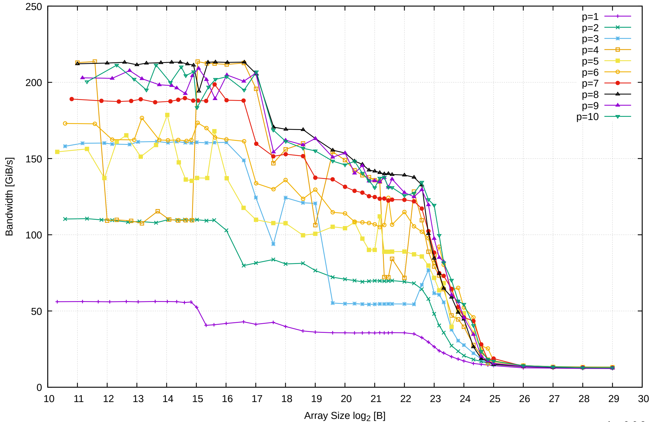
Intel Xeon E3-1260L v5 64GB - Parallel Memory Bandwidth - ScanWrite128PtrUnrollLoop
