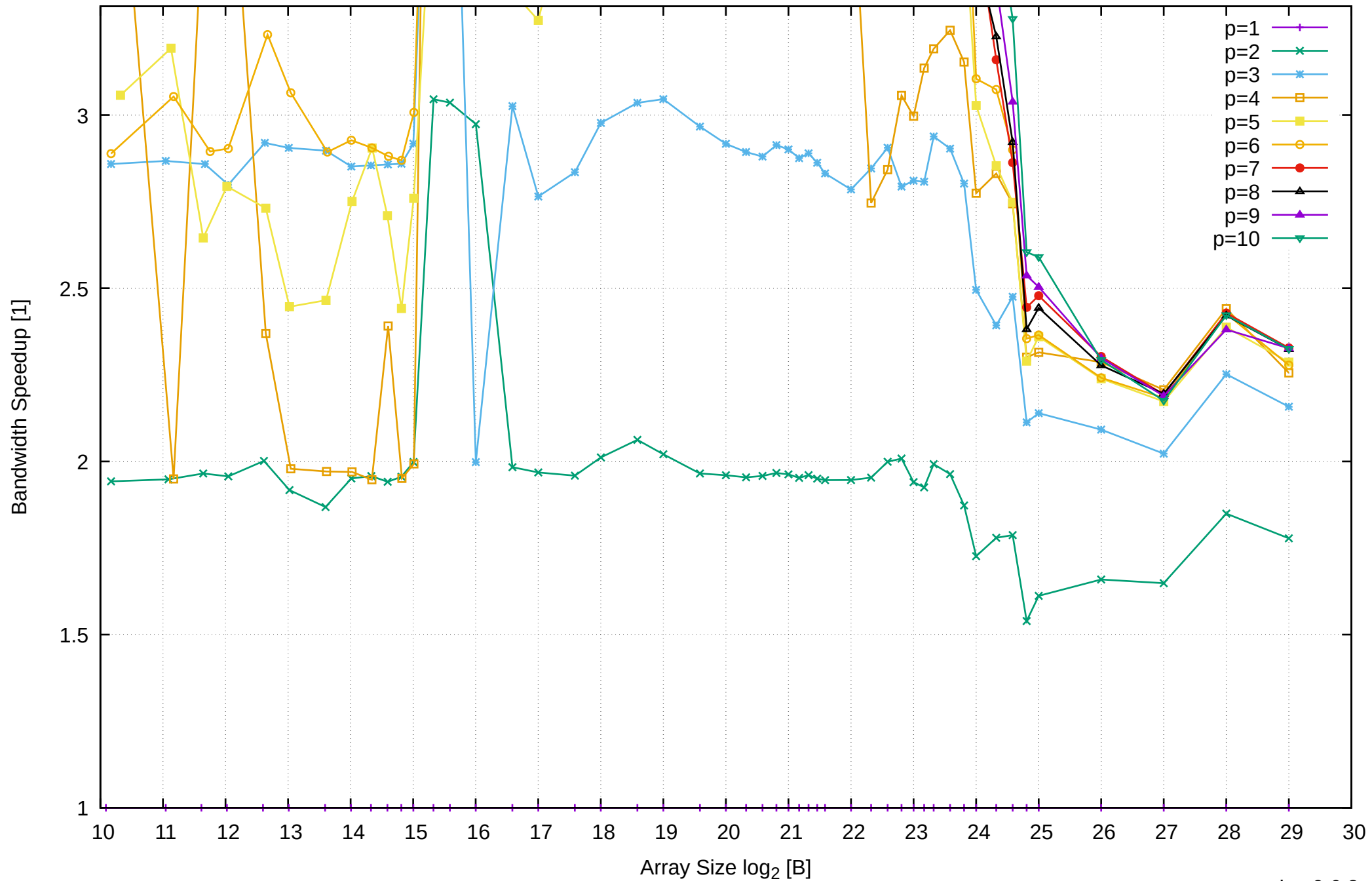
Intel Xeon E3-1260L v5 64GB - Speedup of Parallel Memory Bandwidth (enlarged) - ScanRead32PtrUnrollLoop
