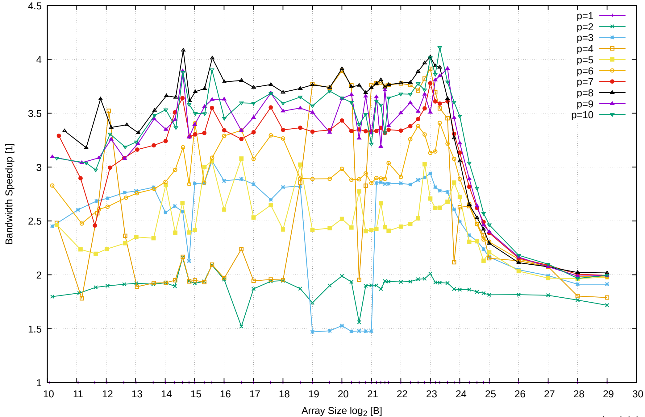
Intel Xeon E3-1260L v5 64GB - Speedup of Parallel Memory Bandwidth - ScanRead32PtrSimpleLoop
