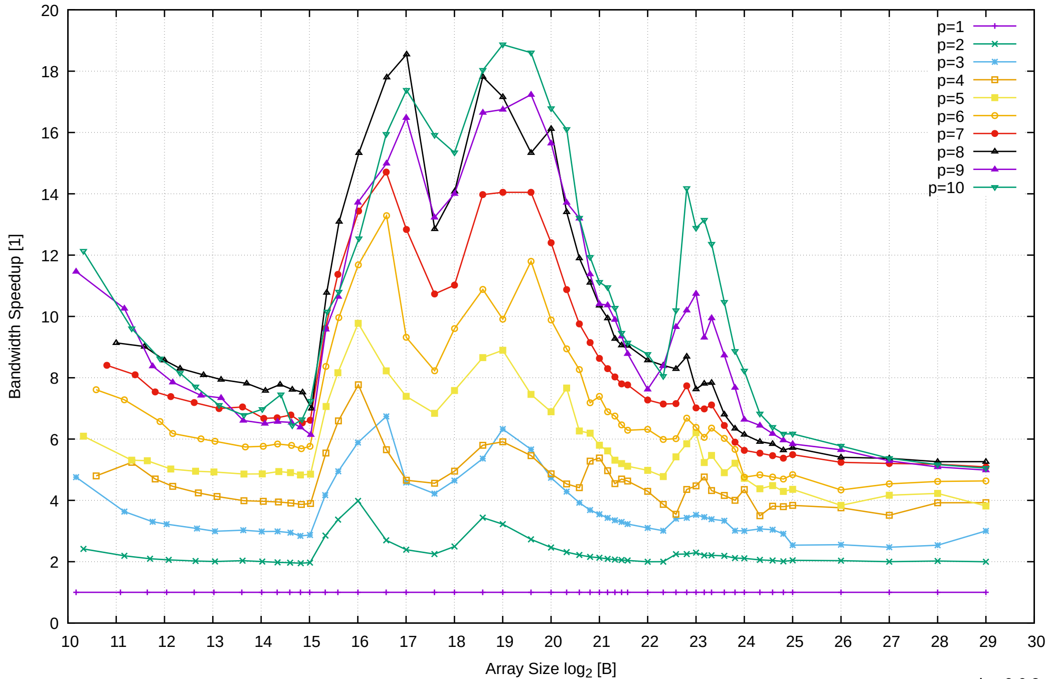
Intel Xeon E3-1260L v5 64GB - Speedup of Parallel Memory Bandwidth - PermRead64UnrollLoop
