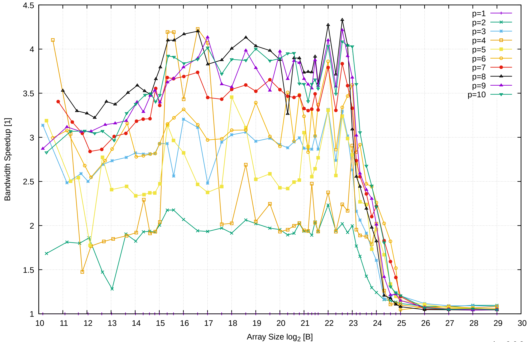
Intel Xeon E3-1260L v5 64GB - Speedup of Parallel Memory Bandwidth - ScanWrite64IndexSimpleLoop
