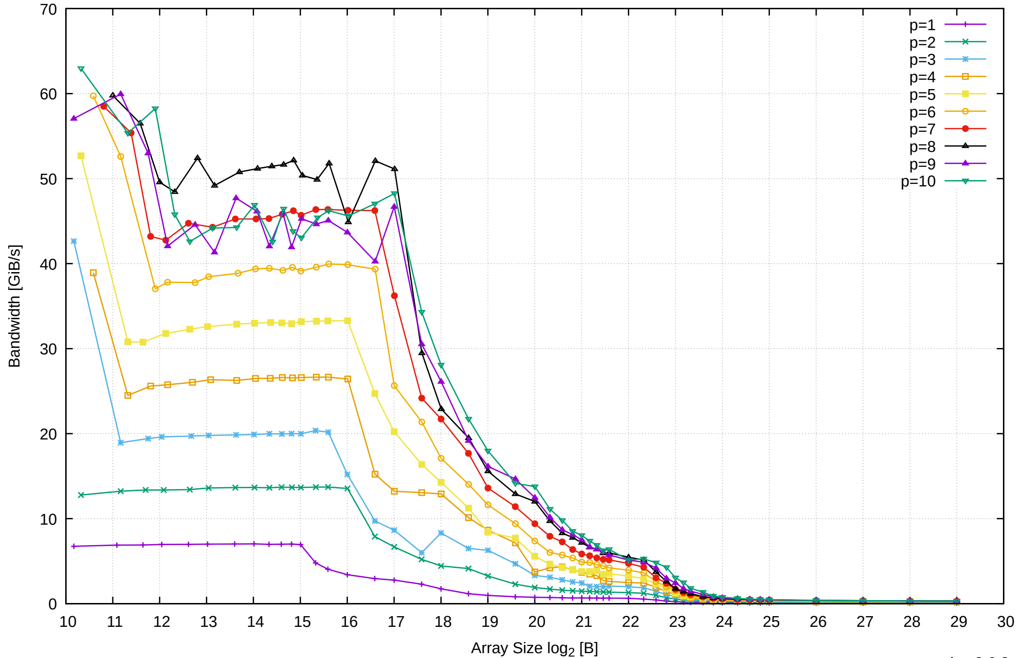
Intel Xeon E3-1260L v5 64GB - Parallel Memory Bandwidth - PermRead64SimpleLoop
