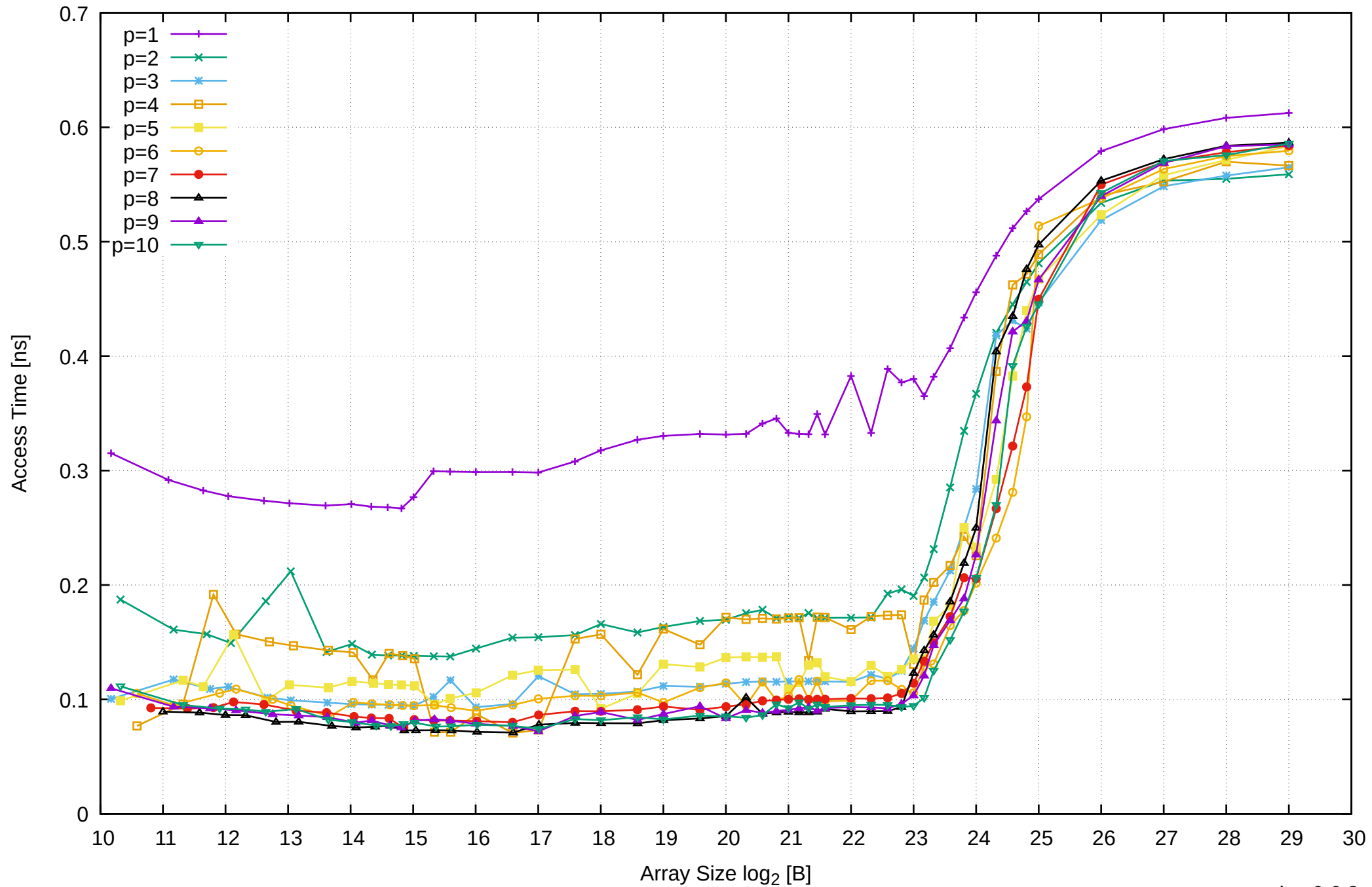
Intel Xeon E3-1260L v5 64GB - Parallel Memory Access Time - ScanWrite64IndexSimpleLoop
