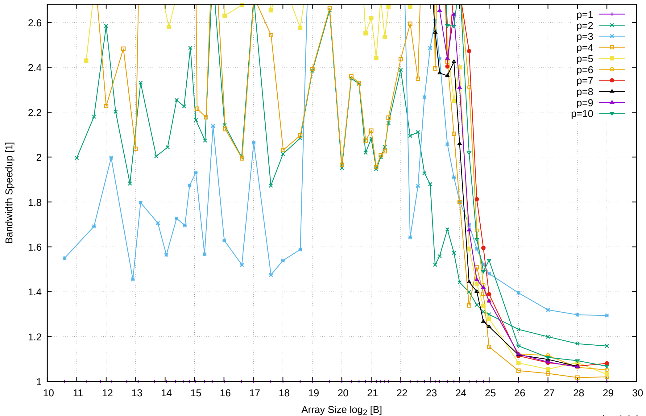
Intel Xeon E3-1260L v5 64GB - Speedup of Parallel Memory Bandwidth (enlarged) - ScanRead256PtrSimpleLoop
