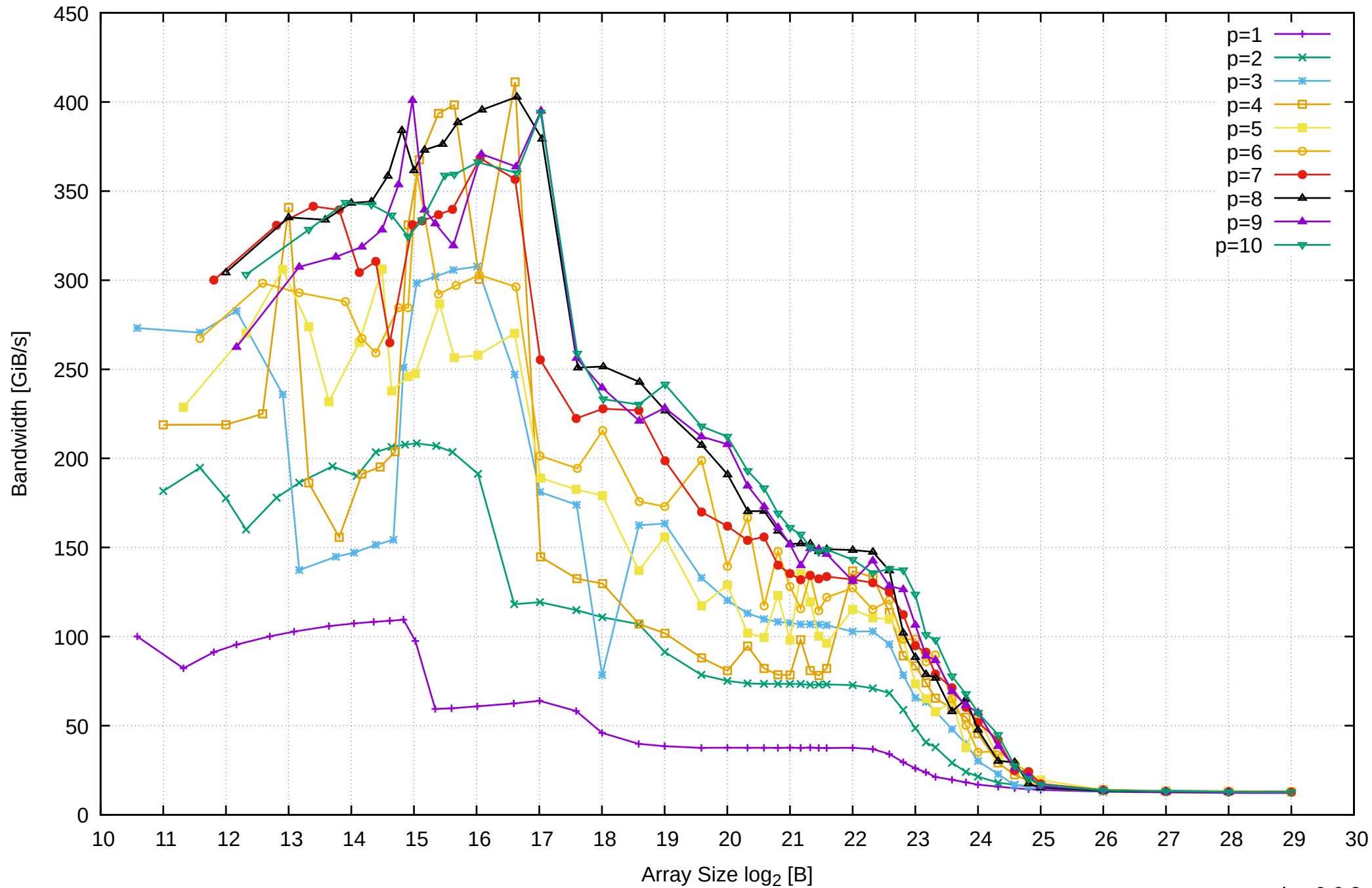
Intel Xeon E3-1260L v5 64GB - Parallel Memory Bandwidth - ScanWrite256PtrSimpleLoop
