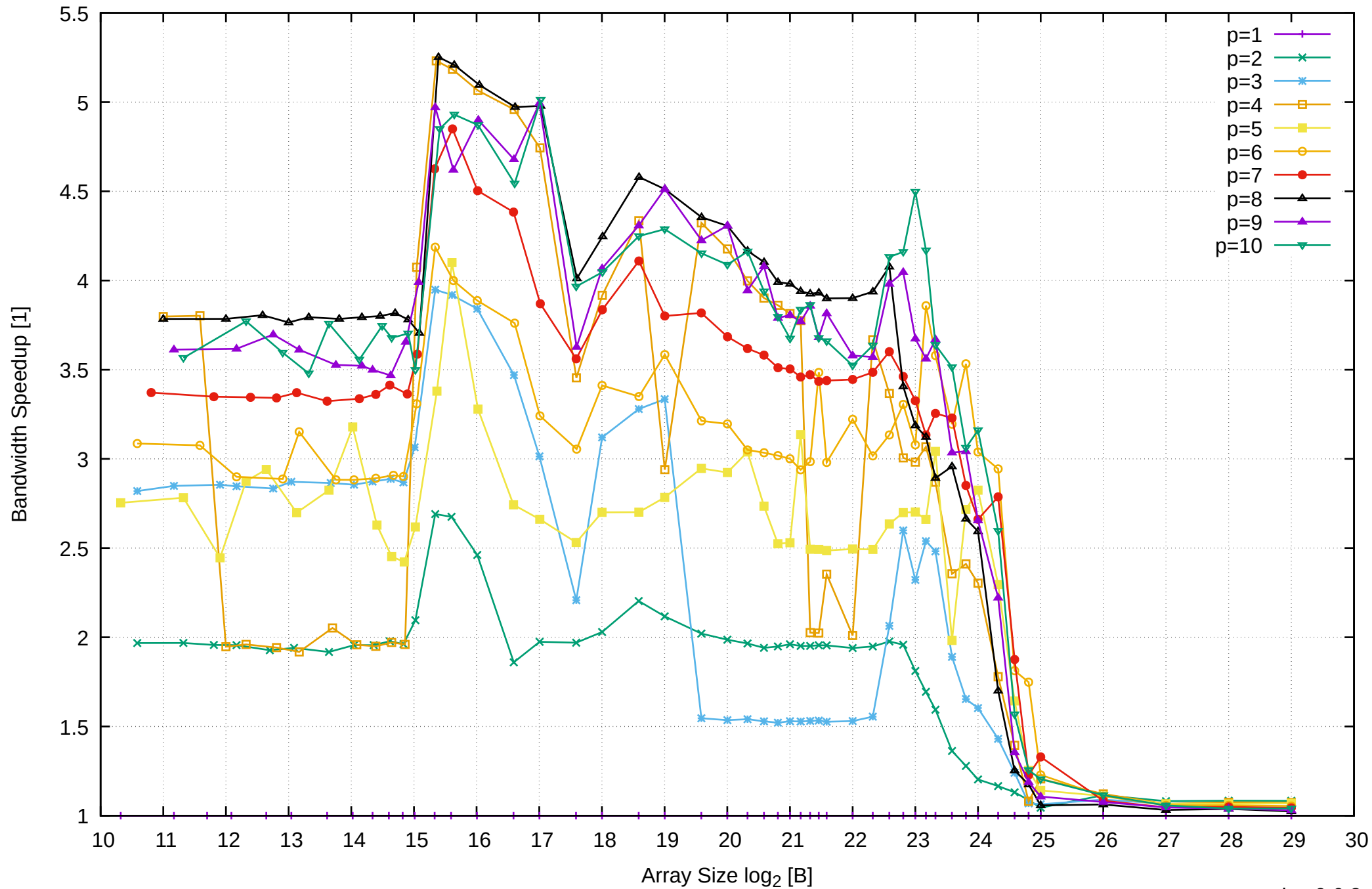
Intel Xeon E3-1260L v5 64GB - Speedup of Parallel Memory Bandwidth - ScanWrite128PtrUnrollLoop
