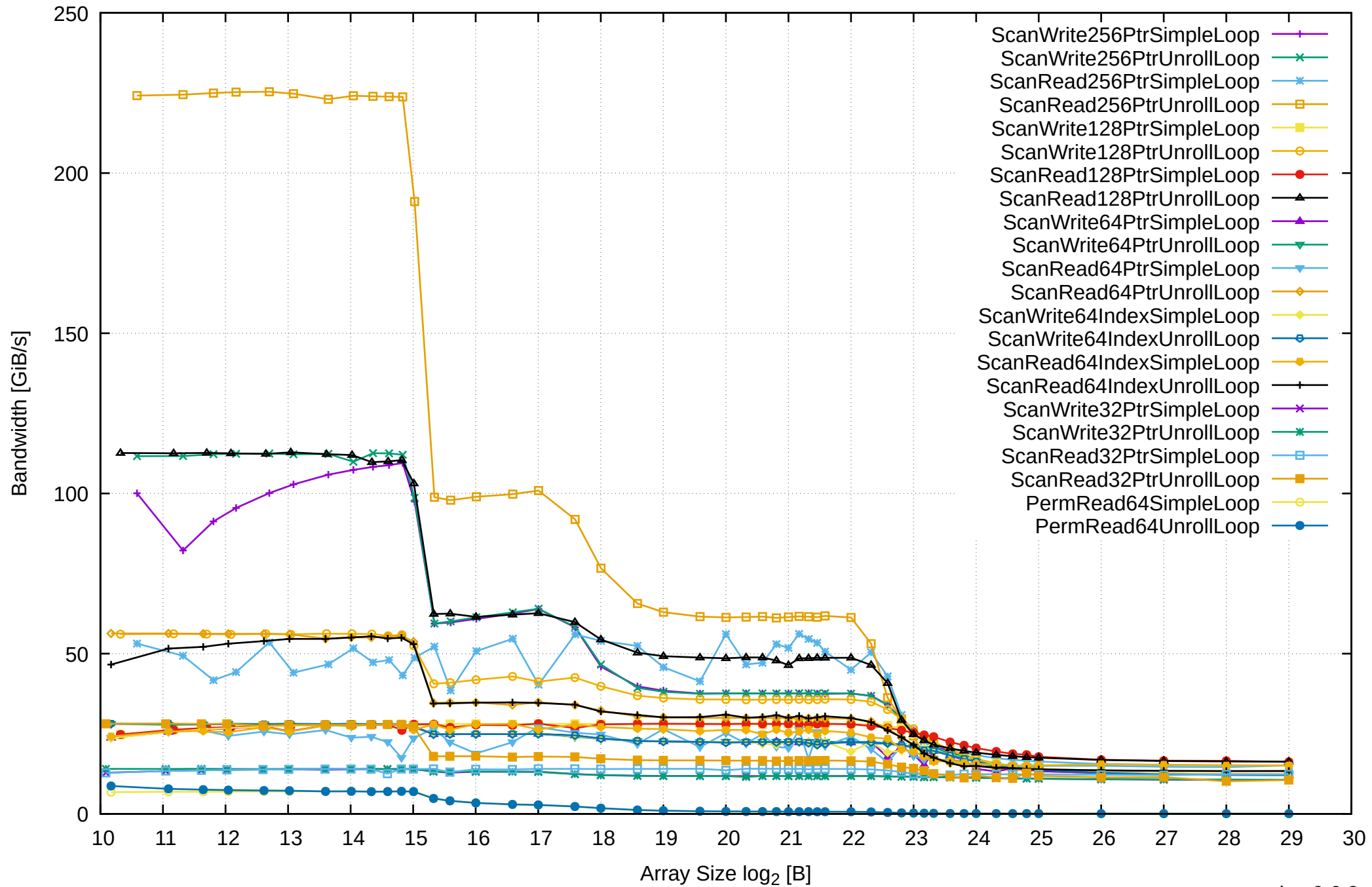
Intel Xeon E3-1260L v5 64GB - One Thread Memory Bandwidth
