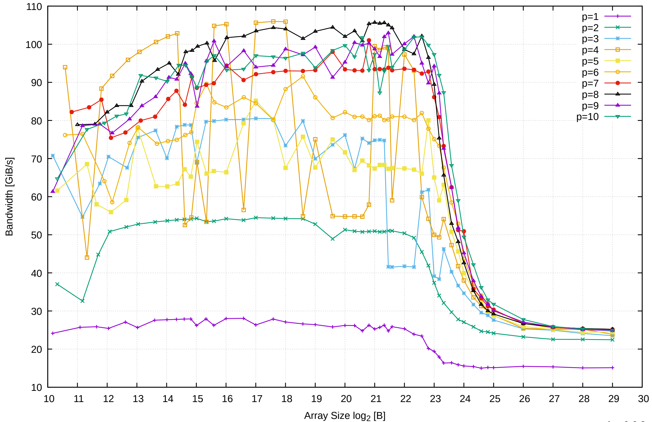
Intel Xeon E3-1260L v5 64GB - Parallel Memory Bandwidth - ScanRead64IndexSimpleLoop
