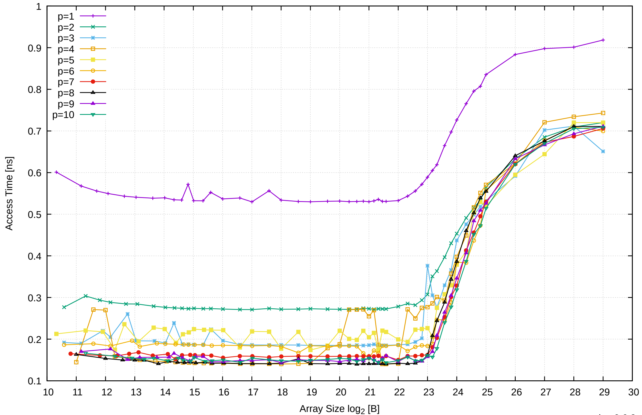
Intel Xeon E3-1260L v5 64GB - Parallel Memory Access Time - ScanRead128PtrSimpleLoop
