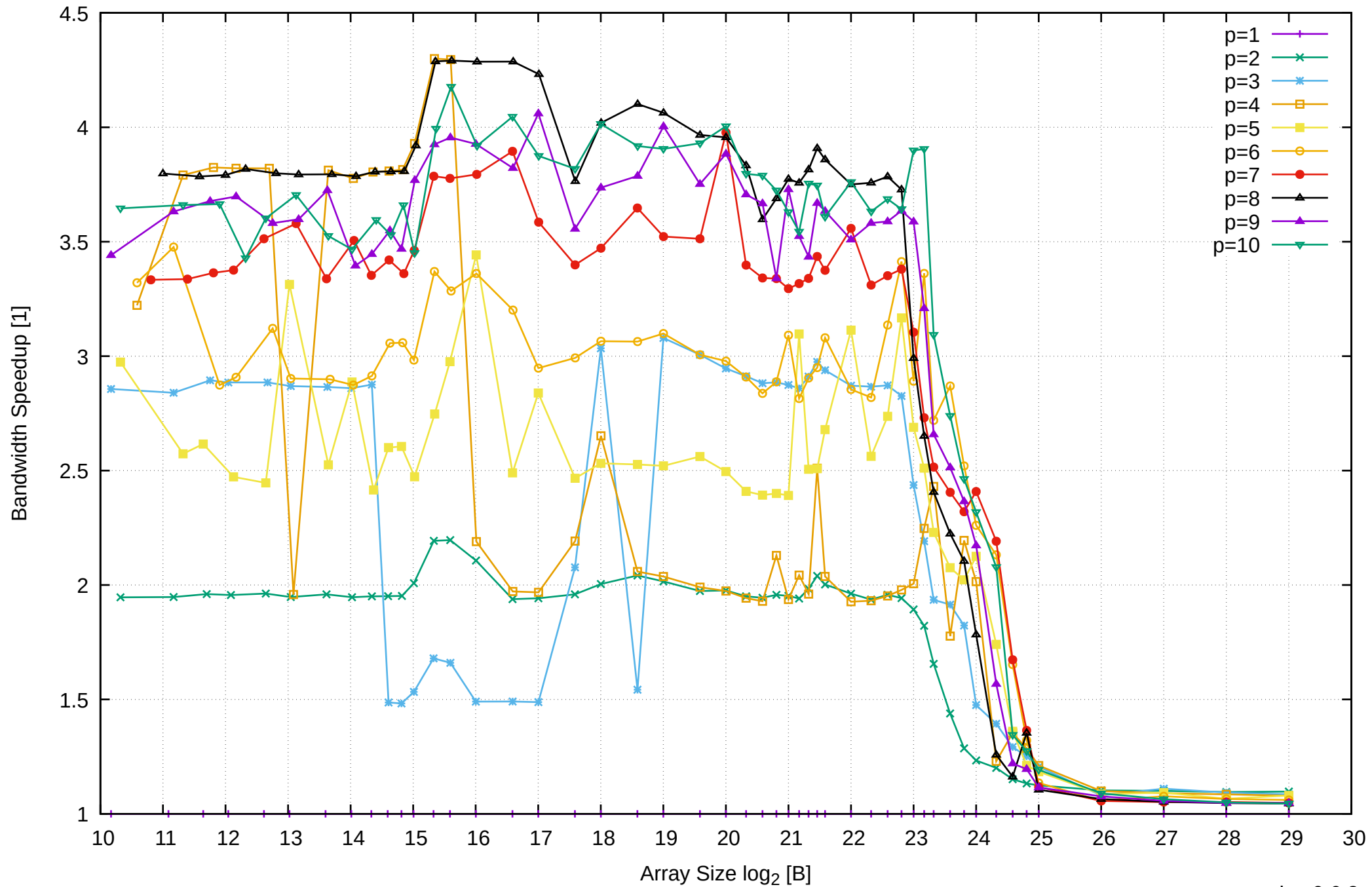
Intel Xeon E3-1260L v5 64GB - Speedup of Parallel Memory Bandwidth - ScanWrite64IndexUnrollLoop
