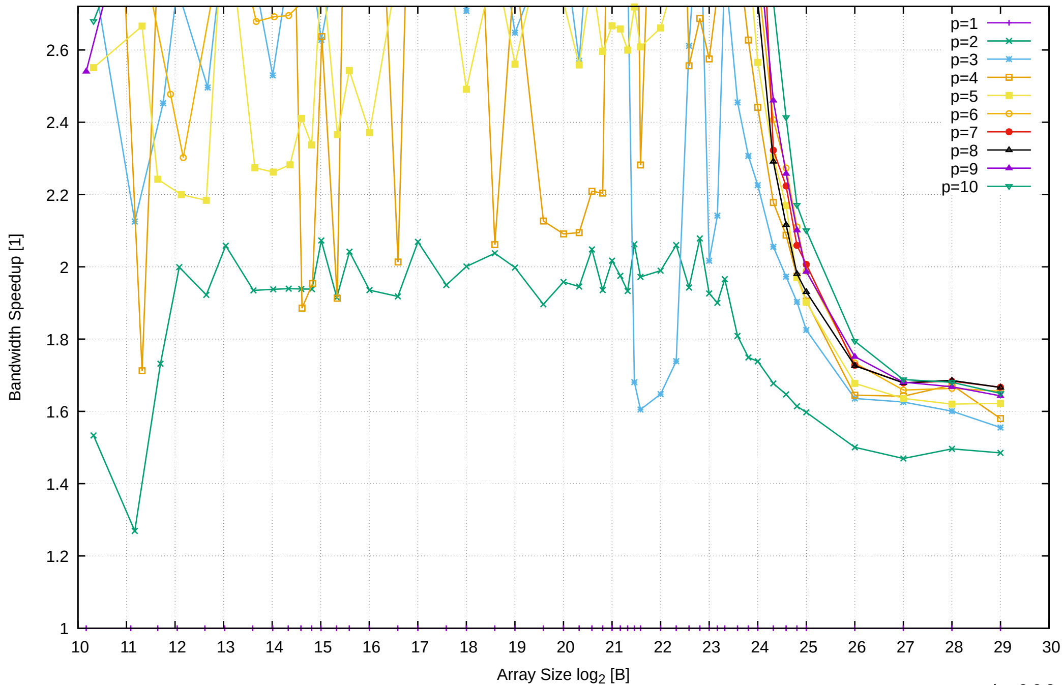
Intel Xeon E3-1260L v5 64GB - Speedup of Parallel Memory Bandwidth (enlarged) - ScanRead64IndexSimpleLoop
