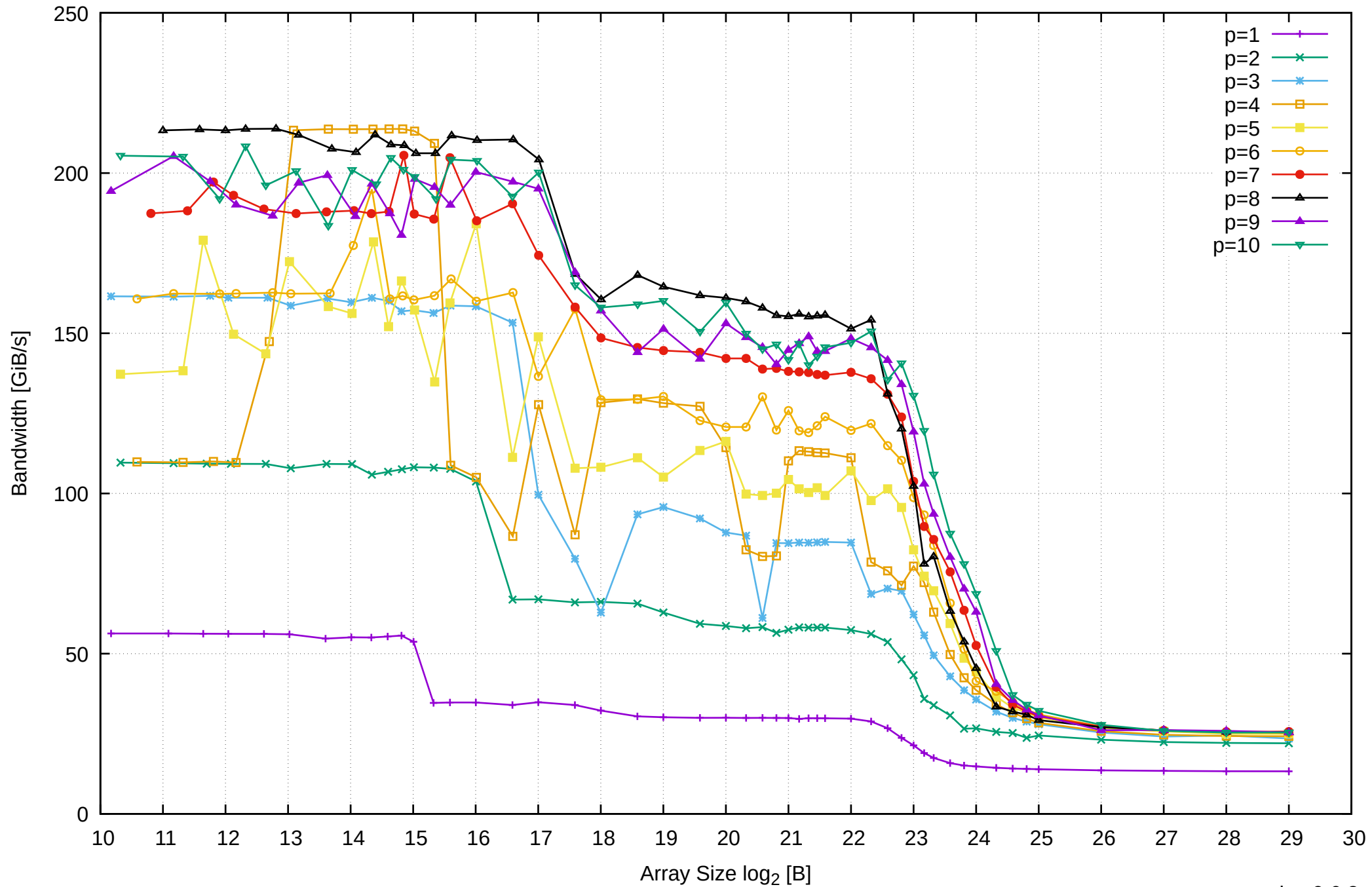
Intel Xeon E3-1260L v5 64GB - Parallel Memory Bandwidth - ScanRead64PtrUnrollLoop
