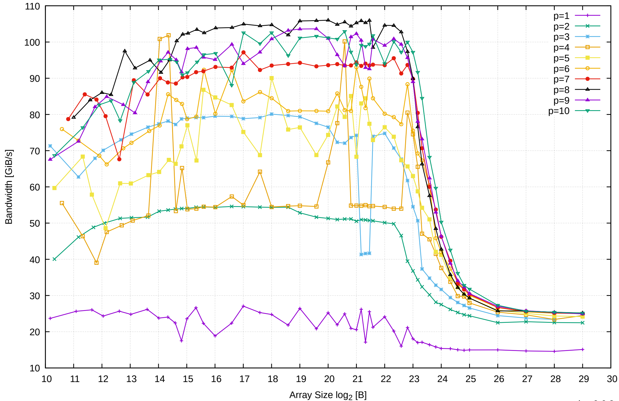
Intel Xeon E3-1260L v5 64GB - Parallel Memory Bandwidth - ScanRead64PtrSimpleLoop
