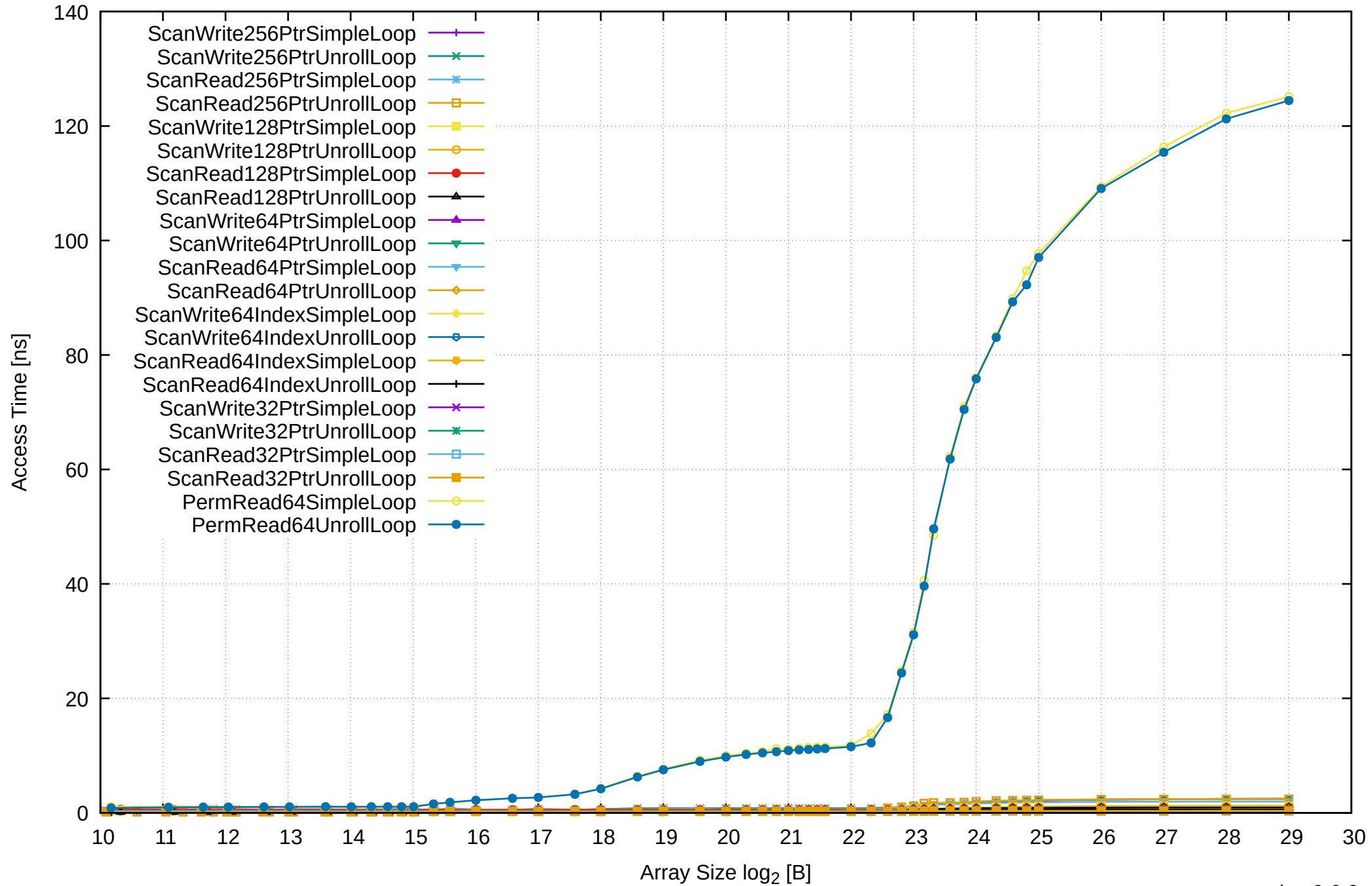
Intel Xeon E3-1260L v5 64GB - One Thread Memory Latency (Access Time)
