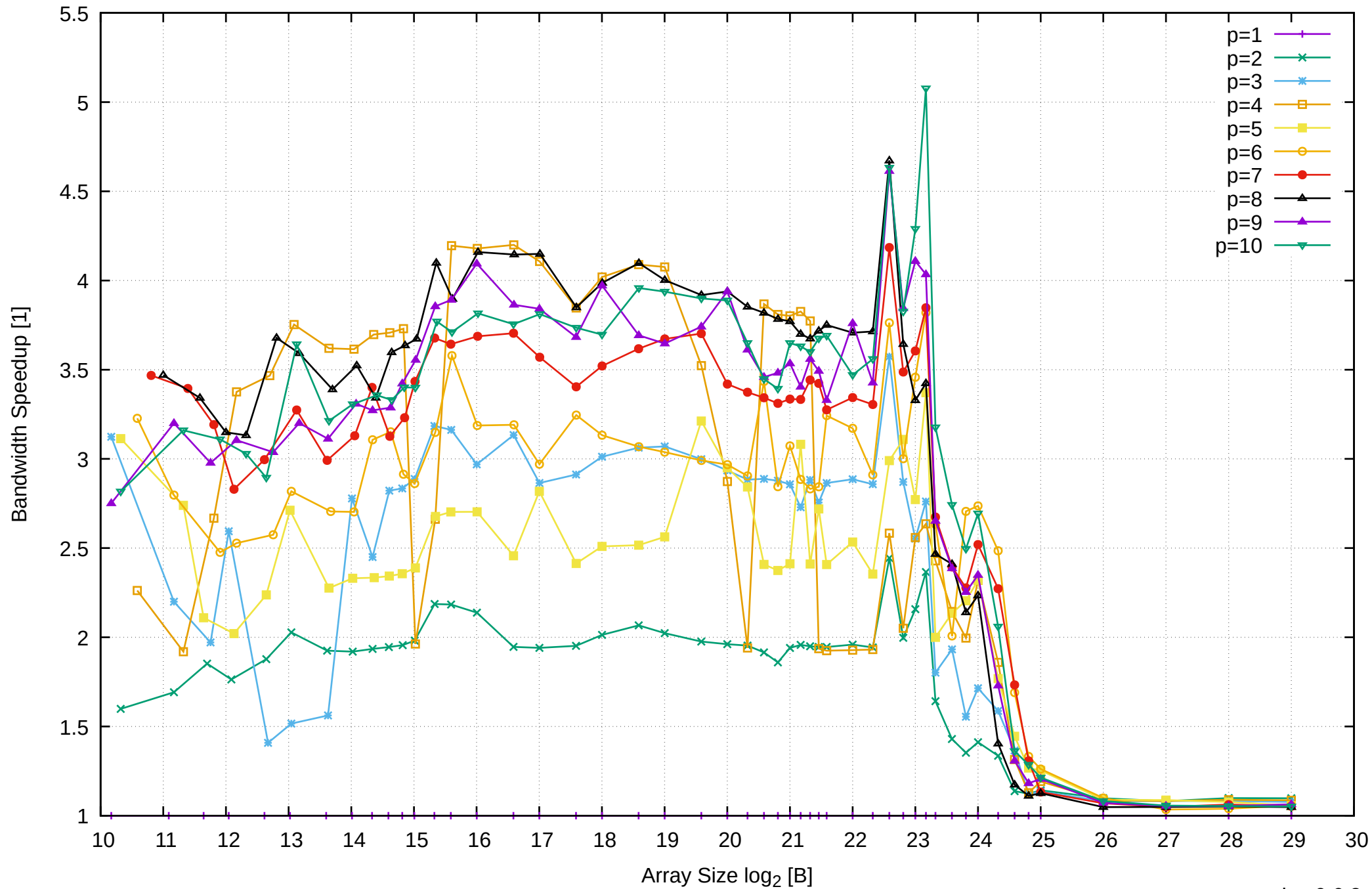
Intel Xeon E3-1260L v5 64GB - Speedup of Parallel Memory Bandwidth - ScanWrite64PtrSimpleLoop
