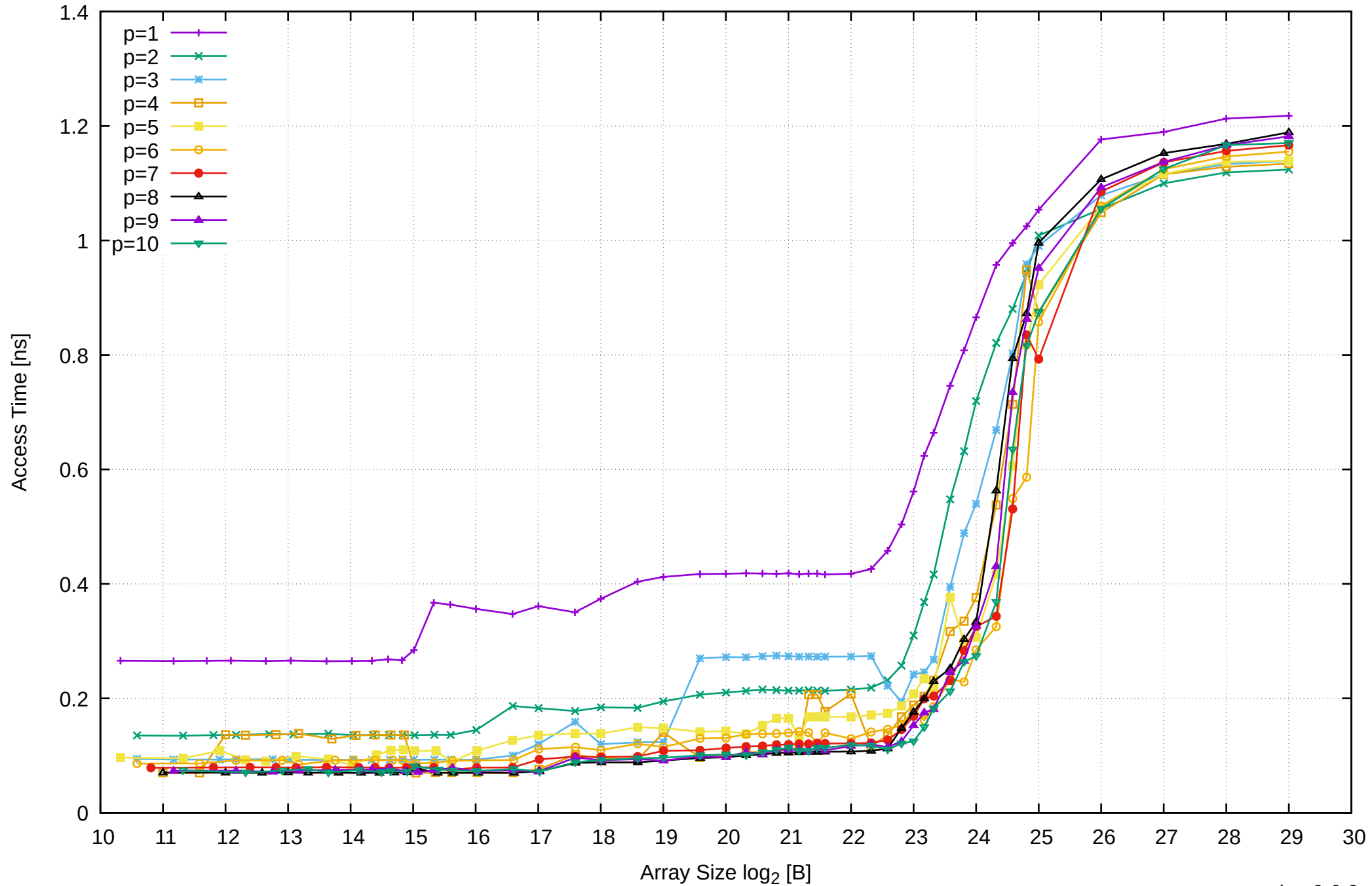
Intel Xeon E3-1260L v5 64GB - Parallel Memory Access Time - ScanWrite128PtrUnrollLoop
