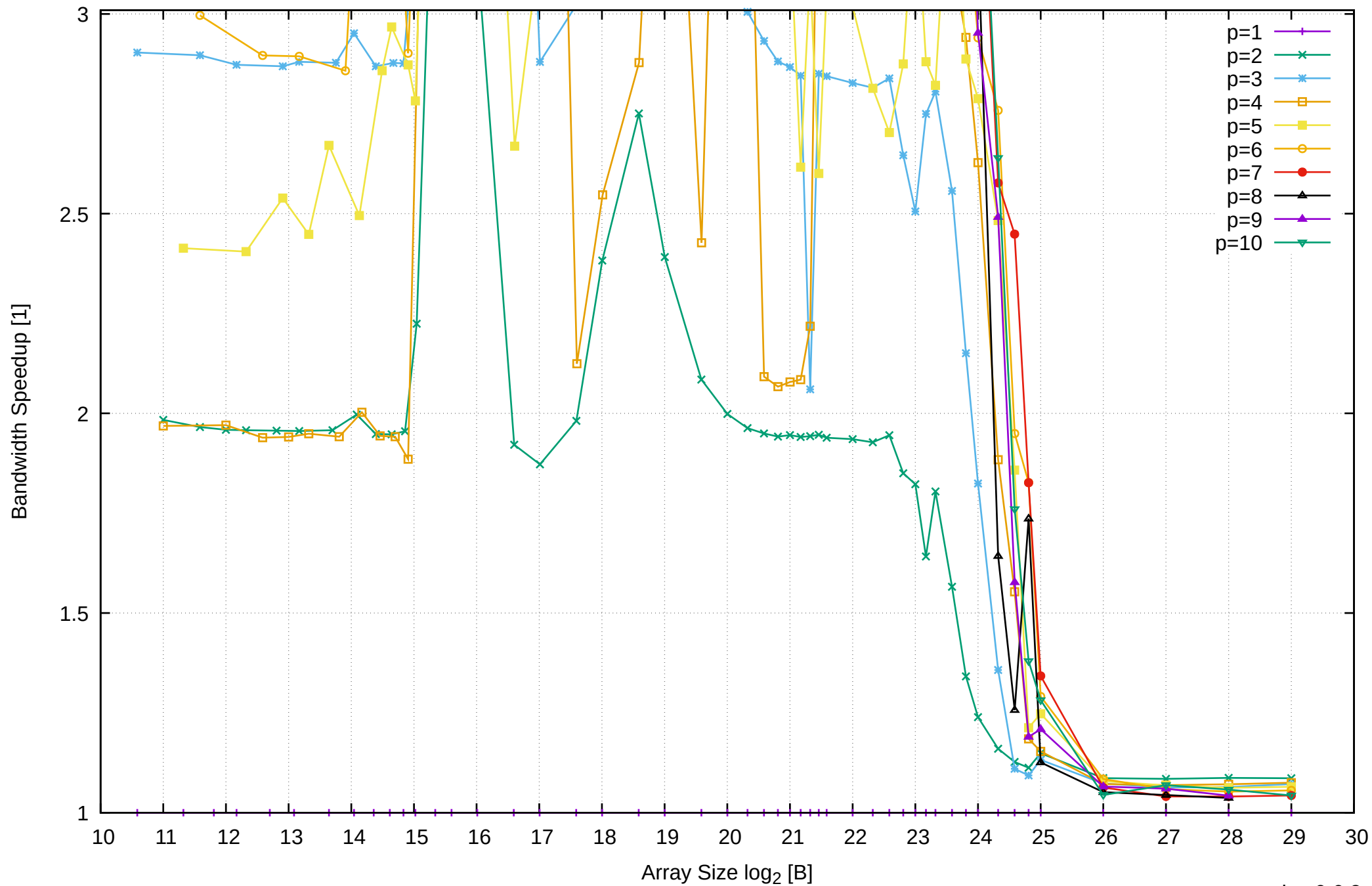
Intel Xeon E3-1260L v5 64GB - Speedup of Parallel Memory Bandwidth (enlarged) - ScanWrite256PtrUnrollLoop
