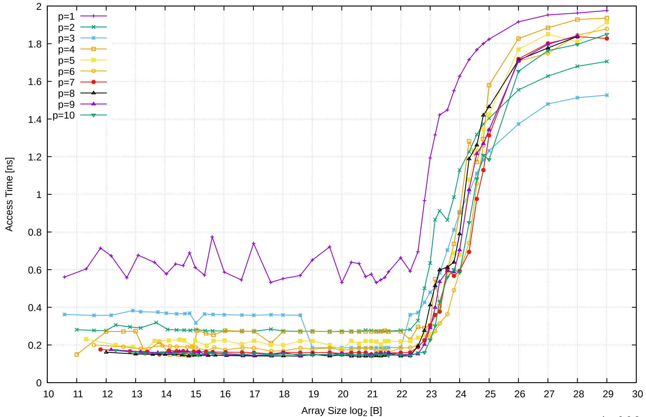
Intel Xeon E3-1260L v5 64GB - Parallel Memory Access Time - ScanRead256PtrSimpleLoop
