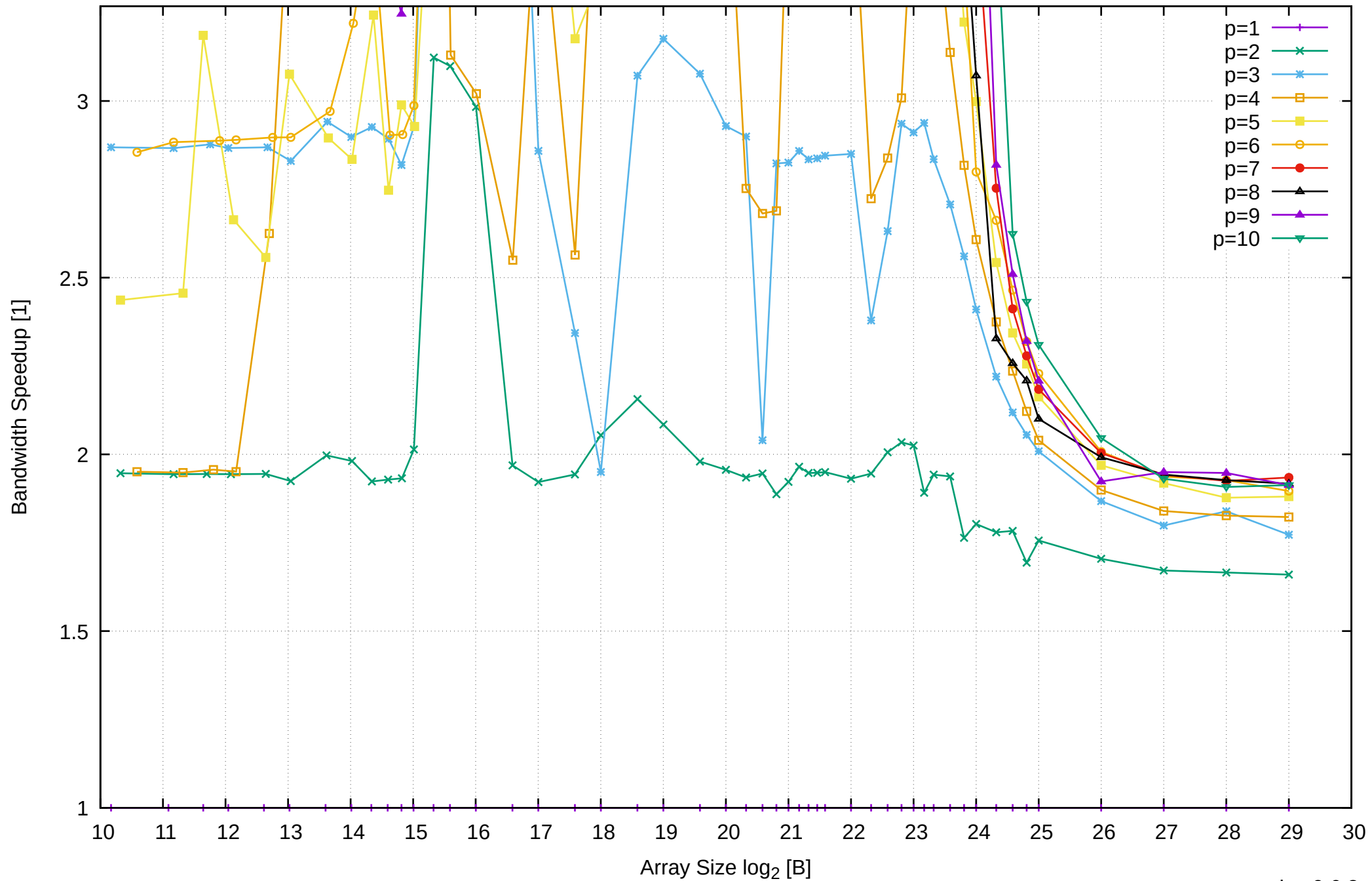
Intel Xeon E3-1260L v5 64GB - Speedup of Parallel Memory Bandwidth (enlarged) - ScanRead64PtrUnrollLoop
