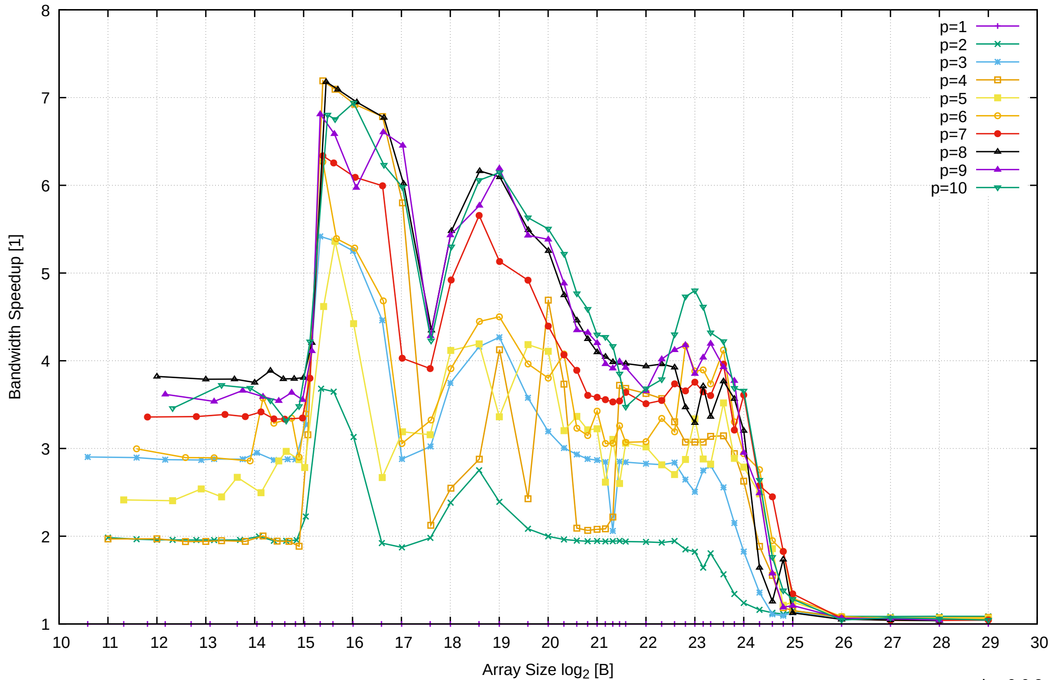
Intel Xeon E3-1260L v5 64GB - Speedup of Parallel Memory Bandwidth - ScanWrite256PtrUnrollLoop
