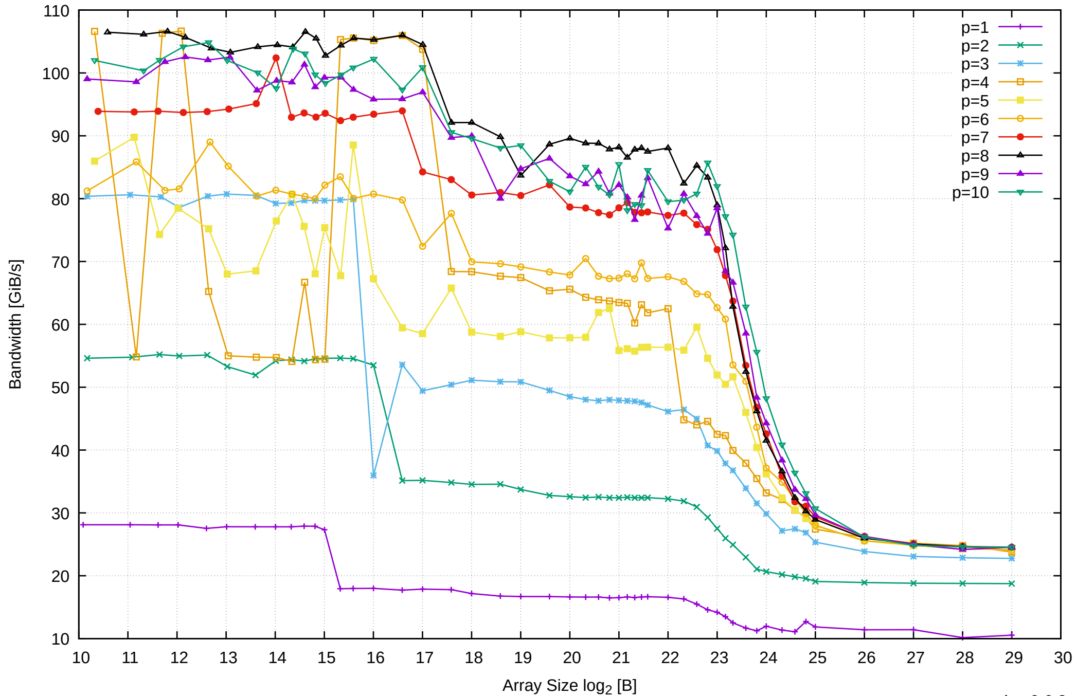
Intel Xeon E3-1260L v5 64GB - Parallel Memory Bandwidth - ScanRead32PtrUnrollLoop
