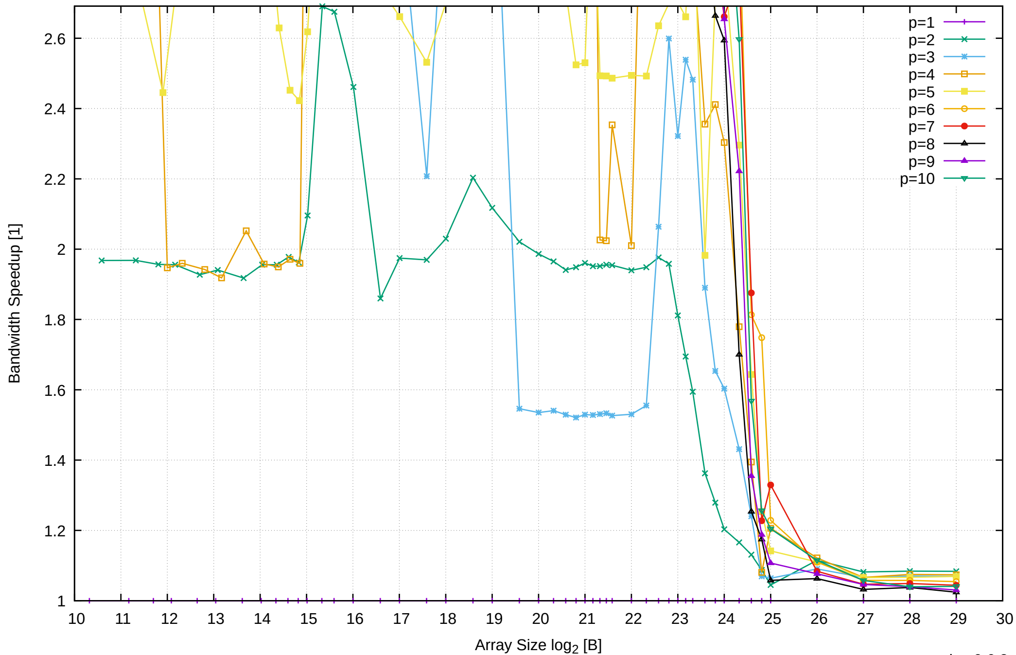
Intel Xeon E3-1260L v5 64GB - Speedup of Parallel Memory Bandwidth (enlarged) - ScanWrite128PtrUnrollLoop
