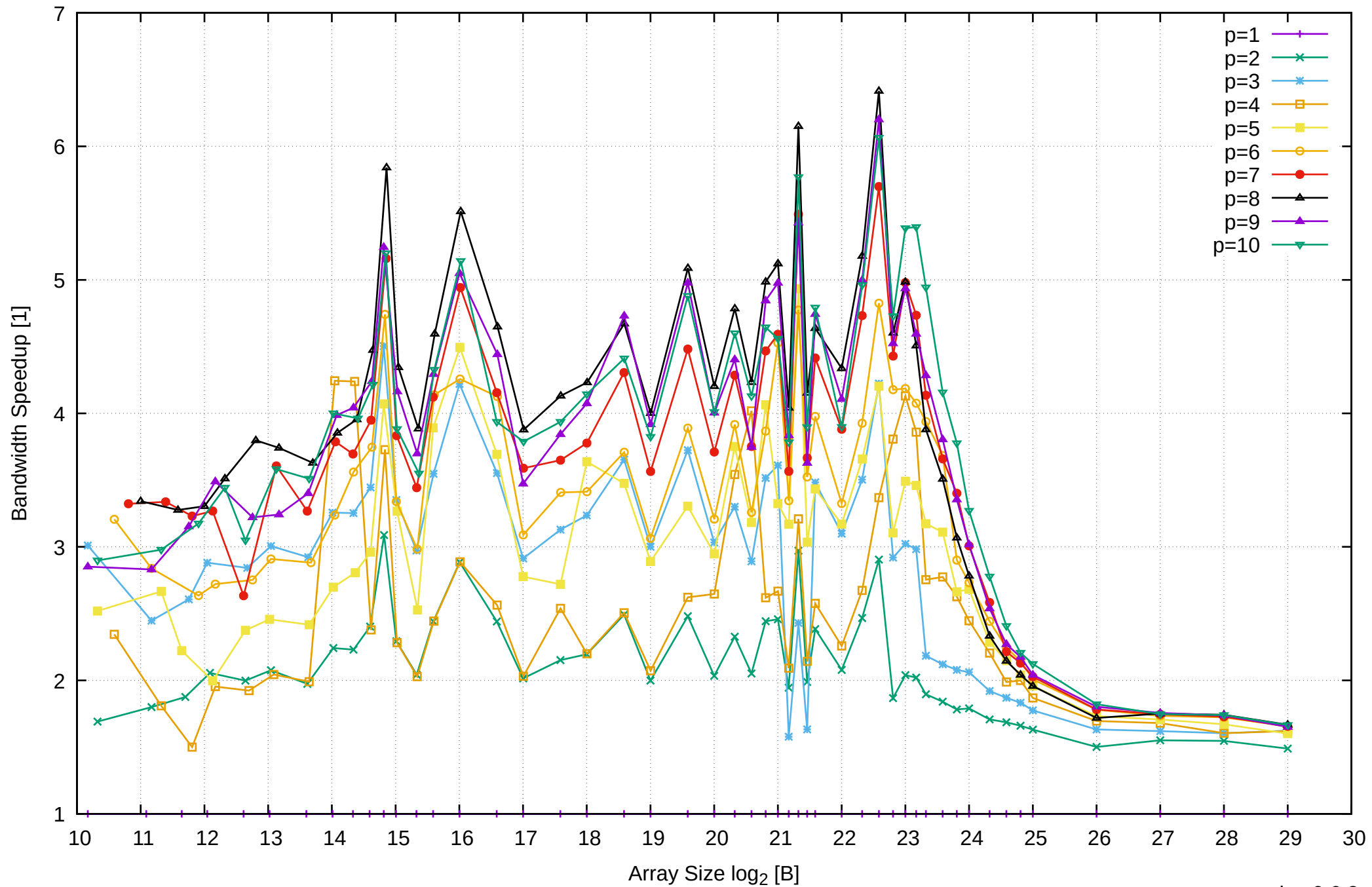
Intel Xeon E3-1260L v5 64GB - Speedup of Parallel Memory Bandwidth - ScanRead64PtrSimpleLoop
