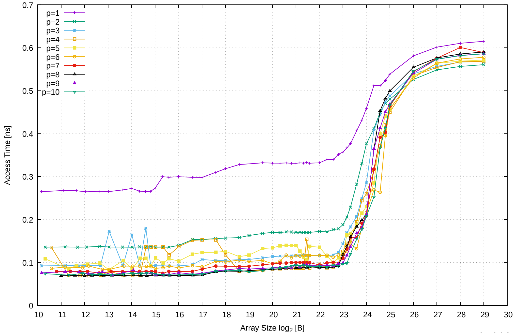
Intel Xeon E3-1260L v5 64GB - Parallel Memory Access Time - ScanWrite64PtrUnrollLoop
