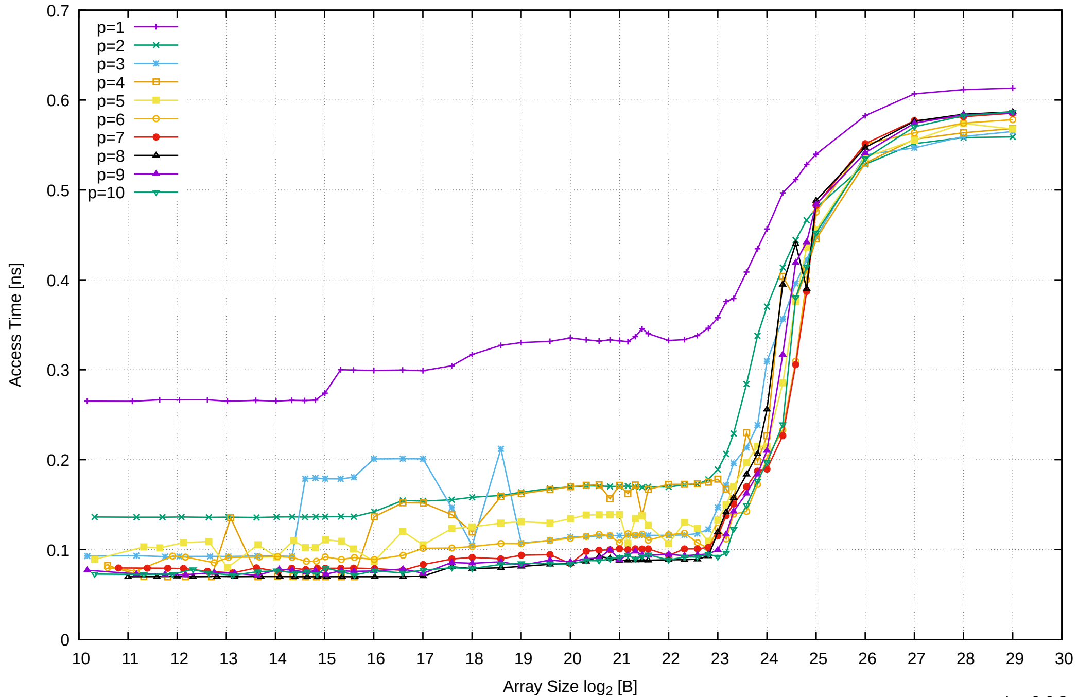
Intel Xeon E3-1260L v5 64GB - Parallel Memory Access Time - ScanWrite64IndexUnrollLoop
