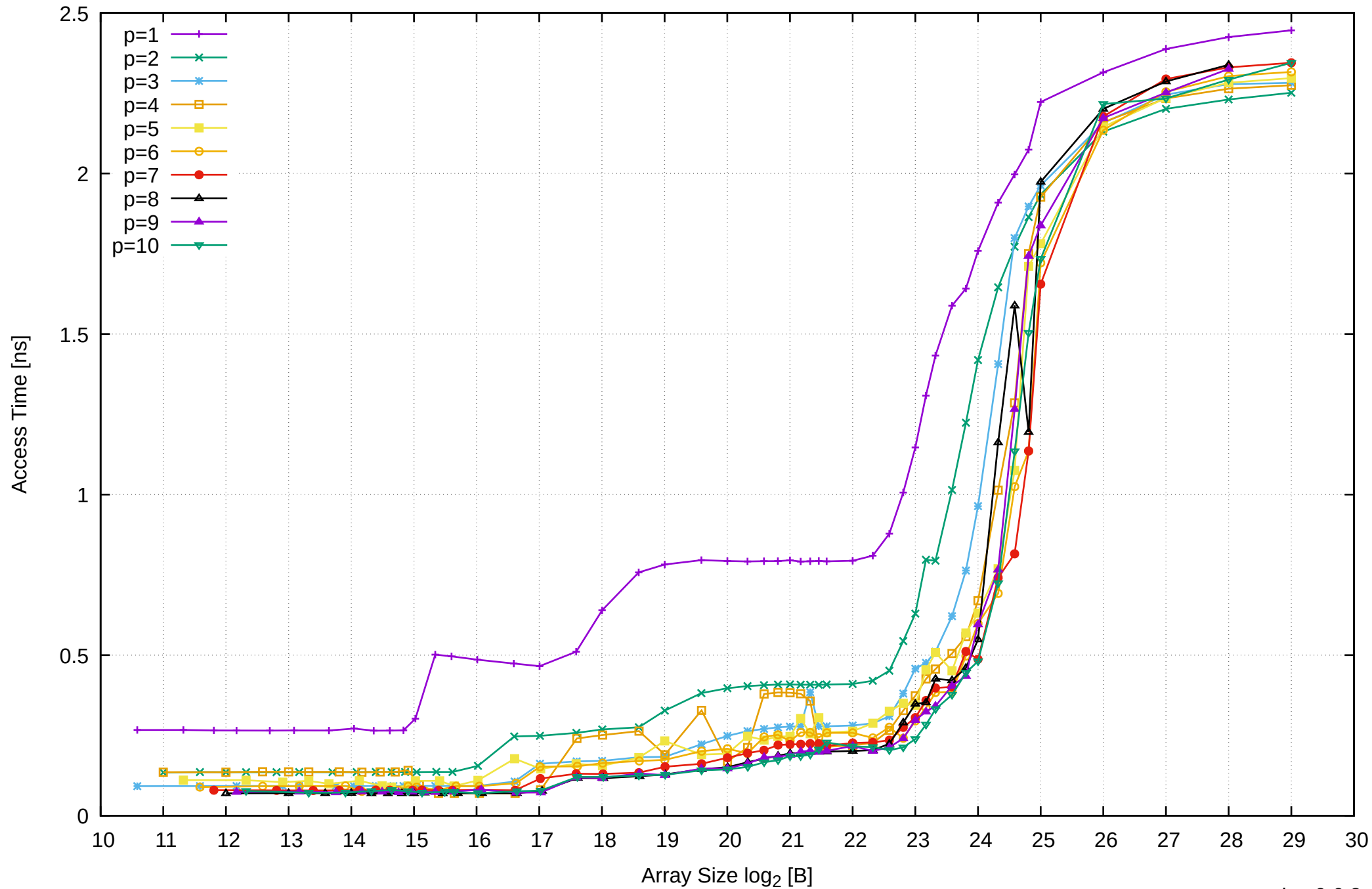
Intel Xeon E3-1260L v5 64GB - Parallel Memory Access Time - ScanWrite256PtrUnrollLoop
