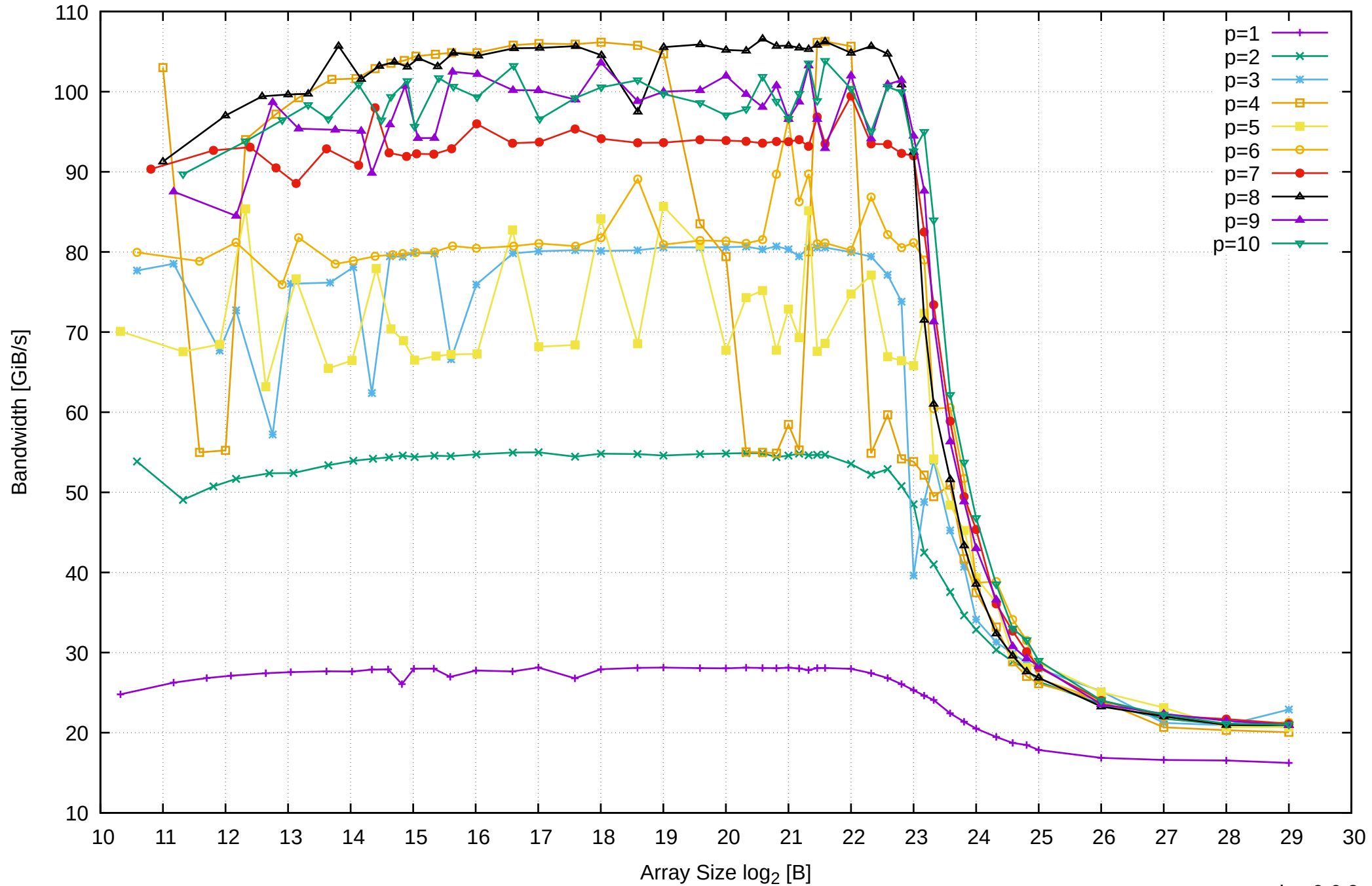
Intel Xeon E3-1260L v5 64GB - Parallel Memory Bandwidth - ScanRead128PtrSimpleLoop
