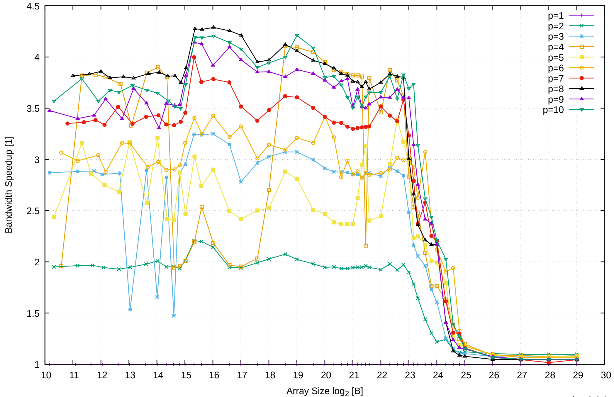
Intel Xeon E3-1260L v5 64GB - Speedup of Parallel Memory Bandwidth - ScanWrite64PtrUnrollLoop
