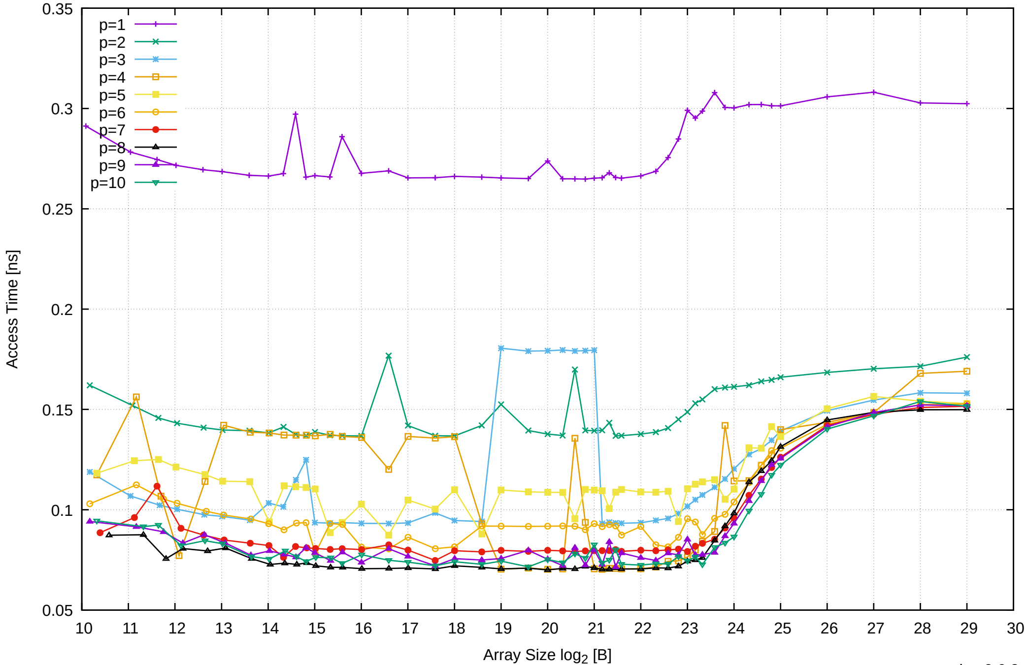
Intel Xeon E3-1260L v5 64GB - Parallel Memory Access Time - ScanRead32PtrSimpleLoop
