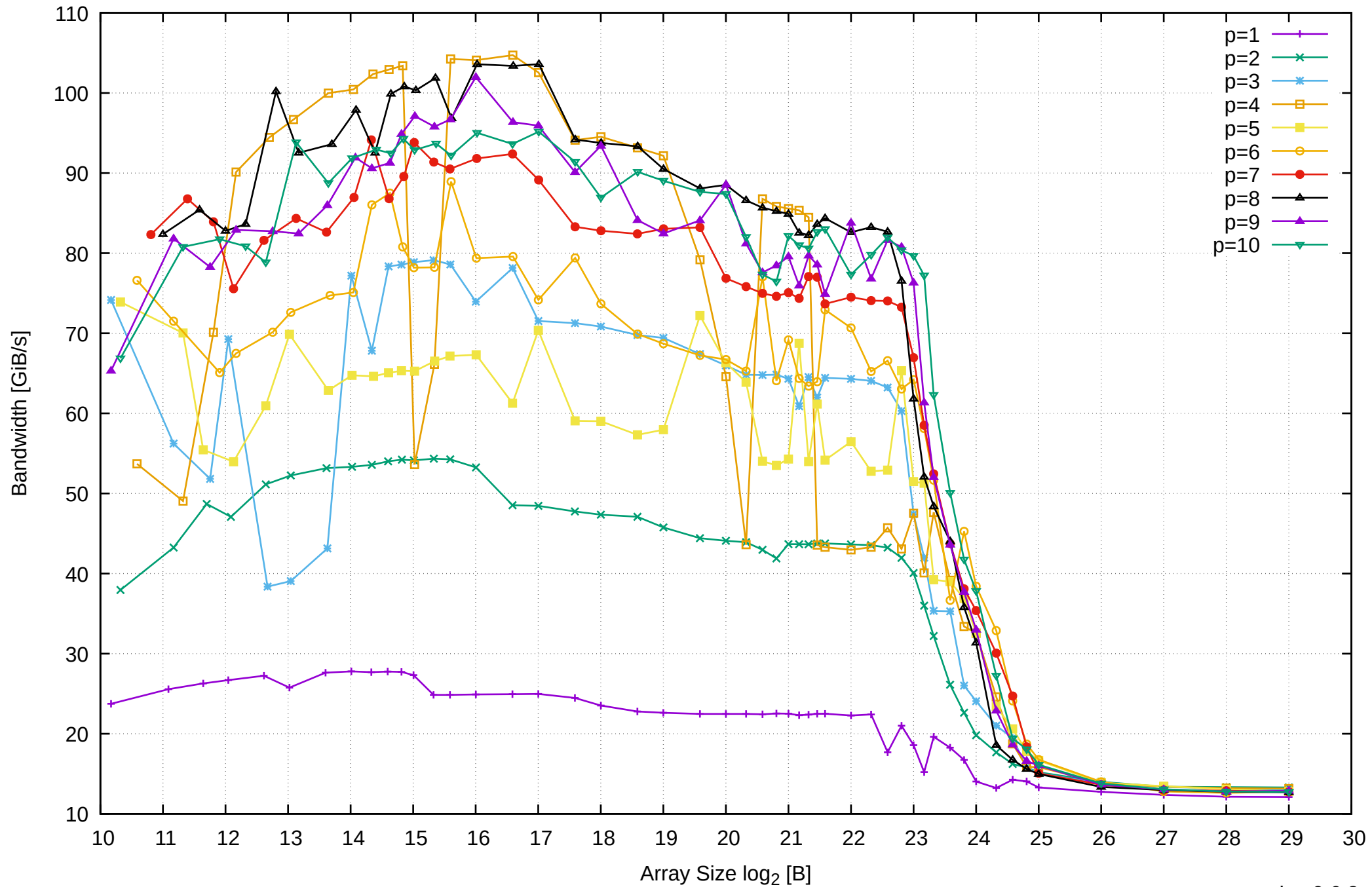
Intel Xeon E3-1260L v5 64GB - Parallel Memory Bandwidth - ScanWrite64PtrSimpleLoop
