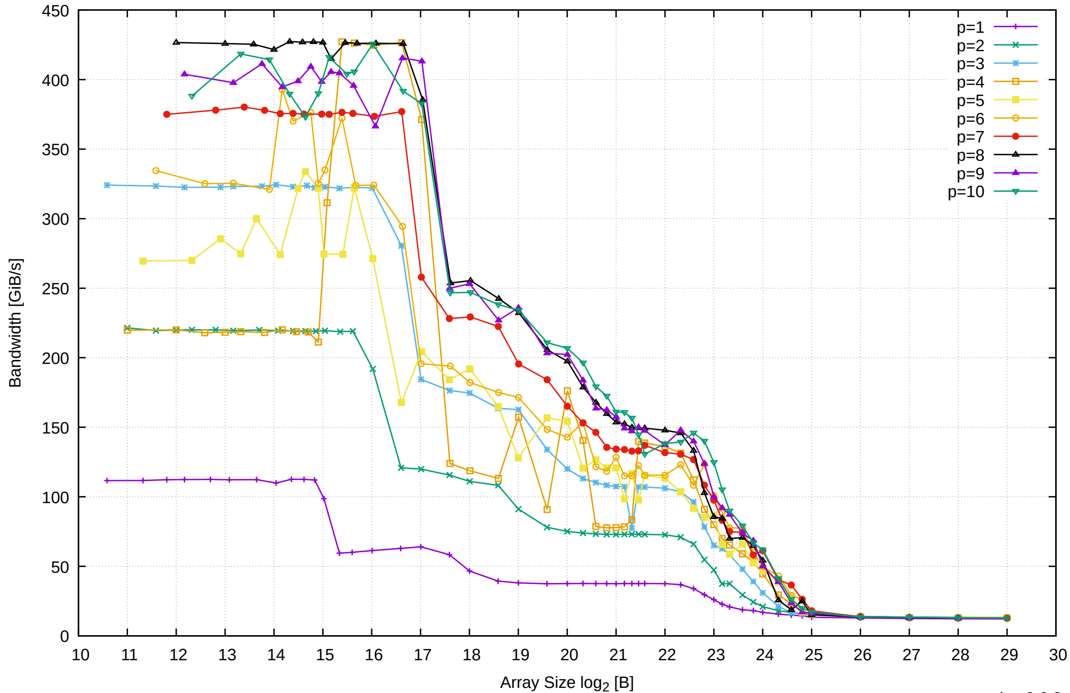
Intel Xeon E3-1260L v5 64GB - Parallel Memory Bandwidth - ScanWrite256PtrUnrollLoop
