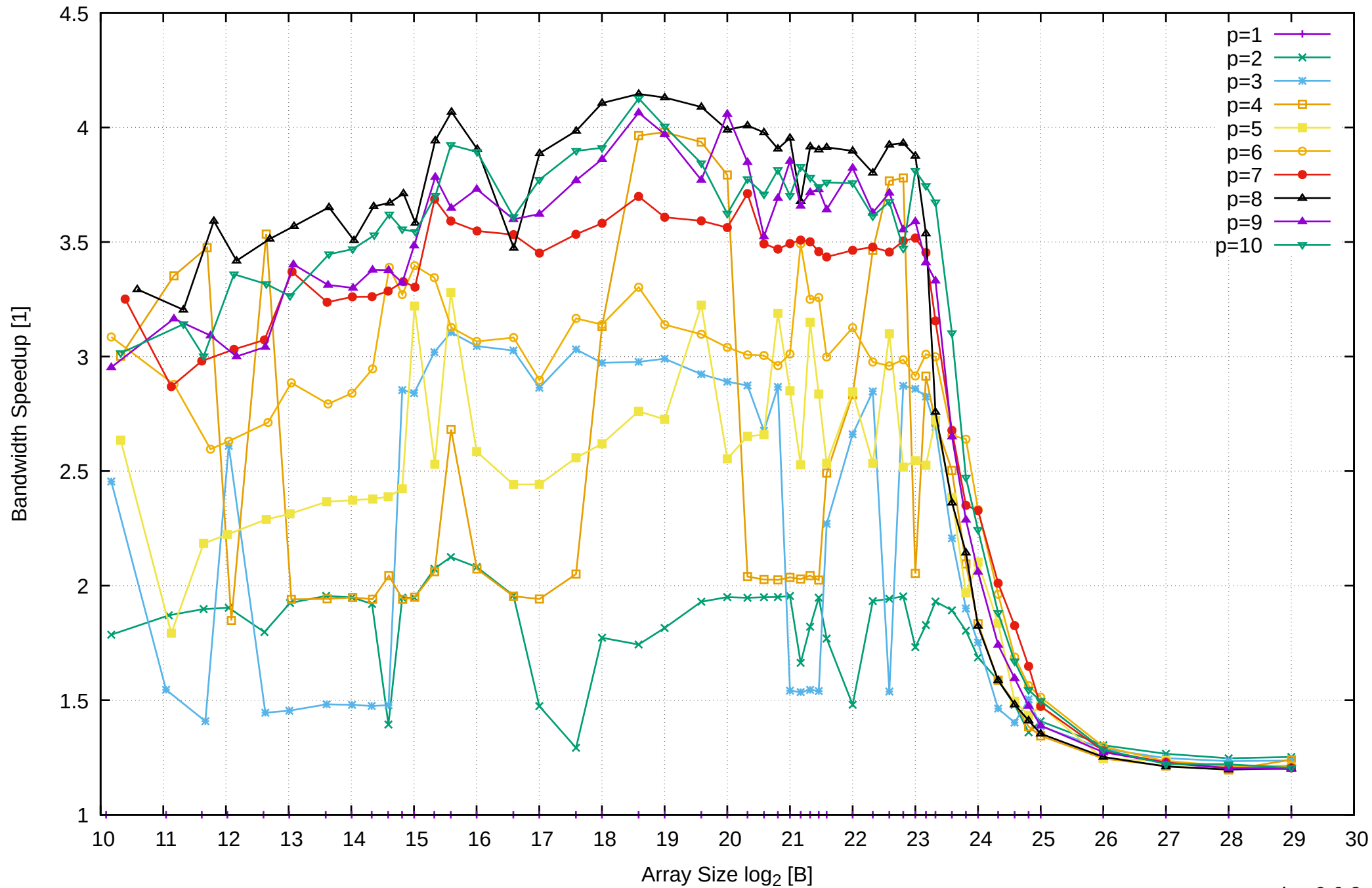
Intel Xeon E3-1260L v5 64GB - Speedup of Parallel Memory Bandwidth - ScanWrite32PtrSimpleLoop
