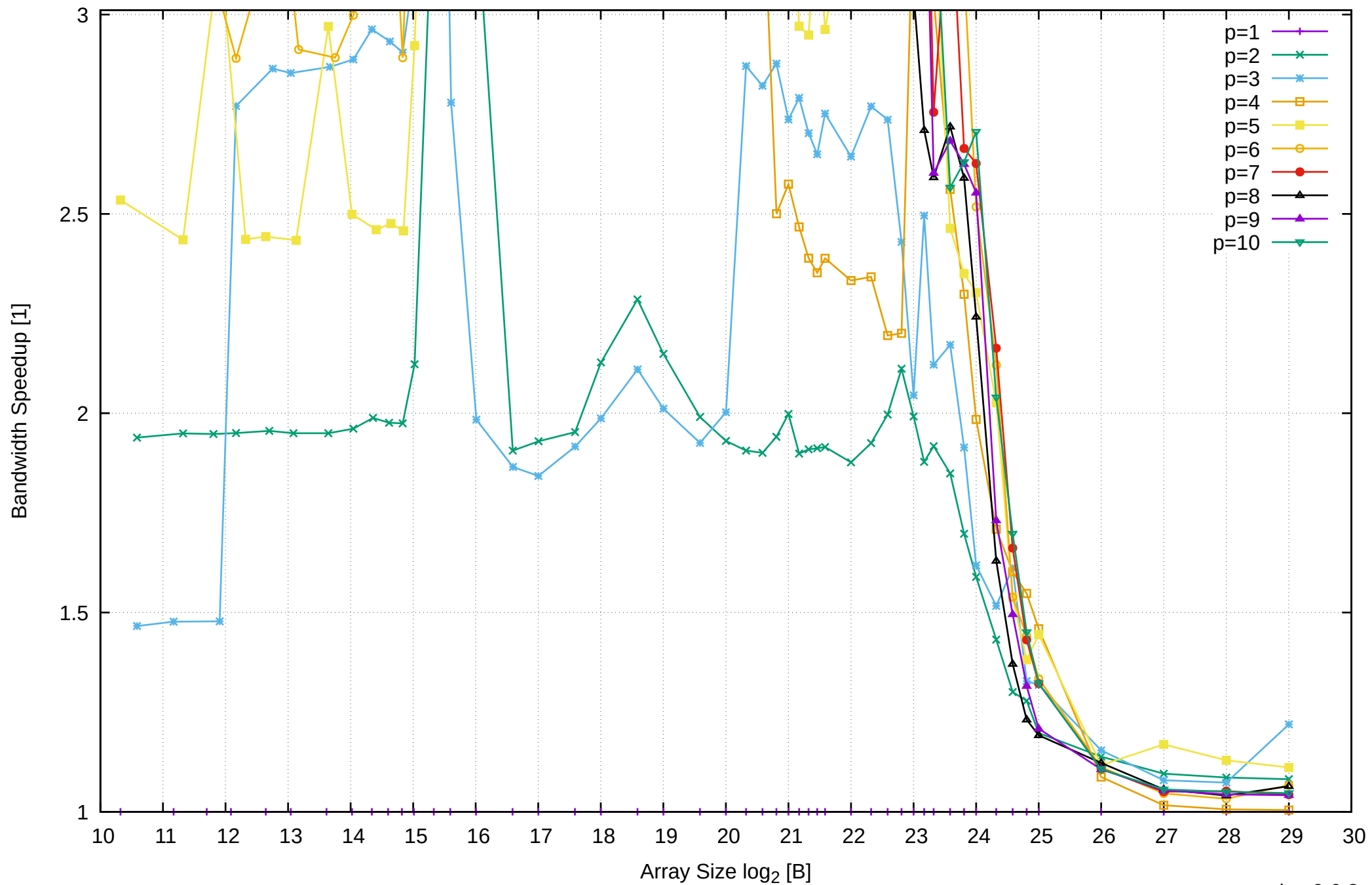
Intel Xeon E3-1260L v5 64GB - Speedup of Parallel Memory Bandwidth (enlarged) - ScanRead128PtrUnrollLoop
