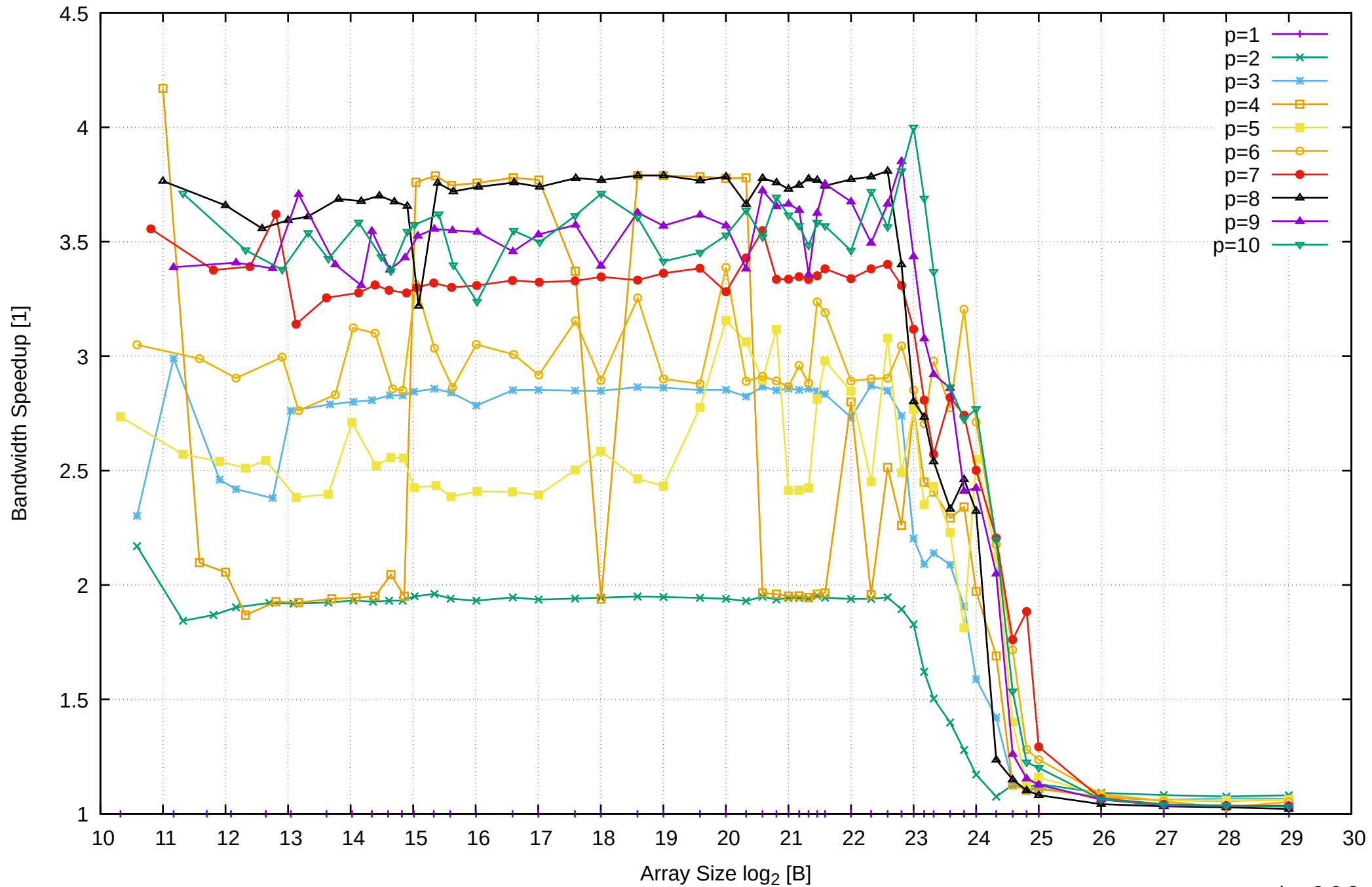
Intel Xeon E3-1260L v5 64GB - Speedup of Parallel Memory Bandwidth - ScanWrite128PtrSimpleLoop
