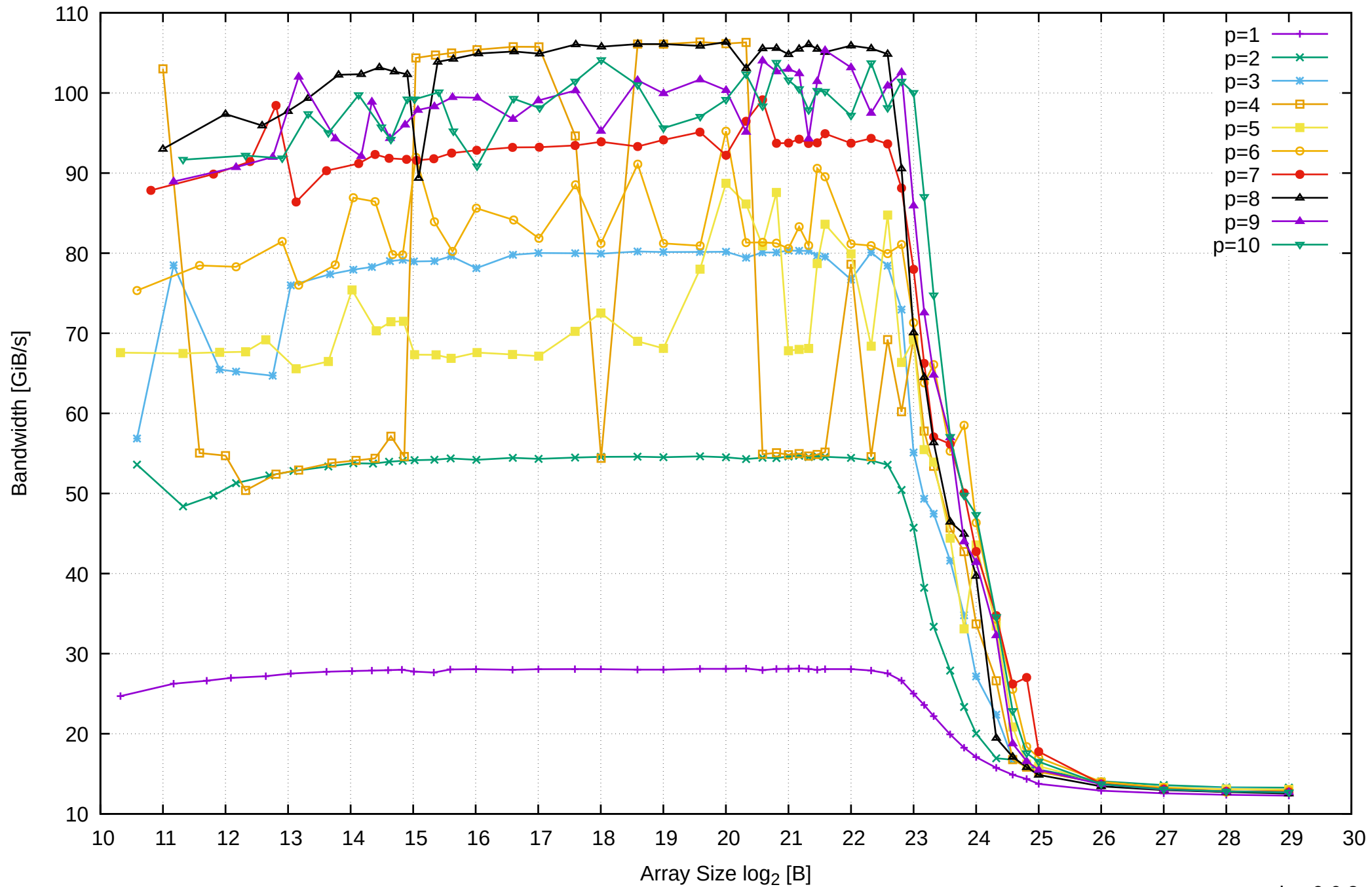
Intel Xeon E3-1260L v5 64GB - Parallel Memory Bandwidth - ScanWrite128PtrSimpleLoop
