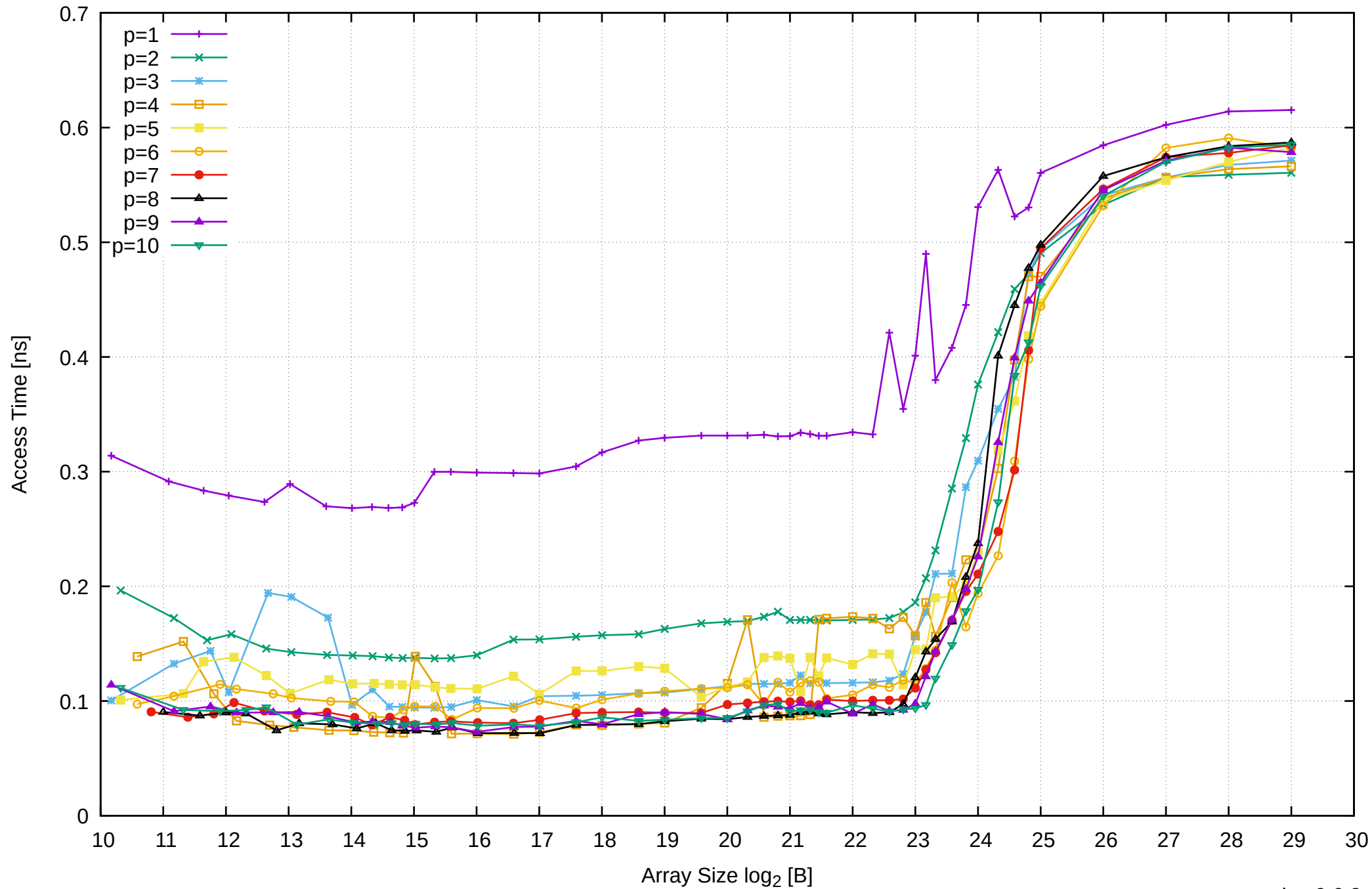
Intel Xeon E3-1260L v5 64GB - Parallel Memory Access Time - ScanWrite64PtrSimpleLoop
