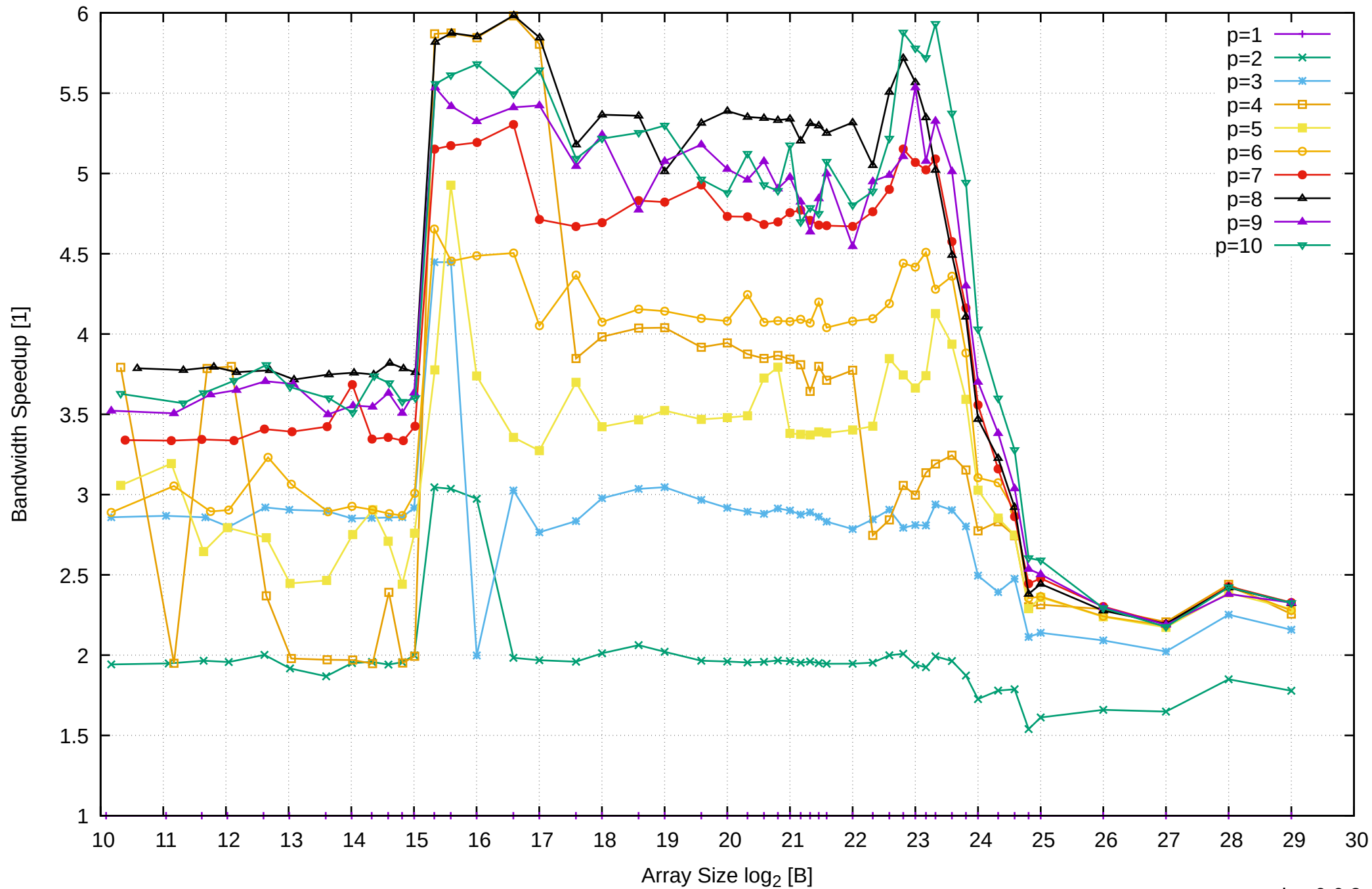
Intel Xeon E3-1260L v5 64GB - Speedup of Parallel Memory Bandwidth - ScanRead32PtrUnrollLoop
