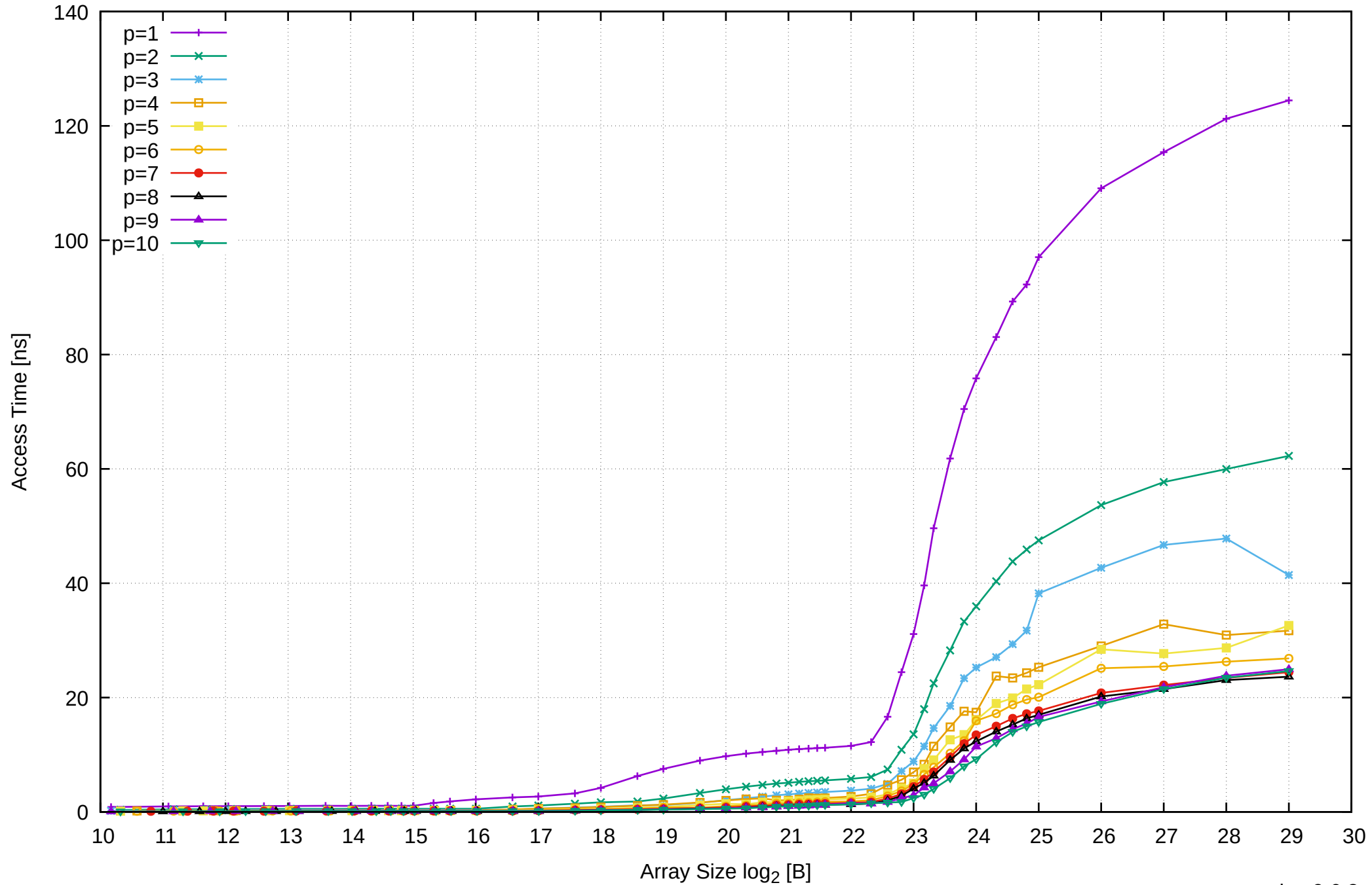
Intel Xeon E3-1260L v5 64GB - Parallel Memory Access Time - PermRead64UnrollLoop
