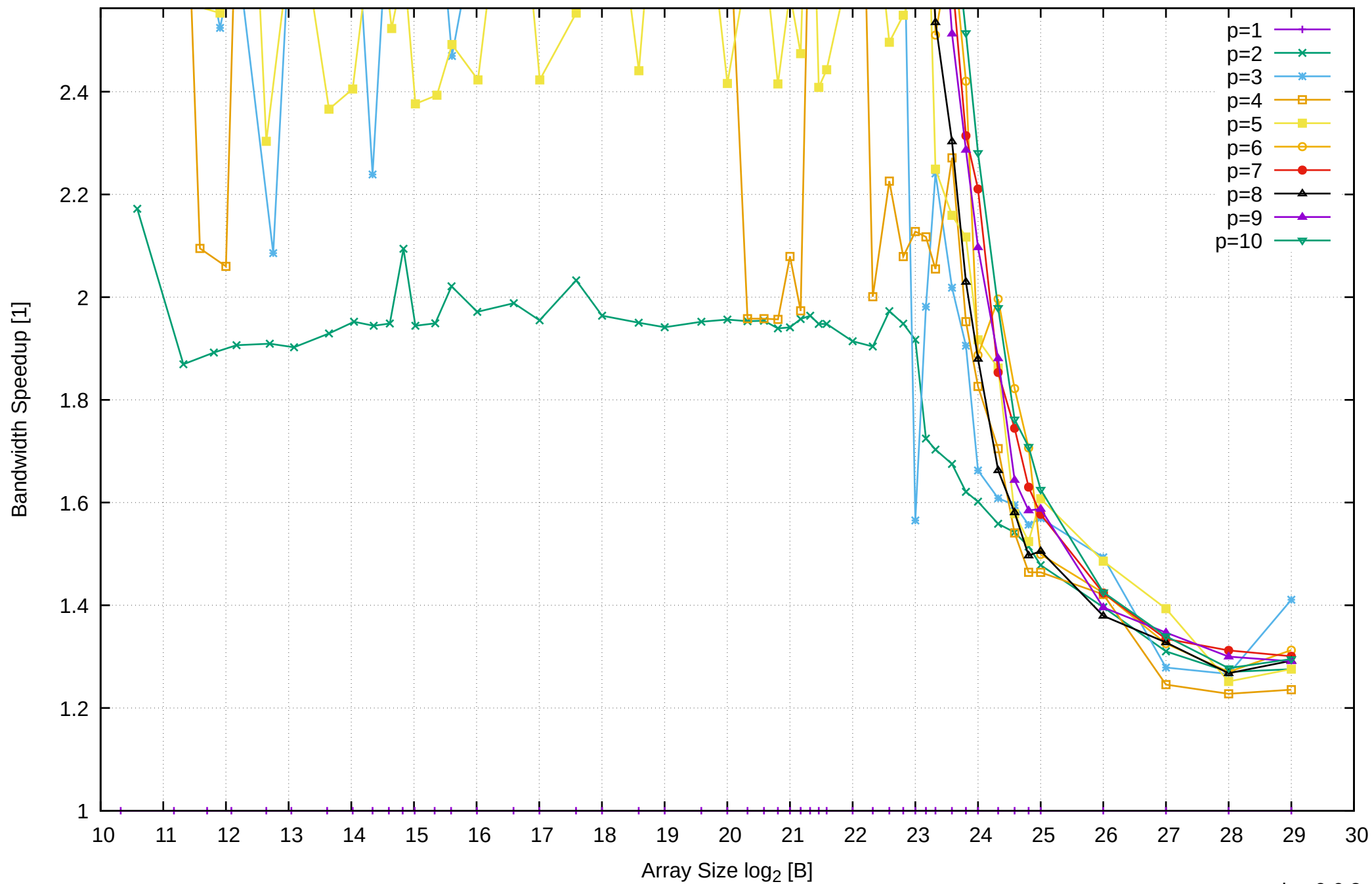
Intel Xeon E3-1260L v5 64GB - Speedup of Parallel Memory Bandwidth (enlarged) - ScanRead128PtrSimpleLoop
