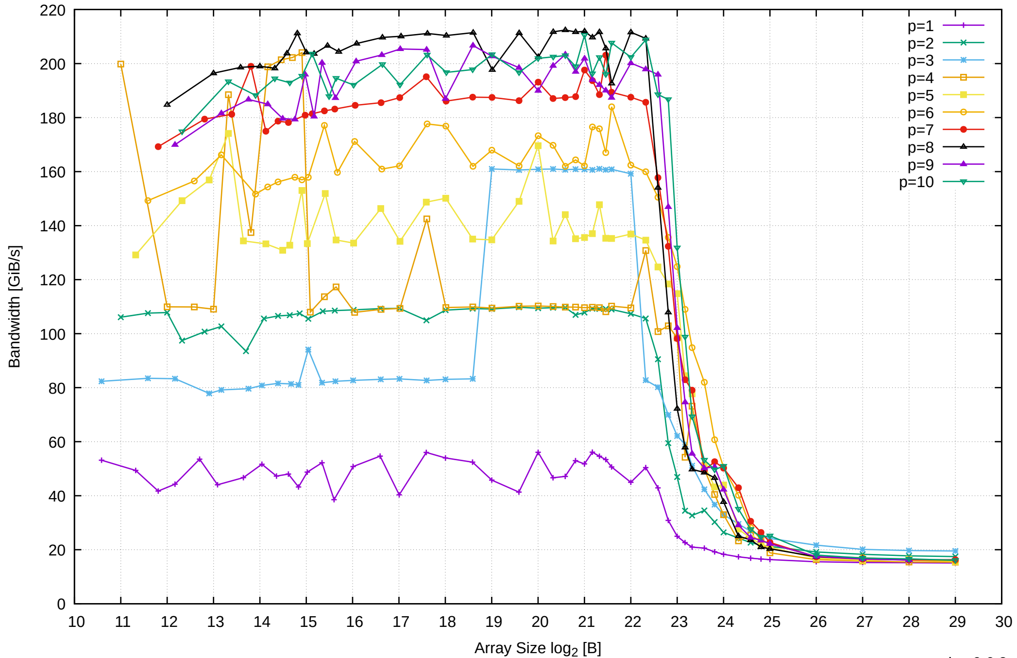
Intel Xeon E3-1260L v5 64GB - Parallel Memory Bandwidth - ScanRead256PtrSimpleLoop
