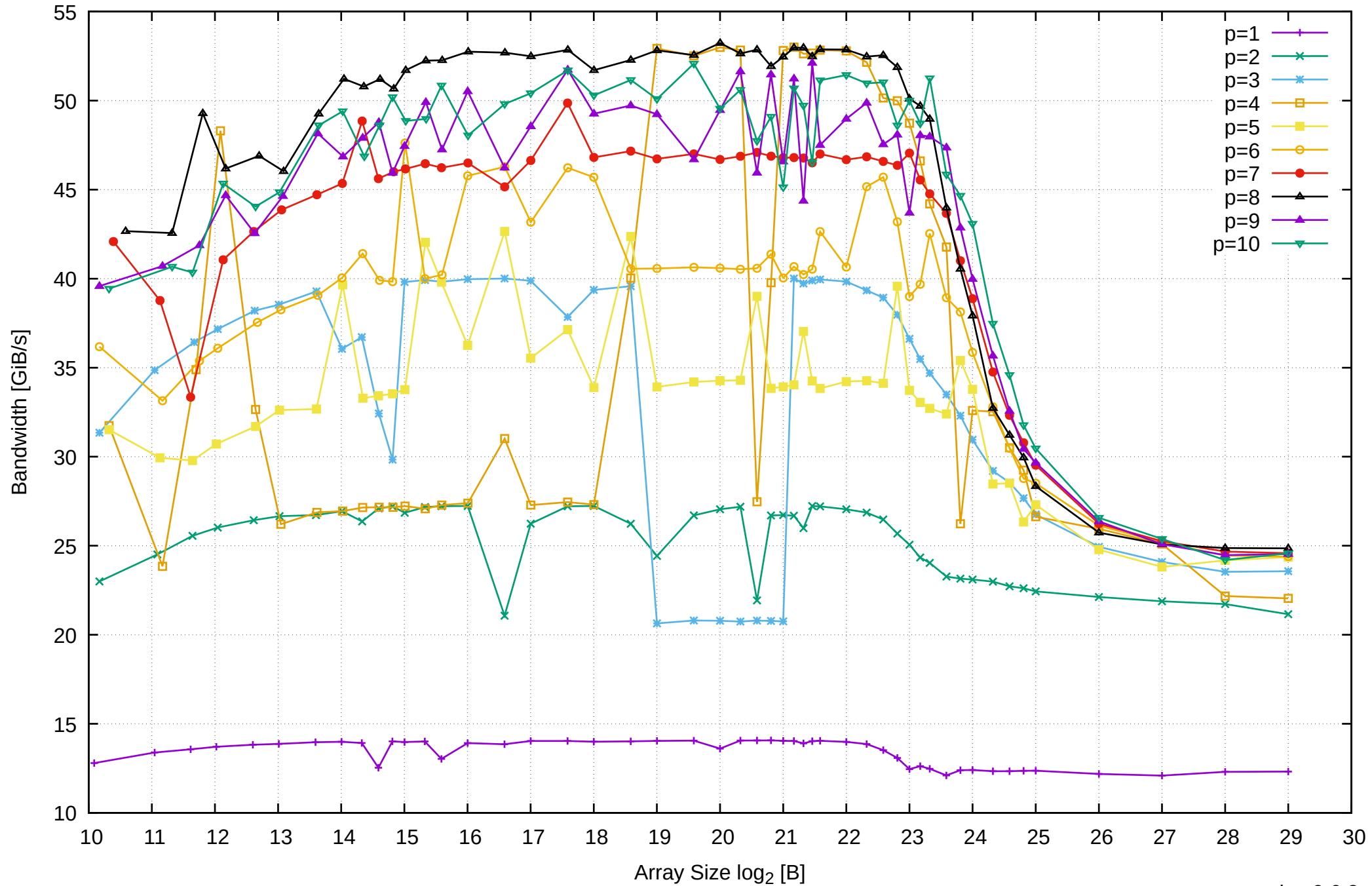
Intel Xeon E3-1260L v5 64GB - Parallel Memory Bandwidth - ScanRead32PtrSimpleLoop
