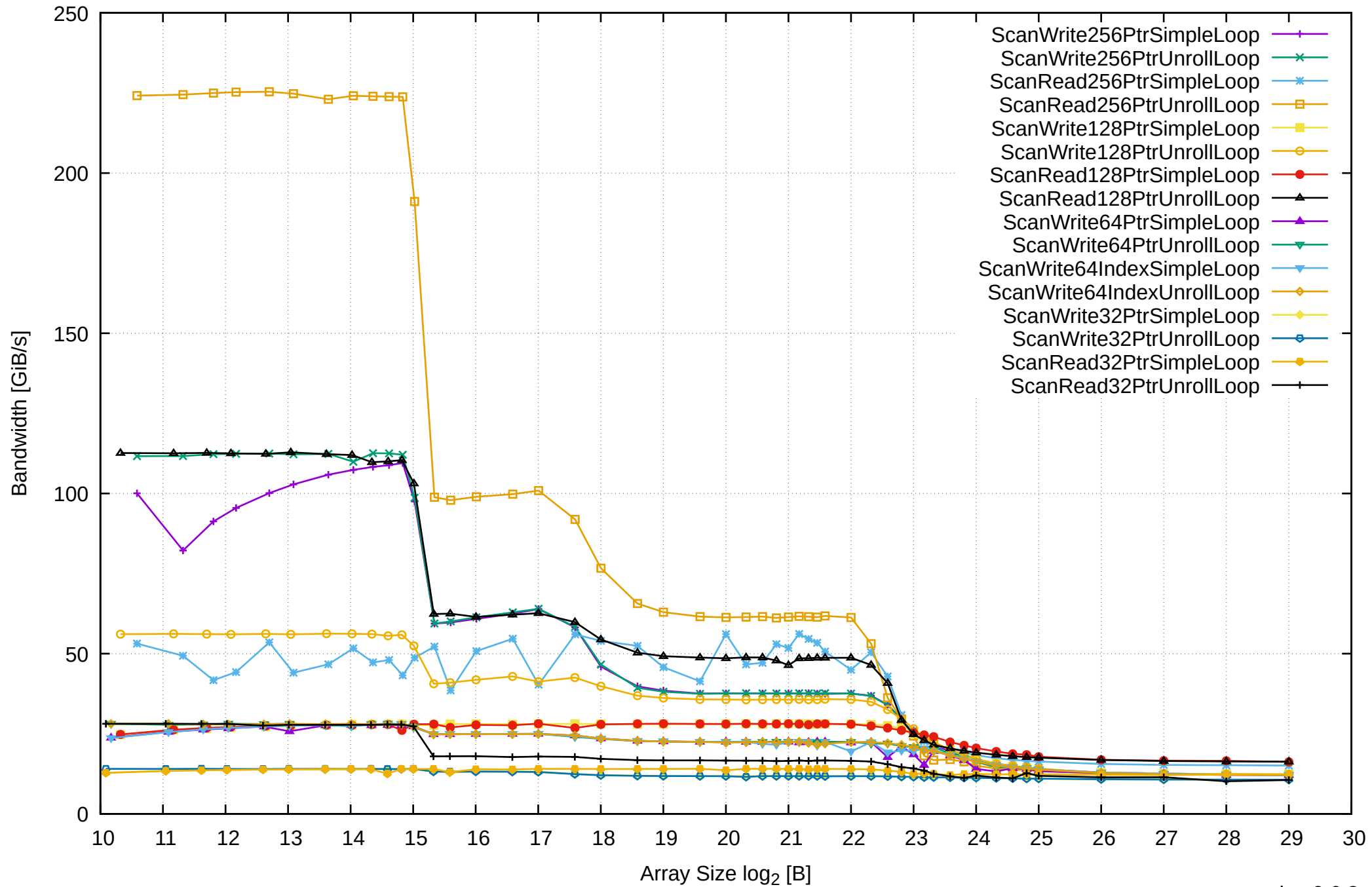
Intel Xeon E3-1260L v5 64GB - One Thread Memory Bandwidth (only 64-bit Reads)
