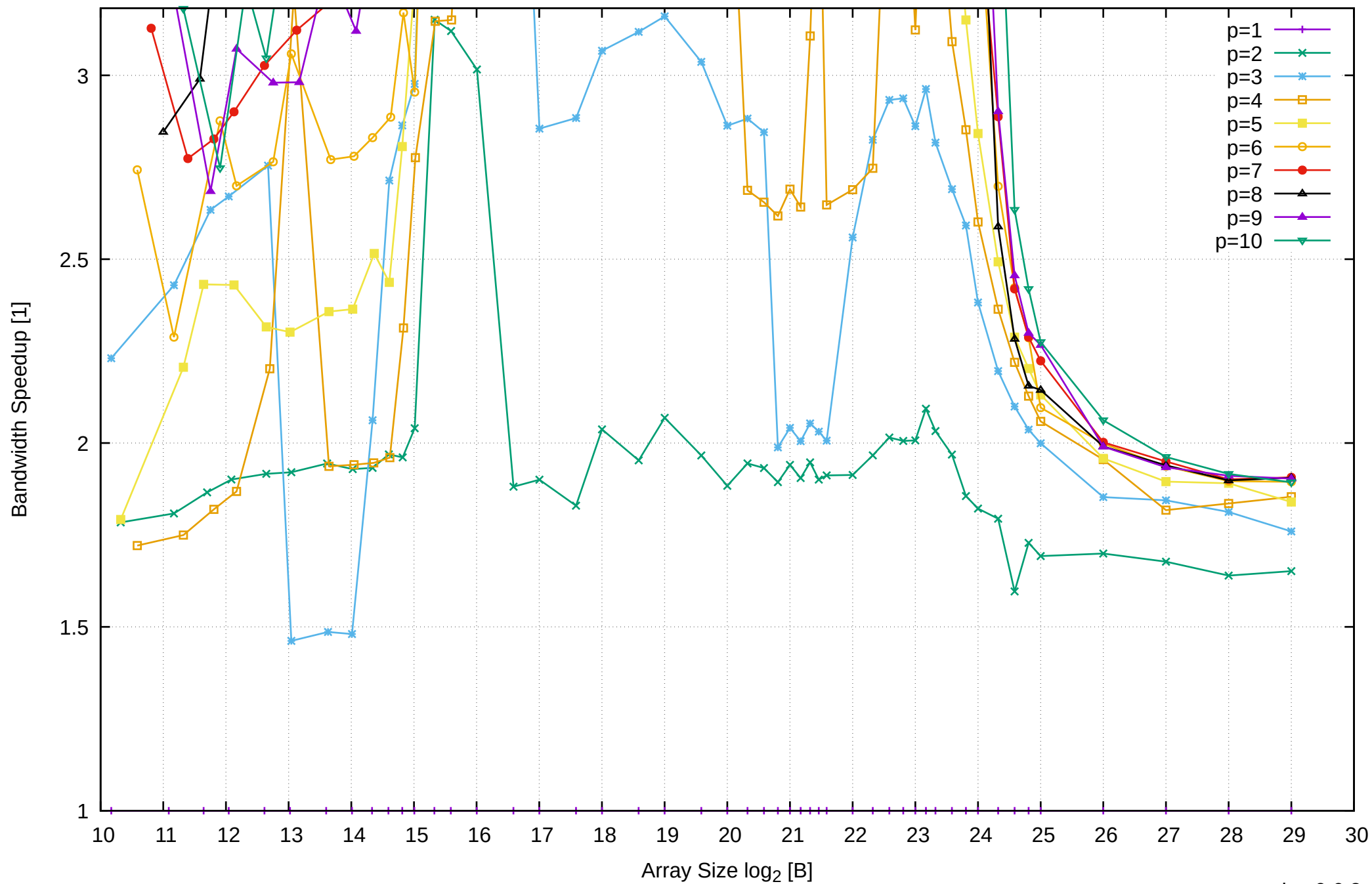
Intel Xeon E3-1260L v5 64GB - Speedup of Parallel Memory Bandwidth (enlarged) - ScanRead64IndexUnrollLoop
