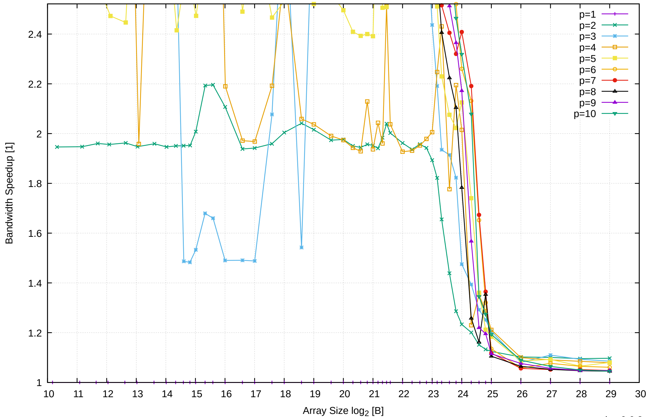
Intel Xeon E3-1260L v5 64GB - Speedup of Parallel Memory Bandwidth (enlarged) - ScanWrite64IndexUnrollLoop
