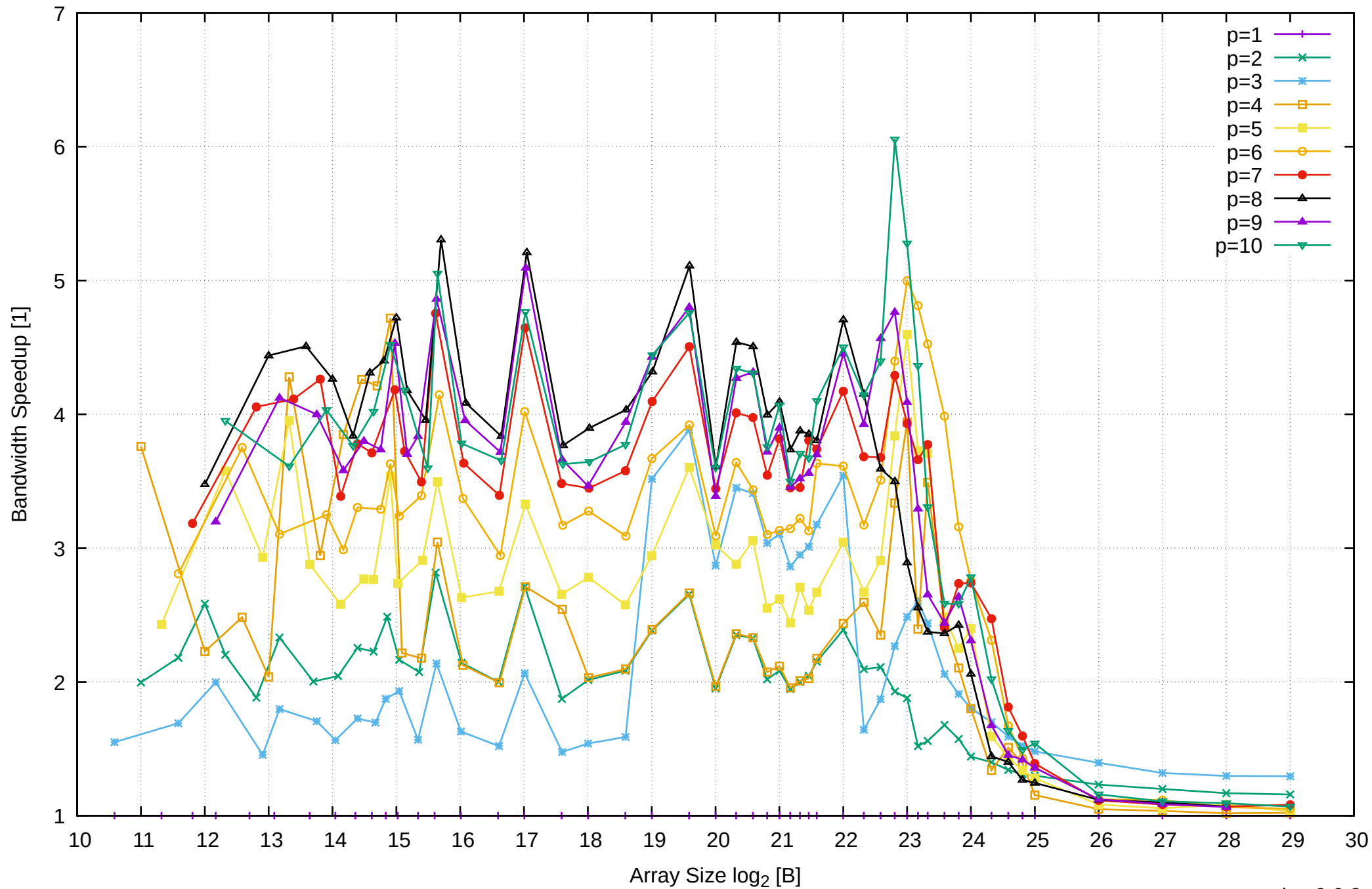
Intel Xeon E3-1260L v5 64GB - Speedup of Parallel Memory Bandwidth - ScanRead256PtrSimpleLoop
