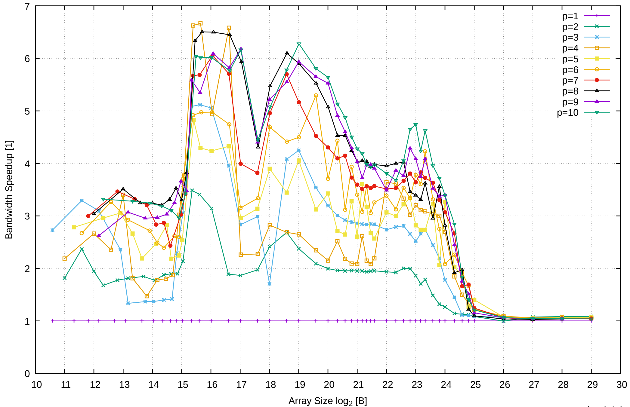
Intel Xeon E3-1260L v5 64GB - Speedup of Parallel Memory Bandwidth - ScanWrite256PtrSimpleLoop
