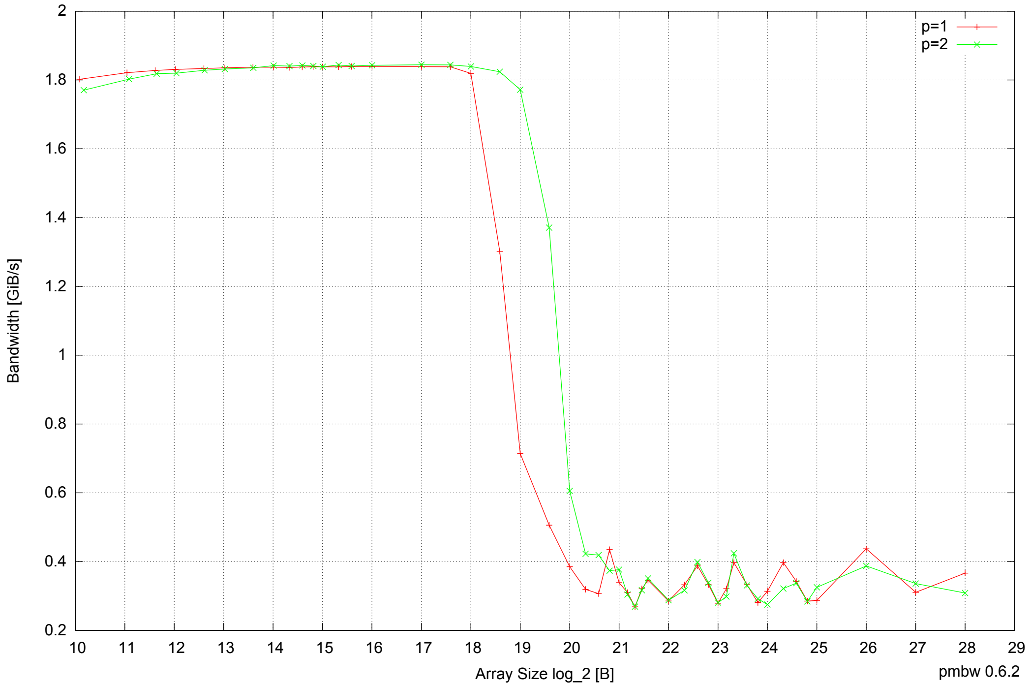
Intel Mobile Pentium III-M 512MB - Parallel Memory Bandwidth - ScanRead32PtrSimpleLoop
