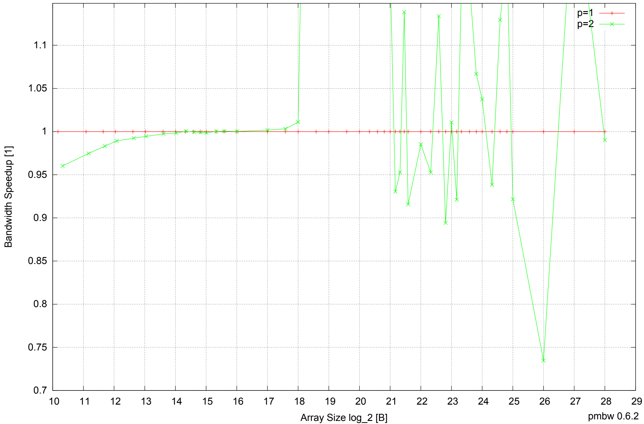
Intel Mobile Pentium III-M 512MB - Speedup of Parallel Memory Bandwidth (enlarged) - ScanRead128PtrSimpleLoop
