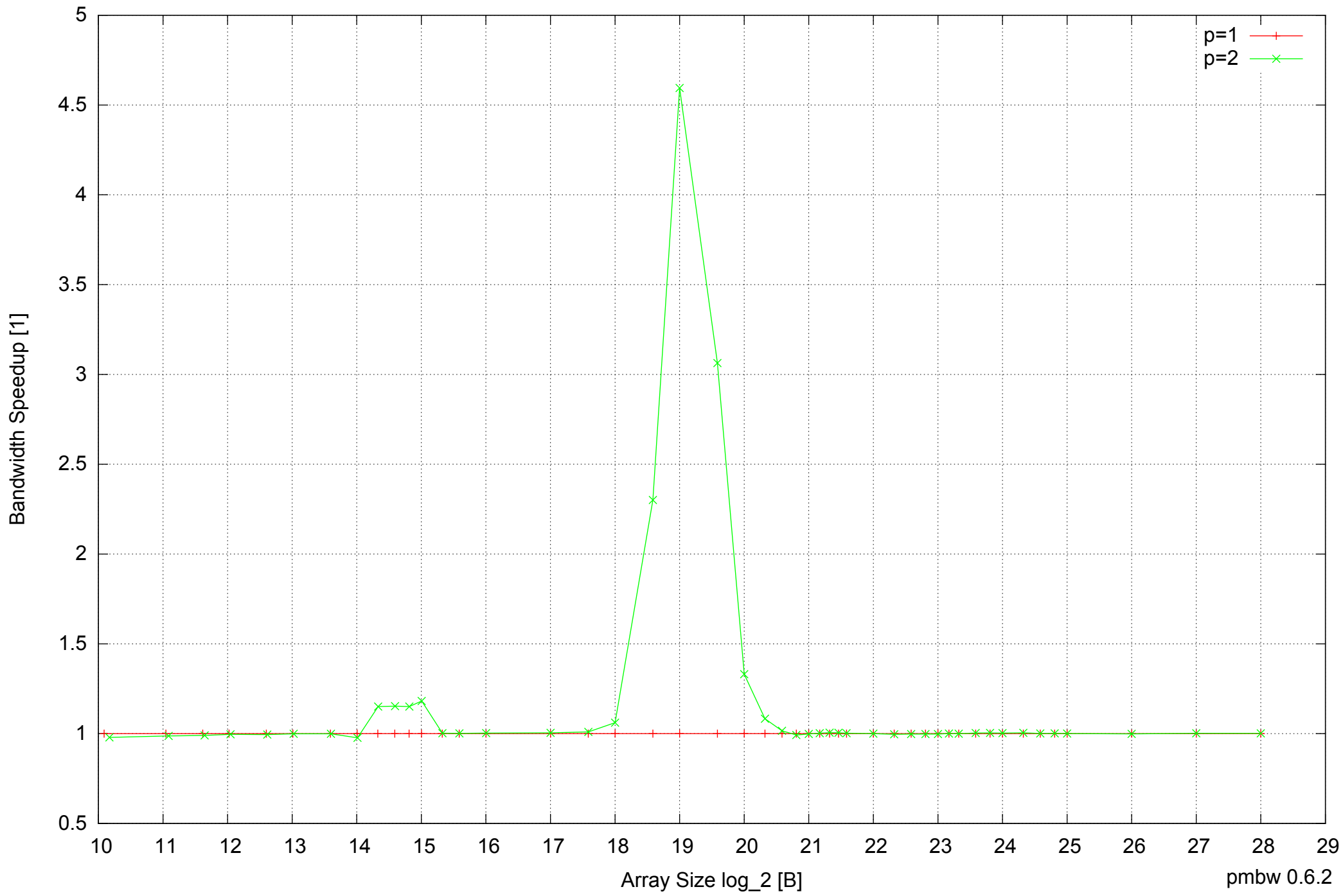
Intel Mobile Pentium III-M 512MB - Speedup of Parallel Memory Bandwidth - ScanWrite32PtrUnrollLoop
