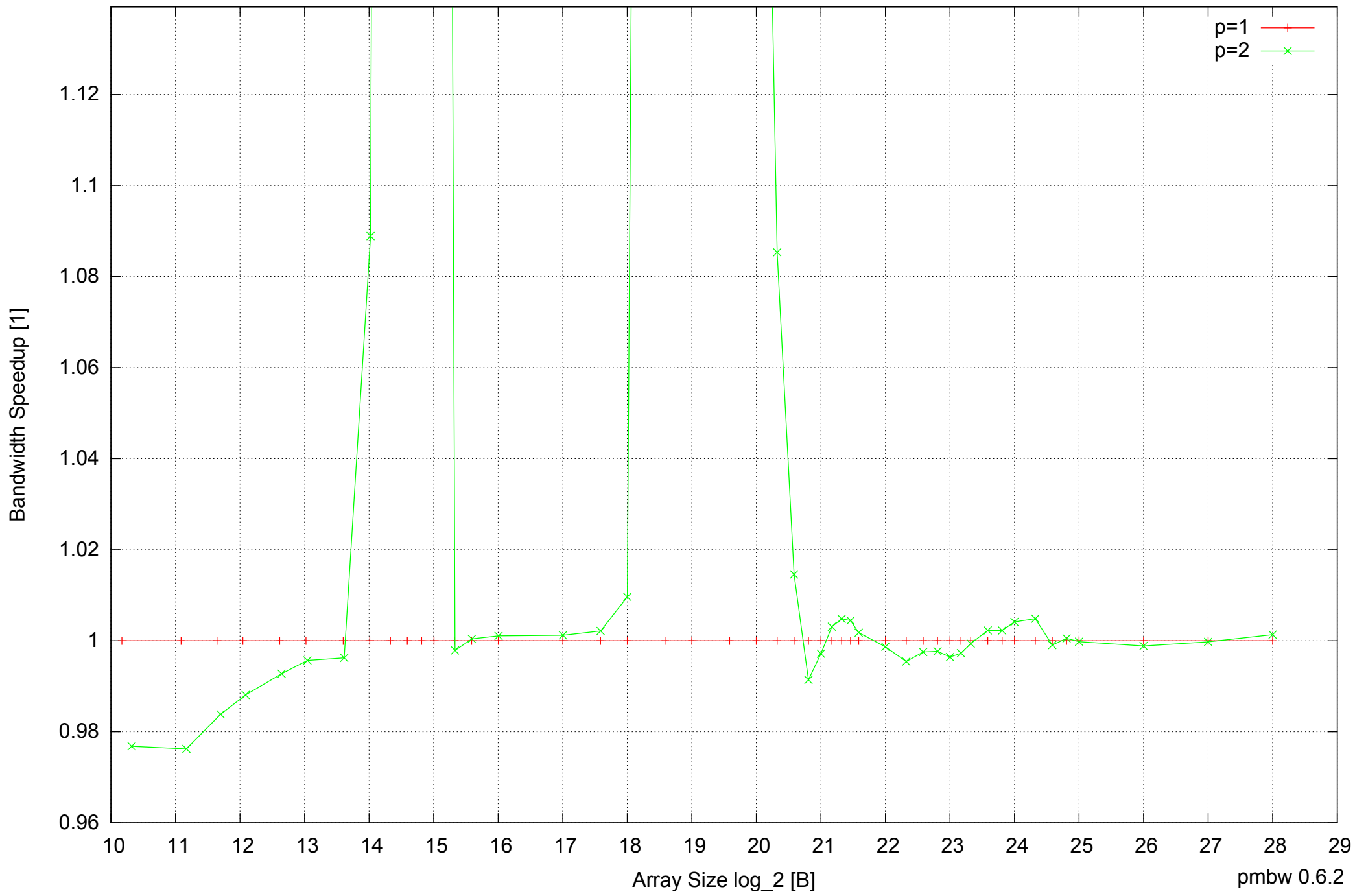
Intel Mobile Pentium III-M 512MB - Speedup of Parallel Memory Bandwidth (enlarged) - ScanWrite64PtrUnrollLoop
