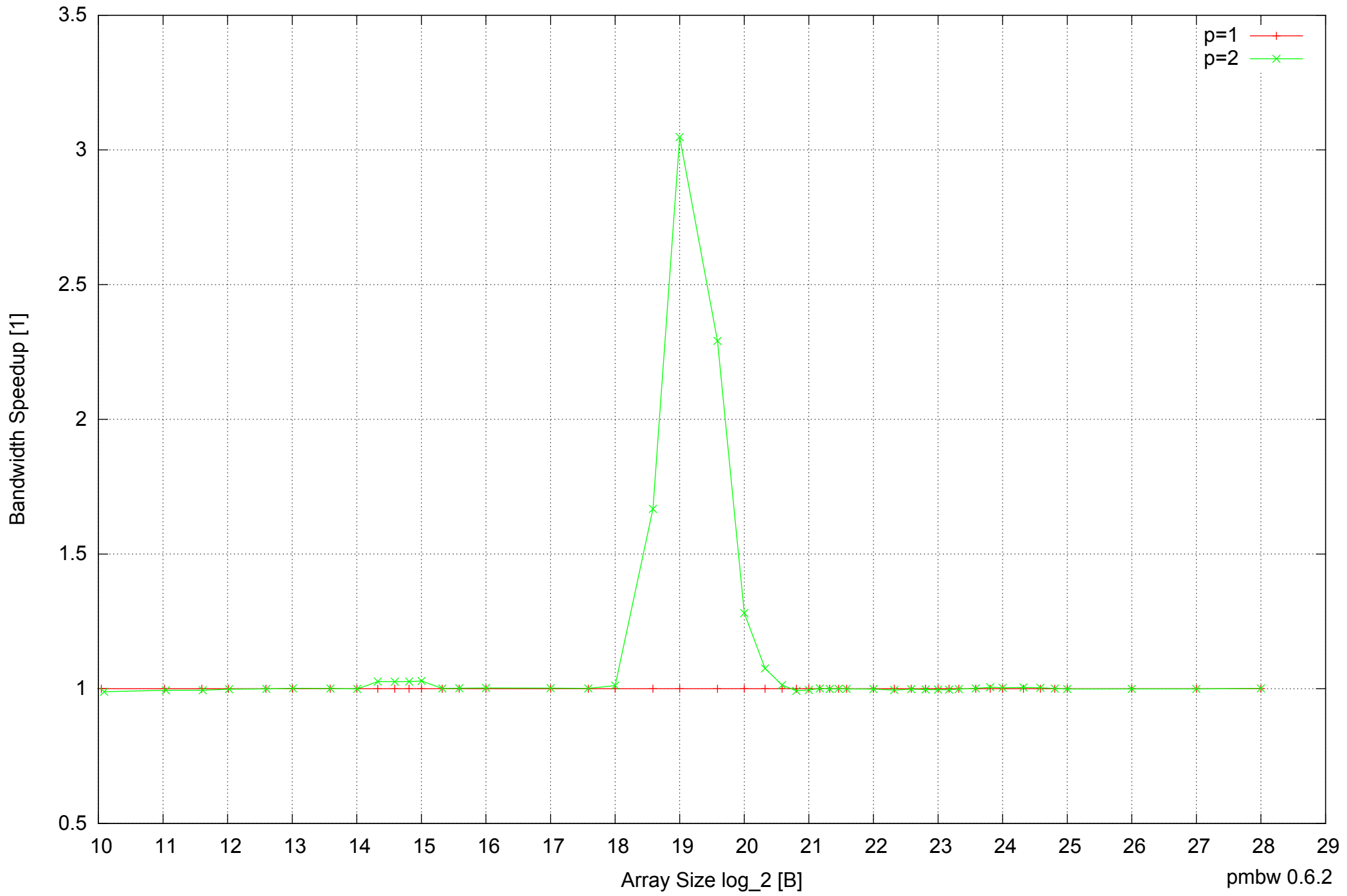
Intel Mobile Pentium III-M 512MB - Speedup of Parallel Memory Bandwidth - ScanWrite16PtrUnrollLoop
