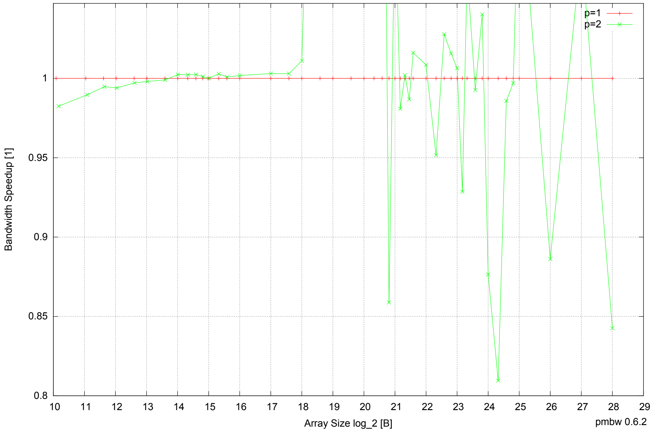
Intel Mobile Pentium III-M 512MB - Speedup of Parallel Memory Bandwidth (enlarged) - ScanRead32PtrSimpleLoop
