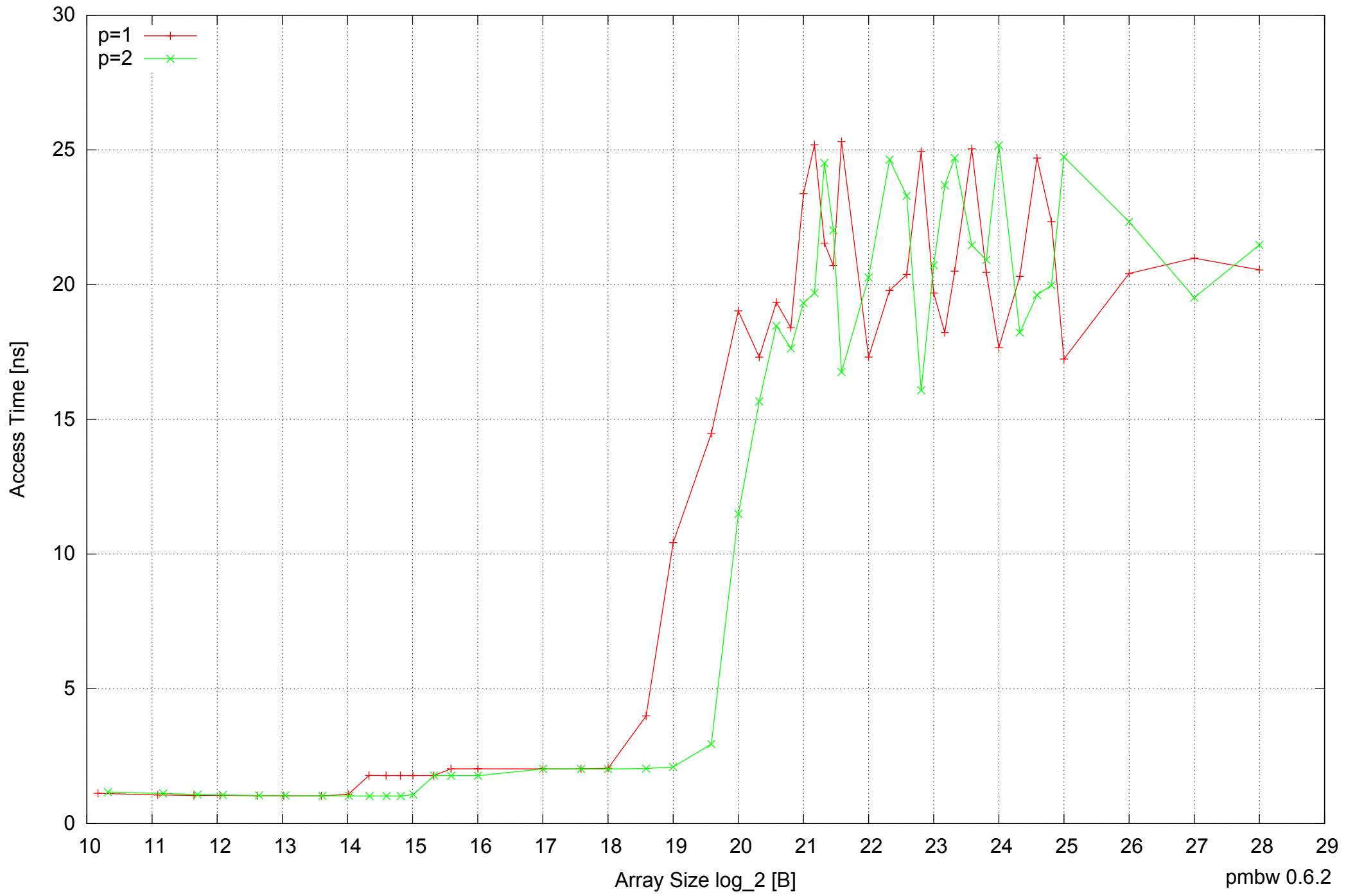
Intel Mobile Pentium III-M 512MB - Parallel Memory Access Time - ScanRead64PtrUnrollLoop
