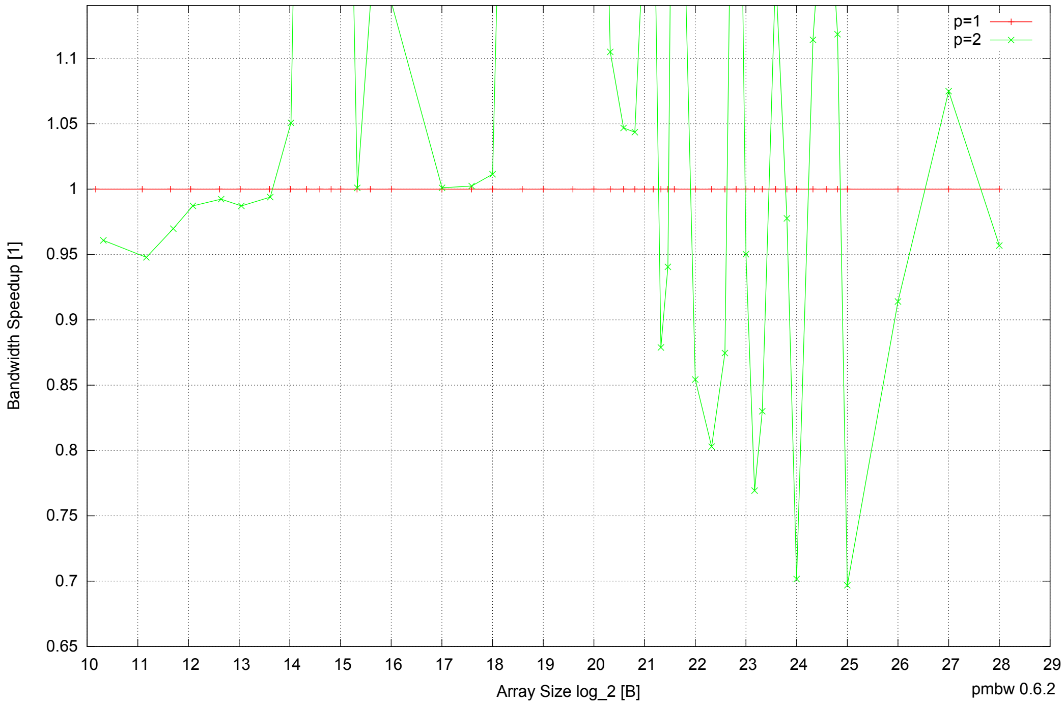
Intel Mobile Pentium III-M 512MB - Speedup of Parallel Memory Bandwidth (enlarged) - ScanRead64PtrUnrollLoop
