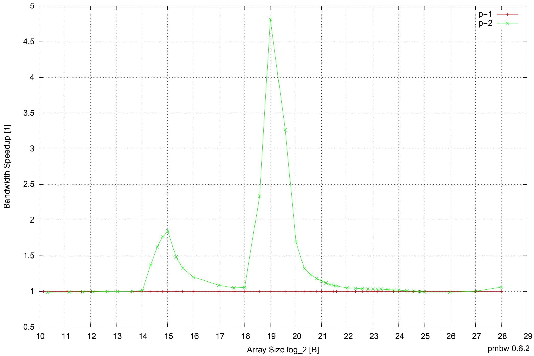
Intel Mobile Pentium III-M 512MB - Speedup of Parallel Memory Bandwidth - PermRead32UnrollLoop
