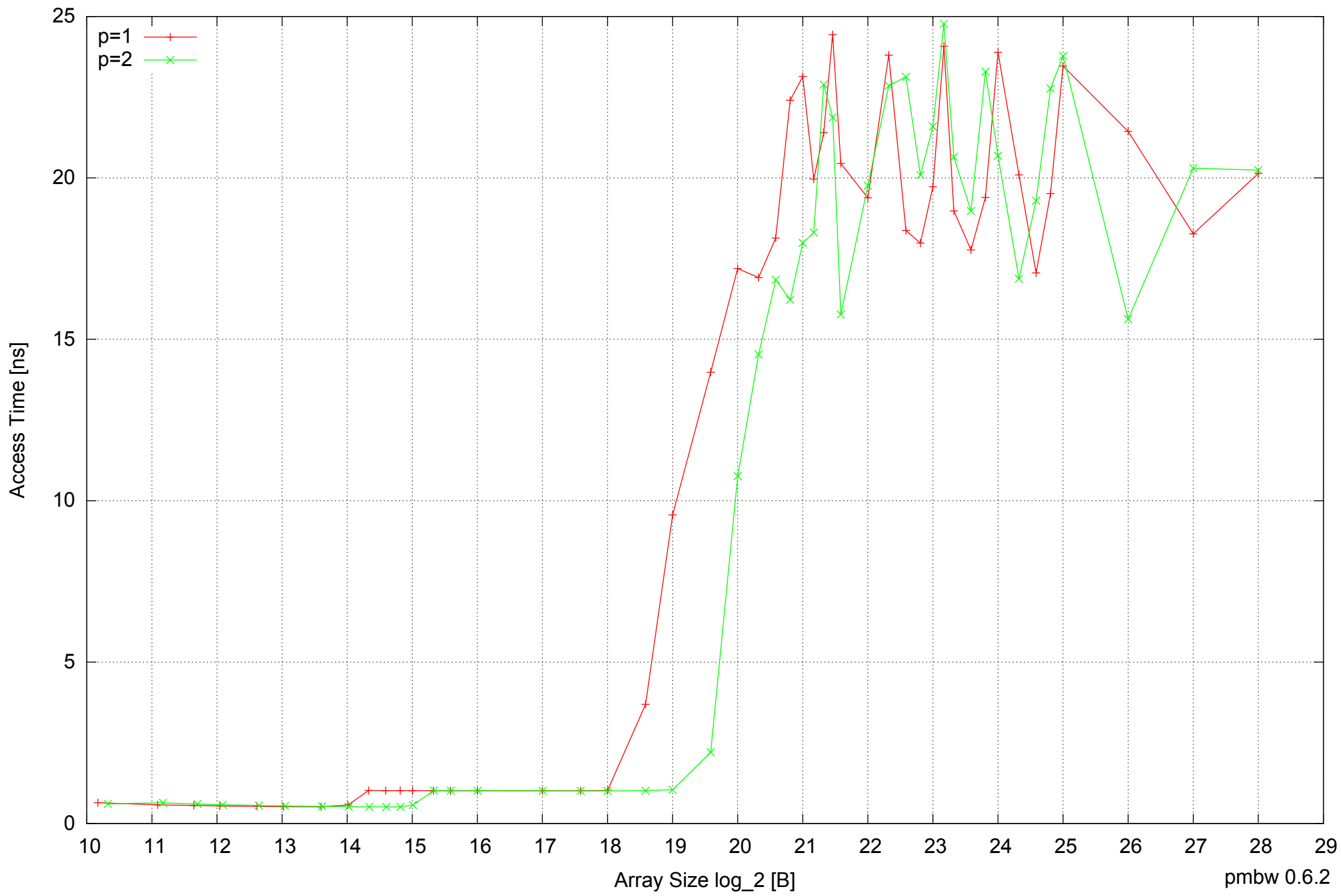
Intel Mobile Pentium III-M 512MB - Parallel Memory Access Time - ScanRead128PtrUnrollLoop
