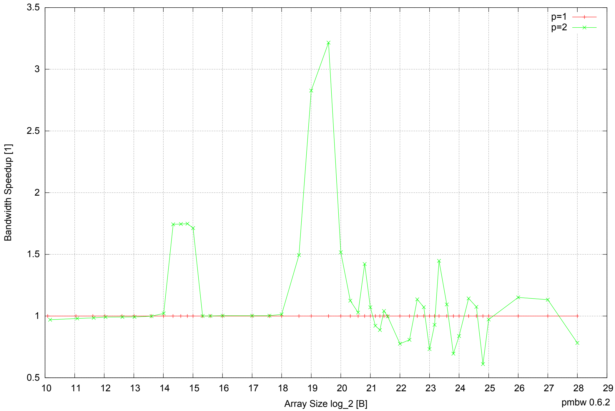
Intel Mobile Pentium III-M 512MB - Speedup of Parallel Memory Bandwidth - ScanRead32IndexUnrollLoop
