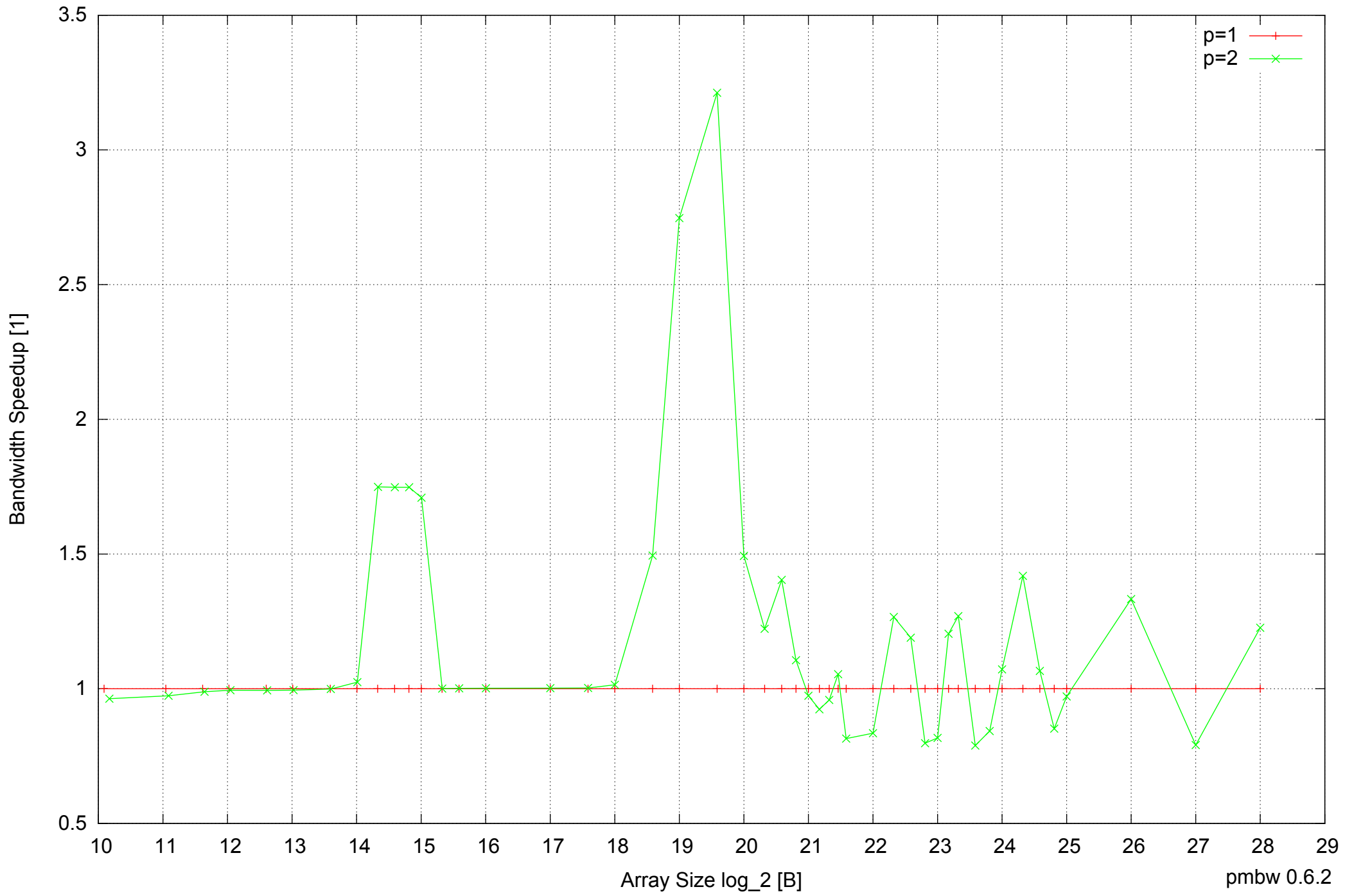
Intel Mobile Pentium III-M 512MB - Speedup of Parallel Memory Bandwidth - ScanRead32PtrUnrollLoop
