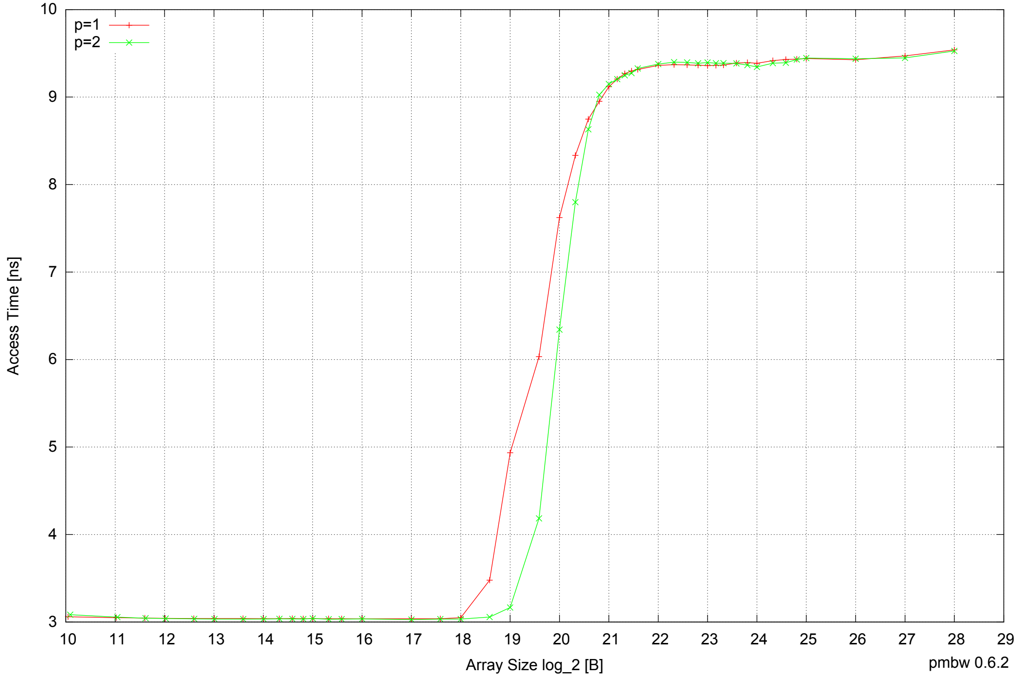
Intel Mobile Pentium III-M 512MB - Parallel Memory Access Time - ScanWrite16PtrSimpleLoop
