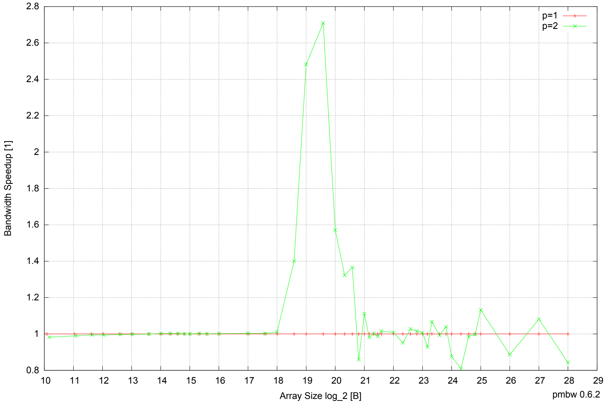
Intel Mobile Pentium III-M 512MB - Speedup of Parallel Memory Bandwidth - ScanRead32PtrSimpleLoop
