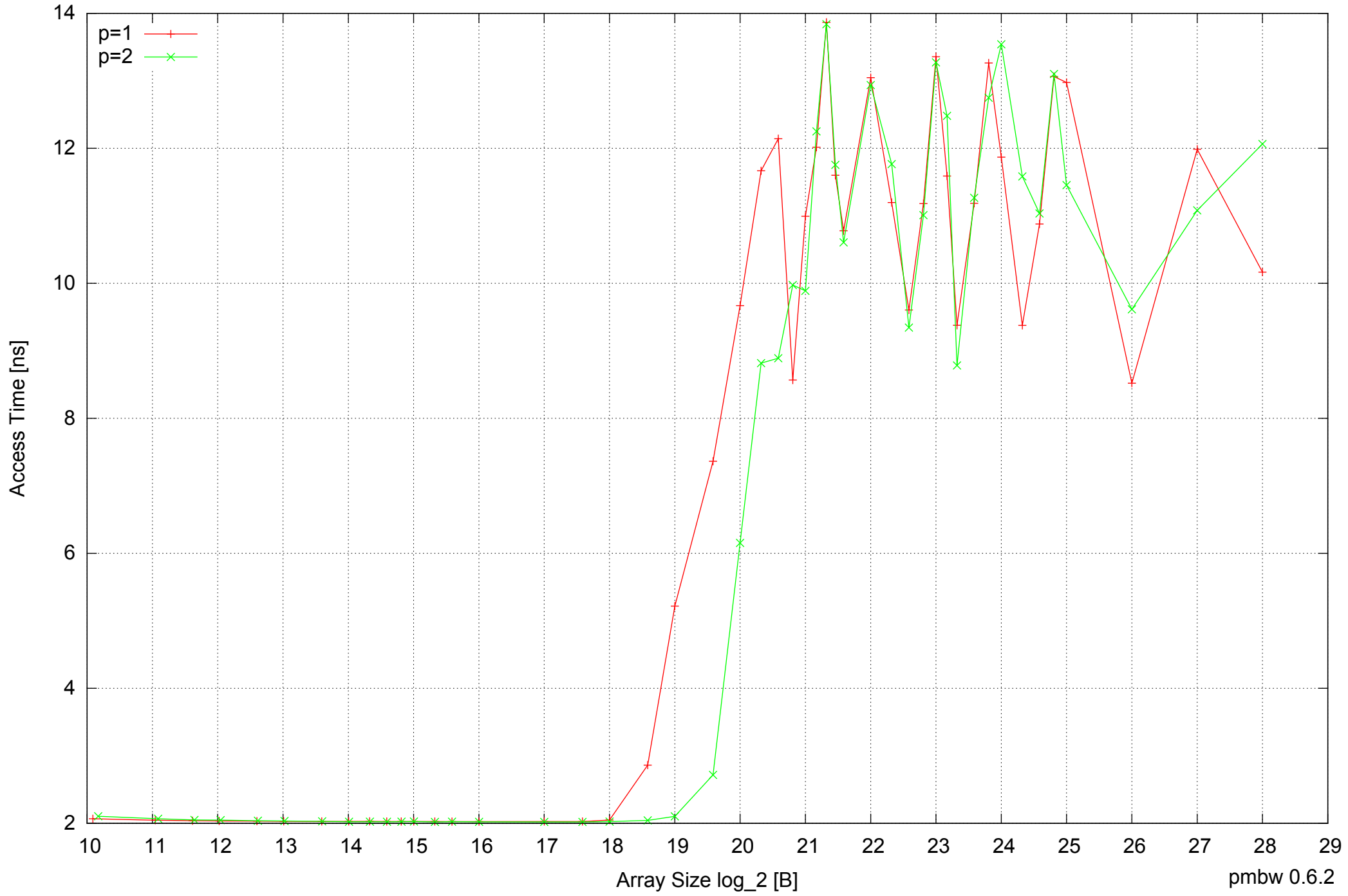
Intel Mobile Pentium III-M 512MB - Parallel Memory Access Time - ScanRead32PtrSimpleLoop
