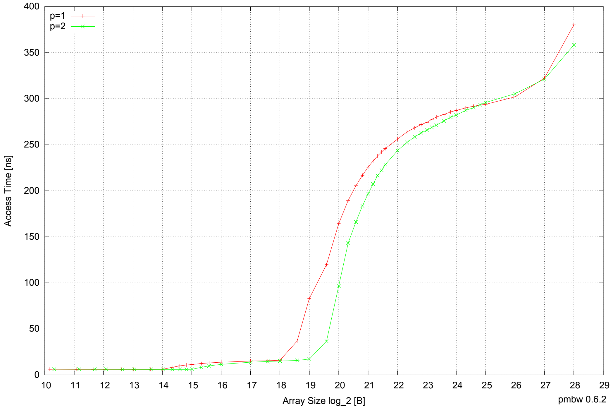
Intel Mobile Pentium III-M 512MB - Parallel Memory Access Time - PermRead32UnrollLoop
