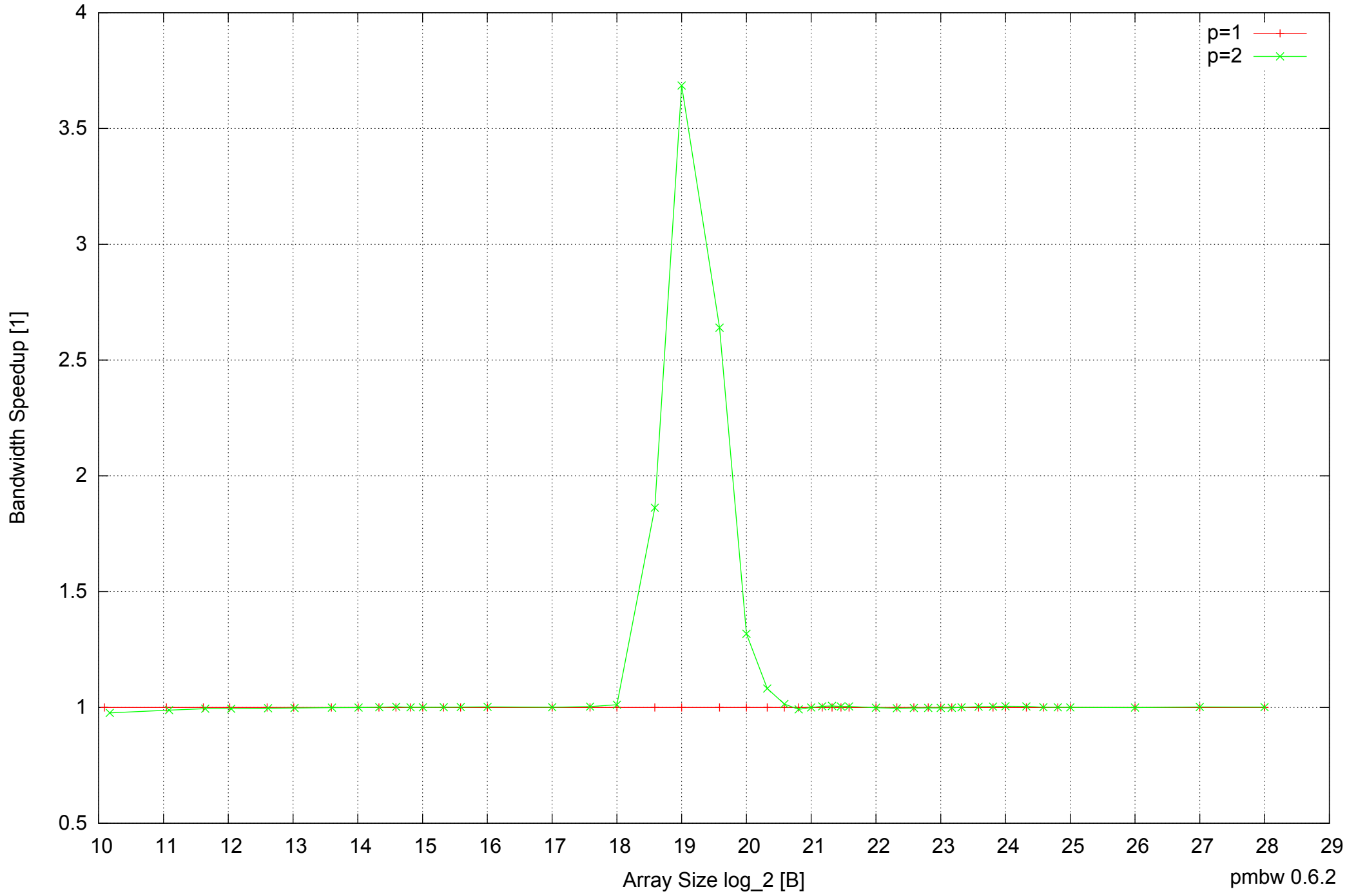
Intel Mobile Pentium III-M 512MB - Speedup of Parallel Memory Bandwidth - ScanWrite32IndexSimpleLoop
