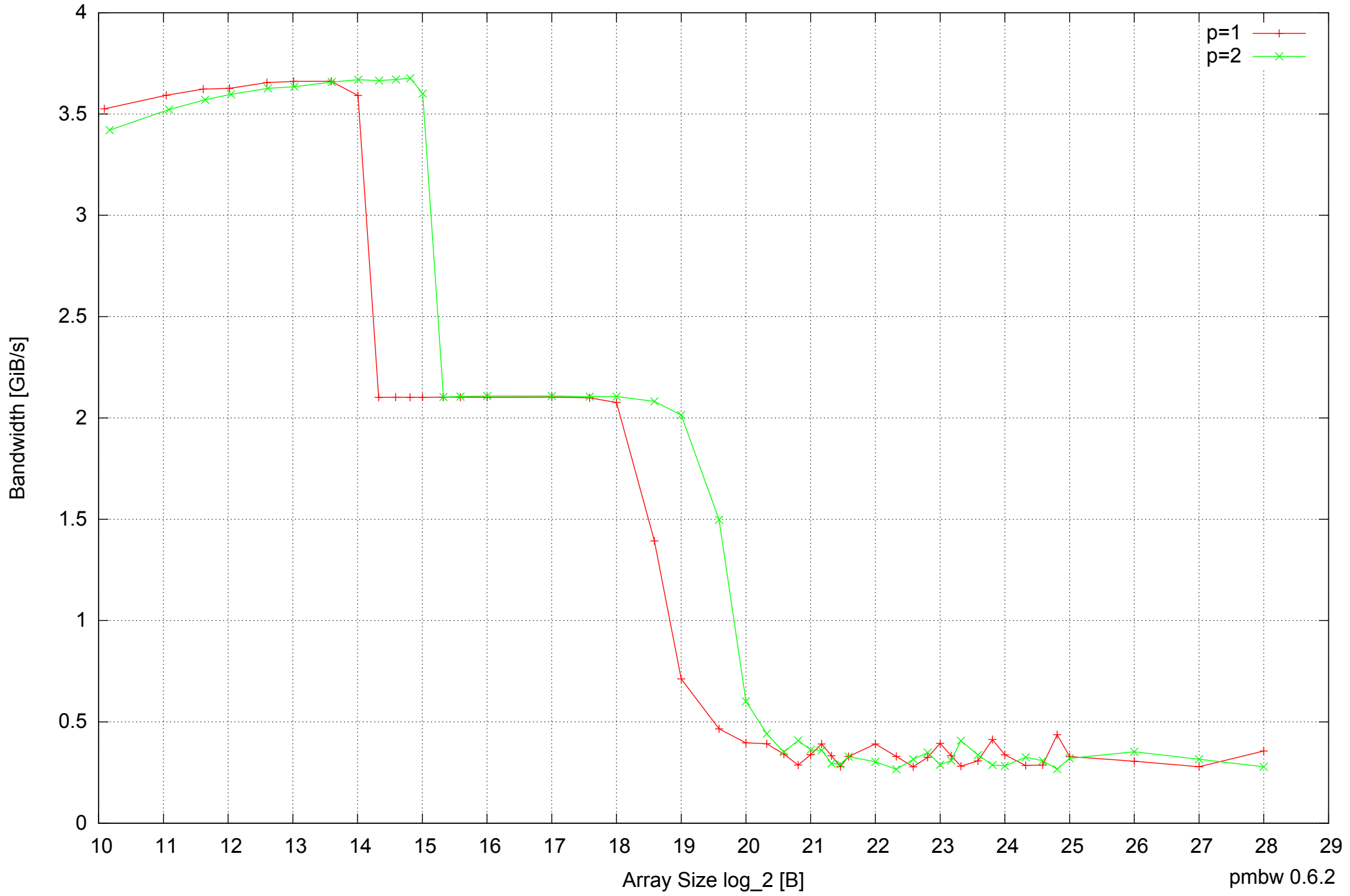
Intel Mobile Pentium III-M 512MB - Parallel Memory Bandwidth - ScanRead32IndexUnrollLoop
