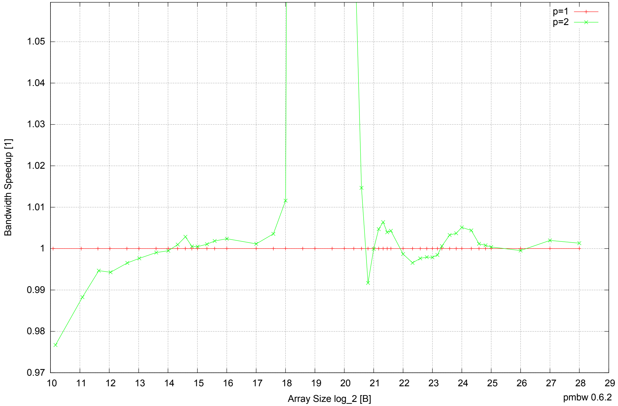
Intel Mobile Pentium III-M 512MB - Speedup of Parallel Memory Bandwidth (enlarged) - ScanWrite32IndexSimpleLoop
