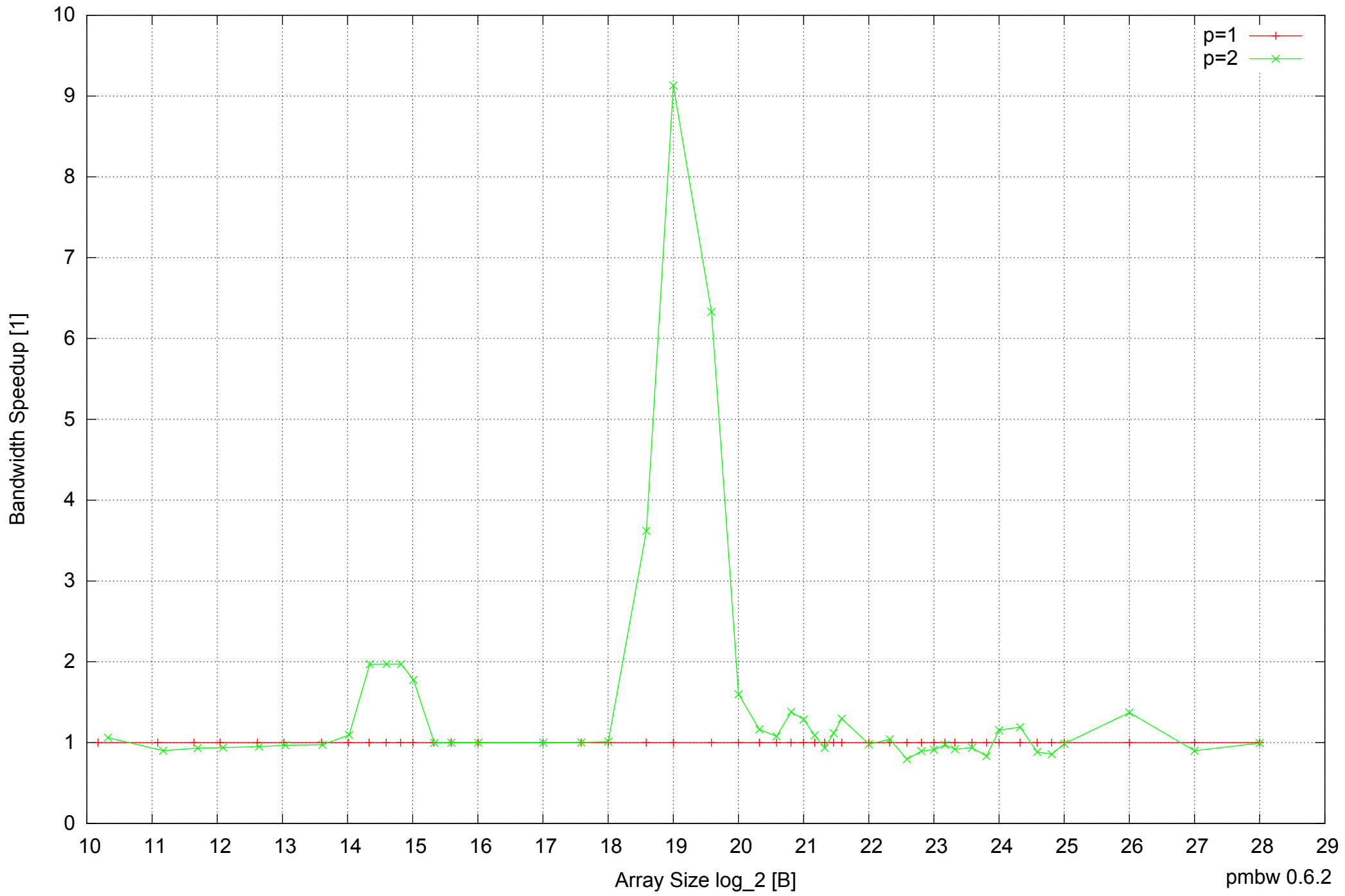
Intel Mobile Pentium III-M 512MB - Speedup of Parallel Memory Bandwidth - ScanRead128PtrUnrollLoop
