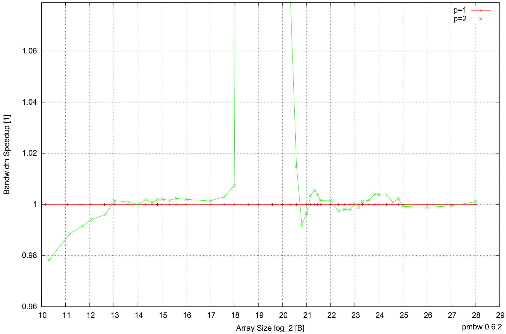
Intel Mobile Pentium III-M 512MB - Speedup of Parallel Memory Bandwidth (enlarged) - ScanWrite64PtrSimpleLoop
