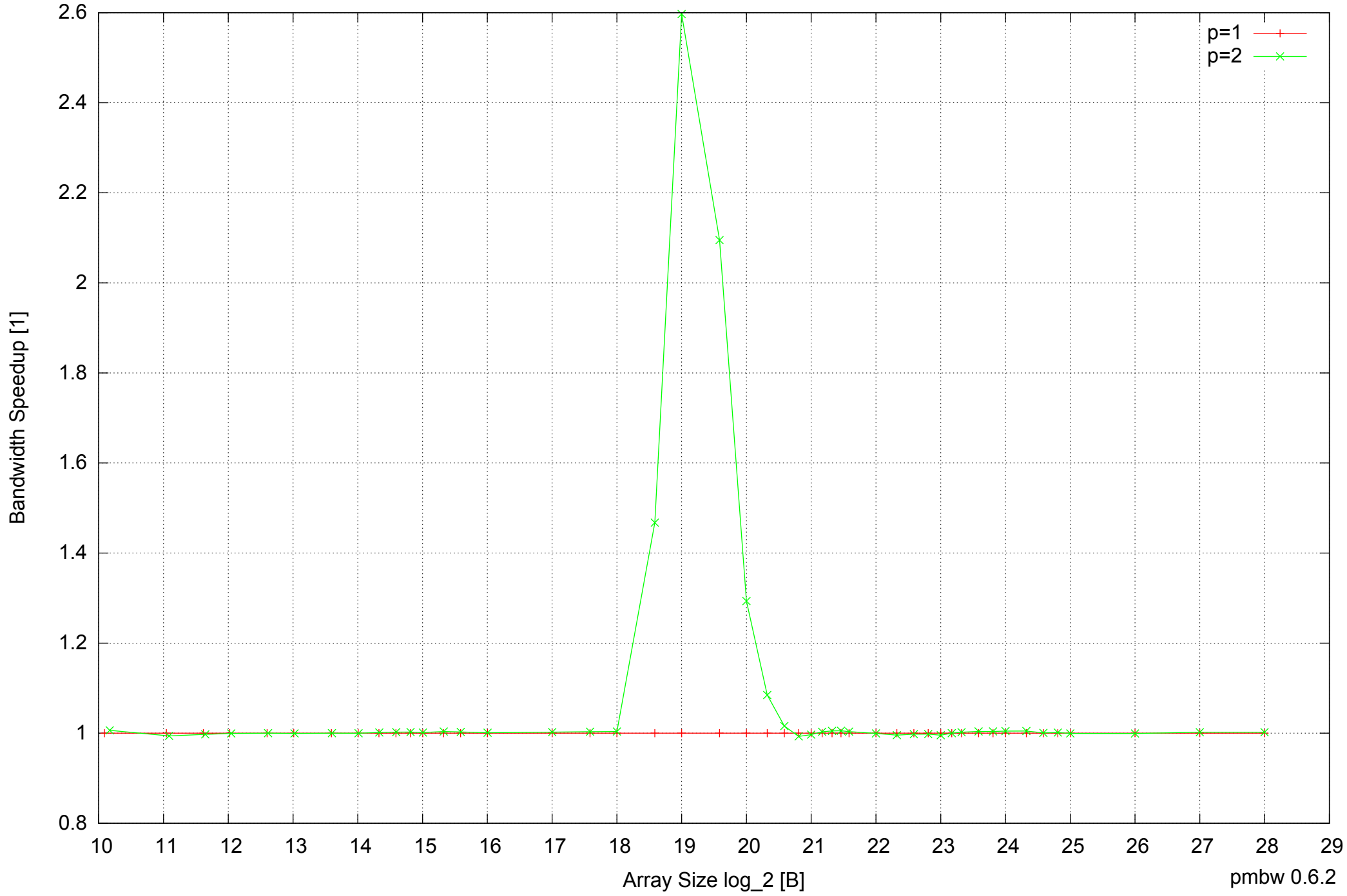
Intel Mobile Pentium III-M 512MB - Speedup of Parallel Memory Bandwidth - ScanWrite32PtrSimpleLoop
