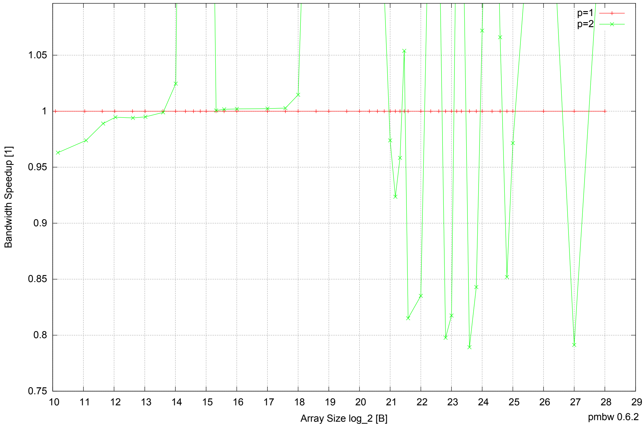
Intel Mobile Pentium III-M 512MB - Speedup of Parallel Memory Bandwidth (enlarged) - ScanRead32PtrUnrollLoop
