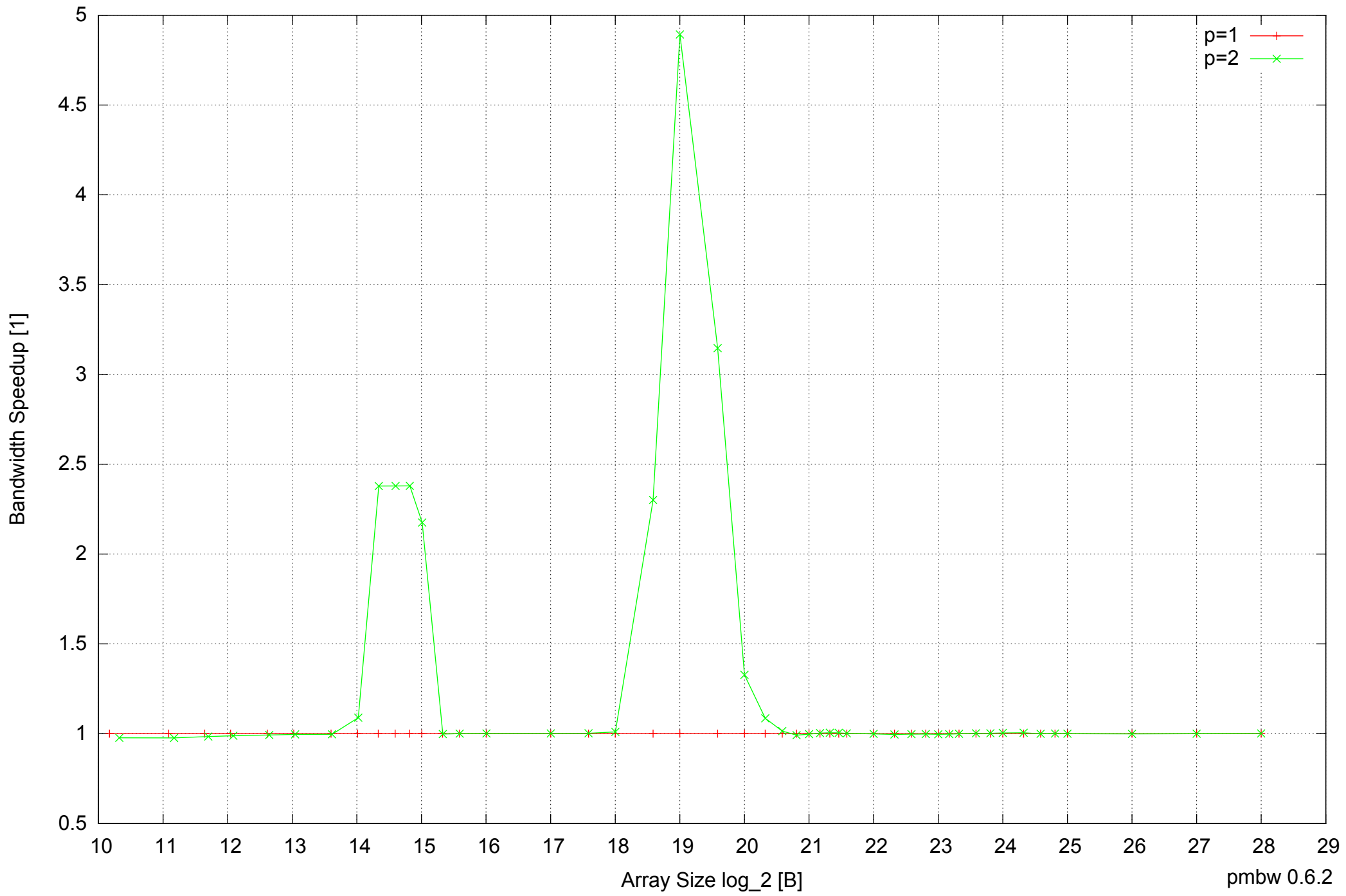
Intel Mobile Pentium III-M 512MB - Speedup of Parallel Memory Bandwidth - ScanWrite64PtrUnrollLoop
