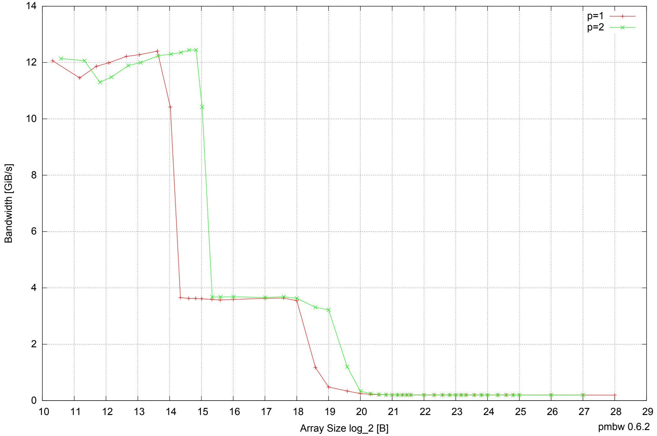
Intel Mobile Pentium III-M 512MB - Parallel Memory Bandwidth - ScanWrite128PtrUnrollLoop
