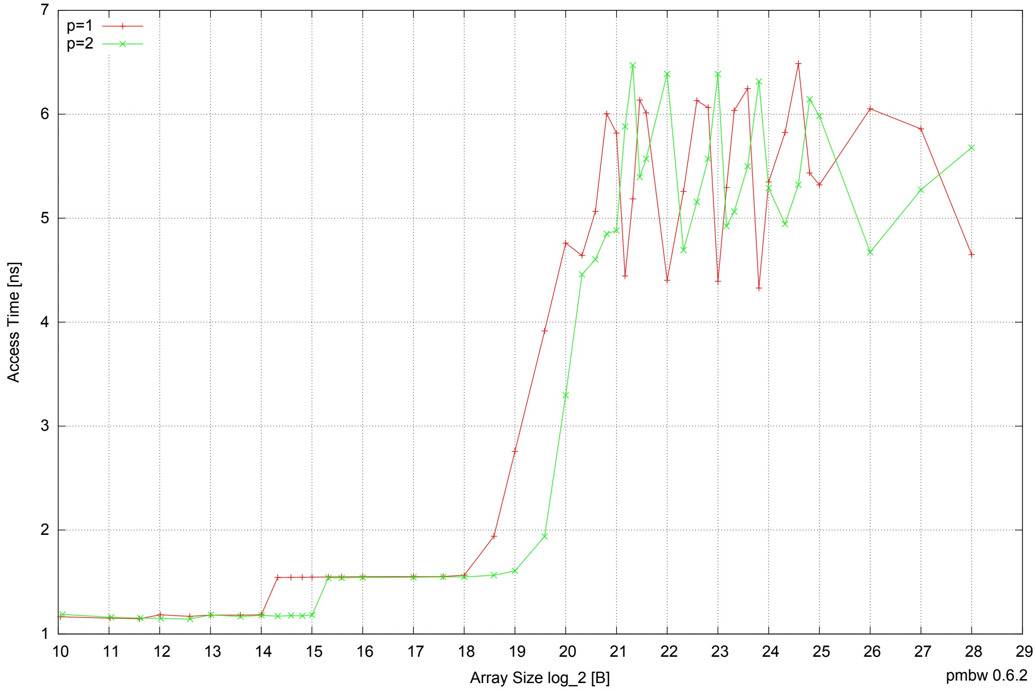
Intel Mobile Pentium III-M 512MB - Parallel Memory Access Time - ScanRead16PtrUnrollLoop
