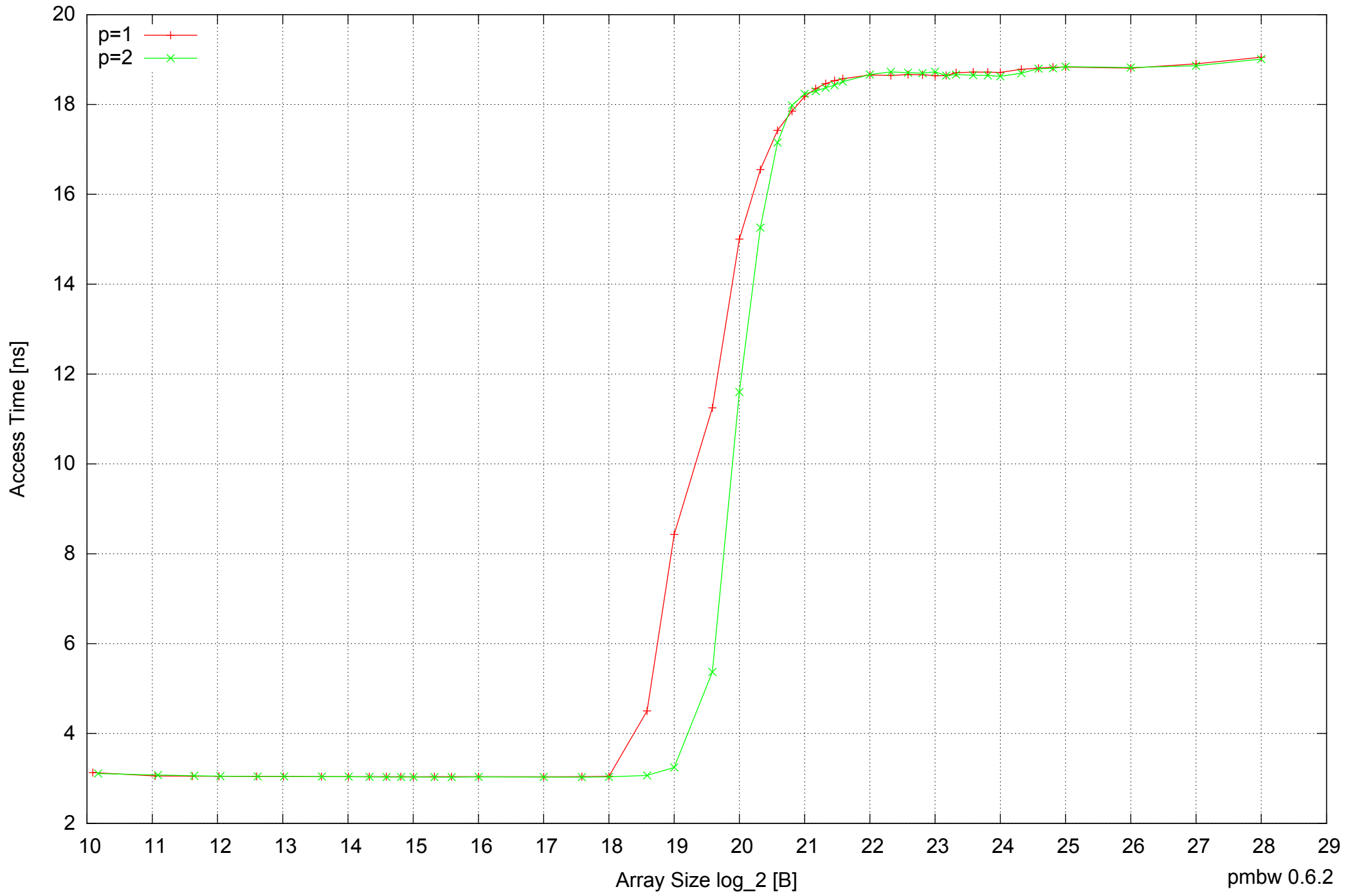
Intel Mobile Pentium III-M 512MB - Parallel Memory Access Time - ScanWrite32PtrSimpleLoop
