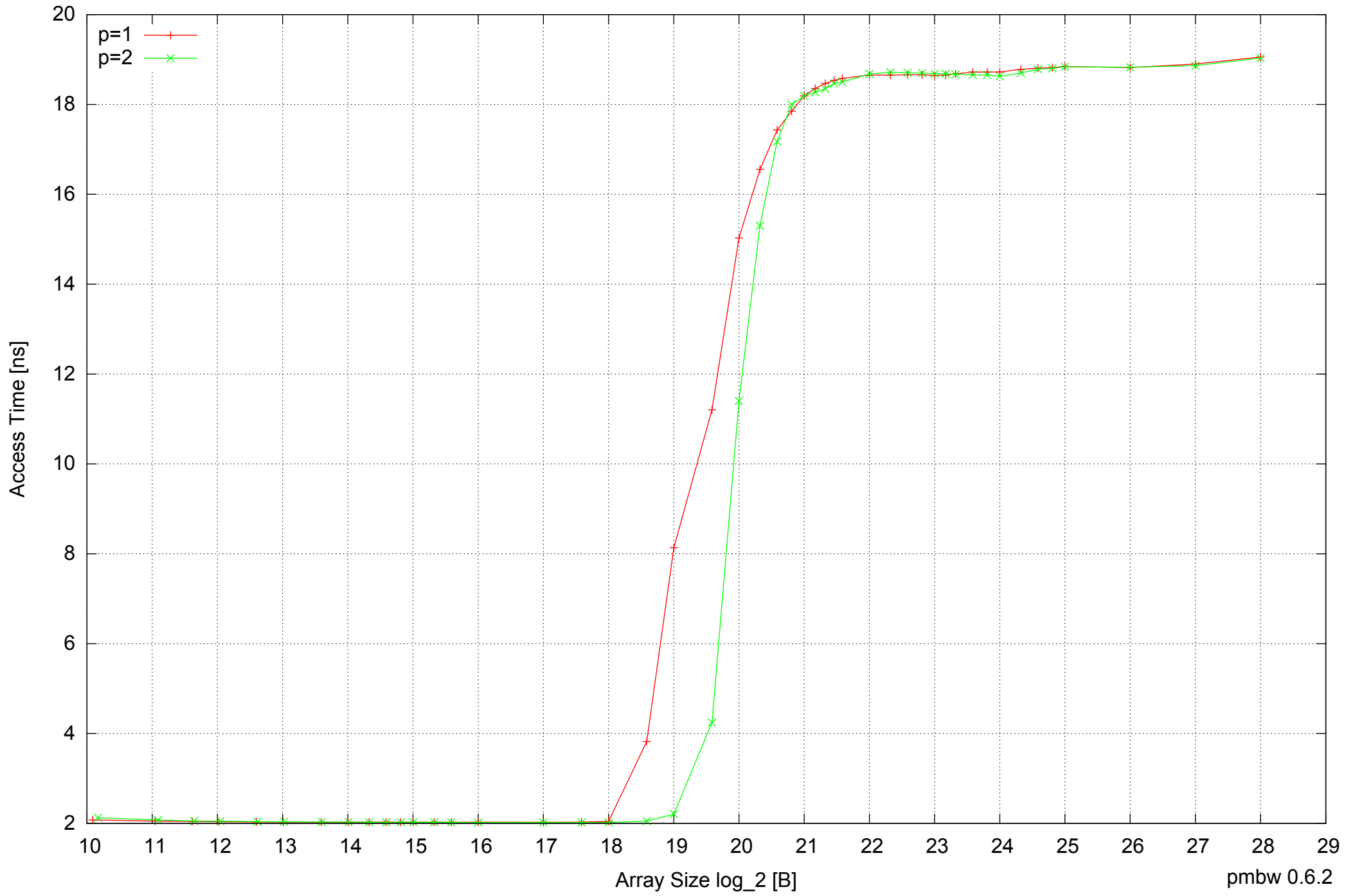
Intel Mobile Pentium III-M 512MB - Parallel Memory Access Time - ScanWrite32IndexSimpleLoop
