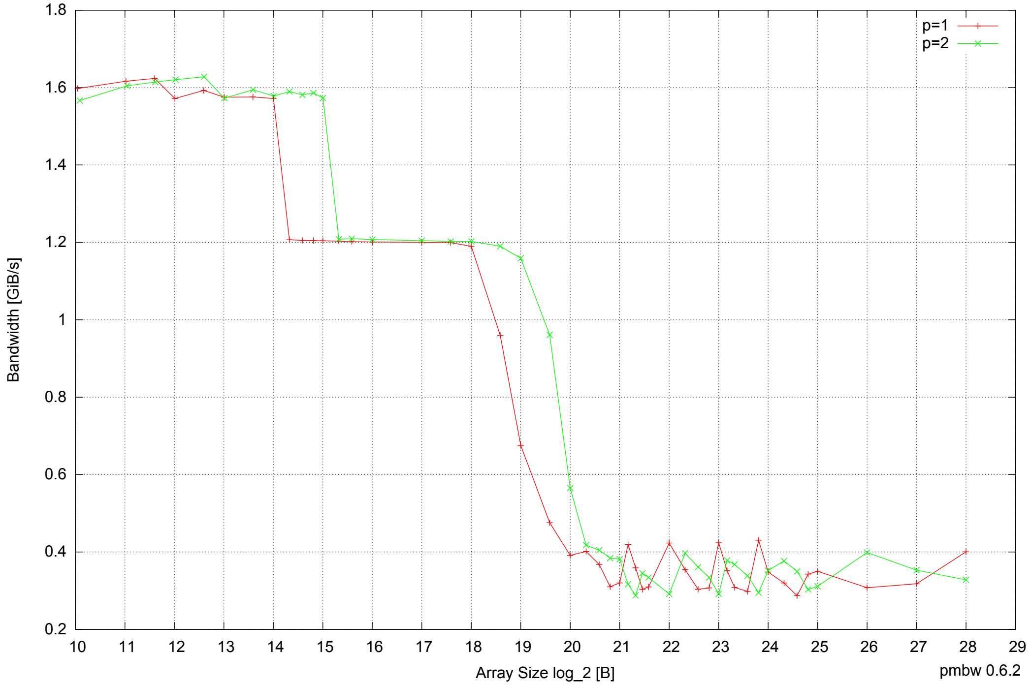
Intel Mobile Pentium III-M 512MB - Parallel Memory Bandwidth - ScanRead16PtrUnrollLoop
