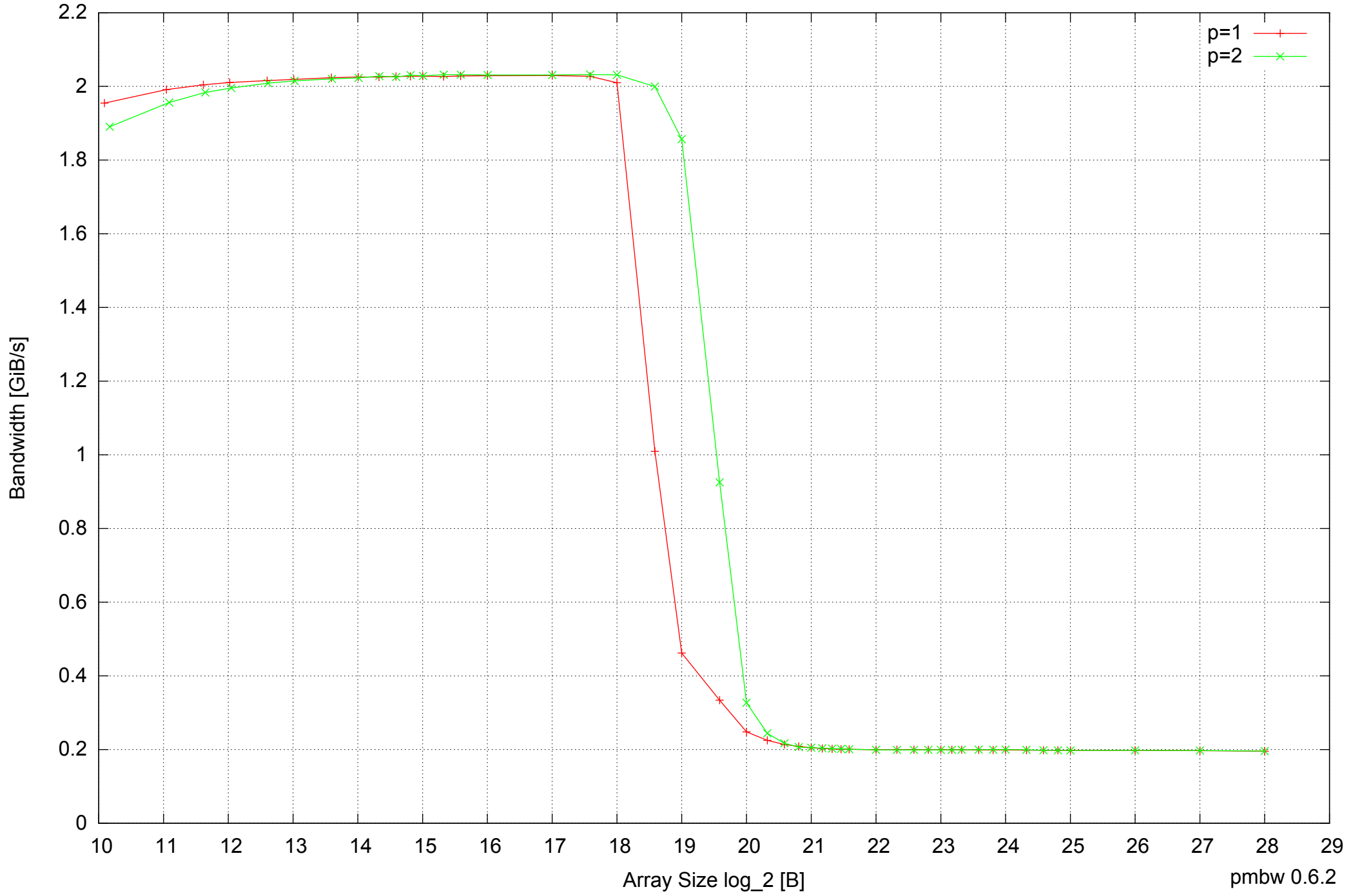
Intel Mobile Pentium III-M 512MB - Parallel Memory Bandwidth - ScanWrite32IndexUnrollLoop
