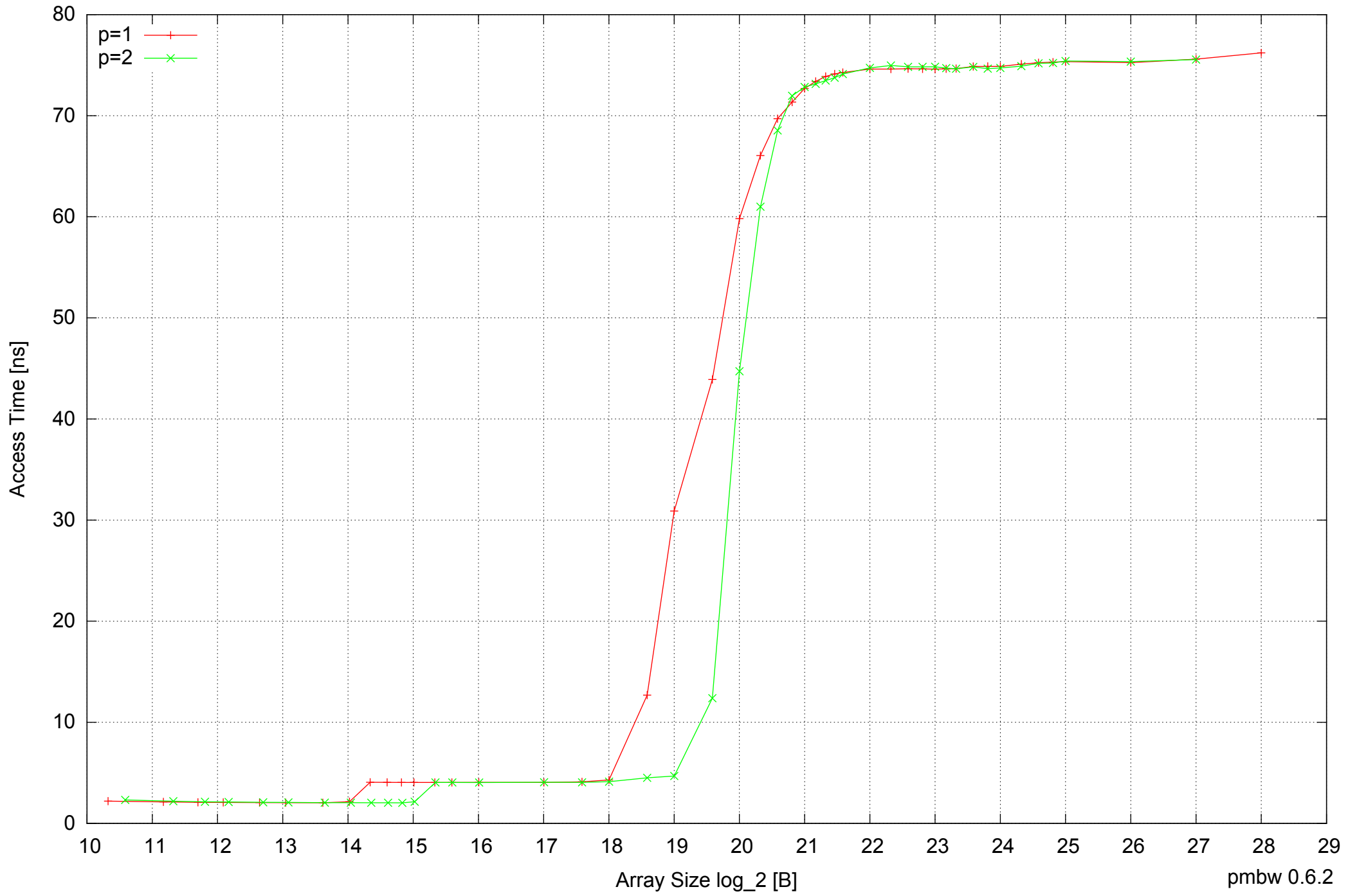
Intel Mobile Pentium III-M 512MB - Parallel Memory Access Time - ScanWrite128PtrSimpleLoop
