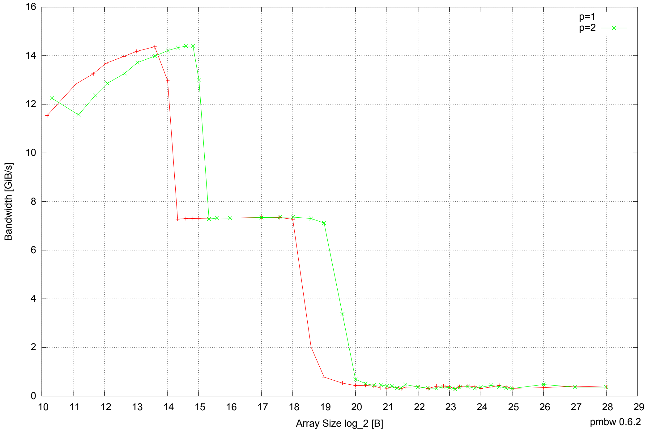
Intel Mobile Pentium III-M 512MB - Parallel Memory Bandwidth - ScanRead128PtrUnrollLoop
