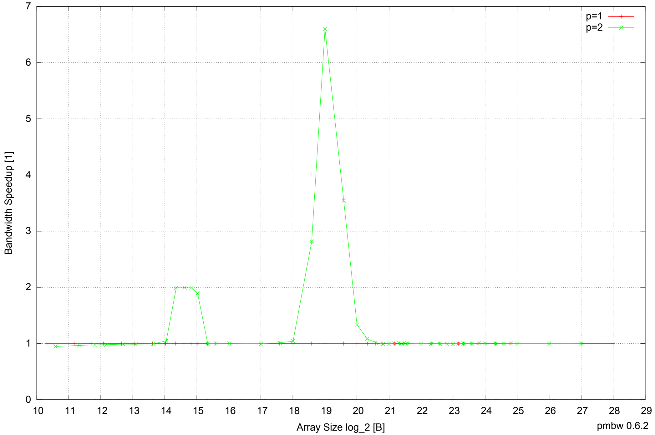
Intel Mobile Pentium III-M 512MB - Speedup of Parallel Memory Bandwidth - ScanWrite128PtrSimpleLoop
