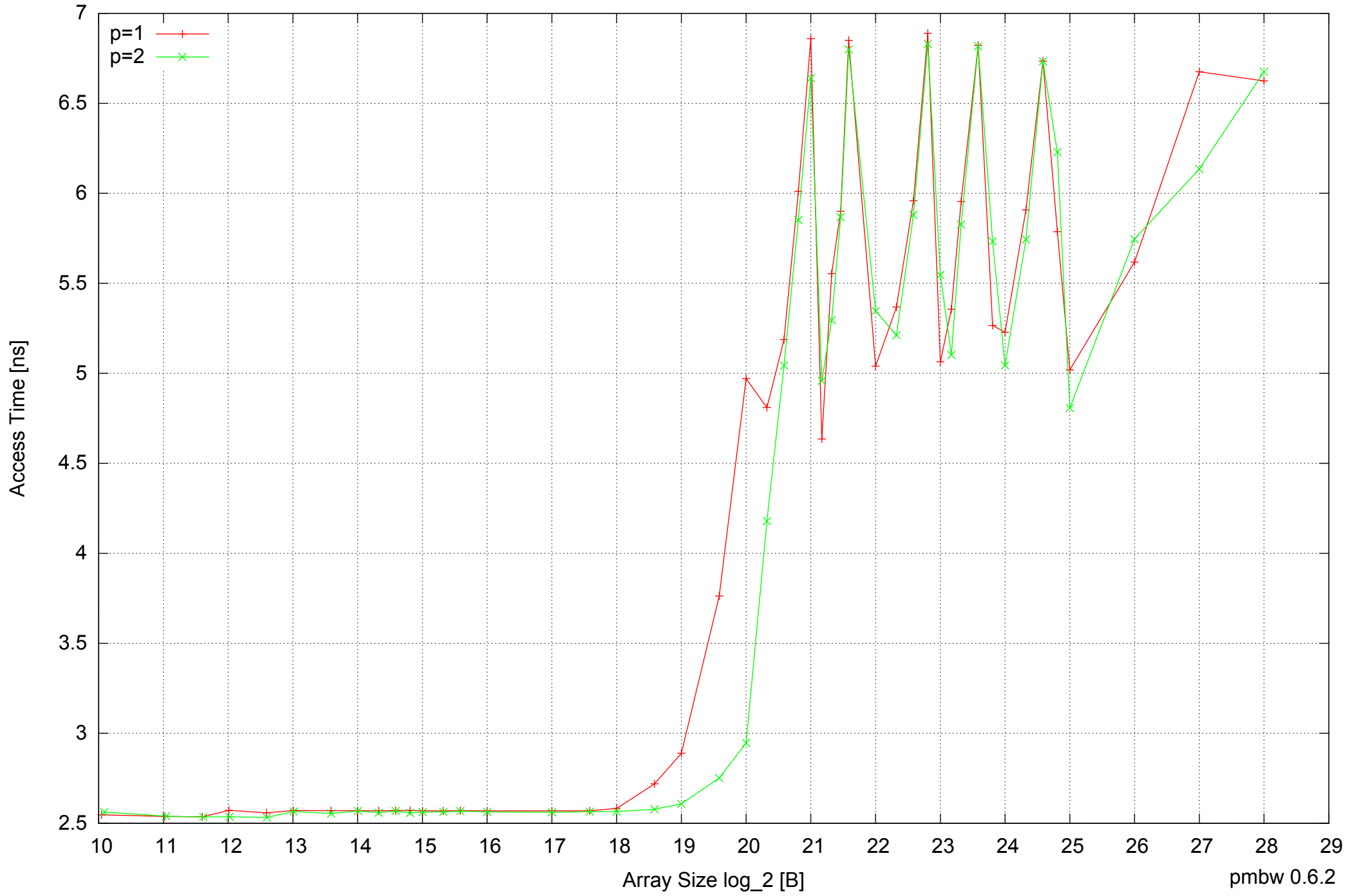
Intel Mobile Pentium III-M 512MB - Parallel Memory Access Time - ScanRead16PtrSimpleLoop
