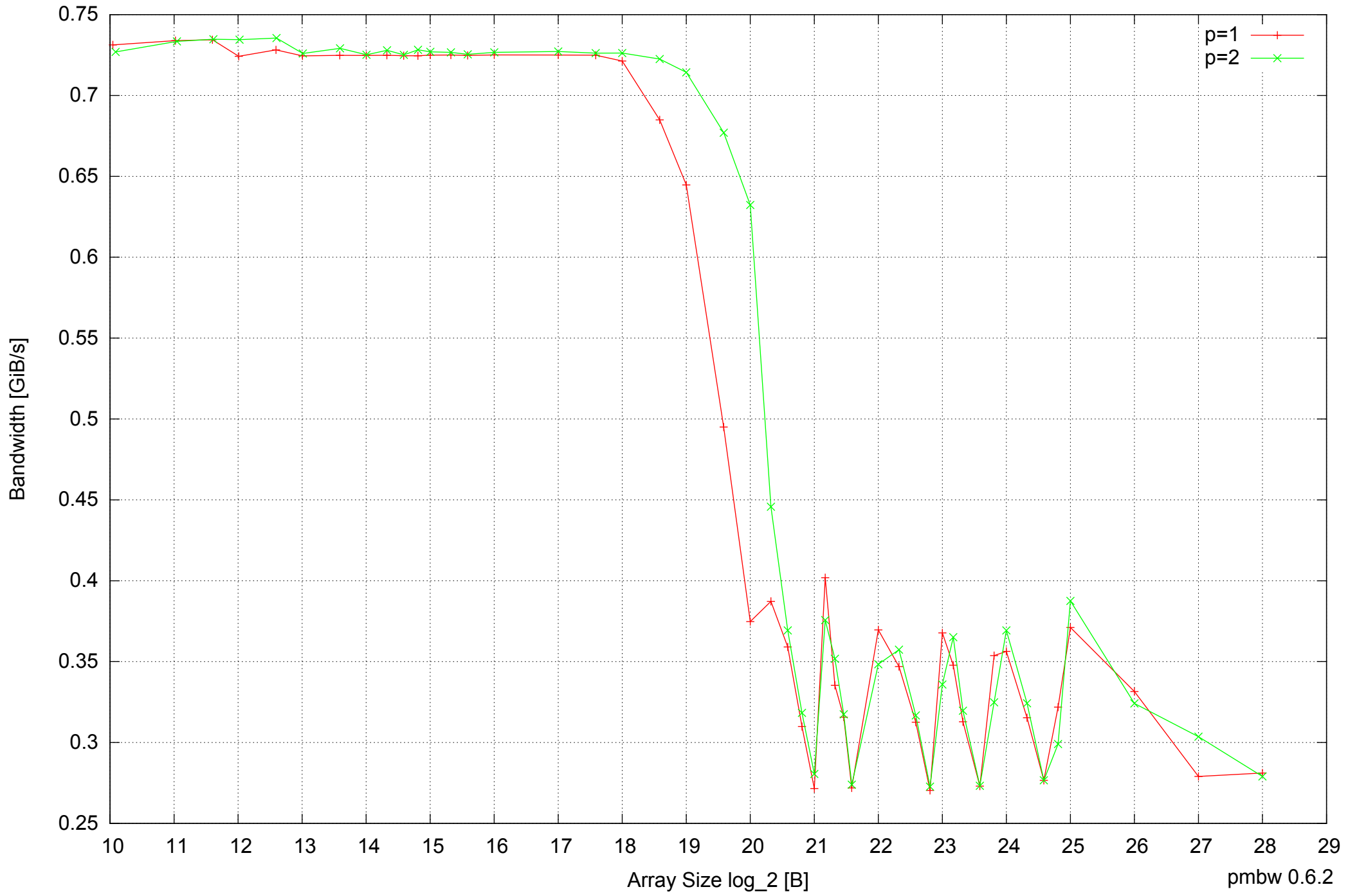
Intel Mobile Pentium III-M 512MB - Parallel Memory Bandwidth - ScanRead16PtrSimpleLoop
