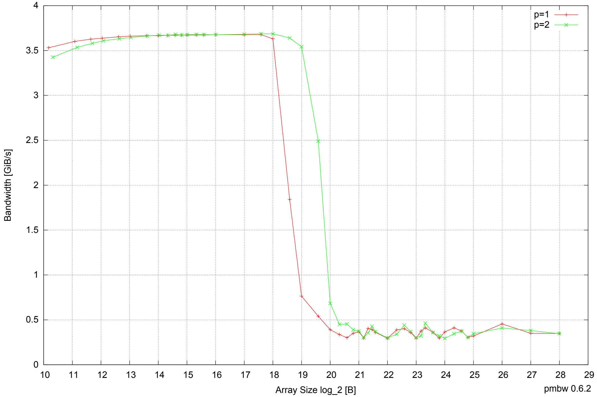
Intel Mobile Pentium III-M 512MB - Parallel Memory Bandwidth - ScanRead64PtrSimpleLoop
