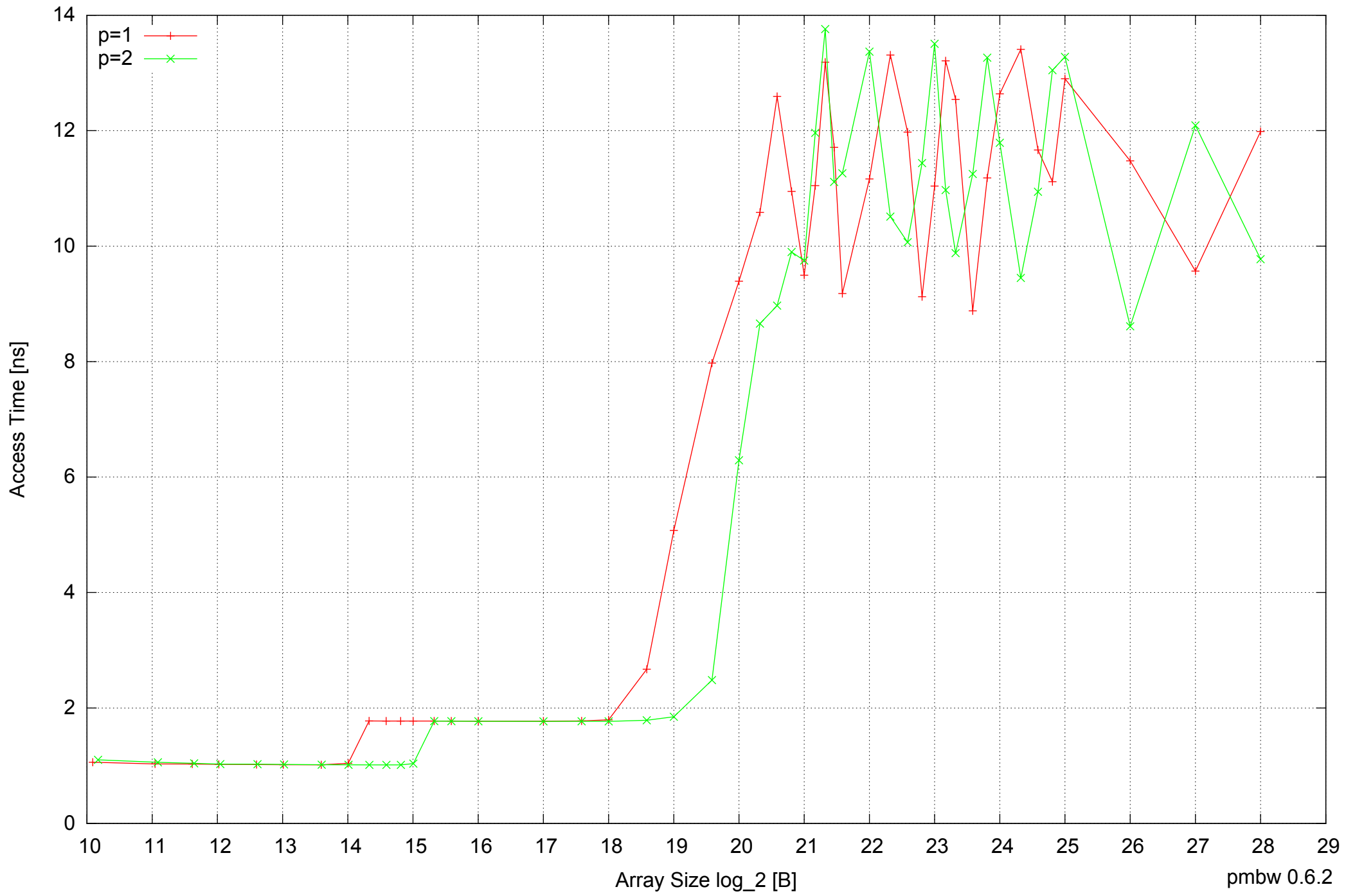
Intel Mobile Pentium III-M 512MB - Parallel Memory Access Time - ScanRead32PtrUnrollLoop
