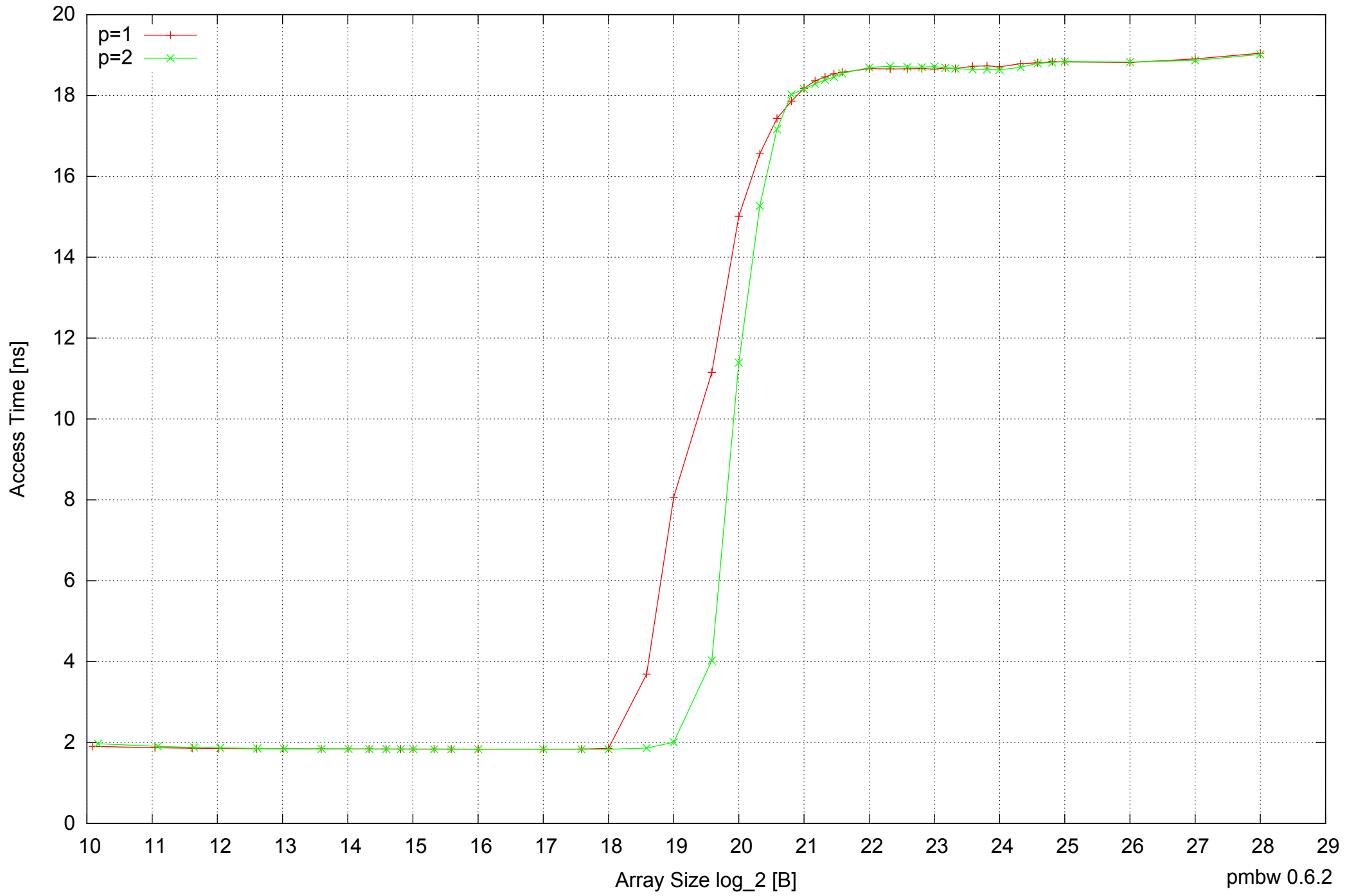
Intel Mobile Pentium III-M 512MB - Parallel Memory Access Time - ScanWrite32IndexUnrollLoop
