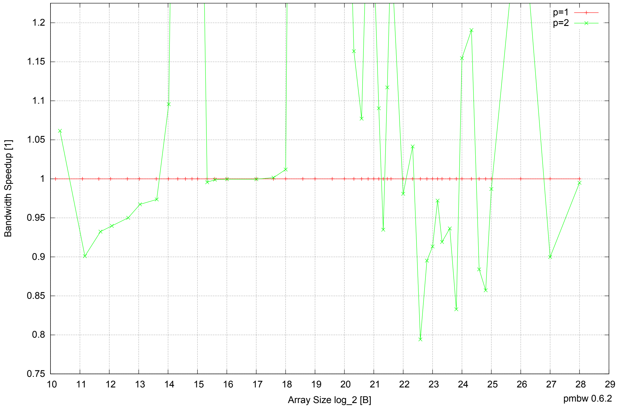
Intel Mobile Pentium III-M 512MB - Speedup of Parallel Memory Bandwidth (enlarged) - ScanRead128PtrUnrollLoop
