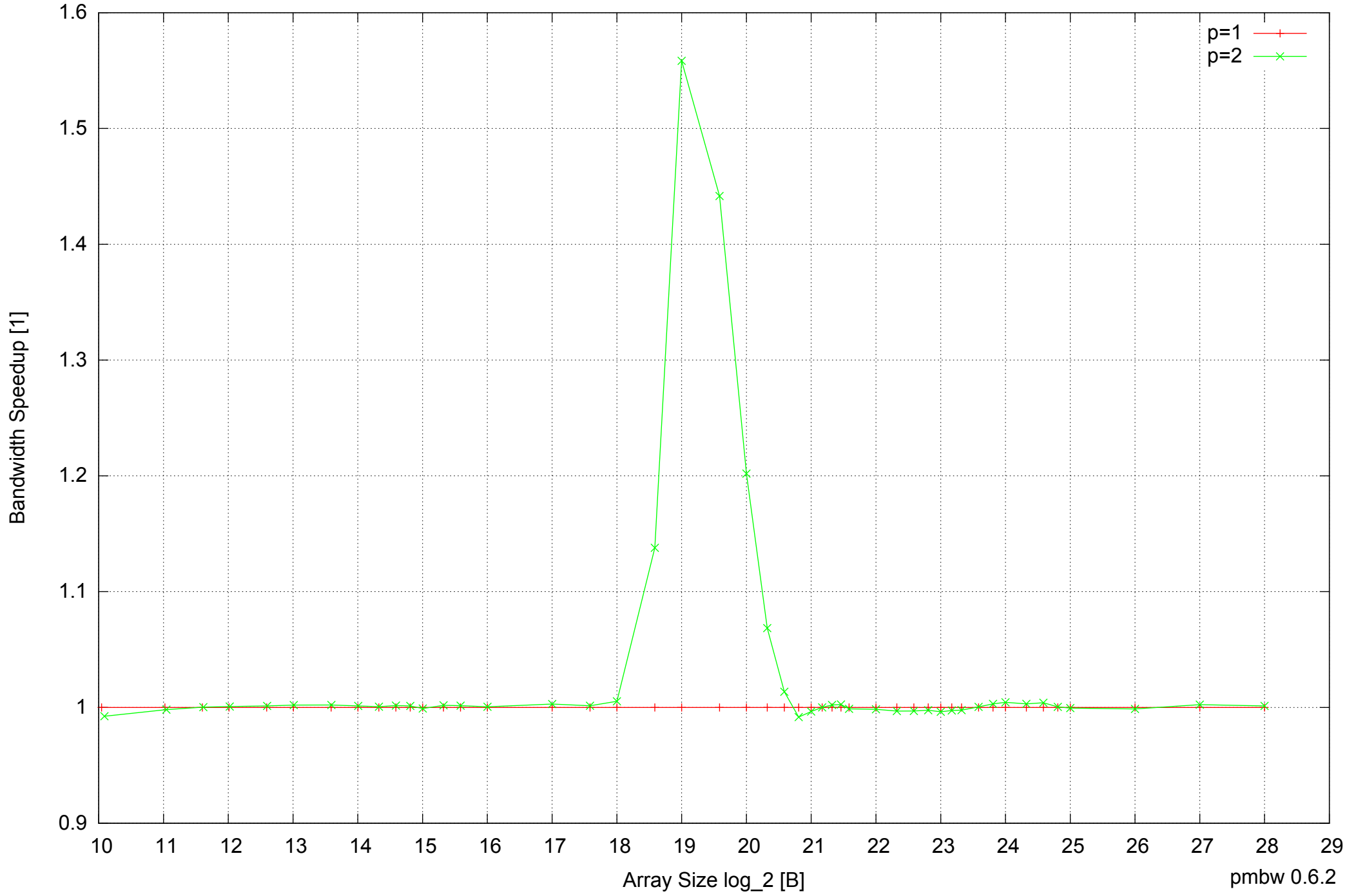
Intel Mobile Pentium III-M 512MB - Speedup of Parallel Memory Bandwidth - ScanWrite16PtrSimpleLoop
