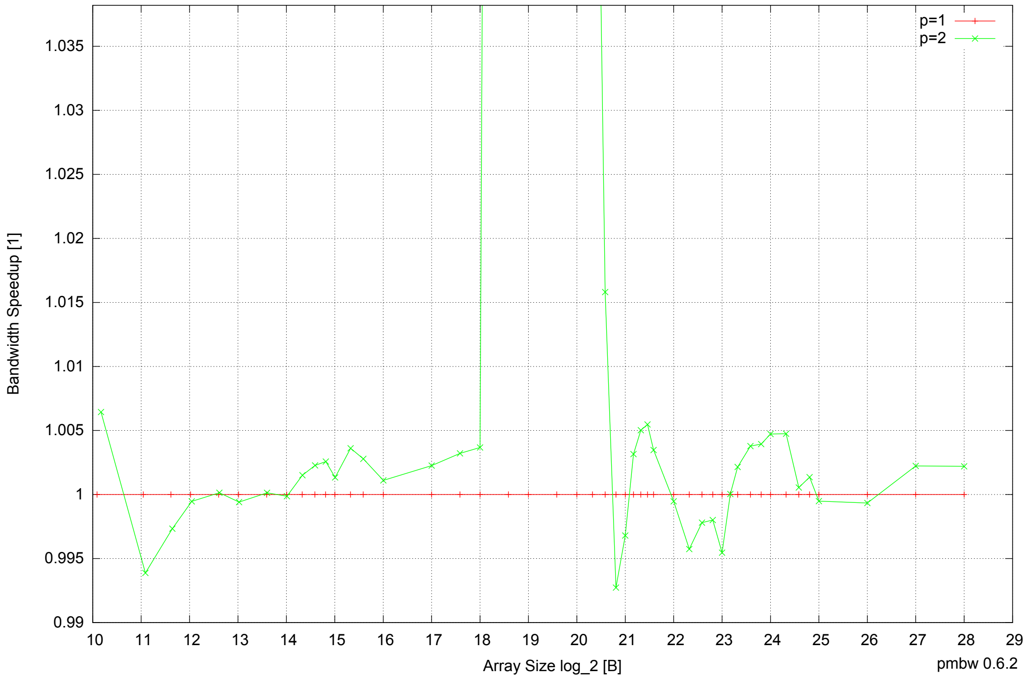
Intel Mobile Pentium III-M 512MB - Speedup of Parallel Memory Bandwidth (enlarged) - ScanWrite32PtrSimpleLoop
