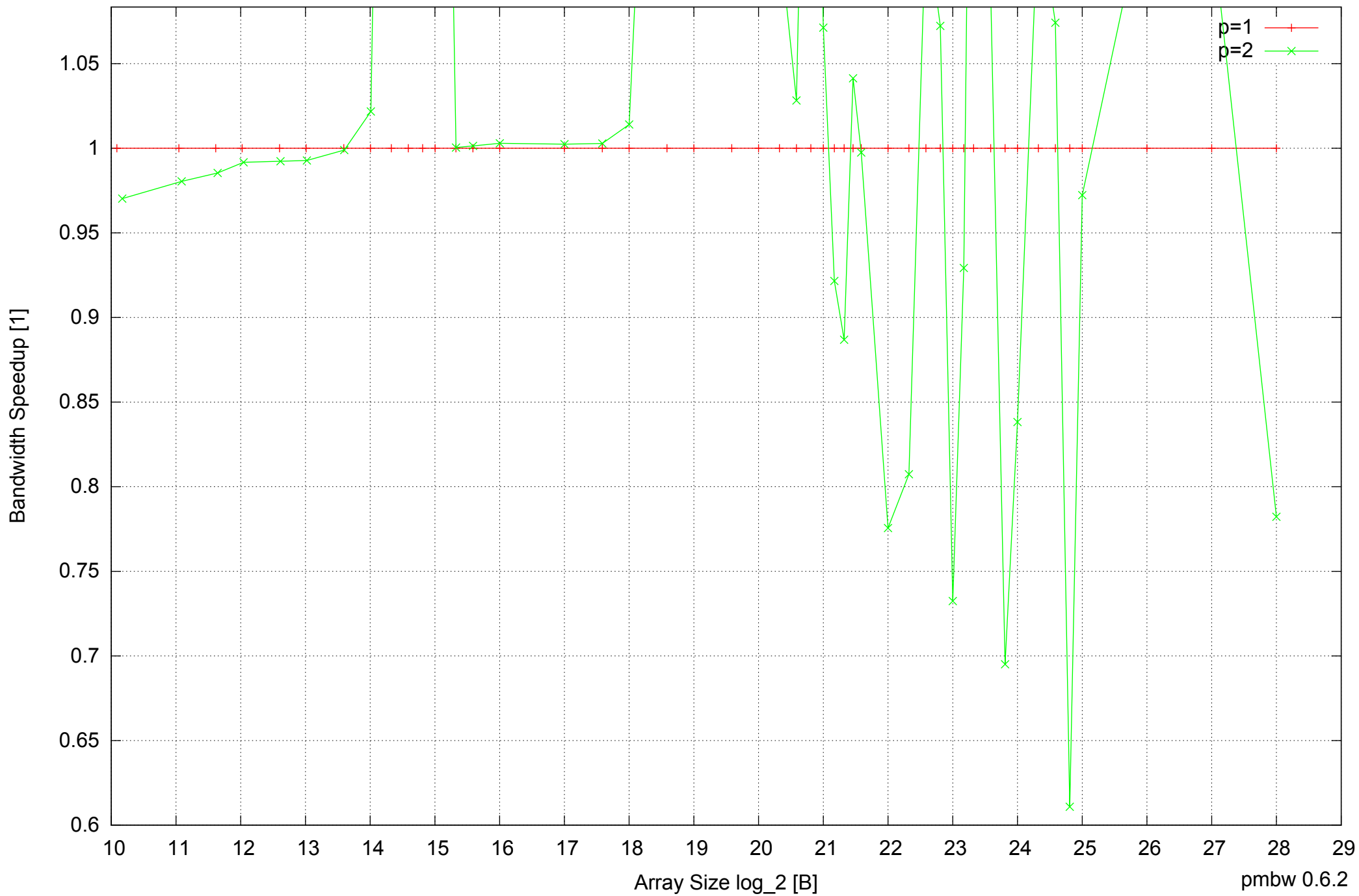
Intel Mobile Pentium III-M 512MB - Speedup of Parallel Memory Bandwidth (enlarged) - ScanRead32IndexUnrollLoop
