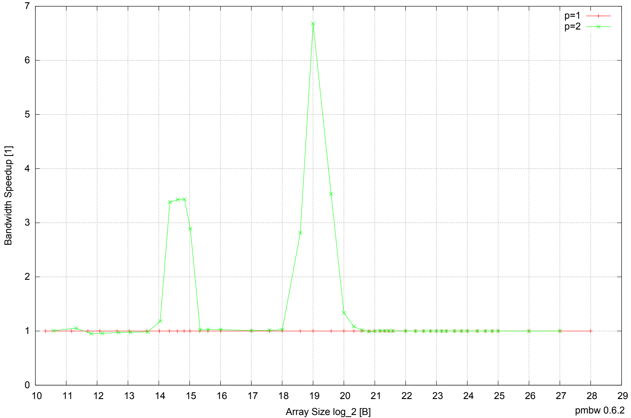
Intel Mobile Pentium III-M 512MB - Speedup of Parallel Memory Bandwidth - ScanWrite128PtrUnrollLoop
