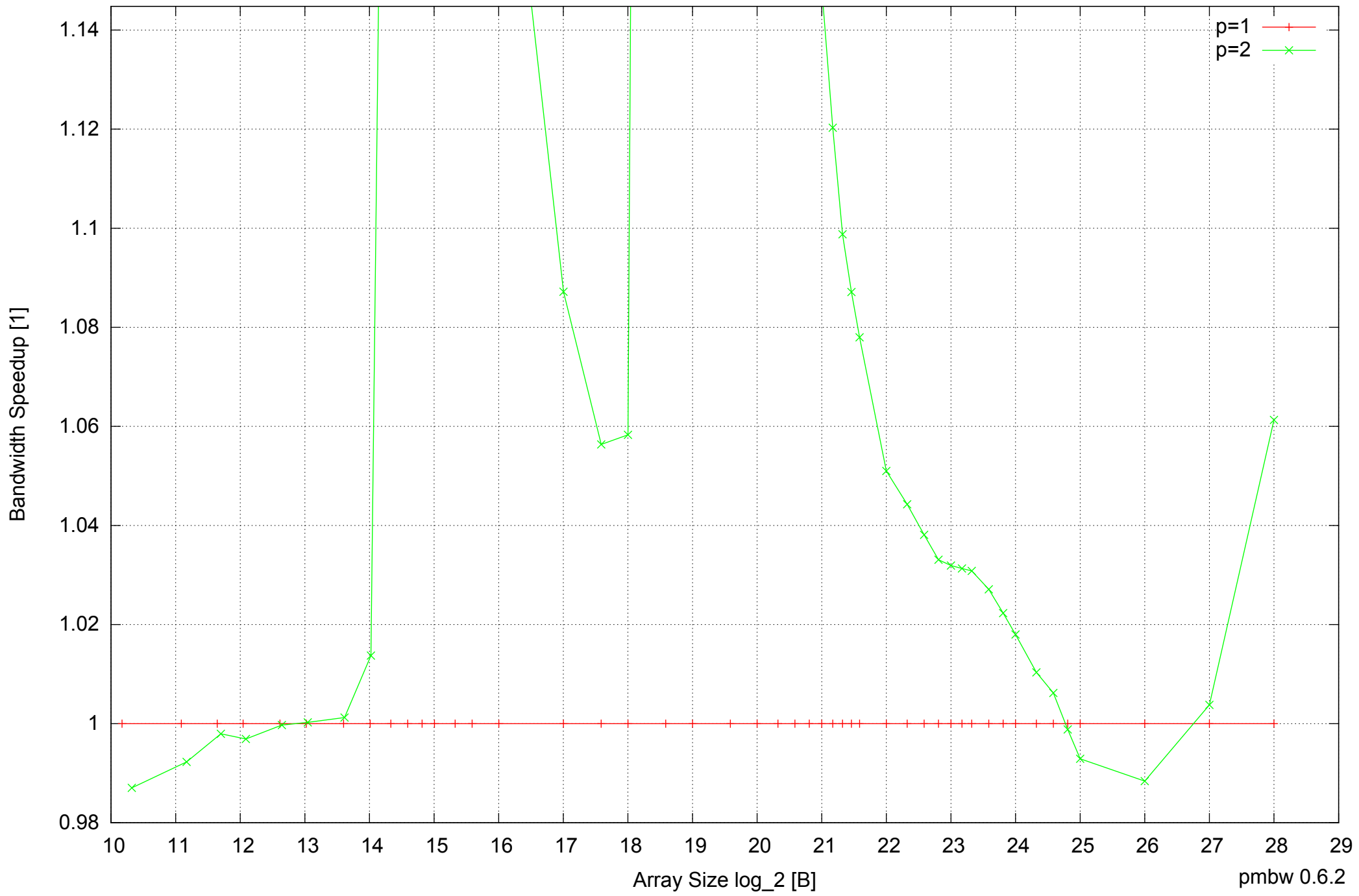
Intel Mobile Pentium III-M 512MB - Speedup of Parallel Memory Bandwidth (enlarged) - PermRead32SimpleLoop
