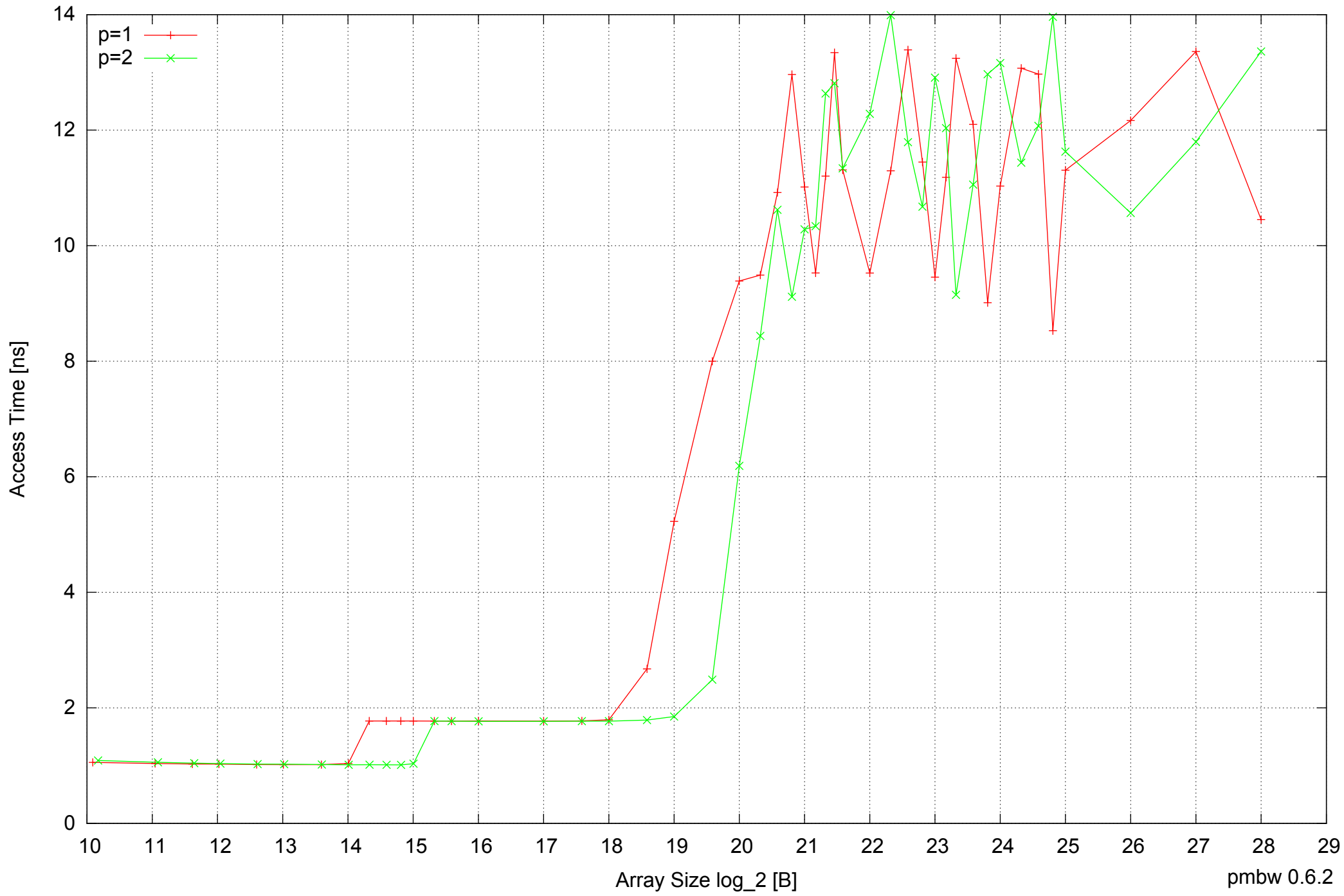
Intel Mobile Pentium III-M 512MB - Parallel Memory Access Time - ScanRead32IndexUnrollLoop
