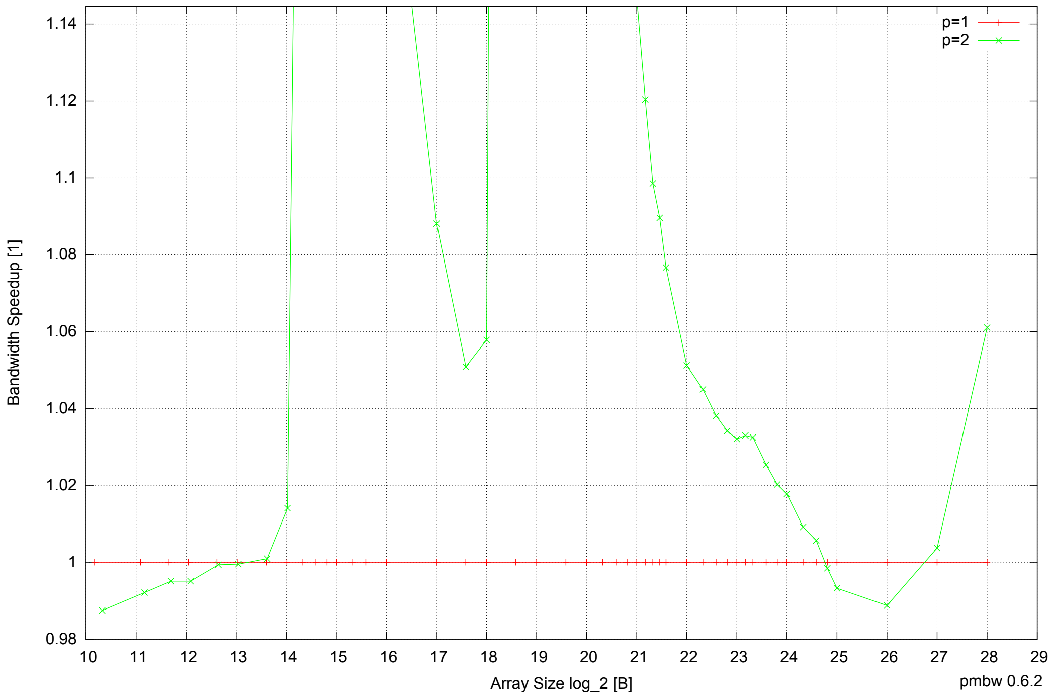
Intel Mobile Pentium III-M 512MB - Speedup of Parallel Memory Bandwidth (enlarged) - PermRead32UnrollLoop
