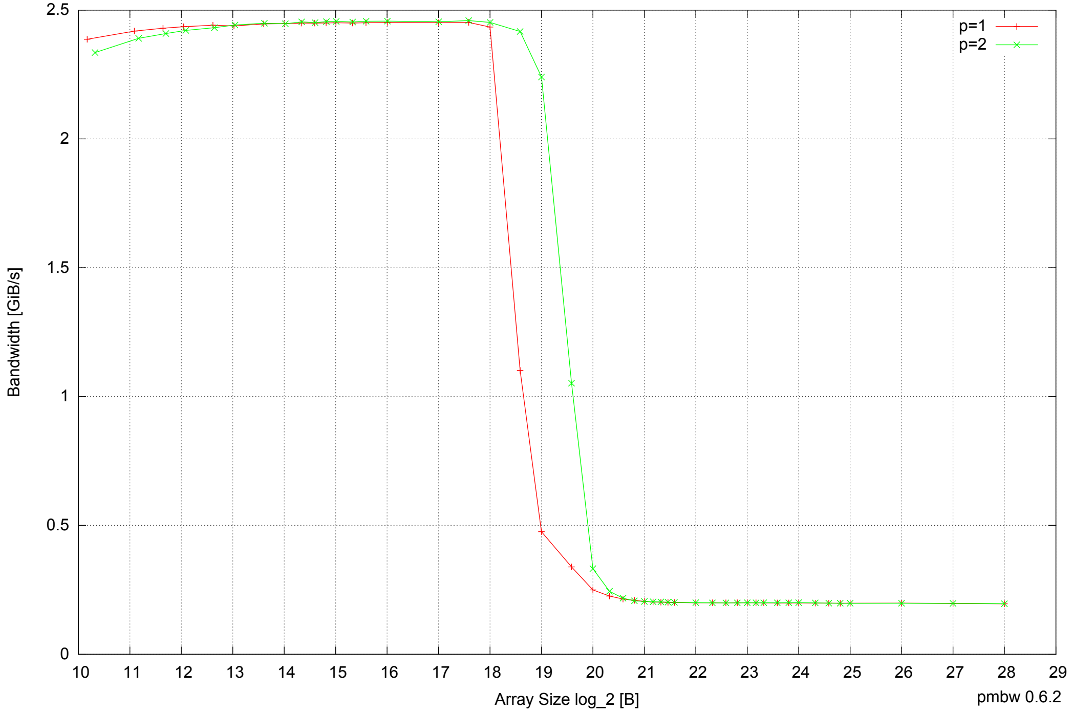
Intel Mobile Pentium III-M 512MB - Parallel Memory Bandwidth - ScanWrite64PtrSimpleLoop
