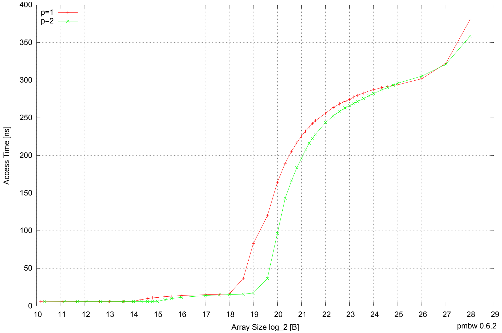
Intel Mobile Pentium III-M 512MB - Parallel Memory Access Time - PermRead32SimpleLoop
