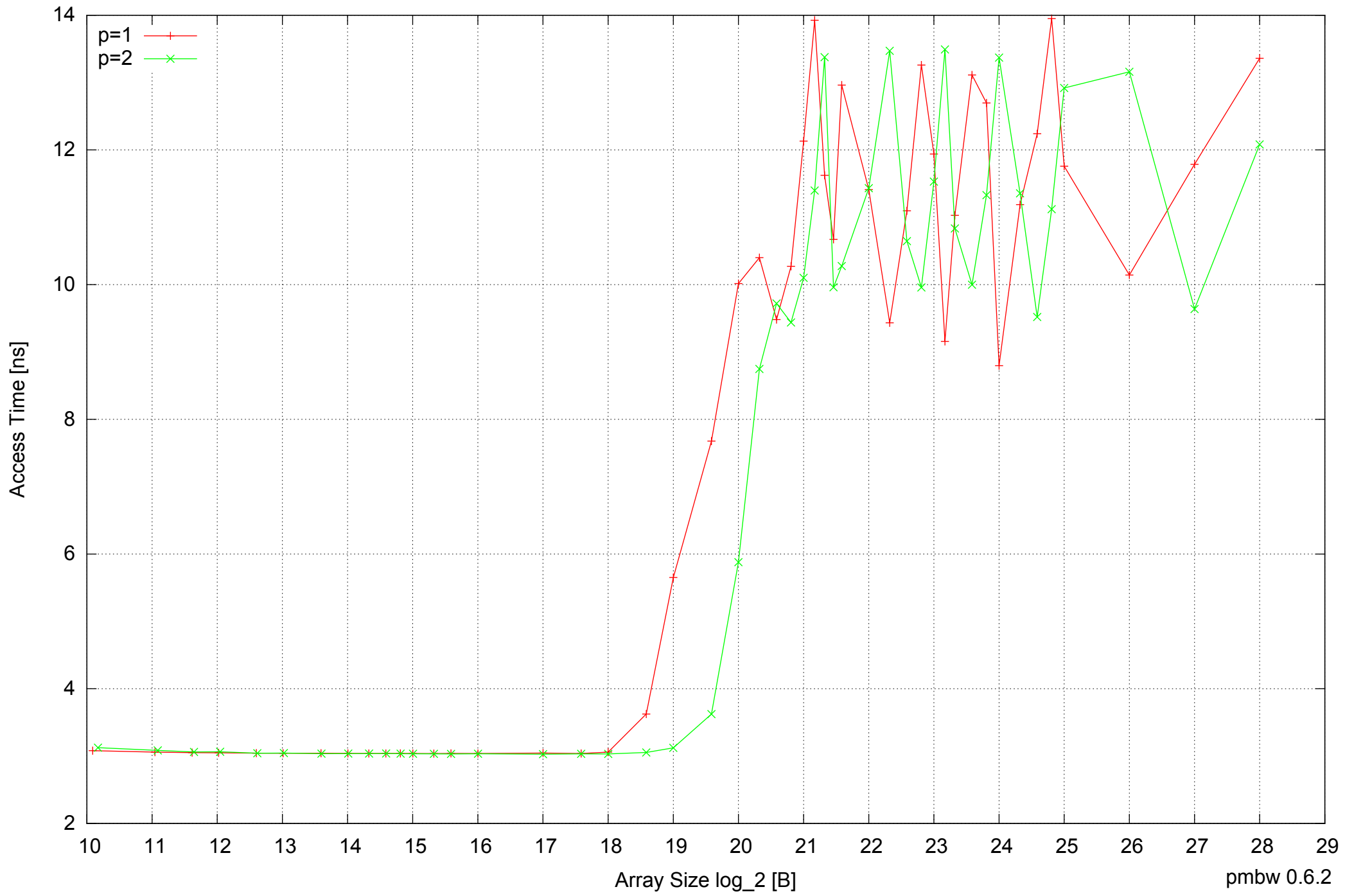
Intel Mobile Pentium III-M 512MB - Parallel Memory Access Time - ScanRead32IndexSimpleLoop
