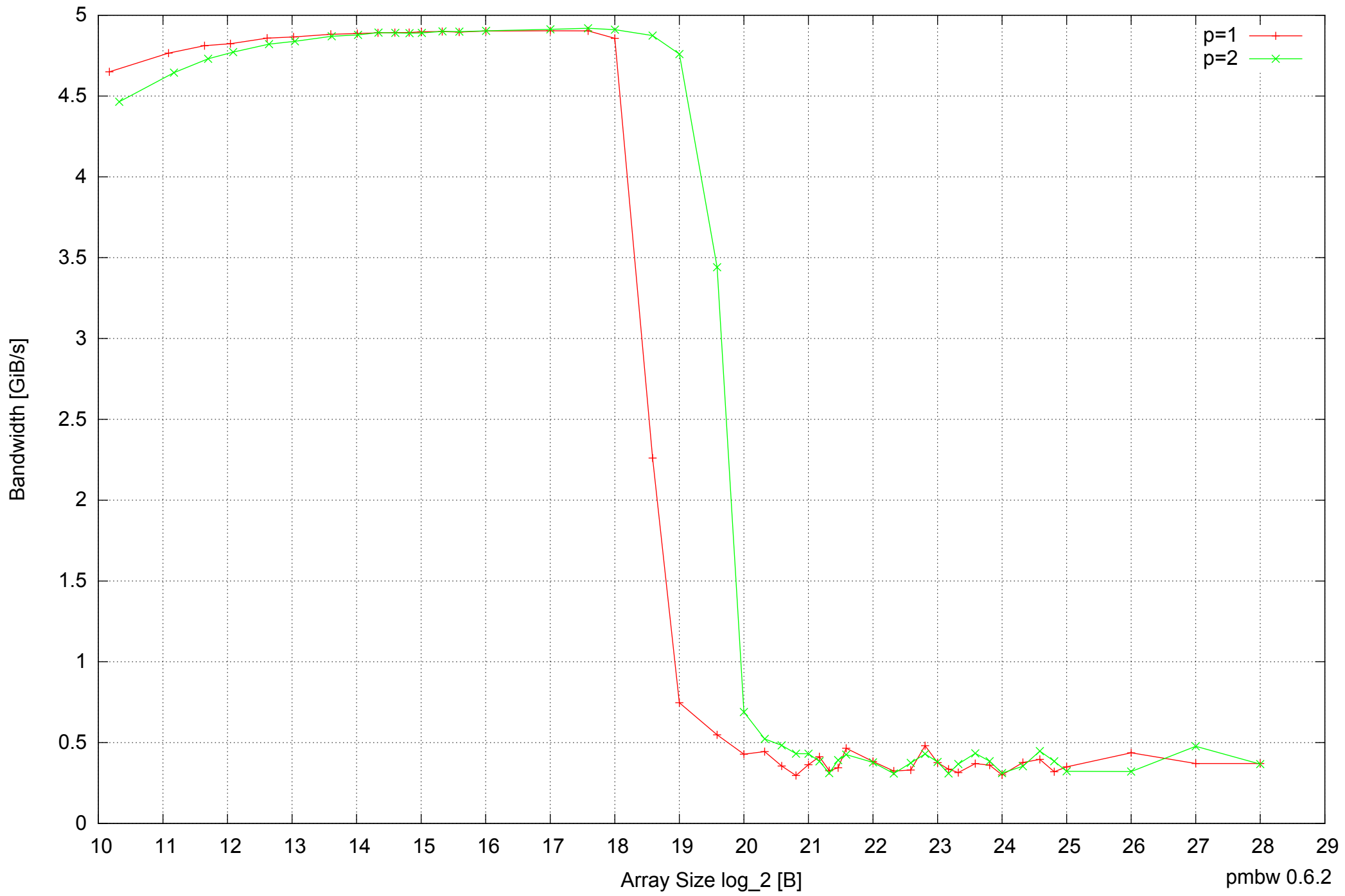
Intel Mobile Pentium III-M 512MB - Parallel Memory Bandwidth - ScanRead128PtrSimpleLoop
