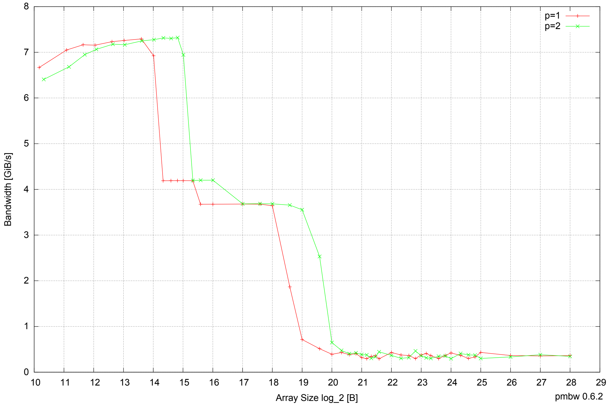
Intel Mobile Pentium III-M 512MB - Parallel Memory Bandwidth - ScanRead64PtrUnrollLoop
