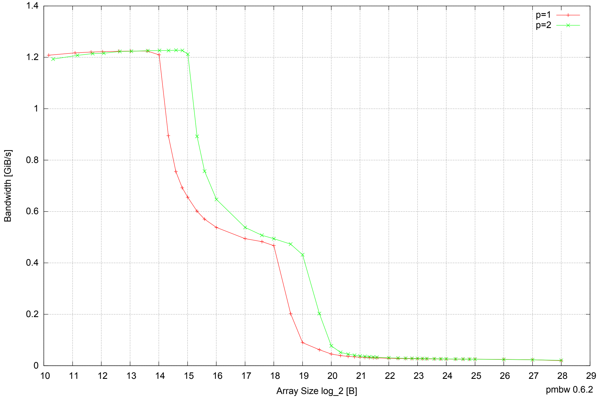
Intel Mobile Pentium III-M 512MB - Parallel Memory Bandwidth - PermRead32UnrollLoop
