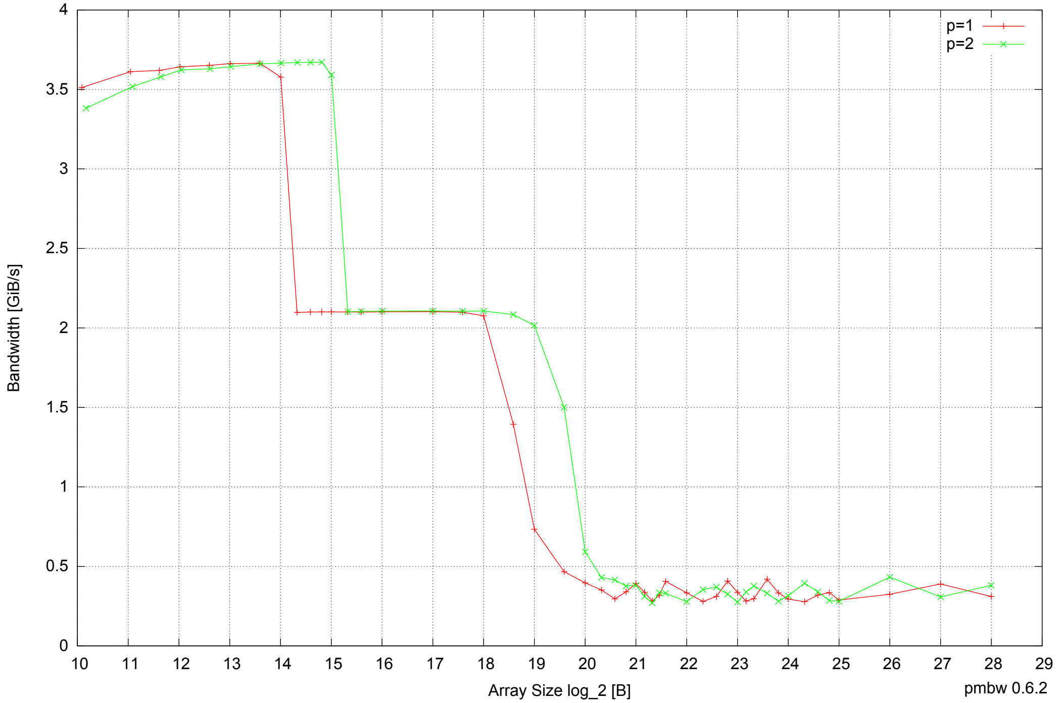
Intel Mobile Pentium III-M 512MB - Parallel Memory Bandwidth - ScanRead32PtrUnrollLoop
