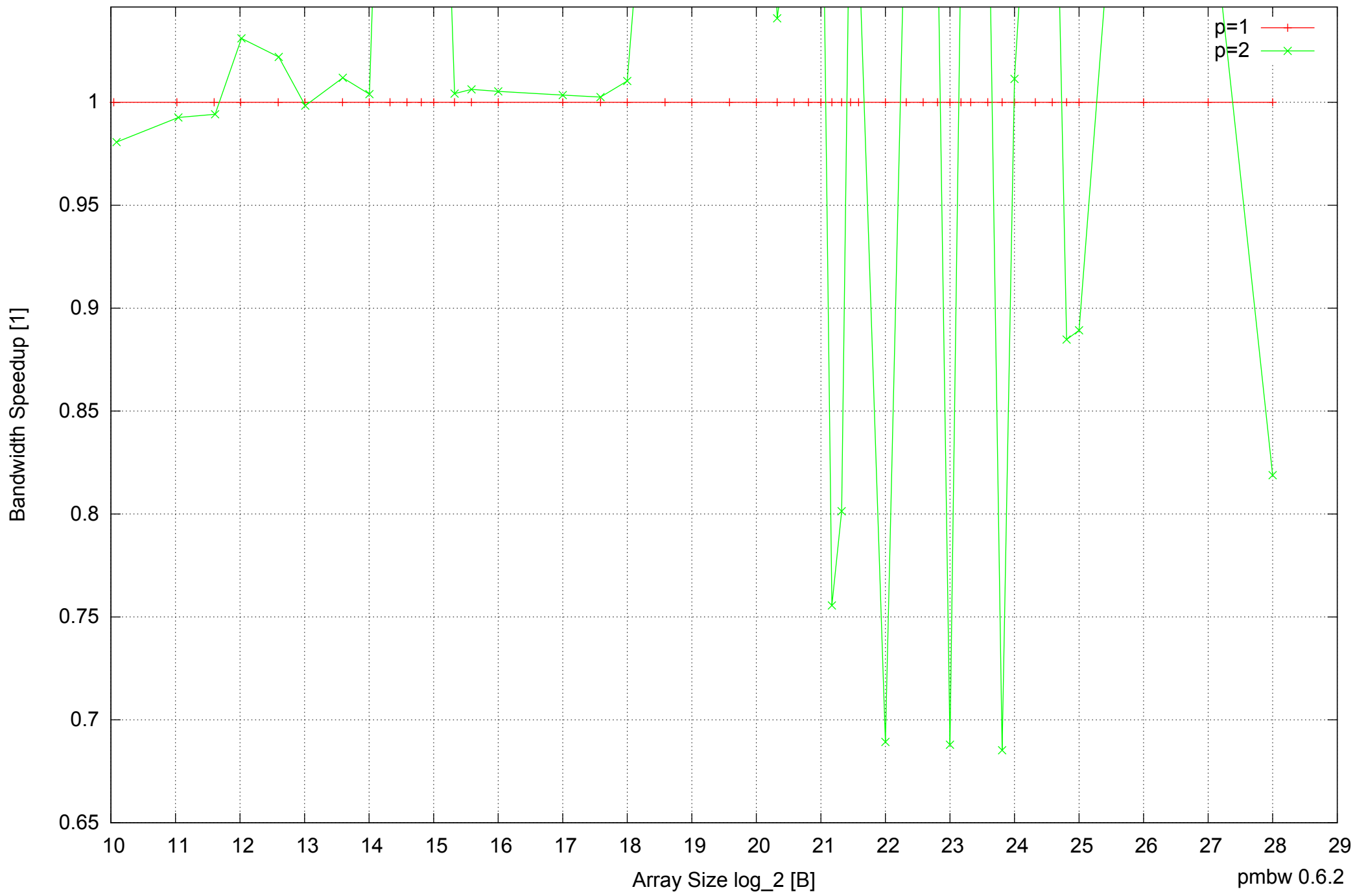
Intel Mobile Pentium III-M 512MB - Speedup of Parallel Memory Bandwidth (enlarged) - ScanRead16PtrUnrollLoop
