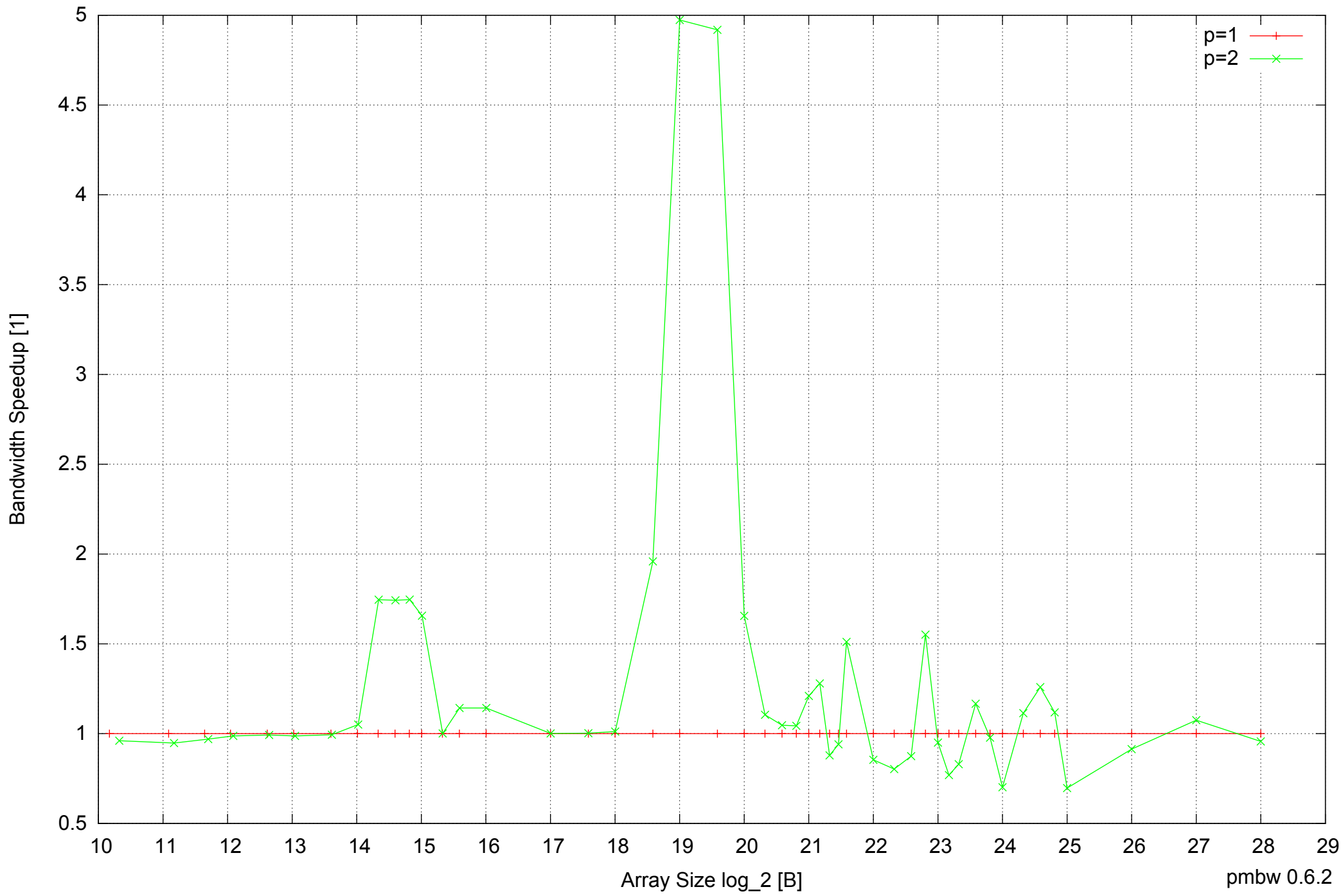
Intel Mobile Pentium III-M 512MB - Speedup of Parallel Memory Bandwidth - ScanRead64PtrUnrollLoop
