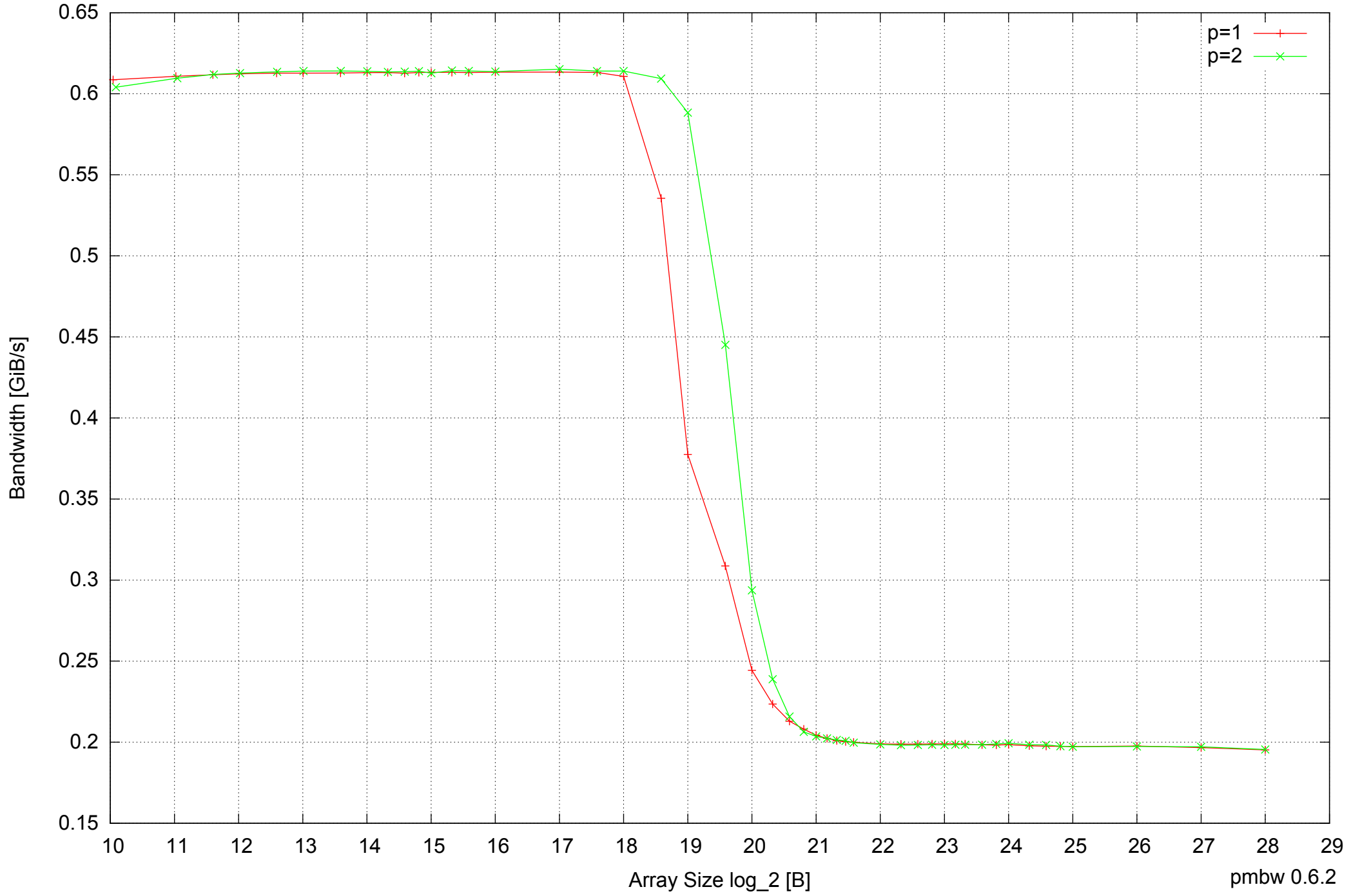
Intel Mobile Pentium III-M 512MB - Parallel Memory Bandwidth - ScanWrite16PtrSimpleLoop
