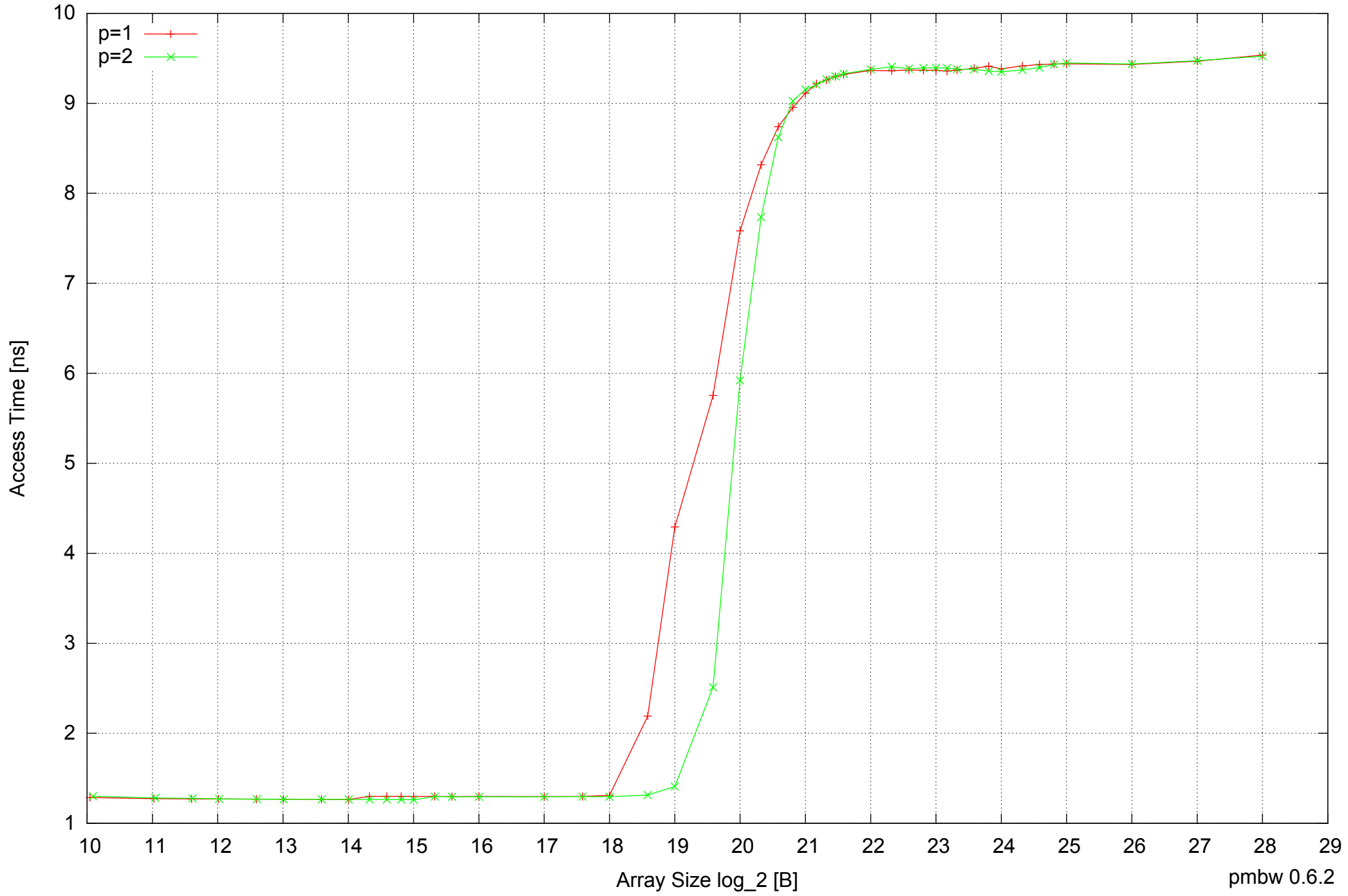
Intel Mobile Pentium III-M 512MB - Parallel Memory Access Time - ScanWrite16PtrUnrollLoop
