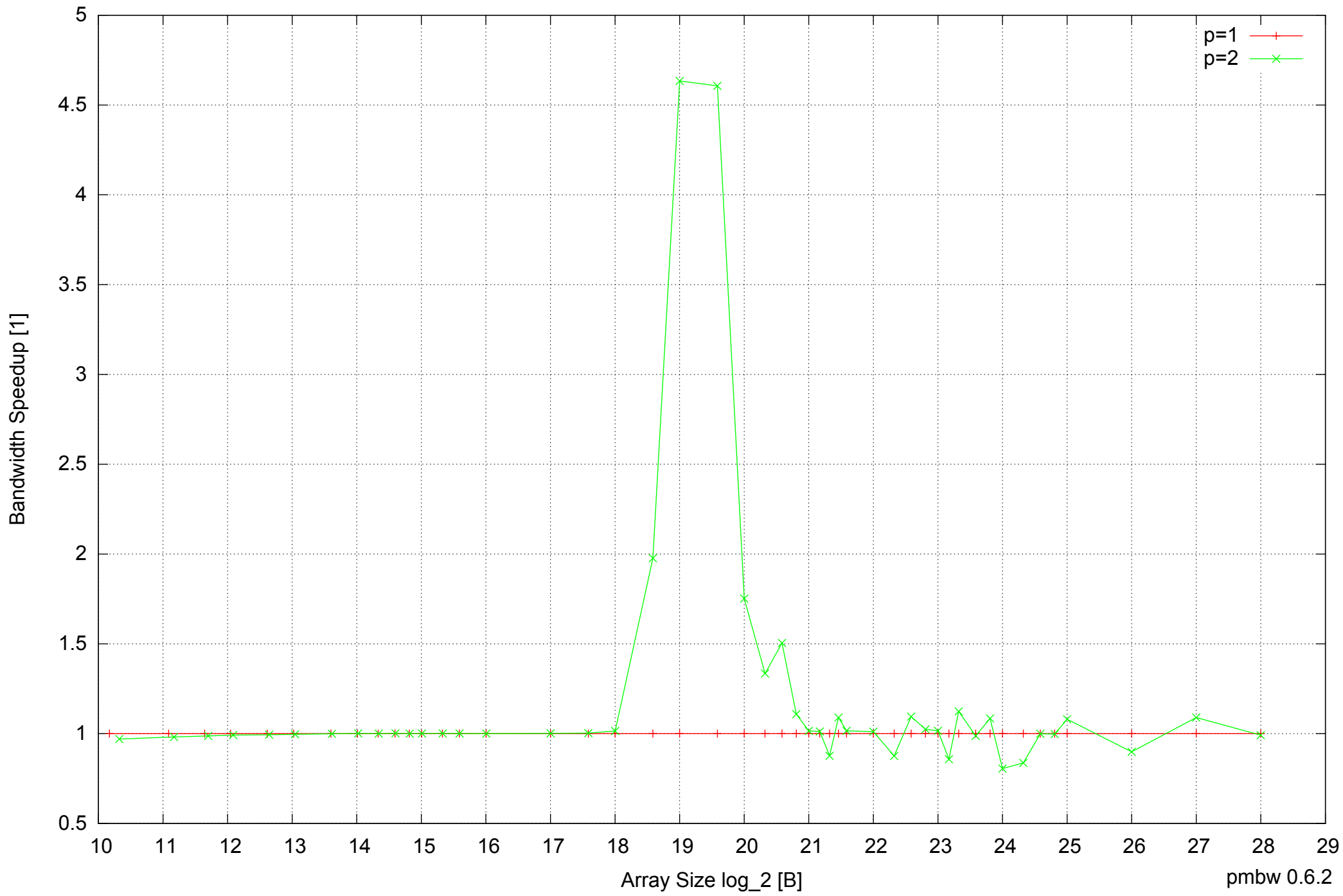
Intel Mobile Pentium III-M 512MB - Speedup of Parallel Memory Bandwidth - ScanRead64PtrSimpleLoop
