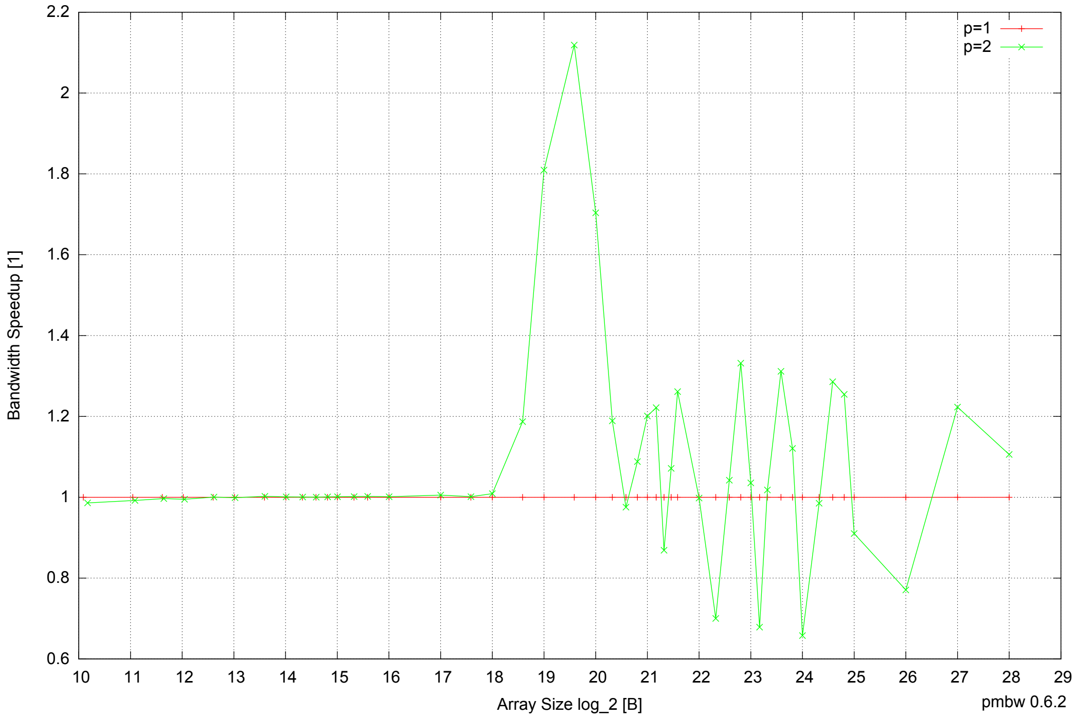
Intel Mobile Pentium III-M 512MB - Speedup of Parallel Memory Bandwidth - ScanRead32IndexSimpleLoop
