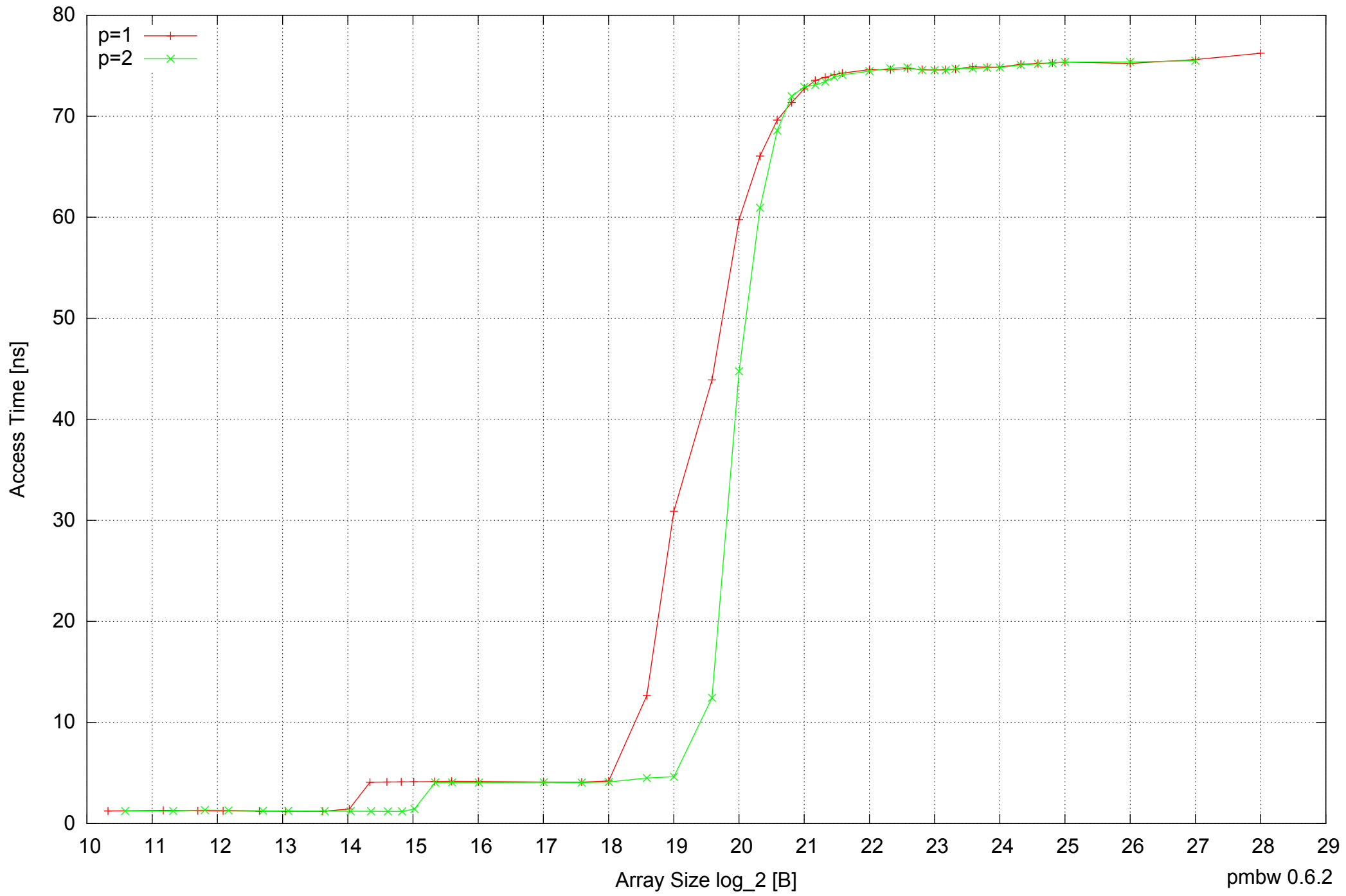
Intel Mobile Pentium III-M 512MB - Parallel Memory Access Time - ScanWrite128PtrUnrollLoop
