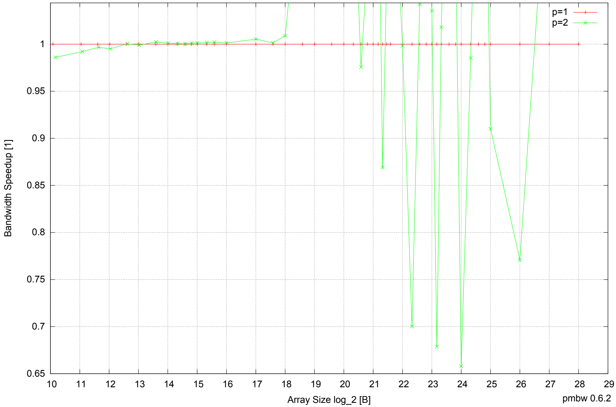
Intel Mobile Pentium III-M 512MB - Speedup of Parallel Memory Bandwidth (enlarged) - ScanRead32IndexSimpleLoop
