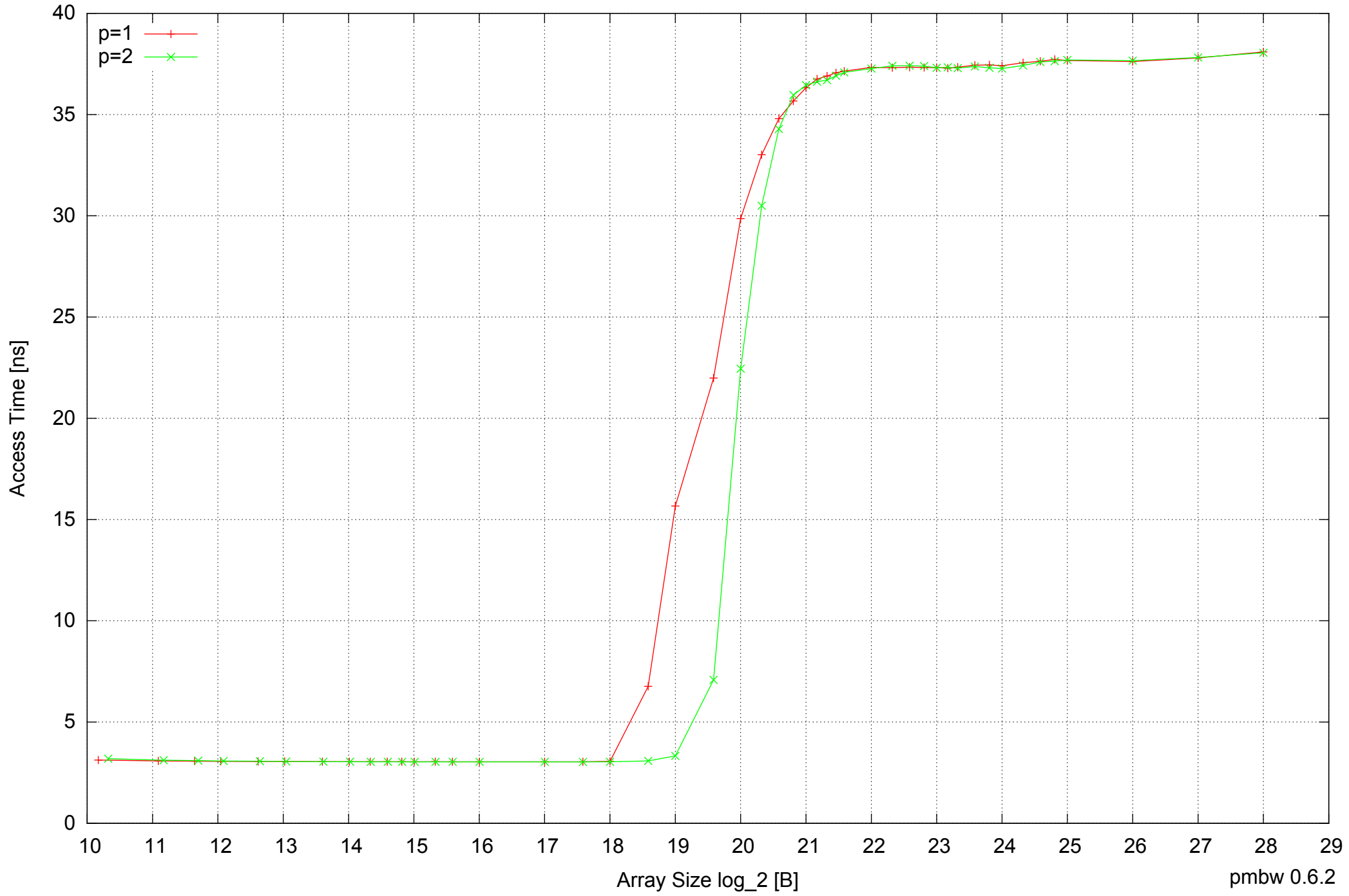
Intel Mobile Pentium III-M 512MB - Parallel Memory Access Time - ScanWrite64PtrSimpleLoop
