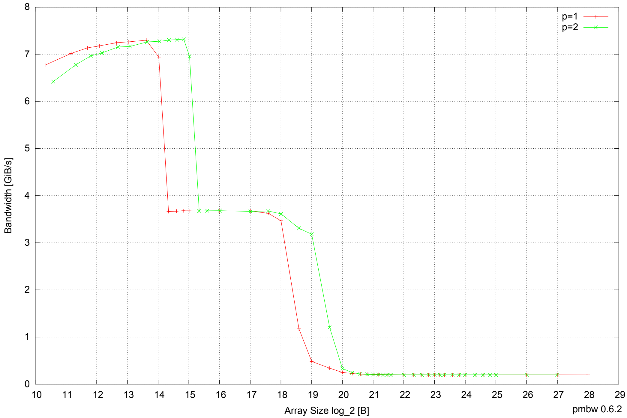
Intel Mobile Pentium III-M 512MB - Parallel Memory Bandwidth - ScanWrite128PtrSimpleLoop
