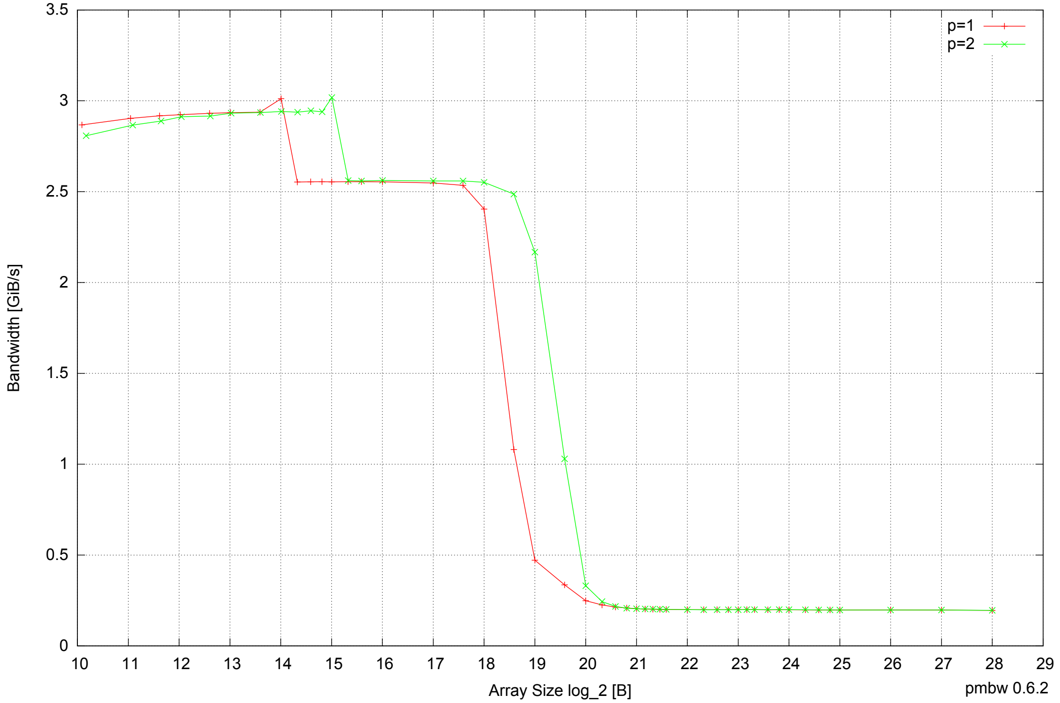
Intel Mobile Pentium III-M 512MB - Parallel Memory Bandwidth - ScanWrite32PtrUnrollLoop
