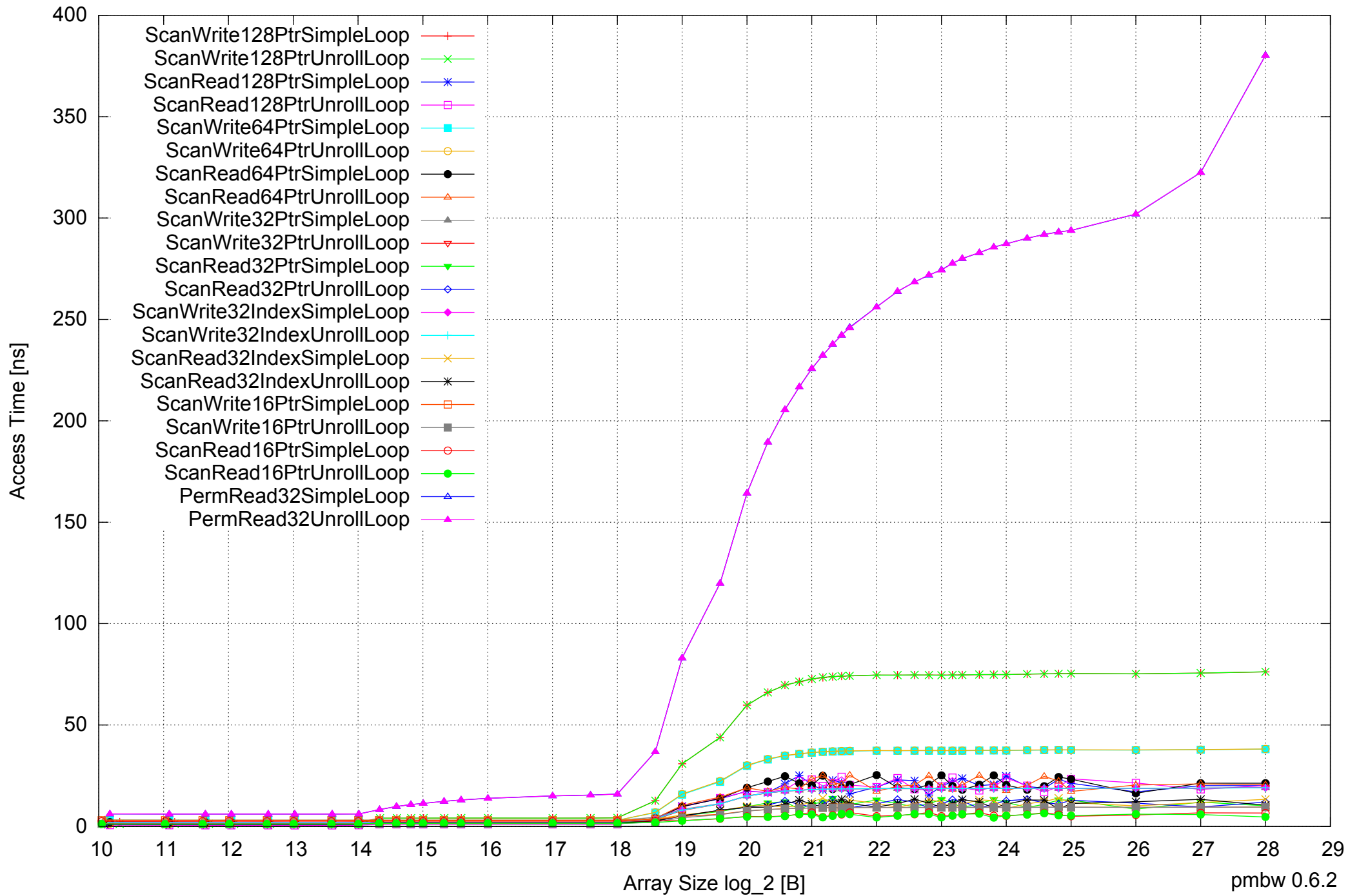
Intel Mobile Pentium III-M 512MB - One Thread Memory Latency (Access Time)
