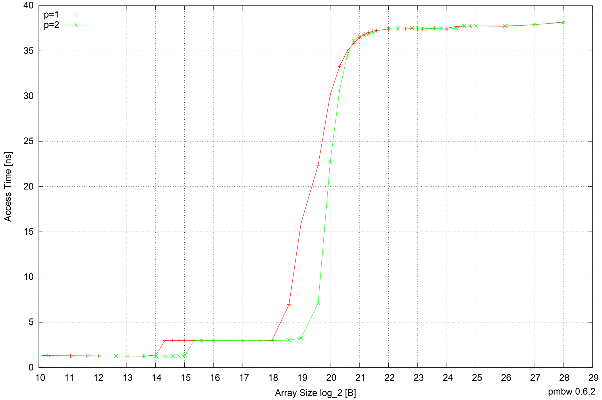
Intel Mobile Pentium III-M 512MB - Parallel Memory Access Time - ScanWrite64PtrUnrollLoop
