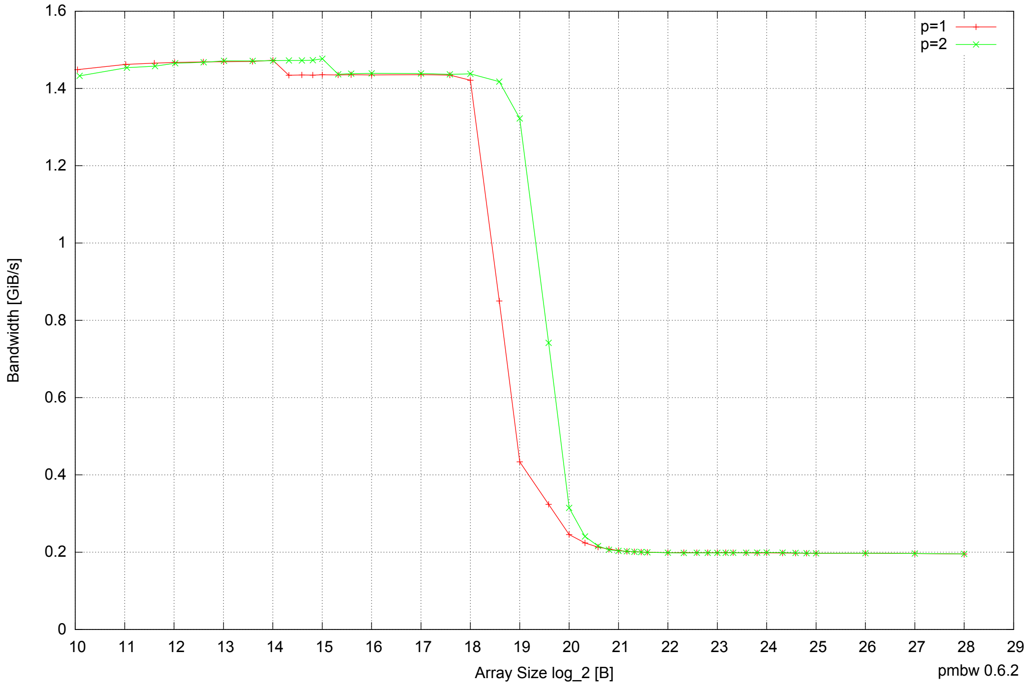
Intel Mobile Pentium III-M 512MB - Parallel Memory Bandwidth - ScanWrite16PtrUnrollLoop
