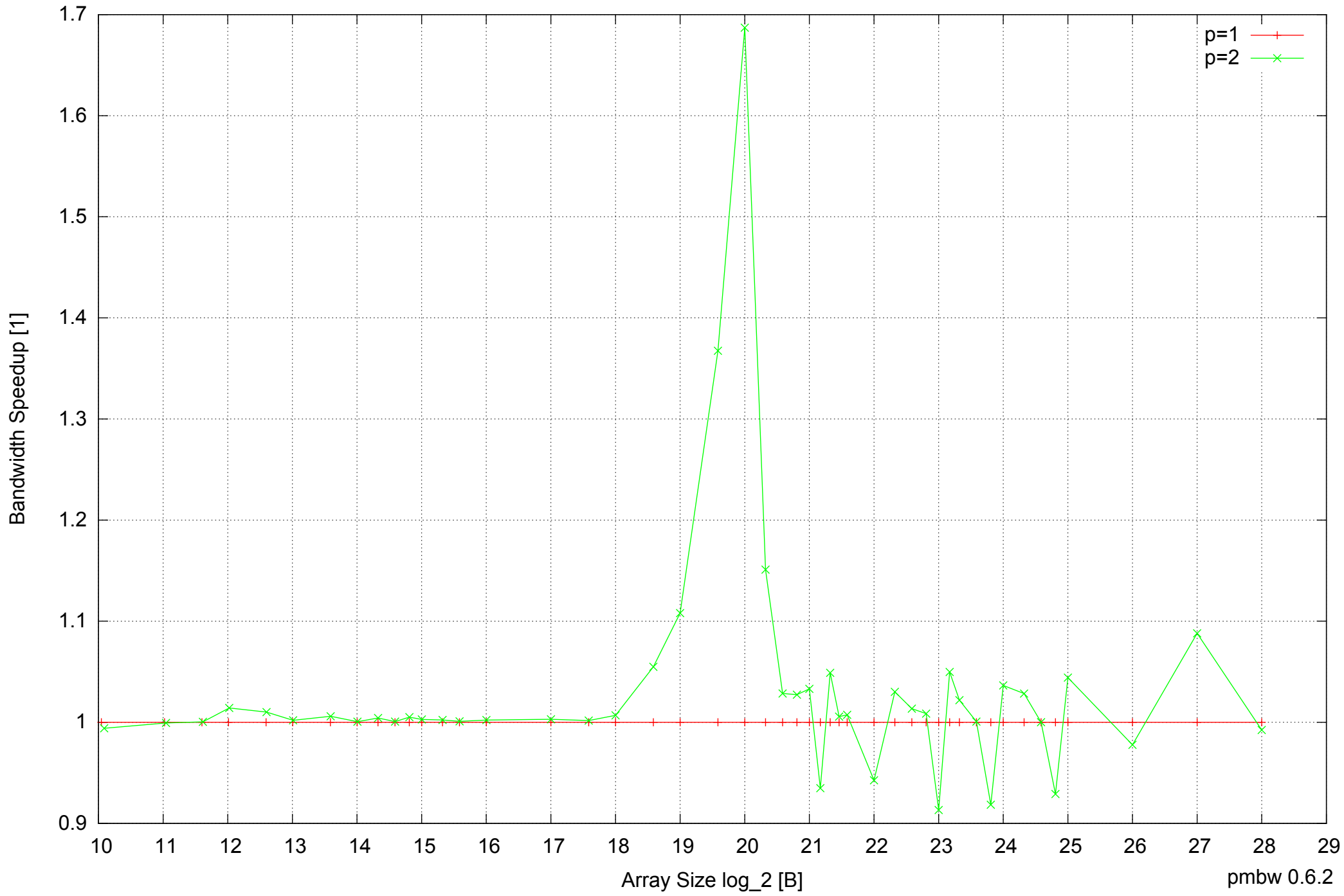
Intel Mobile Pentium III-M 512MB - Speedup of Parallel Memory Bandwidth - ScanRead16PtrSimpleLoop
