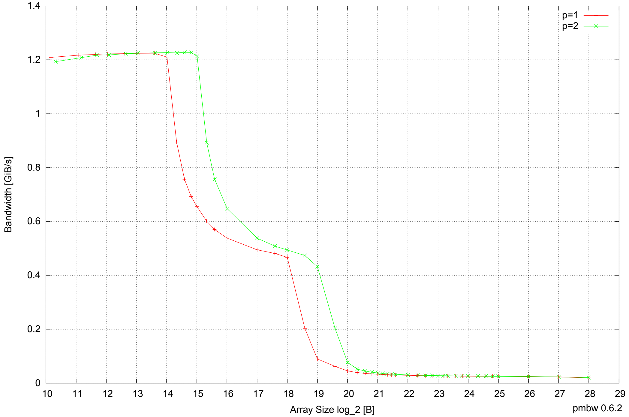
Intel Mobile Pentium III-M 512MB - Parallel Memory Bandwidth - PermRead32SimpleLoop
