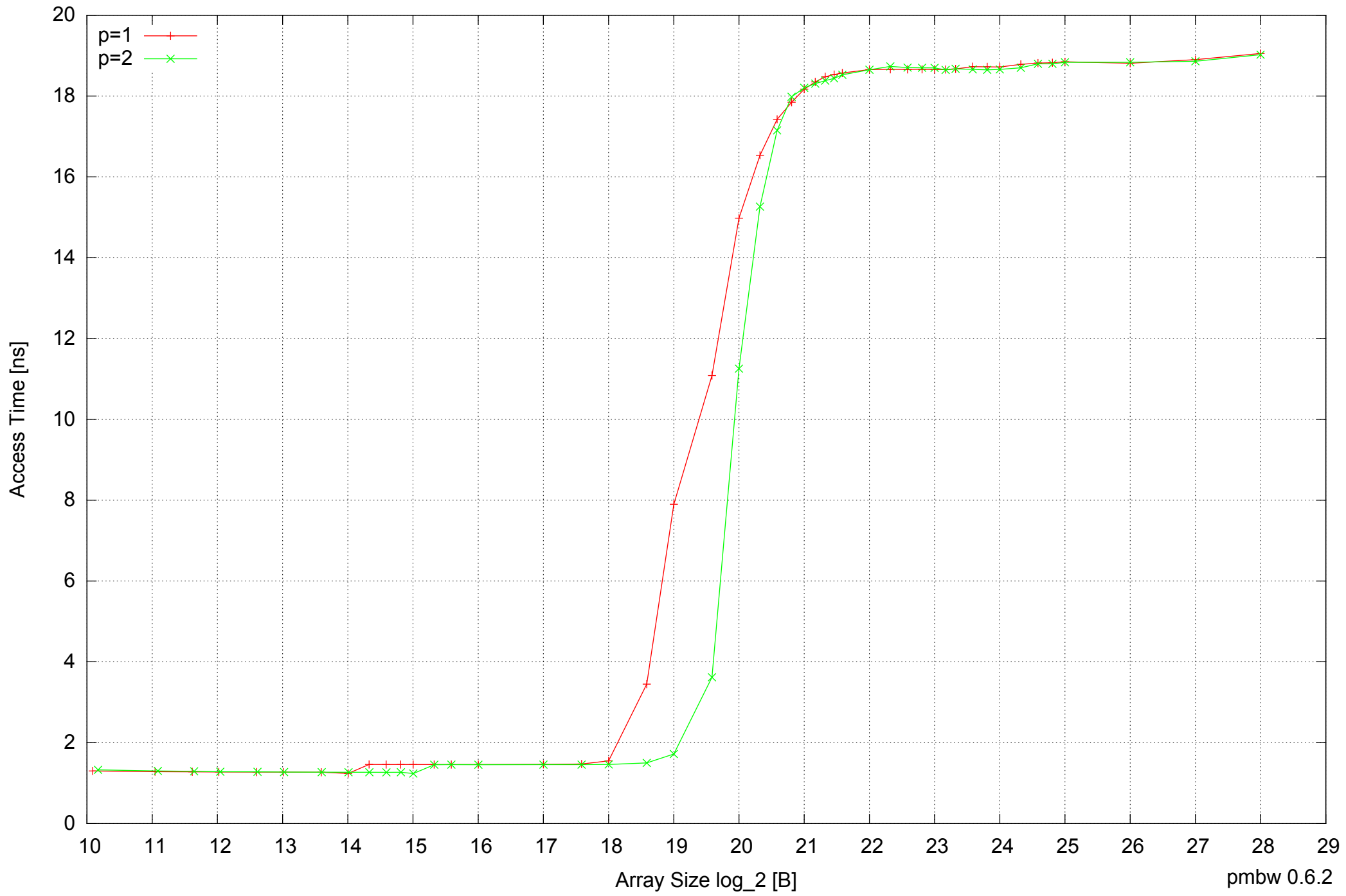
Intel Mobile Pentium III-M 512MB - Parallel Memory Access Time - ScanWrite32PtrUnrollLoop
