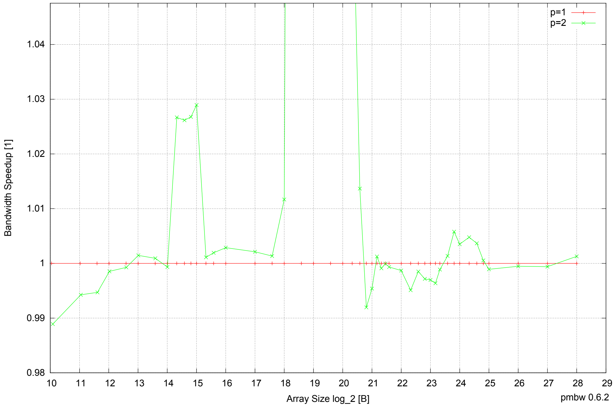
Intel Mobile Pentium III-M 512MB - Speedup of Parallel Memory Bandwidth (enlarged) - ScanWrite16PtrUnrollLoop
