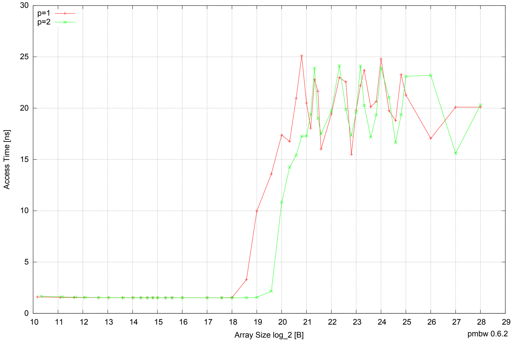
Intel Mobile Pentium III-M 512MB - Parallel Memory Access Time - ScanRead128PtrSimpleLoop
