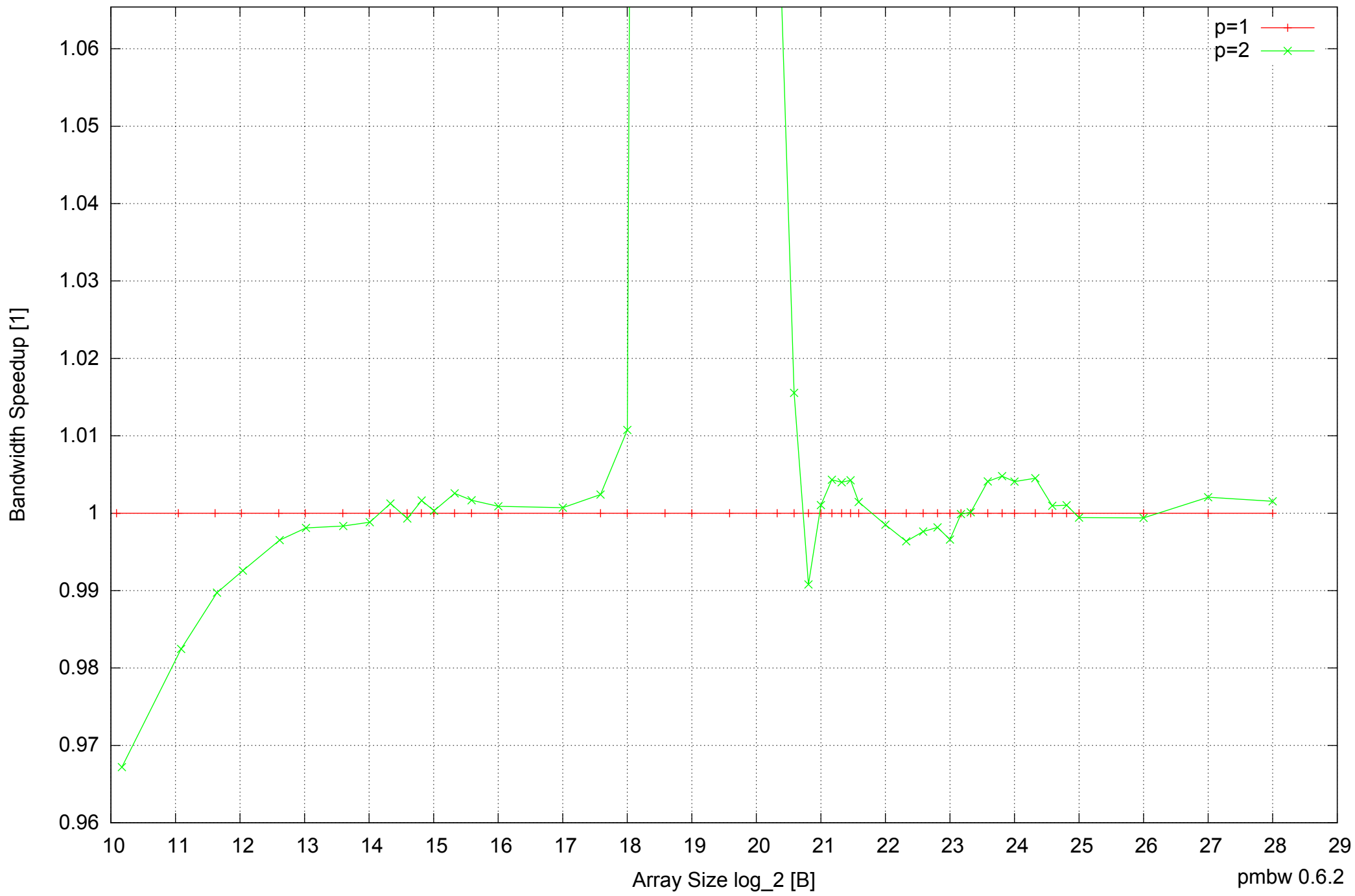
Intel Mobile Pentium III-M 512MB - Speedup of Parallel Memory Bandwidth (enlarged) - ScanWrite32IndexUnrollLoop
