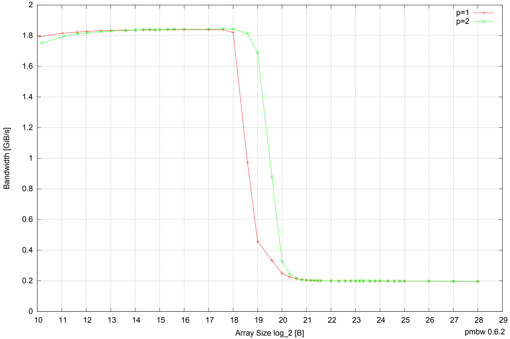
Intel Mobile Pentium III-M 512MB - Parallel Memory Bandwidth - ScanWrite32IndexSimpleLoop
