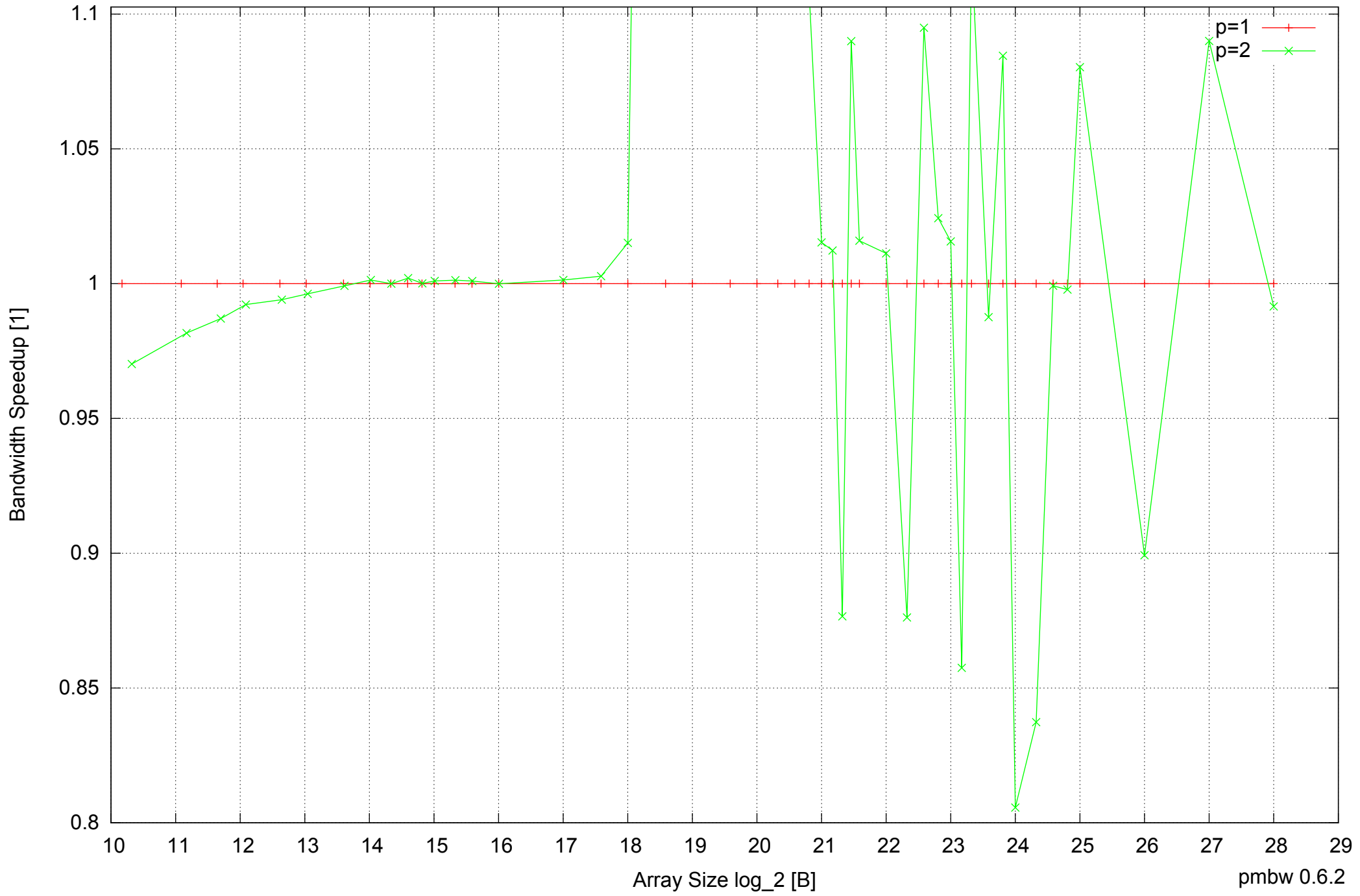
Intel Mobile Pentium III-M 512MB - Speedup of Parallel Memory Bandwidth (enlarged) - ScanRead64PtrSimpleLoop
