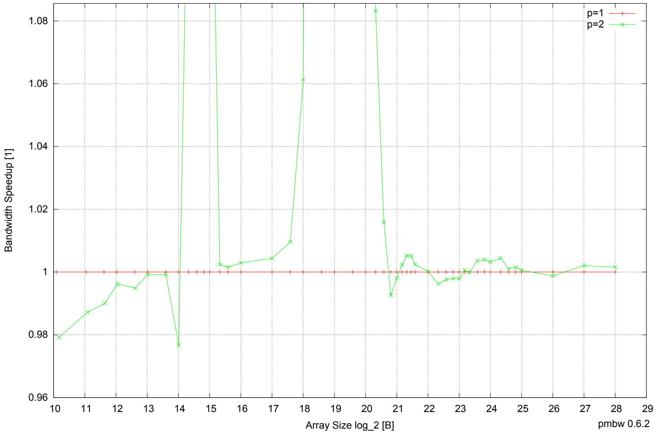
Intel Mobile Pentium III-M 512MB - Speedup of Parallel Memory Bandwidth (enlarged) - ScanWrite32PtrUnrollLoop
