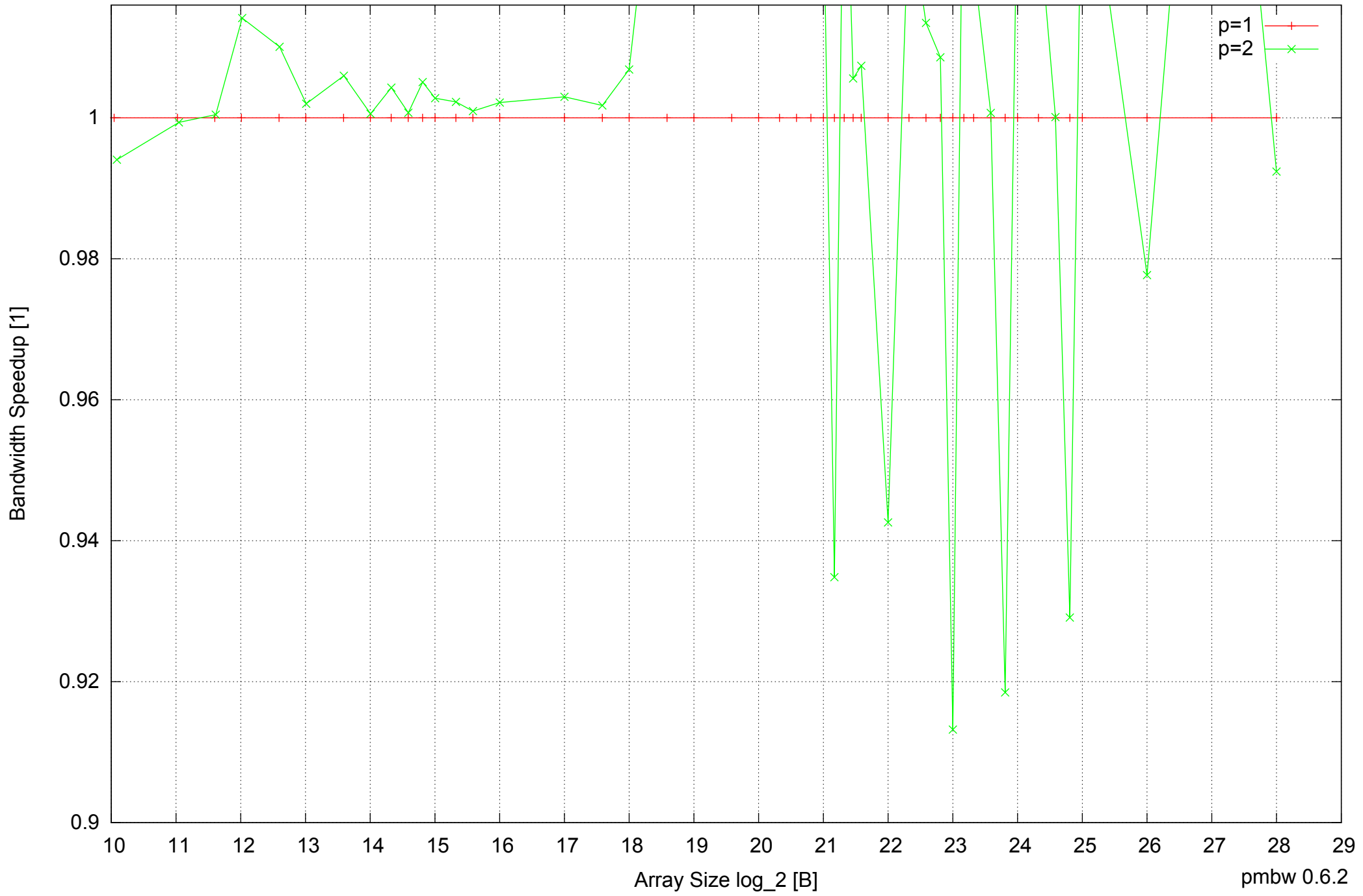
Intel Mobile Pentium III-M 512MB - Speedup of Parallel Memory Bandwidth (enlarged) - ScanRead16PtrSimpleLoop
