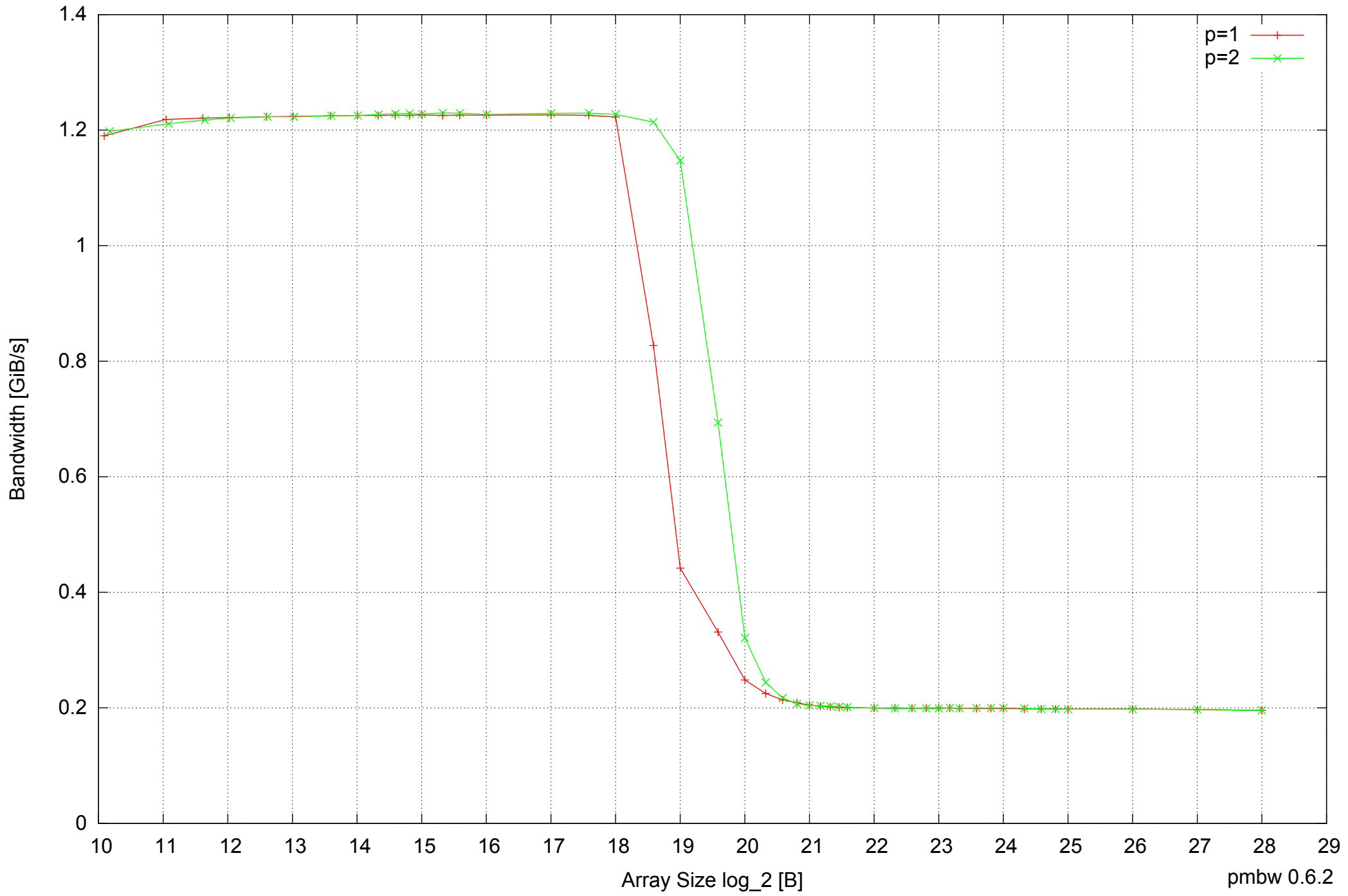
Intel Mobile Pentium III-M 512MB - Parallel Memory Bandwidth - ScanWrite32PtrSimpleLoop
