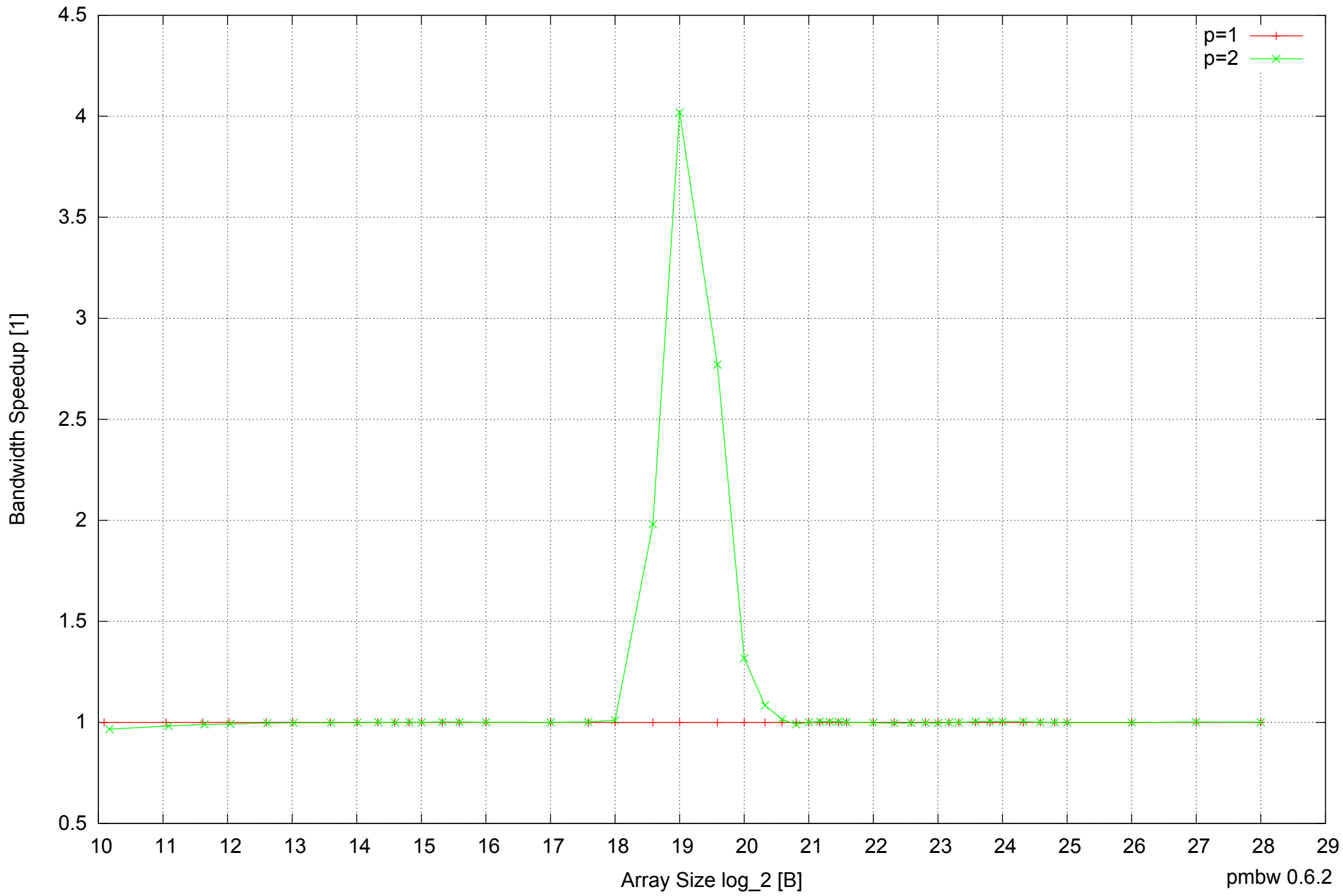
Intel Mobile Pentium III-M 512MB - Speedup of Parallel Memory Bandwidth - ScanWrite32IndexUnrollLoop
