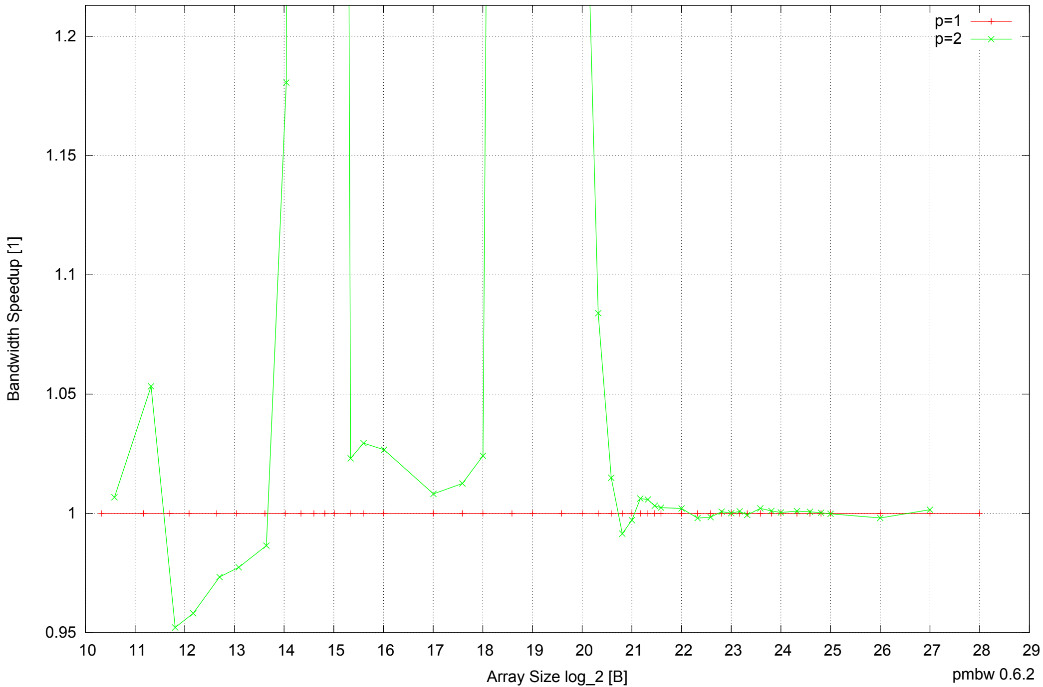
Intel Mobile Pentium III-M 512MB - Speedup of Parallel Memory Bandwidth (enlarged) - ScanWrite128PtrUnrollLoop
