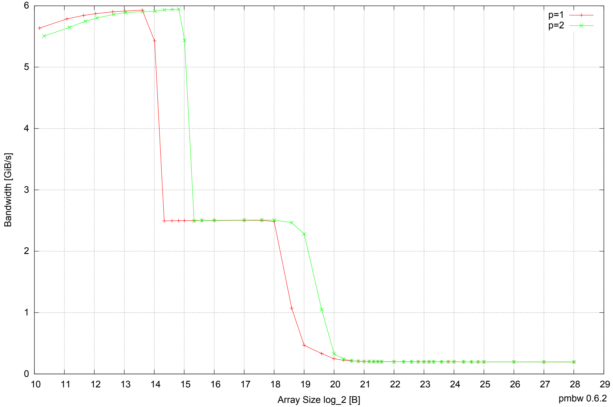
Intel Mobile Pentium III-M 512MB - Parallel Memory Bandwidth - ScanWrite64PtrUnrollLoop
