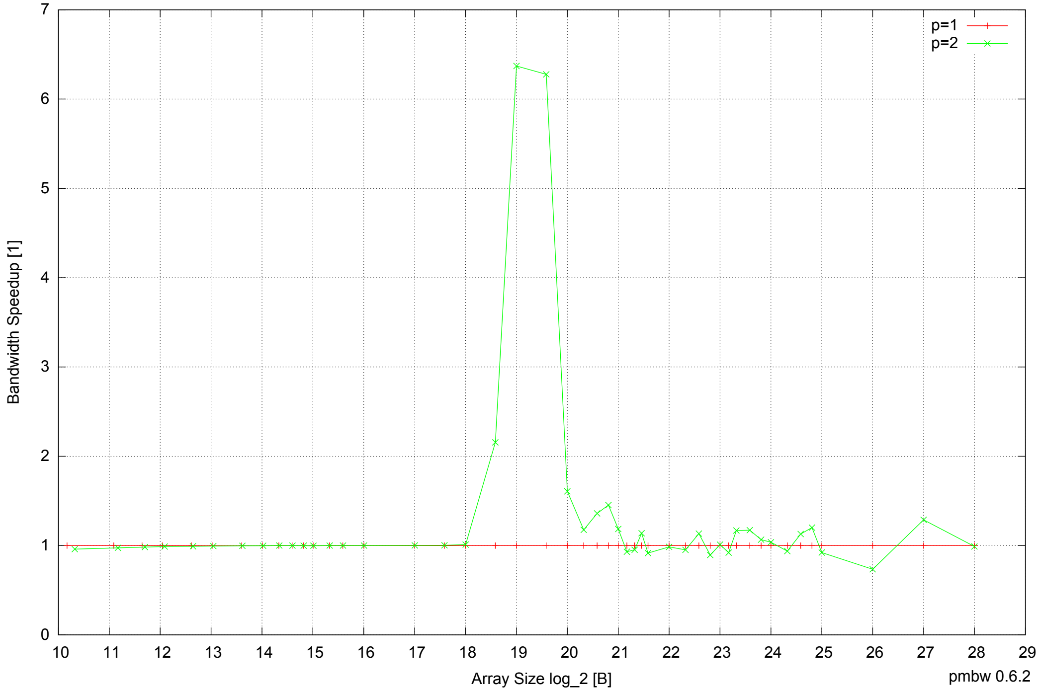
Intel Mobile Pentium III-M 512MB - Speedup of Parallel Memory Bandwidth - ScanRead128PtrSimpleLoop
