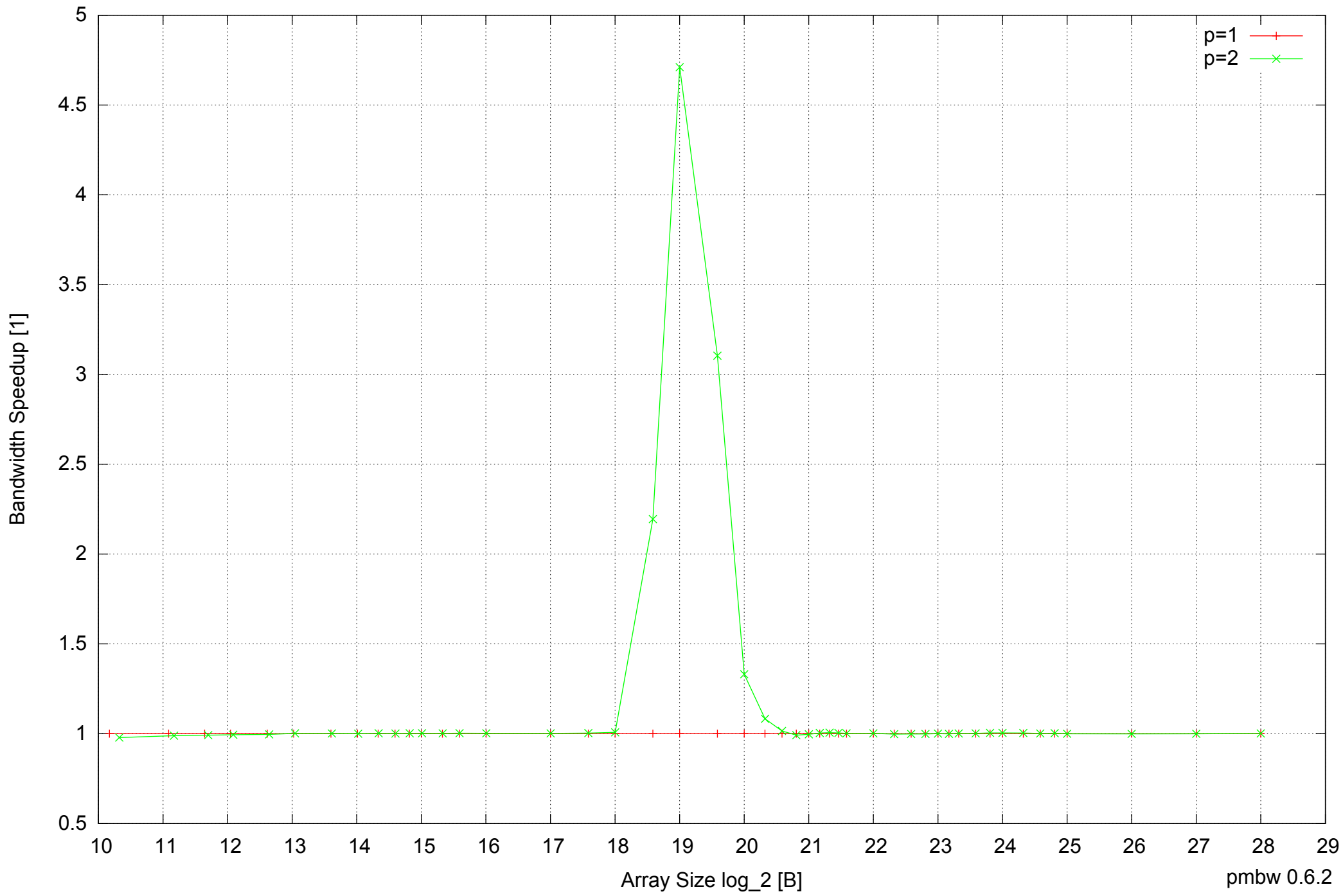
Intel Mobile Pentium III-M 512MB - Speedup of Parallel Memory Bandwidth - ScanWrite64PtrSimpleLoop
