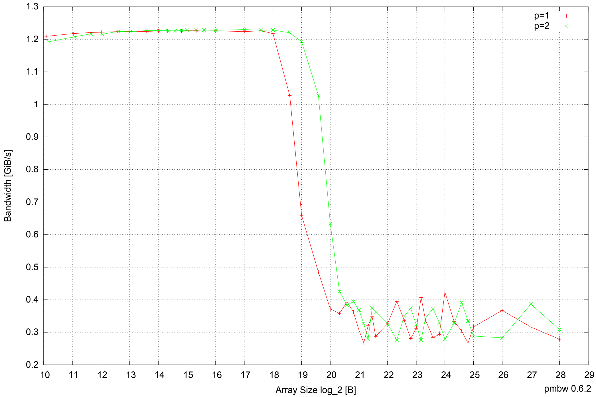
Intel Mobile Pentium III-M 512MB - Parallel Memory Bandwidth - ScanRead32IndexSimpleLoop
