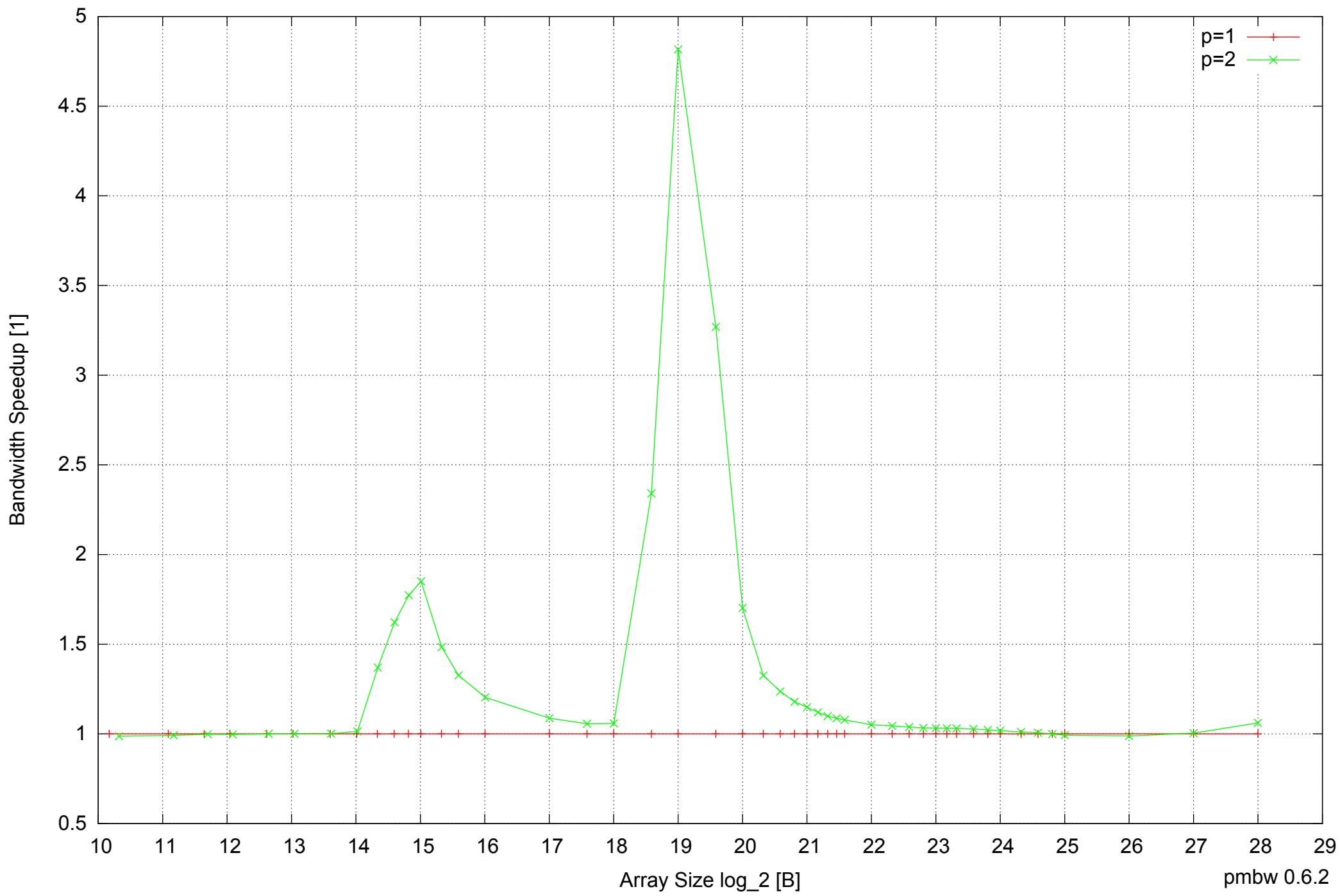
Intel Mobile Pentium III-M 512MB - Speedup of Parallel Memory Bandwidth - PermRead32SimpleLoop
