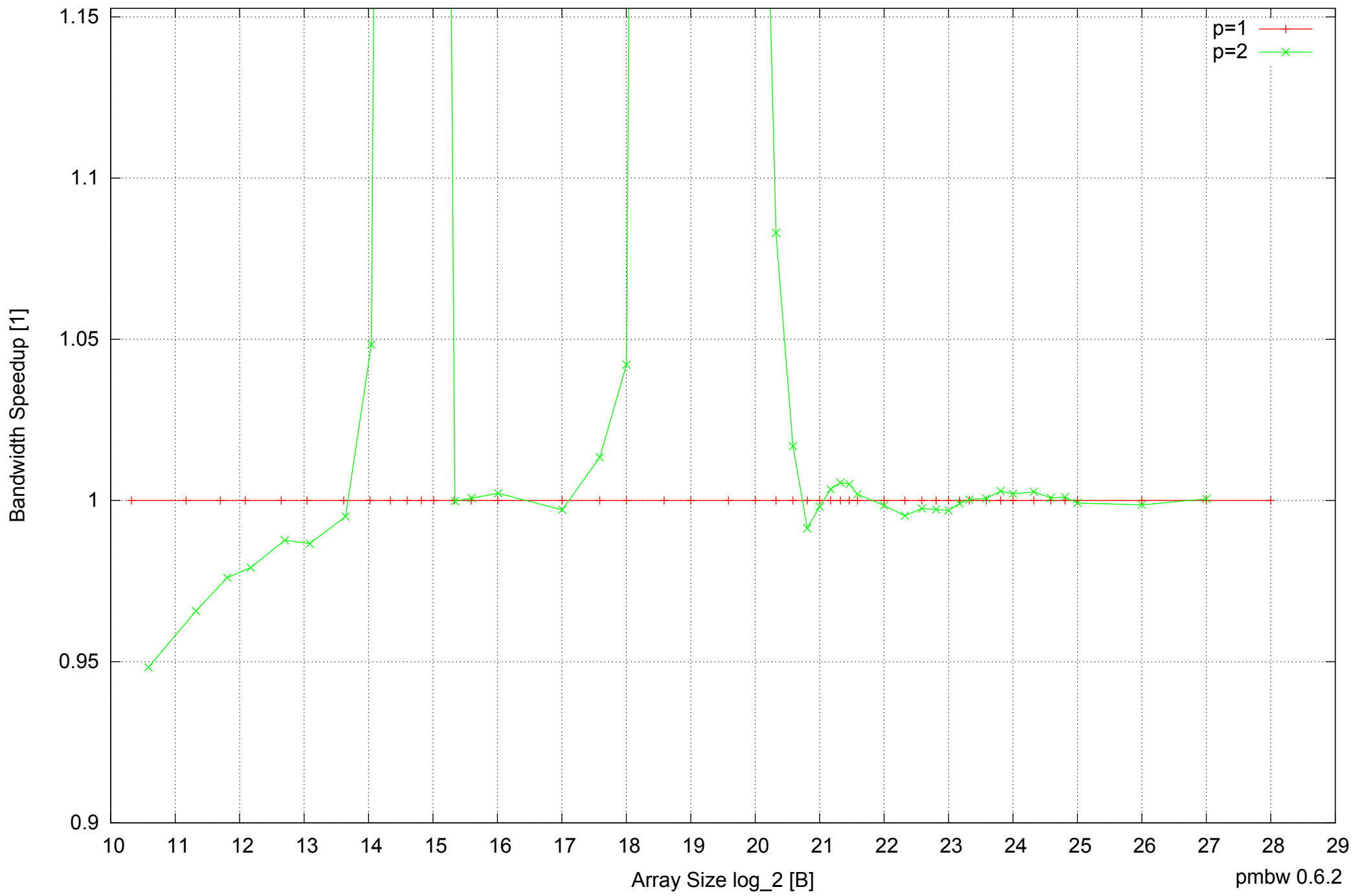
Intel Mobile Pentium III-M 512MB - Speedup of Parallel Memory Bandwidth (enlarged) - ScanWrite128PtrSimpleLoop
