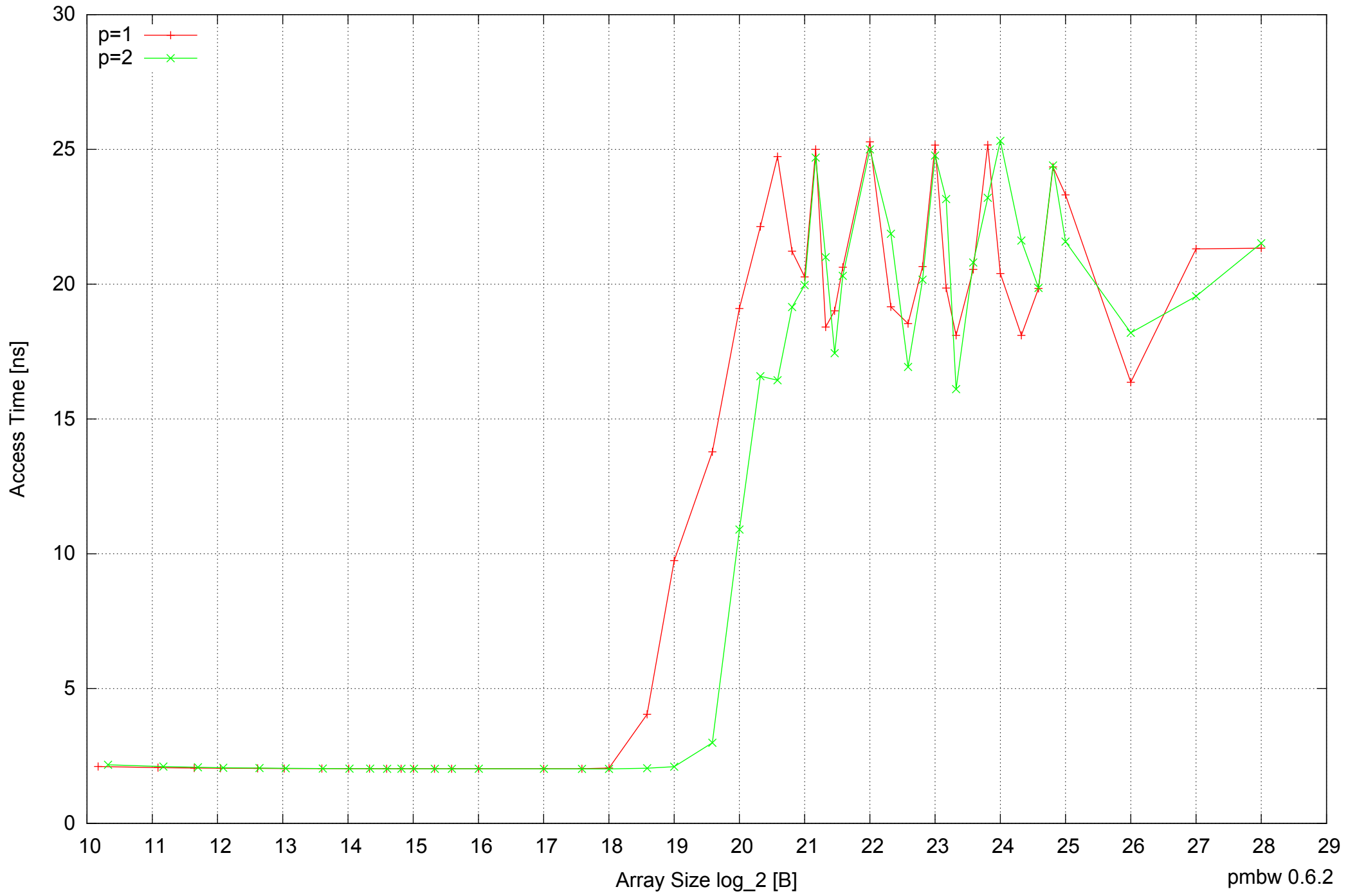
Intel Mobile Pentium III-M 512MB - Parallel Memory Access Time - ScanRead64PtrSimpleLoop
