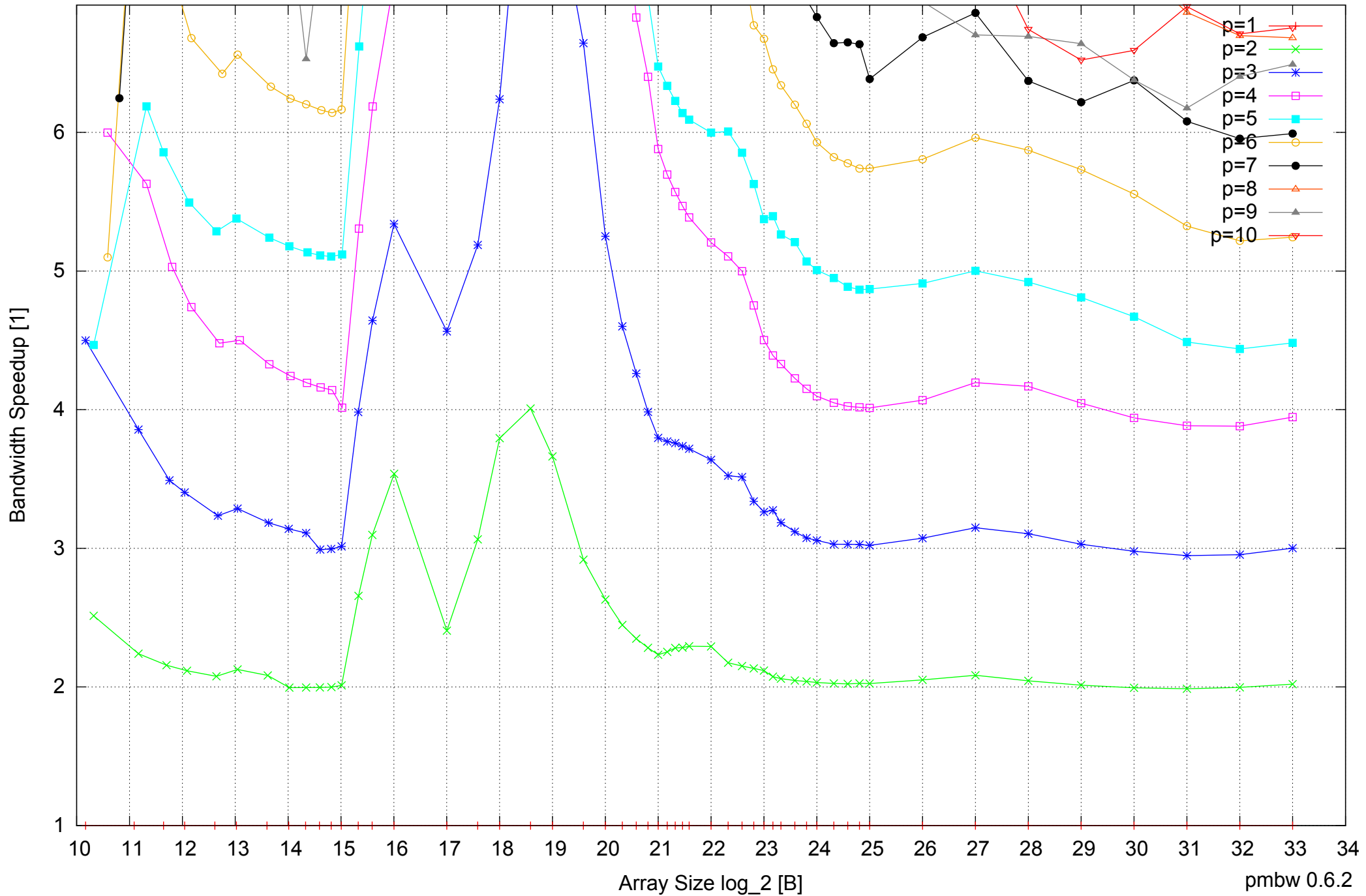
Intel Core i7-920 12GB - Speedup of Parallel Memory Bandwidth (enlarged) - PermRead64UnrollLoop
