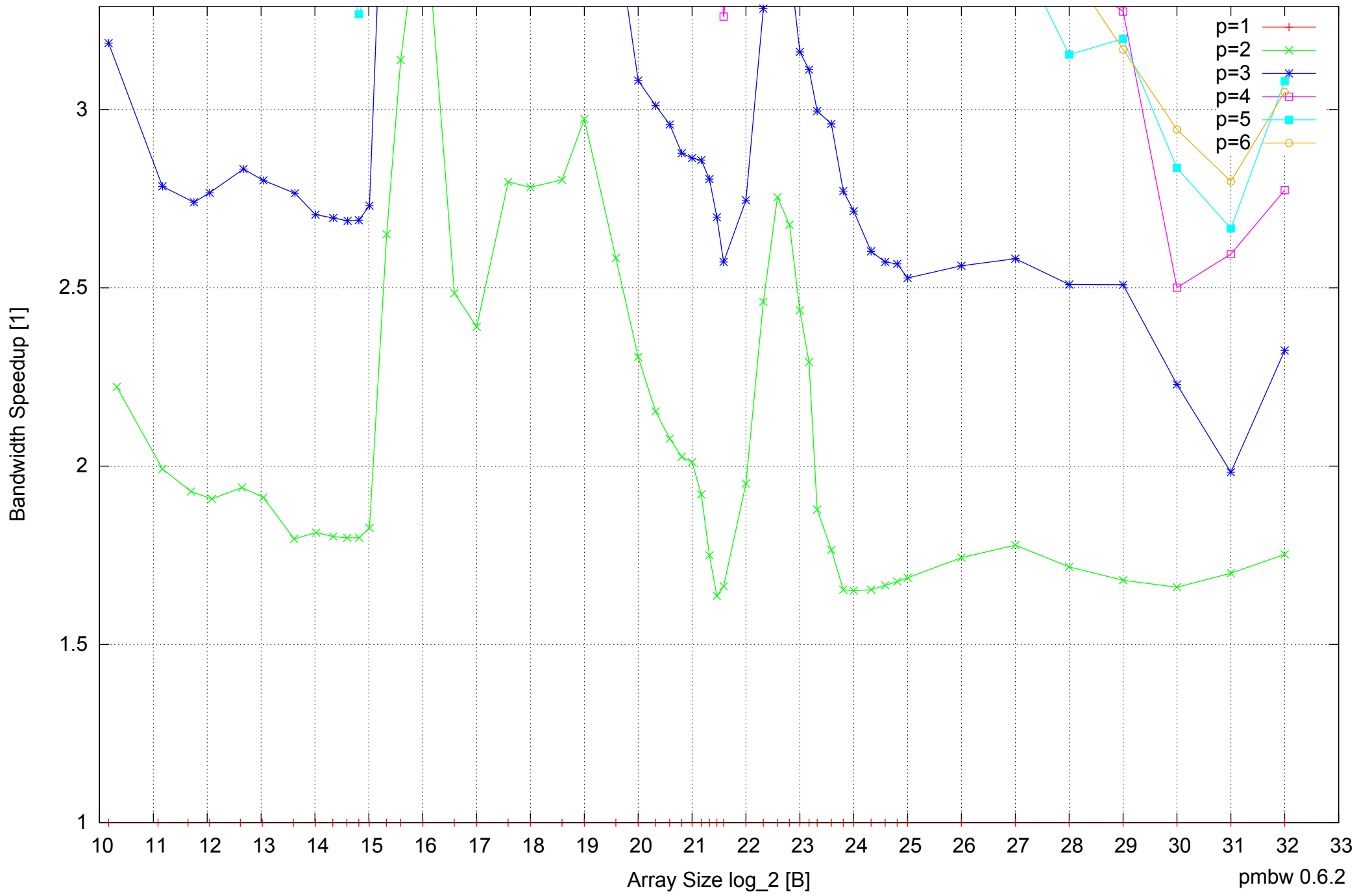
Intel Core i7-4500U 8GB - Speedup of Parallel Memory Bandwidth (enlarged) - PermRead64UnrollLoop
