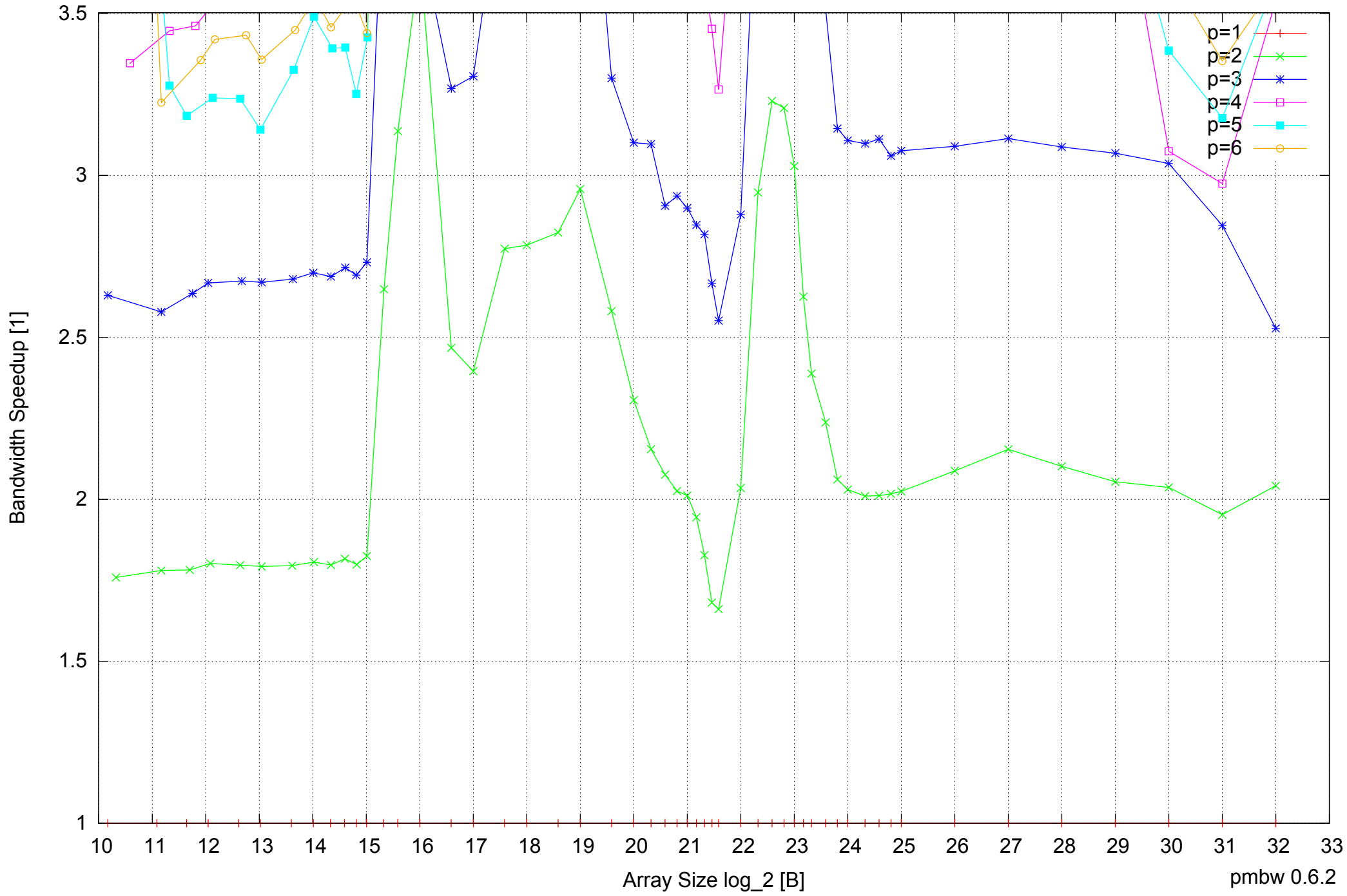
Intel Core i7-4500U 8GB - Speedup of Parallel Memory Bandwidth (enlarged) - PermRead64SimpleLoop
