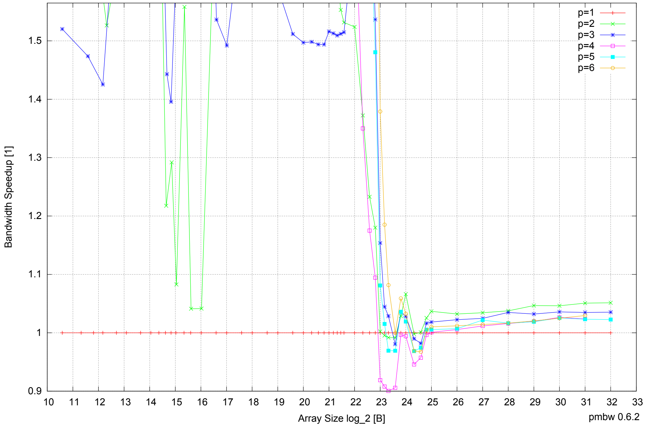
Intel Core i7-4500U 8GB - Speedup of Parallel Memory Bandwidth (enlarged) - ScanWrite256PtrSimpleLoop
