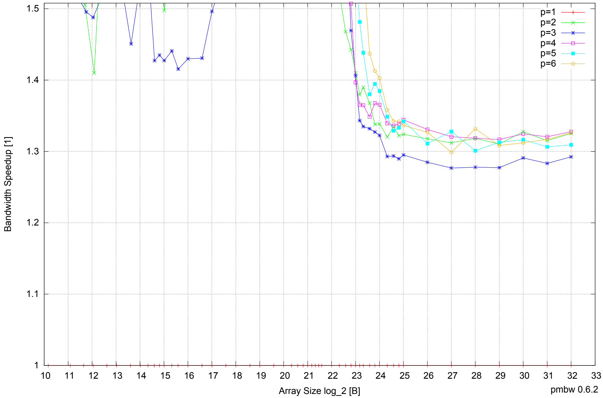
Intel Core i7-4500U 8GB - Speedup of Parallel Memory Bandwidth (enlarged) - ScanRead64IndexSimpleLoop
