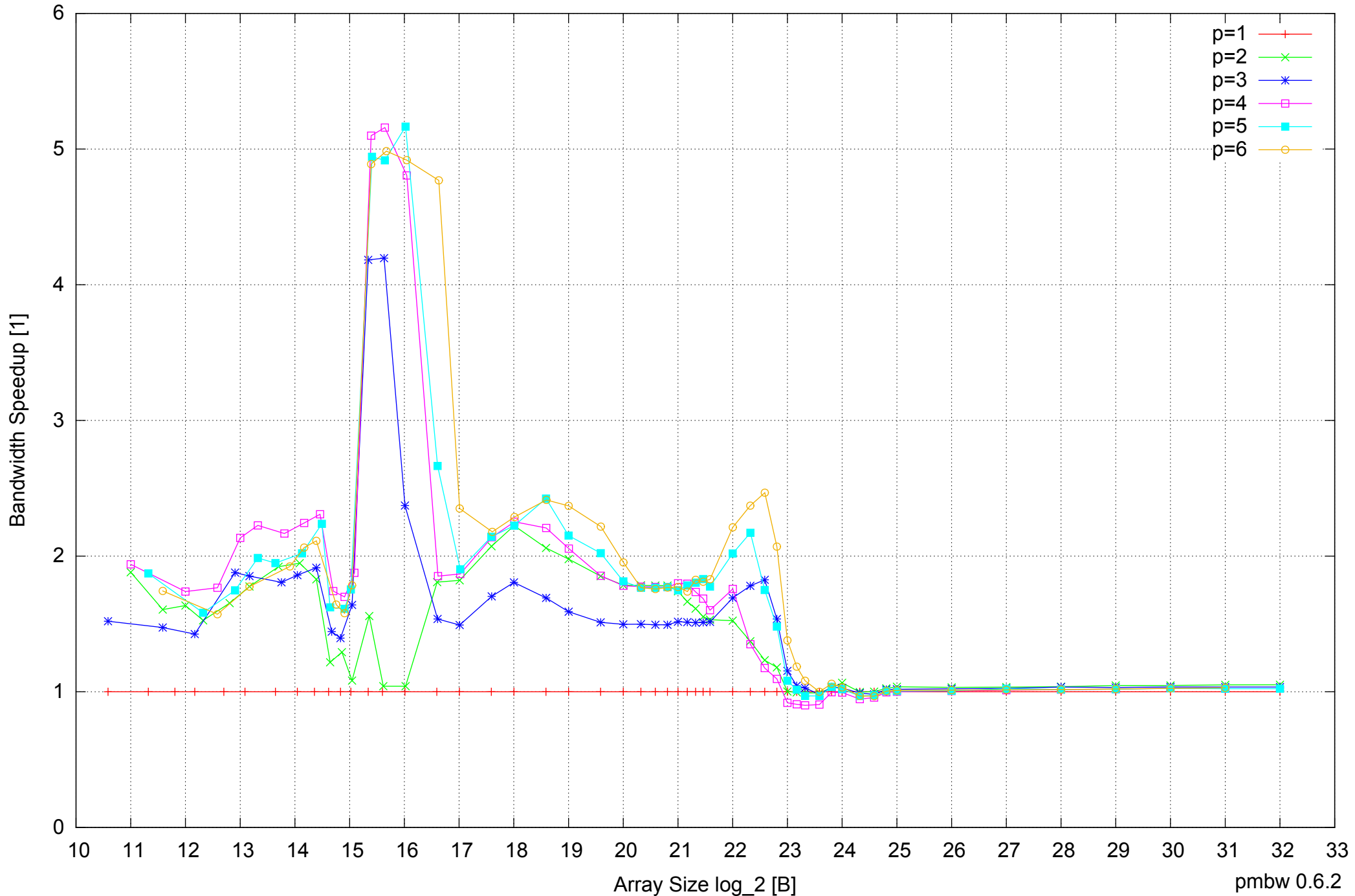
Intel Core i7-4500U 8GB - Speedup of Parallel Memory Bandwidth - ScanWrite256PtrSimpleLoop
