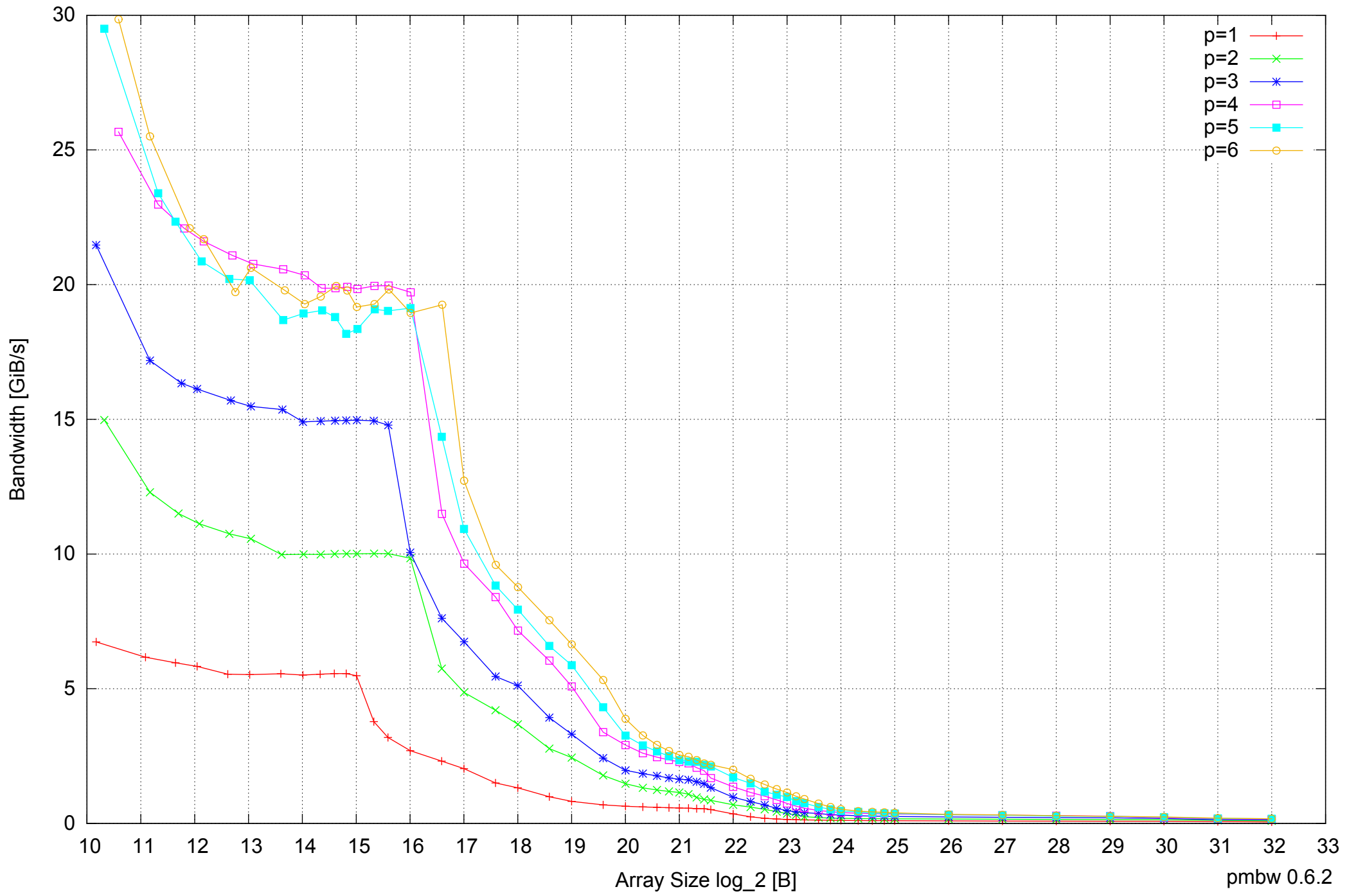
Intel Core i7-4500U 8GB - Parallel Memory Bandwidth - PermRead64UnrollLoop
