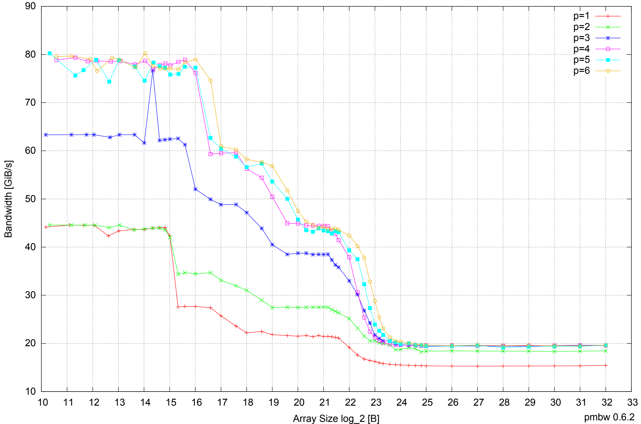
Intel Core i7-4500U 8GB - Parallel Memory Bandwidth - ScanRead64IndexUnrollLoop
