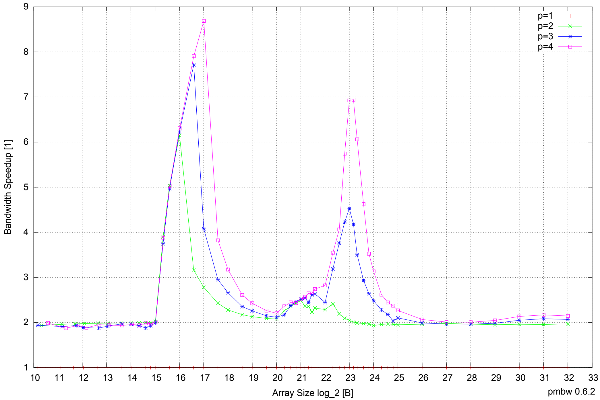
Intel Core 2 Duo E8500 8GB - Speedup of Parallel Memory Bandwidth - PermRead64SimpleLoop
