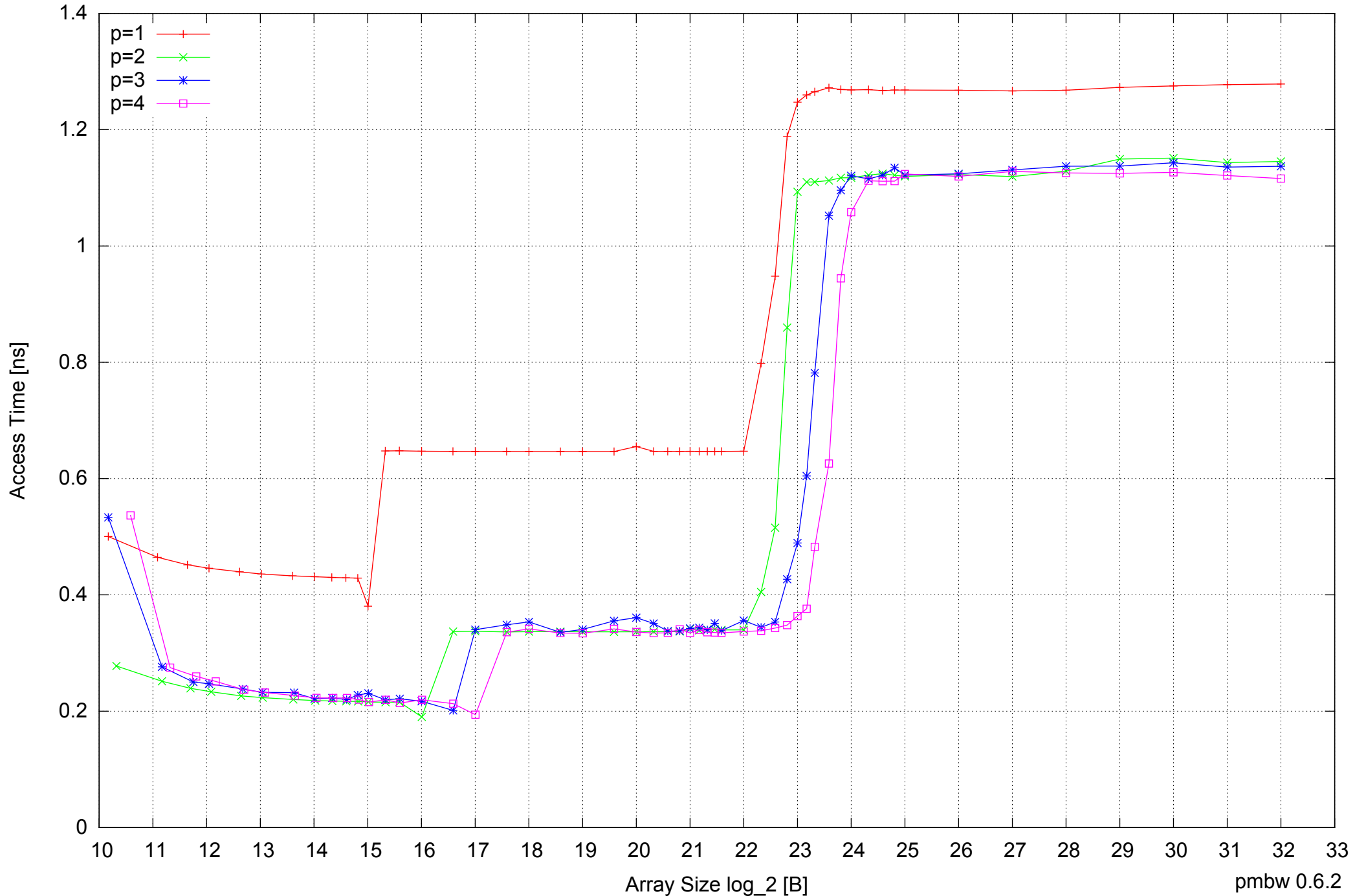
Intel Core 2 Duo E8500 8GB - Parallel Memory Access Time - ScanRead64PtrSimpleLoop
