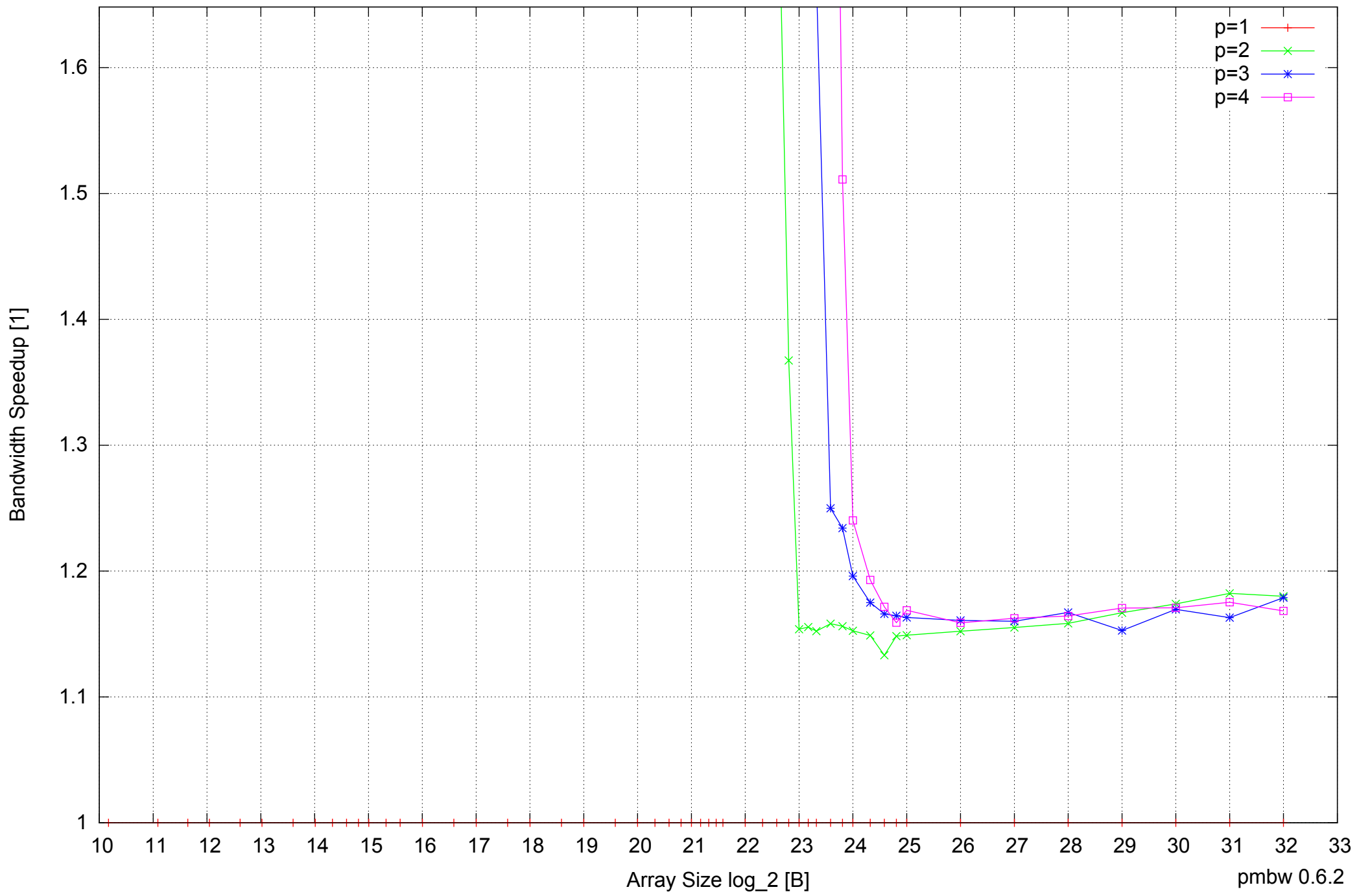
Intel Core 2 Duo E8500 8GB - Speedup of Parallel Memory Bandwidth (enlarged) - ScanRead64IndexUnrollLoop
