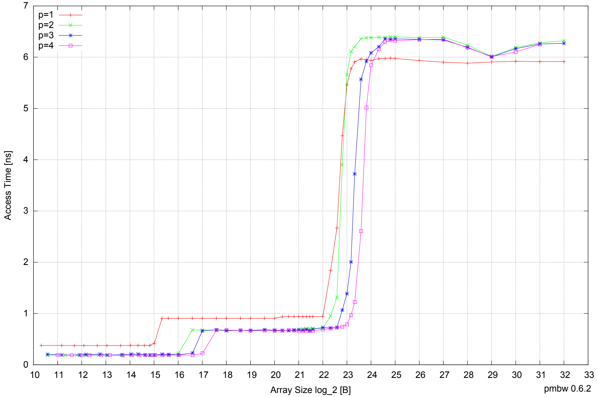
Intel Core 2 Duo E8500 8GB - Parallel Memory Access Time - ScanWrite128PtrUnrollLoop
