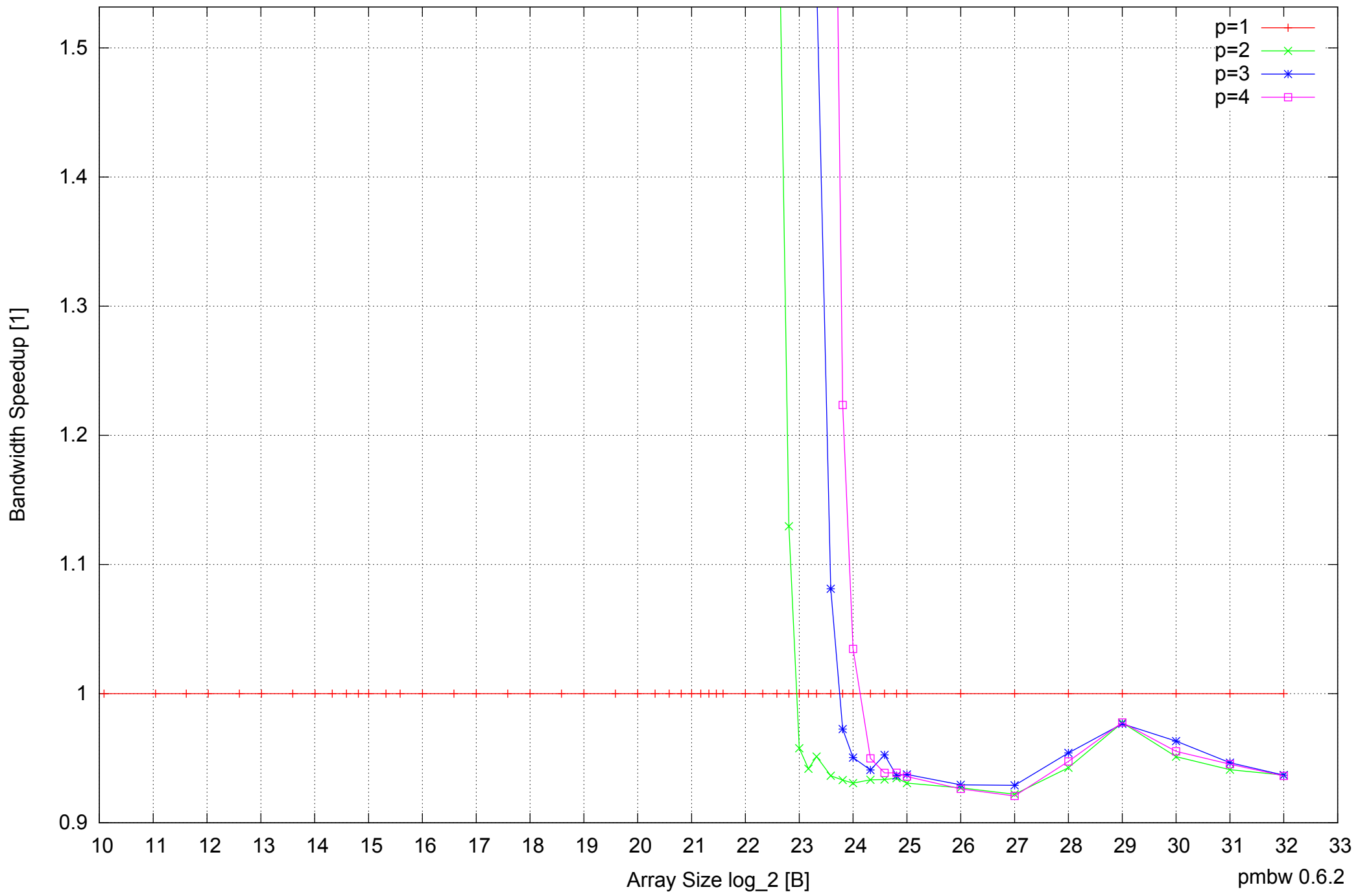
Intel Core 2 Duo E8500 8GB - Speedup of Parallel Memory Bandwidth (enlarged) - ScanWrite32PtrUnrollLoop
