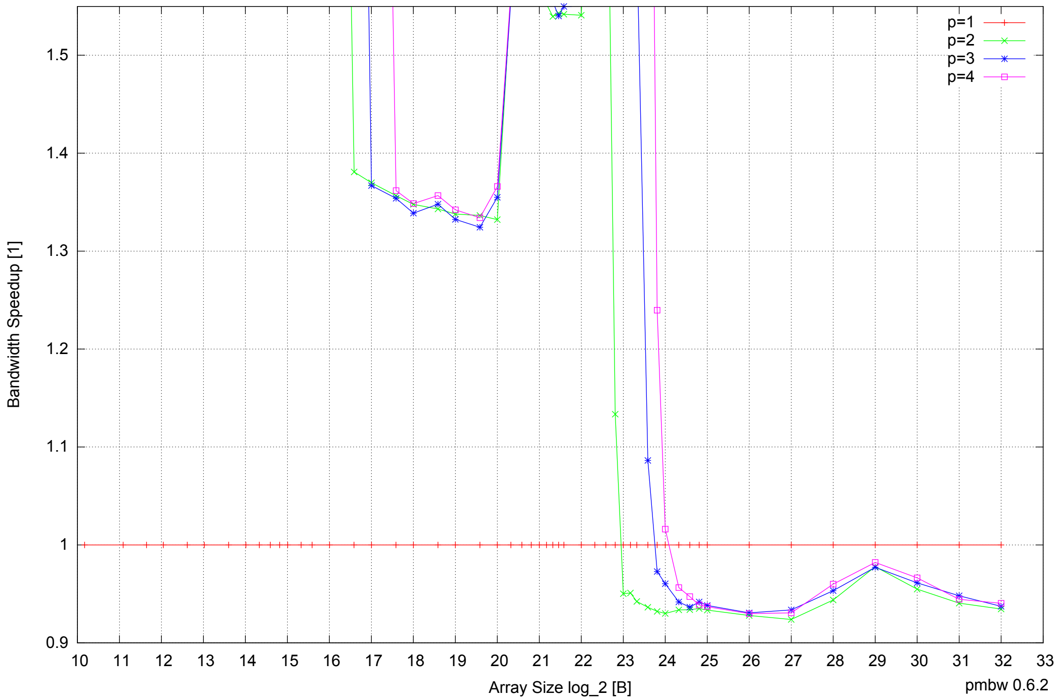
Intel Core 2 Duo E8500 8GB - Speedup of Parallel Memory Bandwidth (enlarged) - ScanWrite64PtrUnrollLoop
