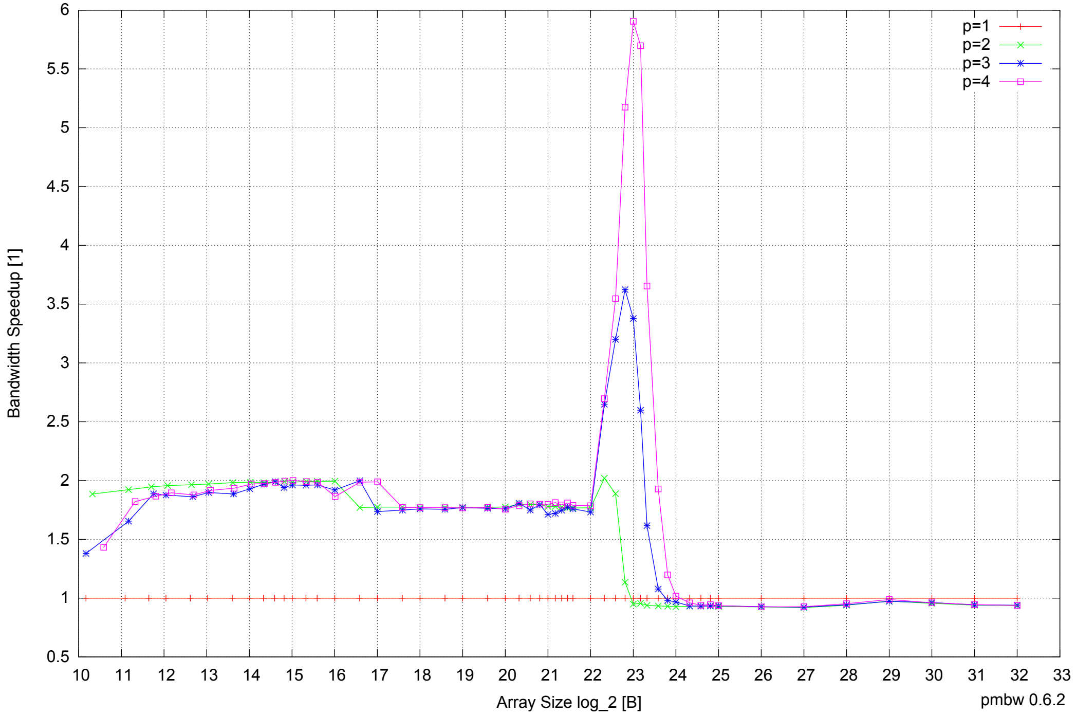
Intel Core 2 Duo E8500 8GB - Speedup of Parallel Memory Bandwidth - ScanWrite64IndexSimpleLoop
