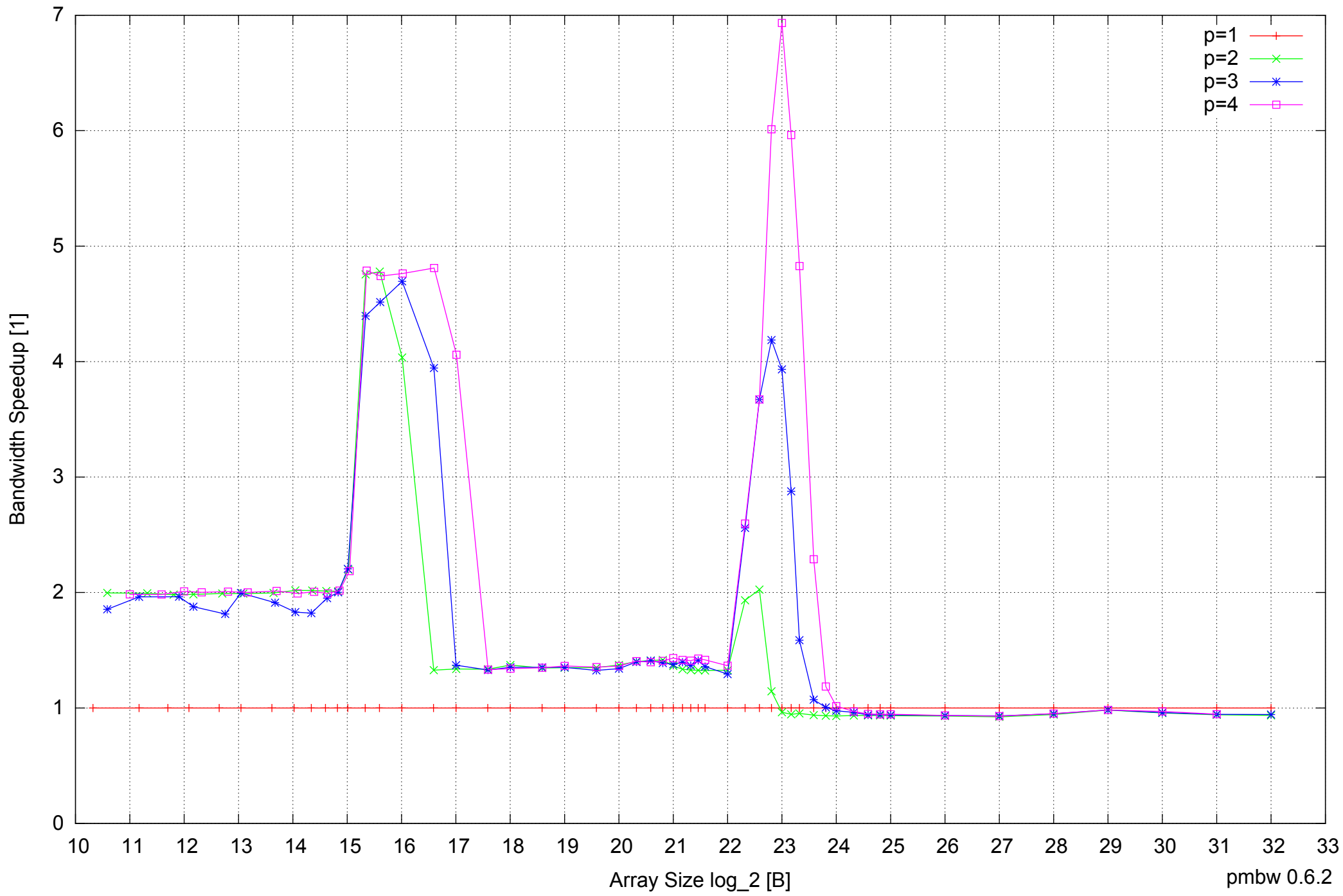
Intel Core 2 Duo E8500 8GB - Speedup of Parallel Memory Bandwidth - ScanWrite128PtrUnrollLoop
