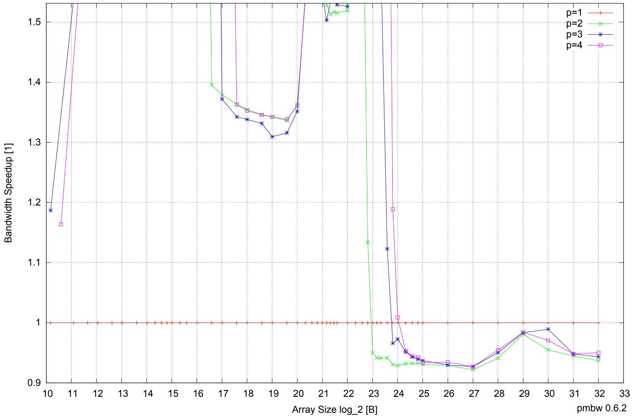
Intel Core 2 Duo E8500 8GB - Speedup of Parallel Memory Bandwidth (enlarged) - ScanWrite64PtrSimpleLoop
