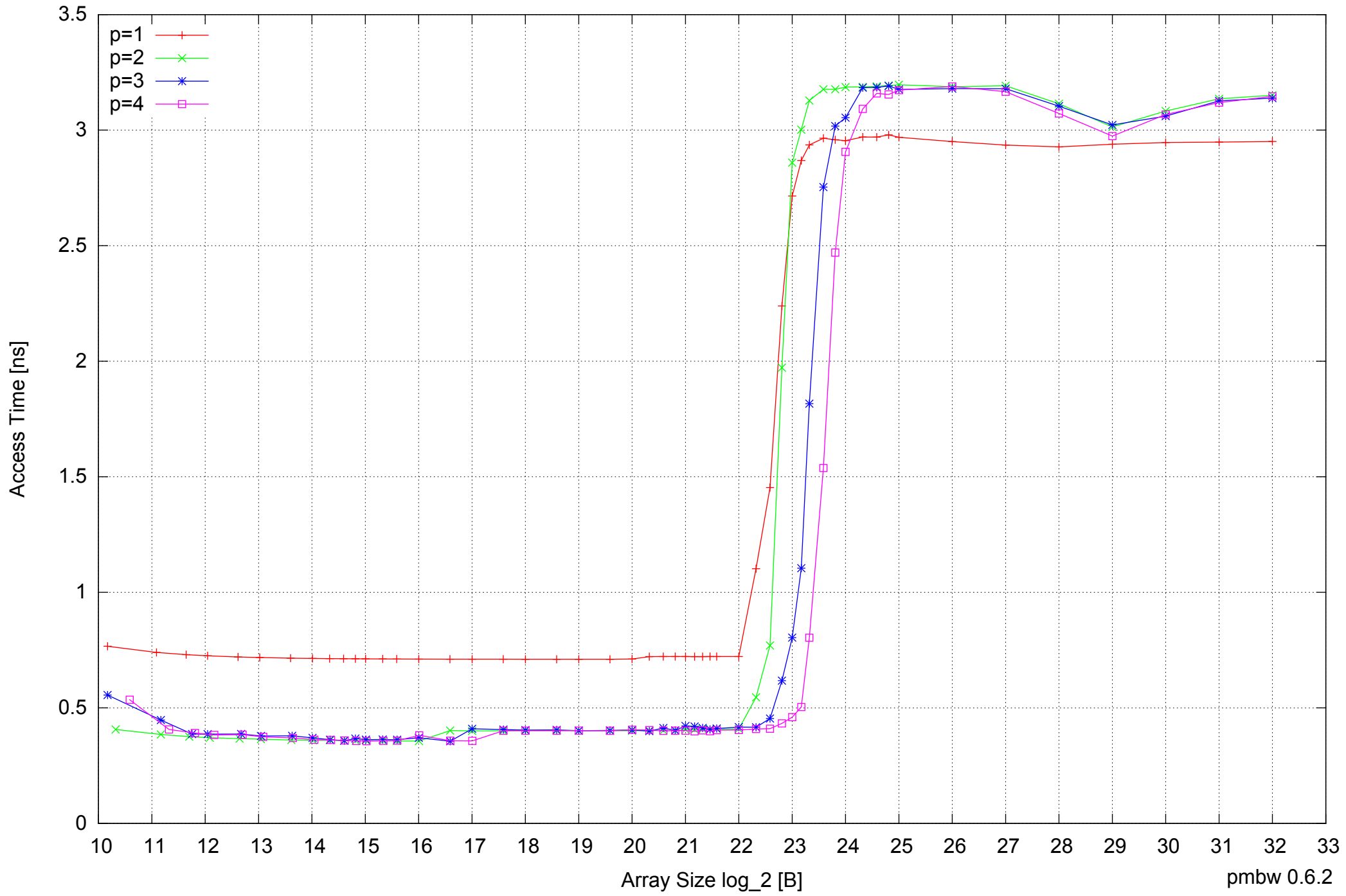
Intel Core 2 Duo E8500 8GB - Parallel Memory Access Time - ScanWrite64IndexSimpleLoop
