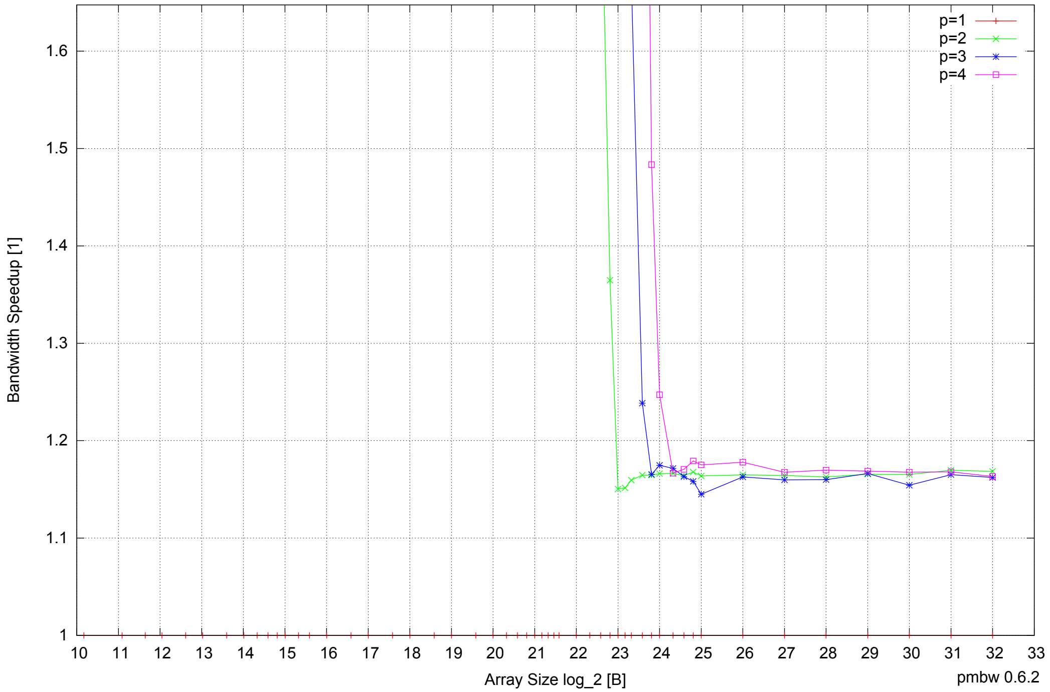
Intel Core 2 Duo E8500 8GB - Speedup of Parallel Memory Bandwidth (enlarged) - ScanRead64PtrUnrollLoop
