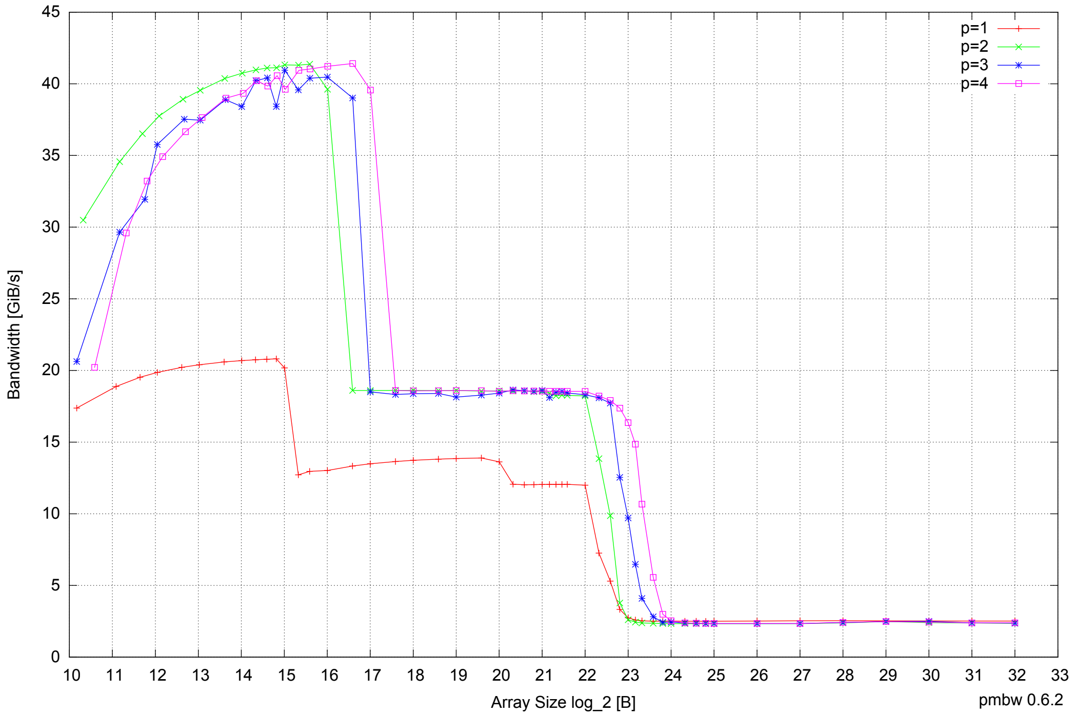
Intel Core 2 Duo E8500 8GB - Parallel Memory Bandwidth - ScanWrite64PtrSimpleLoop
