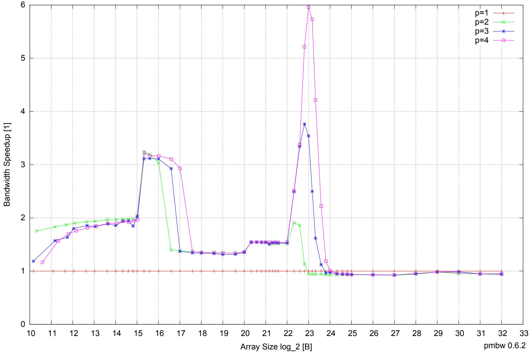
Intel Core 2 Duo E8500 8GB - Speedup of Parallel Memory Bandwidth - ScanWrite64PtrSimpleLoop
