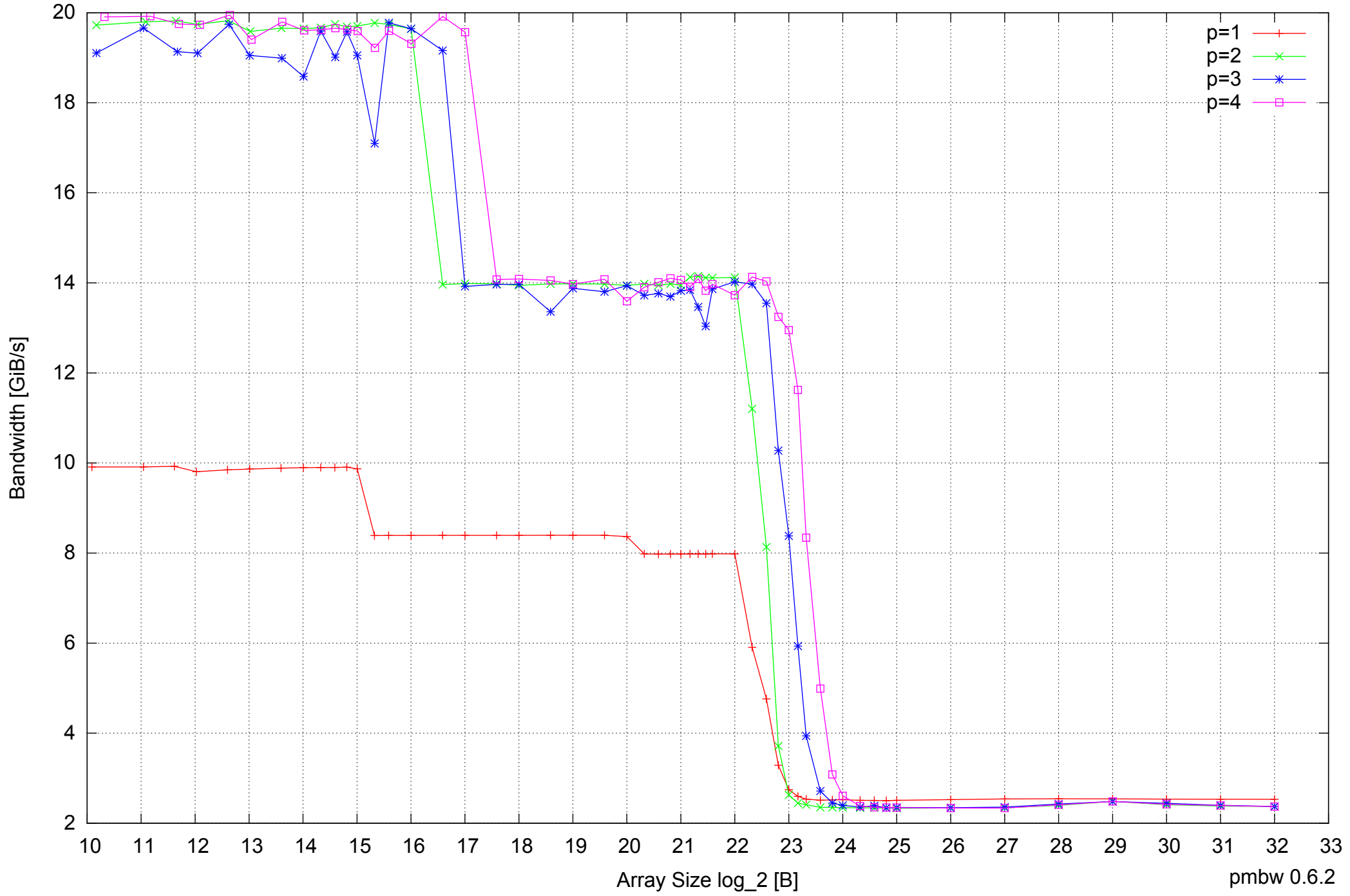
Intel Core 2 Duo E8500 8GB - Parallel Memory Bandwidth - ScanWrite32PtrUnrollLoop
