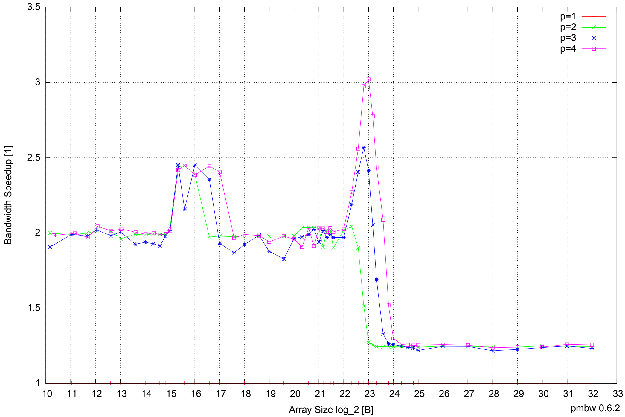
Intel Core 2 Duo E8500 8GB - Speedup of Parallel Memory Bandwidth - ScanRead32PtrUnrollLoop
