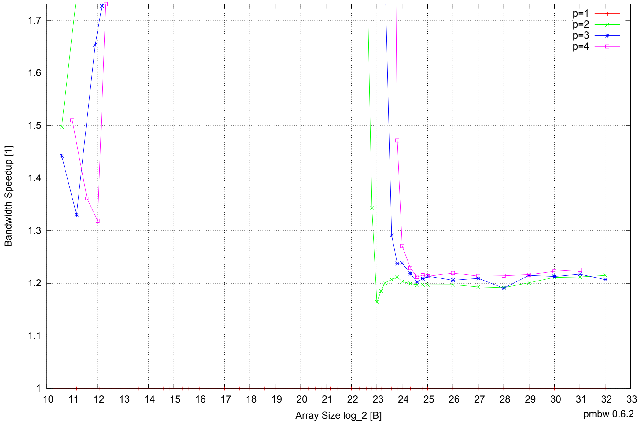
Intel Core 2 Duo E8500 8GB - Speedup of Parallel Memory Bandwidth (enlarged) - ScanRead128PtrSimpleLoop
