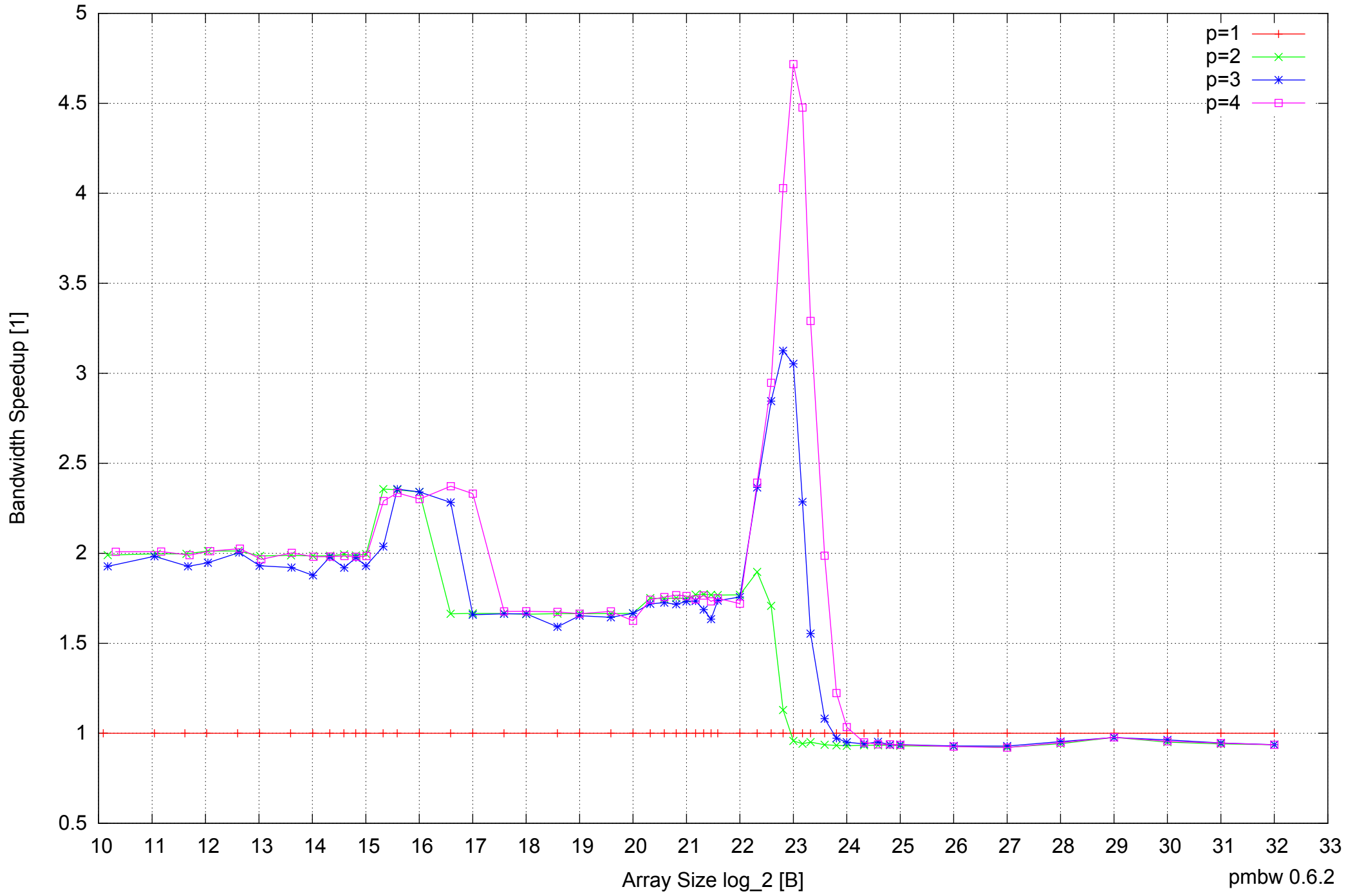
Intel Core 2 Duo E8500 8GB - Speedup of Parallel Memory Bandwidth - ScanWrite32PtrUnrollLoop
