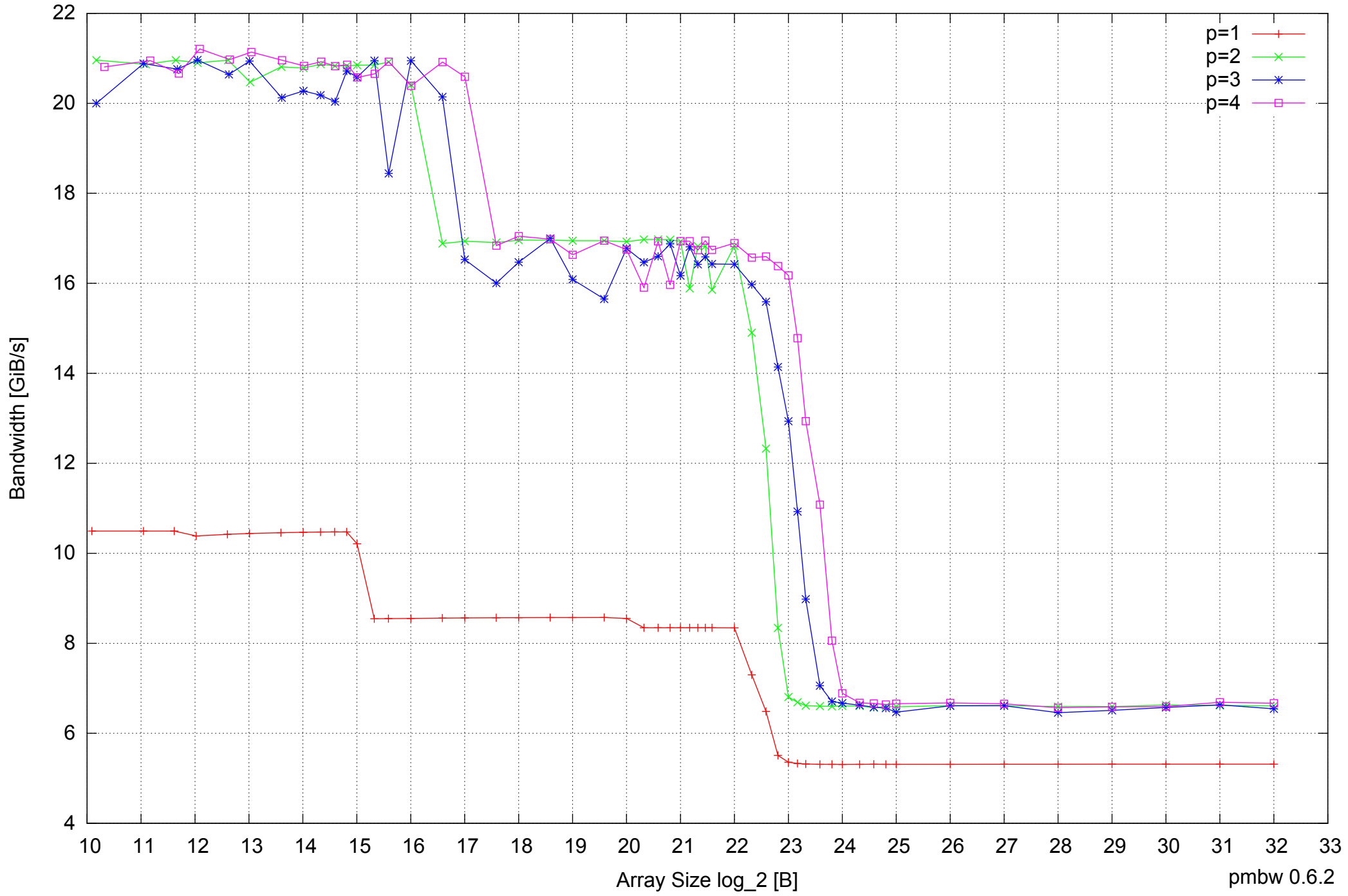
Intel Core 2 Duo E8500 8GB - Parallel Memory Bandwidth - ScanRead32PtrUnrollLoop
