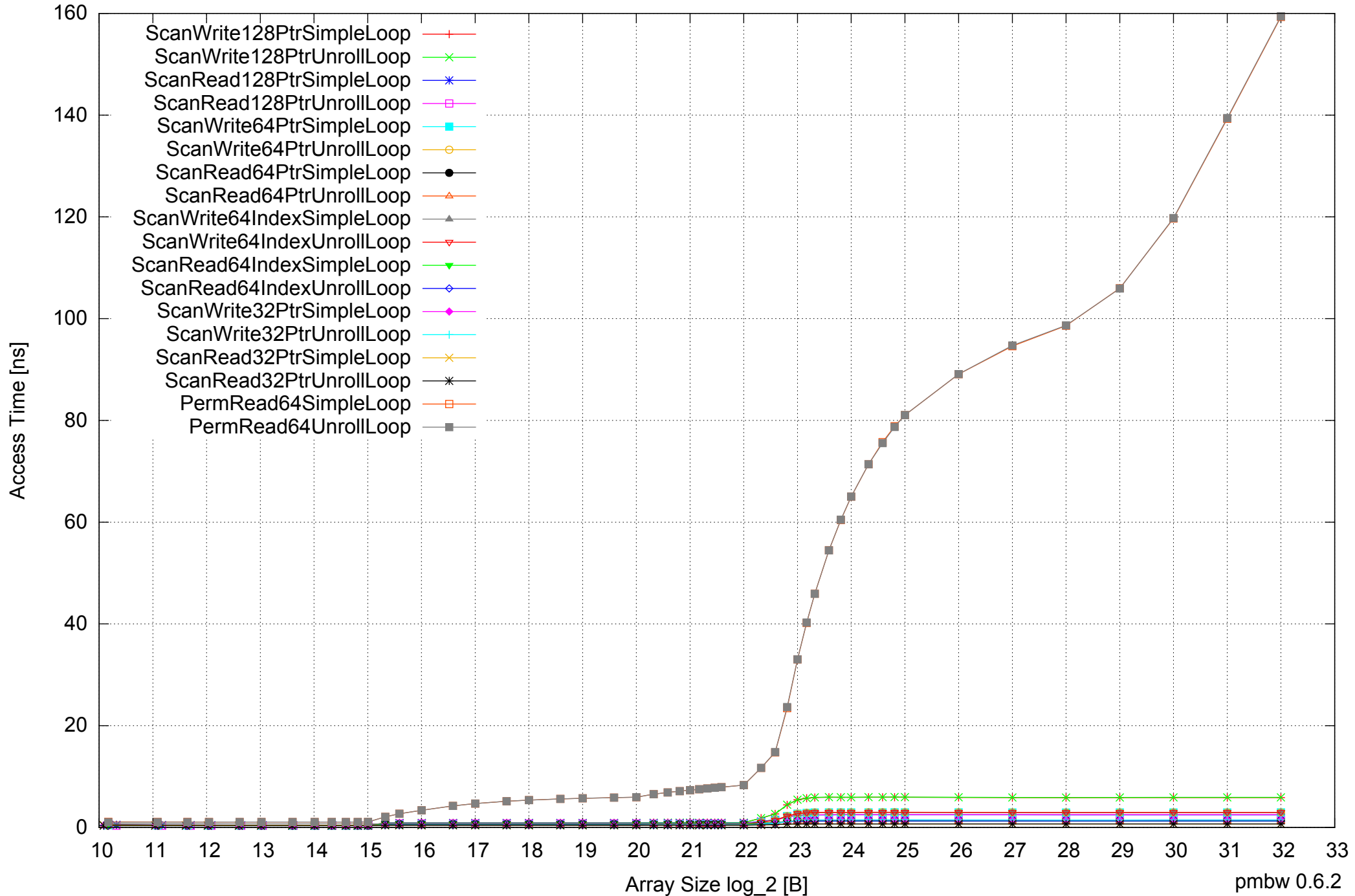
Intel Core 2 Duo E8500 8GB - One Thread Memory Latency (Access Time)
