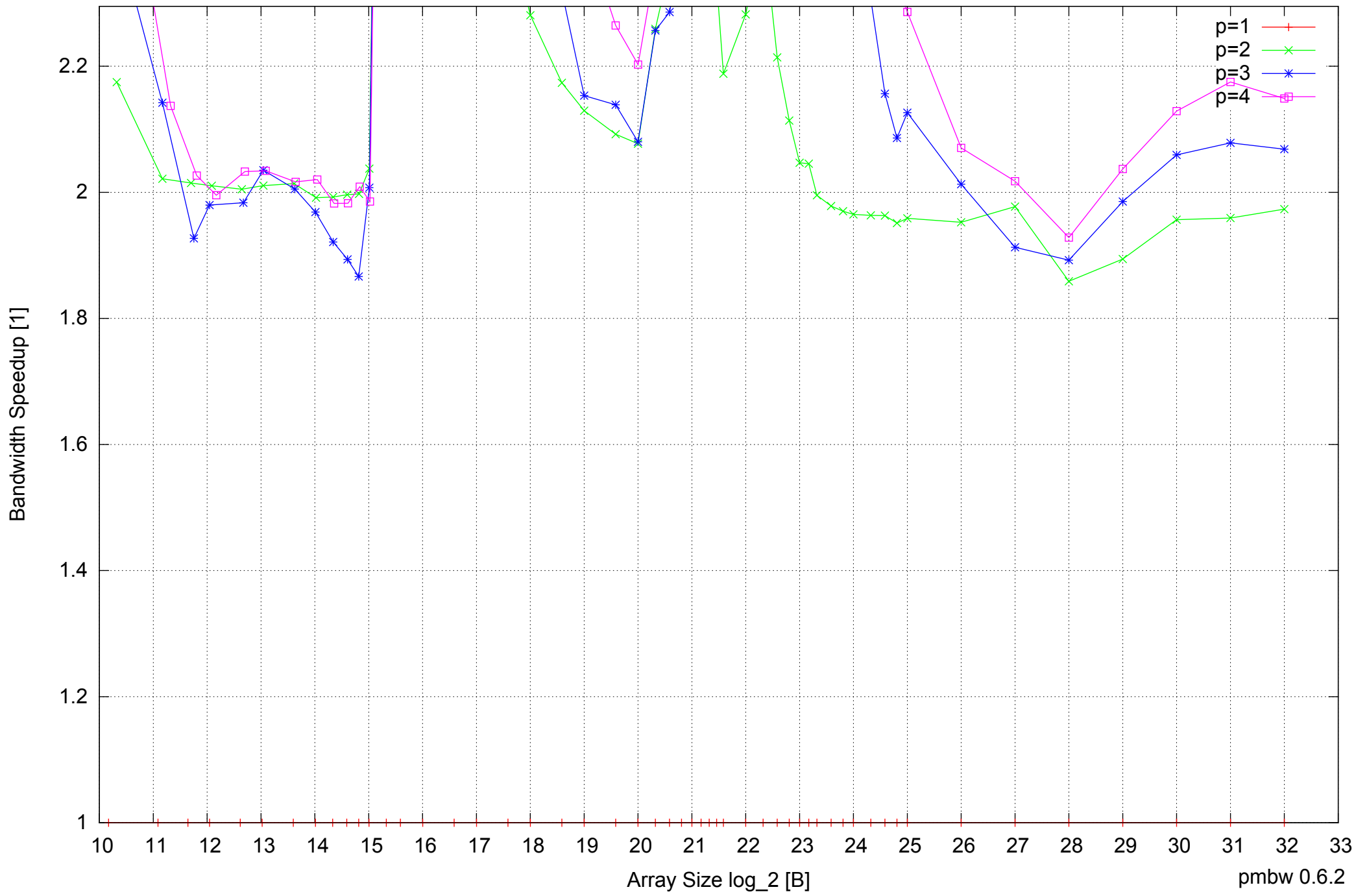
Intel Core 2 Duo E8500 8GB - Speedup of Parallel Memory Bandwidth (enlarged) - PermRead64UnrollLoop
