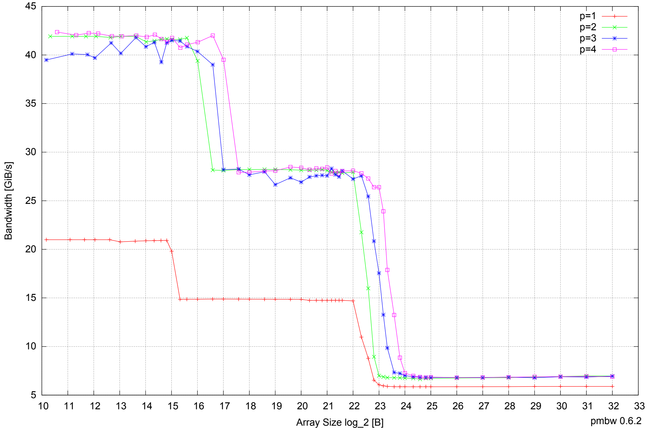
Intel Core 2 Duo E8500 8GB - Parallel Memory Bandwidth - ScanRead64IndexUnrollLoop
