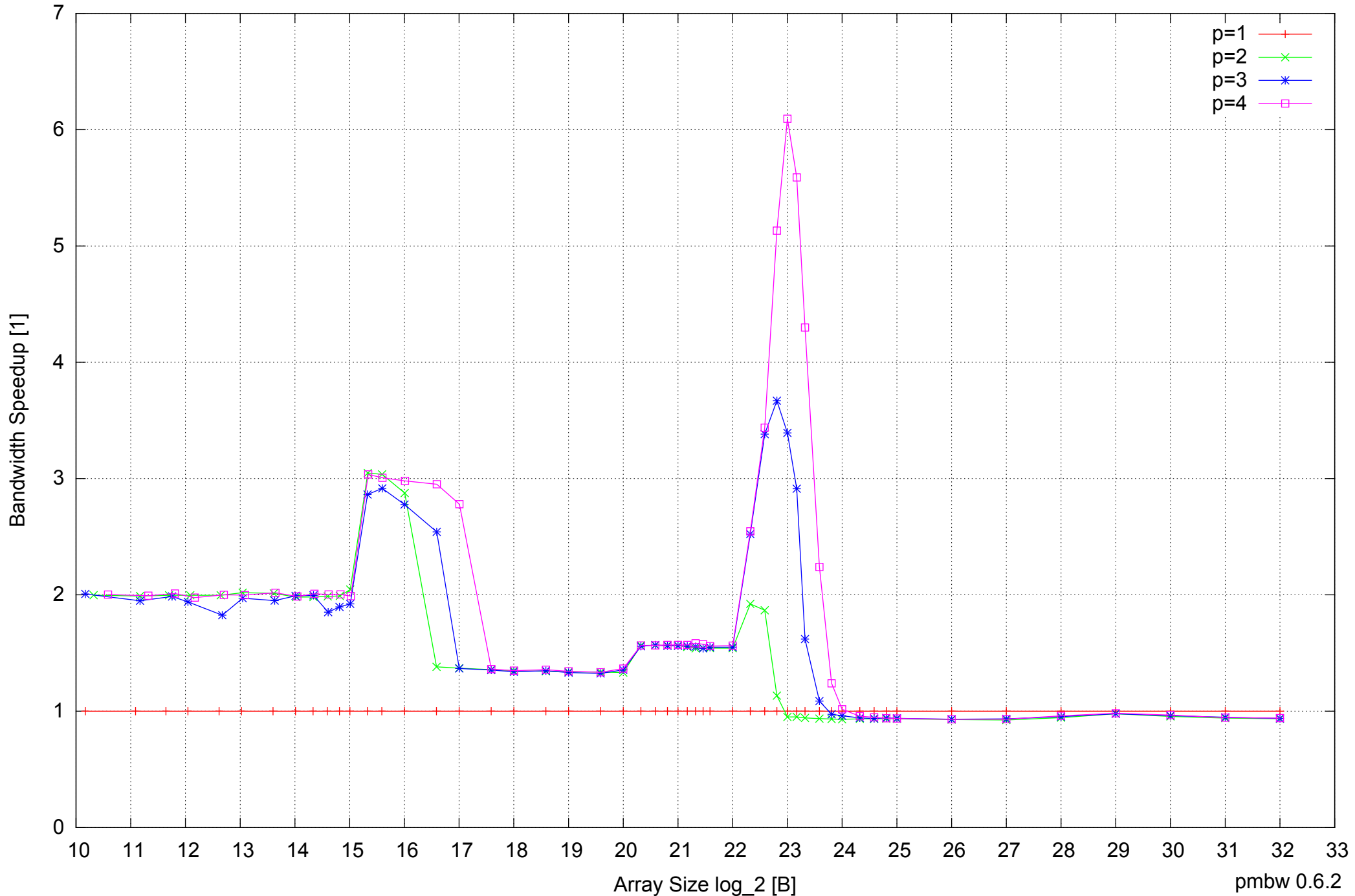
Intel Core 2 Duo E8500 8GB - Speedup of Parallel Memory Bandwidth - ScanWrite64PtrUnrollLoop
