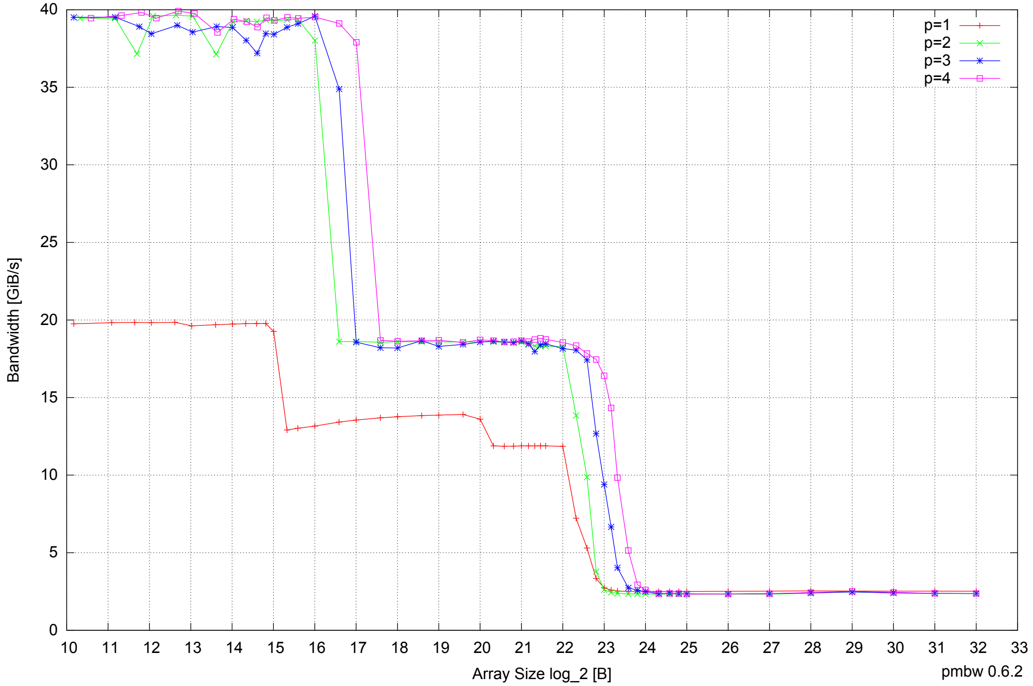
Intel Core 2 Duo E8500 8GB - Parallel Memory Bandwidth - ScanWrite64IndexUnrollLoop
