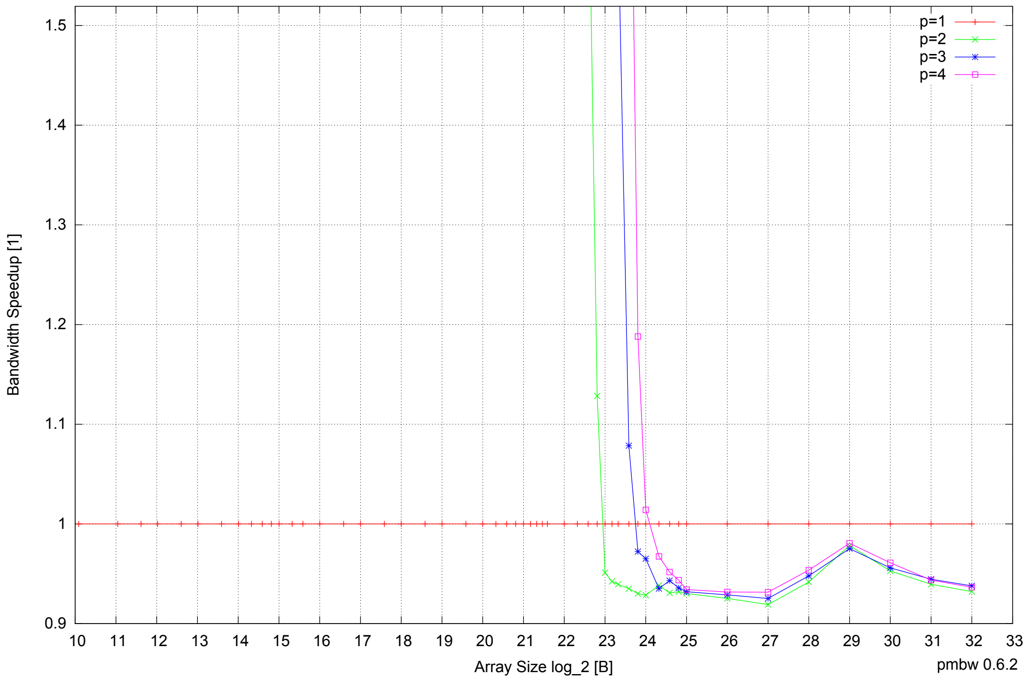
Intel Core 2 Duo E8500 8GB - Speedup of Parallel Memory Bandwidth (enlarged) - ScanWrite32PtrSimpleLoop
