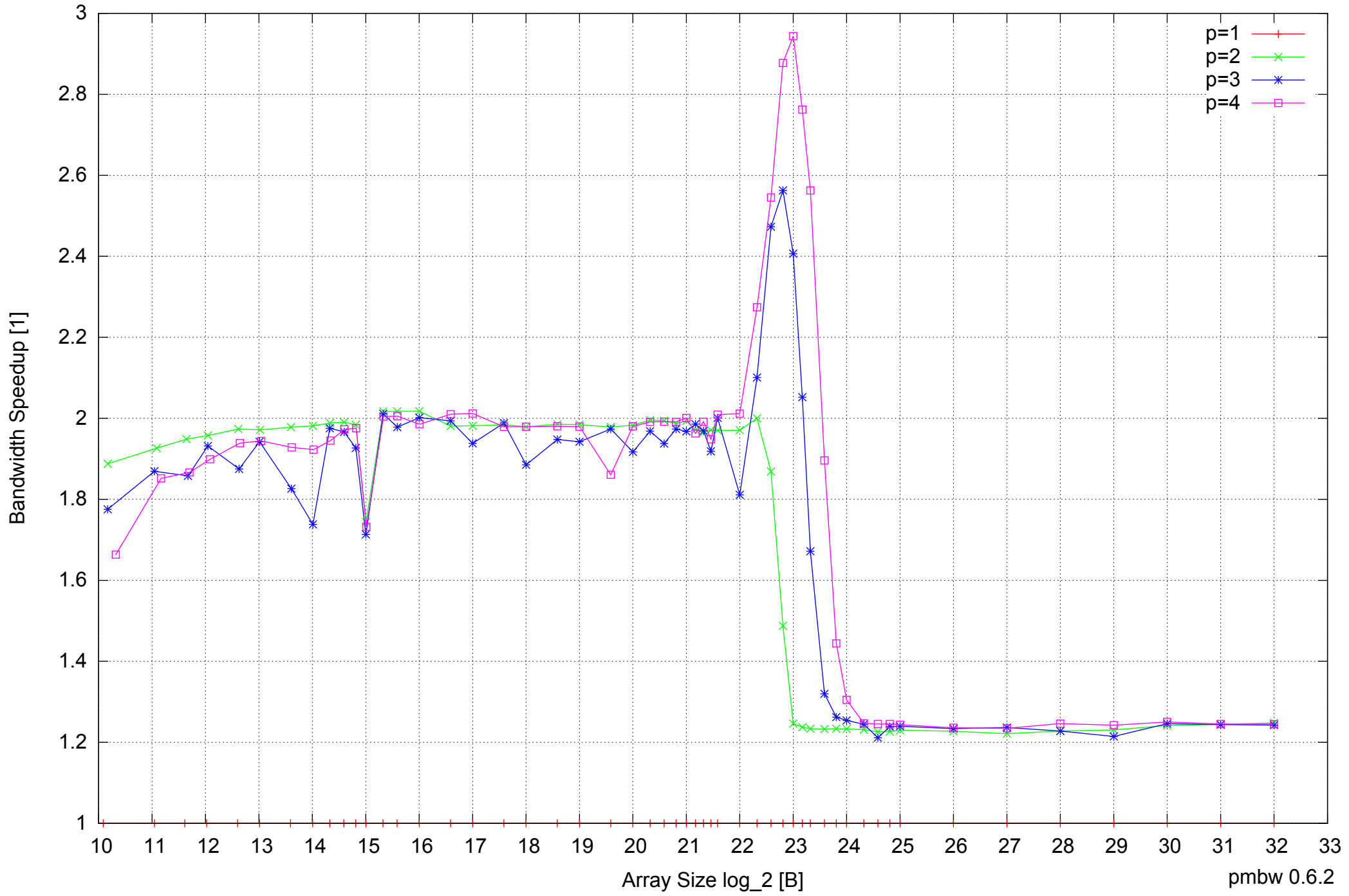
Intel Core 2 Duo E8500 8GB - Speedup of Parallel Memory Bandwidth - ScanRead32PtrSimpleLoop
