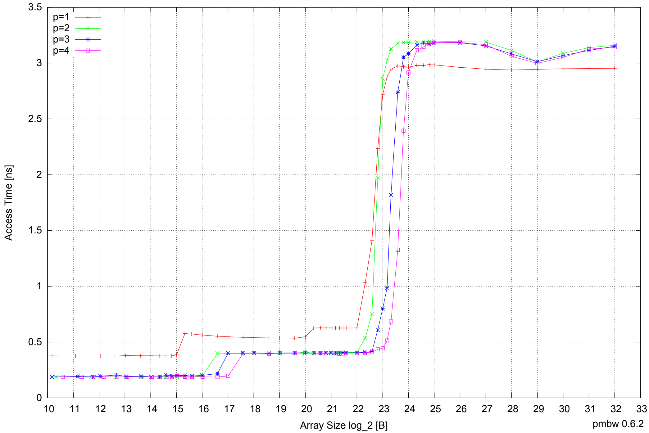
Intel Core 2 Duo E8500 8GB - Parallel Memory Access Time - ScanWrite64PtrUnrollLoop
