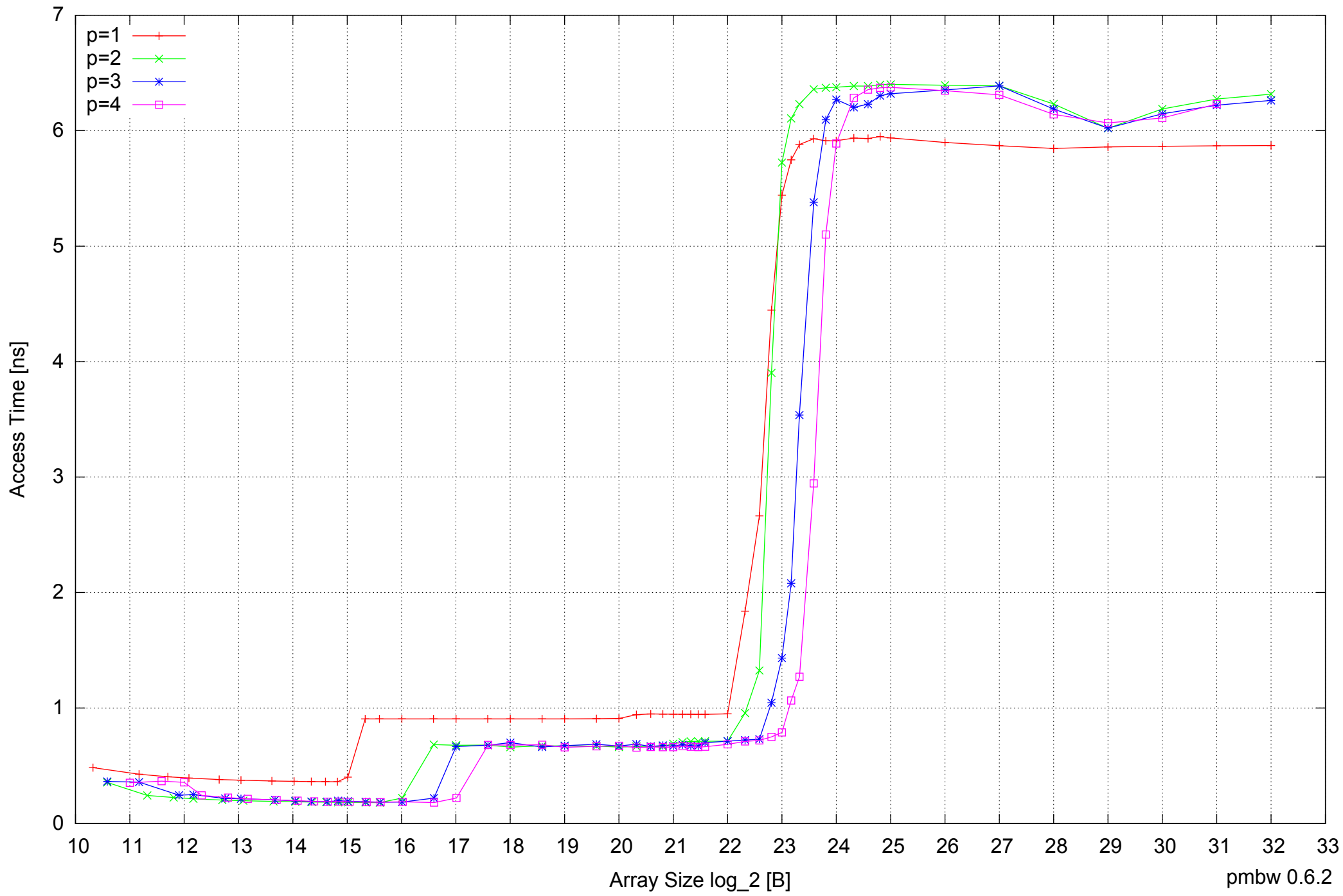
Intel Core 2 Duo E8500 8GB - Parallel Memory Access Time - ScanWrite128PtrSimpleLoop
