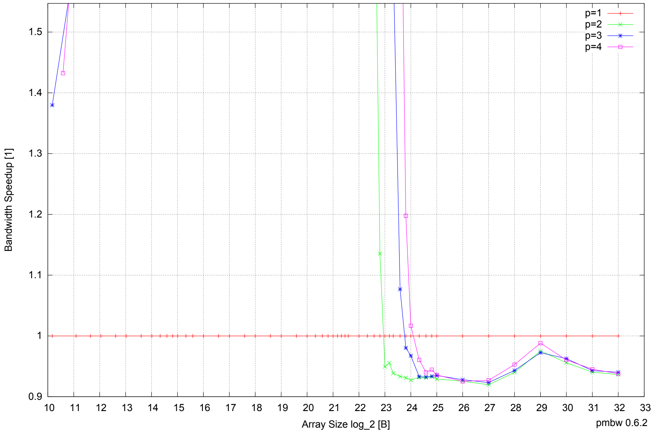
Intel Core 2 Duo E8500 8GB - Speedup of Parallel Memory Bandwidth (enlarged) - ScanWrite64IndexSimpleLoop
