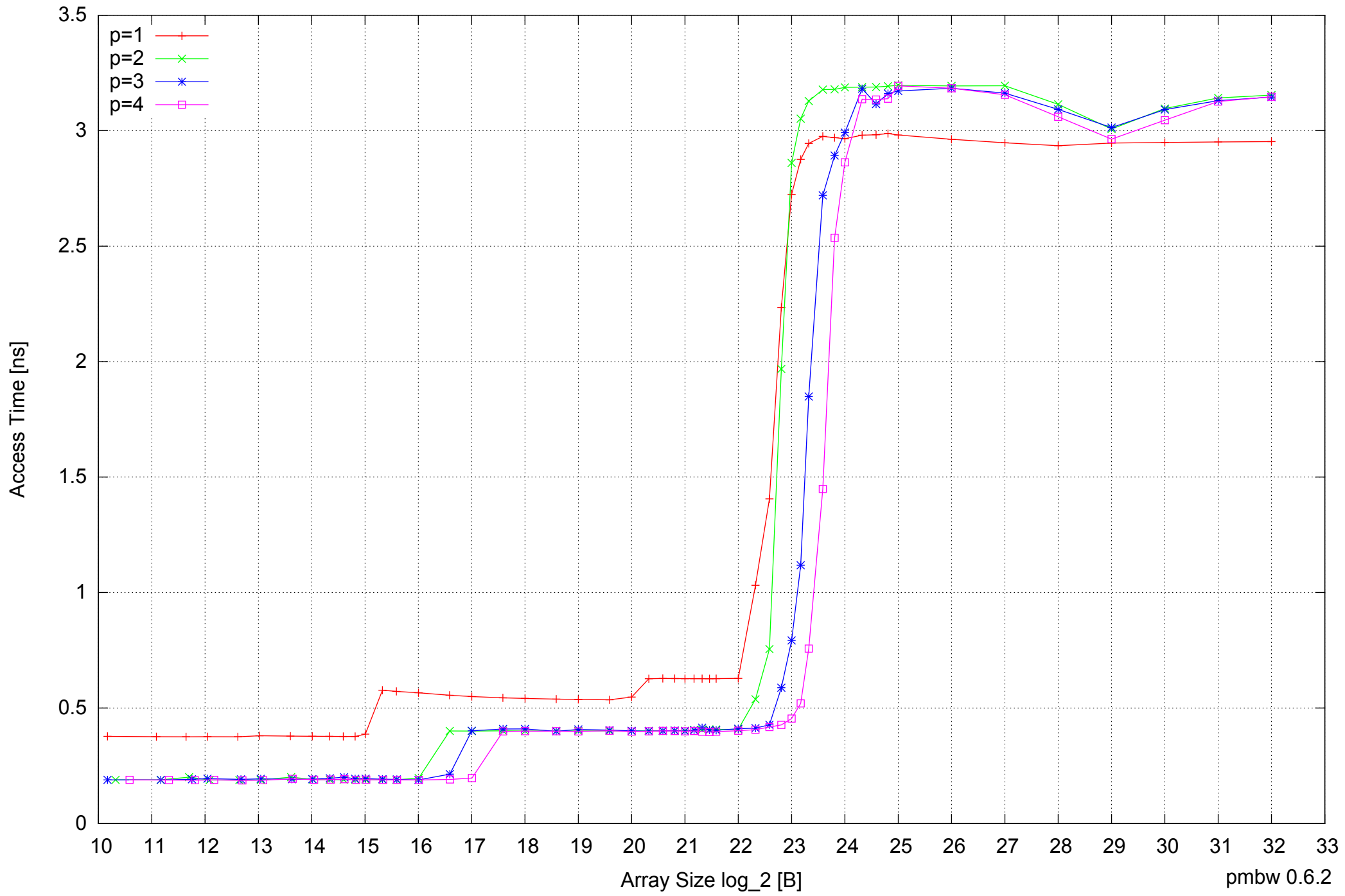
Intel Core 2 Duo E8500 8GB - Parallel Memory Access Time - ScanWrite64IndexUnrollLoop
