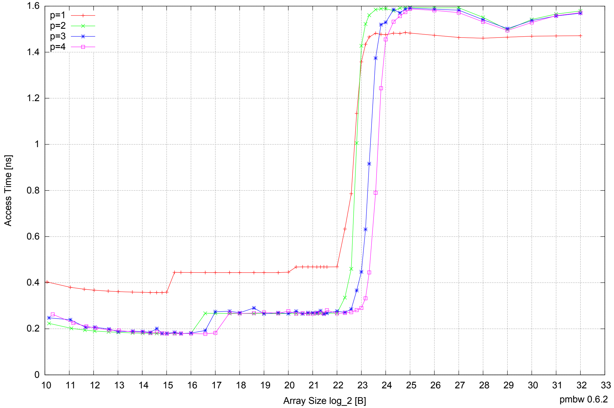
Intel Core 2 Duo E8500 8GB - Parallel Memory Access Time - ScanWrite32PtrSimpleLoop
