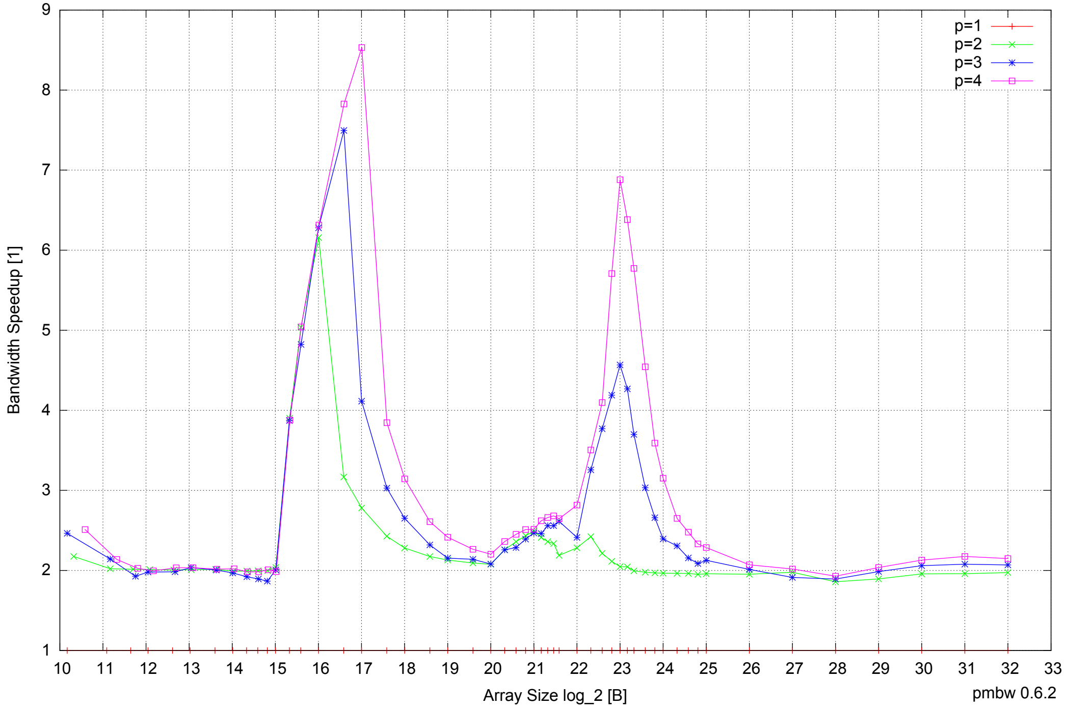
Intel Core 2 Duo E8500 8GB - Speedup of Parallel Memory Bandwidth - PermRead64UnrollLoop
