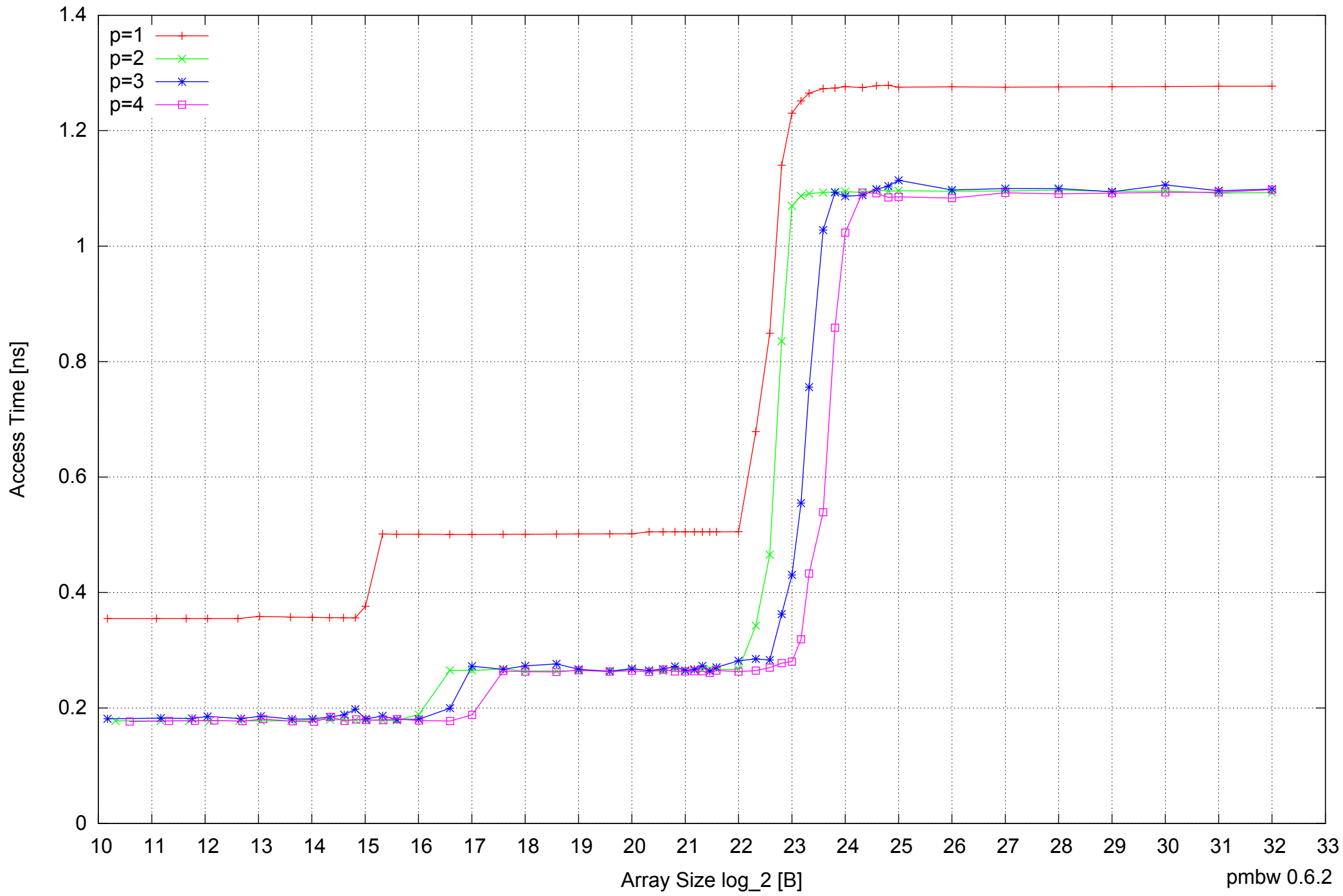
Intel Core 2 Duo E8500 8GB - Parallel Memory Access Time - ScanRead64PtrUnrollLoop
