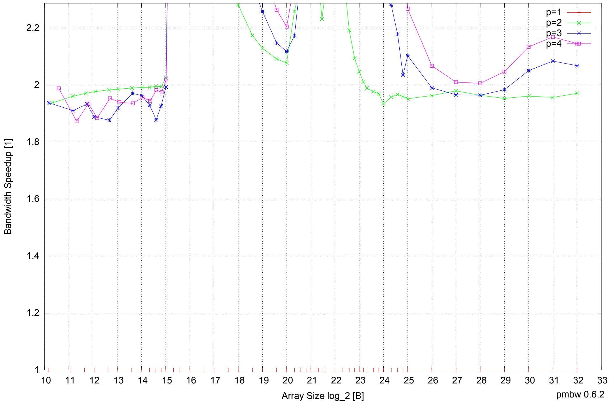
Intel Core 2 Duo E8500 8GB - Speedup of Parallel Memory Bandwidth (enlarged) - PermRead64SimpleLoop
