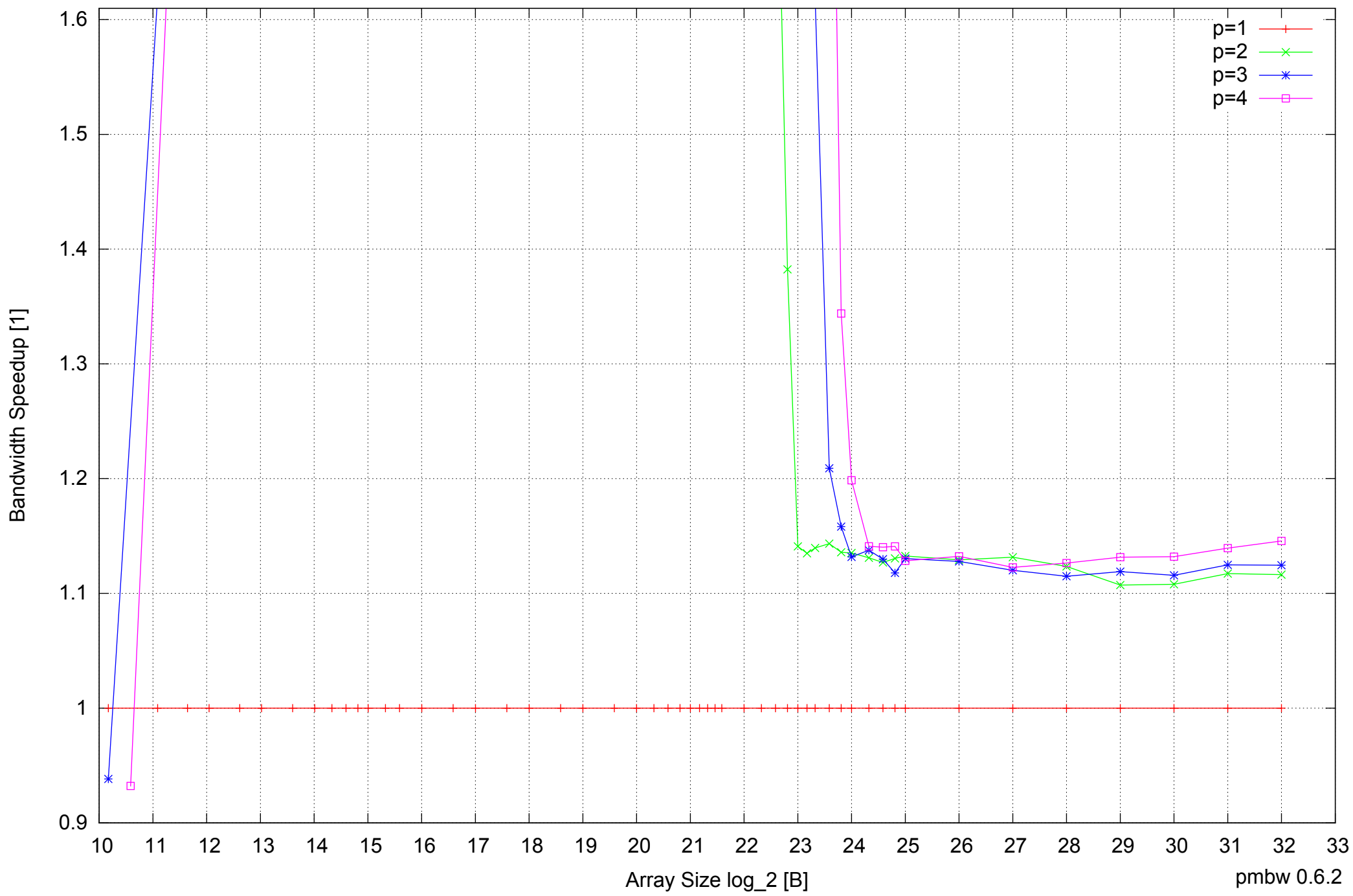
Intel Core 2 Duo E8500 8GB - Speedup of Parallel Memory Bandwidth (enlarged) - ScanRead64PtrSimpleLoop
