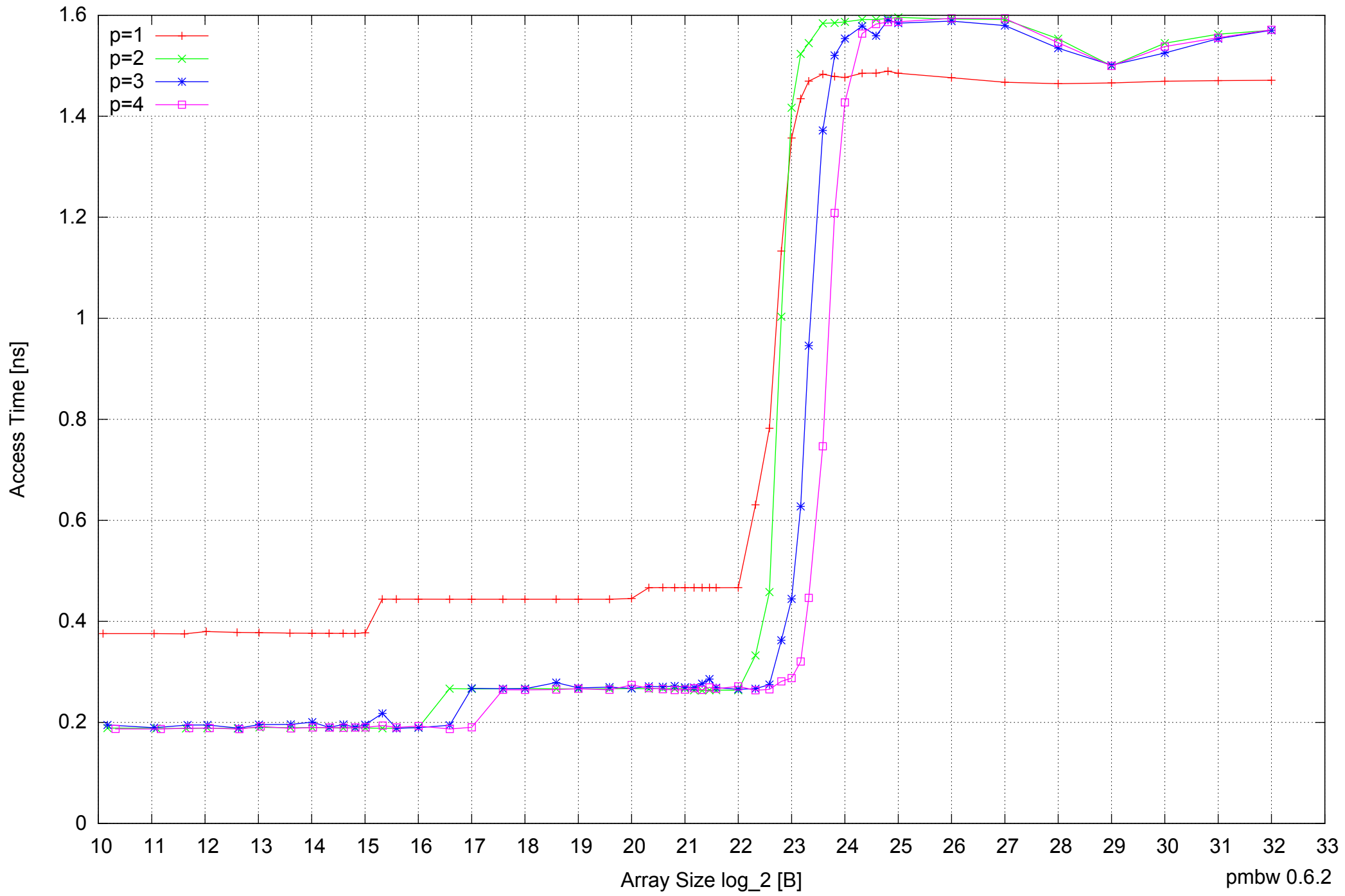
Intel Core 2 Duo E8500 8GB - Parallel Memory Access Time - ScanWrite32PtrUnrollLoop
