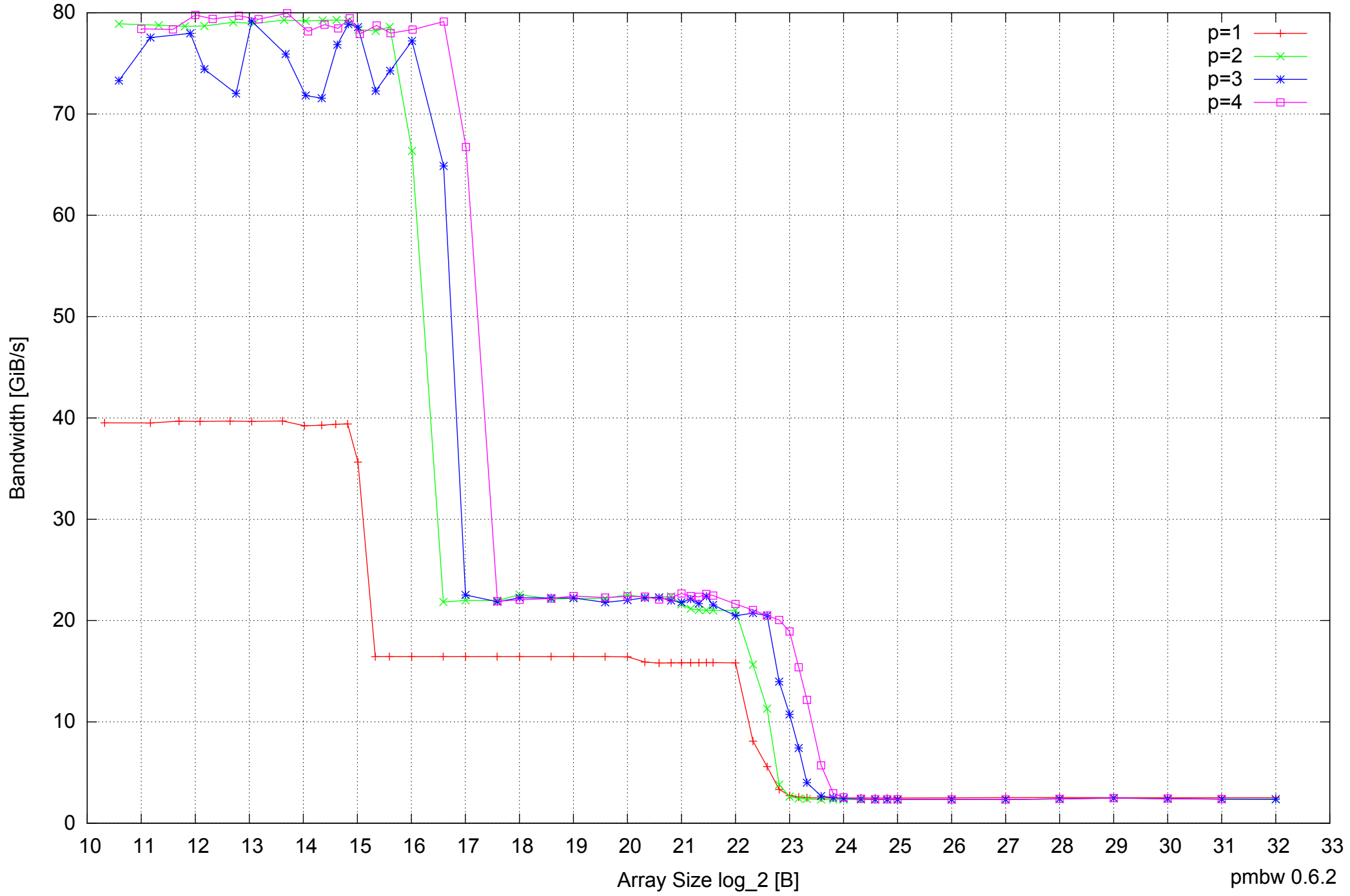
Intel Core 2 Duo E8500 8GB - Parallel Memory Bandwidth - ScanWrite128PtrUnrollLoop
