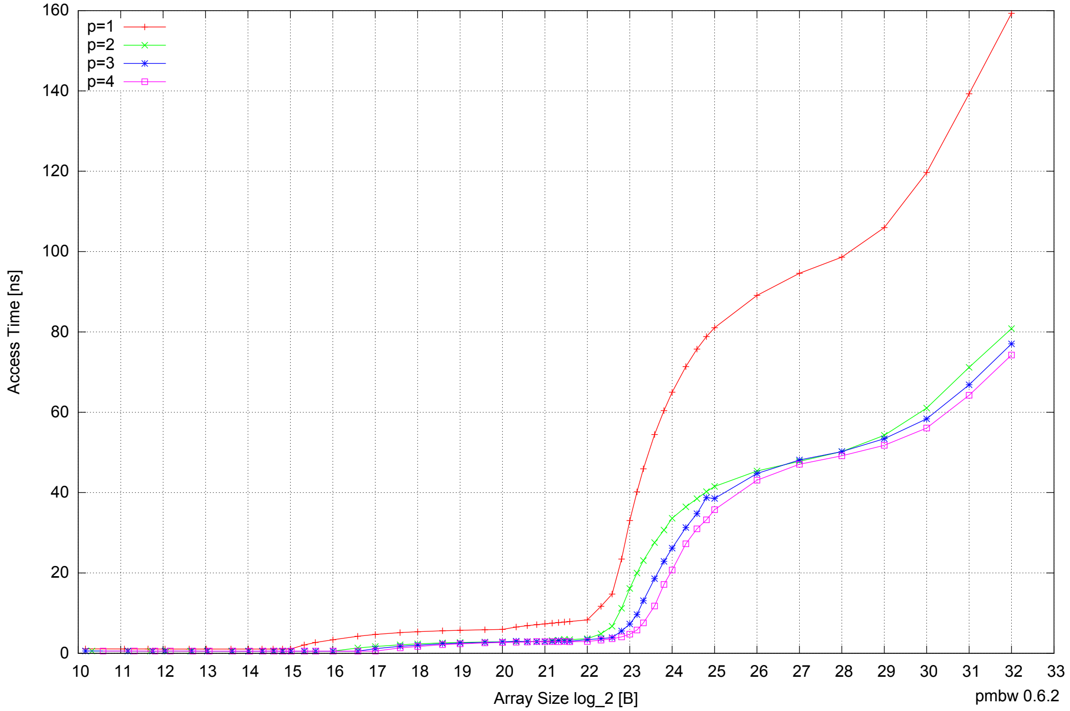
Intel Core 2 Duo E8500 8GB - Parallel Memory Access Time - PermRead64SimpleLoop
