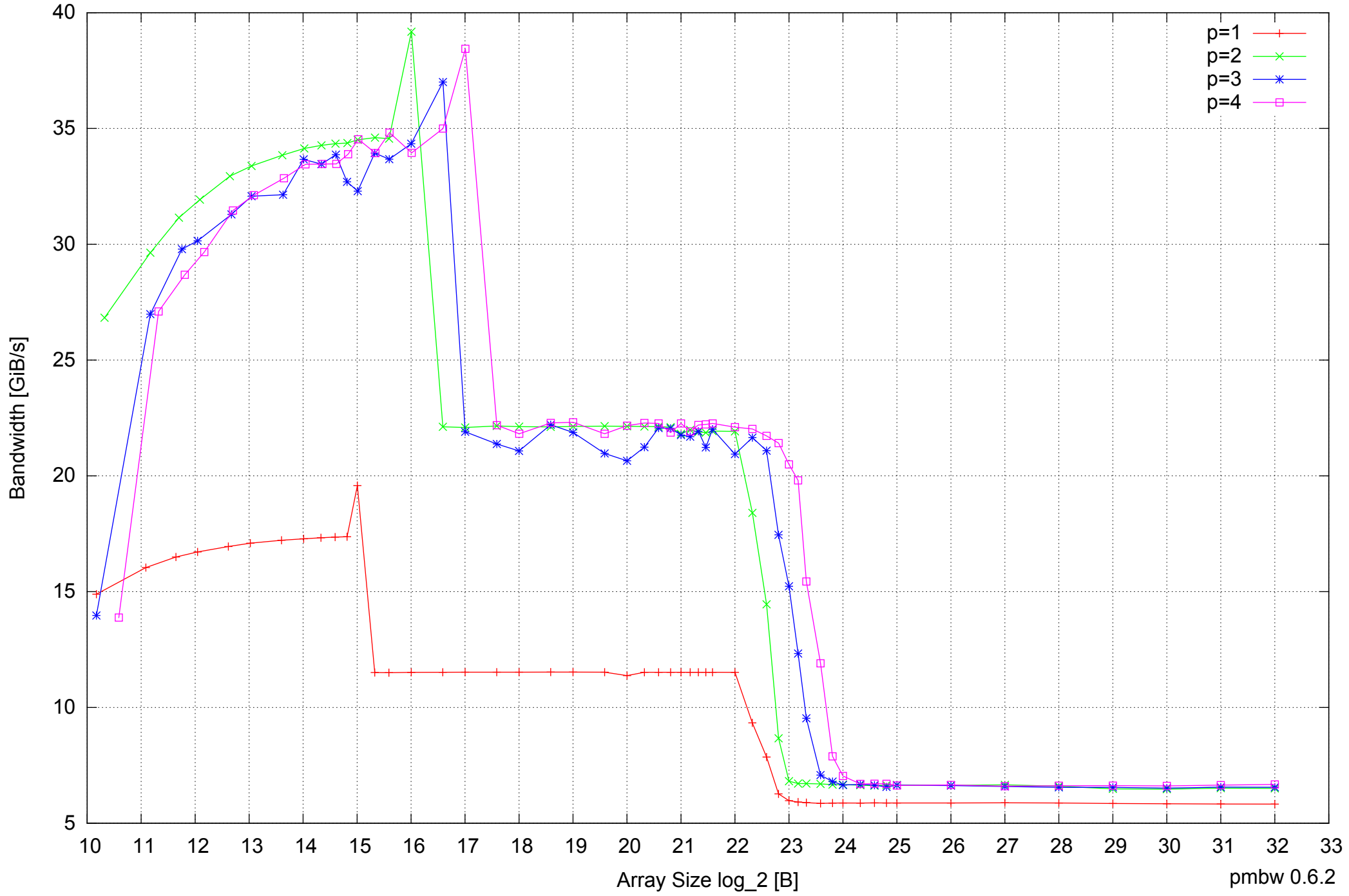
Intel Core 2 Duo E8500 8GB - Parallel Memory Bandwidth - ScanRead64PtrSimpleLoop
