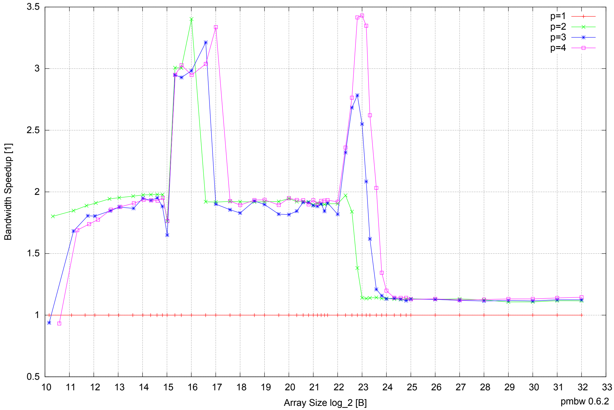
Intel Core 2 Duo E8500 8GB - Speedup of Parallel Memory Bandwidth - ScanRead64PtrSimpleLoop
