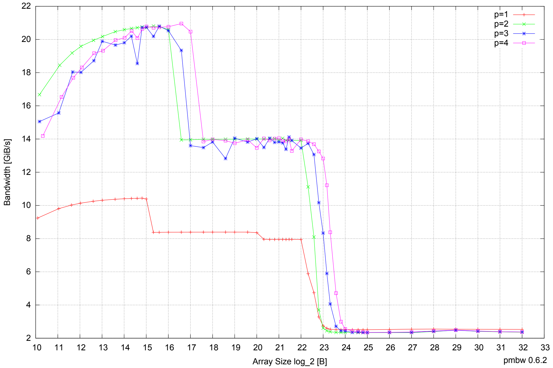
Intel Core 2 Duo E8500 8GB - Parallel Memory Bandwidth - ScanWrite32PtrSimpleLoop
