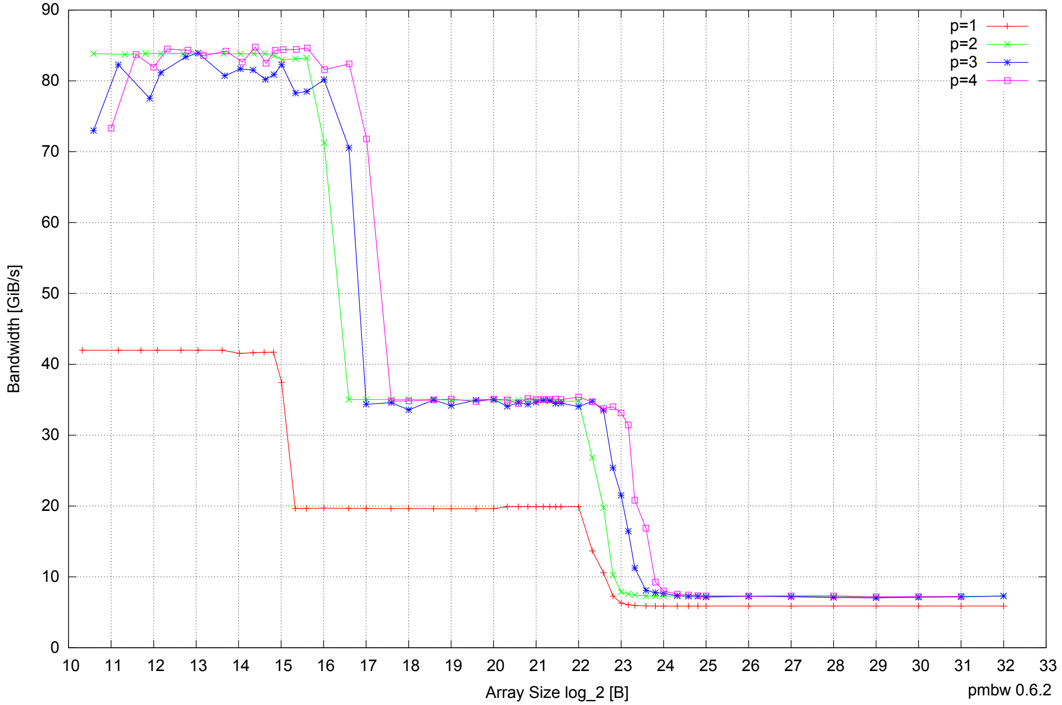
Intel Core 2 Duo E8500 8GB - Parallel Memory Bandwidth - ScanRead128PtrUnrollLoop
