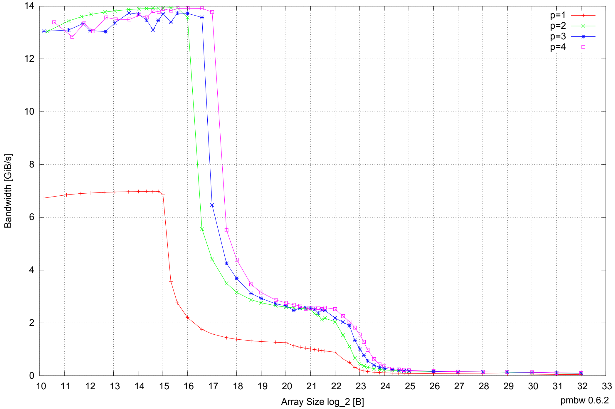
Intel Core 2 Duo E8500 8GB - Parallel Memory Bandwidth - PermRead64SimpleLoop
