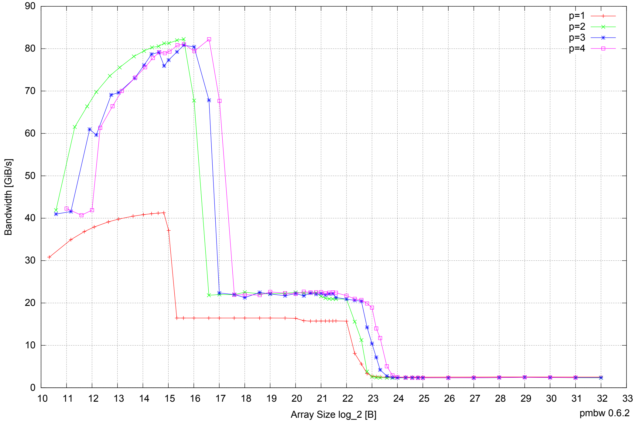
Intel Core 2 Duo E8500 8GB - Parallel Memory Bandwidth - ScanWrite128PtrSimpleLoop
