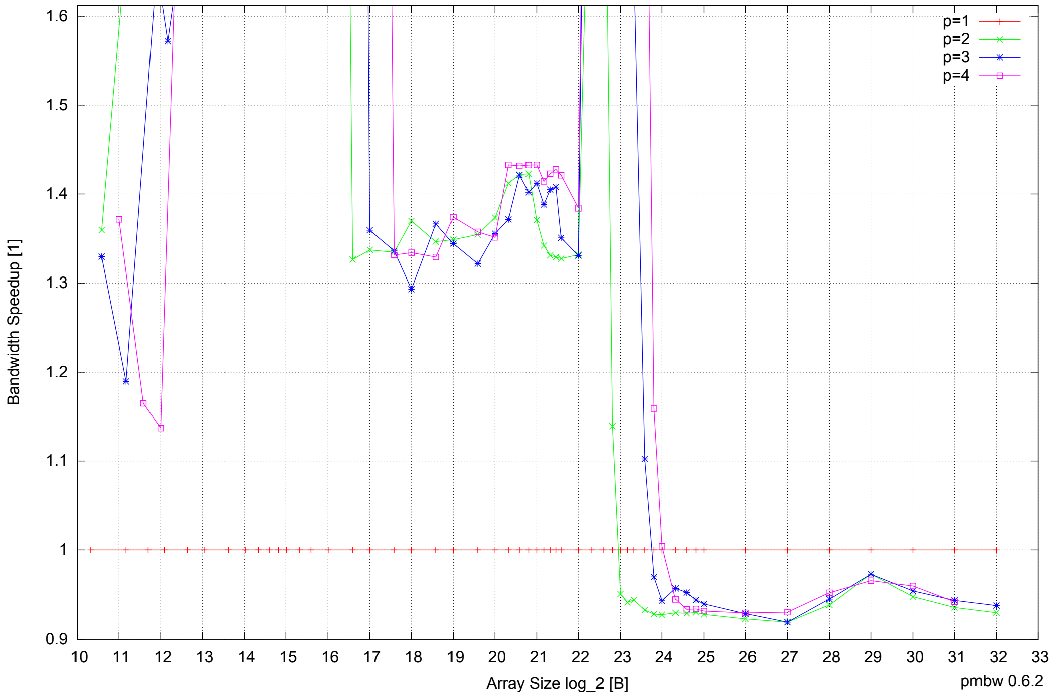
Intel Core 2 Duo E8500 8GB - Speedup of Parallel Memory Bandwidth (enlarged) - ScanWrite128PtrSimpleLoop
