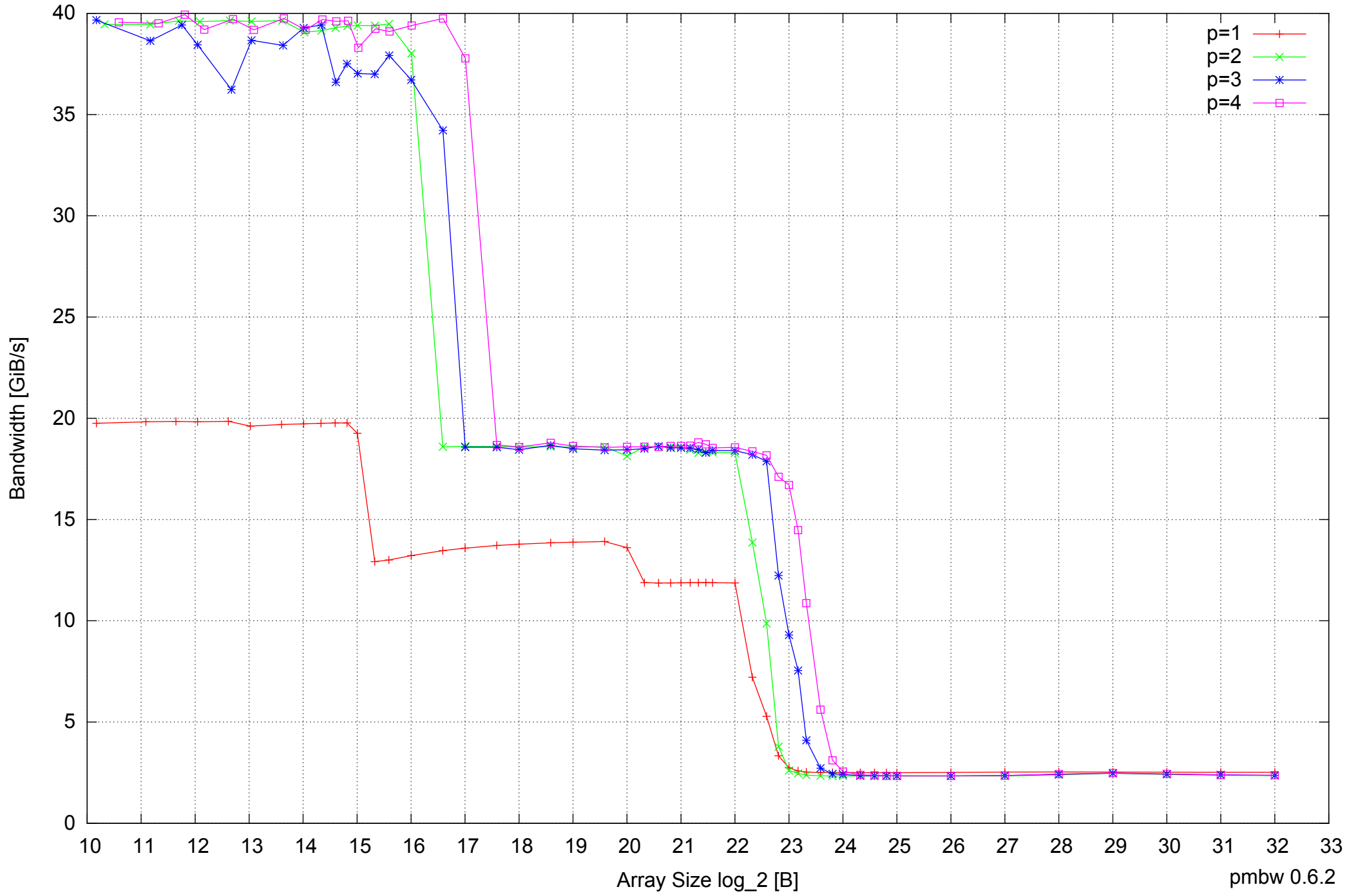
Intel Core 2 Duo E8500 8GB - Parallel Memory Bandwidth - ScanWrite64PtrUnrollLoop
