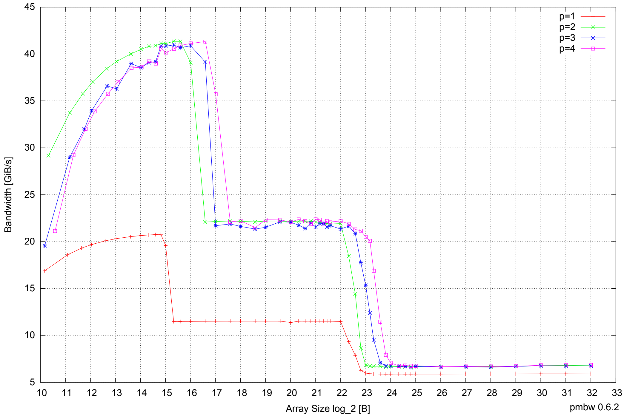
Intel Core 2 Duo E8500 8GB - Parallel Memory Bandwidth - ScanRead64IndexSimpleLoop
