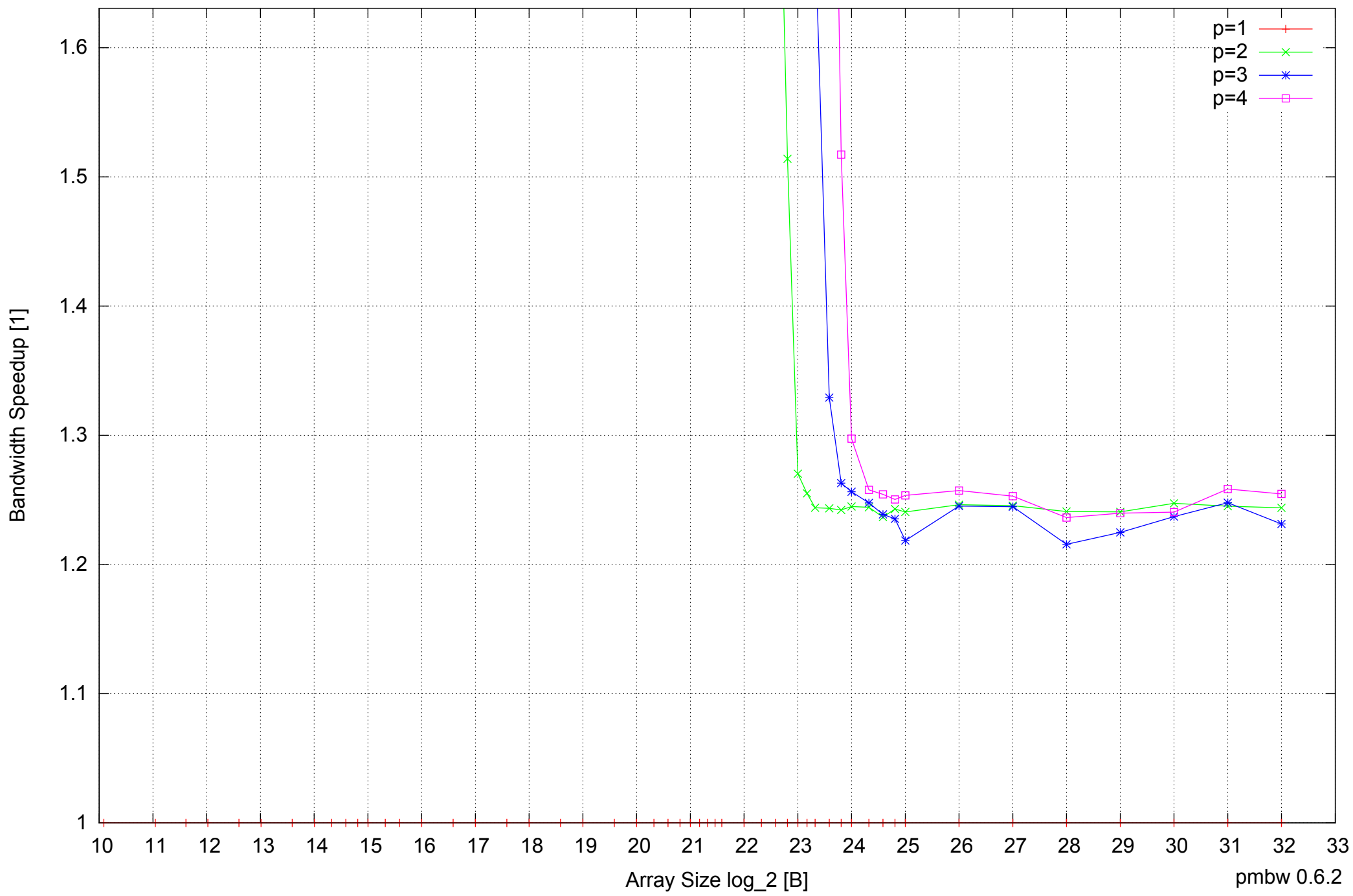
Intel Core 2 Duo E8500 8GB - Speedup of Parallel Memory Bandwidth (enlarged) - ScanRead32PtrUnrollLoop
