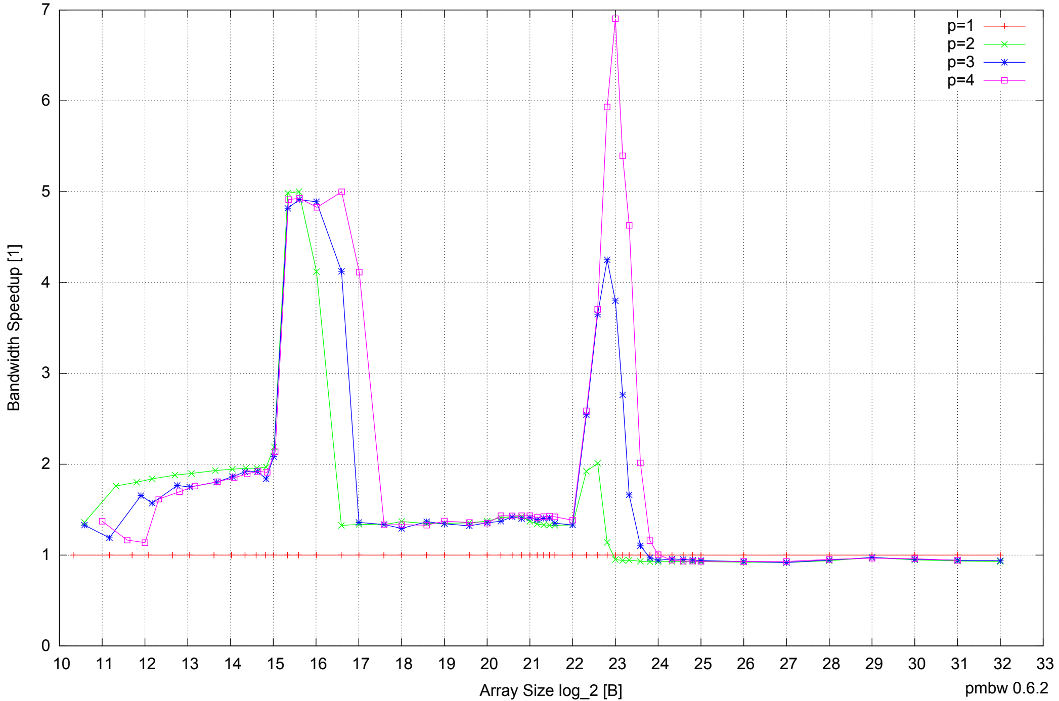
Intel Core 2 Duo E8500 8GB - Speedup of Parallel Memory Bandwidth - ScanWrite128PtrSimpleLoop
