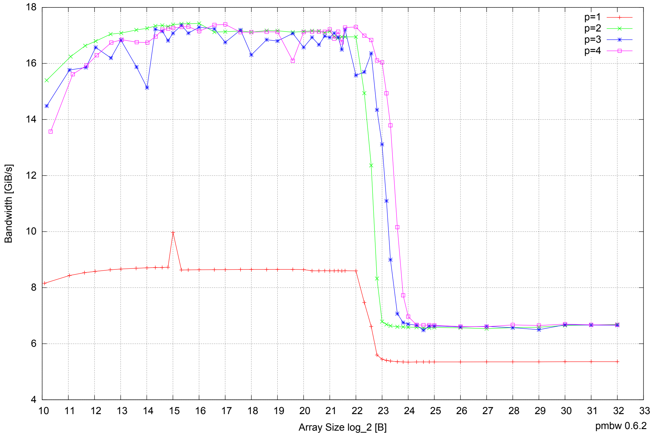
Intel Core 2 Duo E8500 8GB - Parallel Memory Bandwidth - ScanRead32PtrSimpleLoop
