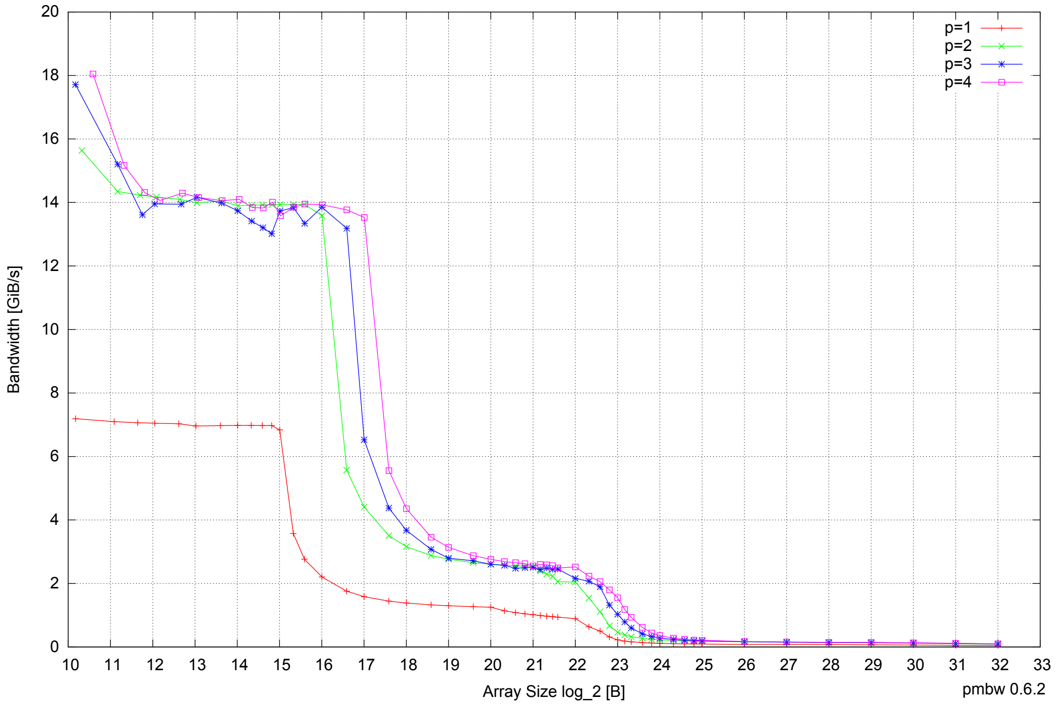
Intel Core 2 Duo E8500 8GB - Parallel Memory Bandwidth - PermRead64UnrollLoop
