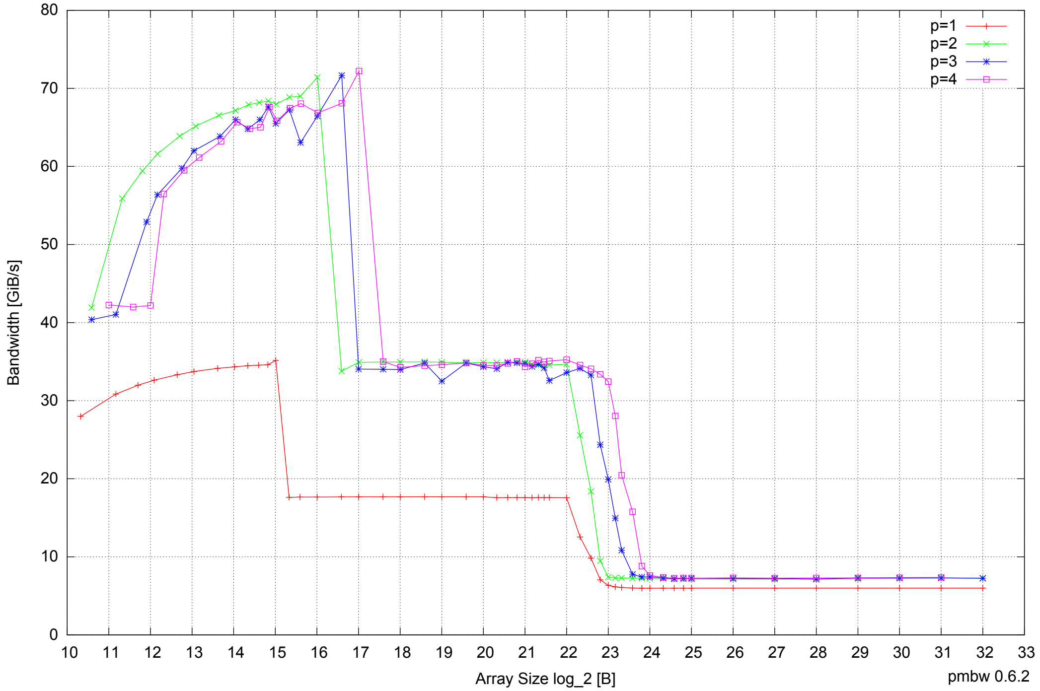
Intel Core 2 Duo E8500 8GB - Parallel Memory Bandwidth - ScanRead128PtrSimpleLoop
