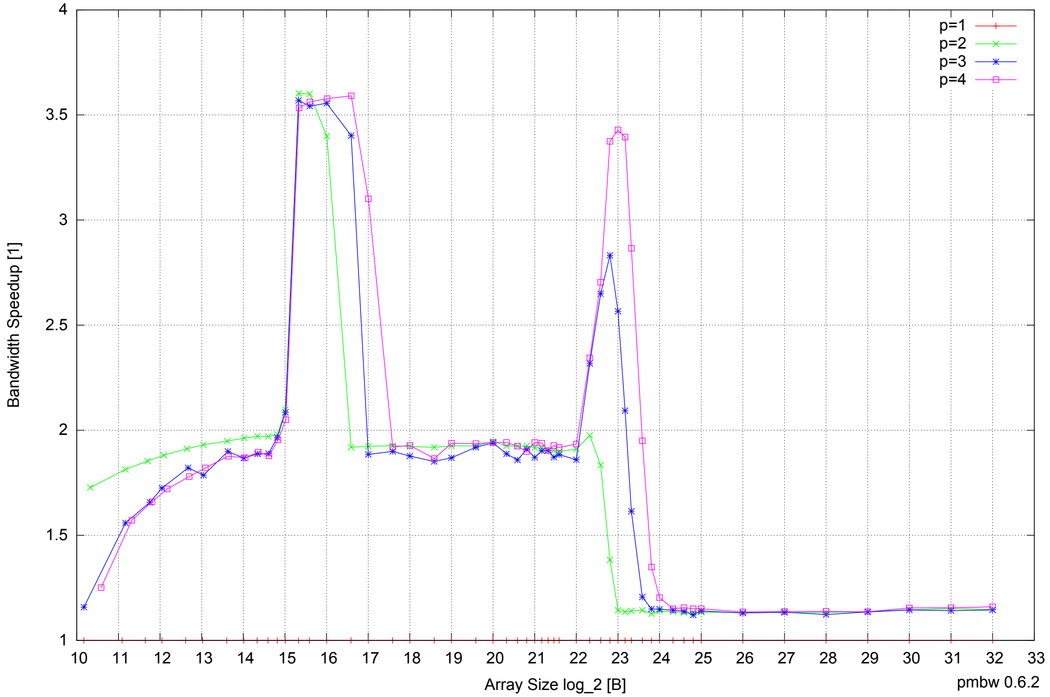
Intel Core 2 Duo E8500 8GB - Speedup of Parallel Memory Bandwidth - ScanRead64IndexSimpleLoop
