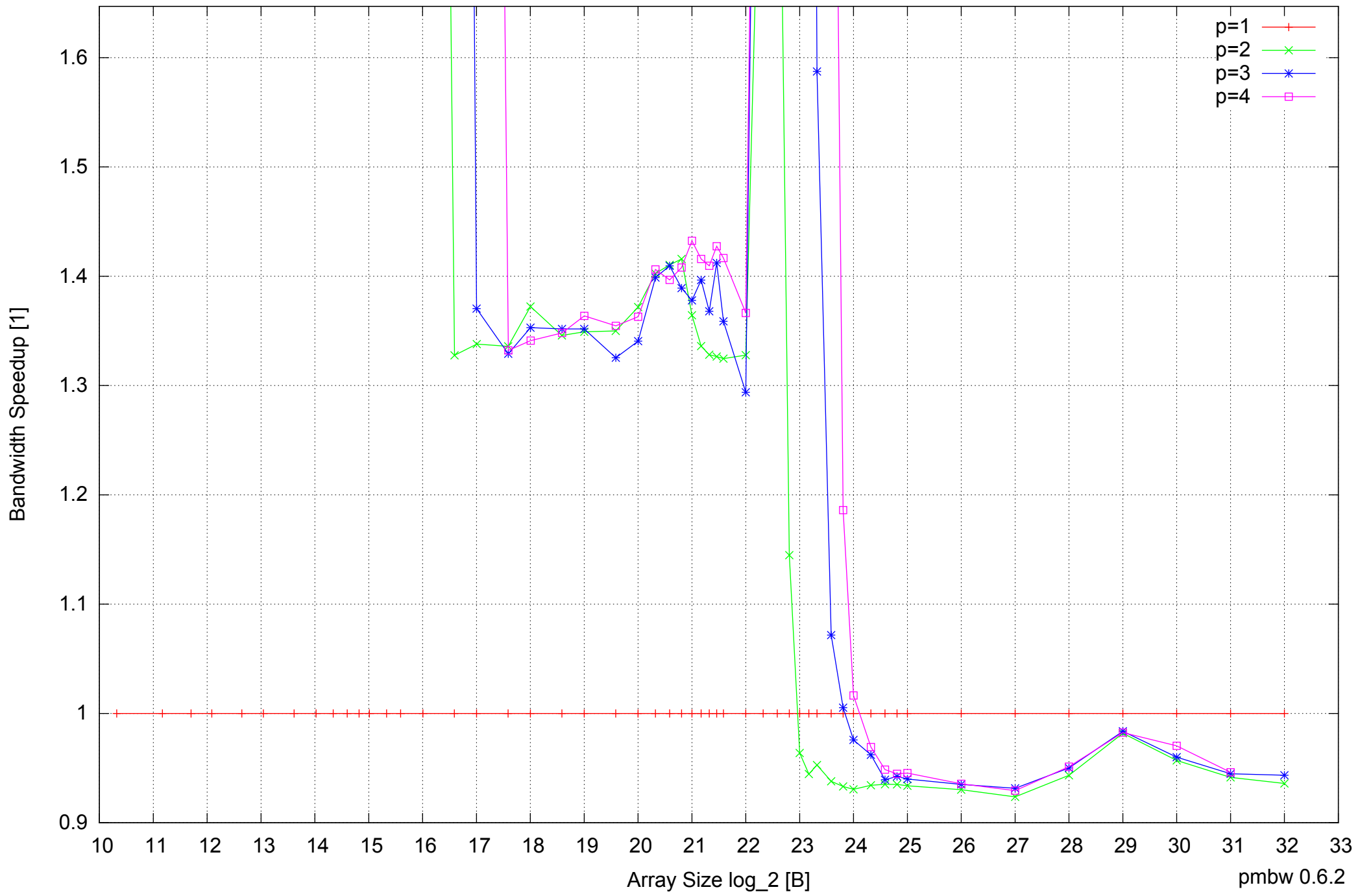
Intel Core 2 Duo E8500 8GB - Speedup of Parallel Memory Bandwidth (enlarged) - ScanWrite128PtrUnrollLoop
