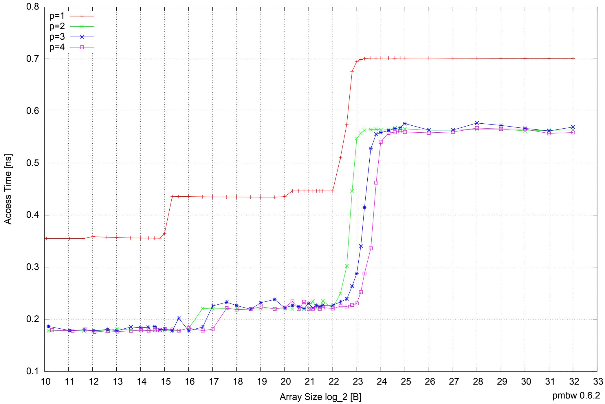
Intel Core 2 Duo E8500 8GB - Parallel Memory Access Time - ScanRead32PtrUnrollLoop
