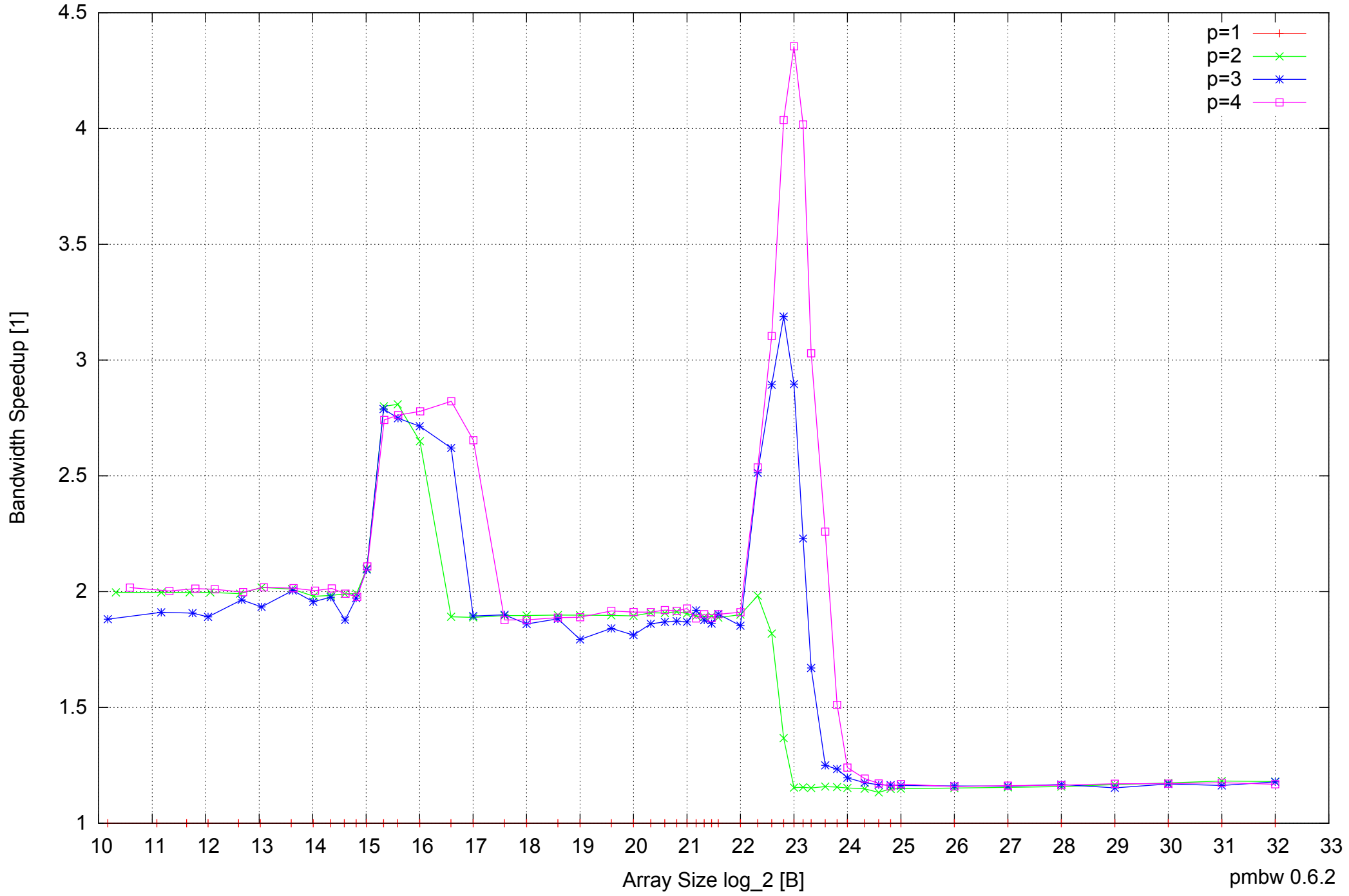
Intel Core 2 Duo E8500 8GB - Speedup of Parallel Memory Bandwidth - ScanRead64IndexUnrollLoop
