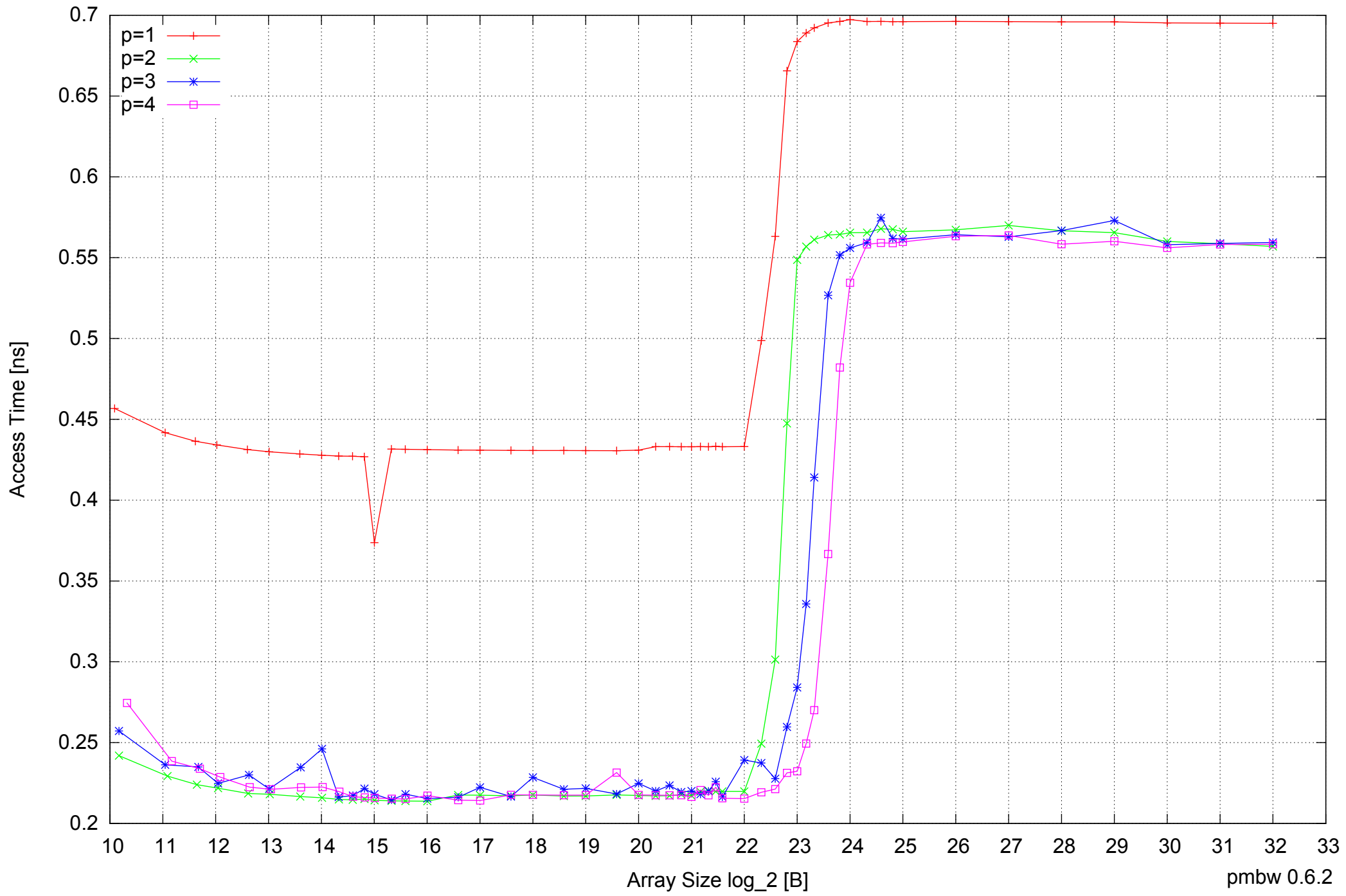
Intel Core 2 Duo E8500 8GB - Parallel Memory Access Time - ScanRead32PtrSimpleLoop
