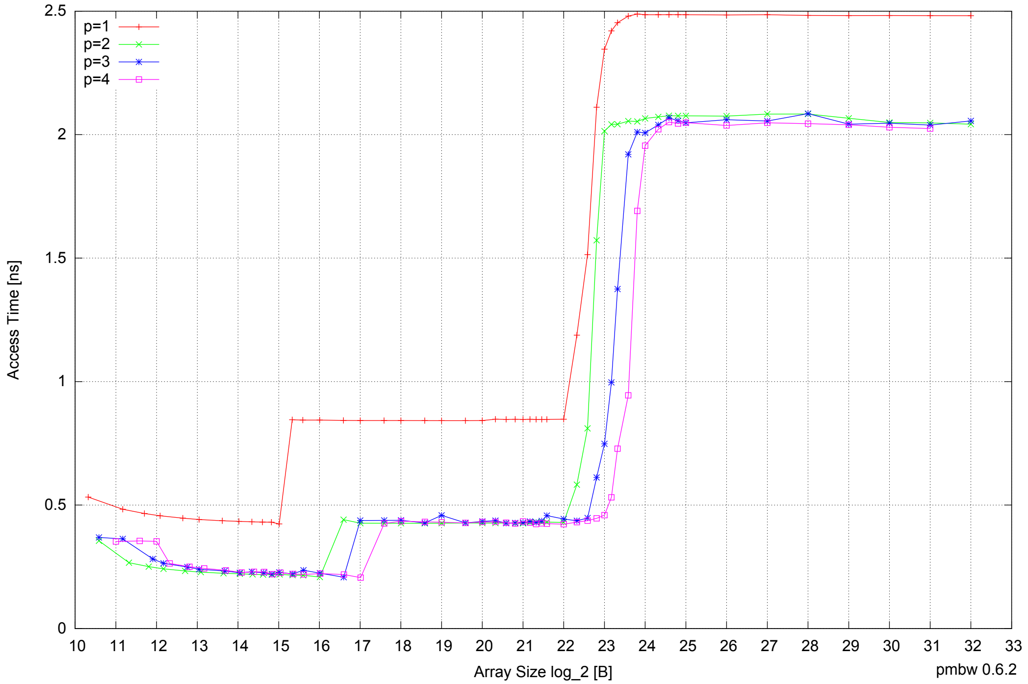
Intel Core 2 Duo E8500 8GB - Parallel Memory Access Time - ScanRead128PtrSimpleLoop
