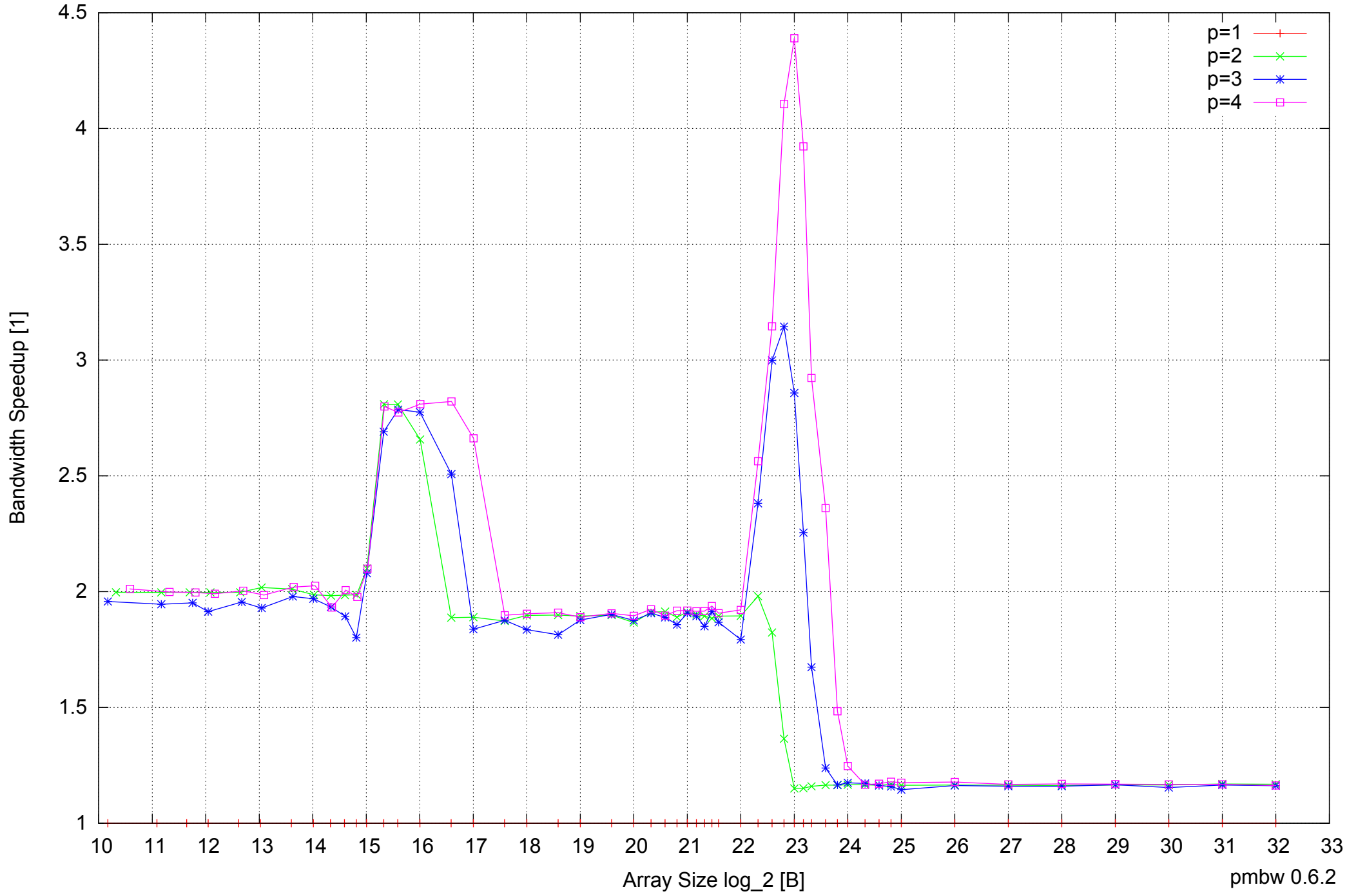
Intel Core 2 Duo E8500 8GB - Speedup of Parallel Memory Bandwidth - ScanRead64PtrUnrollLoop
