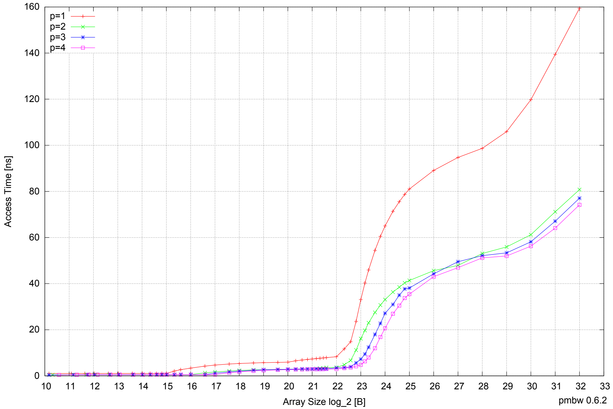
Intel Core 2 Duo E8500 8GB - Parallel Memory Access Time - PermRead64UnrollLoop
