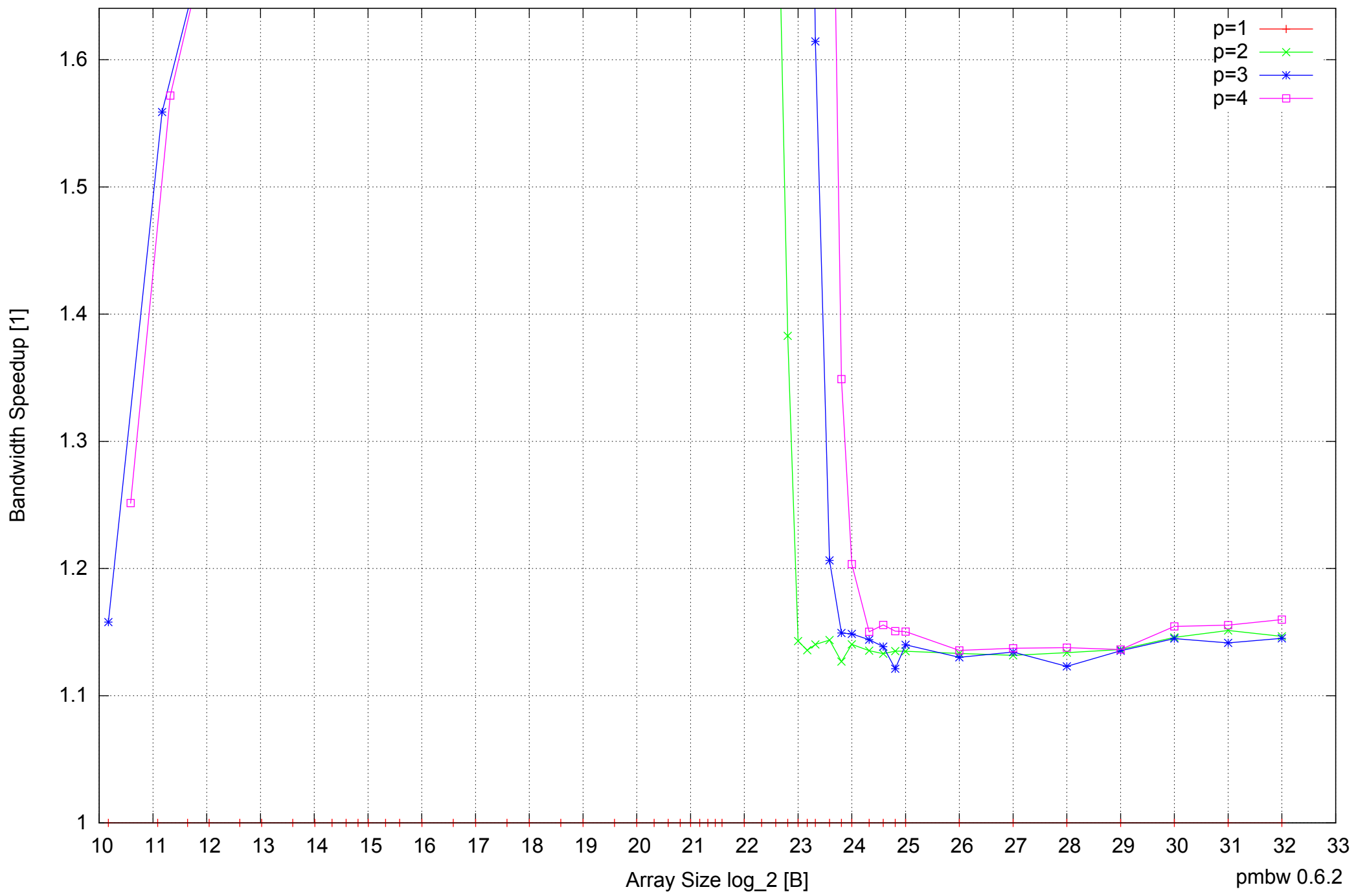
Intel Core 2 Duo E8500 8GB - Speedup of Parallel Memory Bandwidth (enlarged) - ScanRead64IndexSimpleLoop
