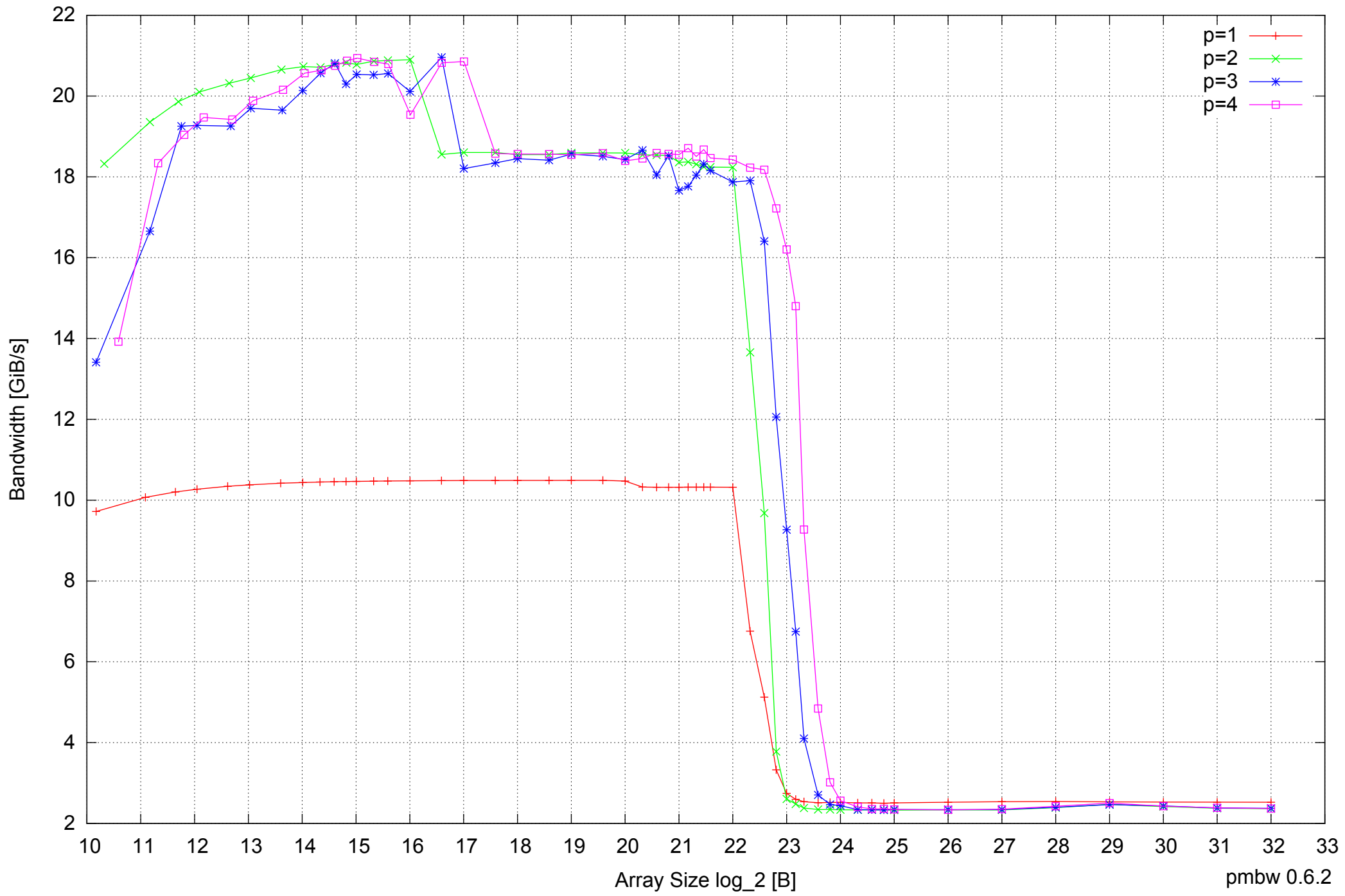
Intel Core 2 Duo E8500 8GB - Parallel Memory Bandwidth - ScanWrite64IndexSimpleLoop
