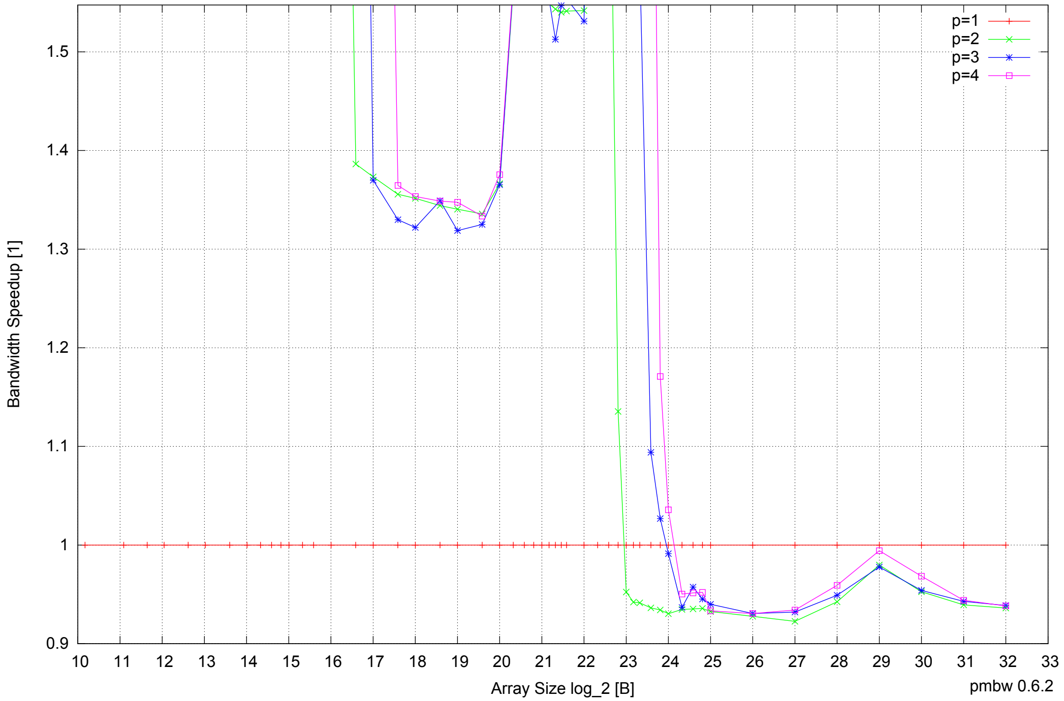
Intel Core 2 Duo E8500 8GB - Speedup of Parallel Memory Bandwidth (enlarged) - ScanWrite64IndexUnrollLoop
