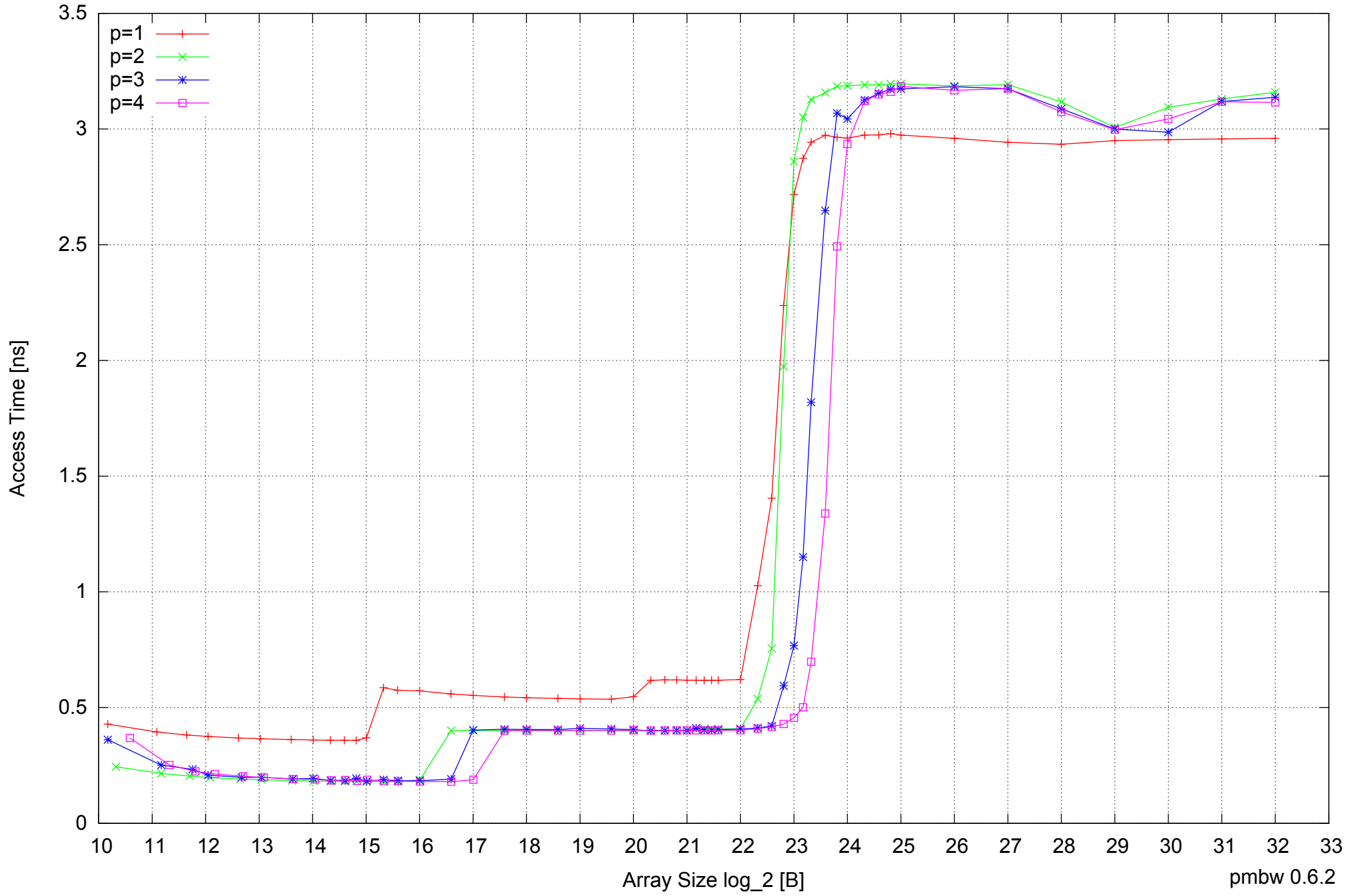
Intel Core 2 Duo E8500 8GB - Parallel Memory Access Time - ScanWrite64PtrSimpleLoop
