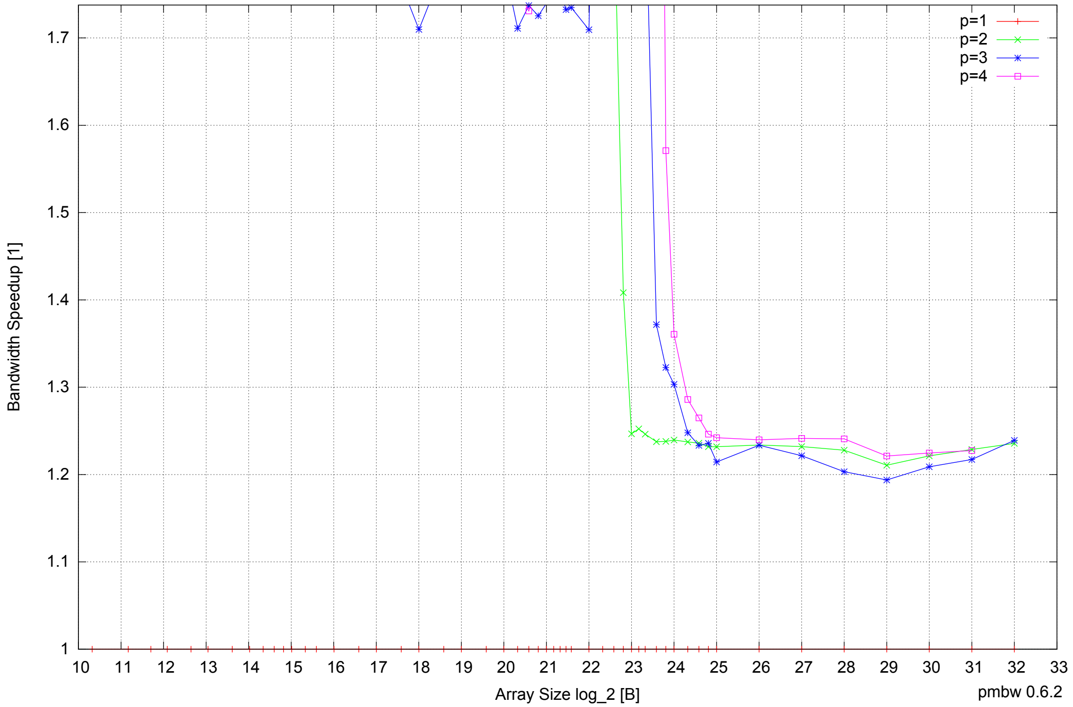
Intel Core 2 Duo E8500 8GB - Speedup of Parallel Memory Bandwidth (enlarged) - ScanRead128PtrUnrollLoop
