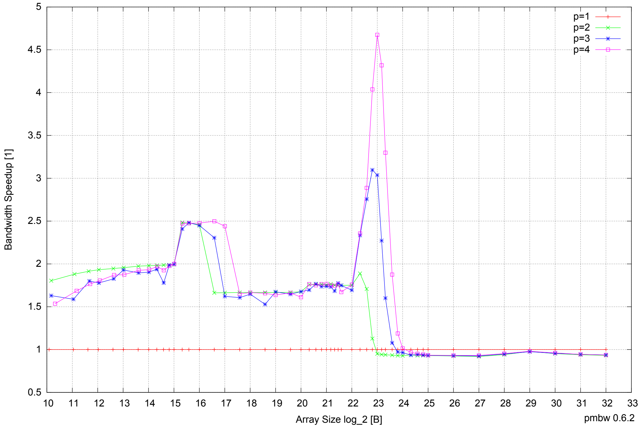
Intel Core 2 Duo E8500 8GB - Speedup of Parallel Memory Bandwidth - ScanWrite32PtrSimpleLoop
