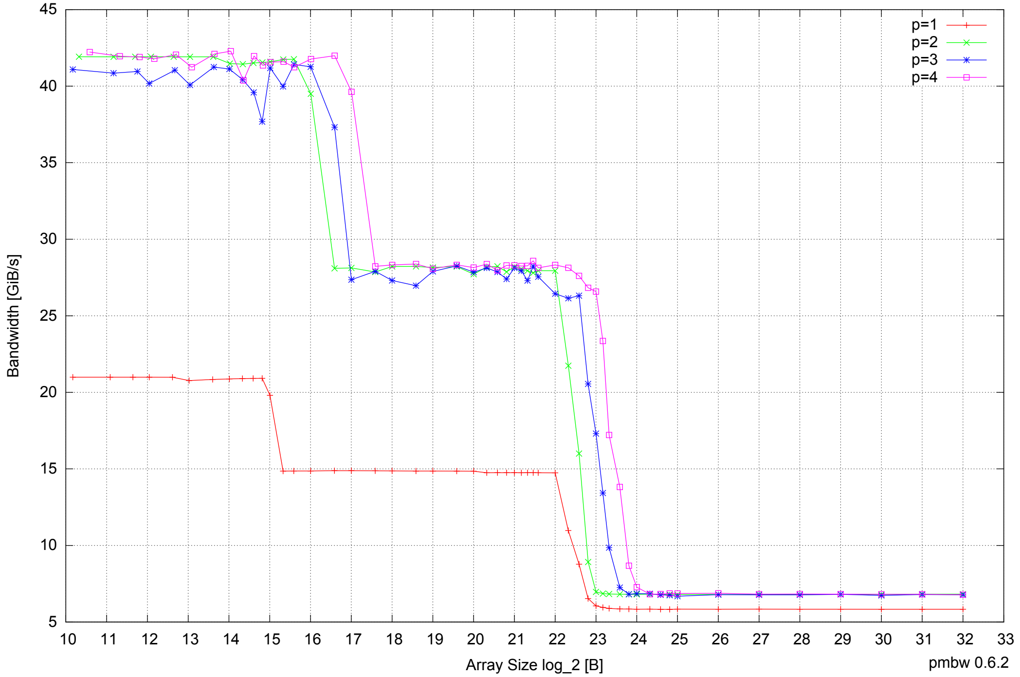
Intel Core 2 Duo E8500 8GB - Parallel Memory Bandwidth - ScanRead64PtrUnrollLoop
