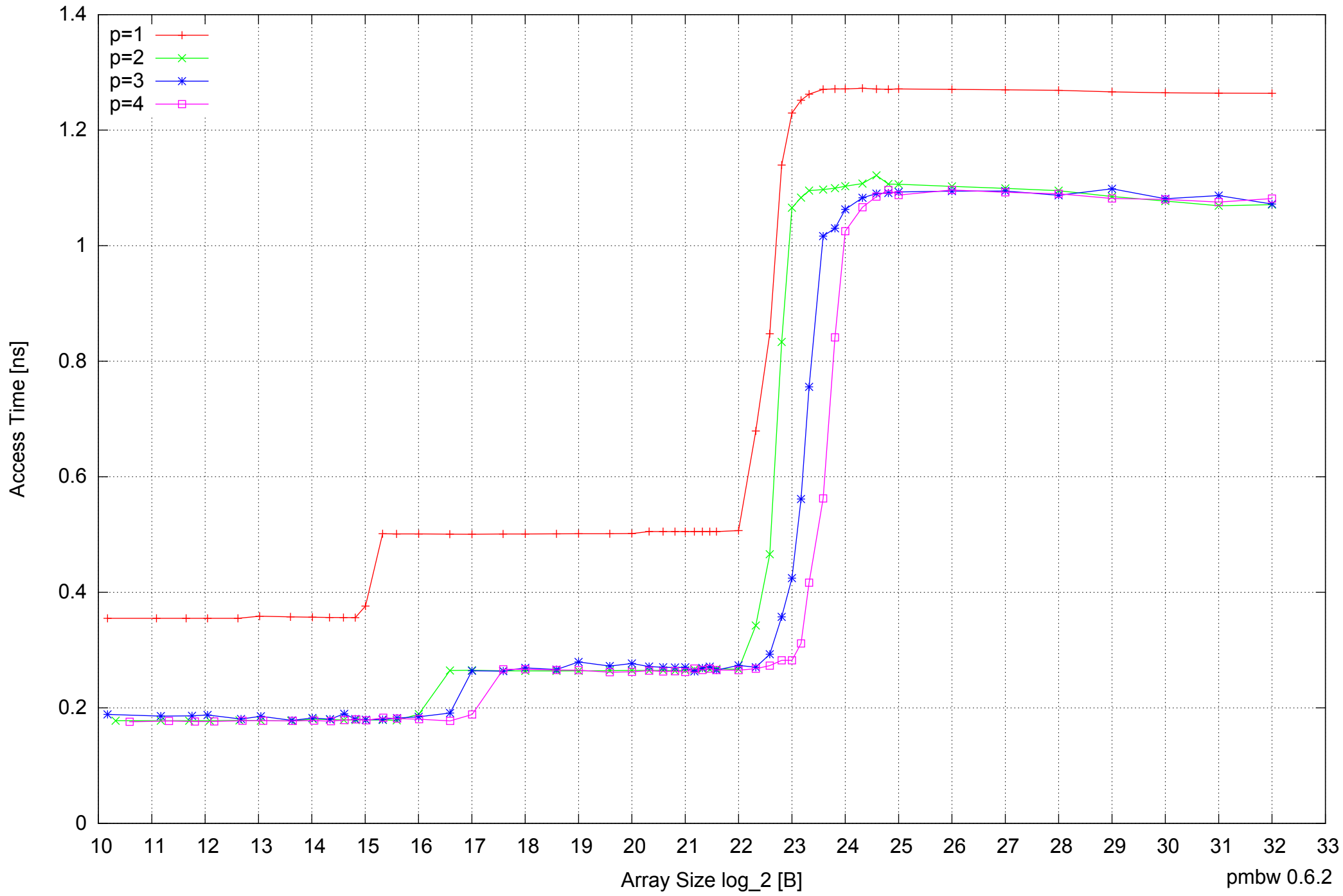
Intel Core 2 Duo E8500 8GB - Parallel Memory Access Time - ScanRead64IndexUnrollLoop
