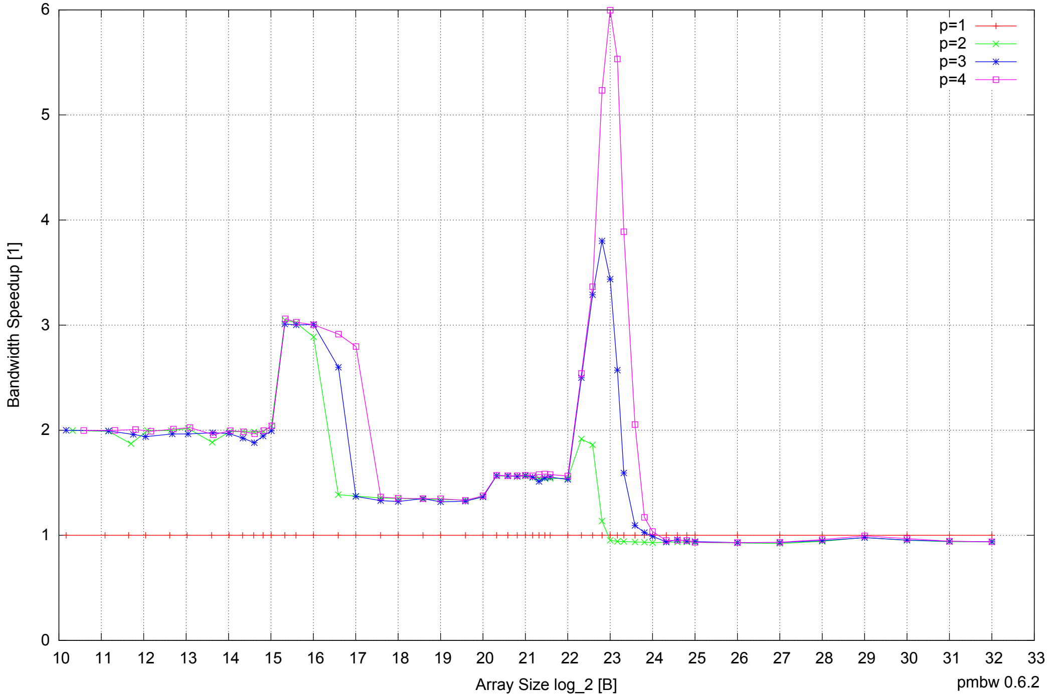
Intel Core 2 Duo E8500 8GB - Speedup of Parallel Memory Bandwidth - ScanWrite64IndexUnrollLoop
