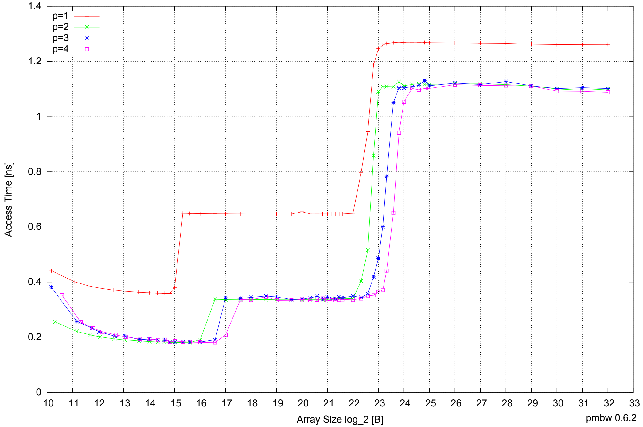
Intel Core 2 Duo E8500 8GB - Parallel Memory Access Time - ScanRead64IndexSimpleLoop
