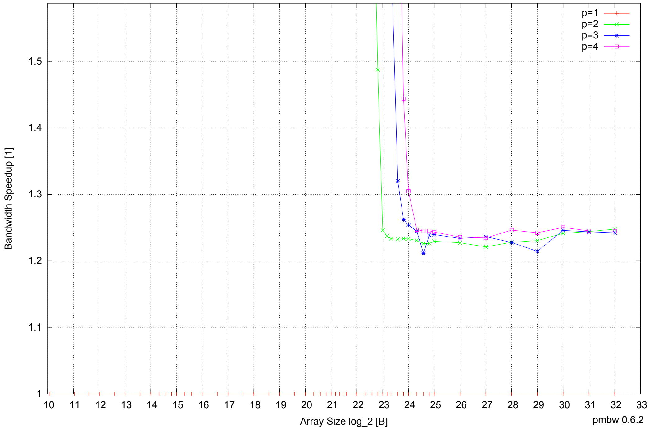
Intel Core 2 Duo E8500 8GB - Speedup of Parallel Memory Bandwidth (enlarged) - ScanRead32PtrSimpleLoop
