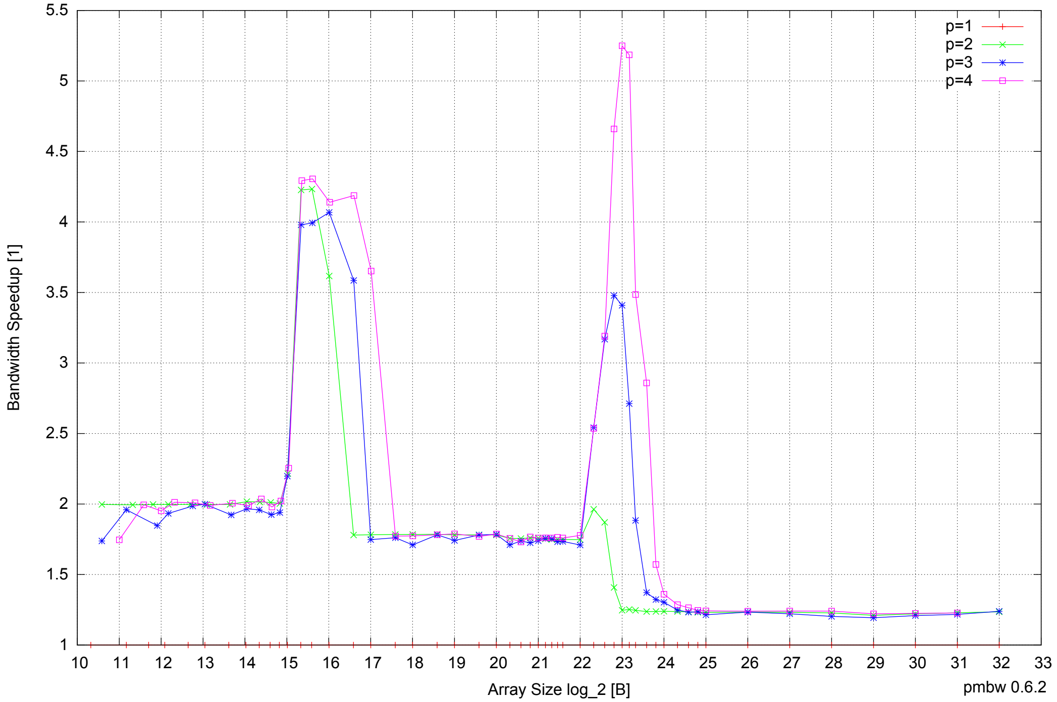
Intel Core 2 Duo E8500 8GB - Speedup of Parallel Memory Bandwidth - ScanRead128PtrUnrollLoop
