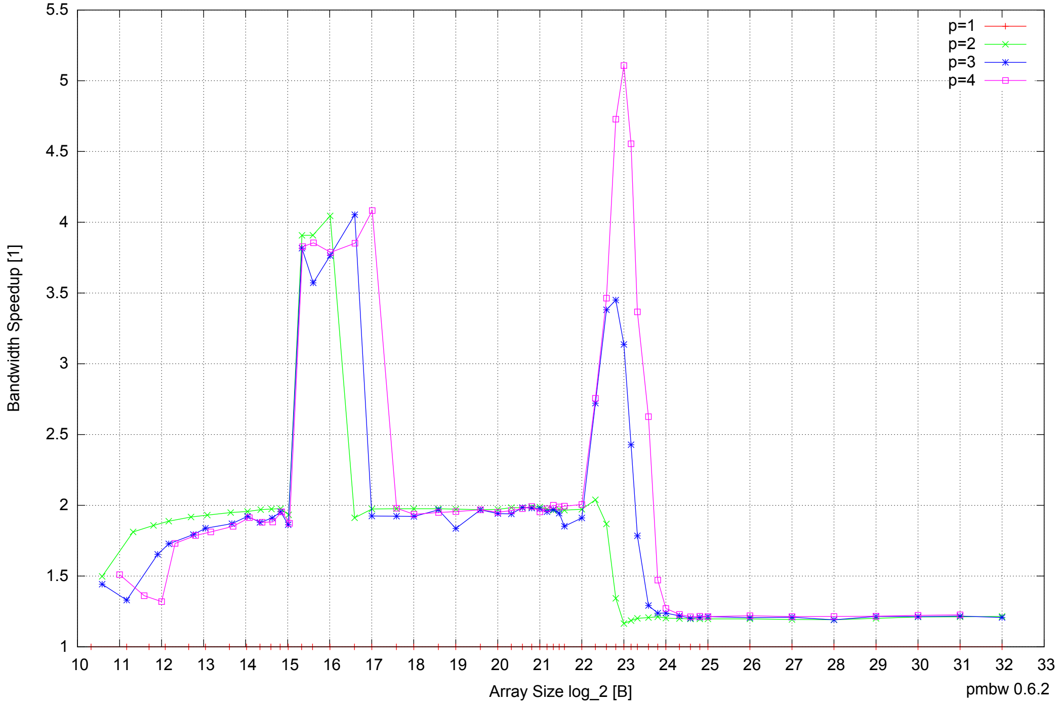
Intel Core 2 Duo E8500 8GB - Speedup of Parallel Memory Bandwidth - ScanRead128PtrSimpleLoop
