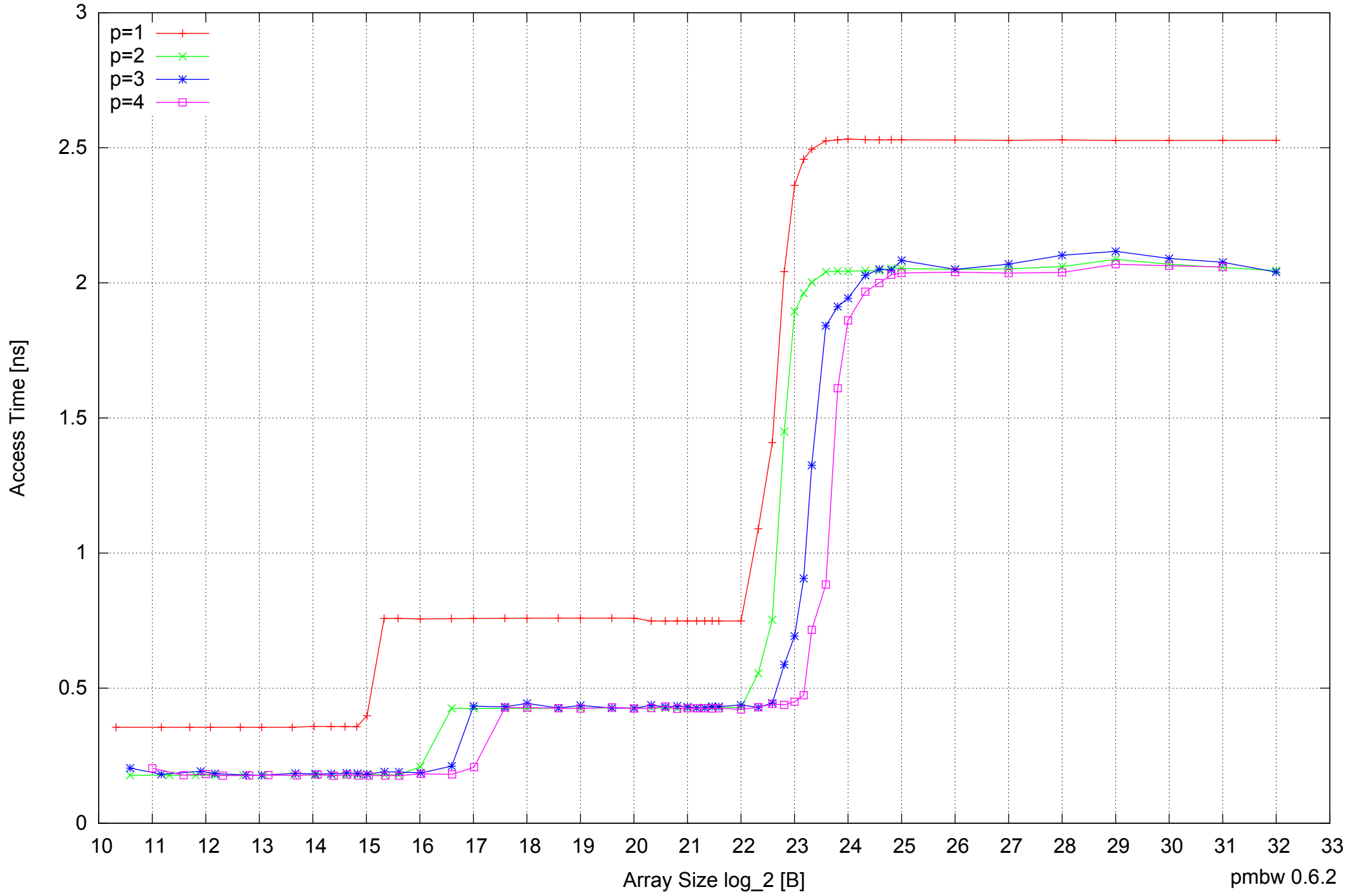
Intel Core 2 Duo E8500 8GB - Parallel Memory Access Time - ScanRead128PtrUnrollLoop
