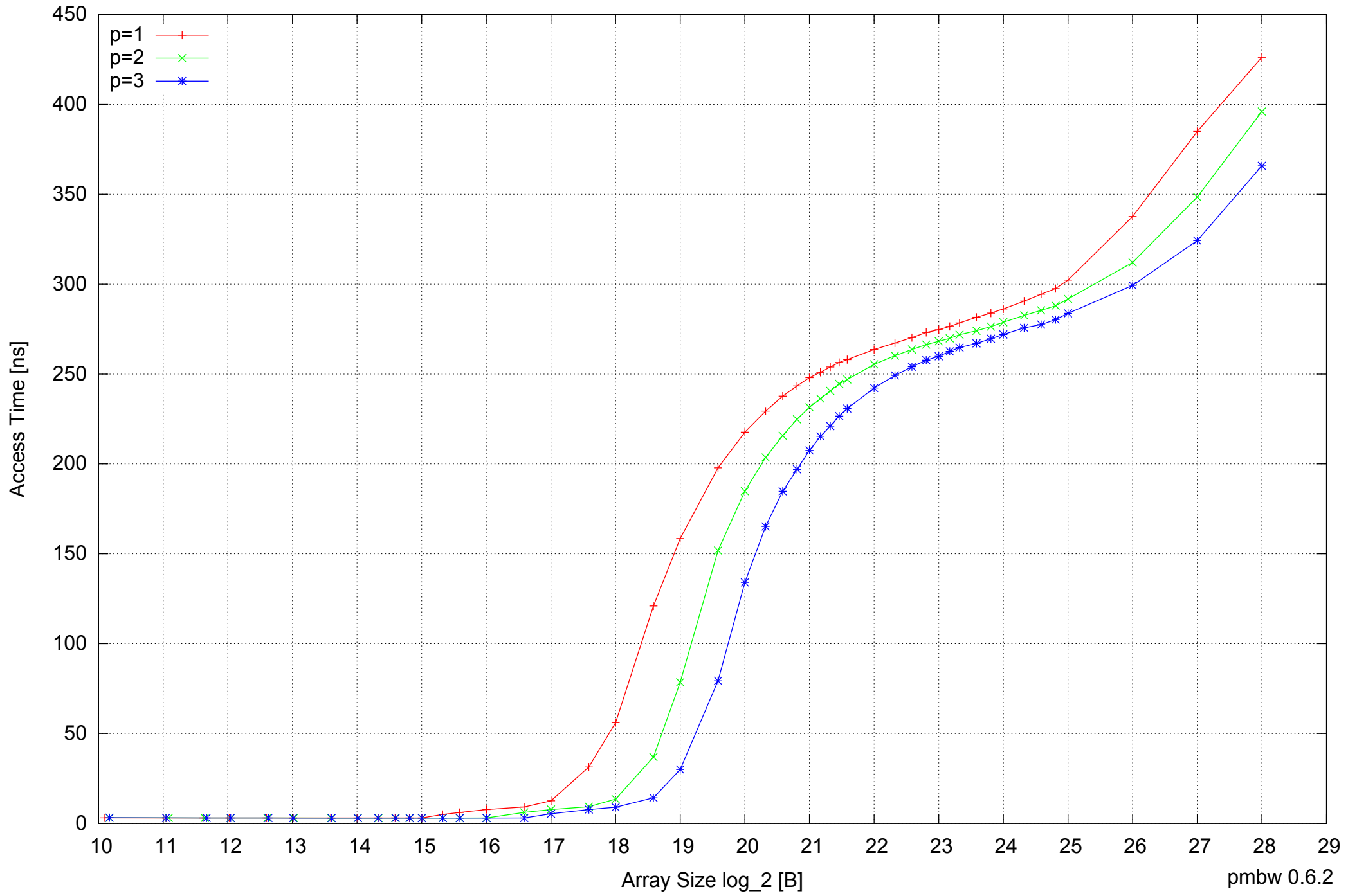
BeagleBone Black: AM335x 1GHz ARM Cortex-A8 512MB - Parallel Memory Access Time - PermRead32SimpleLoop
