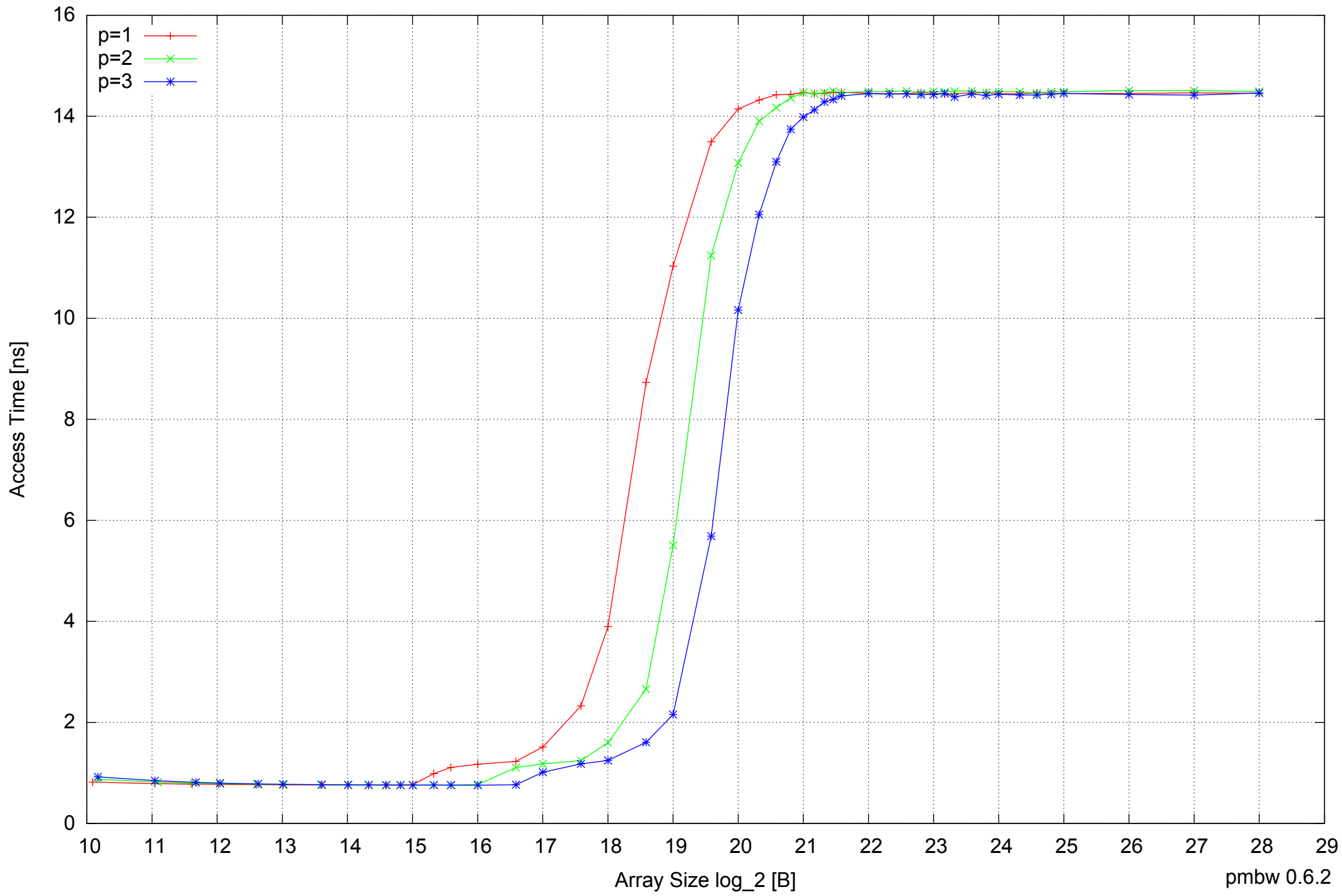
BeagleBone Black: AM335x 1GHz ARM Cortex-A8 512MB - Parallel Memory Access Time - ScanRead32PtrMultiLoop
