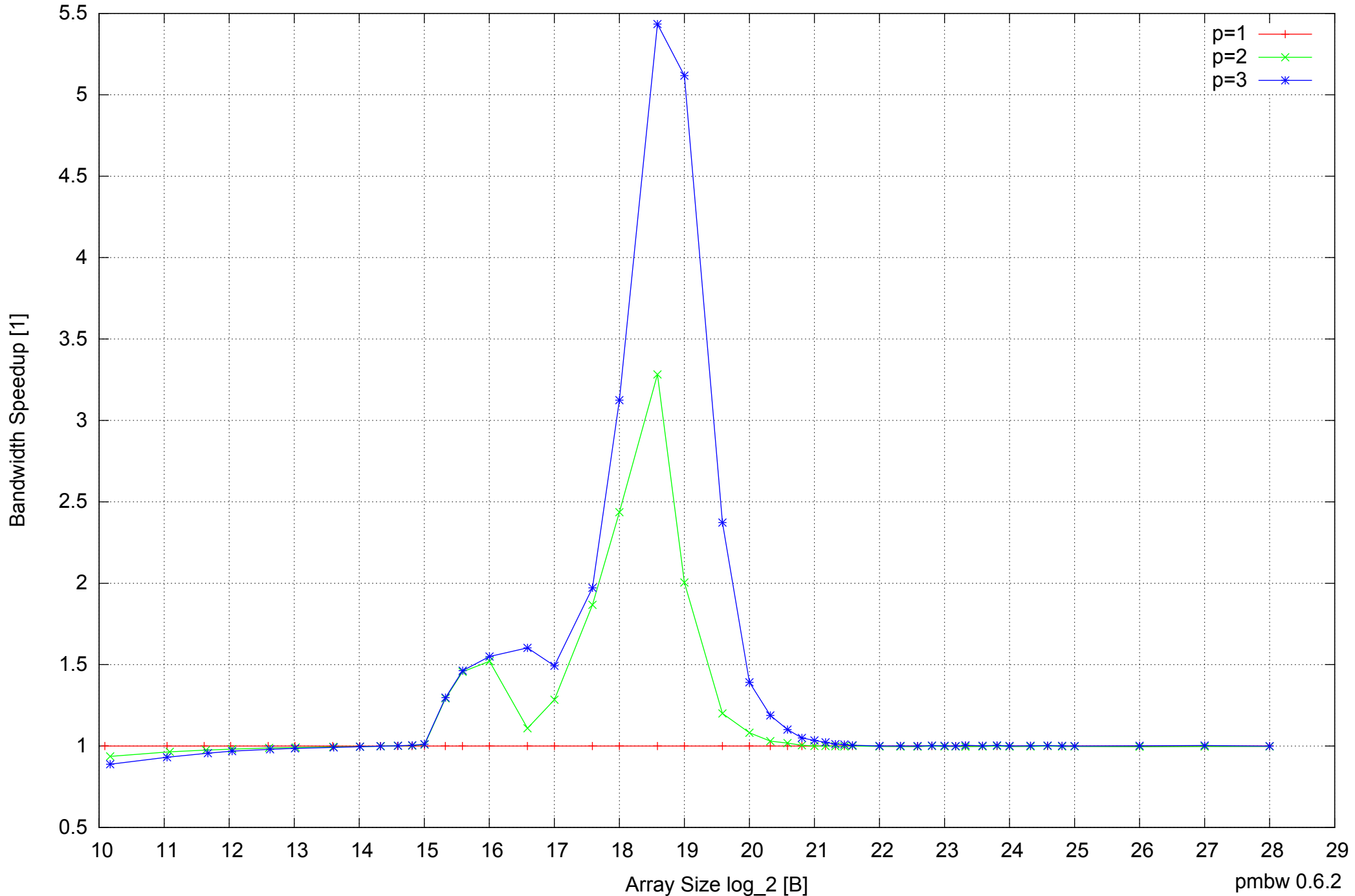
BeagleBone Black: AM335x 1GHz ARM Cortex-A8 512MB - Speedup of Parallel Memory Bandwidth - ScanRead32PtrMultiLoop
