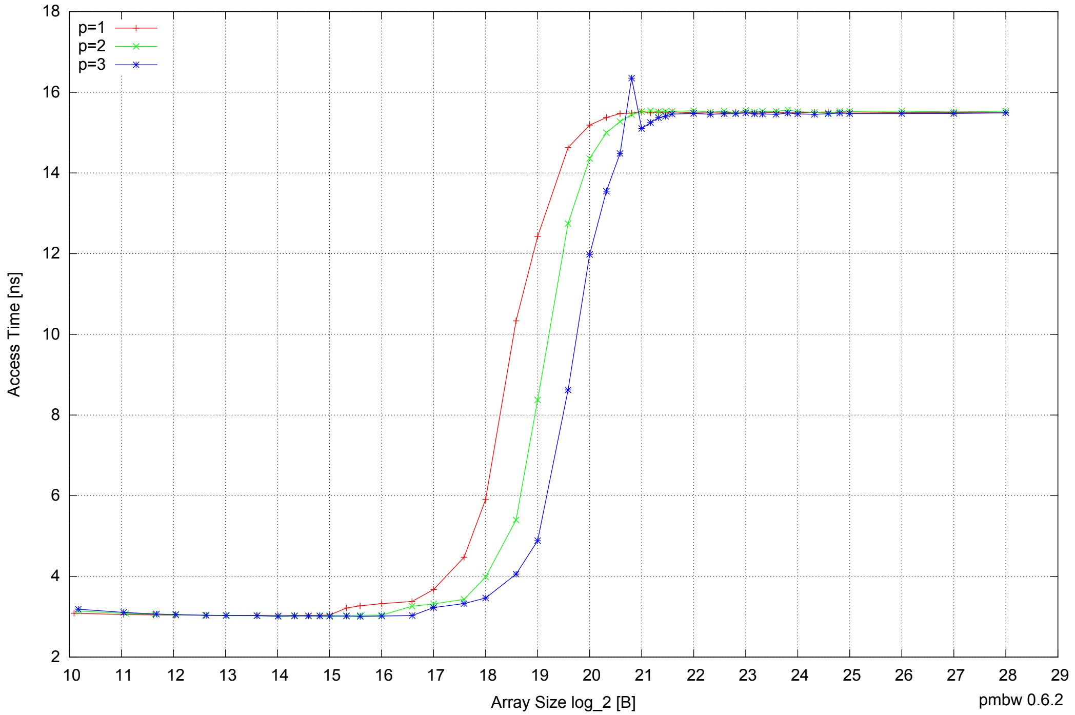
BeagleBone Black: AM335x 1GHz ARM Cortex-A8 512MB - Parallel Memory Access Time - ScanRead32PtrSimpleLoop
