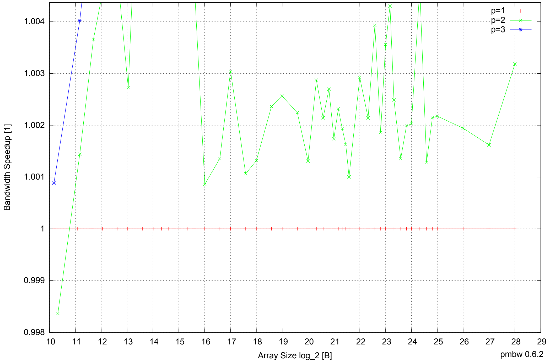
BeagleBone Black: AM335x 1GHz ARM Cortex-A8 512MB - Speedup of Parallel Memory Bandwidth (enlarged) - ScanWrite64PtrSimpleLoop
