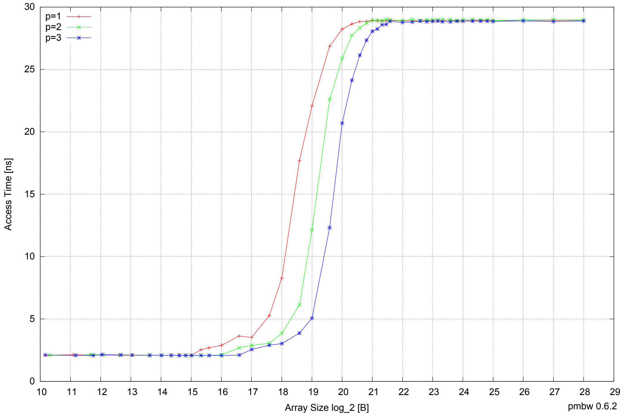
BeagleBone Black: AM335x 1GHz ARM Cortex-A8 512MB - Parallel Memory Access Time - ScanRead64PtrUnrollLoop
