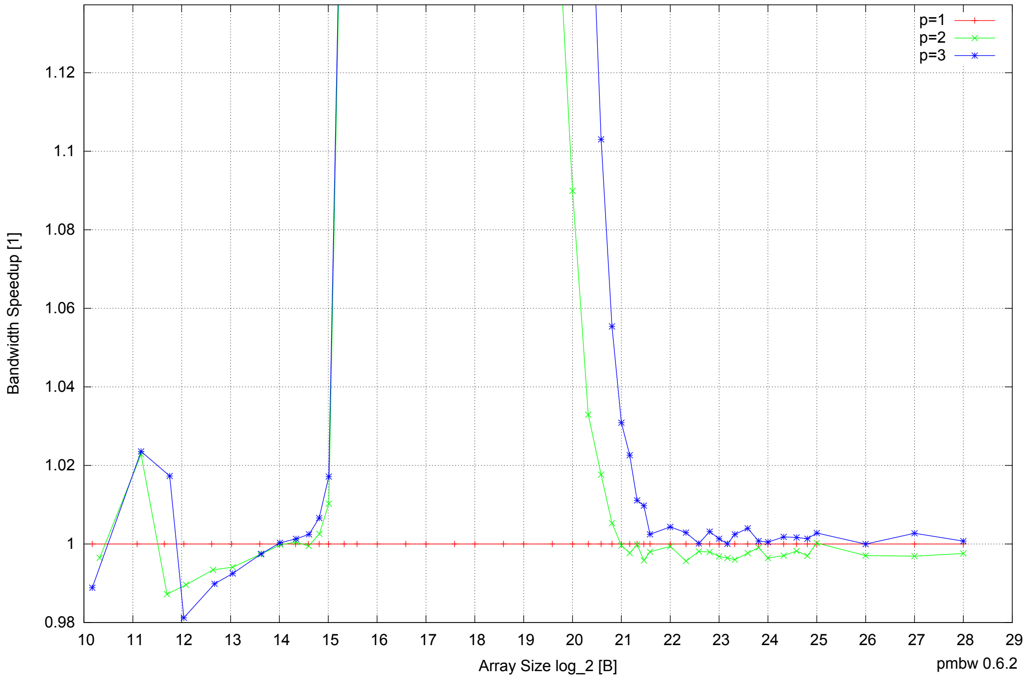
BeagleBone Black: AM335x 1GHz ARM Cortex-A8 512MB - Speedup of Parallel Memory Bandwidth (enlarged) - ScanRead64PtrUnrollLoop
