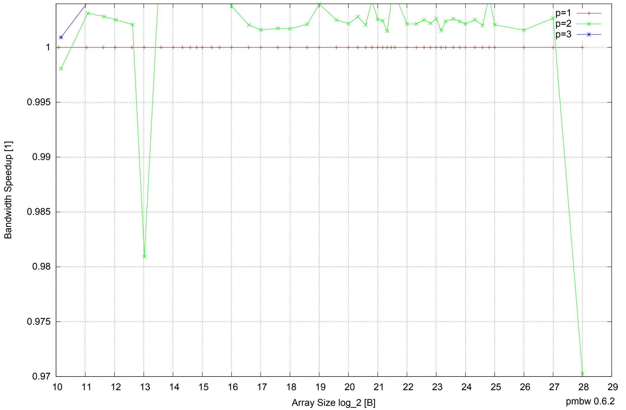
BeagleBone Black: AM335x 1GHz ARM Cortex-A8 512MB - Speedup of Parallel Memory Bandwidth (enlarged) - ScanWrite32PtrMultiLoop
