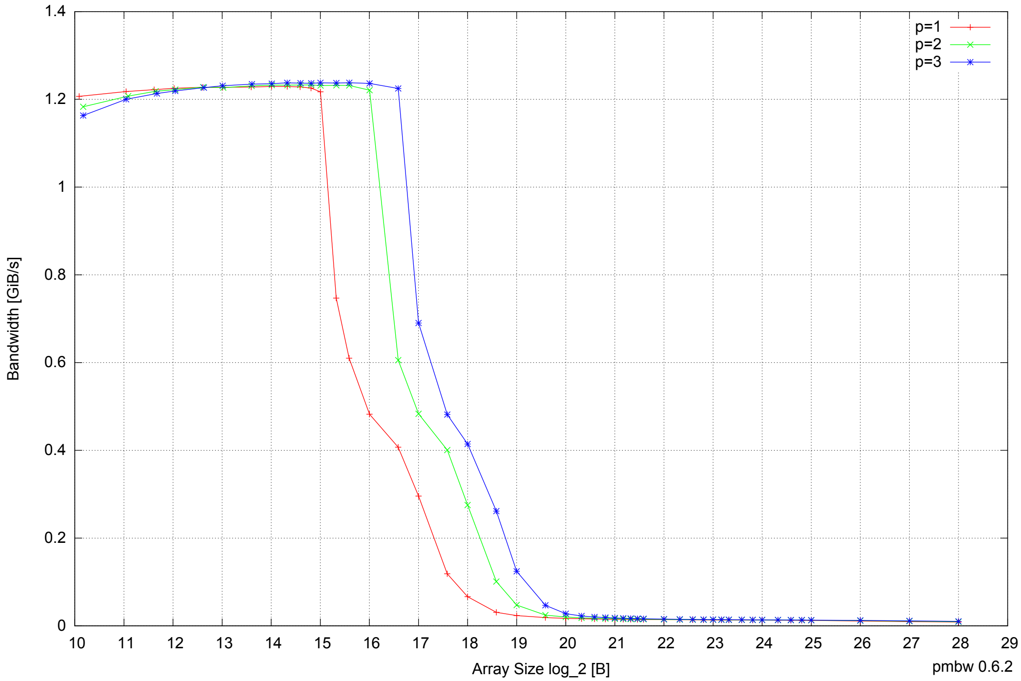
BeagleBone Black: AM335x 1GHz ARM Cortex-A8 512MB - Parallel Memory Bandwidth - PermRead32SimpleLoop
