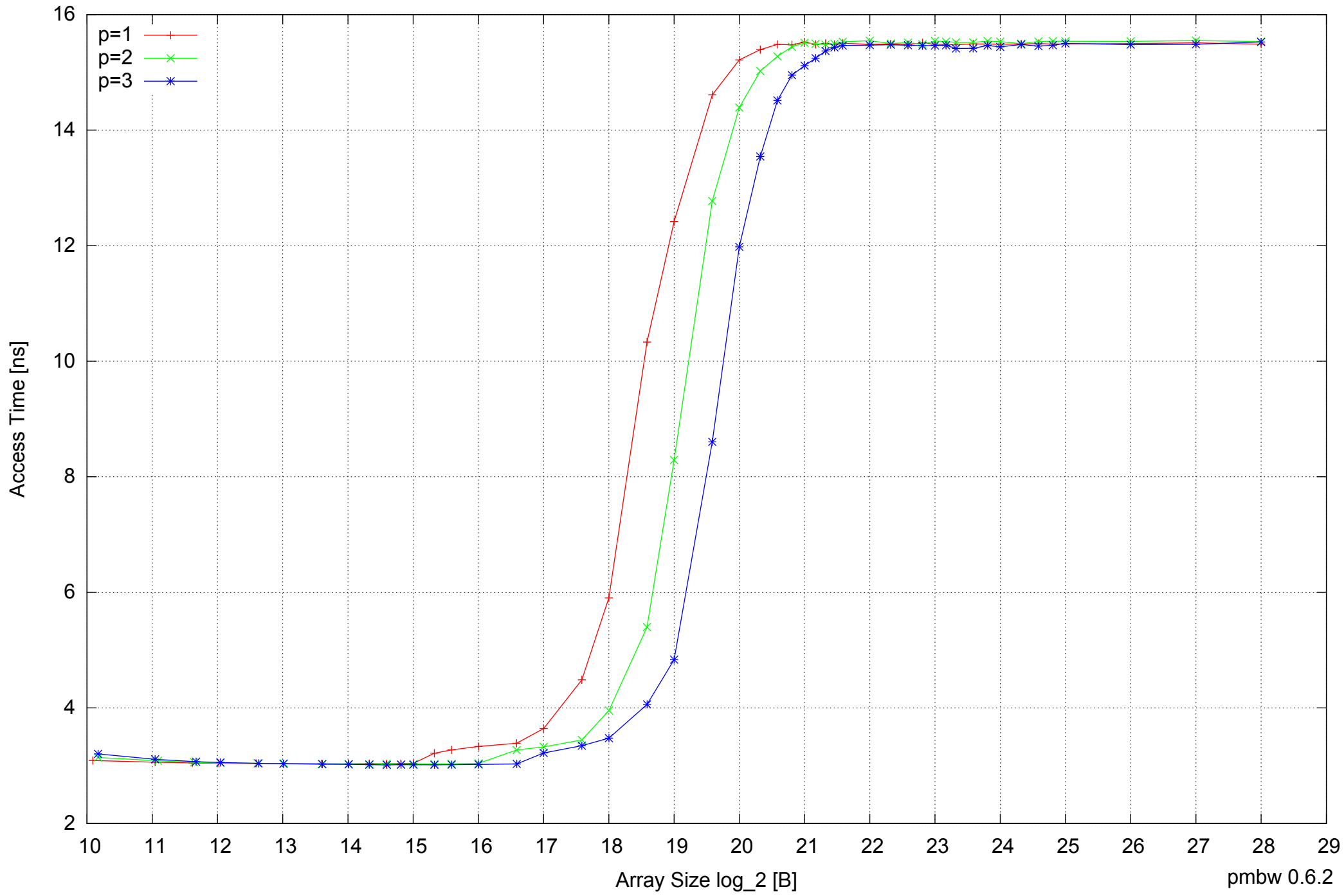
BeagleBone Black: AM335x 1GHz ARM Cortex-A8 512MB - Parallel Memory Access Time - ScanRead32IndexSimpleLoop
