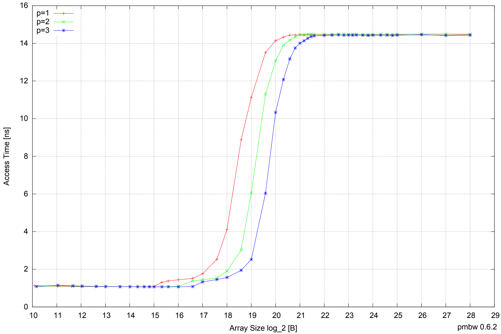
BeagleBone Black: AM335x 1GHz ARM Cortex-A8 512MB - Parallel Memory Access Time - ScanRead32PtrUnrollLoop
