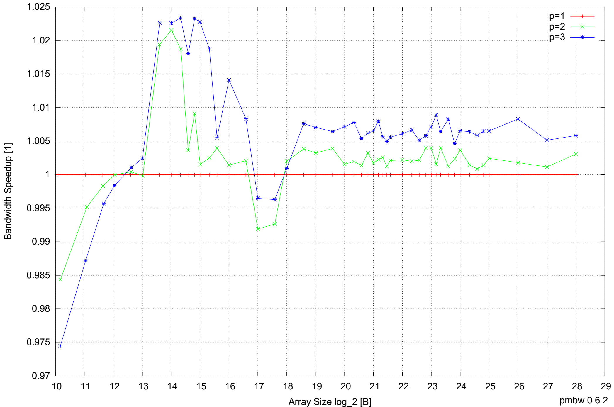
BeagleBone Black: AM335x 1GHz ARM Cortex-A8 512MB - Speedup of Parallel Memory Bandwidth - ScanWrite32PtrSimpleLoop
