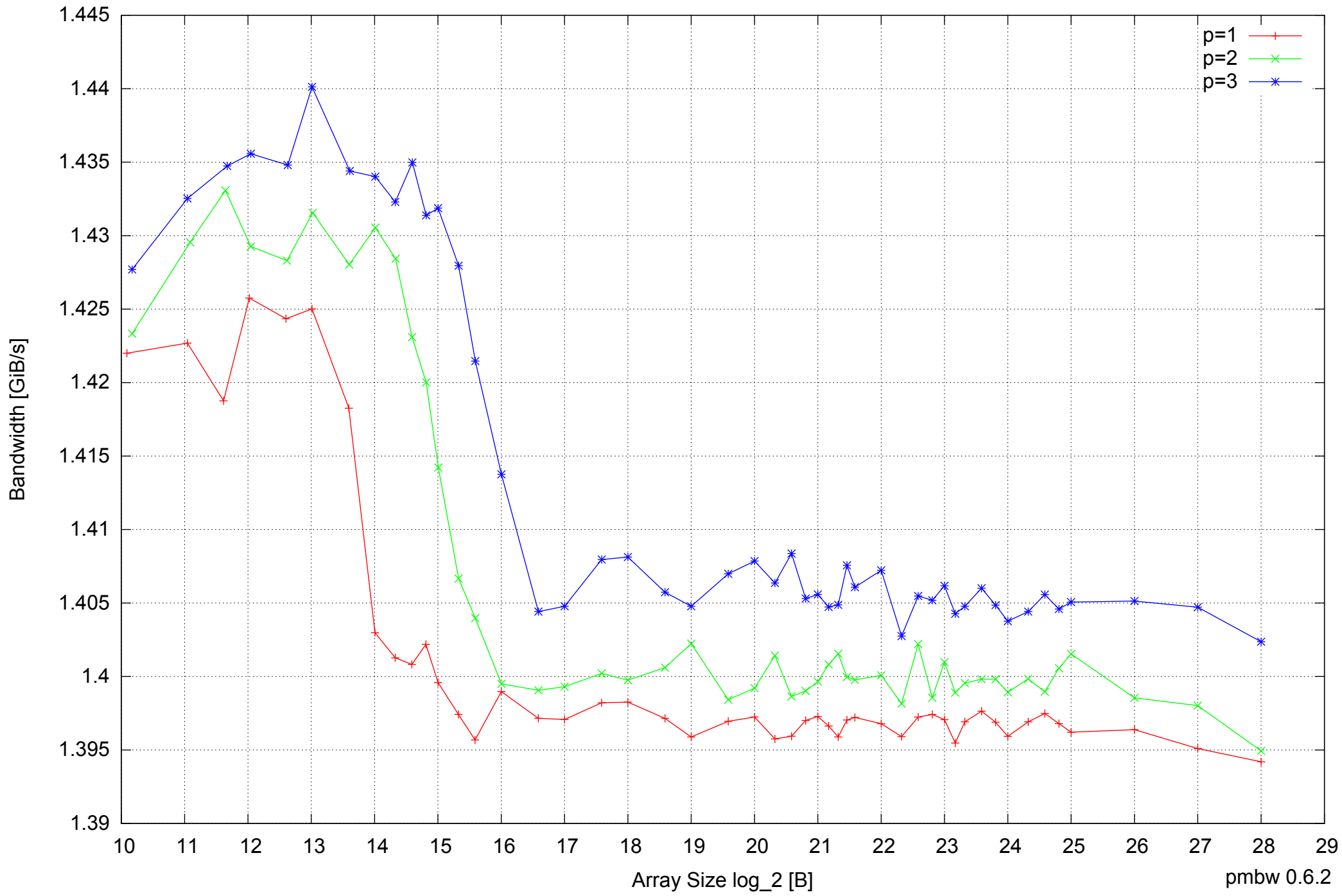
BeagleBone Black: AM335x 1GHz ARM Cortex-A8 512MB - Parallel Memory Bandwidth - ScanWrite32PtrUnrollLoop
