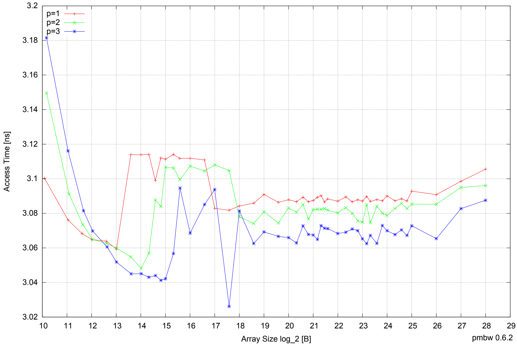
BeagleBone Black: AM335x 1GHz ARM Cortex-A8 512MB - Parallel Memory Access Time - ScanWrite32PtrSimpleLoop
