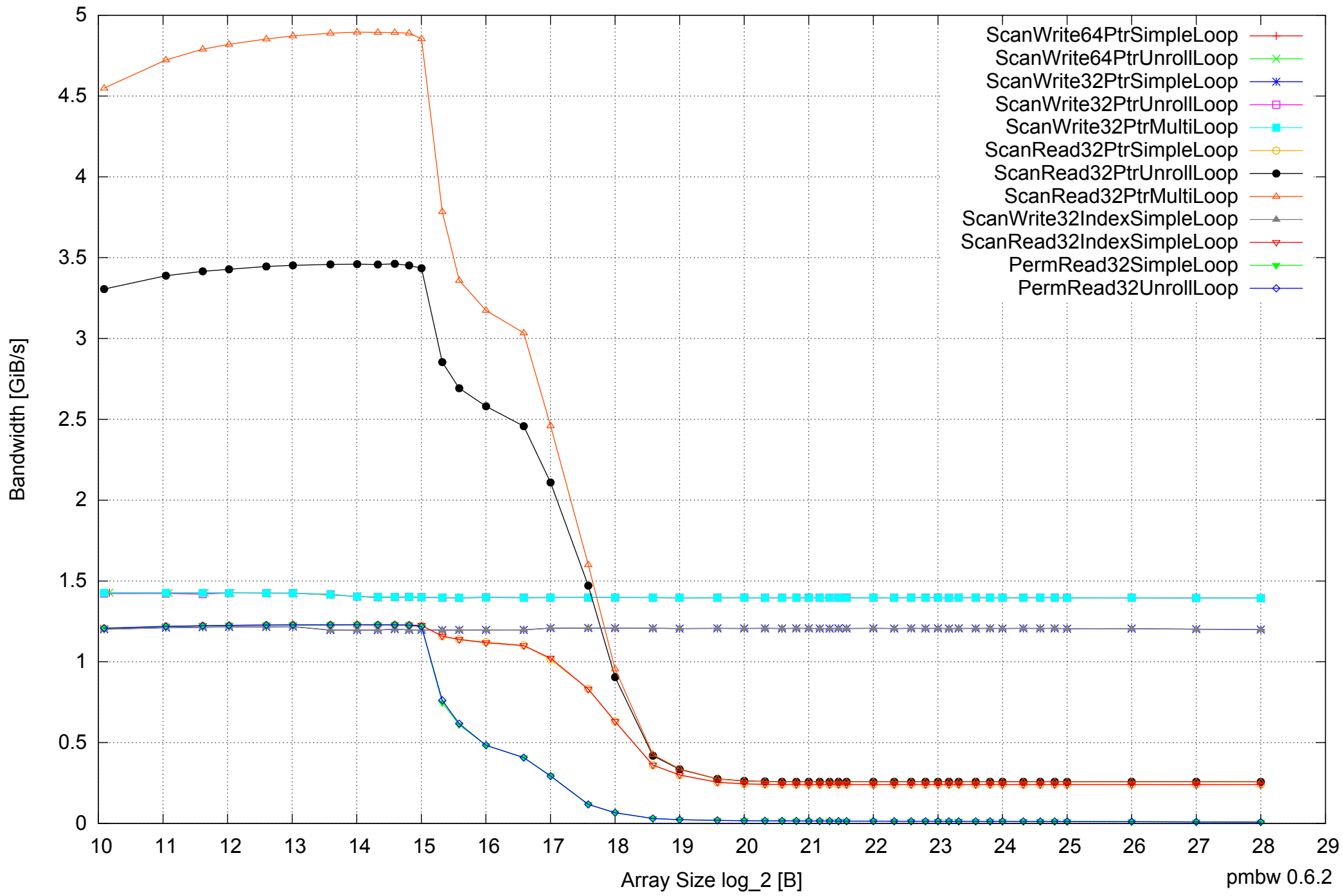
BeagleBone Black: AM335x 1GHz ARM Cortex-A8 512MB - One Thread Memory Bandwidth (only 64-bit Reads)
