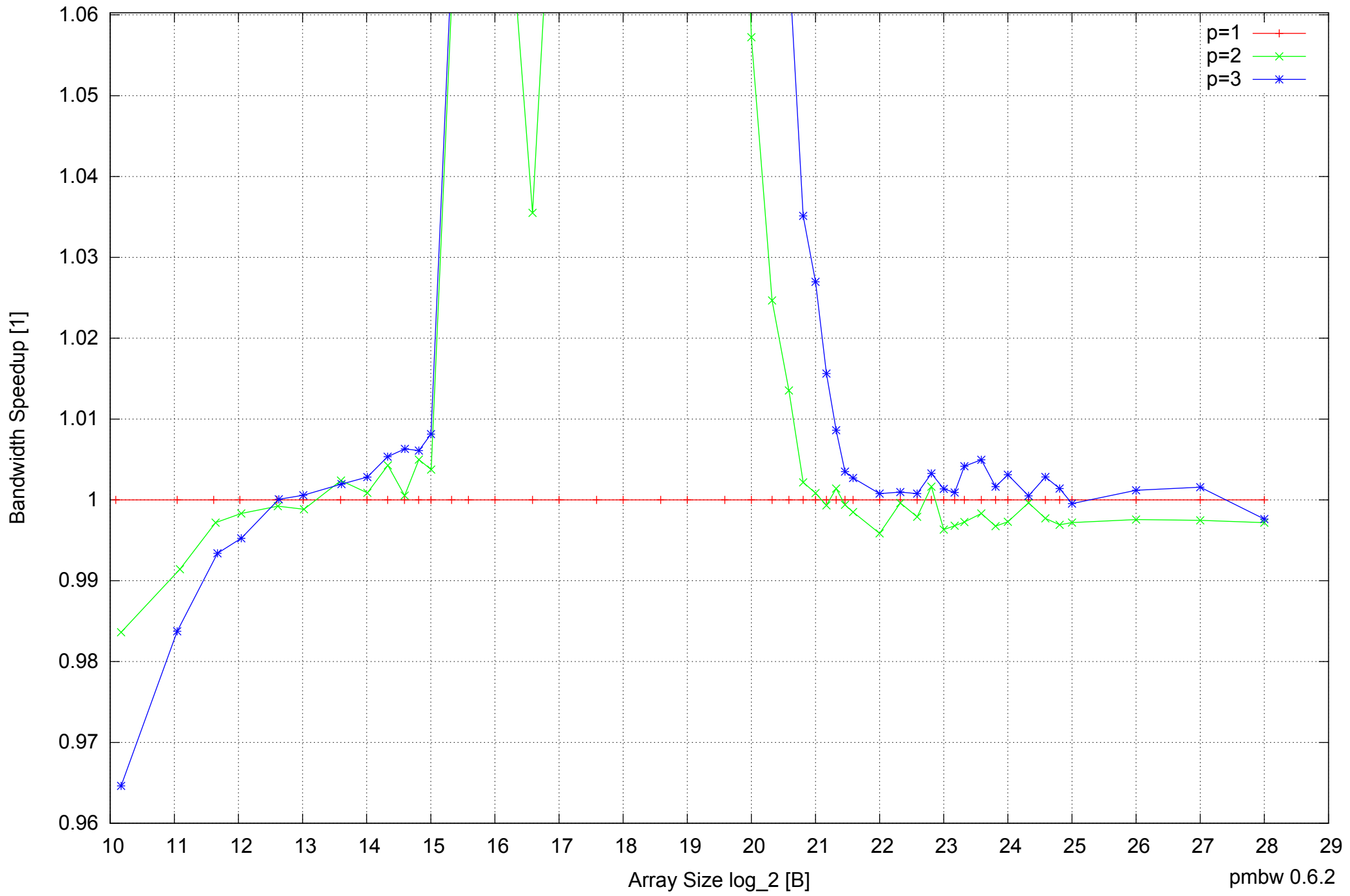
BeagleBone Black: AM335x 1GHz ARM Cortex-A8 512MB - Speedup of Parallel Memory Bandwidth (enlarged) - ScanRead32IndexSimpleLo
