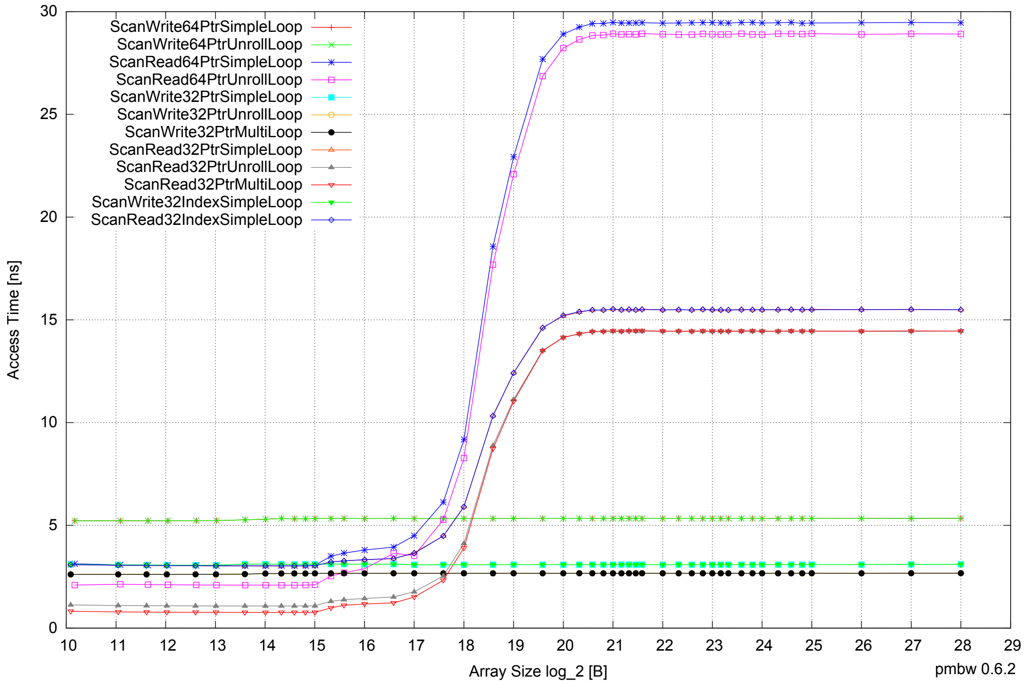
BeagleBone Black: AM335x 1GHz ARM Cortex-A8 512MB - One Thread Memory Latency (excluding Permutation)
