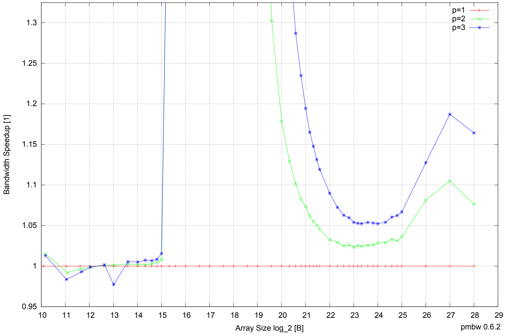
BeagleBone Black: AM335x 1GHz ARM Cortex-A8 512MB - Speedup of Parallel Memory Bandwidth (enlarged) - PermRead32UnrollLoop
