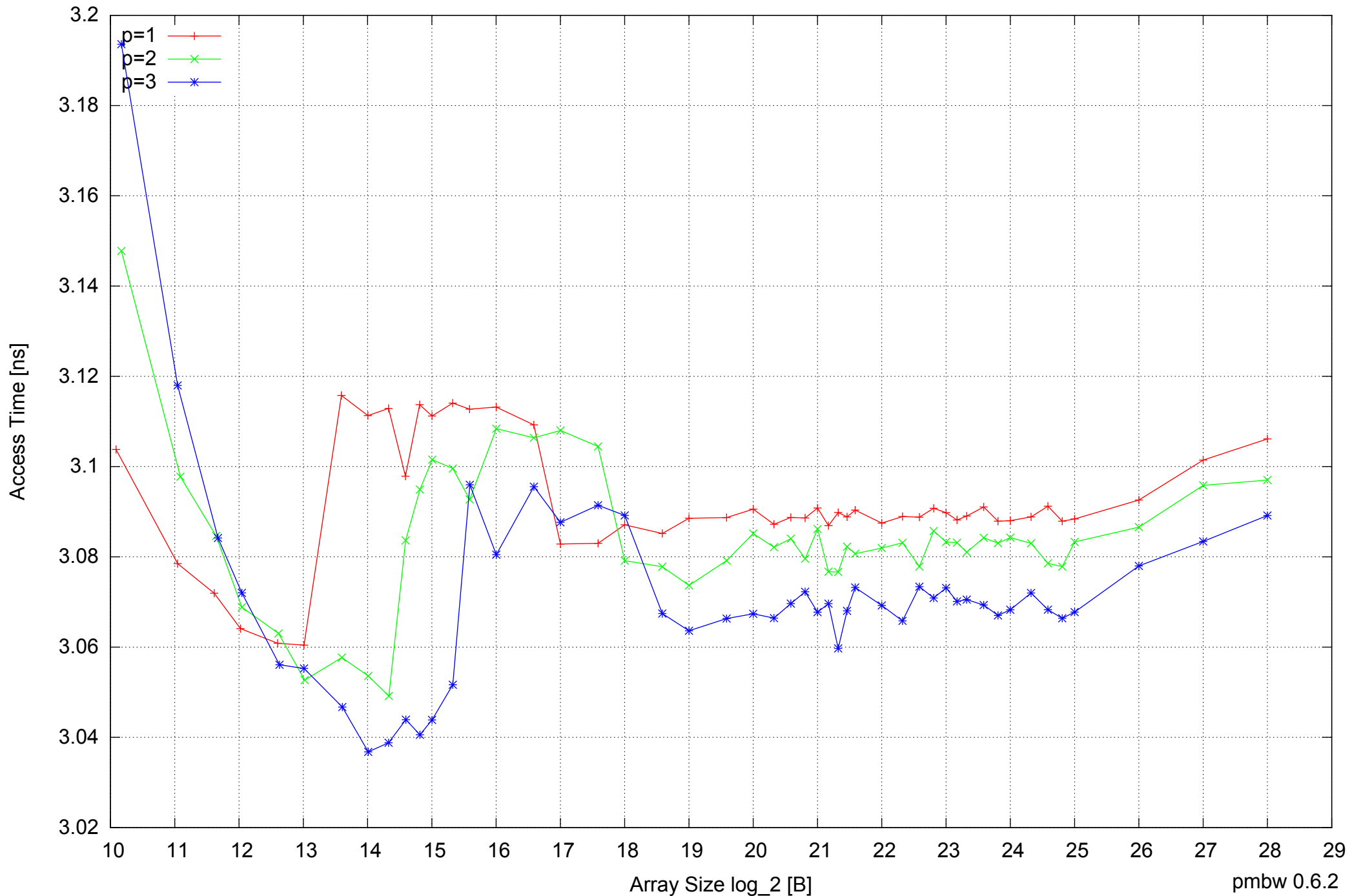
BeagleBone Black: AM335x 1GHz ARM Cortex-A8 512MB - Parallel Memory Access Time - ScanWrite32IndexSimpleLoop
