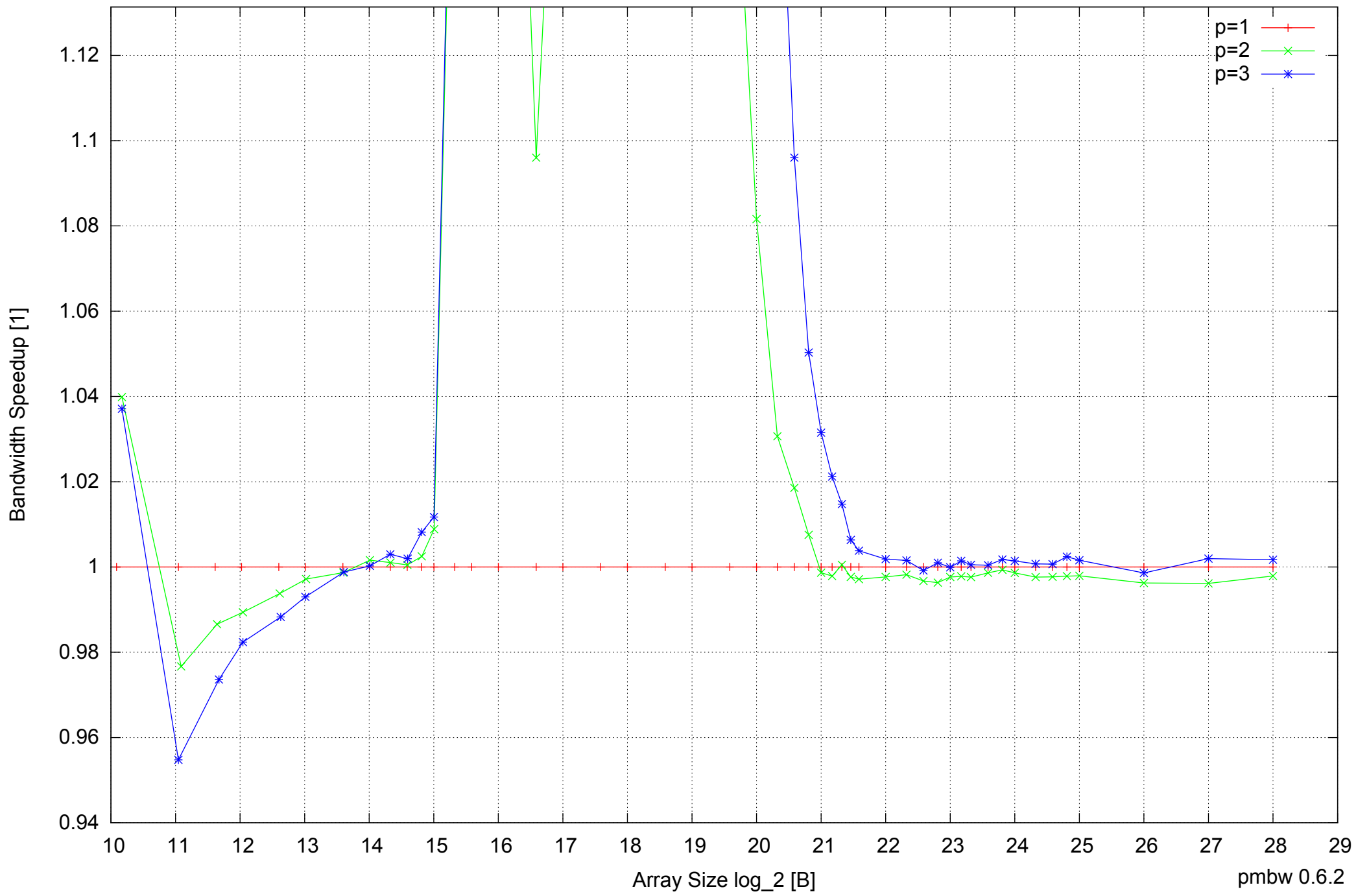
BeagleBone Black: AM335x 1GHz ARM Cortex-A8 512MB - Speedup of Parallel Memory Bandwidth (enlarged) - ScanRead32PtrUnrollLoop
