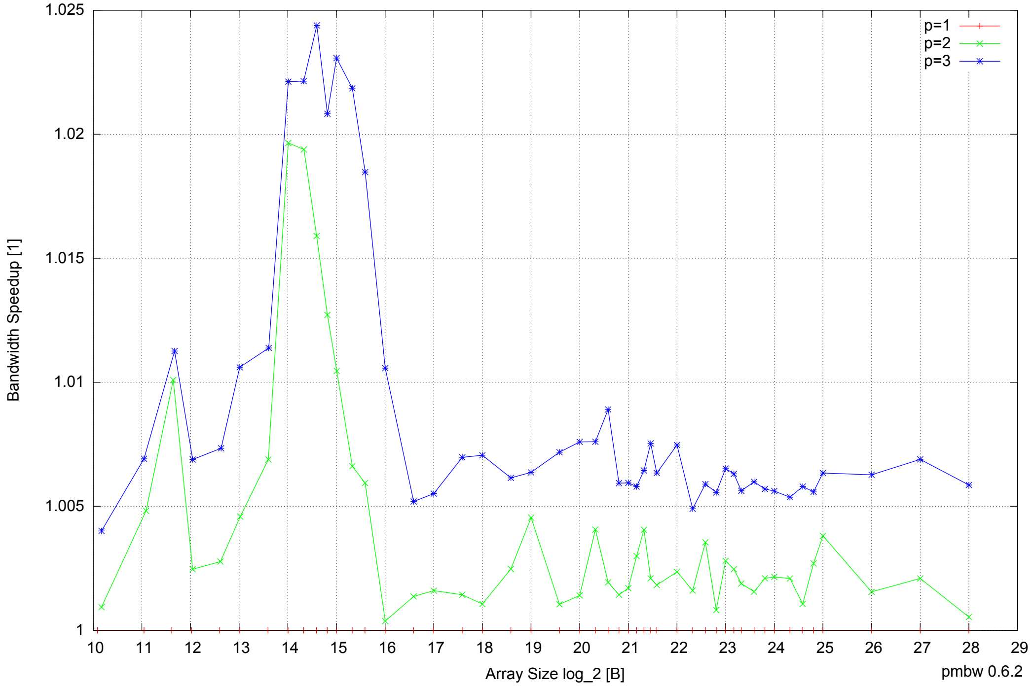
BeagleBone Black: AM335x 1GHz ARM Cortex-A8 512MB - Speedup of Parallel Memory Bandwidth - ScanWrite32PtrUnrollLoop
