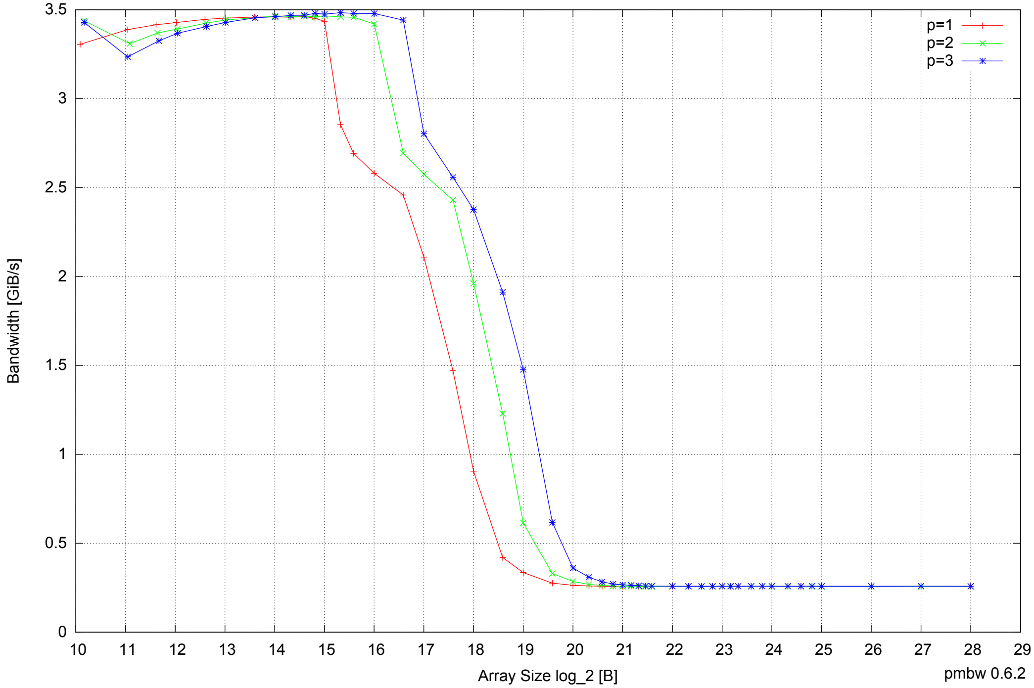
BeagleBone Black: AM335x 1GHz ARM Cortex-A8 512MB - Parallel Memory Bandwidth - ScanRead32PtrUnrollLoop
