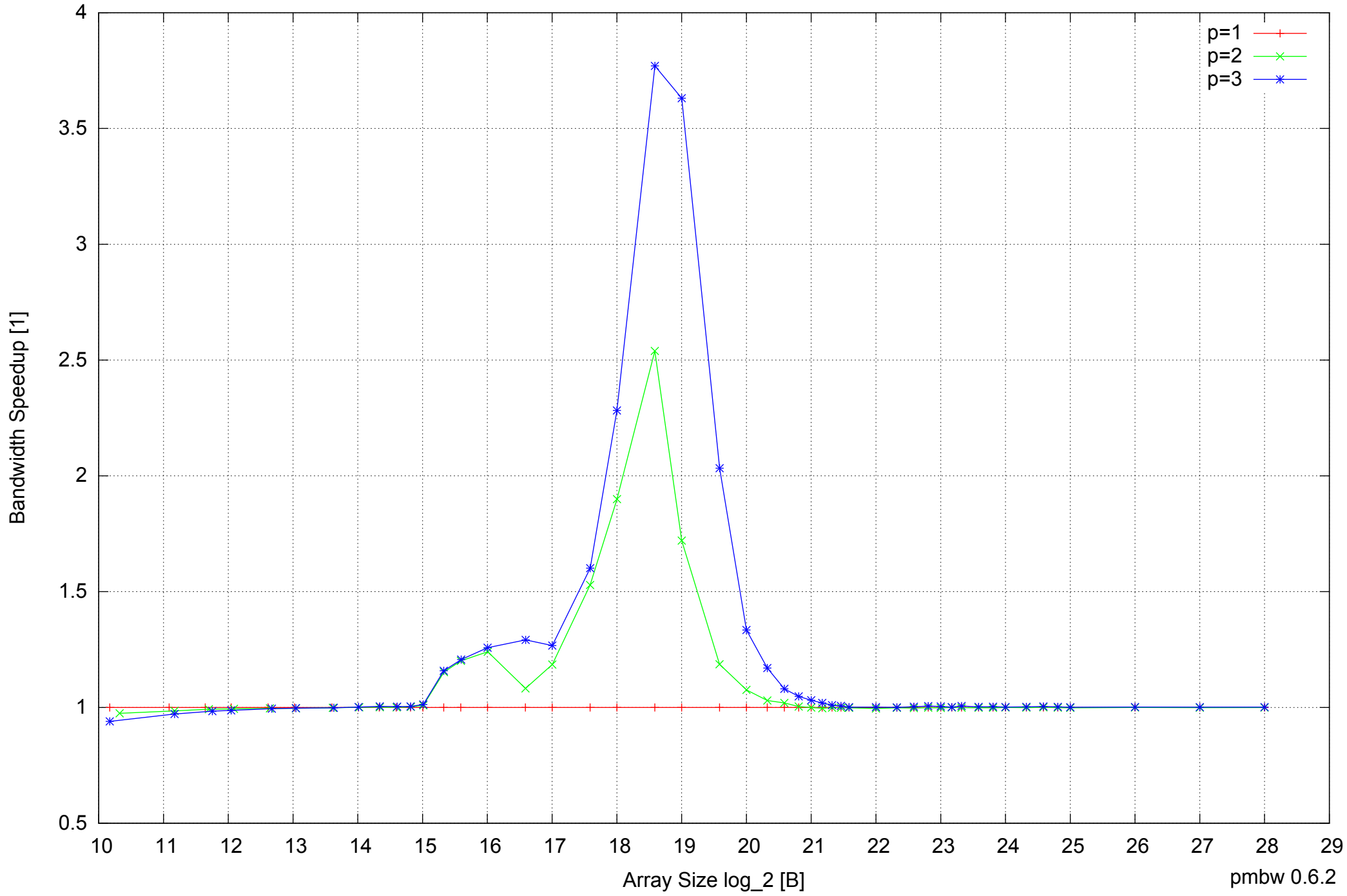
BeagleBone Black: AM335x 1GHz ARM Cortex-A8 512MB - Speedup of Parallel Memory Bandwidth - ScanRead64PtrSimpleLoop
