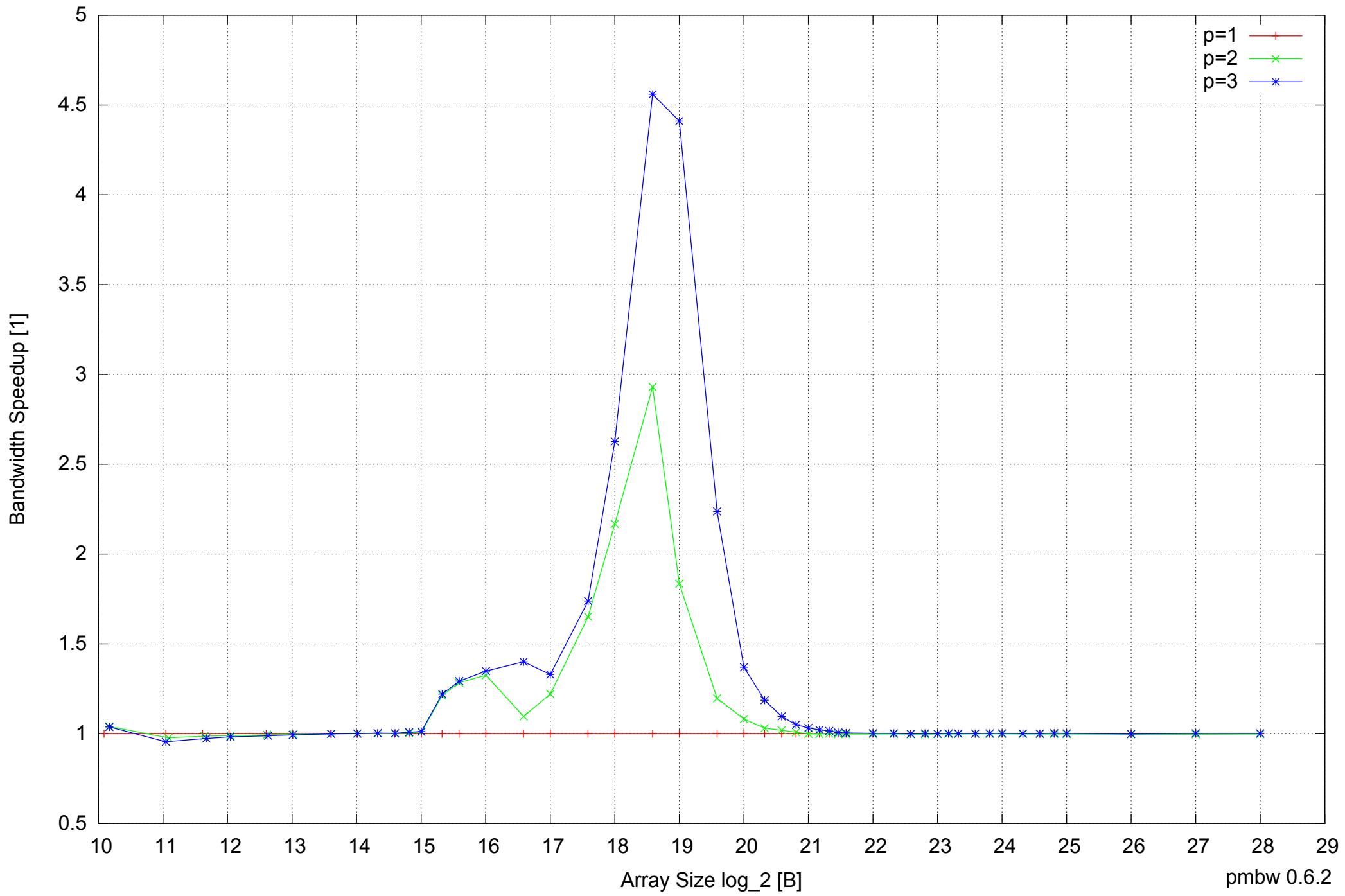
BeagleBone Black: AM335x 1GHz ARM Cortex-A8 512MB - Speedup of Parallel Memory Bandwidth - ScanRead32PtrUnrollLoop
