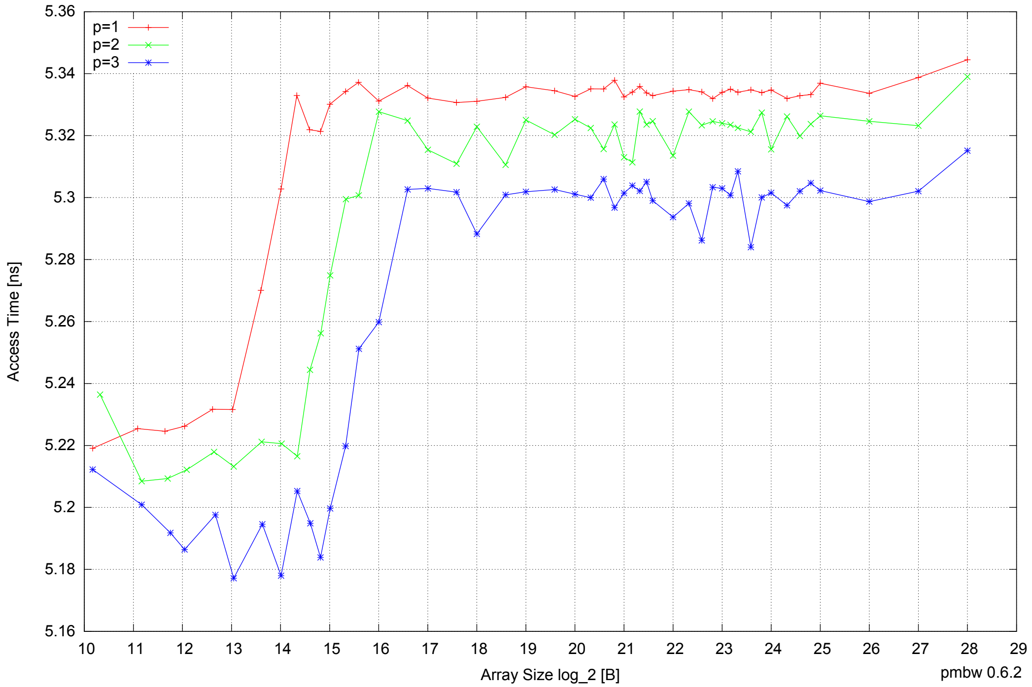
BeagleBone Black: AM335x 1GHz ARM Cortex-A8 512MB - Parallel Memory Access Time - ScanWrite64PtrUnrollLoop
