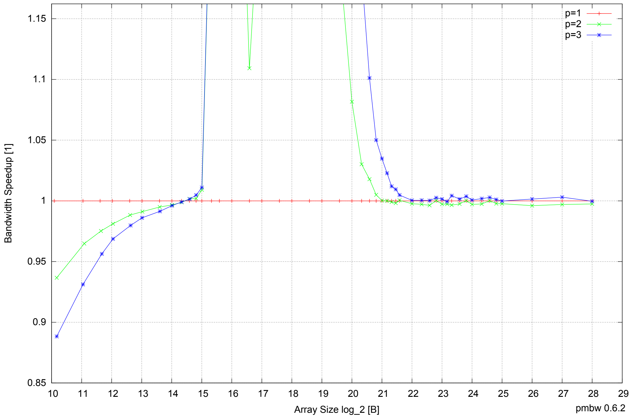
BeagleBone Black: AM335x 1GHz ARM Cortex-A8 512MB - Speedup of Parallel Memory Bandwidth (enlarged) - ScanRead32PtrMultiLoop
