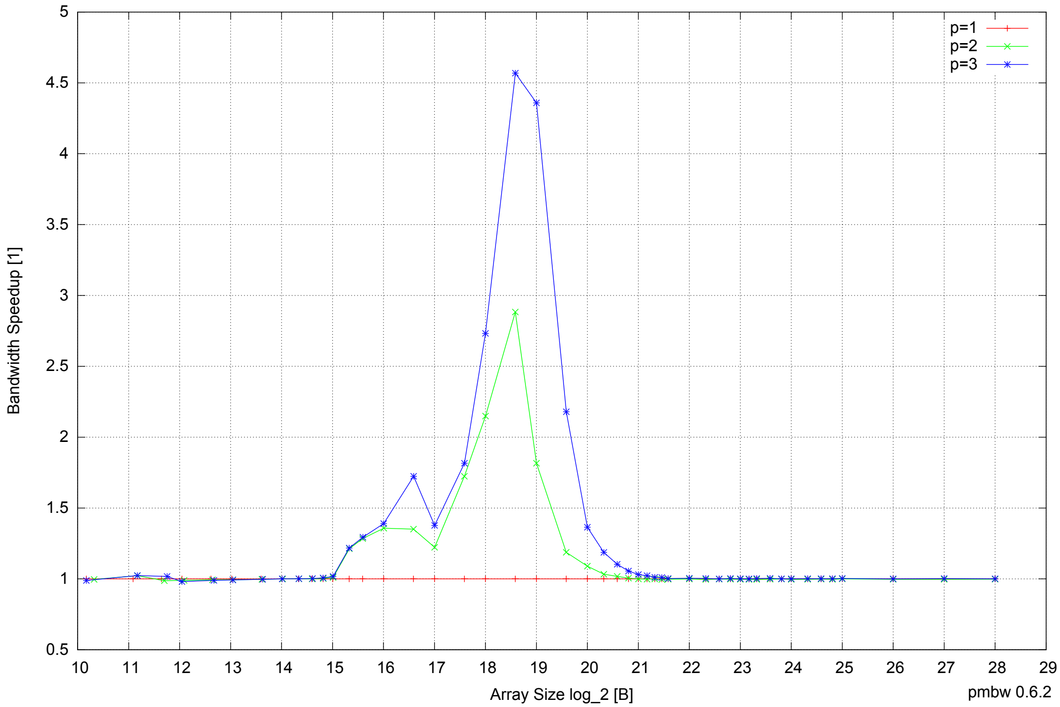
BeagleBone Black: AM335x 1GHz ARM Cortex-A8 512MB - Speedup of Parallel Memory Bandwidth - ScanRead64PtrUnrollLoop
