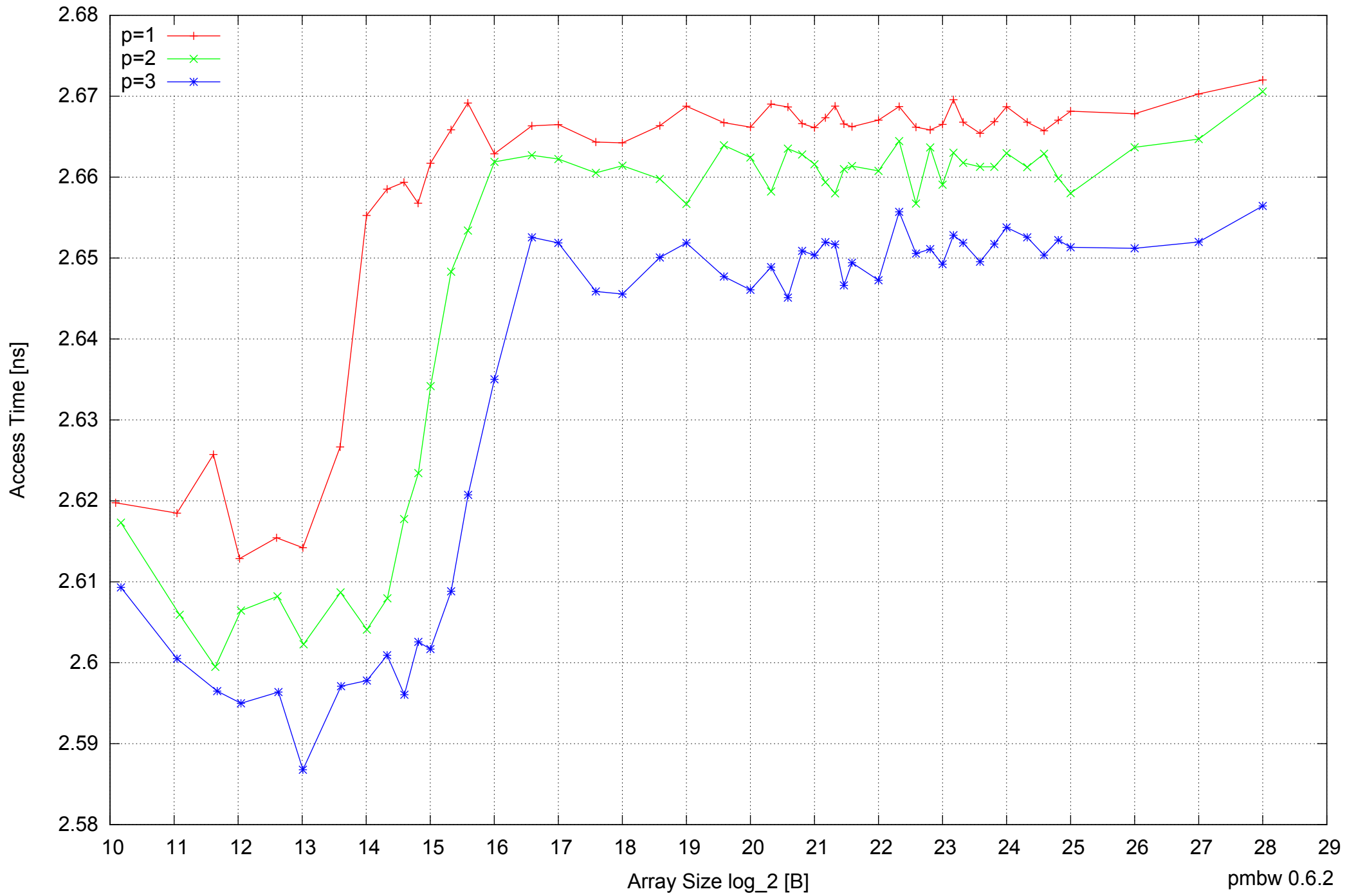
BeagleBone Black: AM335x 1GHz ARM Cortex-A8 512MB - Parallel Memory Access Time - ScanWrite32PtrUnrollLoop
