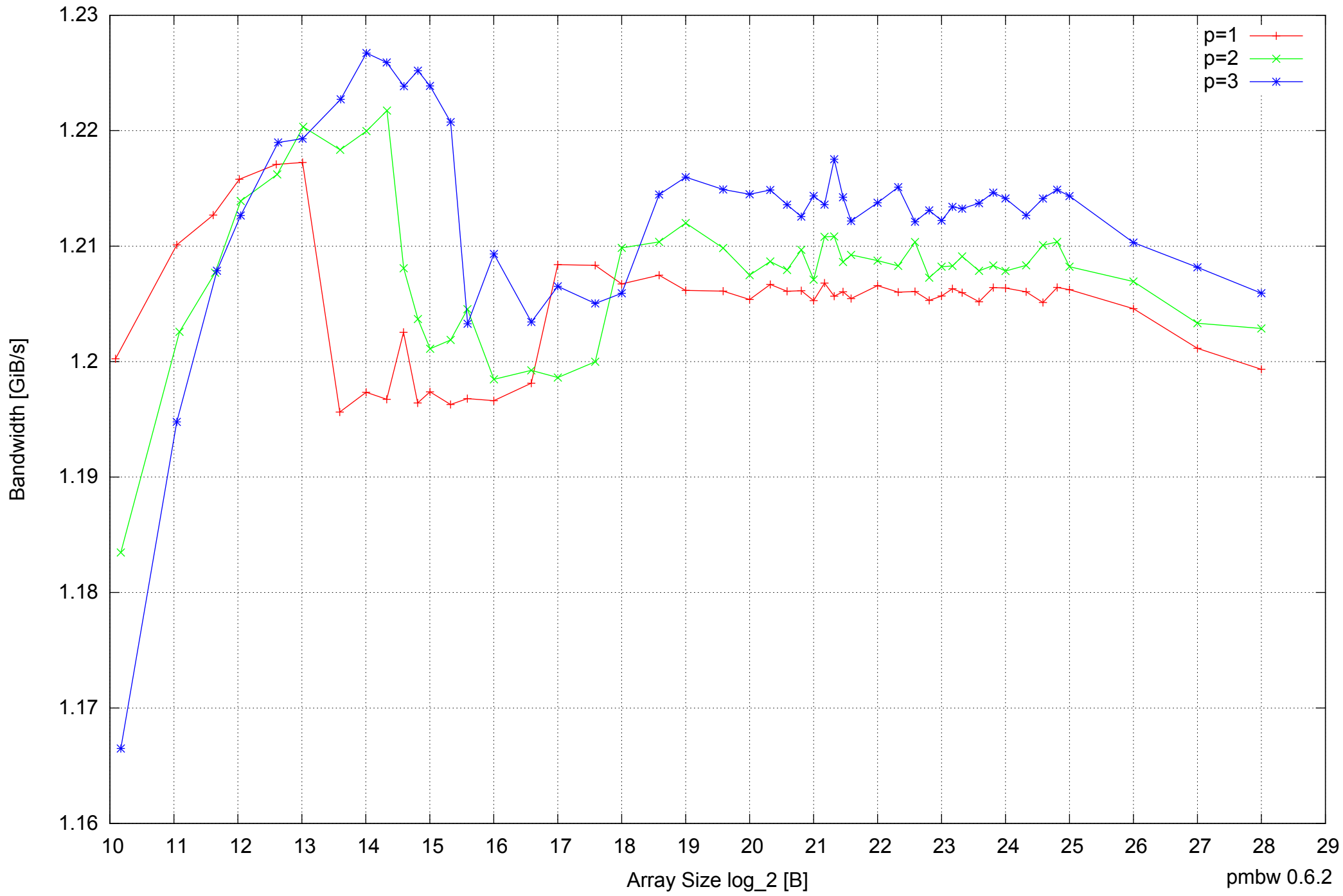
BeagleBone Black: AM335x 1GHz ARM Cortex-A8 512MB - Parallel Memory Bandwidth - ScanWrite32IndexSimpleLoop
