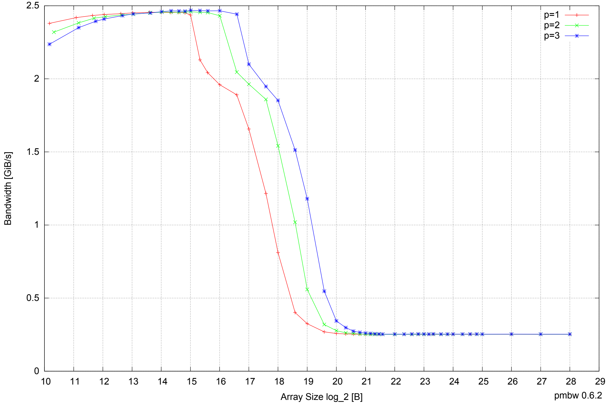
BeagleBone Black: AM335x 1GHz ARM Cortex-A8 512MB - Parallel Memory Bandwidth - ScanRead64PtrSimpleLoop
