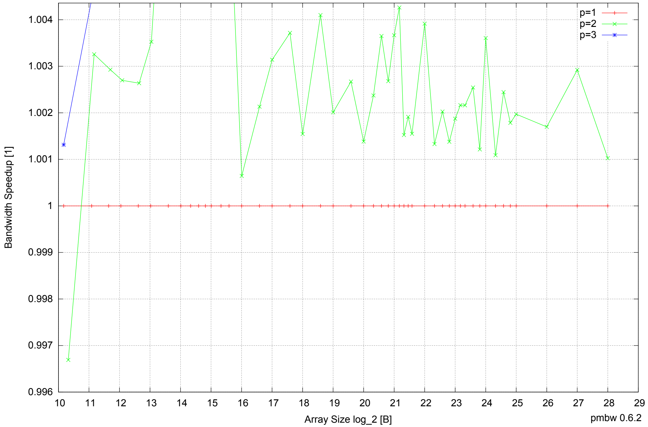
BeagleBone Black: AM335x 1GHz ARM Cortex-A8 512MB - Speedup of Parallel Memory Bandwidth (enlarged) - ScanWrite64PtrUnrollLoop
