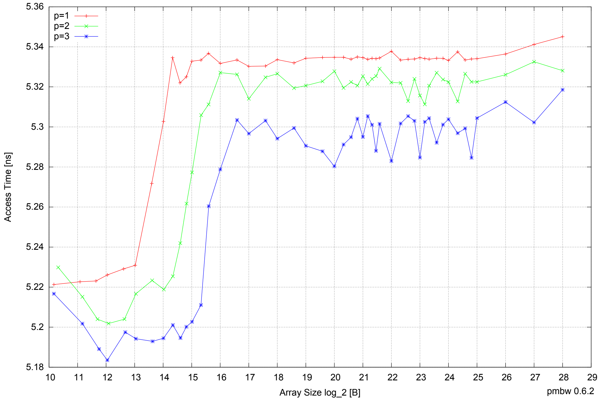
BeagleBone Black: AM335x 1GHz ARM Cortex-A8 512MB - Parallel Memory Access Time - ScanWrite64PtrSimpleLoop
