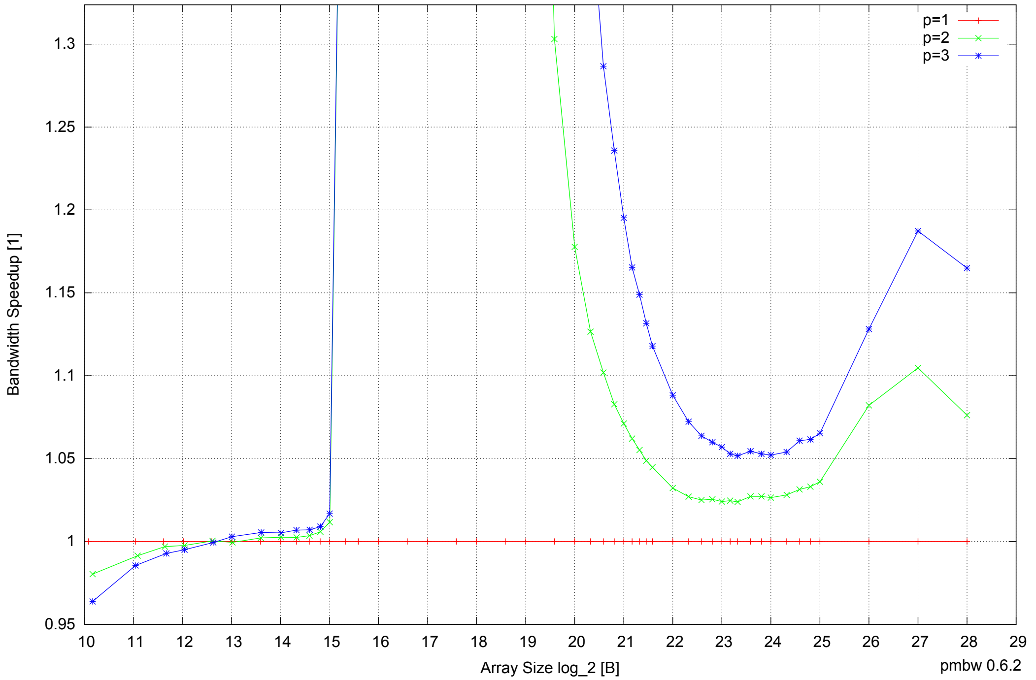
BeagleBone Black: AM335x 1GHz ARM Cortex-A8 512MB - Speedup of Parallel Memory Bandwidth (enlarged) - PermRead32SimpleLoop
