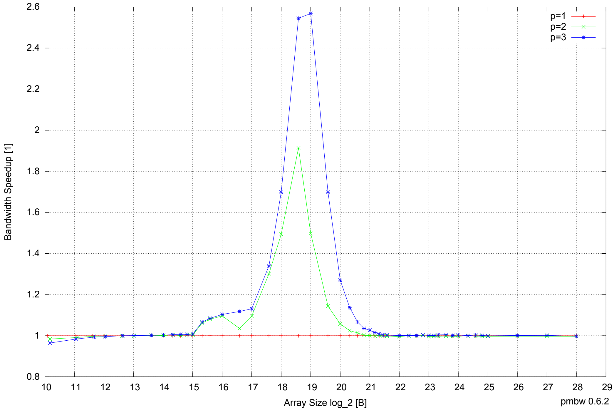
BeagleBone Black: AM335x 1GHz ARM Cortex-A8 512MB - Speedup of Parallel Memory Bandwidth - ScanRead32IndexSimpleLoop
