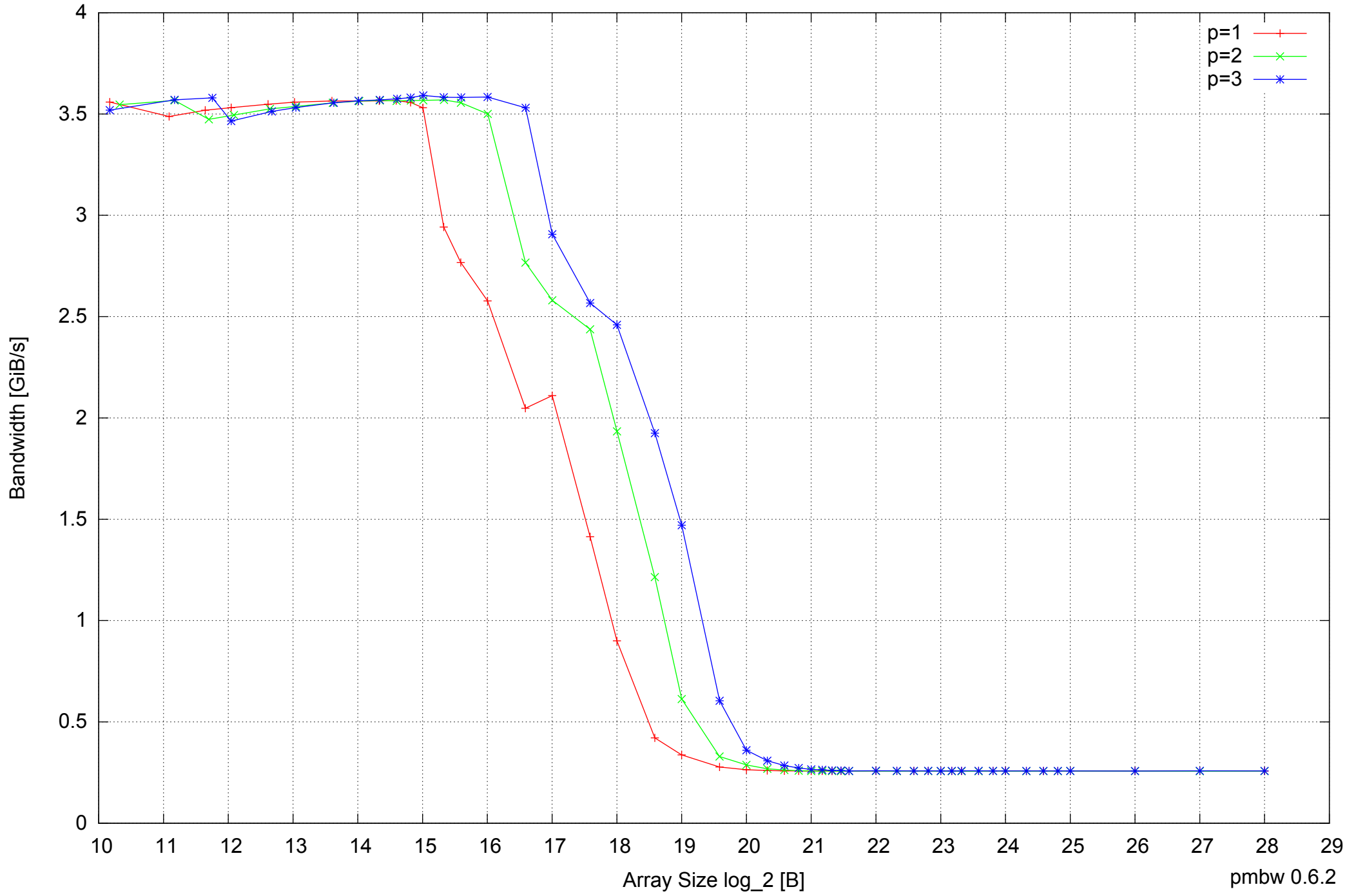
BeagleBone Black: AM335x 1GHz ARM Cortex-A8 512MB - Parallel Memory Bandwidth - ScanRead64PtrUnrollLoop
