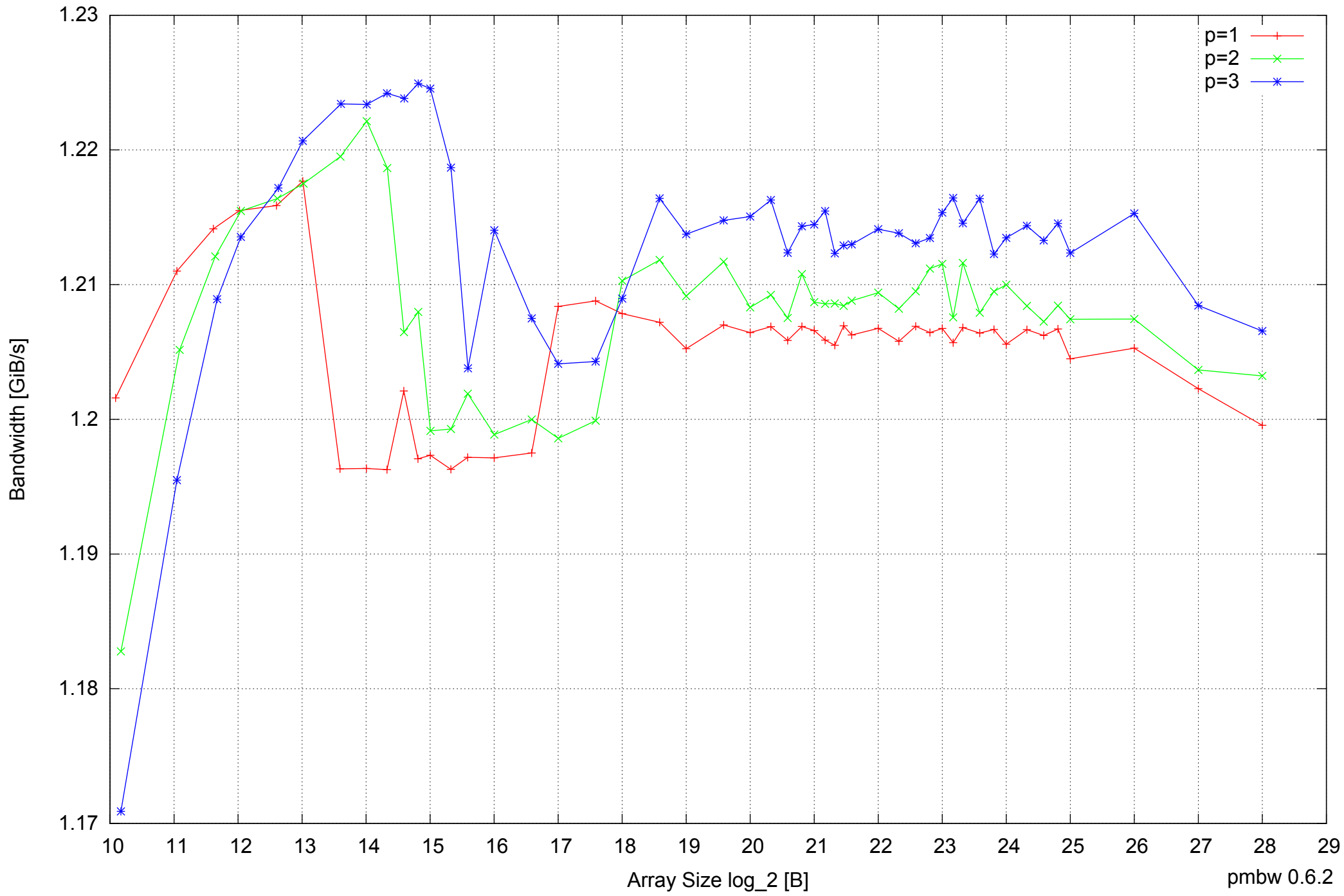
BeagleBone Black: AM335x 1GHz ARM Cortex-A8 512MB - Parallel Memory Bandwidth - ScanWrite32PtrSimpleLoop
