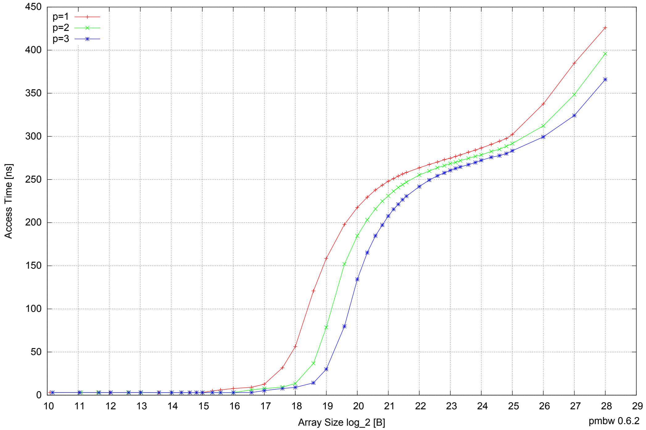
BeagleBone Black: AM335x 1GHz ARM Cortex-A8 512MB - Parallel Memory Access Time - PermRead32UnrollLoop
