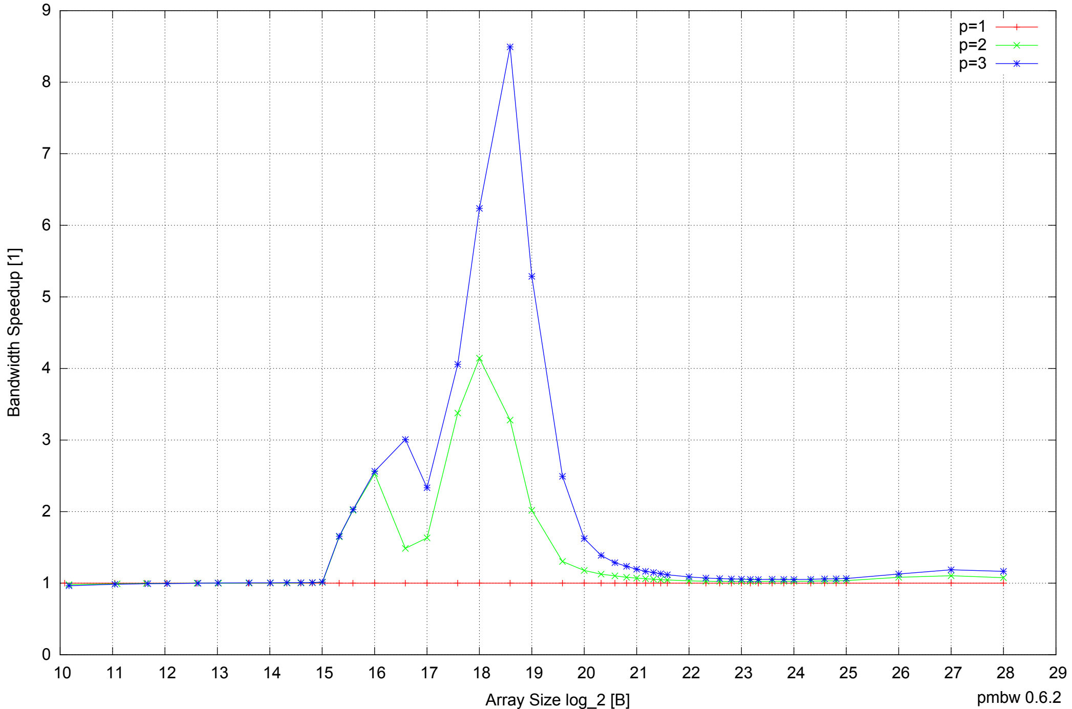
BeagleBone Black: AM335x 1GHz ARM Cortex-A8 512MB - Speedup of Parallel Memory Bandwidth - PermRead32SimpleLoop
