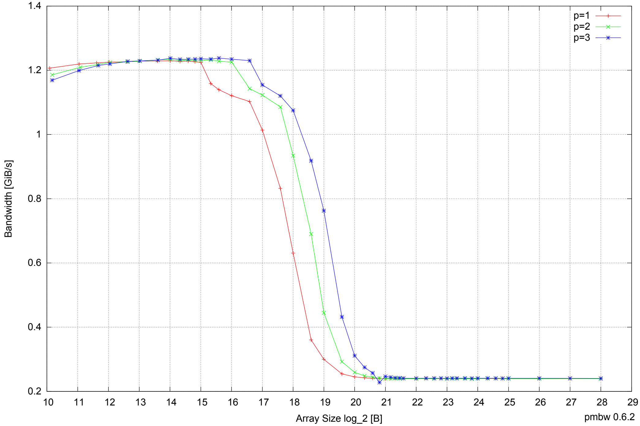
BeagleBone Black: AM335x 1GHz ARM Cortex-A8 512MB - Parallel Memory Bandwidth - ScanRead32PtrSimpleLoop
