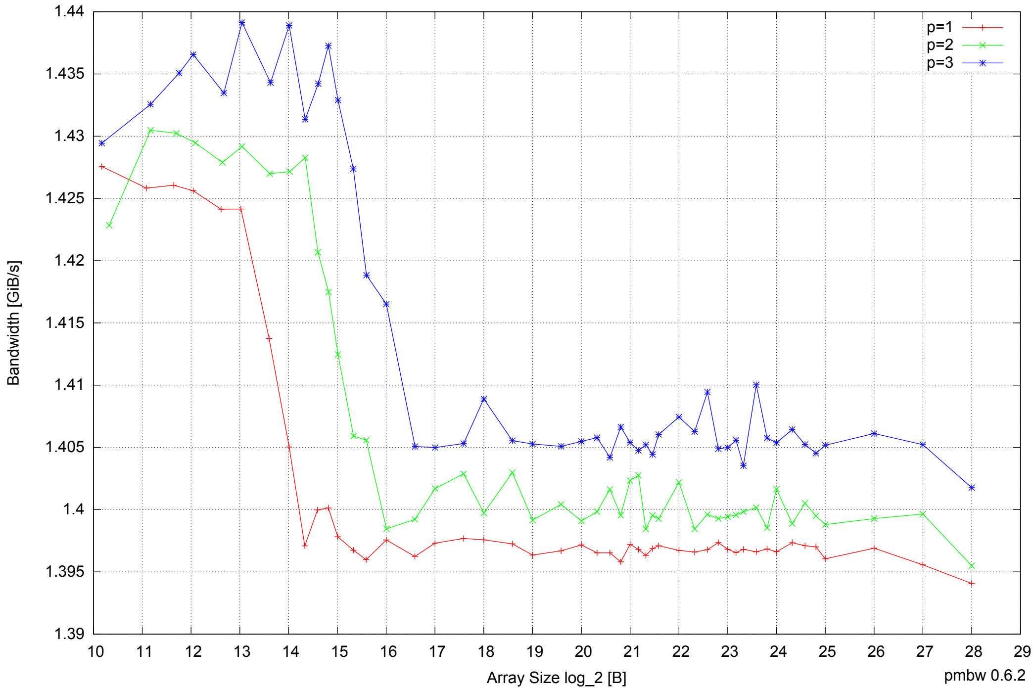
BeagleBone Black: AM335x 1GHz ARM Cortex-A8 512MB - Parallel Memory Bandwidth - ScanWrite64PtrUnrollLoop
