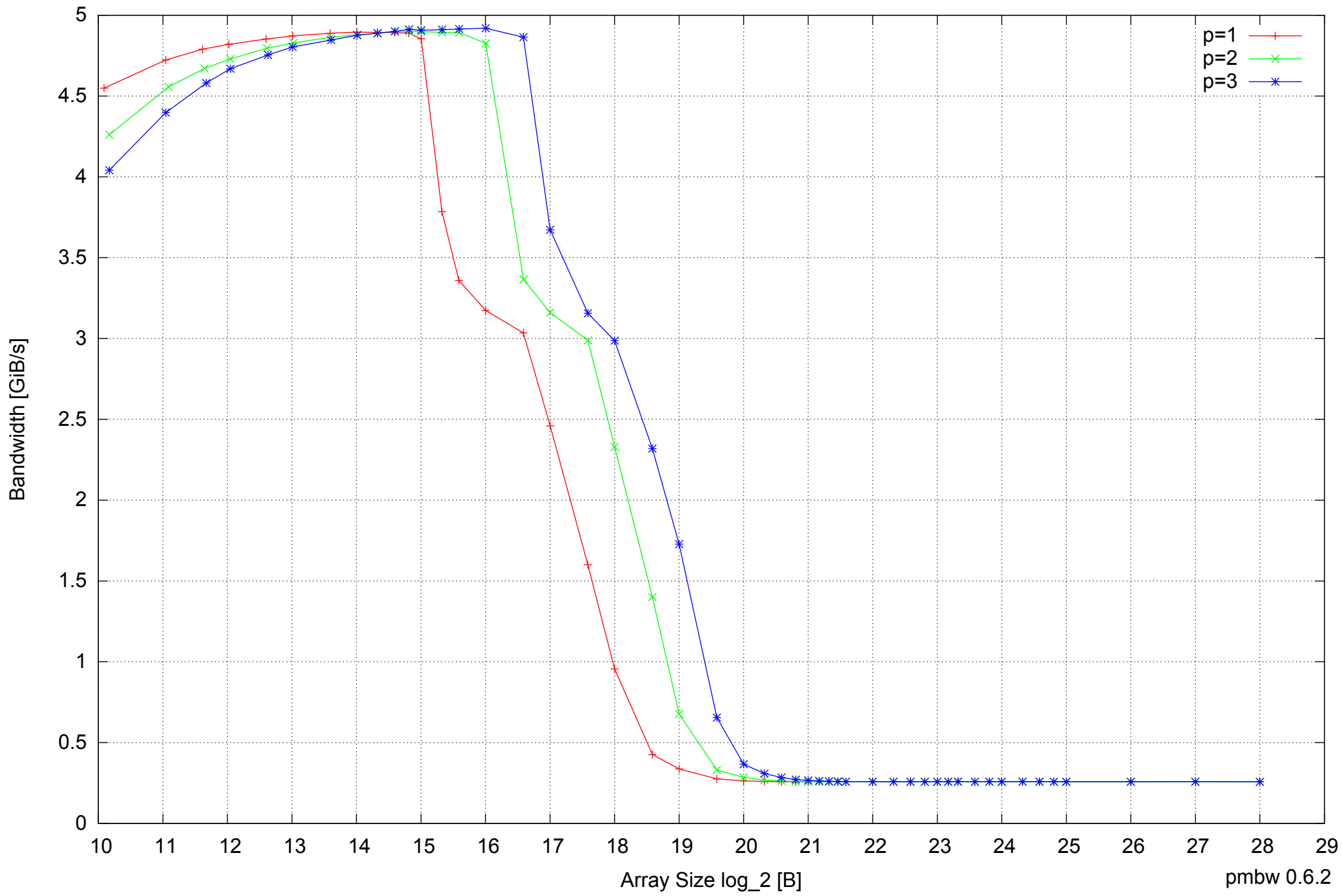
BeagleBone Black: AM335x 1GHz ARM Cortex-A8 512MB - Parallel Memory Bandwidth - ScanRead32PtrMultiLoop
