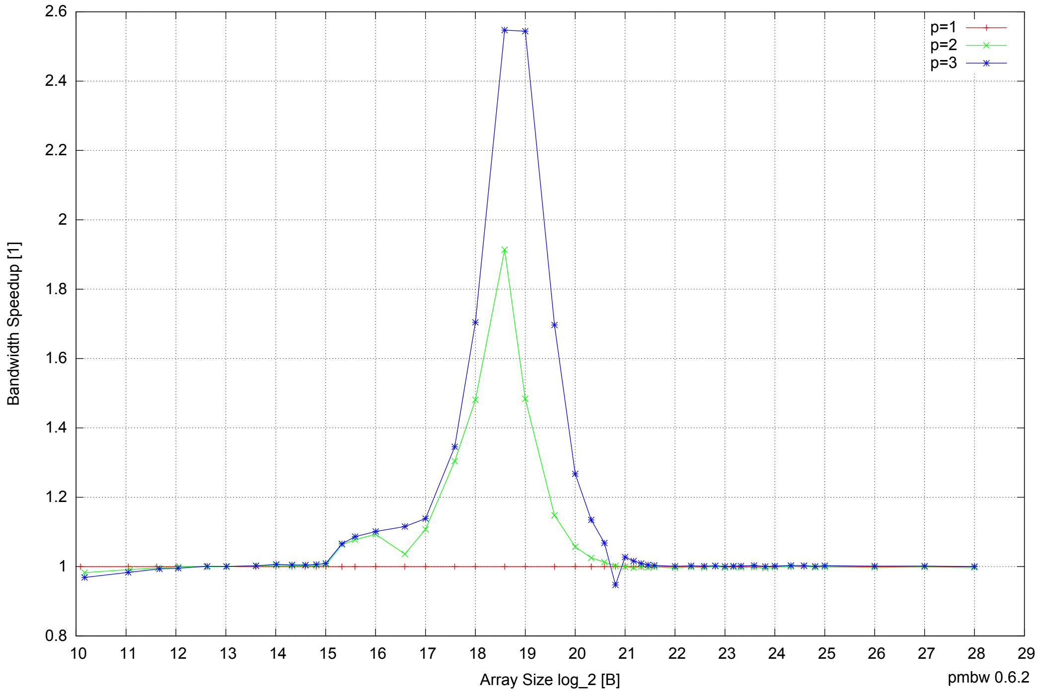
BeagleBone Black: AM335x 1GHz ARM Cortex-A8 512MB - Speedup of Parallel Memory Bandwidth - ScanRead32PtrSimpleLoop
