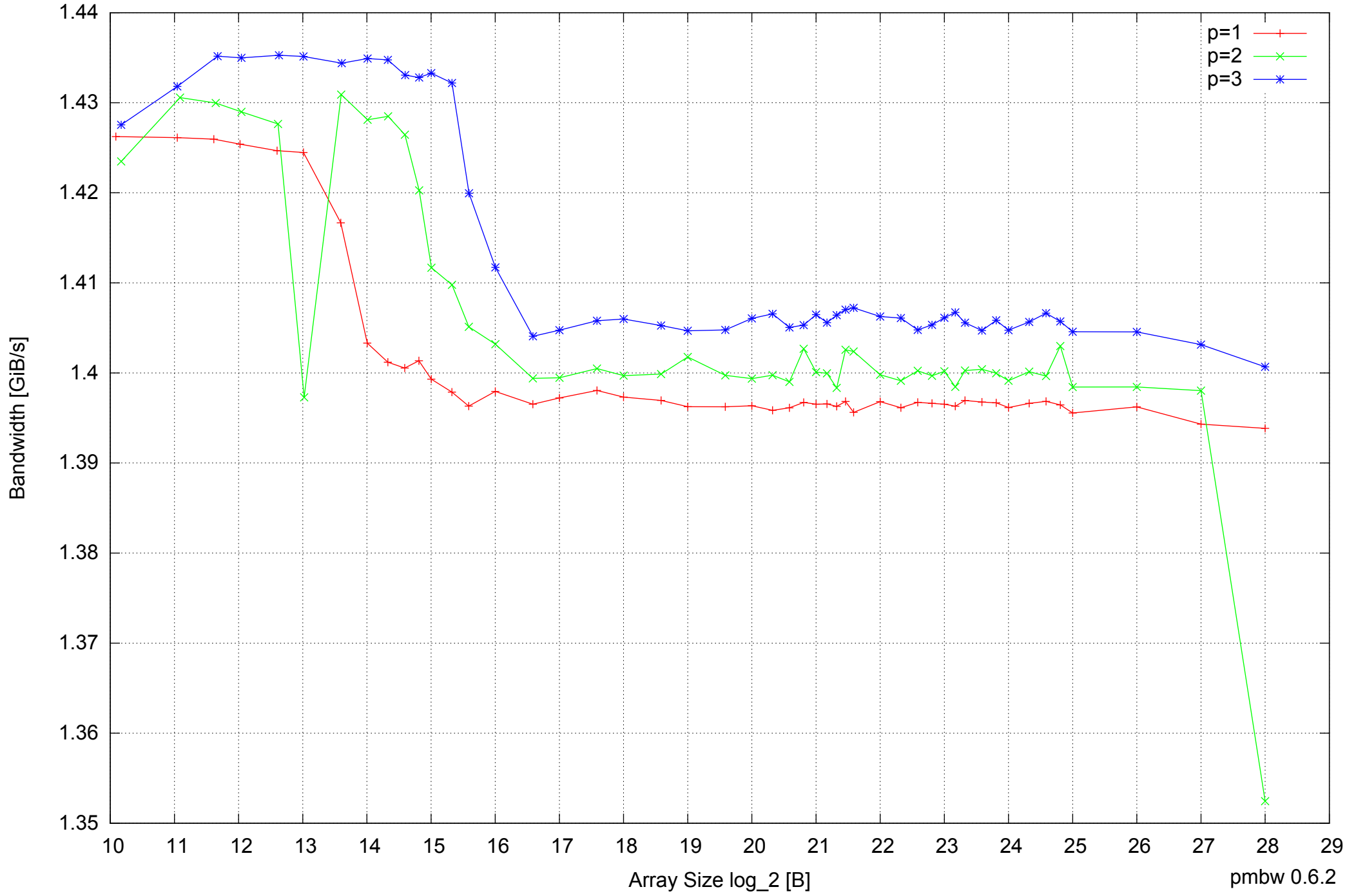
BeagleBone Black: AM335x 1GHz ARM Cortex-A8 512MB - Parallel Memory Bandwidth - ScanWrite32PtrMultiLoop
