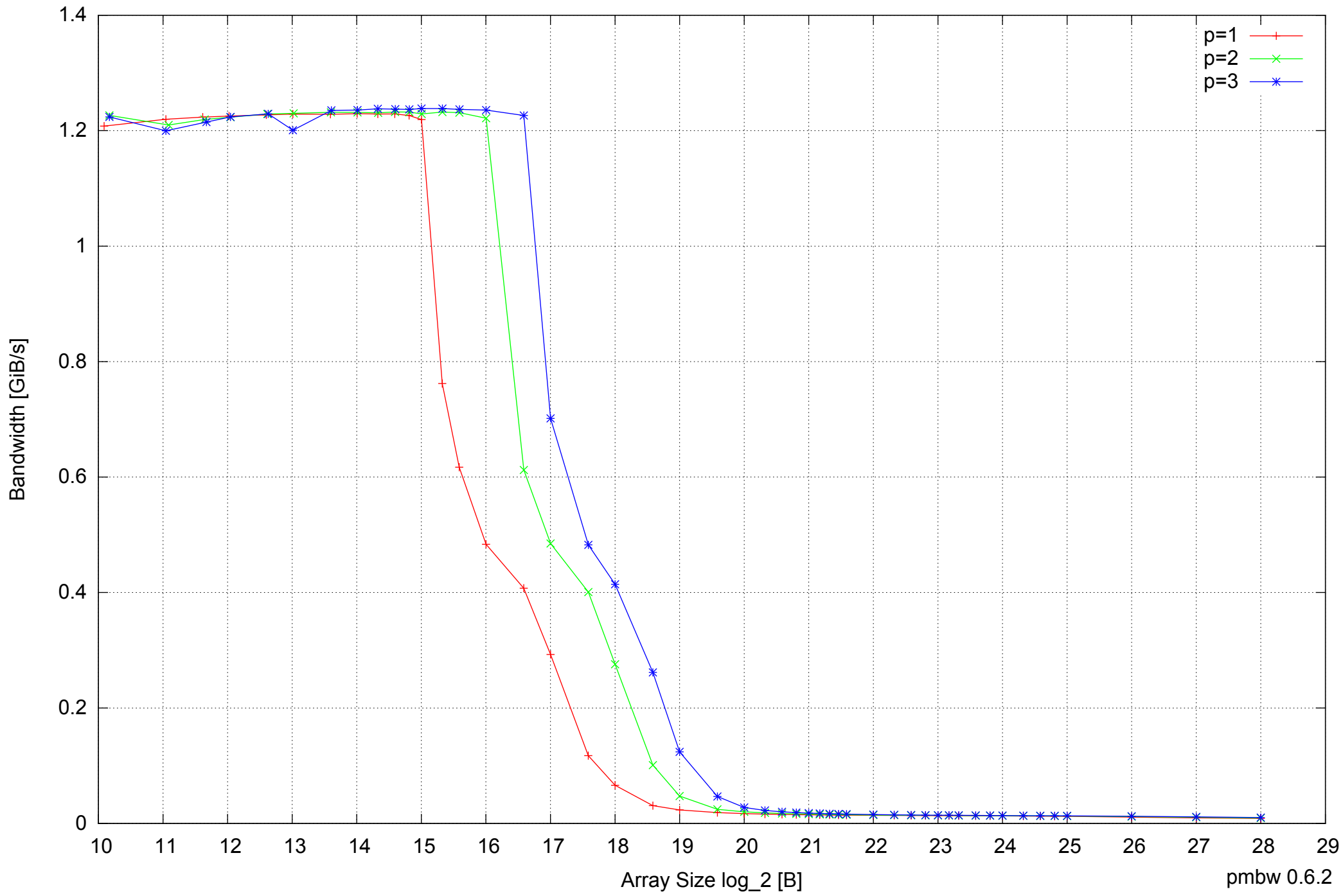
BeagleBone Black: AM335x 1GHz ARM Cortex-A8 512MB - Parallel Memory Bandwidth - PermRead32UnrollLoop
