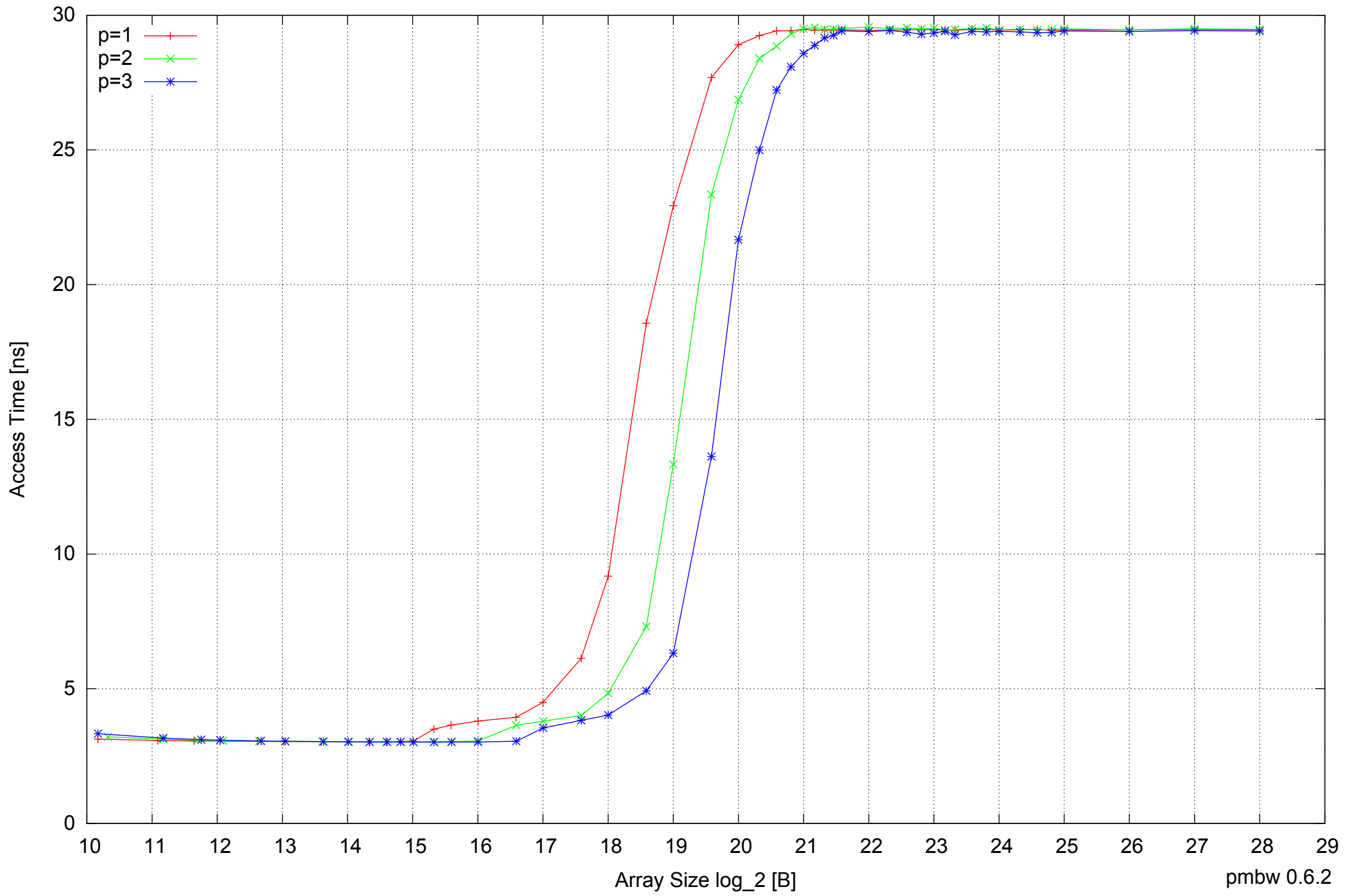
BeagleBone Black: AM335x 1GHz ARM Cortex-A8 512MB - Parallel Memory Access Time - ScanRead64PtrSimpleLoop
