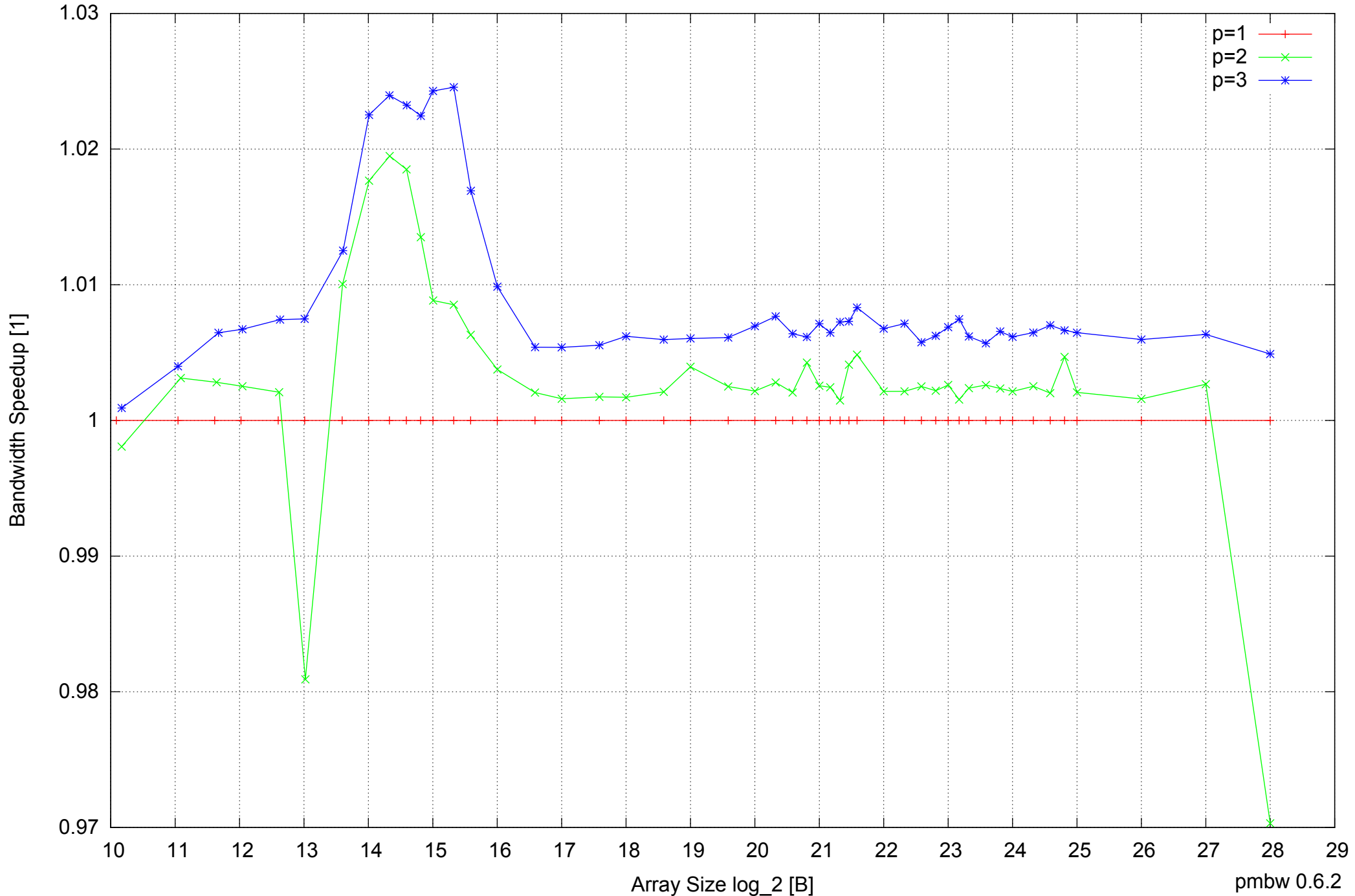
BeagleBone Black: AM335x 1GHz ARM Cortex-A8 512MB - Speedup of Parallel Memory Bandwidth - ScanWrite32PtrMultiLoop
