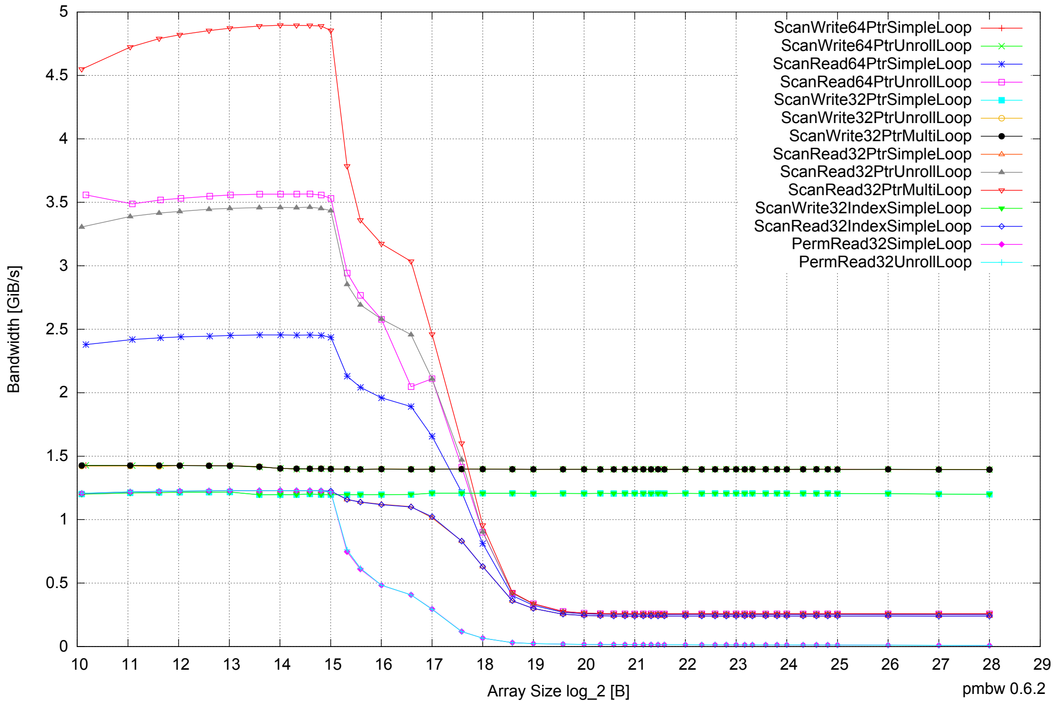
BeagleBone Black: AM335x 1GHz ARM Cortex-A8 512MB - One Thread Memory Bandwidth
