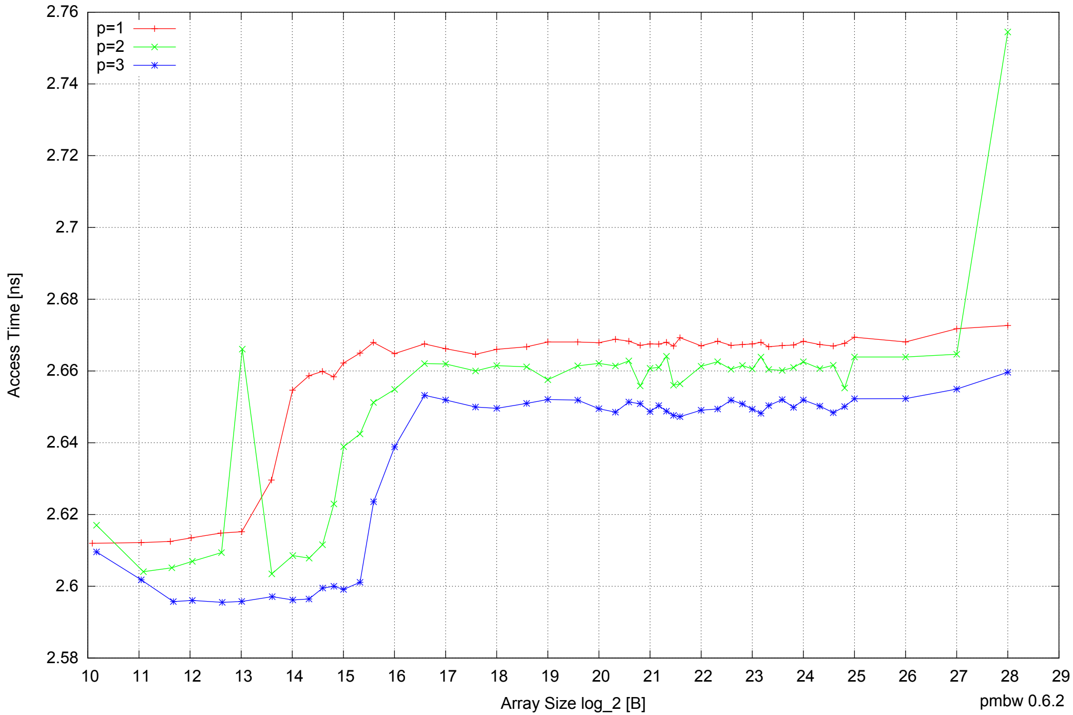
BeagleBone Black: AM335x 1GHz ARM Cortex-A8 512MB - Parallel Memory Access Time - ScanWrite32PtrMultiLoop
