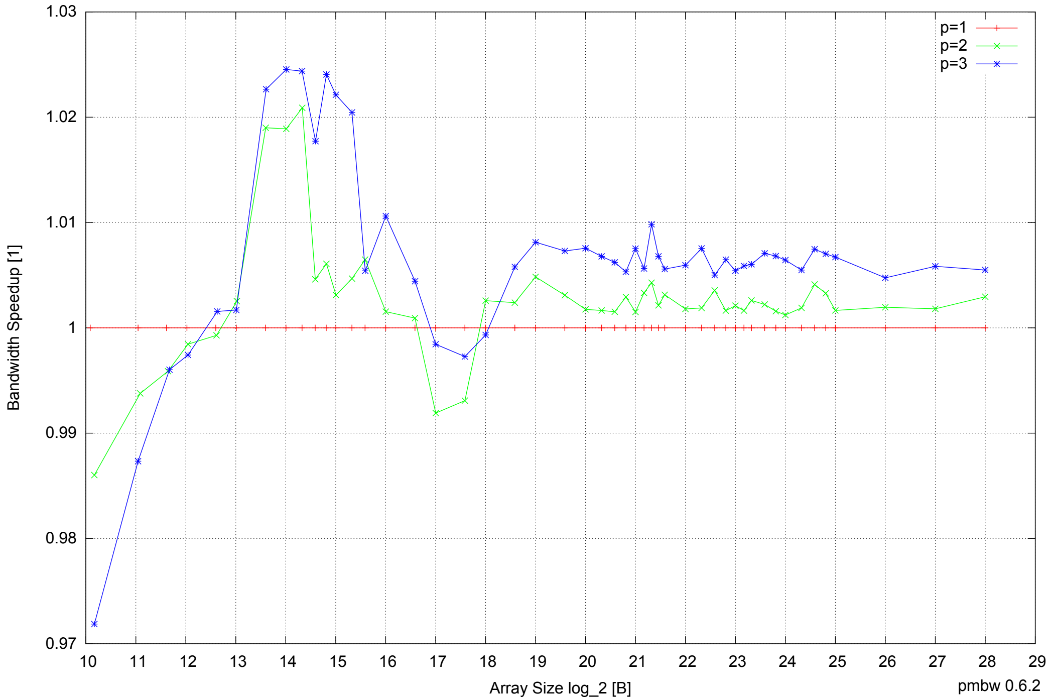
BeagleBone Black: AM335x 1GHz ARM Cortex-A8 512MB - Speedup of Parallel Memory Bandwidth - ScanWrite32IndexSimpleLoop
