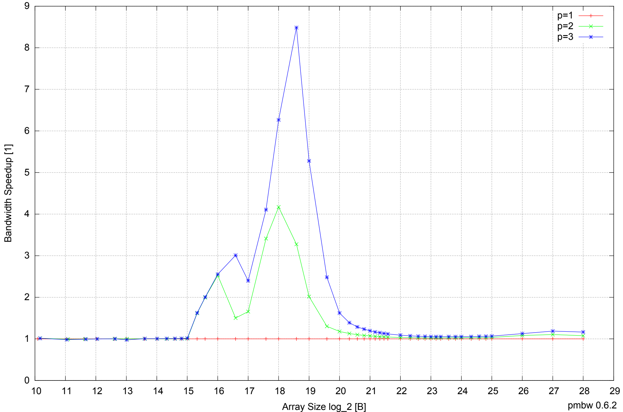
BeagleBone Black: AM335x 1GHz ARM Cortex-A8 512MB - Speedup of Parallel Memory Bandwidth - PermRead32UnrollLoop
