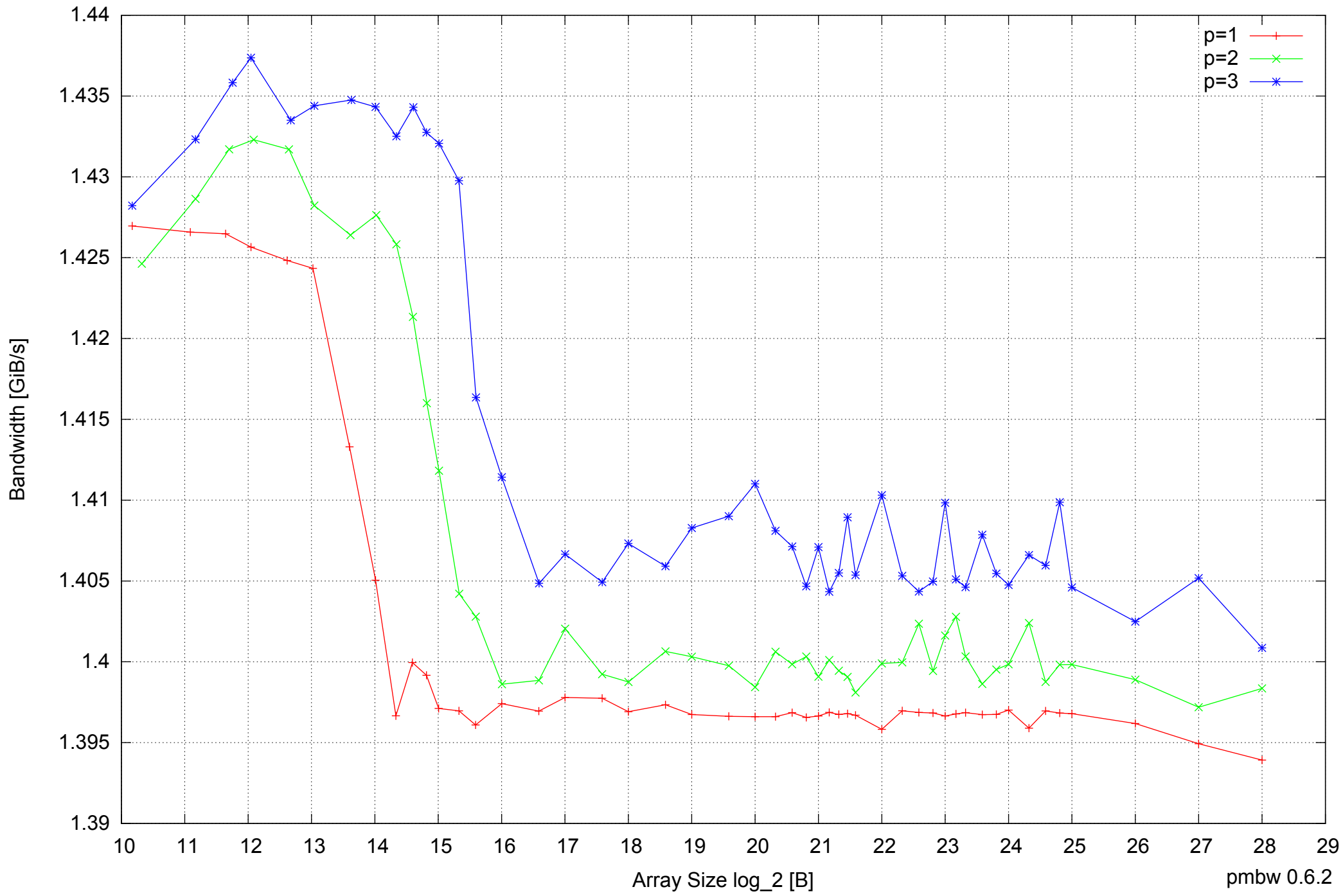
BeagleBone Black: AM335x 1GHz ARM Cortex-A8 512MB - Parallel Memory Bandwidth - ScanWrite64PtrSimpleLoop
