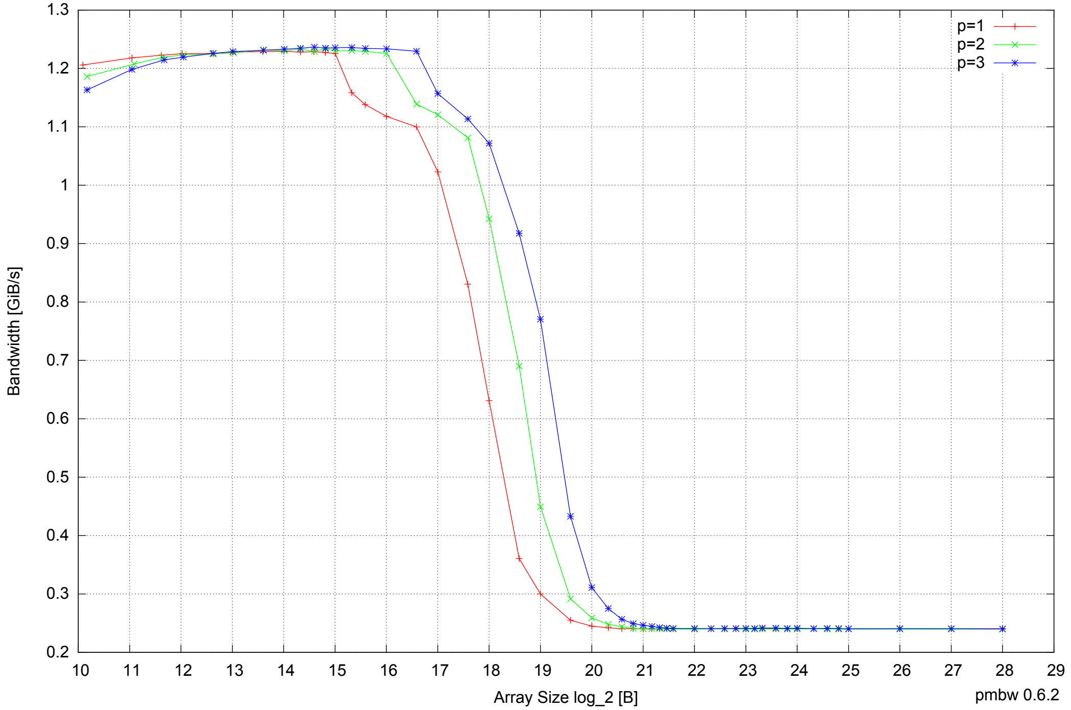
BeagleBone Black: AM335x 1GHz ARM Cortex-A8 512MB - Parallel Memory Bandwidth - ScanRead32IndexSimpleLoop
