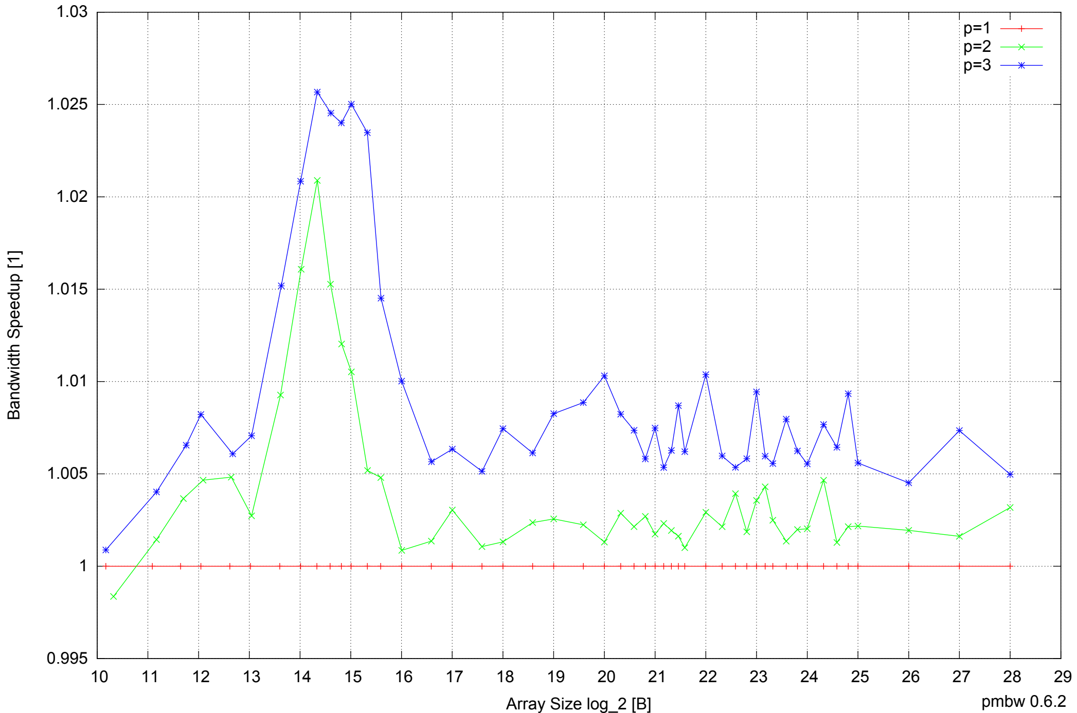
BeagleBone Black: AM335x 1GHz ARM Cortex-A8 512MB - Speedup of Parallel Memory Bandwidth - ScanWrite64PtrSimpleLoop
