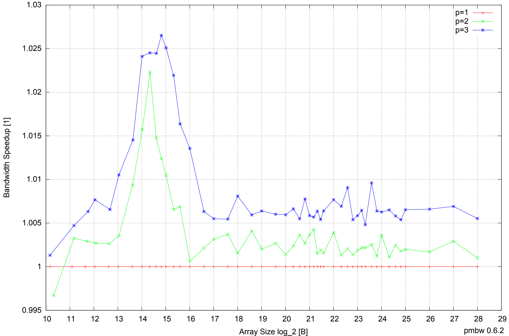
BeagleBone Black: AM335x 1GHz ARM Cortex-A8 512MB - Speedup of Parallel Memory Bandwidth - ScanWrite64PtrUnrollLoop
