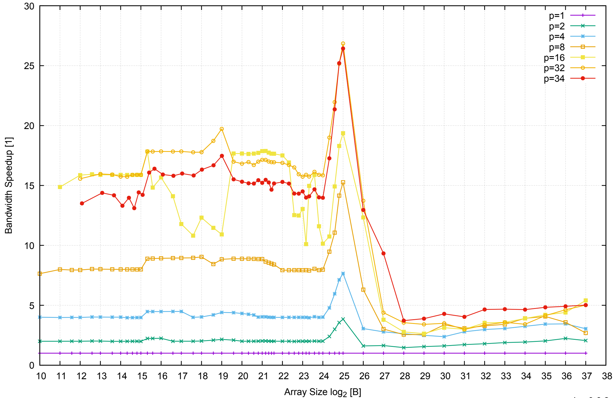
AWS r3.8xlarge - Intel Xeon E5-2676 v3, 2.50 GHz 244GB - Speedup of Parallel Memory Bandwidth - ScanWrite64PtrUnrollLoop
