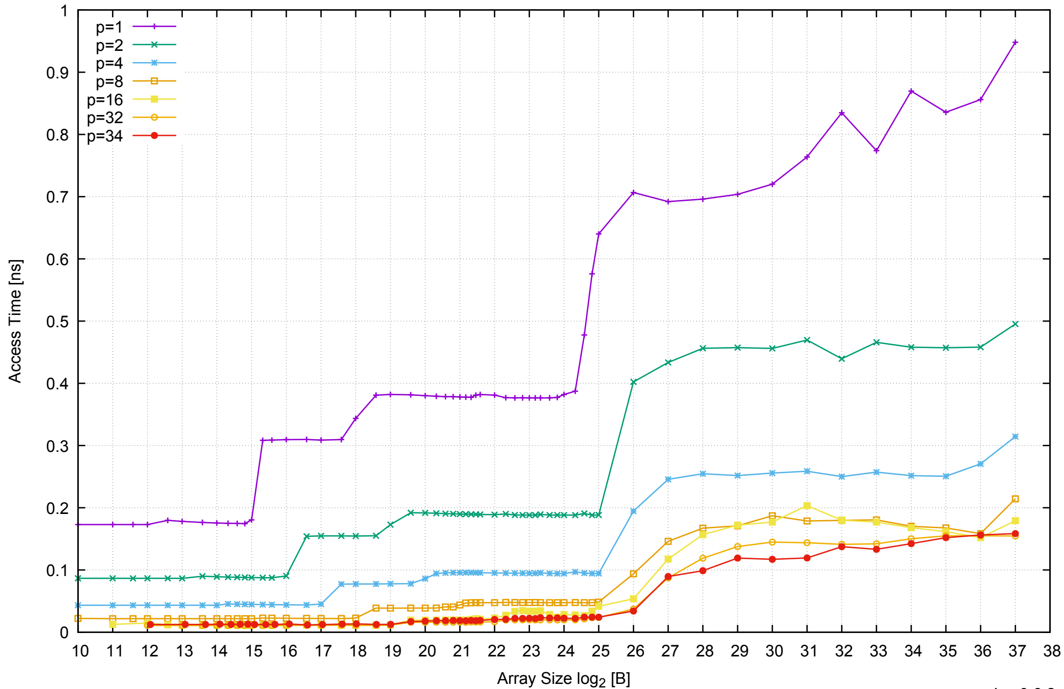
AWS r3.8xlarge - Intel Xeon E5-2676 v3, 2.50 GHz 244GB - Parallel Memory Access Time - ScanRead64PtrUnrollLoop
