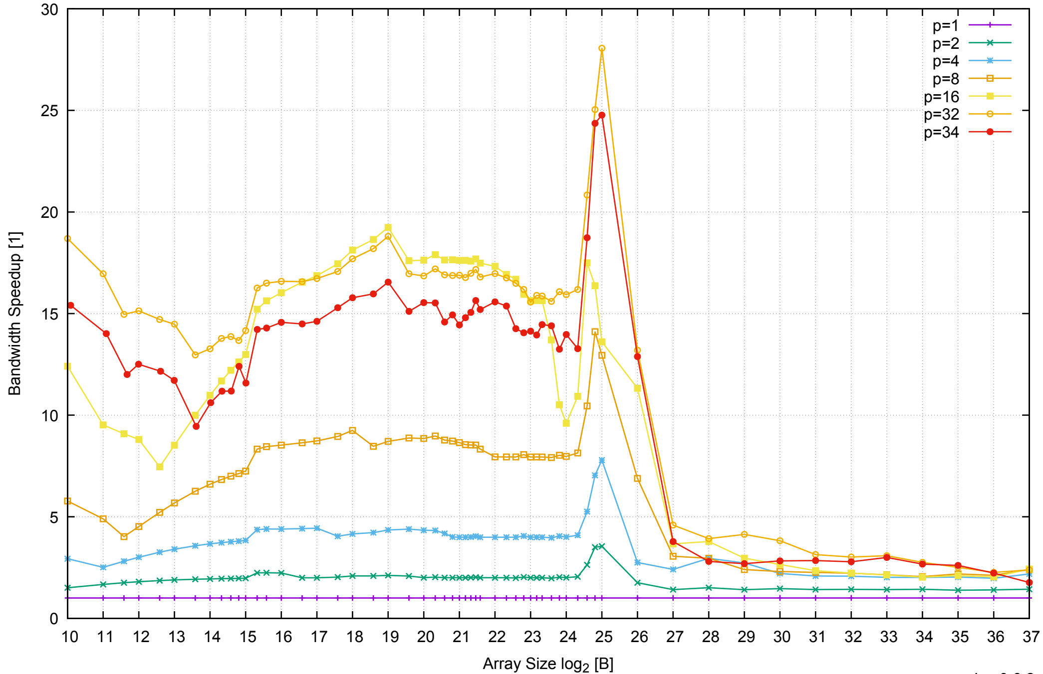
AWS r3.8xlarge - Intel Xeon E5-2676 v3, 2.50 GHz 244GB - Speedup of Parallel Memory Bandwidth - ScanWrite64PtrSimpleLoop
