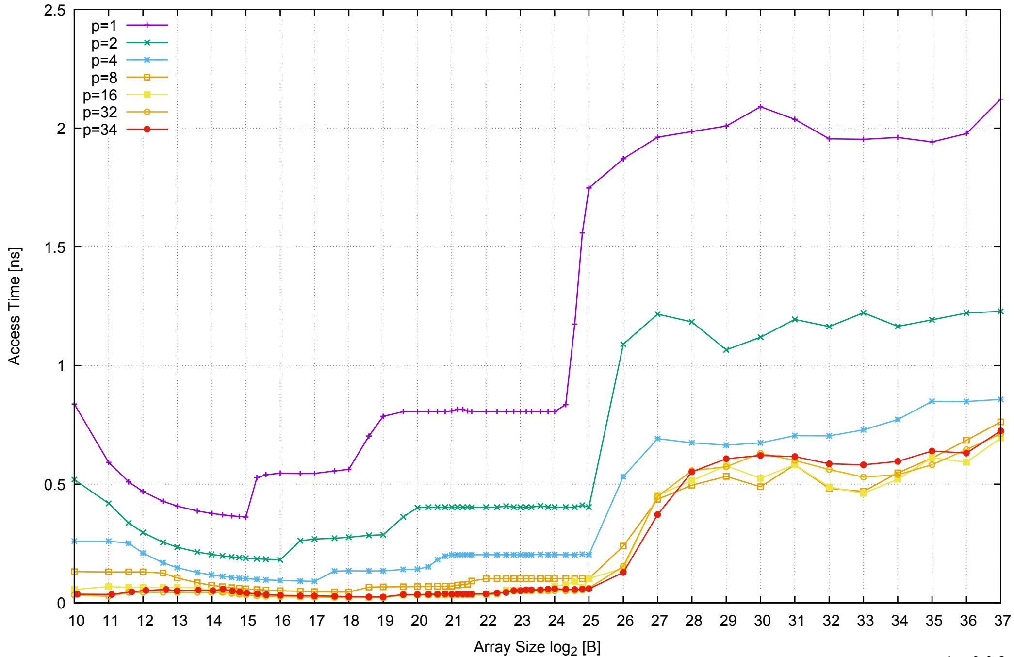
AWS r3.8xlarge - Intel Xeon E5-2676 v3, 2.50 GHz 244GB - Parallel Memory Access Time - ScanWrite128PtrSimpleLoop
