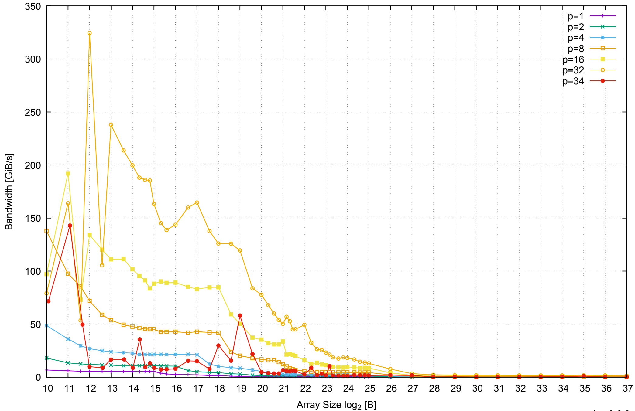
AWS r3.8xlarge - Intel Xeon E5-2676 v3, 2.50 GHz 244GB - Parallel Memory Bandwidth - PermRead64UnrollLoop
