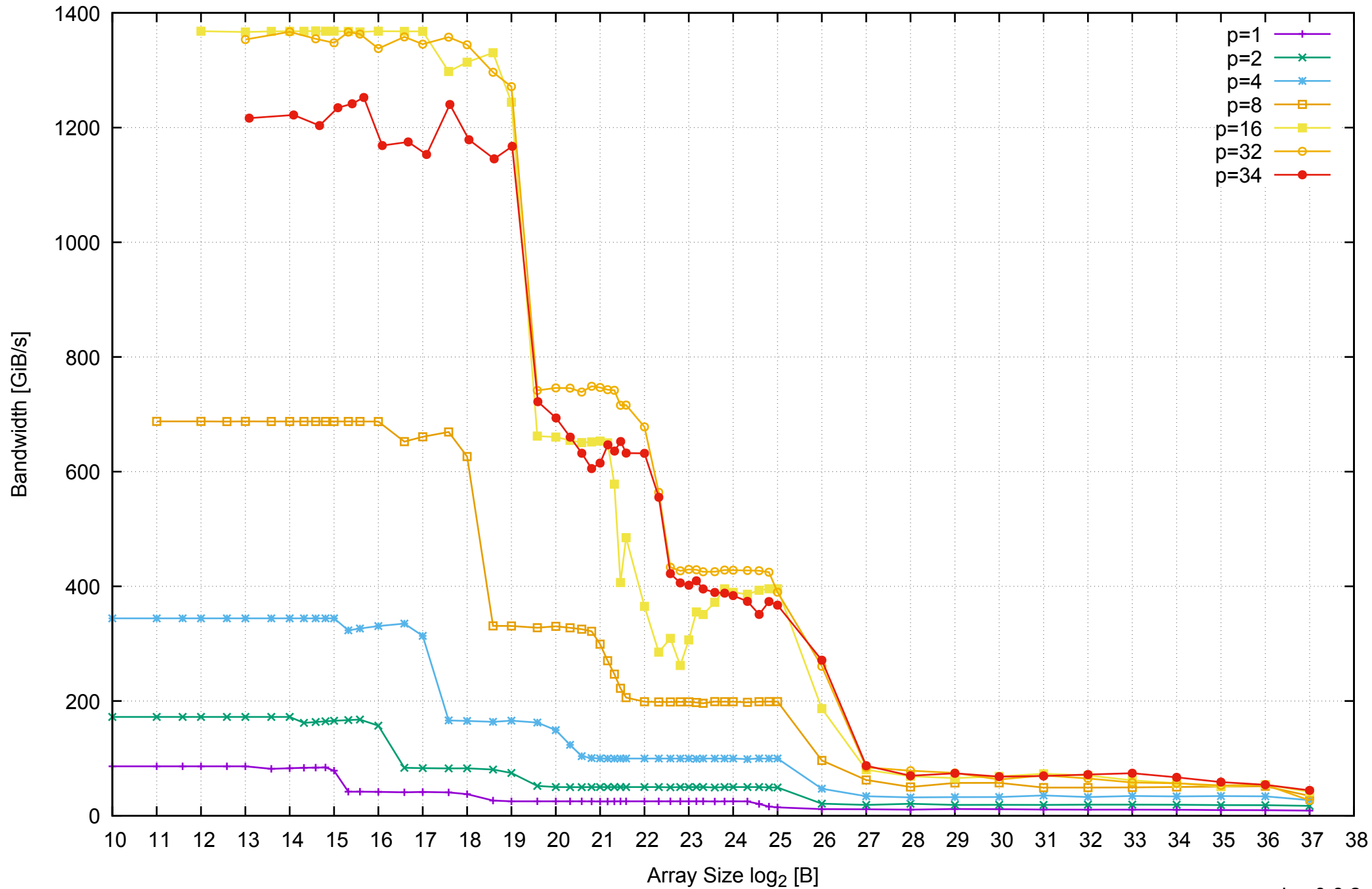
AWS r3.8xlarge - Intel Xeon E5-2676 v3, 2.50 GHz 244GB - Parallel Memory Bandwidth - ScanRead128PtrUnrollLoop
