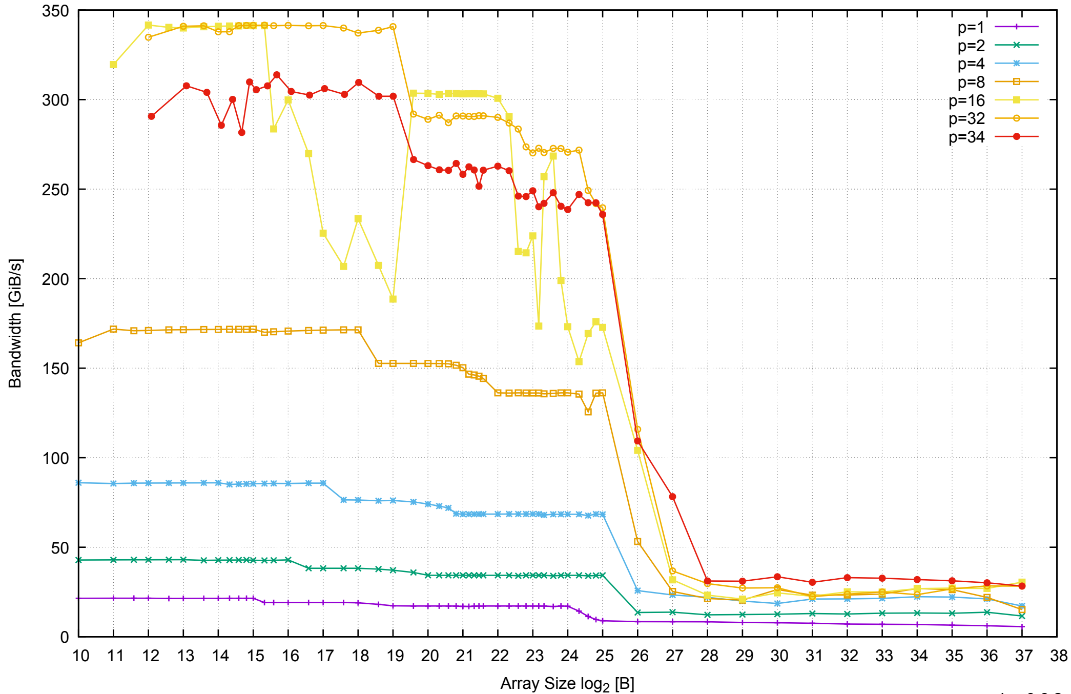
AWS r3.8xlarge - Intel Xeon E5-2676 v3, 2.50 GHz 244GB - Parallel Memory Bandwidth - ScanWrite64PtrUnrollLoop
