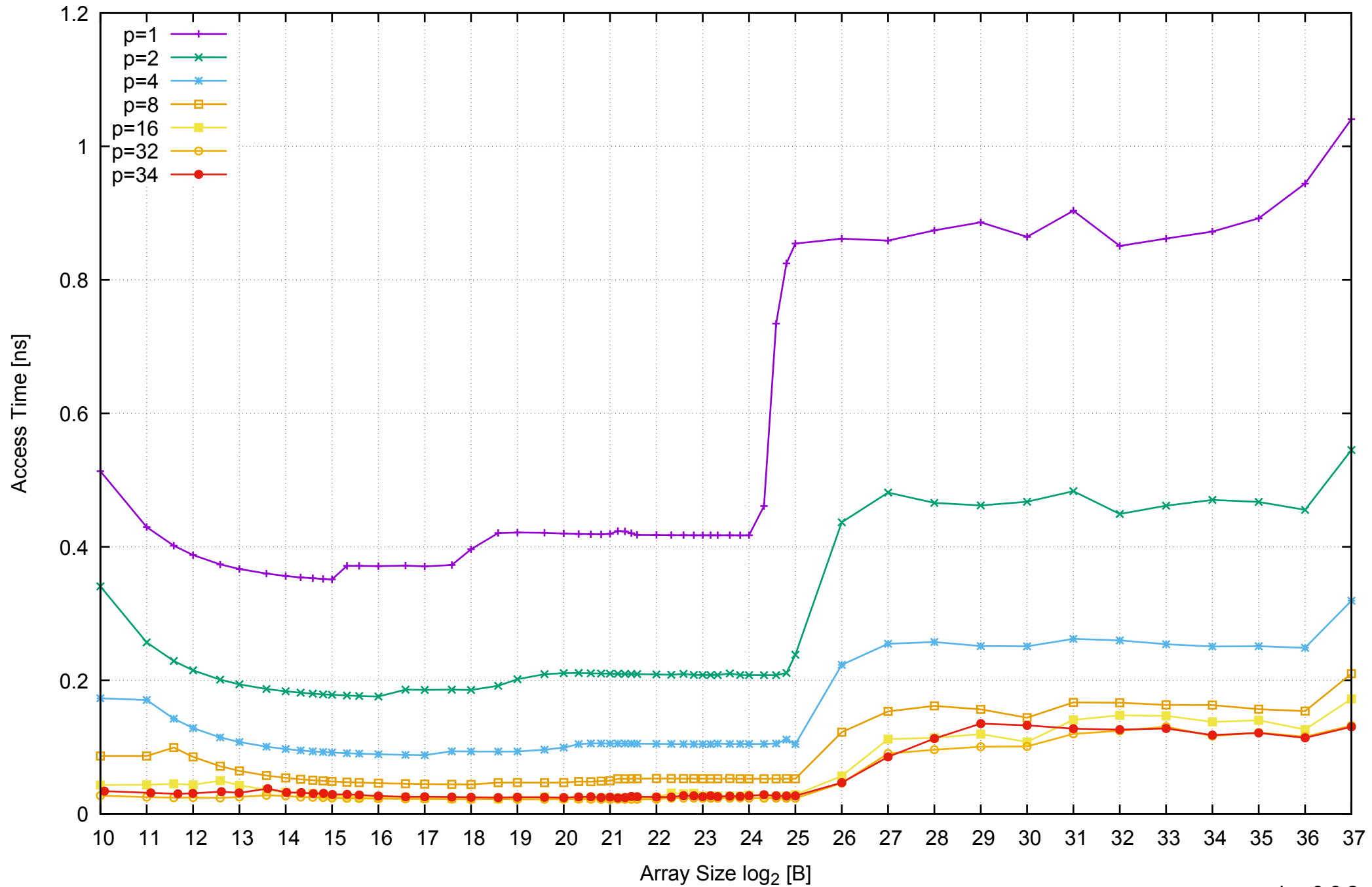
AWS r3.8xlarge - Intel Xeon E5-2676 v3, 2.50 GHz 244GB - Parallel Memory Access Time - ScanRead64PtrSimpleLoop
