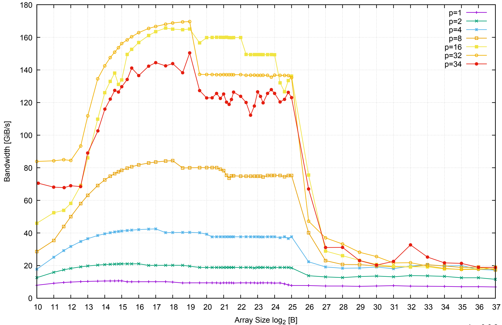
AWS r3.8xlarge - Intel Xeon E5-2676 v3, 2.50 GHz 244GB - Parallel Memory Bandwidth - ScanWrite32PtrSimpleLoop
