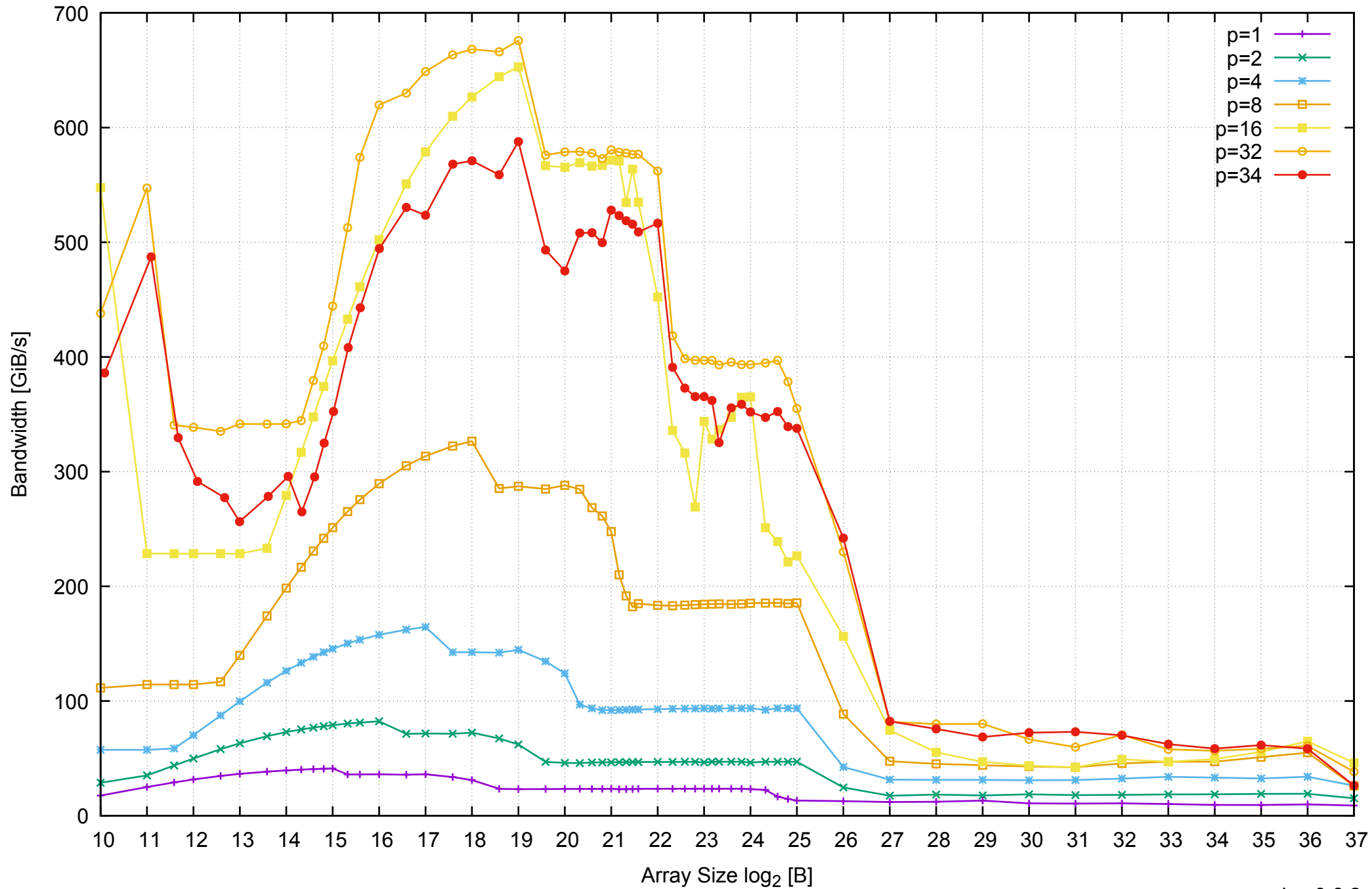
AWS r3.8xlarge - Intel Xeon E5-2676 v3, 2.50 GHz 244GB - Parallel Memory Bandwidth - ScanRead128PtrSimpleLoop
