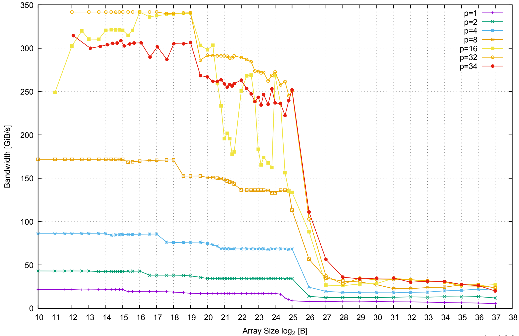
AWS r3.8xlarge - Intel Xeon E5-2676 v3, 2.50 GHz 244GB - Parallel Memory Bandwidth - ScanWrite64IndexUnrollLoop
