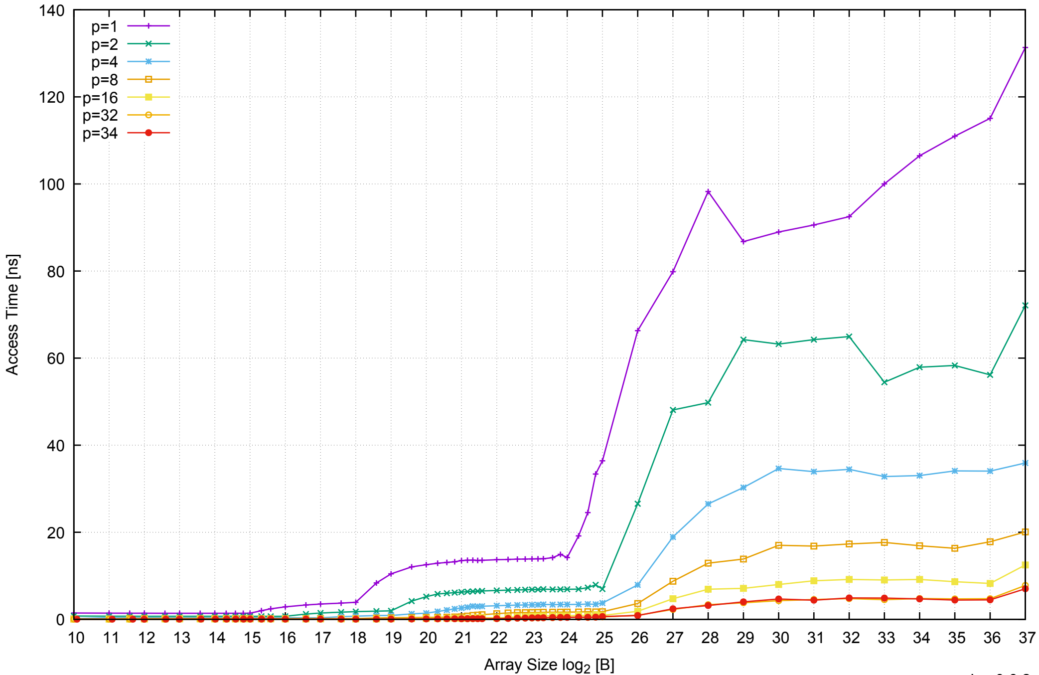
AWS r3.8xlarge - Intel Xeon E5-2676 v3, 2.50 GHz 244GB - Parallel Memory Access Time - PermRead64SimpleLoop
