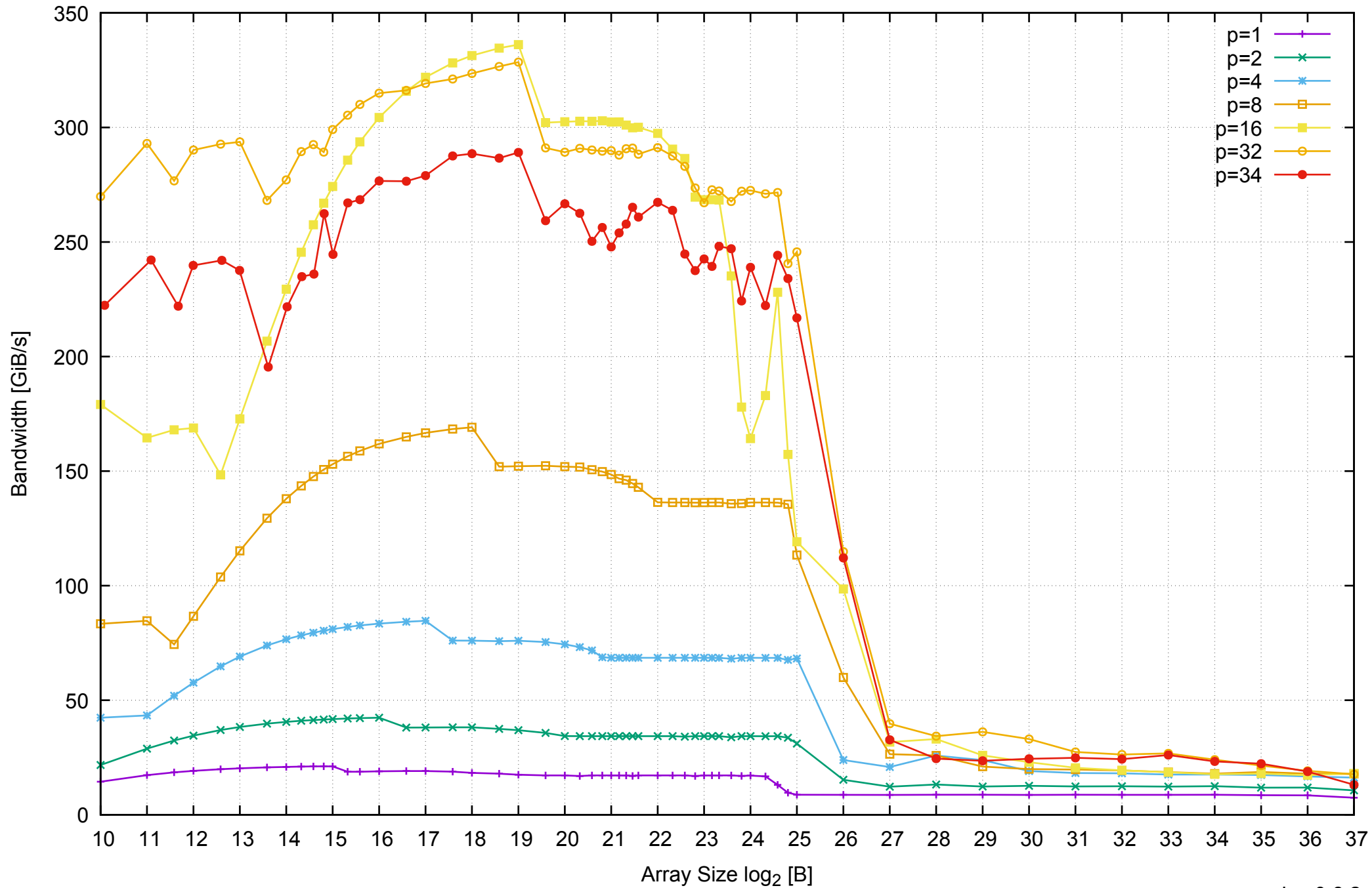
AWS r3.8xlarge - Intel Xeon E5-2676 v3, 2.50 GHz 244GB - Parallel Memory Bandwidth - ScanWrite64PtrSimpleLoop
