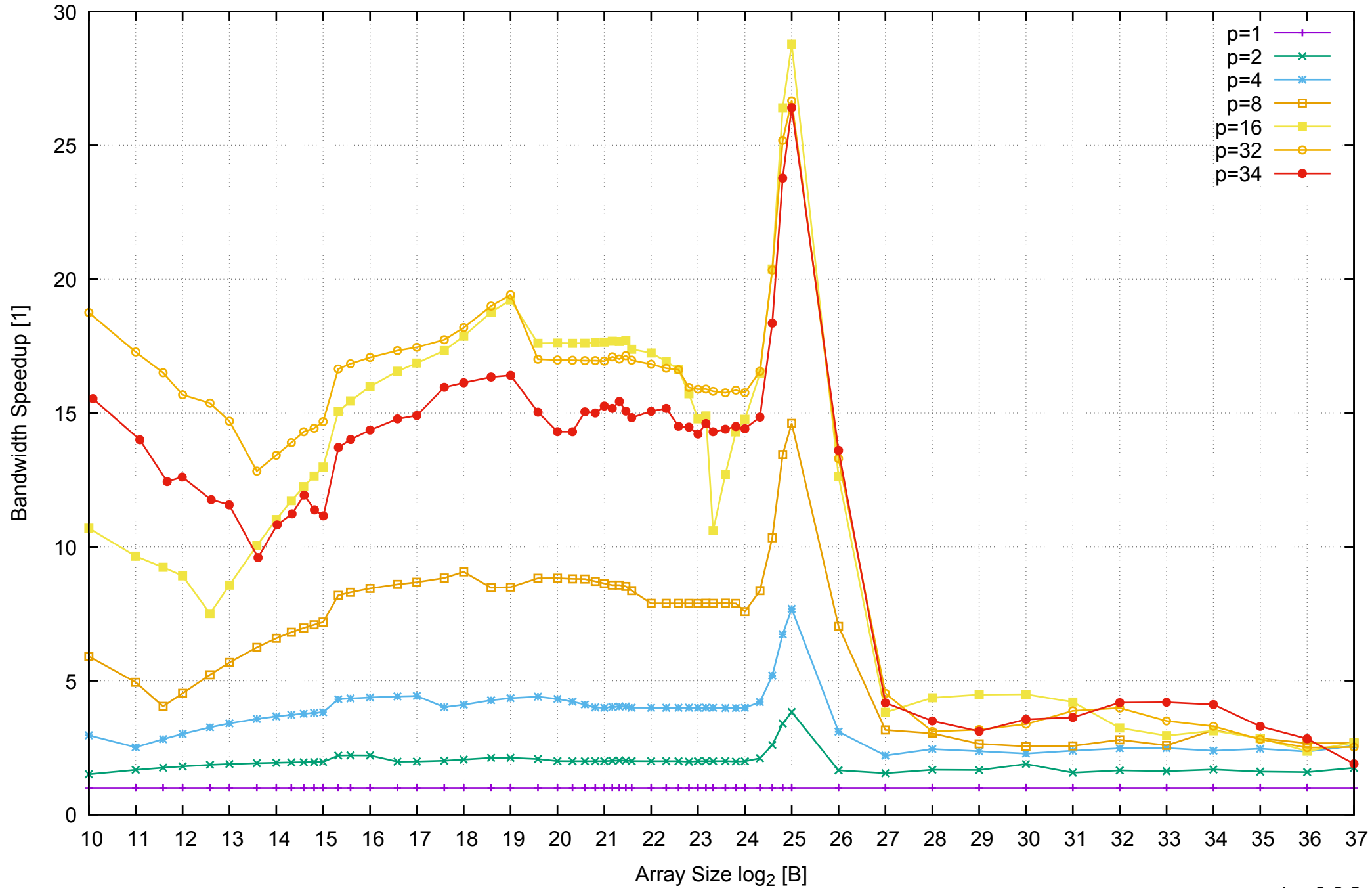
AWS r3.8xlarge - Intel Xeon E5-2676 v3, 2.50 GHz 244GB - Speedup of Parallel Memory Bandwidth - ScanWrite64IndexSimpleLoop
