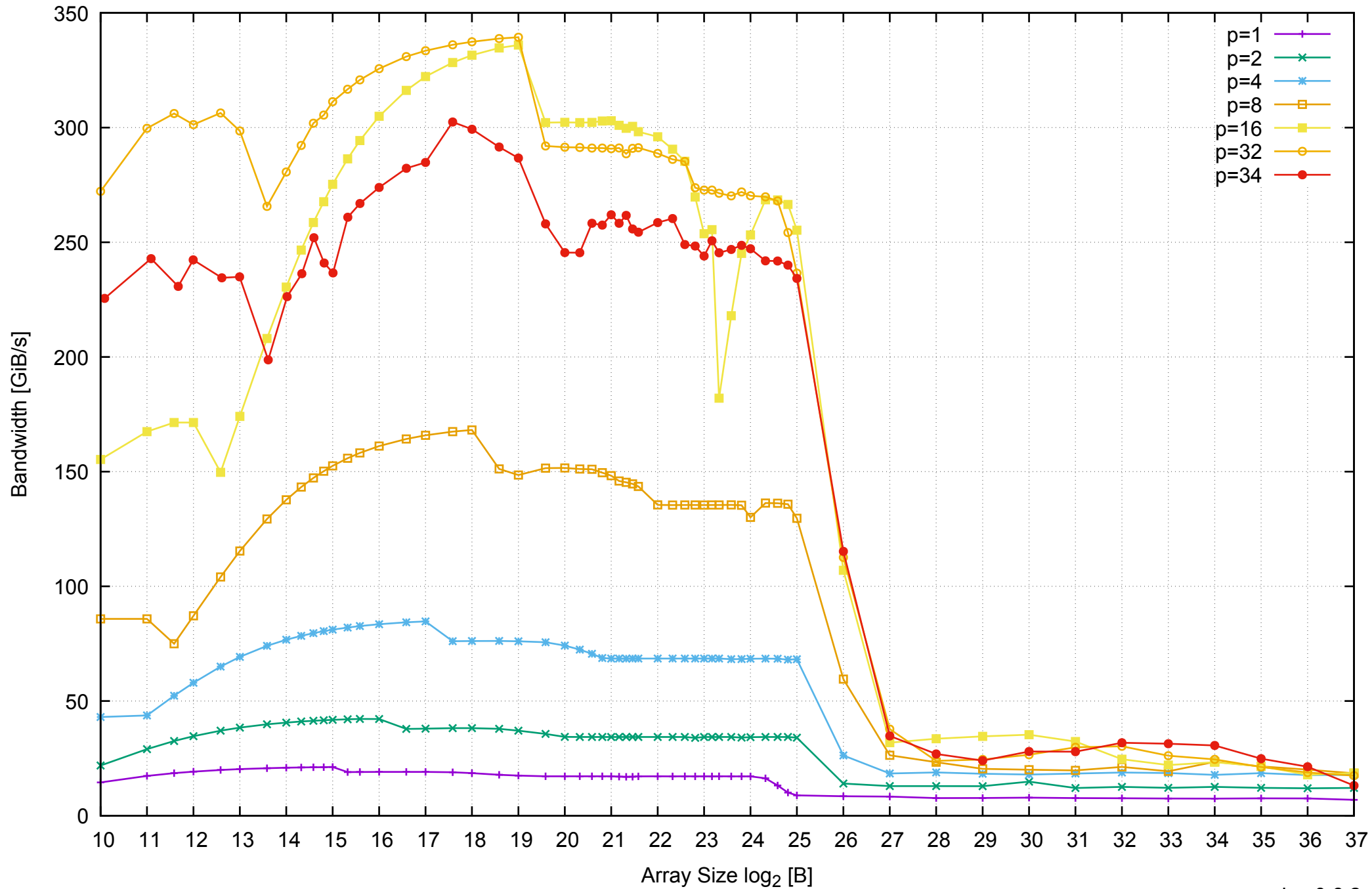
AWS r3.8xlarge - Intel Xeon E5-2676 v3, 2.50 GHz 244GB - Parallel Memory Bandwidth - ScanWrite64IndexSimpleLoop
