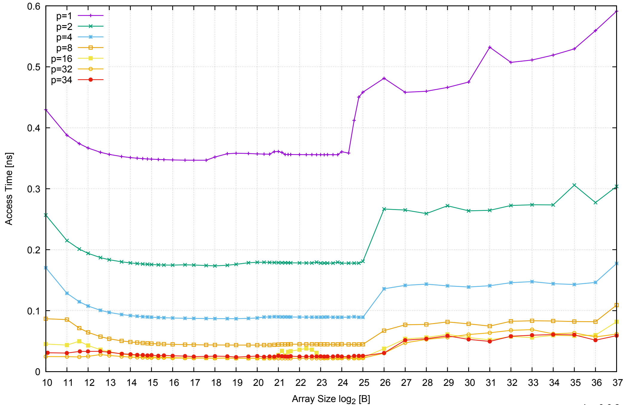
AWS r3.8xlarge - Intel Xeon E5-2676 v3, 2.50 GHz 244GB - Parallel Memory Access Time - ScanRead32PtrSimpleLoop
