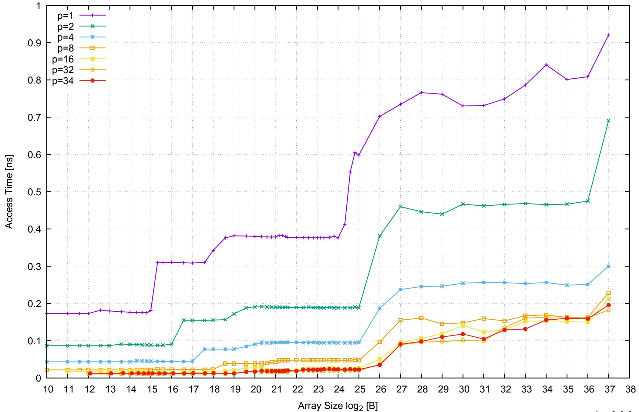
AWS r3.8xlarge - Intel Xeon E5-2676 v3, 2.50 GHz 244GB - Parallel Memory Access Time - ScanRead64IndexUnrollLoop
