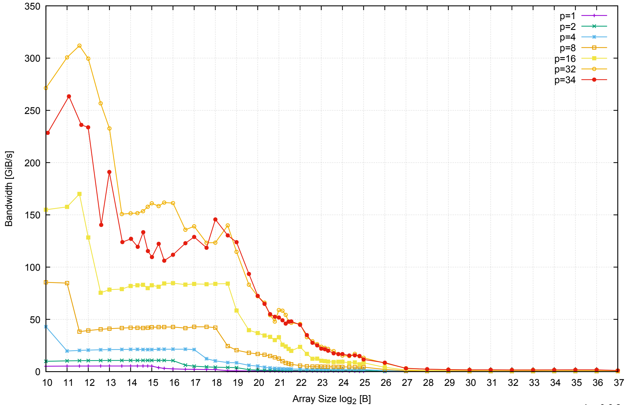
AWS r3.8xlarge - Intel Xeon E5-2676 v3, 2.50 GHz 244GB - Parallel Memory Bandwidth - PermRead64SimpleLoop
