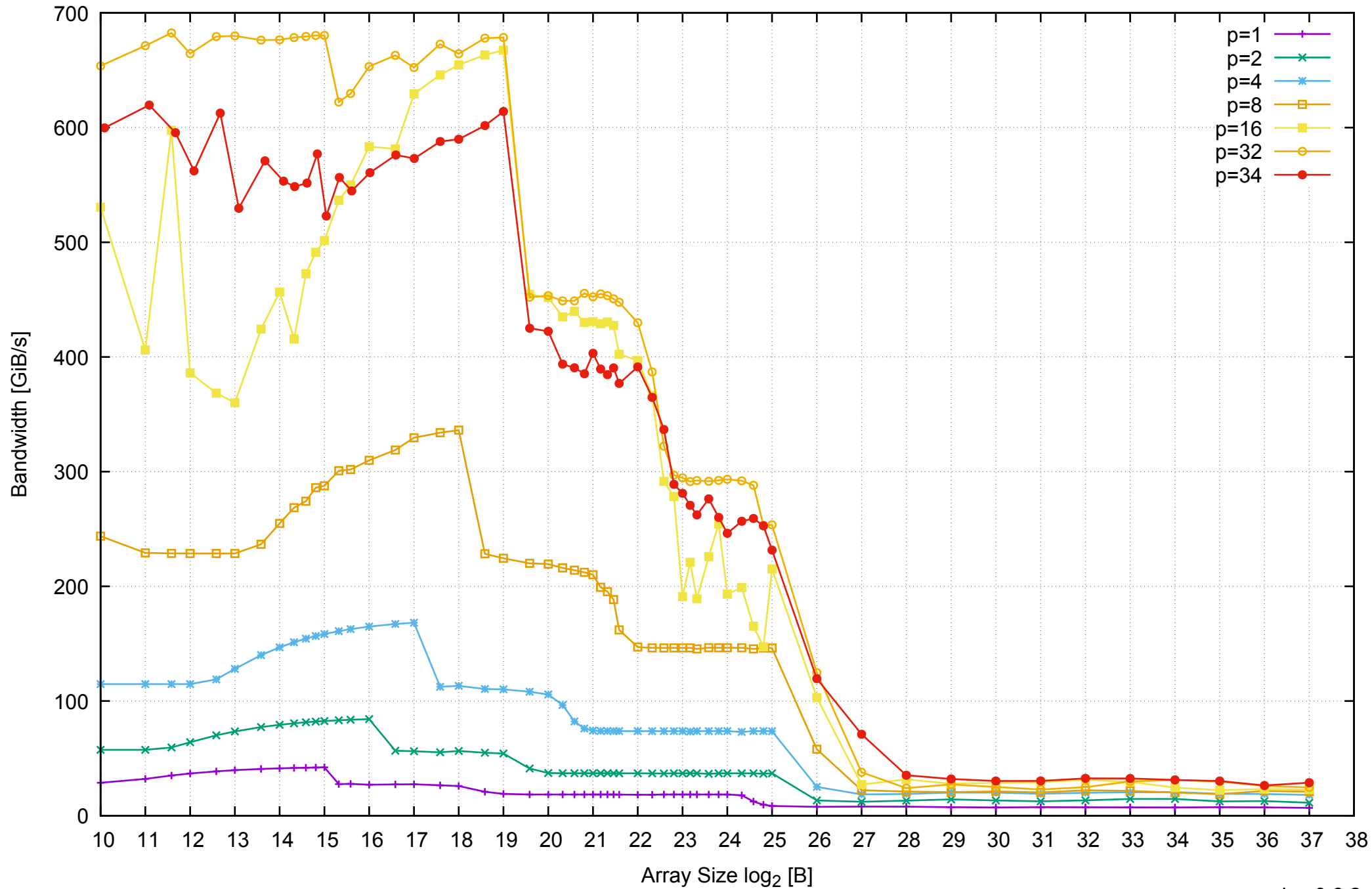
AWS r3.8xlarge - Intel Xeon E5-2676 v3, 2.50 GHz 244GB - Parallel Memory Bandwidth - ScanWrite256PtrSimpleLoop
