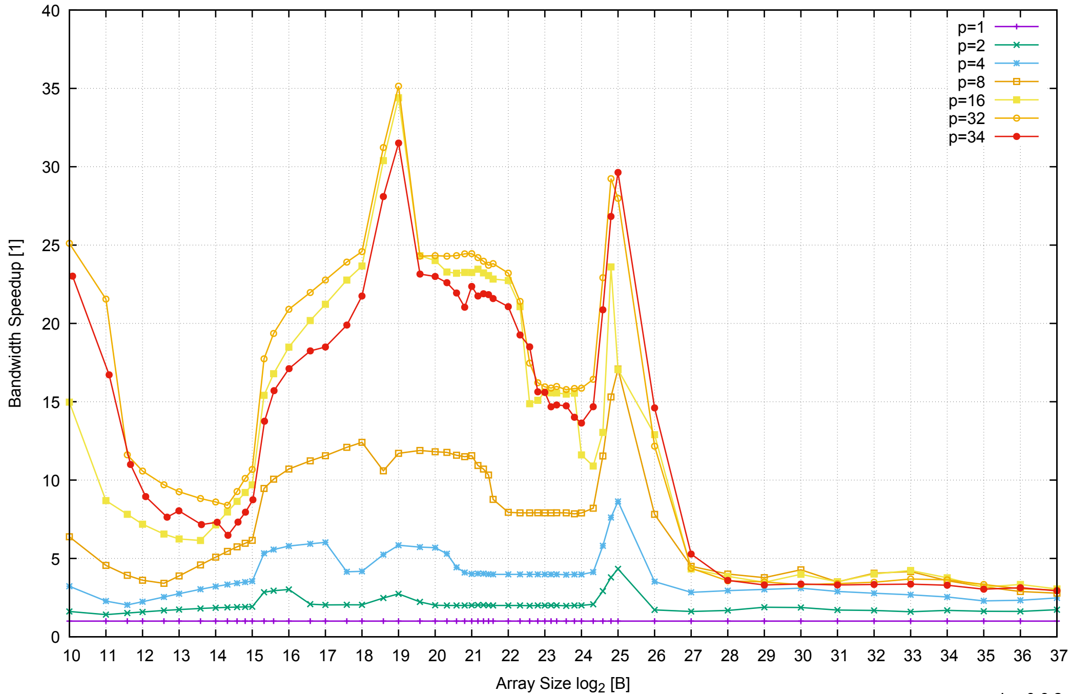
AWS r3.8xlarge - Intel Xeon E5-2676 v3, 2.50 GHz 244GB - Speedup of Parallel Memory Bandwidth - ScanWrite128PtrSimpleLoop
