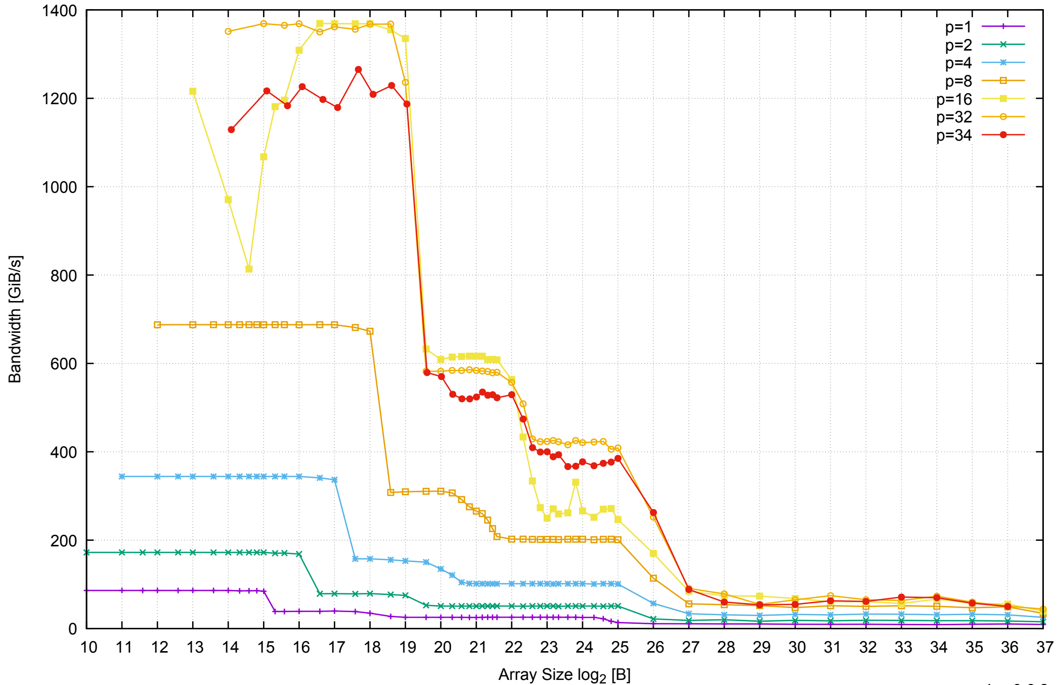
AWS r3.8xlarge - Intel Xeon E5-2676 v3, 2.50 GHz 244GB - Parallel Memory Bandwidth - ScanRead256PtrUnrollLoop
