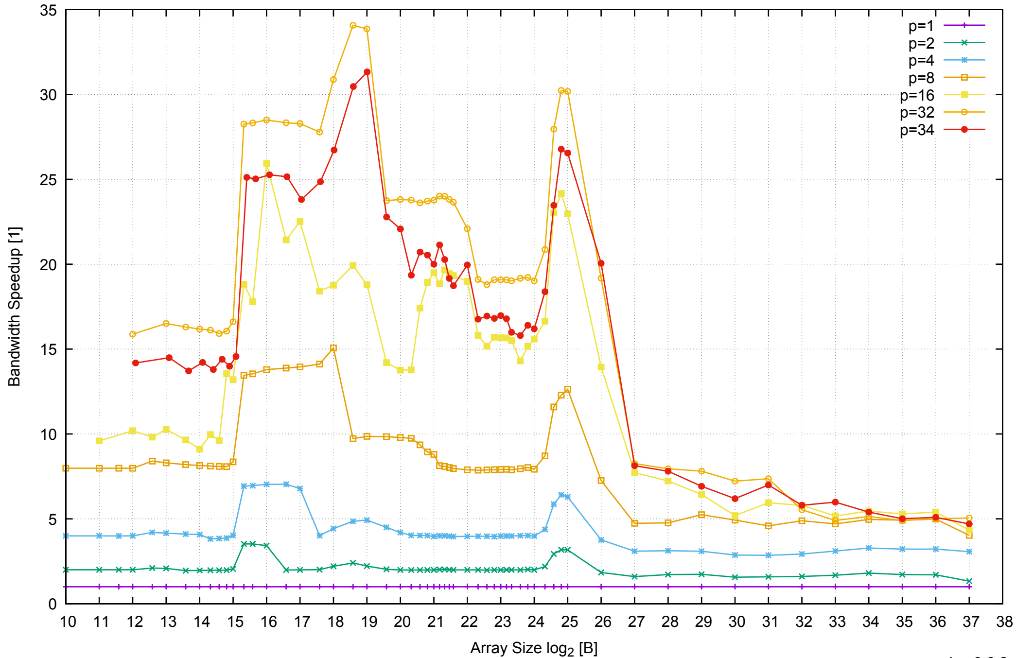
AWS r3.8xlarge - Intel Xeon E5-2676 v3, 2.50 GHz 244GB - Speedup of Parallel Memory Bandwidth - ScanRead64IndexUnrollLoop
