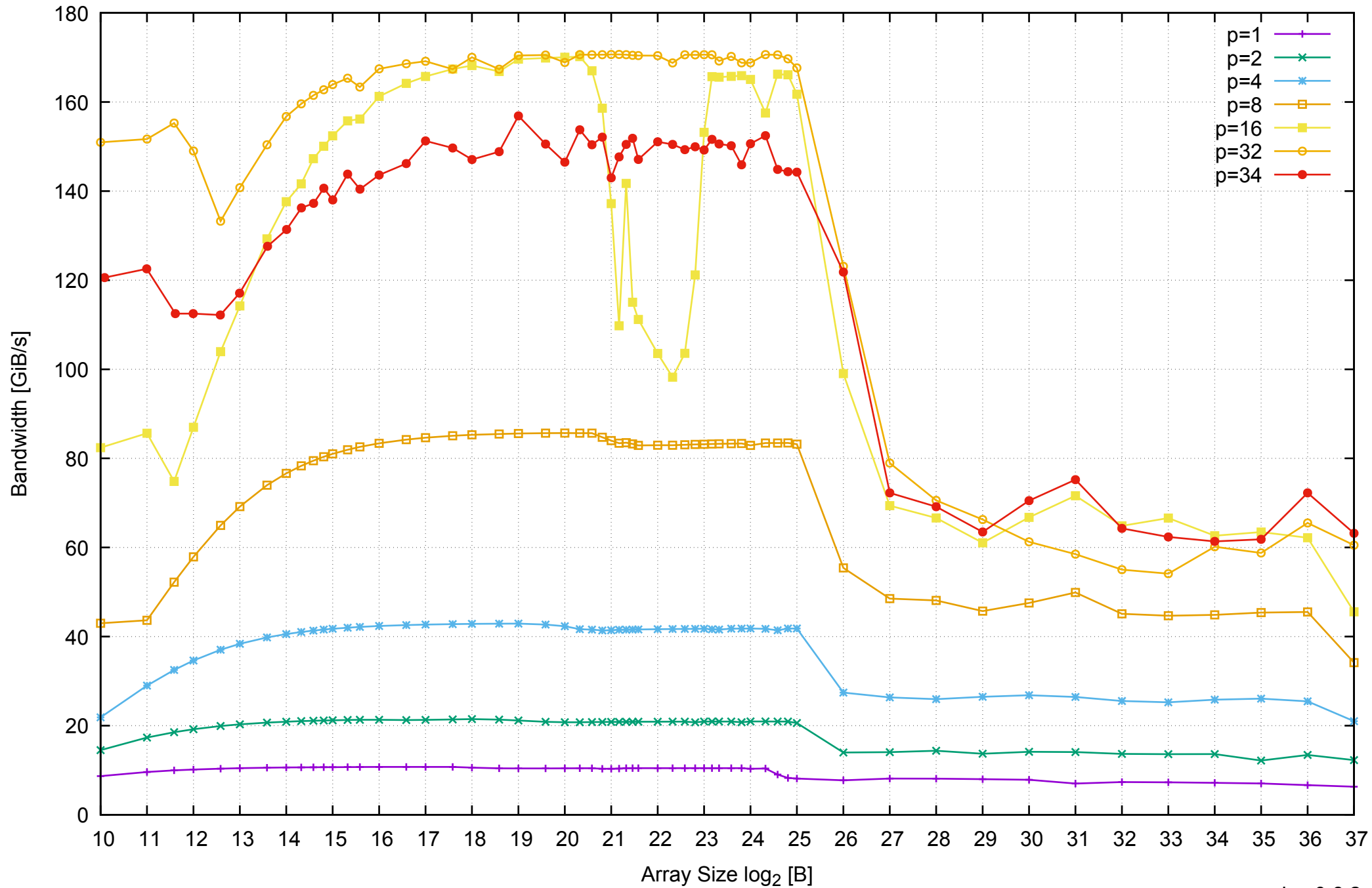
AWS r3.8xlarge - Intel Xeon E5-2676 v3, 2.50 GHz 244GB - Parallel Memory Bandwidth - ScanRead32PtrSimpleLoop
