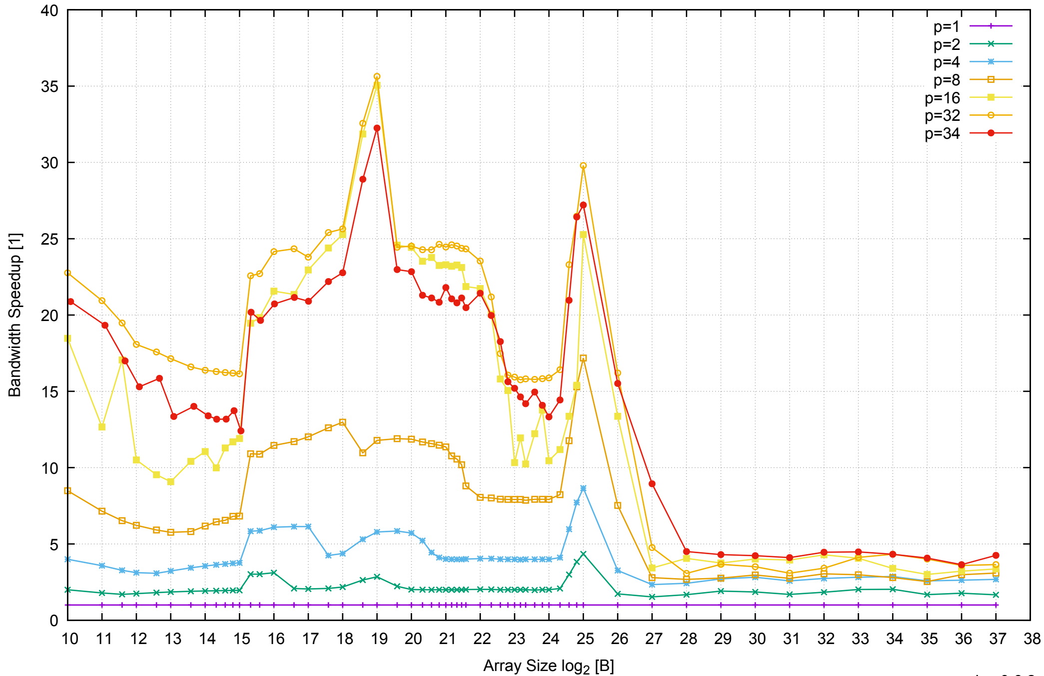
AWS r3.8xlarge - Intel Xeon E5-2676 v3, 2.50 GHz 244GB - Speedup of Parallel Memory Bandwidth - ScanWrite256PtrSimpleLoop
