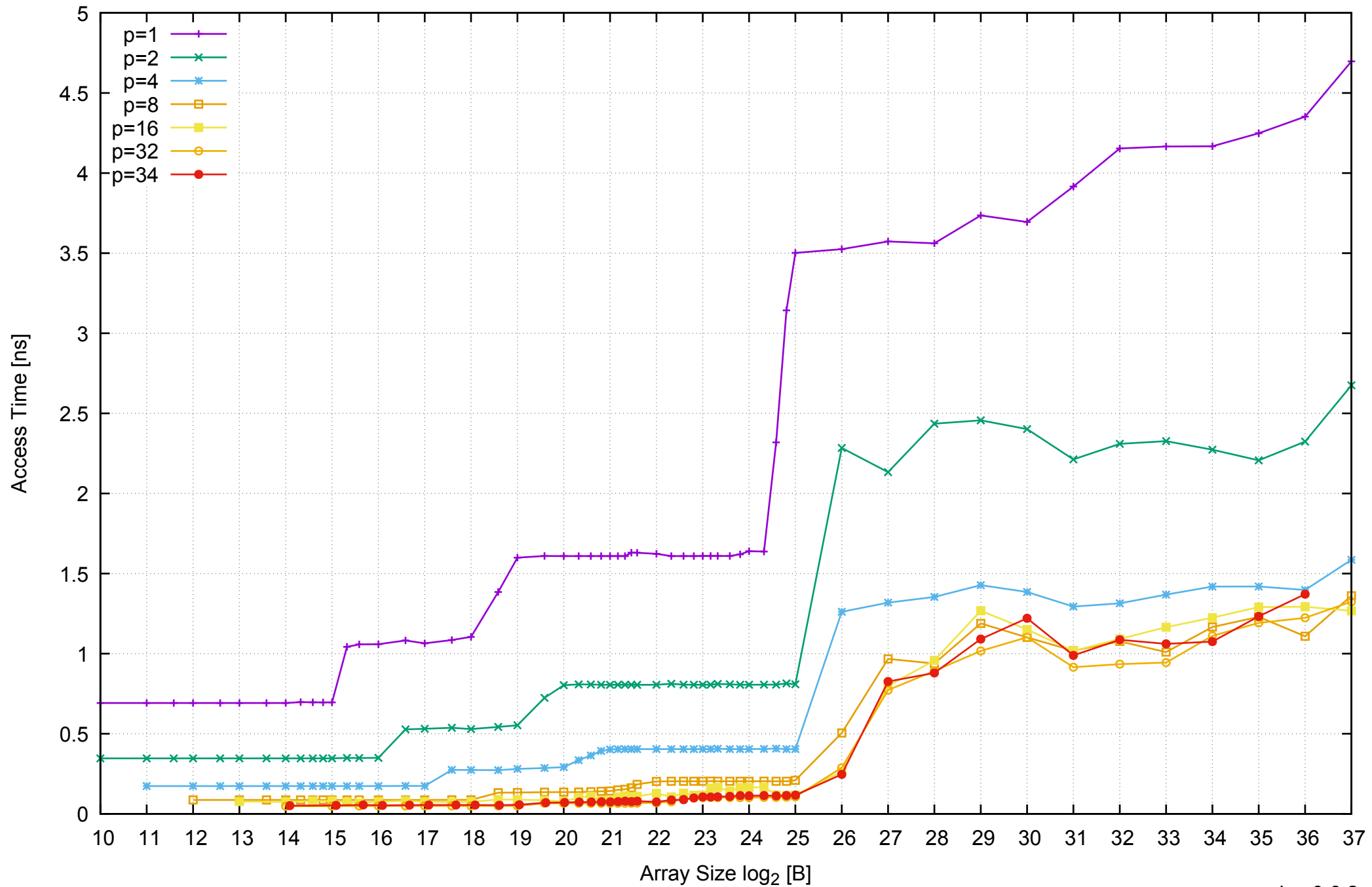
AWS r3.8xlarge - Intel Xeon E5-2676 v3, 2.50 GHz 244GB - Parallel Memory Access Time - ScanWrite256PtrUnrollLoop
