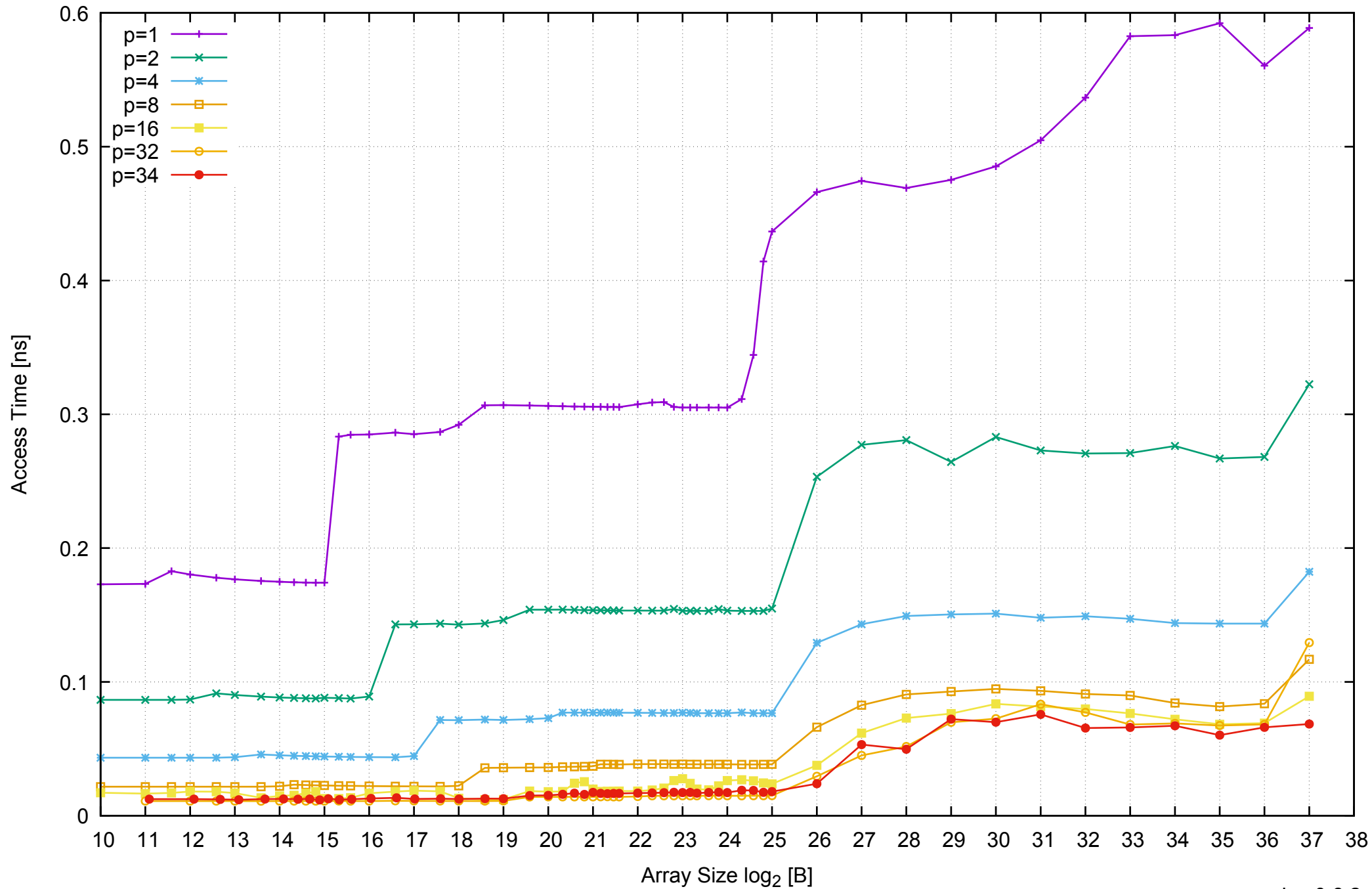
AWS r3.8xlarge - Intel Xeon E5-2676 v3, 2.50 GHz 244GB - Parallel Memory Access Time - ScanRead32PtrUnrollLoop
