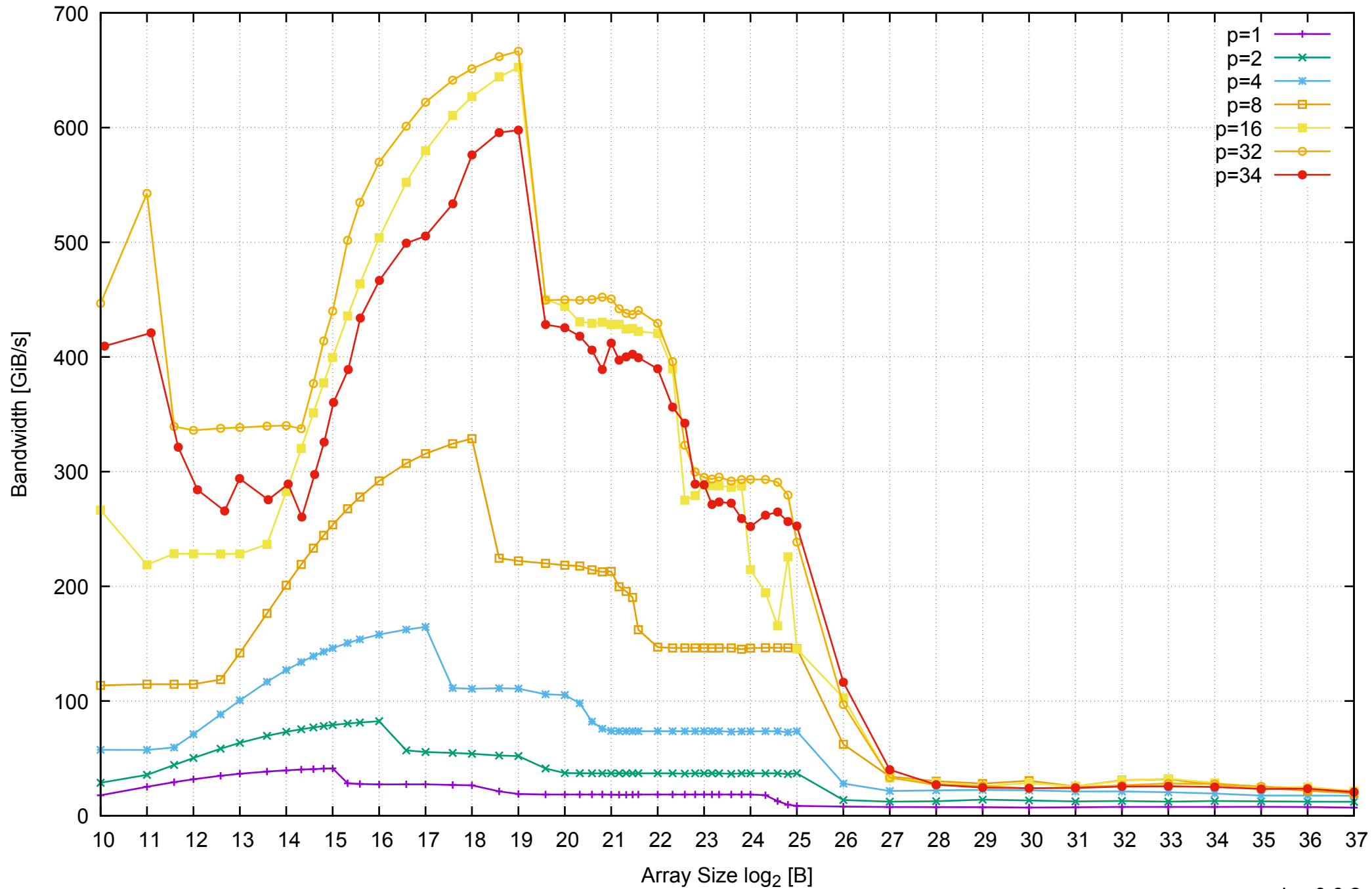
AWS r3.8xlarge - Intel Xeon E5-2676 v3, 2.50 GHz 244GB - Parallel Memory Bandwidth - ScanWrite128PtrSimpleLoop
