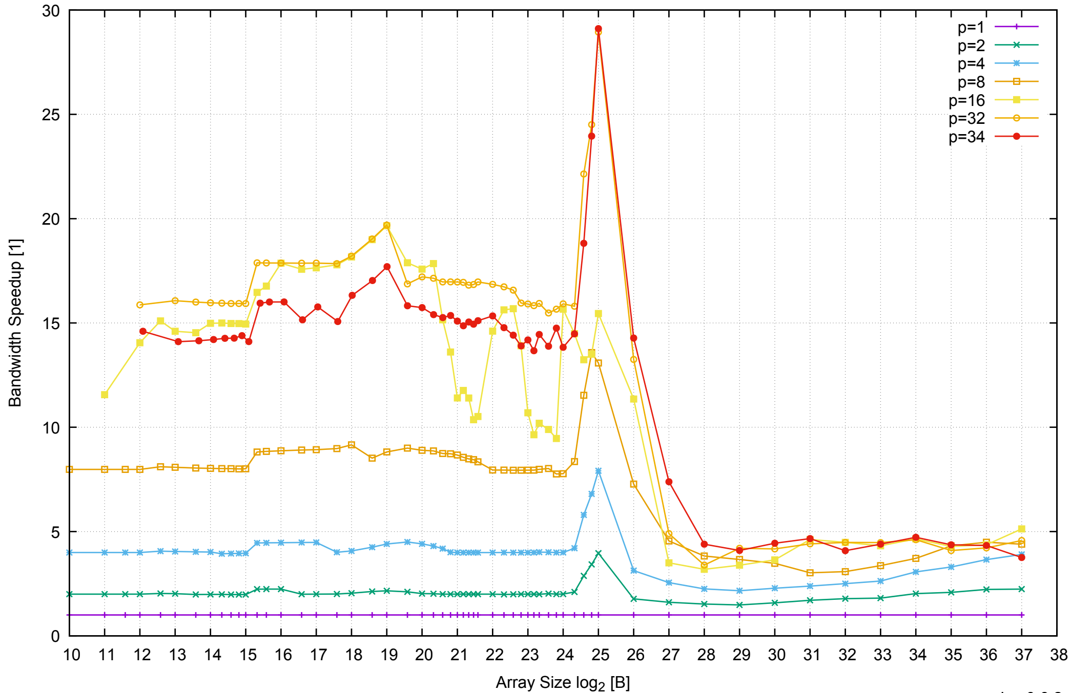
AWS r3.8xlarge - Intel Xeon E5-2676 v3, 2.50 GHz 244GB - Speedup of Parallel Memory Bandwidth - ScanWrite64IndexUnrollLoop
