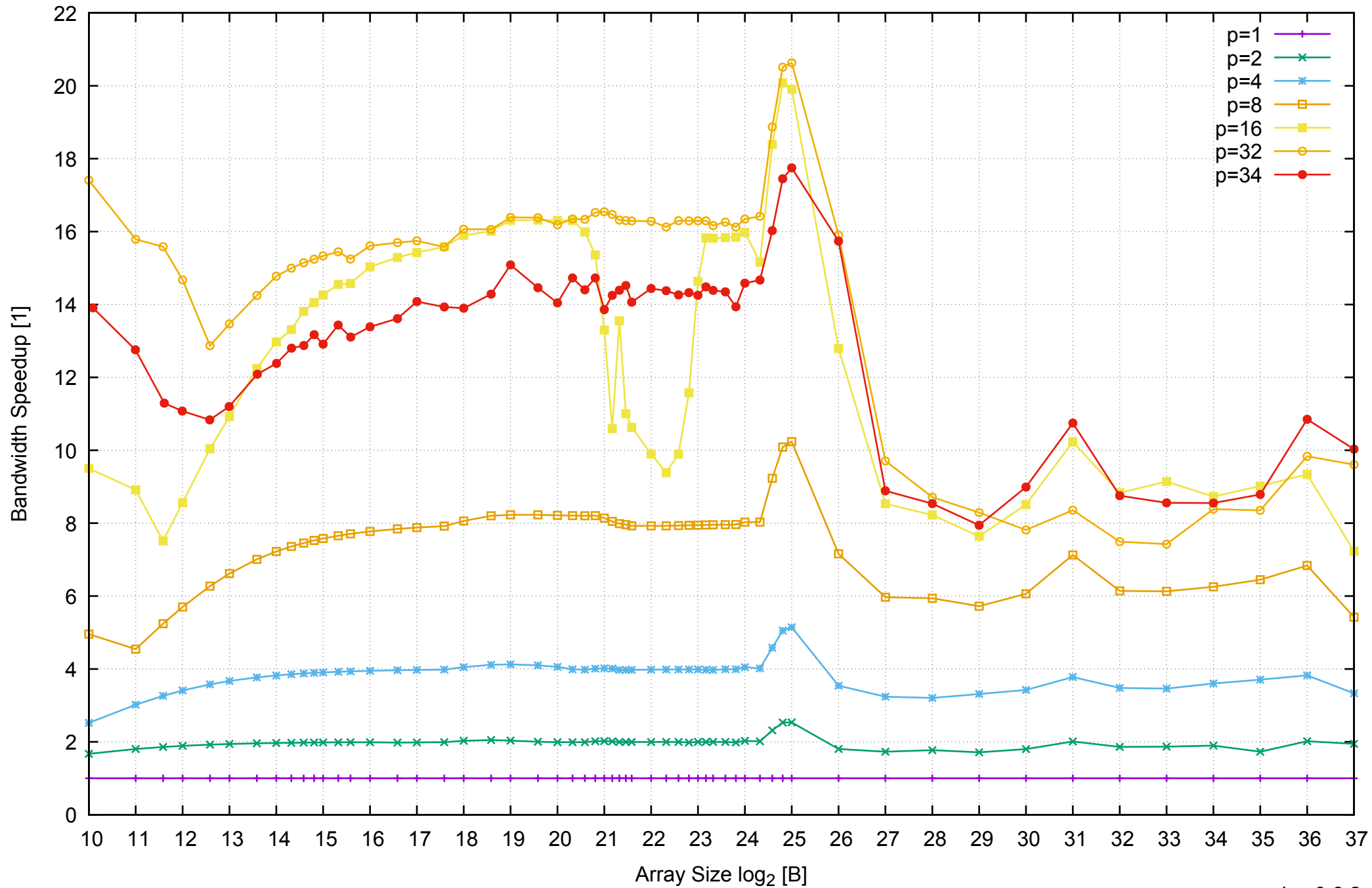
AWS r3.8xlarge - Intel Xeon E5-2676 v3, 2.50 GHz 244GB - Speedup of Parallel Memory Bandwidth - ScanRead32PtrSimpleLoop
