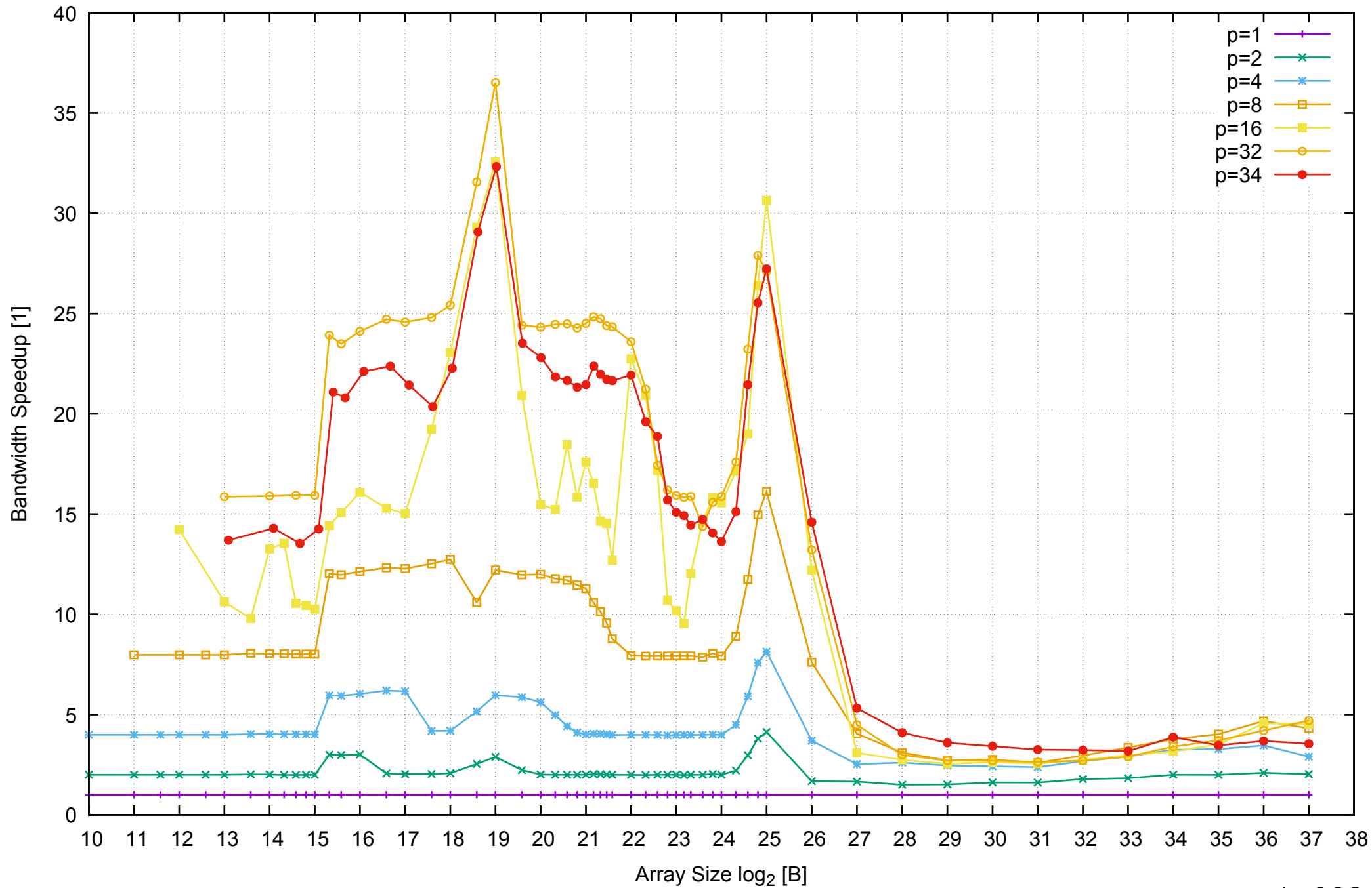
AWS r3.8xlarge - Intel Xeon E5-2676 v3, 2.50 GHz 244GB - Speedup of Parallel Memory Bandwidth - ScanWrite128PtrUnrollLoop
