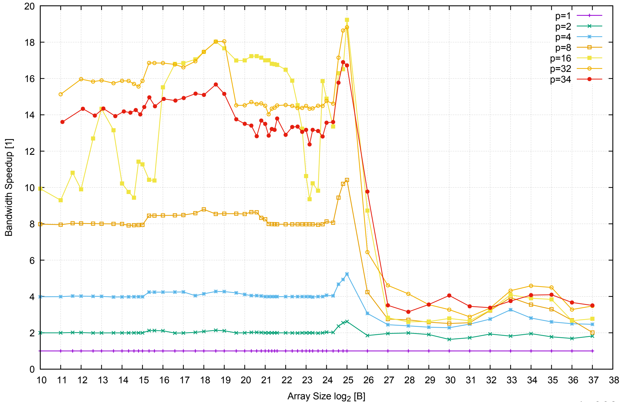
AWS r3.8xlarge - Intel Xeon E5-2676 v3, 2.50 GHz 244GB - Speedup of Parallel Memory Bandwidth - ScanWrite32PtrUnrollLoop
