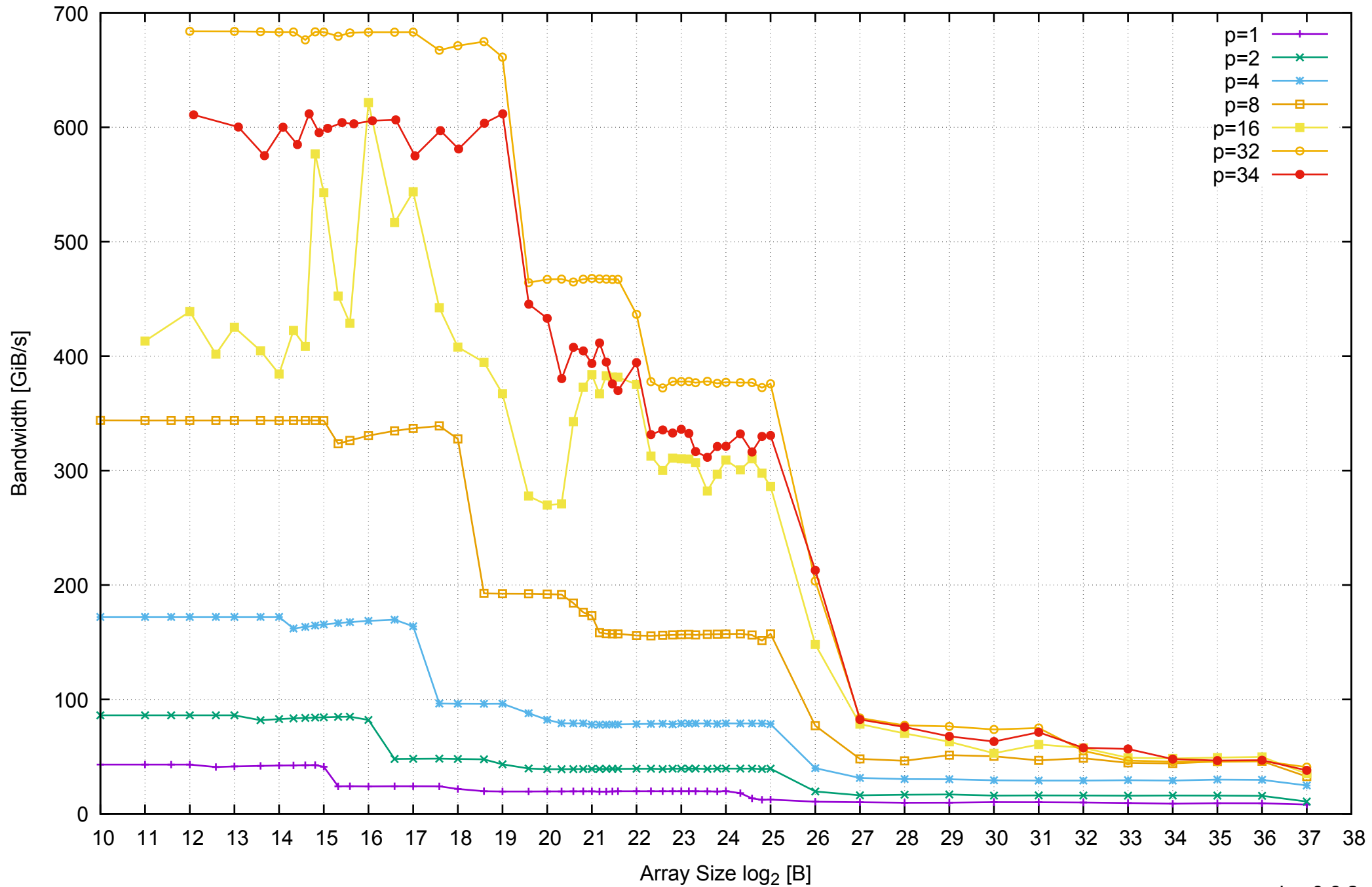
AWS r3.8xlarge - Intel Xeon E5-2676 v3, 2.50 GHz 244GB - Parallel Memory Bandwidth - ScanRead64IndexUnrollLoop
