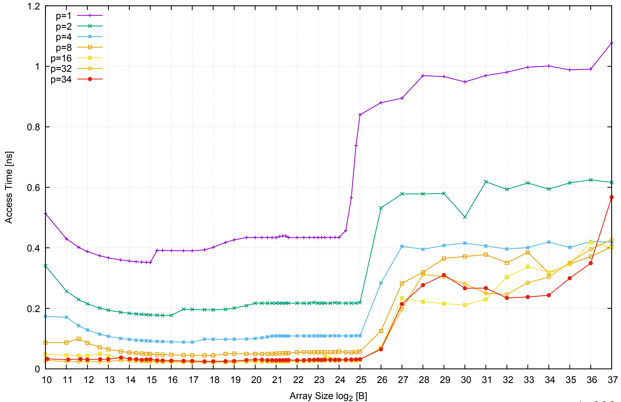
AWS r3.8xlarge - Intel Xeon E5-2676 v3, 2.50 GHz 244GB - Parallel Memory Access Time - ScanWrite64IndexSimpleLoop
