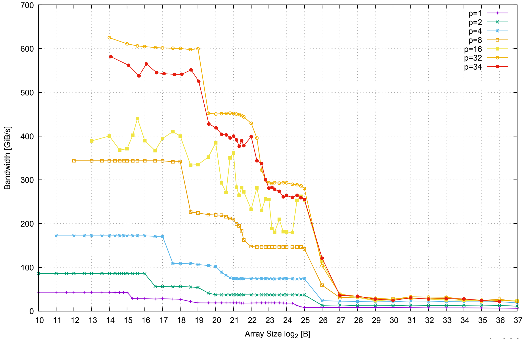
AWS r3.8xlarge - Intel Xeon E5-2676 v3, 2.50 GHz 244GB - Parallel Memory Bandwidth - ScanWrite256PtrUnrollLoop
