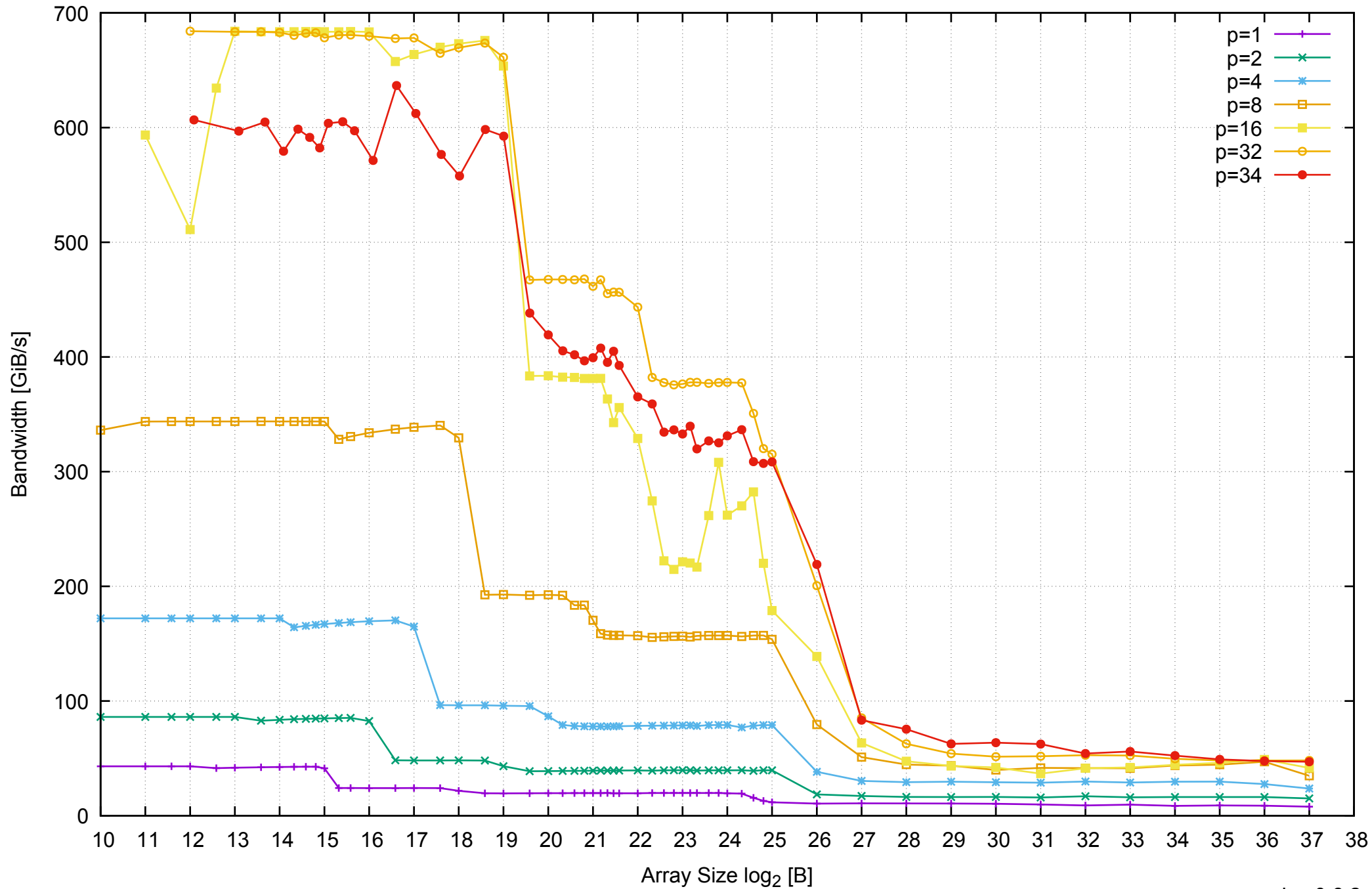
AWS r3.8xlarge - Intel Xeon E5-2676 v3, 2.50 GHz 244GB - Parallel Memory Bandwidth - ScanRead64PtrUnrollLoop
