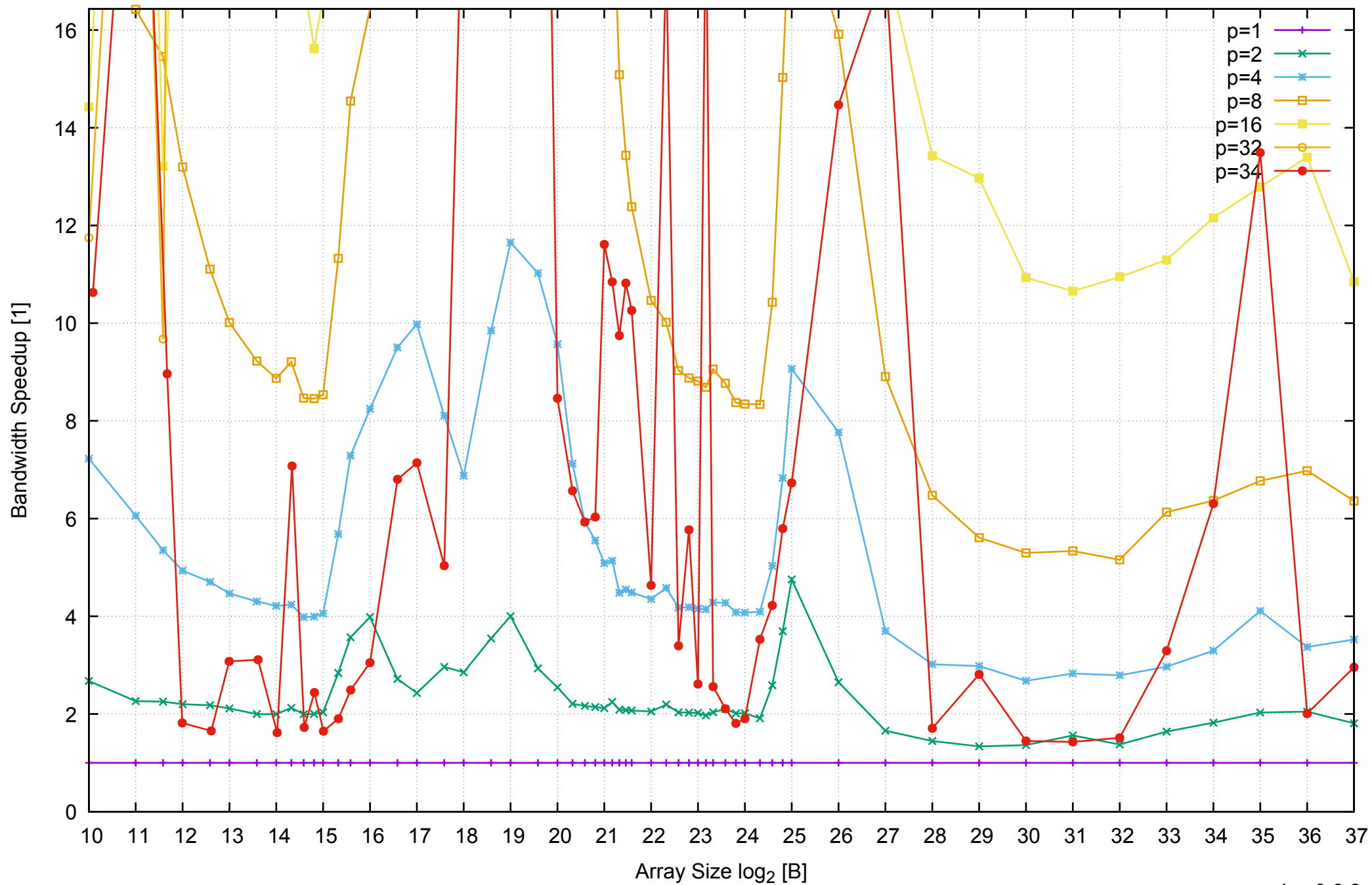
AWS r3.8xlarge - Intel Xeon E5-2676 v3, 2.50 GHz 244GB - Speedup of Parallel Memory Bandwidth (enlarged) - PermRead64UnrollLoop
