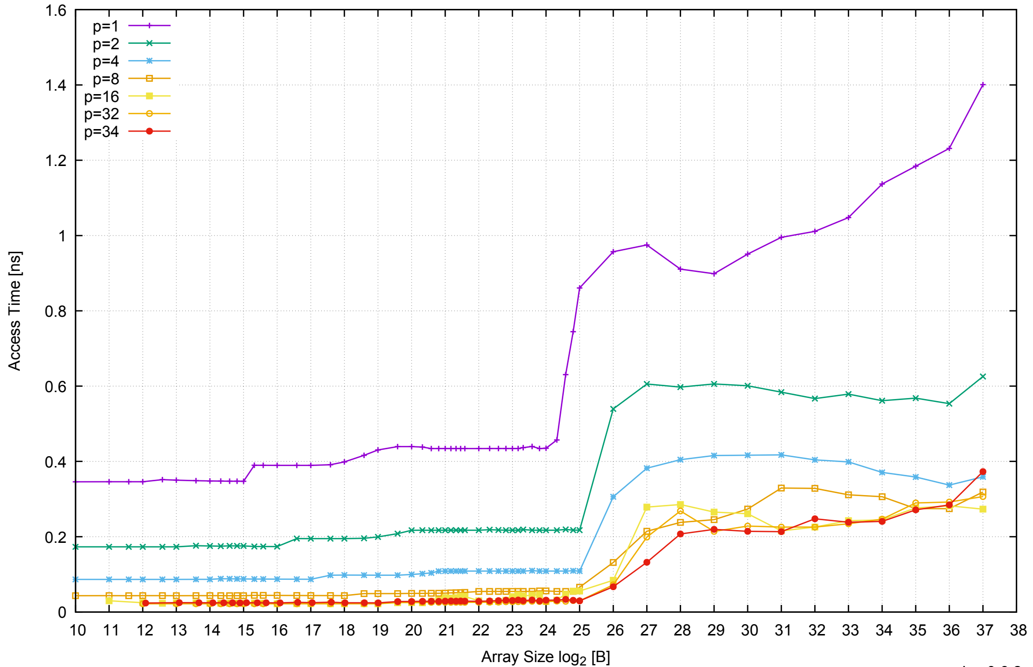
AWS r3.8xlarge - Intel Xeon E5-2676 v3, 2.50 GHz 244GB - Parallel Memory Access Time - ScanWrite64IndexUnrollLoop
