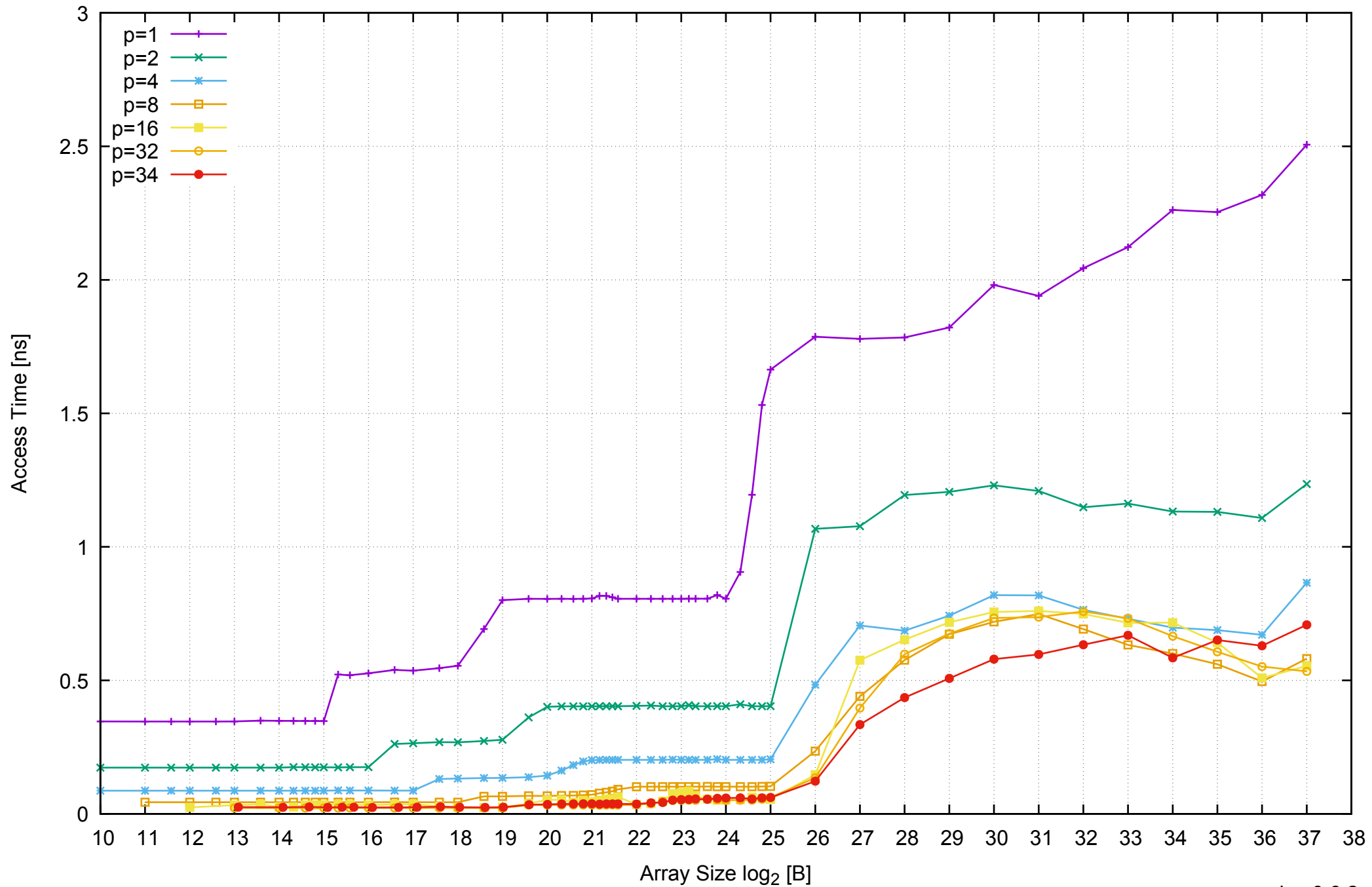
AWS r3.8xlarge - Intel Xeon E5-2676 v3, 2.50 GHz 244GB - Parallel Memory Access Time - ScanWrite128PtrUnrollLoop
