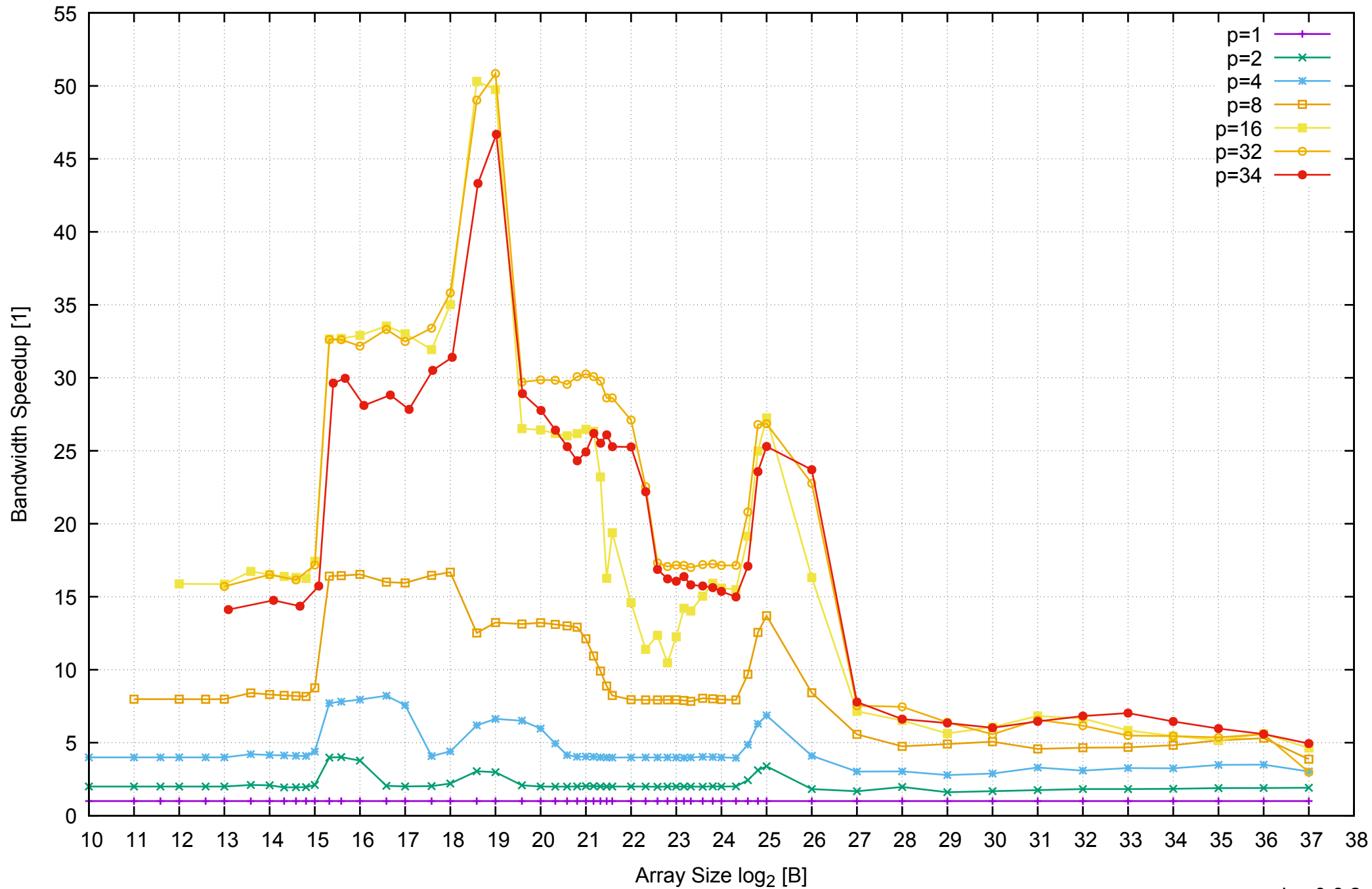
AWS r3.8xlarge - Intel Xeon E5-2676 v3, 2.50 GHz 244GB - Speedup of Parallel Memory Bandwidth - ScanRead128PtrUnrollLoop
