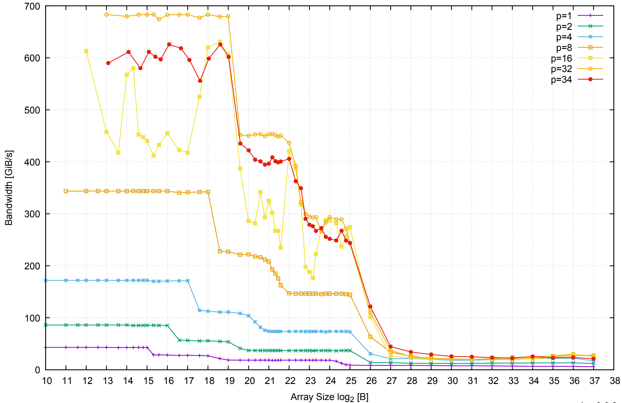
AWS r3.8xlarge - Intel Xeon E5-2676 v3, 2.50 GHz 244GB - Parallel Memory Bandwidth - ScanWrite128PtrUnrollLoop
