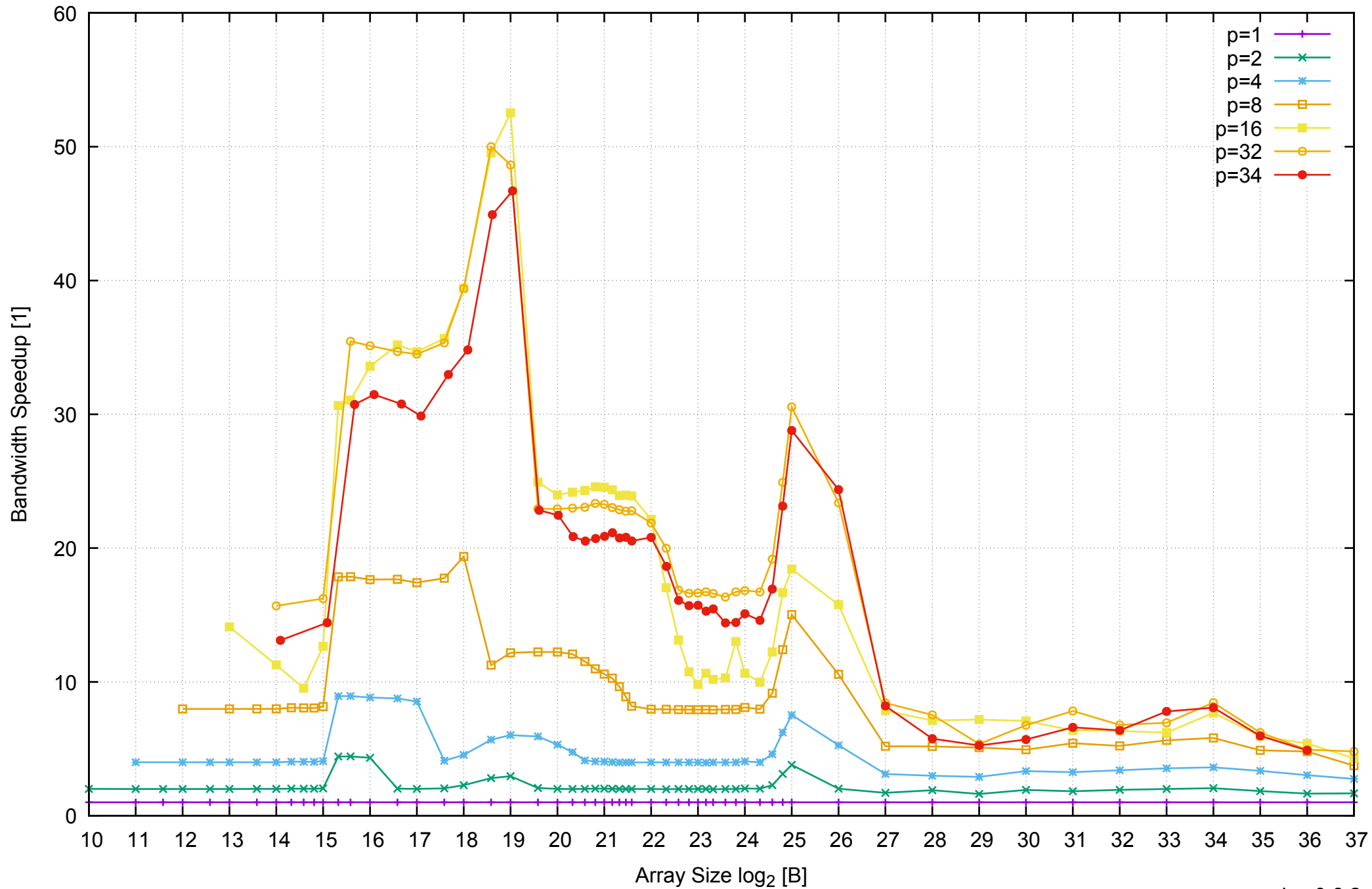
AWS r3.8xlarge - Intel Xeon E5-2676 v3, 2.50 GHz 244GB - Speedup of Parallel Memory Bandwidth - ScanRead256PtrUnrollLoop
