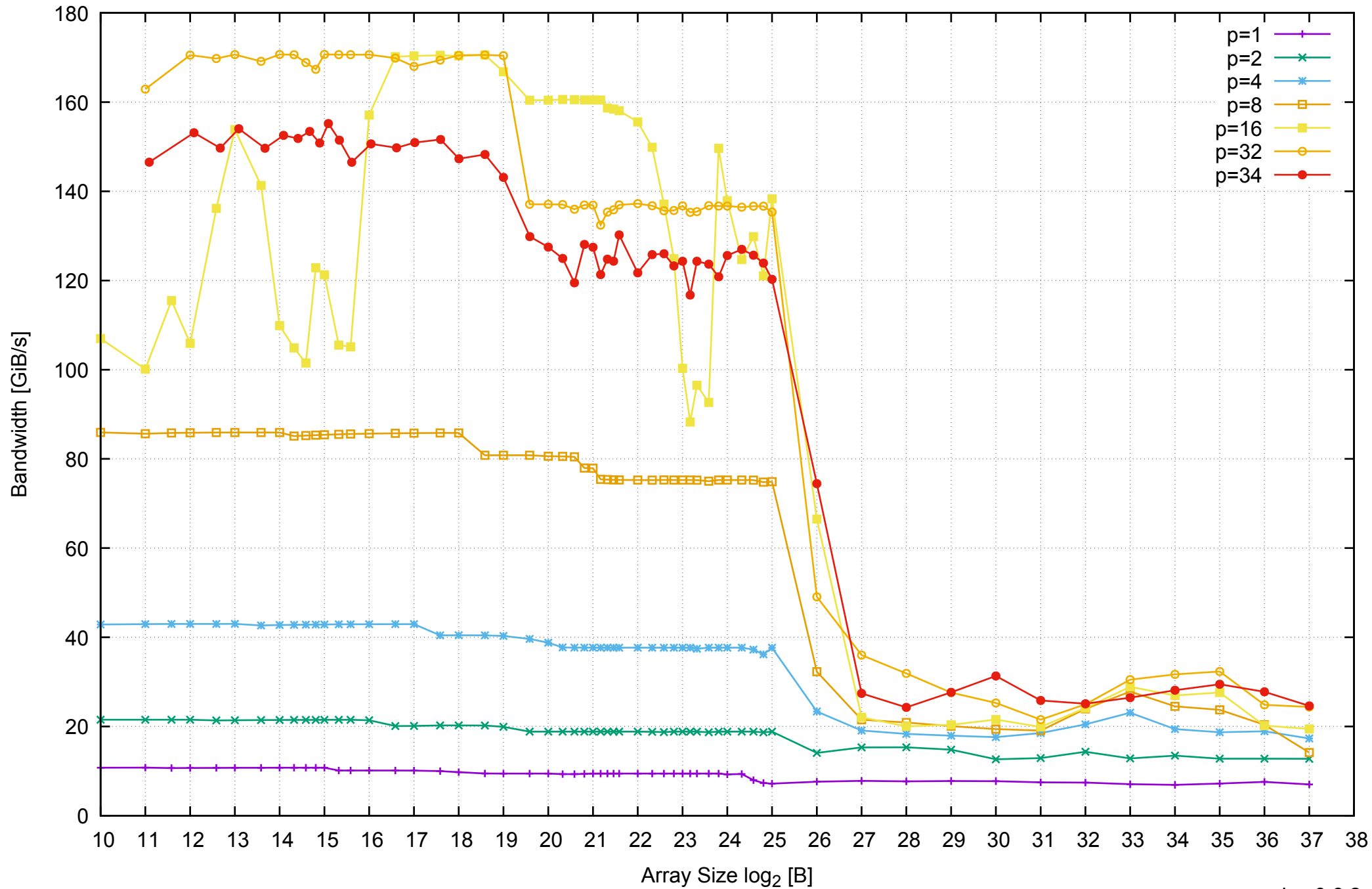
AWS r3.8xlarge - Intel Xeon E5-2676 v3, 2.50 GHz 244GB - Parallel Memory Bandwidth - ScanWrite32PtrUnrollLoop
