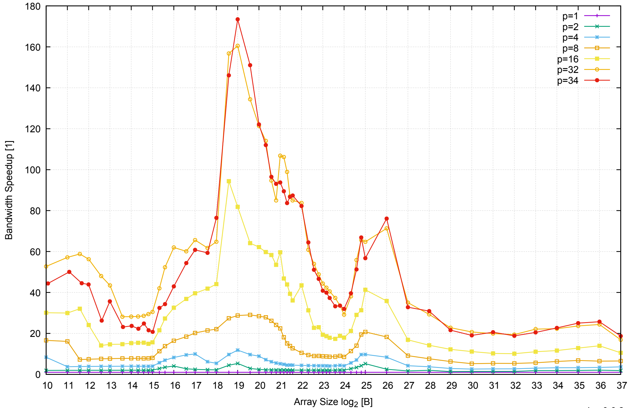
AWS r3.8xlarge - Intel Xeon E5-2676 v3, 2.50 GHz 244GB - Speedup of Parallel Memory Bandwidth - PermRead64SimpleLoop
