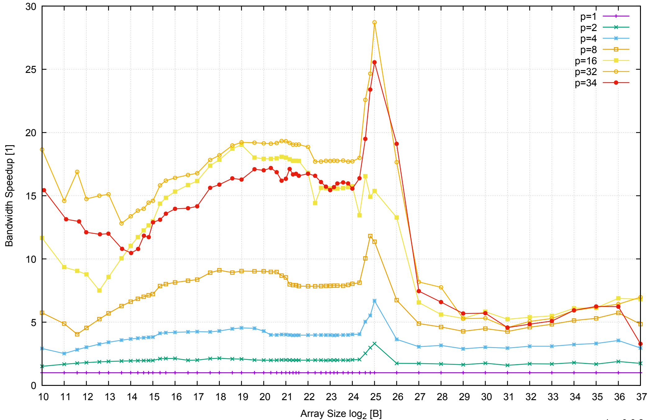
AWS r3.8xlarge - Intel Xeon E5-2676 v3, 2.50 GHz 244GB - Speedup of Parallel Memory Bandwidth - ScanRead64IndexSimpleLoop
