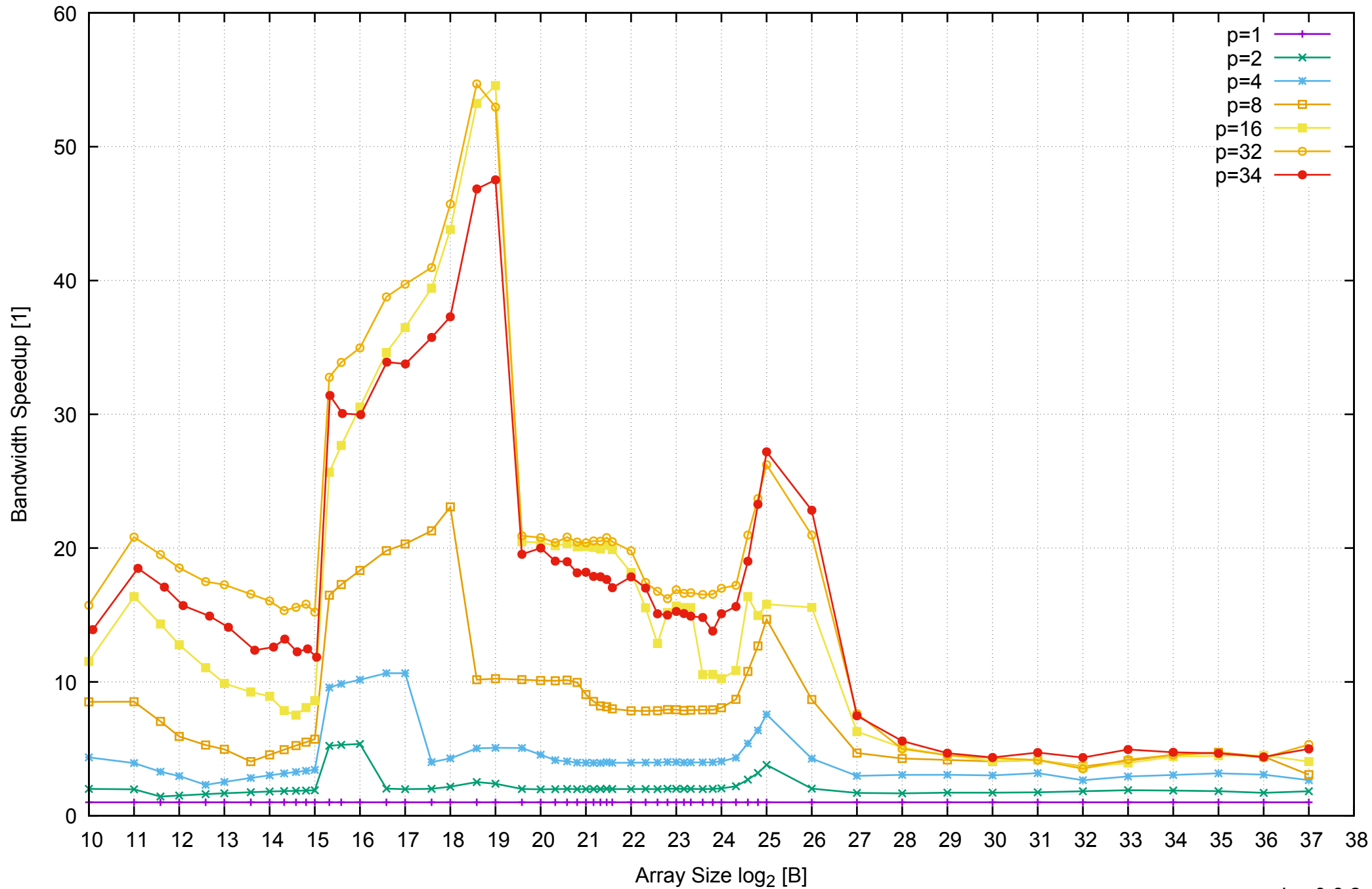
AWS r3.8xlarge - Intel Xeon E5-2676 v3, 2.50 GHz 244GB - Speedup of Parallel Memory Bandwidth - ScanRead256PtrSimpleLoop
