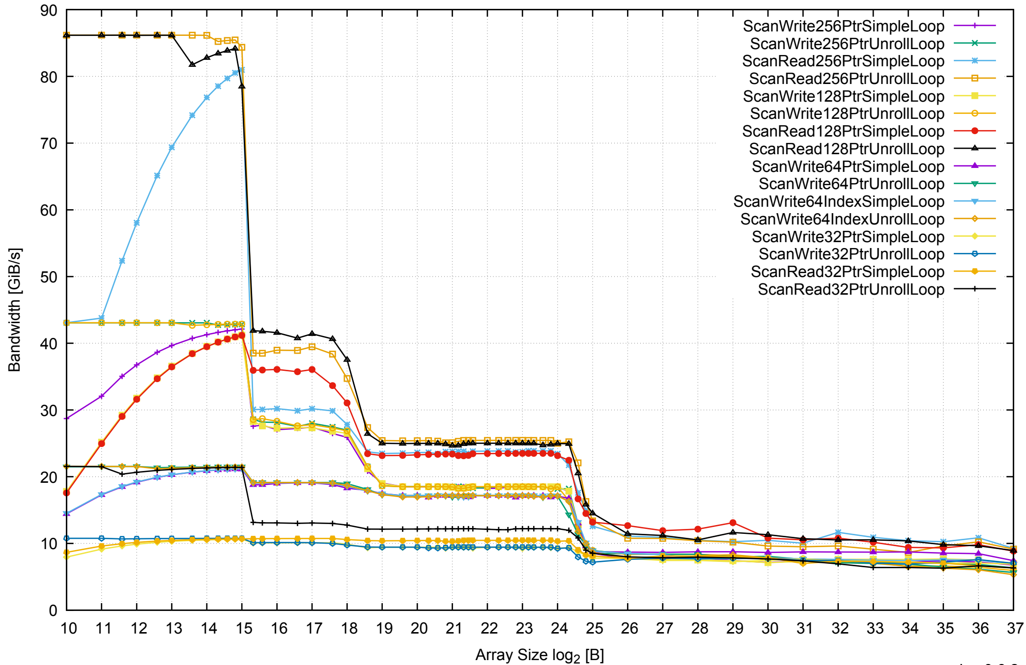
AWS r3.8xlarge - Intel Xeon E5-2676 v3, 2.50 GHz 244GB - One Thread Memory Bandwidth (only 64-bit Reads)
