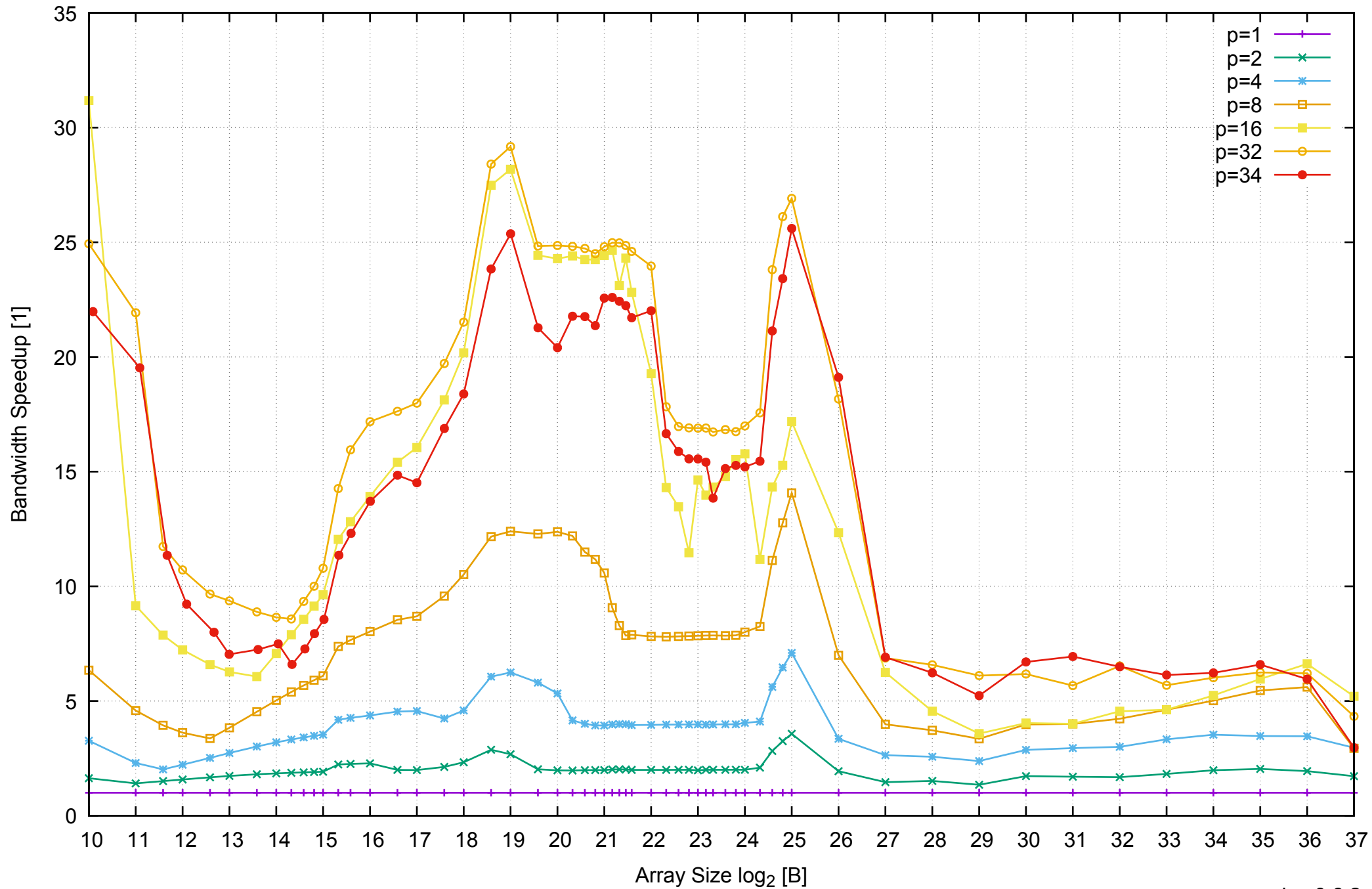
AWS r3.8xlarge - Intel Xeon E5-2676 v3, 2.50 GHz 244GB - Speedup of Parallel Memory Bandwidth - ScanRead128PtrSimpleLoop
