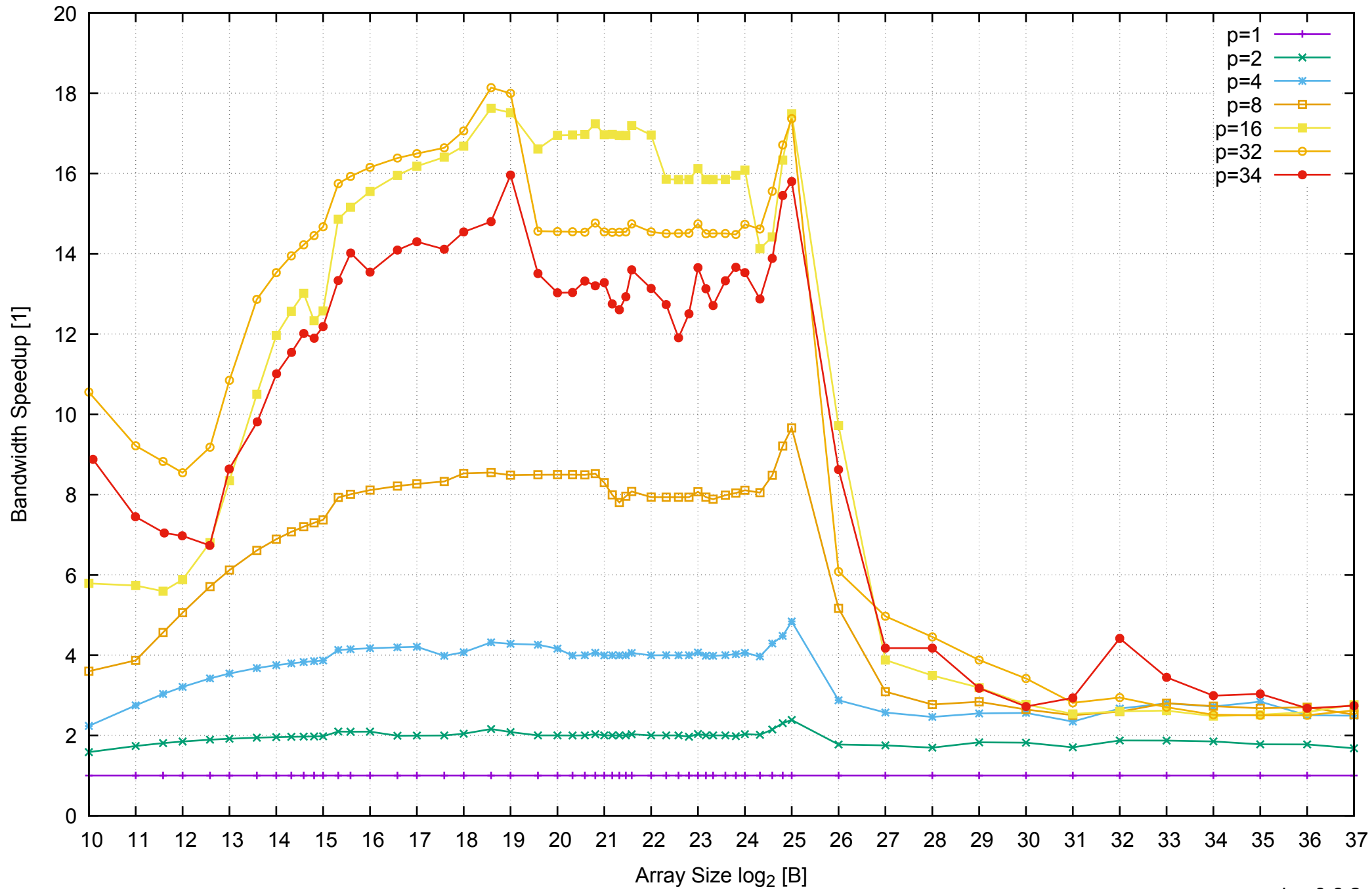
AWS r3.8xlarge - Intel Xeon E5-2676 v3, 2.50 GHz 244GB - Speedup of Parallel Memory Bandwidth - ScanWrite32PtrSimpleLoop
