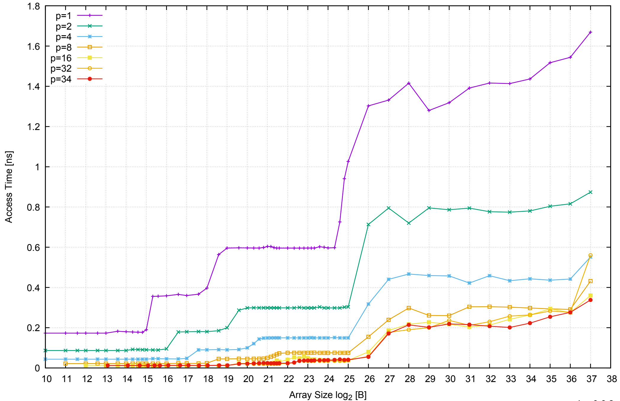
AWS r3.8xlarge - Intel Xeon E5-2676 v3, 2.50 GHz 244GB - Parallel Memory Access Time - ScanRead128PtrUnrollLoop
