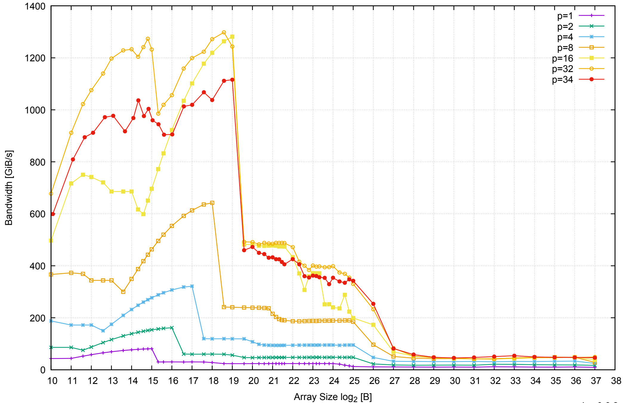
AWS r3.8xlarge - Intel Xeon E5-2676 v3, 2.50 GHz 244GB - Parallel Memory Bandwidth - ScanRead256PtrSimpleLoop
