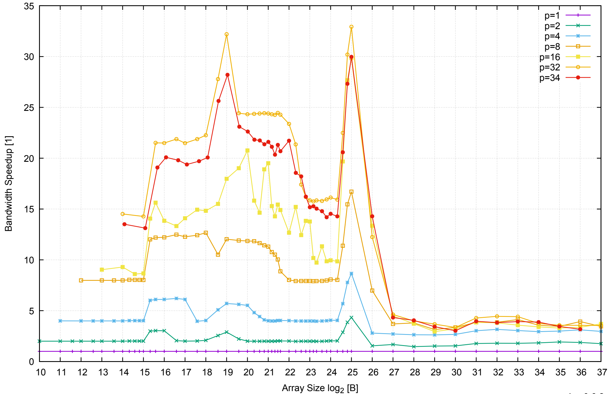
AWS r3.8xlarge - Intel Xeon E5-2676 v3, 2.50 GHz 244GB - Speedup of Parallel Memory Bandwidth - ScanWrite256PtrUnrollLoop
