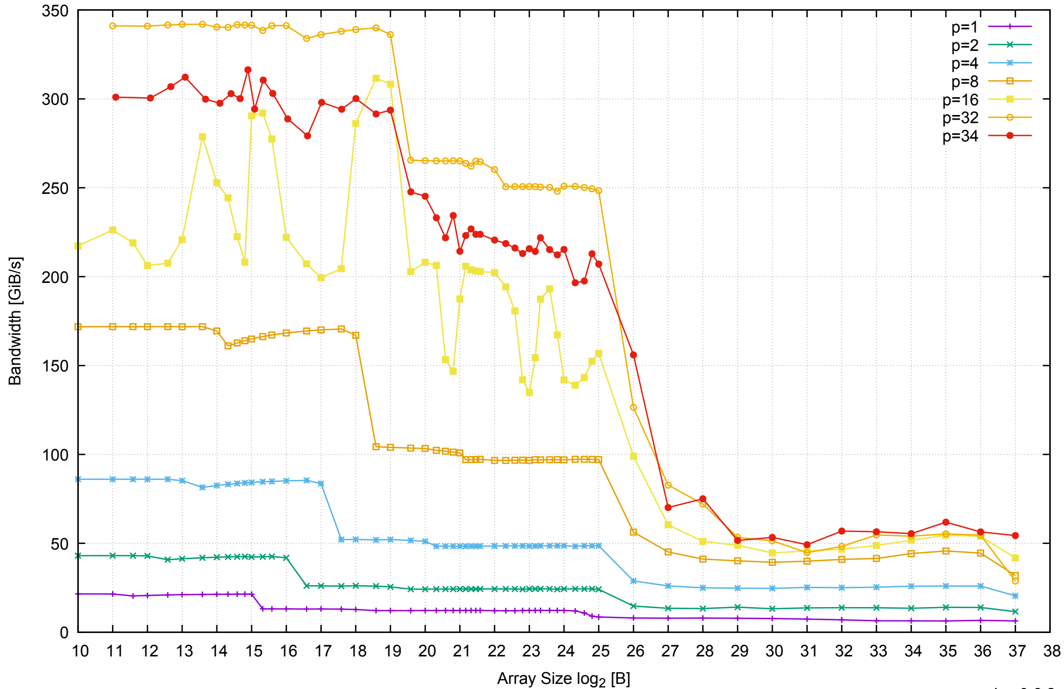
AWS r3.8xlarge - Intel Xeon E5-2676 v3, 2.50 GHz 244GB - Parallel Memory Bandwidth - ScanRead32PtrUnrollLoop
