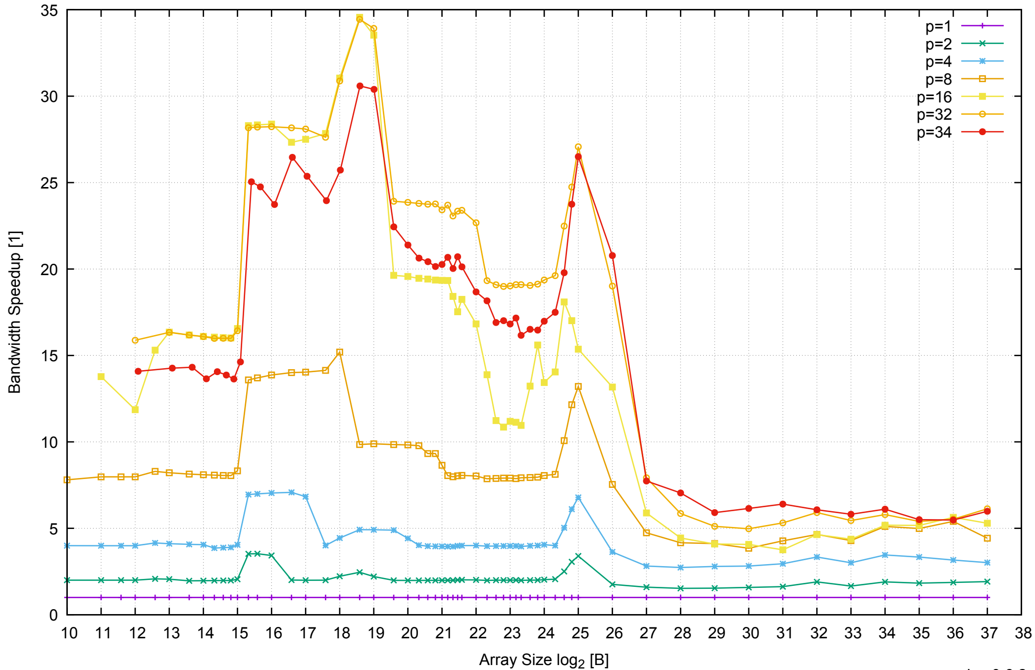
AWS r3.8xlarge - Intel Xeon E5-2676 v3, 2.50 GHz 244GB - Speedup of Parallel Memory Bandwidth - ScanRead64PtrUnrollLoop
