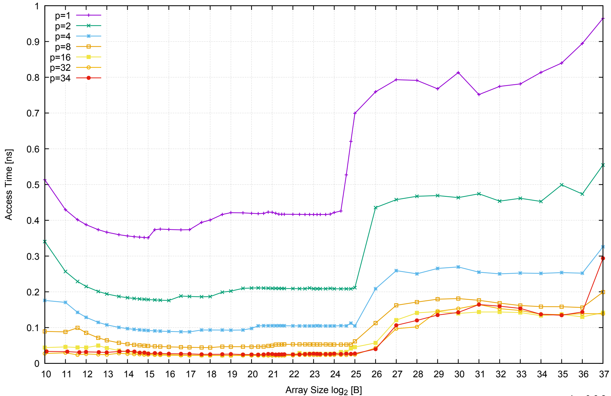
AWS r3.8xlarge - Intel Xeon E5-2676 v3, 2.50 GHz 244GB - Parallel Memory Access Time - ScanRead64IndexSimpleLoop
