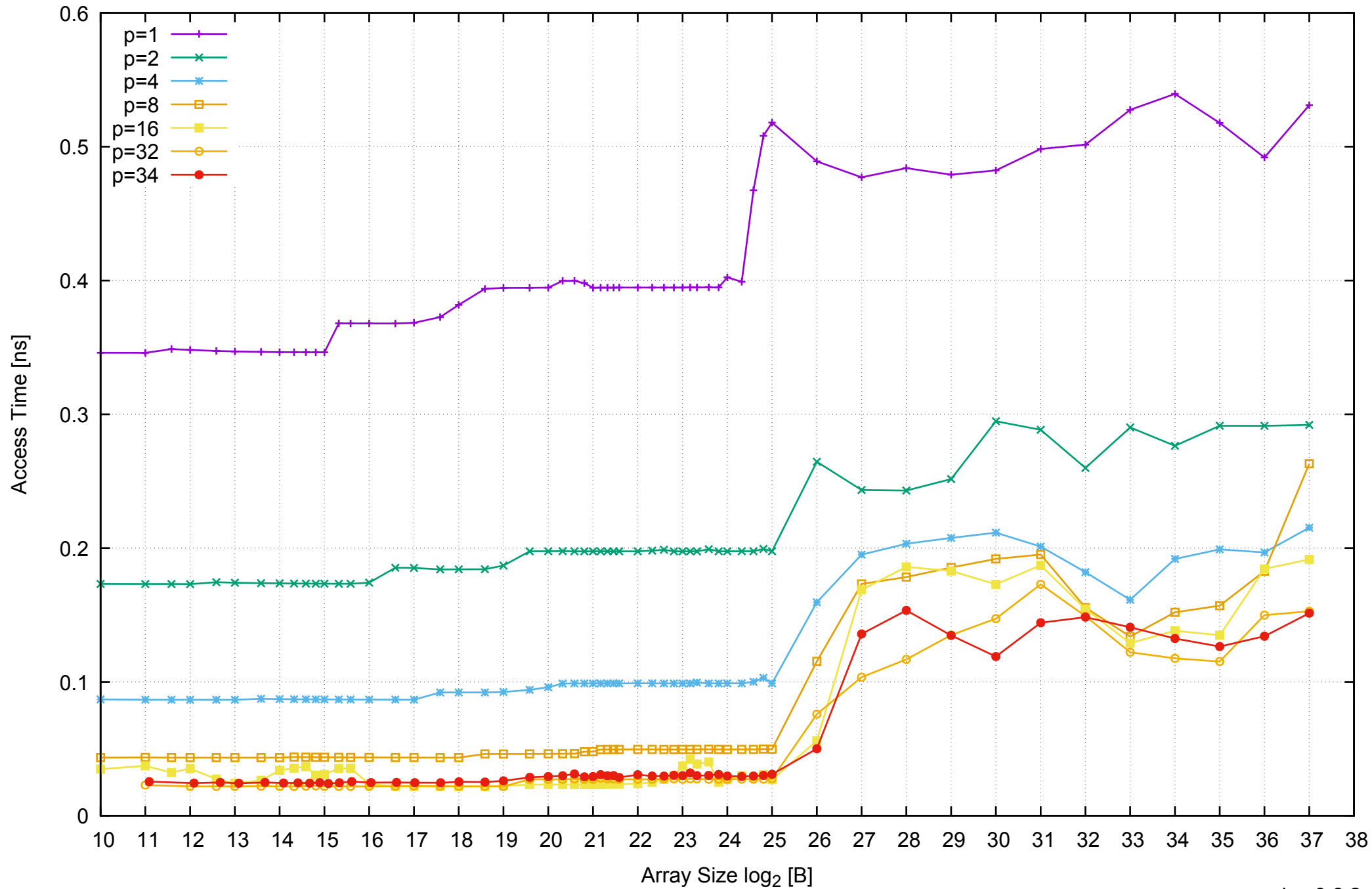
AWS r3.8xlarge - Intel Xeon E5-2676 v3, 2.50 GHz 244GB - Parallel Memory Access Time - ScanWrite32PtrUnrollLoop
