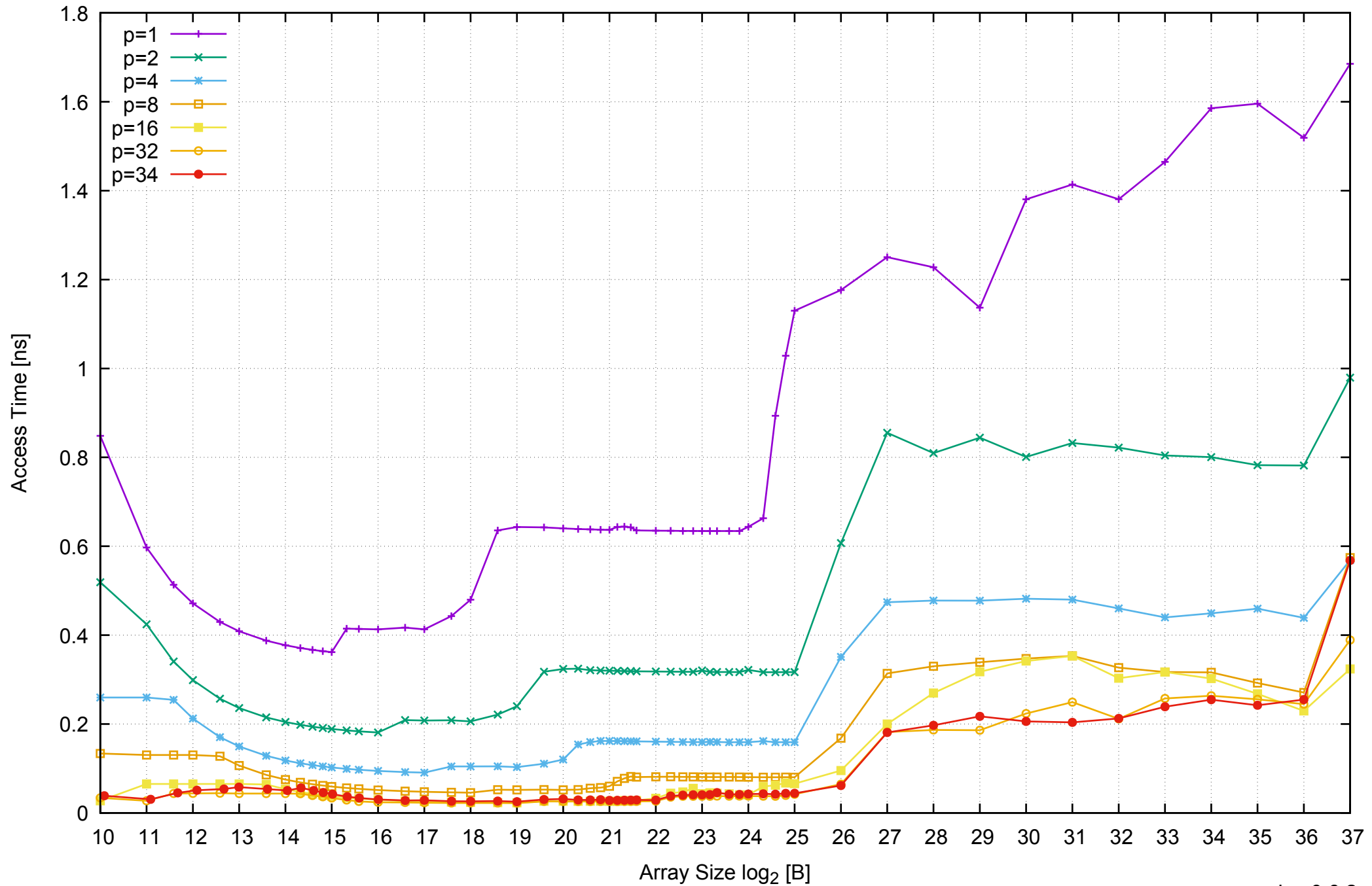
AWS r3.8xlarge - Intel Xeon E5-2676 v3, 2.50 GHz 244GB - Parallel Memory Access Time - ScanRead128PtrSimpleLoop
