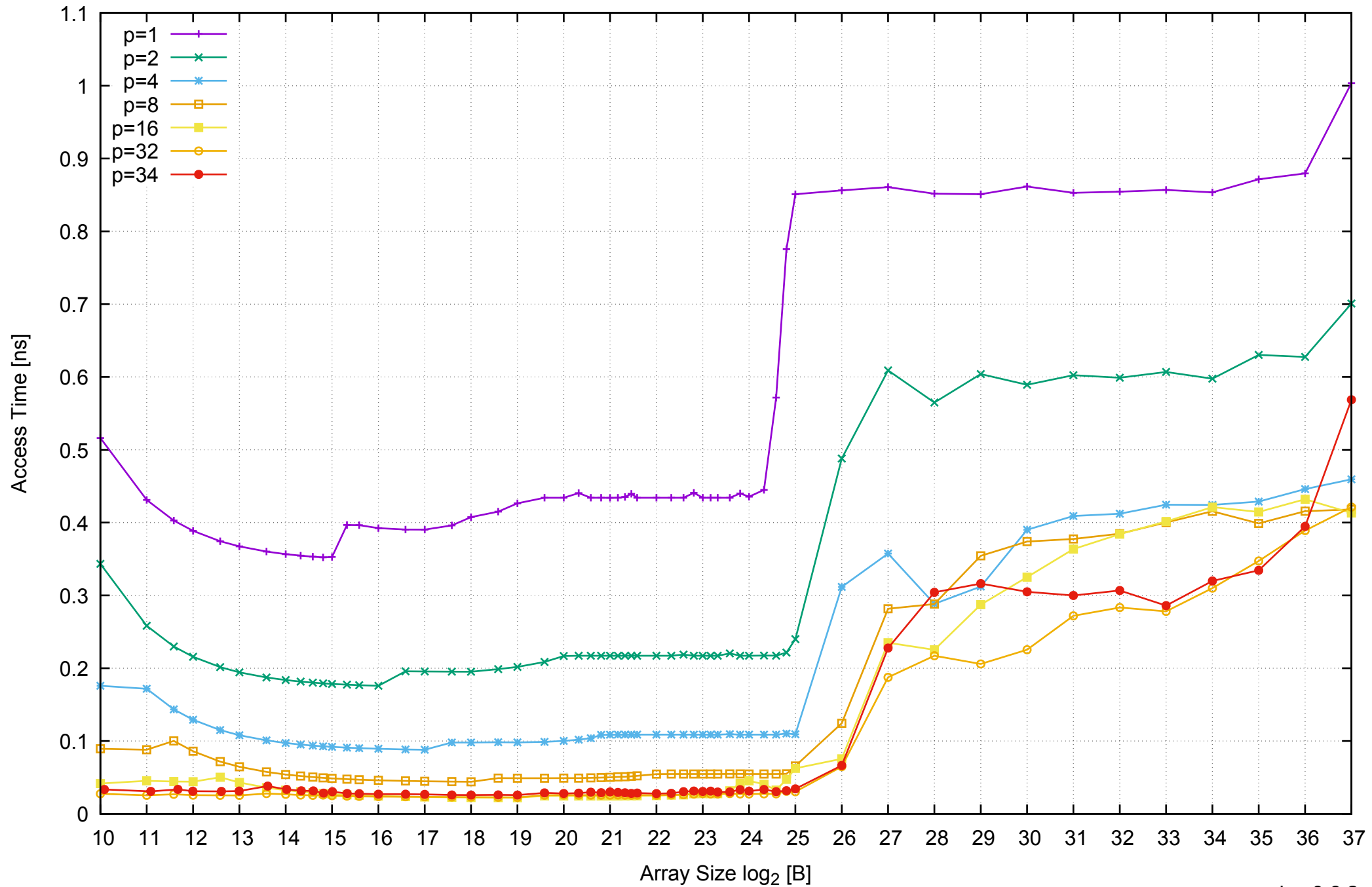
AWS r3.8xlarge - Intel Xeon E5-2676 v3, 2.50 GHz 244GB - Parallel Memory Access Time - ScanWrite64PtrSimpleLoop
