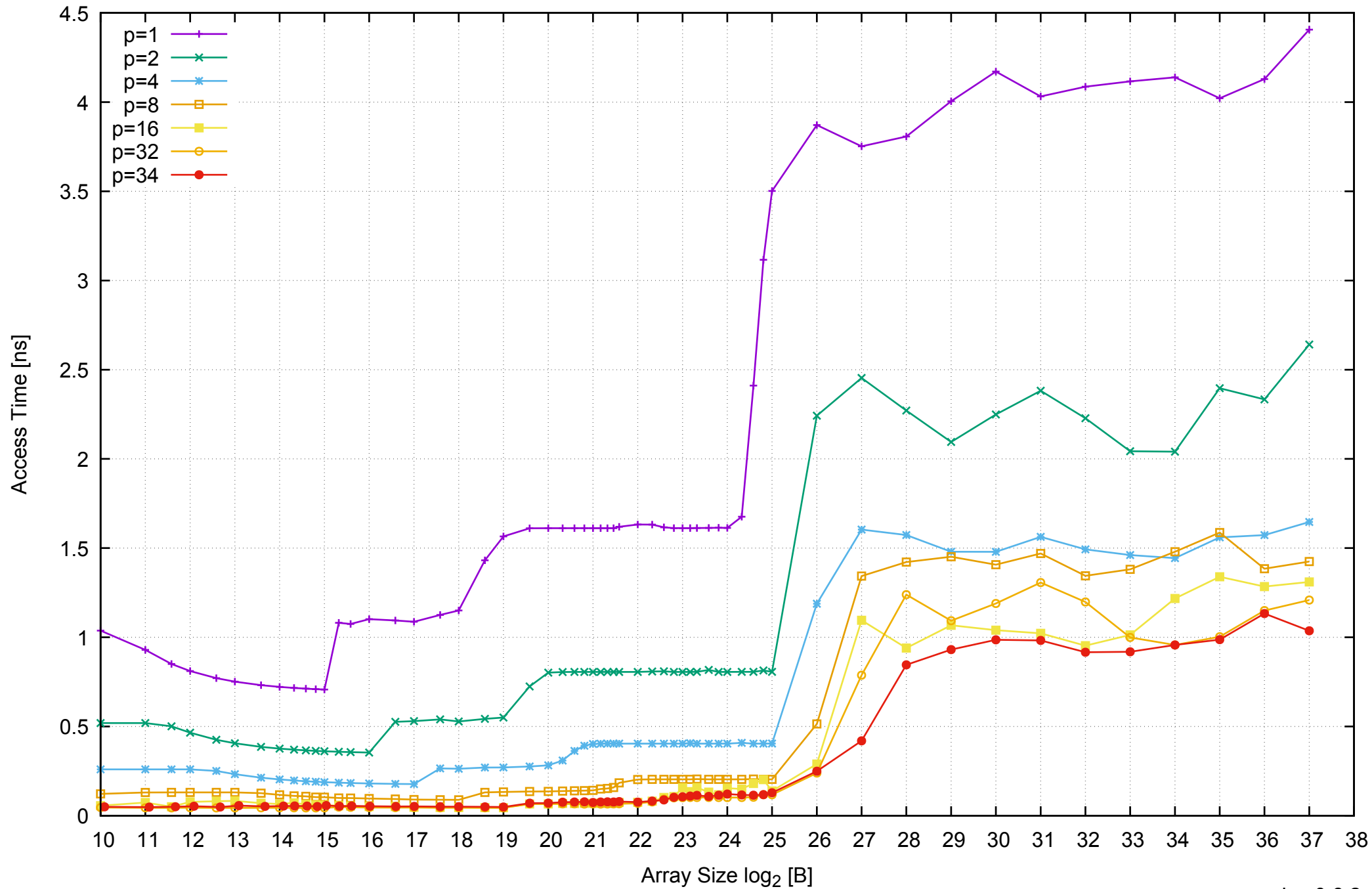
AWS r3.8xlarge - Intel Xeon E5-2676 v3, 2.50 GHz 244GB - Parallel Memory Access Time - ScanWrite256PtrSimpleLoop
