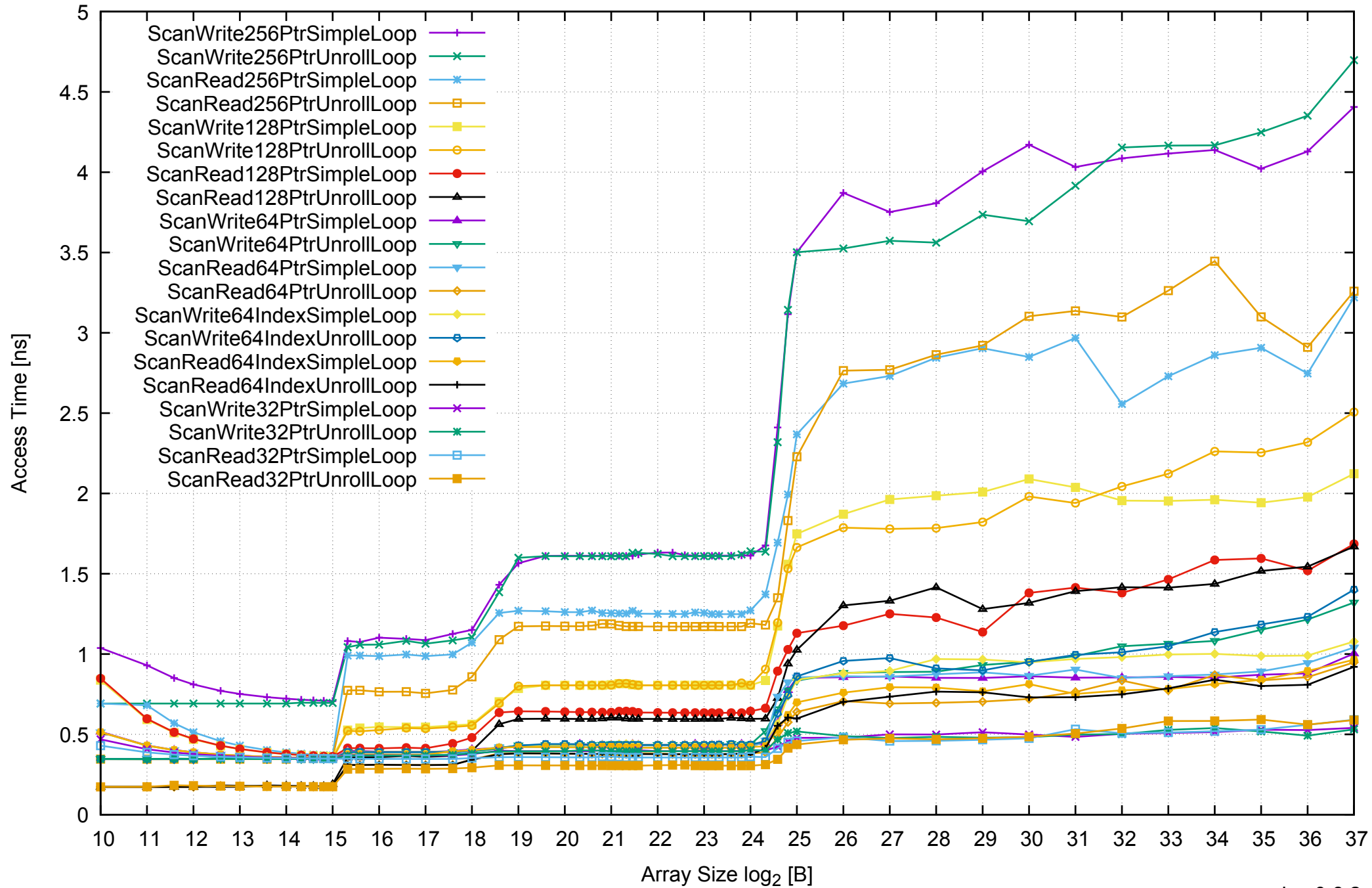
AWS r3.8xlarge - Intel Xeon E5-2676 v3, 2.50 GHz 244GB - One Thread Memory Latency (excluding Permutation)
