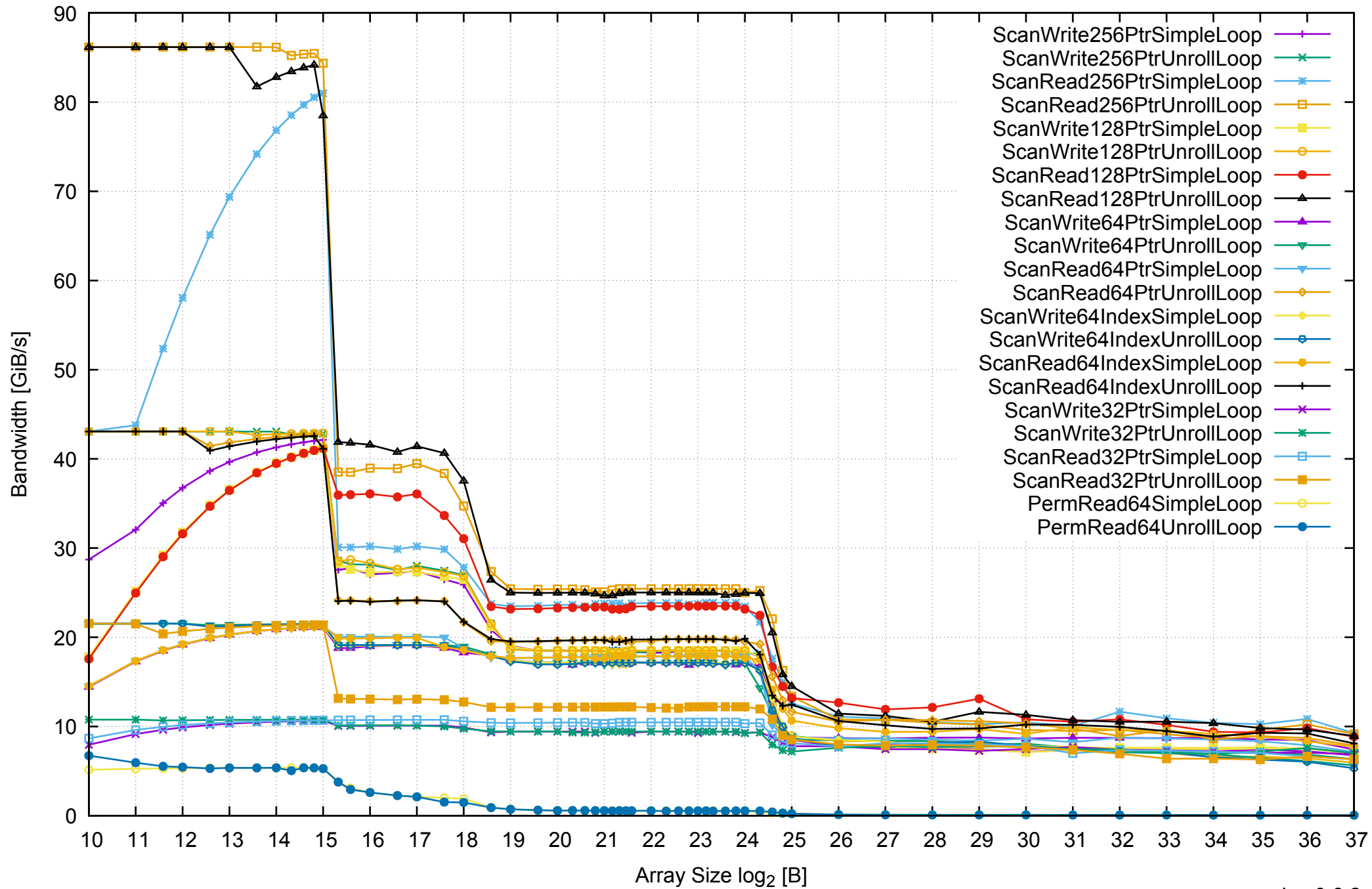
AWS r3.8xlarge - Intel Xeon E5-2676 v3, 2.50 GHz 244GB - One Thread Memory Bandwidth
