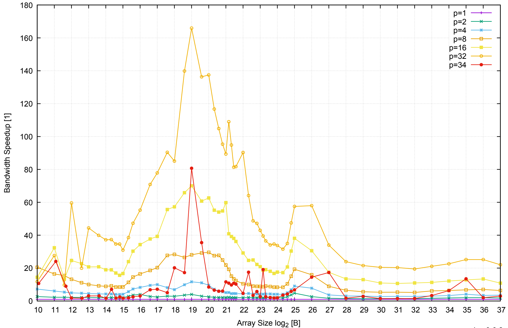
AWS r3.8xlarge - Intel Xeon E5-2676 v3, 2.50 GHz 244GB - Speedup of Parallel Memory Bandwidth - PermRead64UnrollLoop
