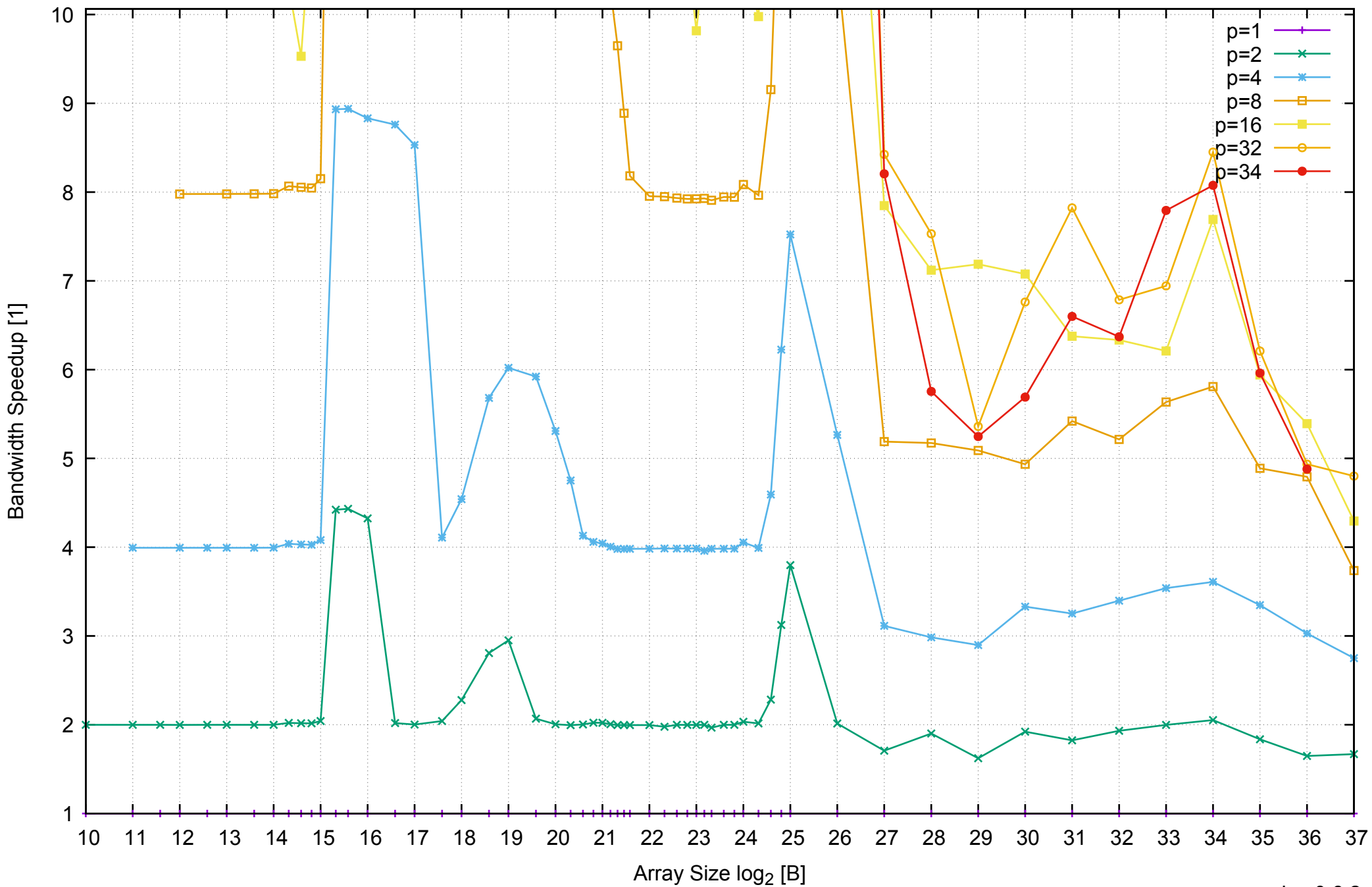
AWS r3.8xlarge - Intel Xeon E5-2676 v3, 2.50 GHz 244GB - Speedup of Parallel Memory Bandwidth (enlarged) - ScanRead256PtrUnrollLoop
