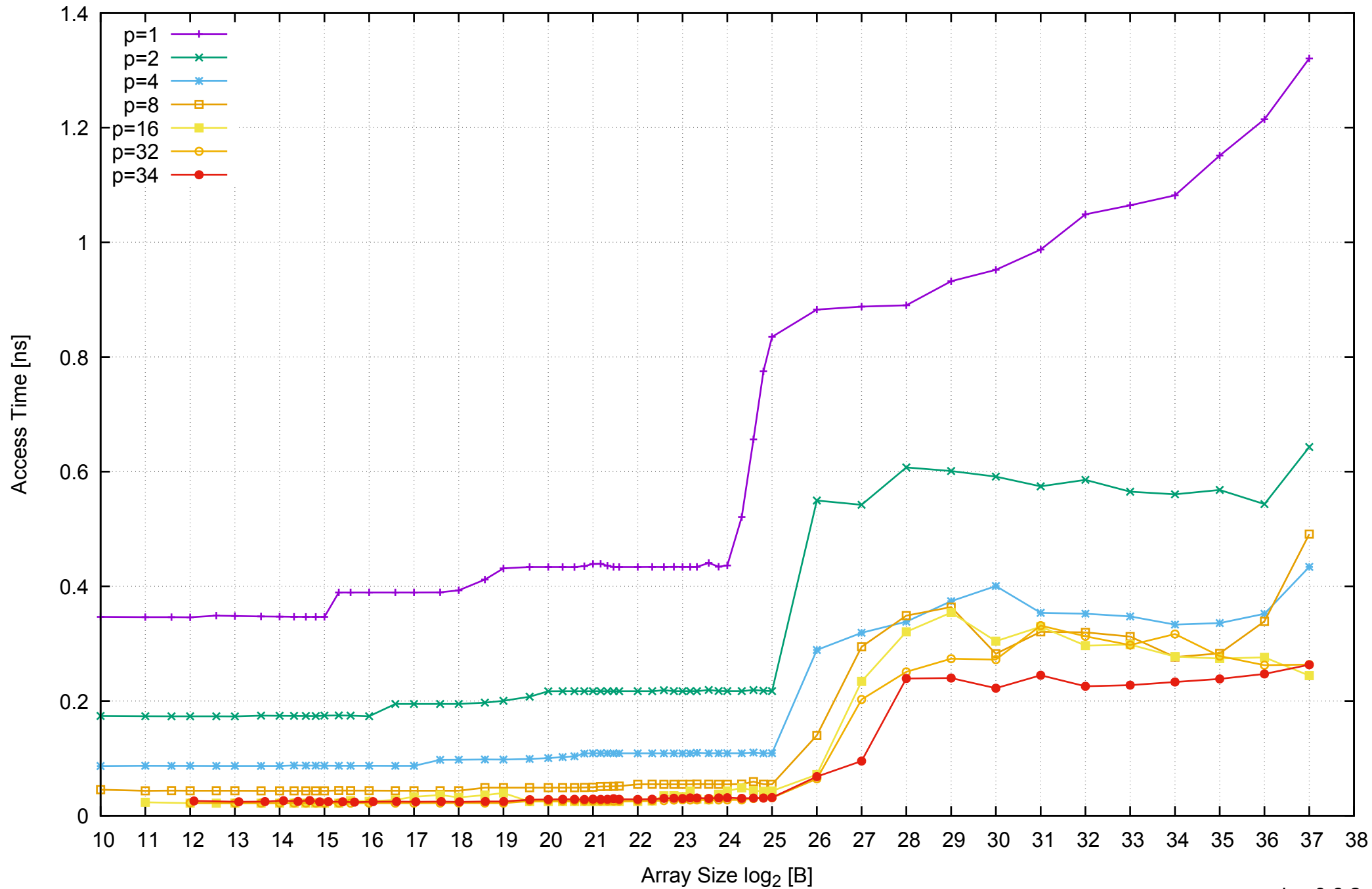
AWS r3.8xlarge - Intel Xeon E5-2676 v3, 2.50 GHz 244GB - Parallel Memory Access Time - ScanWrite64PtrUnrollLoop
