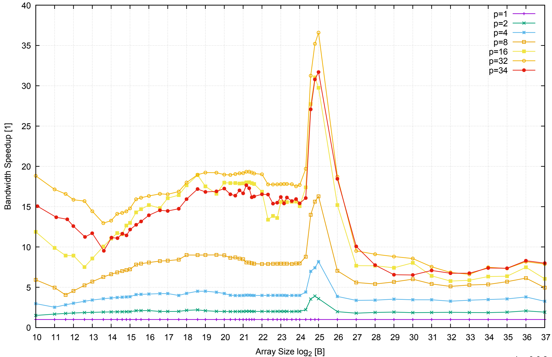
AWS r3.8xlarge - Intel Xeon E5-2676 v3, 2.50 GHz 244GB - Speedup of Parallel Memory Bandwidth - ScanRead64PtrSimpleLoop
