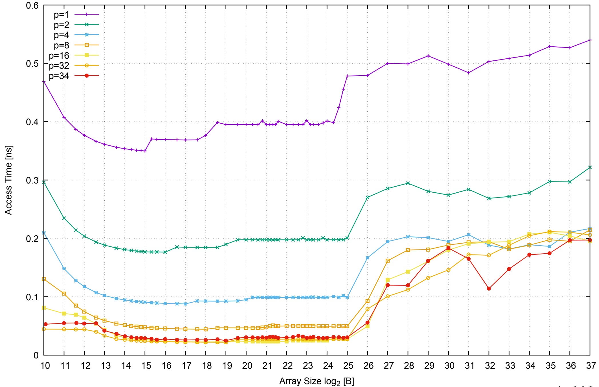
AWS r3.8xlarge - Intel Xeon E5-2676 v3, 2.50 GHz 244GB - Parallel Memory Access Time - ScanWrite32PtrSimpleLoop
