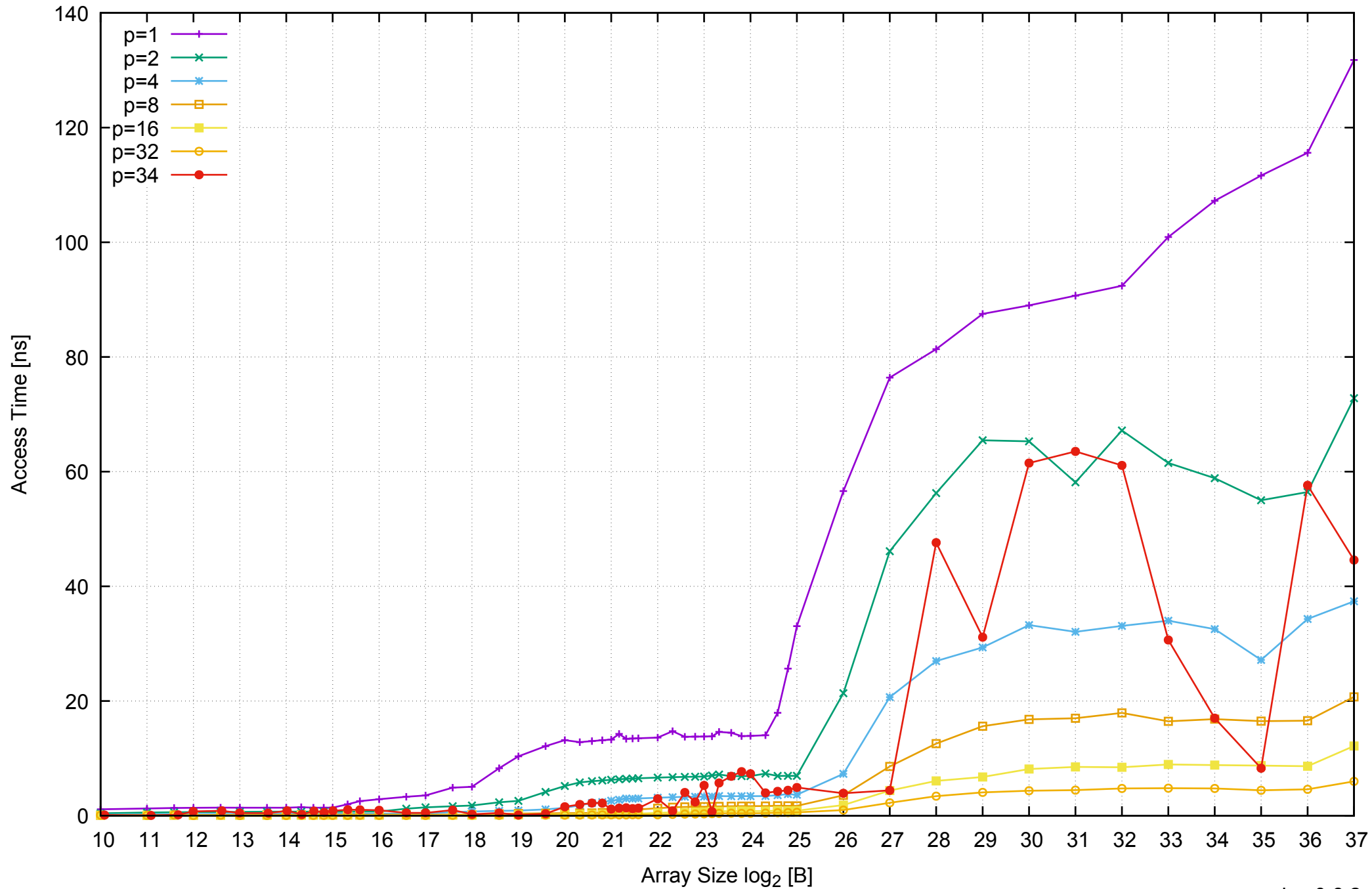
AWS r3.8xlarge - Intel Xeon E5-2676 v3, 2.50 GHz 244GB - Parallel Memory Access Time - PermRead64UnrollLoop
