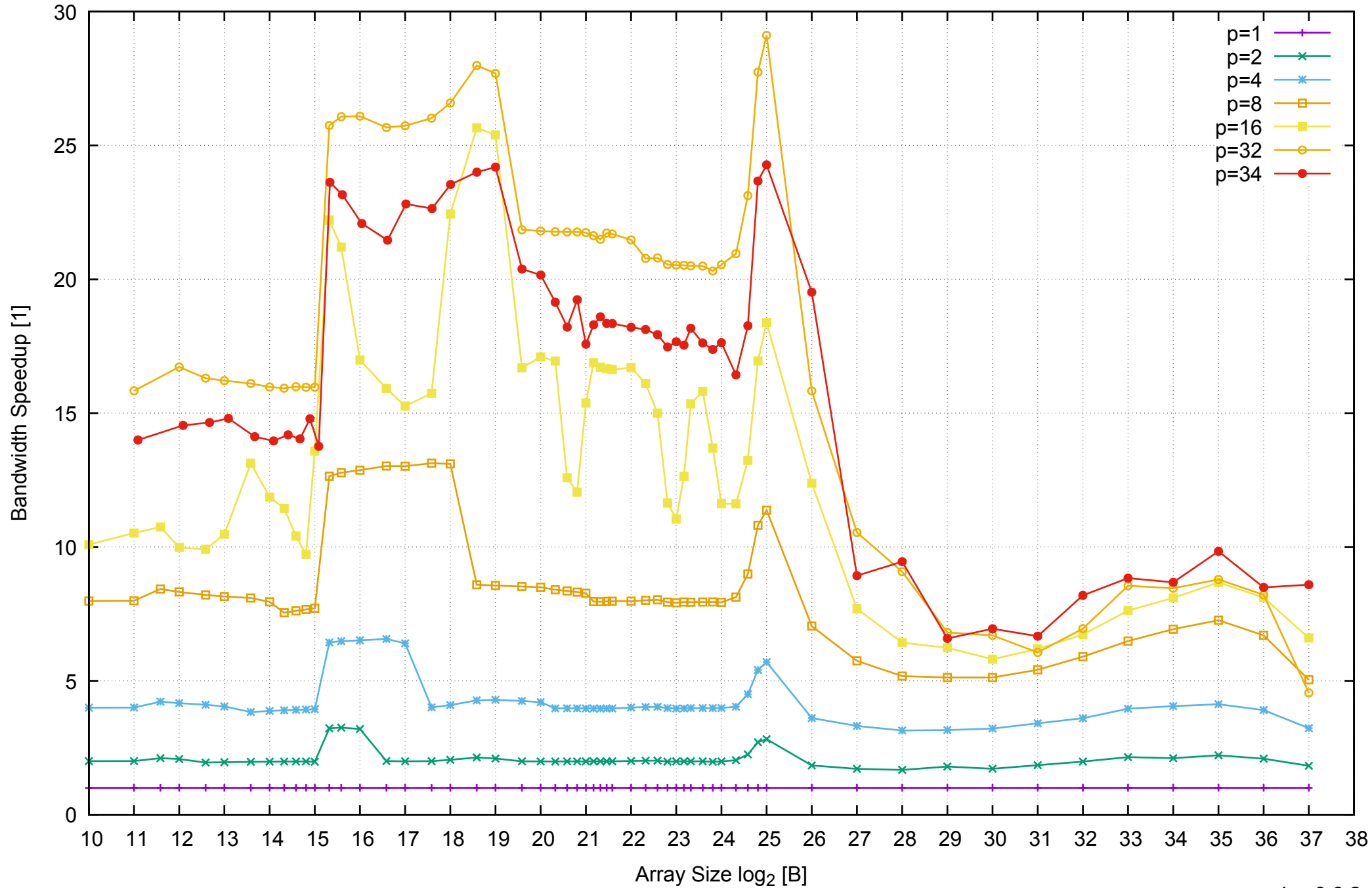
AWS r3.8xlarge - Intel Xeon E5-2676 v3, 2.50 GHz 244GB - Speedup of Parallel Memory Bandwidth - ScanRead32PtrUnrollLoop
