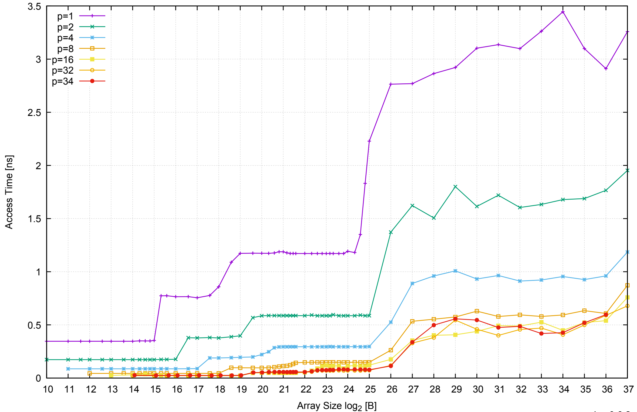
AWS r3.8xlarge - Intel Xeon E5-2676 v3, 2.50 GHz 244GB - Parallel Memory Access Time - ScanRead256PtrUnrollLoop
