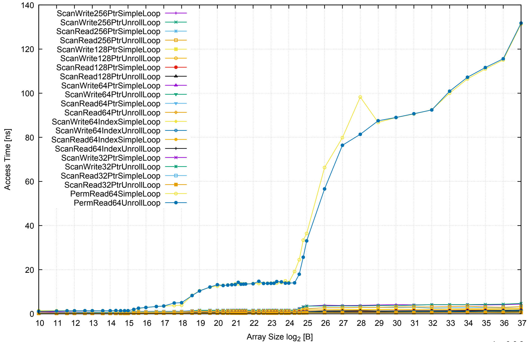
AWS r3.8xlarge - Intel Xeon E5-2676 v3, 2.50 GHz 244GB - One Thread Memory Latency (Access Time)
