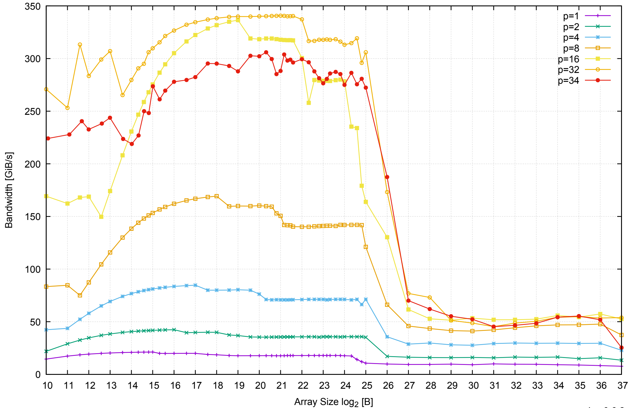
AWS r3.8xlarge - Intel Xeon E5-2676 v3, 2.50 GHz 244GB - Parallel Memory Bandwidth - ScanRead64IndexSimpleLoop
