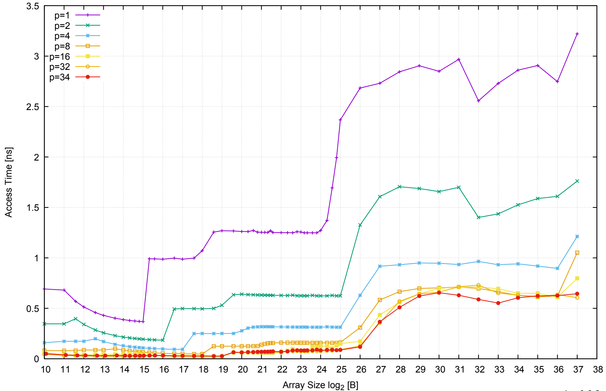
AWS r3.8xlarge - Intel Xeon E5-2676 v3, 2.50 GHz 244GB - Parallel Memory Access Time - ScanRead256PtrSimpleLoop
