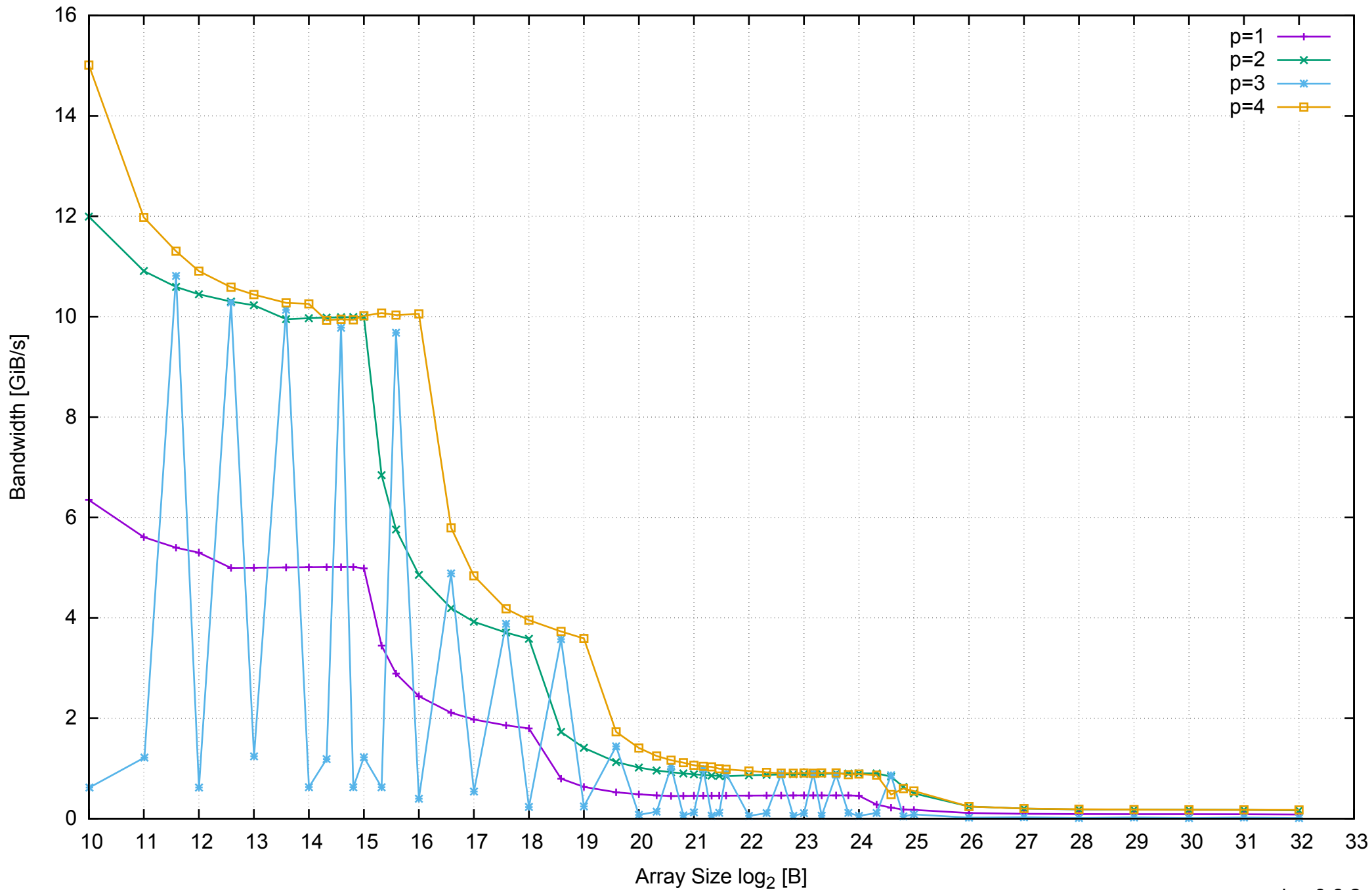
AWS m4.large - Intel Xeon E5-2676 v3, 2.40 GHz 8GB - Parallel Memory Bandwidth - PermRead64UnrollLoop
