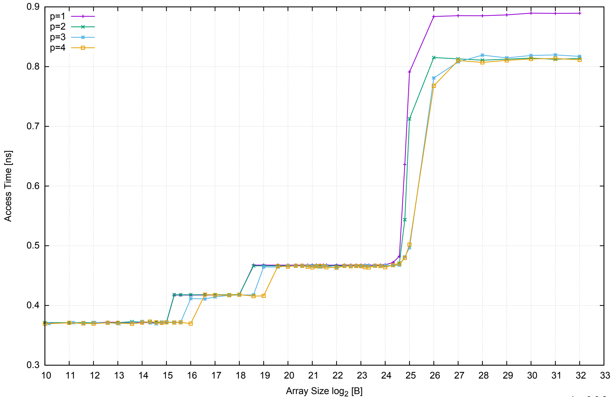
AWS m4.large - Intel Xeon E5-2676 v3, 2.40 GHz 8GB - Parallel Memory Access Time - ScanWrite64IndexUnrollLoop
