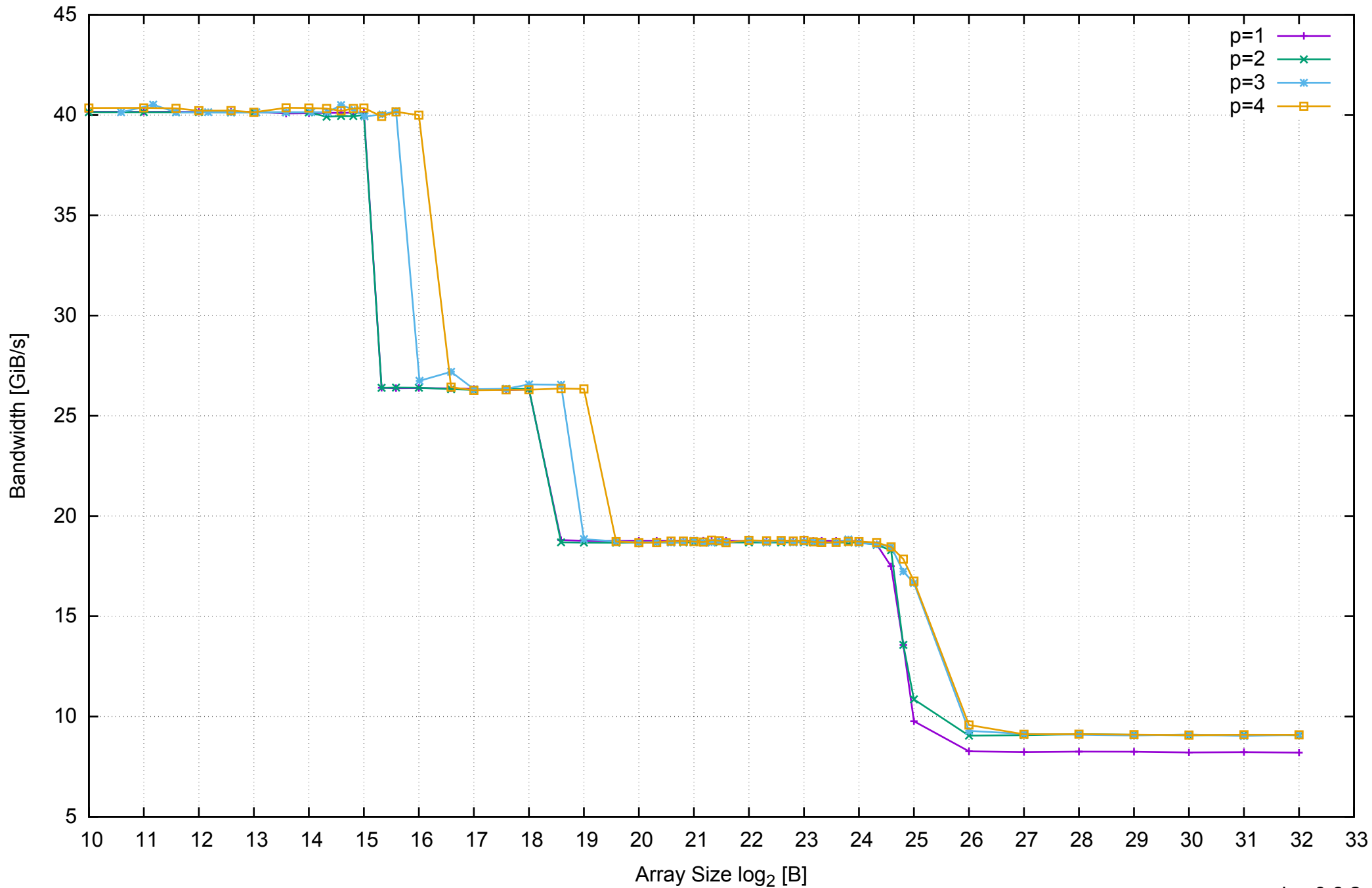
AWS m4.large - Intel Xeon E5-2676 v3, 2.40 GHz 8GB - Parallel Memory Bandwidth - ScanWrite128PtrUnrollLoop
