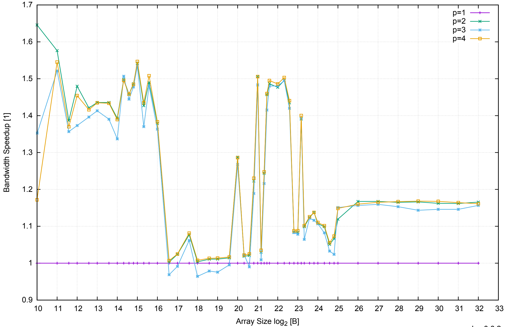
AWS m4.large - Intel Xeon E5-2676 v3, 2.40 GHz 8GB - Speedup of Parallel Memory Bandwidth - ScanRead32PtrSimpleLoop
