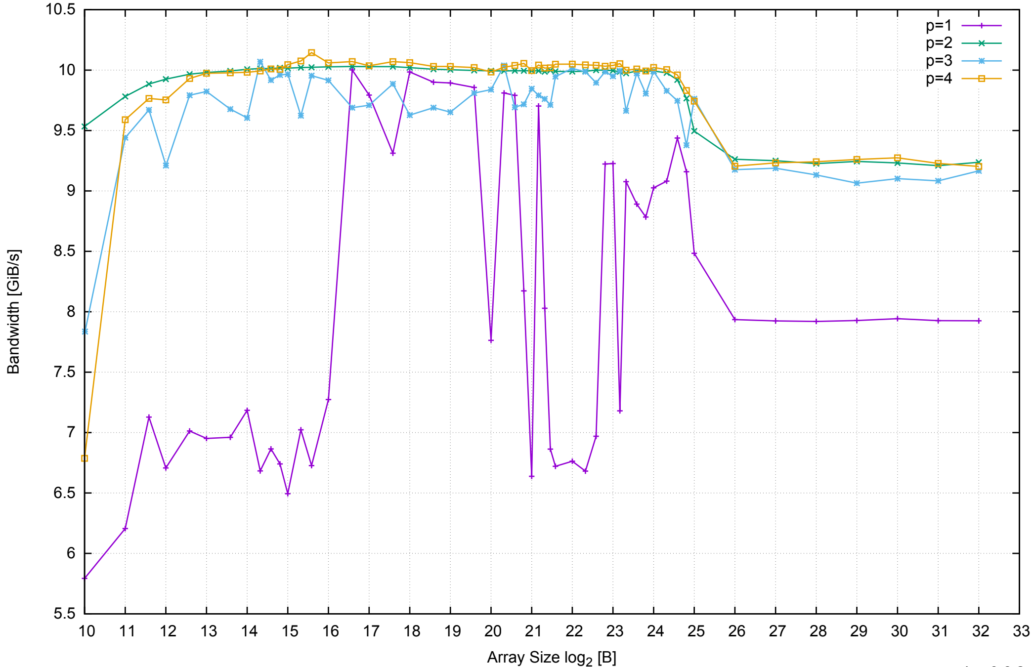
AWS m4.large - Intel Xeon E5-2676 v3, 2.40 GHz 8GB - Parallel Memory Bandwidth - ScanRead32PtrSimpleLoop
