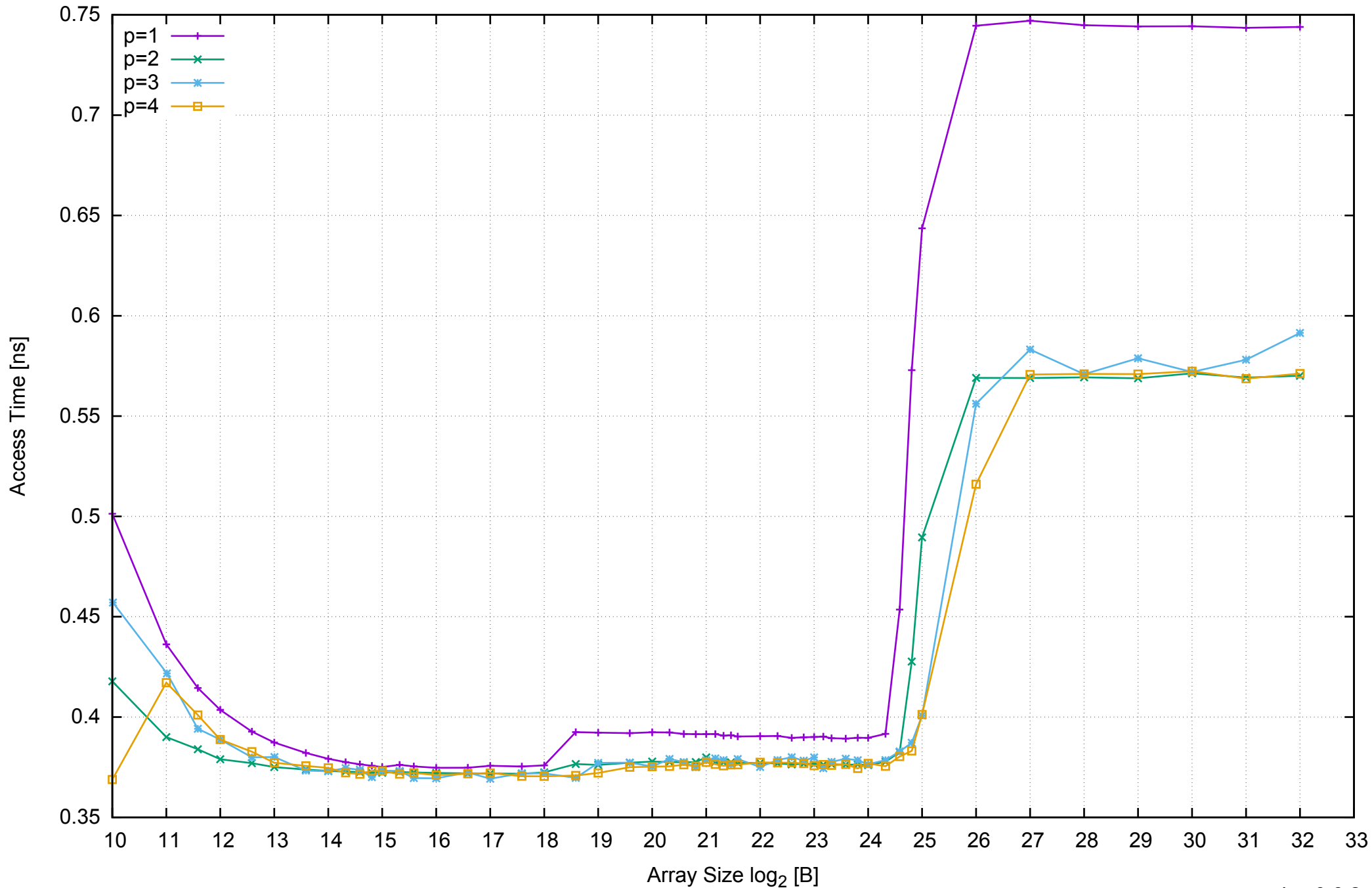
AWS m4.large - Intel Xeon E5-2676 v3, 2.40 GHz 8GB - Parallel Memory Access Time - ScanRead64PtrSimpleLoop
