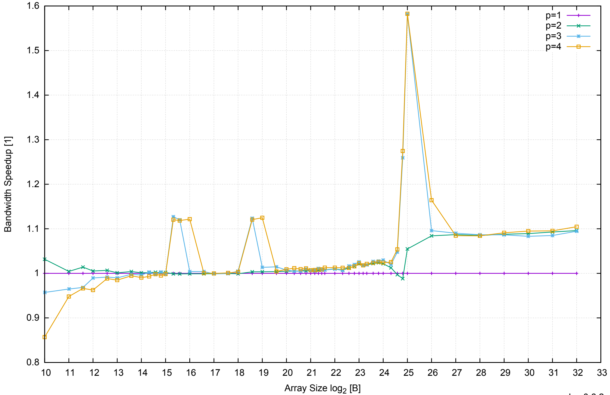
AWS m4.large - Intel Xeon E5-2676 v3, 2.40 GHz 8GB - Speedup of Parallel Memory Bandwidth - ScanWrite64PtrSimpleLoop
