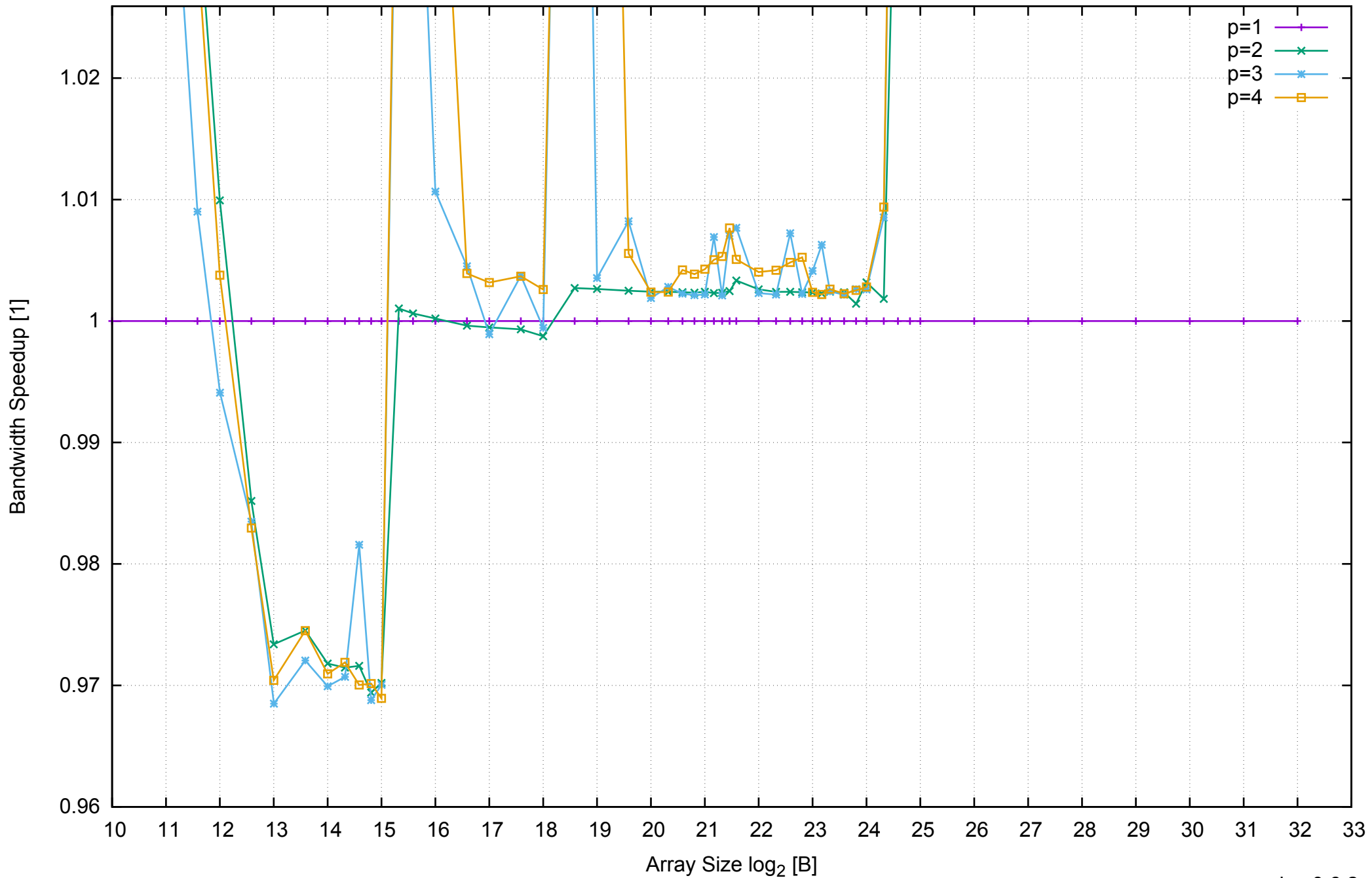
AWS m4.large - Intel Xeon E5-2676 v3, 2.40 GHz 8GB - Speedup of Parallel Memory Bandwidth (enlarged) - ScanWrite64IndexSimpleLoop
