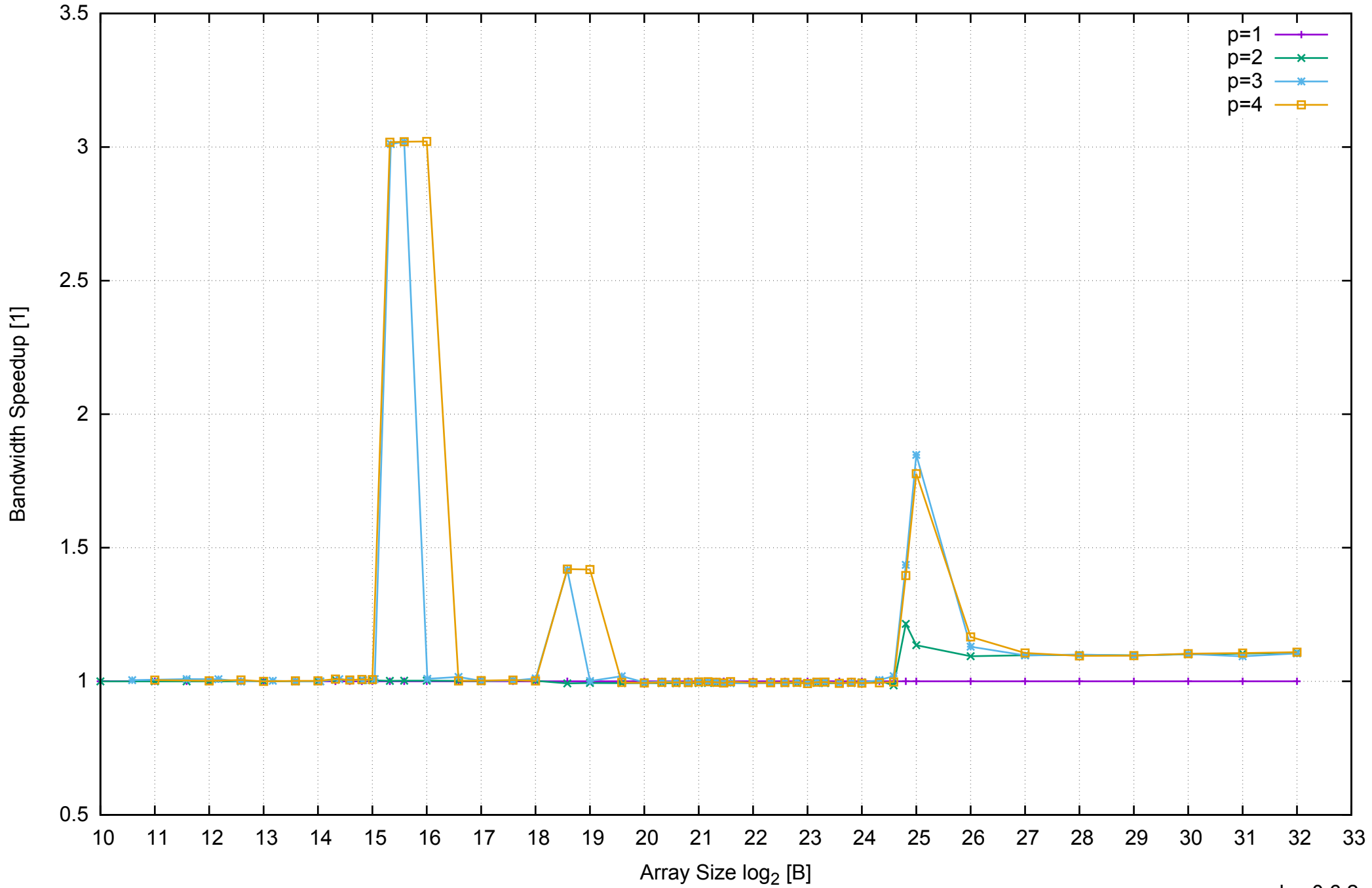
AWS m4.large - Intel Xeon E5-2676 v3, 2.40 GHz 8GB - Speedup of Parallel Memory Bandwidth - ScanWrite256PtrUnrollLoop
