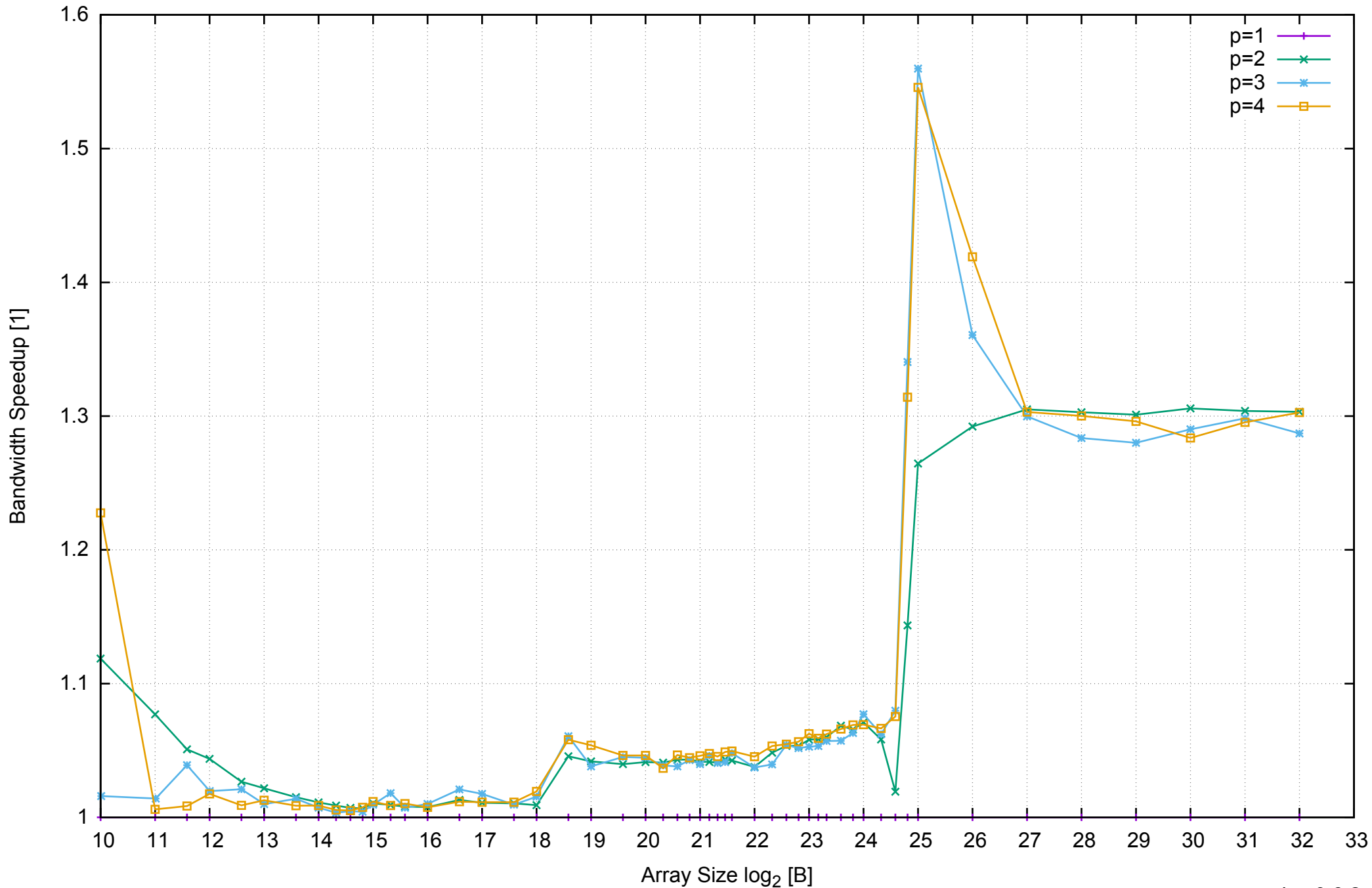
AWS m4.large - Intel Xeon E5-2676 v3, 2.40 GHz 8GB - Speedup of Parallel Memory Bandwidth - ScanRead64IndexSimpleLoop
