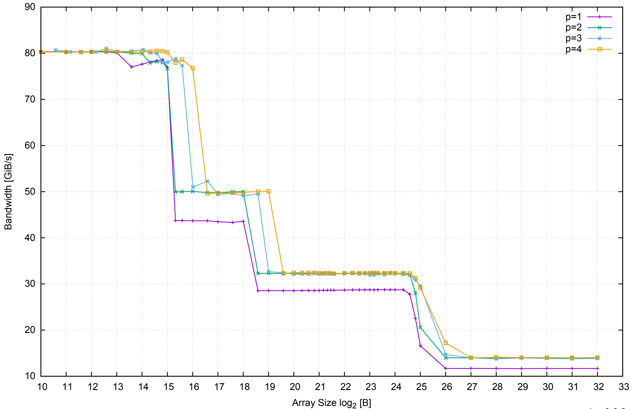
AWS m4.large - Intel Xeon E5-2676 v3, 2.40 GHz 8GB - Parallel Memory Bandwidth - ScanRead128PtrUnrollLoop
