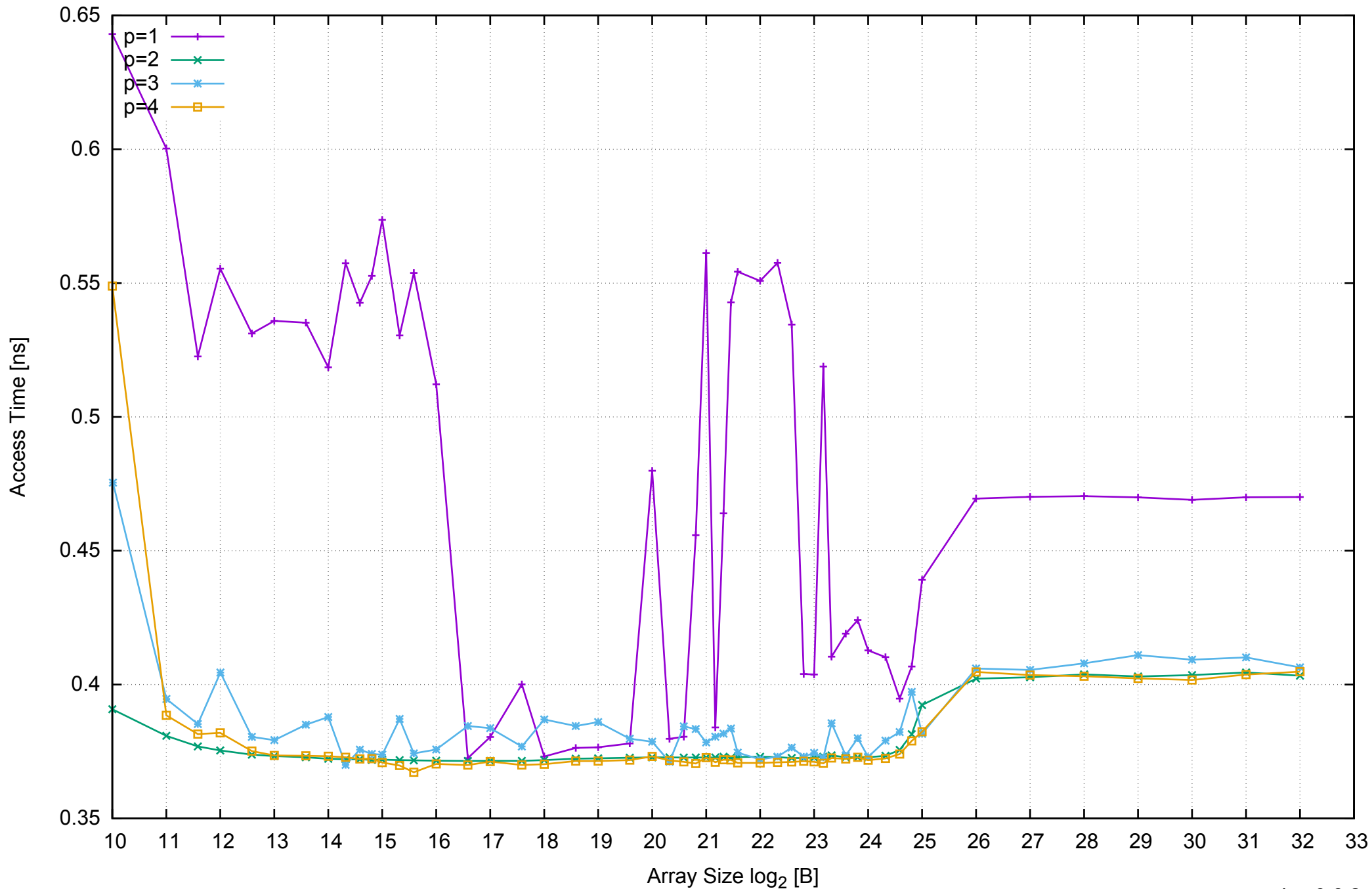
AWS m4.large - Intel Xeon E5-2676 v3, 2.40 GHz 8GB - Parallel Memory Access Time - ScanRead32PtrSimpleLoop
