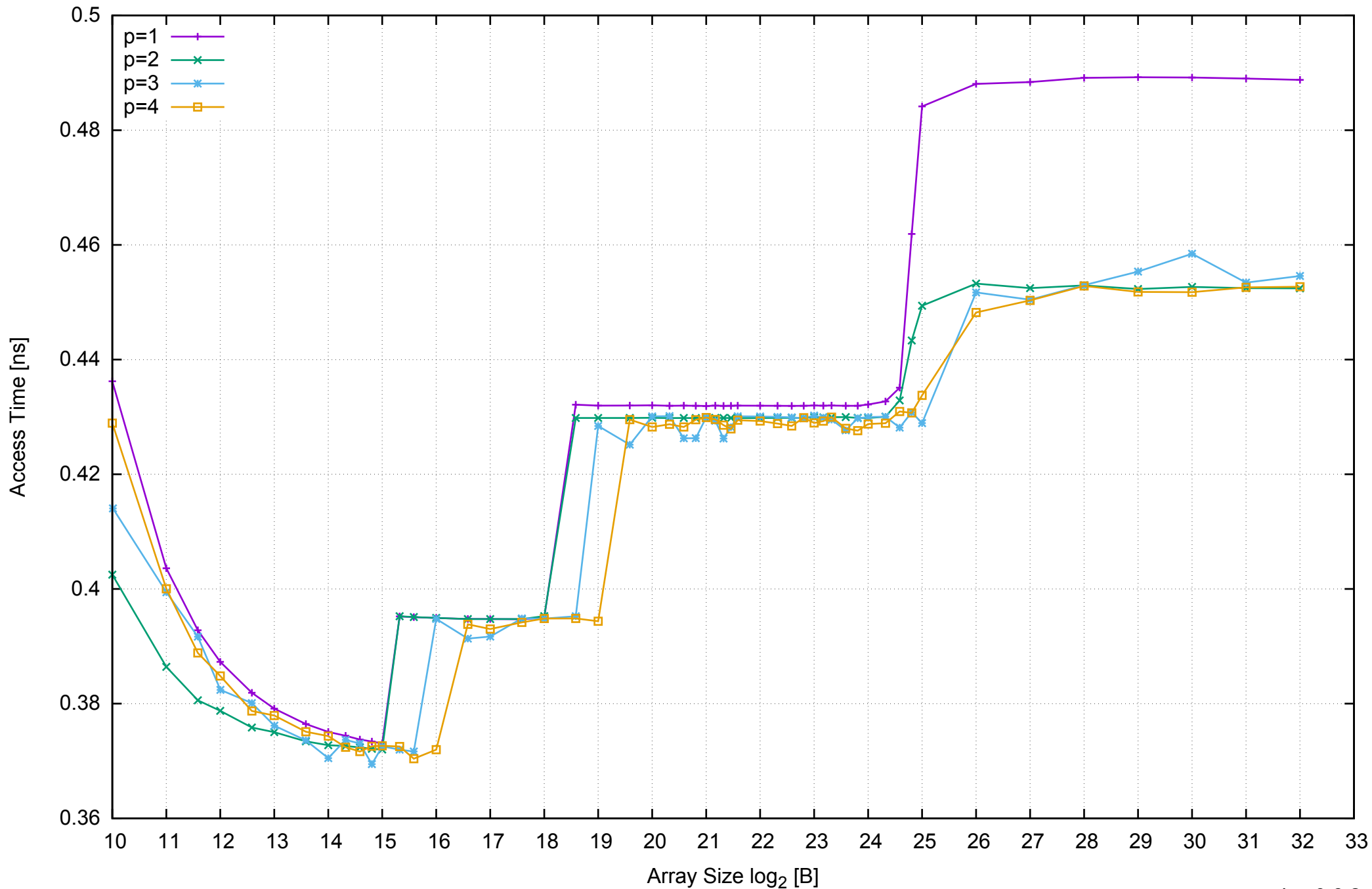
AWS m4.large - Intel Xeon E5-2676 v3, 2.40 GHz 8GB - Parallel Memory Access Time - ScanWrite32PtrSimpleLoop
