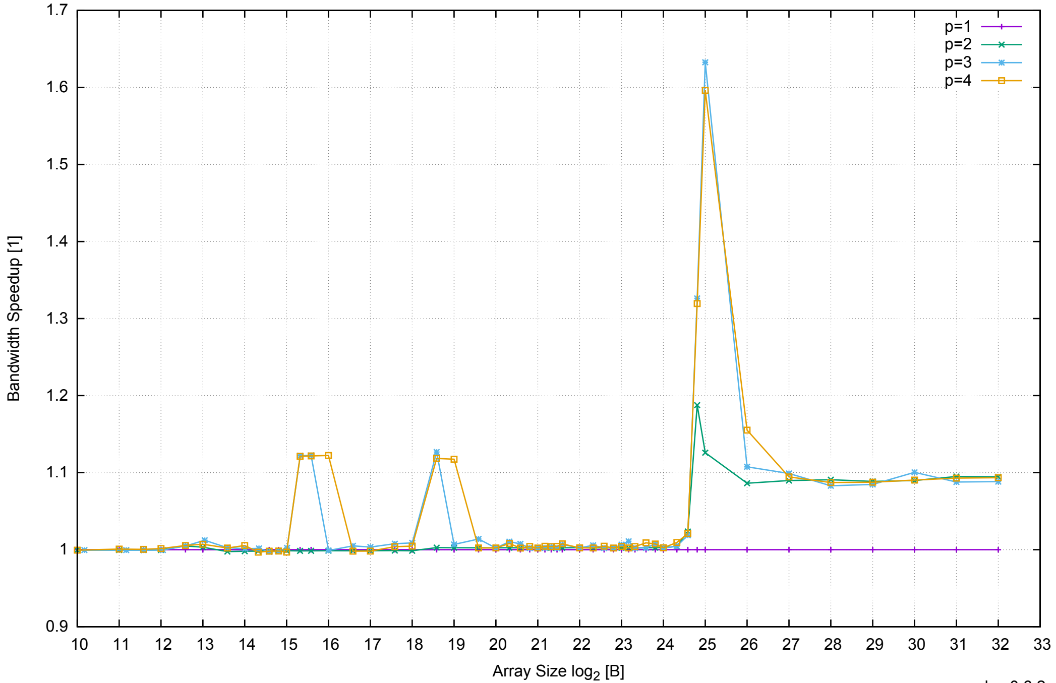
AWS m4.large - Intel Xeon E5-2676 v3, 2.40 GHz 8GB - Speedup of Parallel Memory Bandwidth - ScanWrite64PtrUnrollLoop
