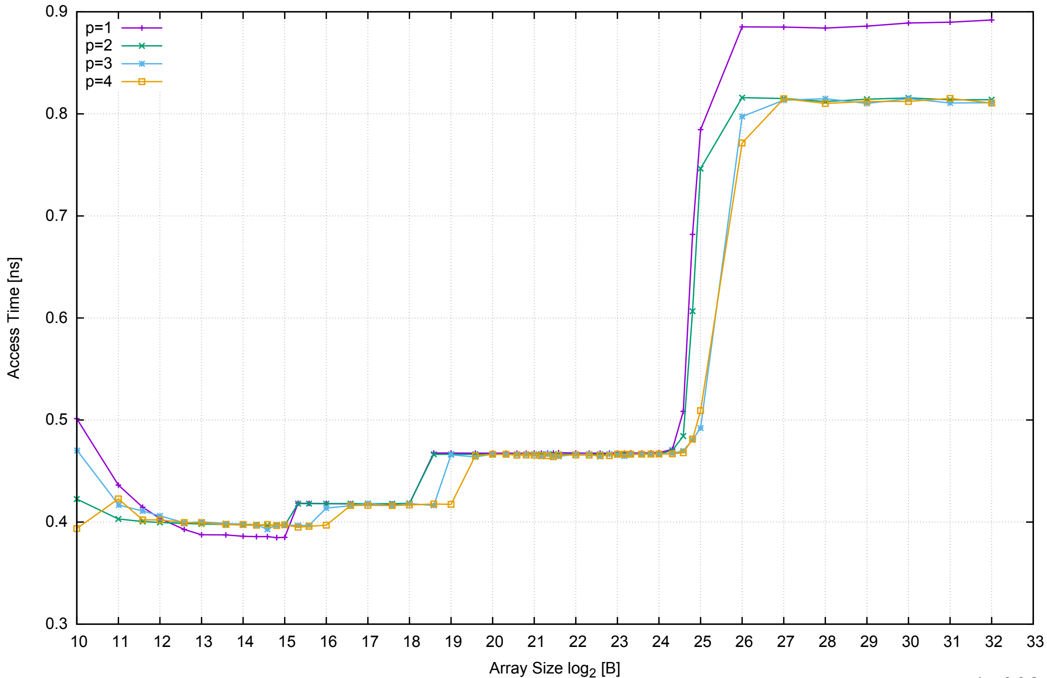
AWS m4.large - Intel Xeon E5-2676 v3, 2.40 GHz 8GB - Parallel Memory Access Time - ScanWrite64IndexSimpleLoop
