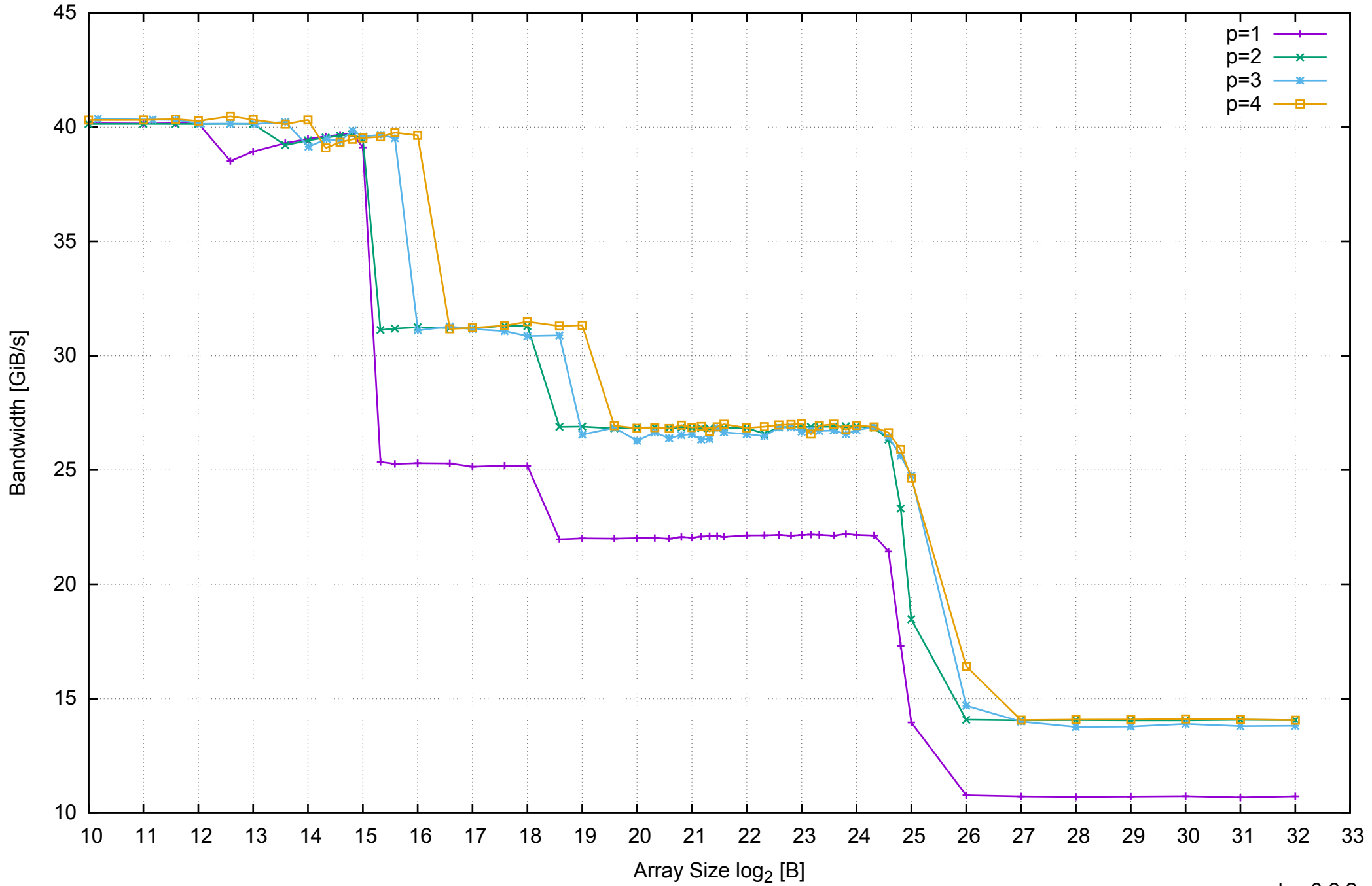
AWS m4.large - Intel Xeon E5-2676 v3, 2.40 GHz 8GB - Parallel Memory Bandwidth - ScanRead64PtrUnrollLoop
