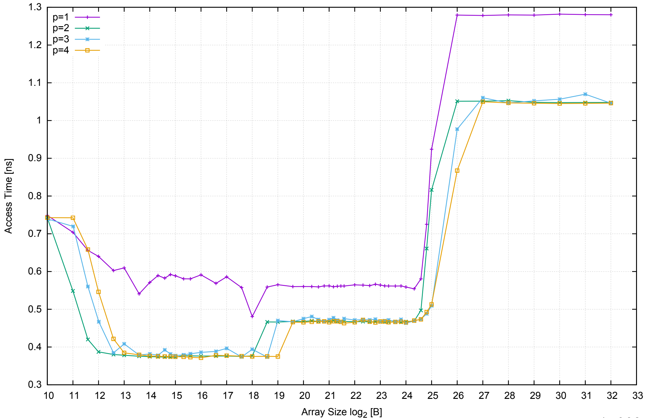
AWS m4.large - Intel Xeon E5-2676 v3, 2.40 GHz 8GB - Parallel Memory Access Time - ScanRead128PtrSimpleLoop
