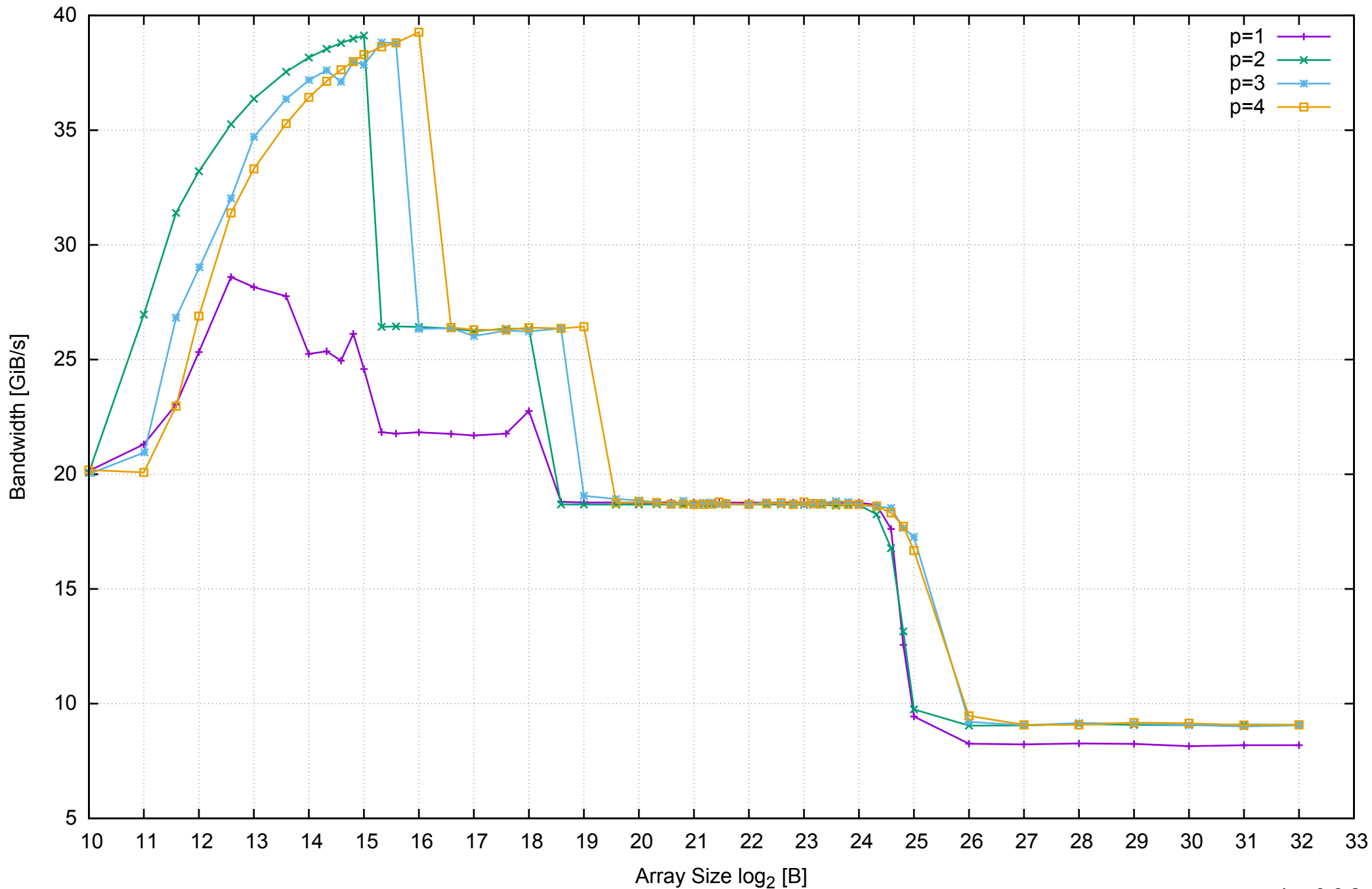
AWS m4.large - Intel Xeon E5-2676 v3, 2.40 GHz 8GB - Parallel Memory Bandwidth - ScanWrite128PtrSimpleLoop
