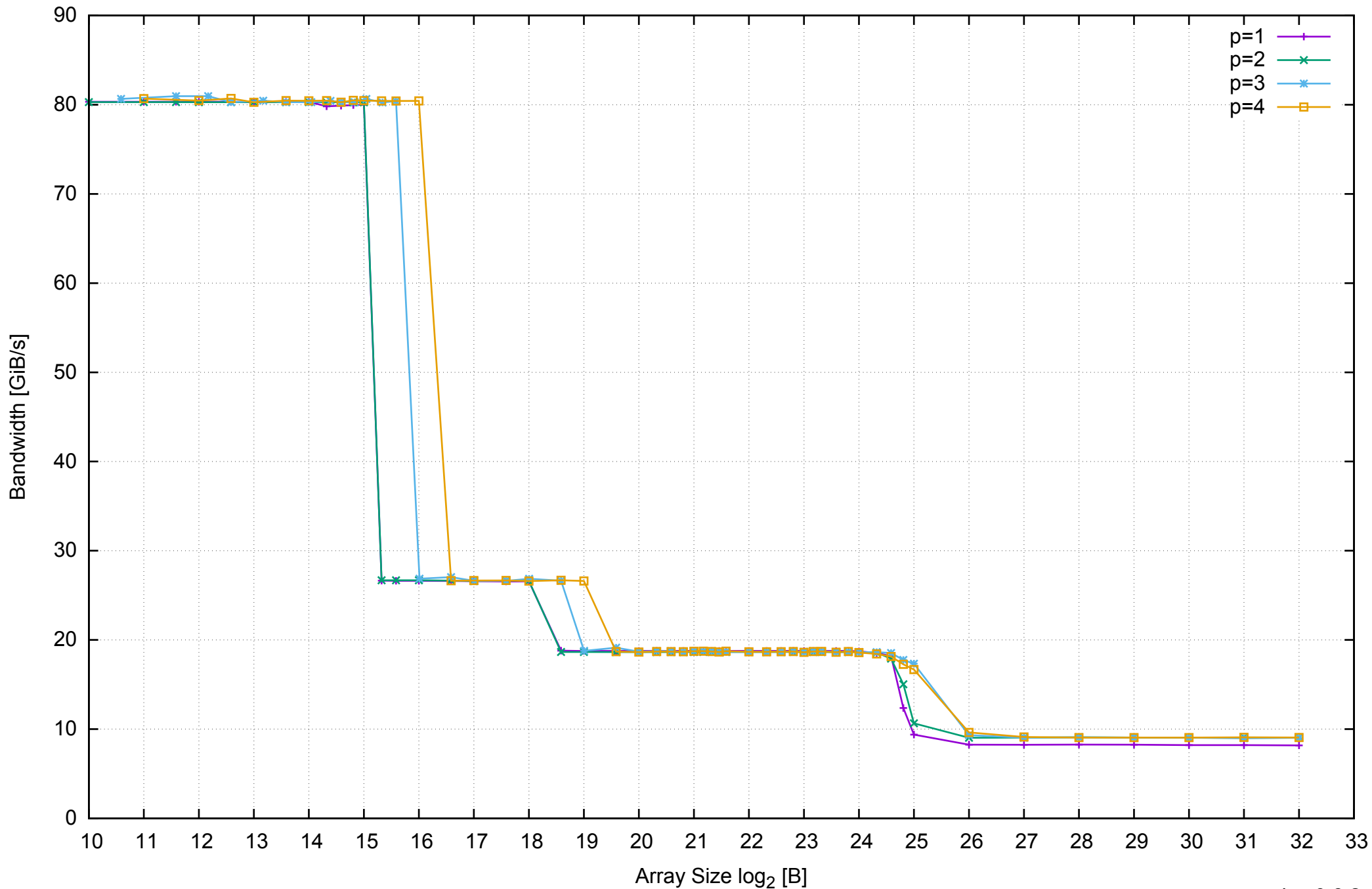
AWS m4.large - Intel Xeon E5-2676 v3, 2.40 GHz 8GB - Parallel Memory Bandwidth - ScanWrite256PtrUnrollLoop
