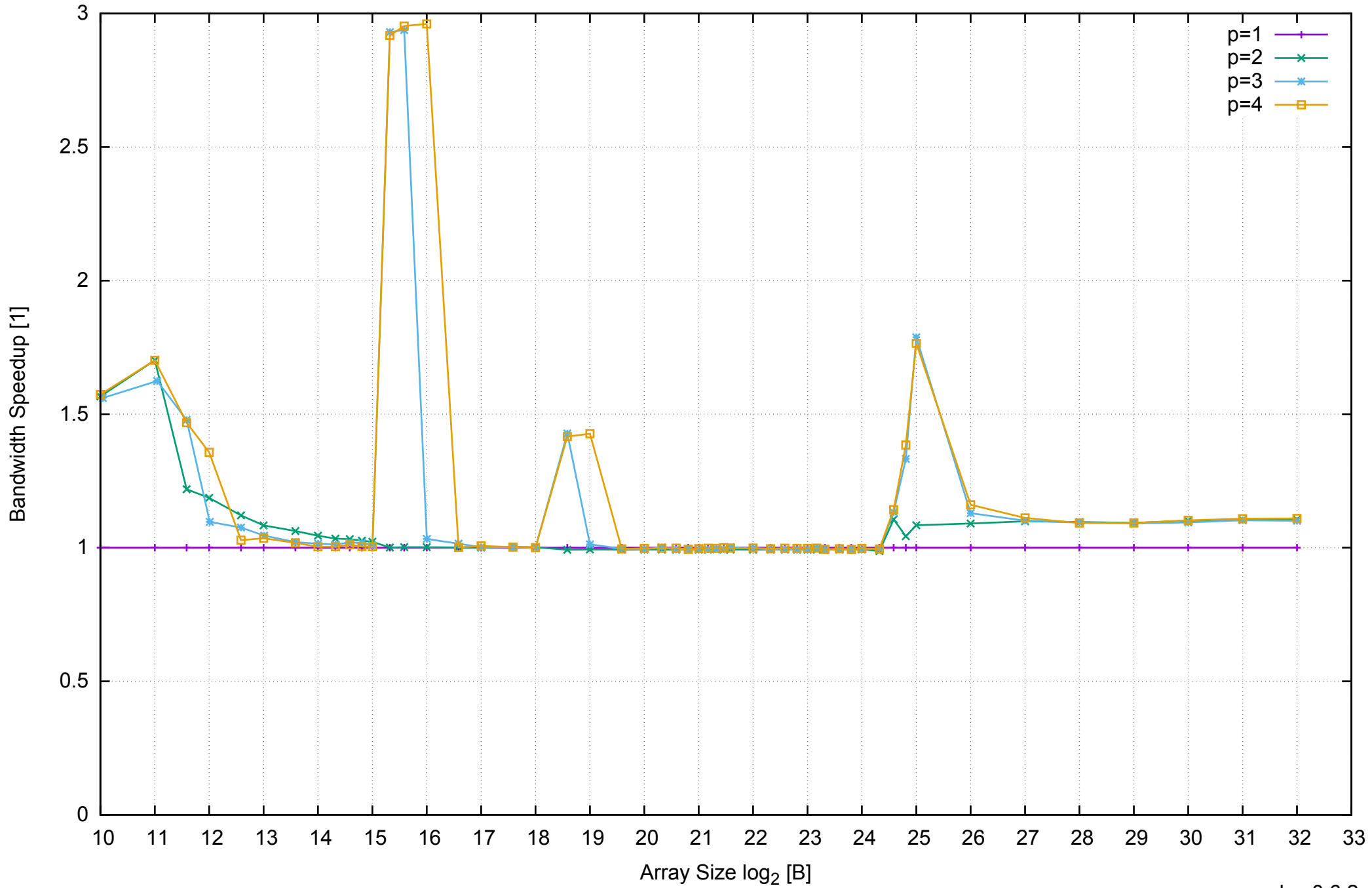
AWS m4.large - Intel Xeon E5-2676 v3, 2.40 GHz 8GB - Speedup of Parallel Memory Bandwidth - ScanWrite256PtrSimpleLoop
