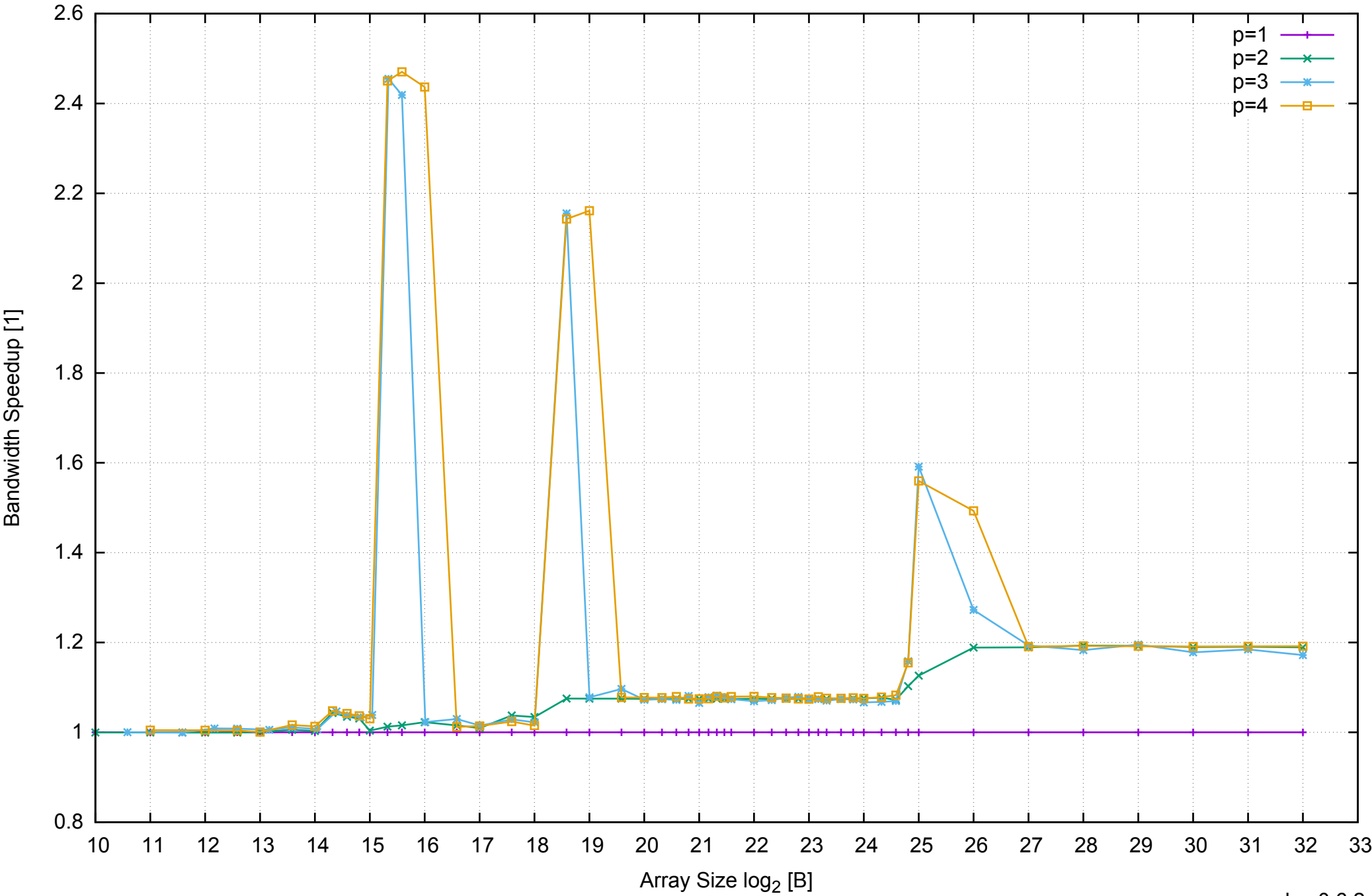
AWS m4.large - Intel Xeon E5-2676 v3, 2.40 GHz 8GB - Speedup of Parallel Memory Bandwidth - ScanRead256PtrUnrollLoop
