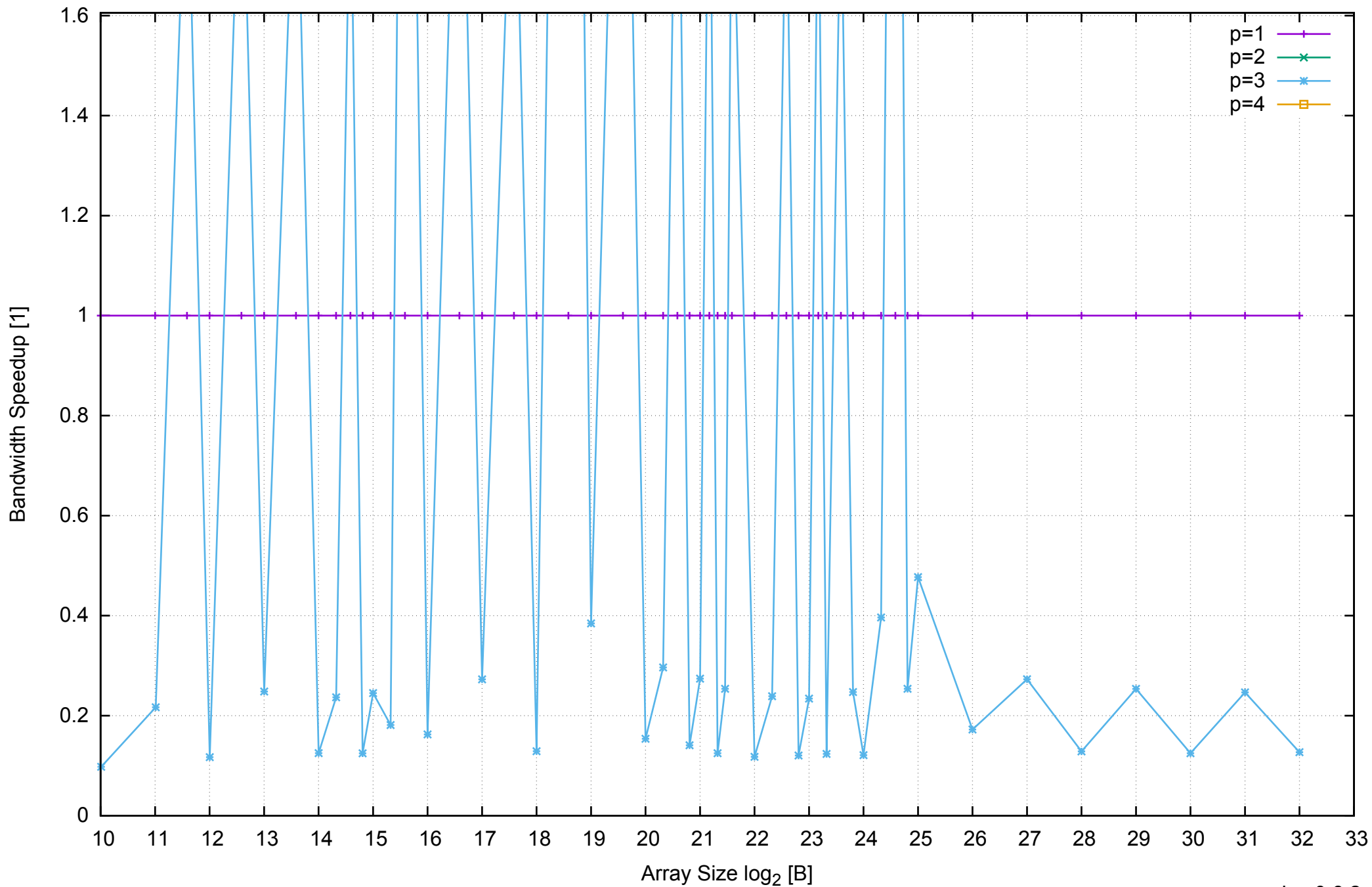
AWS m4.large - Intel Xeon E5-2676 v3, 2.40 GHz 8GB - Speedup of Parallel Memory Bandwidth (enlarged) - PermRead64UnrollLoop
