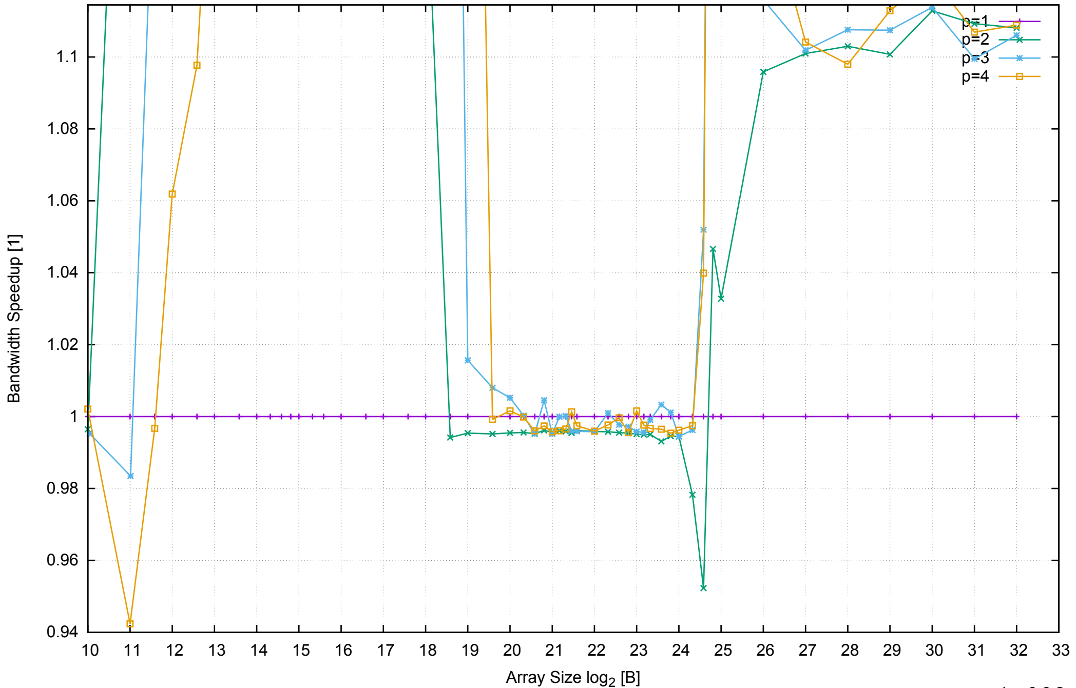
AWS m4.large - Intel Xeon E5-2676 v3, 2.40 GHz 8GB - Speedup of Parallel Memory Bandwidth (enlarged) - ScanWrite128PtrSimpleLoop
