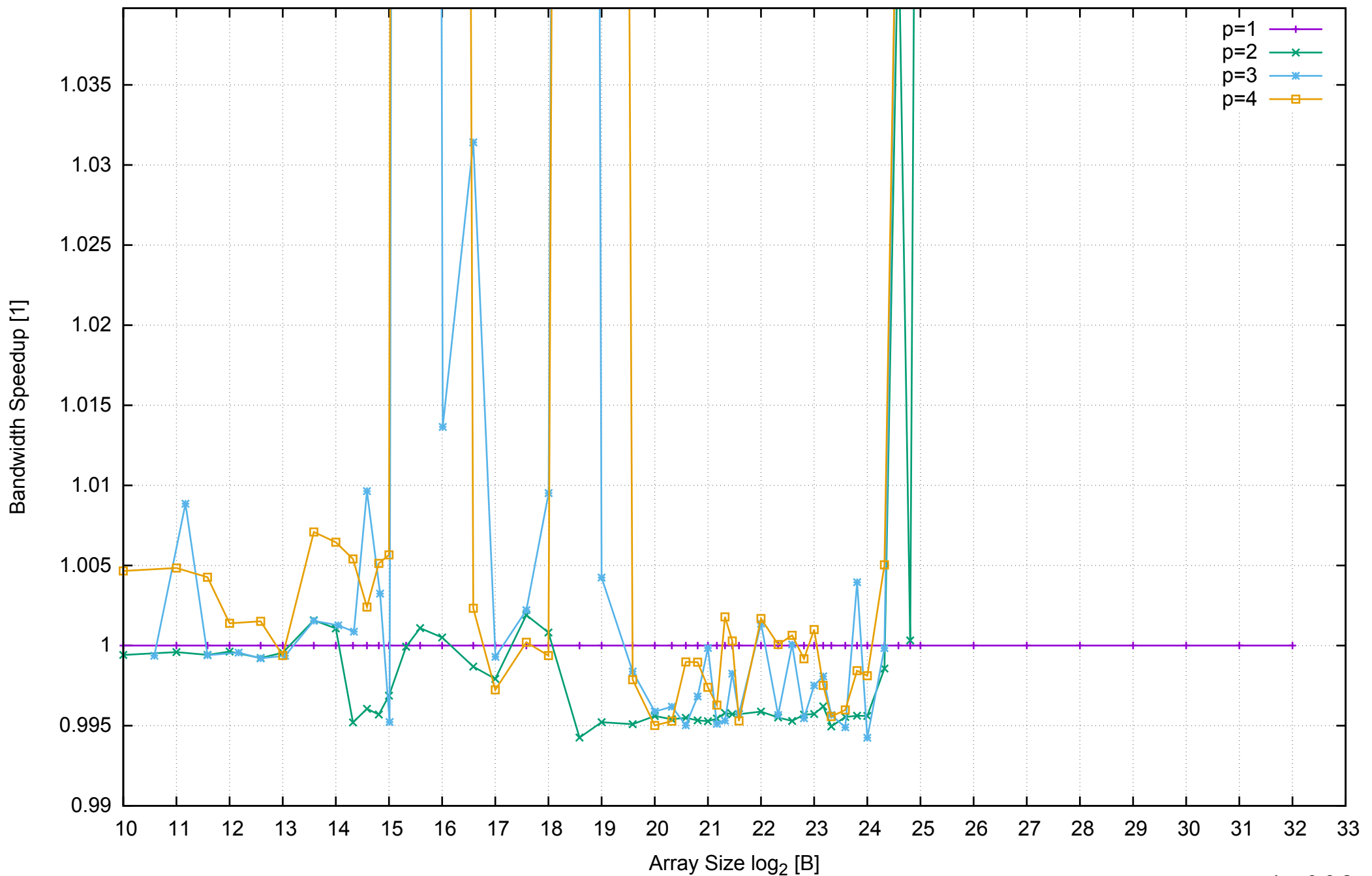
AWS m4.large - Intel Xeon E5-2676 v3, 2.40 GHz 8GB - Speedup of Parallel Memory Bandwidth (enlarged) - ScanWrite128PtrUnrollLoop
