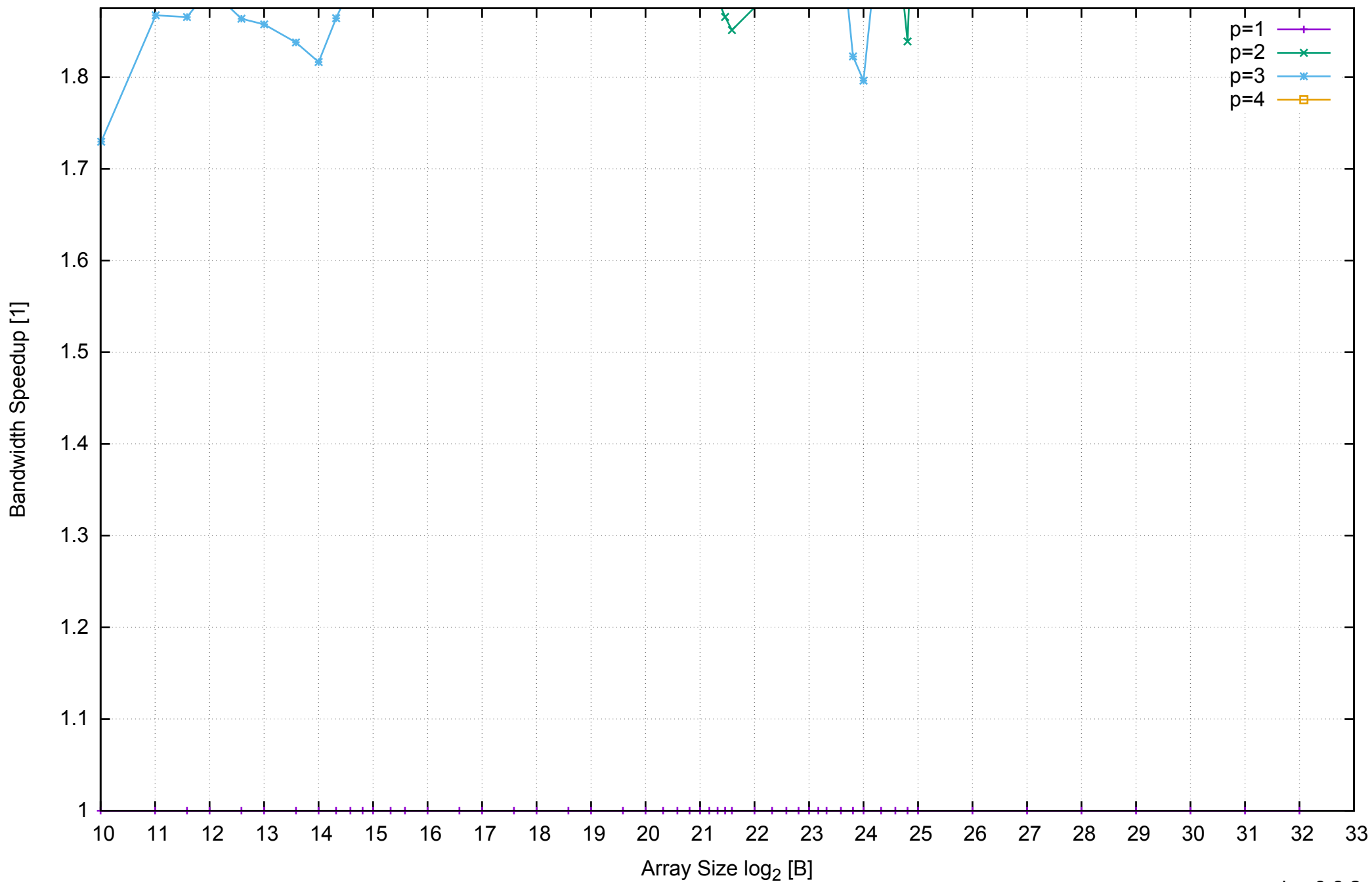
AWS m4.large - Intel Xeon E5-2676 v3, 2.40 GHz 8GB - Speedup of Parallel Memory Bandwidth (enlarged) - PermRead64SimpleLoop
