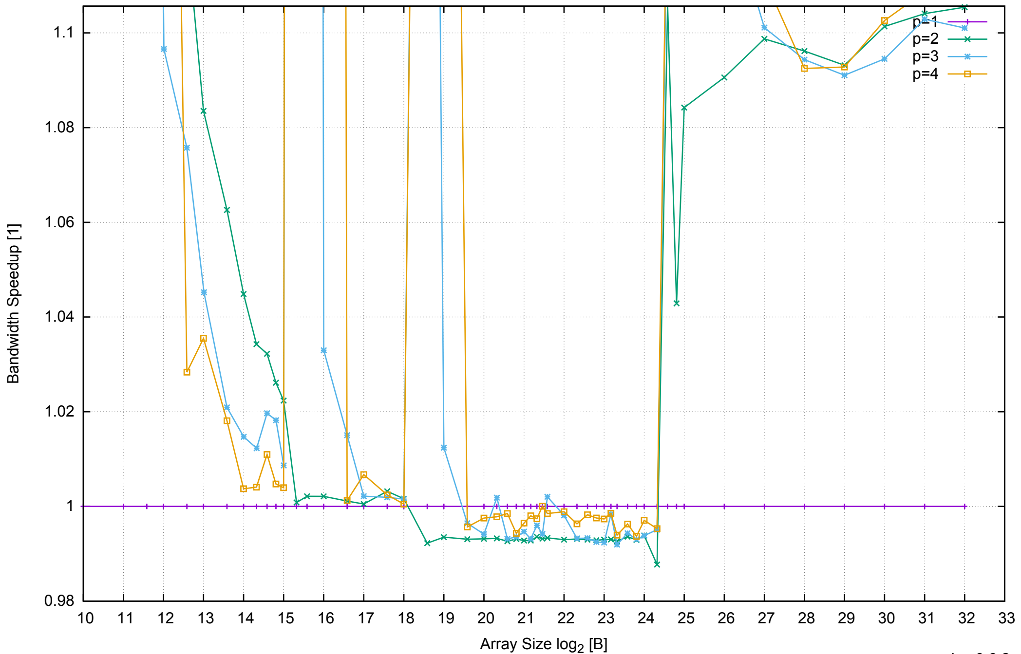
AWS m4.large - Intel Xeon E5-2676 v3, 2.40 GHz 8GB - Speedup of Parallel Memory Bandwidth (enlarged) - ScanWrite256PtrSimpleLoop
