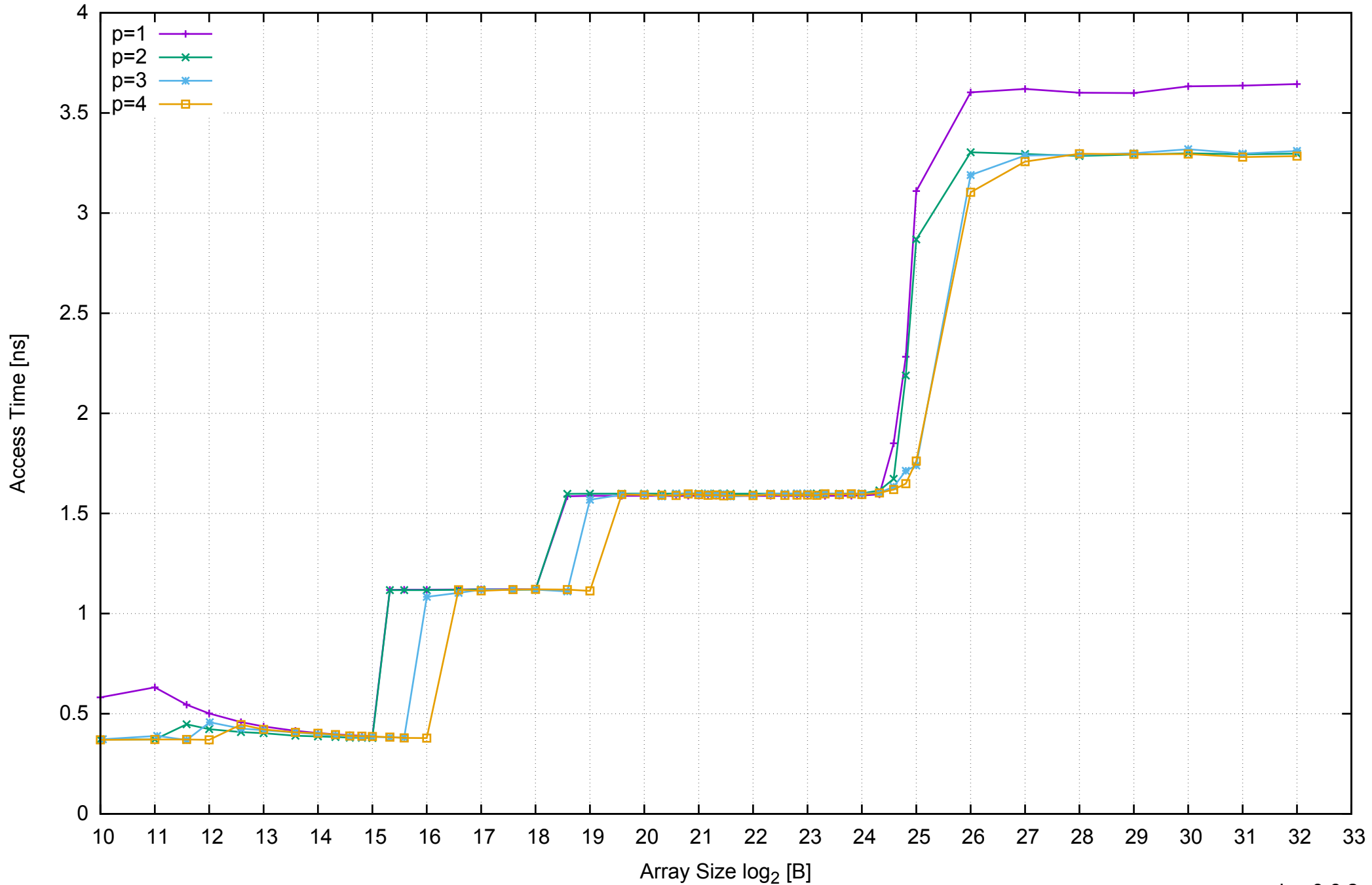
AWS m4.large - Intel Xeon E5-2676 v3, 2.40 GHz 8GB - Parallel Memory Access Time - ScanWrite256PtrSimpleLoop
