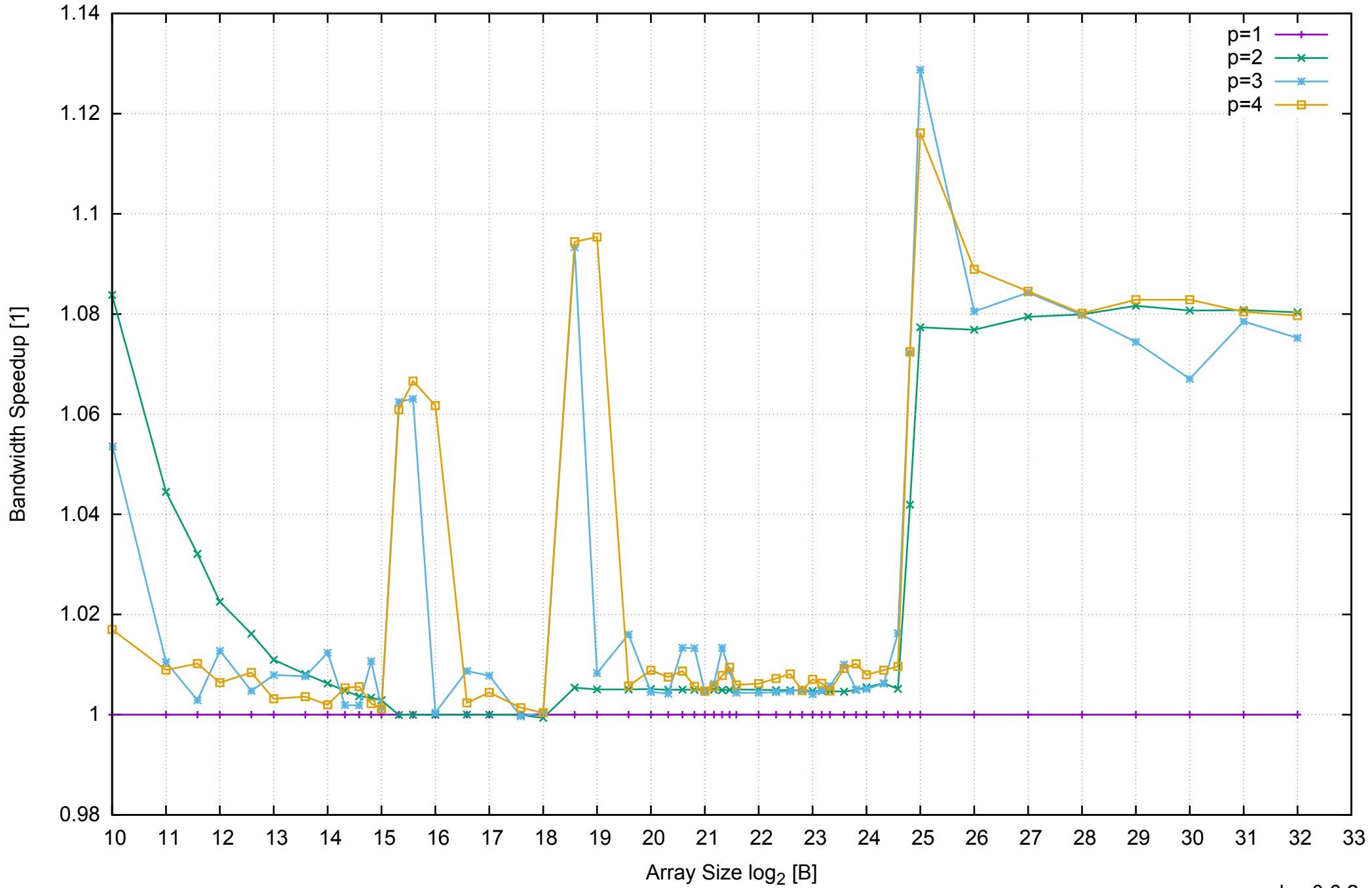
AWS m4.large - Intel Xeon E5-2676 v3, 2.40 GHz 8GB - Speedup of Parallel Memory Bandwidth - ScanWrite32PtrSimpleLoop
