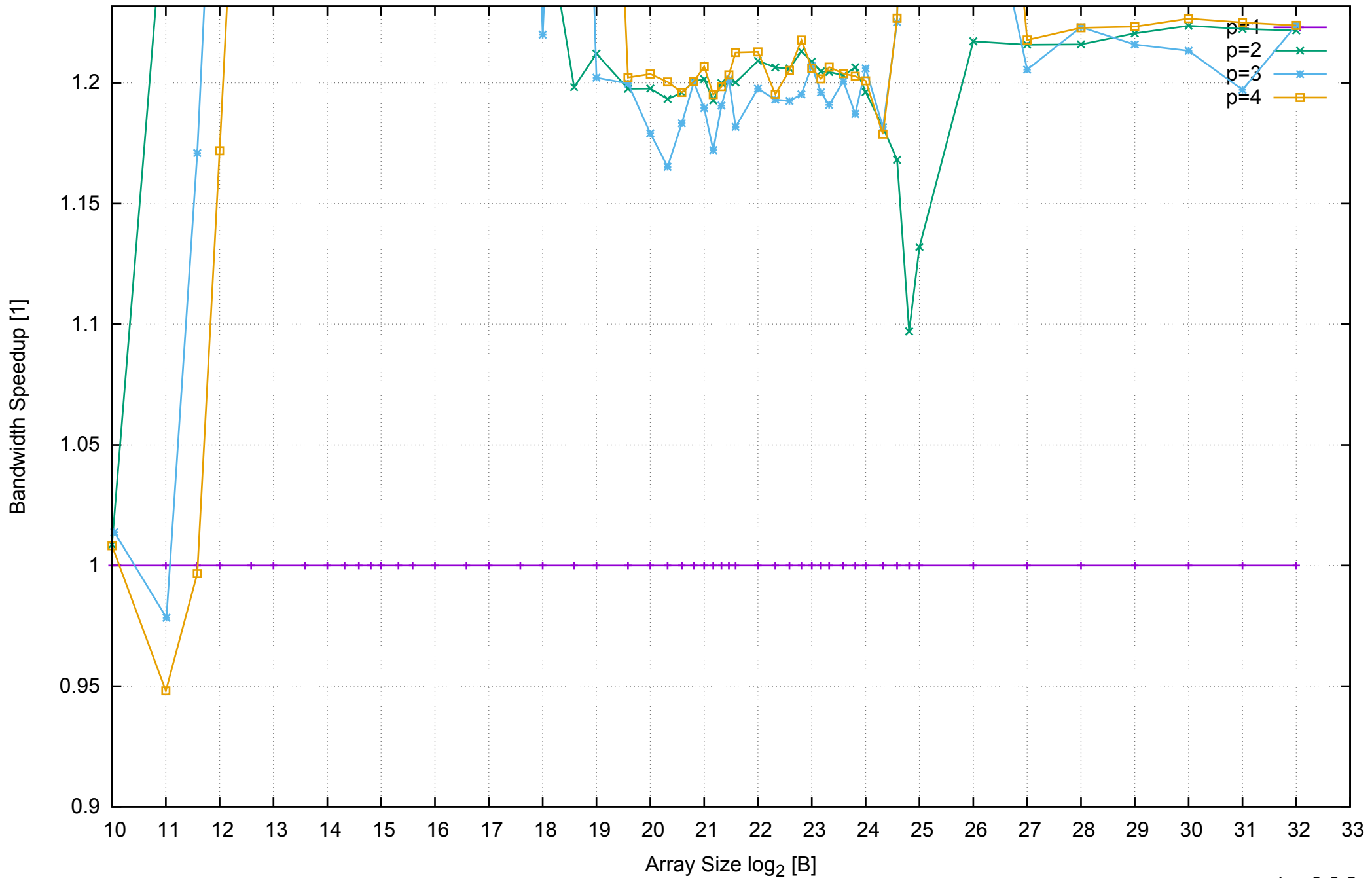
AWS m4.large - Intel Xeon E5-2676 v3, 2.40 GHz 8GB - Speedup of Parallel Memory Bandwidth (enlarged) - ScanRead128PtrSimpleLoop
