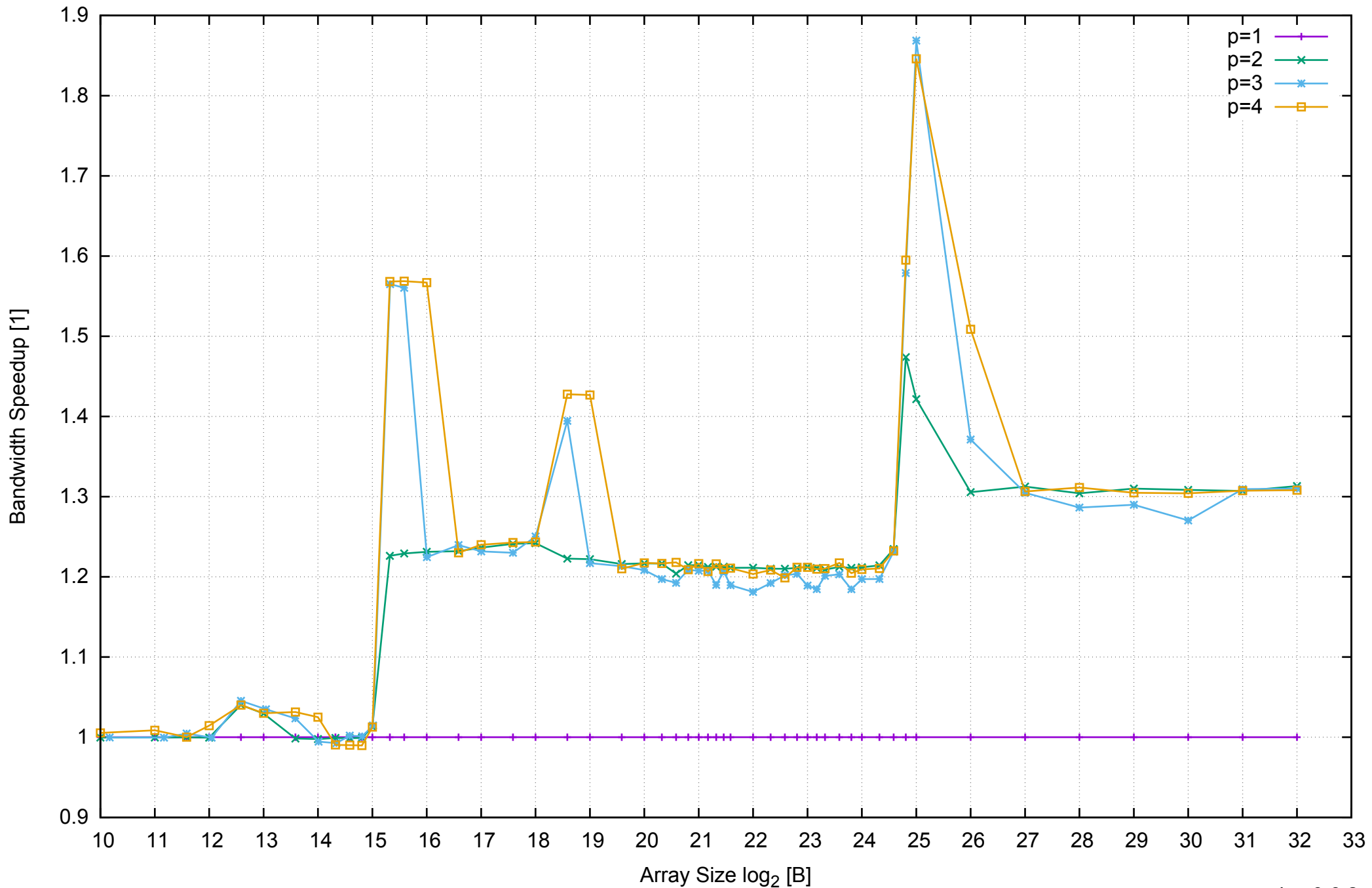
AWS m4.large - Intel Xeon E5-2676 v3, 2.40 GHz 8GB - Speedup of Parallel Memory Bandwidth - ScanRead64IndexUnrollLoop
