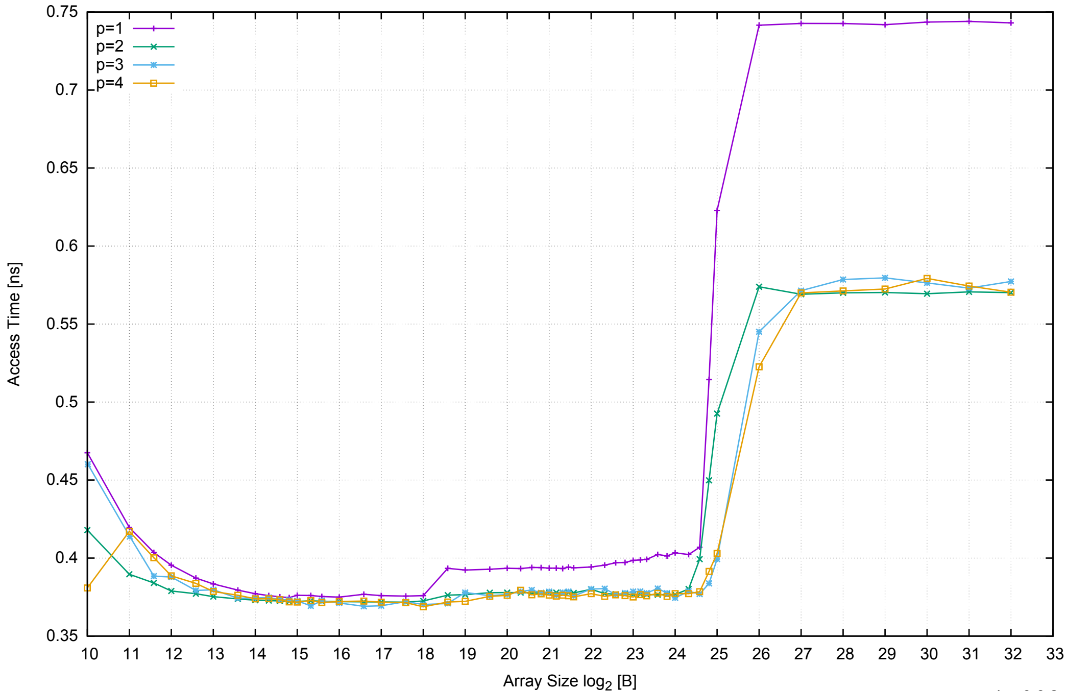
AWS m4.large - Intel Xeon E5-2676 v3, 2.40 GHz 8GB - Parallel Memory Access Time - ScanRead64IndexSimpleLoop
