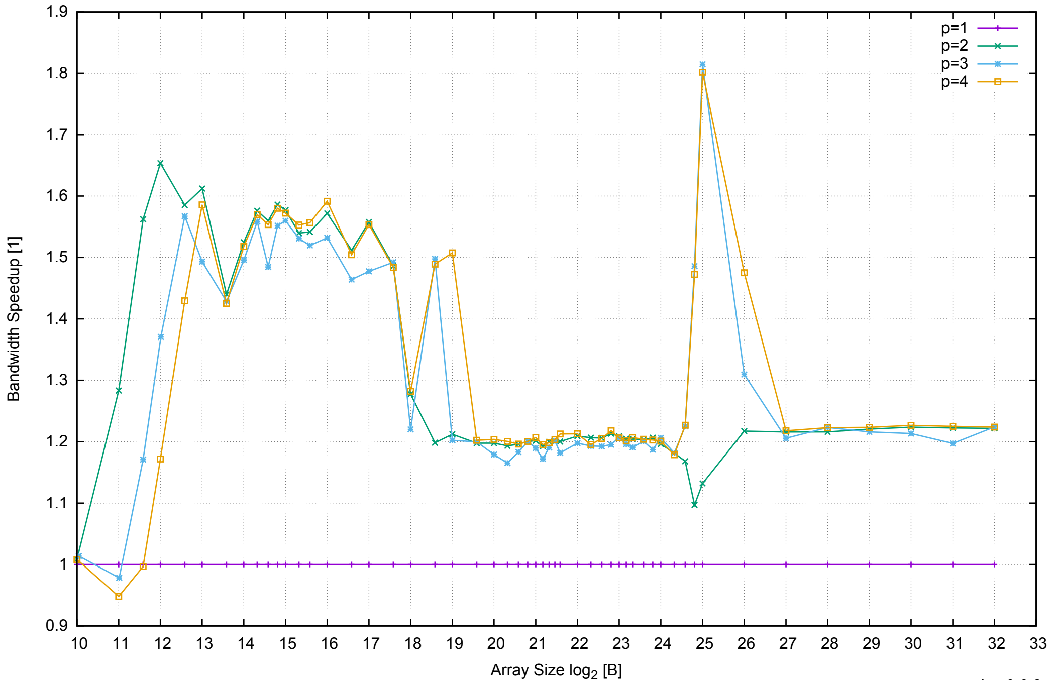
AWS m4.large - Intel Xeon E5-2676 v3, 2.40 GHz 8GB - Speedup of Parallel Memory Bandwidth - ScanRead128PtrSimpleLoop
