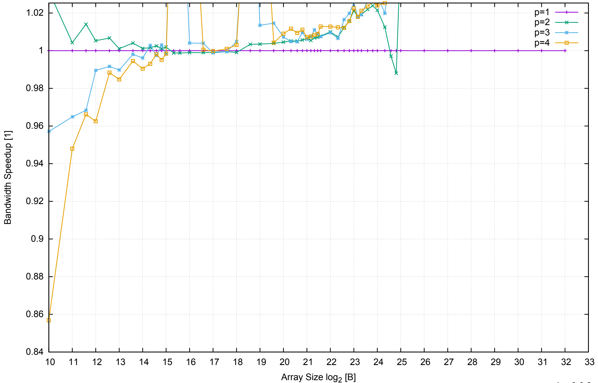
AWS m4.large - Intel Xeon E5-2676 v3, 2.40 GHz 8GB - Speedup of Parallel Memory Bandwidth (enlarged) - ScanWrite64PtrSimpleLoop
