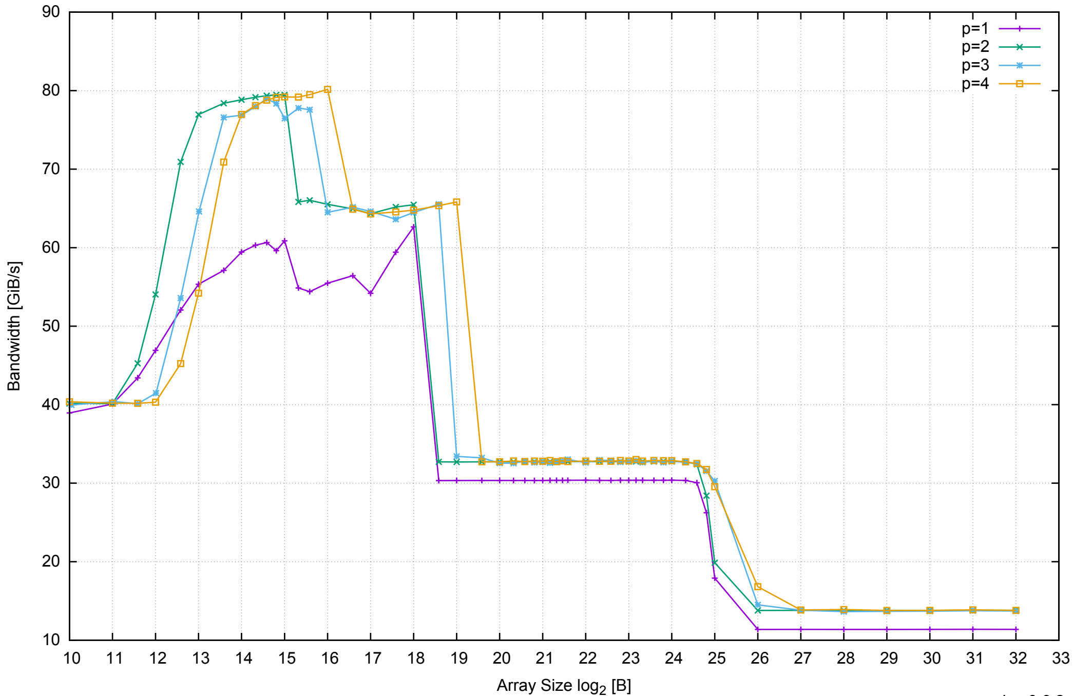
AWS m4.large - Intel Xeon E5-2676 v3, 2.40 GHz 8GB - Parallel Memory Bandwidth - ScanRead256PtrSimpleLoop
