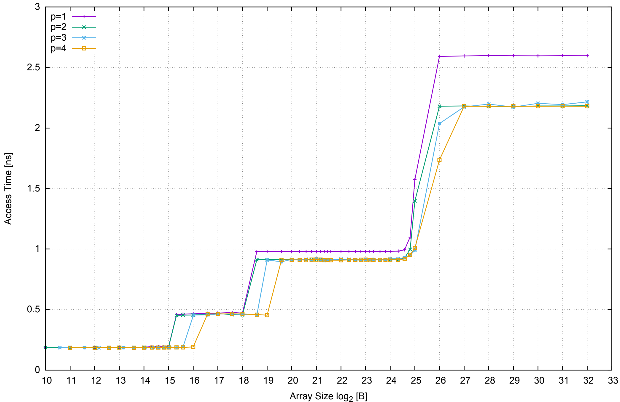
AWS m4.large - Intel Xeon E5-2676 v3, 2.40 GHz 8GB - Parallel Memory Access Time - ScanRead256PtrUnrollLoop
