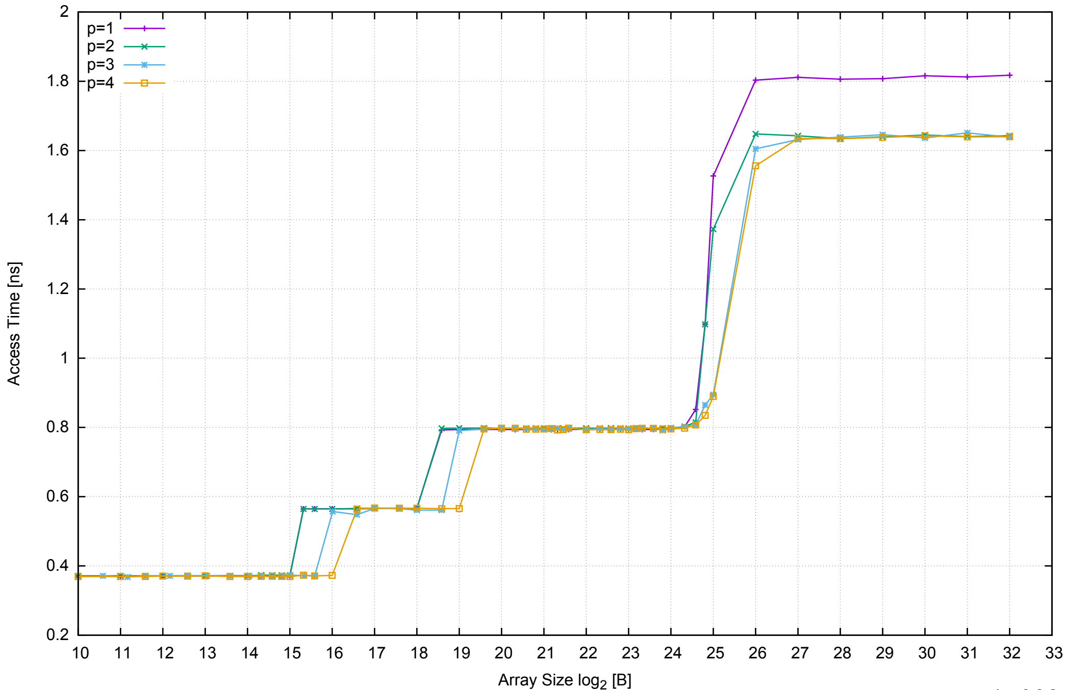
AWS m4.large - Intel Xeon E5-2676 v3, 2.40 GHz 8GB - Parallel Memory Access Time - ScanWrite128PtrUnrollLoop
