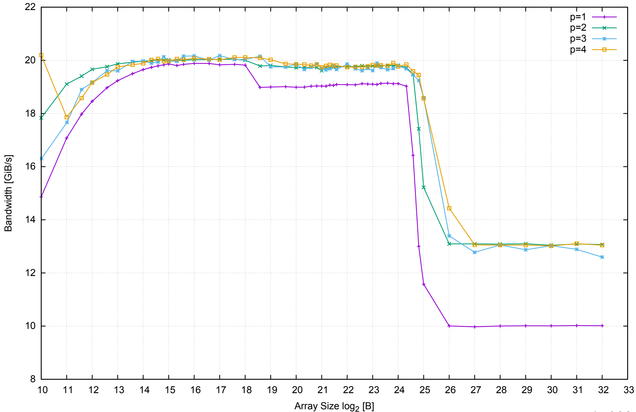
AWS m4.large - Intel Xeon E5-2676 v3, 2.40 GHz 8GB - Parallel Memory Bandwidth - ScanRead64PtrSimpleLoop
