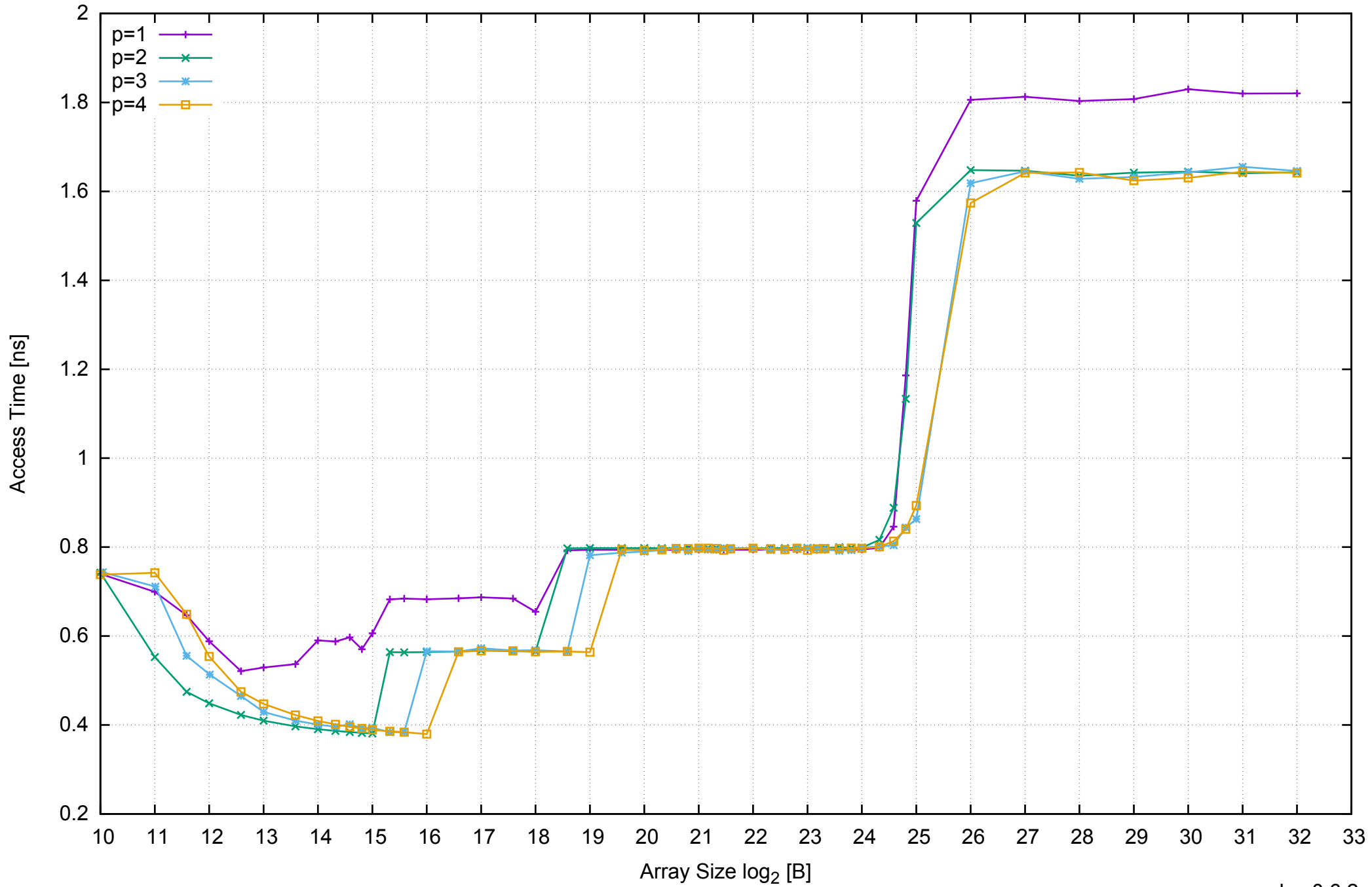
AWS m4.large - Intel Xeon E5-2676 v3, 2.40 GHz 8GB - Parallel Memory Access Time - ScanWrite128PtrSimpleLoop
