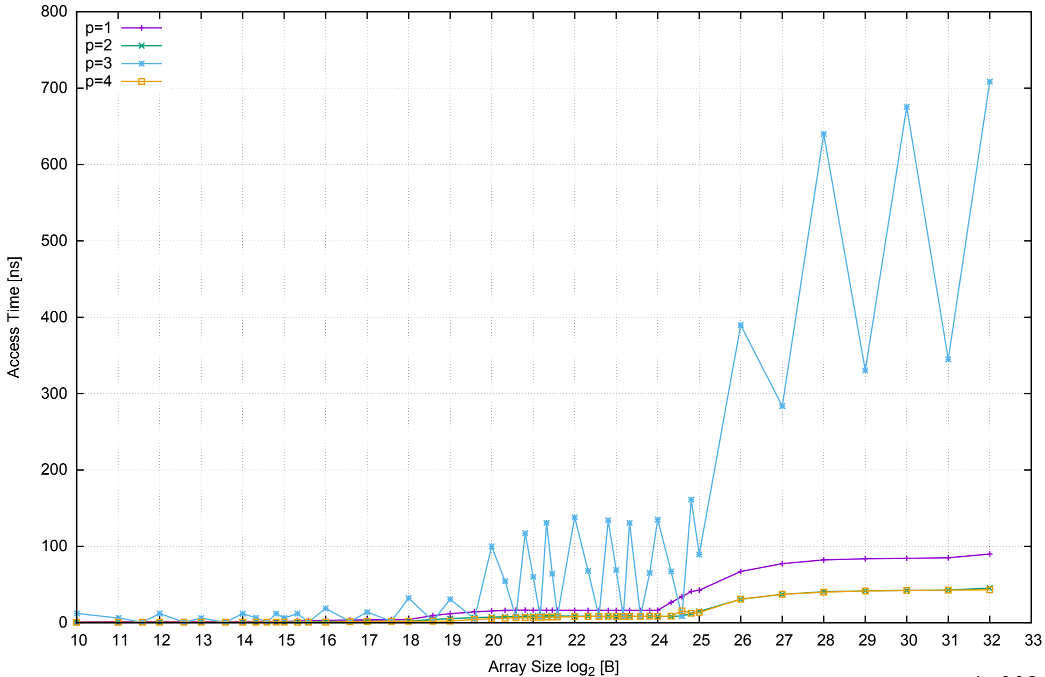
AWS m4.large - Intel Xeon E5-2676 v3, 2.40 GHz 8GB - Parallel Memory Access Time - PermRead64UnrollLoop
