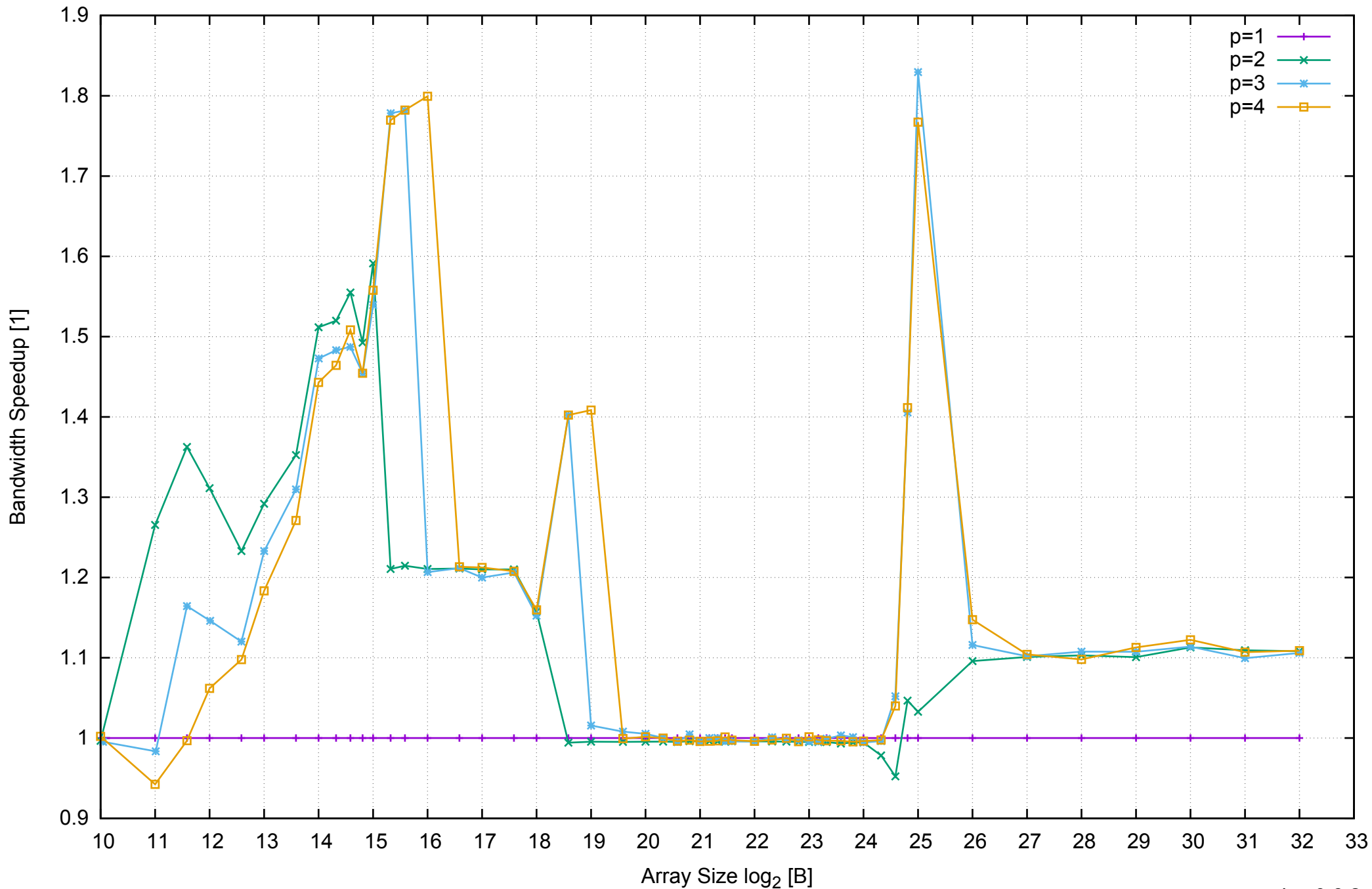
AWS m4.large - Intel Xeon E5-2676 v3, 2.40 GHz 8GB - Speedup of Parallel Memory Bandwidth - ScanWrite128PtrSimpleLoop
