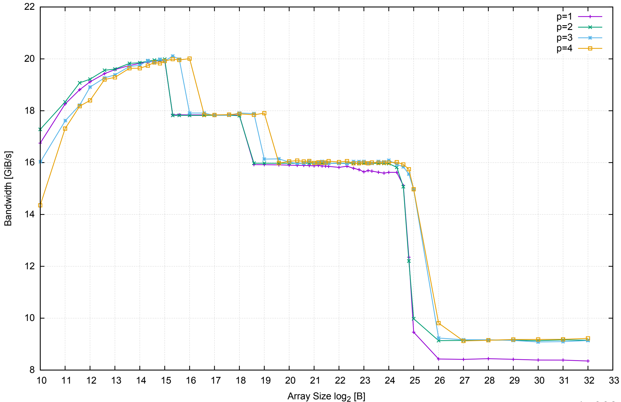
AWS m4.large - Intel Xeon E5-2676 v3, 2.40 GHz 8GB - Parallel Memory Bandwidth - ScanWrite64PtrSimpleLoop
