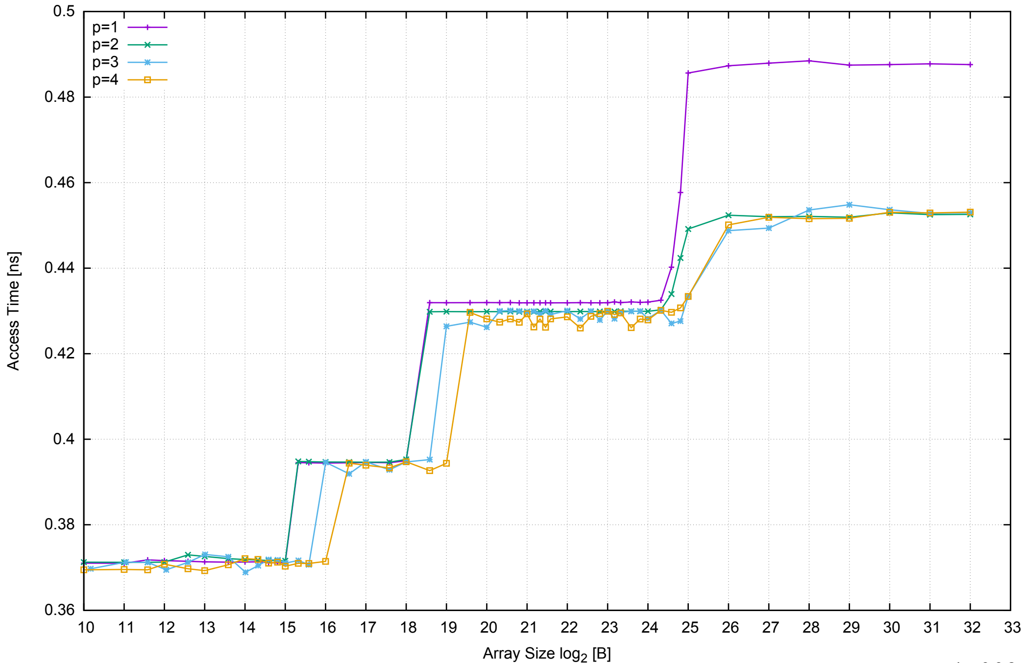
AWS m4.large - Intel Xeon E5-2676 v3, 2.40 GHz 8GB - Parallel Memory Access Time - ScanWrite32PtrUnrollLoop
