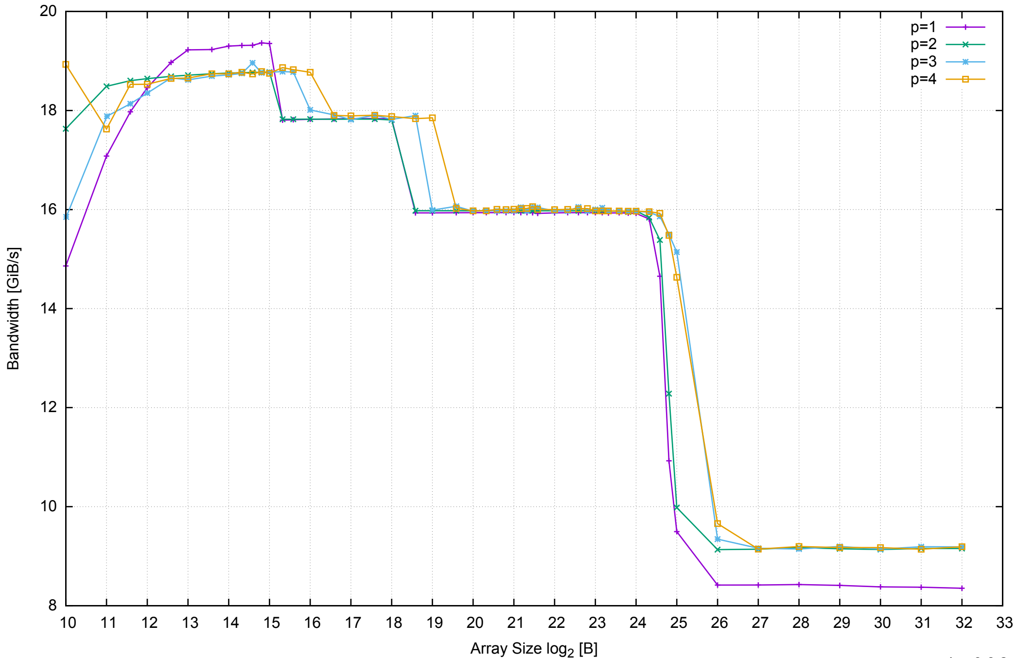
AWS m4.large - Intel Xeon E5-2676 v3, 2.40 GHz 8GB - Parallel Memory Bandwidth - ScanWrite64IndexSimpleLoop
