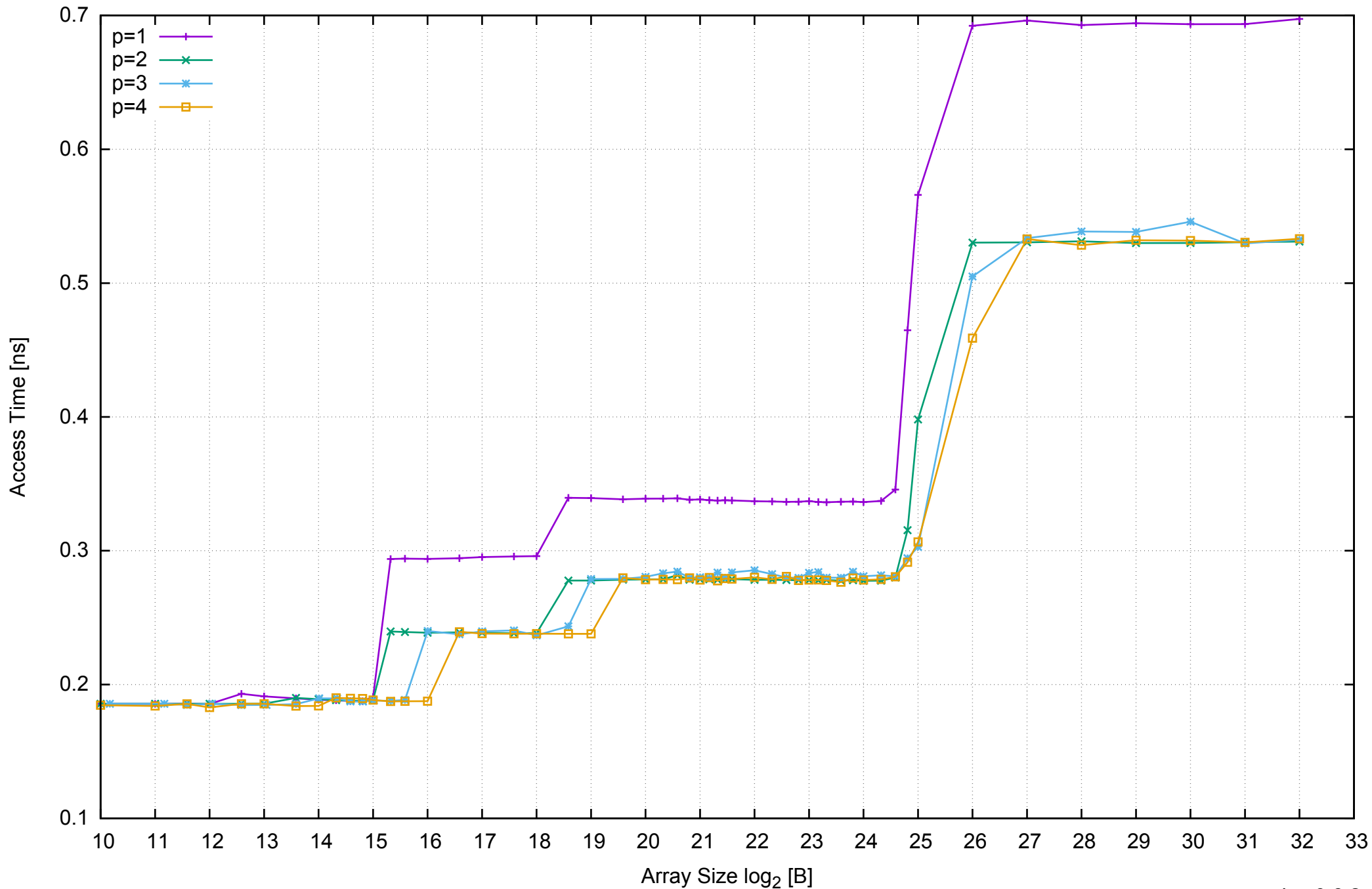
AWS m4.large - Intel Xeon E5-2676 v3, 2.40 GHz 8GB - Parallel Memory Access Time - ScanRead64IndexUnrollLoop
