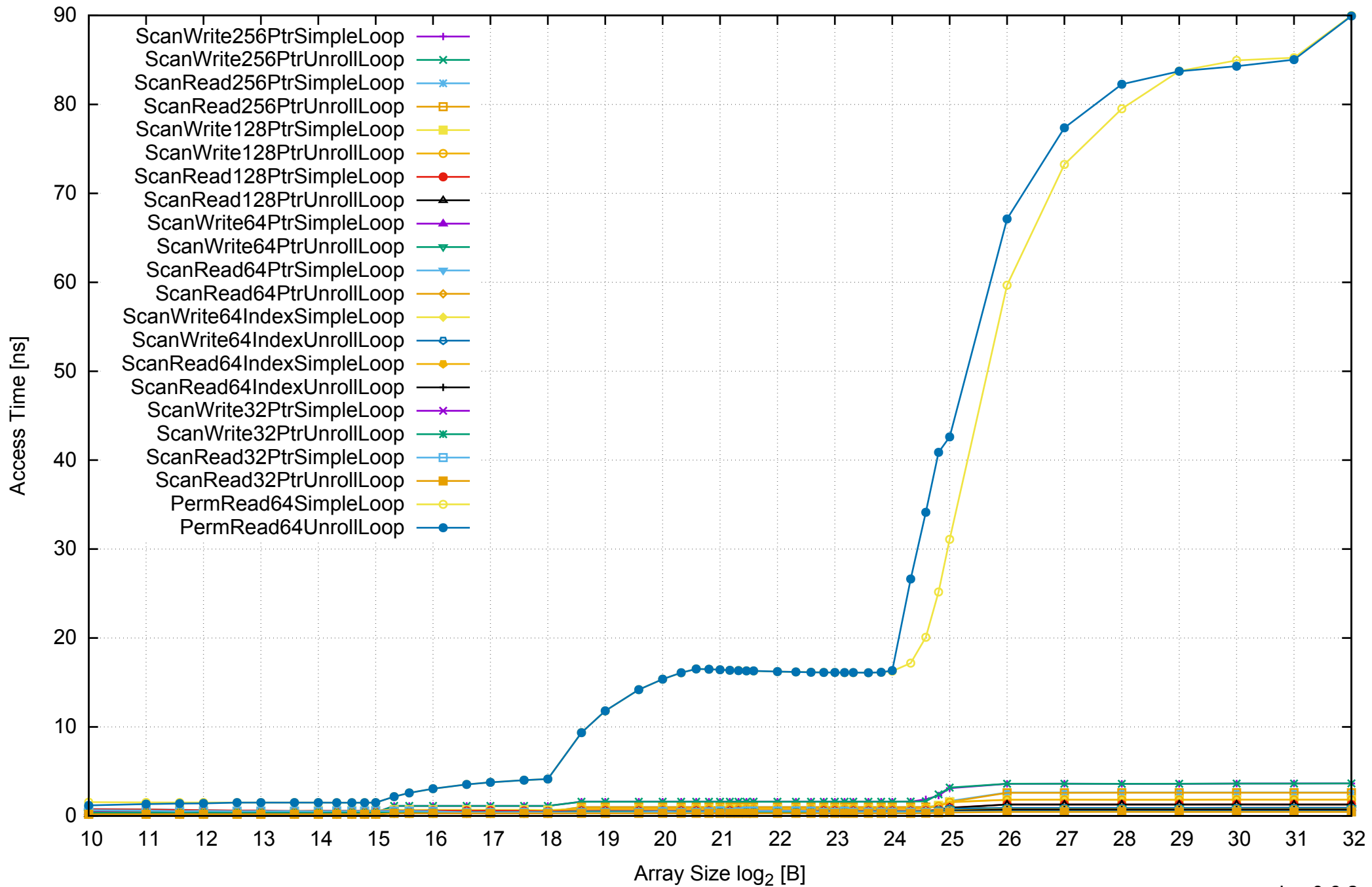
AWS m4.large - Intel Xeon E5-2676 v3, 2.40 GHz 8GB - One Thread Memory Latency (Access Time)
