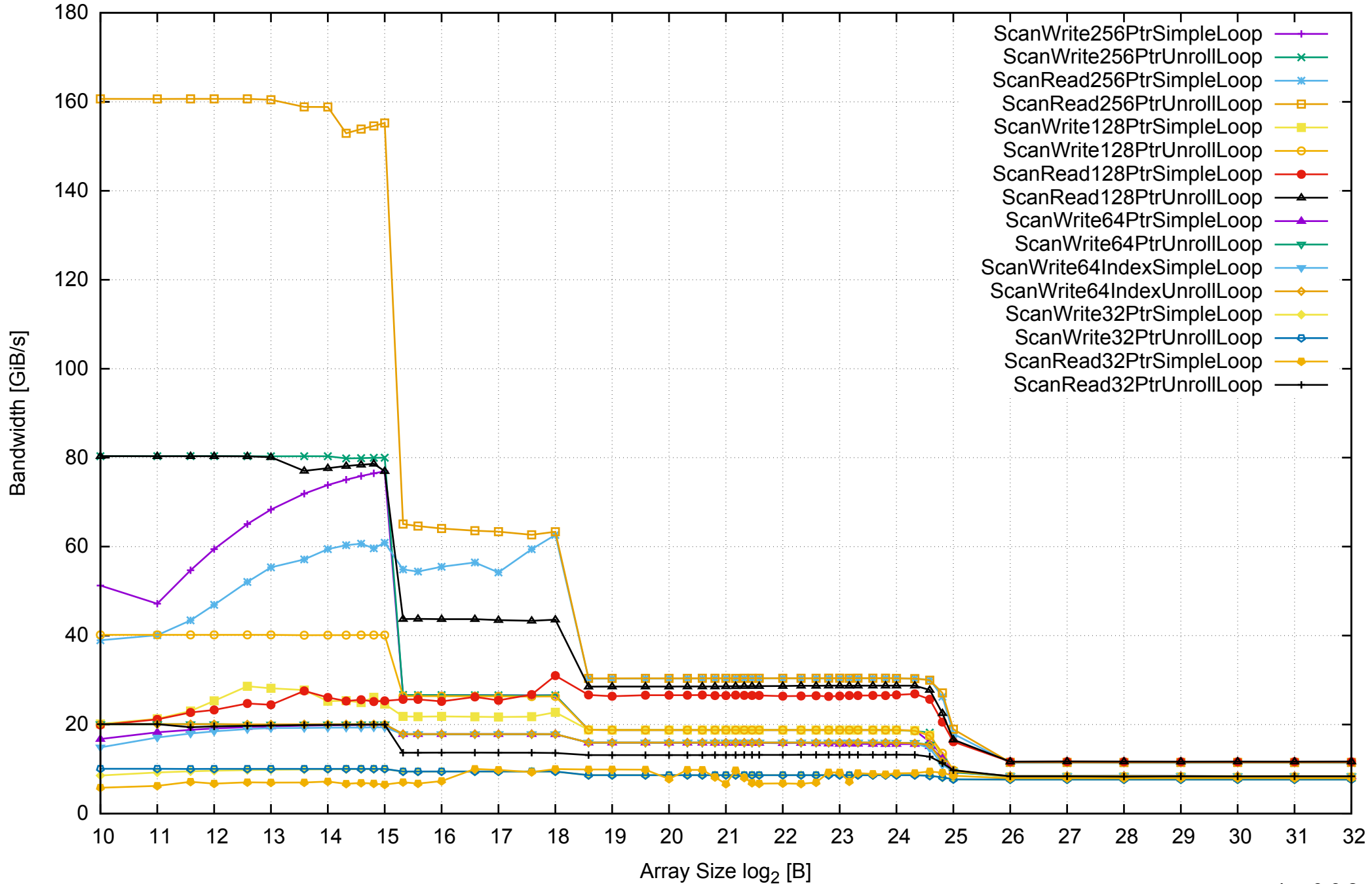
AWS m4.large - Intel Xeon E5-2676 v3, 2.40 GHz 8GB - One Thread Memory Bandwidth (only 64-bit Reads)
