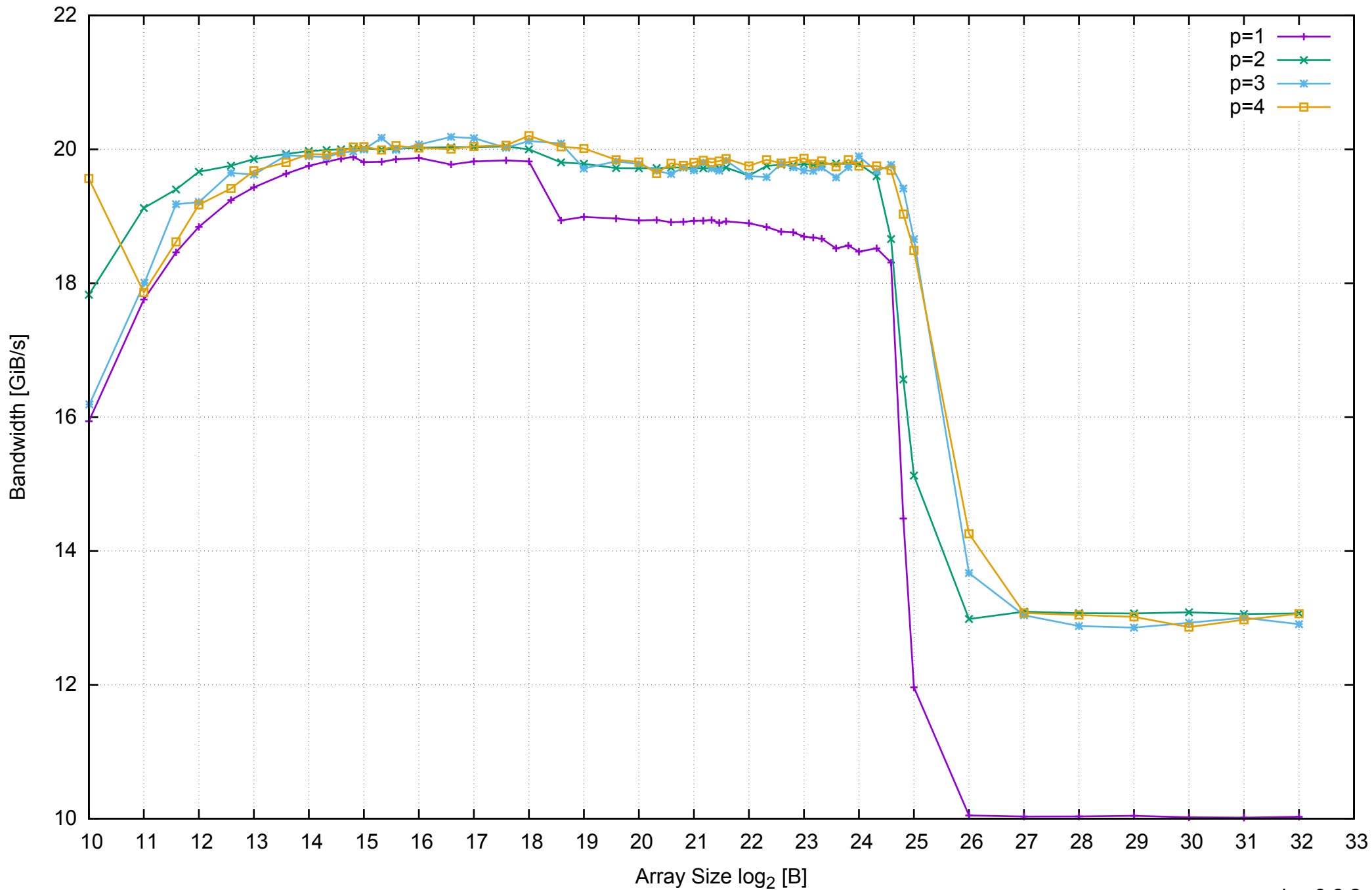
AWS m4.large - Intel Xeon E5-2676 v3, 2.40 GHz 8GB - Parallel Memory Bandwidth - ScanRead64IndexSimpleLoop
