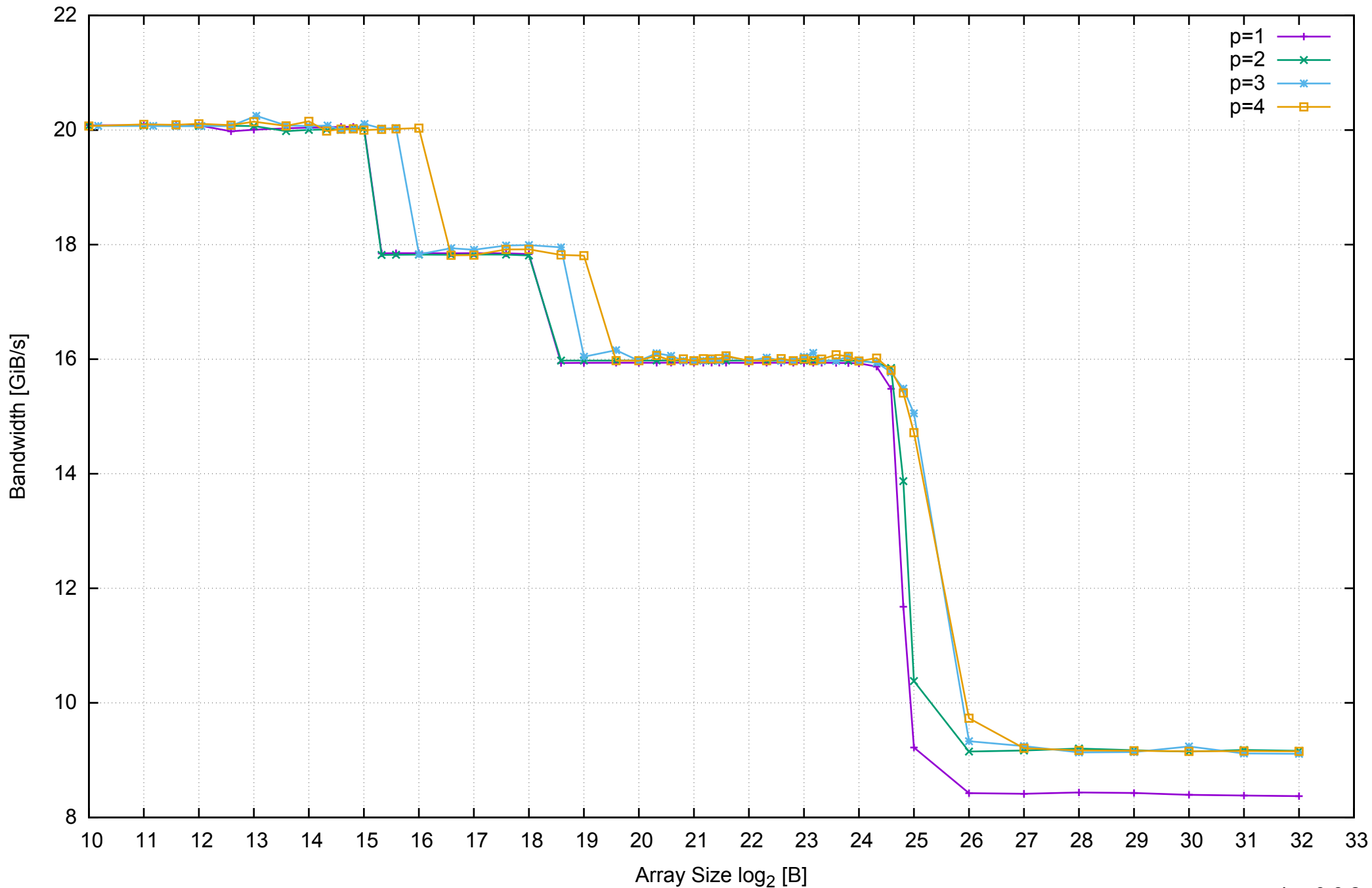
AWS m4.large - Intel Xeon E5-2676 v3, 2.40 GHz 8GB - Parallel Memory Bandwidth - ScanWrite64PtrUnrollLoop
