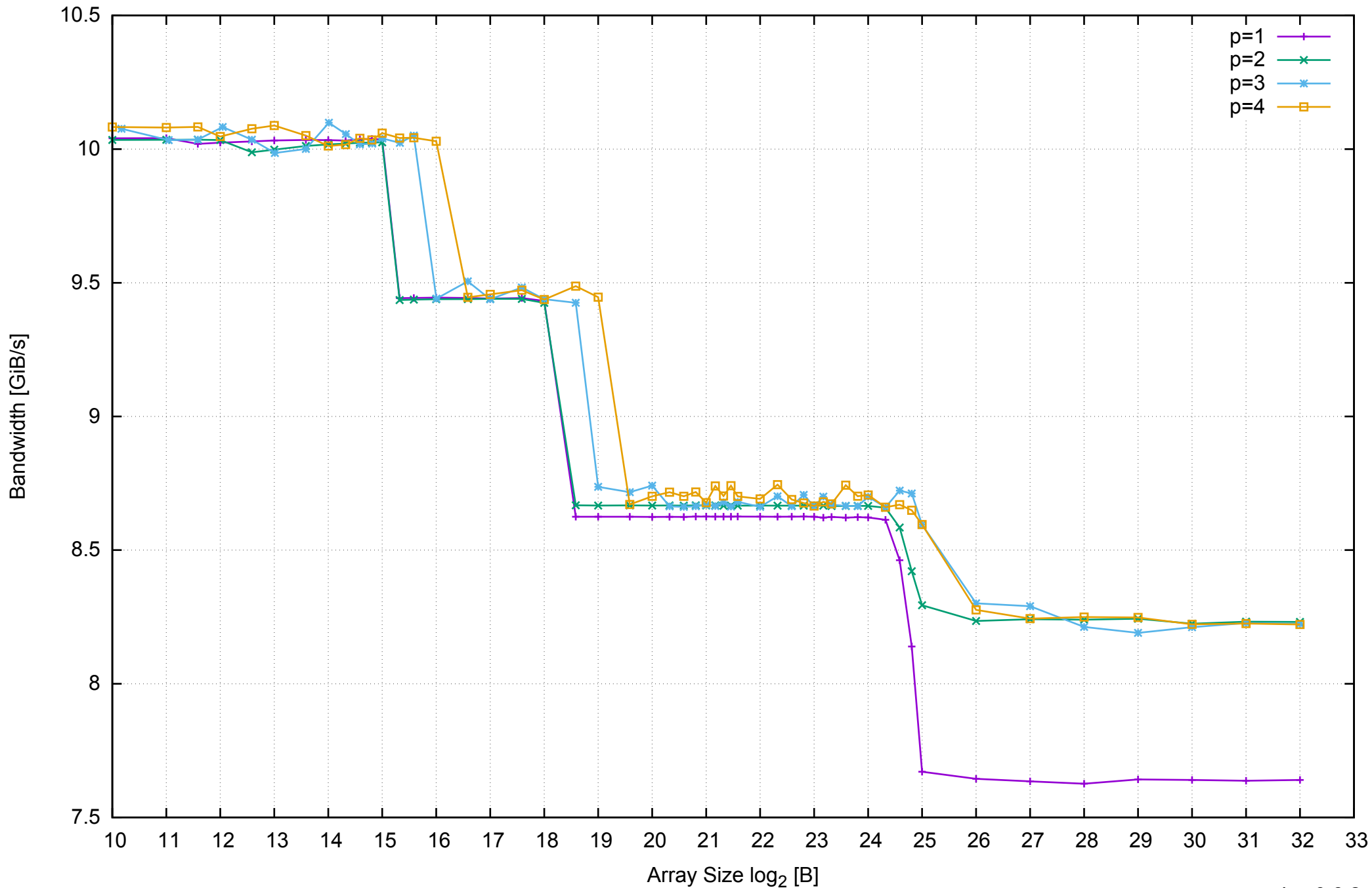
AWS m4.large - Intel Xeon E5-2676 v3, 2.40 GHz 8GB - Parallel Memory Bandwidth - ScanWrite32PtrUnrollLoop
