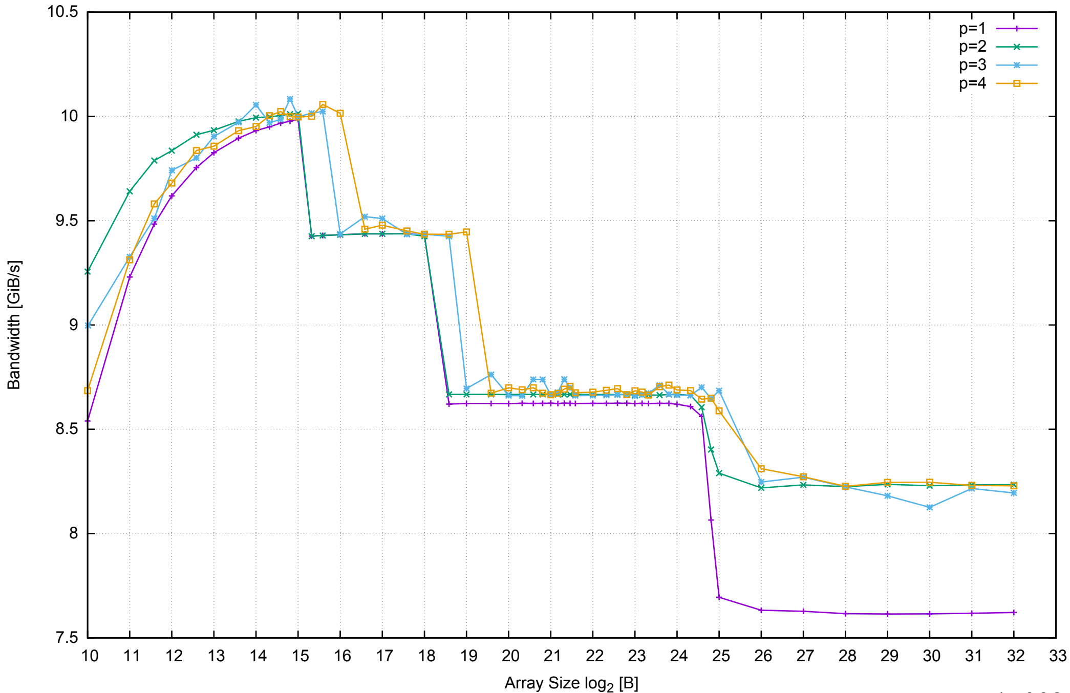
AWS m4.large - Intel Xeon E5-2676 v3, 2.40 GHz 8GB - Parallel Memory Bandwidth - ScanWrite32PtrSimpleLoop
