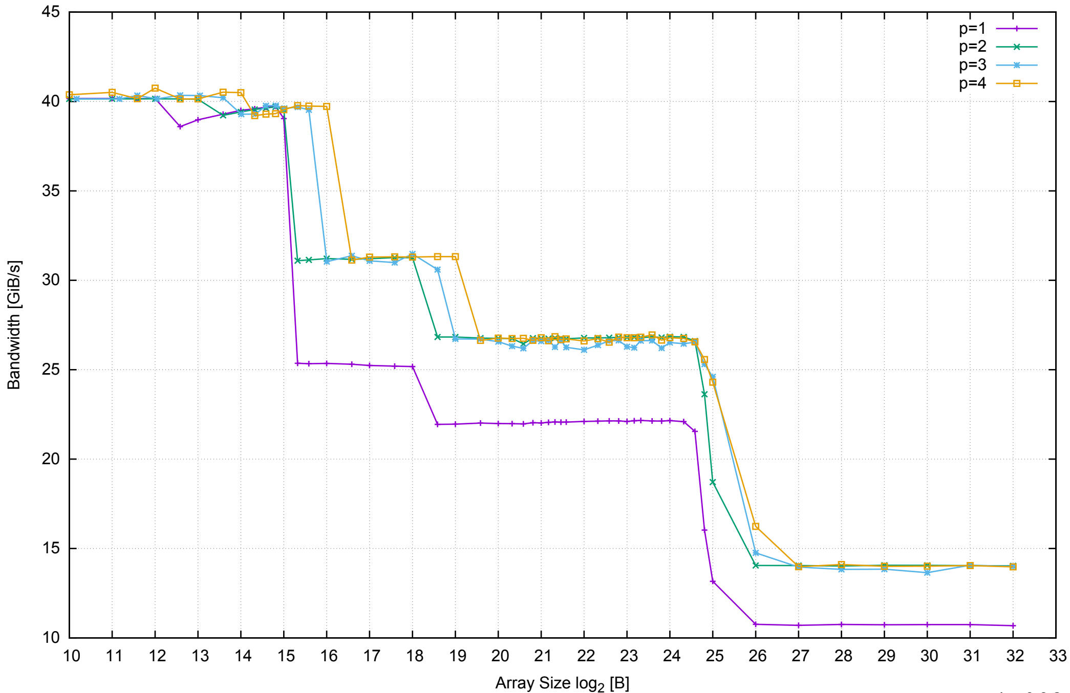
AWS m4.large - Intel Xeon E5-2676 v3, 2.40 GHz 8GB - Parallel Memory Bandwidth - ScanRead64IndexUnrollLoop
