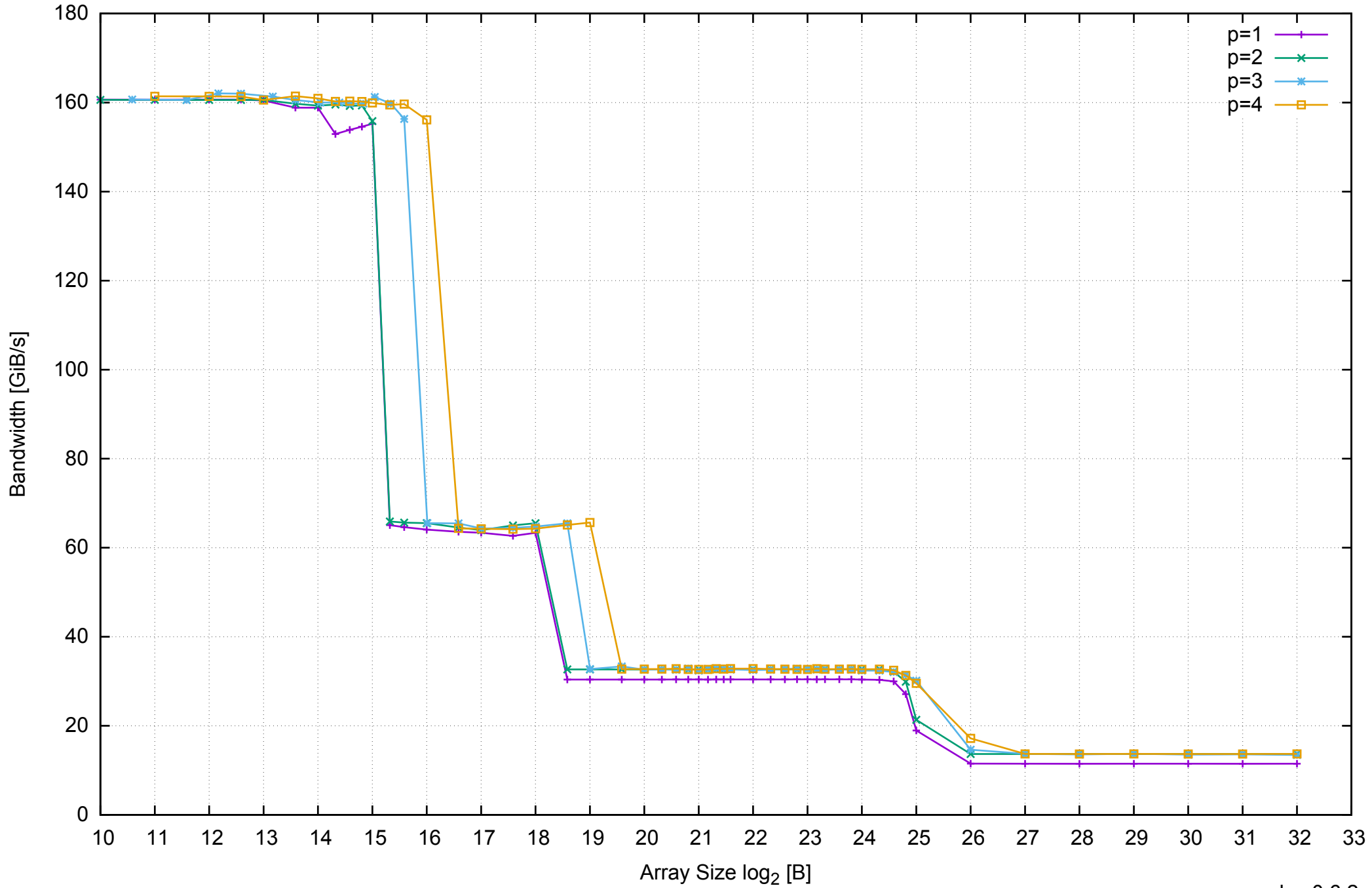
AWS m4.large - Intel Xeon E5-2676 v3, 2.40 GHz 8GB - Parallel Memory Bandwidth - ScanRead256PtrUnrollLoop
