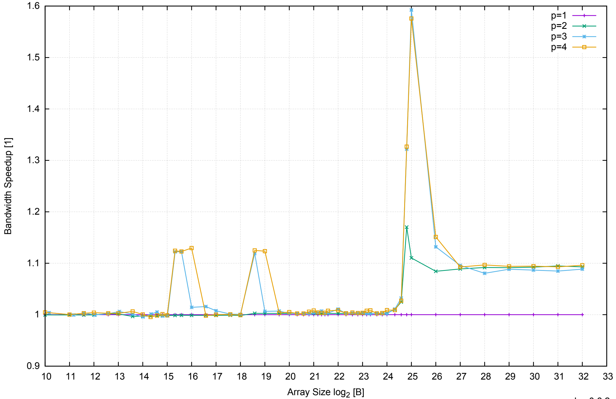
AWS m4.large - Intel Xeon E5-2676 v3, 2.40 GHz 8GB - Speedup of Parallel Memory Bandwidth - ScanWrite64IndexUnrollLoop
