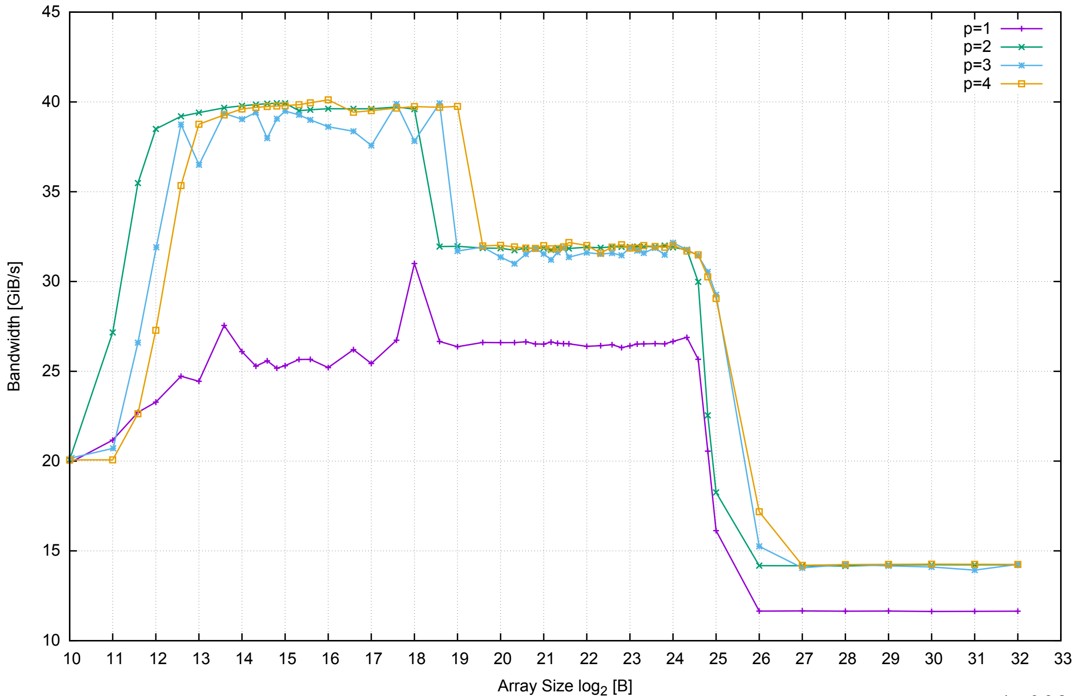
AWS m4.large - Intel Xeon E5-2676 v3, 2.40 GHz 8GB - Parallel Memory Bandwidth - ScanRead128PtrSimpleLoop
