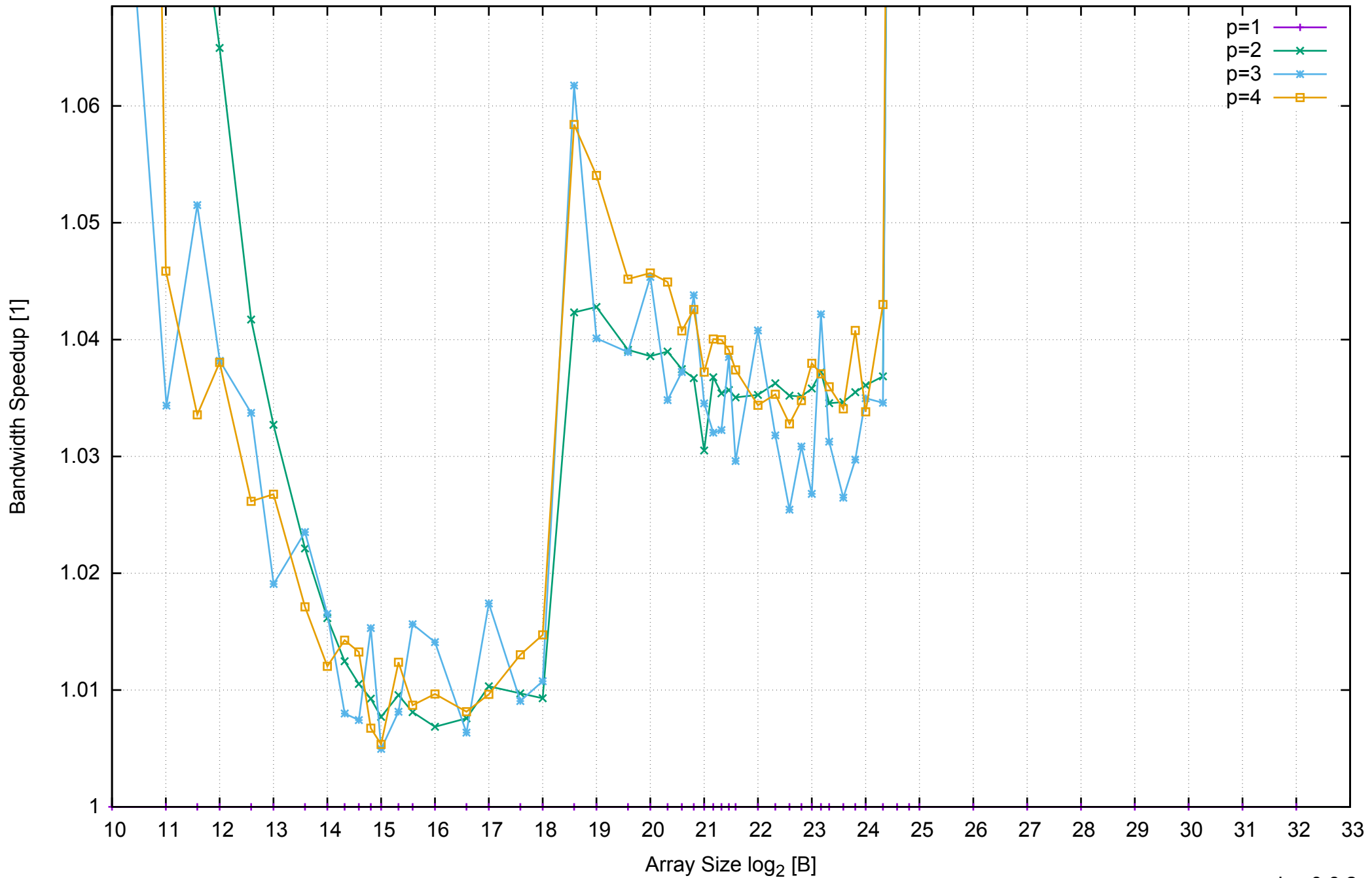
AWS m4.large - Intel Xeon E5-2676 v3, 2.40 GHz 8GB - Speedup of Parallel Memory Bandwidth (enlarged) - ScanRead64PtrSimpleLoop
