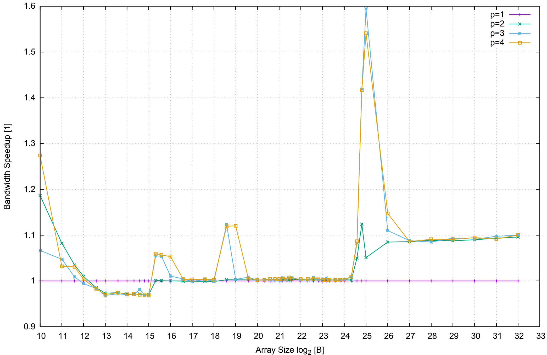
AWS m4.large - Intel Xeon E5-2676 v3, 2.40 GHz 8GB - Speedup of Parallel Memory Bandwidth - ScanWrite64IndexSimpleLoop
