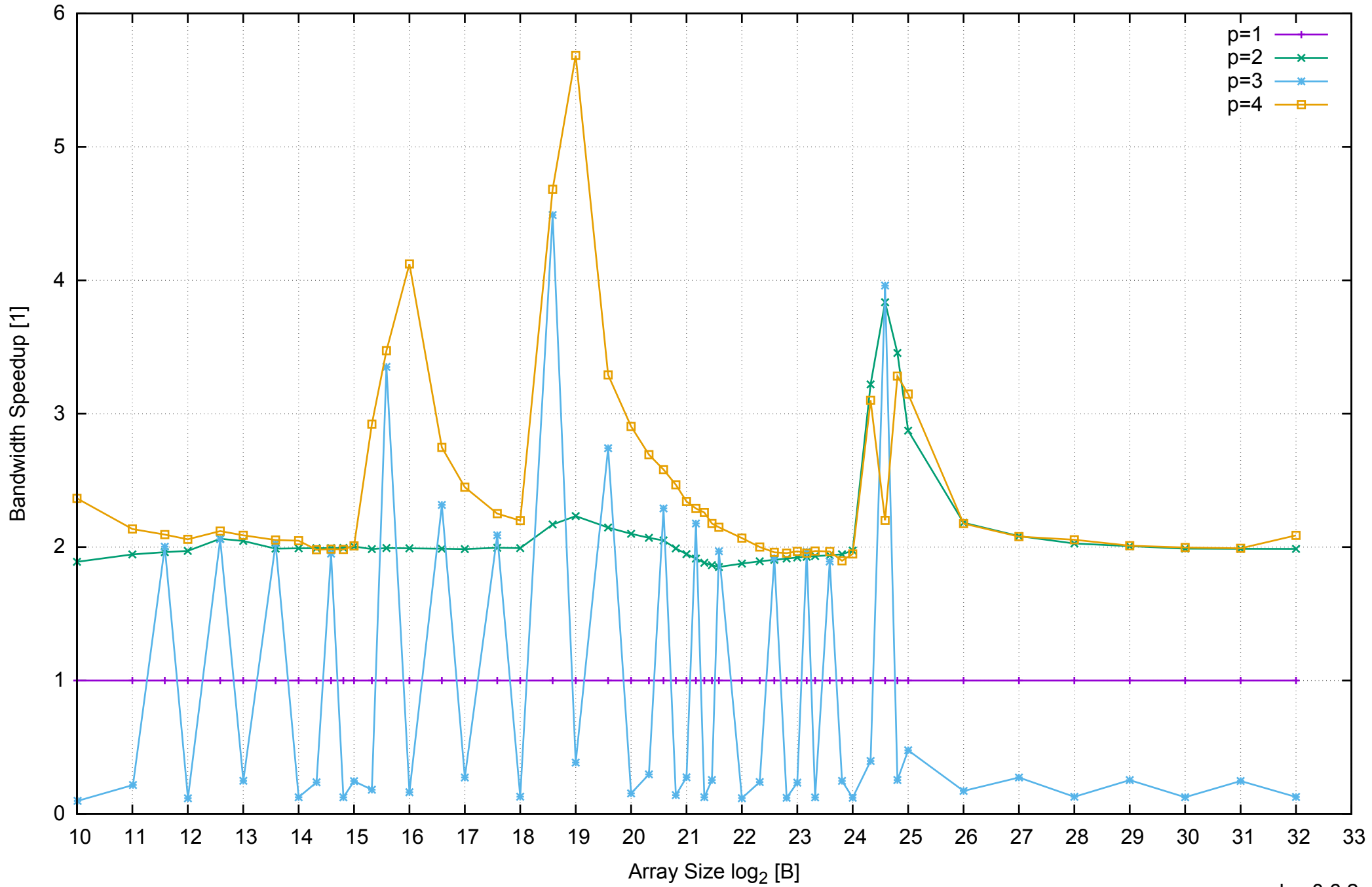
AWS m4.large - Intel Xeon E5-2676 v3, 2.40 GHz 8GB - Speedup of Parallel Memory Bandwidth - PermRead64UnrollLoop
