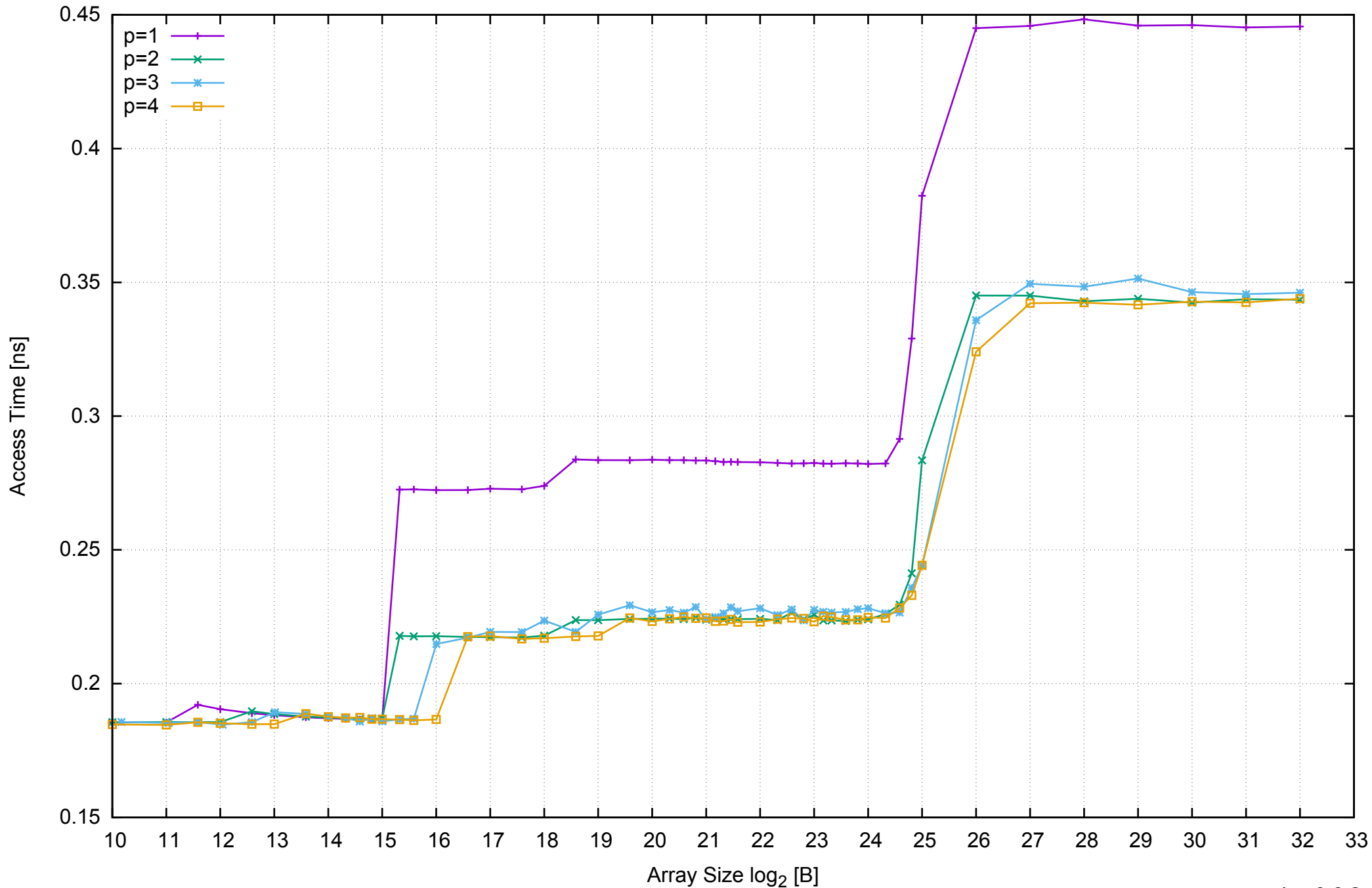
AWS m4.large - Intel Xeon E5-2676 v3, 2.40 GHz 8GB - Parallel Memory Access Time - ScanRead32PtrUnrollLoop
