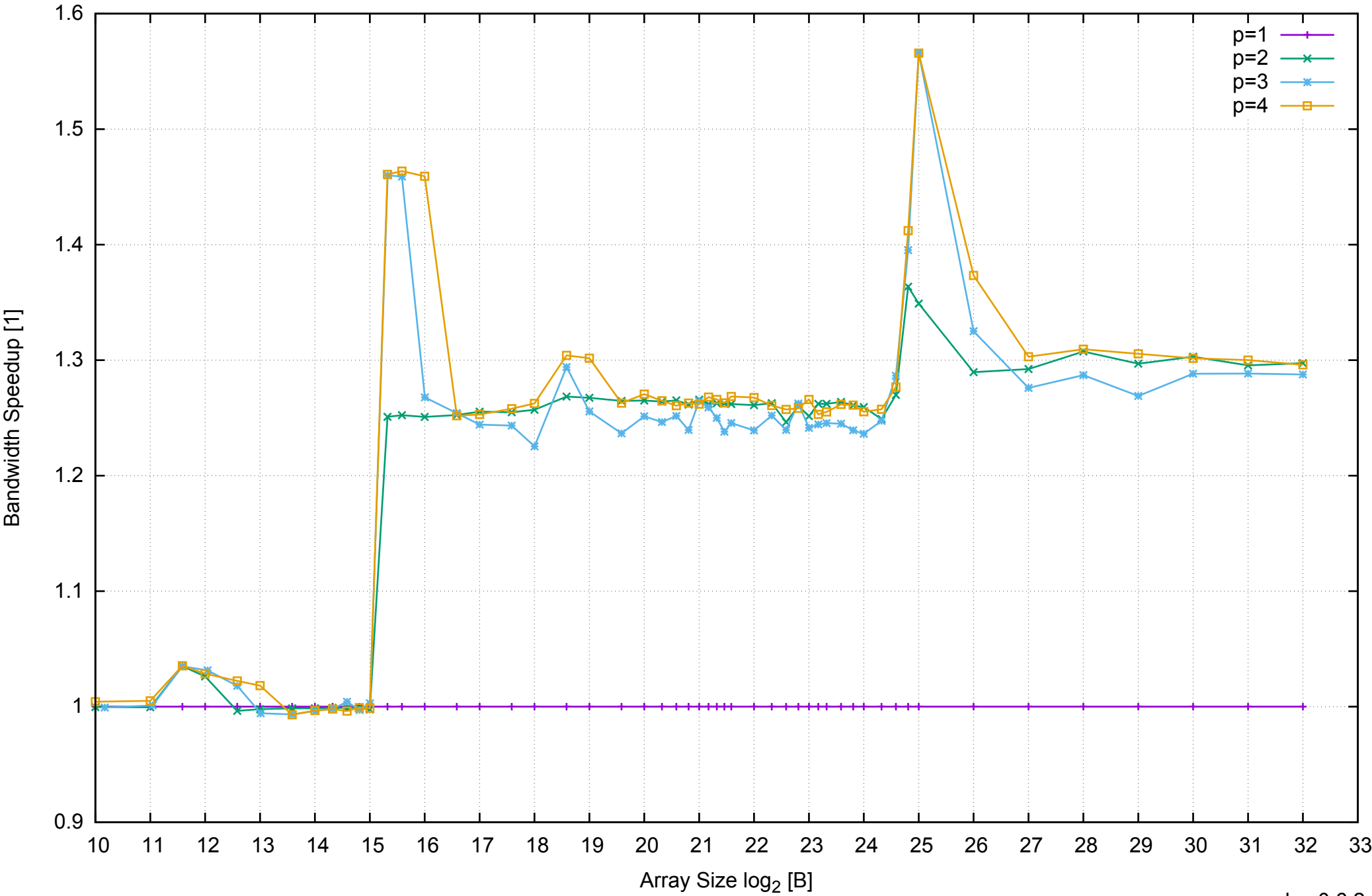
AWS m4.large - Intel Xeon E5-2676 v3, 2.40 GHz 8GB - Speedup of Parallel Memory Bandwidth - ScanRead32PtrUnrollLoop
