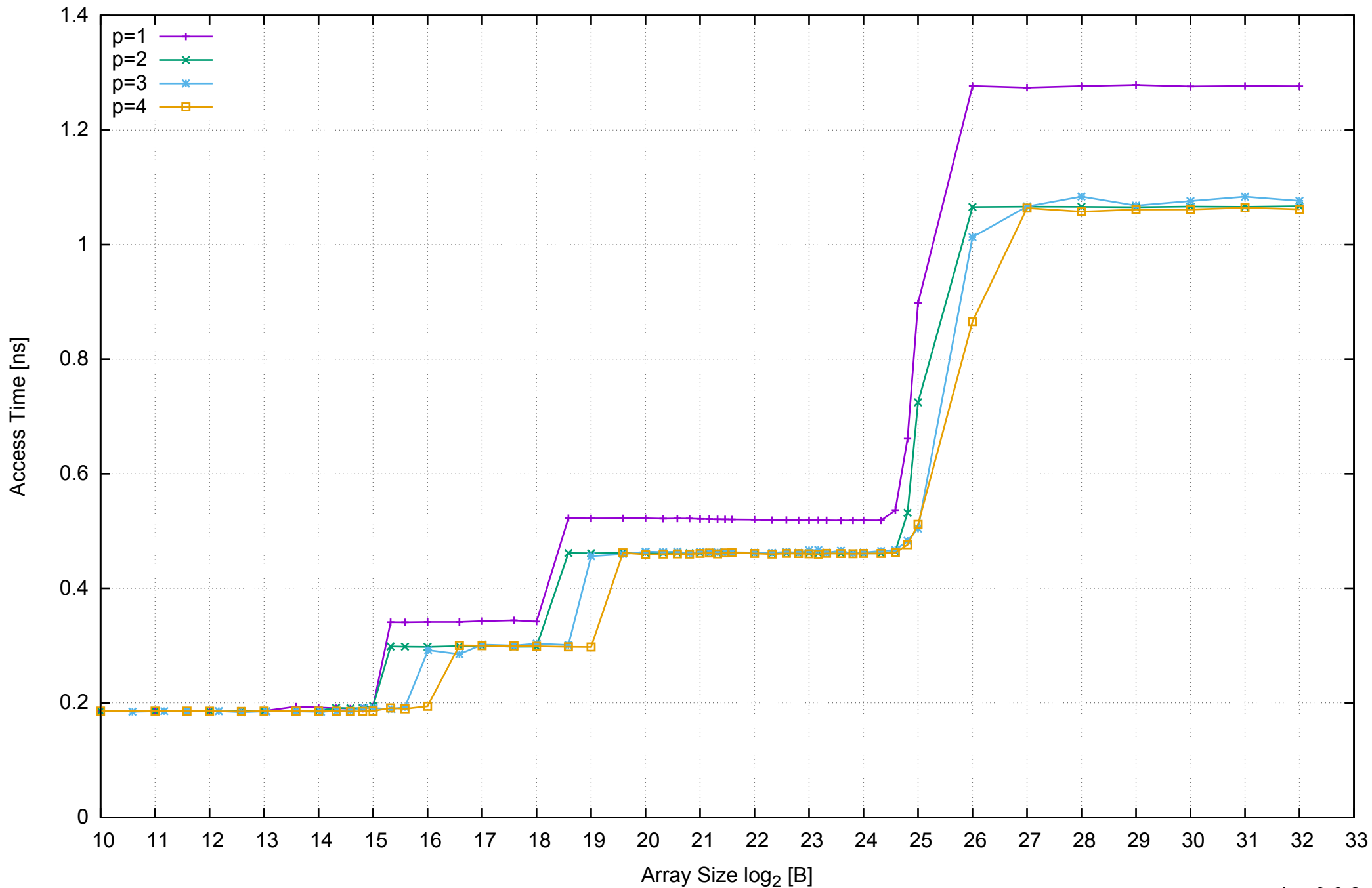
AWS m4.large - Intel Xeon E5-2676 v3, 2.40 GHz 8GB - Parallel Memory Access Time - ScanRead128PtrUnrollLoop
