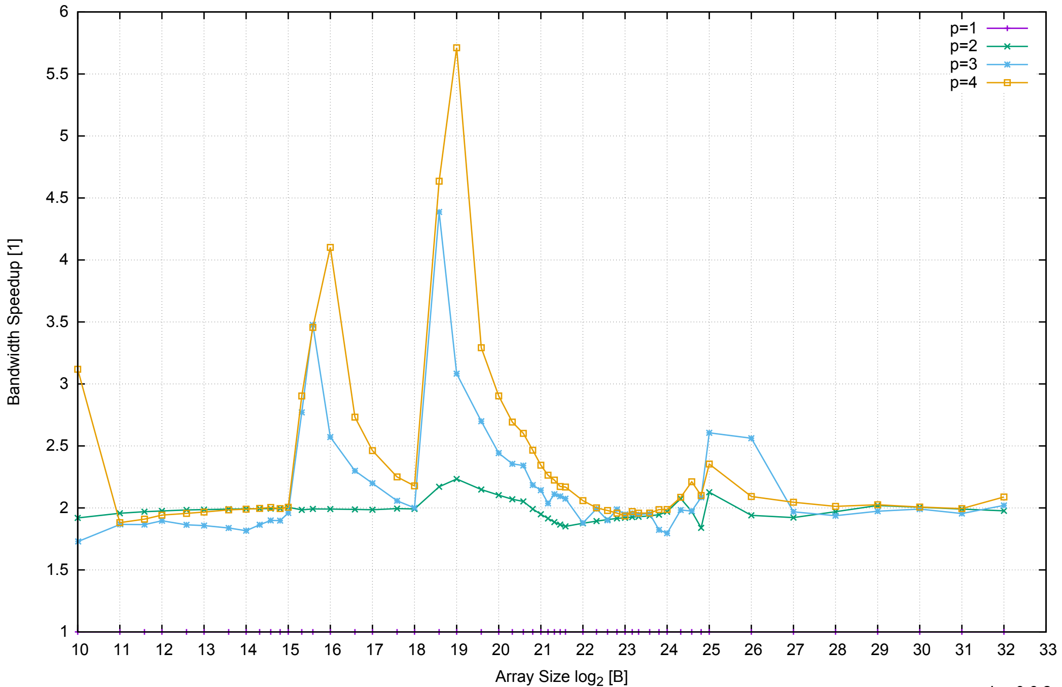
AWS m4.large - Intel Xeon E5-2676 v3, 2.40 GHz 8GB - Speedup of Parallel Memory Bandwidth - PermRead64SimpleLoop
