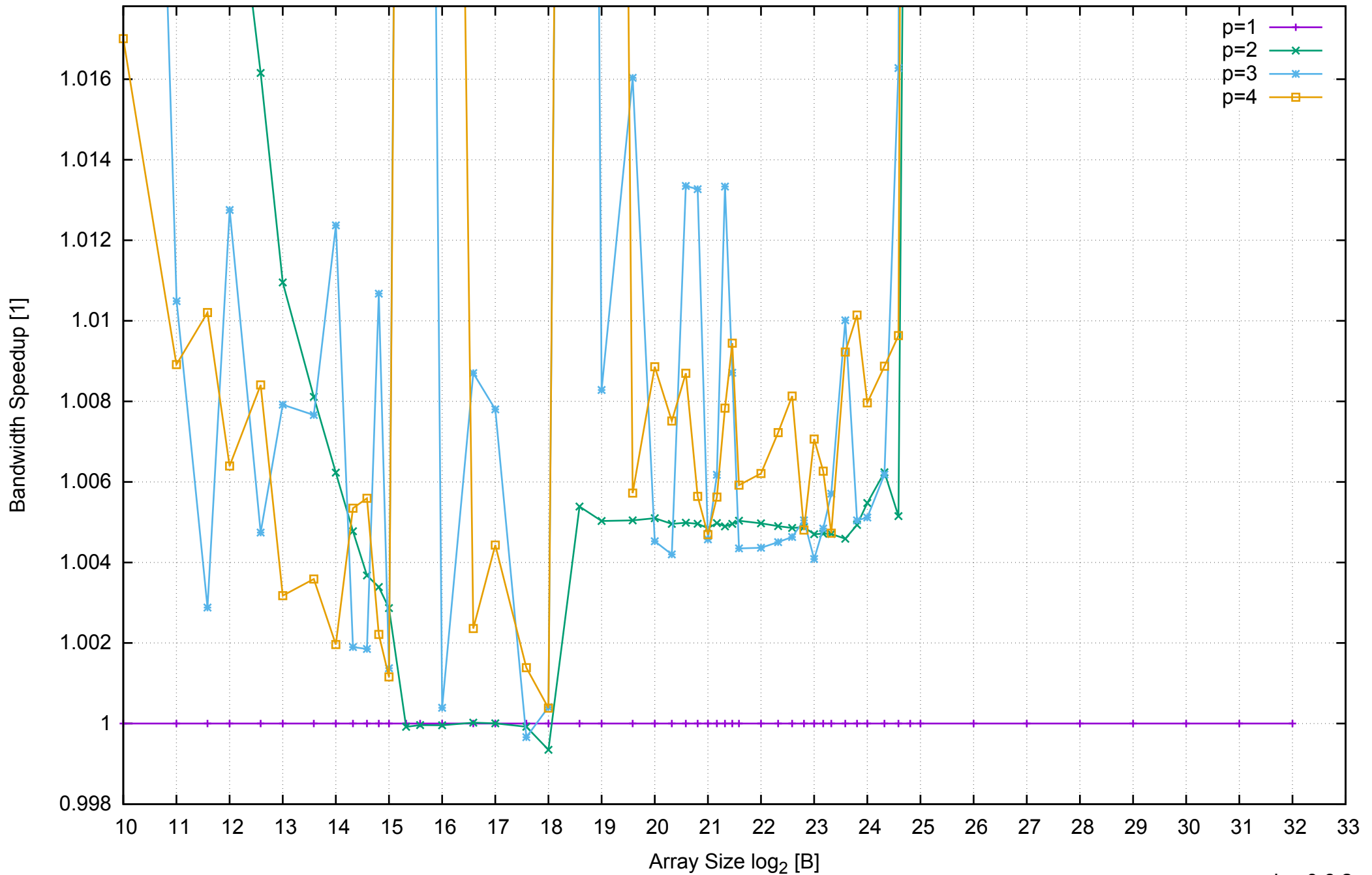
AWS m4.large - Intel Xeon E5-2676 v3, 2.40 GHz 8GB - Speedup of Parallel Memory Bandwidth (enlarged) - ScanWrite32PtrSimpleLoop
