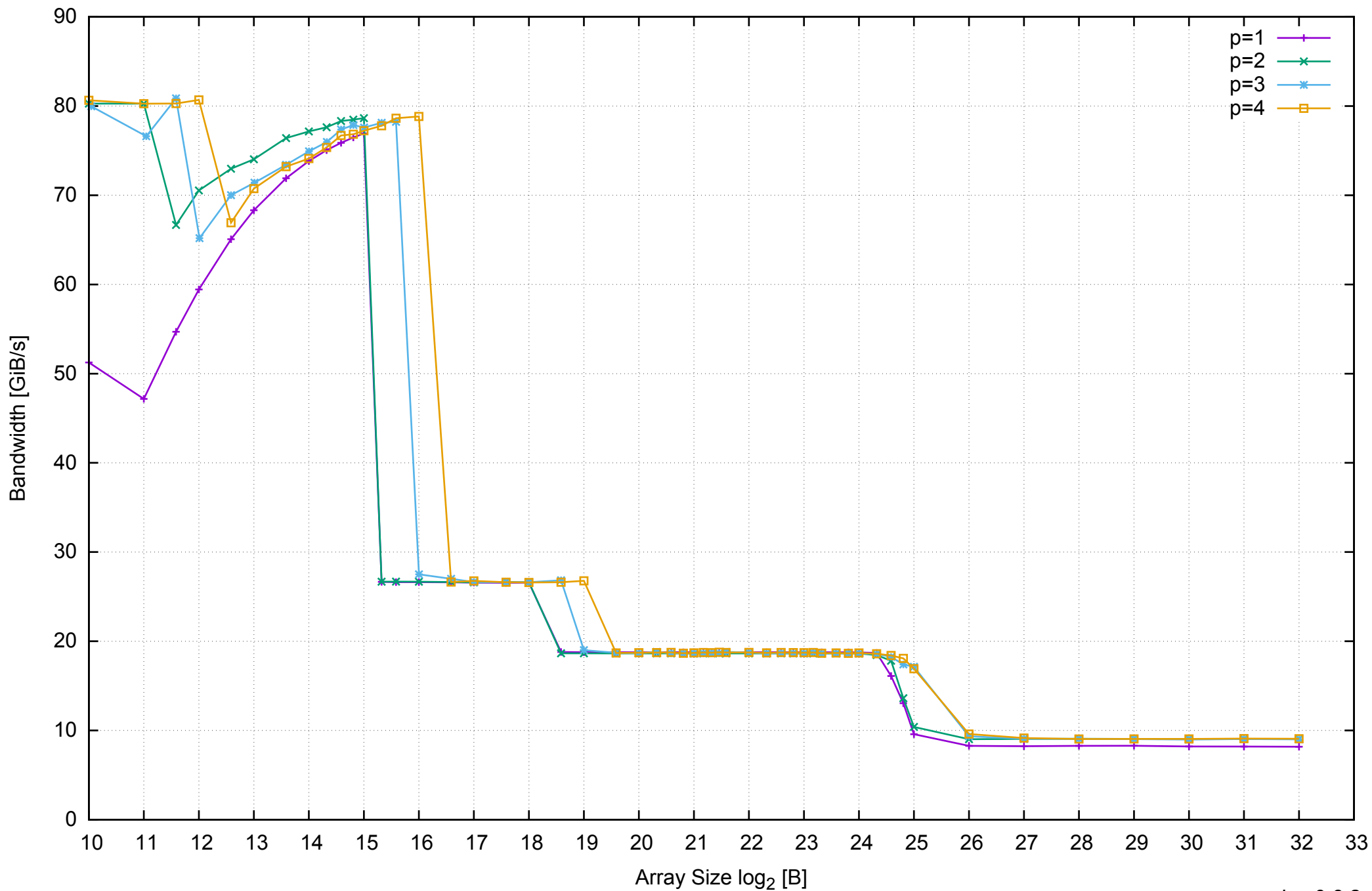
AWS m4.large - Intel Xeon E5-2676 v3, 2.40 GHz 8GB - Parallel Memory Bandwidth - ScanWrite256PtrSimpleLoop
