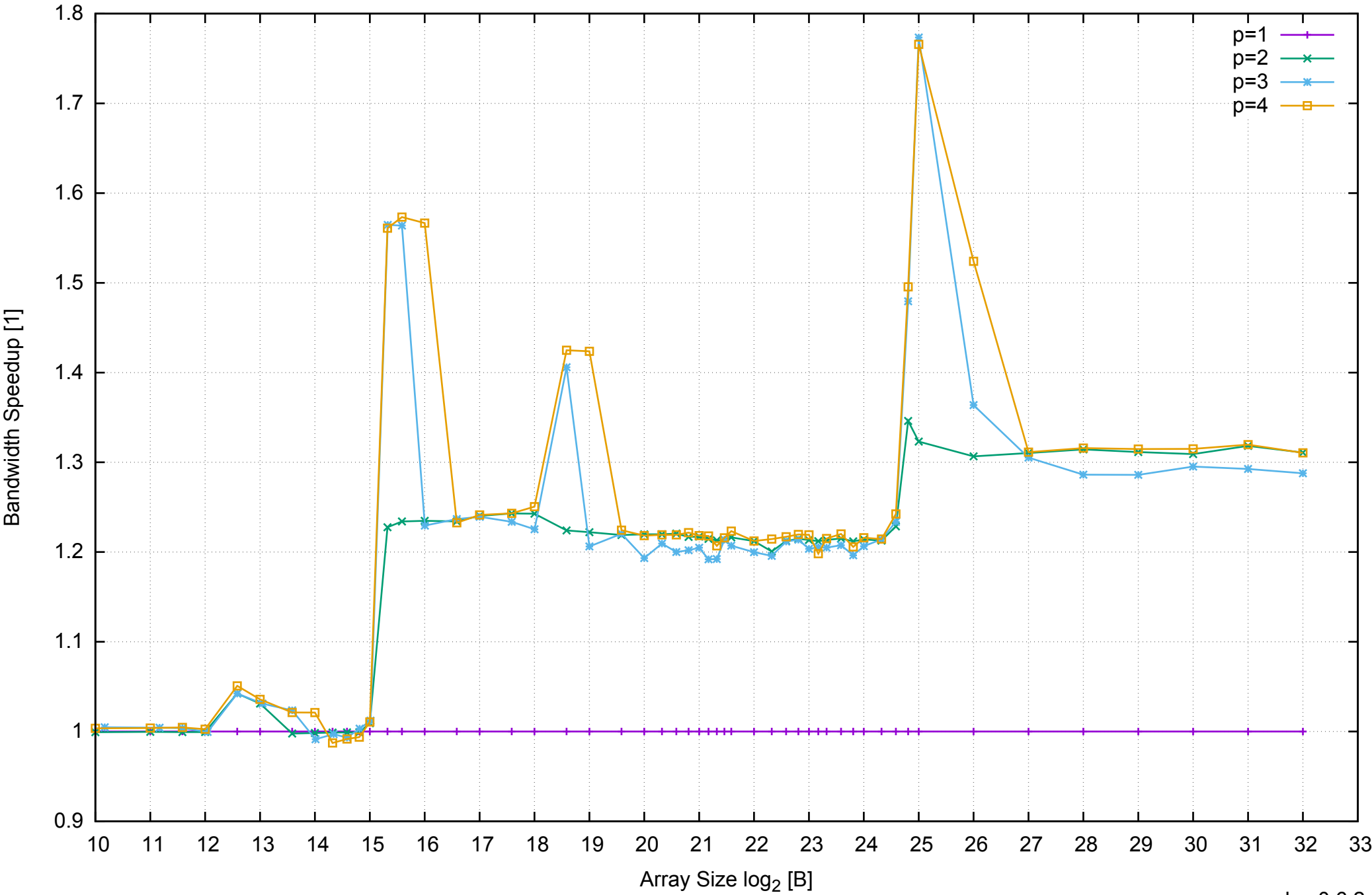
AWS m4.large - Intel Xeon E5-2676 v3, 2.40 GHz 8GB - Speedup of Parallel Memory Bandwidth - ScanRead64PtrUnrollLoop
