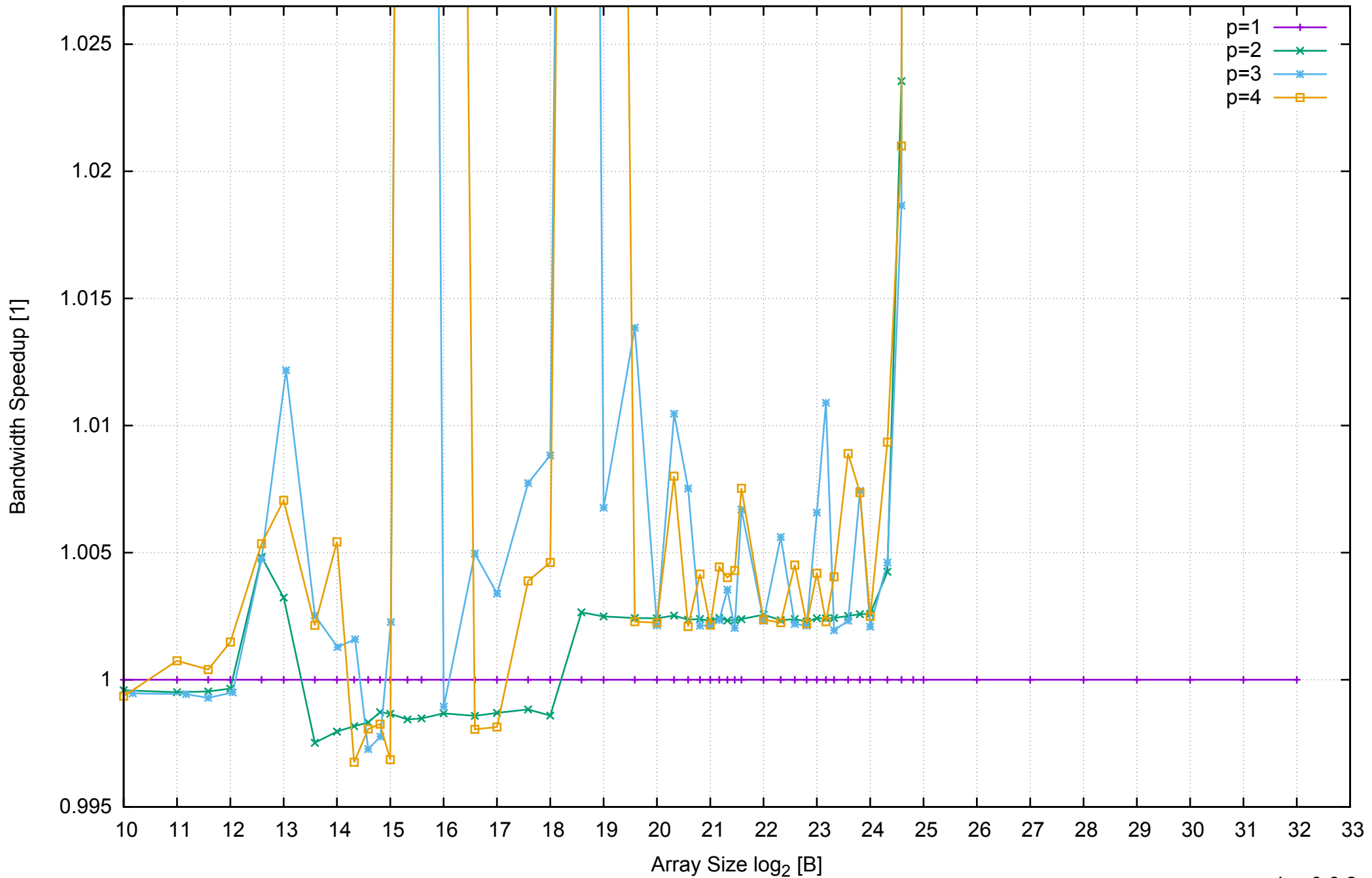
AWS m4.large - Intel Xeon E5-2676 v3, 2.40 GHz 8GB - Speedup of Parallel Memory Bandwidth (enlarged) - ScanWrite64PtrUnrollLoop
