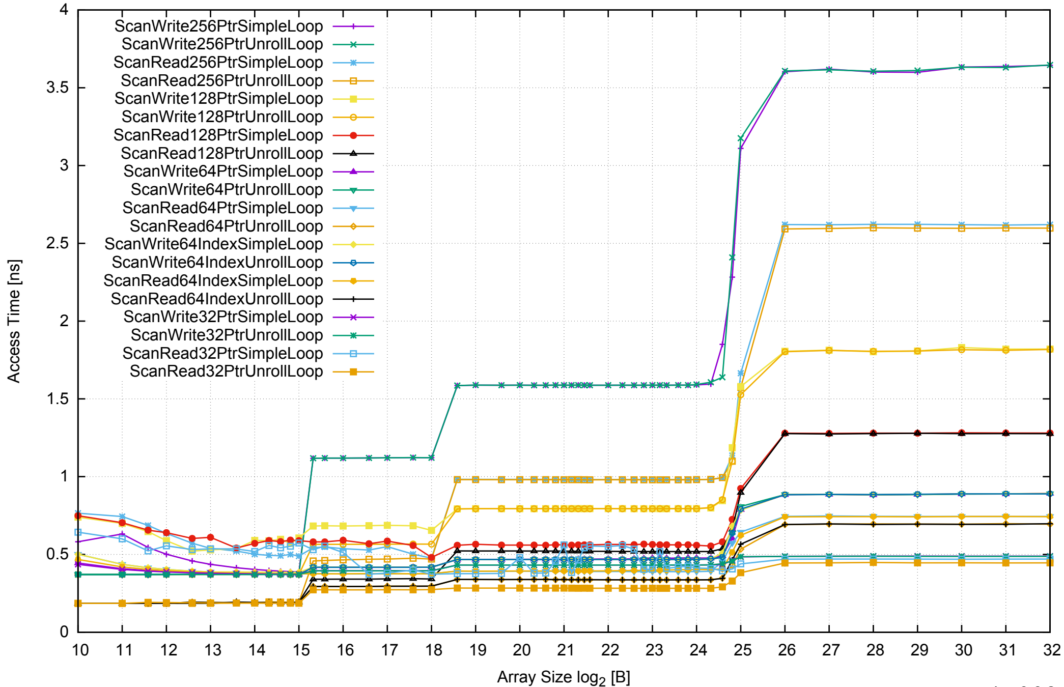
AWS m4.large - Intel Xeon E5-2676 v3, 2.40 GHz 8GB - One Thread Memory Latency (excluding Permutation)
