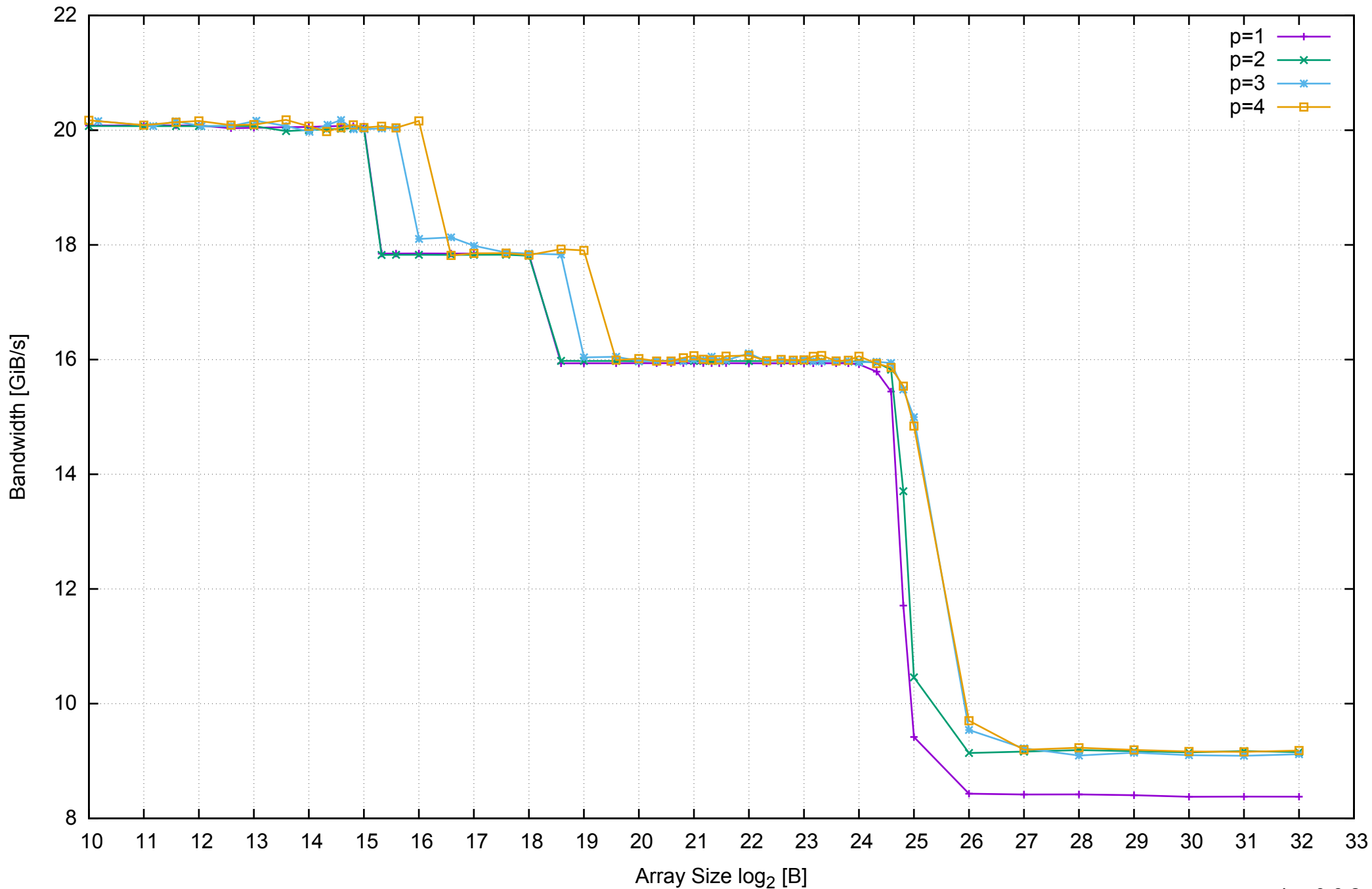
AWS m4.large - Intel Xeon E5-2676 v3, 2.40 GHz 8GB - Parallel Memory Bandwidth - ScanWrite64IndexUnrollLoop
