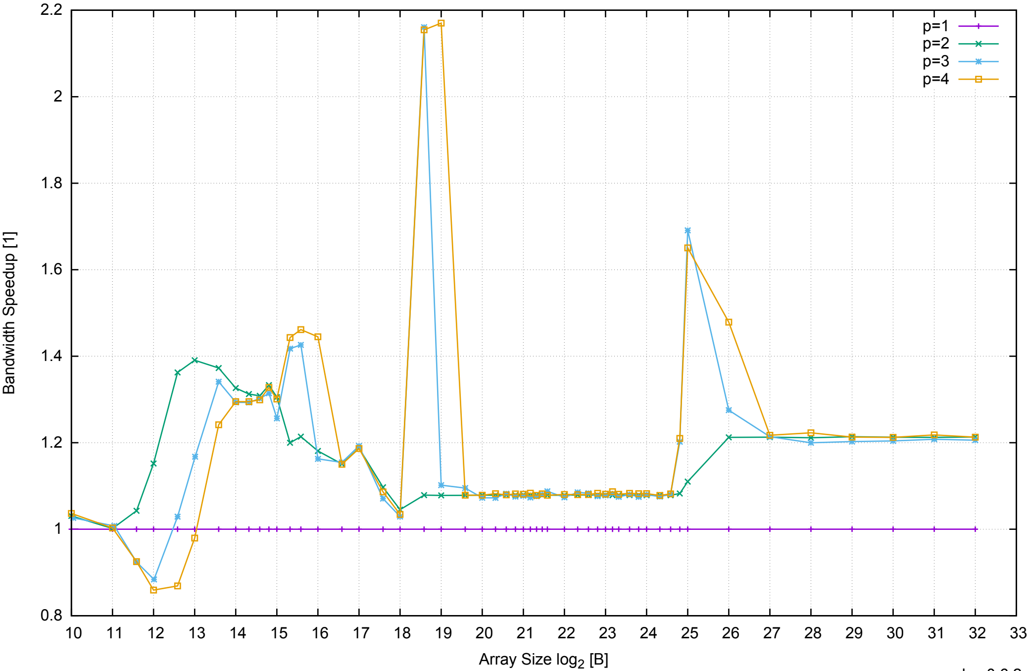
AWS m4.large - Intel Xeon E5-2676 v3, 2.40 GHz 8GB - Speedup of Parallel Memory Bandwidth - ScanRead256PtrSimpleLoop
