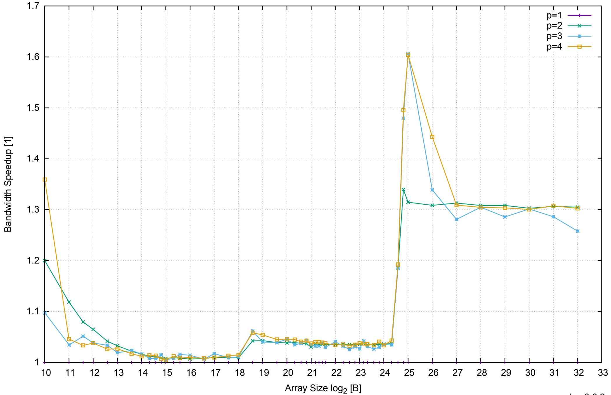
AWS m4.large - Intel Xeon E5-2676 v3, 2.40 GHz 8GB - Speedup of Parallel Memory Bandwidth - ScanRead64PtrSimpleLoop
