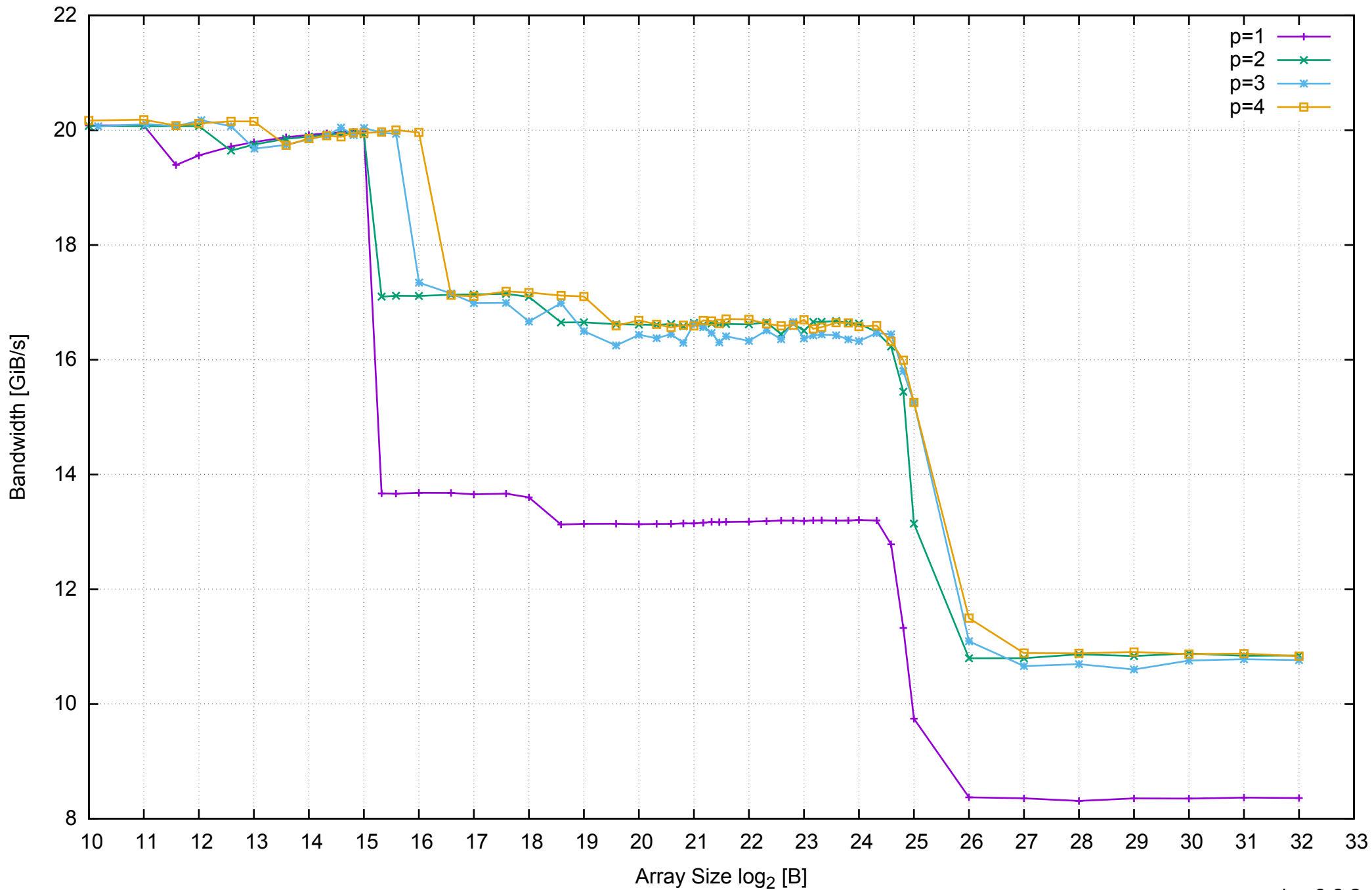
AWS m4.large - Intel Xeon E5-2676 v3, 2.40 GHz 8GB - Parallel Memory Bandwidth - ScanRead32PtrUnrollLoop
