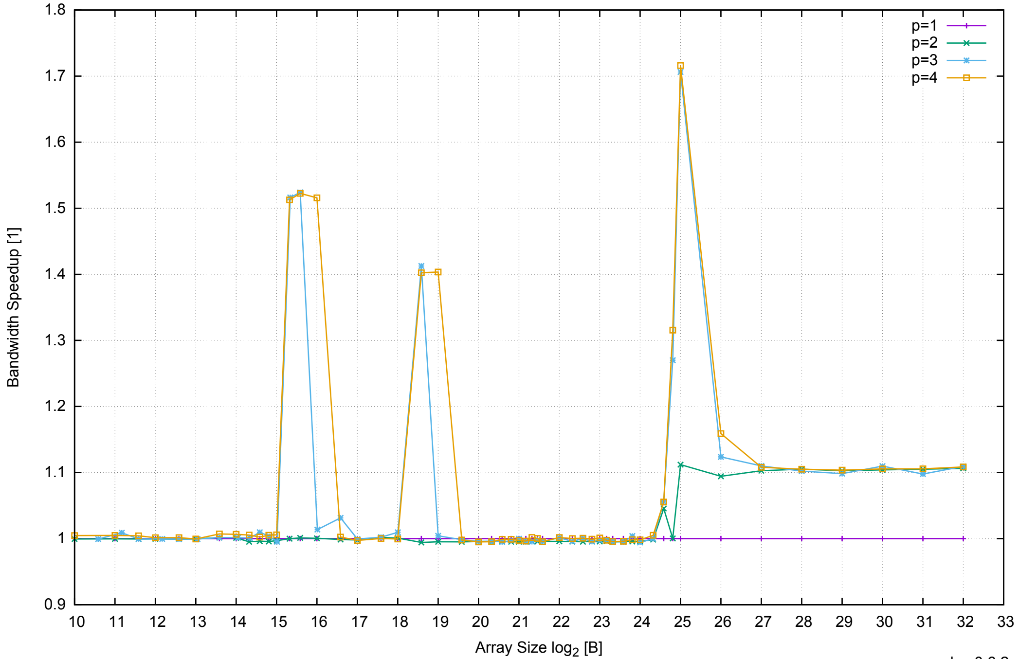
AWS m4.large - Intel Xeon E5-2676 v3, 2.40 GHz 8GB - Speedup of Parallel Memory Bandwidth - ScanWrite128PtrUnrollLoop
