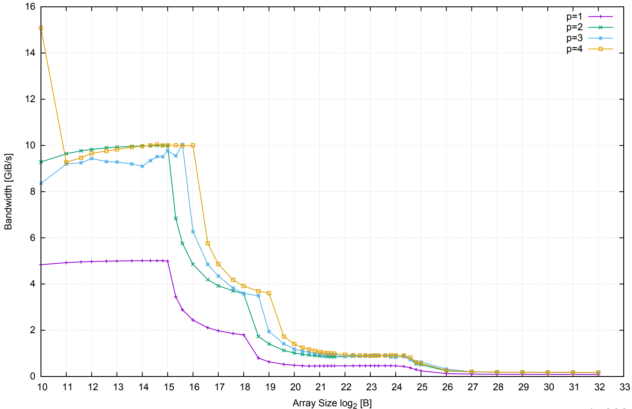
AWS m4.large - Intel Xeon E5-2676 v3, 2.40 GHz 8GB - Parallel Memory Bandwidth - PermRead64SimpleLoop
