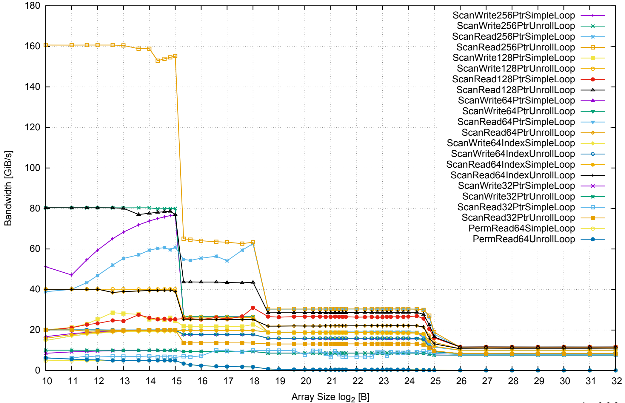
AWS m4.large - Intel Xeon E5-2676 v3, 2.40 GHz 8GB - One Thread Memory Bandwidth
