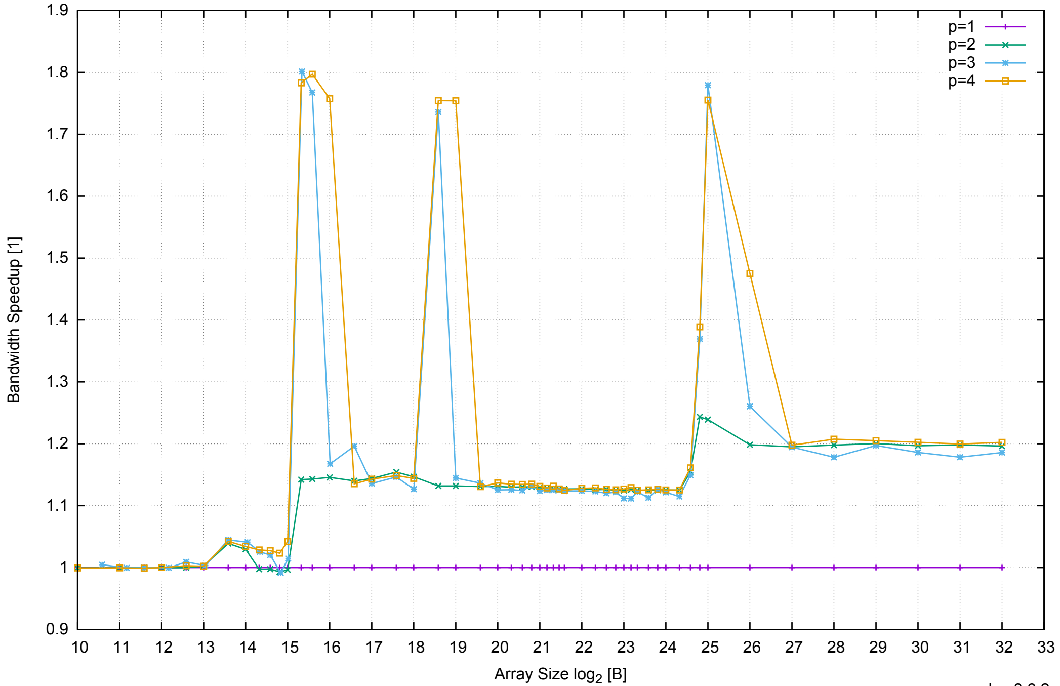
AWS m4.large - Intel Xeon E5-2676 v3, 2.40 GHz 8GB - Speedup of Parallel Memory Bandwidth - ScanRead128PtrUnrollLoop
