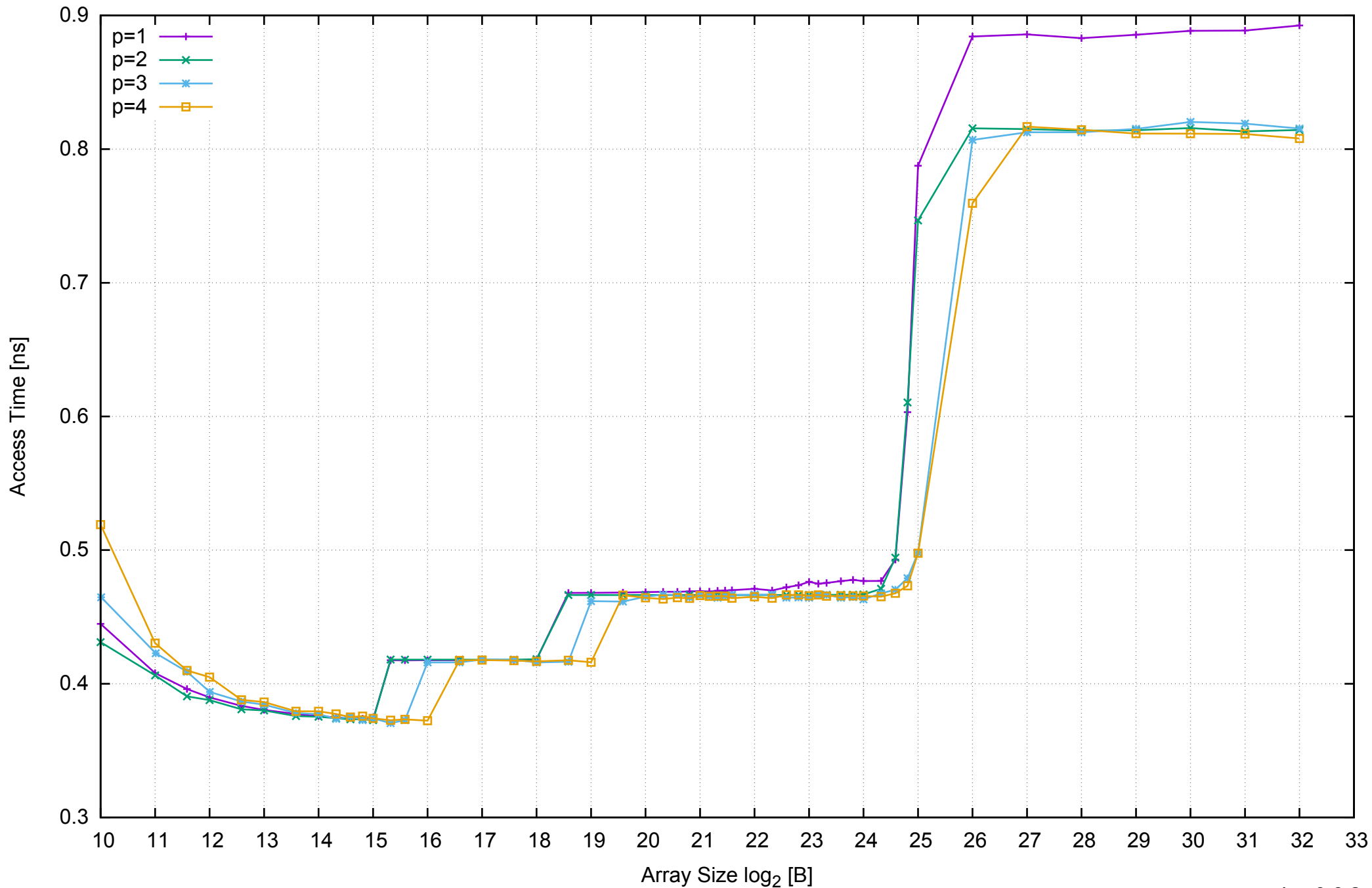
AWS m4.large - Intel Xeon E5-2676 v3, 2.40 GHz 8GB - Parallel Memory Access Time - ScanWrite64PtrSimpleLoop
