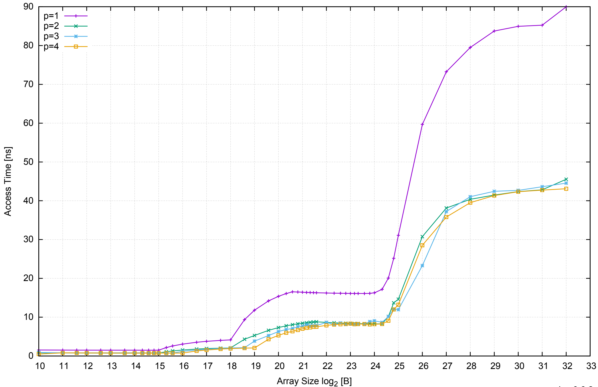
AWS m4.large - Intel Xeon E5-2676 v3, 2.40 GHz 8GB - Parallel Memory Access Time - PermRead64SimpleLoop
