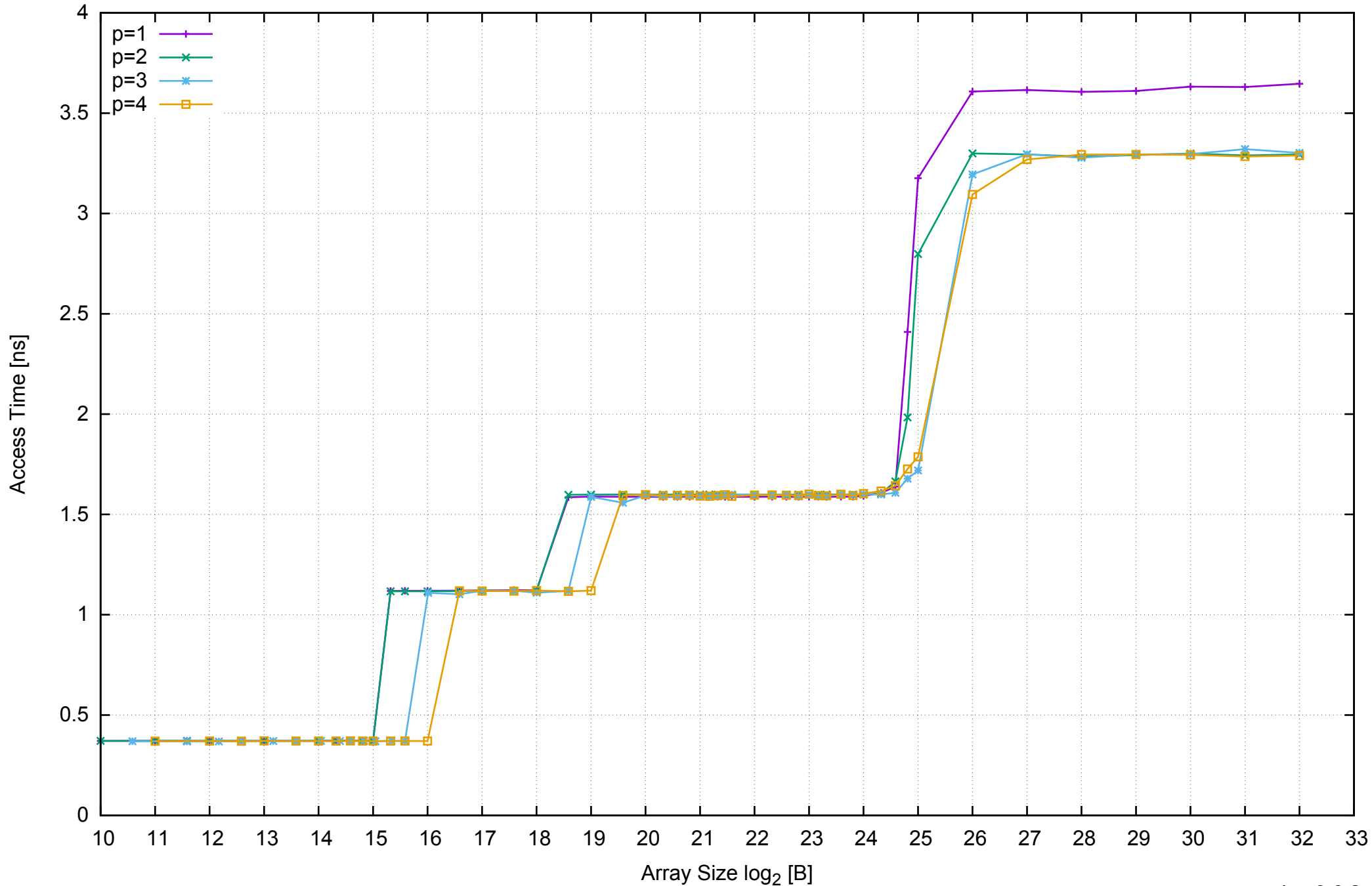
AWS m4.large - Intel Xeon E5-2676 v3, 2.40 GHz 8GB - Parallel Memory Access Time - ScanWrite256PtrUnrollLoop
