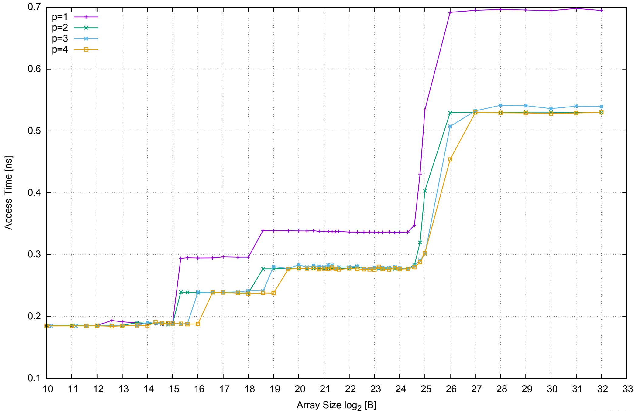
AWS m4.large - Intel Xeon E5-2676 v3, 2.40 GHz 8GB - Parallel Memory Access Time - ScanRead64PtrUnrollLoop
