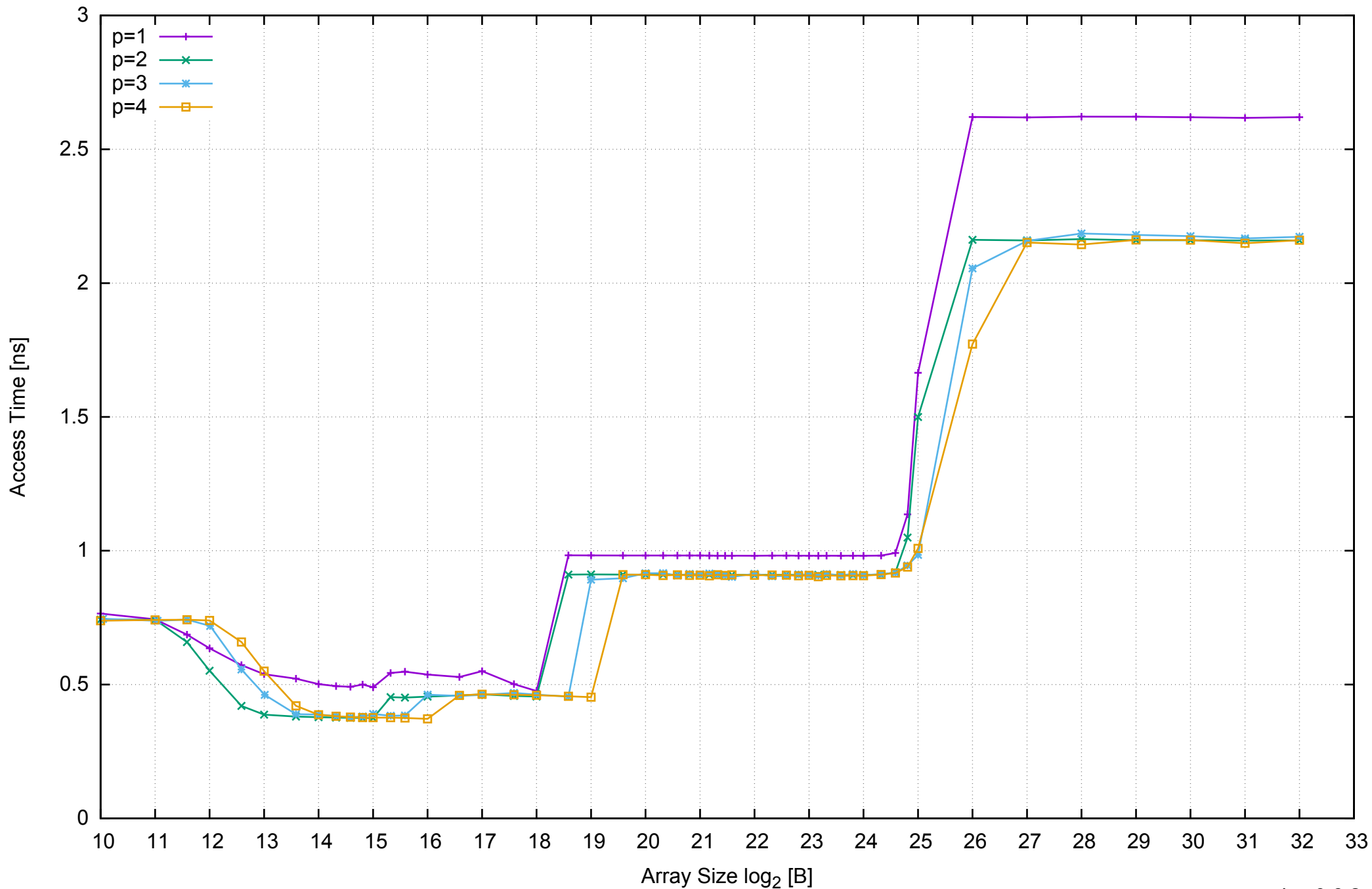
AWS m4.large - Intel Xeon E5-2676 v3, 2.40 GHz 8GB - Parallel Memory Access Time - ScanRead256PtrSimpleLoop
