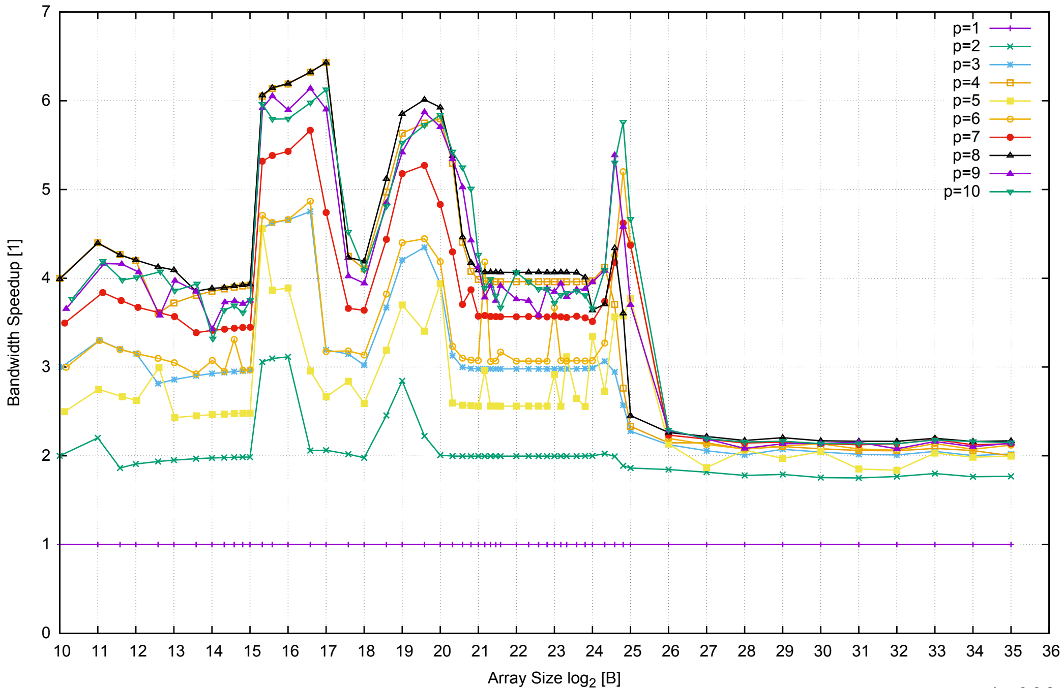
AWS i2.2xlarge - Intel Xeon E5-2670 v2, 2.50 GHz 61GB - Speedup of Parallel Memory Bandwidth - ScanWrite256PtrSimpleLoop
