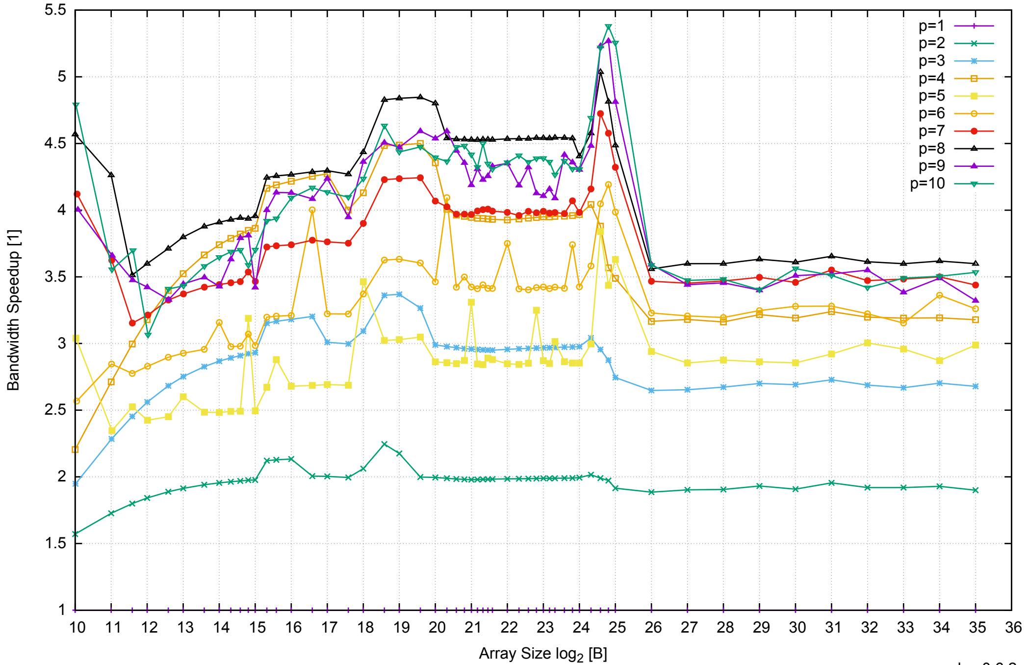
AWS i2.2xlarge - Intel Xeon E5-2670 v2, 2.50 GHz 61GB - Speedup of Parallel Memory Bandwidth - ScanRead64IndexSimpleLoop
