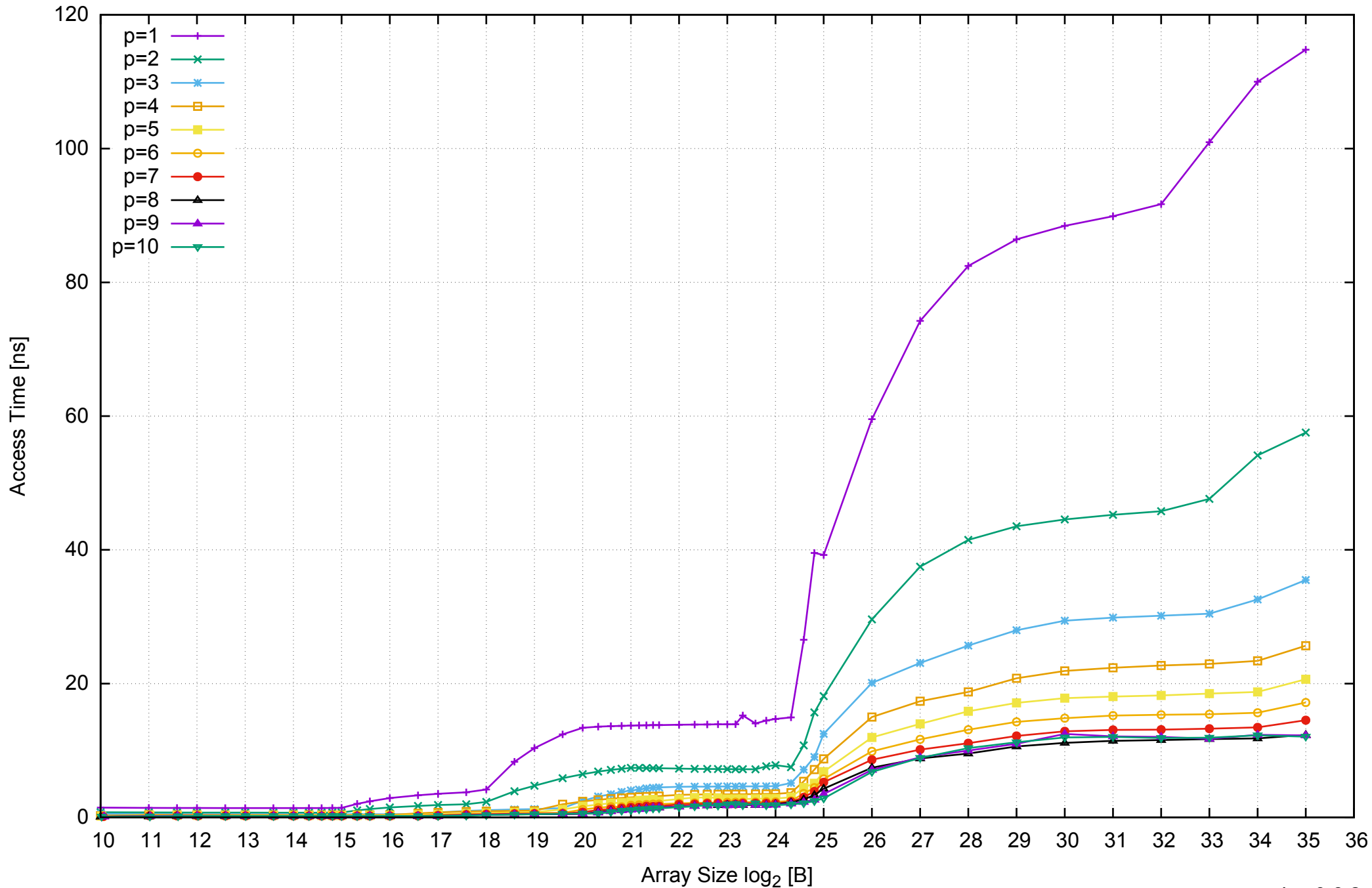
AWS i2.2xlarge - Intel Xeon E5-2670 v2, 2.50 GHz 61GB - Parallel Memory Access Time - PermRead64SimpleLoop
