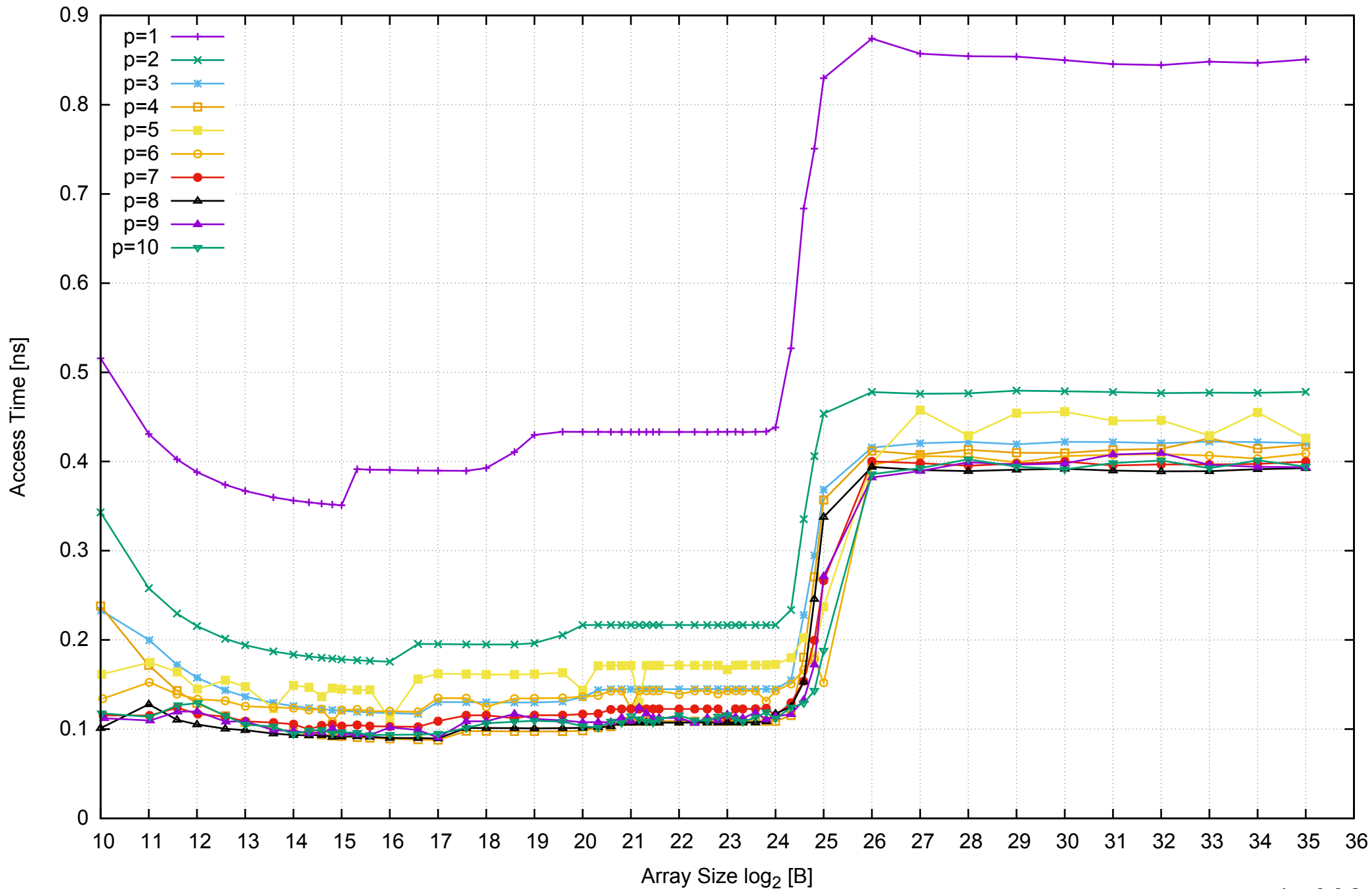
AWS i2.2xlarge - Intel Xeon E5-2670 v2, 2.50 GHz 61GB - Parallel Memory Access Time - ScanWrite64PtrSimpleLoop
