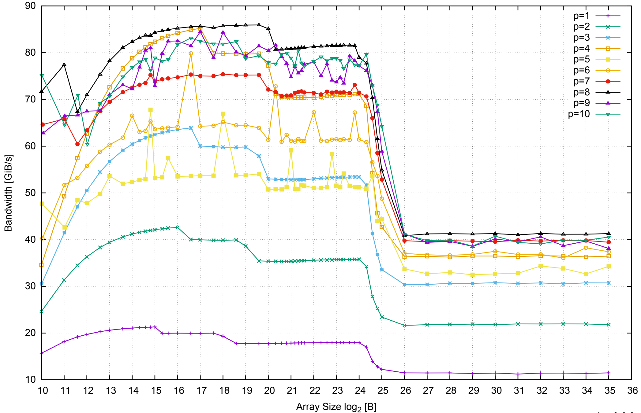
AWS i2.2xlarge - Intel Xeon E5-2670 v2, 2.50 GHz 61GB - Parallel Memory Bandwidth - ScanRead64IndexSimpleLoop
