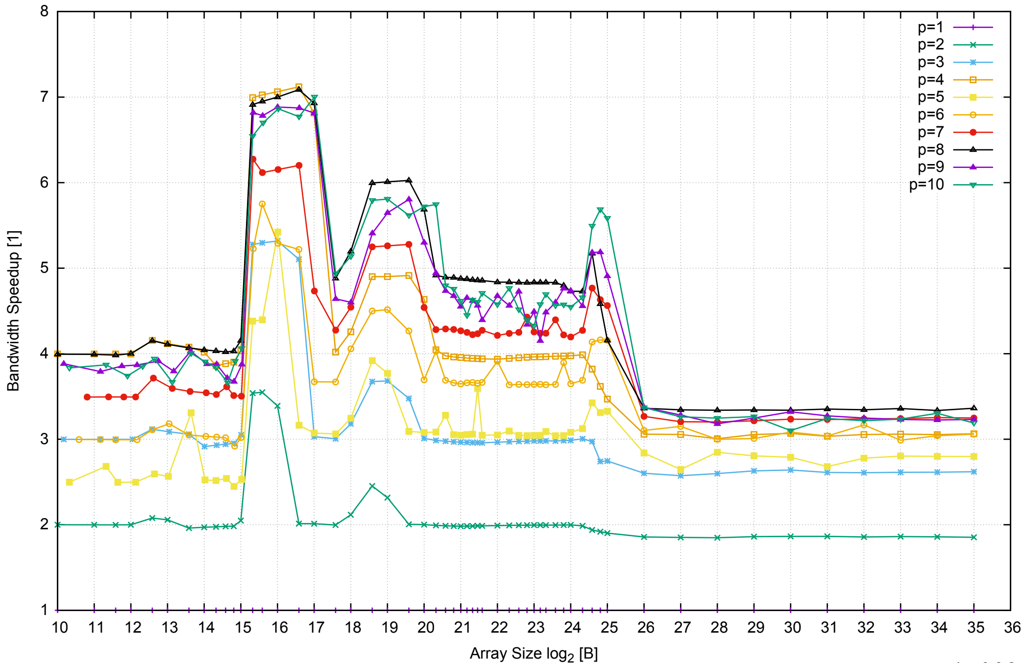
AWS i2.2xlarge - Intel Xeon E5-2670 v2, 2.50 GHz 61GB - Speedup of Parallel Memory Bandwidth - ScanRead64PtrUnrollLoop
