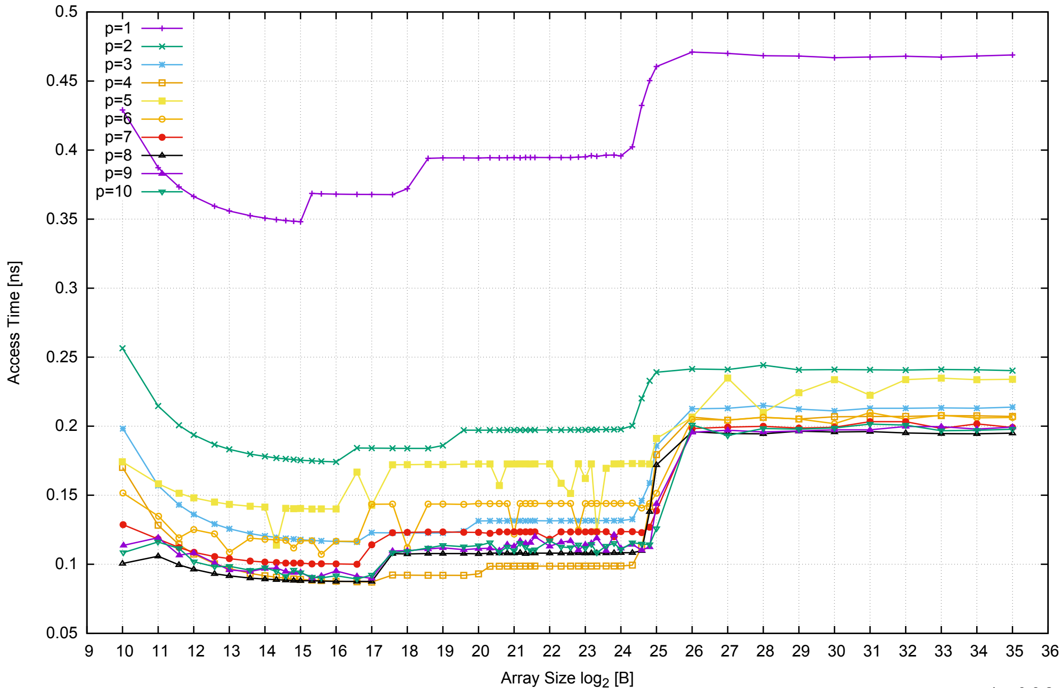
AWS i2.2xlarge - Intel Xeon E5-2670 v2, 2.50 GHz 61GB - Parallel Memory Access Time - ScanWrite32PtrSimpleLoop
