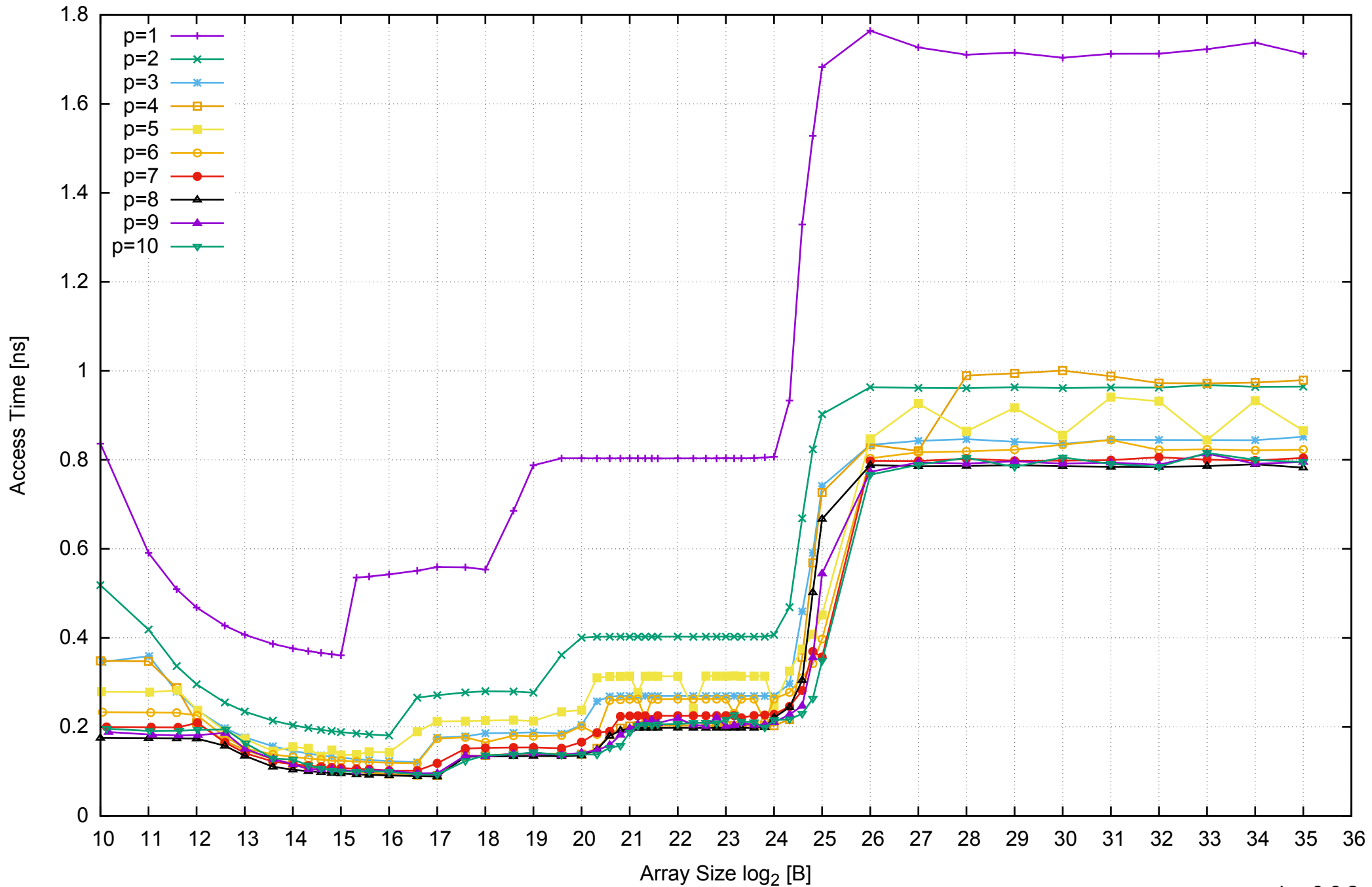
AWS i2.2xlarge - Intel Xeon E5-2670 v2, 2.50 GHz 61GB - Parallel Memory Access Time - ScanWrite128PtrSimpleLoop
