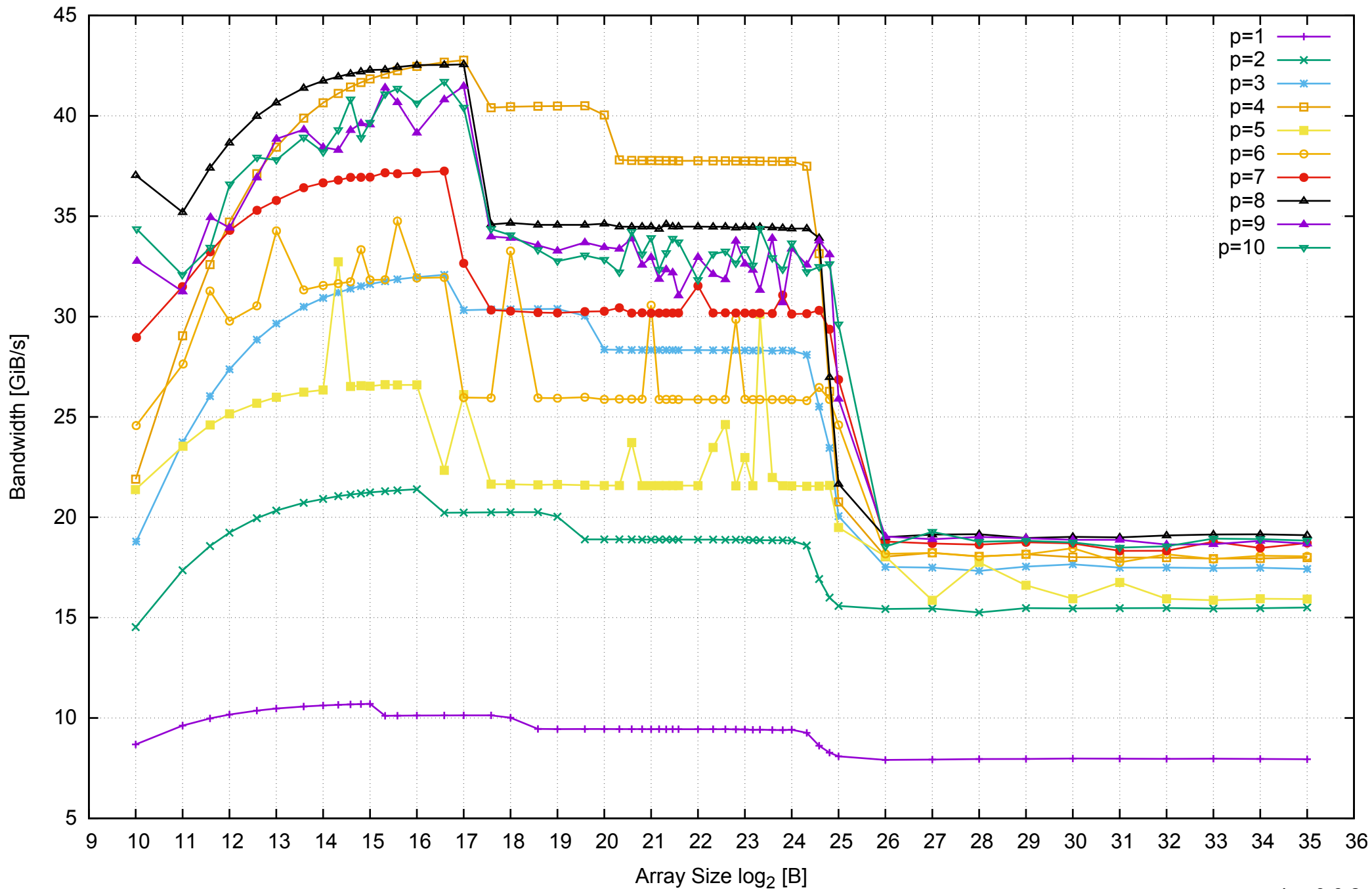
AWS i2.2xlarge - Intel Xeon E5-2670 v2, 2.50 GHz 61GB - Parallel Memory Bandwidth - ScanWrite32PtrSimpleLoop
