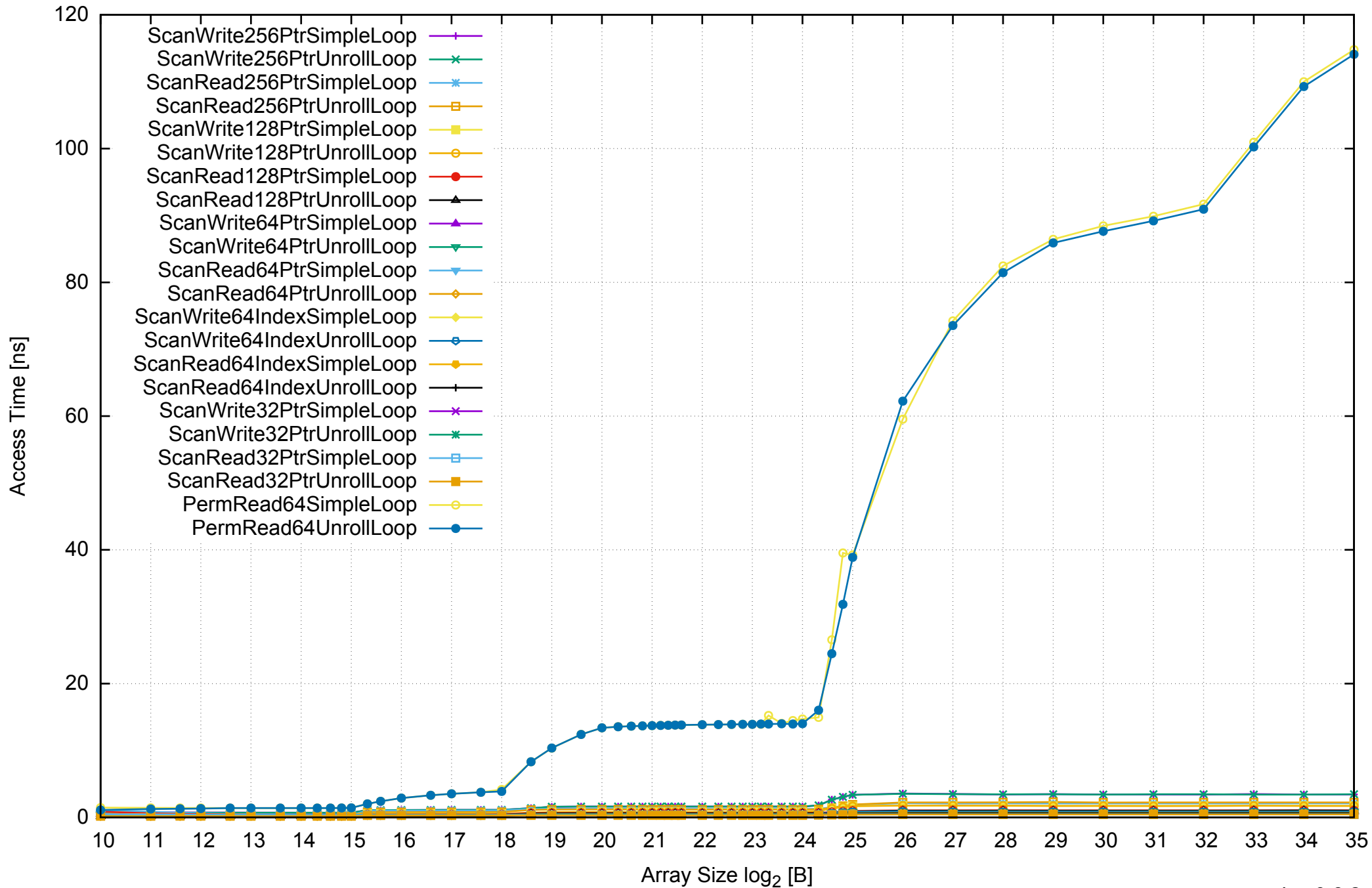
AWS i2.2xlarge - Intel Xeon E5-2670 v2, 2.50 GHz 61GB - One Thread Memory Latency (Access Time)
