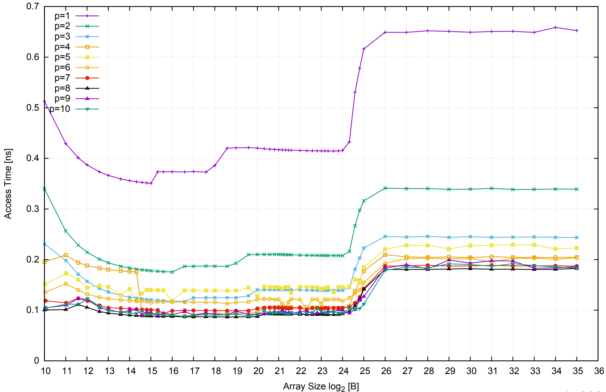
AWS i2.2xlarge - Intel Xeon E5-2670 v2, 2.50 GHz 61GB - Parallel Memory Access Time - ScanRead64PtrSimpleLoop
