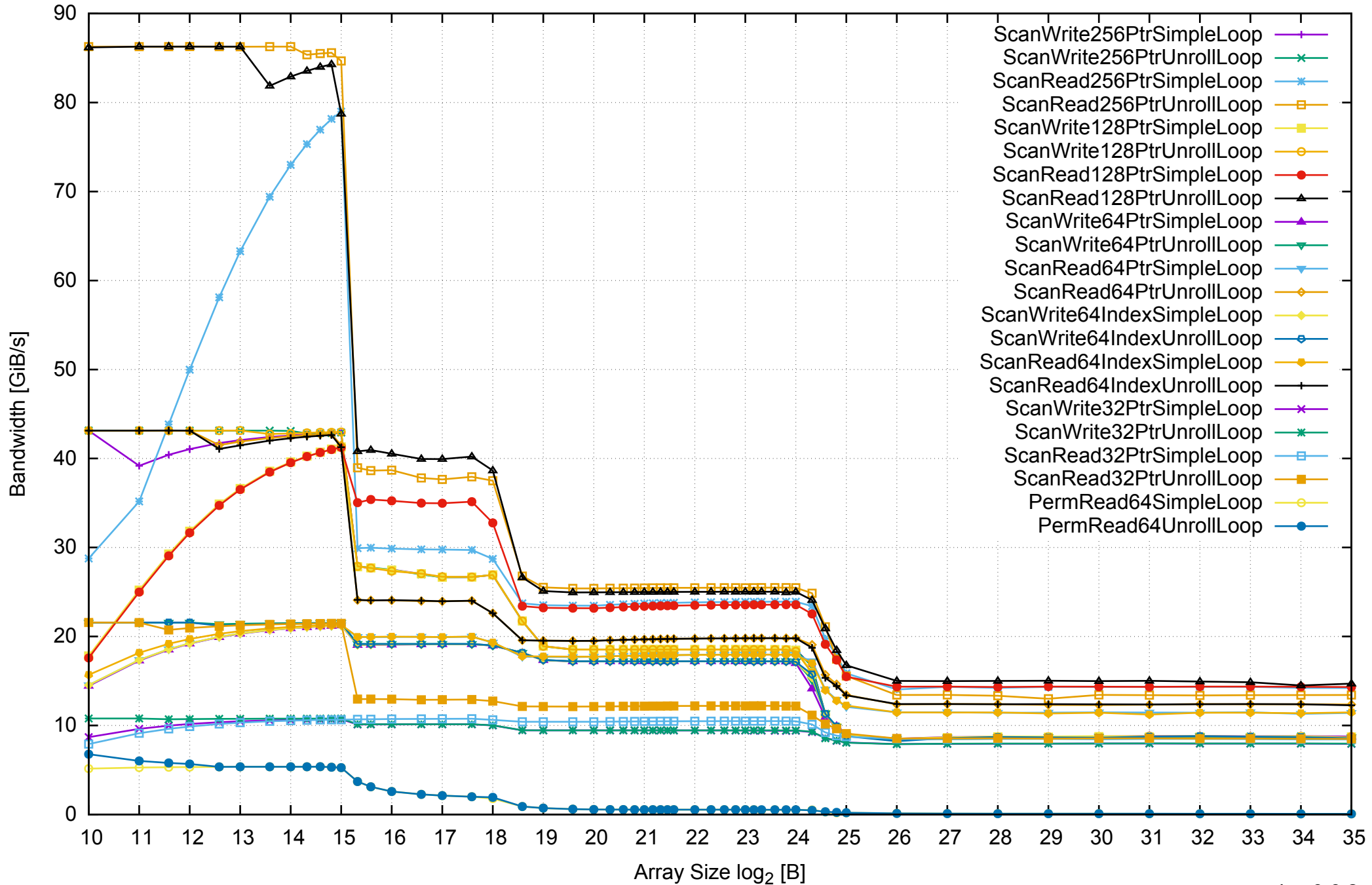
AWS i2.2xlarge - Intel Xeon E5-2670 v2, 2.50 GHz 61GB - One Thread Memory Bandwidth
