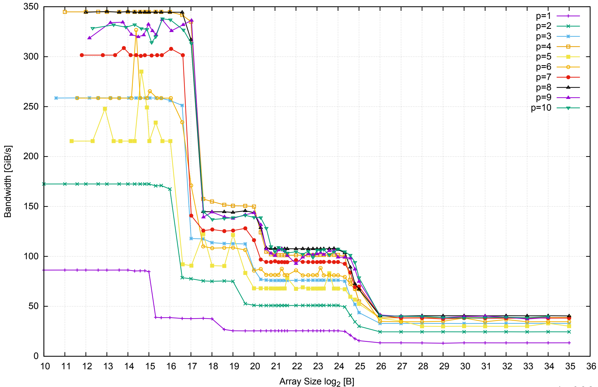
AWS i2.2xlarge - Intel Xeon E5-2670 v2, 2.50 GHz 61GB - Parallel Memory Bandwidth - ScanRead256PtrUnrollLoop
