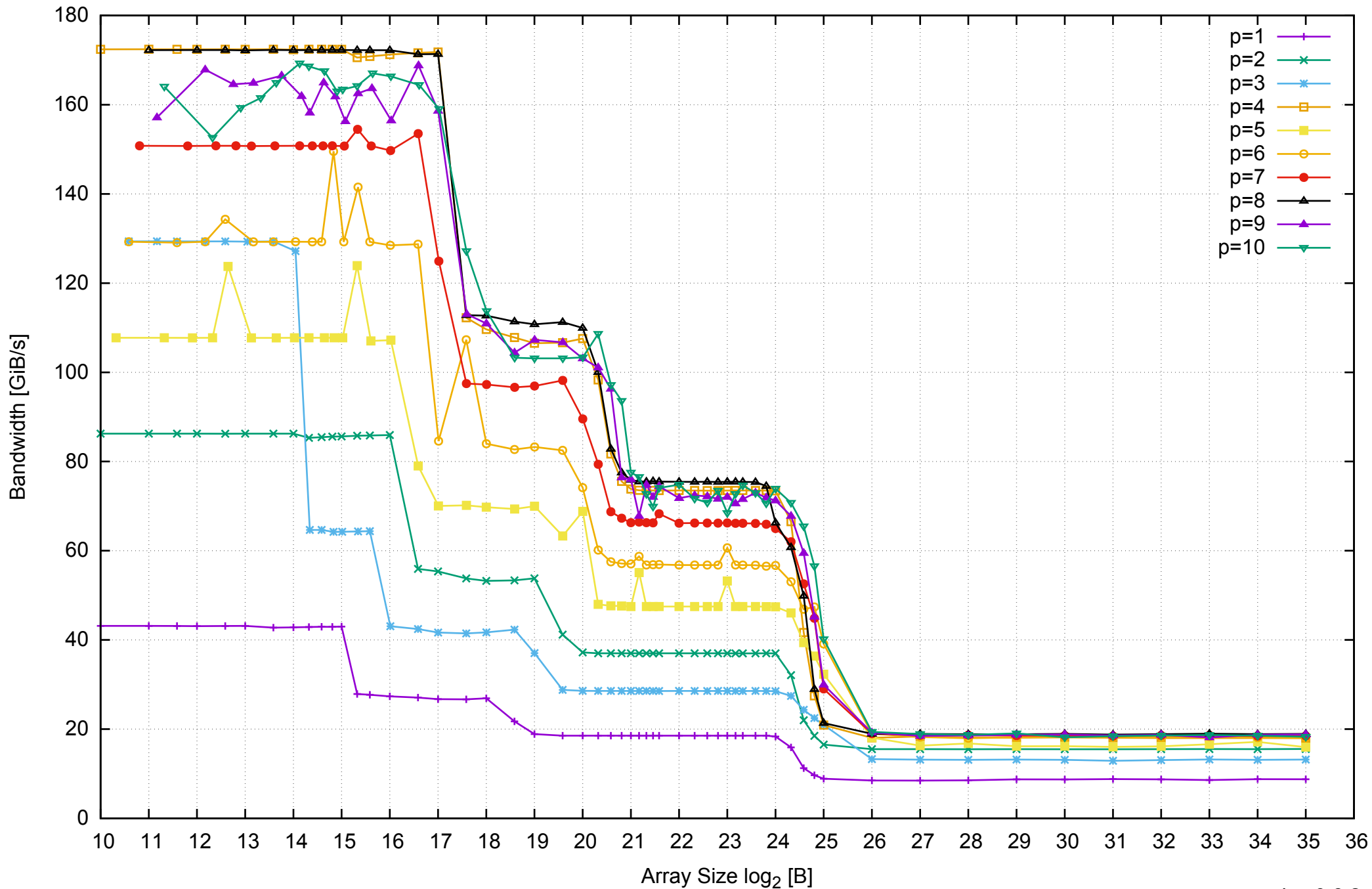
AWS i2.2xlarge - Intel Xeon E5-2670 v2, 2.50 GHz 61GB - Parallel Memory Bandwidth - ScanWrite128PtrUnrollLoop
