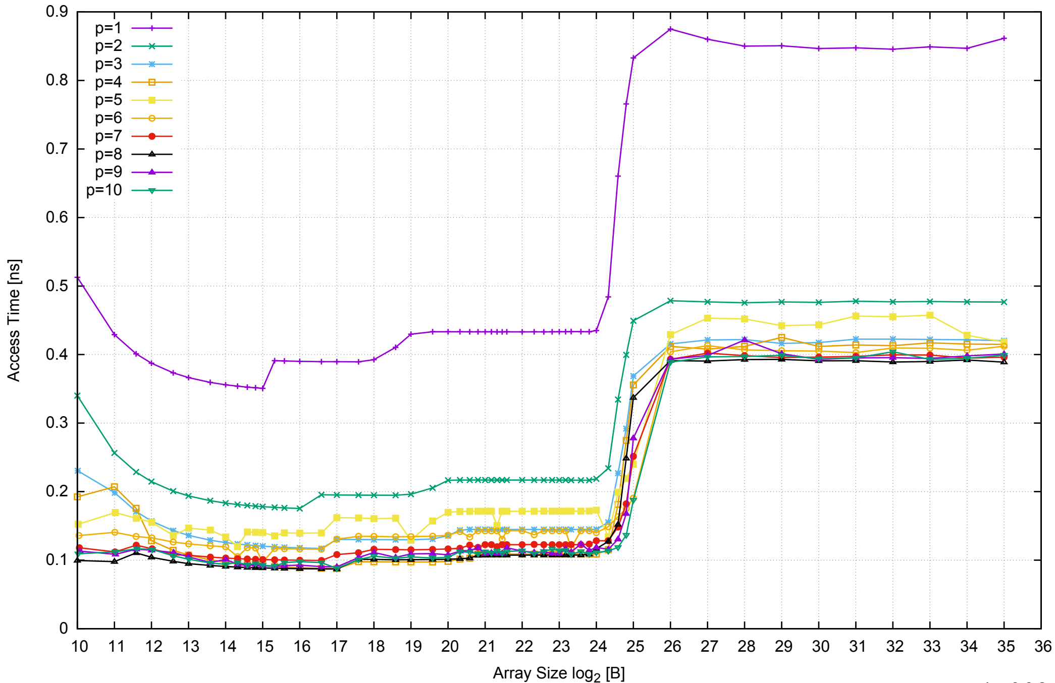
AWS i2.2xlarge - Intel Xeon E5-2670 v2, 2.50 GHz 61GB - Parallel Memory Access Time - ScanWrite64IndexSimpleLoop
