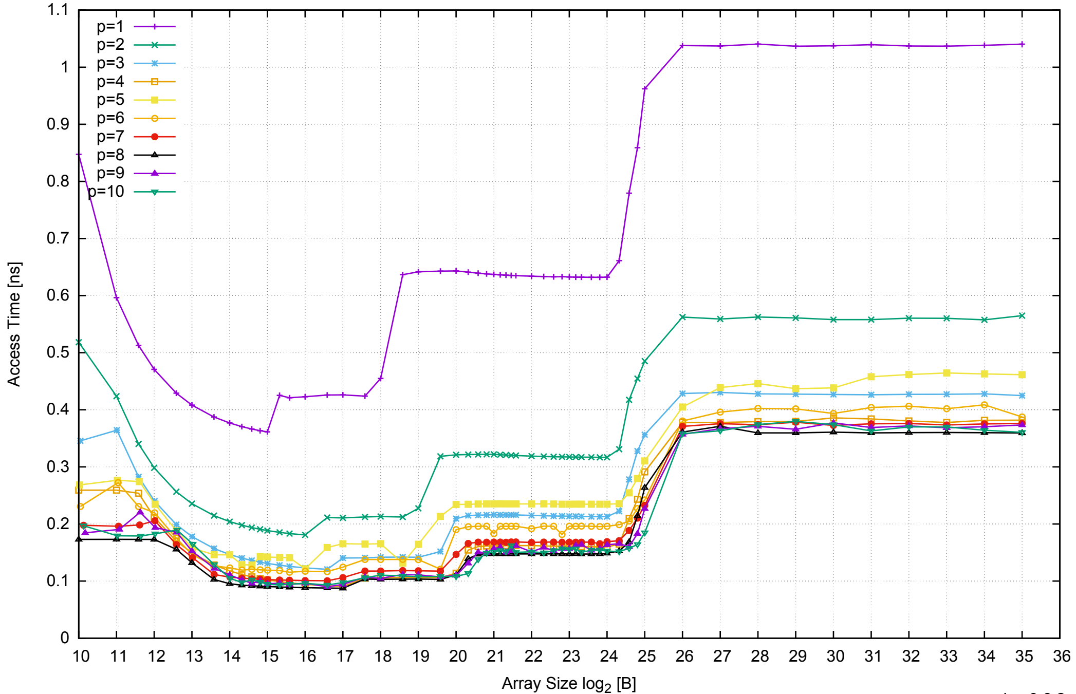
AWS i2.2xlarge - Intel Xeon E5-2670 v2, 2.50 GHz 61GB - Parallel Memory Access Time - ScanRead128PtrSimpleLoop
