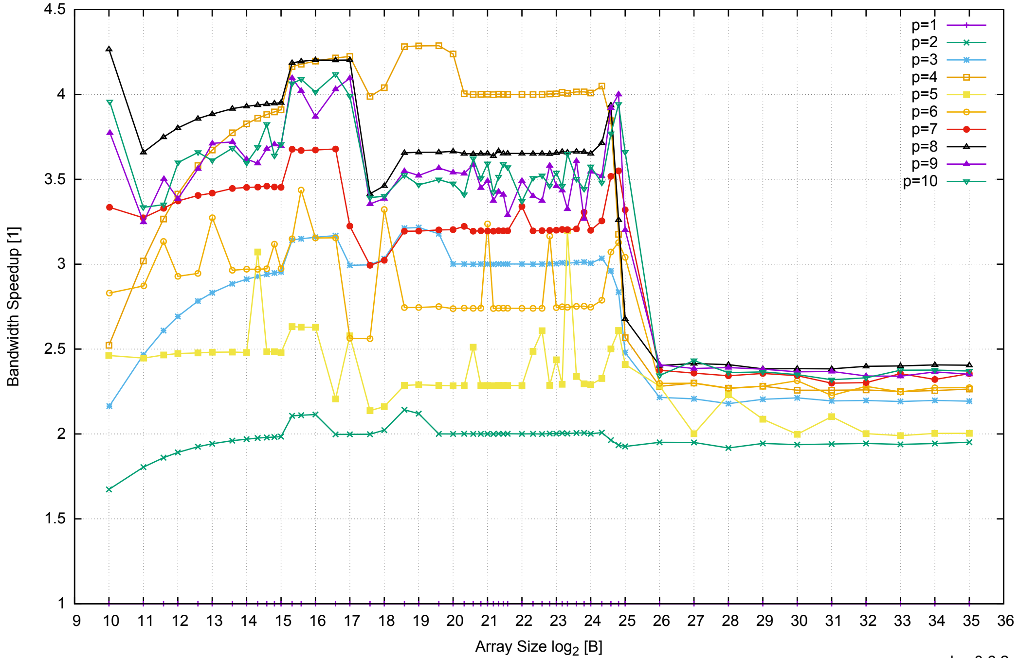
AWS i2.2xlarge - Intel Xeon E5-2670 v2, 2.50 GHz 61GB - Speedup of Parallel Memory Bandwidth - ScanWrite32PtrSimpleLoop
