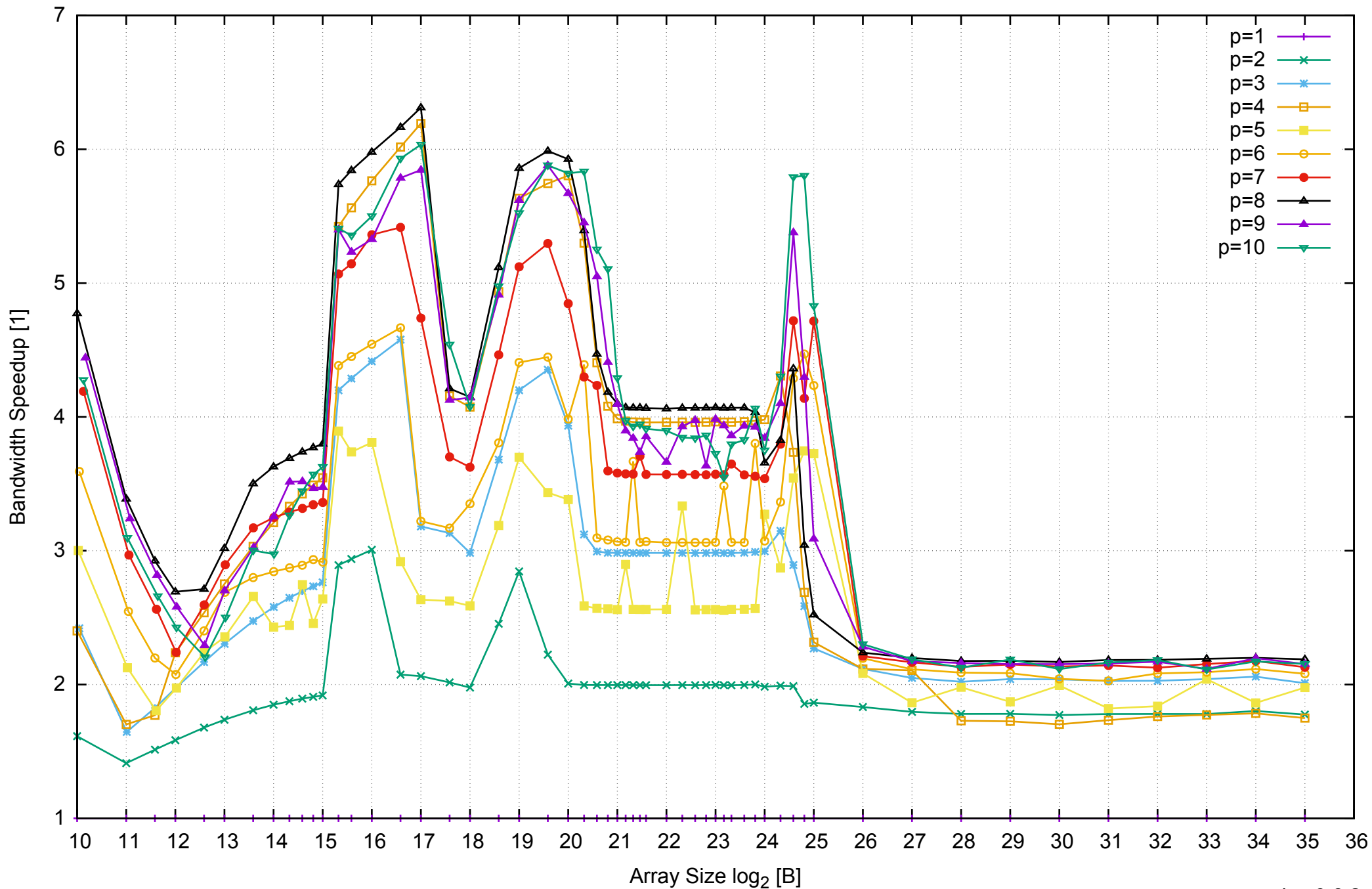
AWS i2.2xlarge - Intel Xeon E5-2670 v2, 2.50 GHz 61GB - Speedup of Parallel Memory Bandwidth - ScanWrite128PtrSimpleLoop
