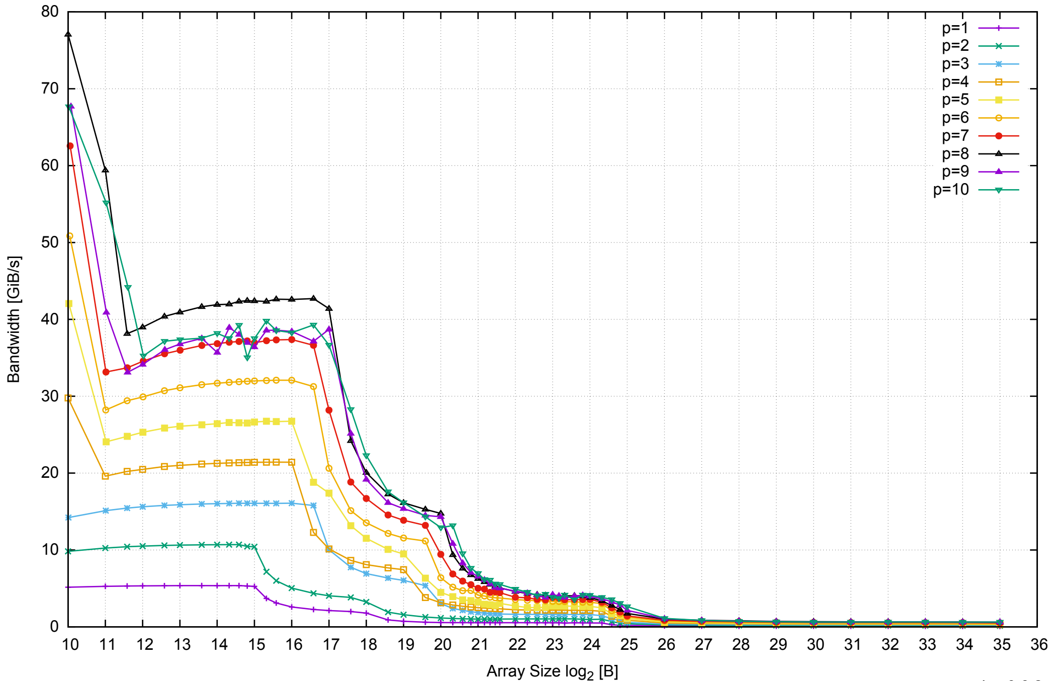
AWS i2.2xlarge - Intel Xeon E5-2670 v2, 2.50 GHz 61GB - Parallel Memory Bandwidth - PermRead64SimpleLoop
