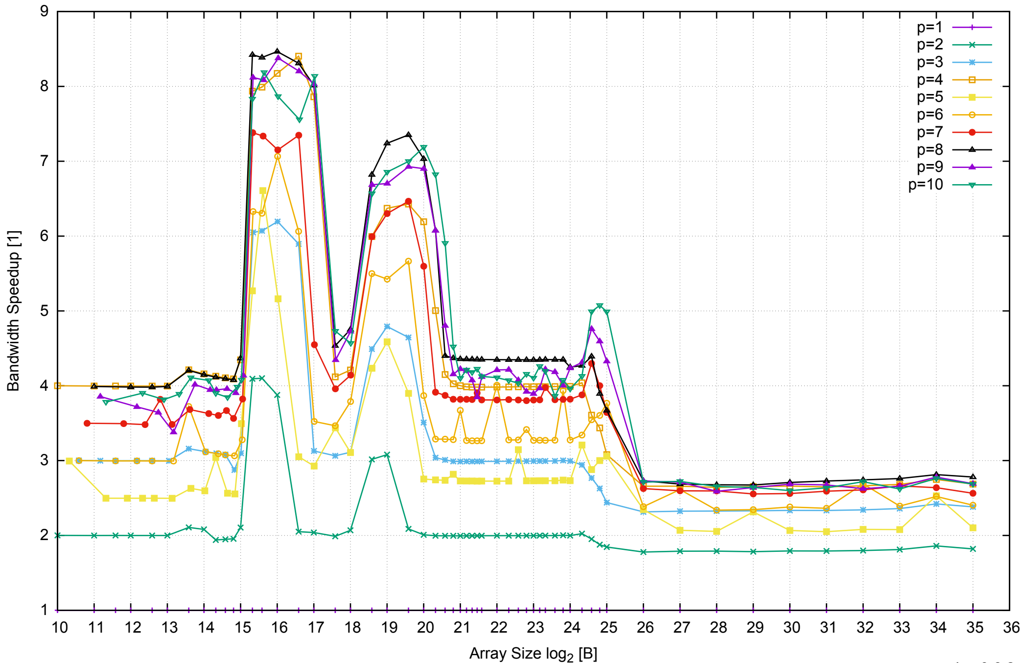
AWS i2.2xlarge - Intel Xeon E5-2670 v2, 2.50 GHz 61GB - Speedup of Parallel Memory Bandwidth - ScanRead128PtrUnrollLoop
