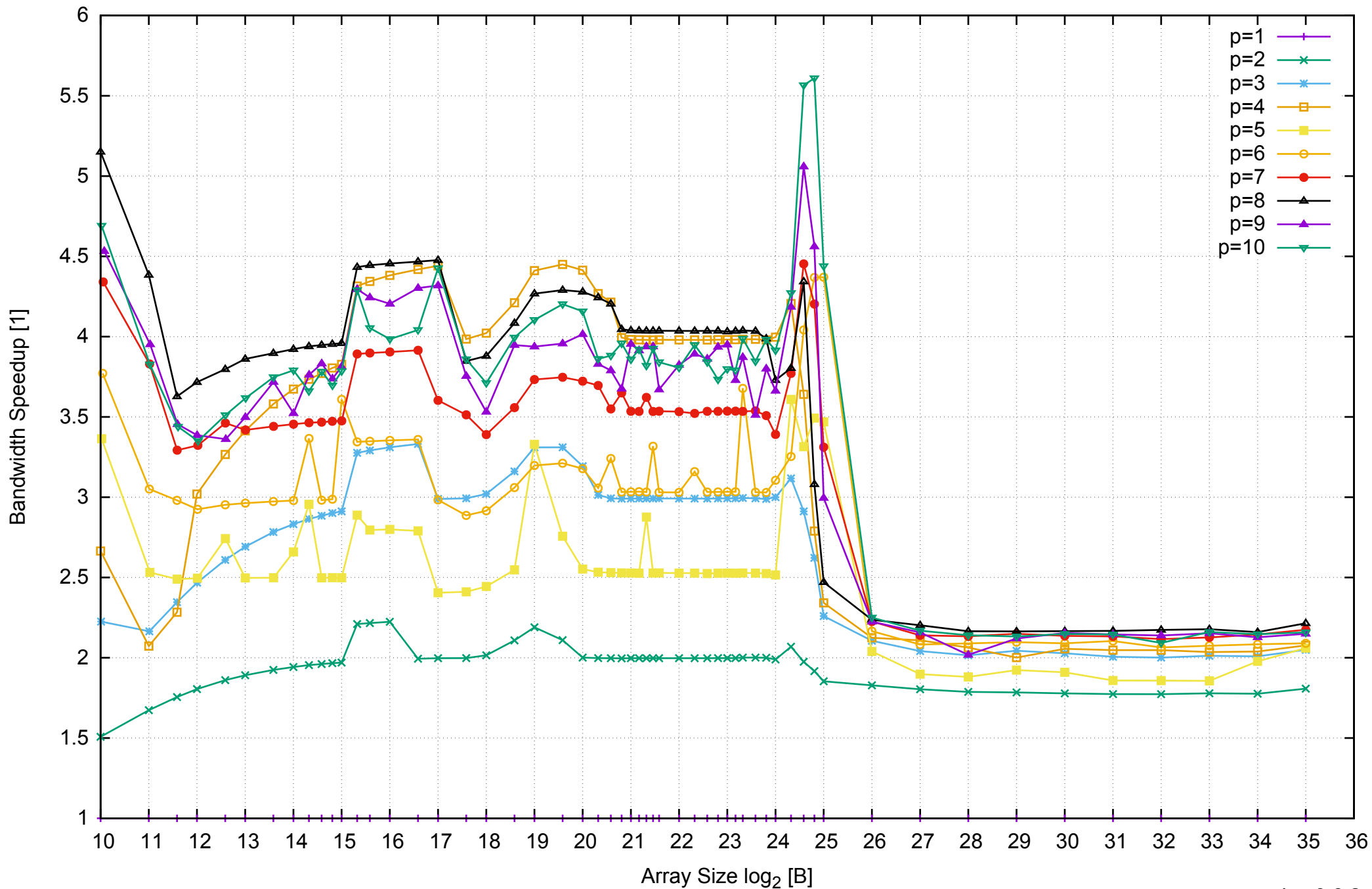
AWS i2.2xlarge - Intel Xeon E5-2670 v2, 2.50 GHz 61GB - Speedup of Parallel Memory Bandwidth - ScanWrite64IndexSimpleLoop
