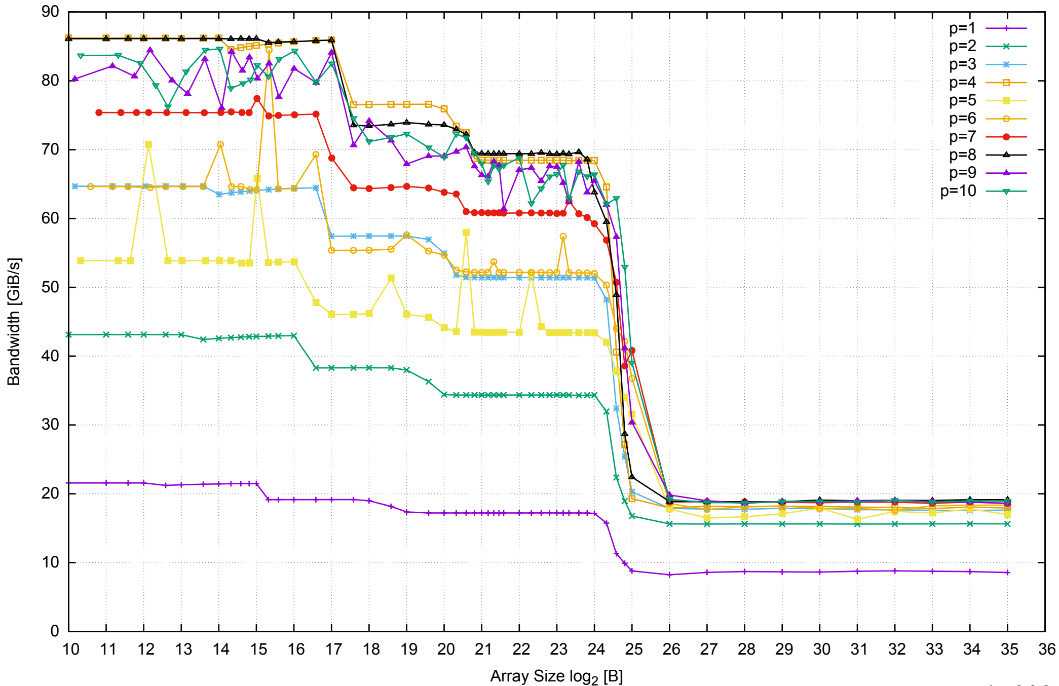
AWS i2.2xlarge - Intel Xeon E5-2670 v2, 2.50 GHz 61GB - Parallel Memory Bandwidth - ScanWrite64IndexUnrollLoop
