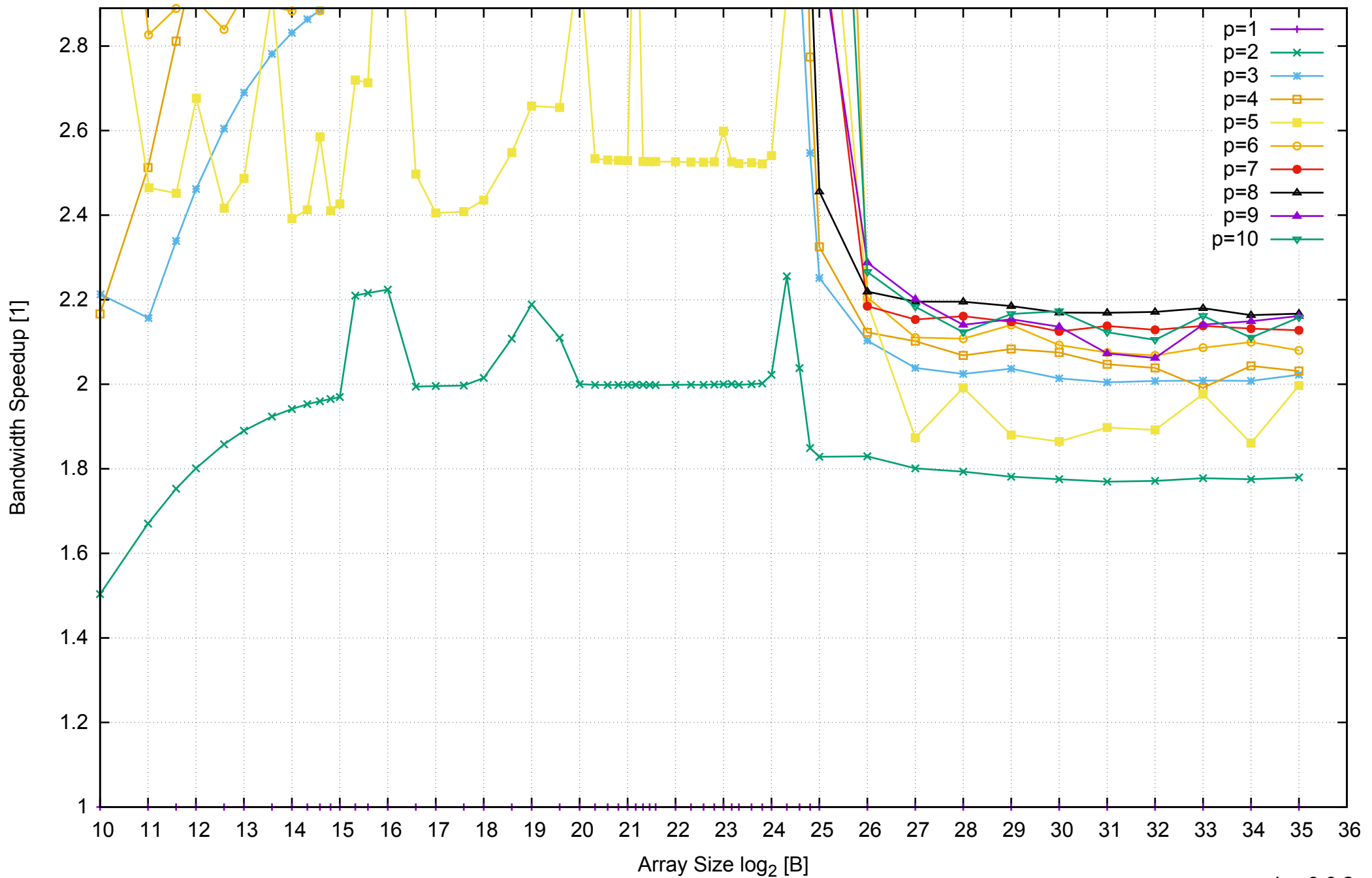
AWS i2.2xlarge - Intel Xeon E5-2670 v2, 2.50 GHz 61GB - Speedup of Parallel Memory Bandwidth (enlarged) - ScanWrite64PtrSimpleLoop
