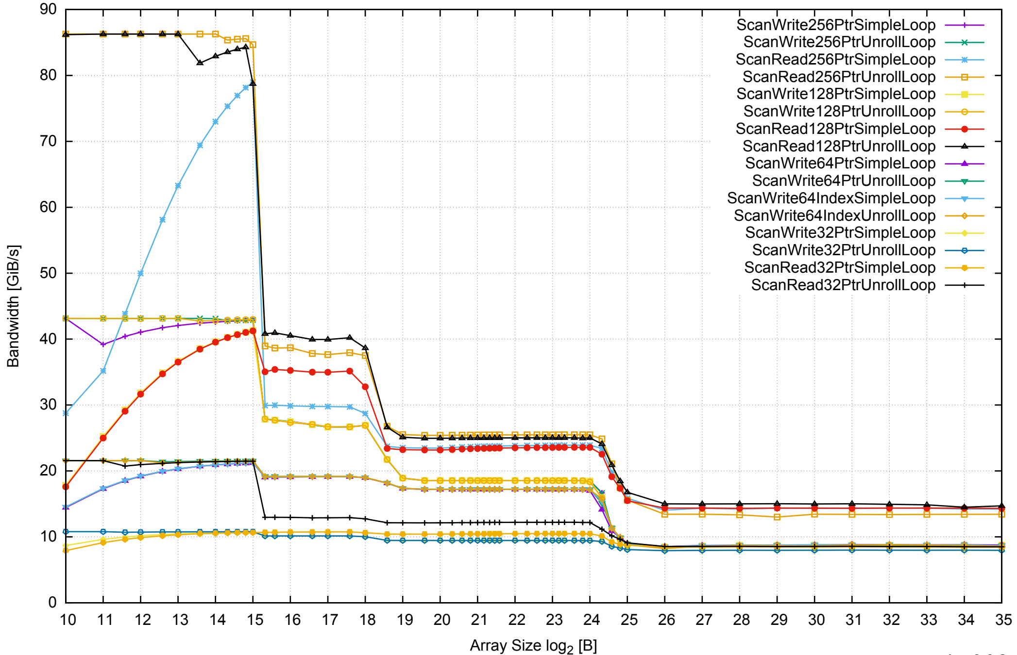
AWS i2.2xlarge - Intel Xeon E5-2670 v2, 2.50 GHz 61GB - One Thread Memory Bandwidth (only 64-bit Reads)
