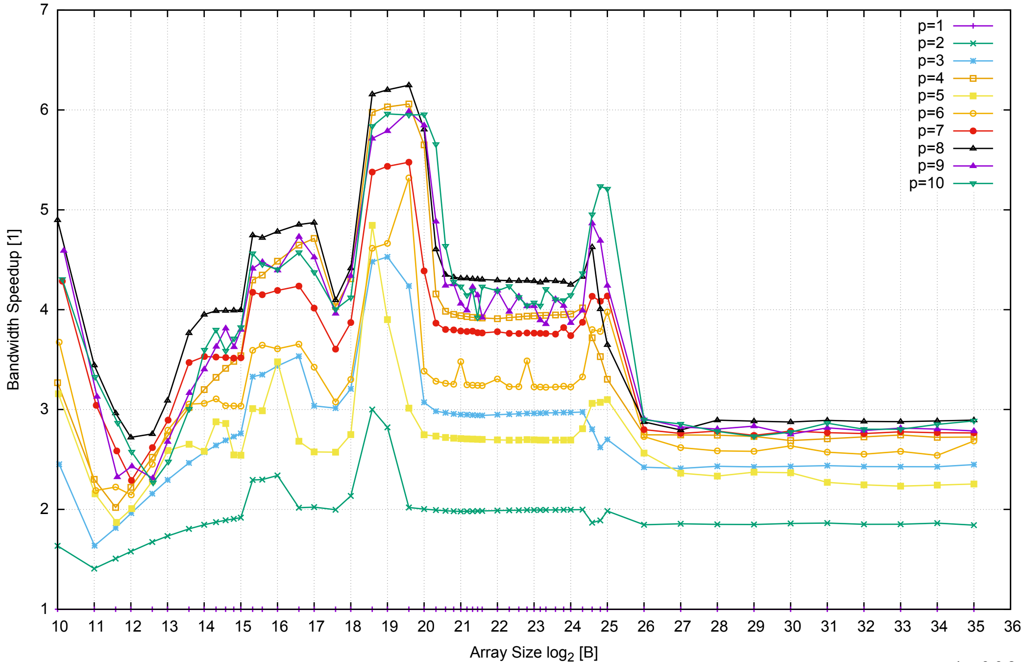
AWS i2.2xlarge - Intel Xeon E5-2670 v2, 2.50 GHz 61GB - Speedup of Parallel Memory Bandwidth - ScanRead128PtrSimpleLoop
