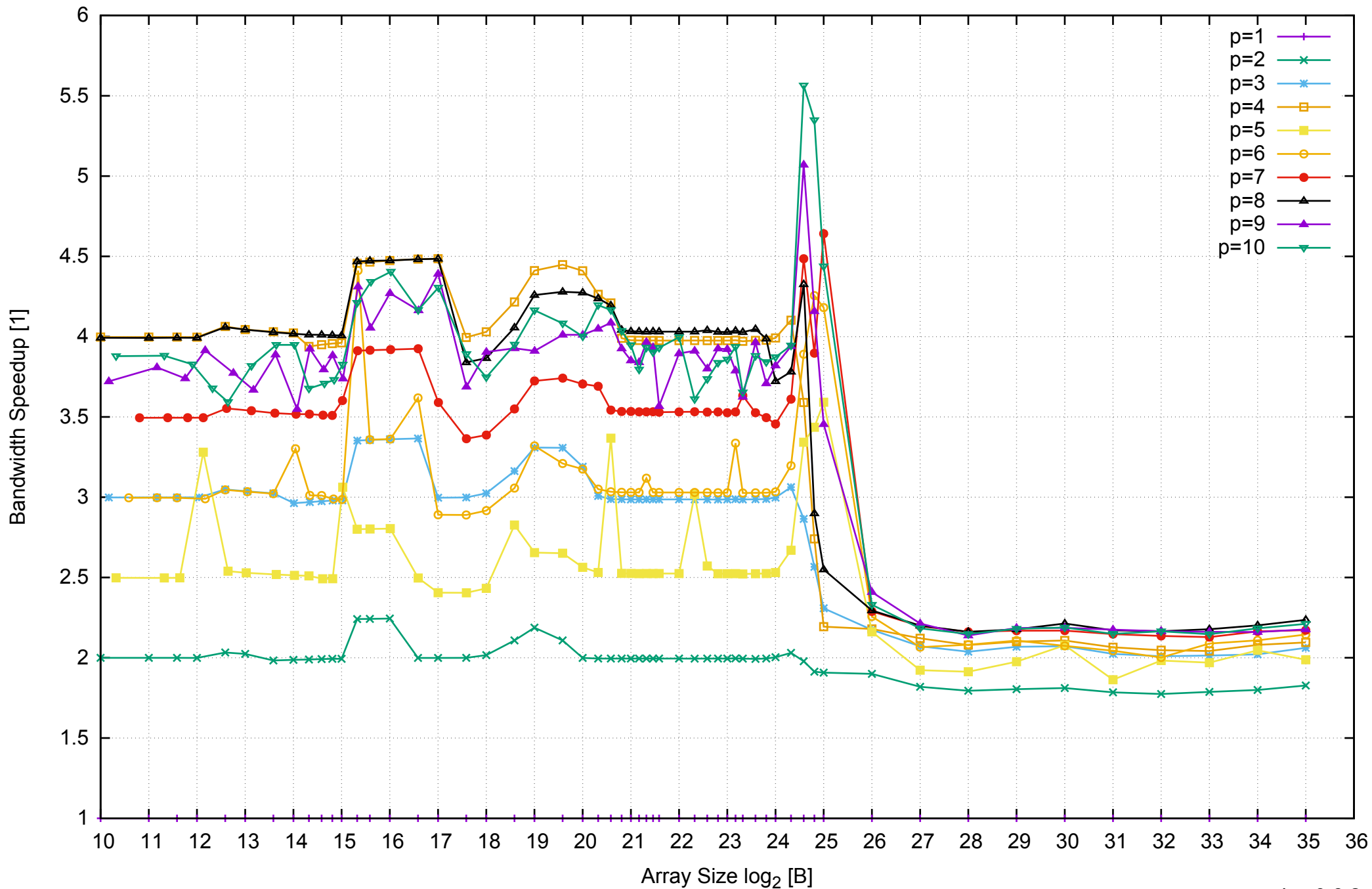
AWS i2.2xlarge - Intel Xeon E5-2670 v2, 2.50 GHz 61GB - Speedup of Parallel Memory Bandwidth - ScanWrite64IndexUnrollLoop
