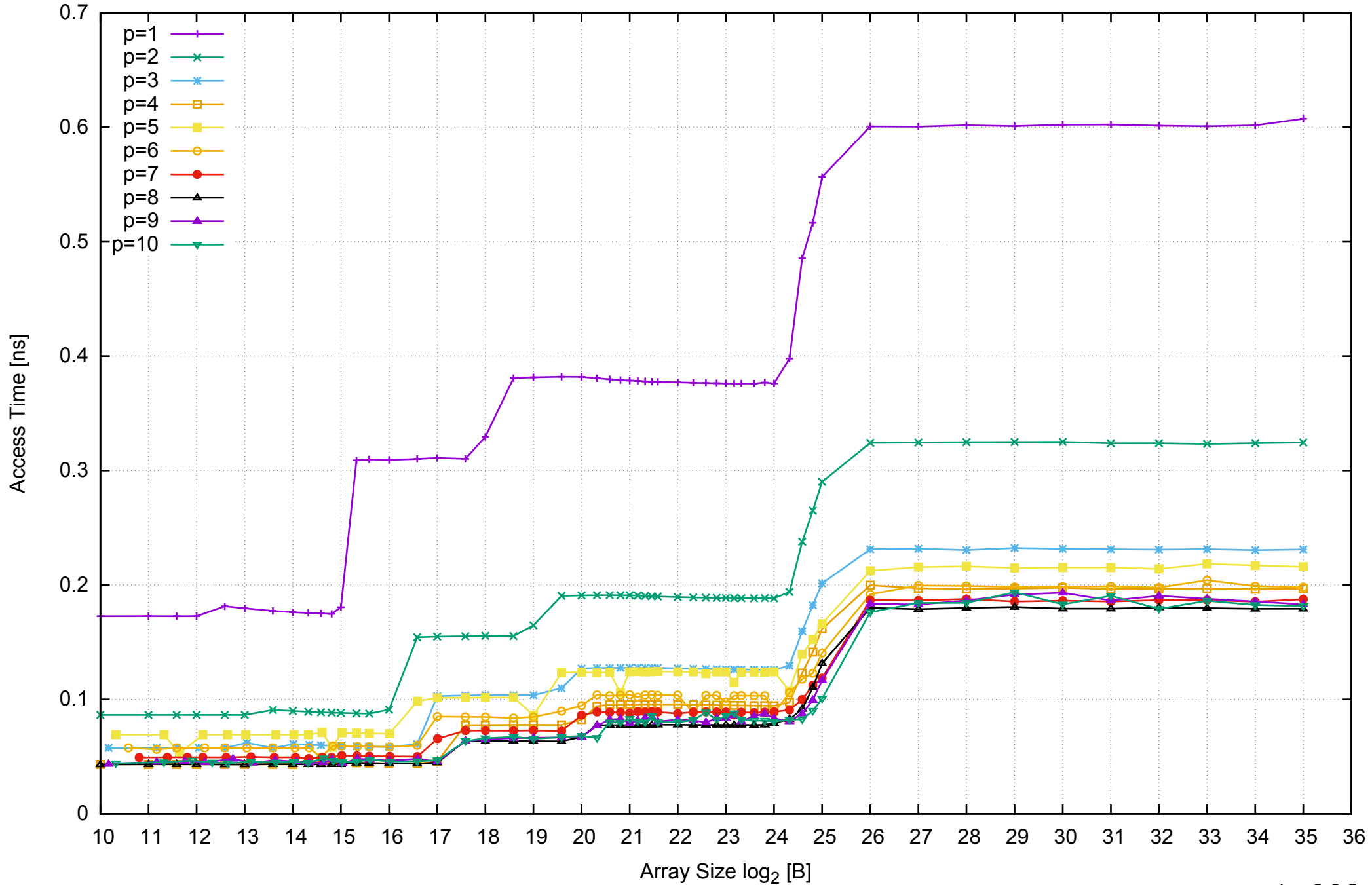
AWS i2.2xlarge - Intel Xeon E5-2670 v2, 2.50 GHz 61GB - Parallel Memory Access Time - ScanRead64IndexUnrollLoop
