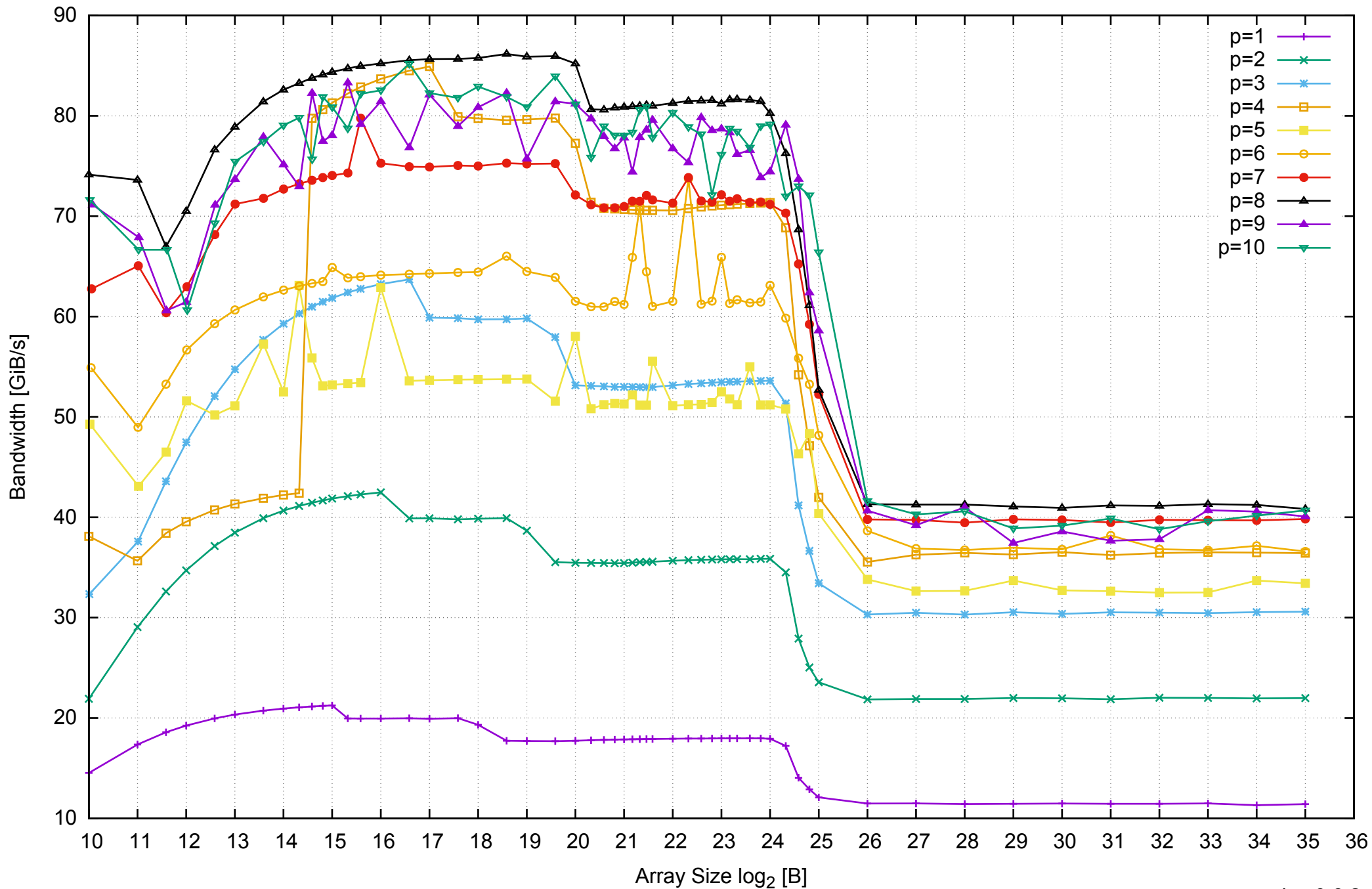
AWS i2.2xlarge - Intel Xeon E5-2670 v2, 2.50 GHz 61GB - Parallel Memory Bandwidth - ScanRead64PtrSimpleLoop
