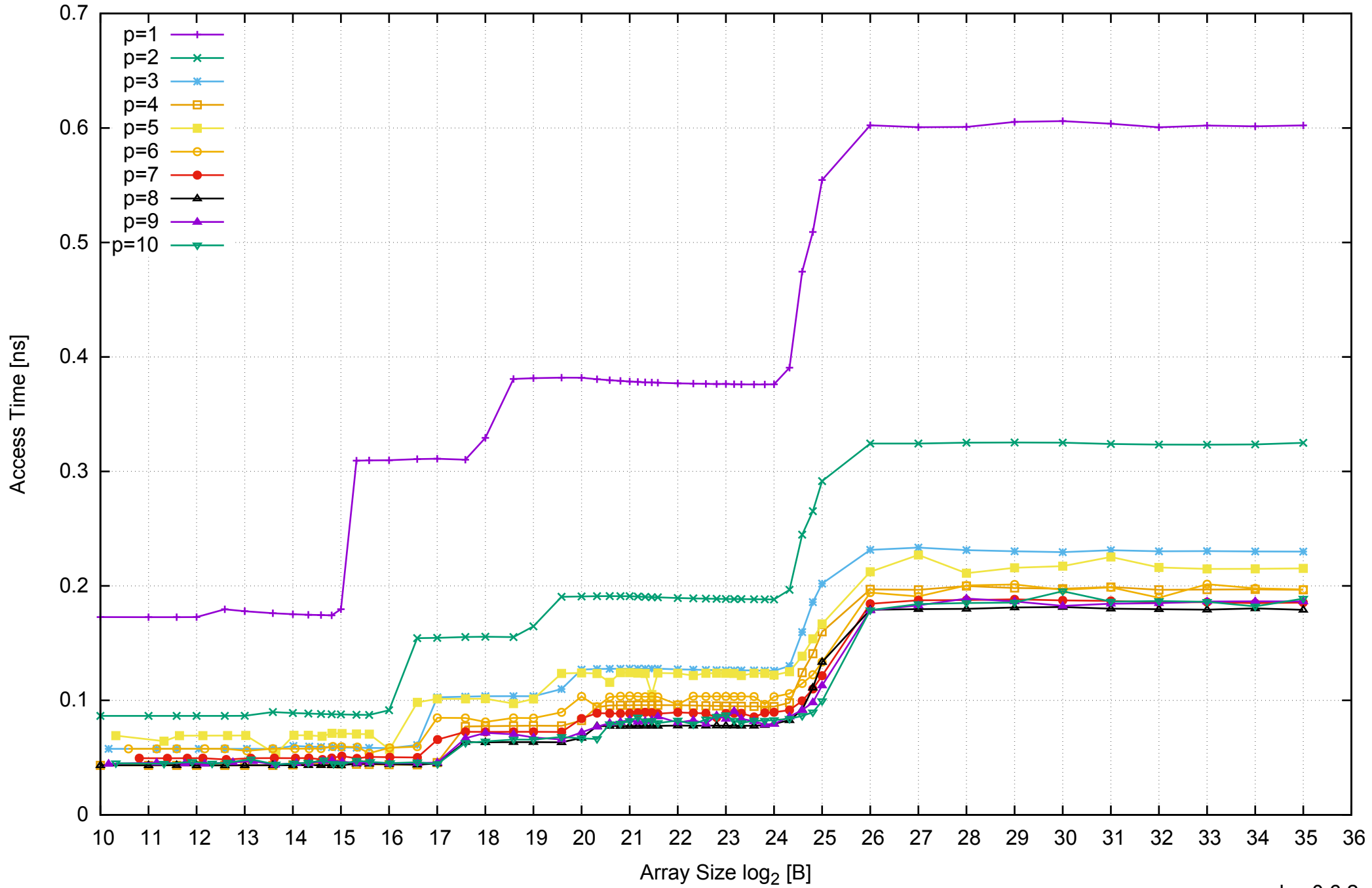
AWS i2.2xlarge - Intel Xeon E5-2670 v2, 2.50 GHz 61GB - Parallel Memory Access Time - ScanRead64PtrUnrollLoop
