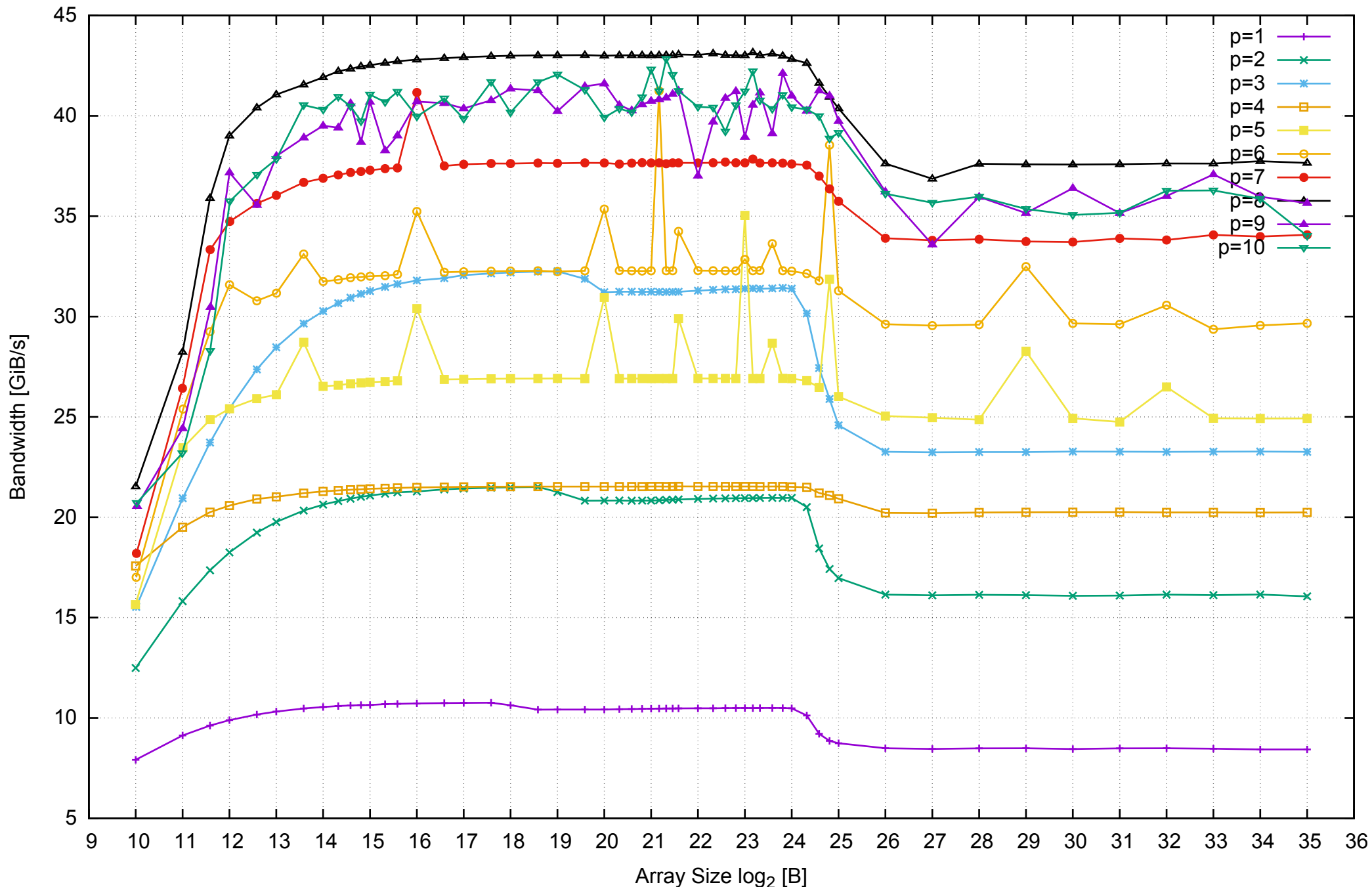
AWS i2.2xlarge - Intel Xeon E5-2670 v2, 2.50 GHz 61GB - Parallel Memory Bandwidth - ScanRead32PtrSimpleLoop
