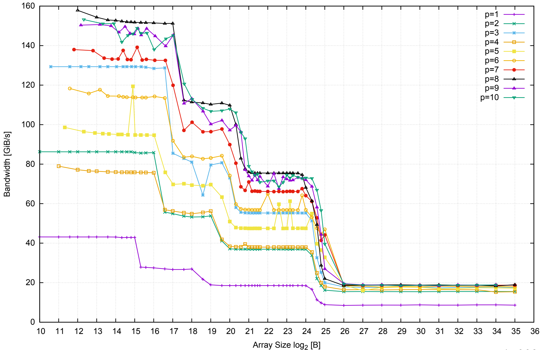
AWS i2.2xlarge - Intel Xeon E5-2670 v2, 2.50 GHz 61GB - Parallel Memory Bandwidth - ScanWrite256PtrUnrollLoop
