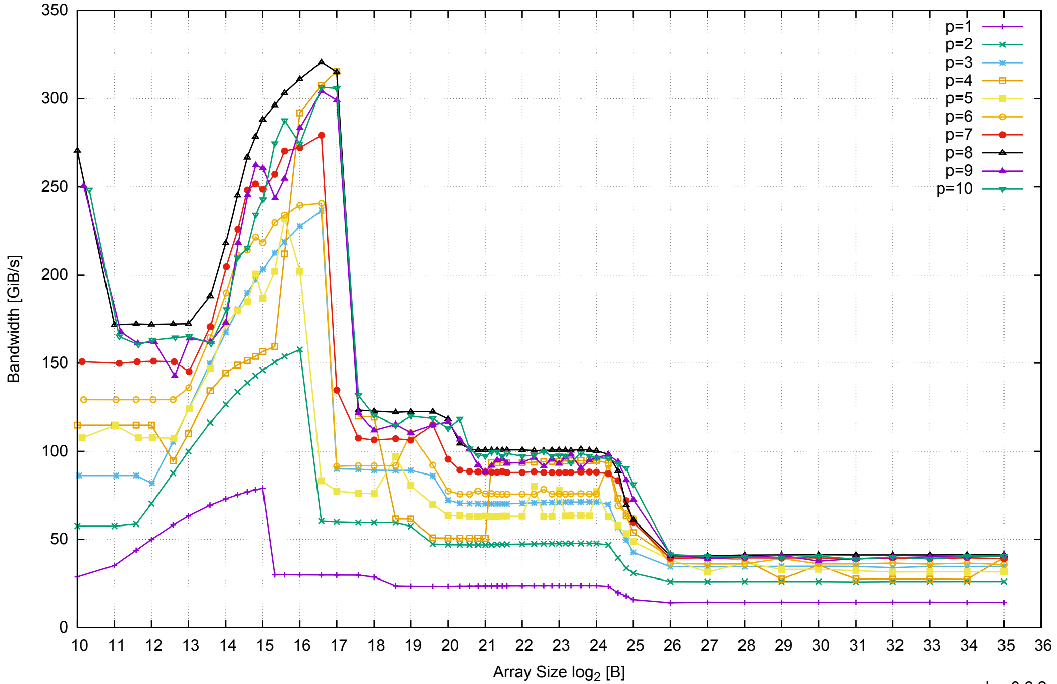
AWS i2.2xlarge - Intel Xeon E5-2670 v2, 2.50 GHz 61GB - Parallel Memory Bandwidth - ScanRead256PtrSimpleLoop
