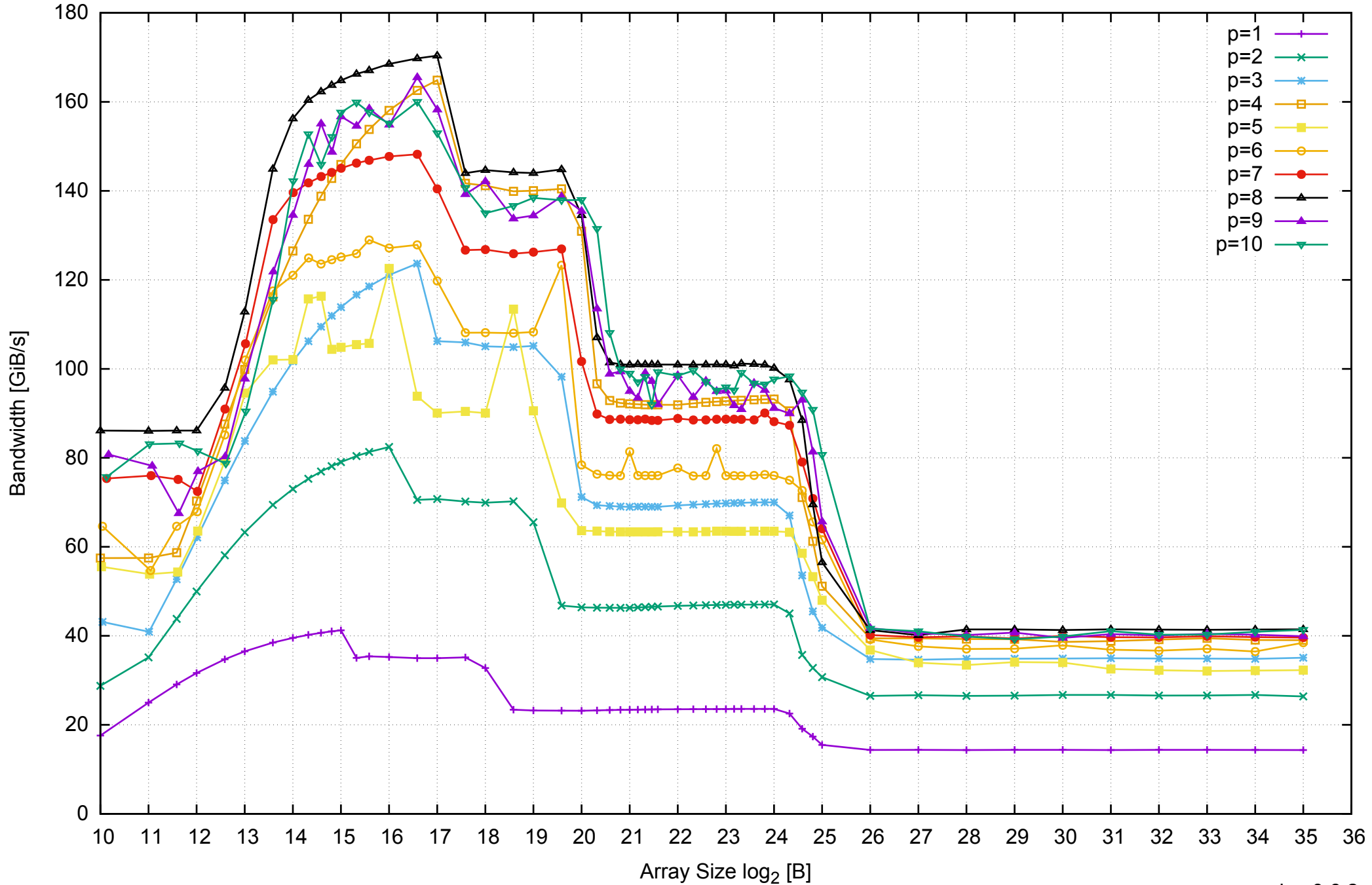
AWS i2.2xlarge - Intel Xeon E5-2670 v2, 2.50 GHz 61GB - Parallel Memory Bandwidth - ScanRead128PtrSimpleLoop
