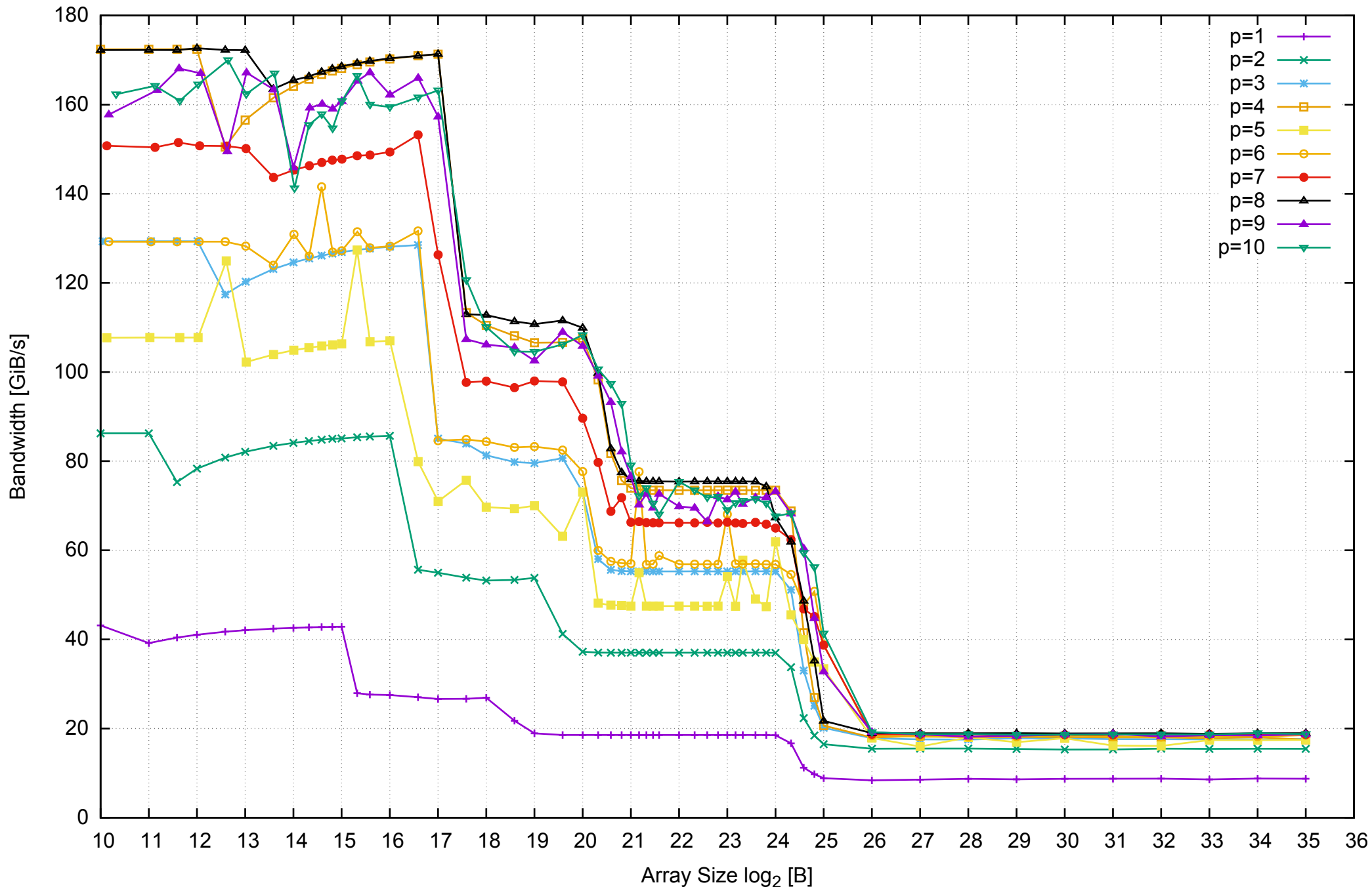
AWS i2.2xlarge - Intel Xeon E5-2670 v2, 2.50 GHz 61GB - Parallel Memory Bandwidth - ScanWrite256PtrSimpleLoop
