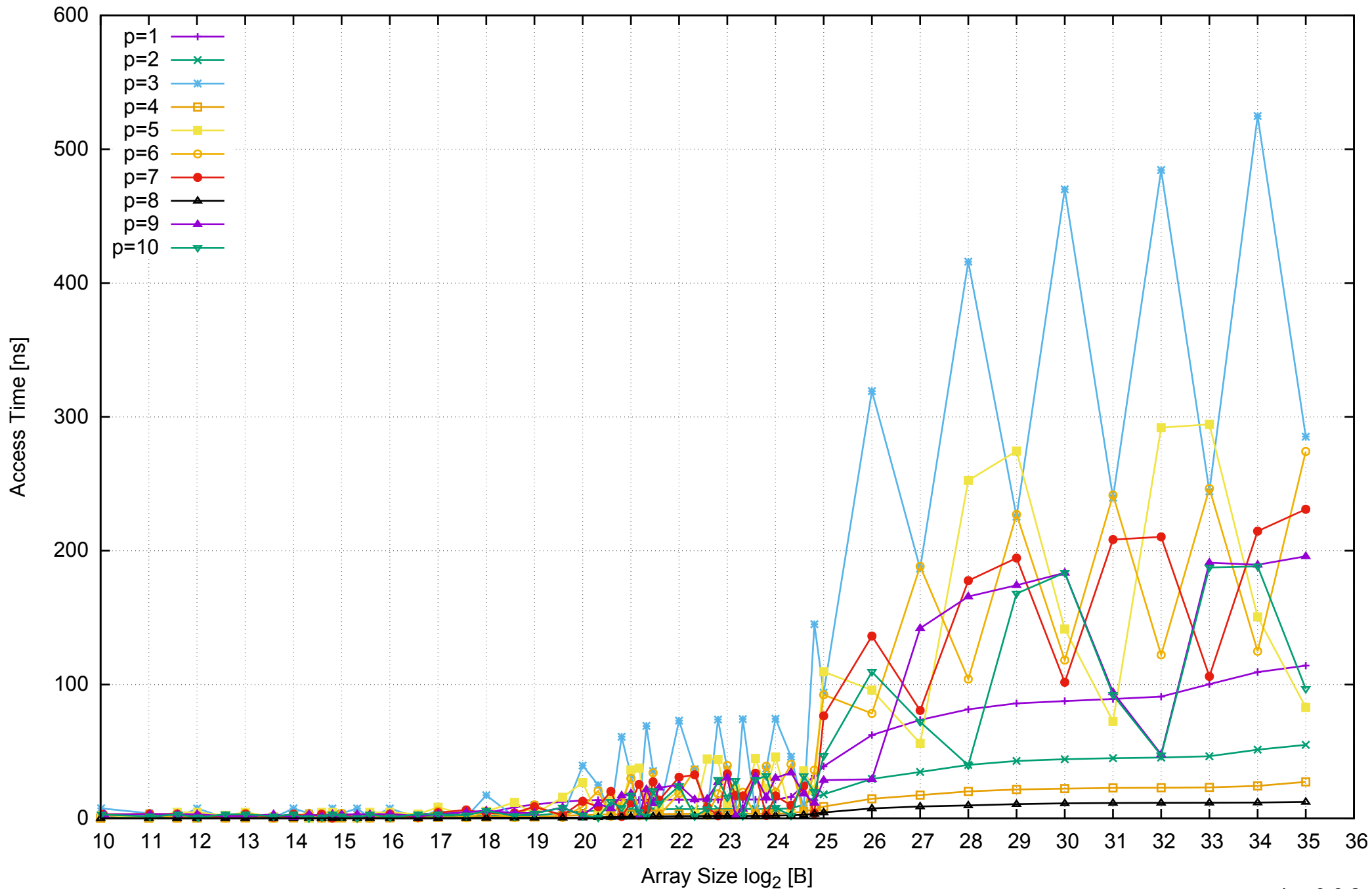
AWS i2.2xlarge - Intel Xeon E5-2670 v2, 2.50 GHz 61GB - Parallel Memory Access Time - PermRead64UnrollLoop
