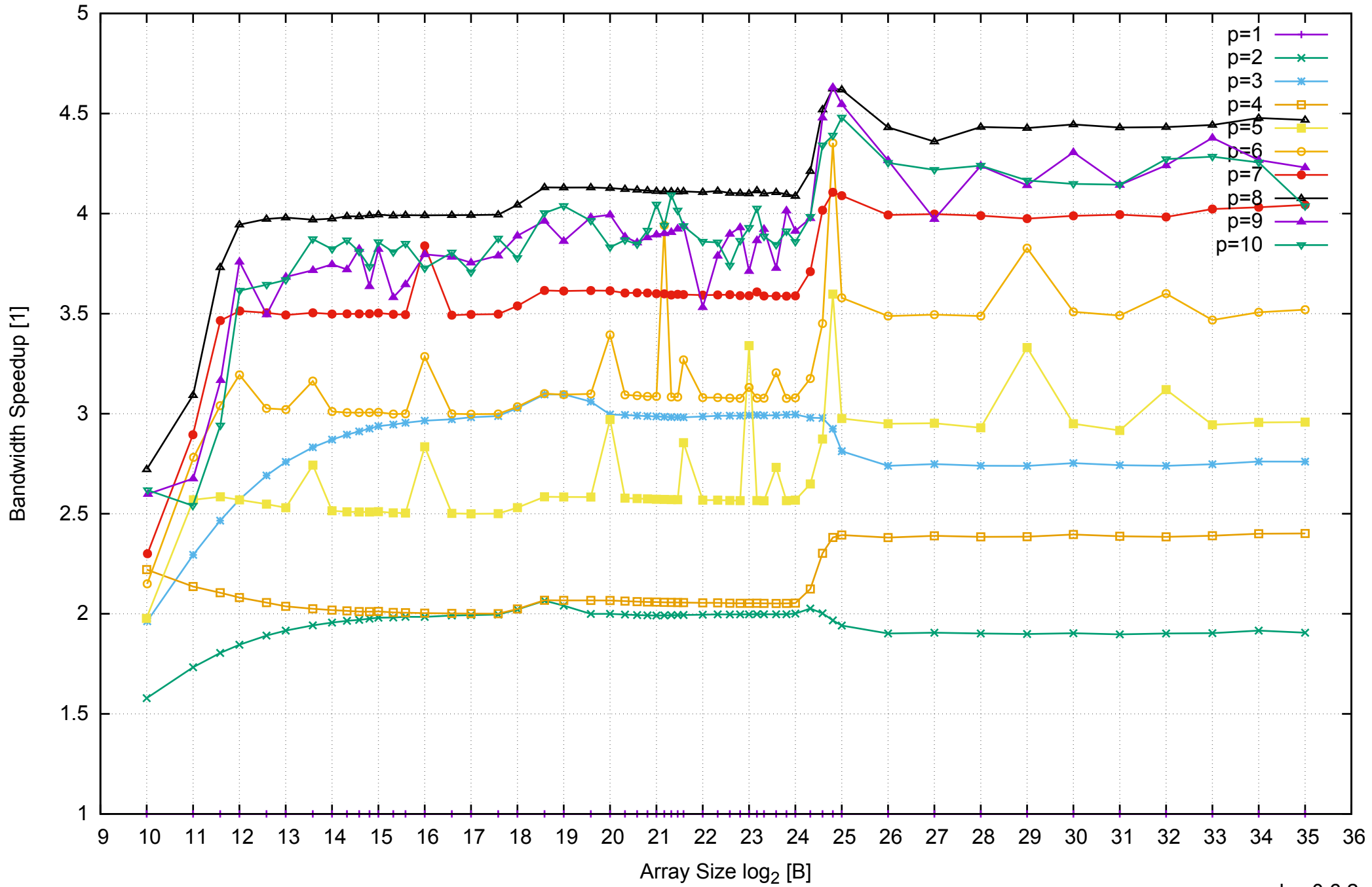
AWS i2.2xlarge - Intel Xeon E5-2670 v2, 2.50 GHz 61GB - Speedup of Parallel Memory Bandwidth - ScanRead32PtrSimpleLoop
