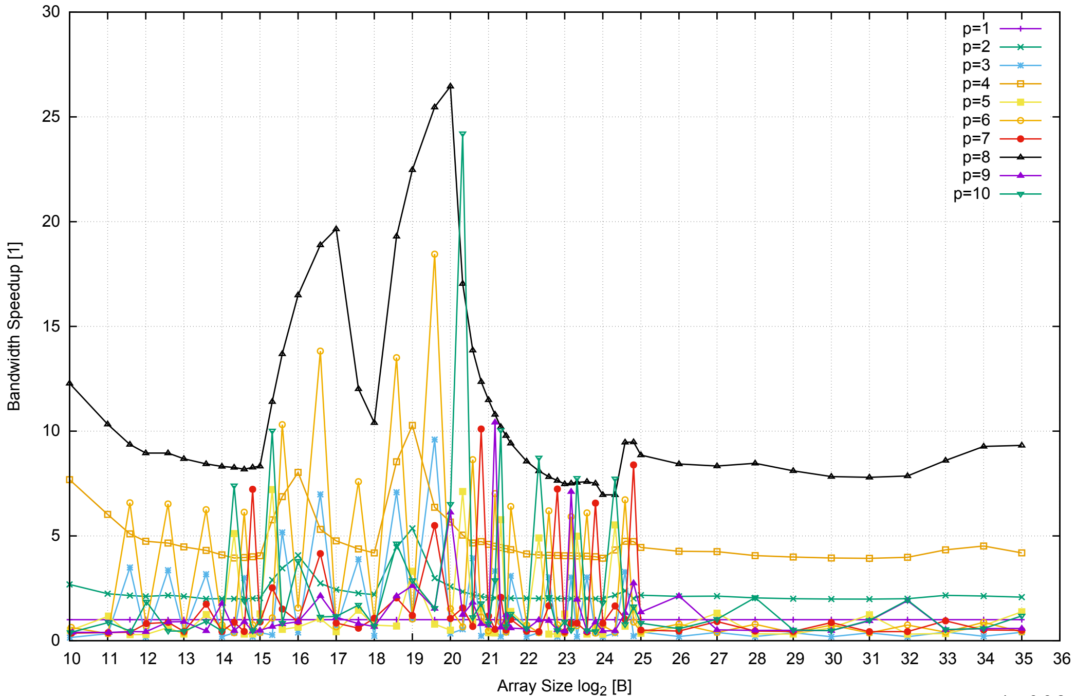
AWS i2.2xlarge - Intel Xeon E5-2670 v2, 2.50 GHz 61GB - Speedup of Parallel Memory Bandwidth - PermRead64UnrollLoop
