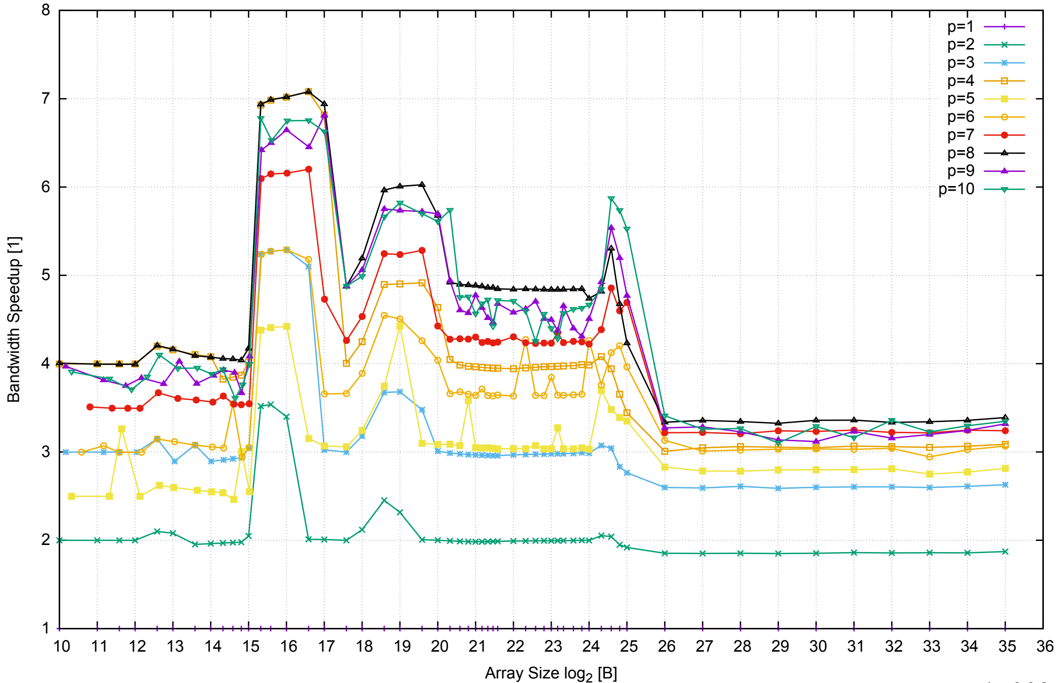
AWS i2.2xlarge - Intel Xeon E5-2670 v2, 2.50 GHz 61GB - Speedup of Parallel Memory Bandwidth - ScanRead64IndexUnrollLoop
