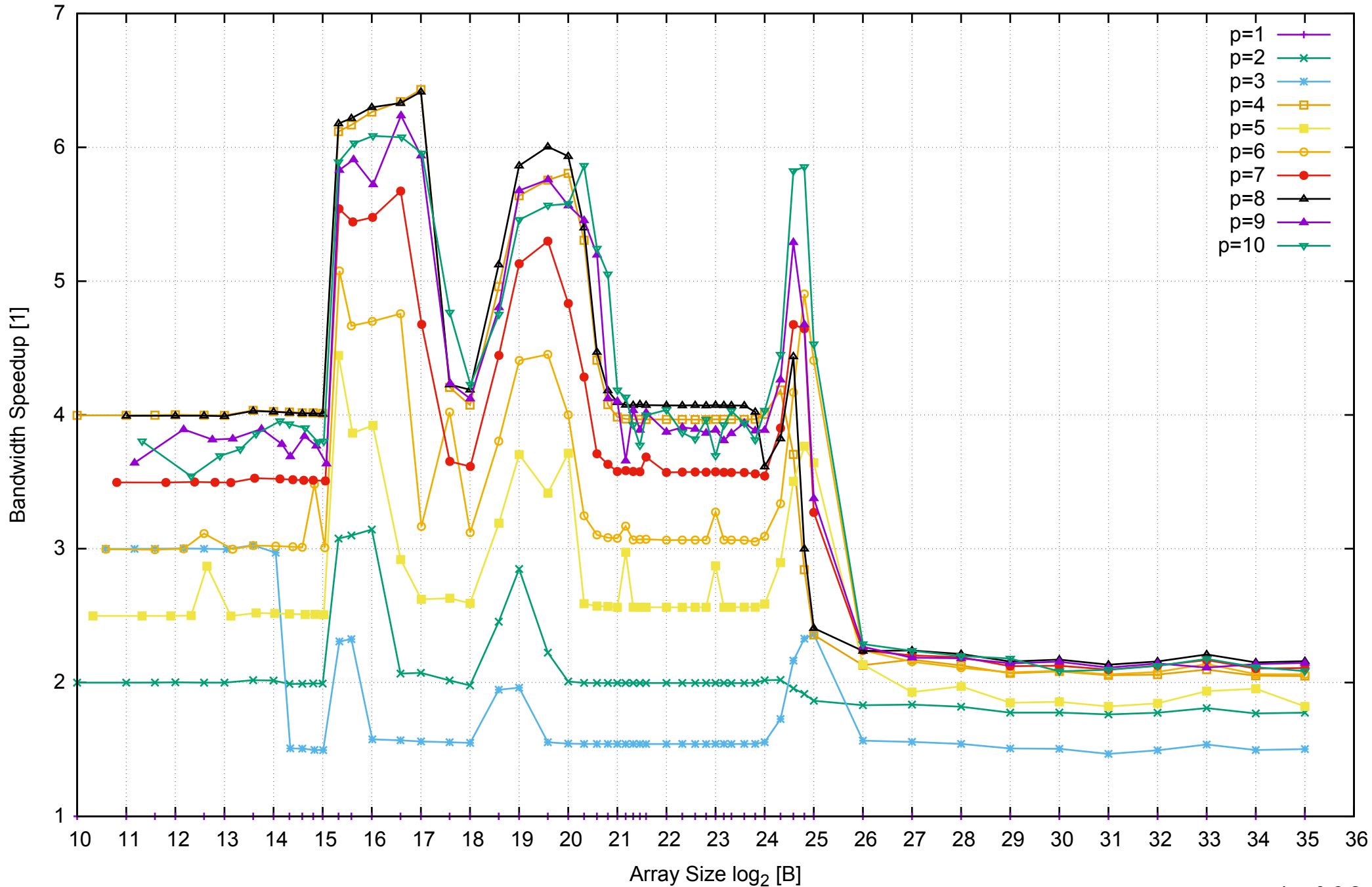
AWS i2.2xlarge - Intel Xeon E5-2670 v2, 2.50 GHz 61GB - Speedup of Parallel Memory Bandwidth - ScanWrite128PtrUnrollLoop
