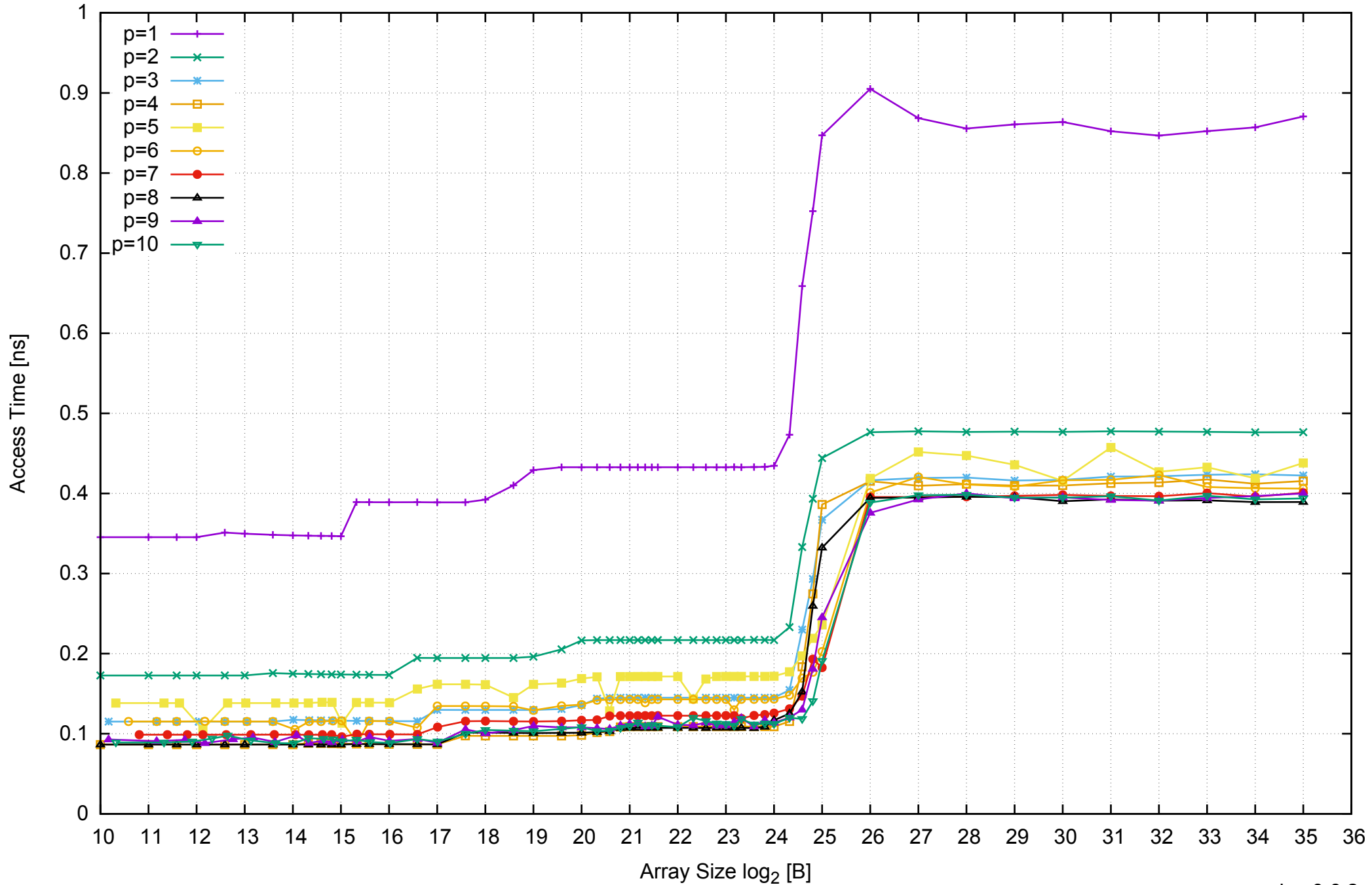
AWS i2.2xlarge - Intel Xeon E5-2670 v2, 2.50 GHz 61GB - Parallel Memory Access Time - ScanWrite64IndexUnrollLoop
