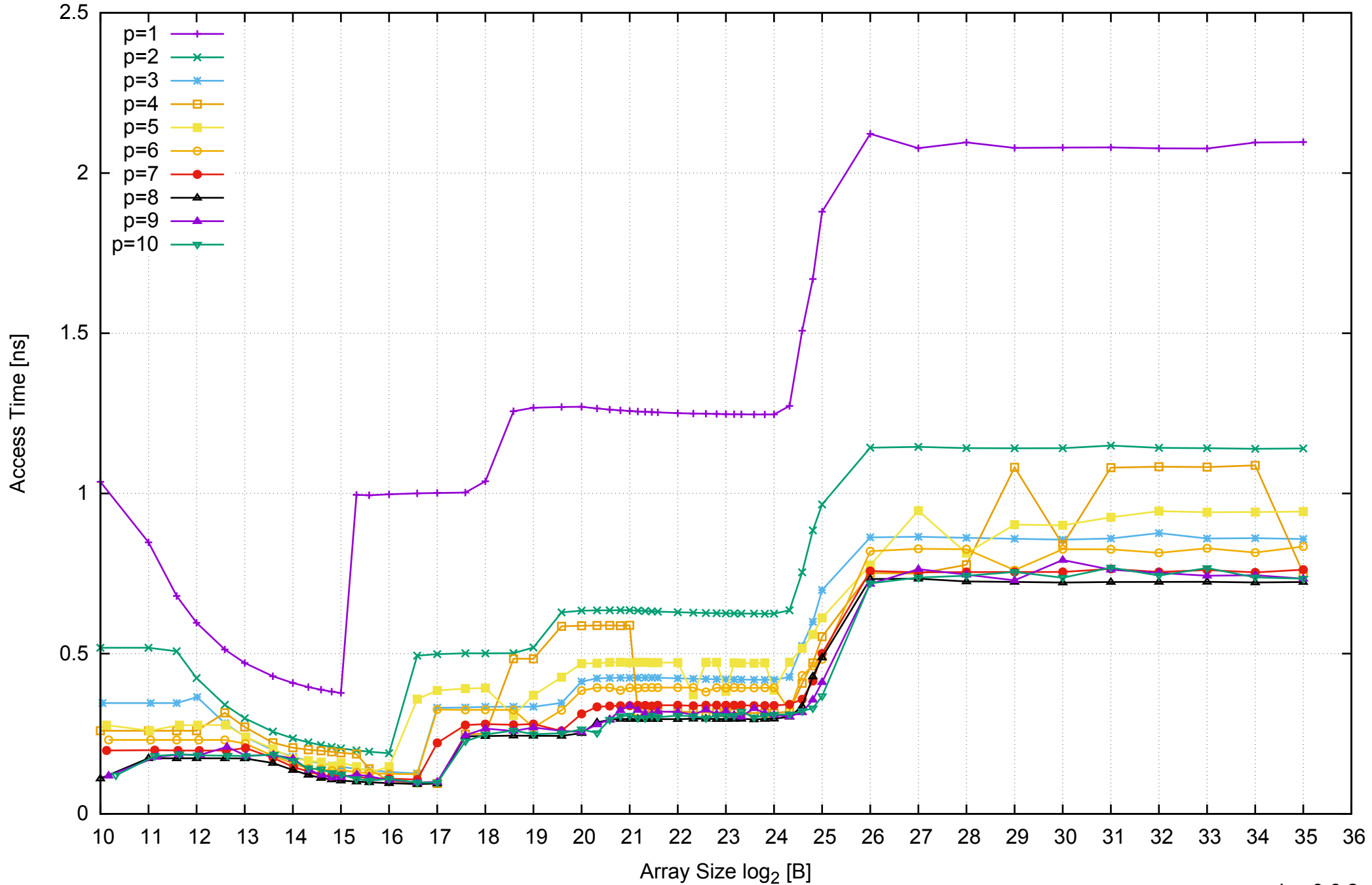
AWS i2.2xlarge - Intel Xeon E5-2670 v2, 2.50 GHz 61GB - Parallel Memory Access Time - ScanRead256PtrSimpleLoop
