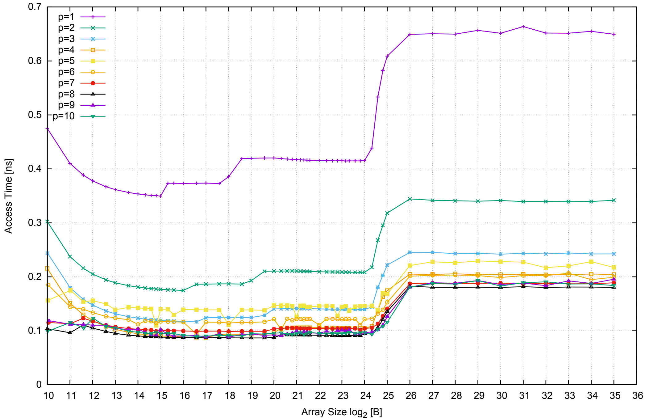
AWS i2.2xlarge - Intel Xeon E5-2670 v2, 2.50 GHz 61GB - Parallel Memory Access Time - ScanRead64IndexSimpleLoop
