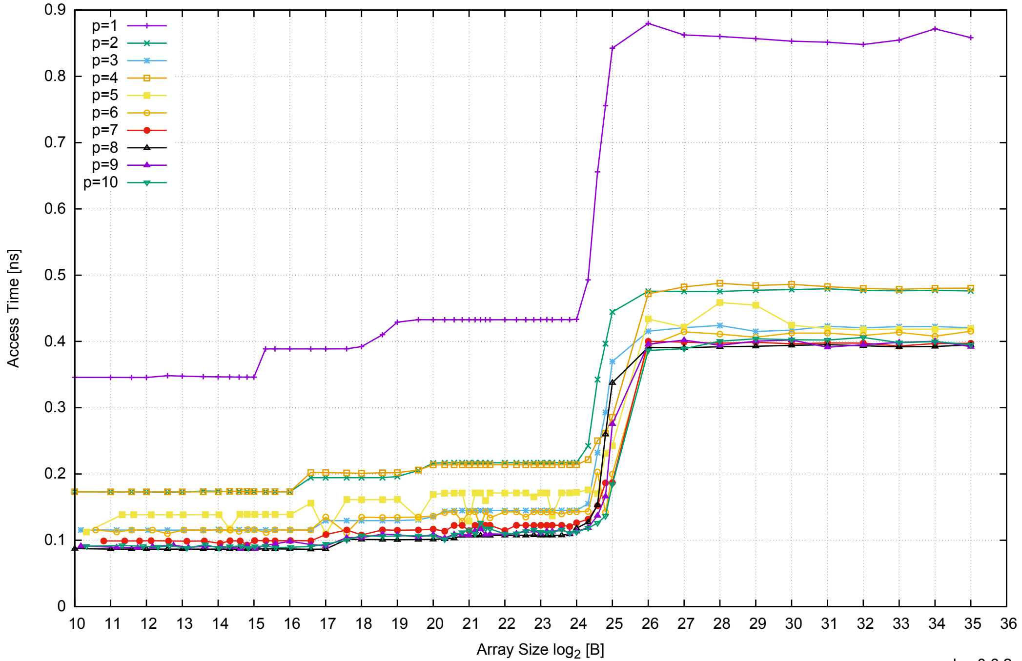
AWS i2.2xlarge - Intel Xeon E5-2670 v2, 2.50 GHz 61GB - Parallel Memory Access Time - ScanWrite64PtrUnrollLoop
