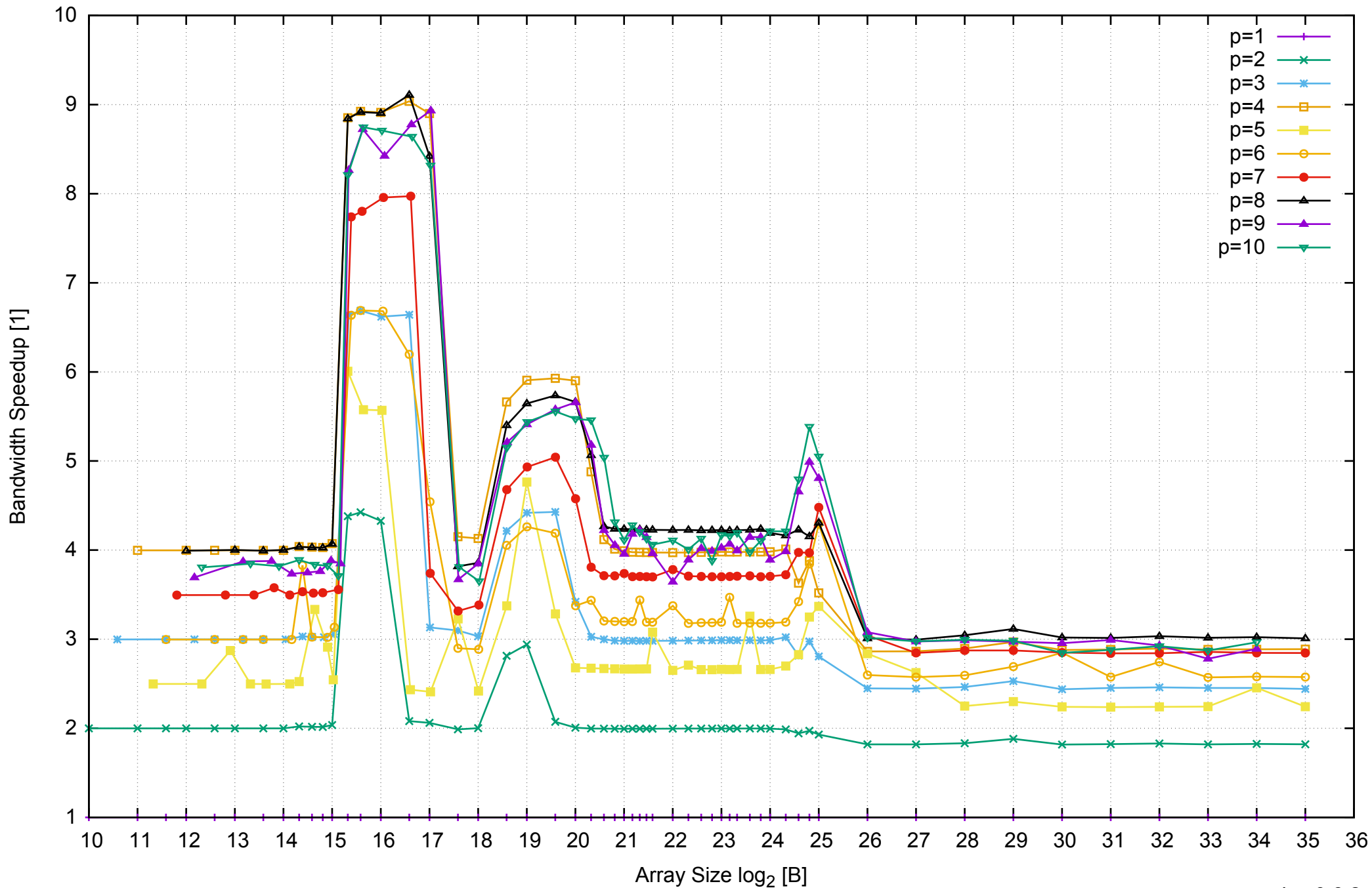
AWS i2.2xlarge - Intel Xeon E5-2670 v2, 2.50 GHz 61GB - Speedup of Parallel Memory Bandwidth - ScanRead256PtrUnrollLoop
