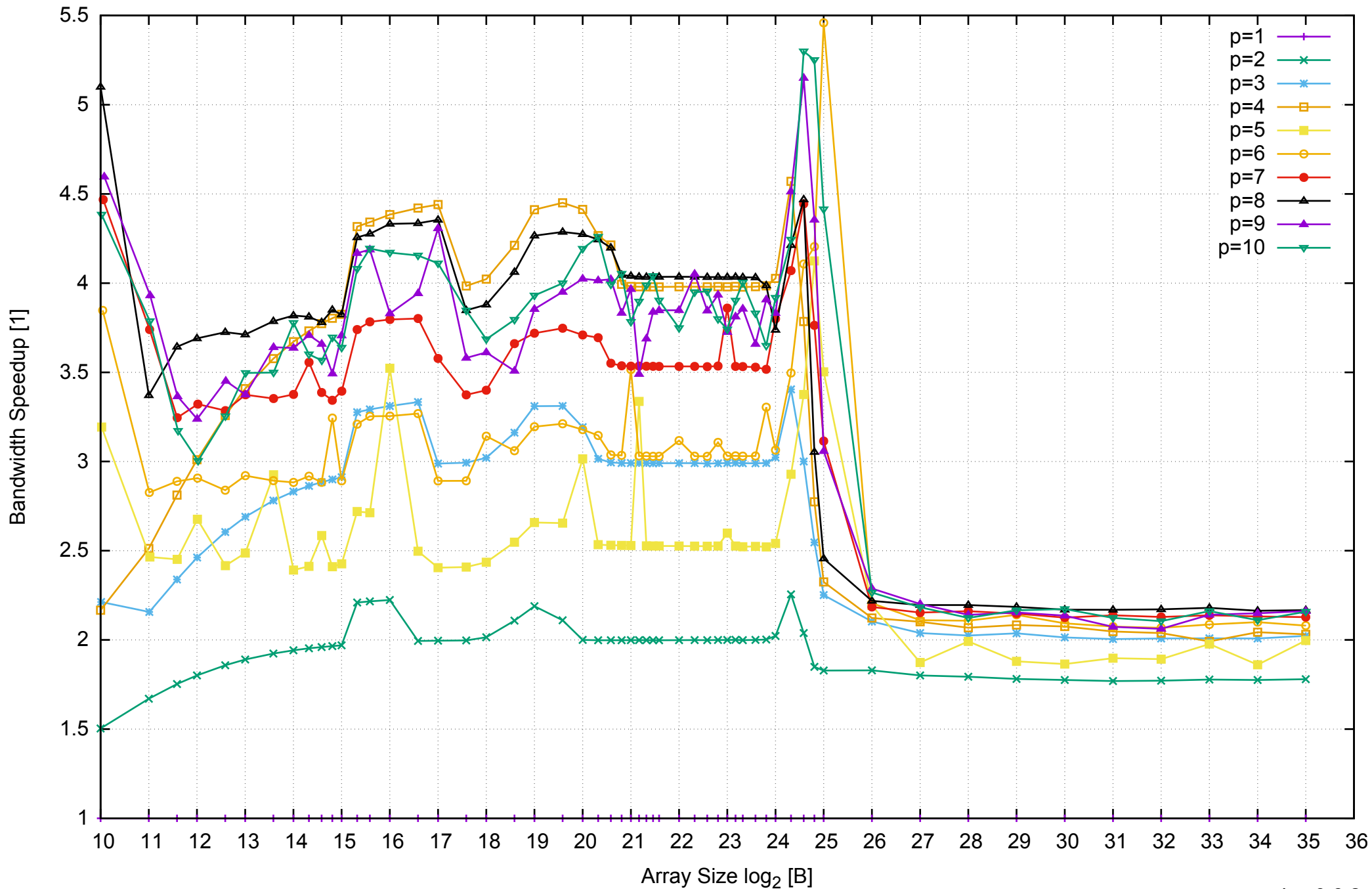
AWS i2.2xlarge - Intel Xeon E5-2670 v2, 2.50 GHz 61GB - Speedup of Parallel Memory Bandwidth - ScanWrite64PtrSimpleLoop
