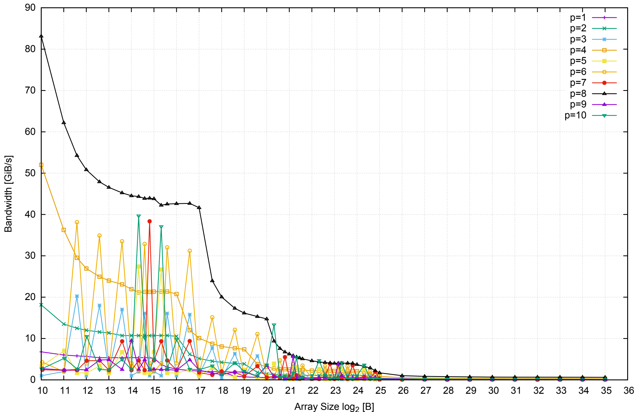
AWS i2.2xlarge - Intel Xeon E5-2670 v2, 2.50 GHz 61GB - Parallel Memory Bandwidth - PermRead64UnrollLoop
