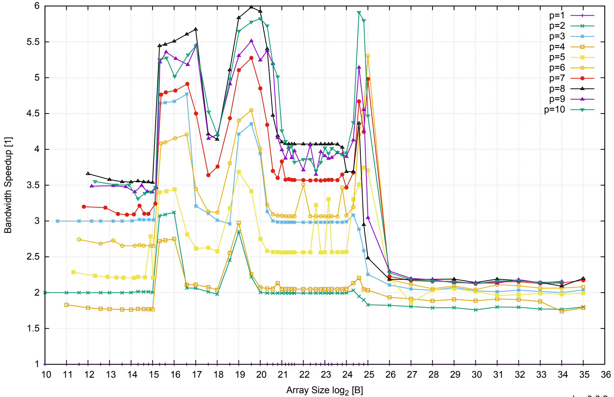
AWS i2.2xlarge - Intel Xeon E5-2670 v2, 2.50 GHz 61GB - Speedup of Parallel Memory Bandwidth - ScanWrite256PtrUnrollLoop
