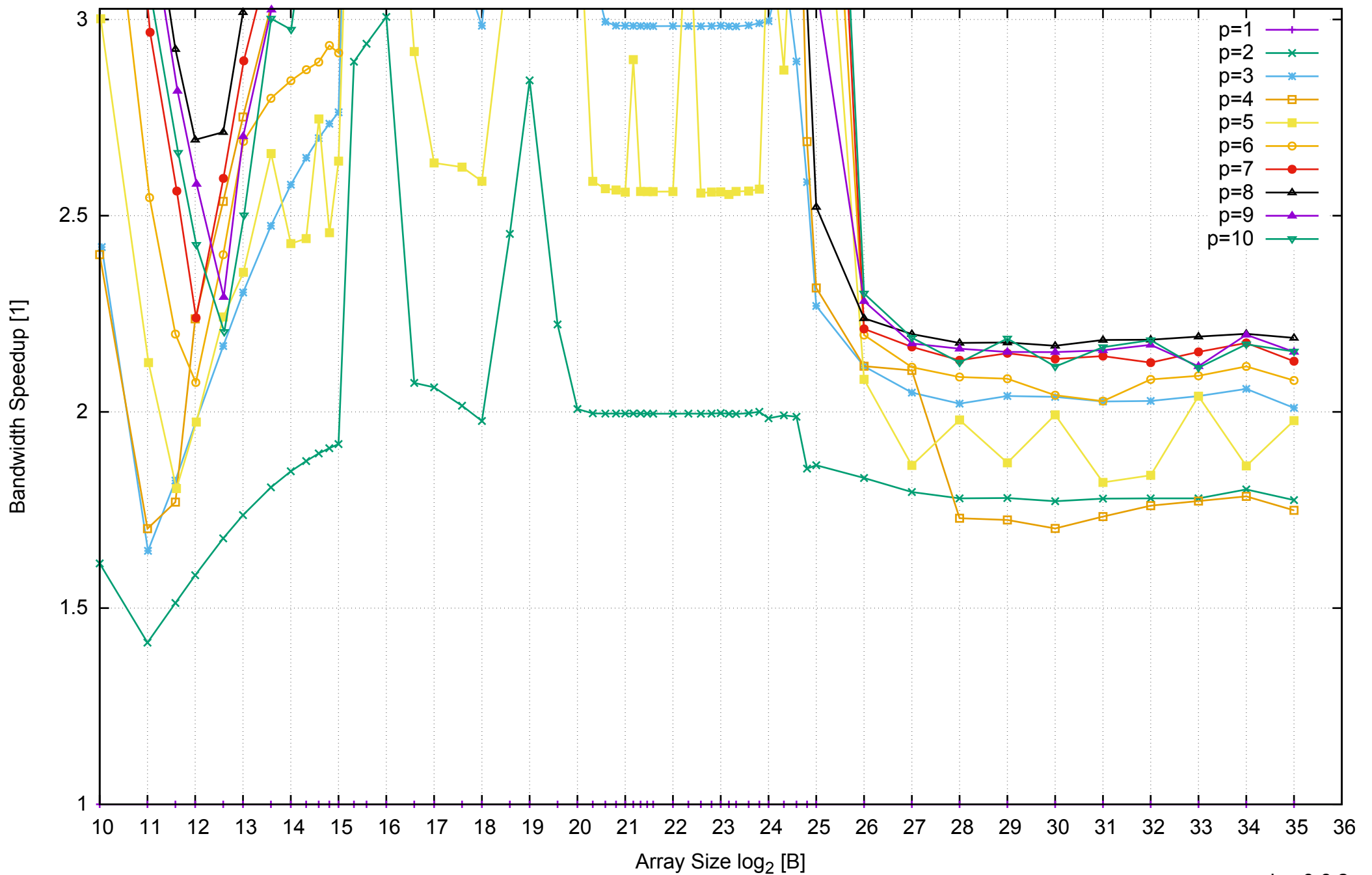
AWS i2.2xlarge - Intel Xeon E5-2670 v2, 2.50 GHz 61GB - Speedup of Parallel Memory Bandwidth (enlarged) - ScanWrite128PtrSimpleLoop
