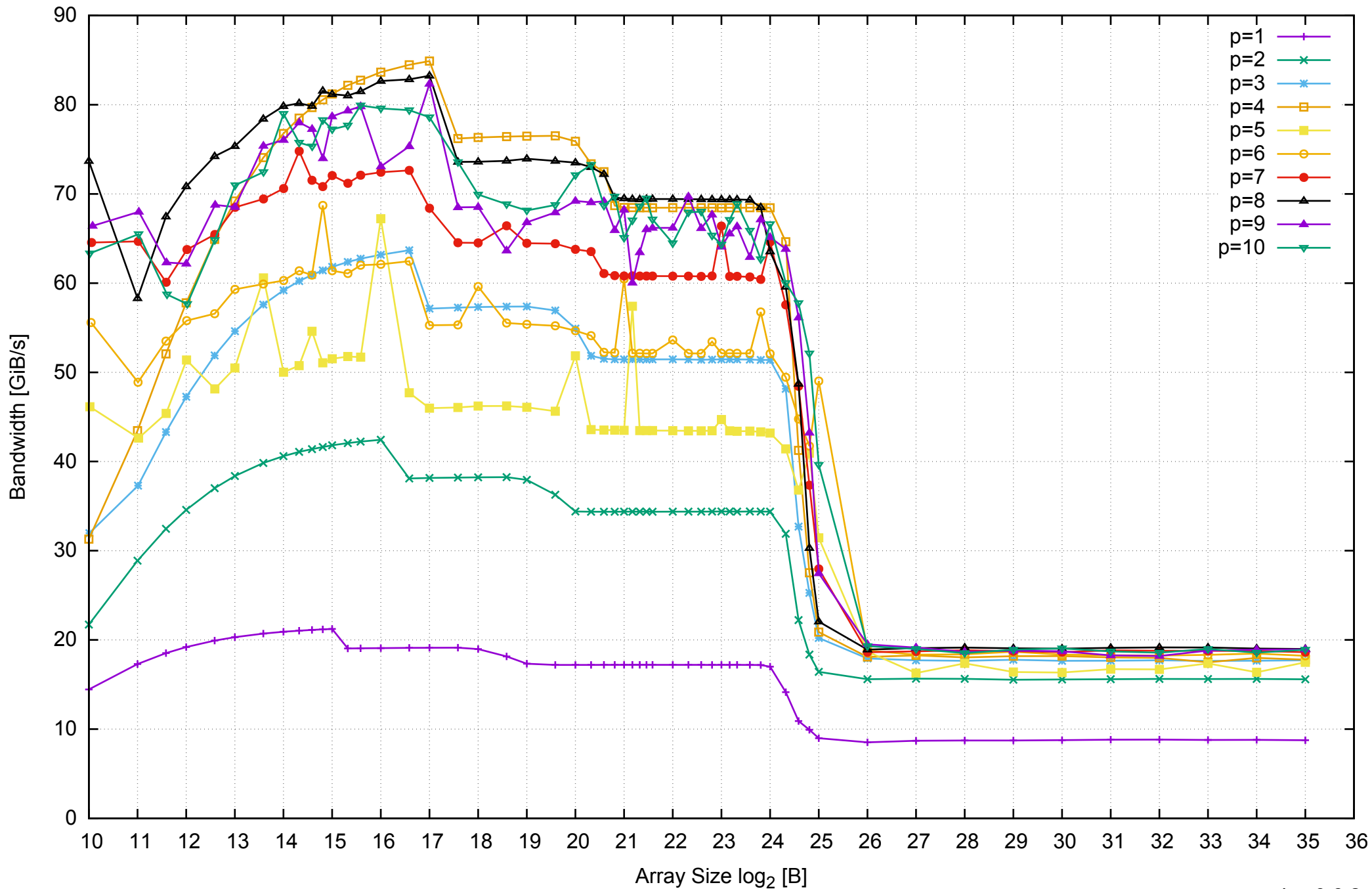
AWS i2.2xlarge - Intel Xeon E5-2670 v2, 2.50 GHz 61GB - Parallel Memory Bandwidth - ScanWrite64PtrSimpleLoop
