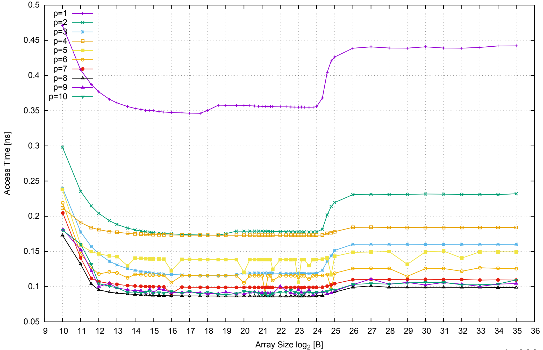
AWS i2.2xlarge - Intel Xeon E5-2670 v2, 2.50 GHz 61GB - Parallel Memory Access Time - ScanRead32PtrSimpleLoop
