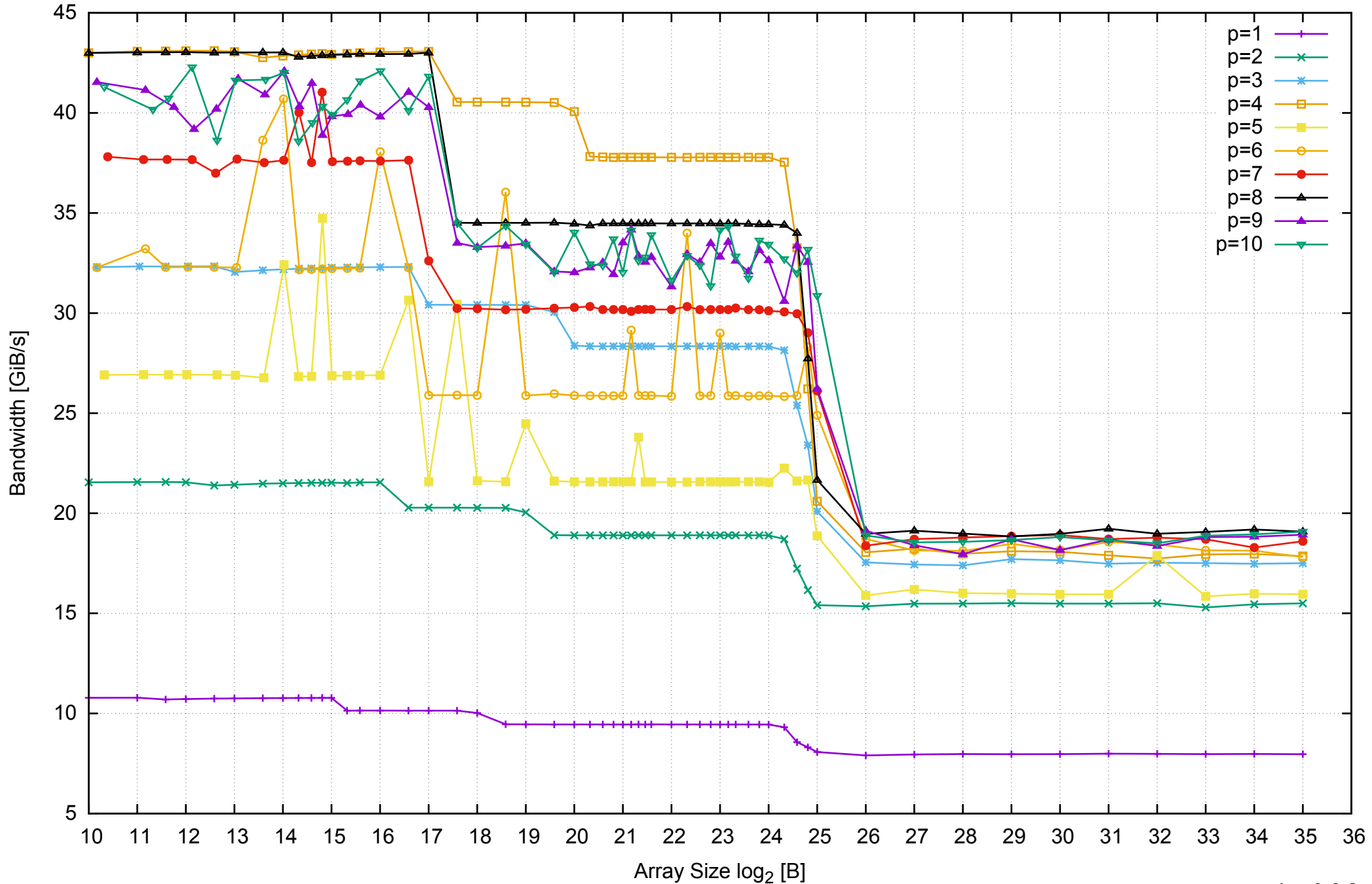
AWS i2.2xlarge - Intel Xeon E5-2670 v2, 2.50 GHz 61GB - Parallel Memory Bandwidth - ScanWrite32PtrUnrollLoop
