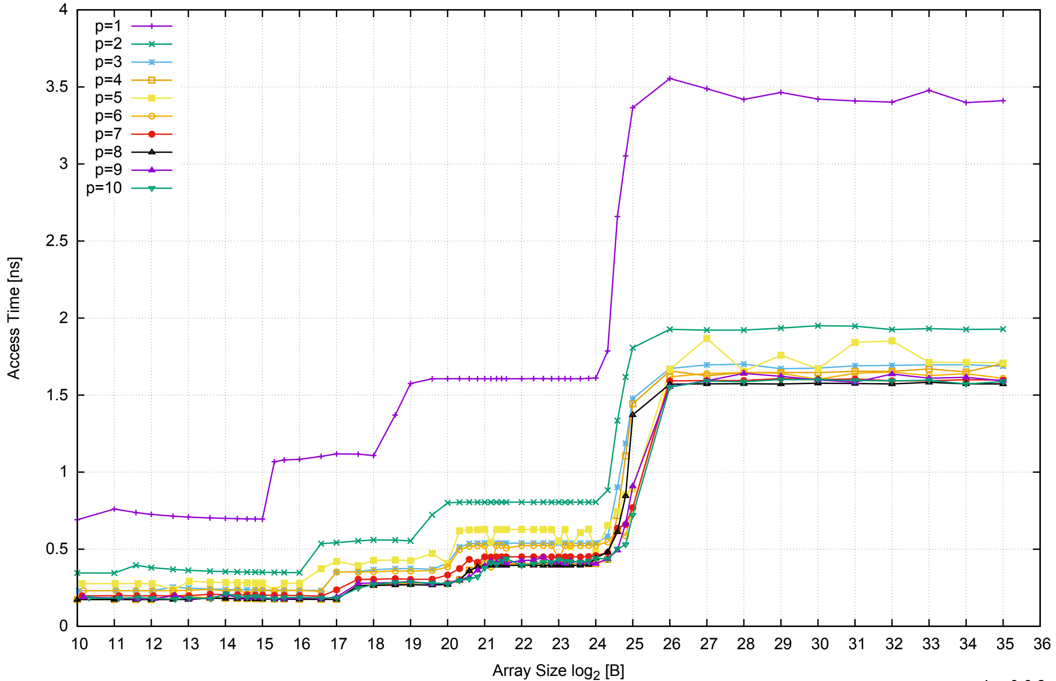
AWS i2.2xlarge - Intel Xeon E5-2670 v2, 2.50 GHz 61GB - Parallel Memory Access Time - ScanWrite256PtrSimpleLoop
