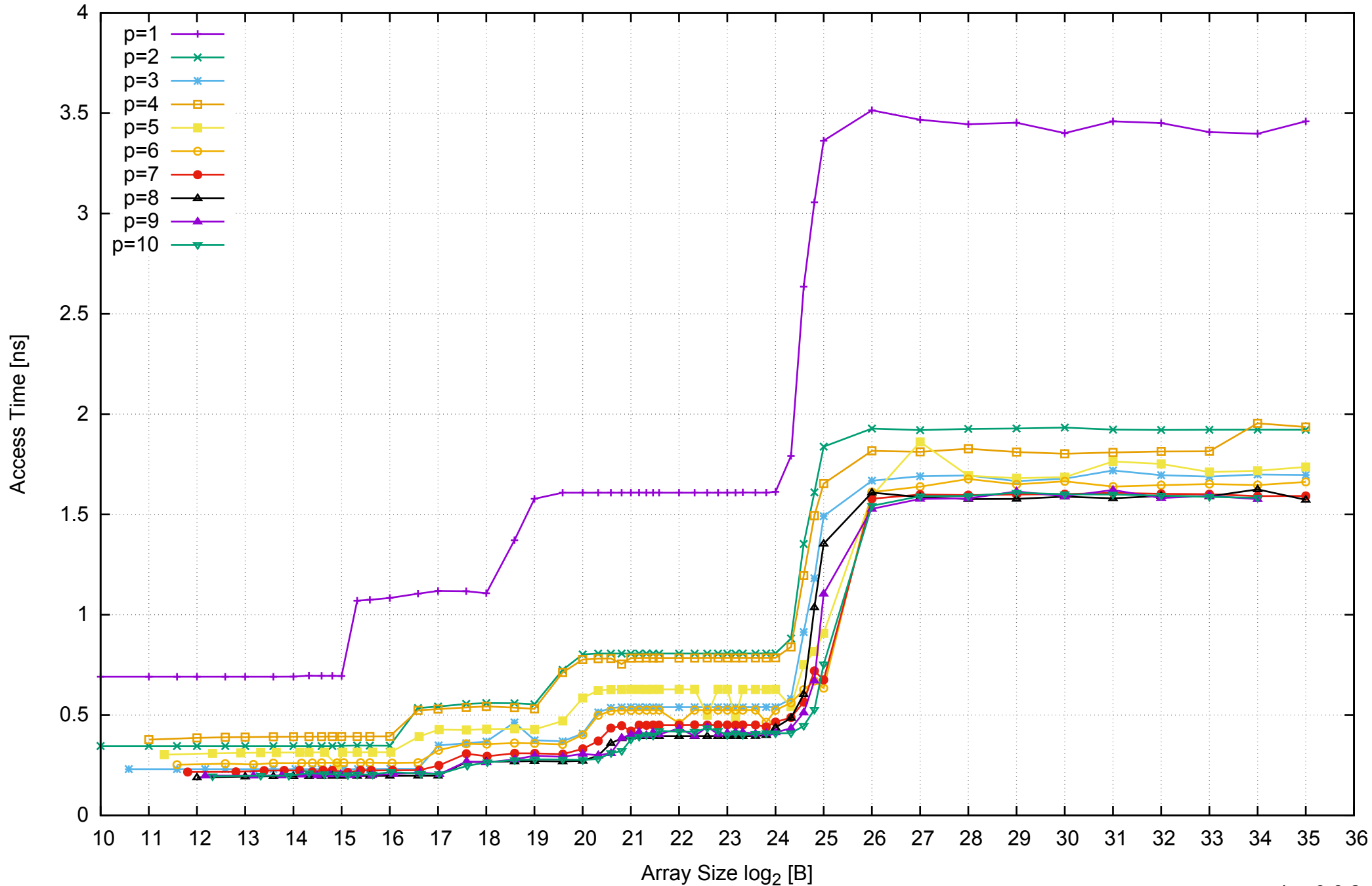
AWS i2.2xlarge - Intel Xeon E5-2670 v2, 2.50 GHz 61GB - Parallel Memory Access Time - ScanWrite256PtrUnrollLoop
