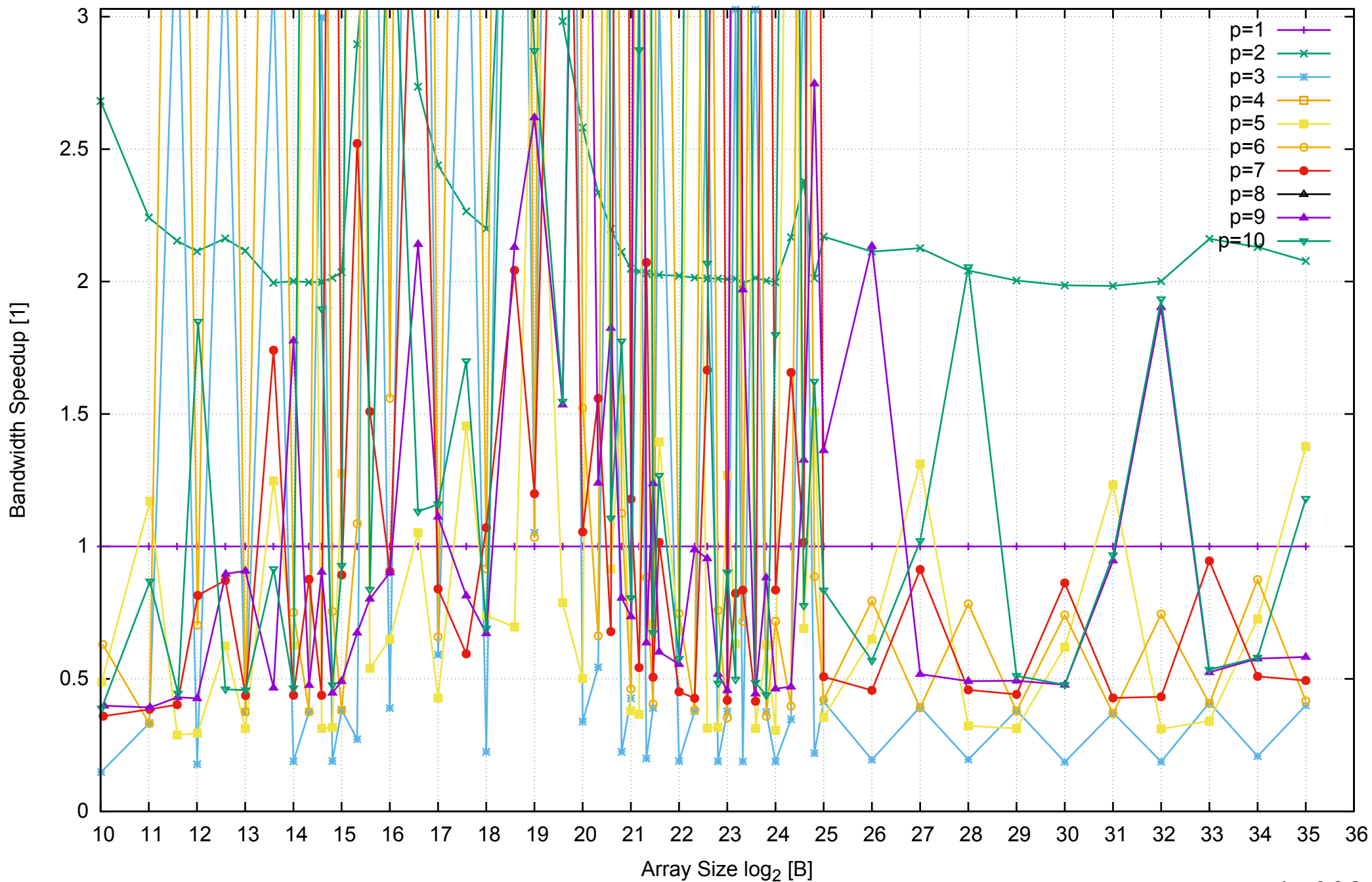
AWS i2.2xlarge - Intel Xeon E5-2670 v2, 2.50 GHz 61GB - Speedup of Parallel Memory Bandwidth (enlarged) - PermRead64UnrollLoop
