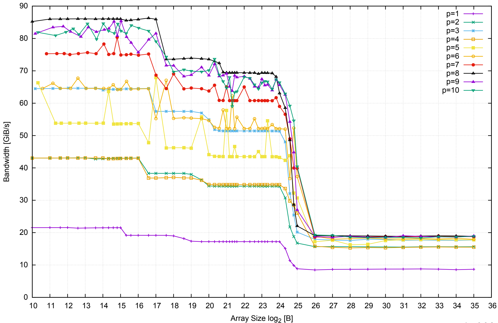
AWS i2.2xlarge - Intel Xeon E5-2670 v2, 2.50 GHz 61GB - Parallel Memory Bandwidth - ScanWrite64PtrUnrollLoop
