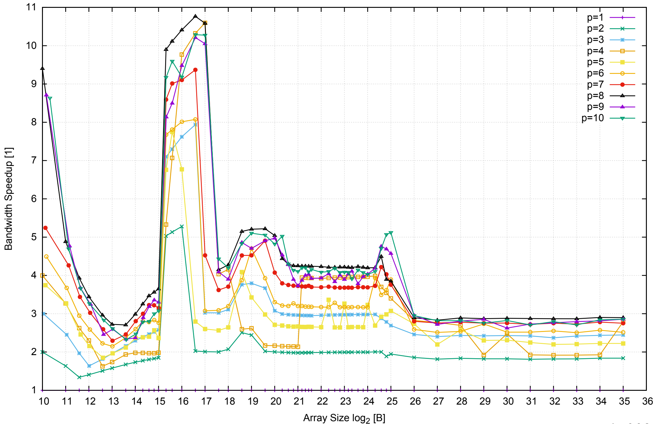
AWS i2.2xlarge - Intel Xeon E5-2670 v2, 2.50 GHz 61GB - Speedup of Parallel Memory Bandwidth - ScanRead256PtrSimpleLoop
