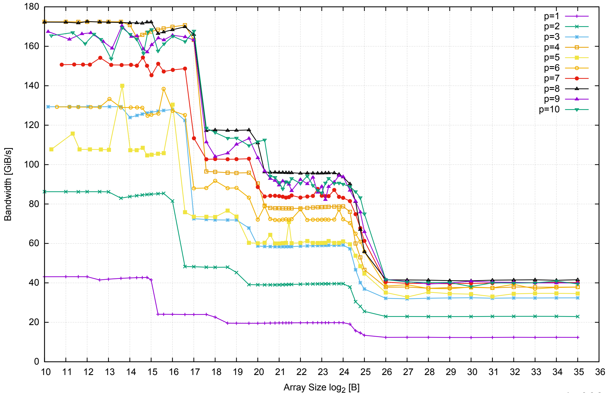
AWS i2.2xlarge - Intel Xeon E5-2670 v2, 2.50 GHz 61GB - Parallel Memory Bandwidth - ScanRead64PtrUnrollLoop
