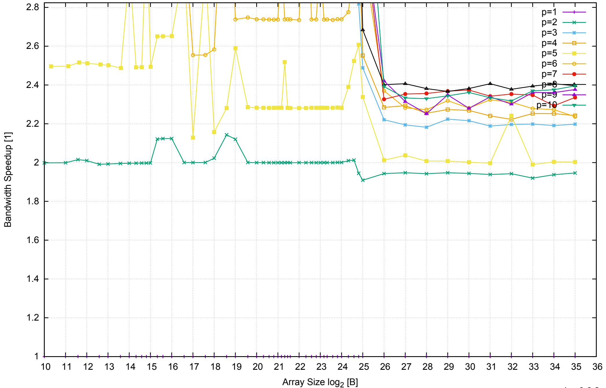
AWS i2.2xlarge - Intel Xeon E5-2670 v2, 2.50 GHz 61GB - Speedup of Parallel Memory Bandwidth (enlarged) - ScanWrite32PtrUnrollLoop
