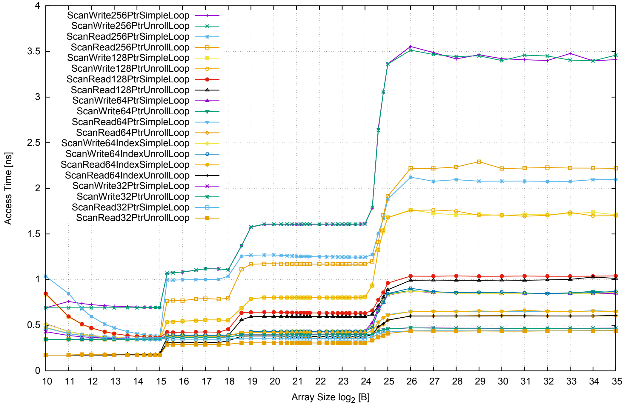
AWS i2.2xlarge - Intel Xeon E5-2670 v2, 2.50 GHz 61GB - One Thread Memory Latency (excluding Permutation)
