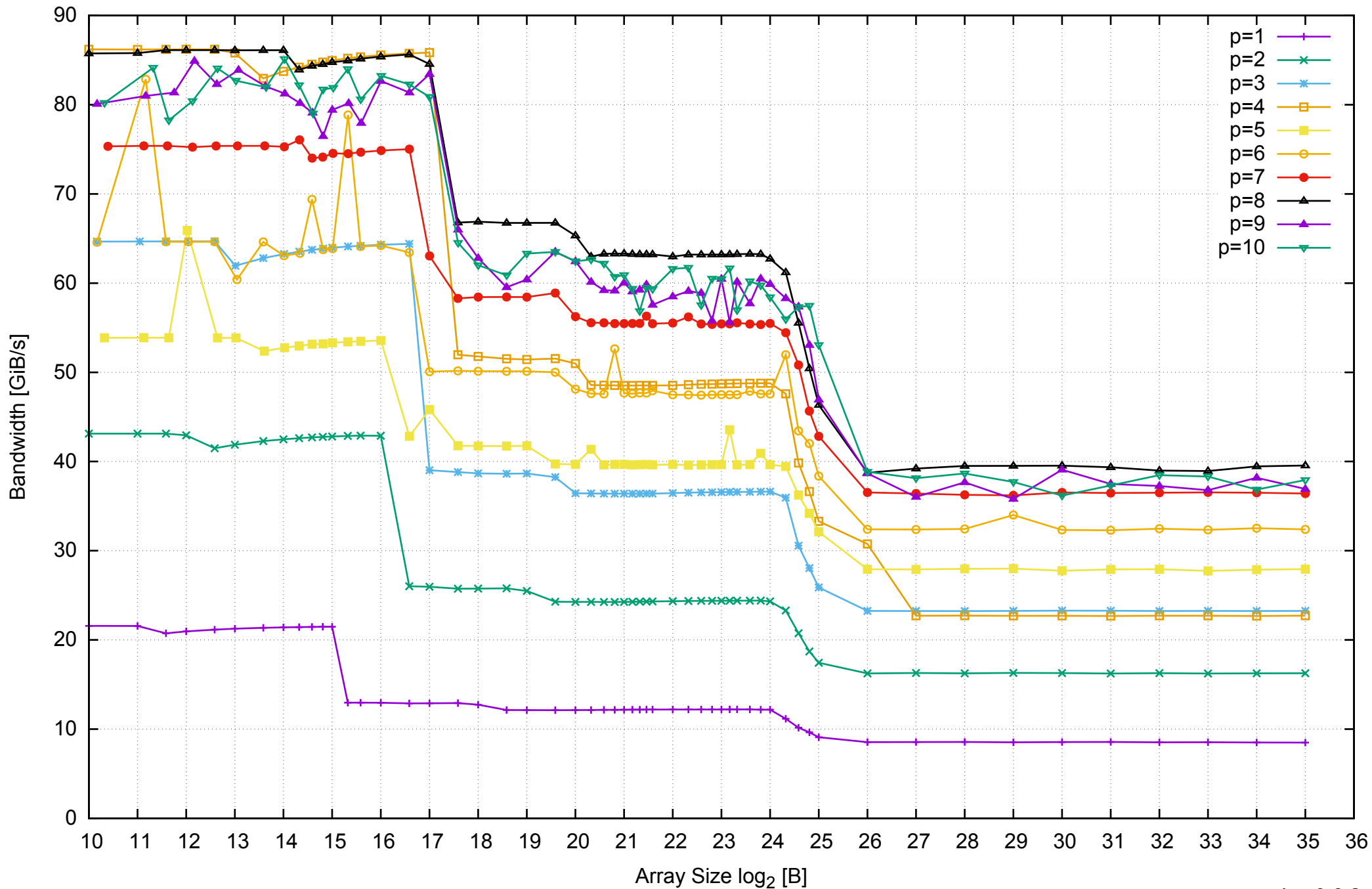
AWS i2.2xlarge - Intel Xeon E5-2670 v2, 2.50 GHz 61GB - Parallel Memory Bandwidth - ScanRead32PtrUnrollLoop
