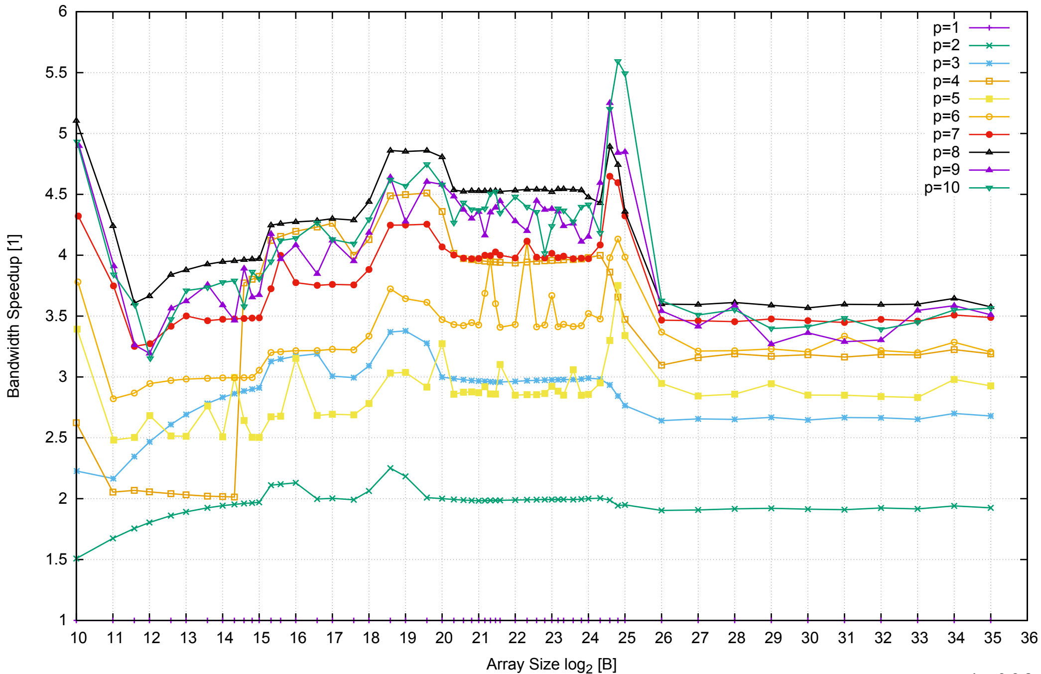
AWS i2.2xlarge - Intel Xeon E5-2670 v2, 2.50 GHz 61GB - Speedup of Parallel Memory Bandwidth - ScanRead64PtrSimpleLoop
