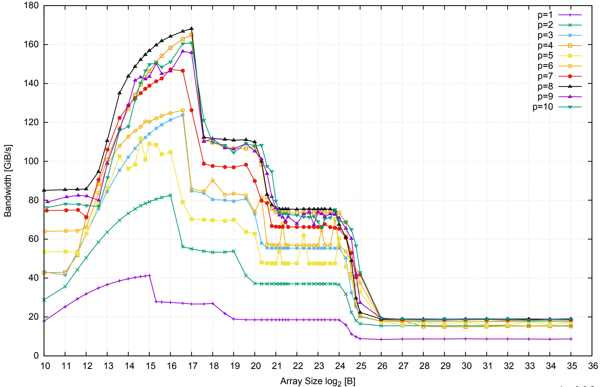
AWS i2.2xlarge - Intel Xeon E5-2670 v2, 2.50 GHz 61GB - Parallel Memory Bandwidth - ScanWrite128PtrSimpleLoop
