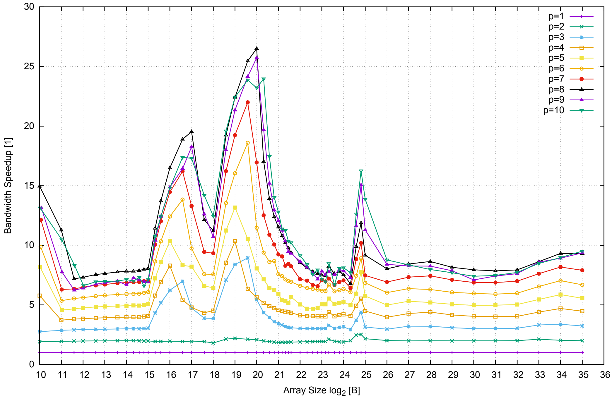
AWS i2.2xlarge - Intel Xeon E5-2670 v2, 2.50 GHz 61GB - Speedup of Parallel Memory Bandwidth - PermRead64SimpleLoop
