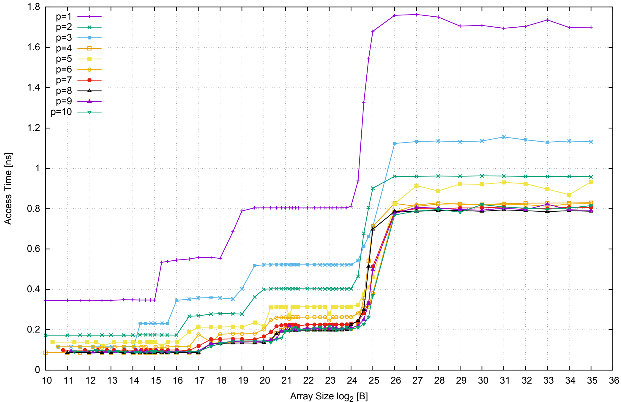
AWS i2.2xlarge - Intel Xeon E5-2670 v2, 2.50 GHz 61GB - Parallel Memory Access Time - ScanWrite128PtrUnrollLoop
