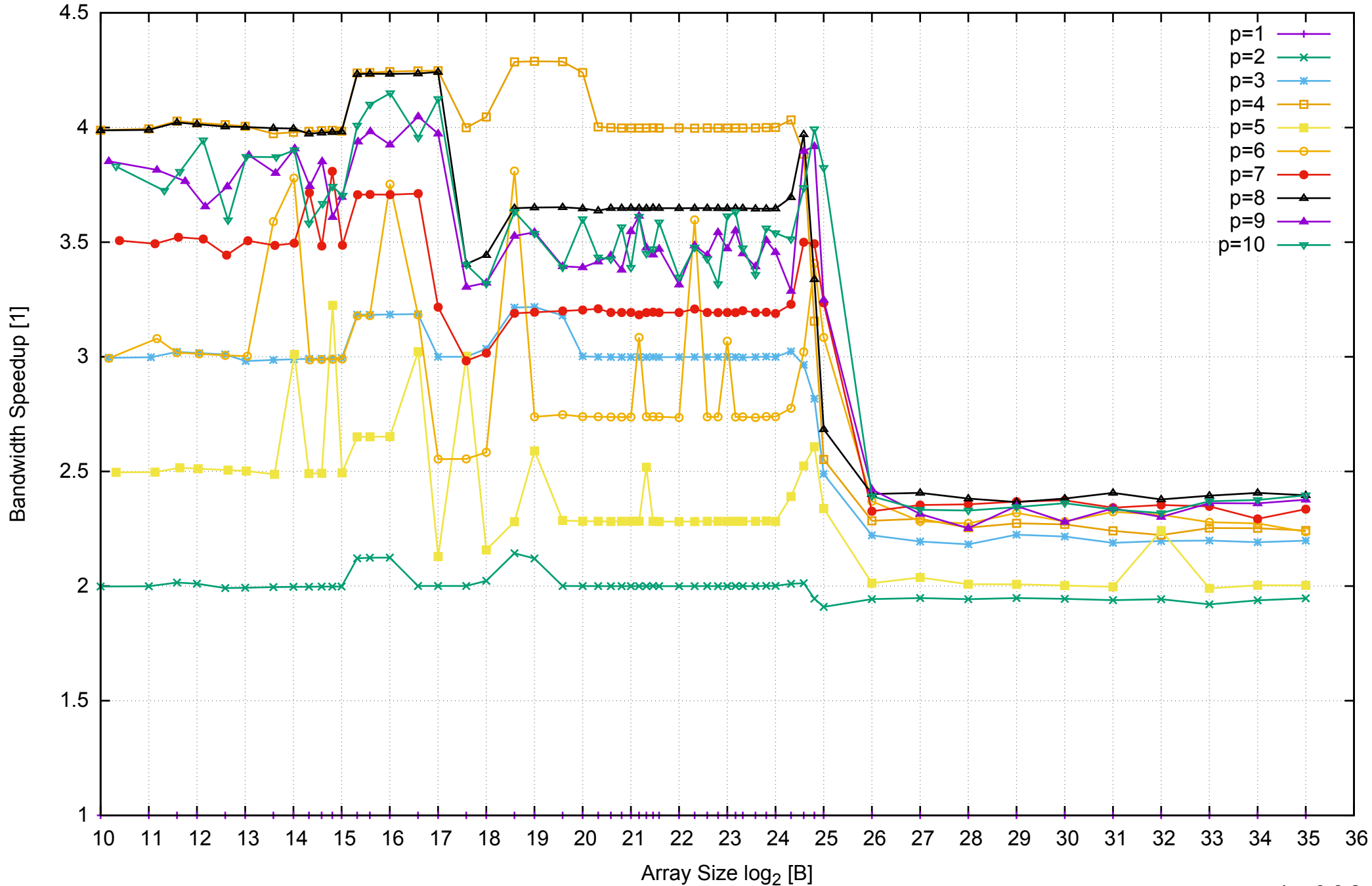
AWS i2.2xlarge - Intel Xeon E5-2670 v2, 2.50 GHz 61GB - Speedup of Parallel Memory Bandwidth - ScanWrite32PtrUnrollLoop
