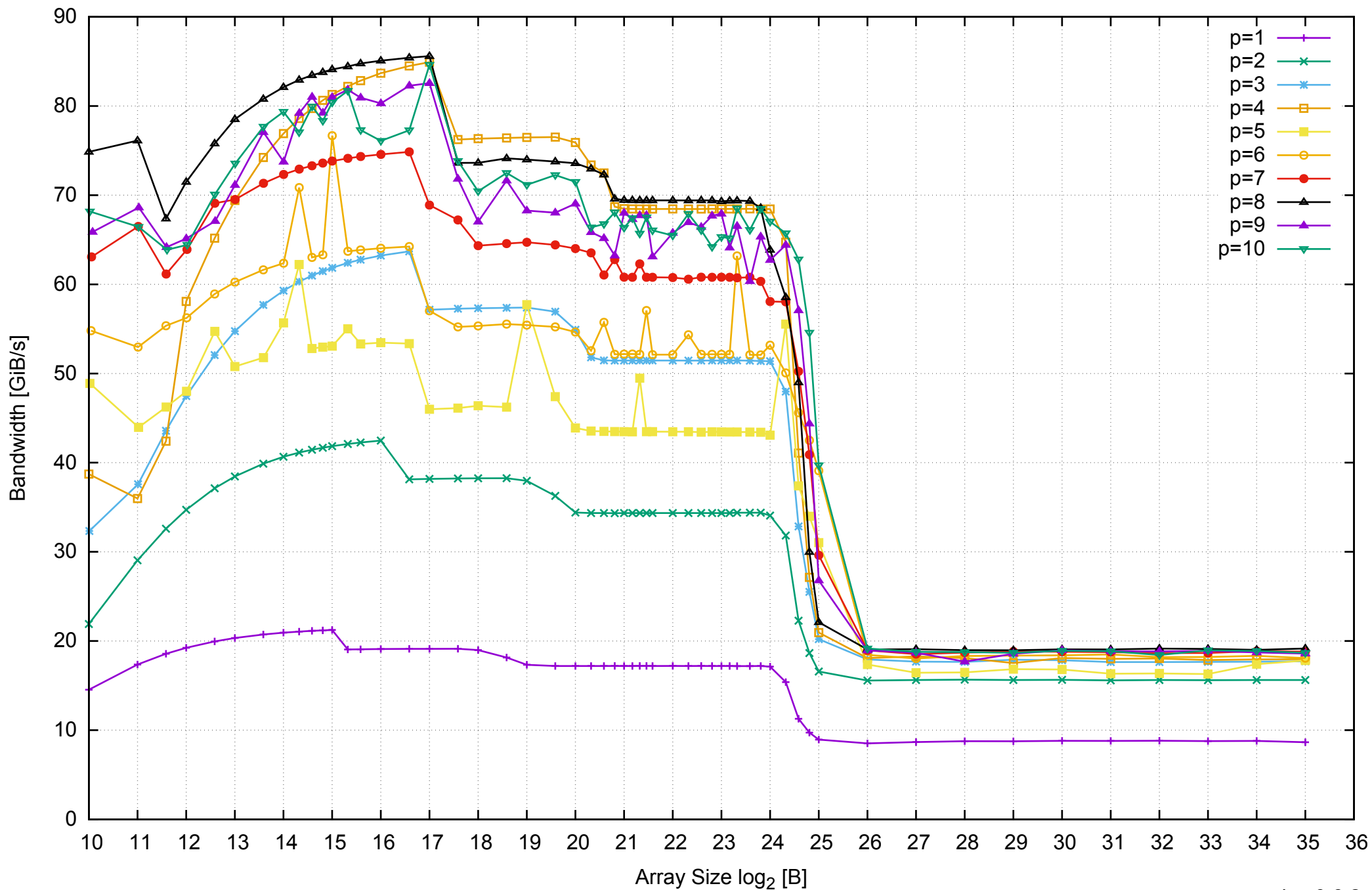
AWS i2.2xlarge - Intel Xeon E5-2670 v2, 2.50 GHz 61GB - Parallel Memory Bandwidth - ScanWrite64IndexSimpleLoop
