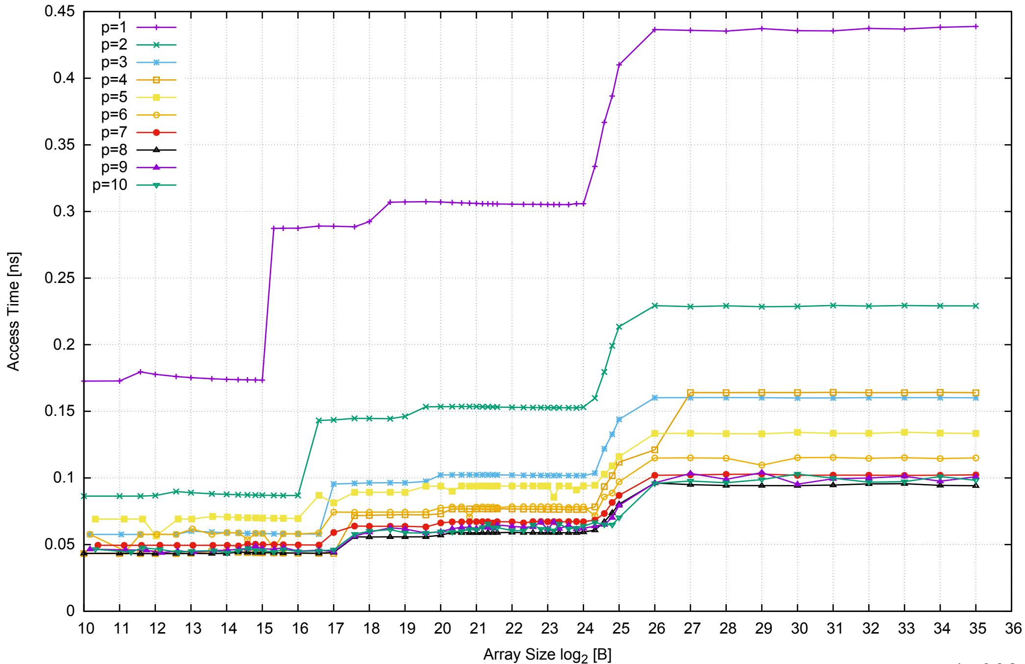
AWS i2.2xlarge - Intel Xeon E5-2670 v2, 2.50 GHz 61GB - Parallel Memory Access Time - ScanRead32PtrUnrollLoop
