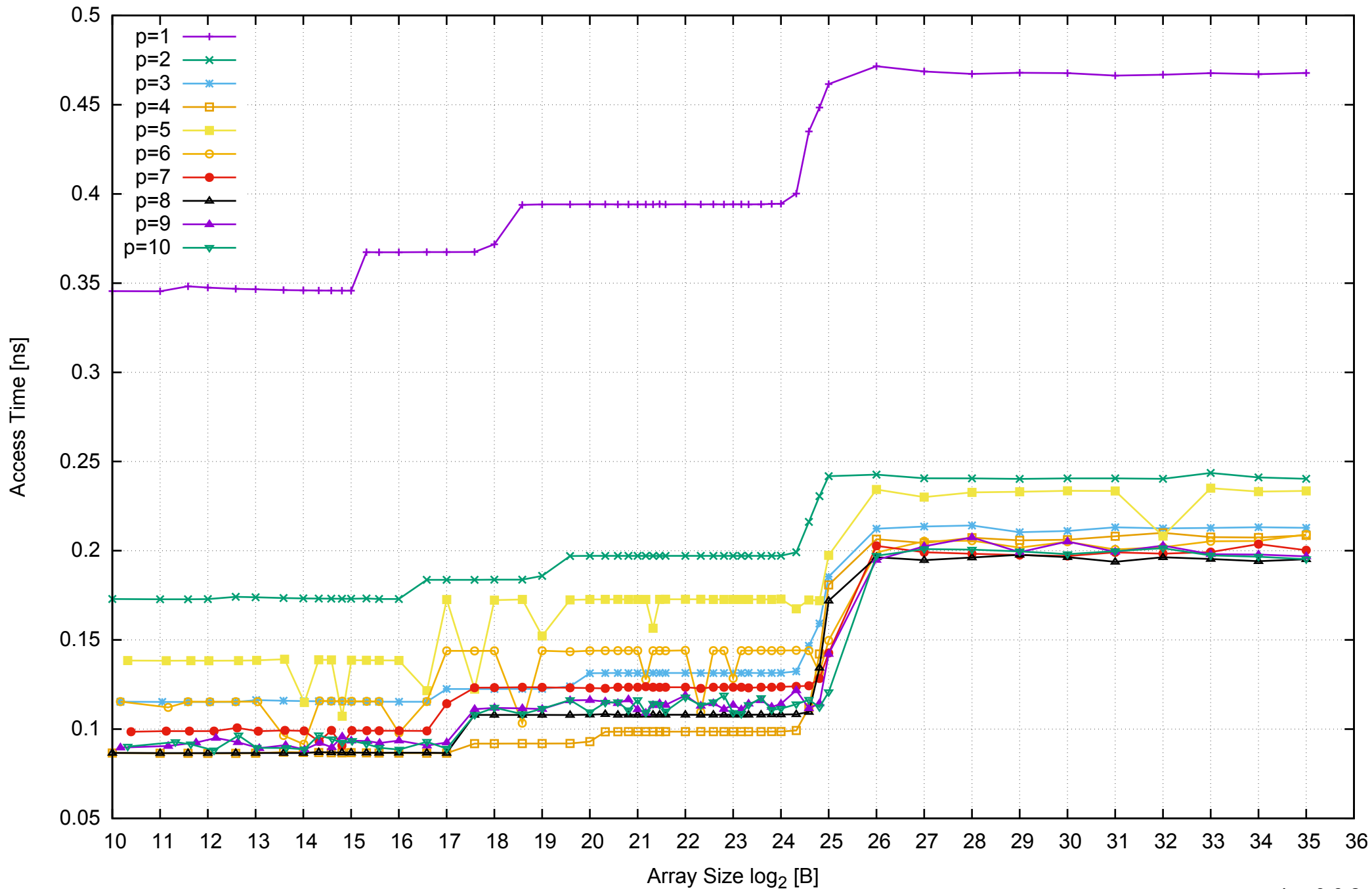
AWS i2.2xlarge - Intel Xeon E5-2670 v2, 2.50 GHz 61GB - Parallel Memory Access Time - ScanWrite32PtrUnrollLoop
