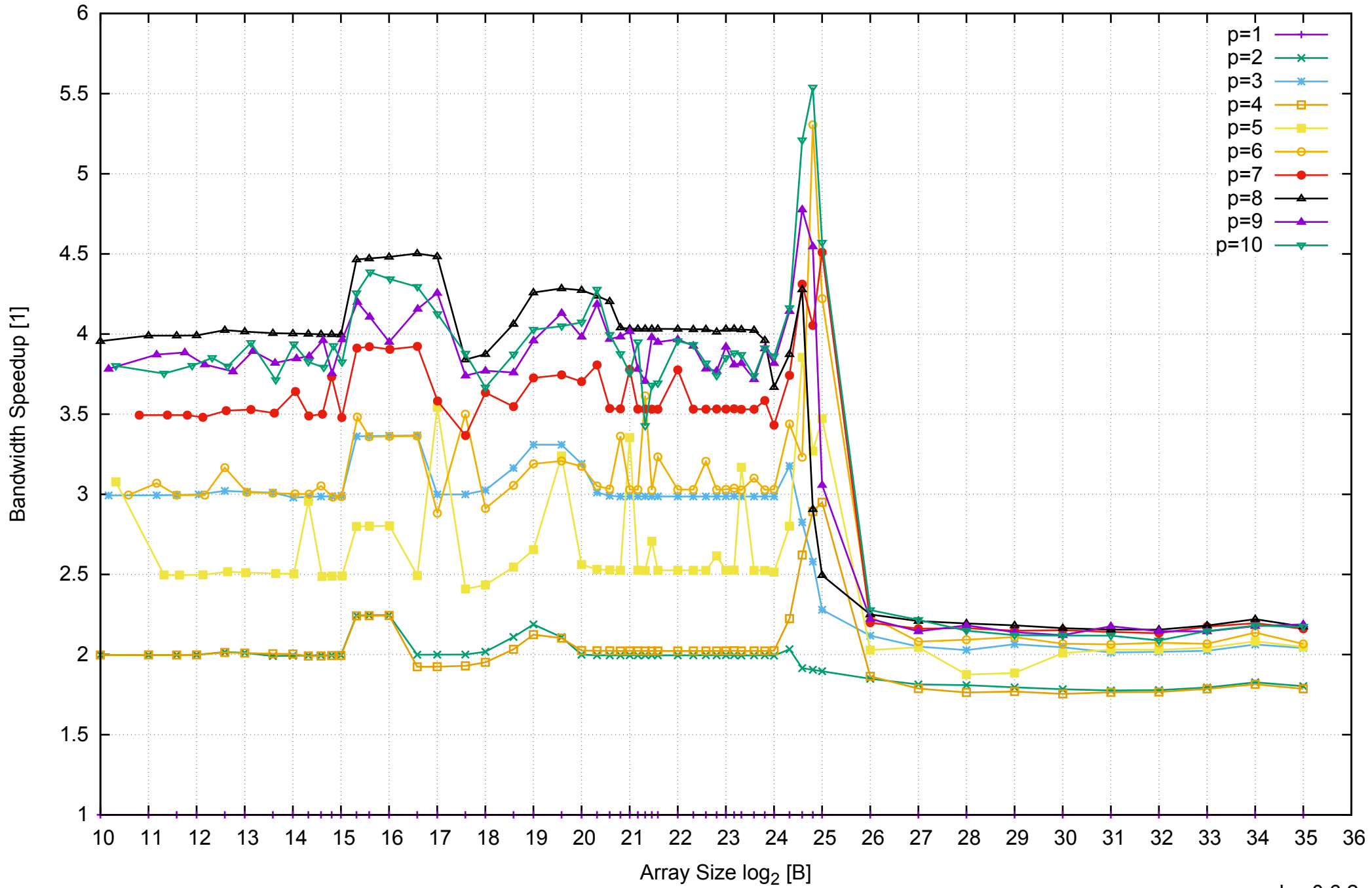
AWS i2.2xlarge - Intel Xeon E5-2670 v2, 2.50 GHz 61GB - Speedup of Parallel Memory Bandwidth - ScanWrite64PtrUnrollLoop
