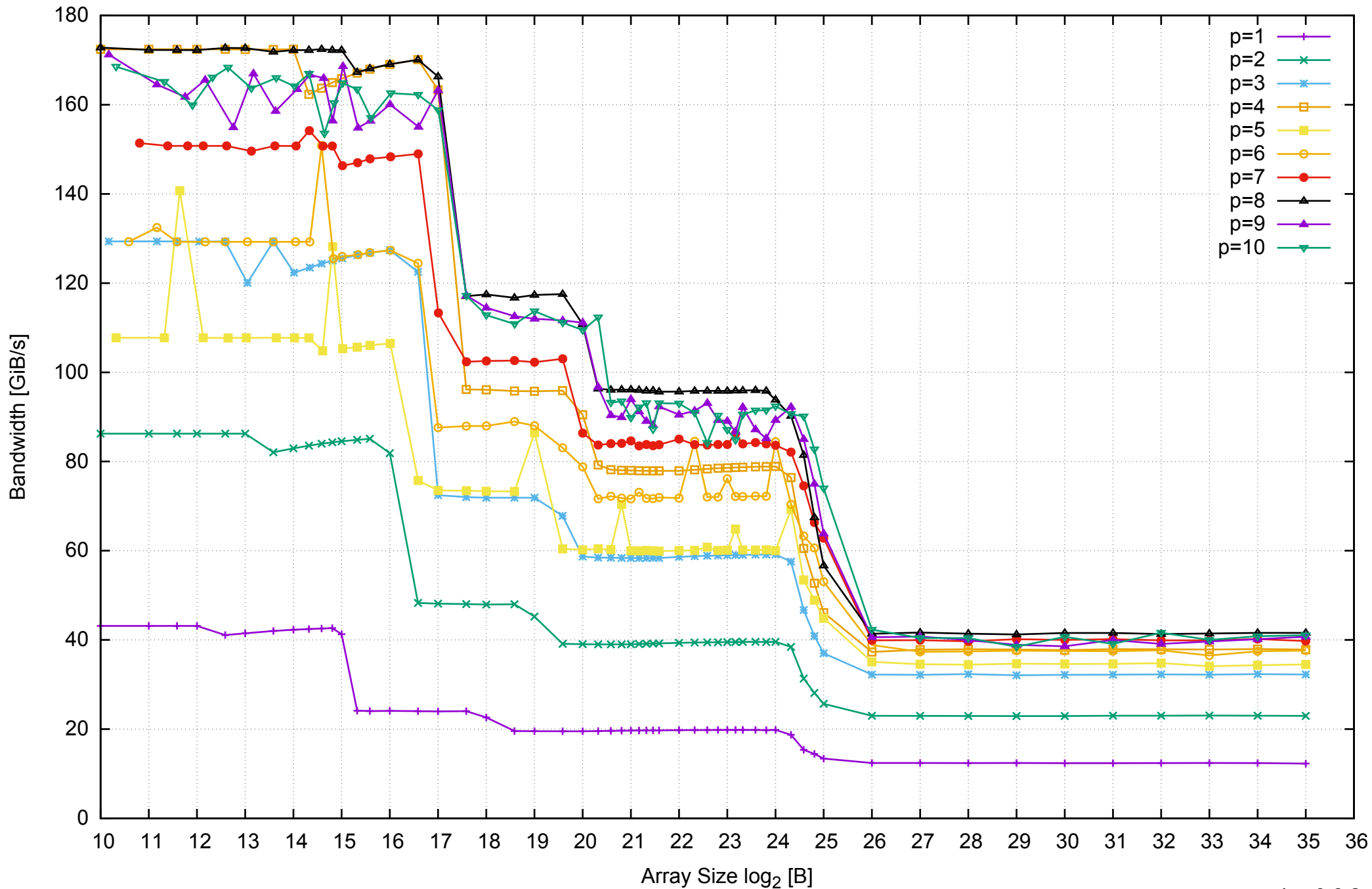
AWS i2.2xlarge - Intel Xeon E5-2670 v2, 2.50 GHz 61GB - Parallel Memory Bandwidth - ScanRead64IndexUnrollLoop
