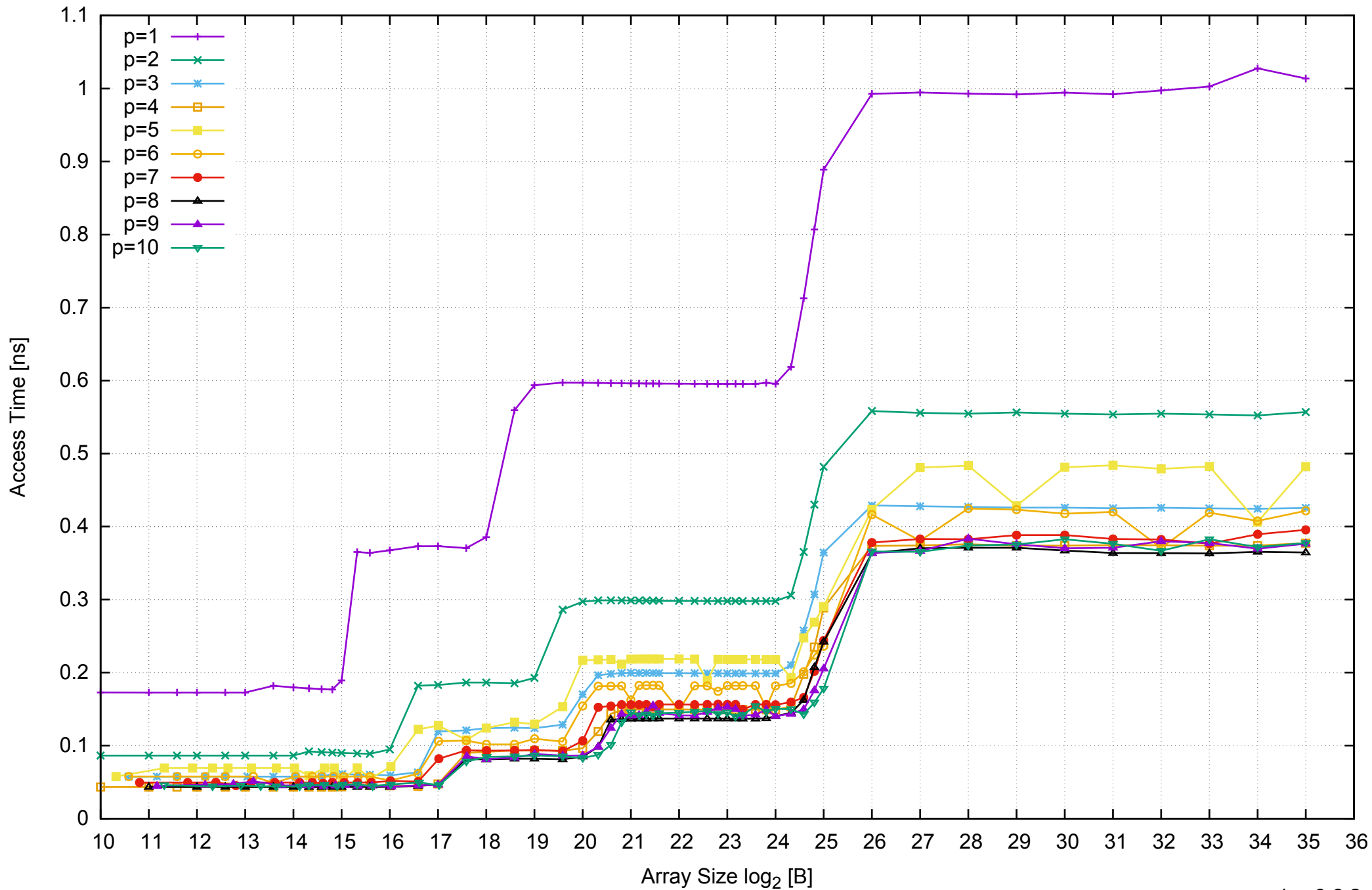
AWS i2.2xlarge - Intel Xeon E5-2670 v2, 2.50 GHz 61GB - Parallel Memory Access Time - ScanRead128PtrUnrollLoop
