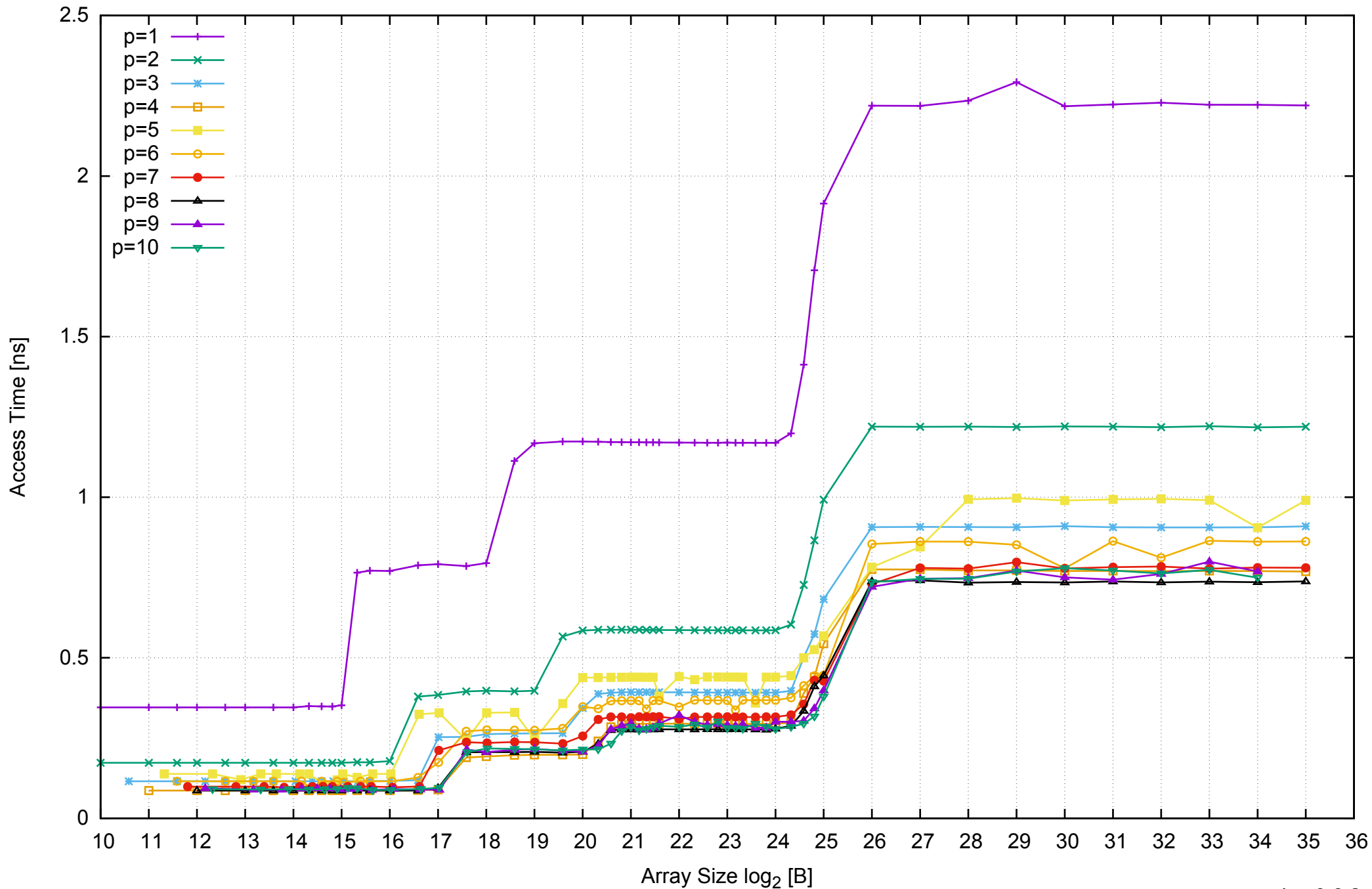
AWS i2.2xlarge - Intel Xeon E5-2670 v2, 2.50 GHz 61GB - Parallel Memory Access Time - ScanRead256PtrUnrollLoop
