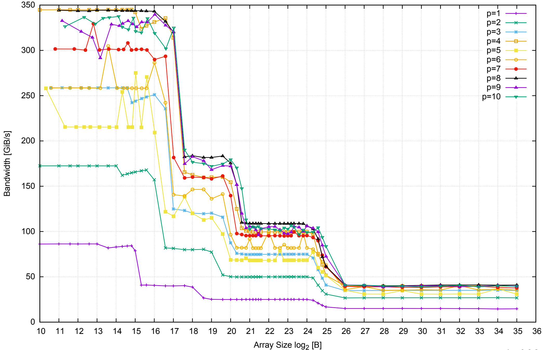
AWS i2.2xlarge - Intel Xeon E5-2670 v2, 2.50 GHz 61GB - Parallel Memory Bandwidth - ScanRead128PtrUnrollLoop
