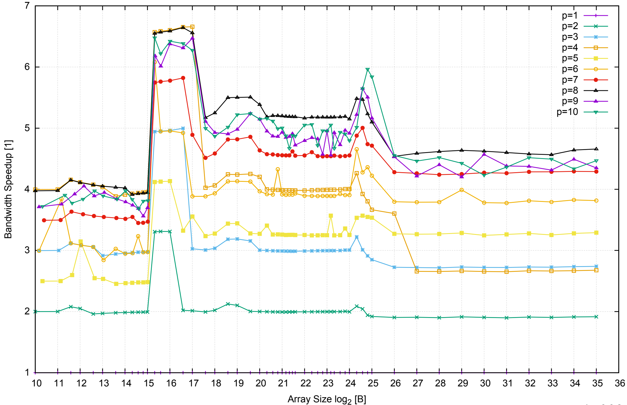
AWS i2.2xlarge - Intel Xeon E5-2670 v2, 2.50 GHz 61GB - Speedup of Parallel Memory Bandwidth - ScanRead32PtrUnrollLoop
