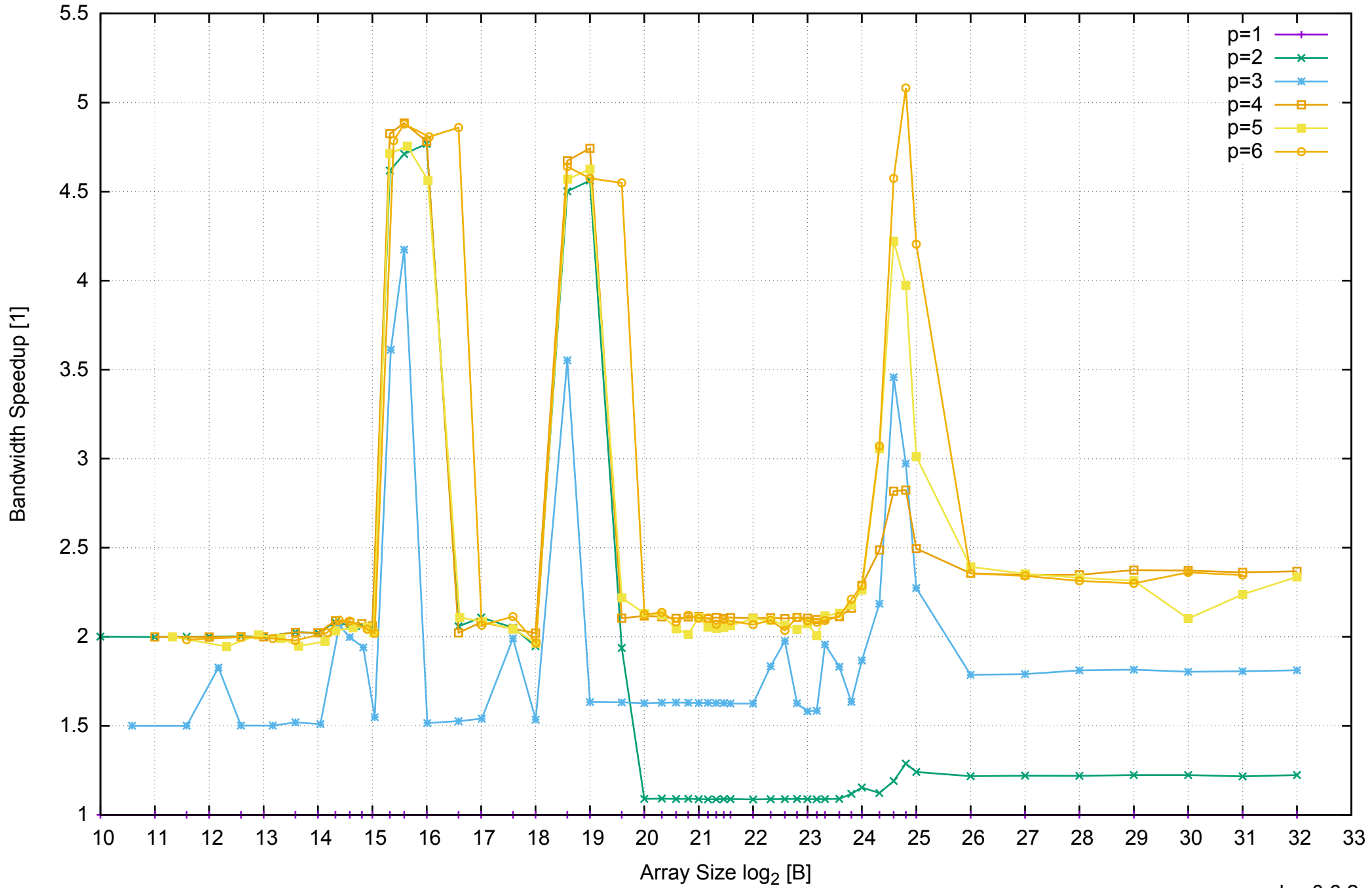
AWS c4.xlarge - Intel Xeon E5-2666 v3 2.90 GHz 7.5GB - Speedup of Parallel Memory Bandwidth - ScanRead256PtrUnrollLoop
