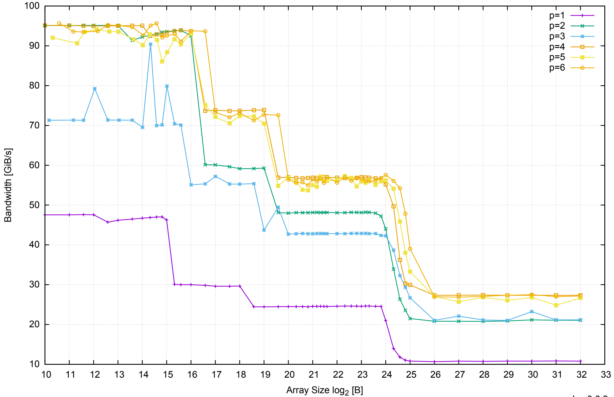
AWS c4.xlarge - Intel Xeon E5-2666 v3 2.90 GHz 7.5GB - Parallel Memory Bandwidth - ScanRead64IndexUnrollLoop
