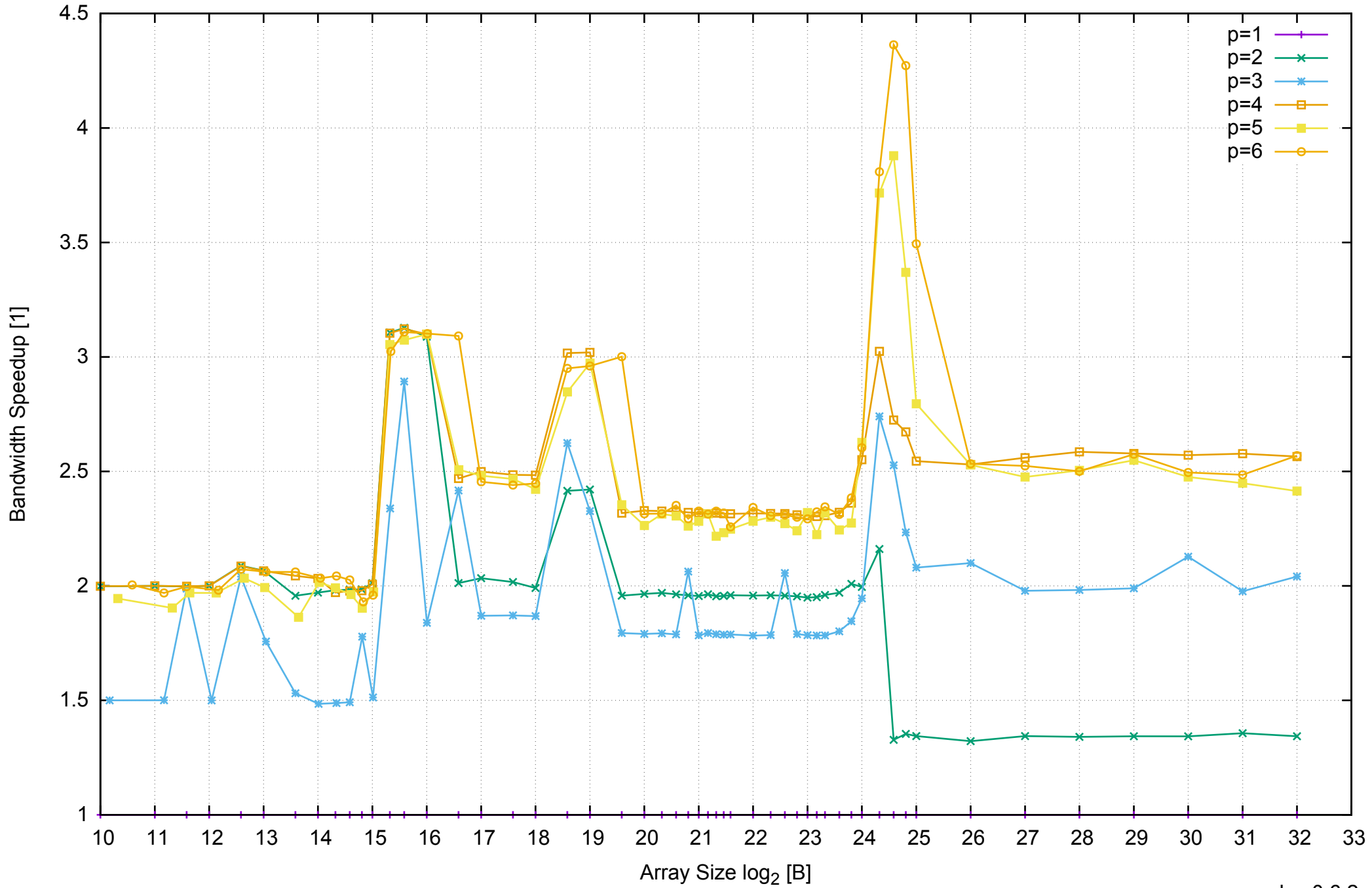
AWS c4.xlarge - Intel Xeon E5-2666 v3 2.90 GHz 7.5GB - Speedup of Parallel Memory Bandwidth - ScanRead64PtrUnrollLoop
