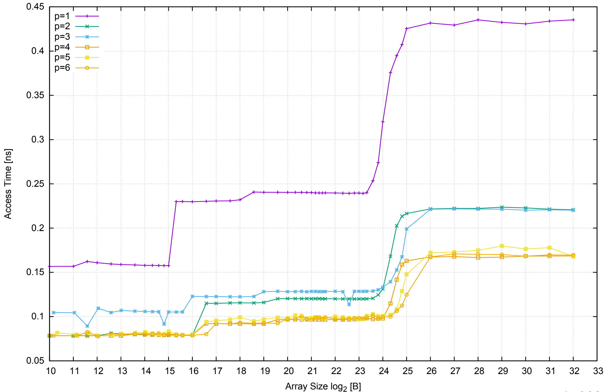
AWS c4.xlarge - Intel Xeon E5-2666 v3 2.90 GHz 7.5GB - Parallel Memory Access Time - ScanRead32PtrUnrollLoop
