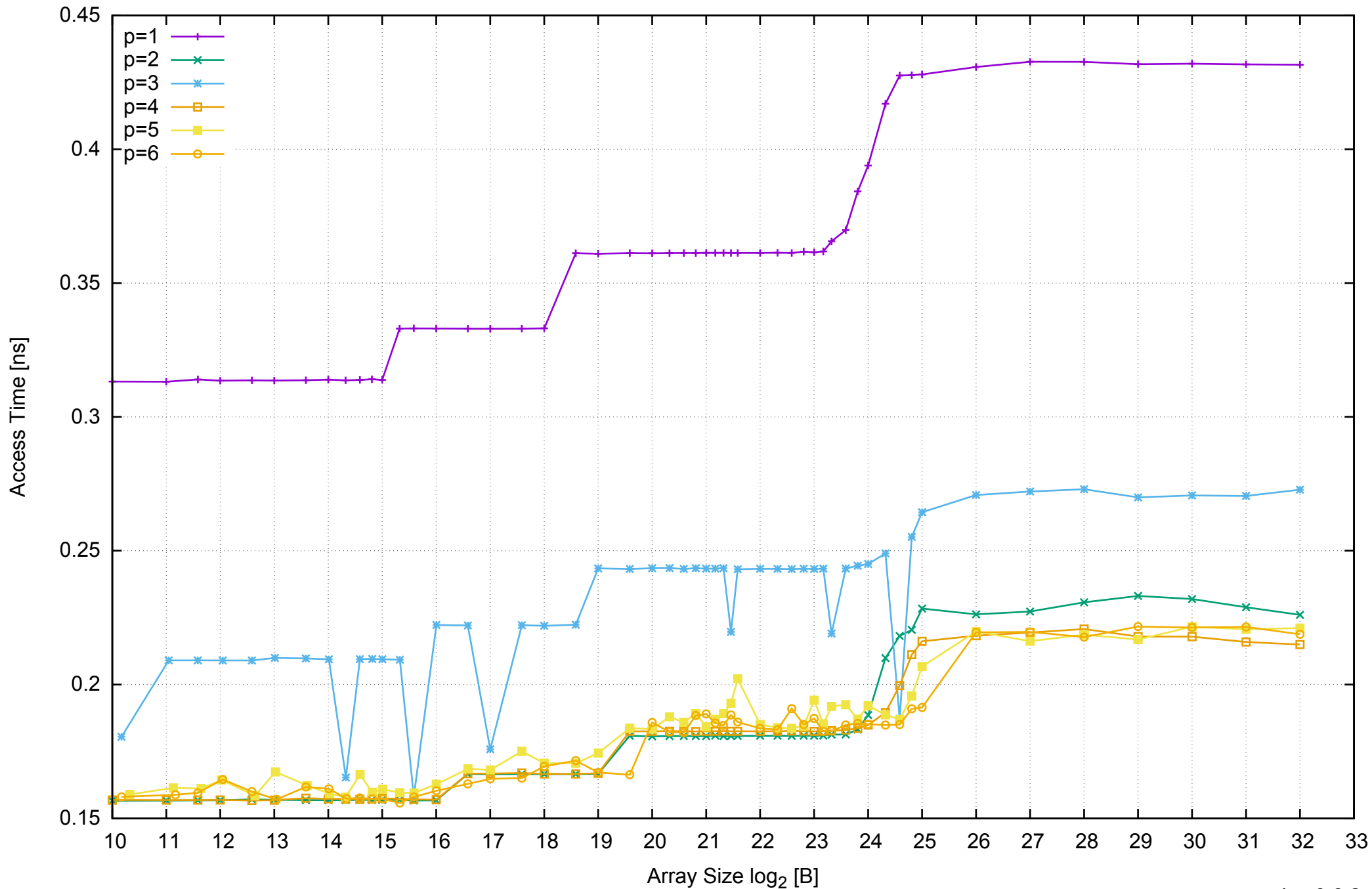
AWS c4.xlarge - Intel Xeon E5-2666 v3 2.90 GHz 7.5GB - Parallel Memory Access Time - ScanWrite32PtrUnrollLoop
