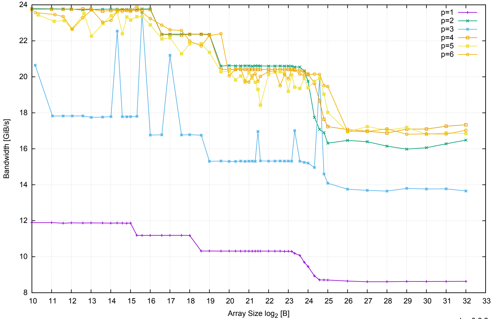
AWS c4.xlarge - Intel Xeon E5-2666 v3 2.90 GHz 7.5GB - Parallel Memory Bandwidth - ScanWrite32PtrUnrollLoop
