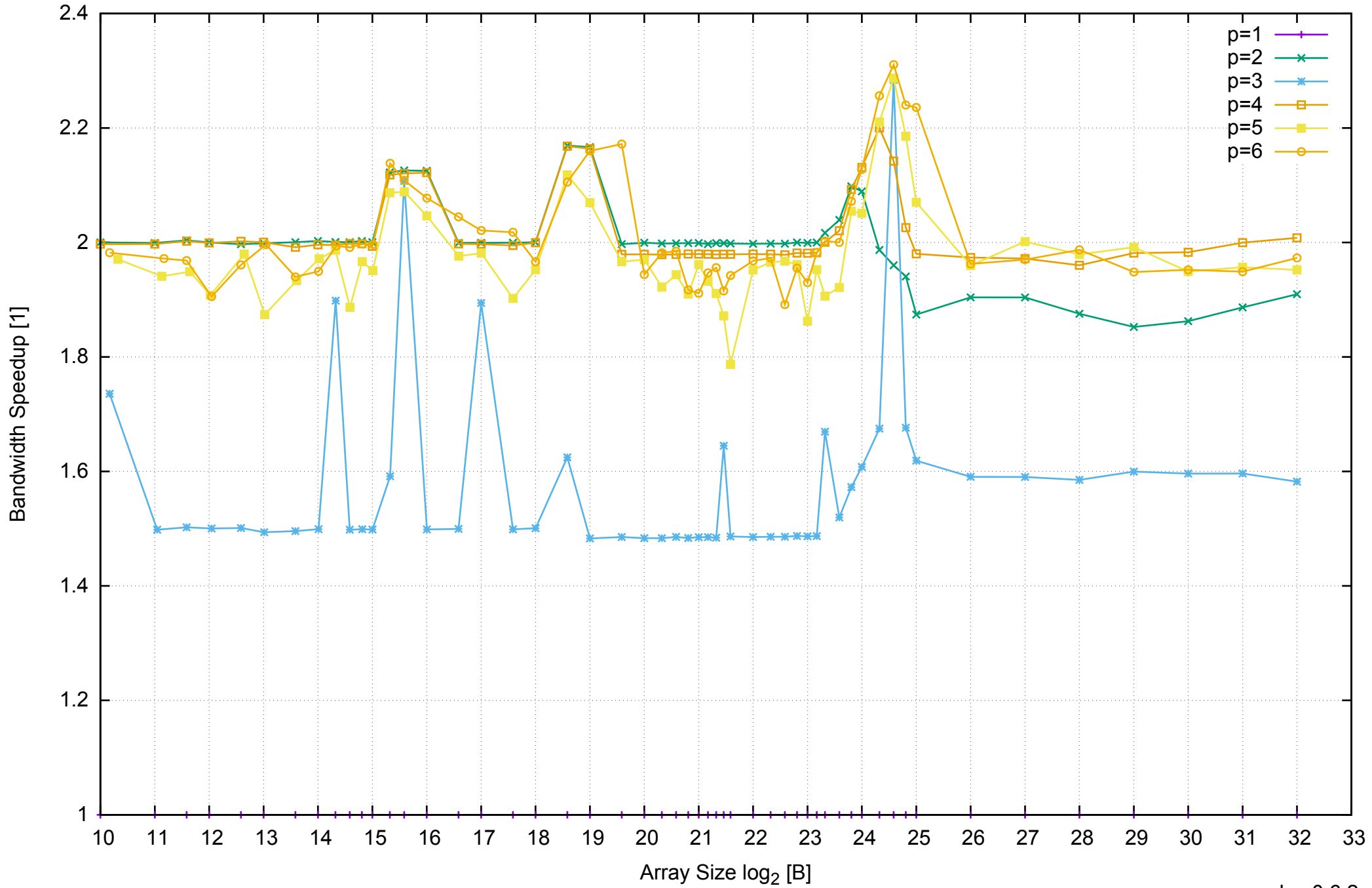
AWS c4.xlarge - Intel Xeon E5-2666 v3 2.90 GHz 7.5GB - Speedup of Parallel Memory Bandwidth - ScanWrite32PtrUnrollLoop
