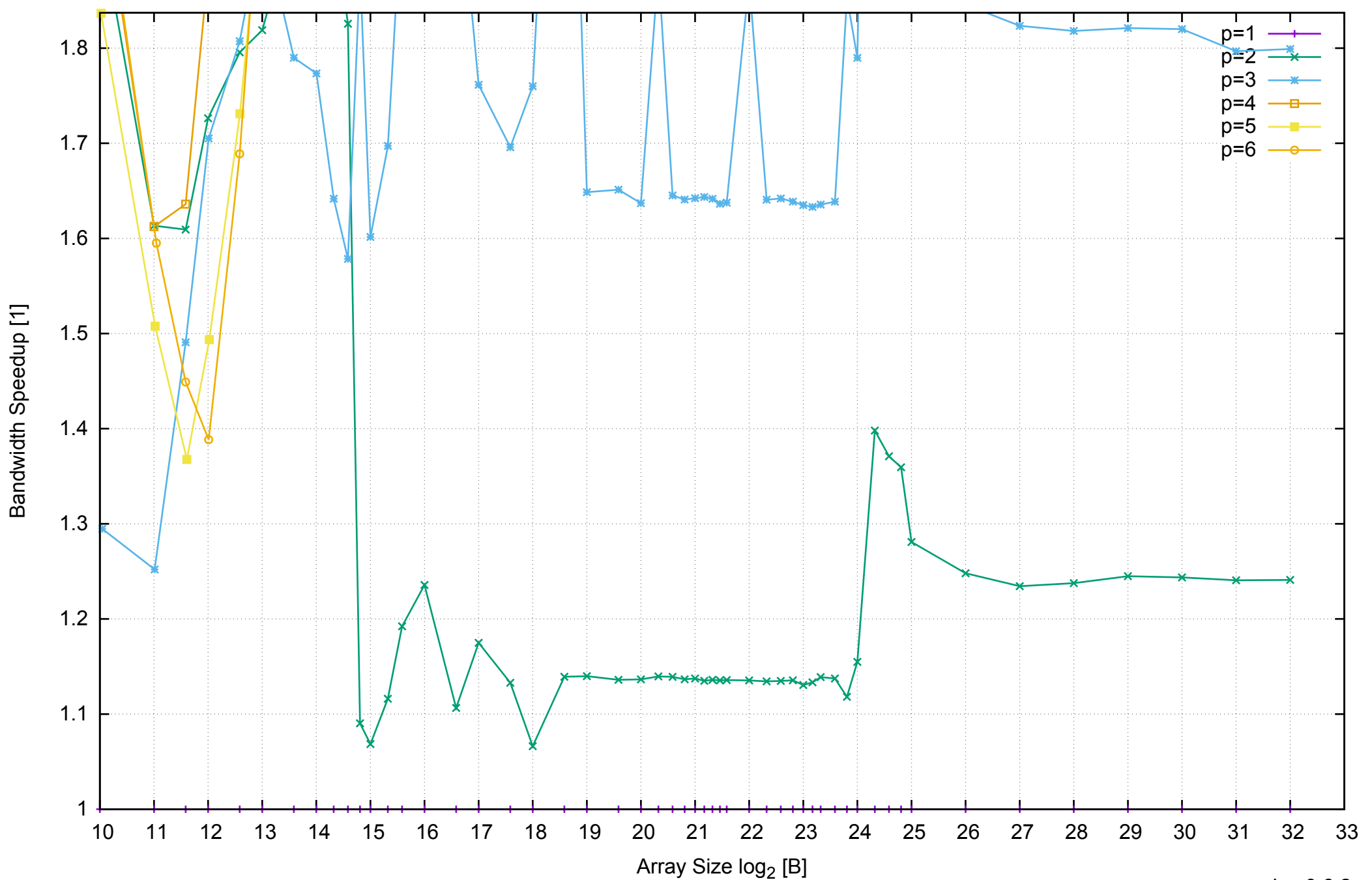
AWS c4.xlarge - Intel Xeon E5-2666 v3 2.90 GHz 7.5GB - Speedup of Parallel Memory Bandwidth (enlarged) - ScanRead128PtrSimpleLoop
