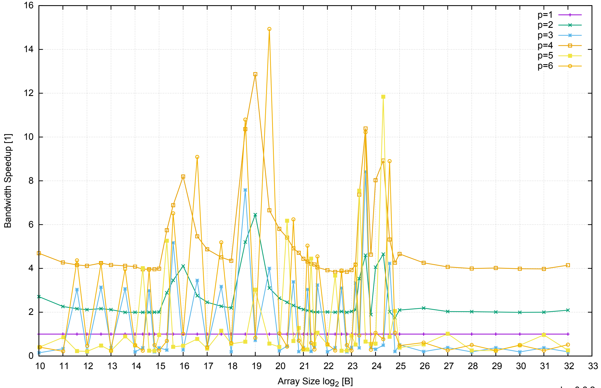
AWS c4.xlarge - Intel Xeon E5-2666 v3 2.90 GHz 7.5GB - Speedup of Parallel Memory Bandwidth - PermRead64UnrollLoop
