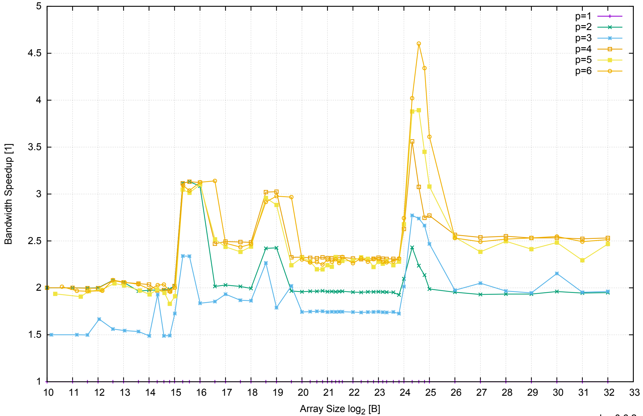
AWS c4.xlarge - Intel Xeon E5-2666 v3 2.90 GHz 7.5GB - Speedup of Parallel Memory Bandwidth - ScanRead64IndexUnrollLoop
