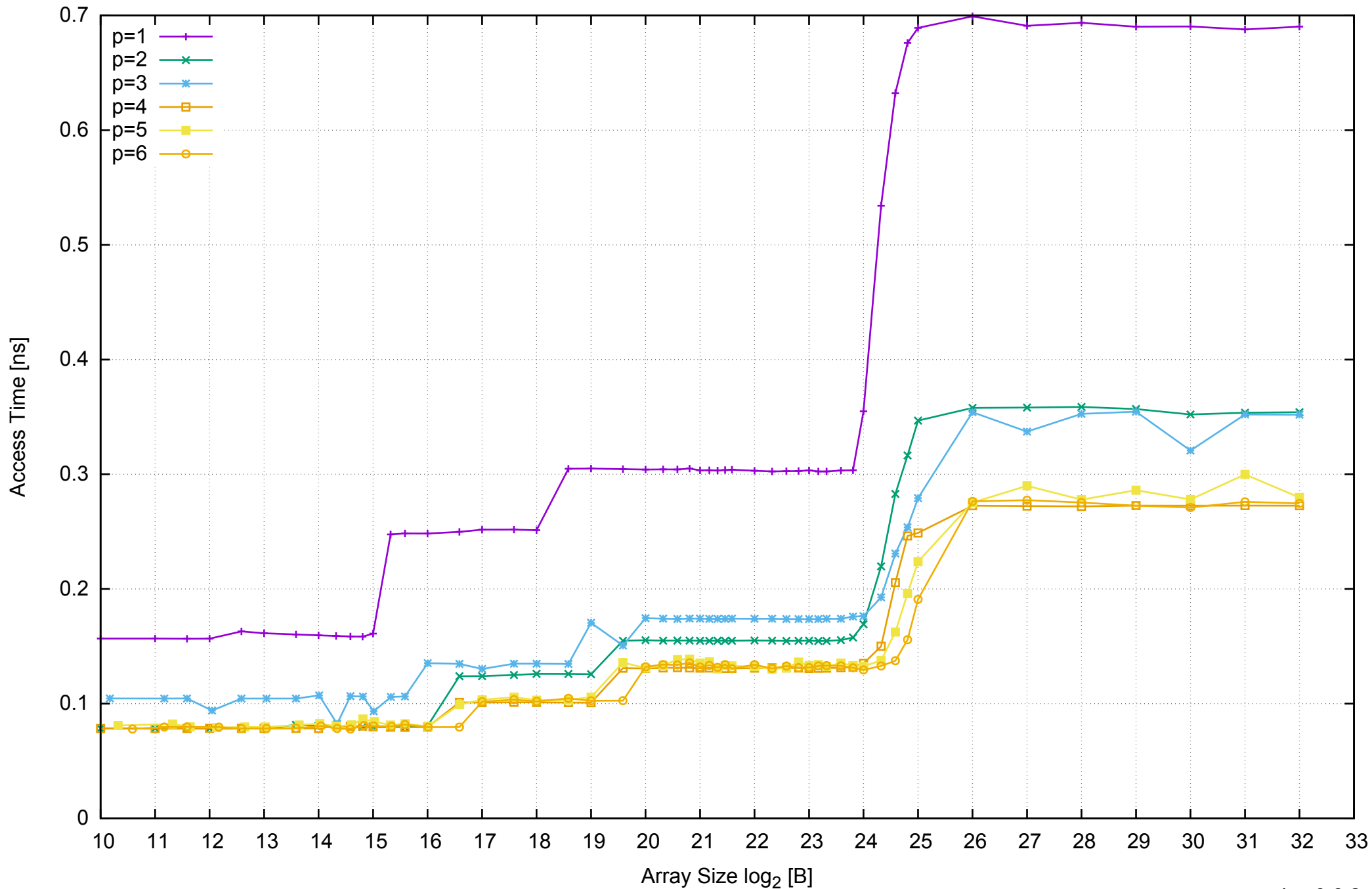
AWS c4.xlarge - Intel Xeon E5-2666 v3 2.90 GHz 7.5GB - Parallel Memory Access Time - ScanRead64IndexUnrollLoop
