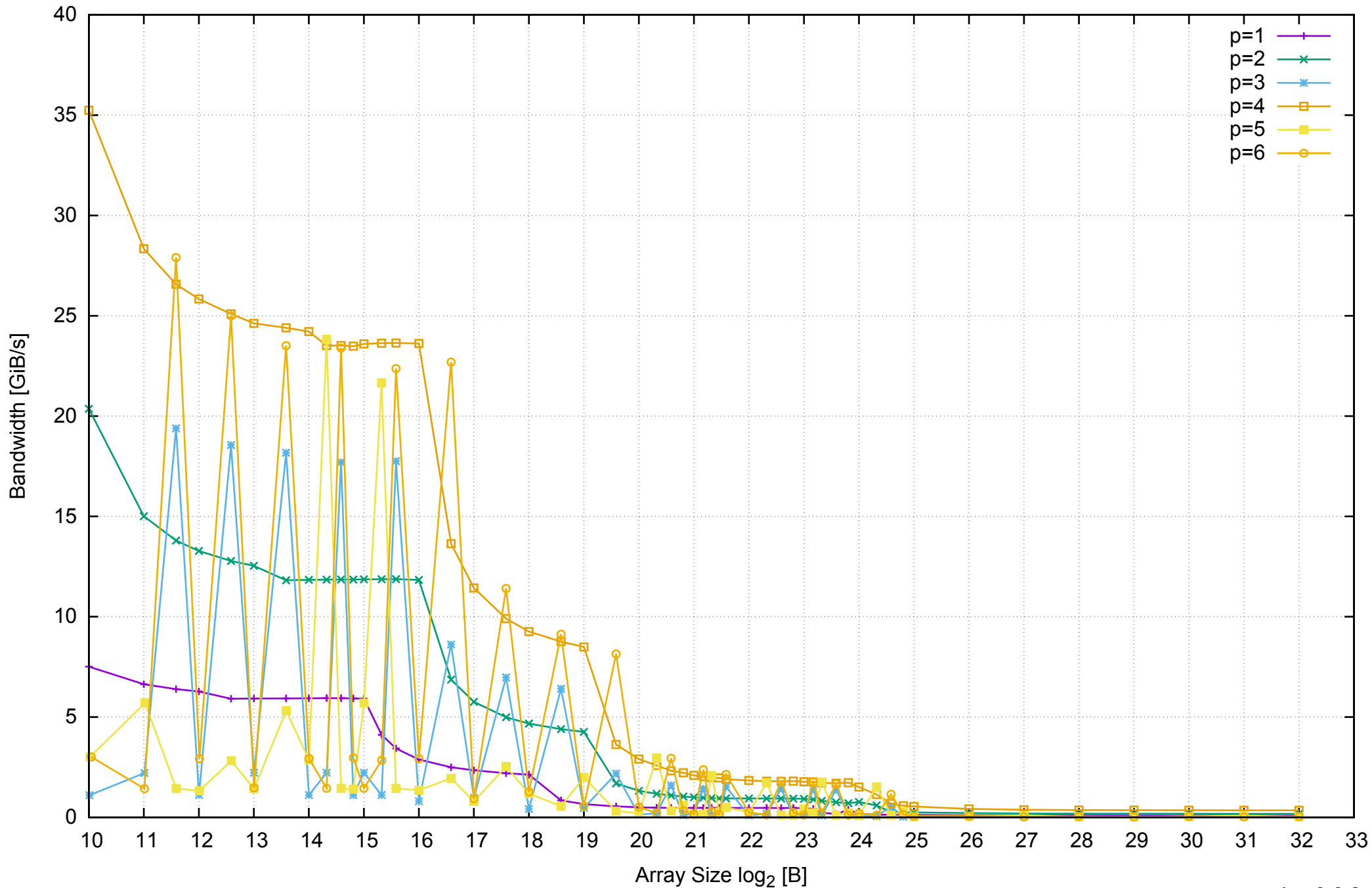
AWS c4.xlarge - Intel Xeon E5-2666 v3 2.90 GHz 7.5GB - Parallel Memory Bandwidth - PermRead64UnrollLoop
