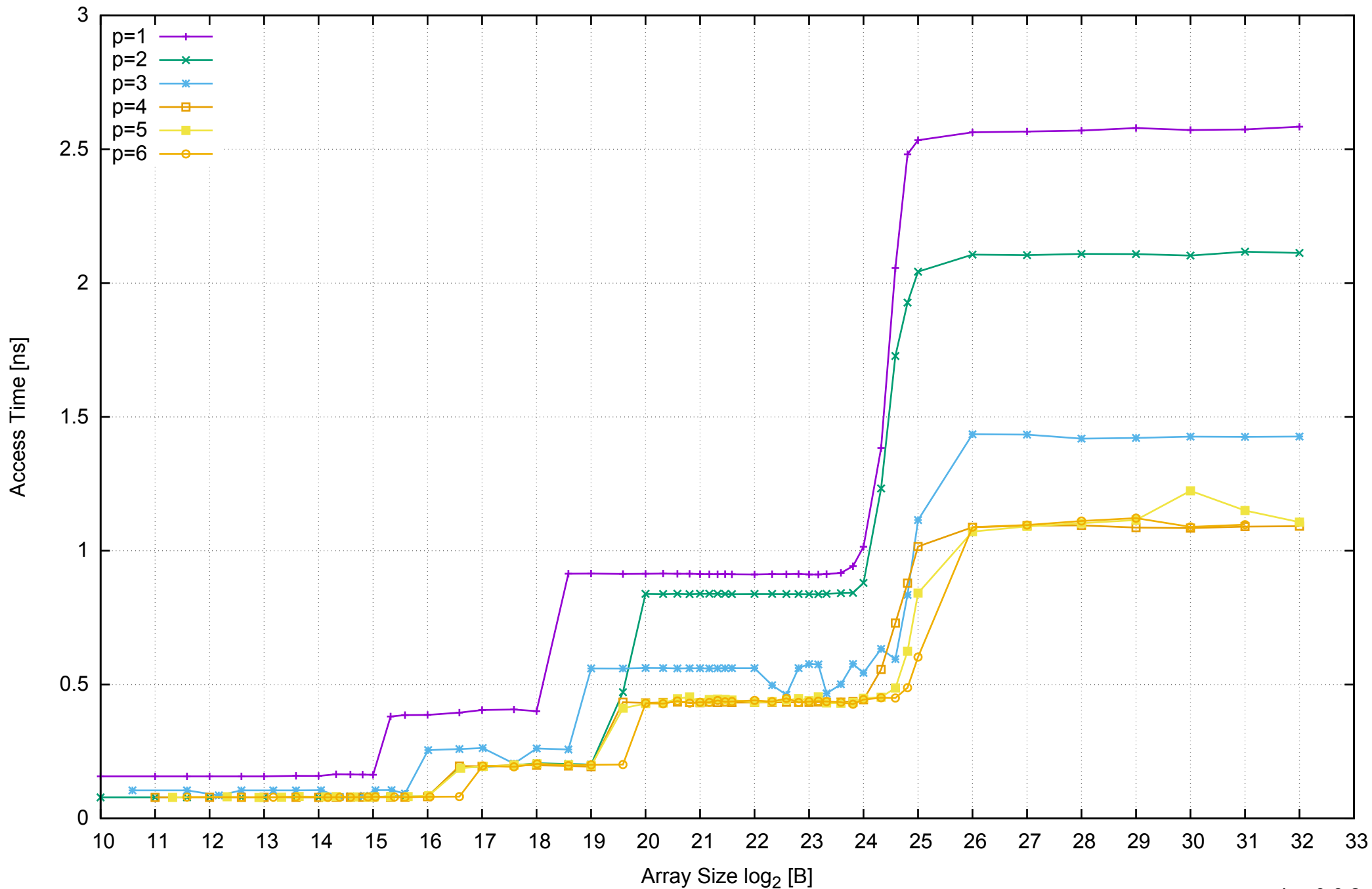
AWS c4.xlarge - Intel Xeon E5-2666 v3 2.90 GHz 7.5GB - Parallel Memory Access Time - ScanRead256PtrUnrollLoop
