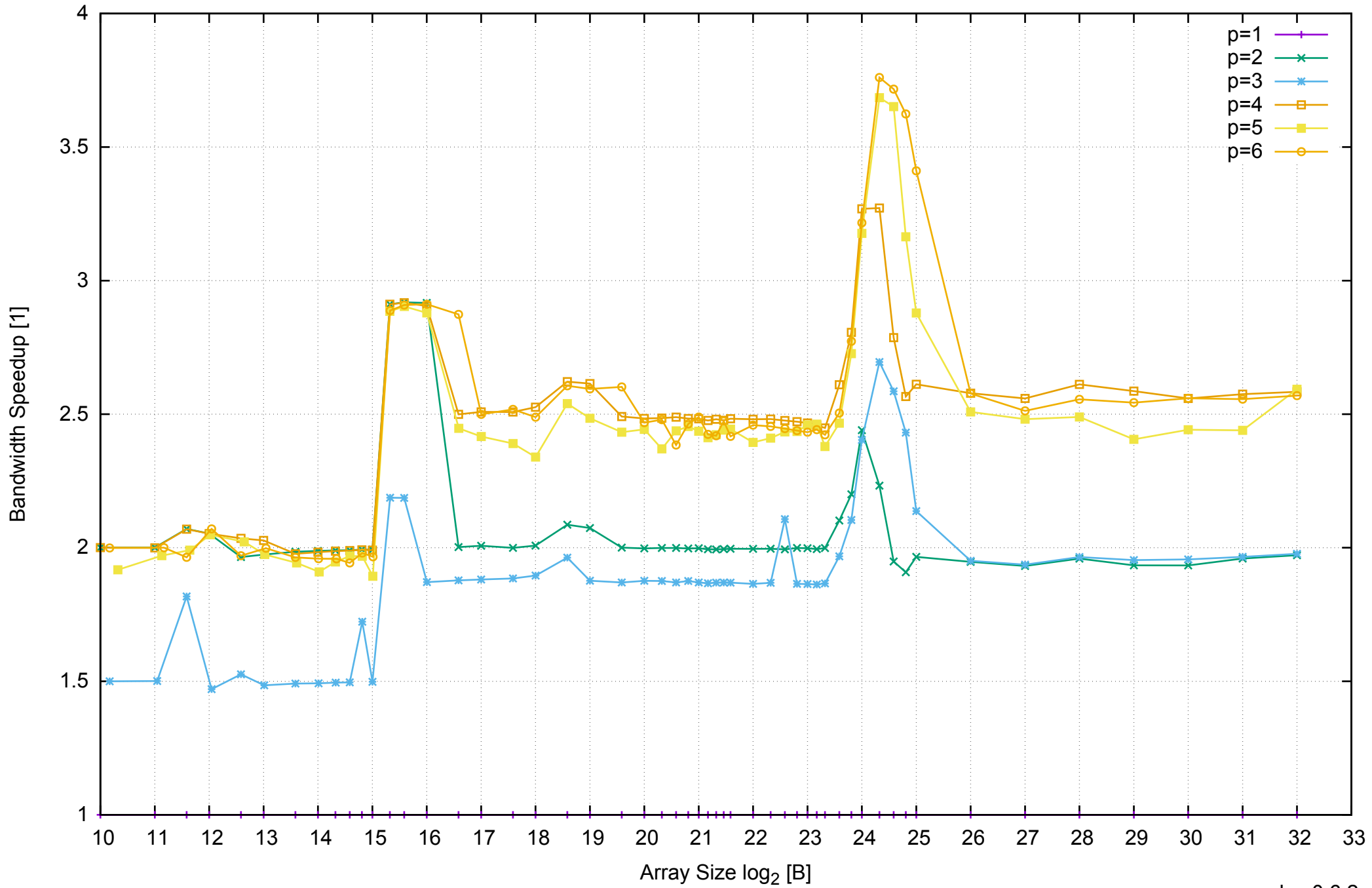
AWS c4.xlarge - Intel Xeon E5-2666 v3 2.90 GHz 7.5GB - Speedup of Parallel Memory Bandwidth - ScanRead32PtrUnrollLoop
