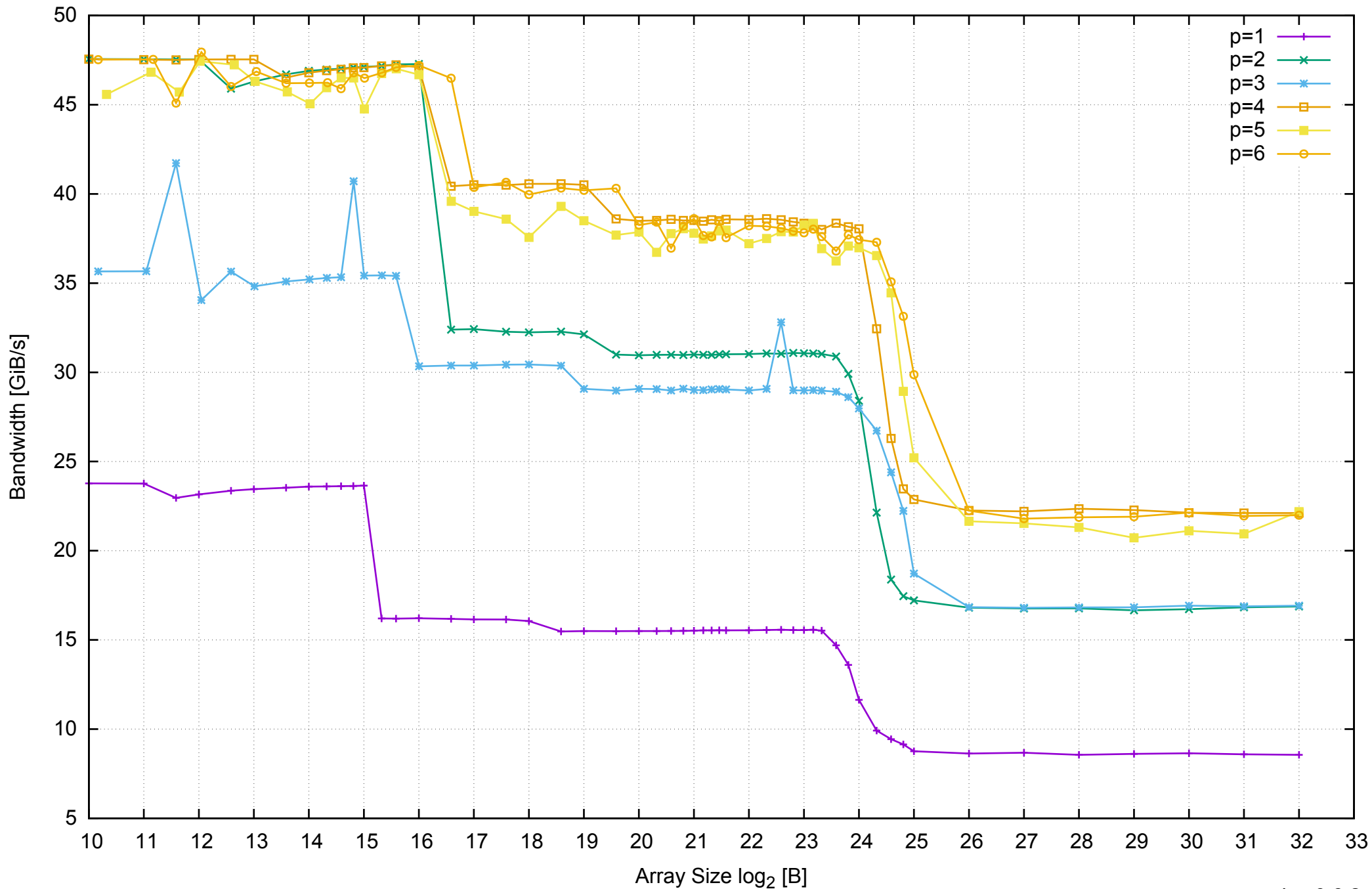
AWS c4.xlarge - Intel Xeon E5-2666 v3 2.90 GHz 7.5GB - Parallel Memory Bandwidth - ScanRead32PtrUnrollLoop
