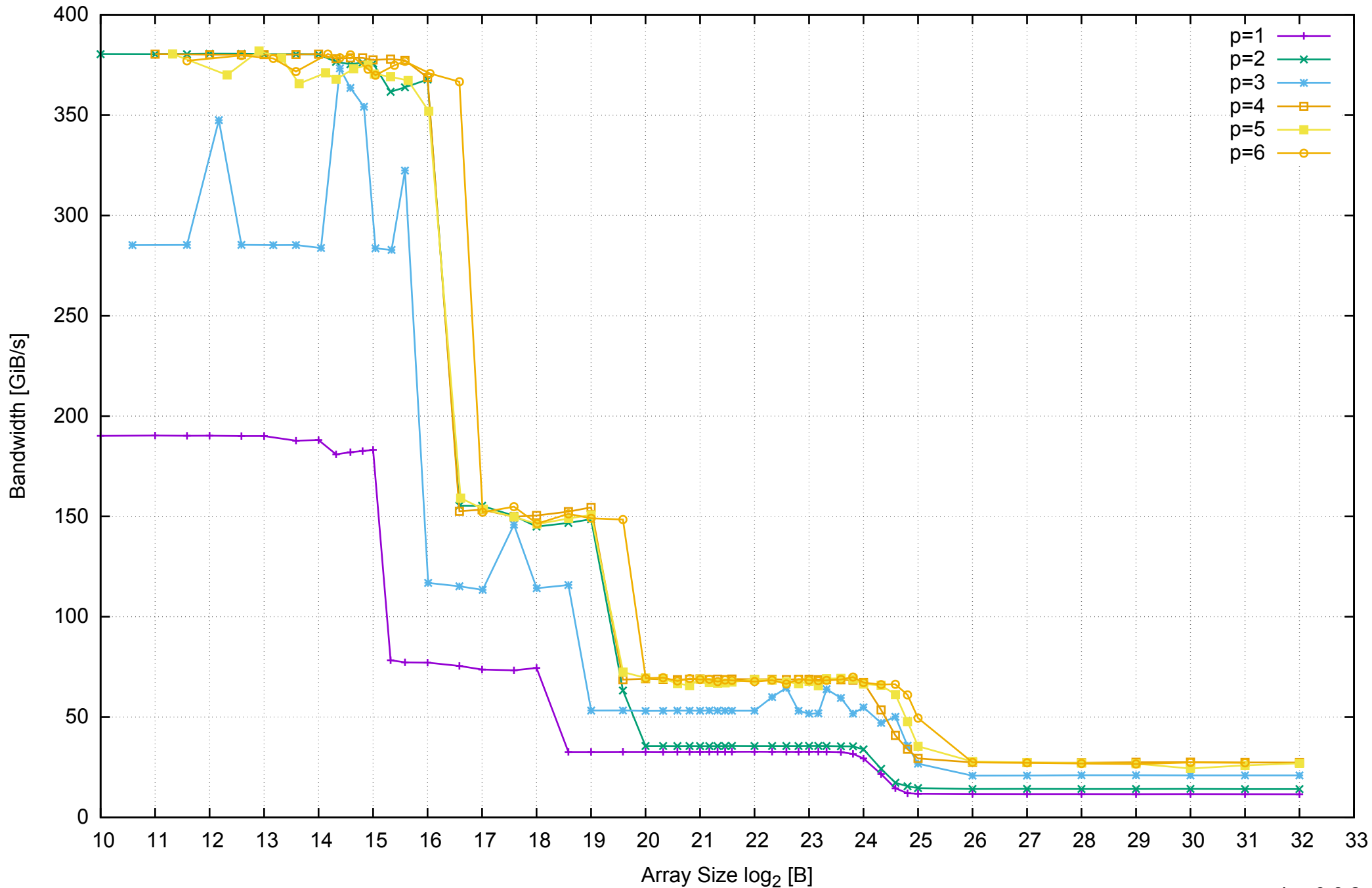
AWS c4.xlarge - Intel Xeon E5-2666 v3 2.90 GHz 7.5GB - Parallel Memory Bandwidth - ScanRead256PtrUnrollLoop
