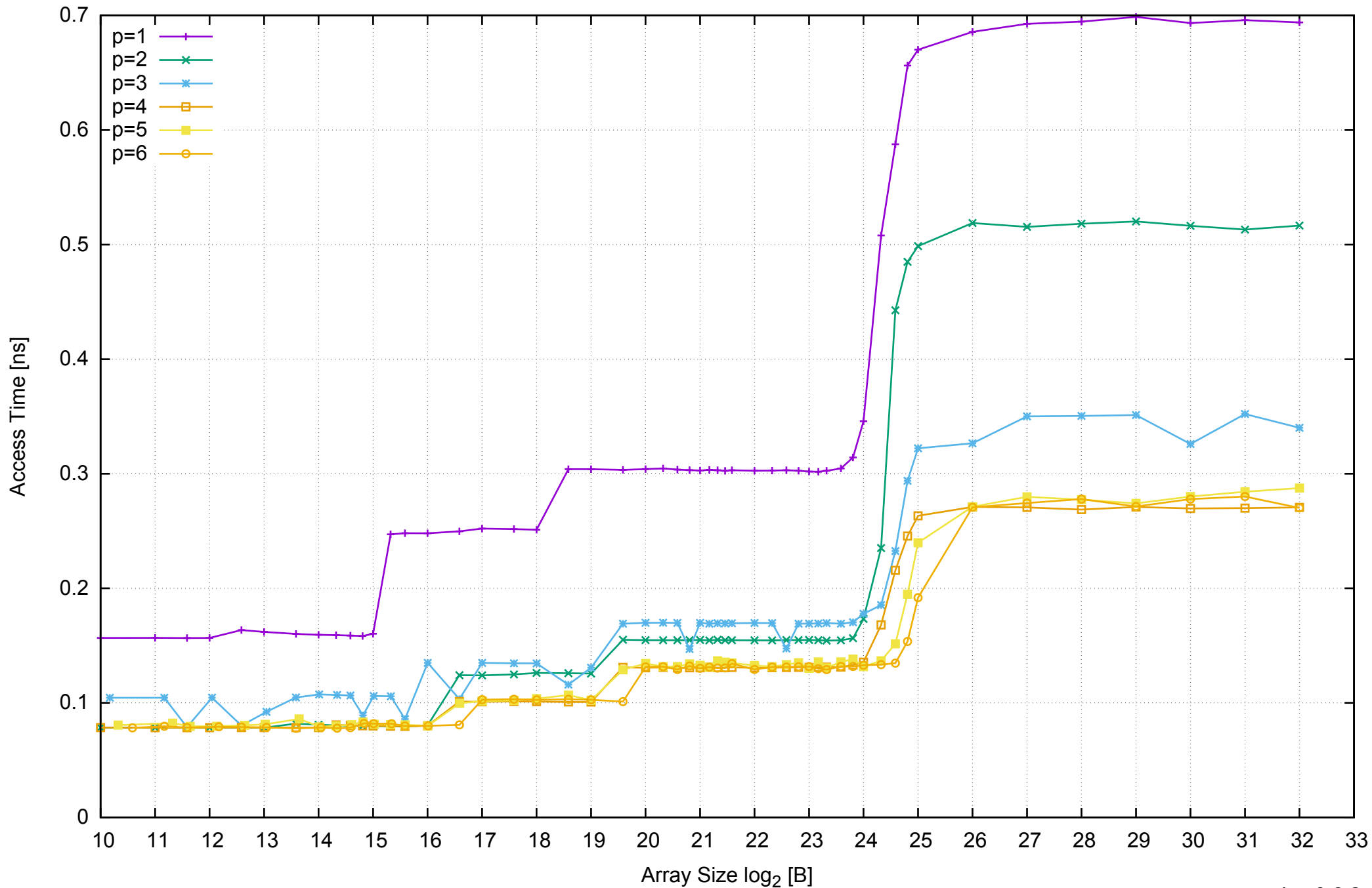
AWS c4.xlarge - Intel Xeon E5-2666 v3 2.90 GHz 7.5GB - Parallel Memory Access Time - ScanRead64PtrUnrollLoop
