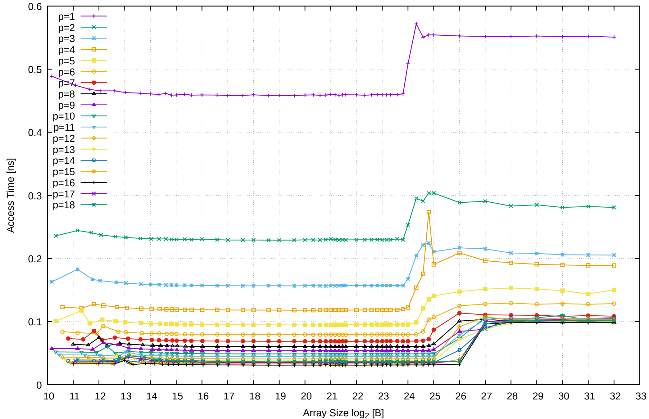
AMD Ryzen Threadripper 3955WX 128GB - Parallel Memory Access Time - ScanRead64PtrSimpleLoop
