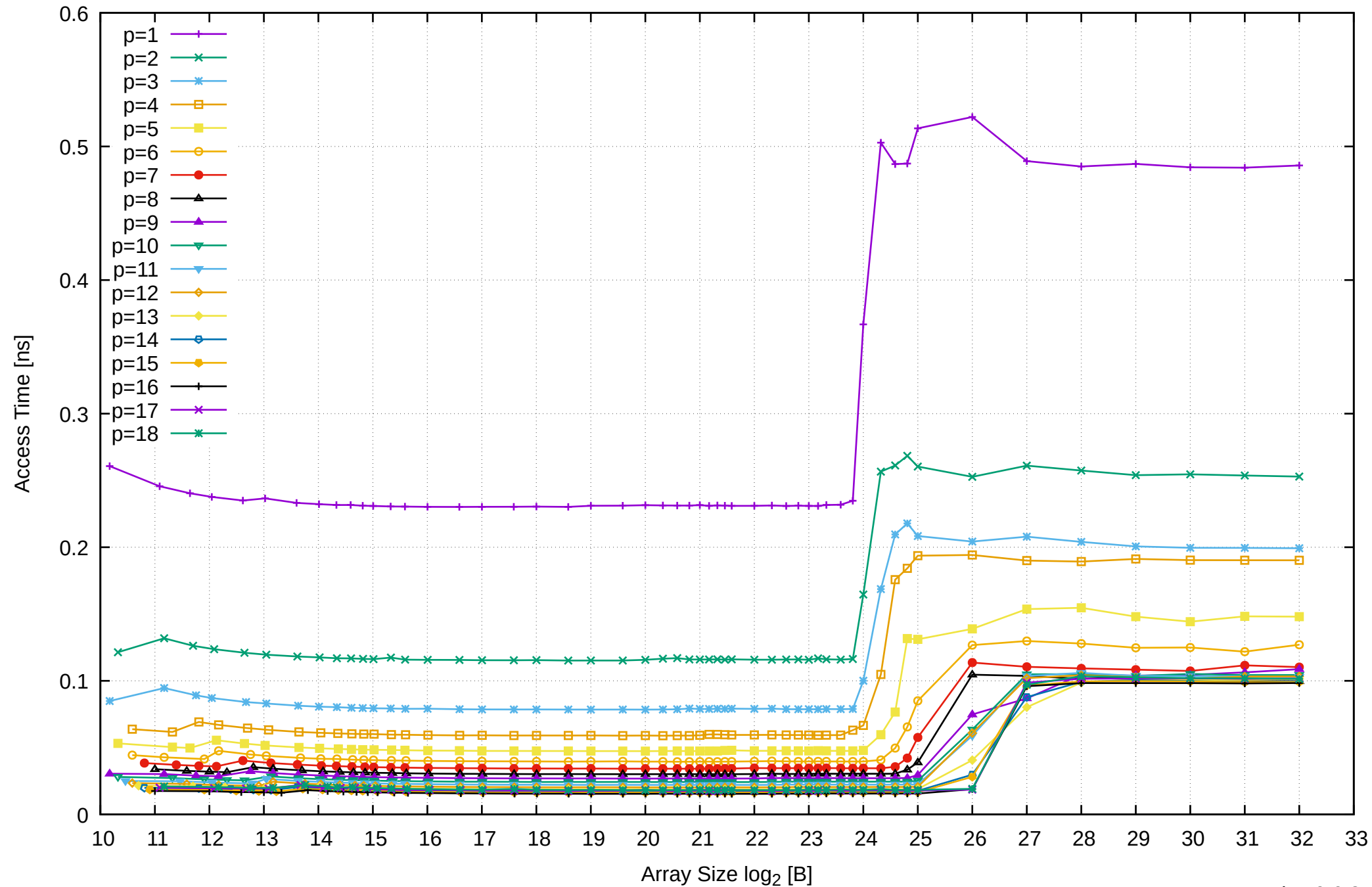
AMD Ryzen Threadripper 3955WX 128GB - Parallel Memory Access Time - ScanRead64IndexSimpleLoop
