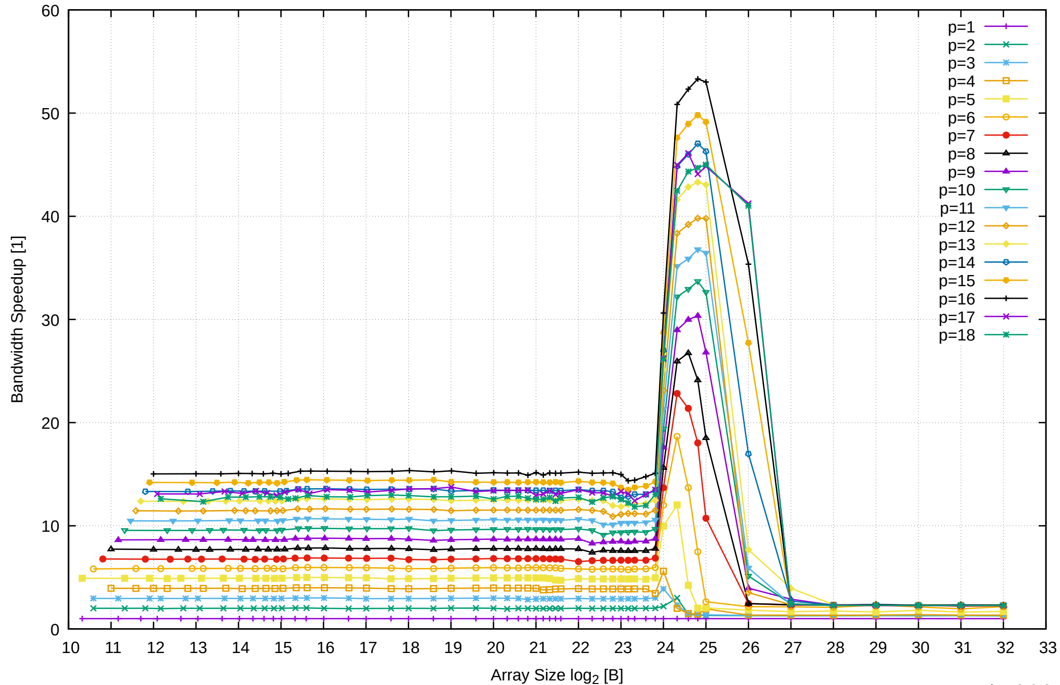
AMD Ryzen Threadripper 3955WX 128GB - Speedup of Parallel Memory Bandwidth - ScanWrite128PtrUnrollLoop
