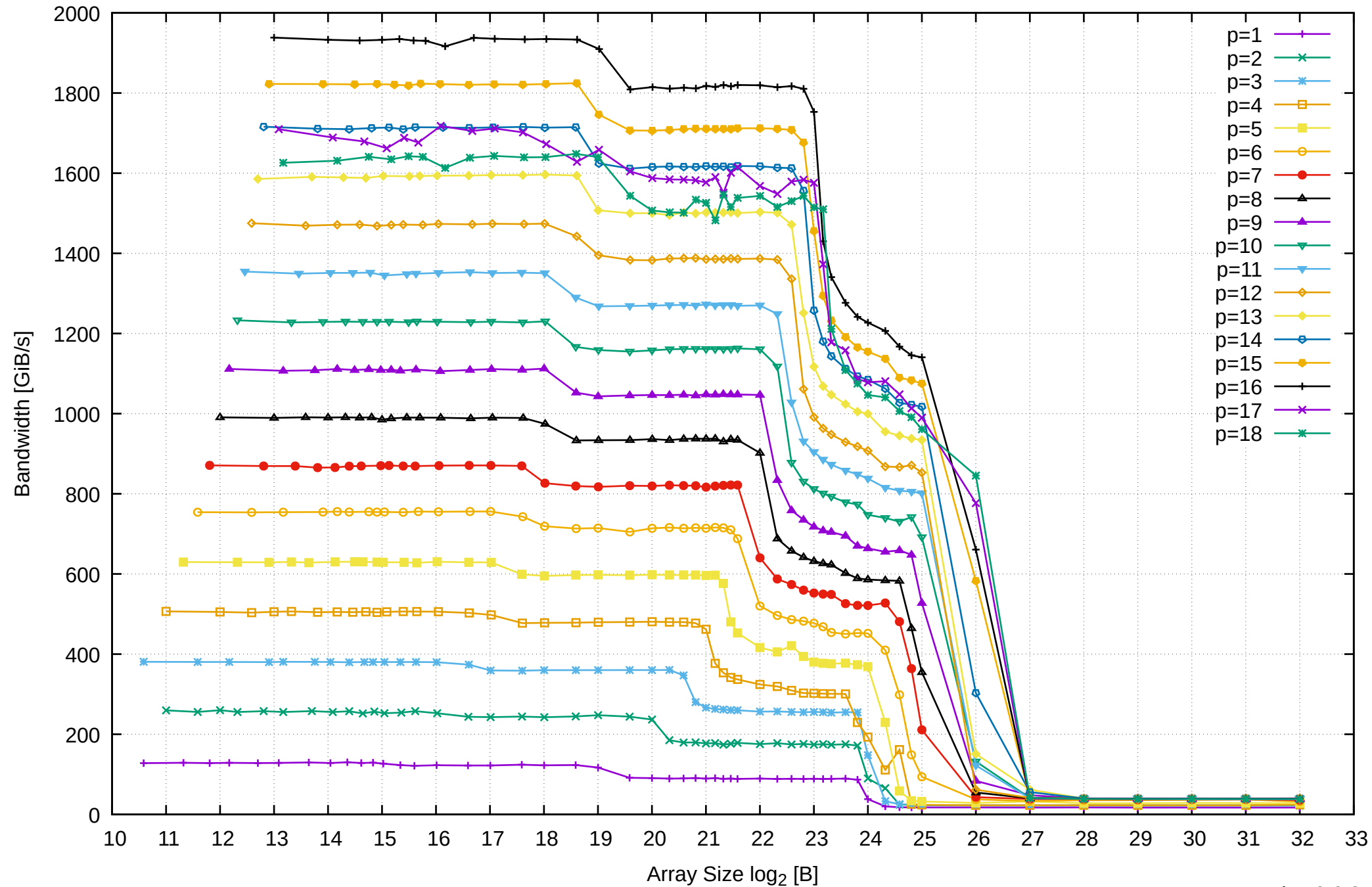
AMD Ryzen Threadripper 3955WX 128GB - Parallel Memory Bandwidth - ScanWrite256PtrUnrollLoop
