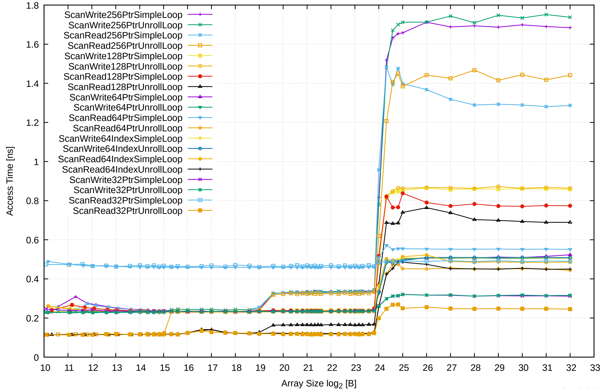
AMD Ryzen Threadripper 3955WX 128GB - One Thread Memory Latency (excluding Permutation)
