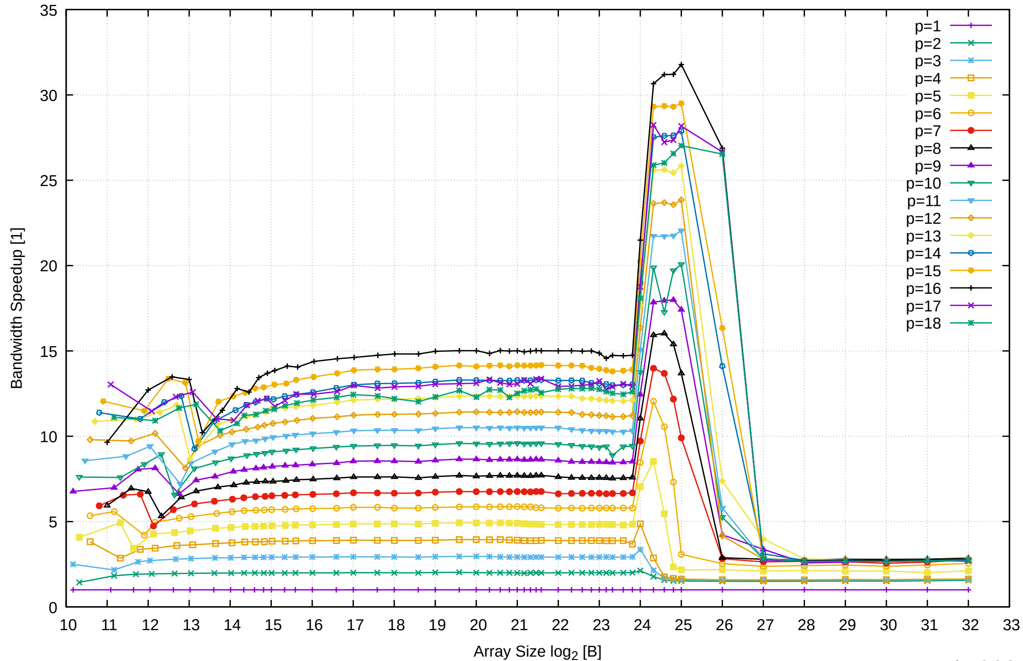
AMD Ryzen Threadripper 3955WX 128GB - Speedup of Parallel Memory Bandwidth - ScanWrite64PtrSimpleLoop
