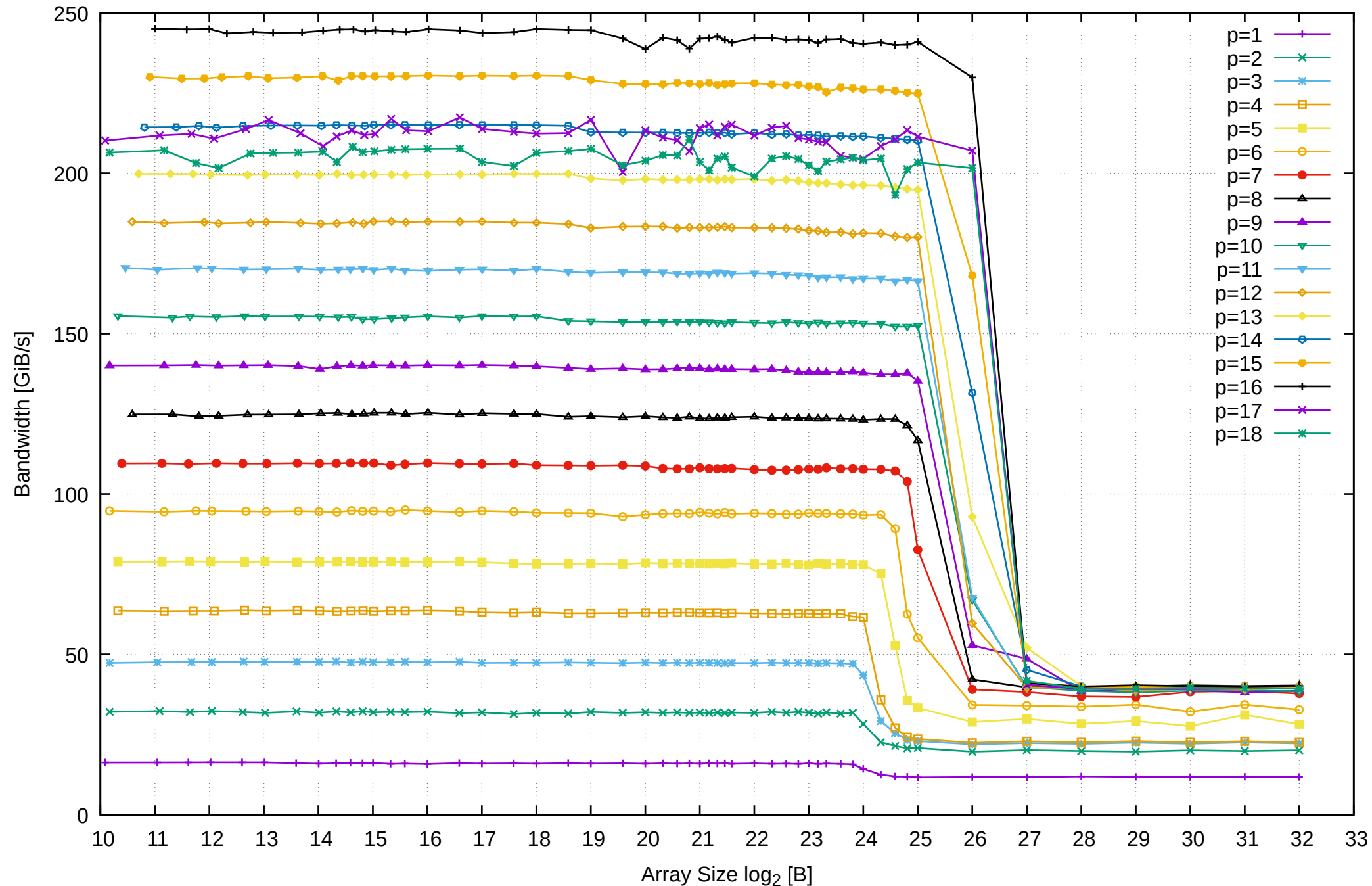
AMD Ryzen Threadripper 3955WX 128GB - Parallel Memory Bandwidth - ScanWrite32PtrUnrollLoop
