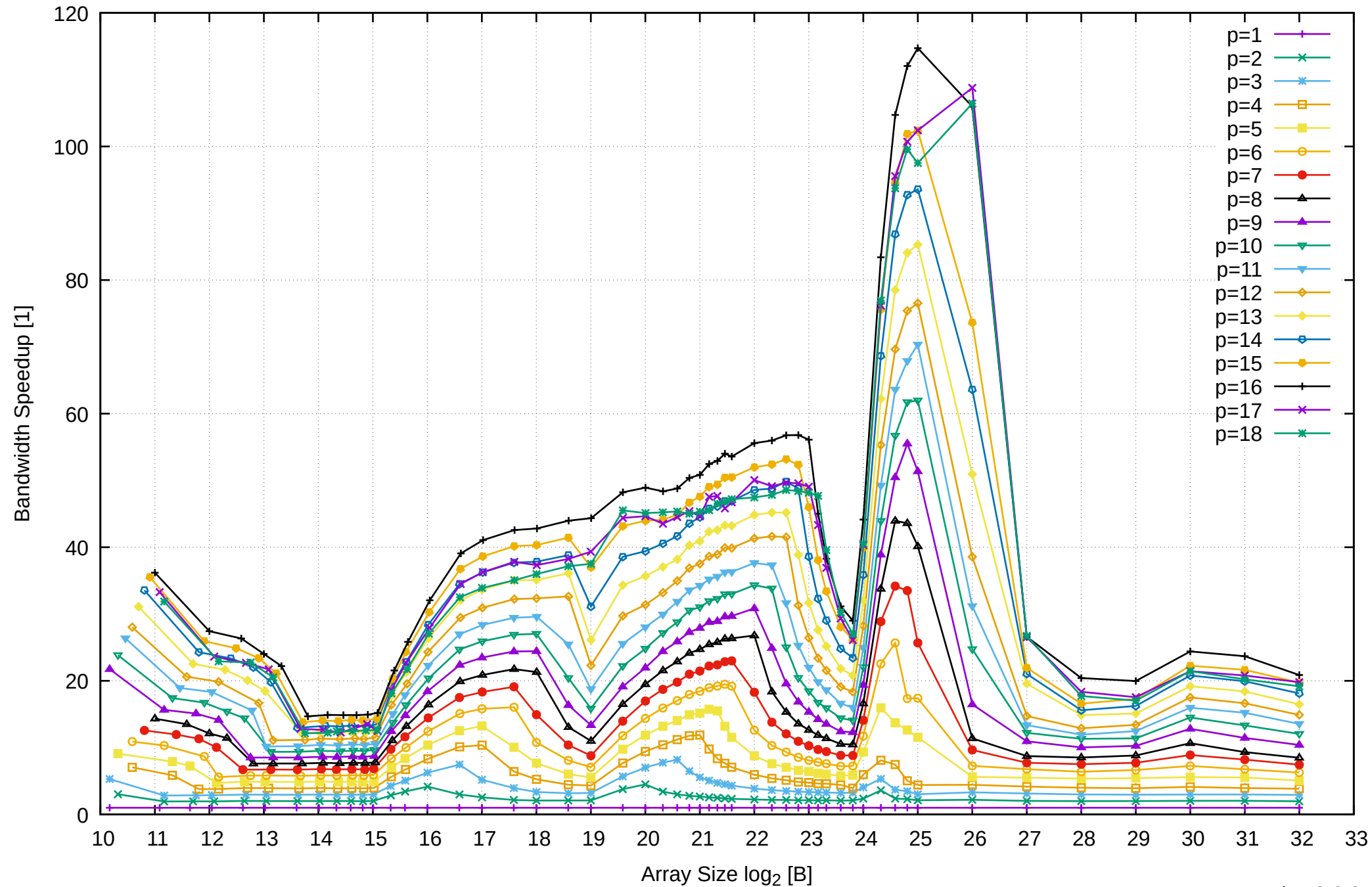
AMD Ryzen Threadripper 3955WX 128GB - Speedup of Parallel Memory Bandwidth - PermRead64SimpleLoop
