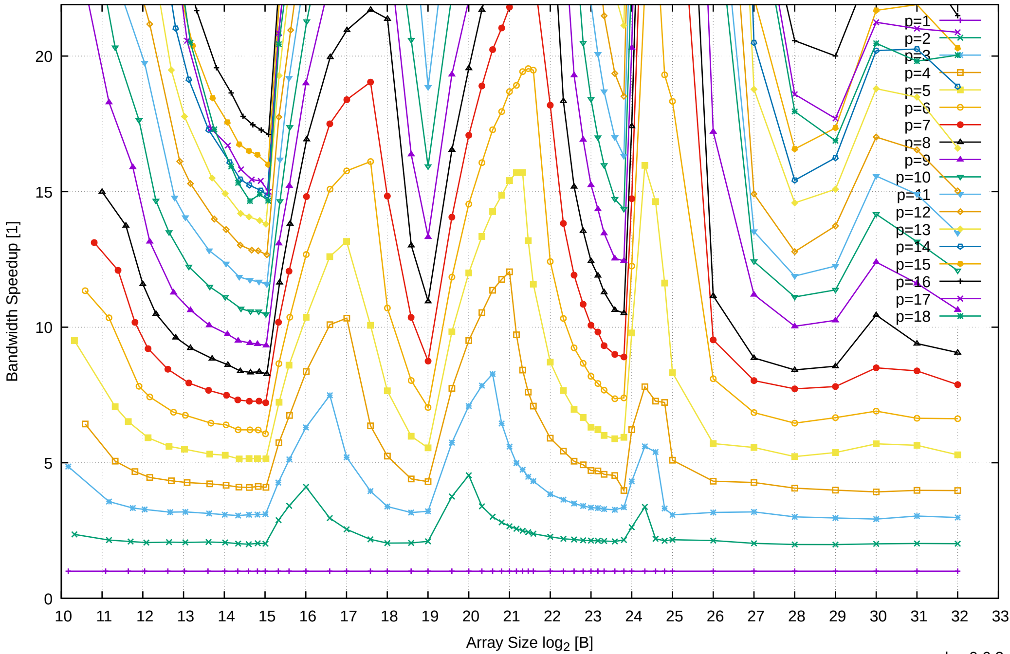
AMD Ryzen Threadripper 3955WX 128GB - Speedup of Parallel Memory Bandwidth (enlarged) - PermRead64UnrollLoop
