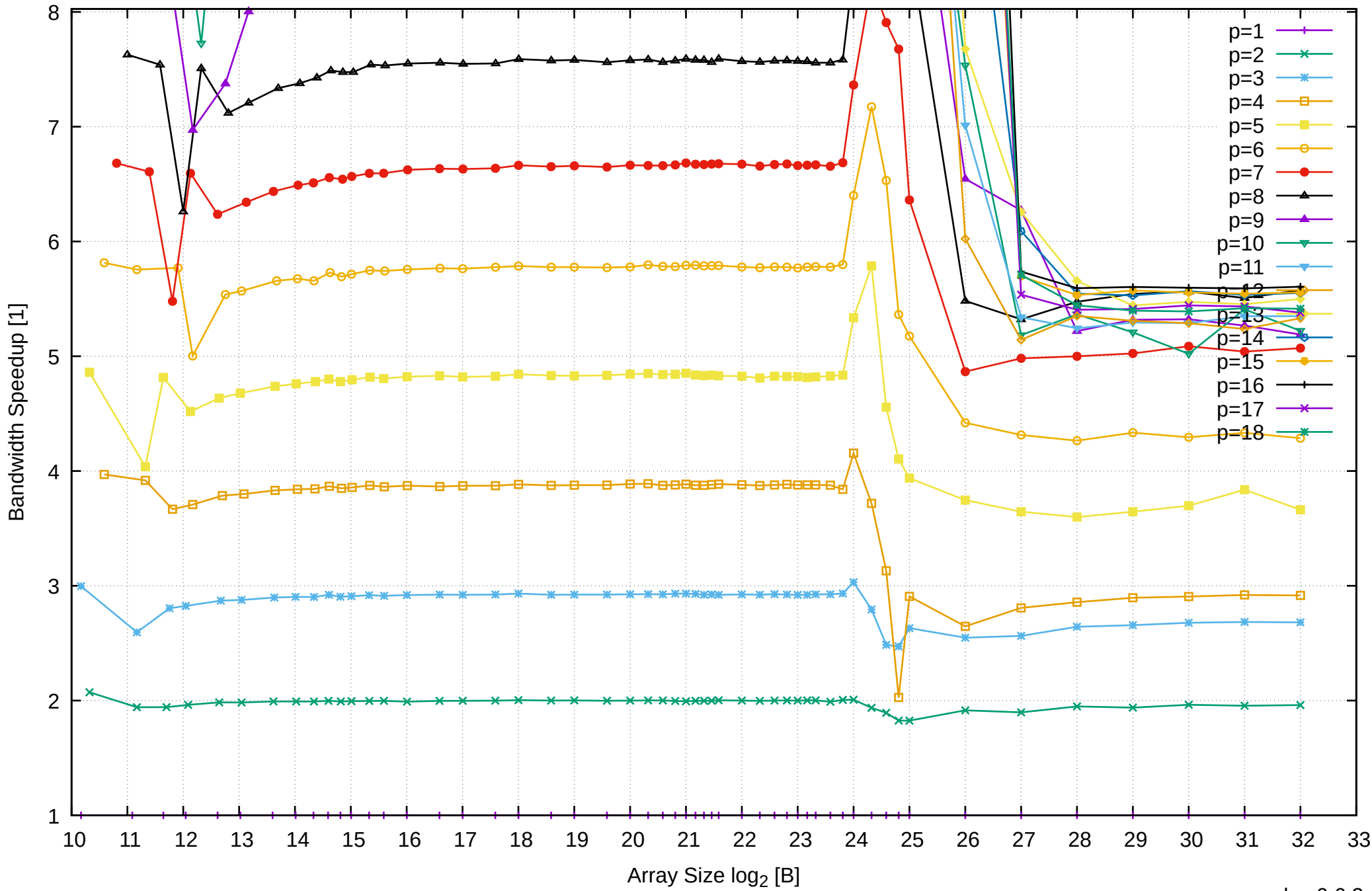
AMD Ryzen Threadripper 3955WX 128GB - Speedup of Parallel Memory Bandwidth (enlarged) - ScanRead64PtrSimpleLoop
