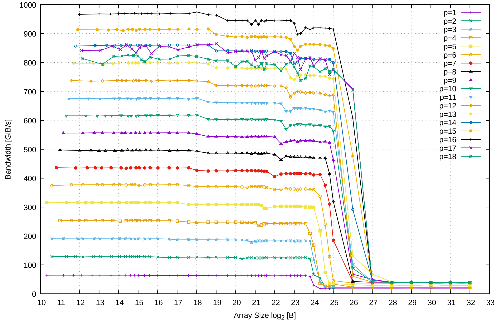
AMD Ryzen Threadripper 3955WX 128GB - Parallel Memory Bandwidth - ScanWrite128PtrUnrollLoop
