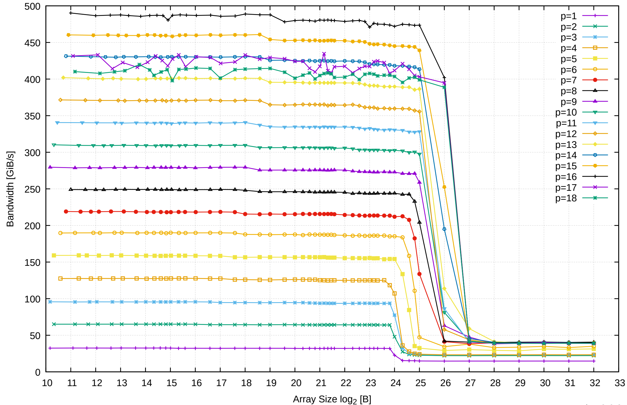
AMD Ryzen Threadripper 3955WX 128GB - Parallel Memory Bandwidth - ScanWrite64PtrUnrollLoop
