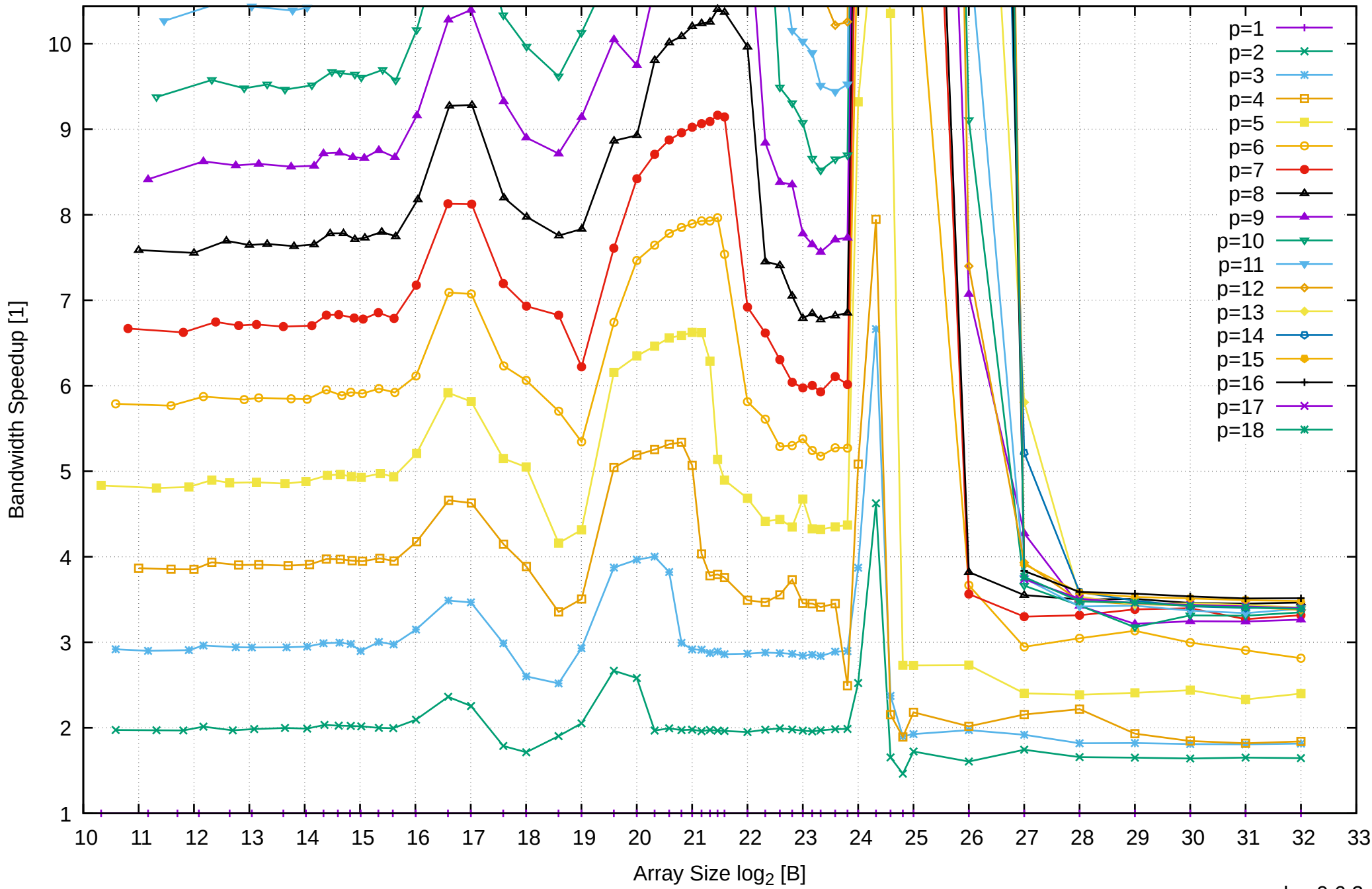
AMD Ryzen Threadripper 3955WX 128GB - Speedup of Parallel Memory Bandwidth (enlarged) - ScanRead128PtrUnrollLoop
