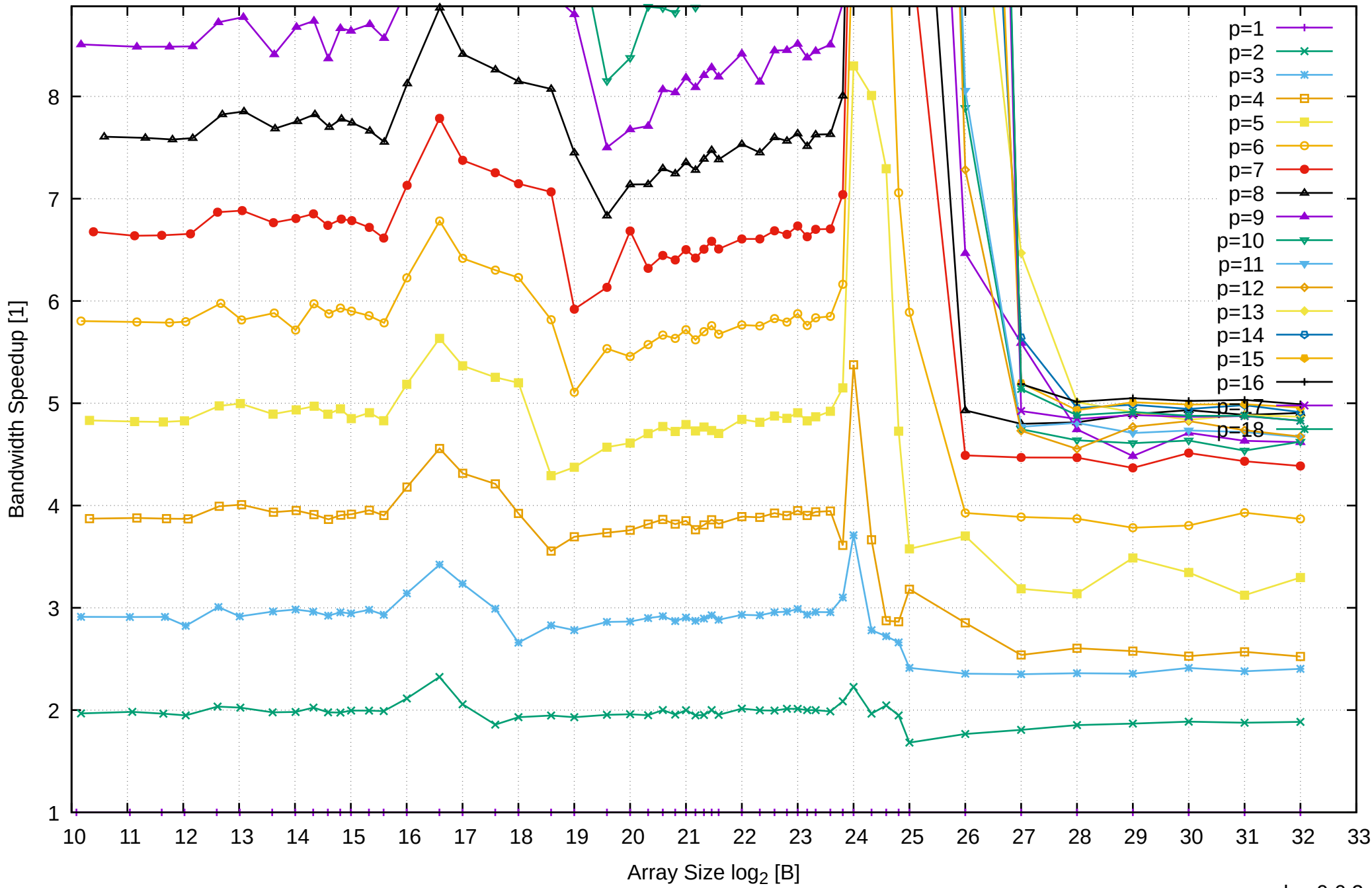
AMD Ryzen Threadripper 3955WX 128GB - Speedup of Parallel Memory Bandwidth (enlarged) - ScanRead32PtrUnrollLoop
