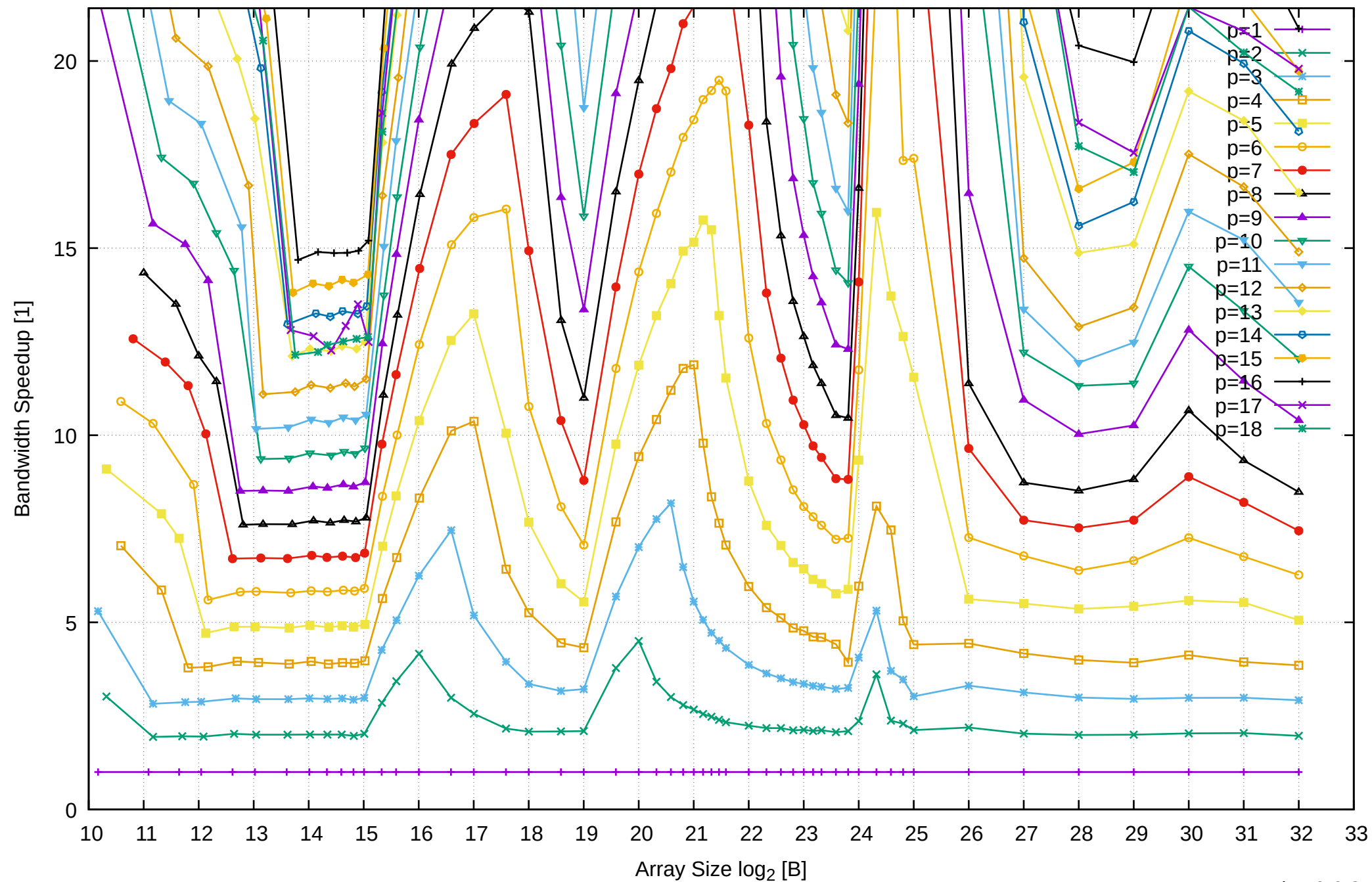
AMD Ryzen Threadripper 3955WX 128GB - Speedup of Parallel Memory Bandwidth (enlarged) - PermRead64SimpleLoop
