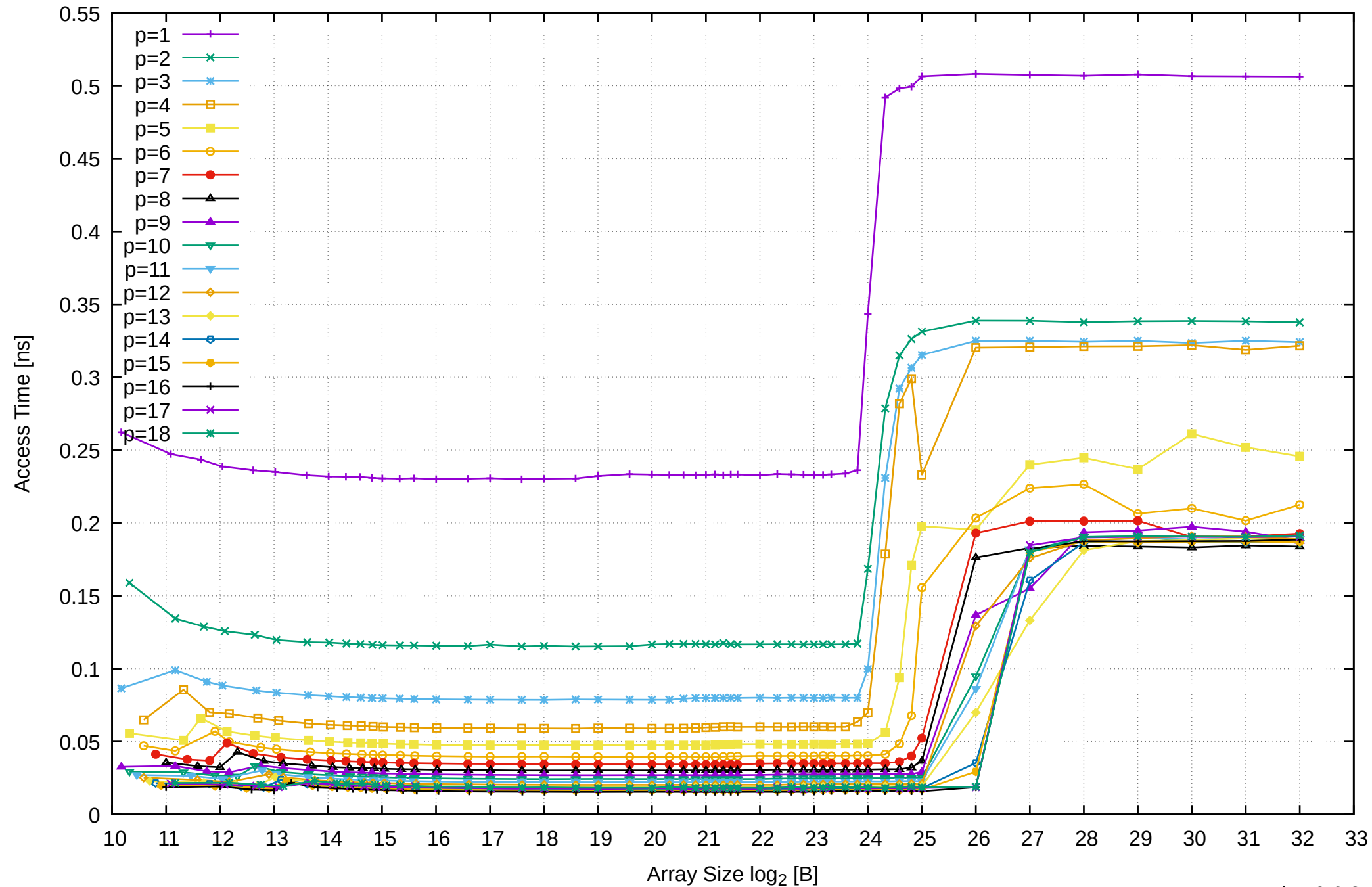
AMD Ryzen Threadripper 3955WX 128GB - Parallel Memory Access Time - ScanWrite64IndexSimpleLoop
