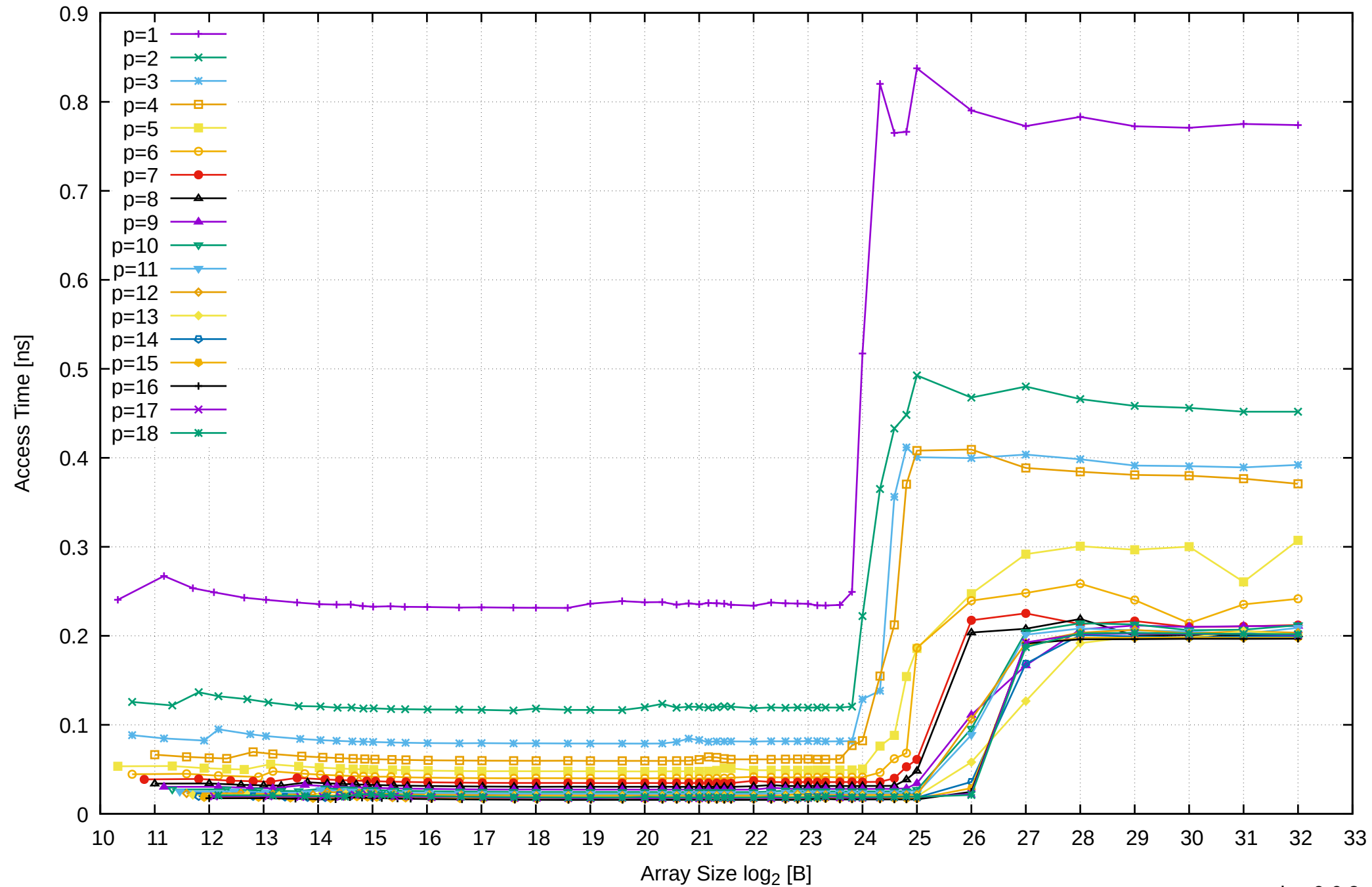
AMD Ryzen Threadripper 3955WX 128GB - Parallel Memory Access Time - ScanRead128PtrSimpleLoop
