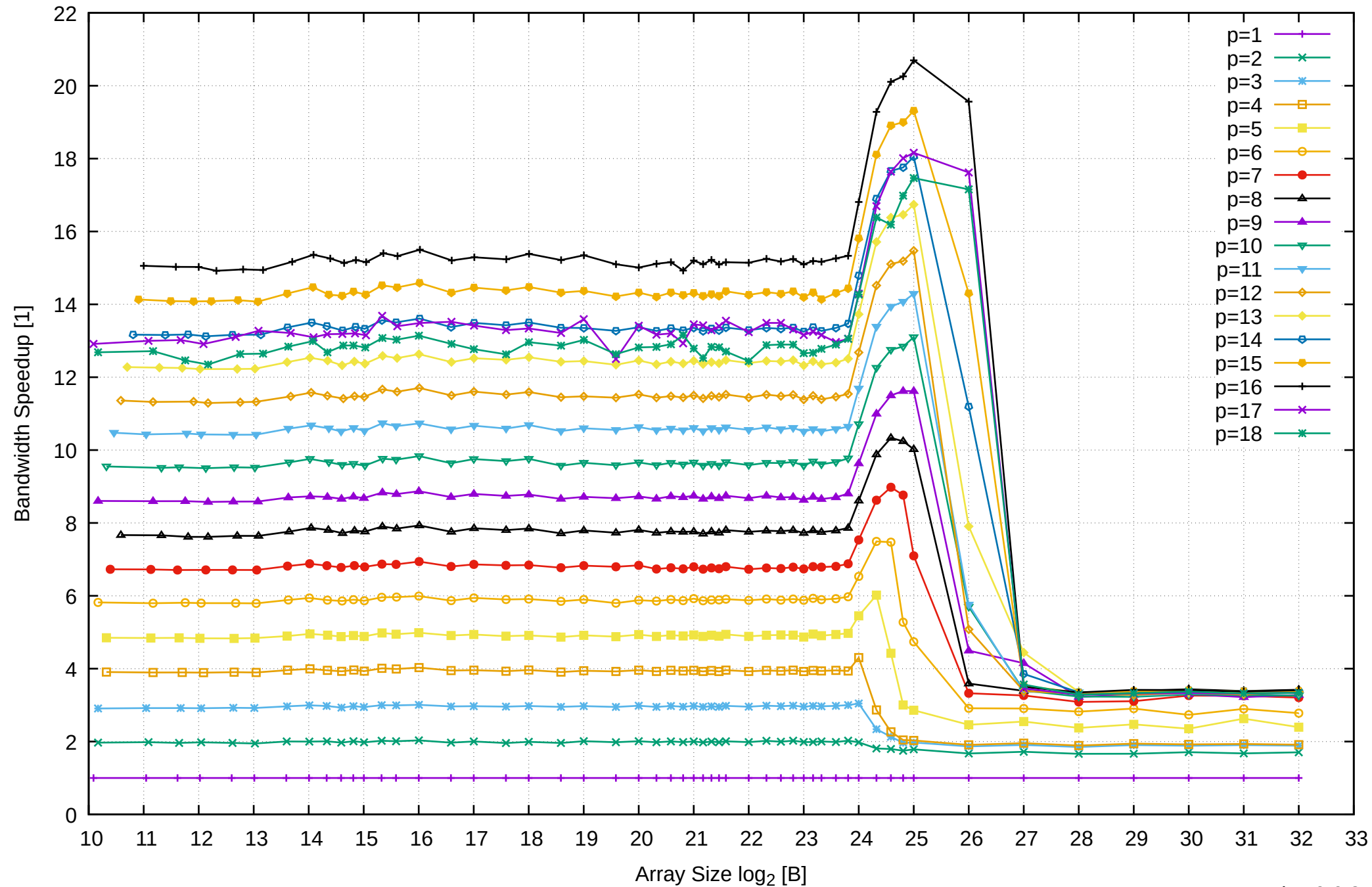
AMD Ryzen Threadripper 3955WX 128GB - Speedup of Parallel Memory Bandwidth - ScanWrite32PtrUnrollLoop
