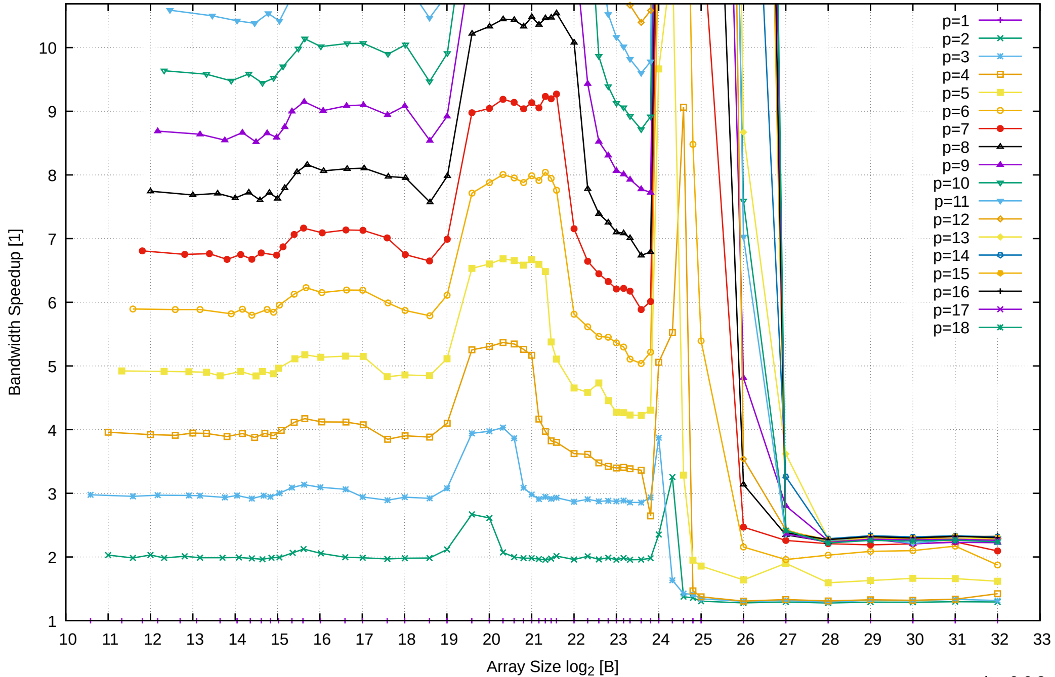
AMD Ryzen Threadripper 3955WX 128GB - Speedup of Parallel Memory Bandwidth (enlarged) - ScanWrite256PtrUnrollLoop
