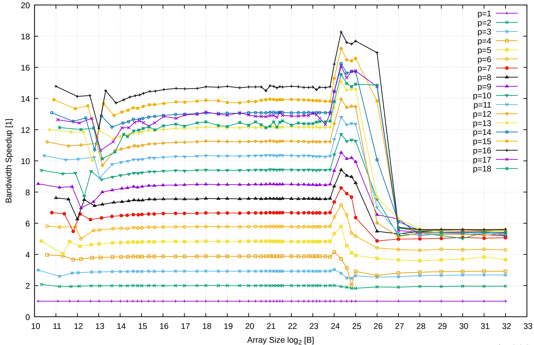
AMD Ryzen Threadripper 3955WX 128GB - Speedup of Parallel Memory Bandwidth - ScanRead64PtrSimpleLoop
