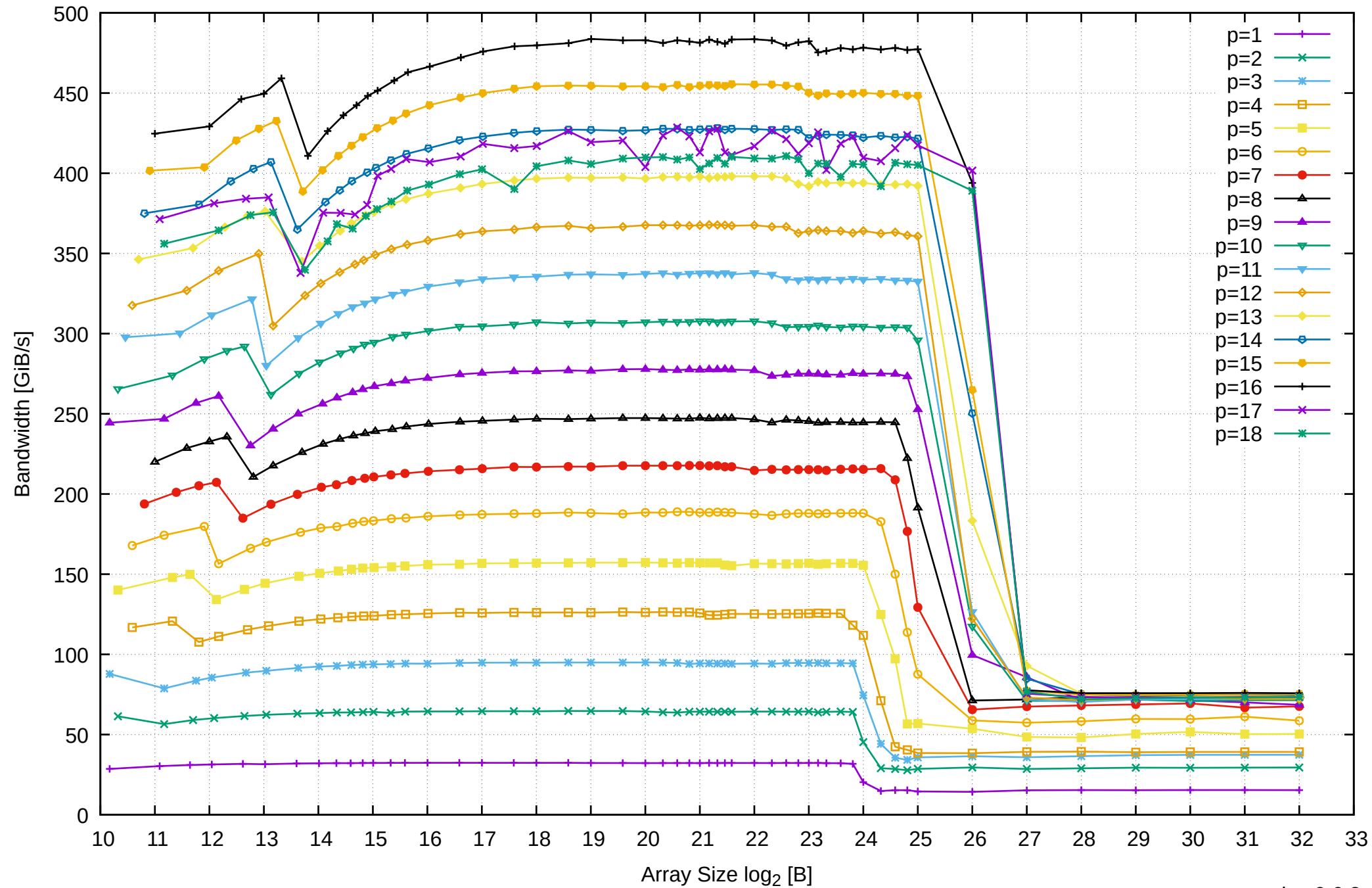
AMD Ryzen Threadripper 3955WX 128GB - Parallel Memory Bandwidth - ScanRead64IndexSimpleLoop
