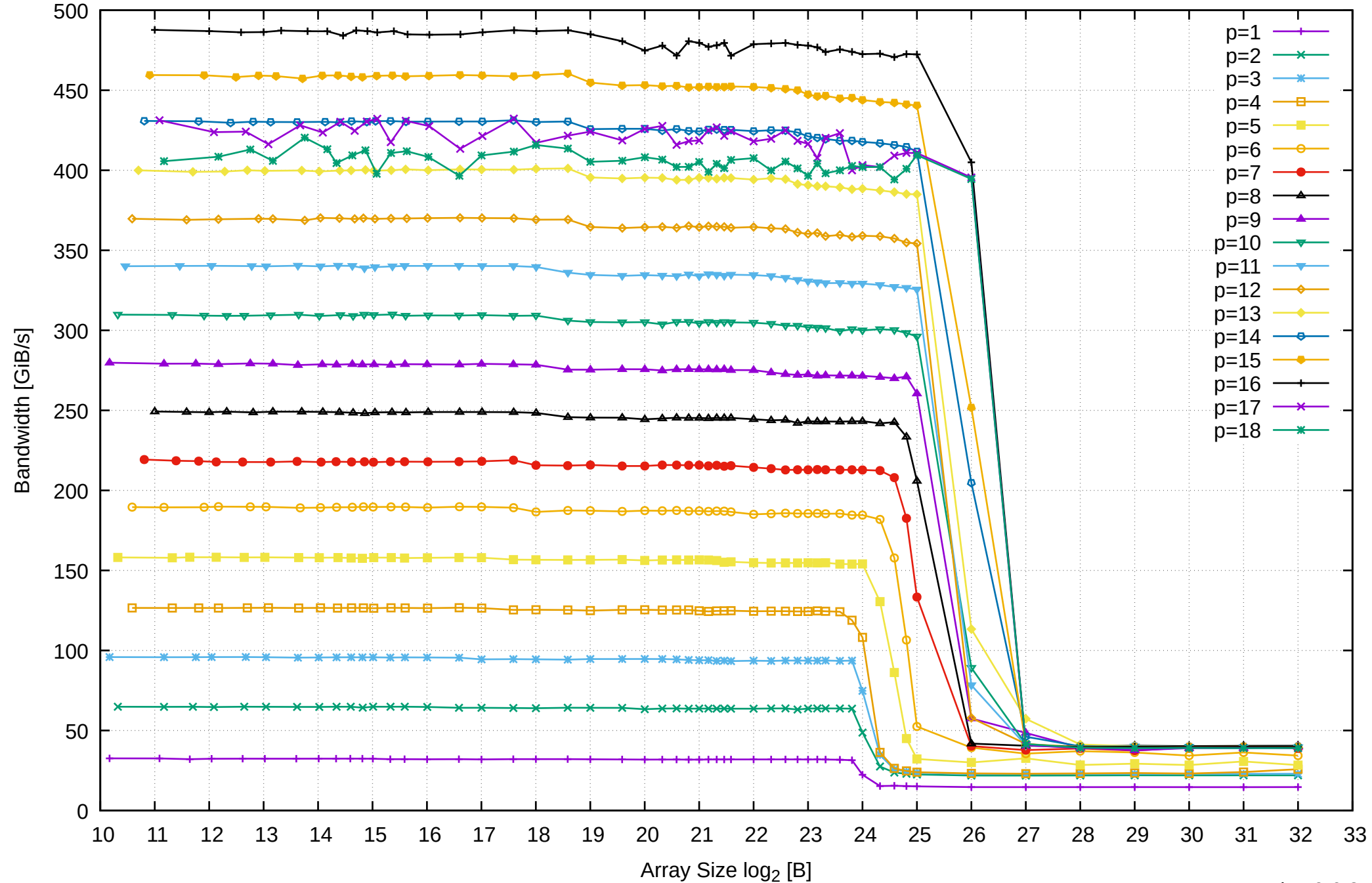
AMD Ryzen Threadripper 3955WX 128GB - Parallel Memory Bandwidth - ScanWrite64IndexUnrollLoop
