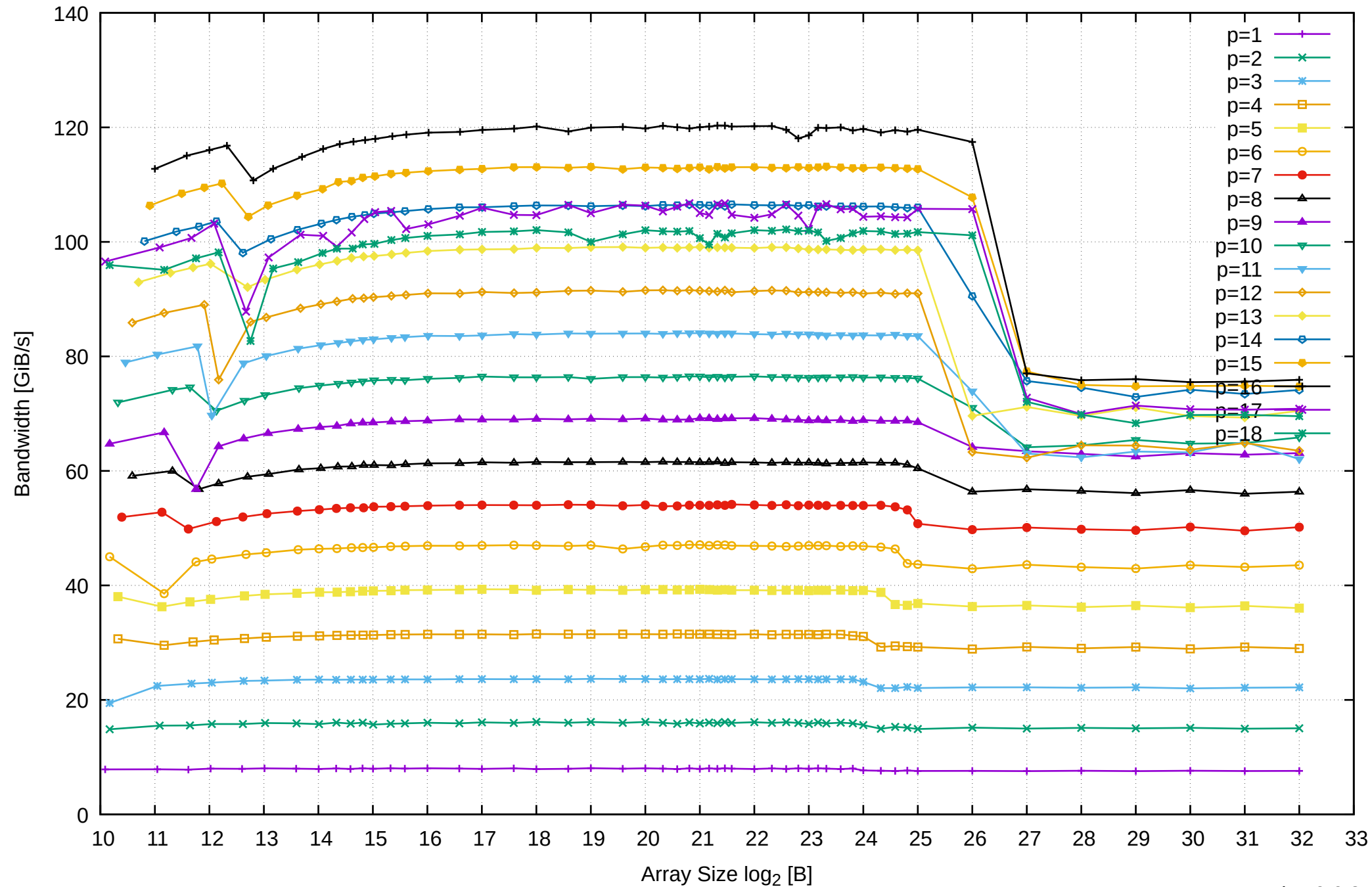
AMD Ryzen Threadripper 3955WX 128GB - Parallel Memory Bandwidth - ScanRead32PtrSimpleLoop
