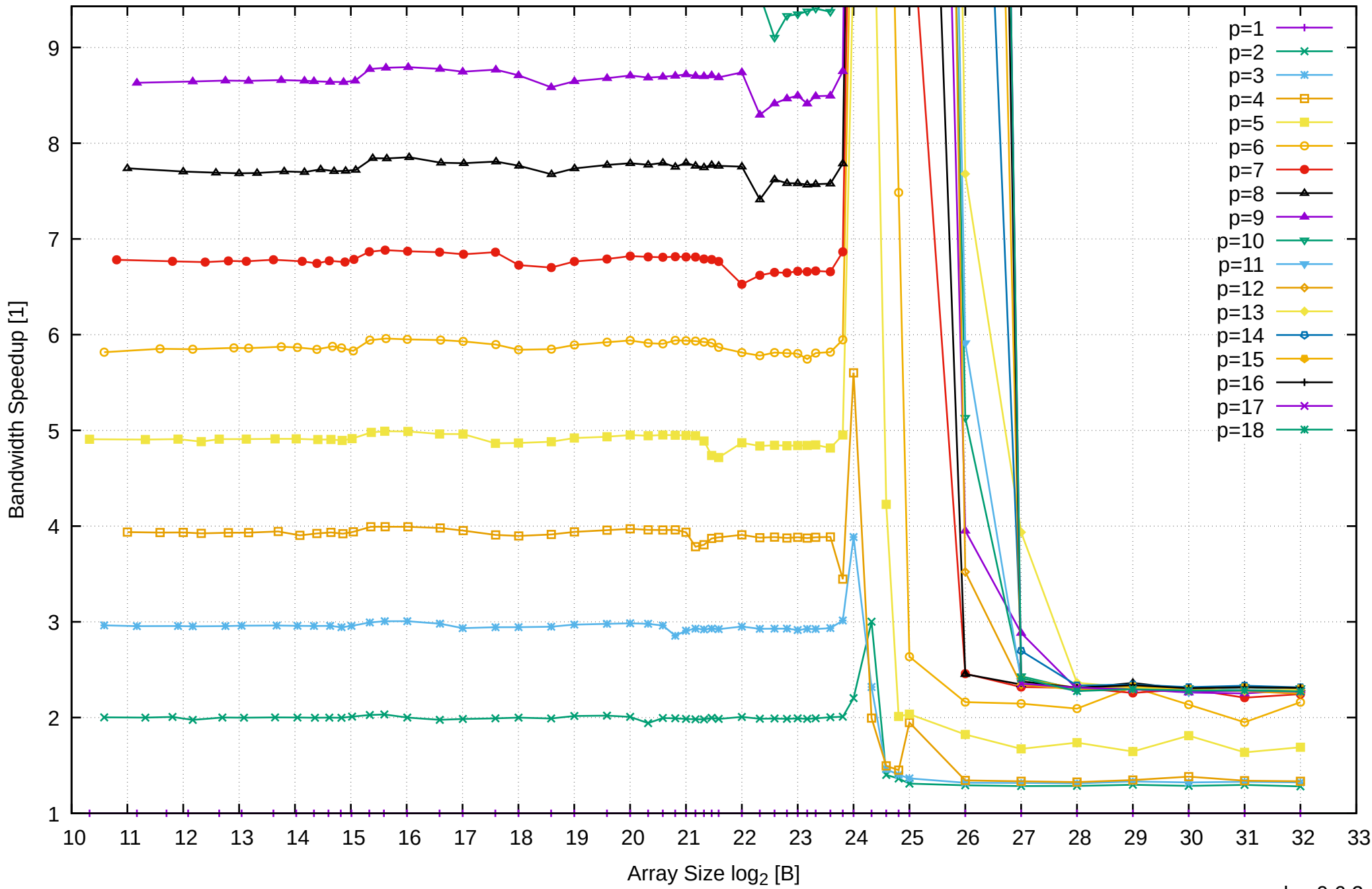
AMD Ryzen Threadripper 3955WX 128GB - Speedup of Parallel Memory Bandwidth (enlarged) - ScanWrite128PtrUnrollLoop
