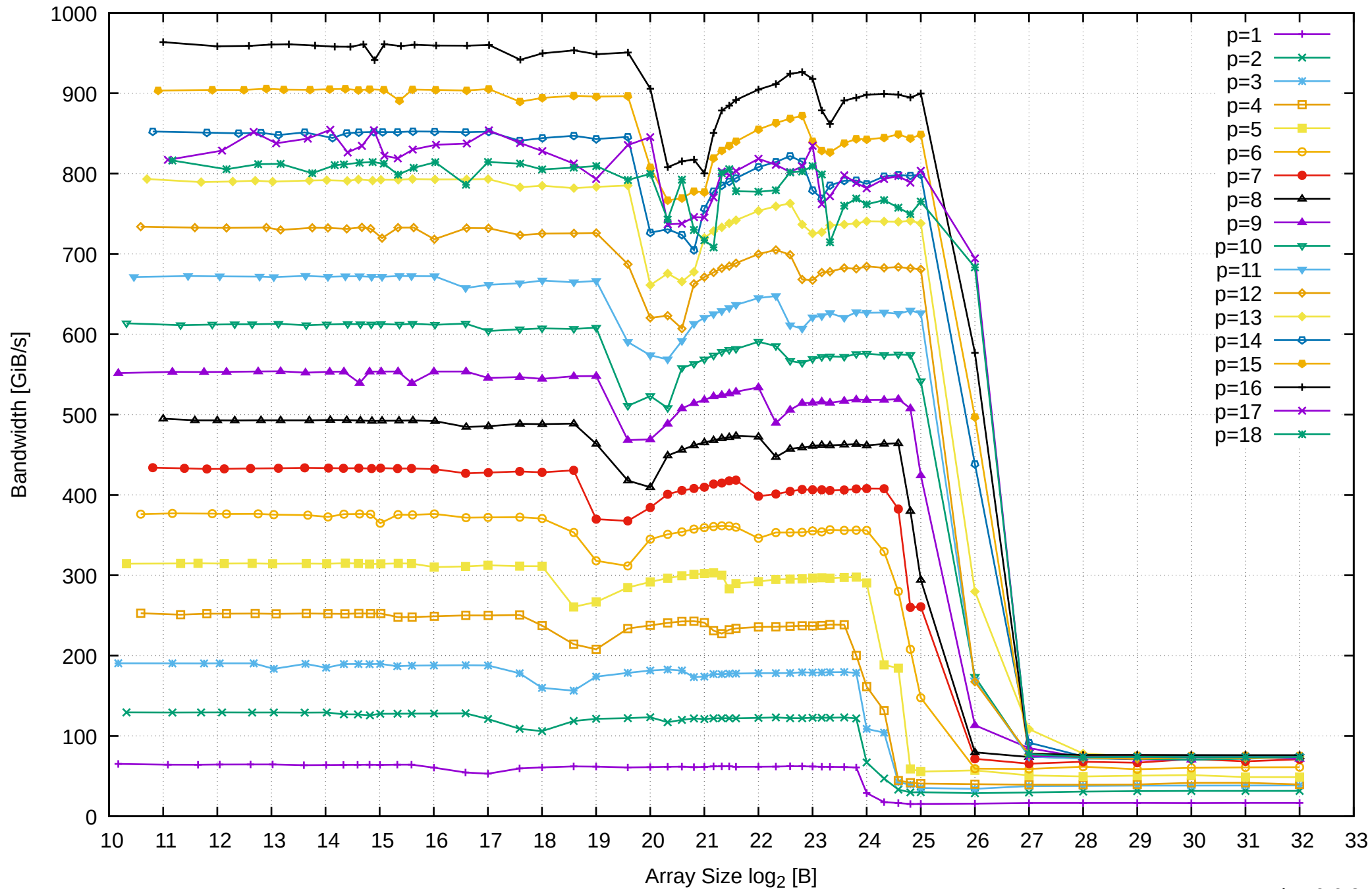
AMD Ryzen Threadripper 3955WX 128GB - Parallel Memory Bandwidth - ScanRead64IndexUnrollLoop
