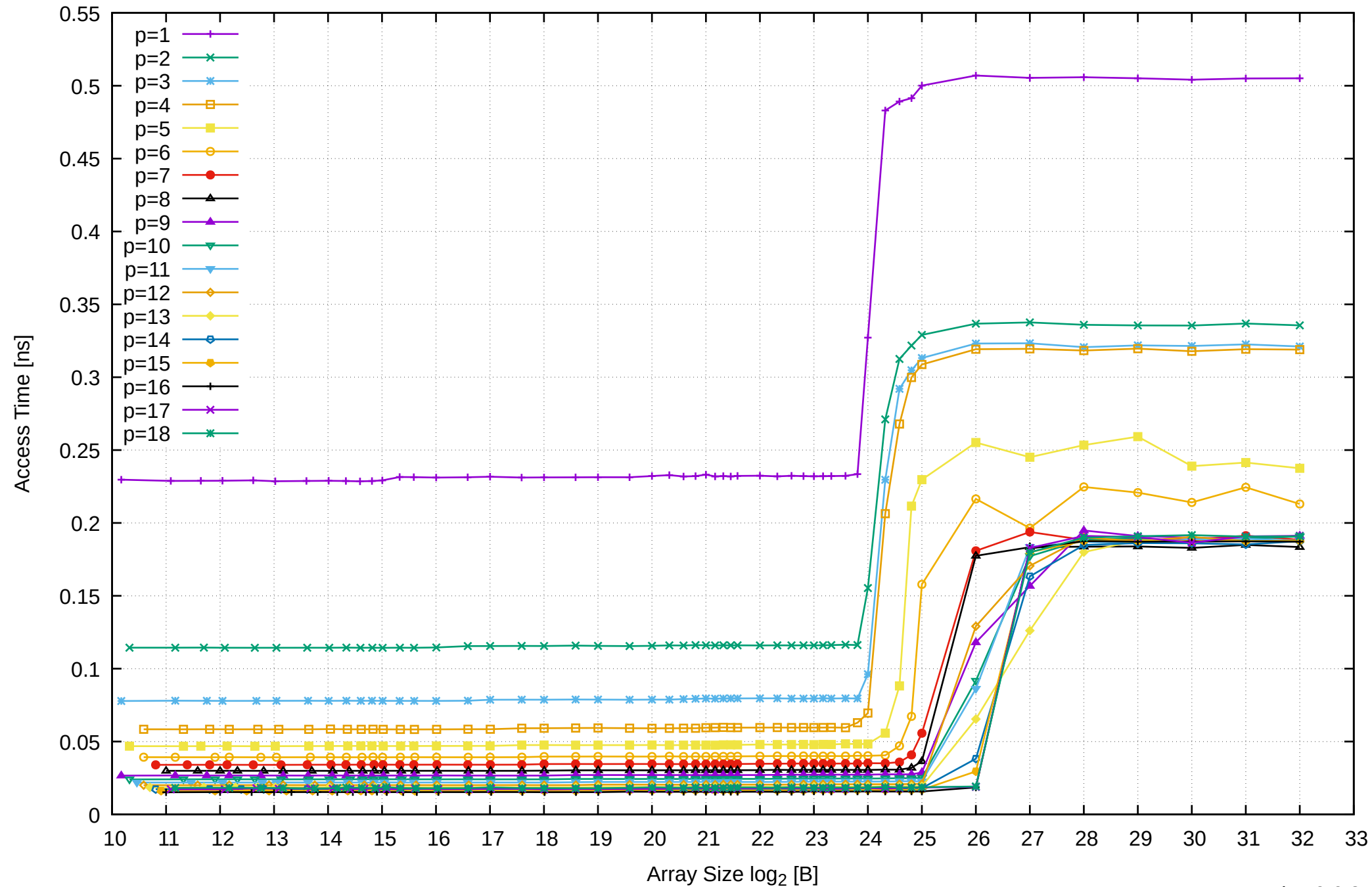
AMD Ryzen Threadripper 3955WX 128GB - Parallel Memory Access Time - ScanWrite64PtrUnrollLoop
