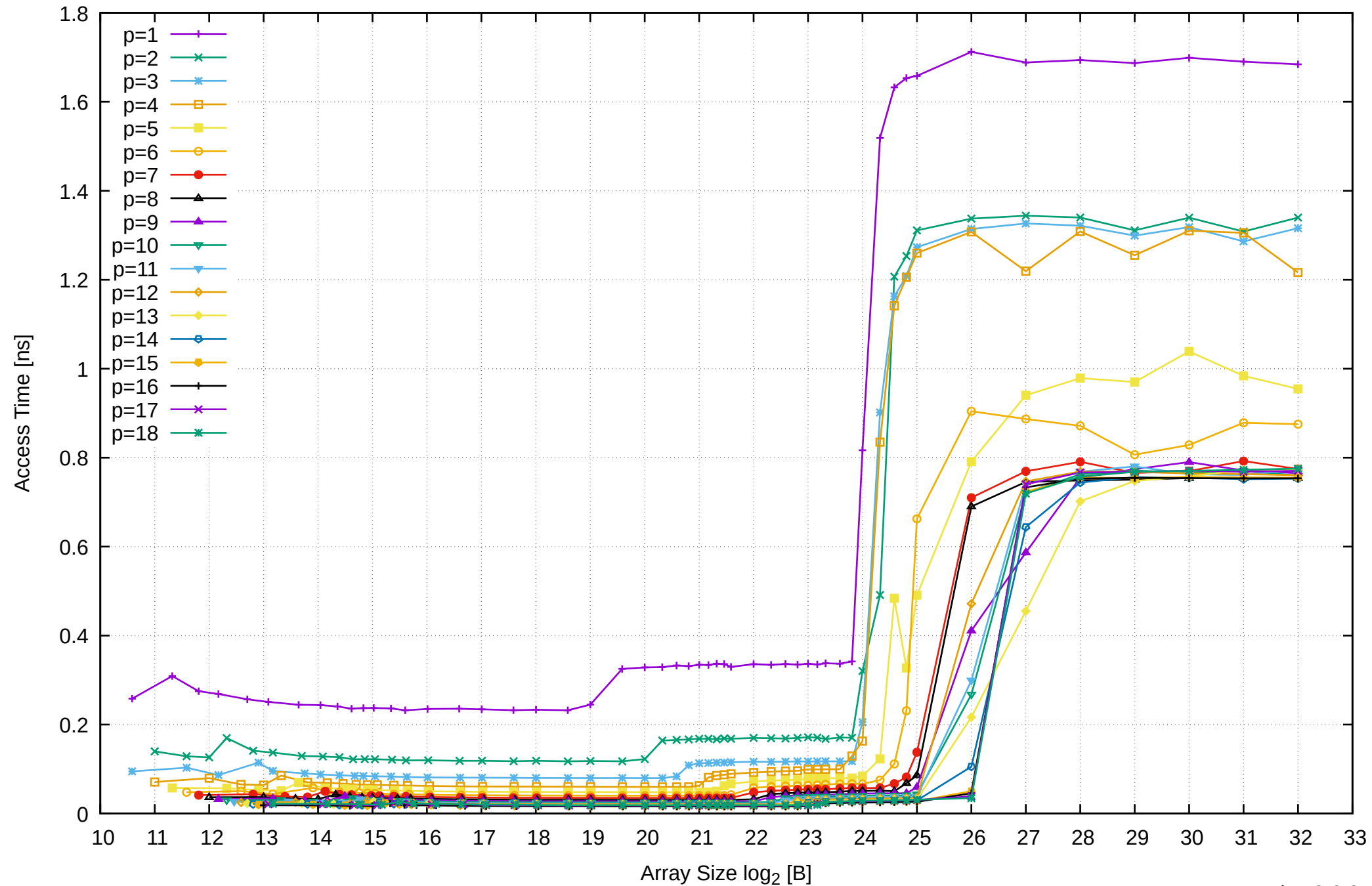
AMD Ryzen Threadripper 3955WX 128GB - Parallel Memory Access Time - ScanWrite256PtrSimpleLoop
