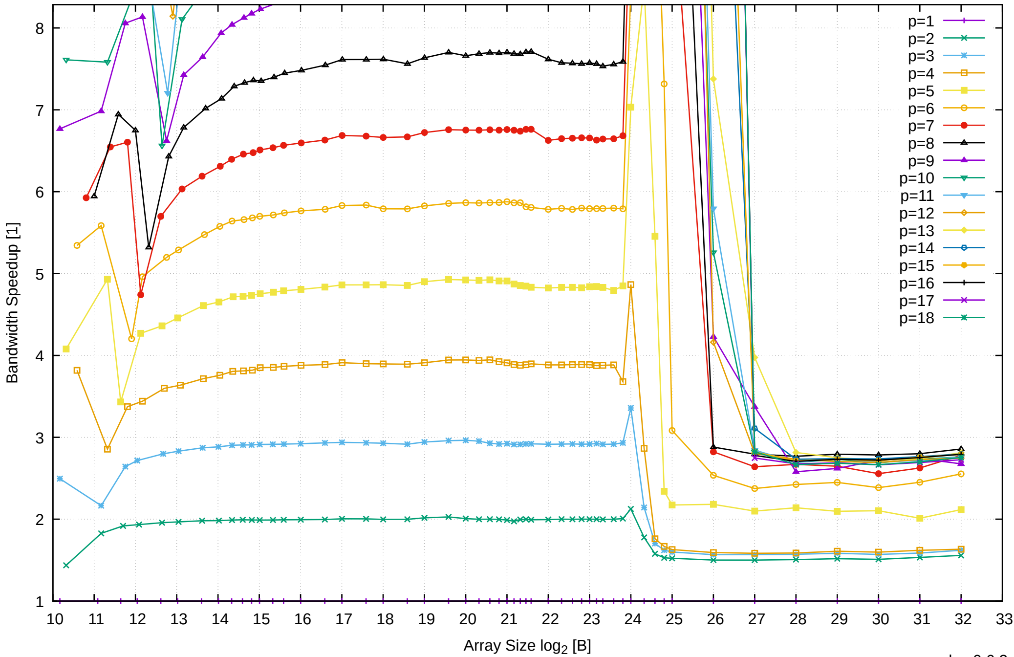
AMD Ryzen Threadripper 3955WX 128GB - Speedup of Parallel Memory Bandwidth (enlarged) - ScanWrite64PtrSimpleLoop
