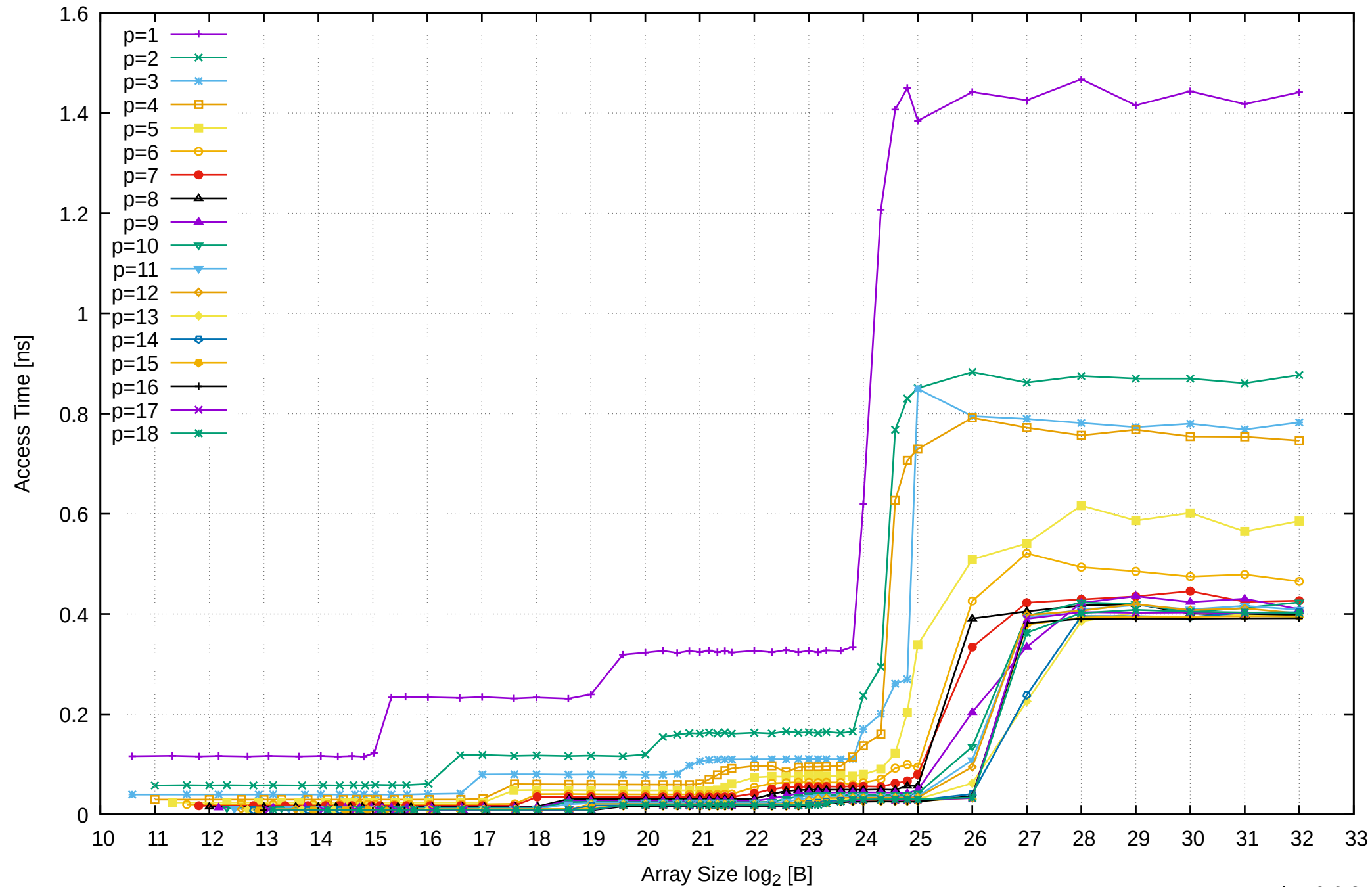
AMD Ryzen Threadripper 3955WX 128GB - Parallel Memory Access Time - ScanRead256PtrUnrollLoop
