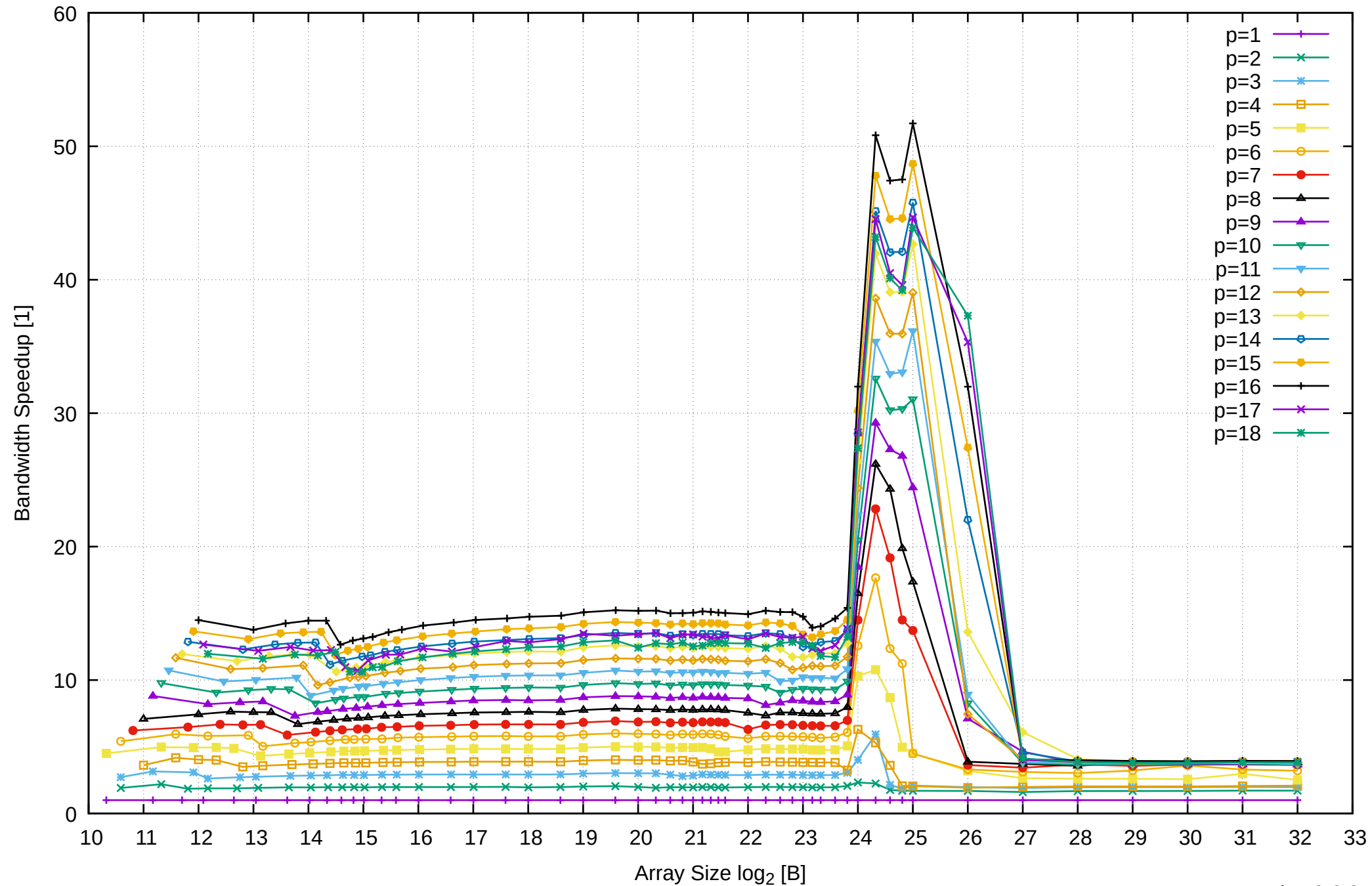
AMD Ryzen Threadripper 3955WX 128GB - Speedup of Parallel Memory Bandwidth - ScanRead128PtrSimpleLoop
