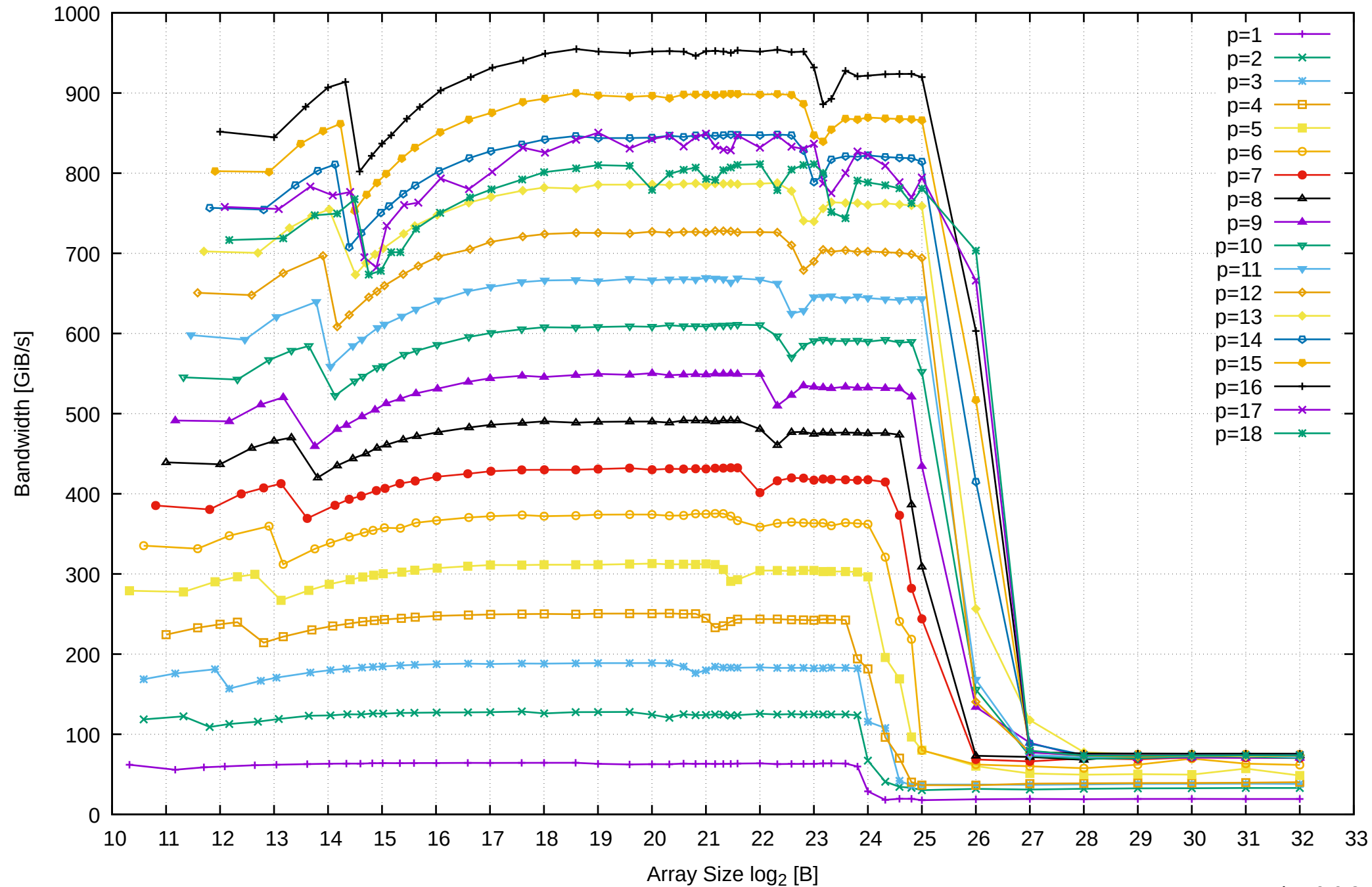
AMD Ryzen Threadripper 3955WX 128GB - Parallel Memory Bandwidth - ScanRead128PtrSimpleLoop
