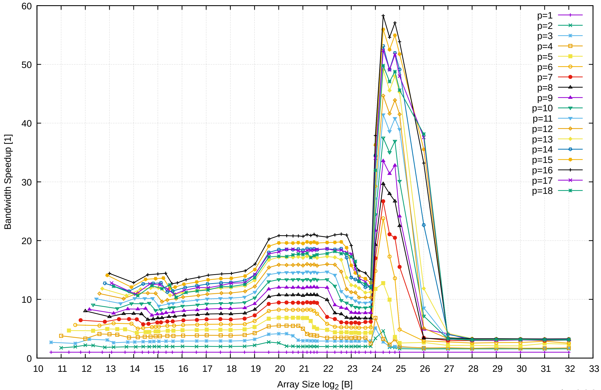
AMD Ryzen Threadripper 3955WX 128GB - Speedup of Parallel Memory Bandwidth - ScanRead256PtrSimpleLoop
