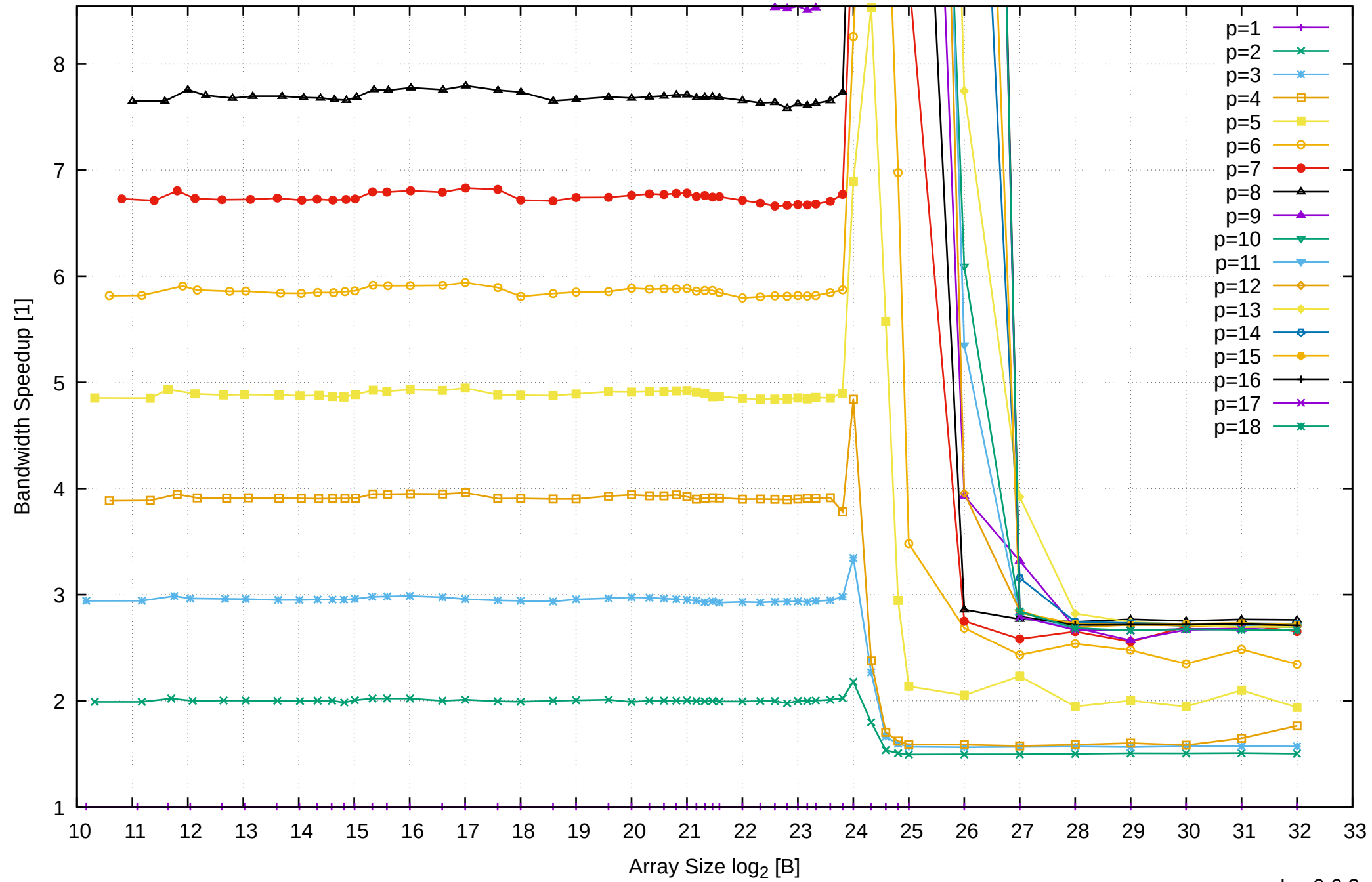
AMD Ryzen Threadripper 3955WX 128GB - Speedup of Parallel Memory Bandwidth (enlarged) - ScanWrite64IndexUnrollLoop
