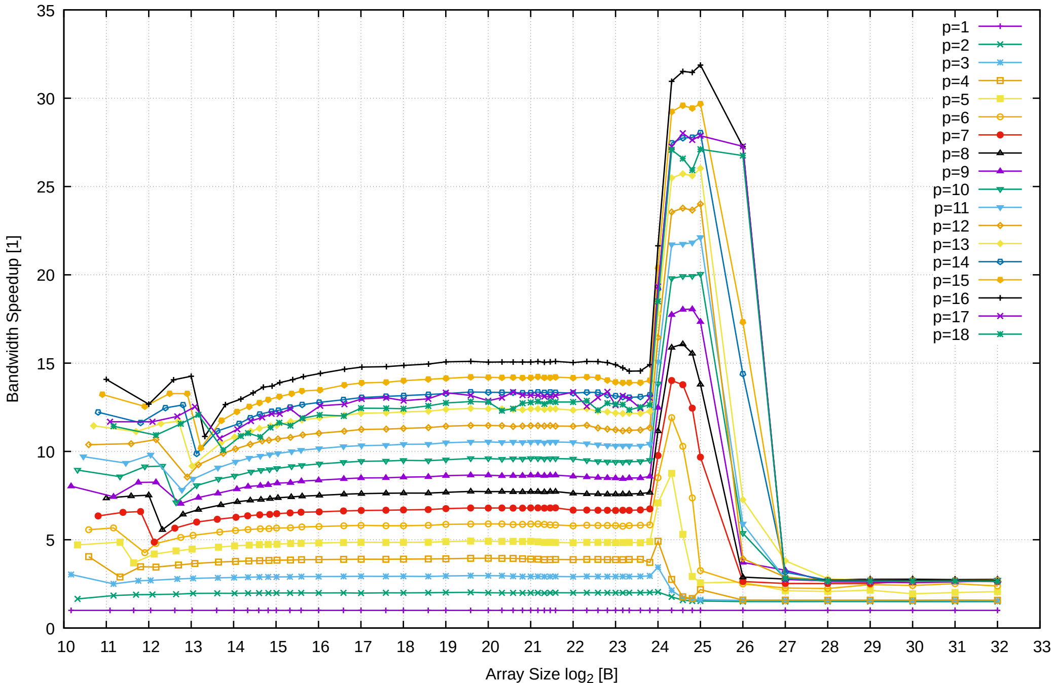
AMD Ryzen Threadripper 3955WX 128GB - Speedup of Parallel Memory Bandwidth - ScanWrite64IndexSimpleLoop
