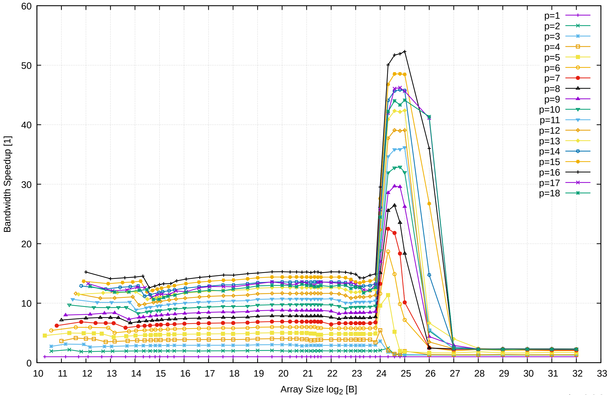
AMD Ryzen Threadripper 3955WX 128GB - Speedup of Parallel Memory Bandwidth - ScanWrite128PtrSimpleLoop
