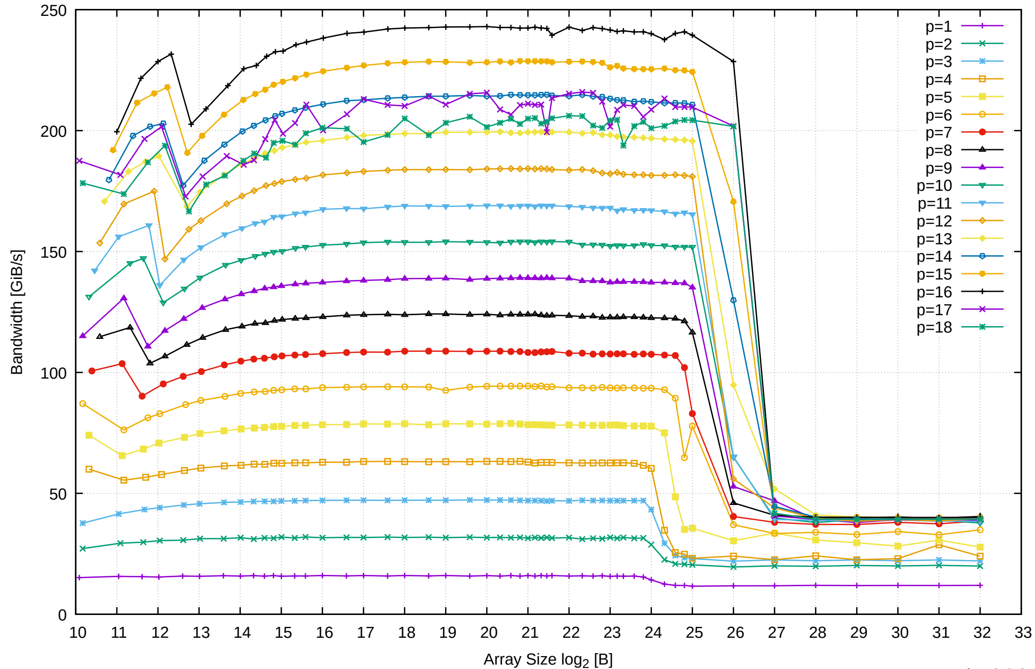
AMD Ryzen Threadripper 3955WX 128GB - Parallel Memory Bandwidth - ScanWrite32PtrSimpleLoop
