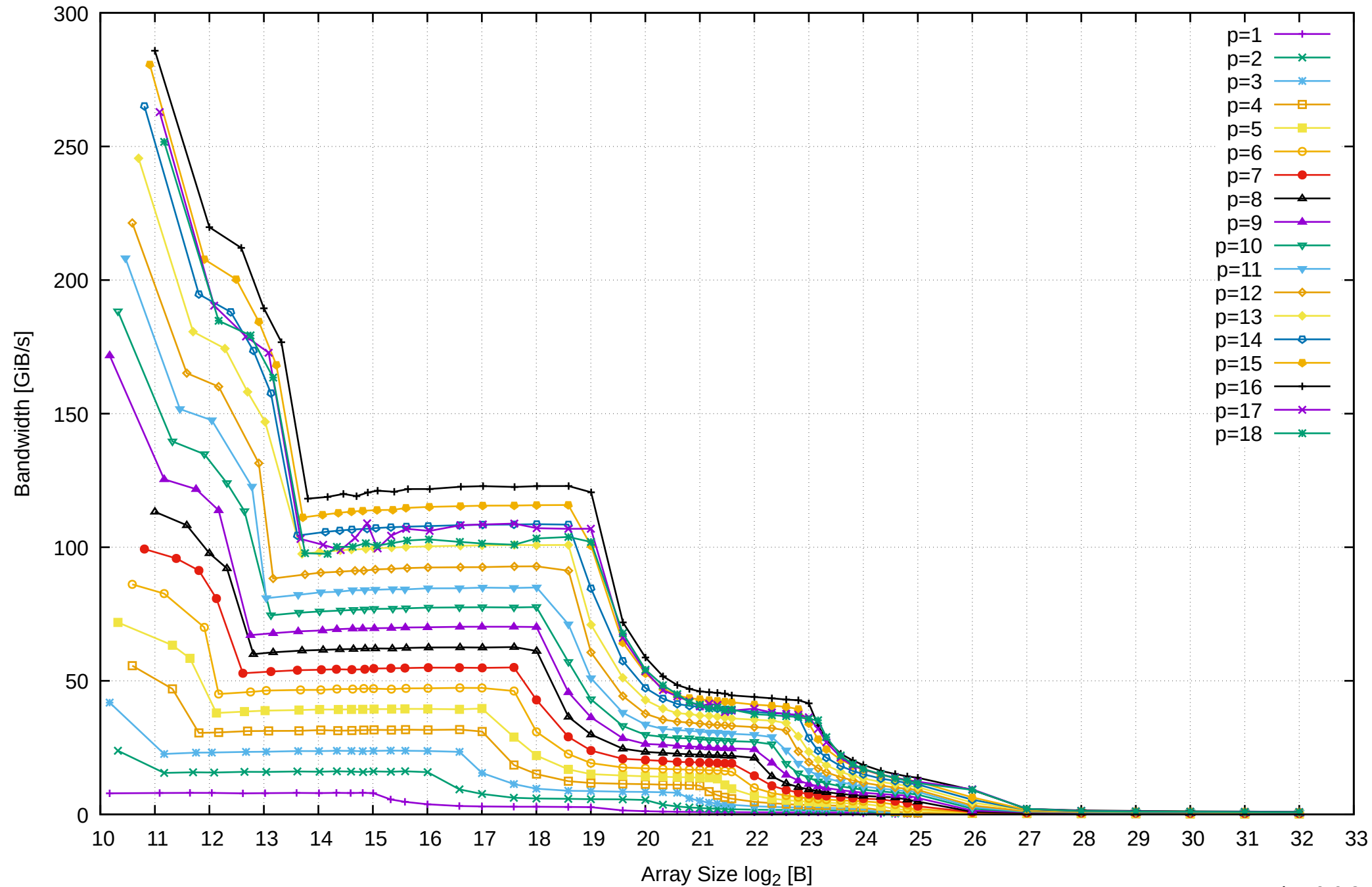
AMD Ryzen Threadripper 3955WX 128GB - Parallel Memory Bandwidth - PermRead64SimpleLoop
