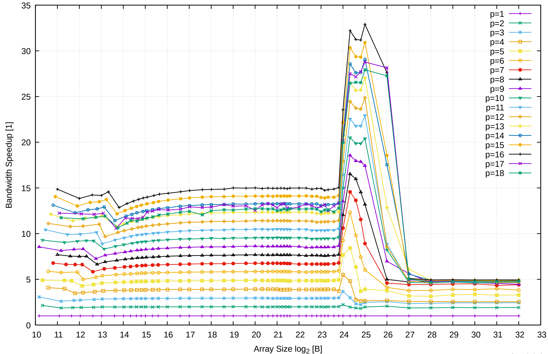
AMD Ryzen Threadripper 3955WX 128GB - Speedup of Parallel Memory Bandwidth - ScanRead64IndexSimpleLoop
