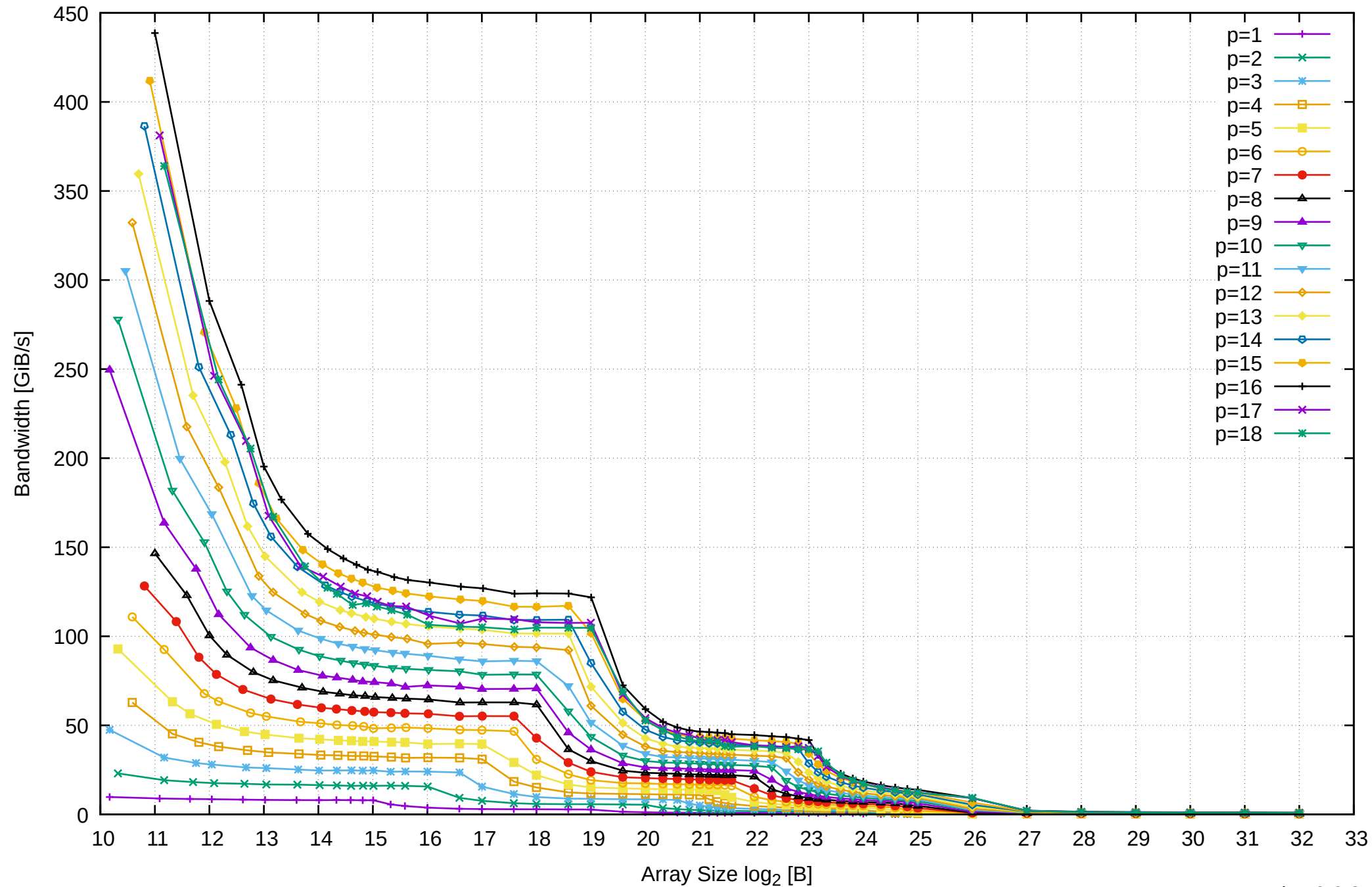
AMD Ryzen Threadripper 3955WX 128GB - Parallel Memory Bandwidth - PermRead64UnrollLoop
