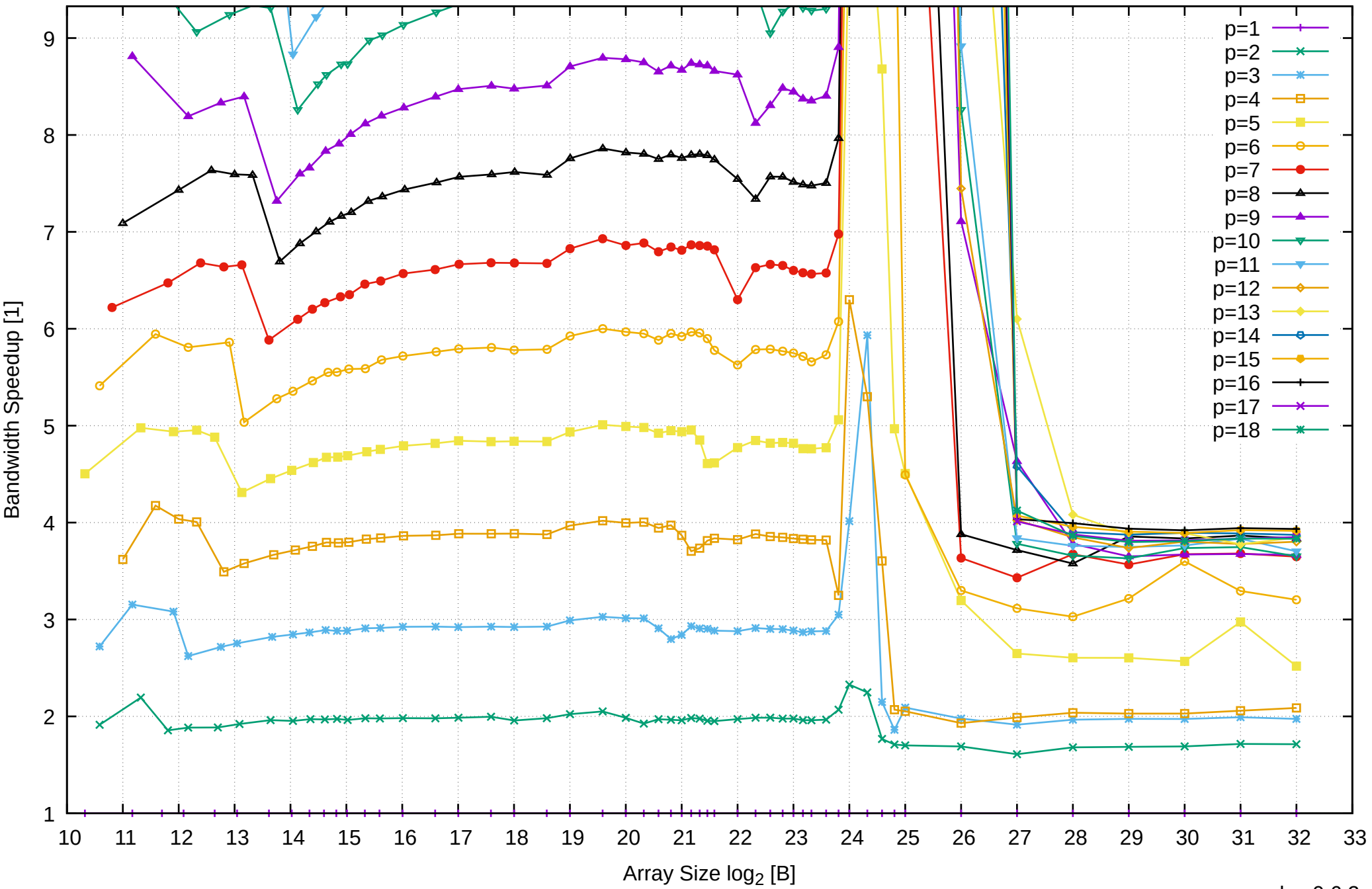
AMD Ryzen Threadripper 3955WX 128GB - Speedup of Parallel Memory Bandwidth (enlarged) - ScanRead128PtrSimpleLoop
