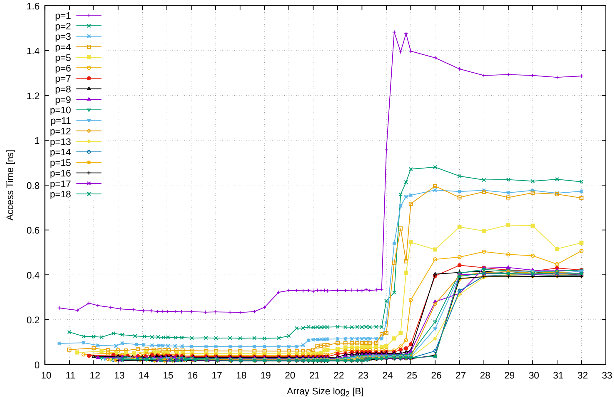
AMD Ryzen Threadripper 3955WX 128GB - Parallel Memory Access Time - ScanRead256PtrSimpleLoop
