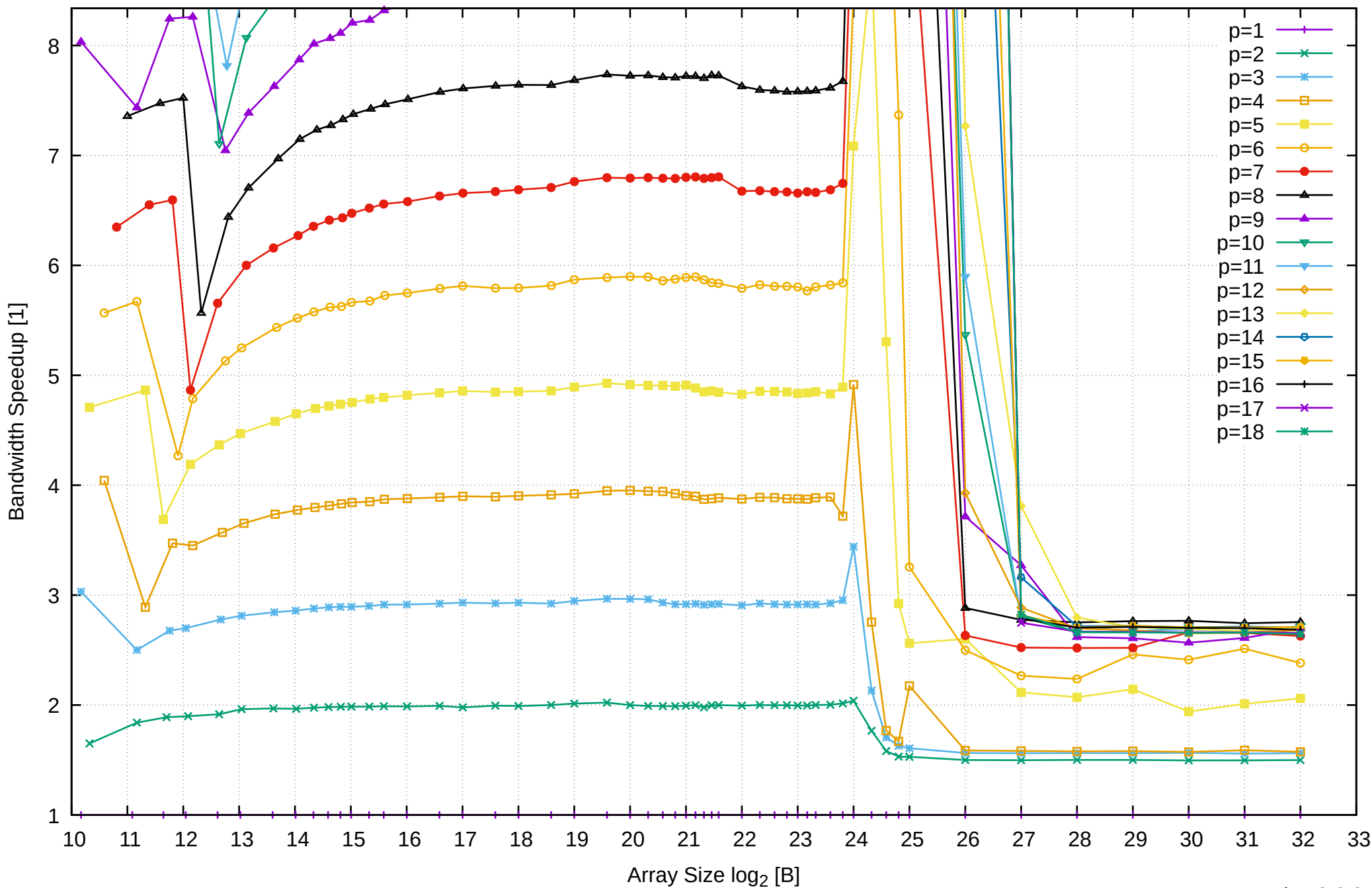
AMD Ryzen Threadripper 3955WX 128GB - Speedup of Parallel Memory Bandwidth (enlarged) - ScanWrite64IndexSimpleLoop
