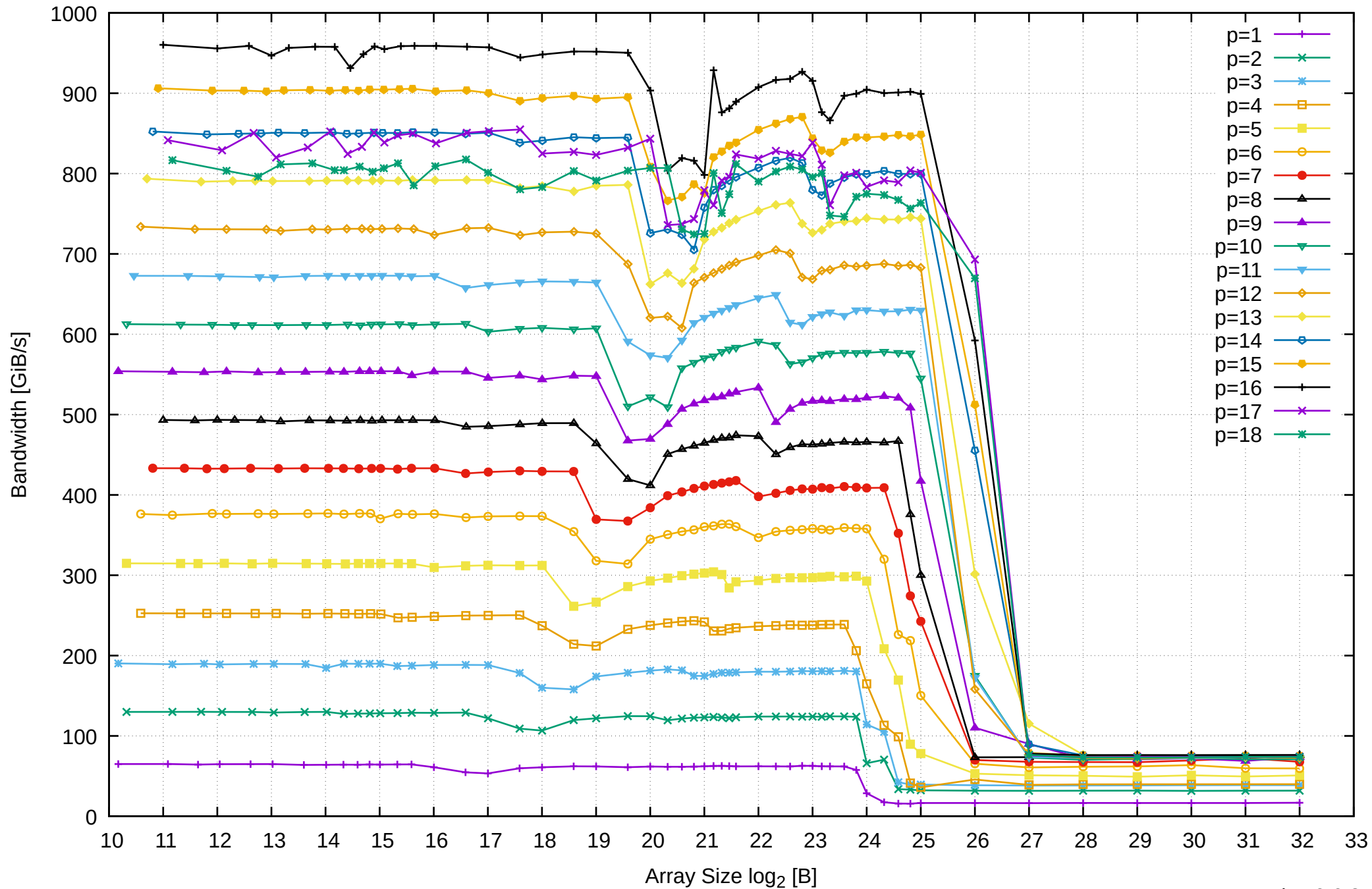
AMD Ryzen Threadripper 3955WX 128GB - Parallel Memory Bandwidth - ScanRead64PtrUnrollLoop
