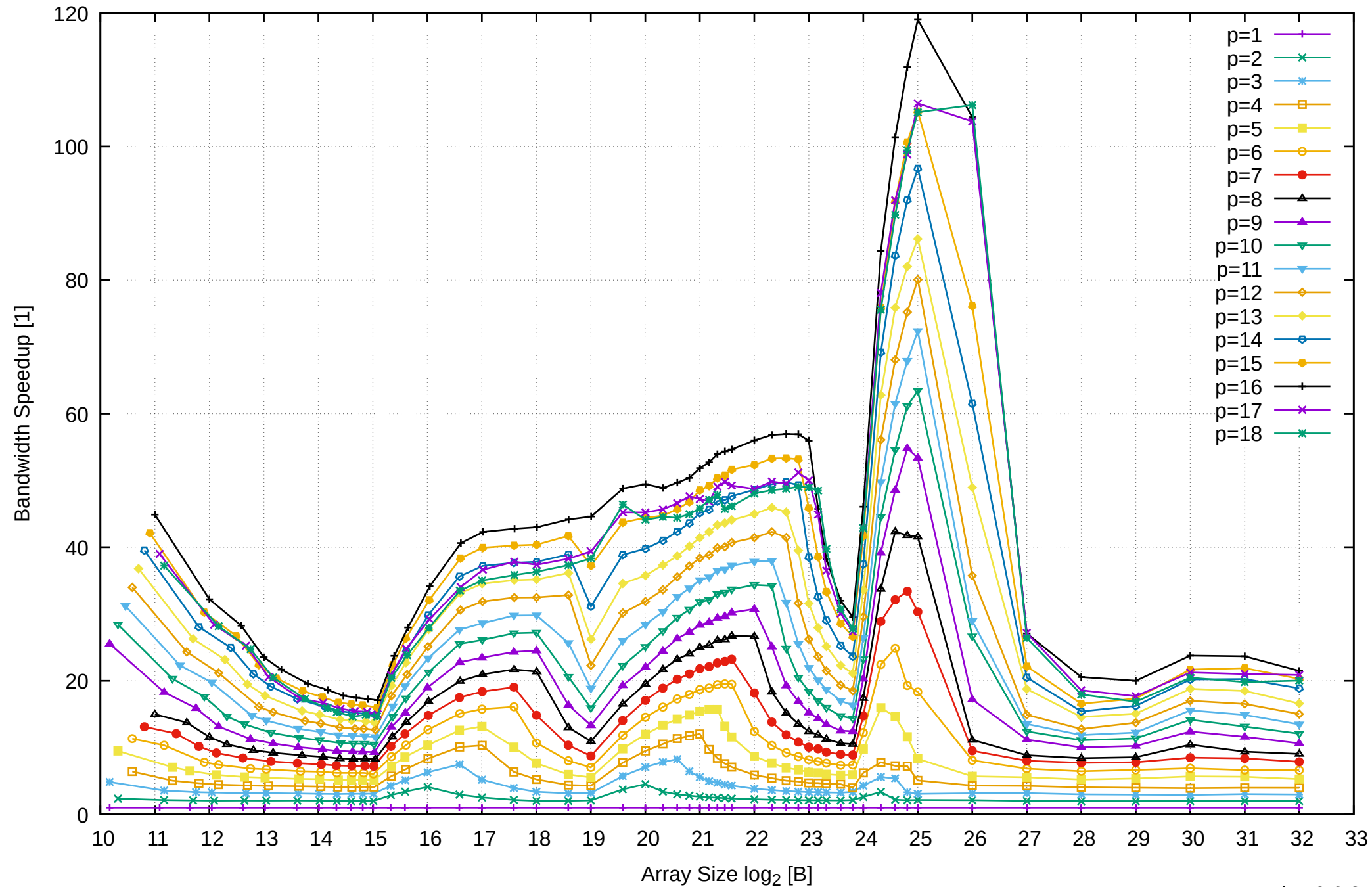
AMD Ryzen Threadripper 3955WX 128GB - Speedup of Parallel Memory Bandwidth - PermRead64UnrollLoop
