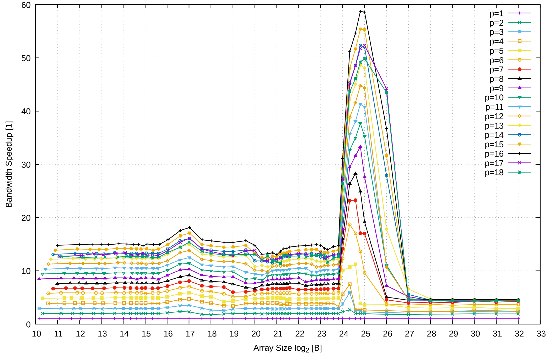
AMD Ryzen Threadripper 3955WX 128GB - Speedup of Parallel Memory Bandwidth - ScanRead64IndexUnrollLoop
