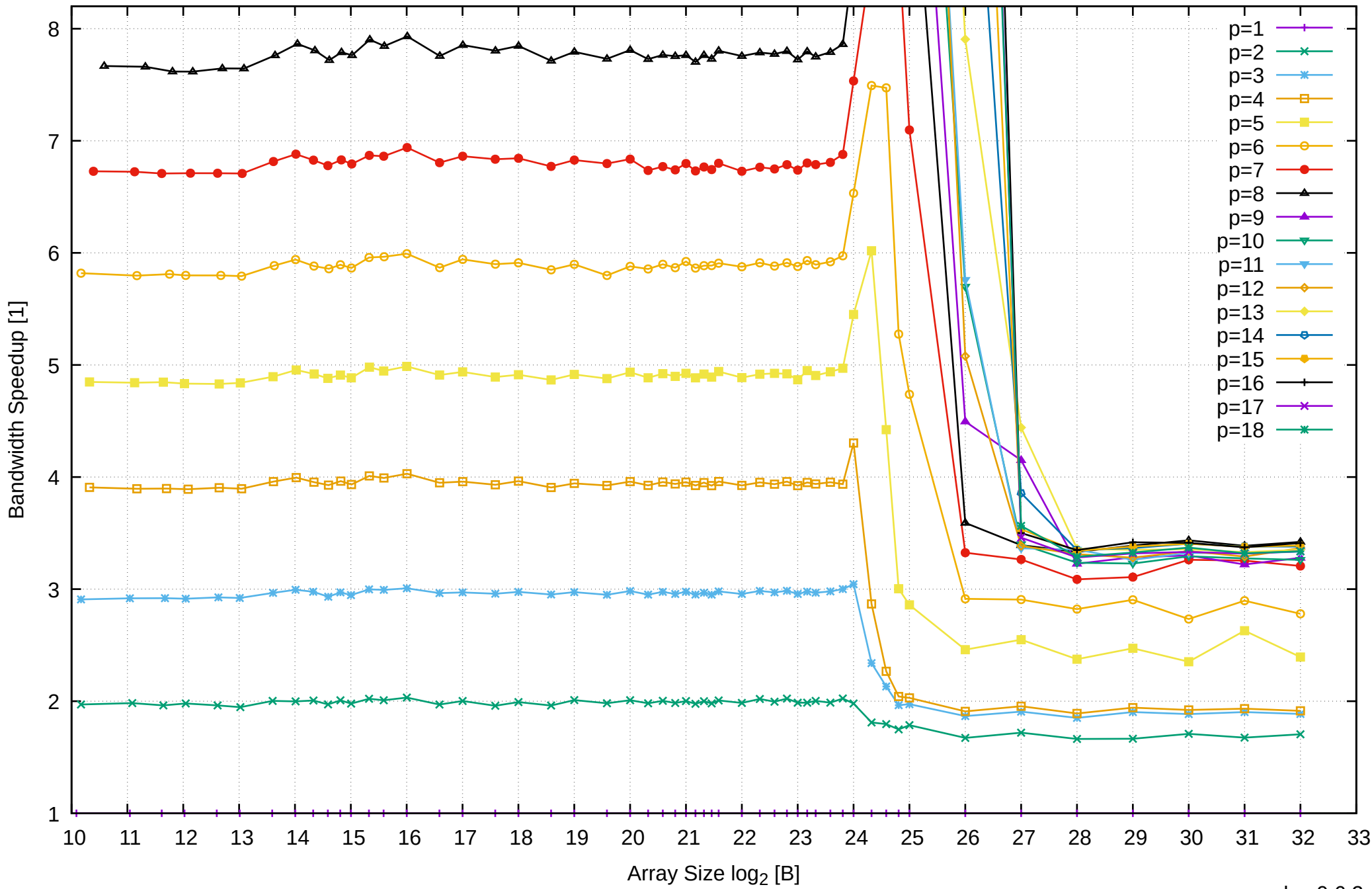
AMD Ryzen Threadripper 3955WX 128GB - Speedup of Parallel Memory Bandwidth (enlarged) - ScanWrite32PtrUnrollLoop
