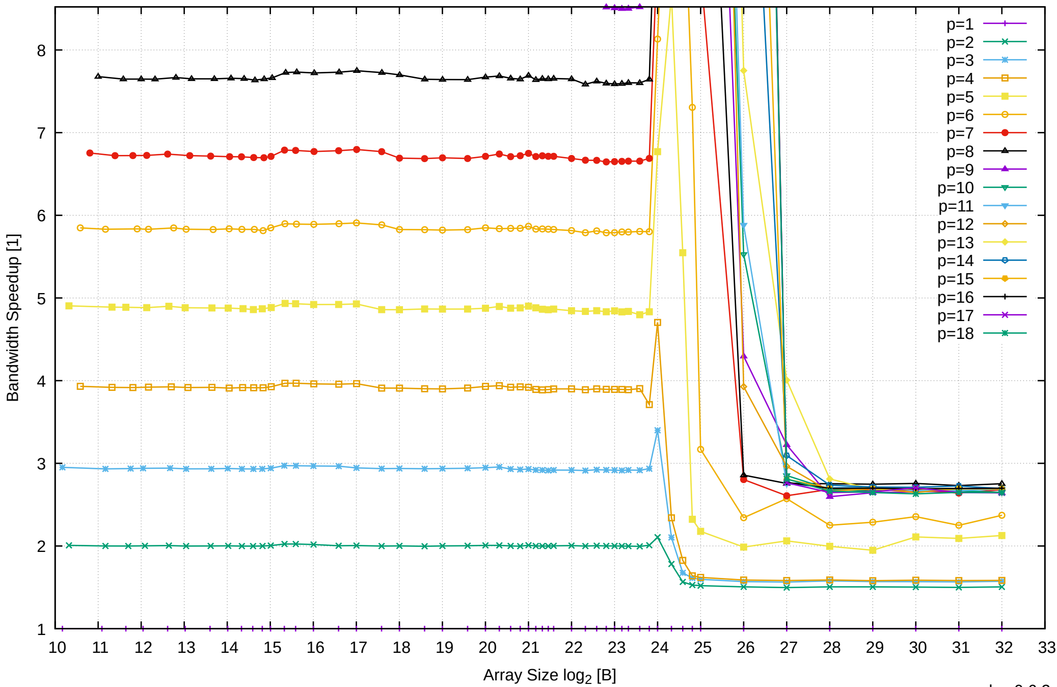
AMD Ryzen Threadripper 3955WX 128GB - Speedup of Parallel Memory Bandwidth (enlarged) - ScanWrite64PtrUnrollLoop
