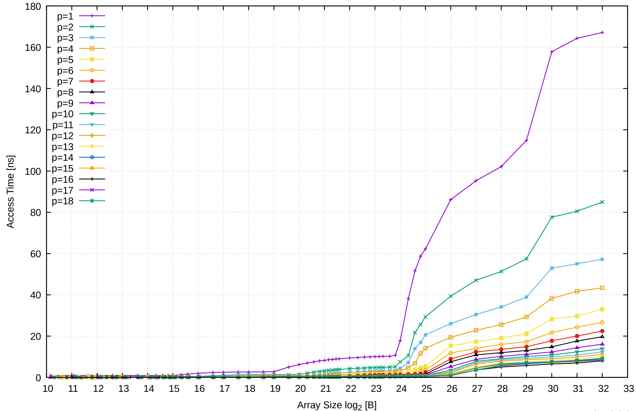
AMD Ryzen Threadripper 3955WX 128GB - Parallel Memory Access Time - PermRead64SimpleLoop
