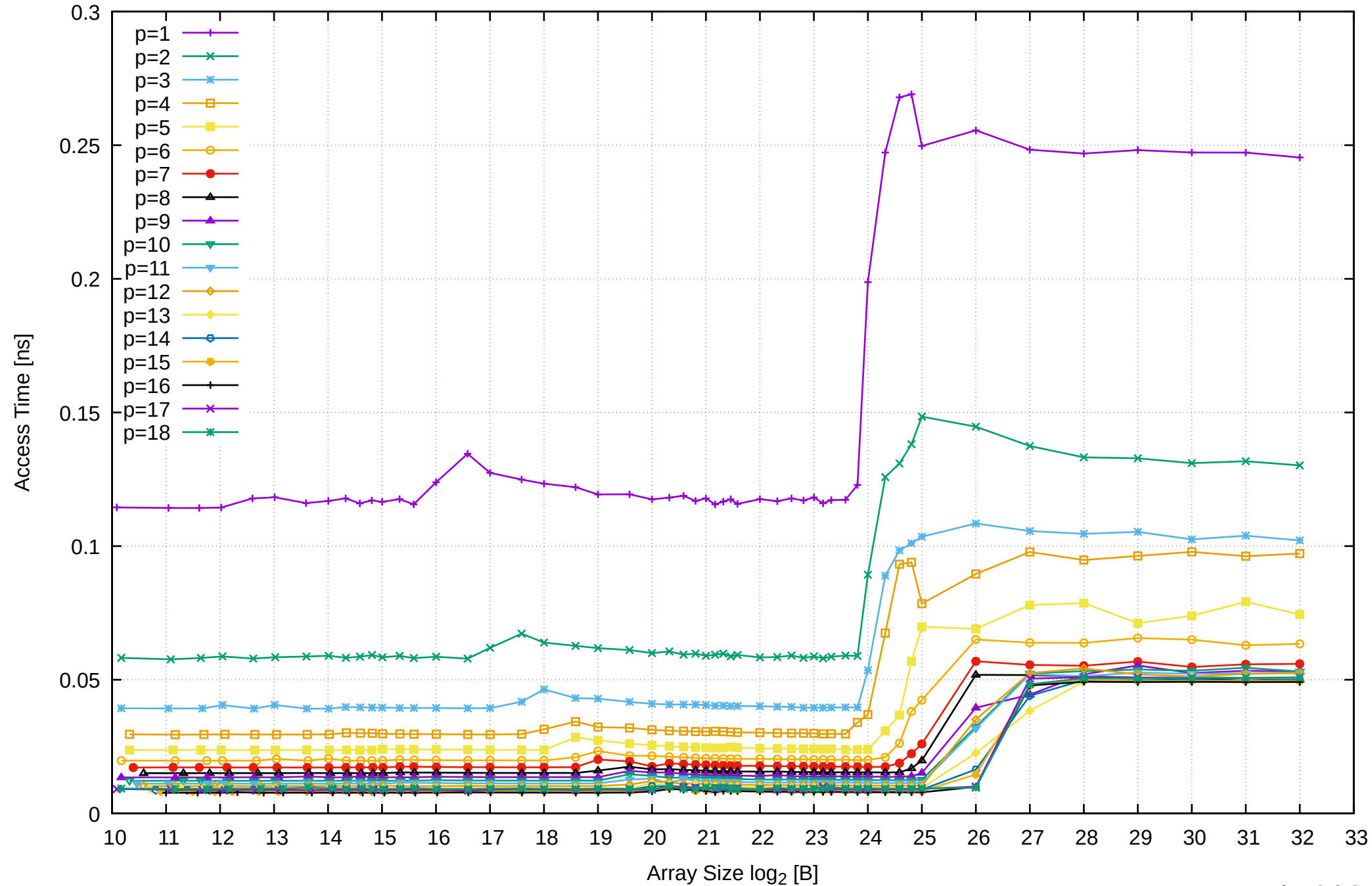
AMD Ryzen Threadripper 3955WX 128GB - Parallel Memory Access Time - ScanRead32PtrUnrollLoop
