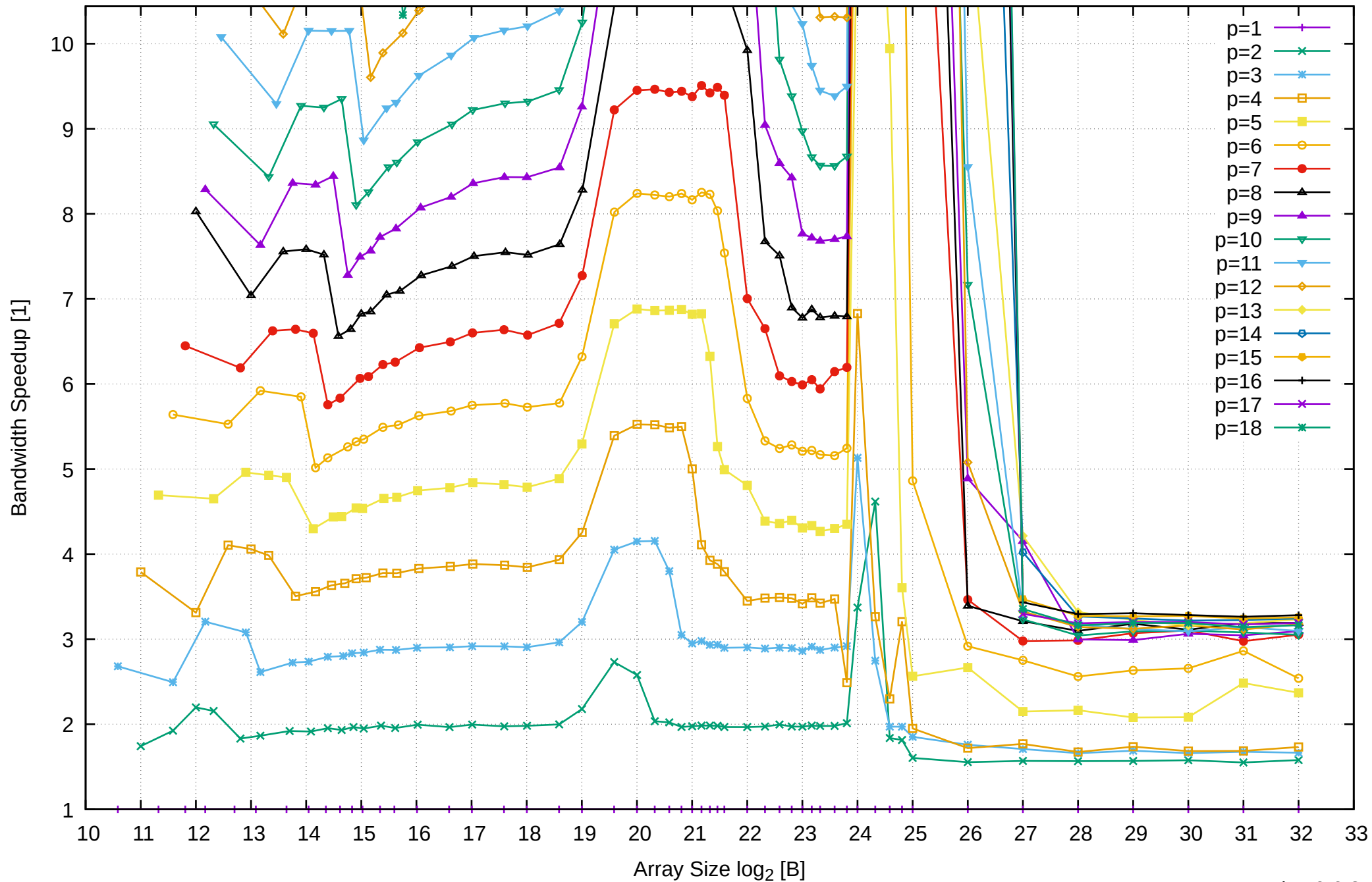
AMD Ryzen Threadripper 3955WX 128GB - Speedup of Parallel Memory Bandwidth (enlarged) - ScanRead256PtrSimpleLoop
