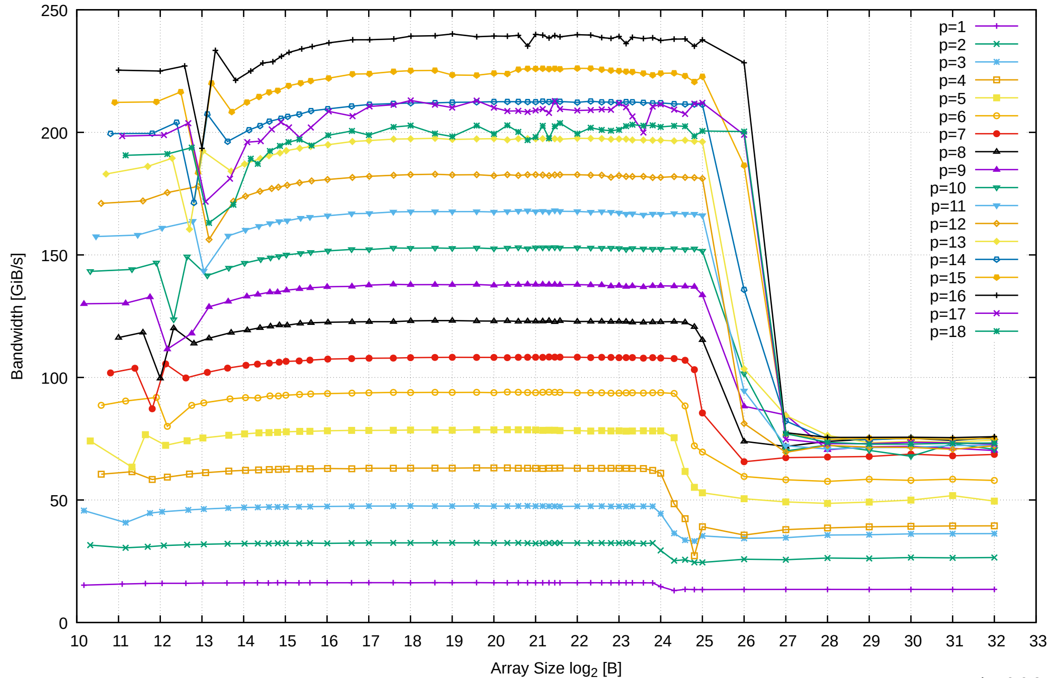
AMD Ryzen Threadripper 3955WX 128GB - Parallel Memory Bandwidth - ScanRead64PtrSimpleLoop
