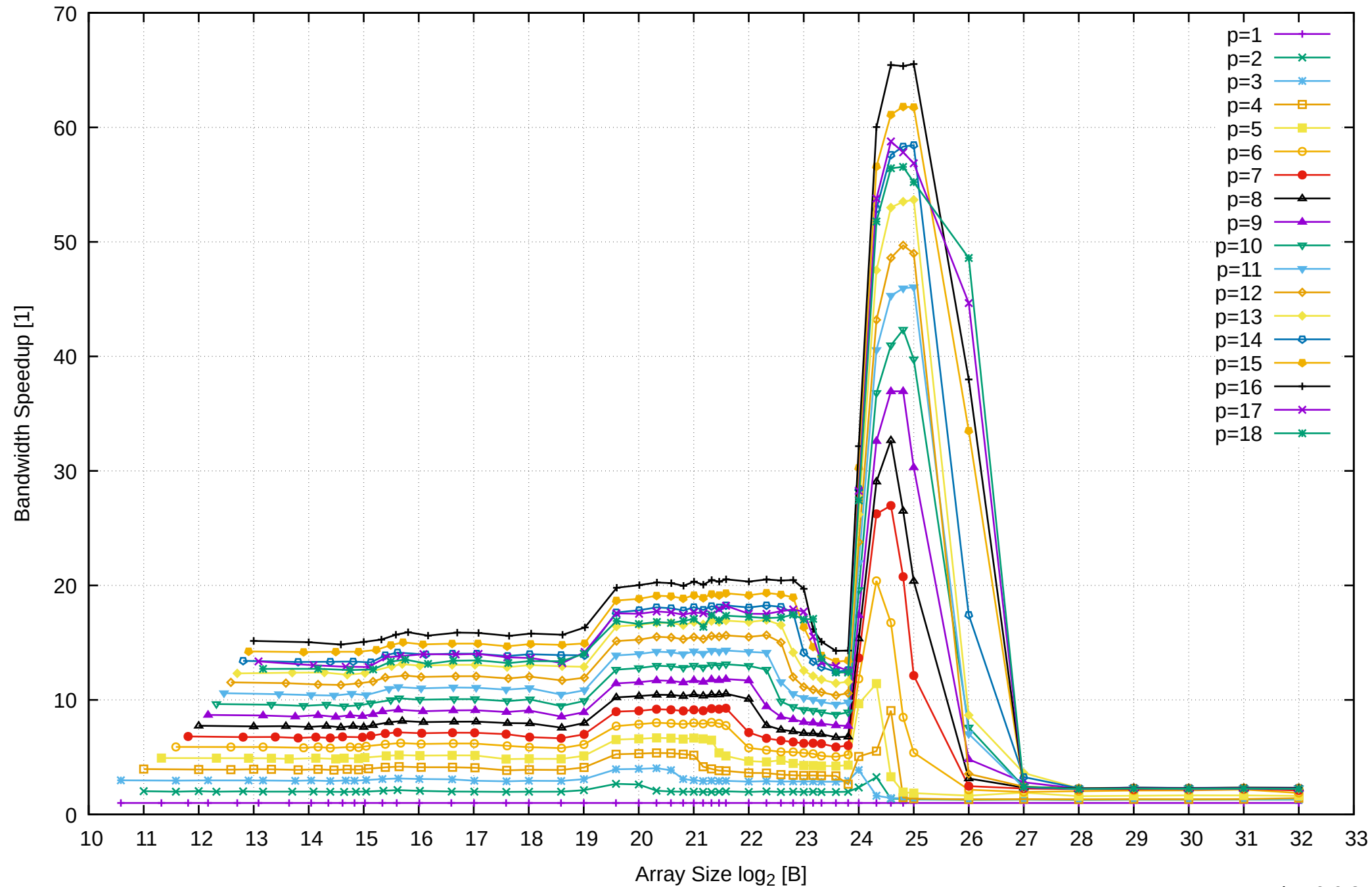
AMD Ryzen Threadripper 3955WX 128GB - Speedup of Parallel Memory Bandwidth - ScanWrite256PtrUnrollLoop
