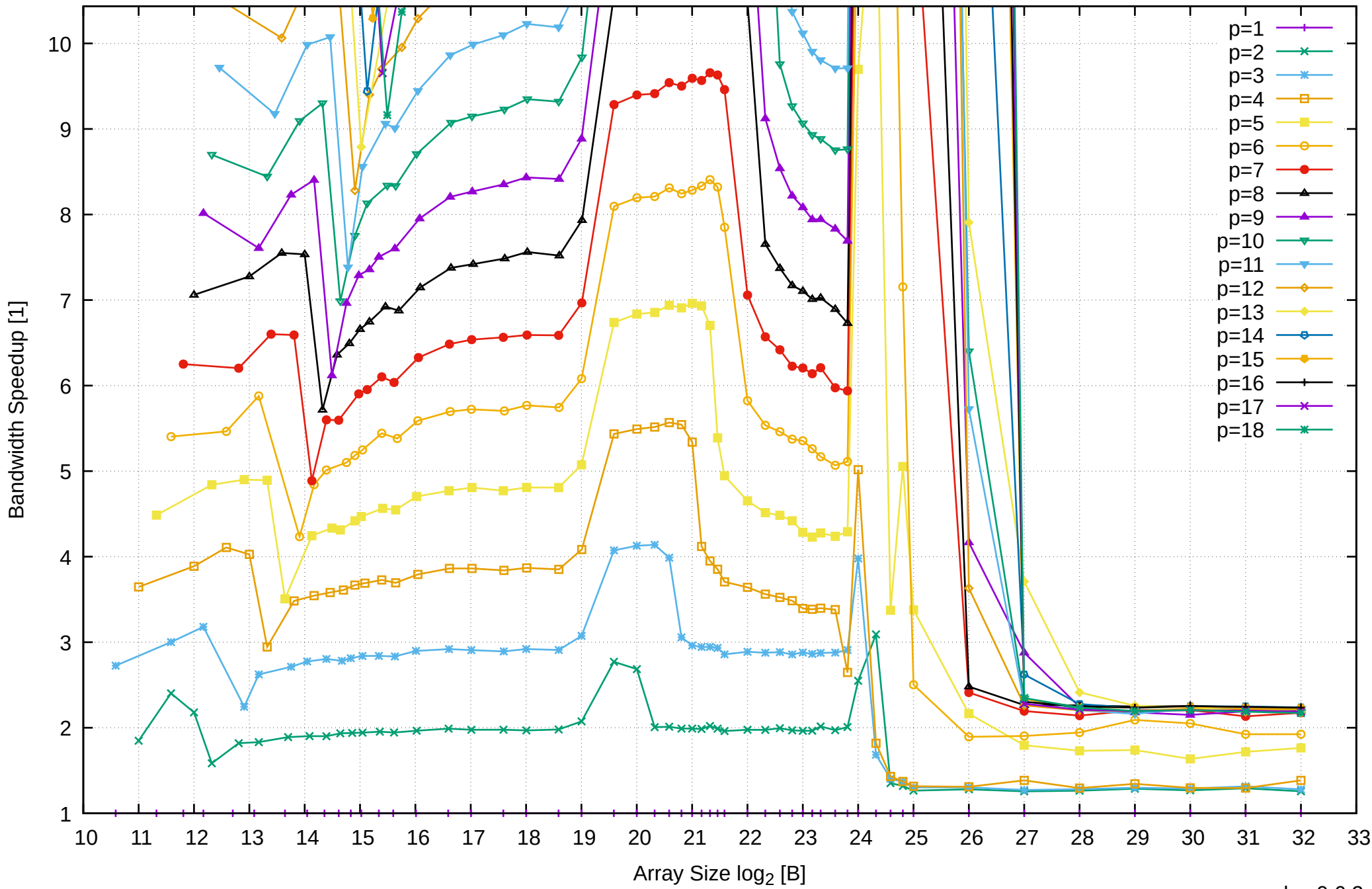
AMD Ryzen Threadripper 3955WX 128GB - Speedup of Parallel Memory Bandwidth (enlarged) - ScanWrite256PtrSimpleLoop
