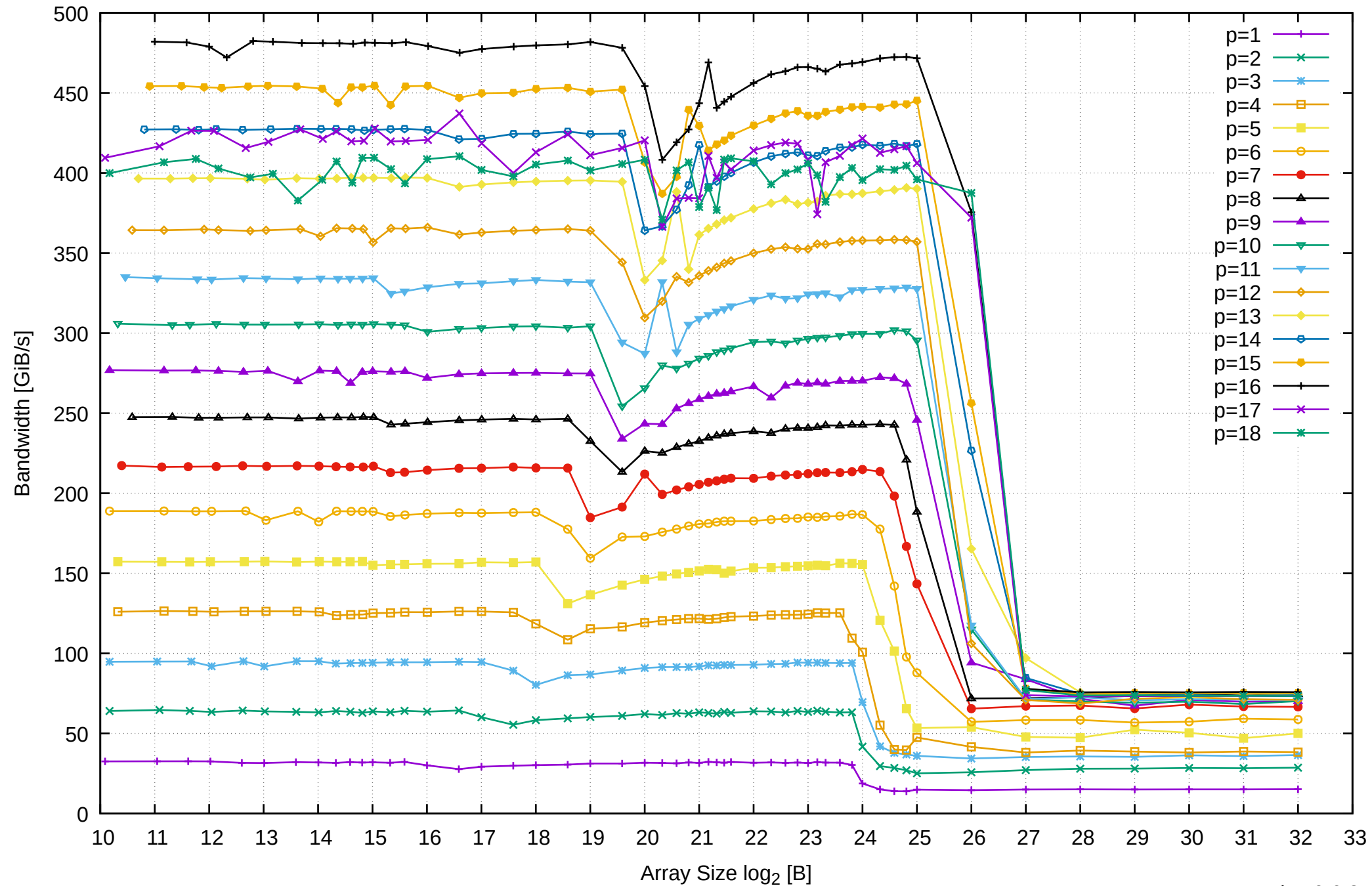
AMD Ryzen Threadripper 3955WX 128GB - Parallel Memory Bandwidth - ScanRead32PtrUnrollLoop
