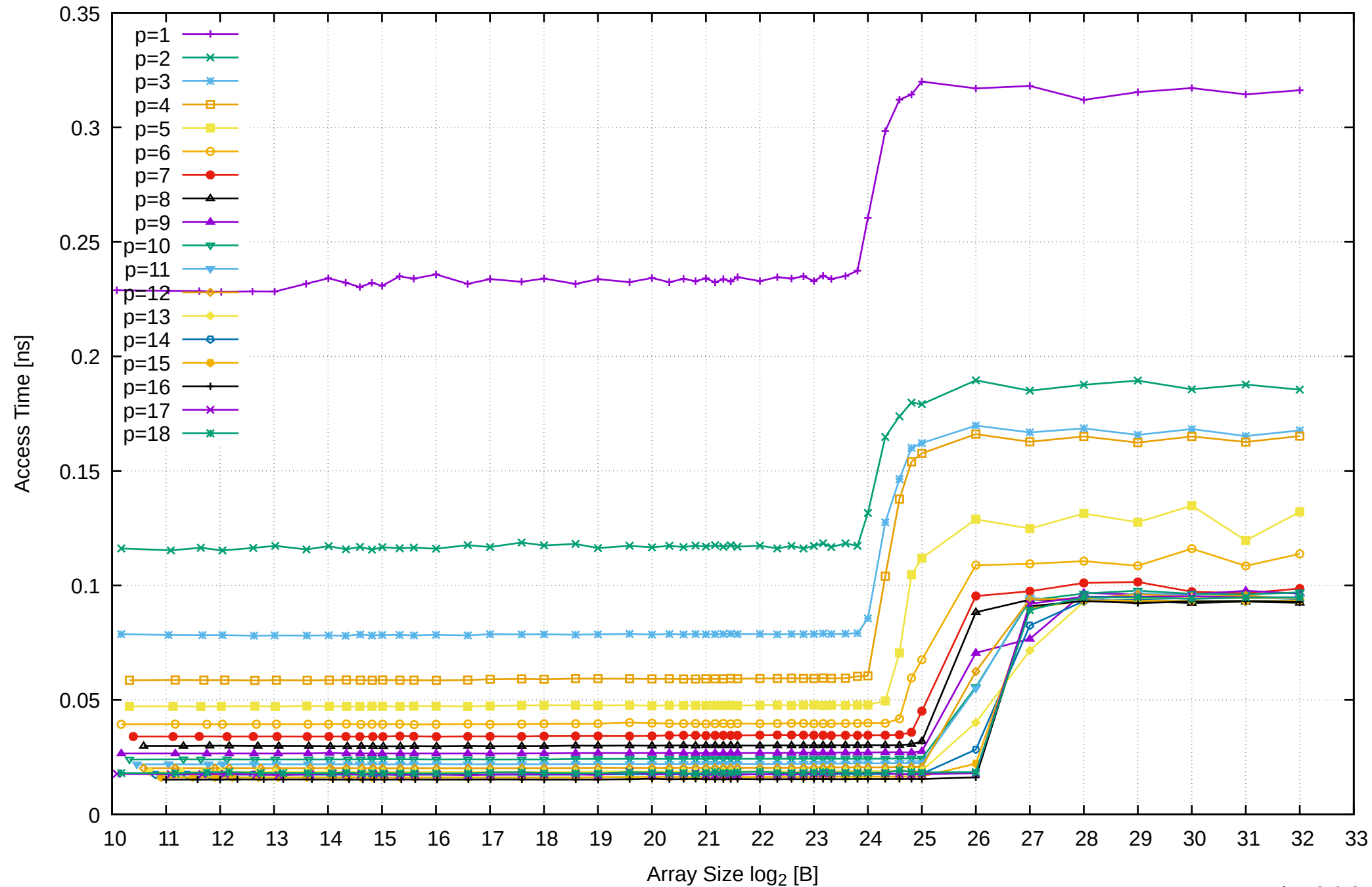
AMD Ryzen Threadripper 3955WX 128GB - Parallel Memory Access Time - ScanWrite32PtrUnrollLoop
