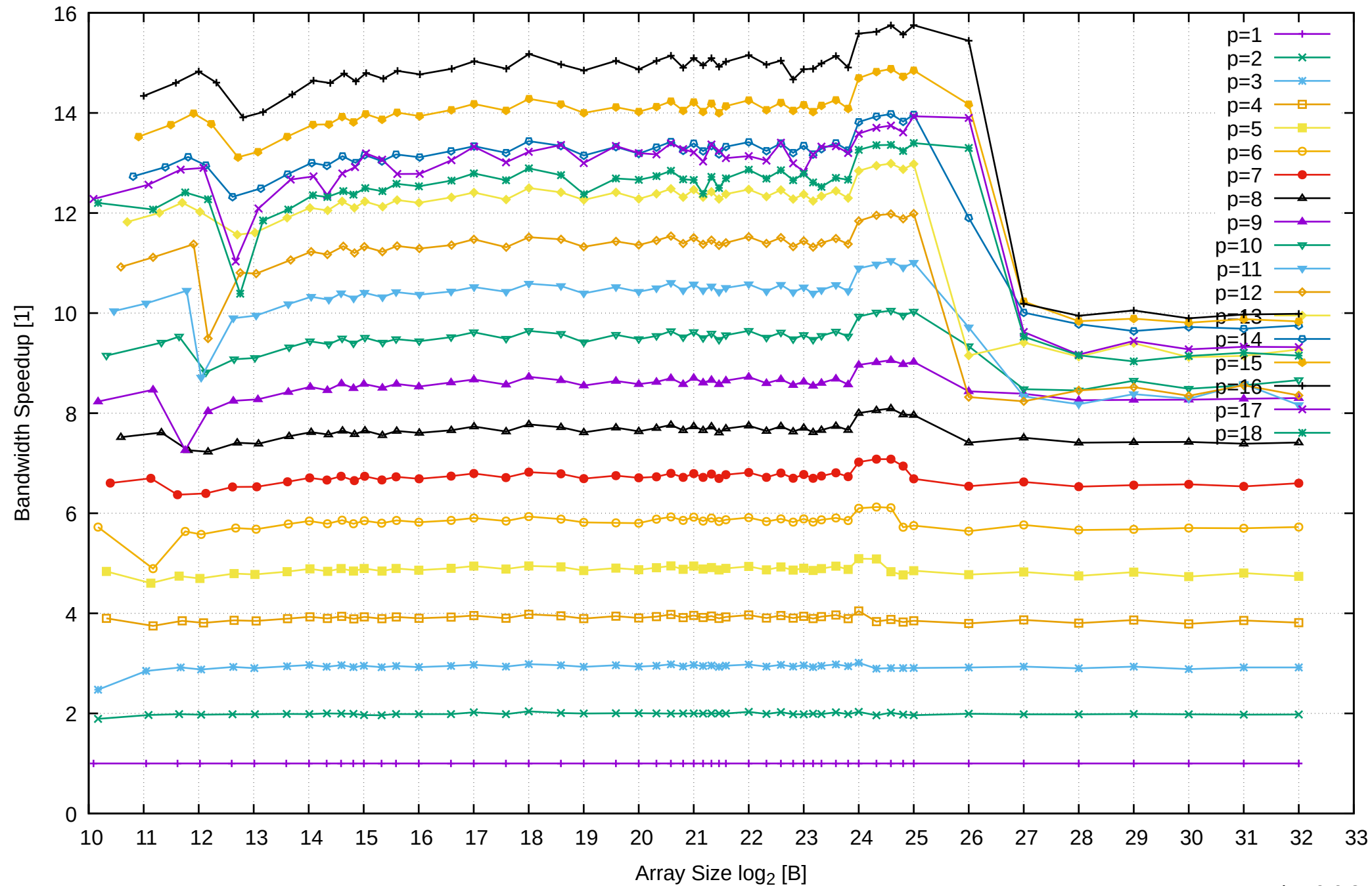
AMD Ryzen Threadripper 3955WX 128GB - Speedup of Parallel Memory Bandwidth - ScanRead32PtrSimpleLoop
