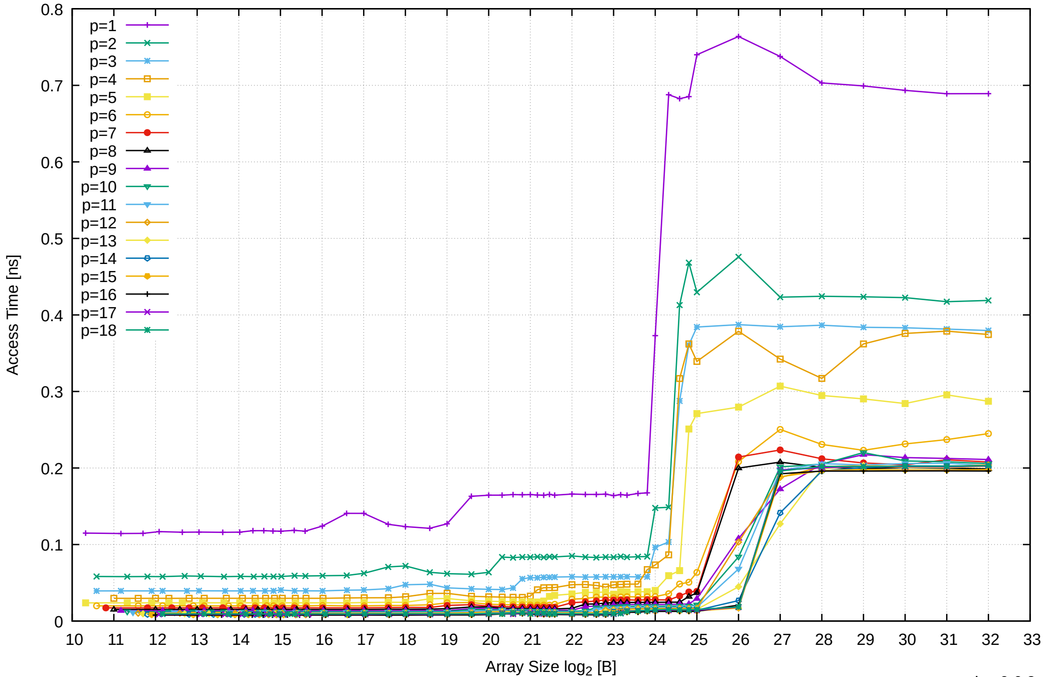
AMD Ryzen Threadripper 3955WX 128GB - Parallel Memory Access Time - ScanRead128PtrUnrollLoop
