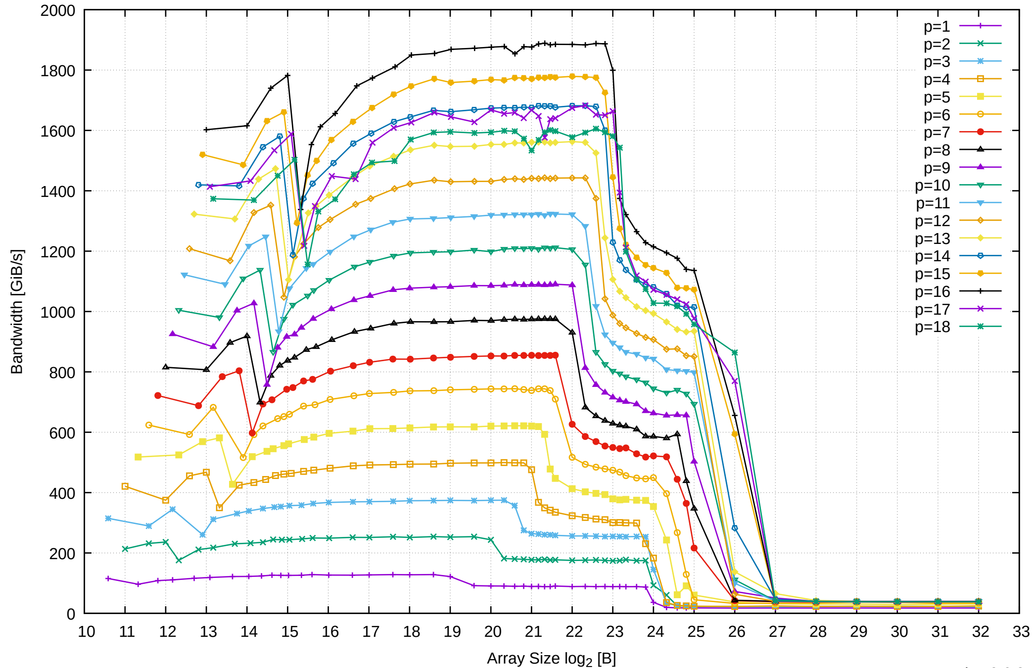
AMD Ryzen Threadripper 3955WX 128GB - Parallel Memory Bandwidth - ScanWrite256PtrSimpleLoop
