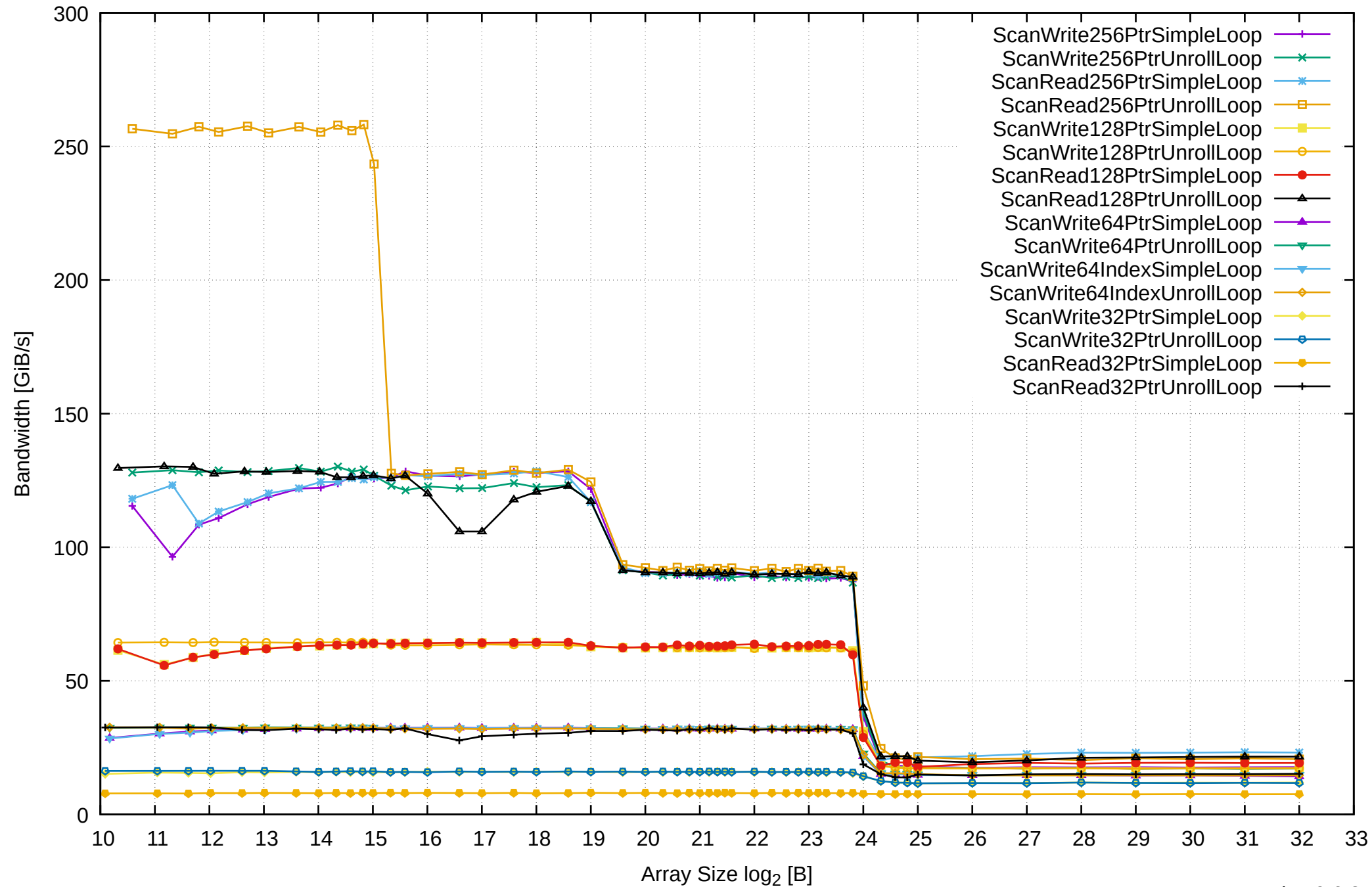
AMD Ryzen Threadripper 3955WX 128GB - One Thread Memory Bandwidth (only 64-bit Reads)
