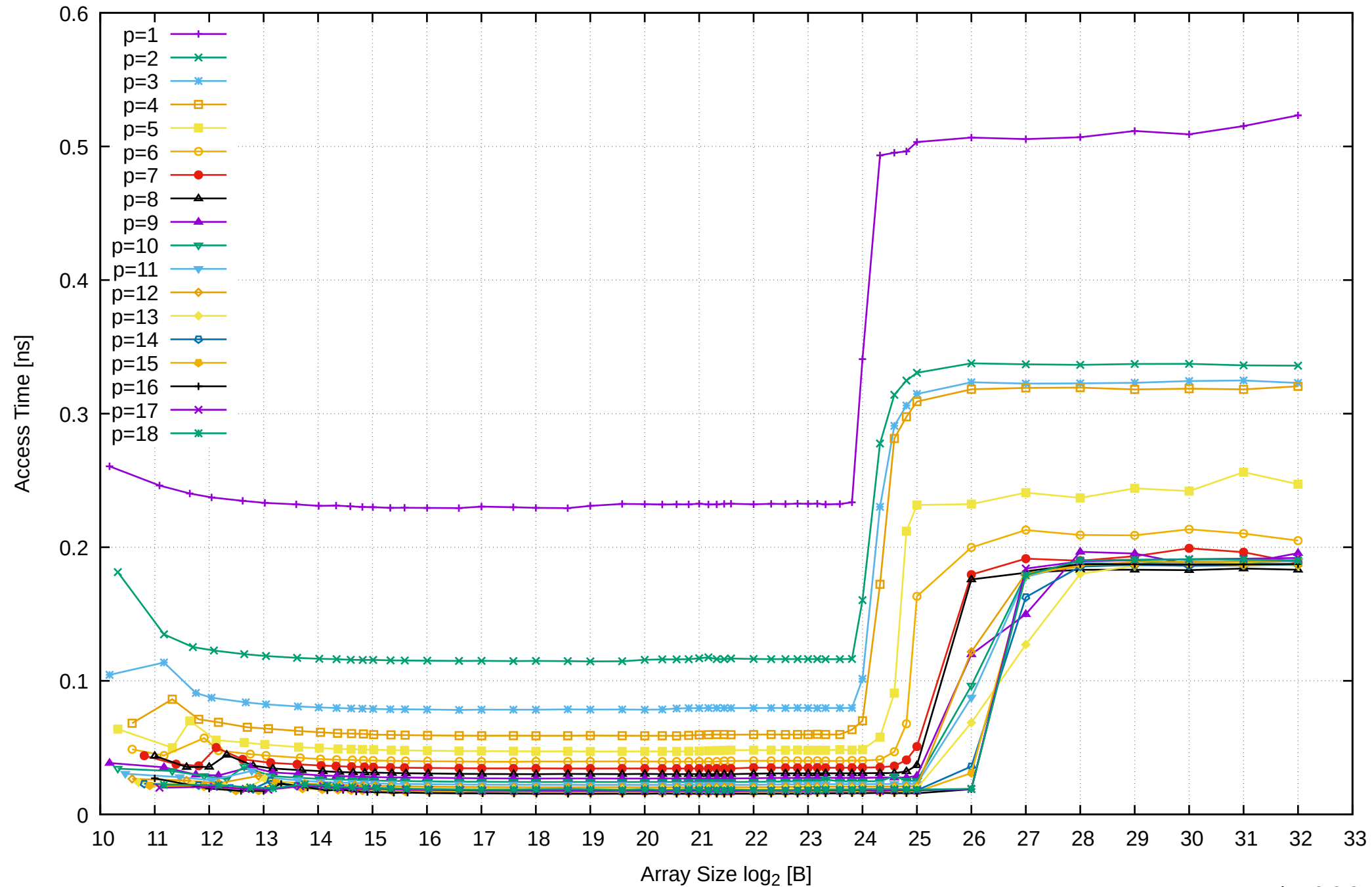
AMD Ryzen Threadripper 3955WX 128GB - Parallel Memory Access Time - ScanWrite64PtrSimpleLoop
