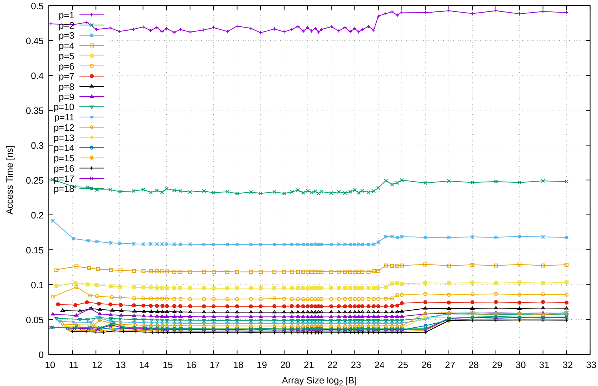
AMD Ryzen Threadripper 3955WX 128GB - Parallel Memory Access Time - ScanRead32PtrSimpleLoop
