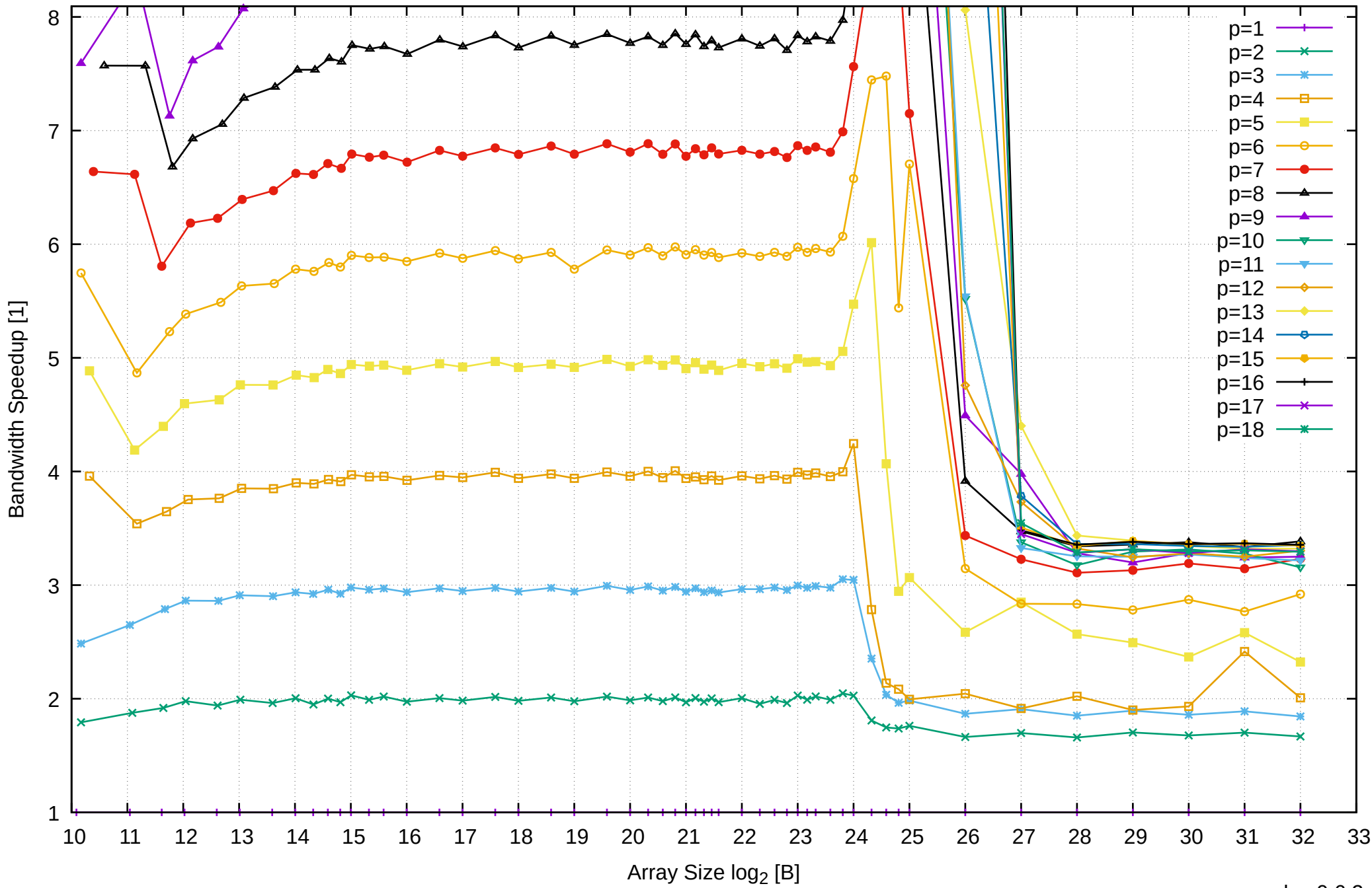
AMD Ryzen Threadripper 3955WX 128GB - Speedup of Parallel Memory Bandwidth (enlarged) - ScanWrite32PtrSimpleLoop
