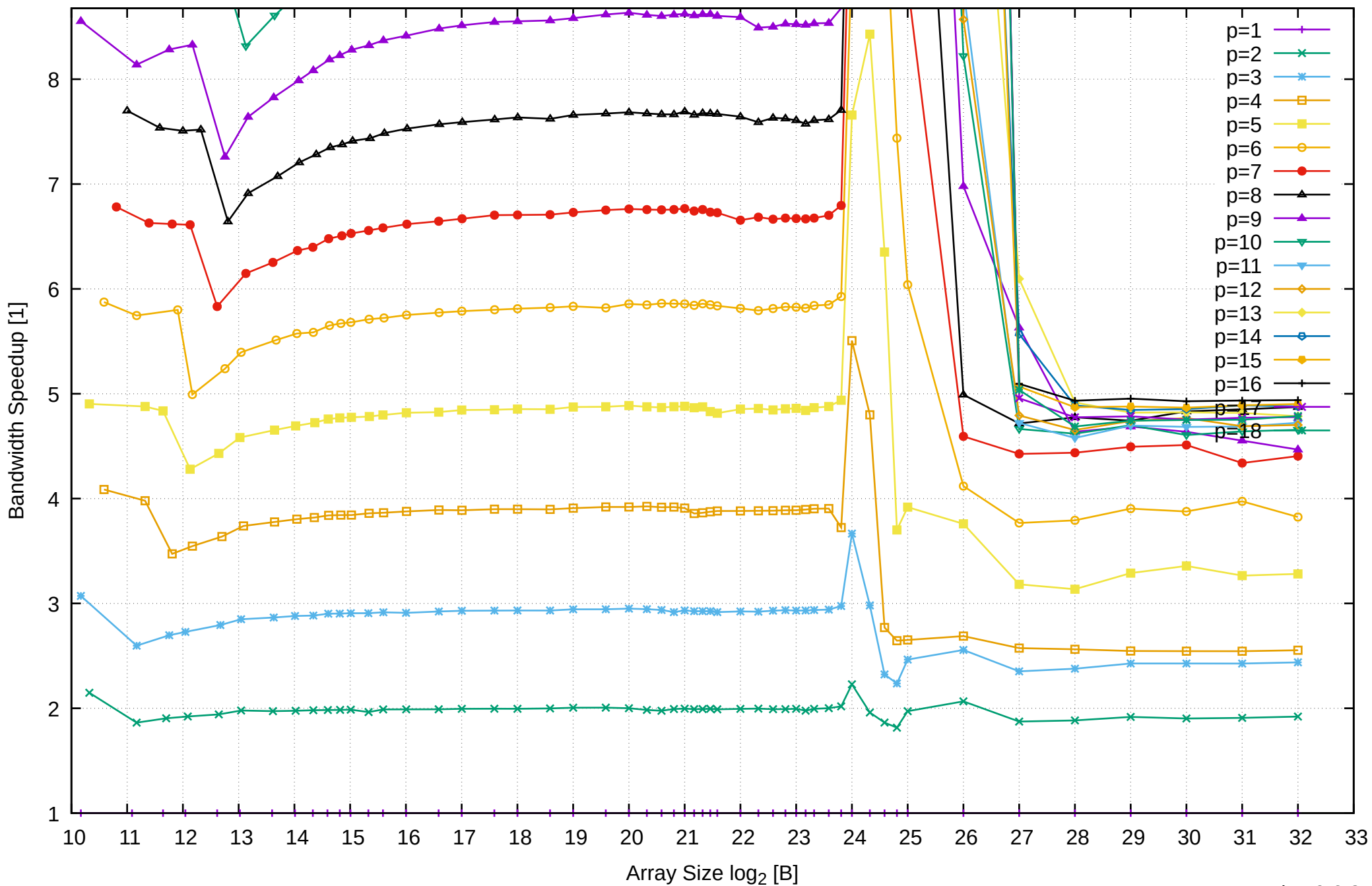
AMD Ryzen Threadripper 3955WX 128GB - Speedup of Parallel Memory Bandwidth (enlarged) - ScanRead64IndexSimpleLoop
