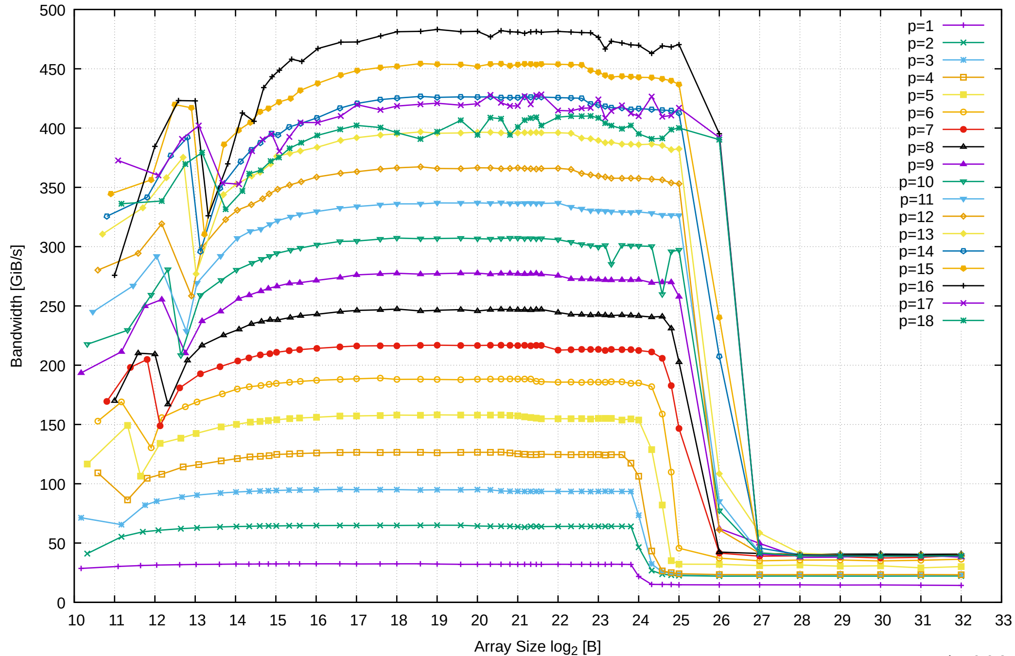
AMD Ryzen Threadripper 3955WX 128GB - Parallel Memory Bandwidth - ScanWrite64PtrSimpleLoop
