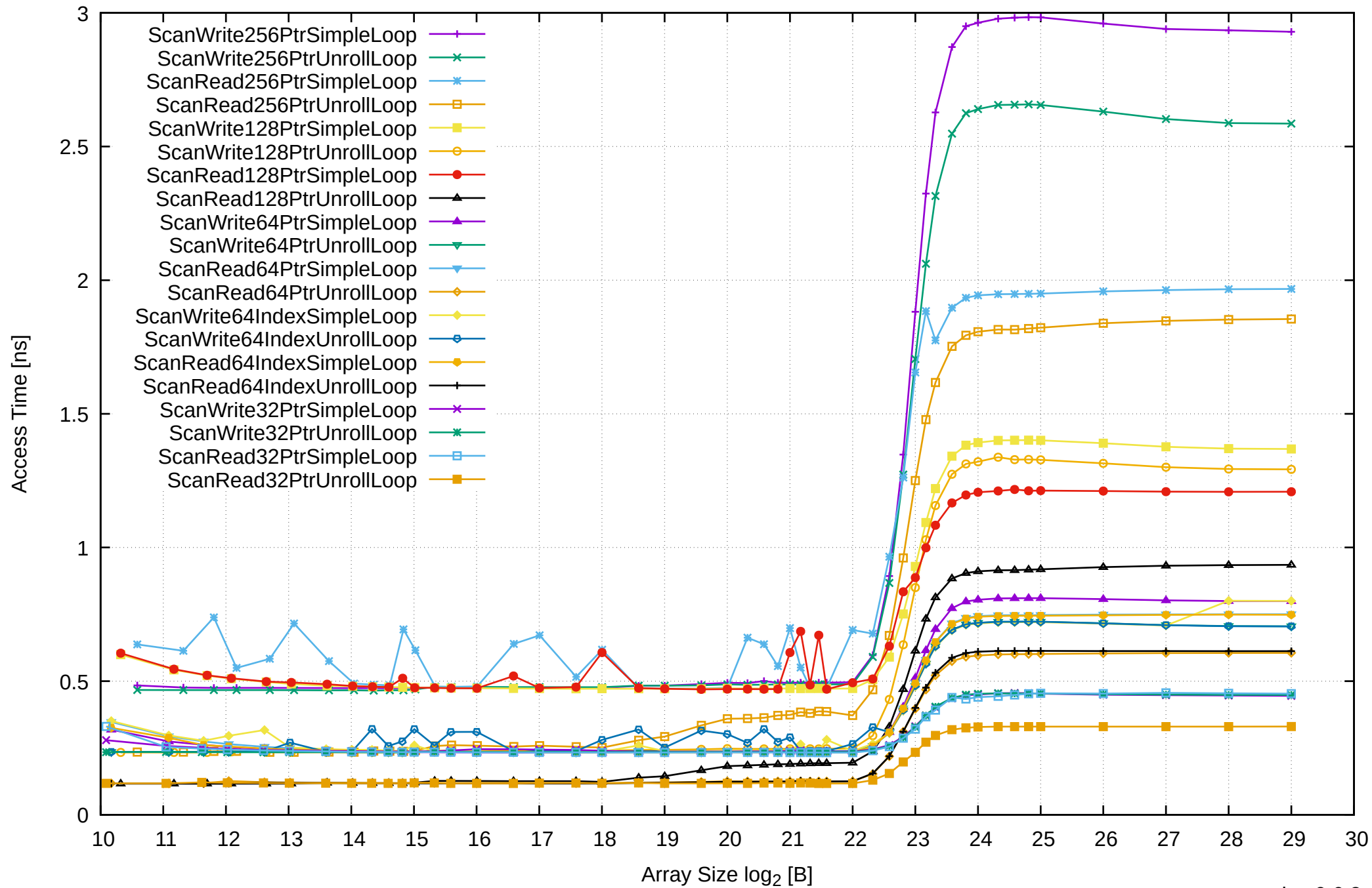
AMD Ryzen Threadripper 2950X 128GB - One Thread Memory Latency (excluding Permutation)
