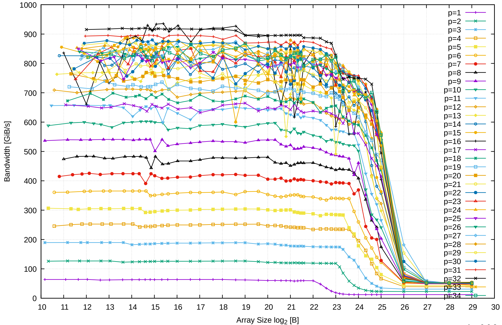
AMD Ryzen Threadripper 2950X 128GB - Parallel Memory Bandwidth - ScanRead64IndexUnrollLoop
