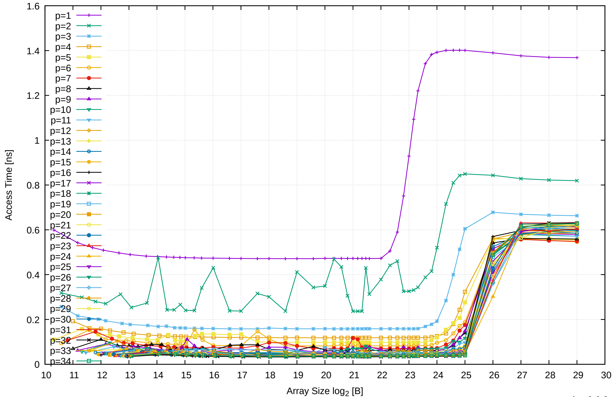
AMD Ryzen Threadripper 2950X 128GB - Parallel Memory Access Time - ScanWrite128PtrSimpleLoop
