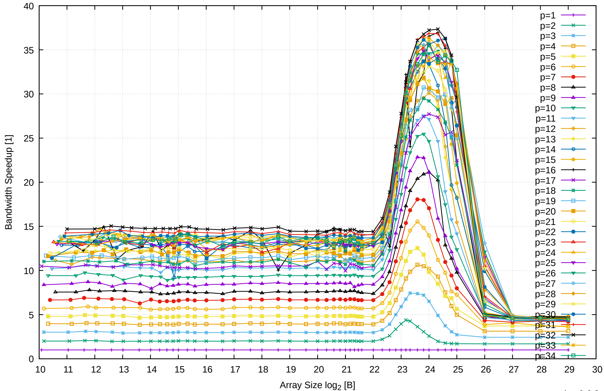
AMD Ryzen Threadripper 2950X 128GB - Speedup of Parallel Memory Bandwidth - ScanRead32PtrUnrollLoop
