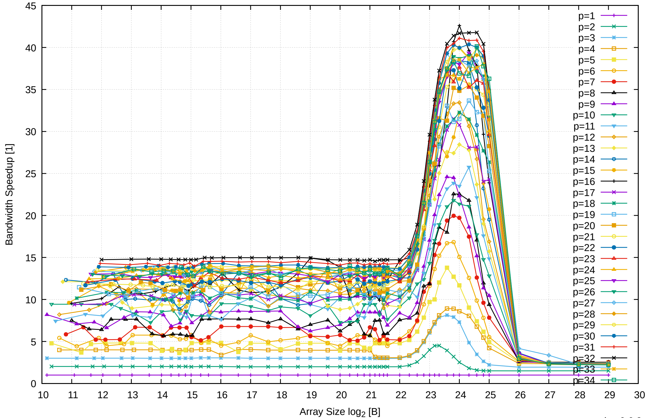
AMD Ryzen Threadripper 2950X 128GB - Speedup of Parallel Memory Bandwidth - ScanWrite64PtrUnrollLoop
