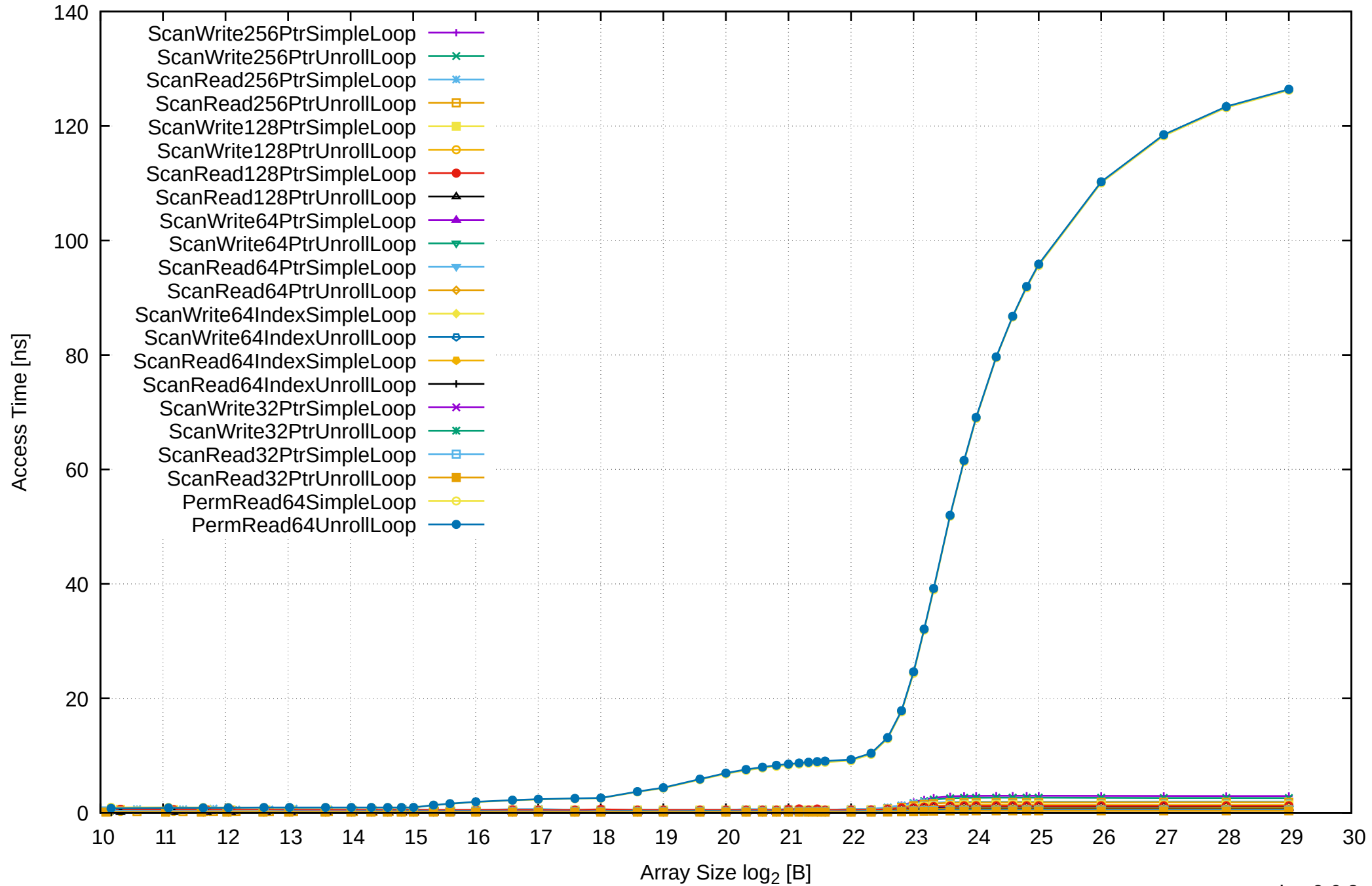
AMD Ryzen Threadripper 2950X 128GB - One Thread Memory Latency (Access Time)
