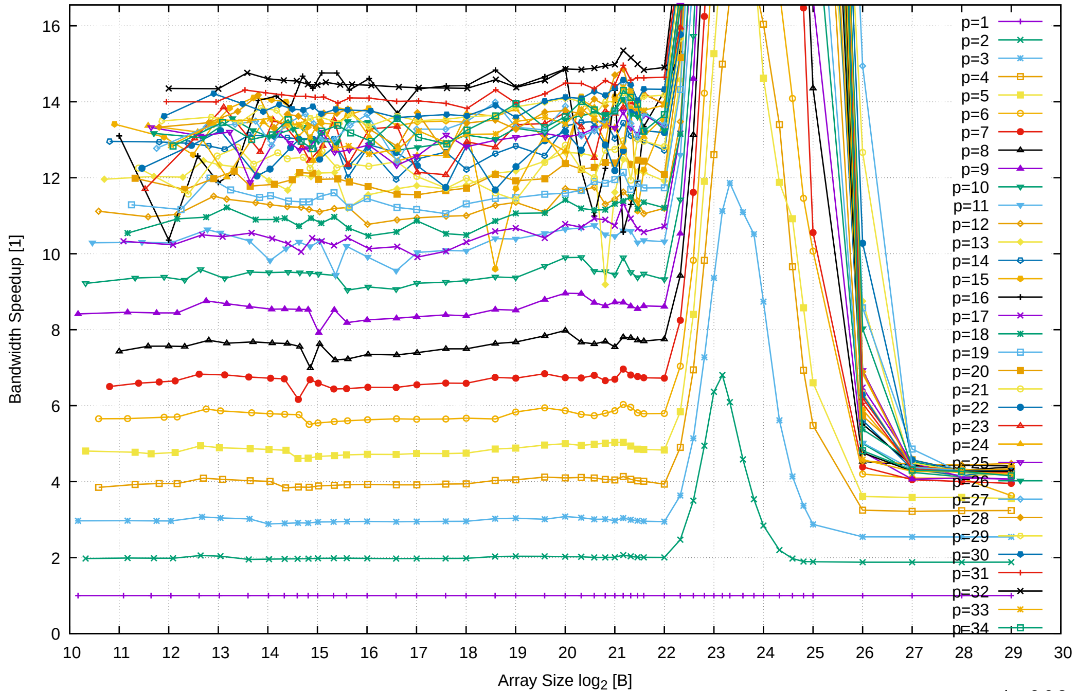
AMD Ryzen Threadripper 2950X 128GB - Speedup of Parallel Memory Bandwidth (enlarged) - ScanRead64IndexUnrollLoop
