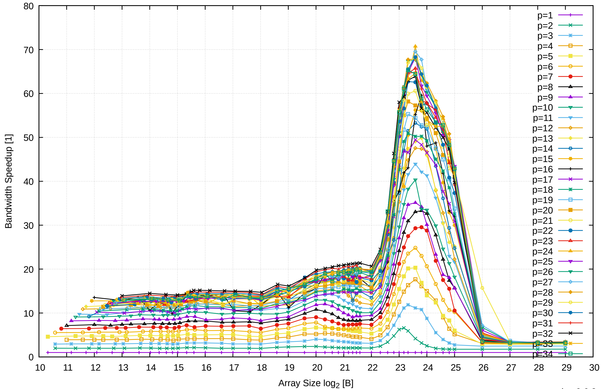
AMD Ryzen Threadripper 2950X 128GB - Speedup of Parallel Memory Bandwidth - ScanRead128PtrUnrollLoop
