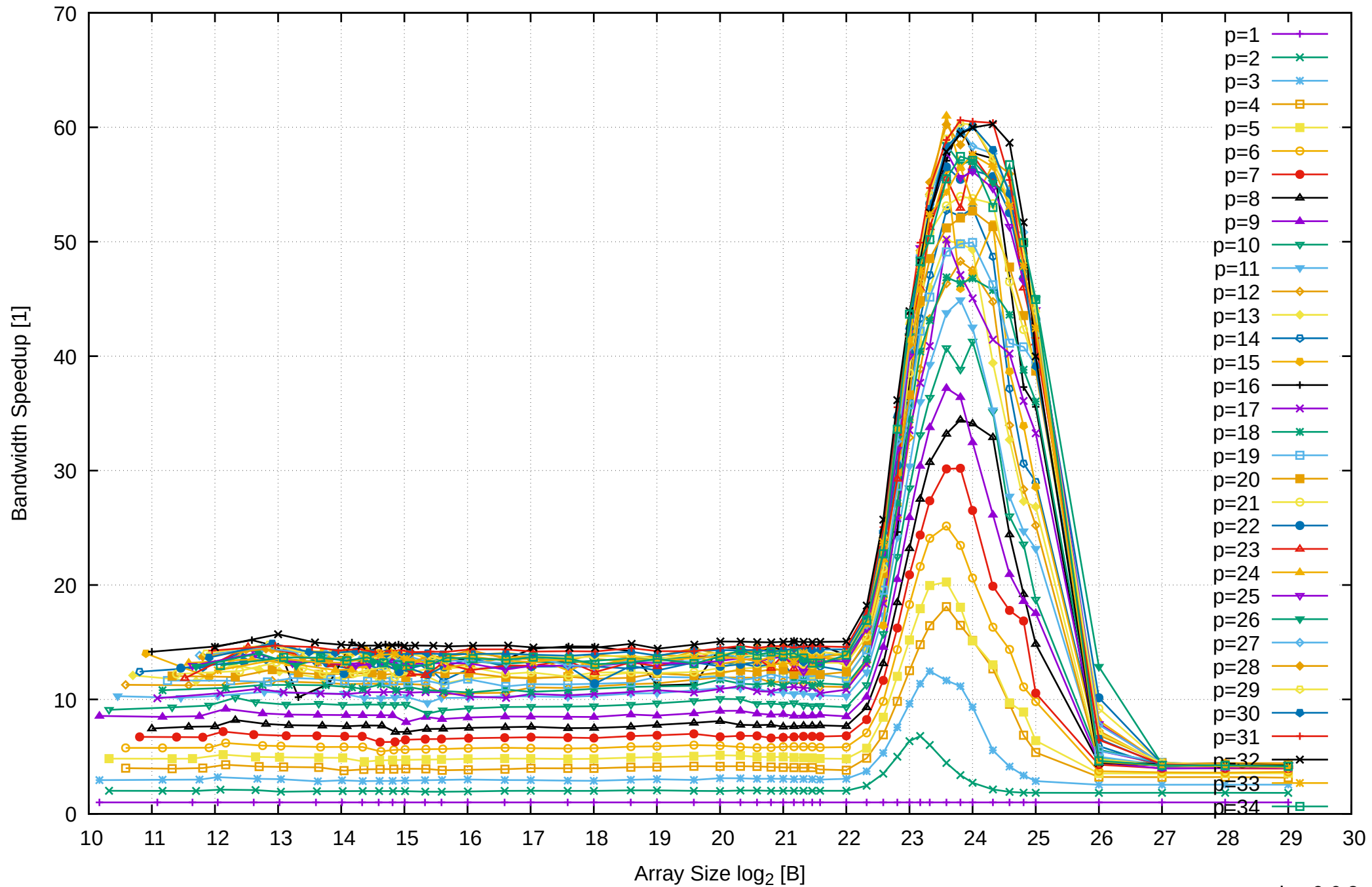
AMD Ryzen Threadripper 2950X 128GB - Speedup of Parallel Memory Bandwidth - ScanRead64PtrUnrollLoop
