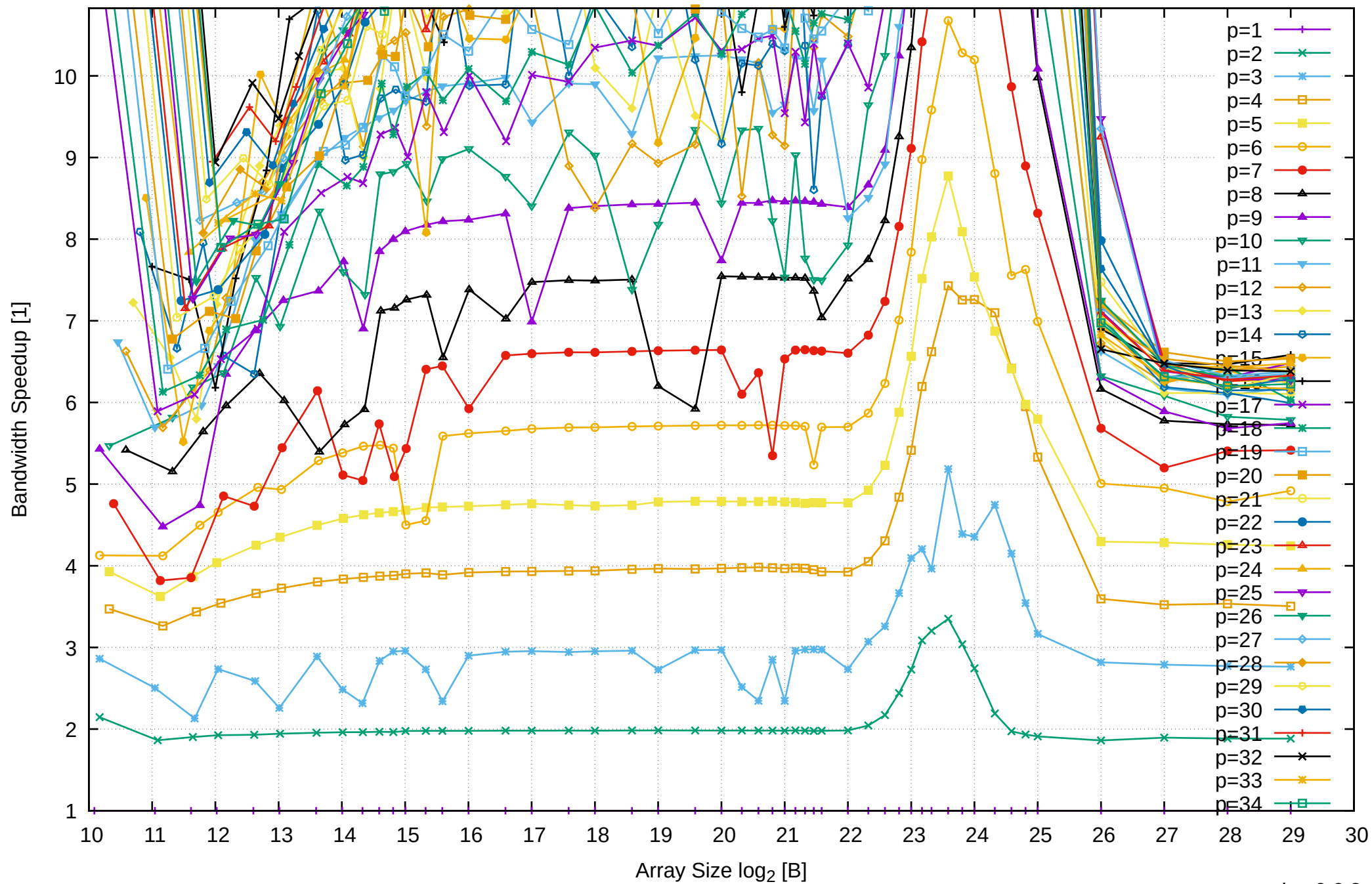
AMD Ryzen Threadripper 2950X 128GB - Speedup of Parallel Memory Bandwidth (enlarged) - ScanRead32PtrSimpleLoop
