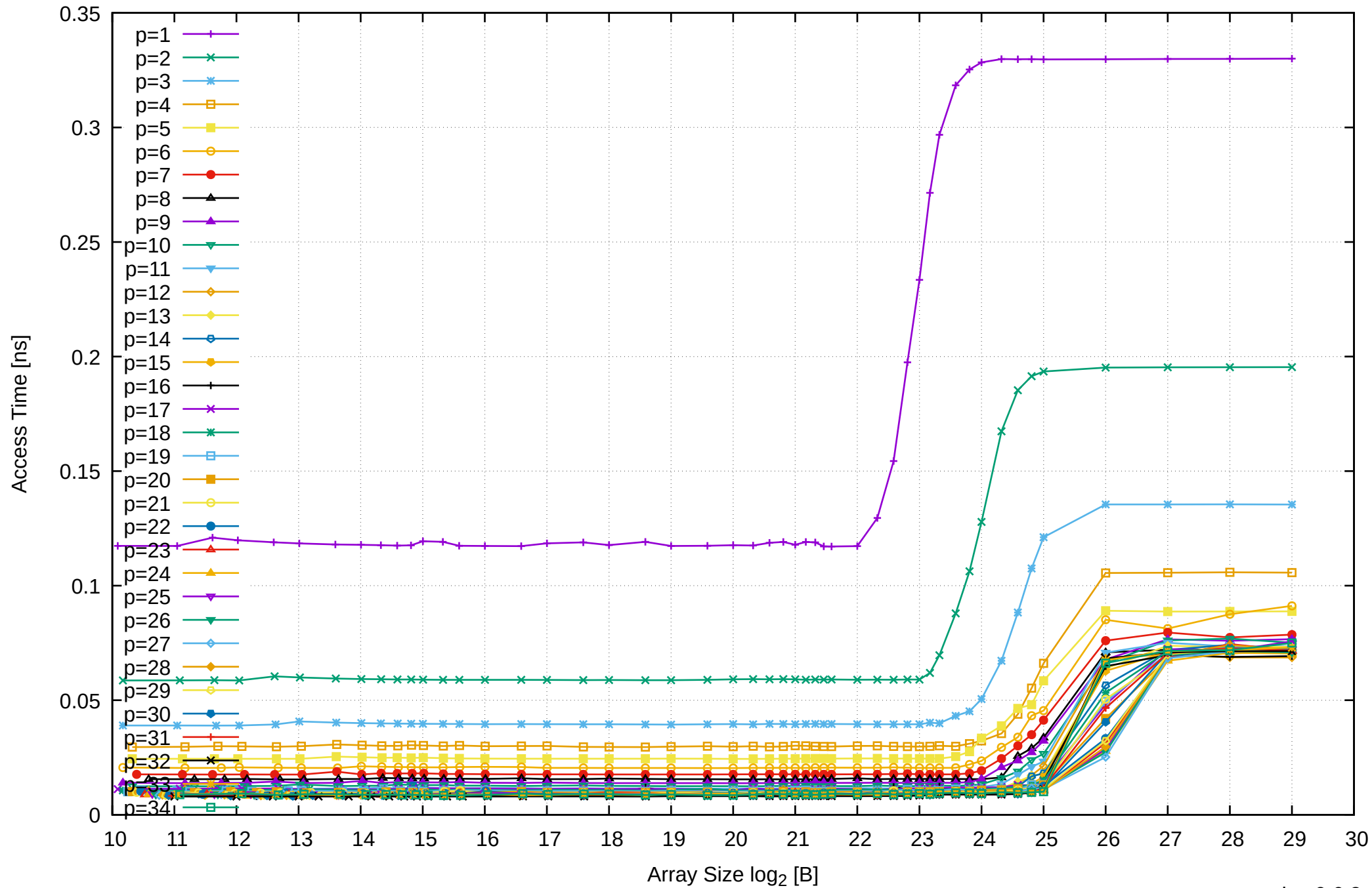
AMD Ryzen Threadripper 2950X 128GB - Parallel Memory Access Time - ScanRead32PtrUnrollLoop
