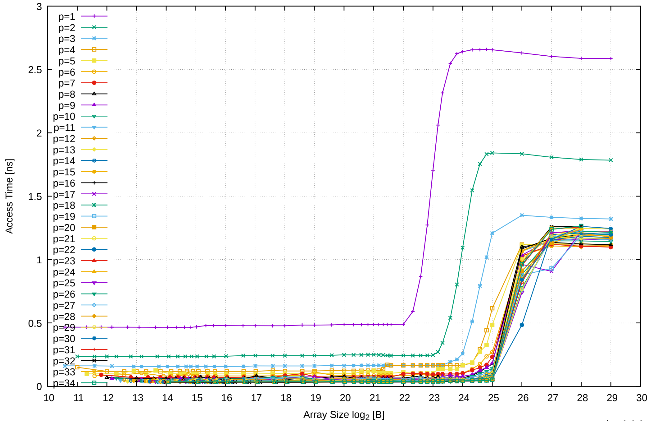
AMD Ryzen Threadripper 2950X 128GB - Parallel Memory Access Time - ScanWrite256PtrUnrollLoop
