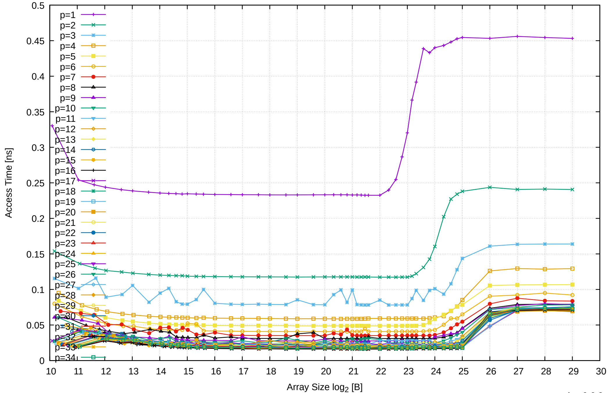
AMD Ryzen Threadripper 2950X 128GB - Parallel Memory Access Time - ScanRead32PtrSimpleLoop
