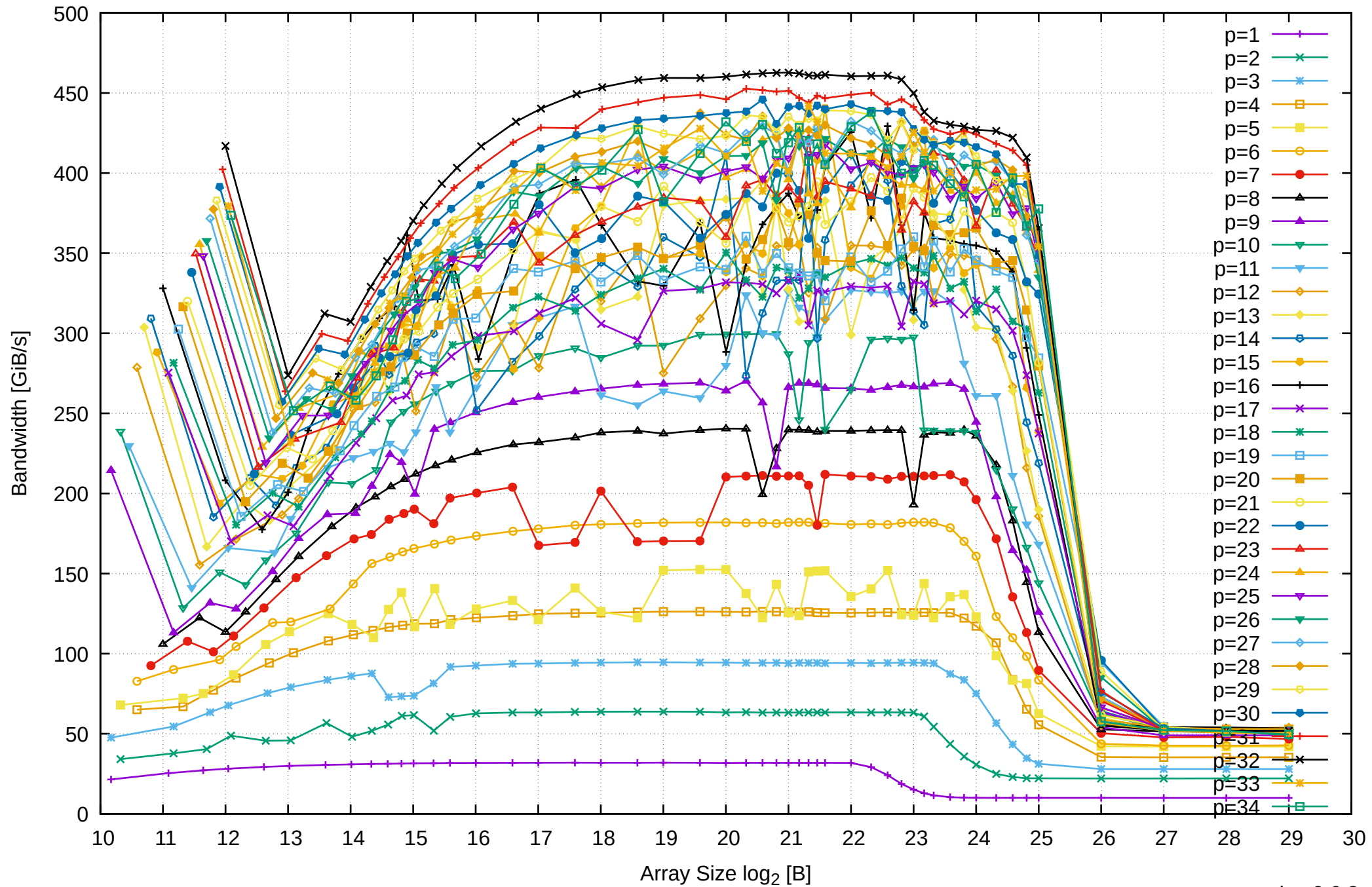
AMD Ryzen Threadripper 2950X 128GB - Parallel Memory Bandwidth - ScanRead64PtrSimpleLoop
