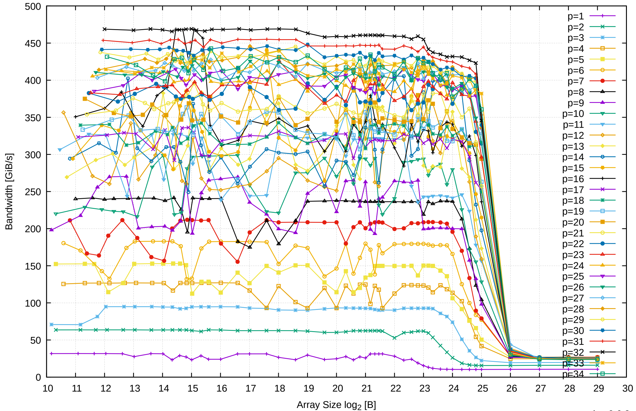
AMD Ryzen Threadripper 2950X 128GB - Parallel Memory Bandwidth - ScanWrite64IndexUnrollLoop
