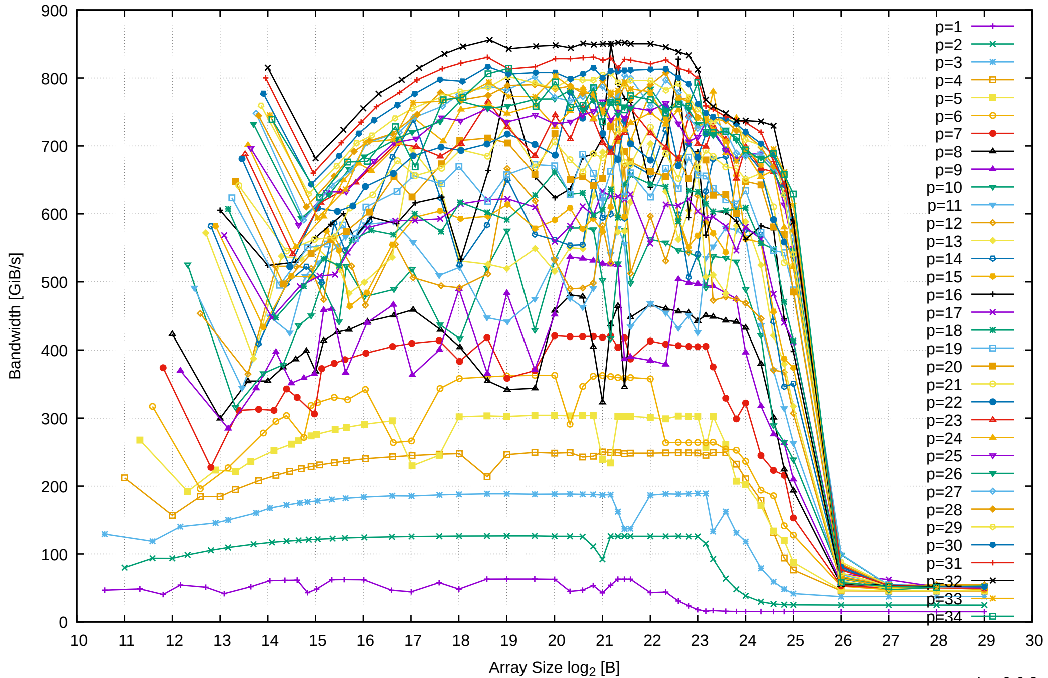
AMD Ryzen Threadripper 2950X 128GB - Parallel Memory Bandwidth - ScanRead256PtrSimpleLoop
