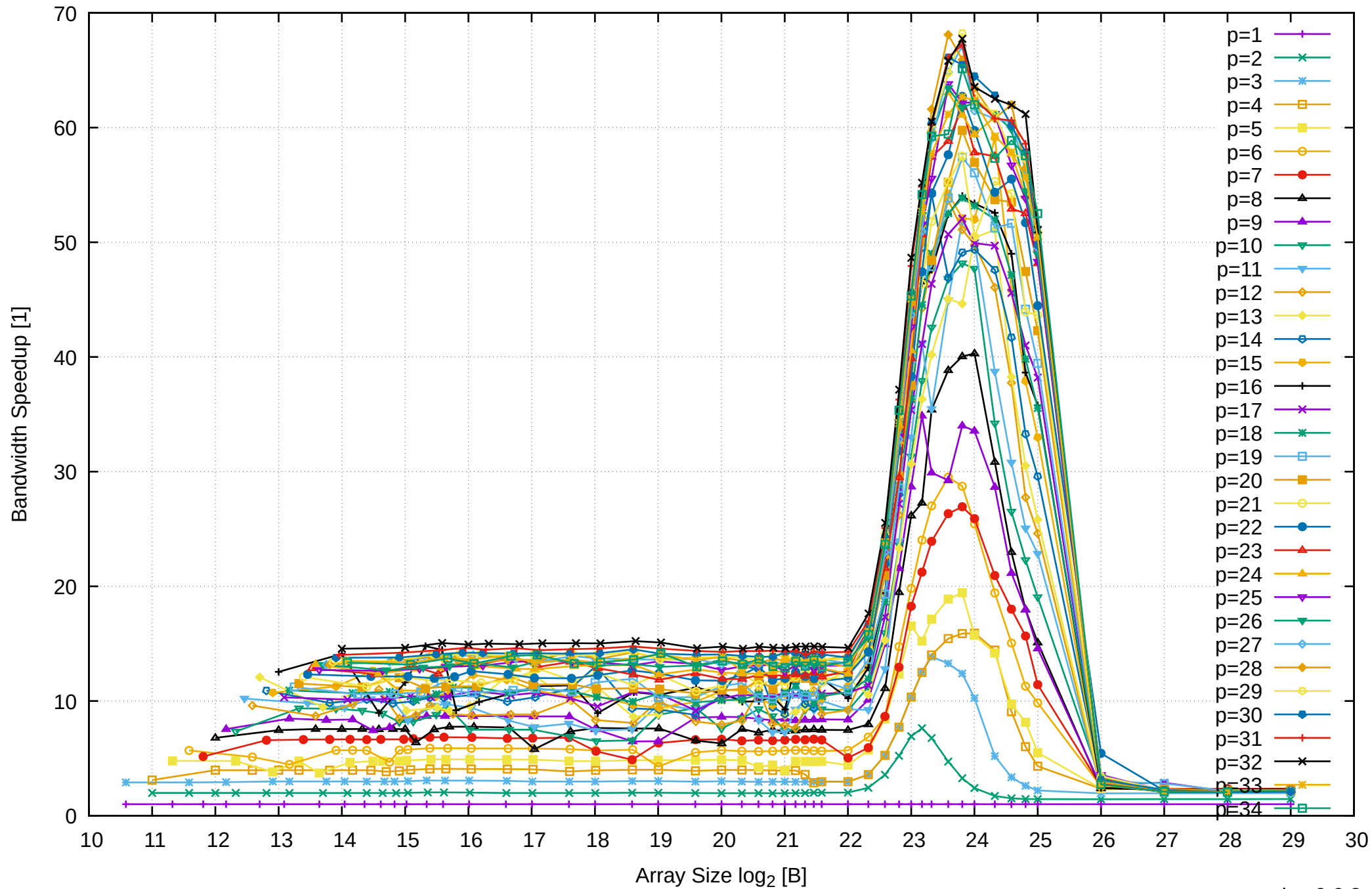
AMD Ryzen Threadripper 2950X 128GB - Speedup of Parallel Memory Bandwidth - ScanWrite256PtrUnrollLoop
