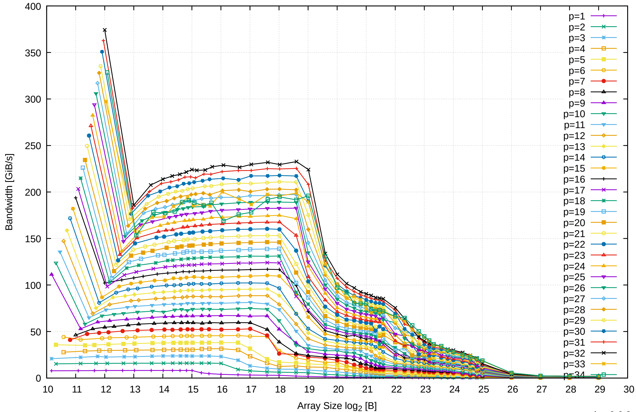
AMD Ryzen Threadripper 2950X 128GB - Parallel Memory Bandwidth - PermRead64SimpleLoop
