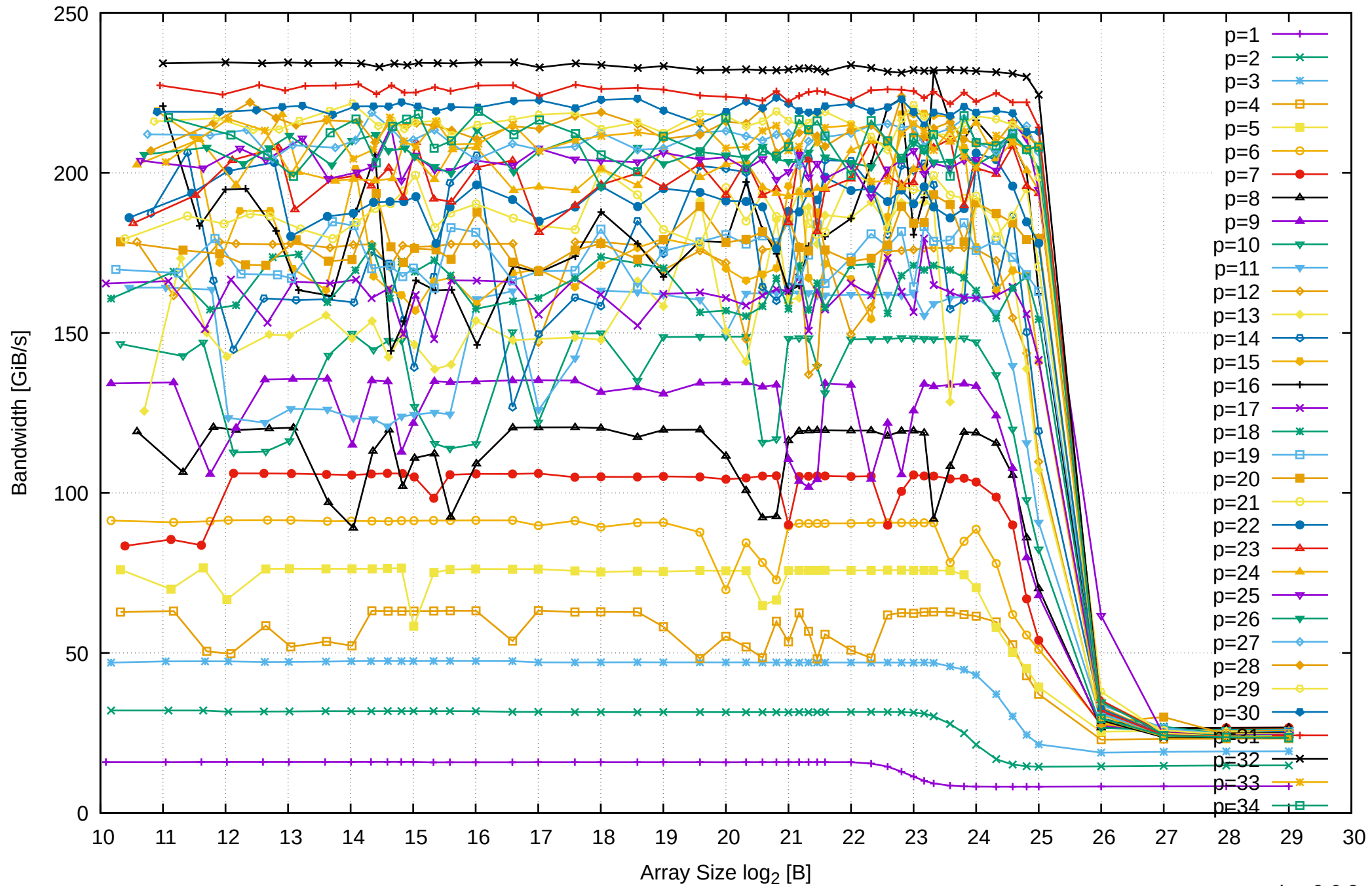
AMD Ryzen Threadripper 2950X 128GB - Parallel Memory Bandwidth - ScanWrite32PtrUnrollLoop
