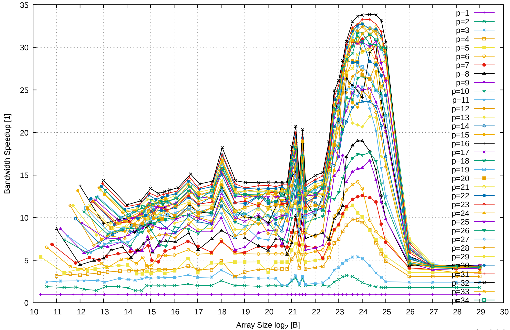
AMD Ryzen Threadripper 2950X 128GB - Speedup of Parallel Memory Bandwidth - ScanRead128PtrSimpleLoop
