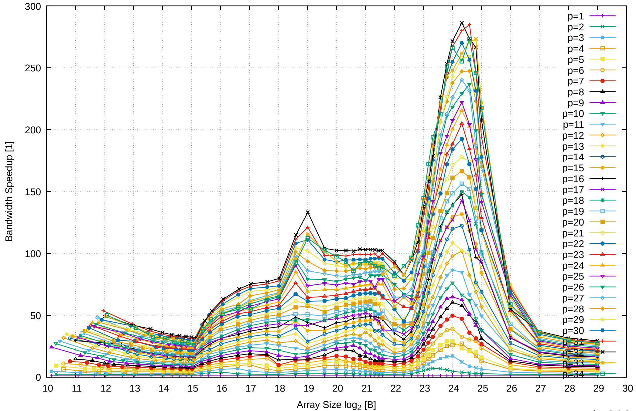
AMD Ryzen Threadripper 2950X 128GB - Speedup of Parallel Memory Bandwidth - PermRead64UnrollLoop
