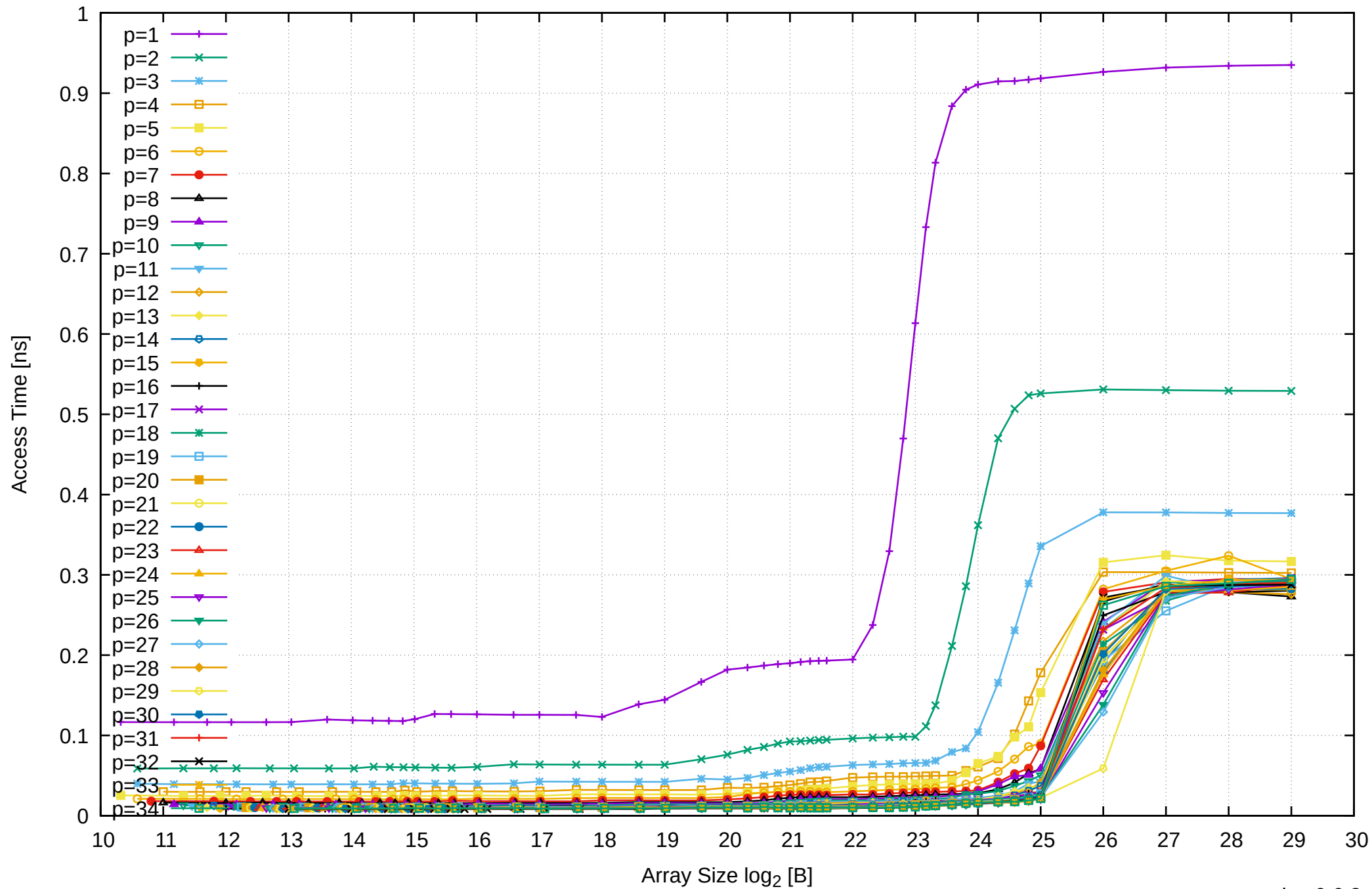
AMD Ryzen Threadripper 2950X 128GB - Parallel Memory Access Time - ScanRead128PtrUnrollLoop
