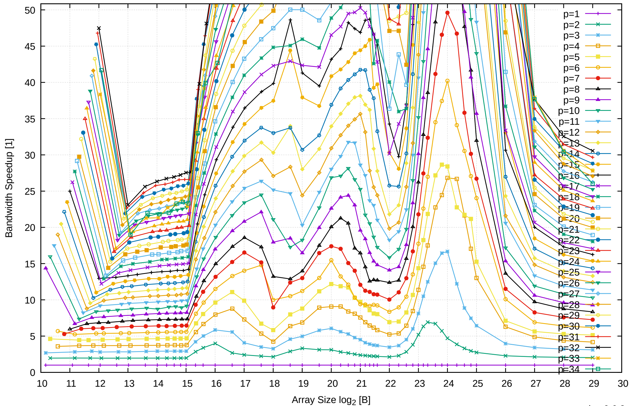
AMD Ryzen Threadripper 2950X 128GB - Speedup of Parallel Memory Bandwidth (enlarged) - PermRead64SimpleLoop
