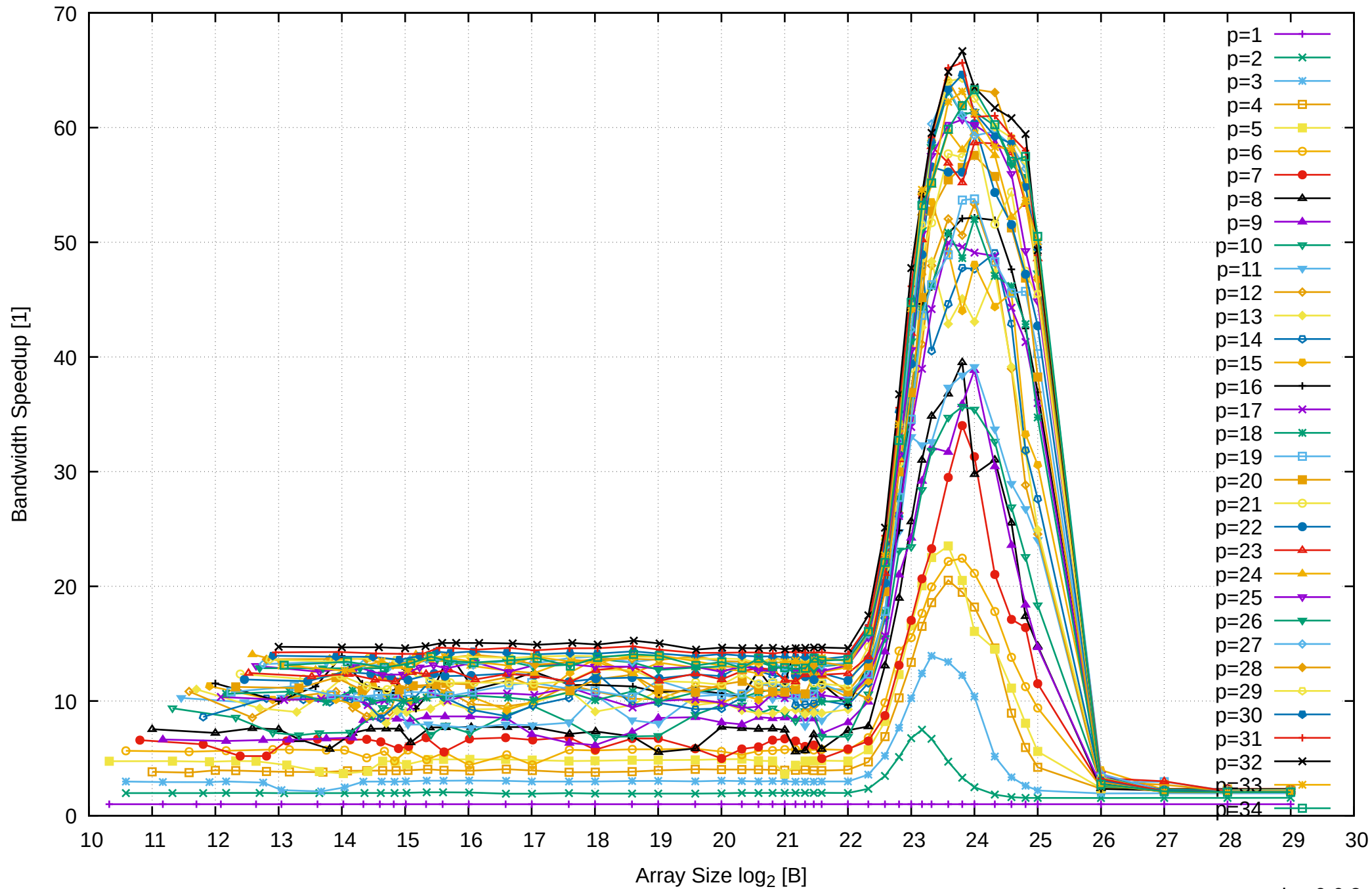
AMD Ryzen Threadripper 2950X 128GB - Speedup of Parallel Memory Bandwidth - ScanWrite128PtrUnrollLoop
