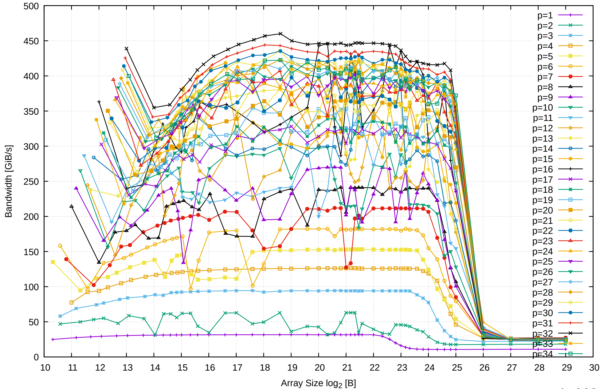
AMD Ryzen Threadripper 2950X 128GB - Parallel Memory Bandwidth - ScanWrite128PtrSimpleLoop
