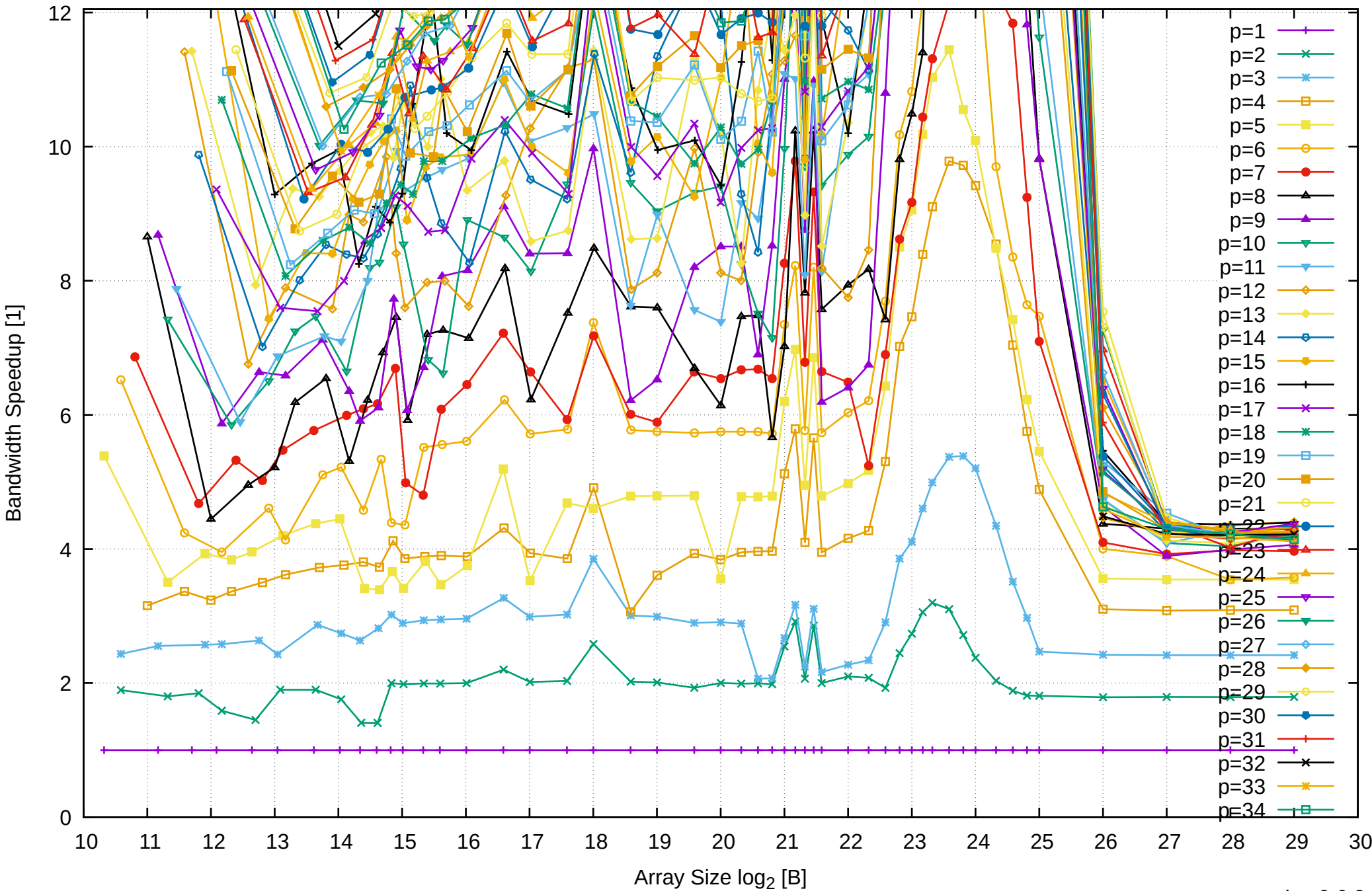
AMD Ryzen Threadripper 2950X 128GB - Speedup of Parallel Memory Bandwidth (enlarged) - ScanRead128PtrSimpleLoop
