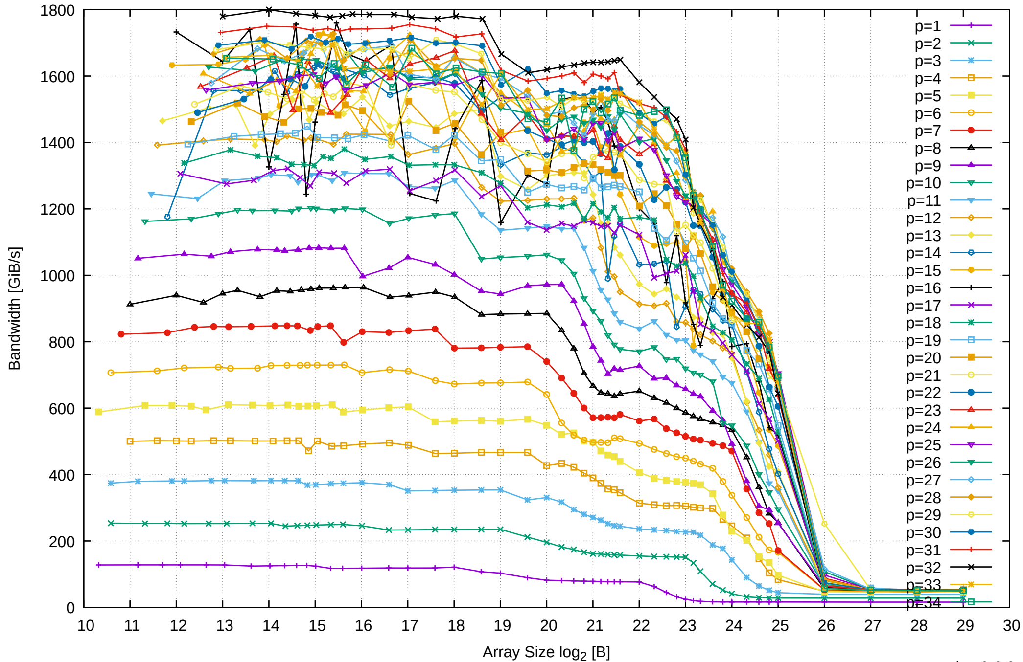
AMD Ryzen Threadripper 2950X 128GB - Parallel Memory Bandwidth - ScanRead128PtrUnrollLoop
