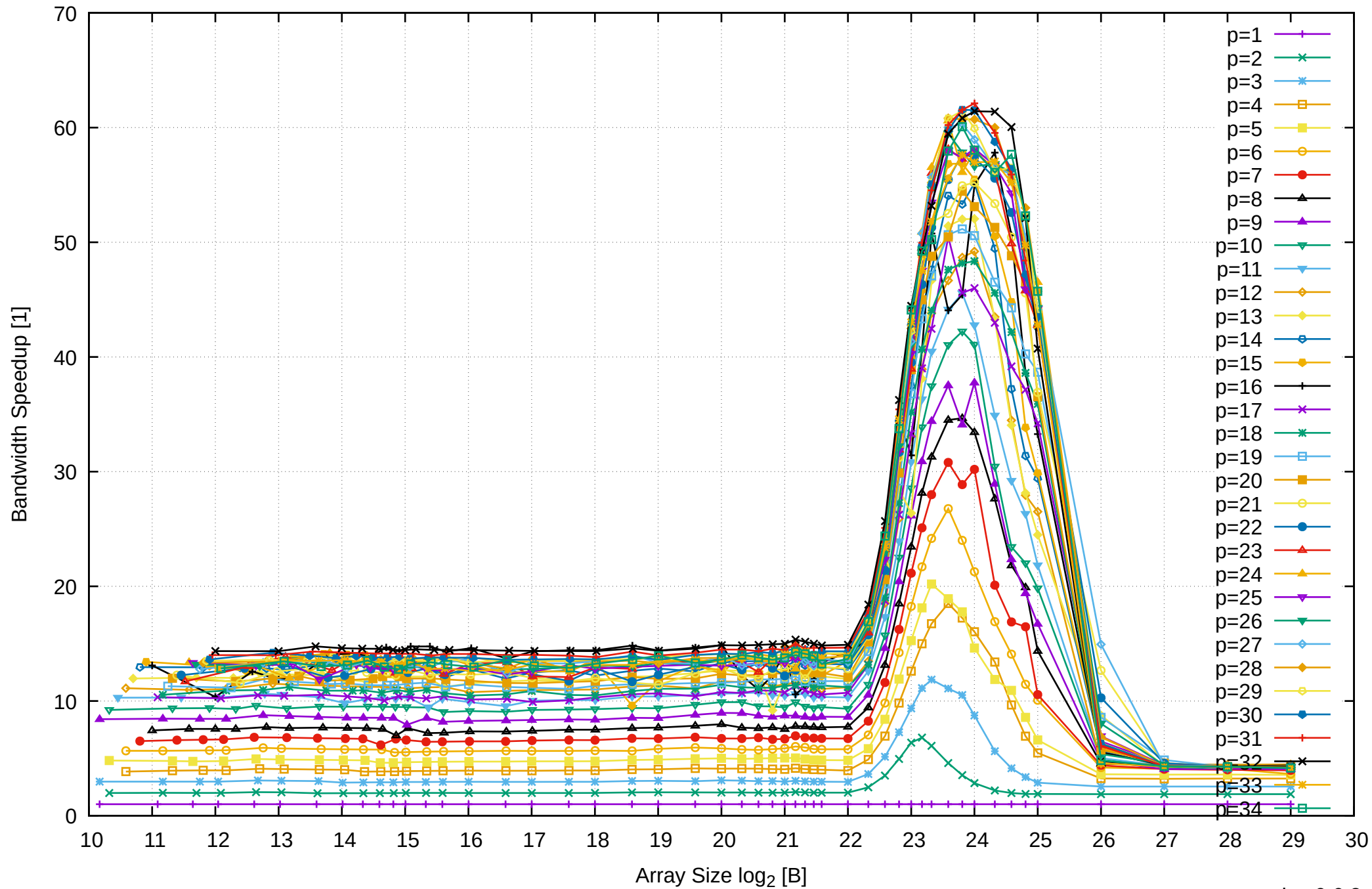
AMD Ryzen Threadripper 2950X 128GB - Speedup of Parallel Memory Bandwidth - ScanRead64IndexUnrollLoop
