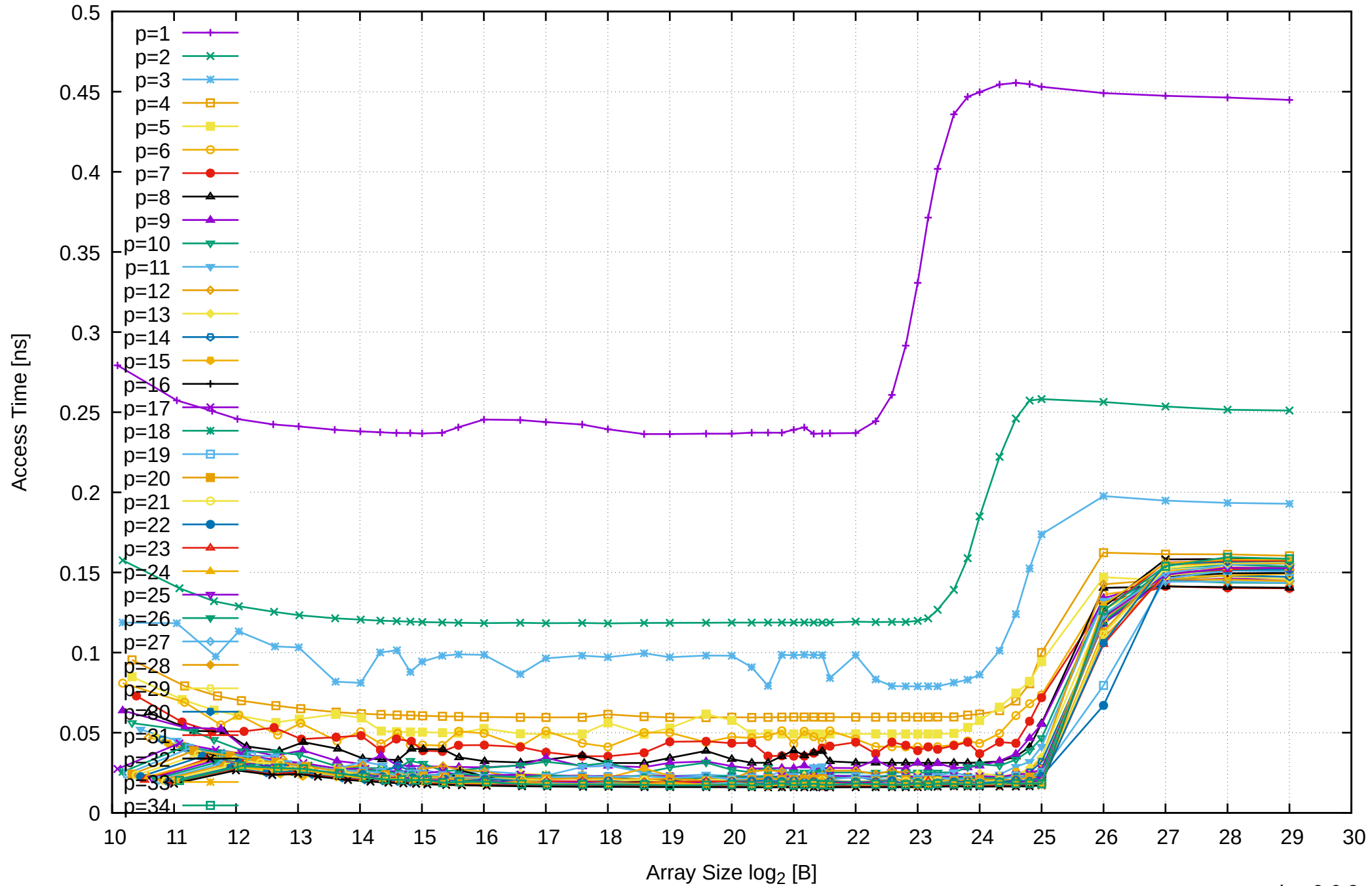
AMD Ryzen Threadripper 2950X 128GB - Parallel Memory Access Time - ScanWrite32PtrSimpleLoop
