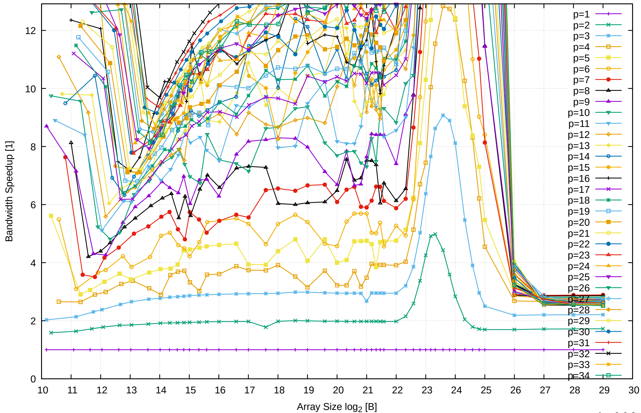
AMD Ryzen Threadripper 2950X 128GB - Speedup of Parallel Memory Bandwidth (enlarged) - ScanWrite64PtrSimpleLoop
