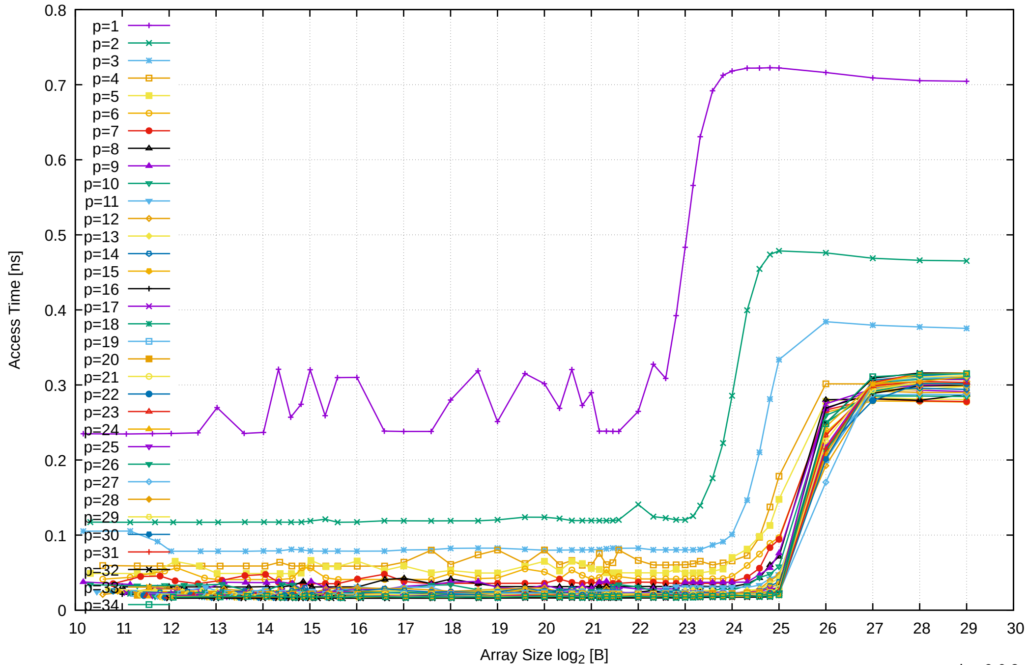
AMD Ryzen Threadripper 2950X 128GB - Parallel Memory Access Time - ScanWrite64IndexUnrollLoop
