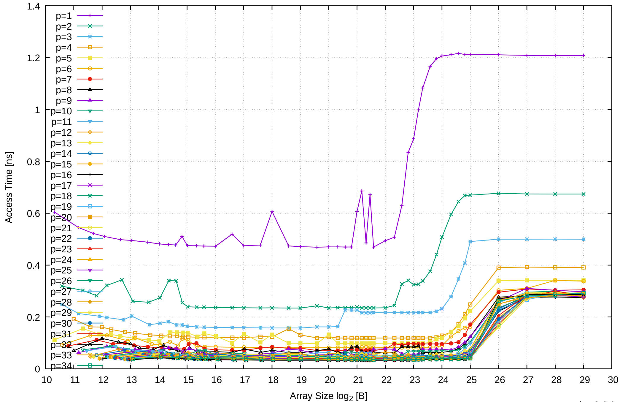
AMD Ryzen Threadripper 2950X 128GB - Parallel Memory Access Time - ScanRead128PtrSimpleLoop
