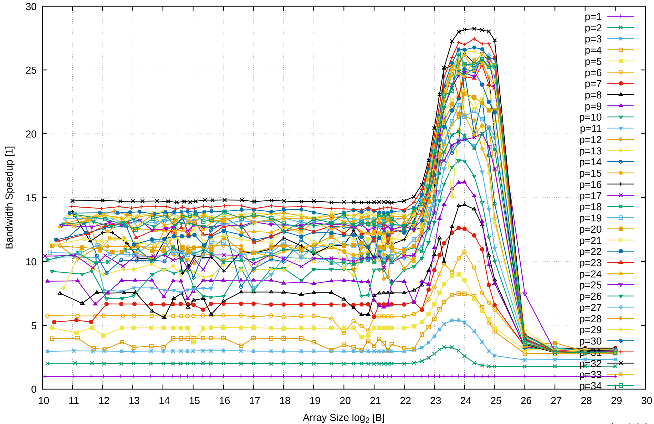
AMD Ryzen Threadripper 2950X 128GB - Speedup of Parallel Memory Bandwidth - ScanWrite32PtrUnrollLoop
