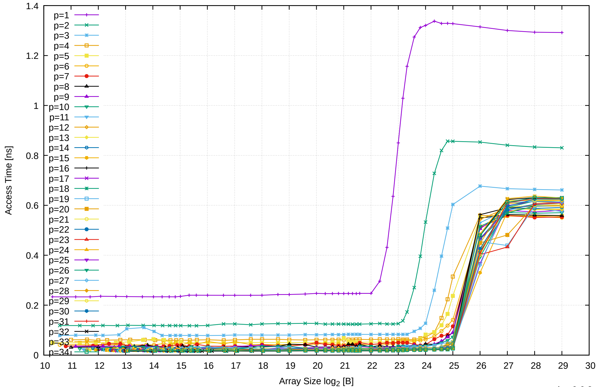
AMD Ryzen Threadripper 2950X 128GB - Parallel Memory Access Time - ScanWrite128PtrUnrollLoop
