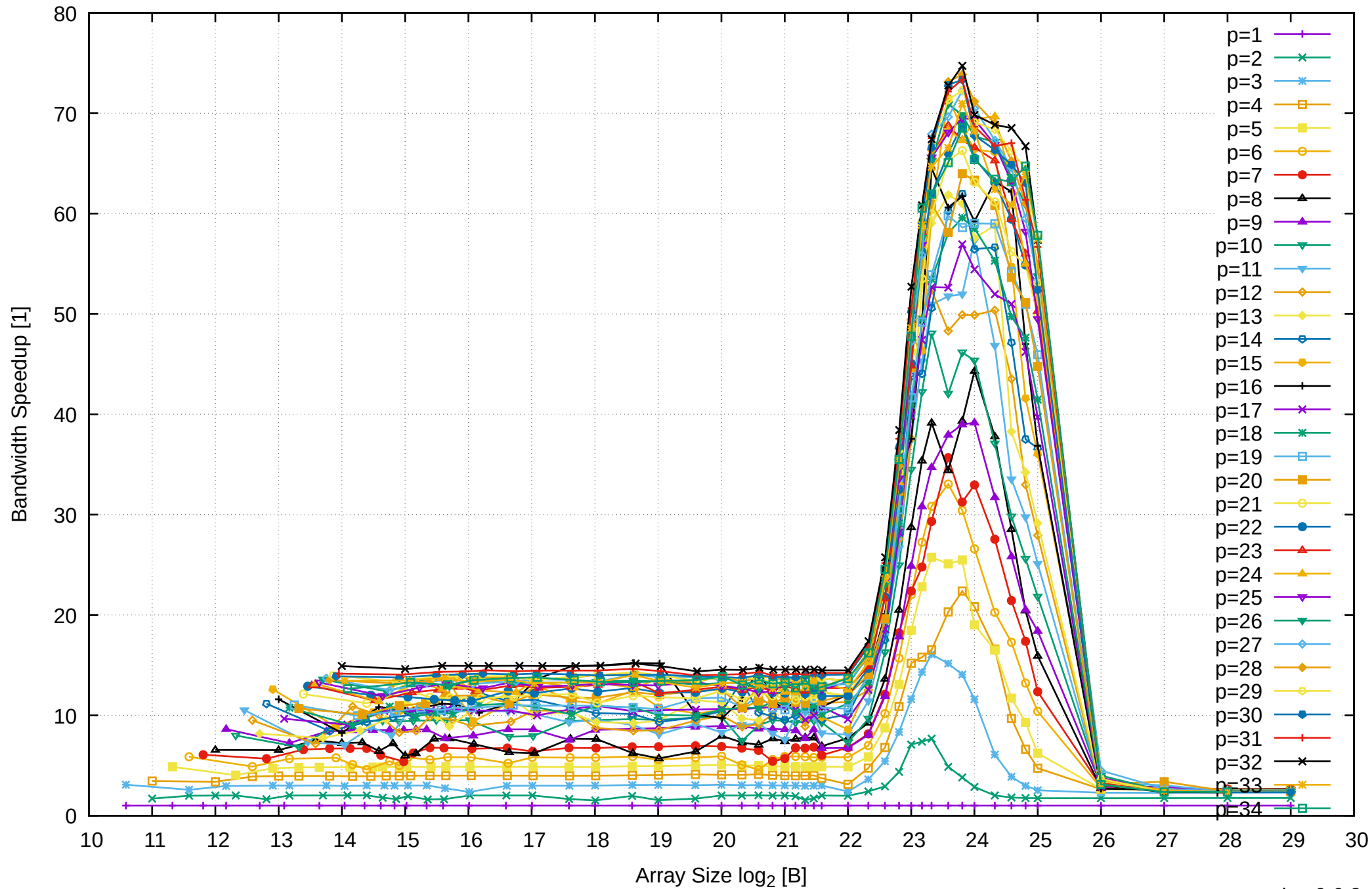
AMD Ryzen Threadripper 2950X 128GB - Speedup of Parallel Memory Bandwidth - ScanWrite256PtrSimpleLoop
