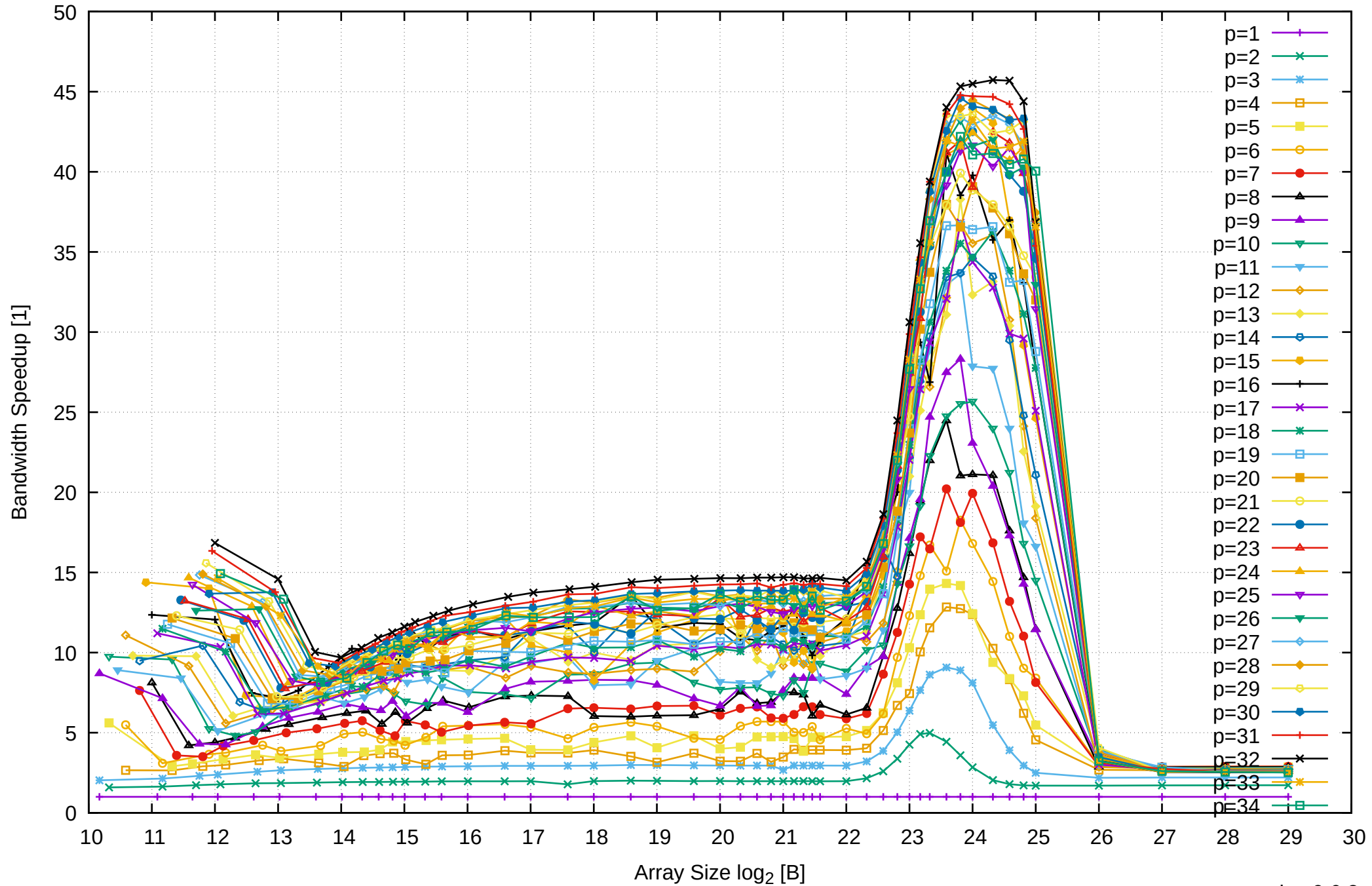
AMD Ryzen Threadripper 2950X 128GB - Speedup of Parallel Memory Bandwidth - ScanWrite64PtrSimpleLoop
