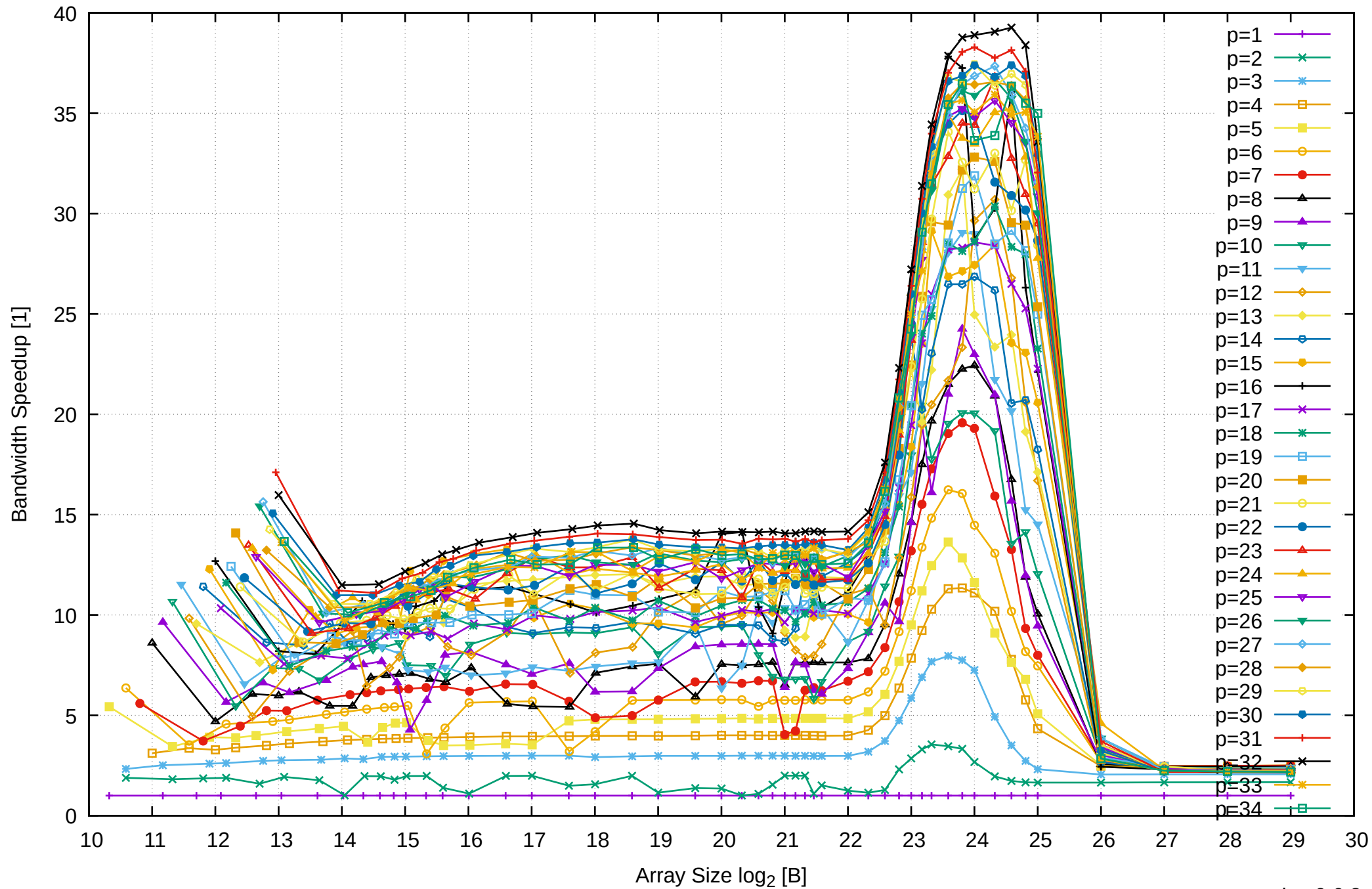
AMD Ryzen Threadripper 2950X 128GB - Speedup of Parallel Memory Bandwidth - ScanWrite128PtrSimpleLoop
