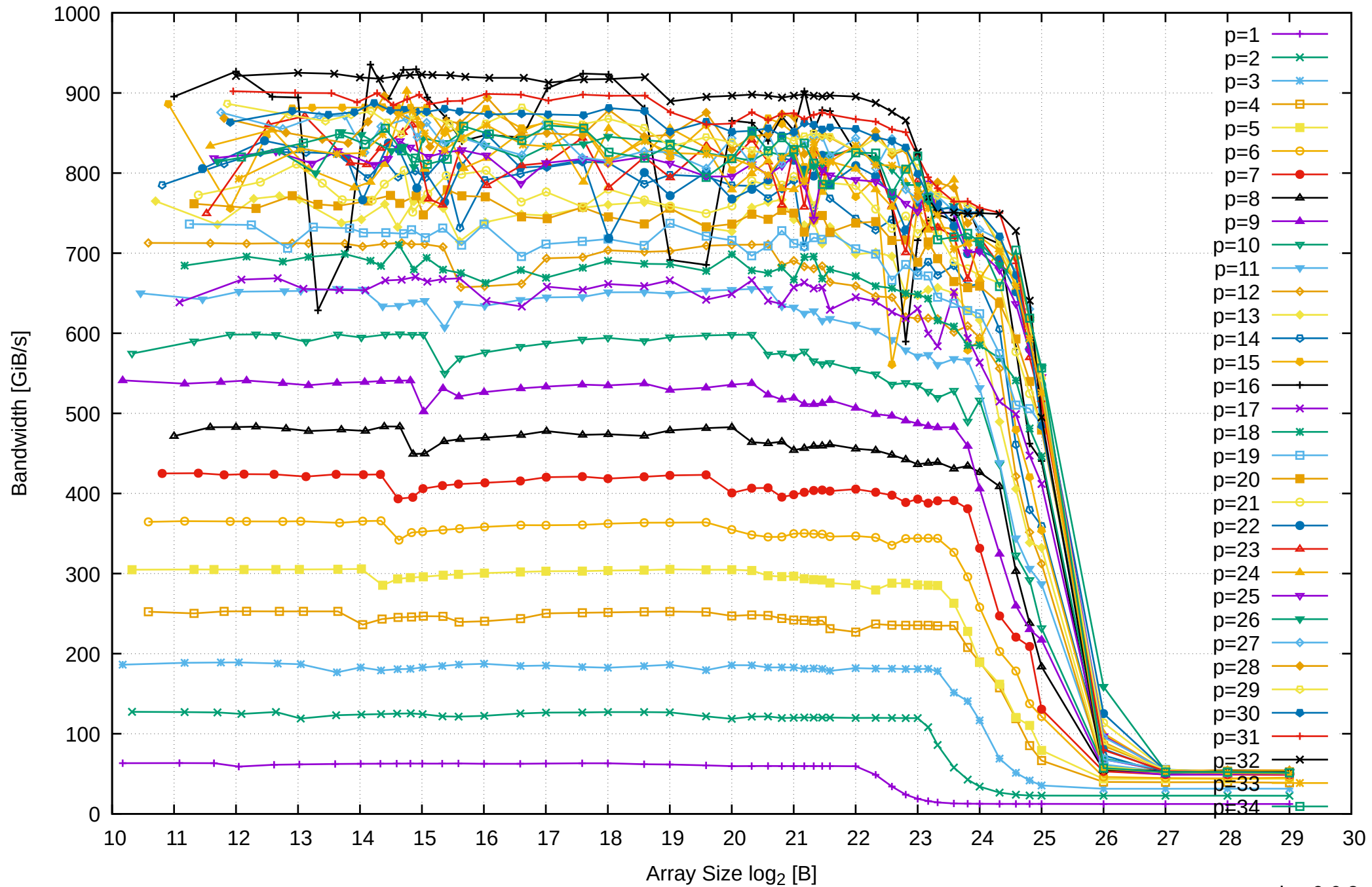
AMD Ryzen Threadripper 2950X 128GB - Parallel Memory Bandwidth - ScanRead64PtrUnrollLoop
