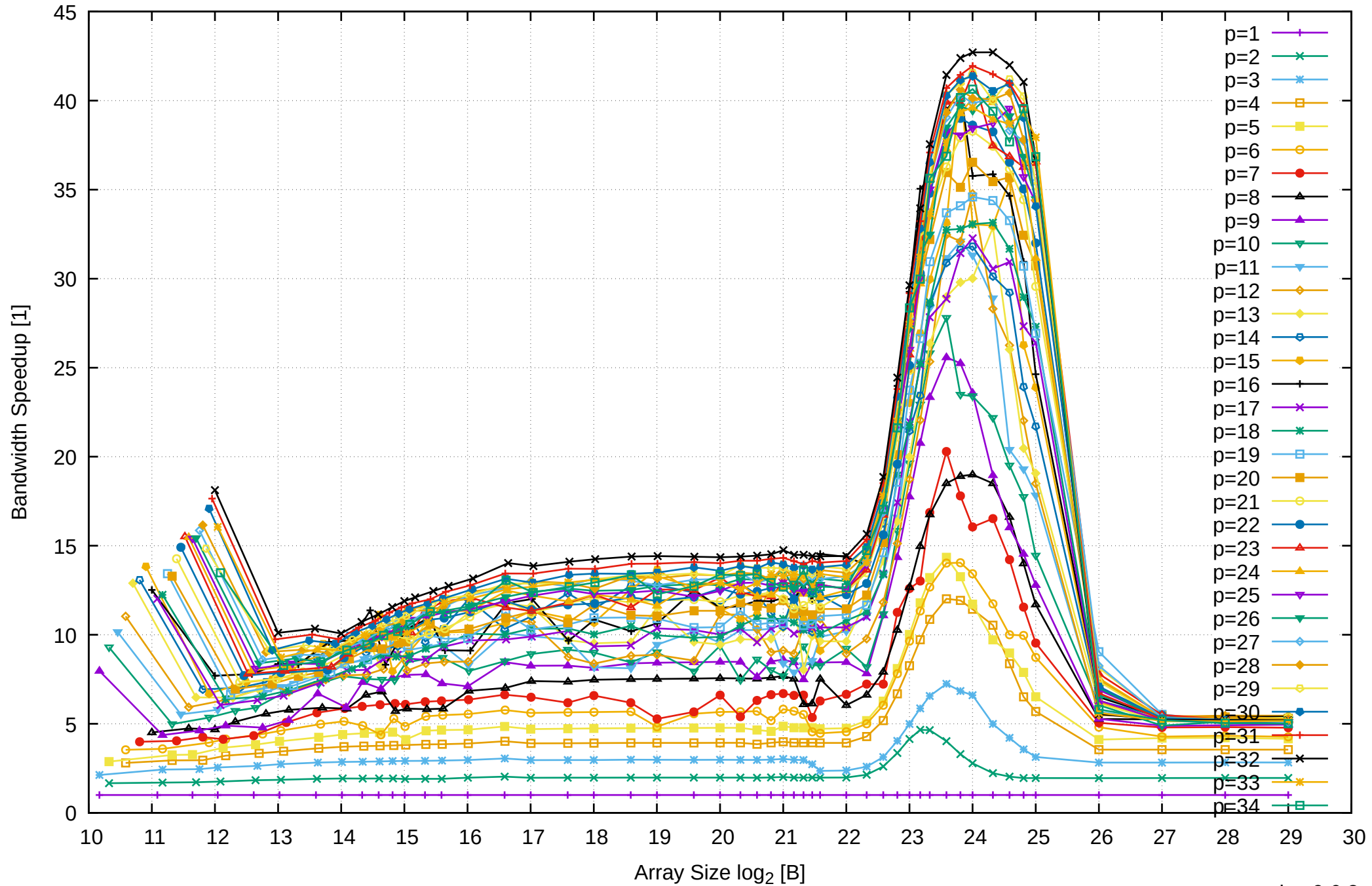
AMD Ryzen Threadripper 2950X 128GB - Speedup of Parallel Memory Bandwidth - ScanRead64IndexSimpleLoop
