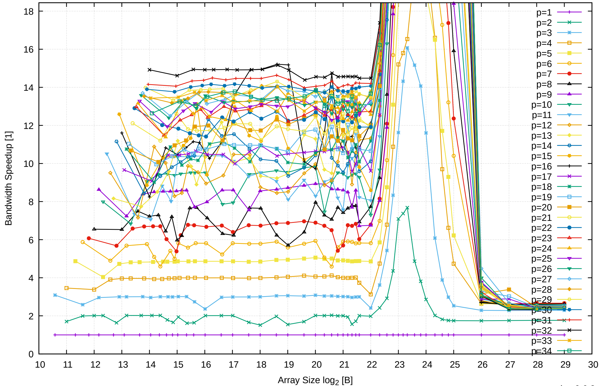
AMD Ryzen Threadripper 2950X 128GB - Speedup of Parallel Memory Bandwidth (enlarged) - ScanWrite256PtrSimpleLoop
