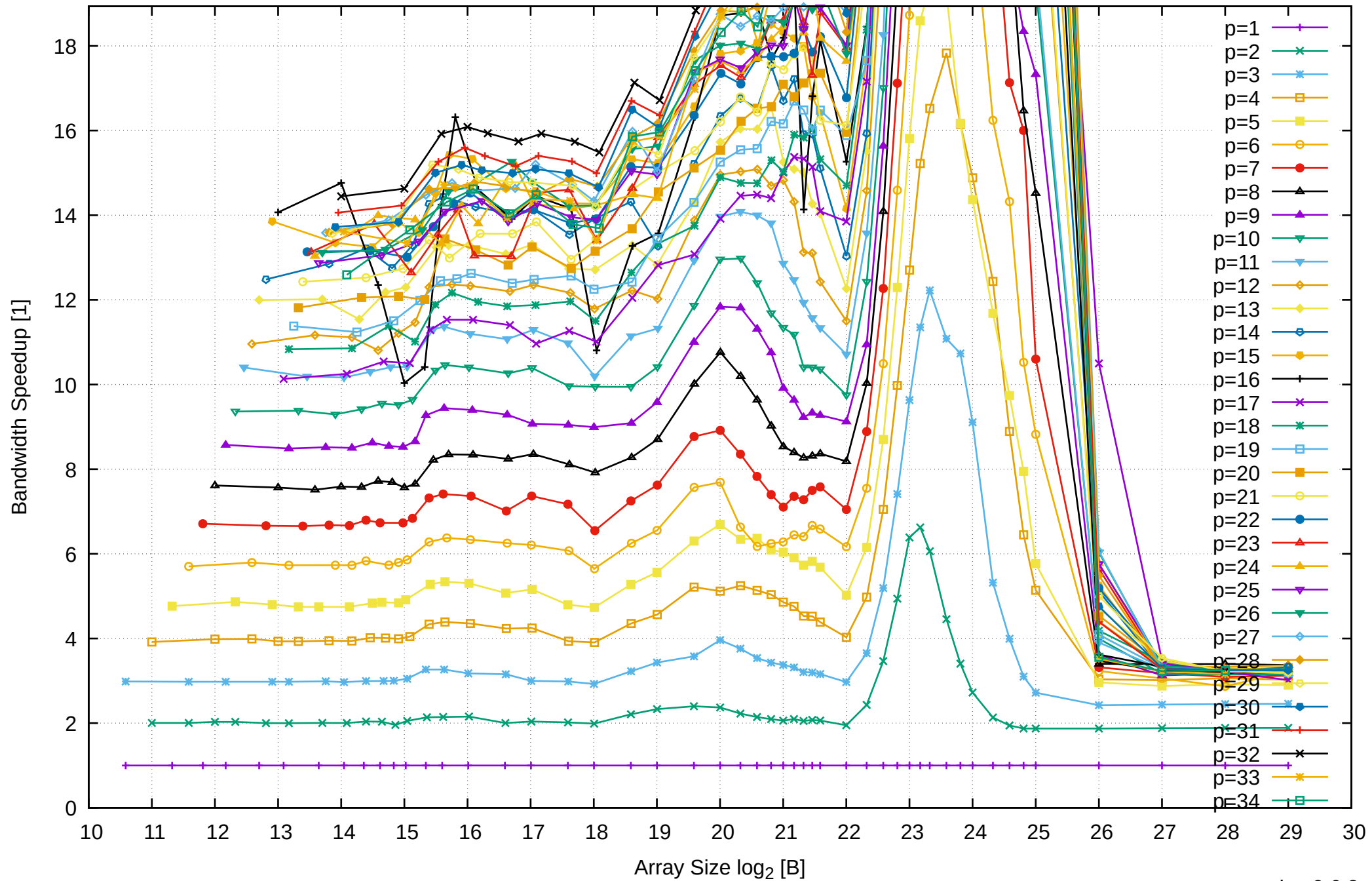
AMD Ryzen Threadripper 2950X 128GB - Speedup of Parallel Memory Bandwidth (enlarged) - ScanRead256PtrUnrollLoop
