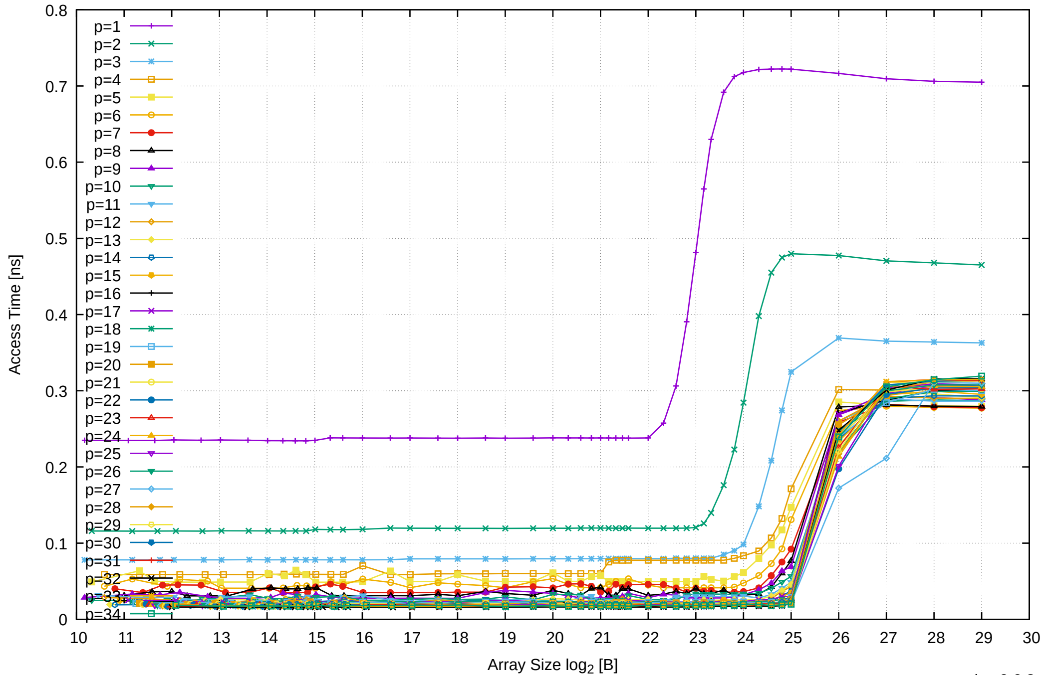
AMD Ryzen Threadripper 2950X 128GB - Parallel Memory Access Time - ScanWrite64PtrUnrollLoop
