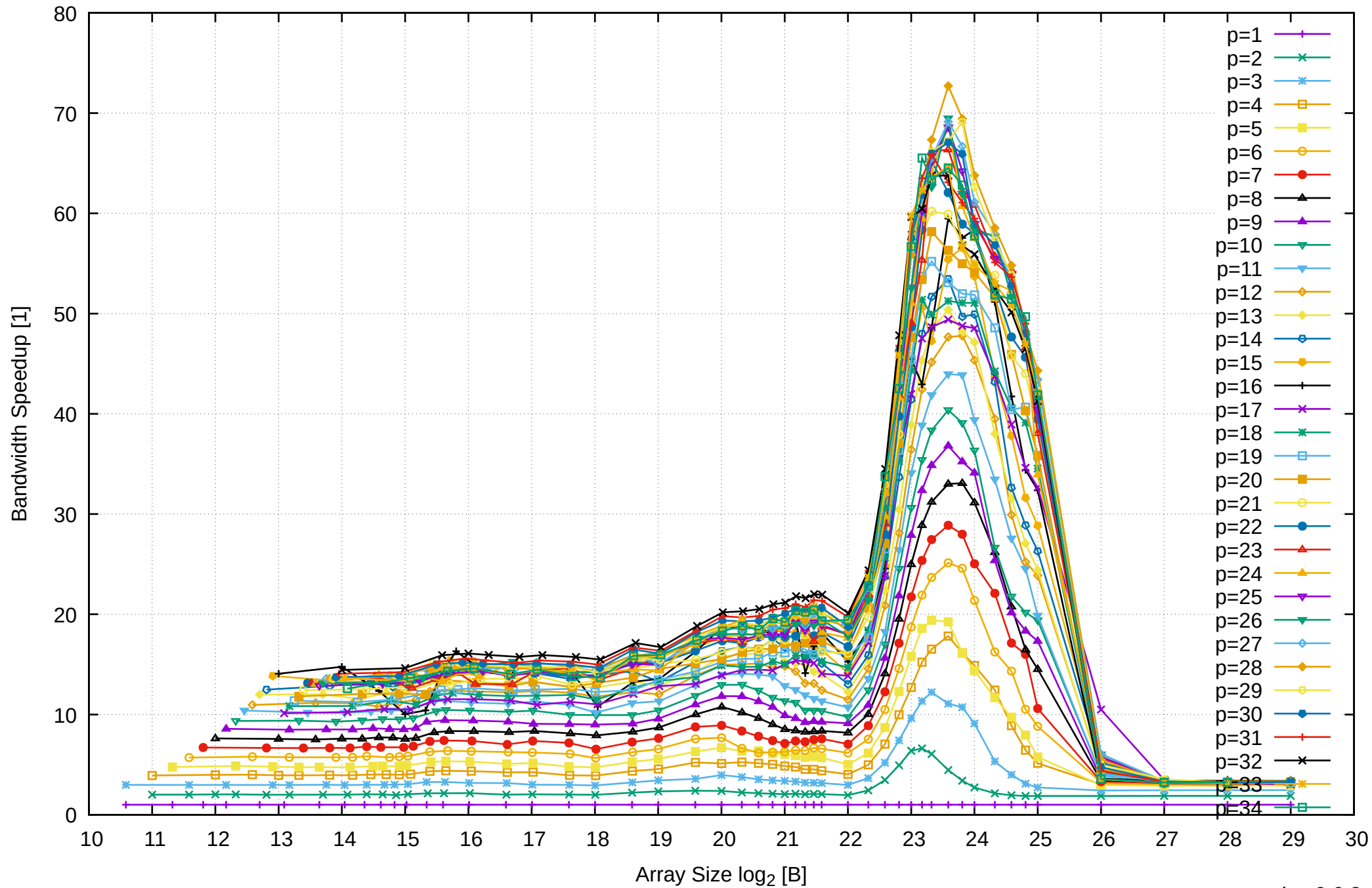
AMD Ryzen Threadripper 2950X 128GB - Speedup of Parallel Memory Bandwidth - ScanRead256PtrUnrollLoop
