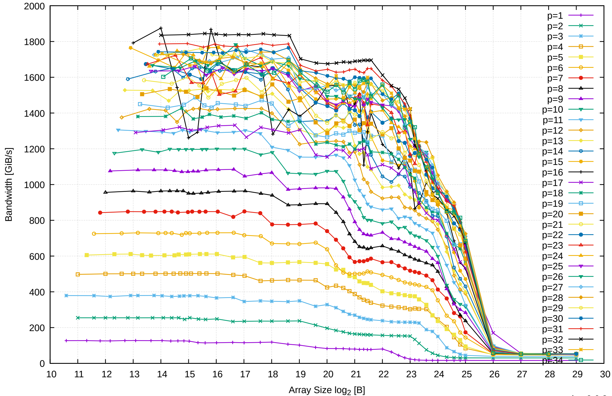
AMD Ryzen Threadripper 2950X 128GB - Parallel Memory Bandwidth - ScanRead256PtrUnrollLoop
