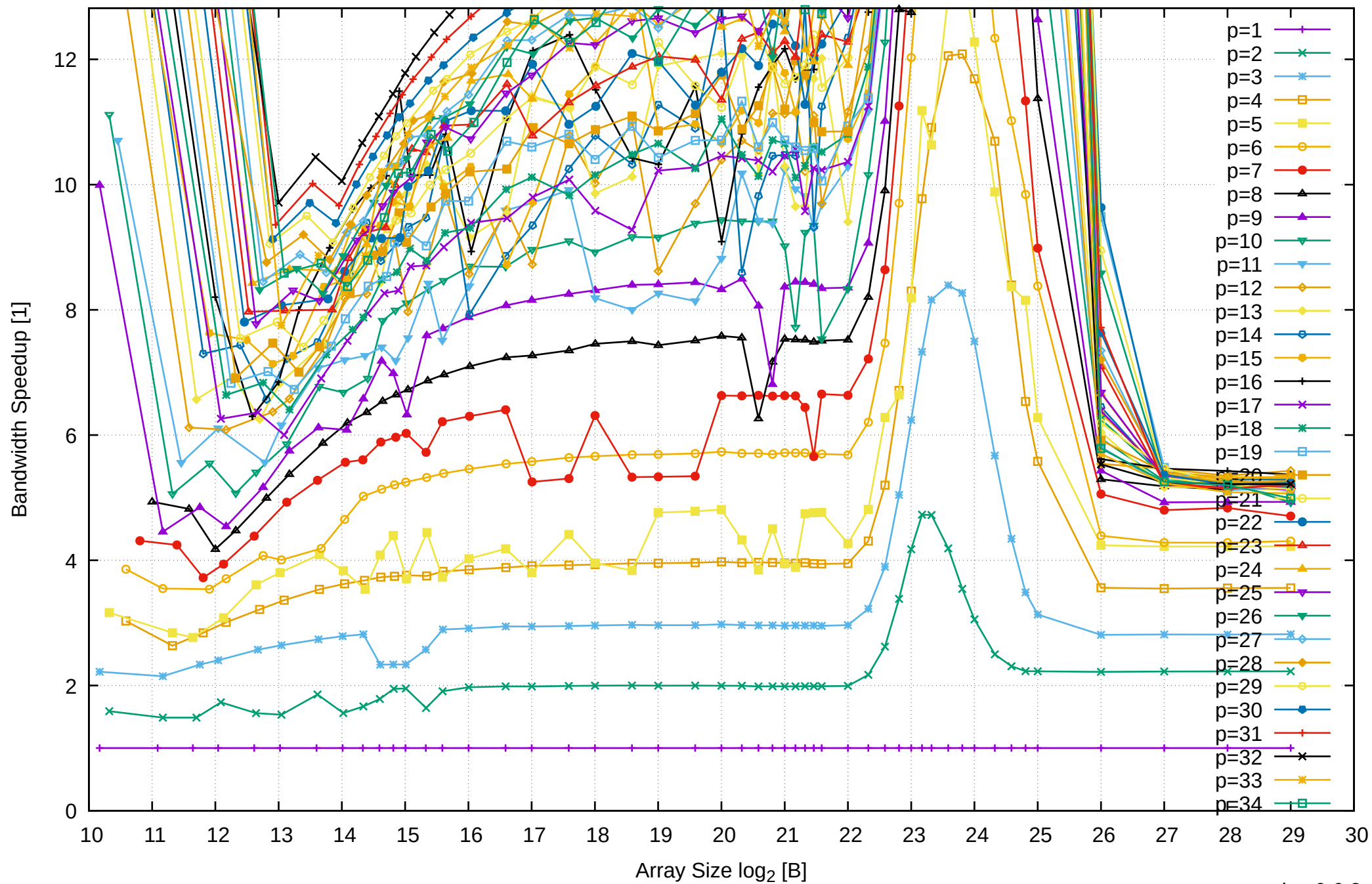
AMD Ryzen Threadripper 2950X 128GB - Speedup of Parallel Memory Bandwidth (enlarged) - ScanRead64PtrSimpleLoop
