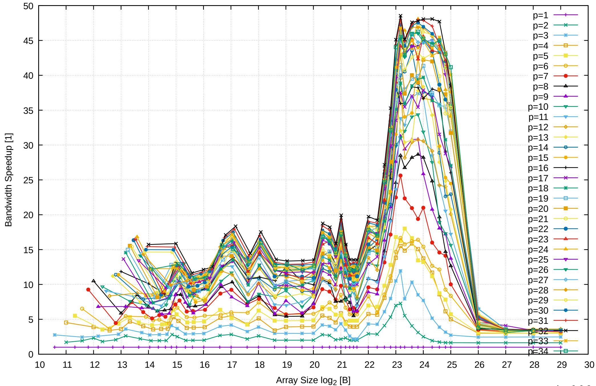
AMD Ryzen Threadripper 2950X 128GB - Speedup of Parallel Memory Bandwidth - ScanRead256PtrSimpleLoop
