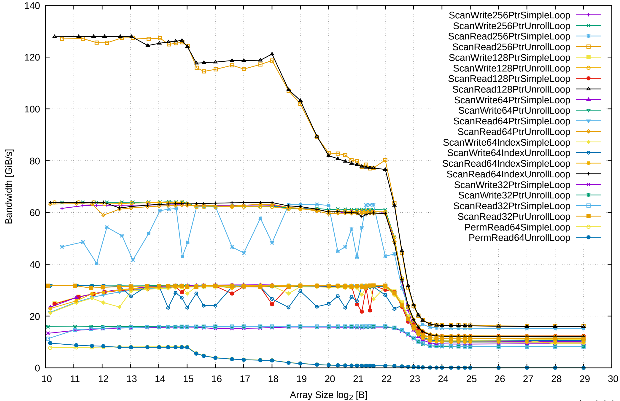
AMD Ryzen Threadripper 2950X 128GB - One Thread Memory Bandwidth
