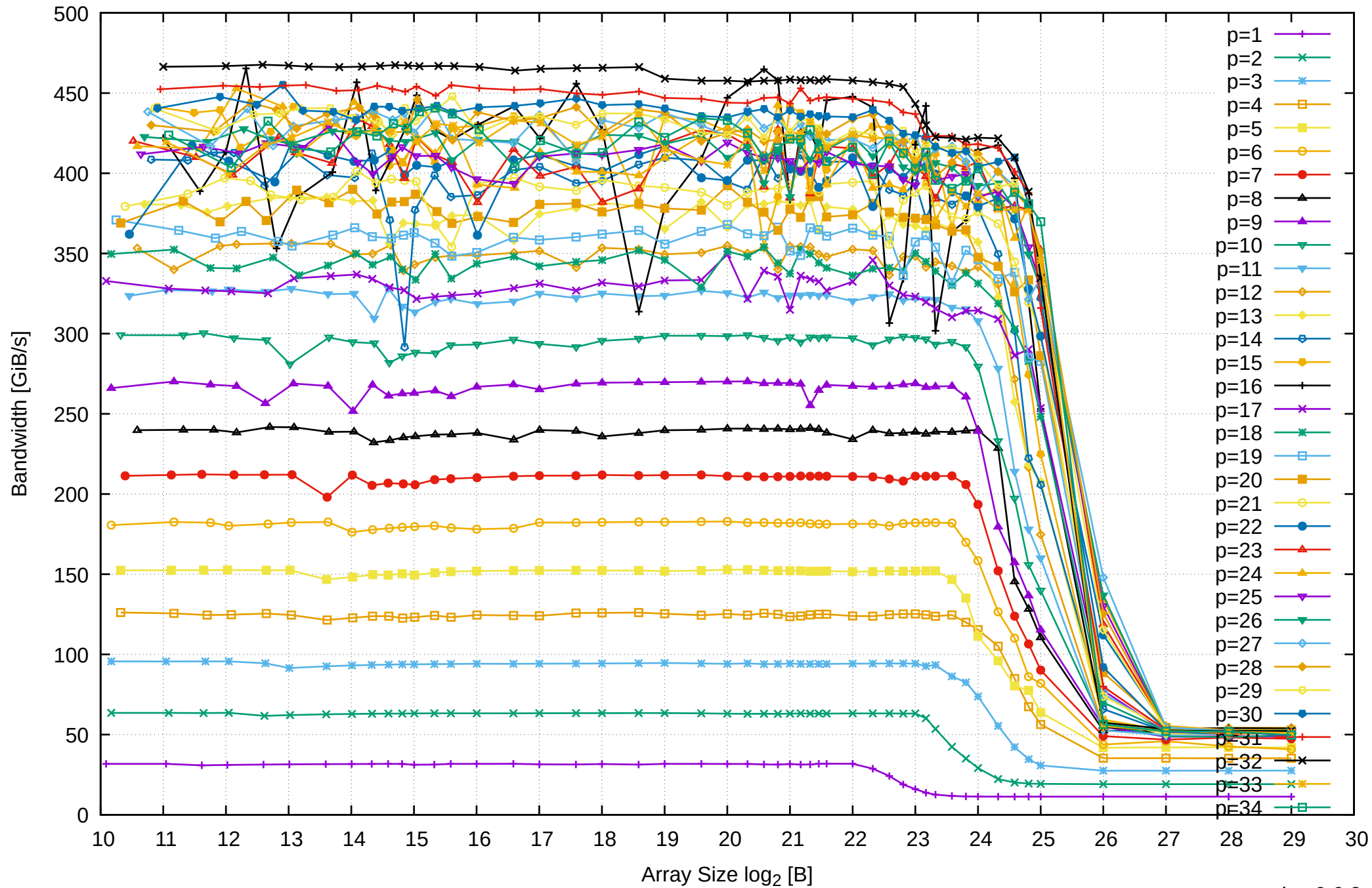
AMD Ryzen Threadripper 2950X 128GB - Parallel Memory Bandwidth - ScanRead32PtrUnrollLoop
