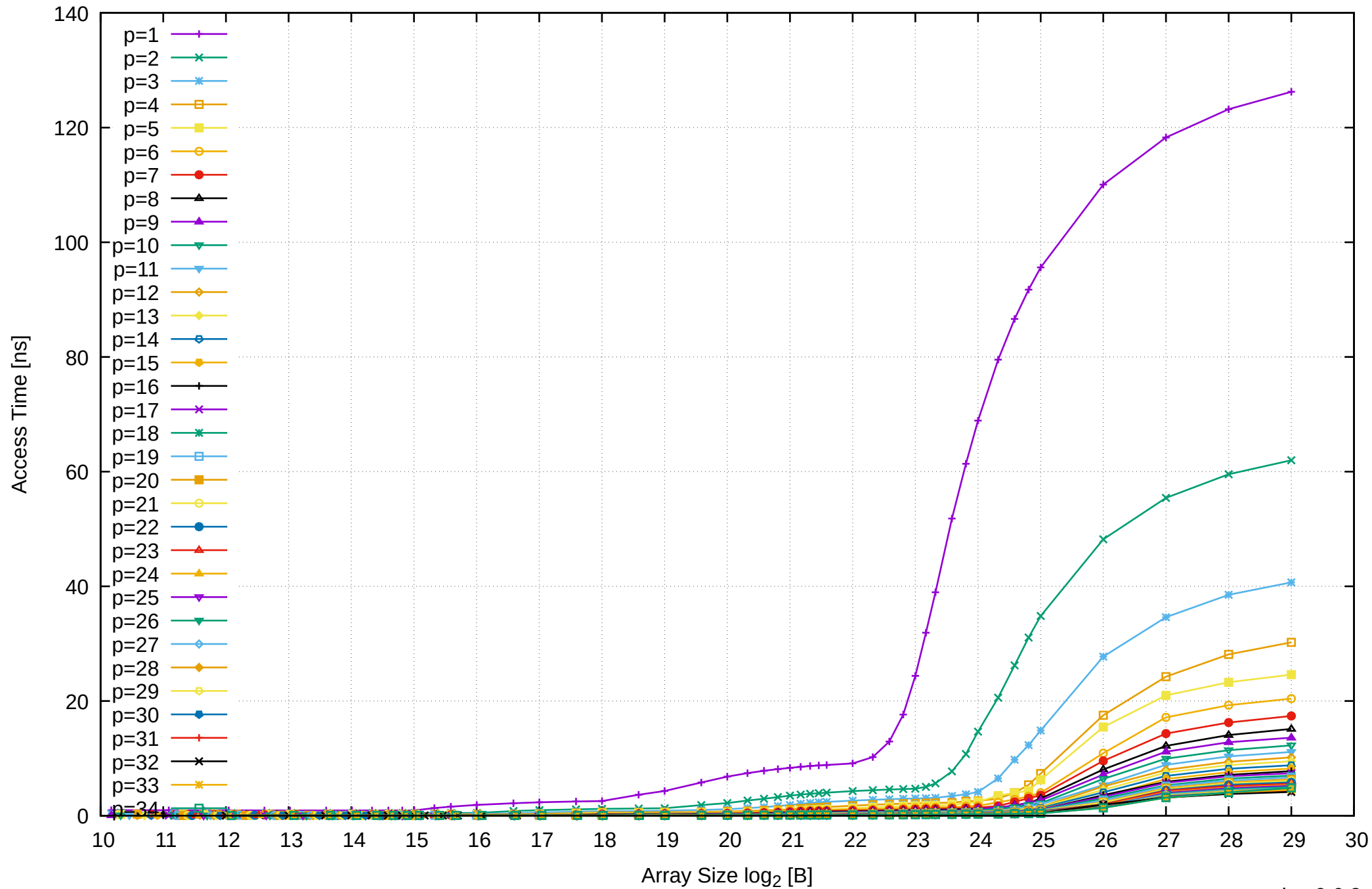
AMD Ryzen Threadripper 2950X 128GB - Parallel Memory Access Time - PermRead64SimpleLoop
