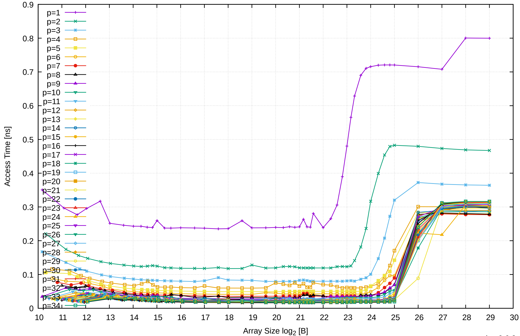
AMD Ryzen Threadripper 2950X 128GB - Parallel Memory Access Time - ScanWrite64IndexSimpleLoop
