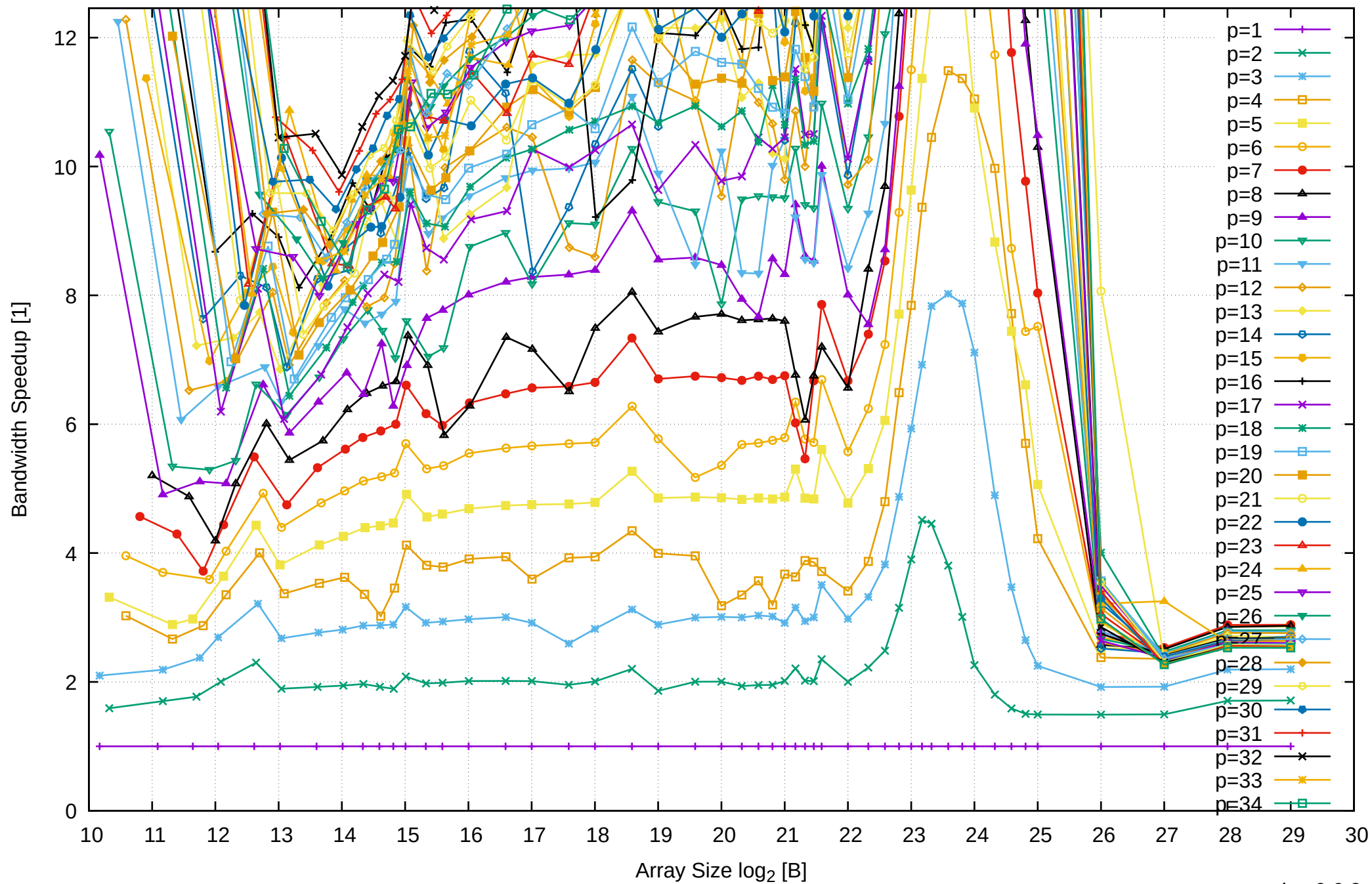
AMD Ryzen Threadripper 2950X 128GB - Speedup of Parallel Memory Bandwidth (enlarged) - ScanWrite64IndexSimpleLoop
