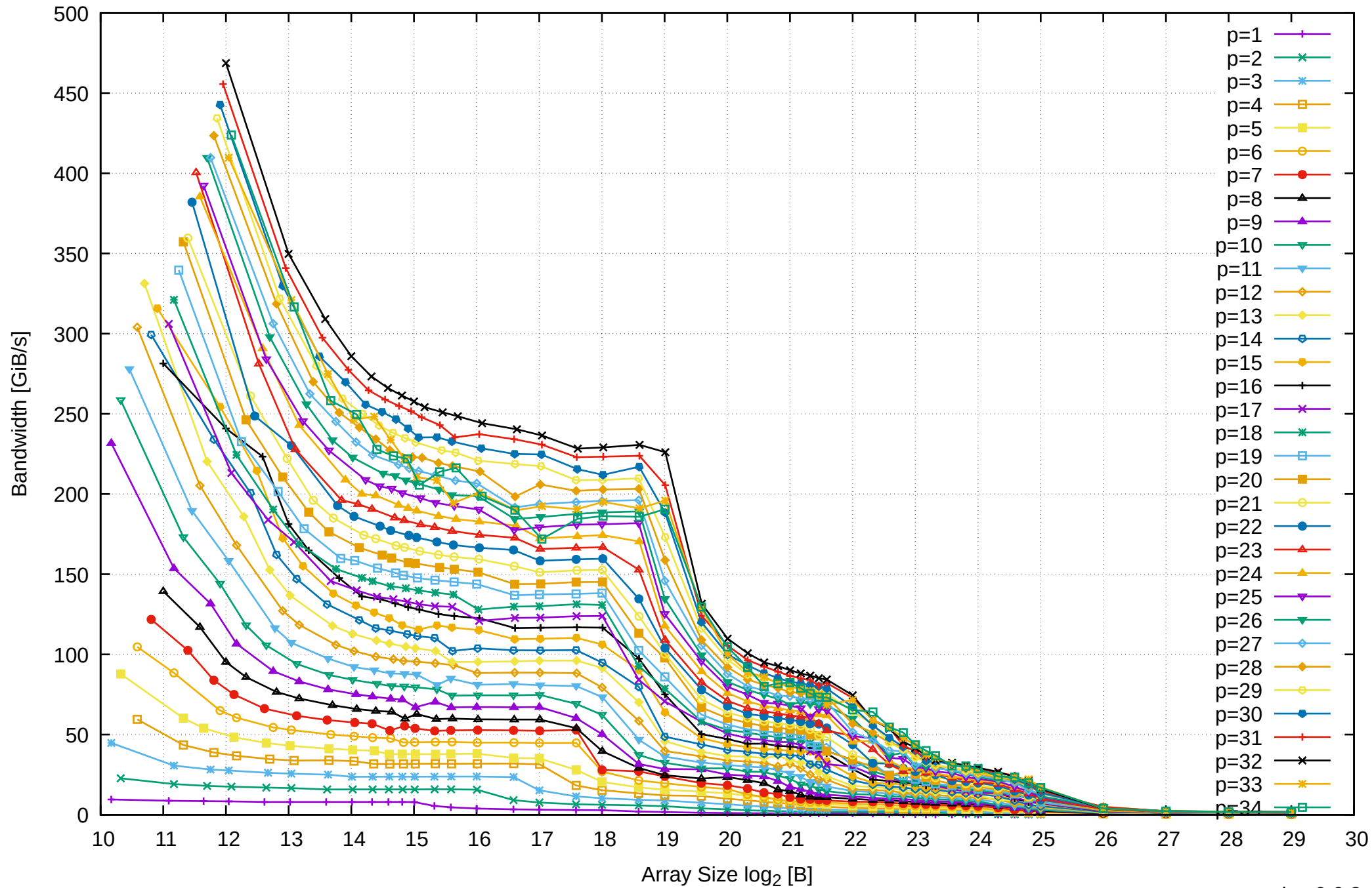
AMD Ryzen Threadripper 2950X 128GB - Parallel Memory Bandwidth - PermRead64UnrollLoop
