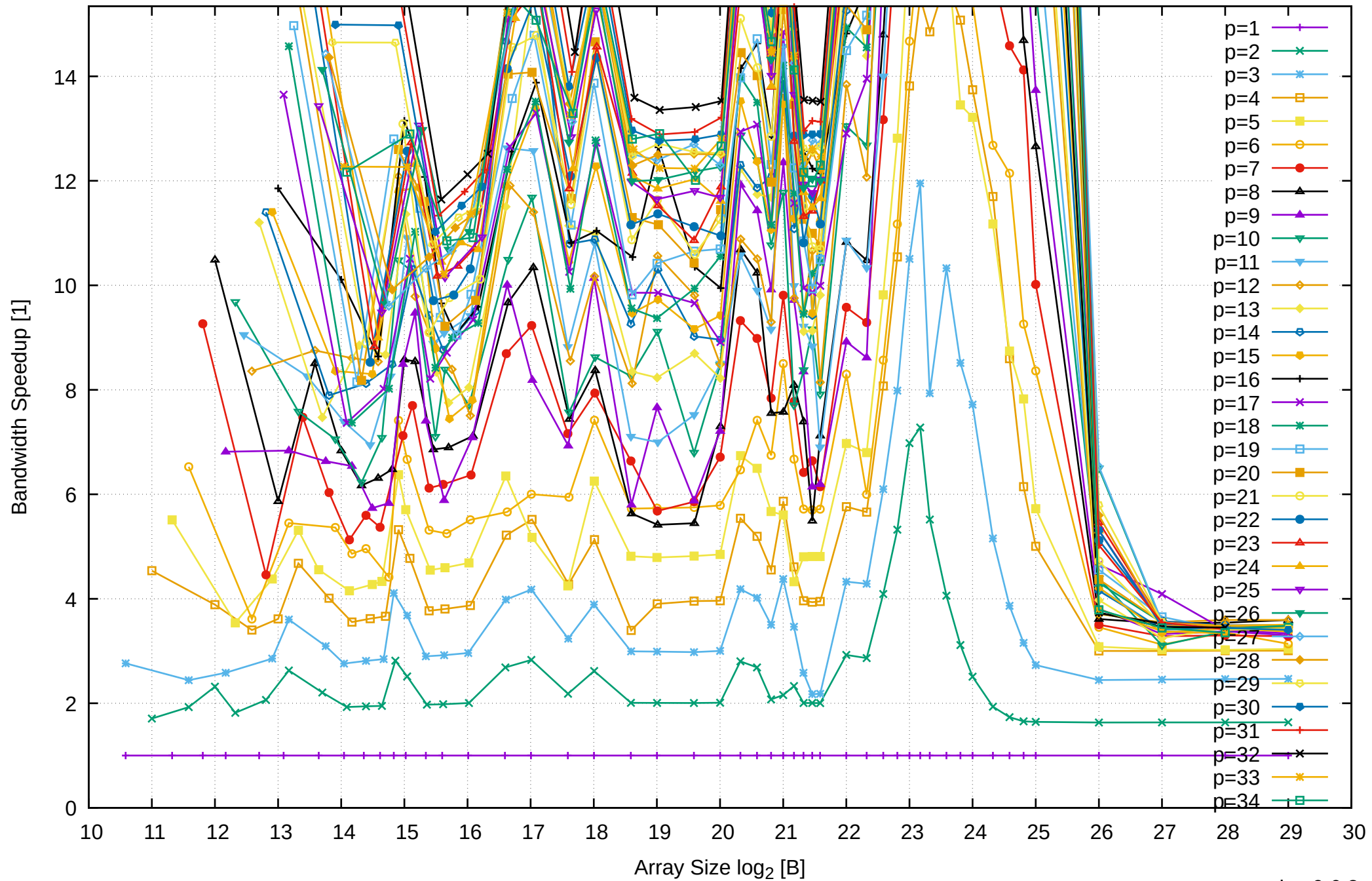
AMD Ryzen Threadripper 2950X 128GB - Speedup of Parallel Memory Bandwidth (enlarged) - ScanRead256PtrSimpleLoop
