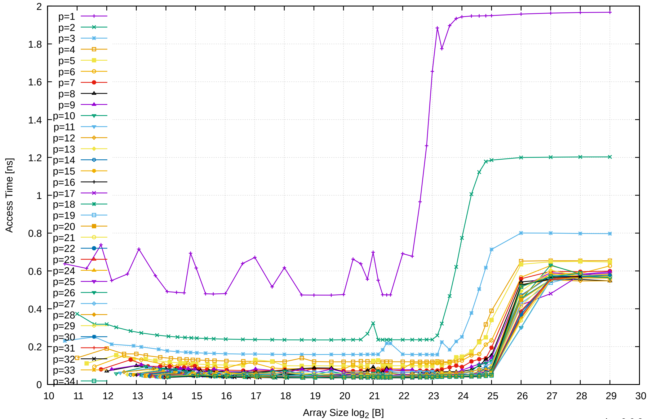
AMD Ryzen Threadripper 2950X 128GB - Parallel Memory Access Time - ScanRead256PtrSimpleLoop
