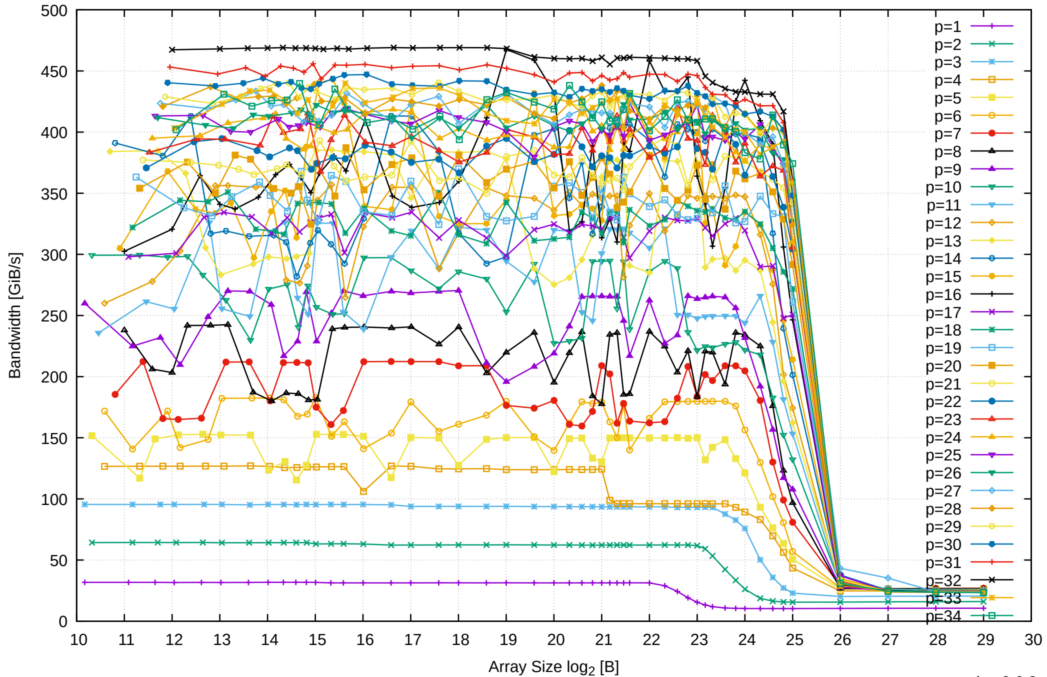
AMD Ryzen Threadripper 2950X 128GB - Parallel Memory Bandwidth - ScanWrite64PtrUnrollLoop
