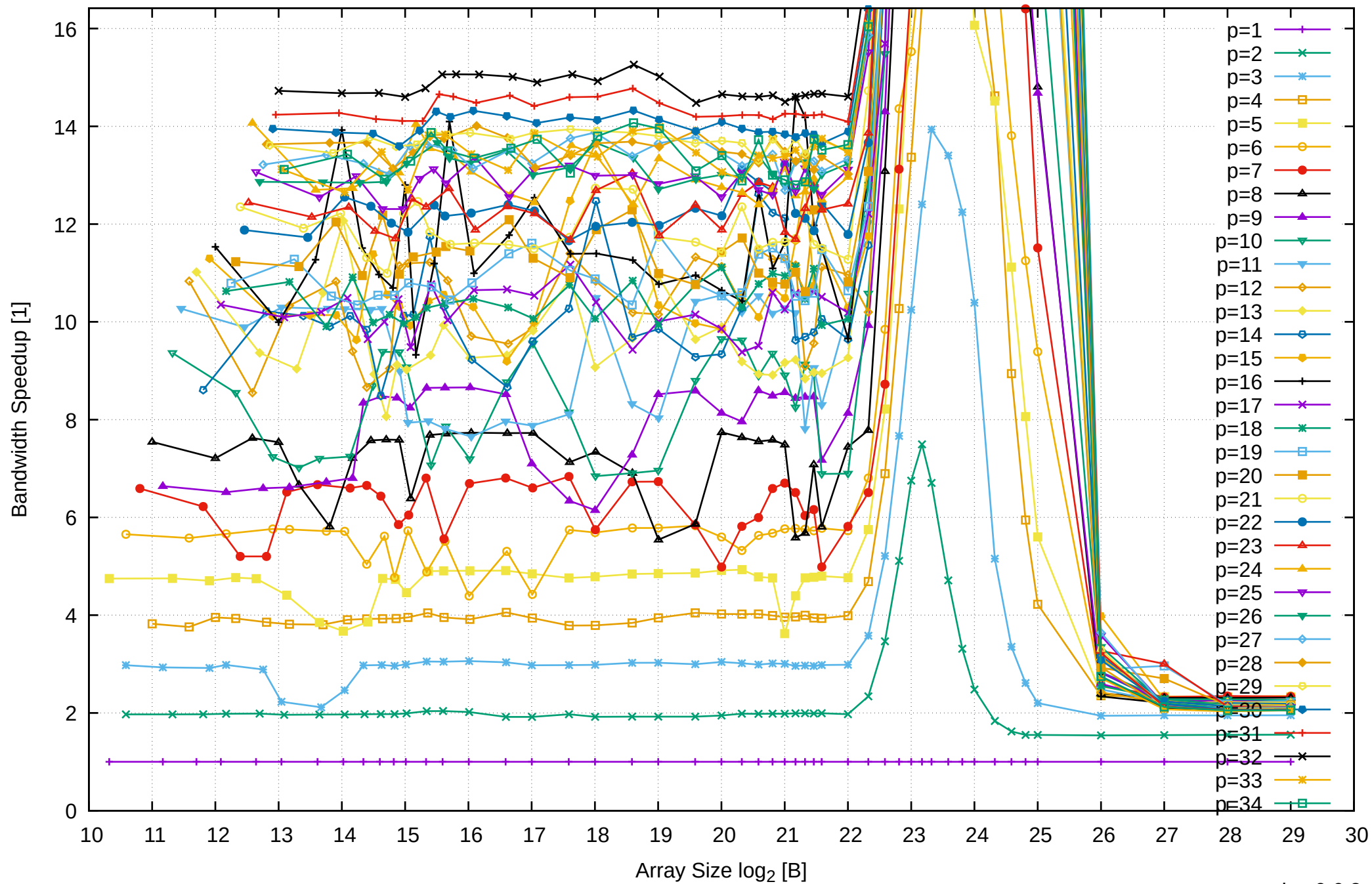
AMD Ryzen Threadripper 2950X 128GB - Speedup of Parallel Memory Bandwidth (enlarged) - ScanWrite128PtrUnrollLoop
