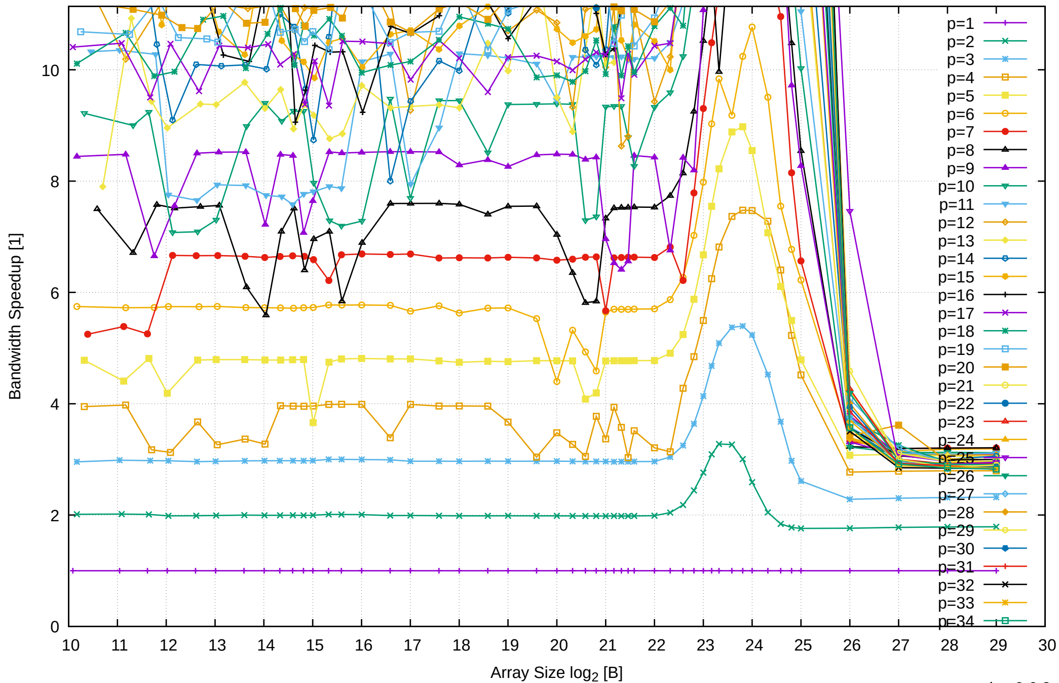
AMD Ryzen Threadripper 2950X 128GB - Speedup of Parallel Memory Bandwidth (enlarged) - ScanWrite32PtrUnrollLoop
