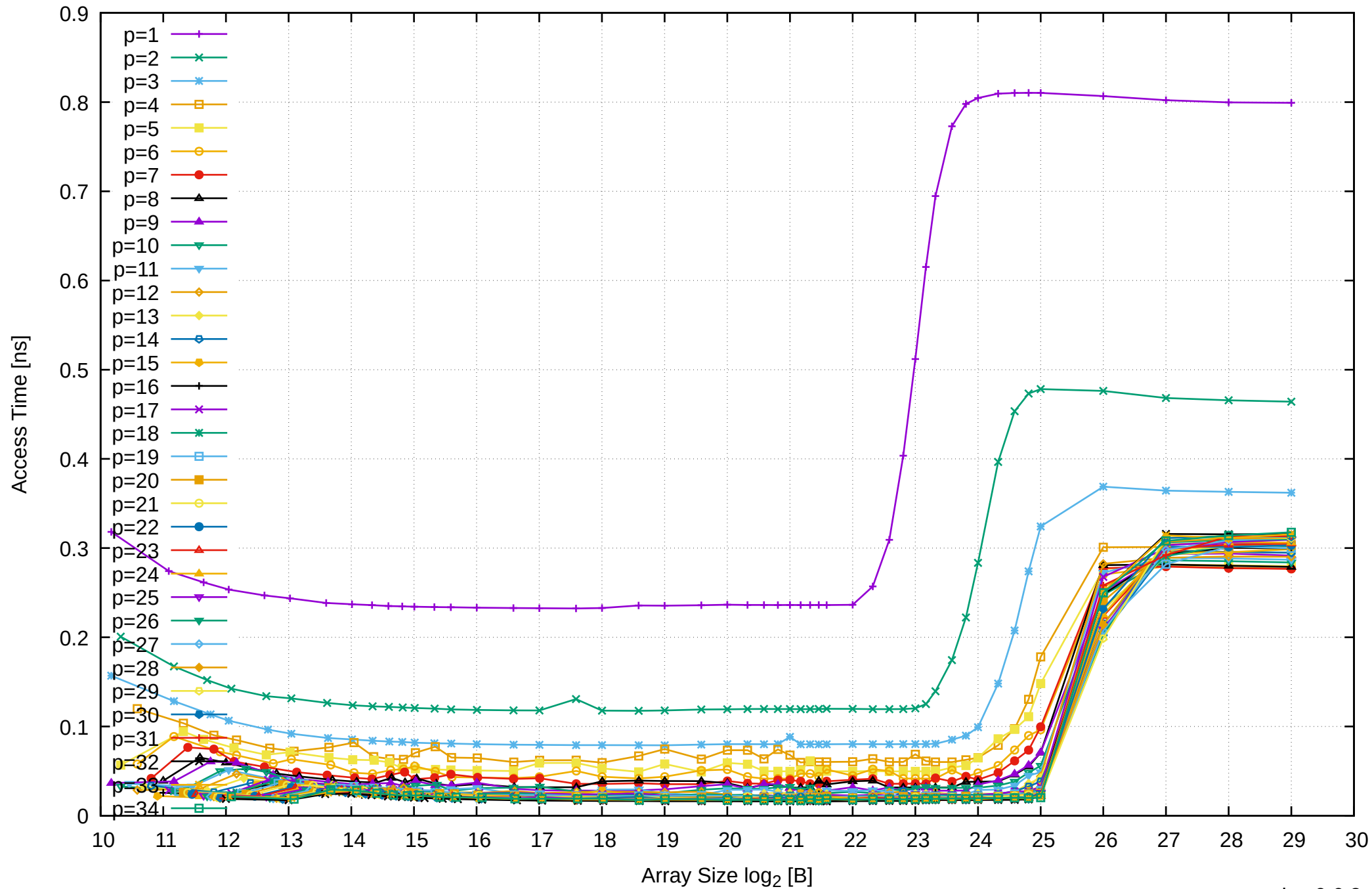
AMD Ryzen Threadripper 2950X 128GB - Parallel Memory Access Time - ScanWrite64PtrSimpleLoop
