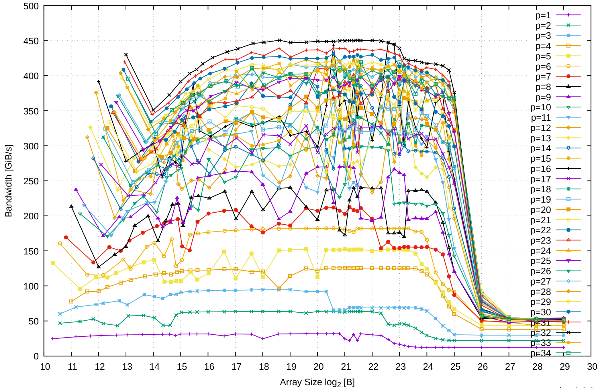
AMD Ryzen Threadripper 2950X 128GB - Parallel Memory Bandwidth - ScanRead128PtrSimpleLoop
