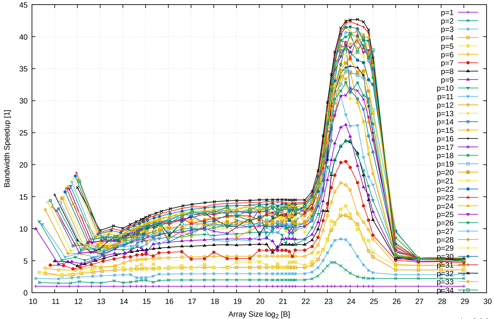
AMD Ryzen Threadripper 2950X 128GB - Speedup of Parallel Memory Bandwidth - ScanRead64PtrSimpleLoop
