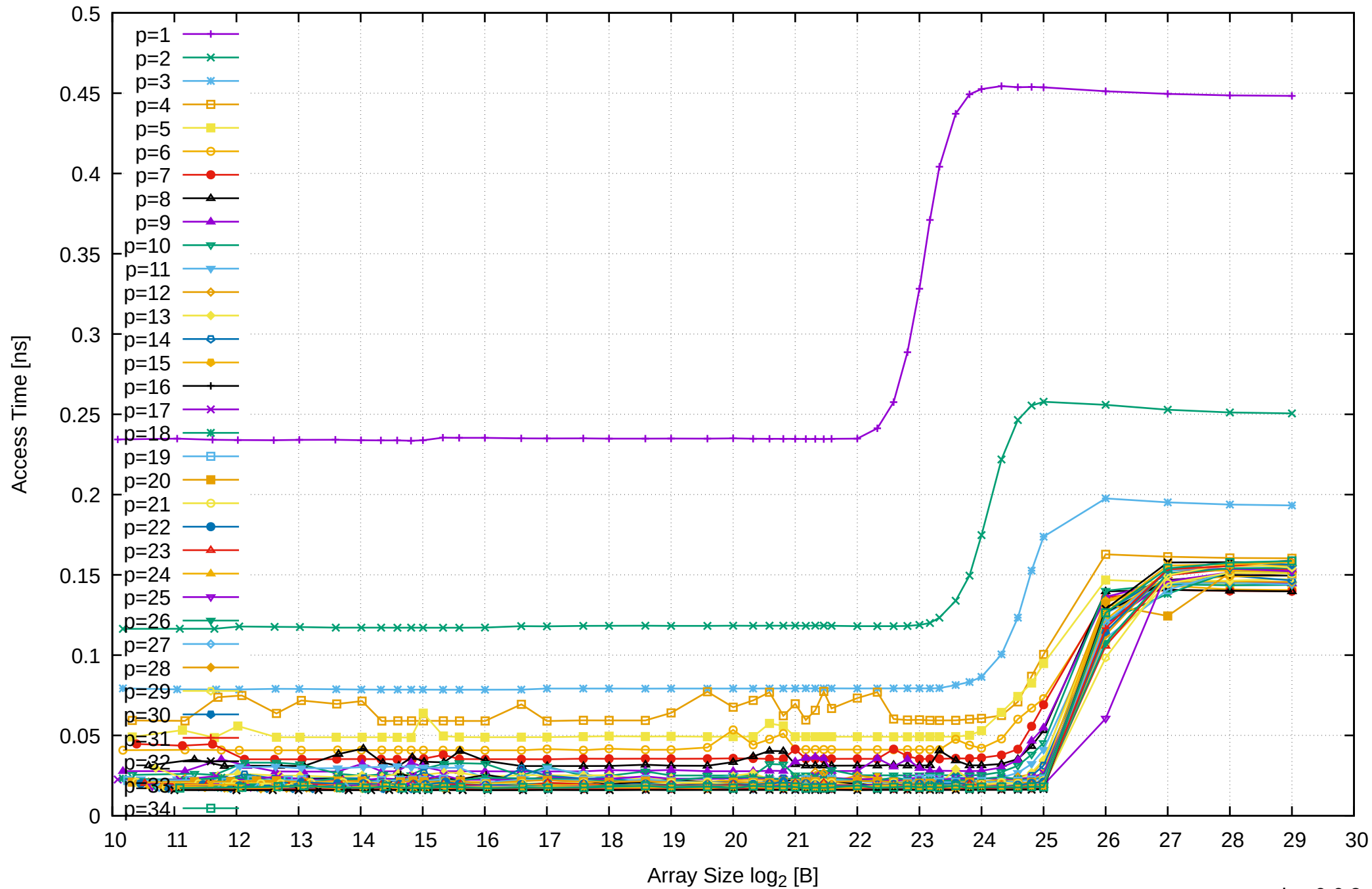
AMD Ryzen Threadripper 2950X 128GB - Parallel Memory Access Time - ScanWrite32PtrUnrollLoop
