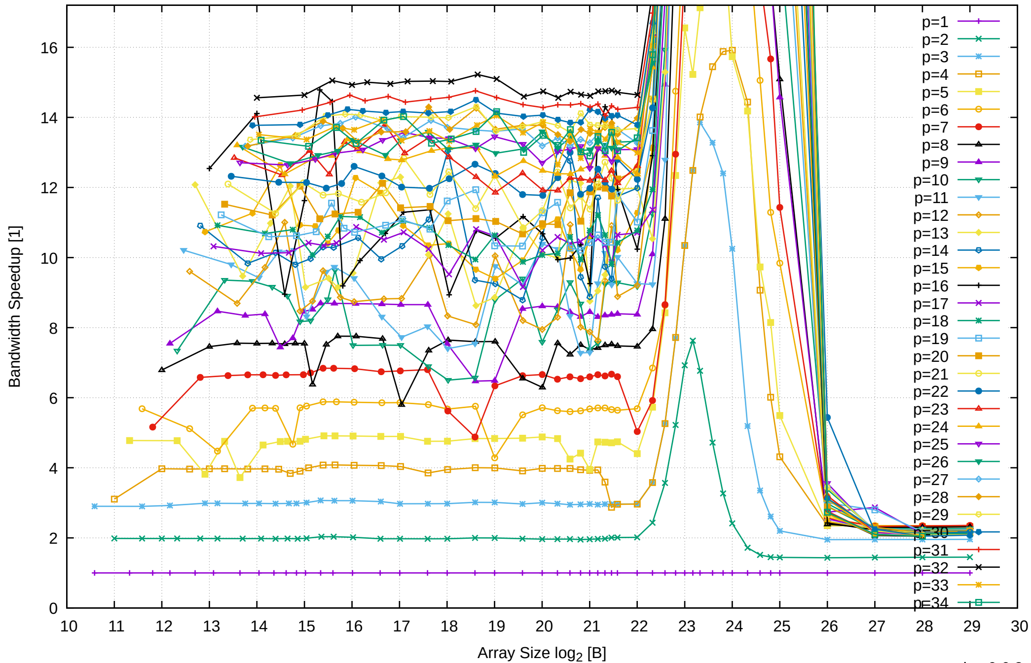
AMD Ryzen Threadripper 2950X 128GB - Speedup of Parallel Memory Bandwidth (enlarged) - ScanWrite256PtrUnrollLoop
