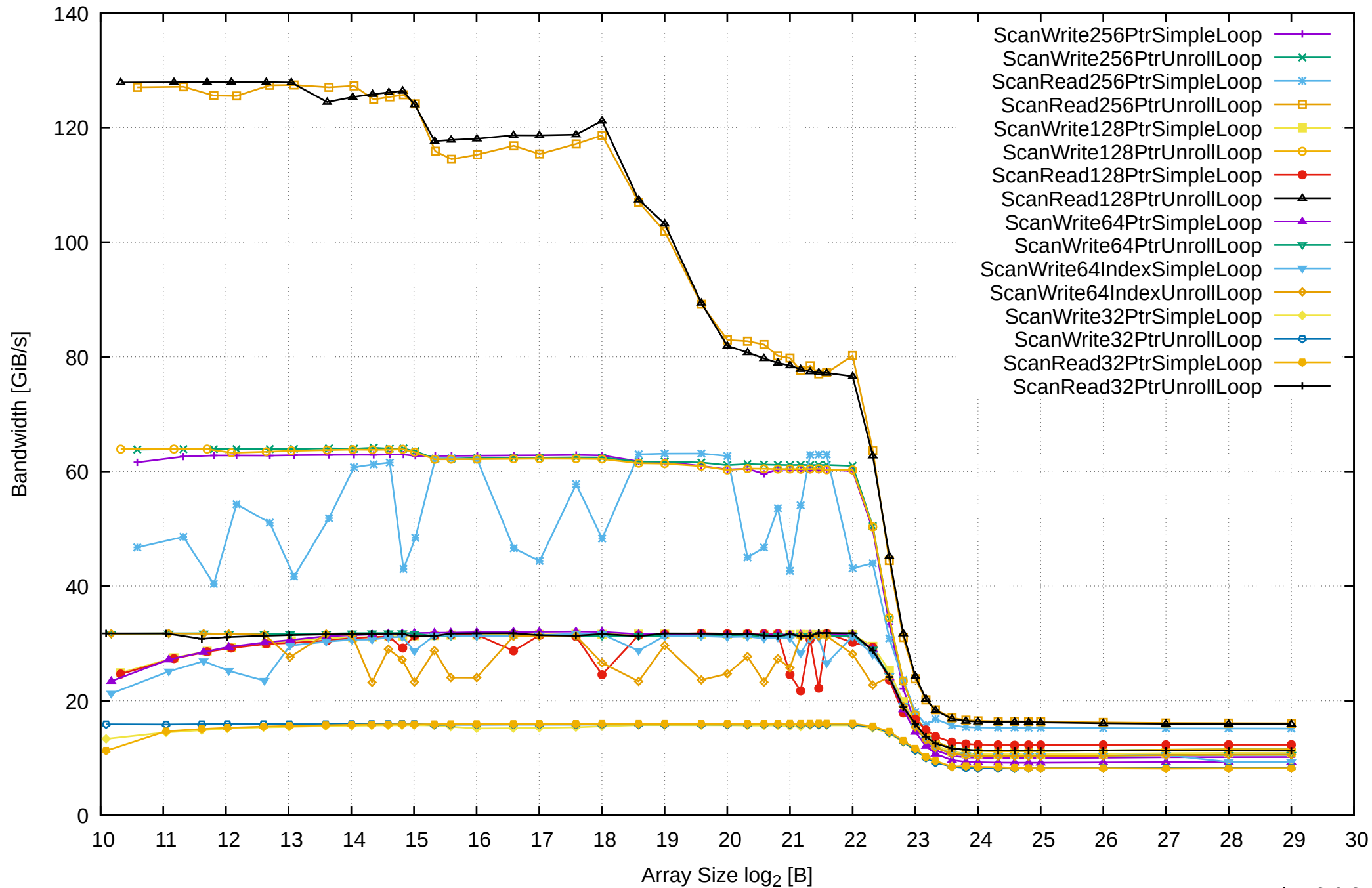
AMD Ryzen Threadripper 2950X 128GB - One Thread Memory Bandwidth (only 64-bit Reads)
