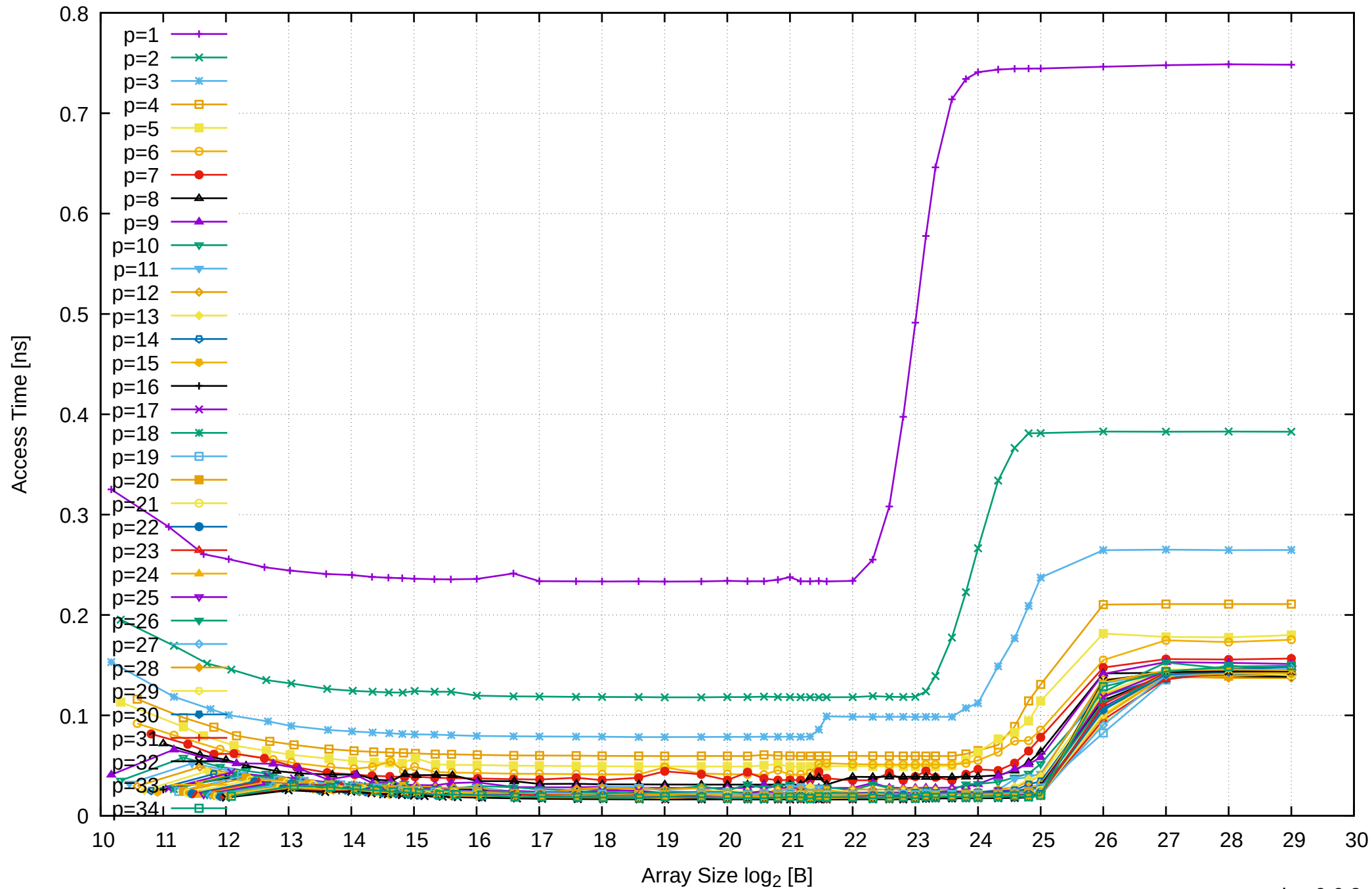
AMD Ryzen Threadripper 2950X 128GB - Parallel Memory Access Time - ScanRead64IndexSimpleLoop
