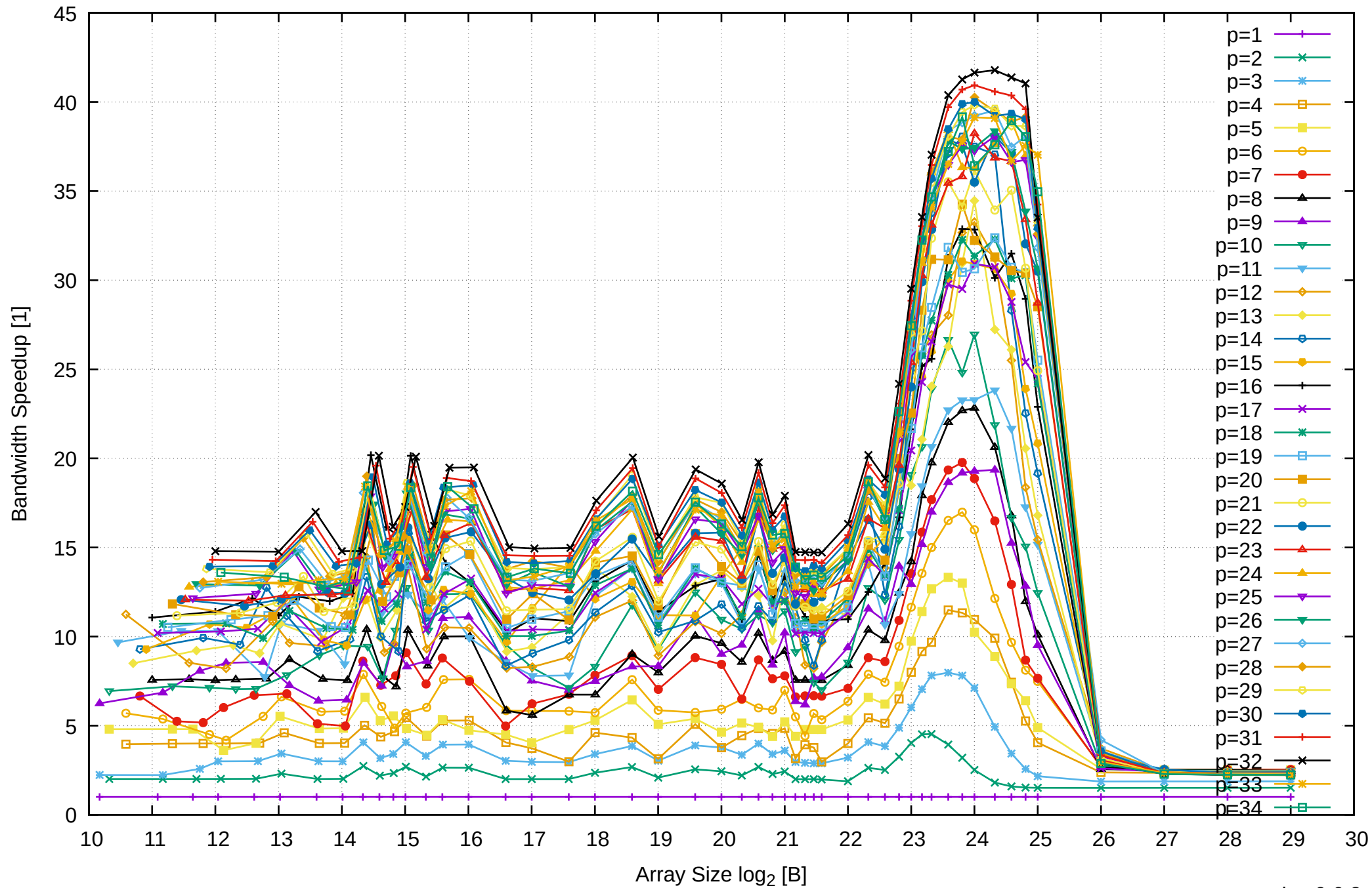
AMD Ryzen Threadripper 2950X 128GB - Speedup of Parallel Memory Bandwidth - ScanWrite64IndexUnrollLoop
