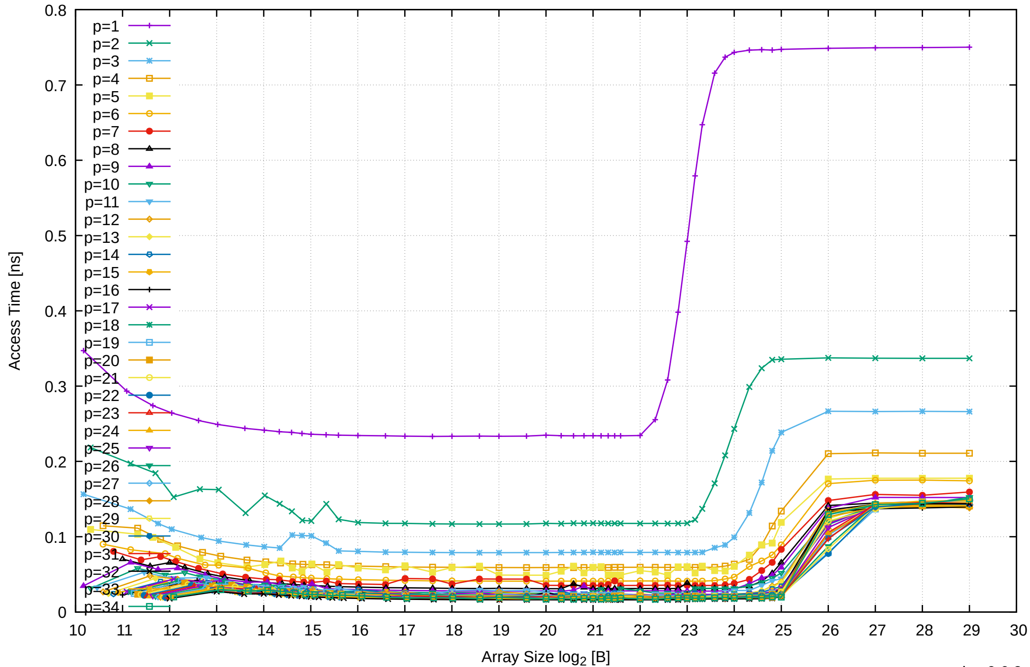
AMD Ryzen Threadripper 2950X 128GB - Parallel Memory Access Time - ScanRead64PtrSimpleLoop
