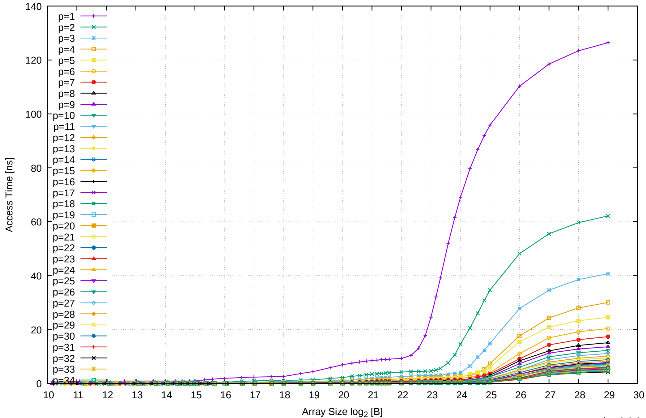
AMD Ryzen Threadripper 2950X 128GB - Parallel Memory Access Time - PermRead64UnrollLoop
