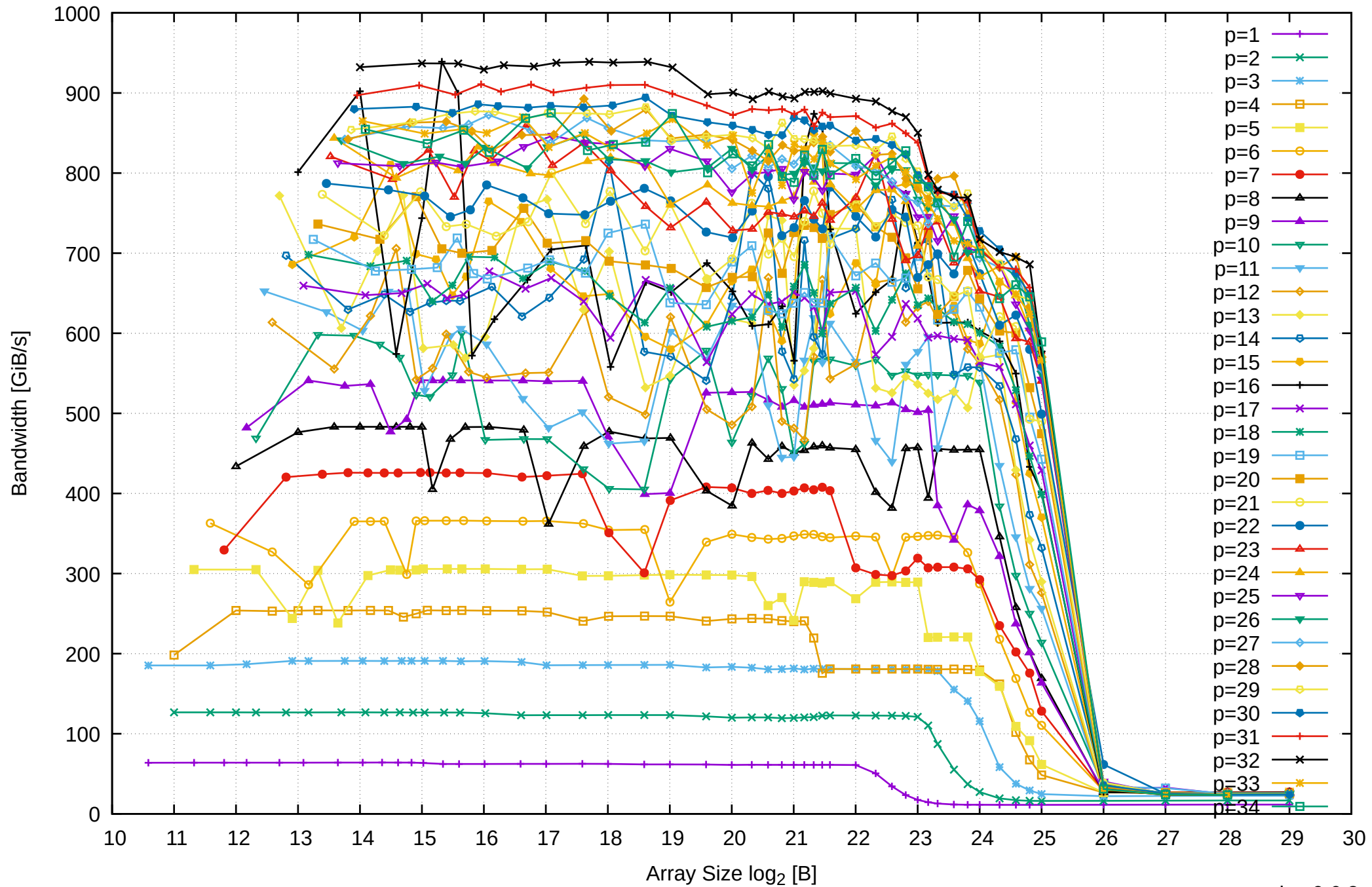
AMD Ryzen Threadripper 2950X 128GB - Parallel Memory Bandwidth - ScanWrite256PtrUnrollLoop
