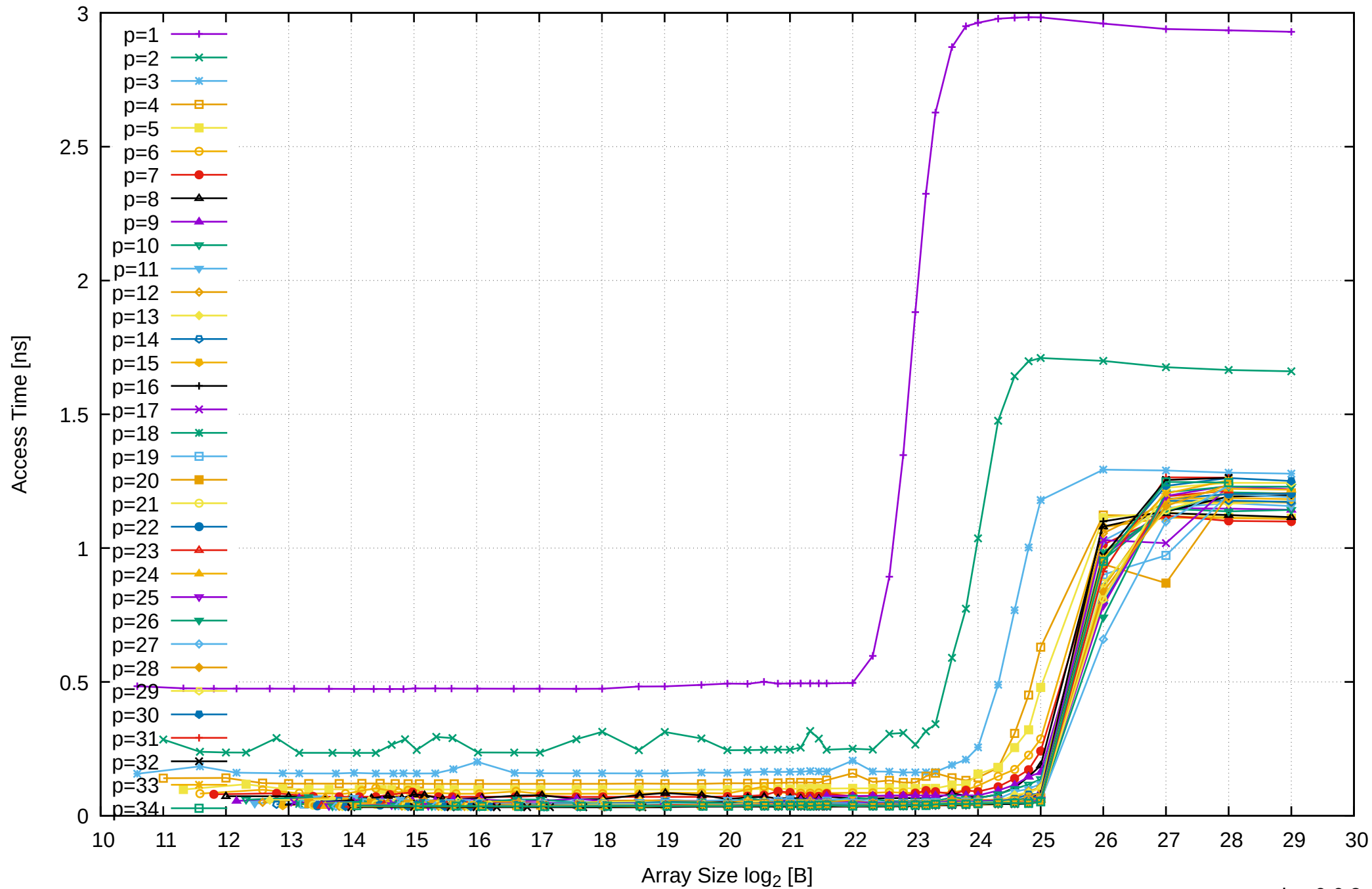
AMD Ryzen Threadripper 2950X 128GB - Parallel Memory Access Time - ScanWrite256PtrSimpleLoop
