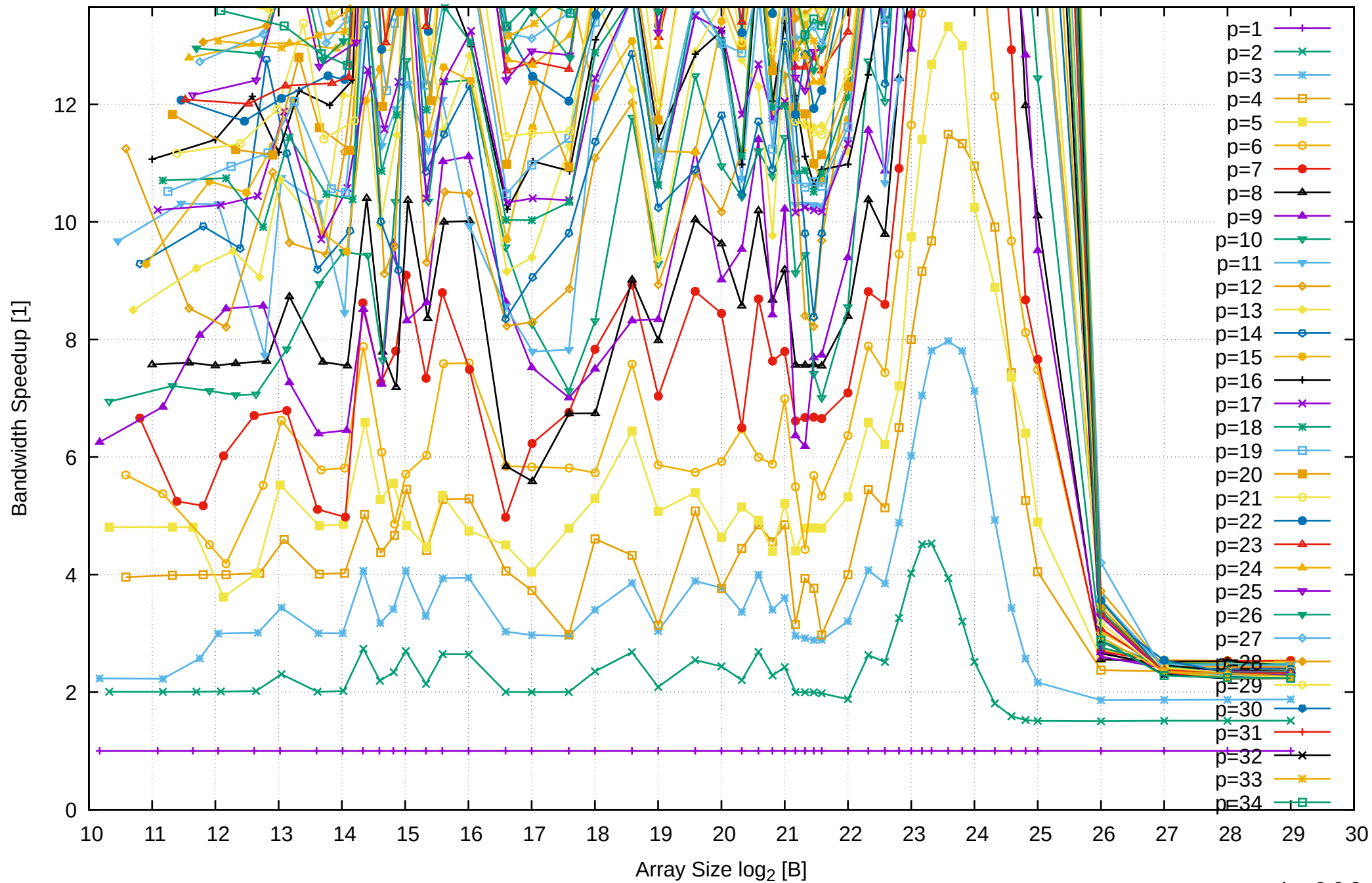
AMD Ryzen Threadripper 2950X 128GB - Speedup of Parallel Memory Bandwidth (enlarged) - ScanWrite64IndexUnrollLoop
