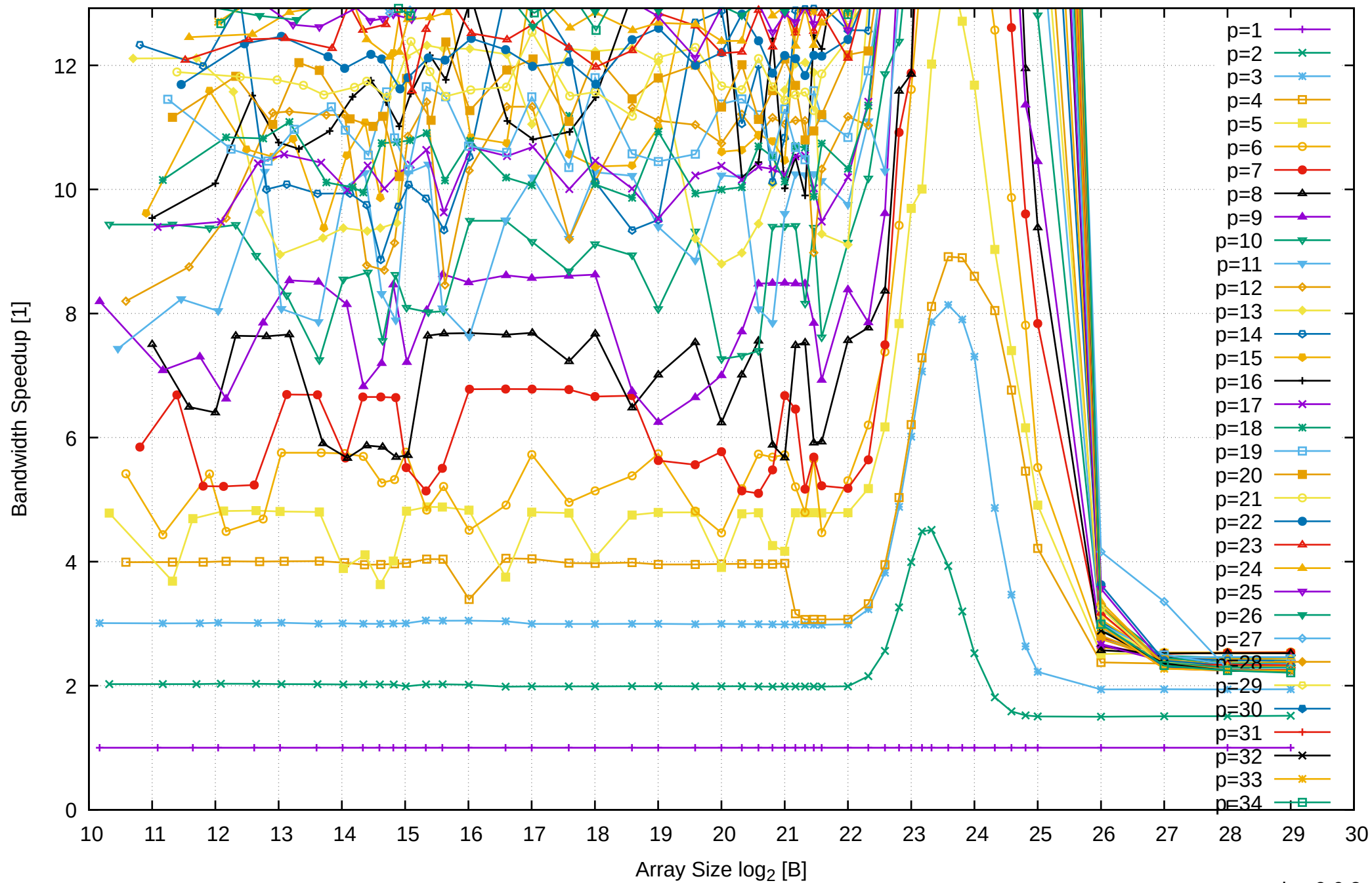
AMD Ryzen Threadripper 2950X 128GB - Speedup of Parallel Memory Bandwidth (enlarged) - ScanWrite64PtrUnrollLoop
