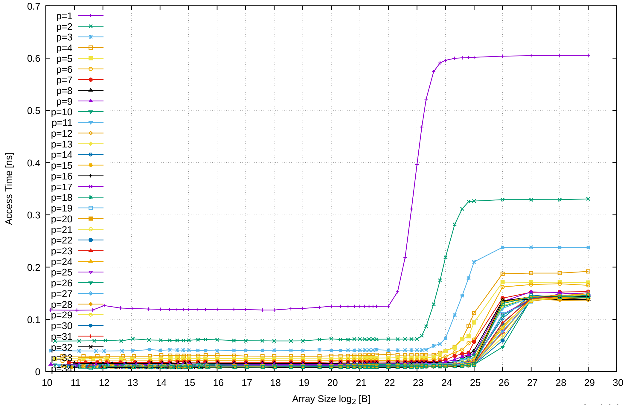
AMD Ryzen Threadripper 2950X 128GB - Parallel Memory Access Time - ScanRead64PtrUnrollLoop
