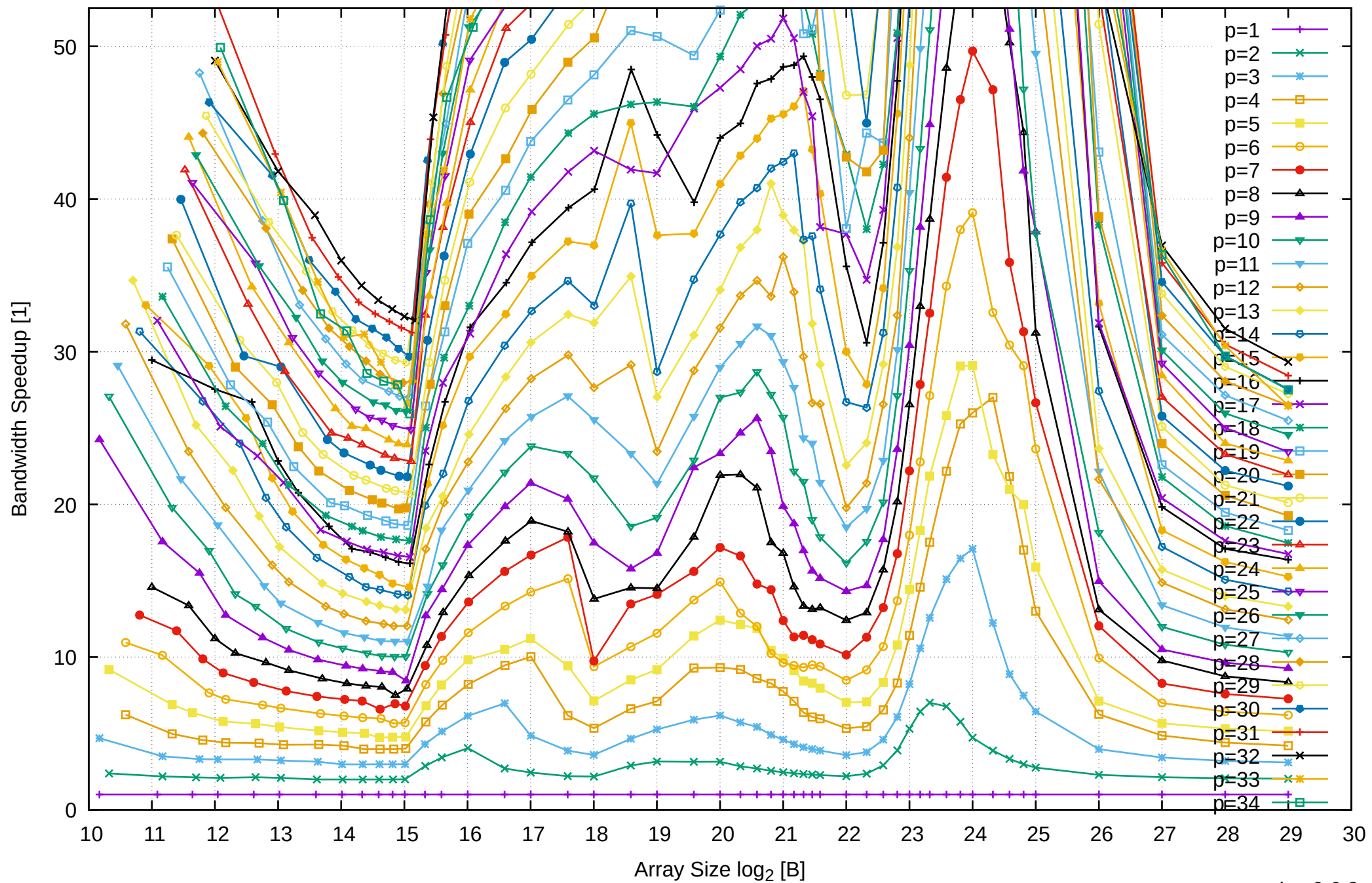
AMD Ryzen Threadripper 2950X 128GB - Speedup of Parallel Memory Bandwidth (enlarged) - PermRead64UnrollLoop
