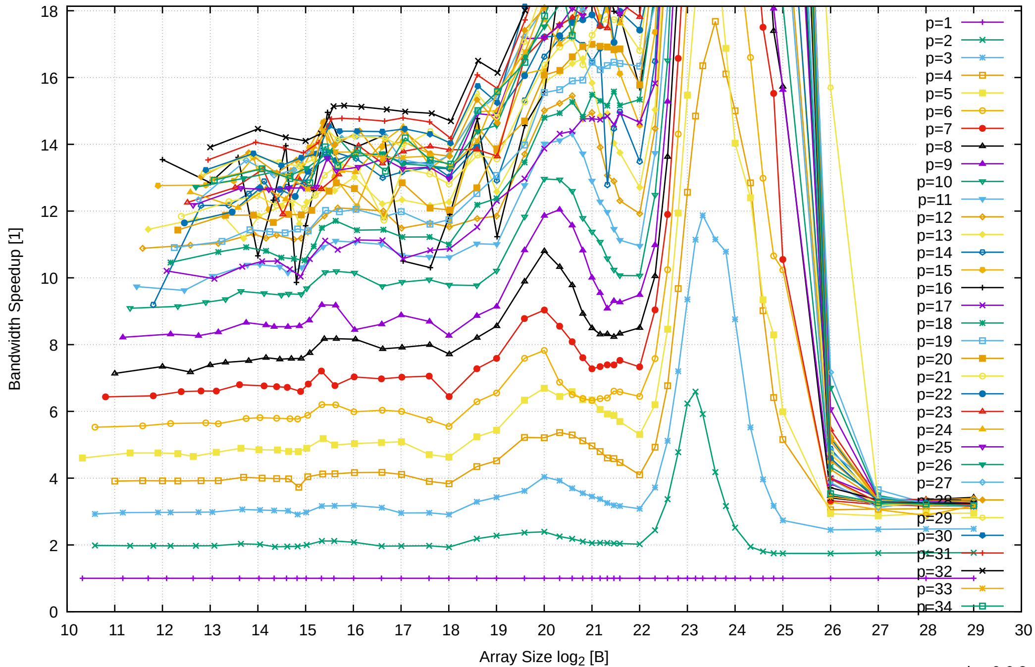
AMD Ryzen Threadripper 2950X 128GB - Speedup of Parallel Memory Bandwidth (enlarged) - ScanRead128PtrUnrollLoop
