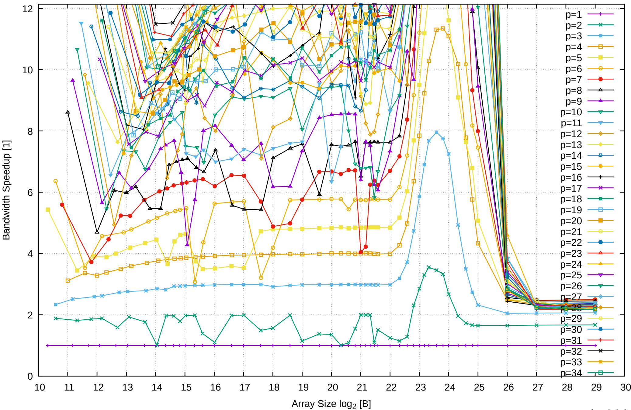
AMD Ryzen Threadripper 2950X 128GB - Speedup of Parallel Memory Bandwidth (enlarged) - ScanWrite128PtrSimpleLoop
