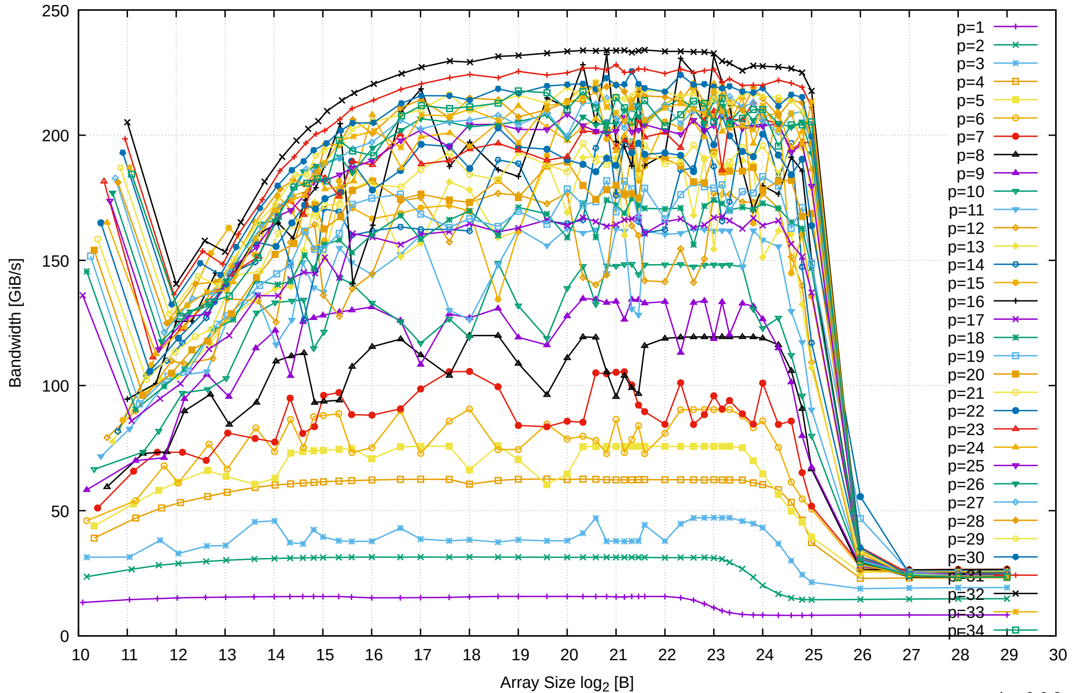
AMD Ryzen Threadripper 2950X 128GB - Parallel Memory Bandwidth - ScanWrite32PtrSimpleLoop
