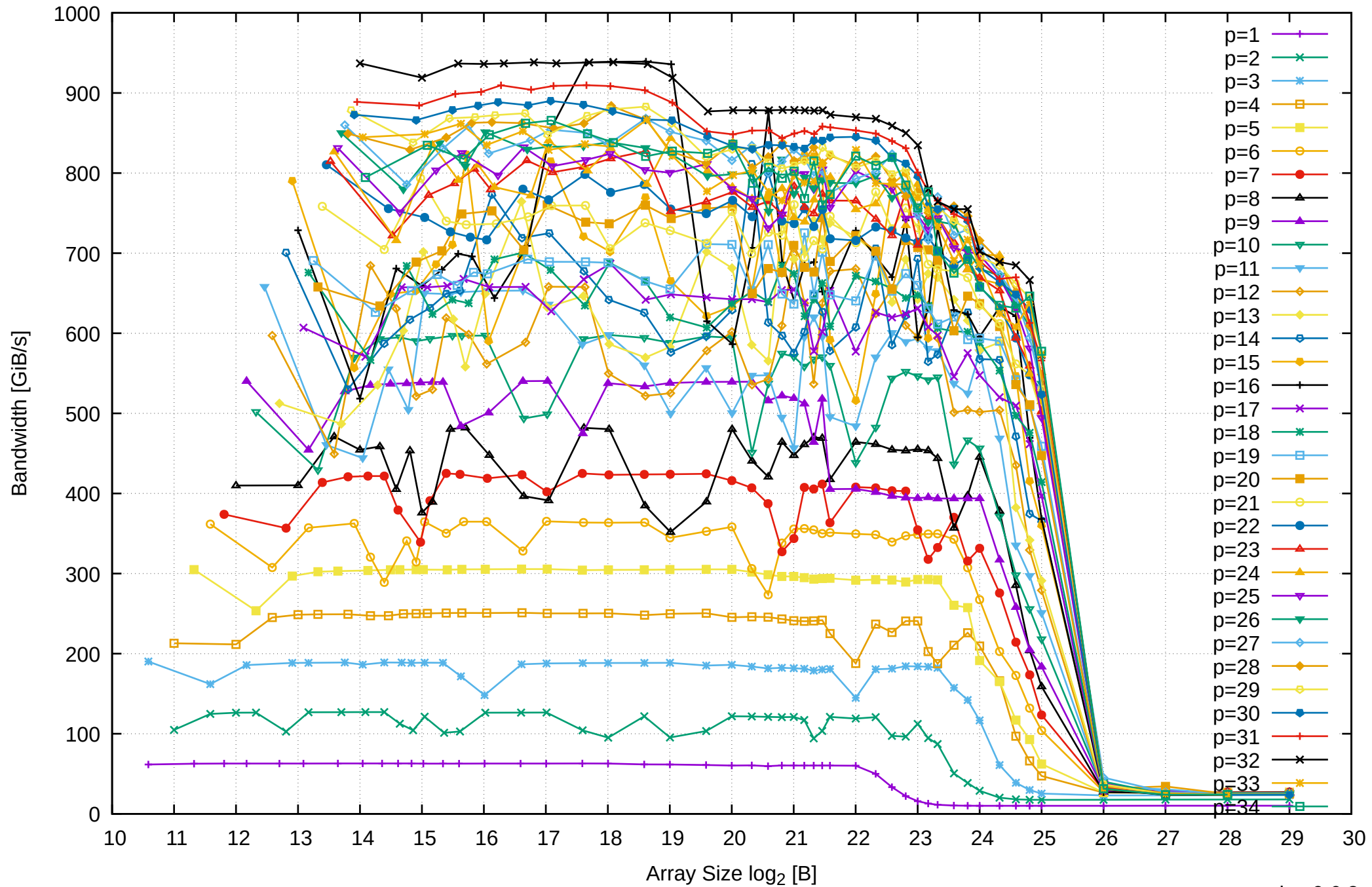
AMD Ryzen Threadripper 2950X 128GB - Parallel Memory Bandwidth - ScanWrite256PtrSimpleLoop
