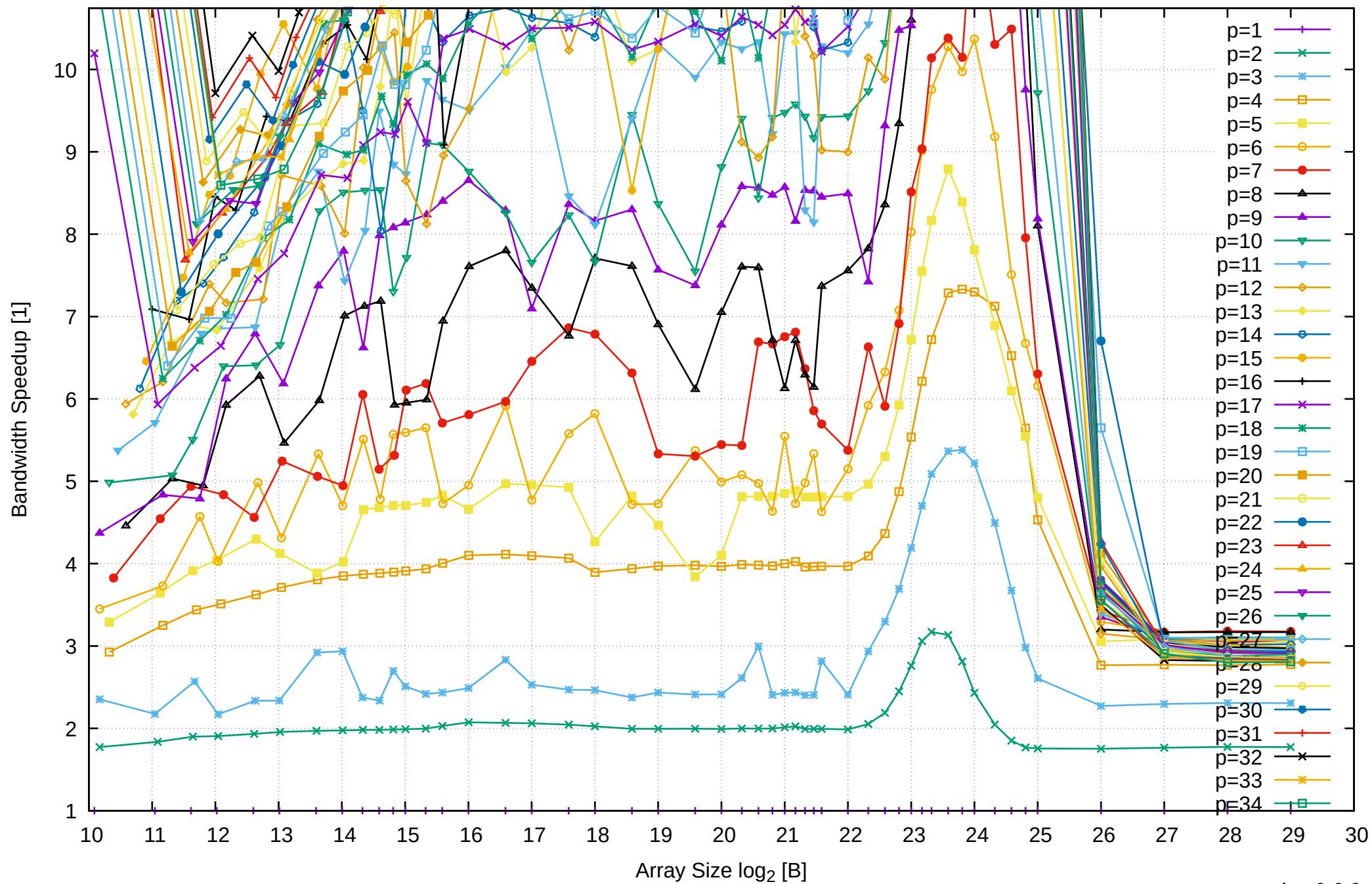
AMD Ryzen Threadripper 2950X 128GB - Speedup of Parallel Memory Bandwidth (enlarged) - ScanWrite32PtrSimpleLoop
