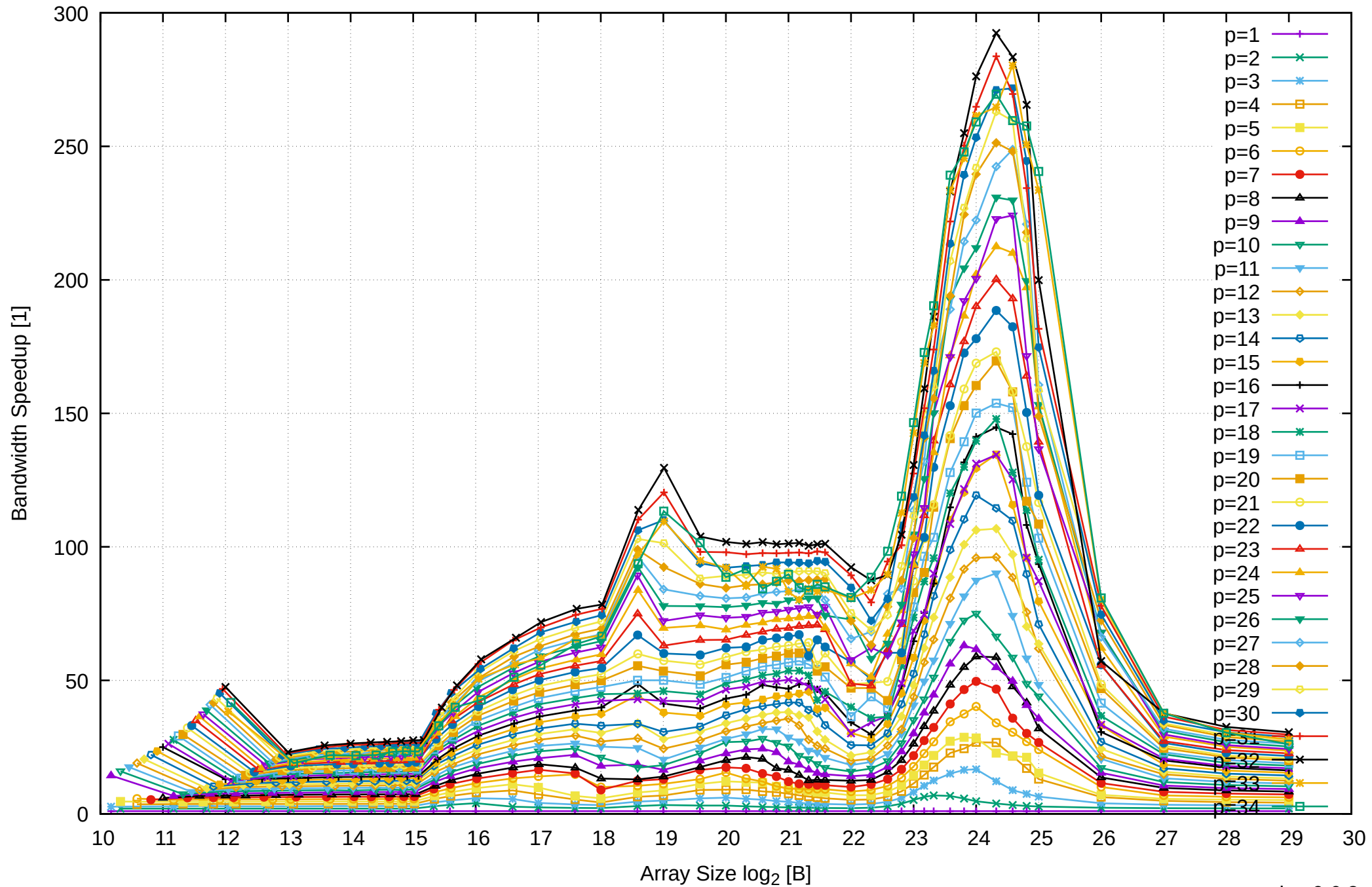
AMD Ryzen Threadripper 2950X 128GB - Speedup of Parallel Memory Bandwidth - PermRead64SimpleLoop
