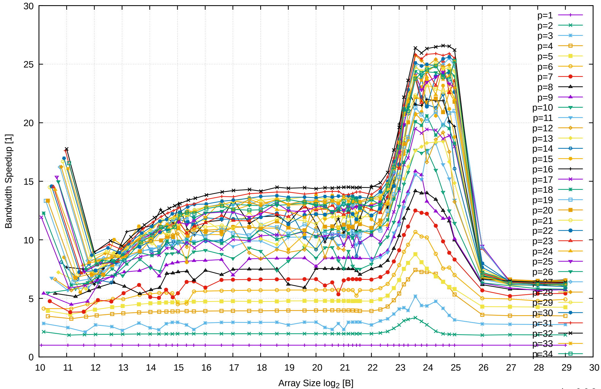
AMD Ryzen Threadripper 2950X 128GB - Speedup of Parallel Memory Bandwidth - ScanRead32PtrSimpleLoop
