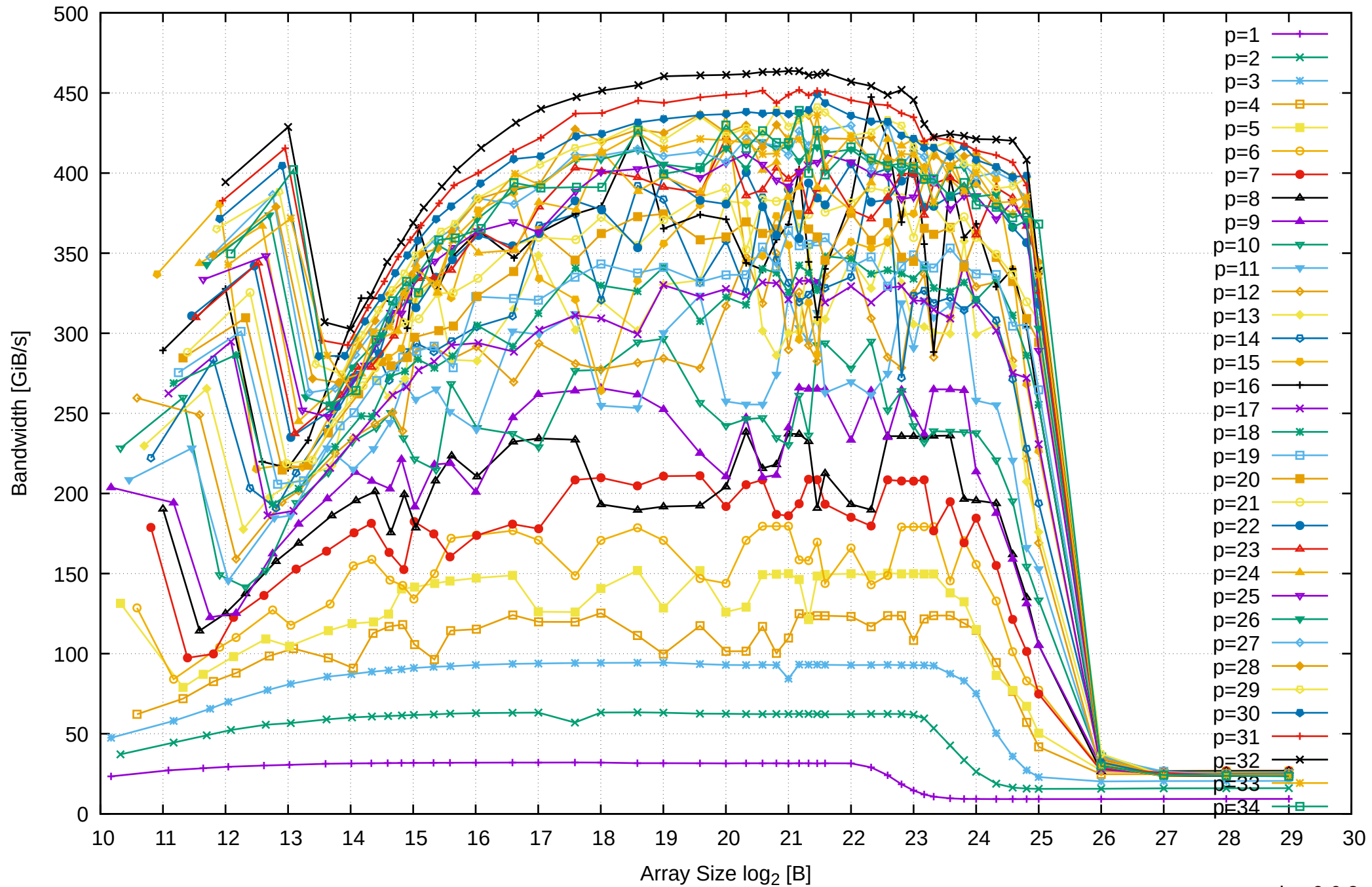
AMD Ryzen Threadripper 2950X 128GB - Parallel Memory Bandwidth - ScanWrite64PtrSimpleLoop
