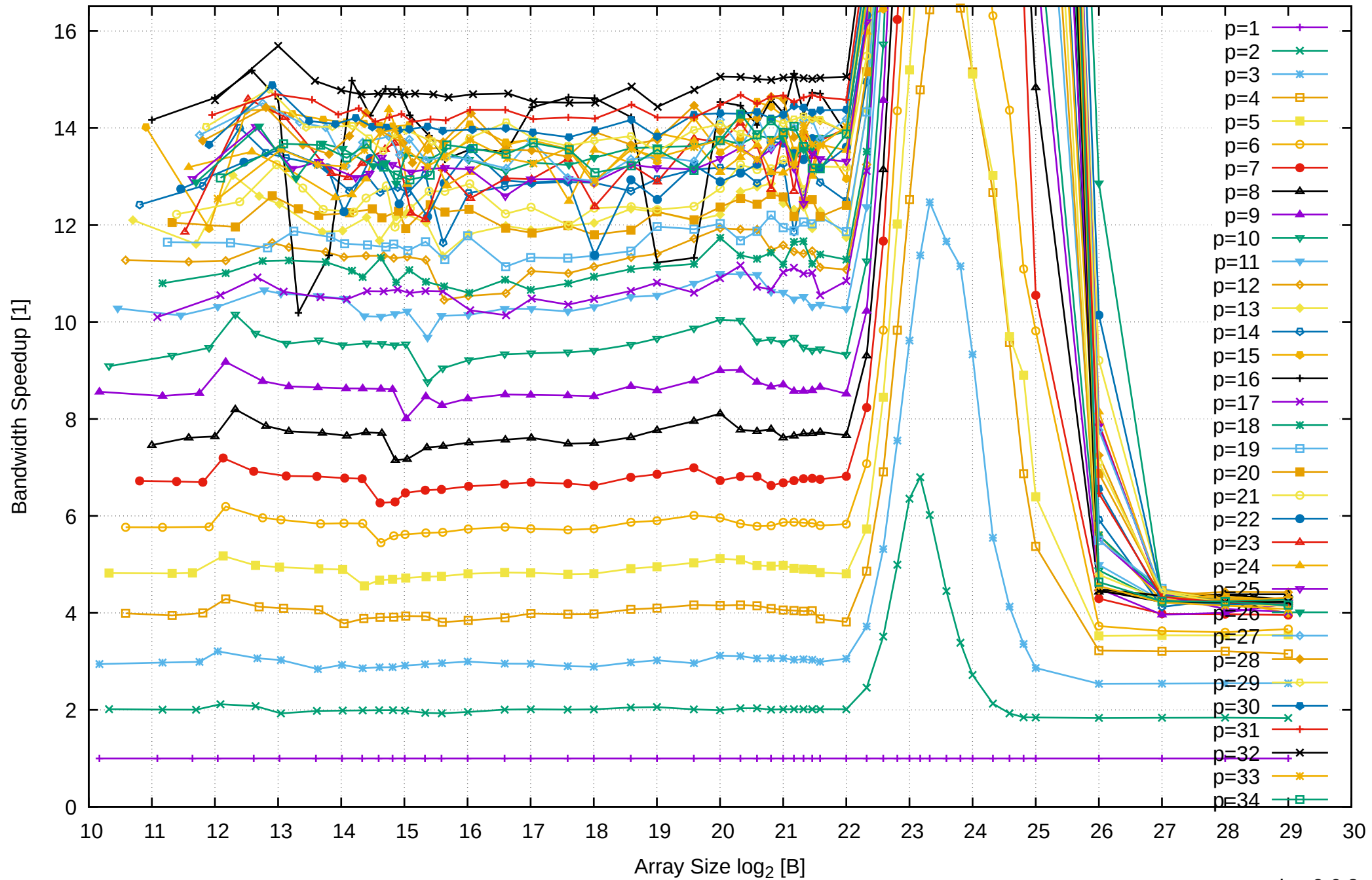
AMD Ryzen Threadripper 2950X 128GB - Speedup of Parallel Memory Bandwidth (enlarged) - ScanRead64PtrUnrollLoop
