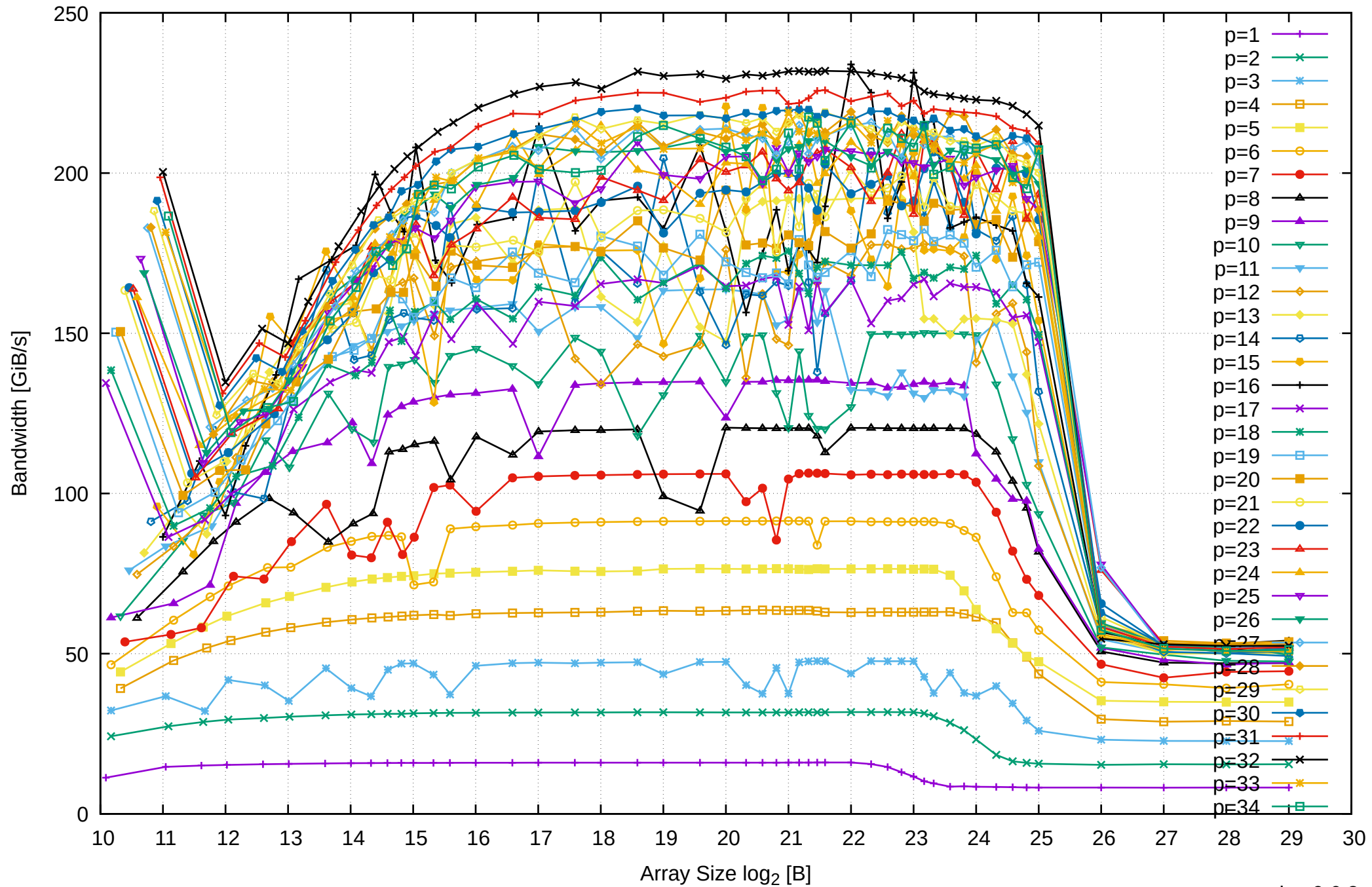
AMD Ryzen Threadripper 2950X 128GB - Parallel Memory Bandwidth - ScanRead32PtrSimpleLoop
