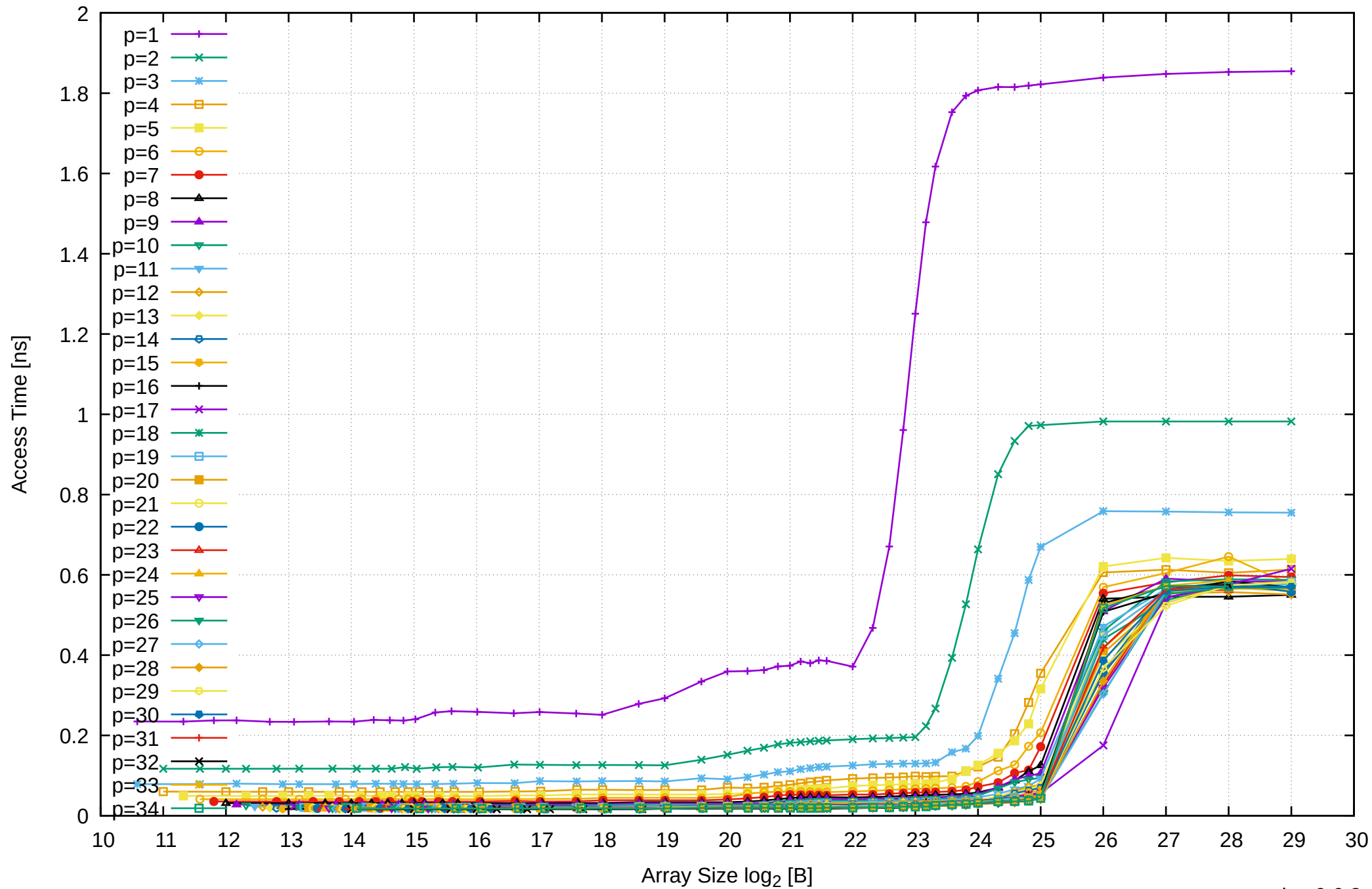
AMD Ryzen Threadripper 2950X 128GB - Parallel Memory Access Time - ScanRead256PtrUnrollLoop
