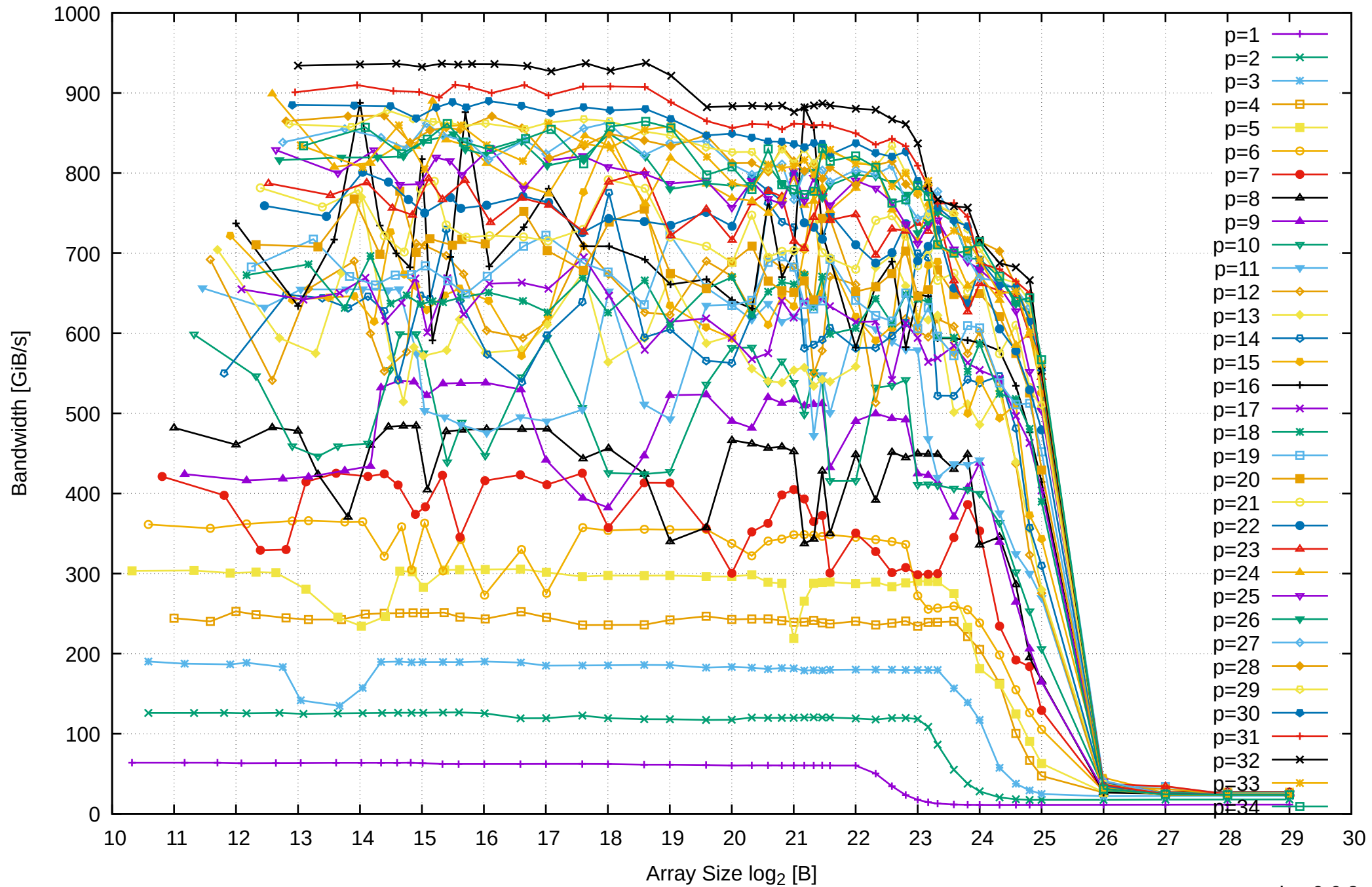
AMD Ryzen Threadripper 2950X 128GB - Parallel Memory Bandwidth - ScanWrite128PtrUnrollLoop
