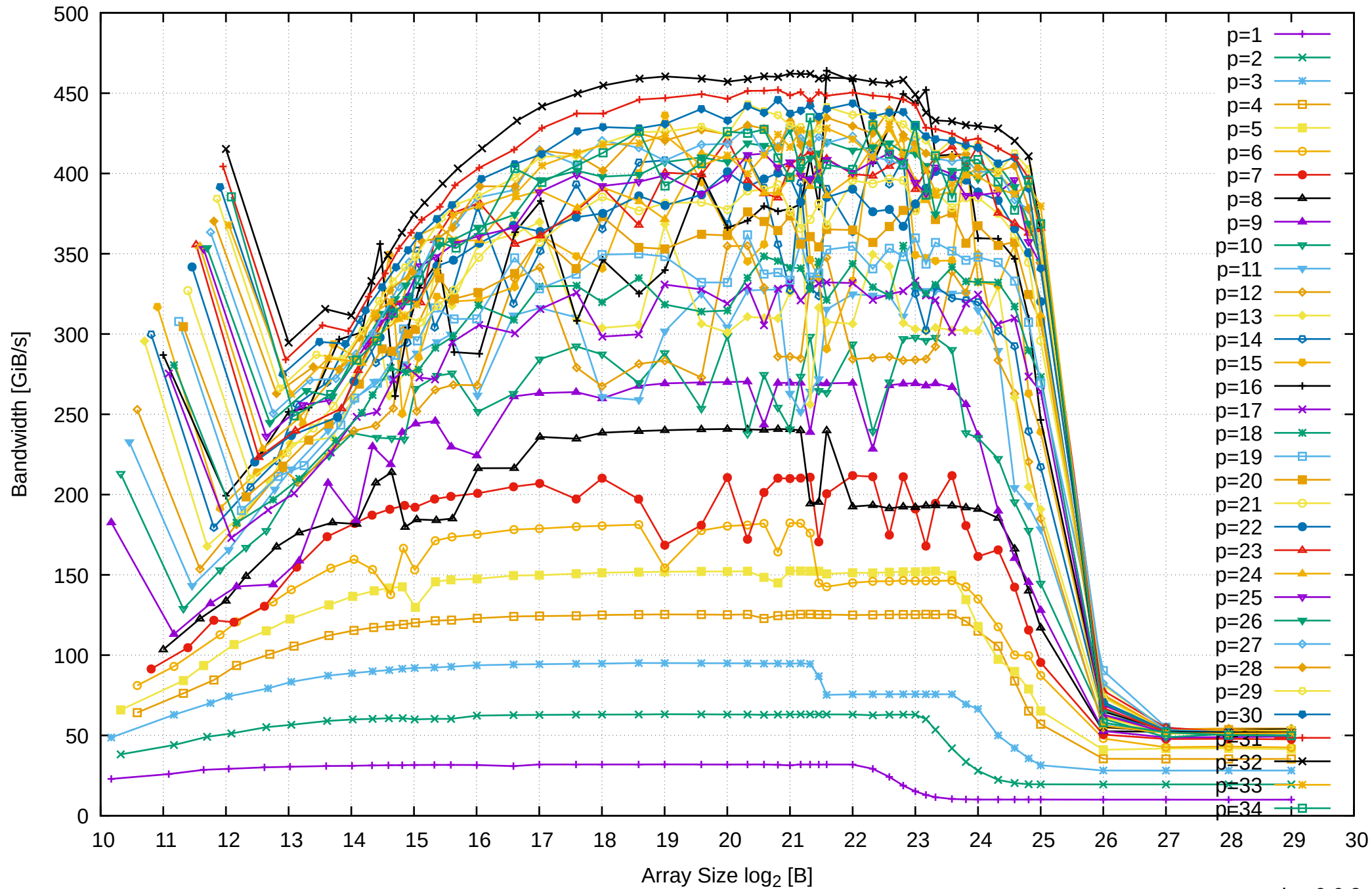
AMD Ryzen Threadripper 2950X 128GB - Parallel Memory Bandwidth - ScanRead64IndexSimpleLoop
