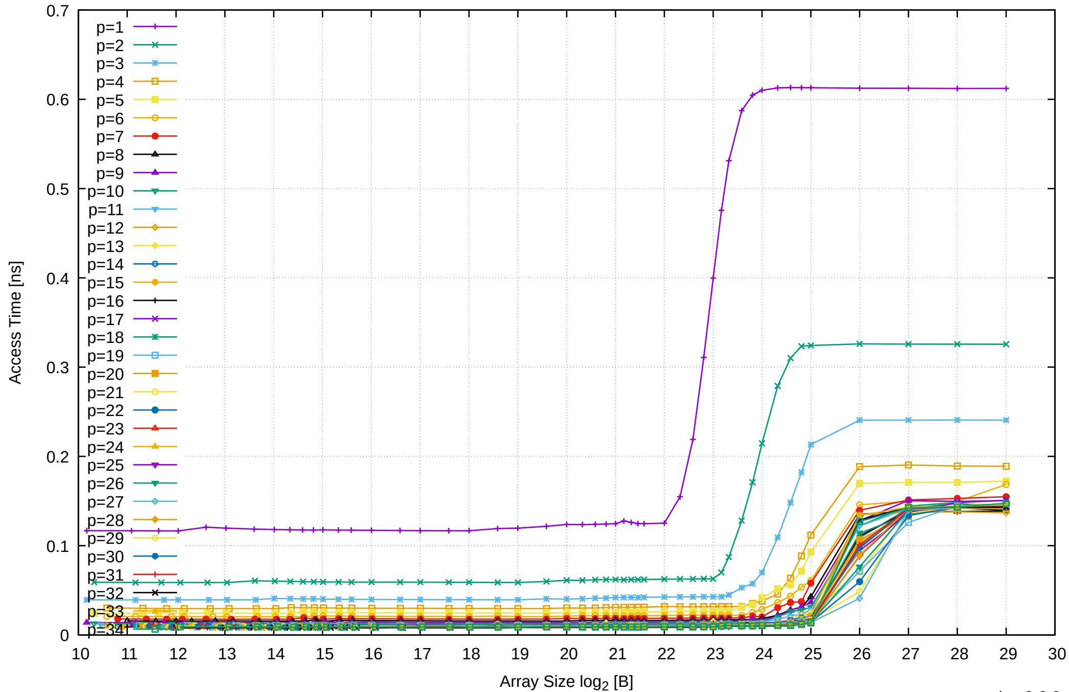
AMD Ryzen Threadripper 2950X 128GB - Parallel Memory Access Time - ScanRead64IndexUnrollLoop
