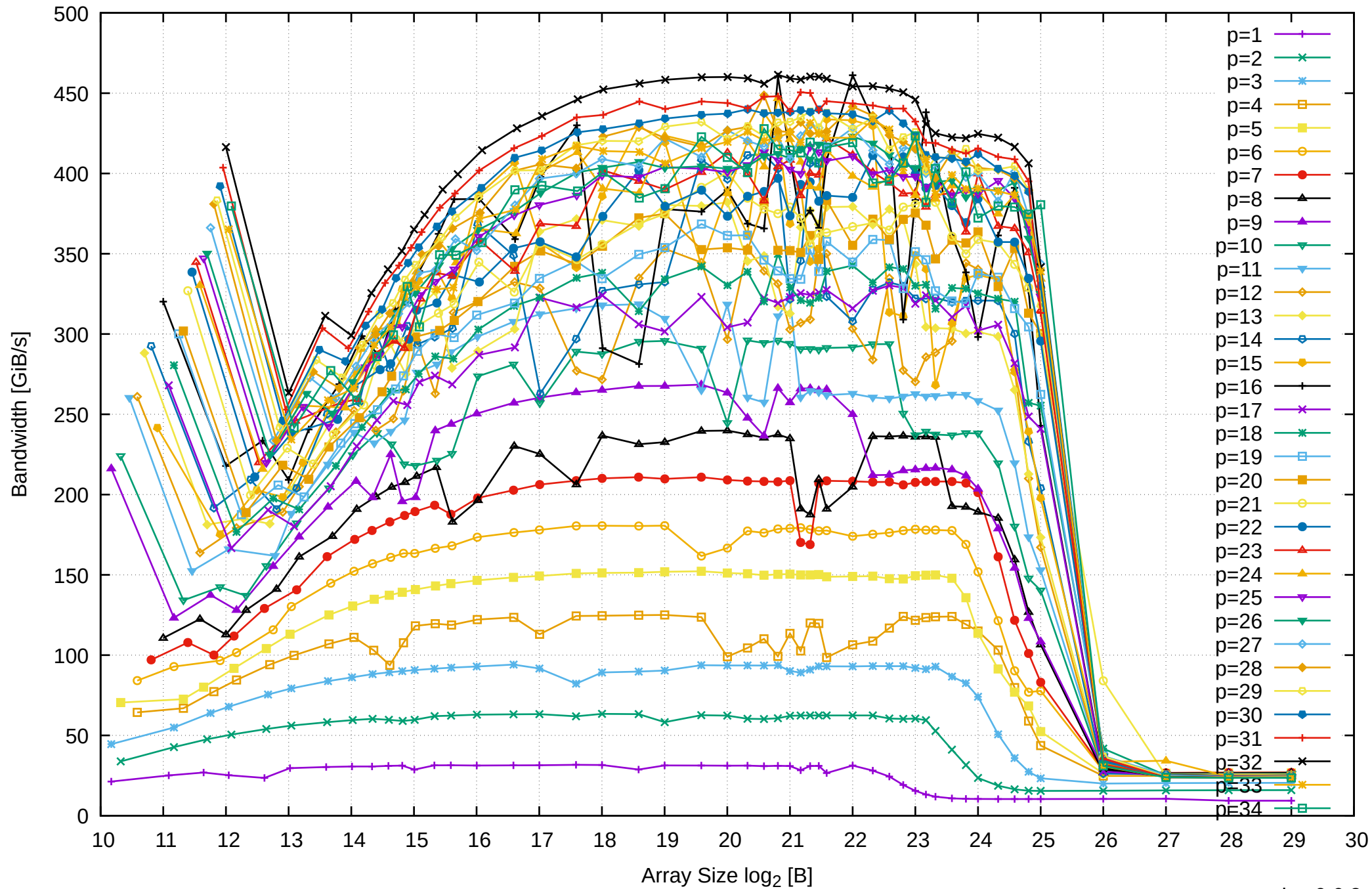
AMD Ryzen Threadripper 2950X 128GB - Parallel Memory Bandwidth - ScanWrite64IndexSimpleLoop
