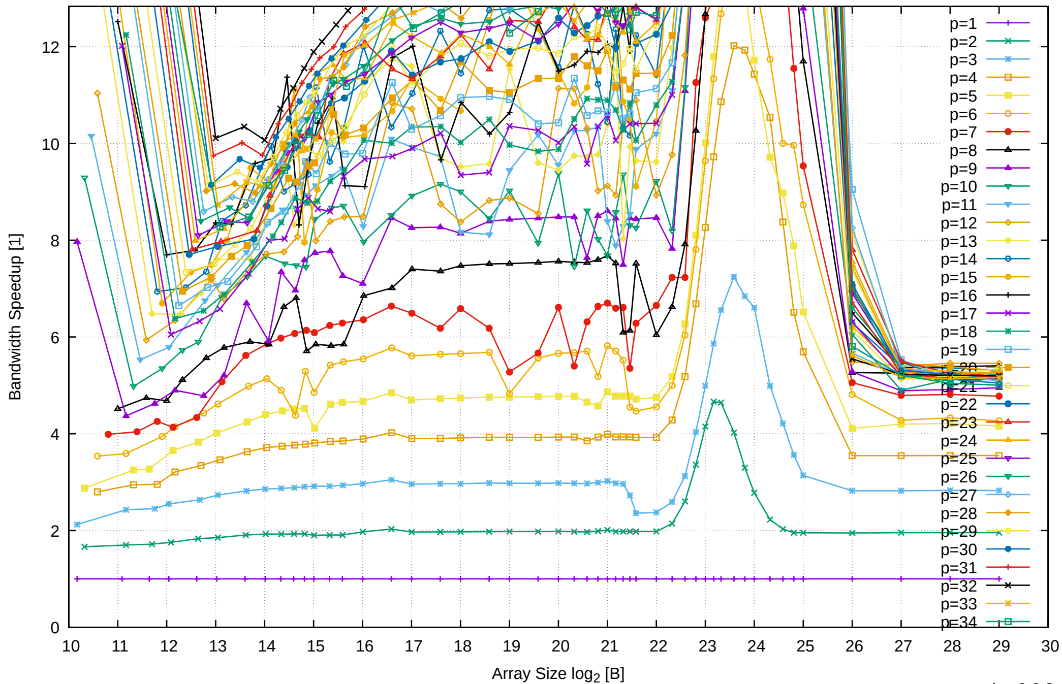
AMD Ryzen Threadripper 2950X 128GB - Speedup of Parallel Memory Bandwidth (enlarged) - ScanRead64IndexSimpleLoop
