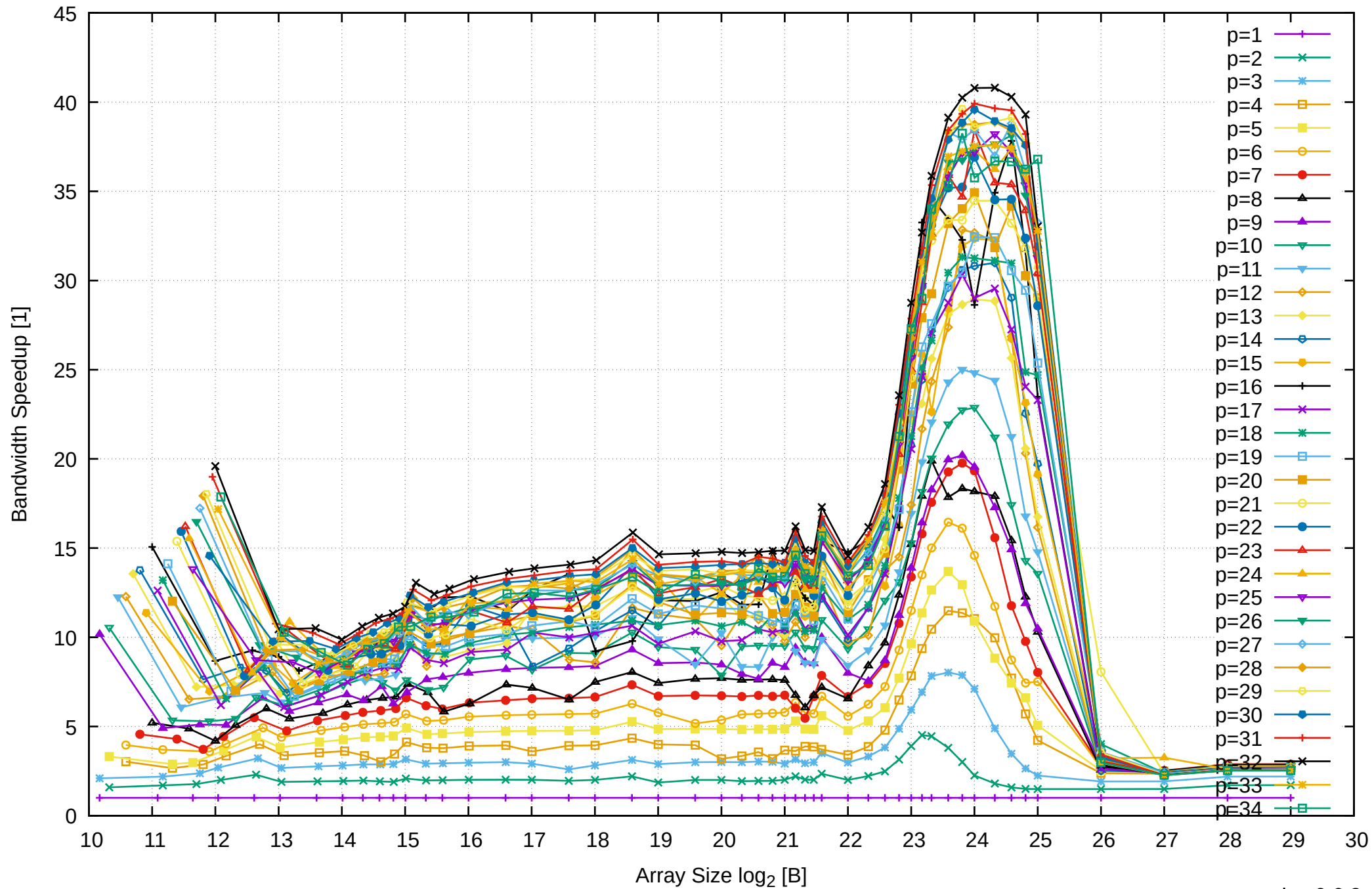
AMD Ryzen Threadripper 2950X 128GB - Speedup of Parallel Memory Bandwidth - ScanWrite64IndexSimpleLoop
