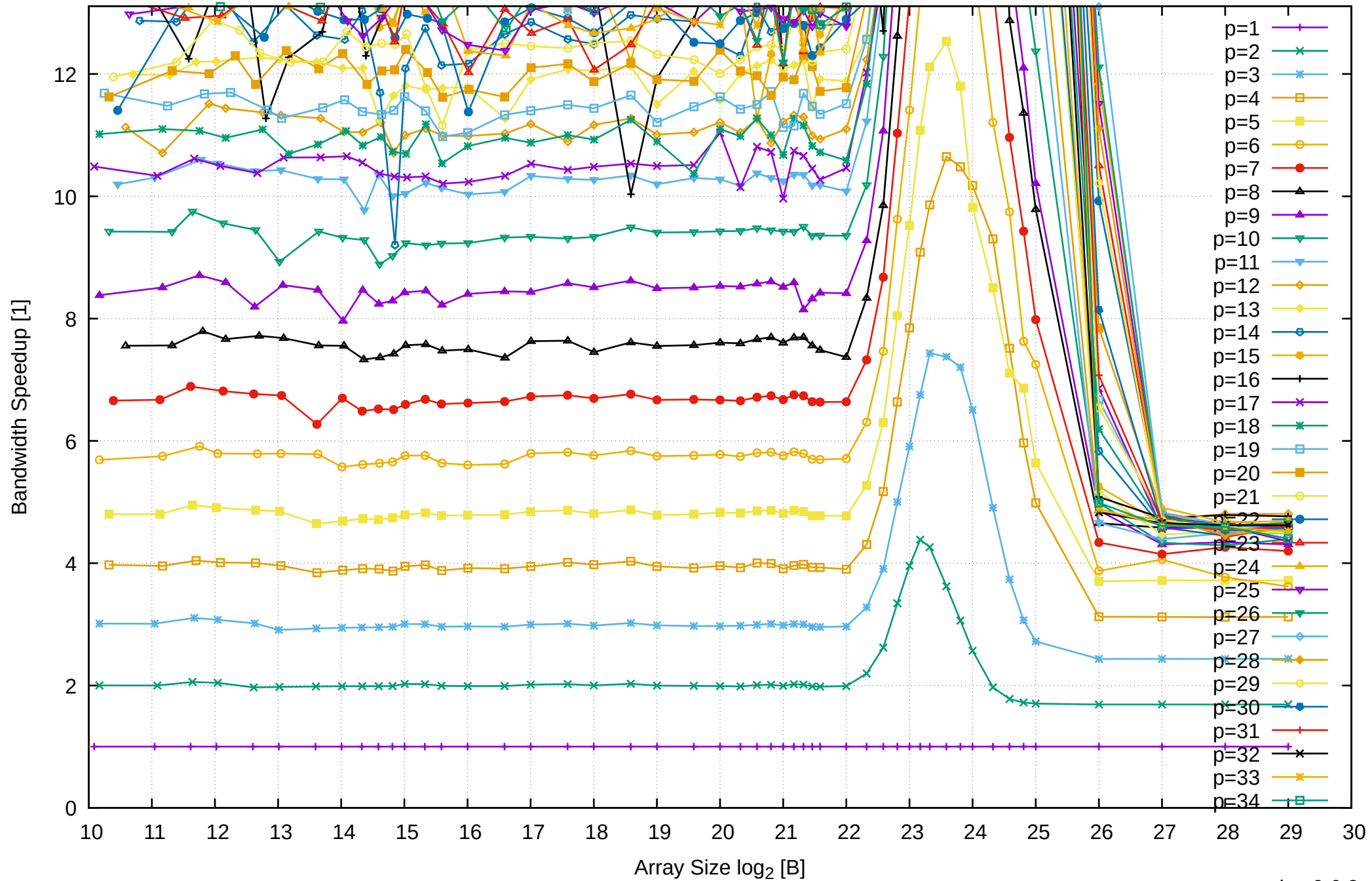
AMD Ryzen Threadripper 2950X 128GB - Speedup of Parallel Memory Bandwidth (enlarged) - ScanRead32PtrUnrollLoop
