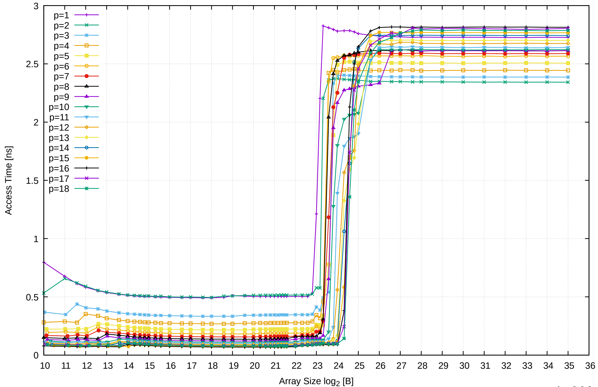
AMD Ryzen 7 1800X 64GB - Parallel Memory Access Time - ScanWrite256PtrSimpleLoop
