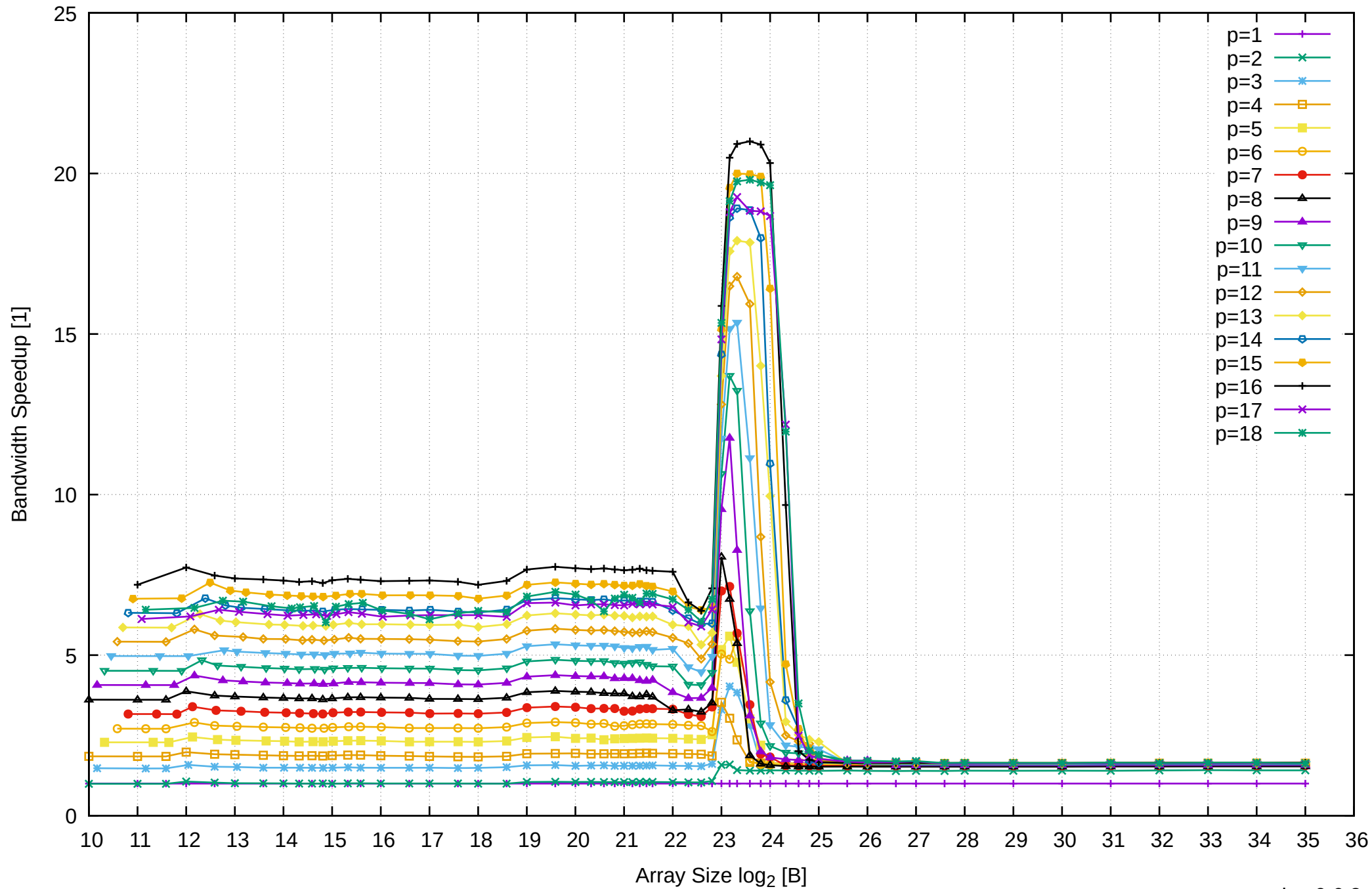
AMD Ryzen 7 1800X 64GB - Speedup of Parallel Memory Bandwidth - ScanRead64IndexUnrollLoop
