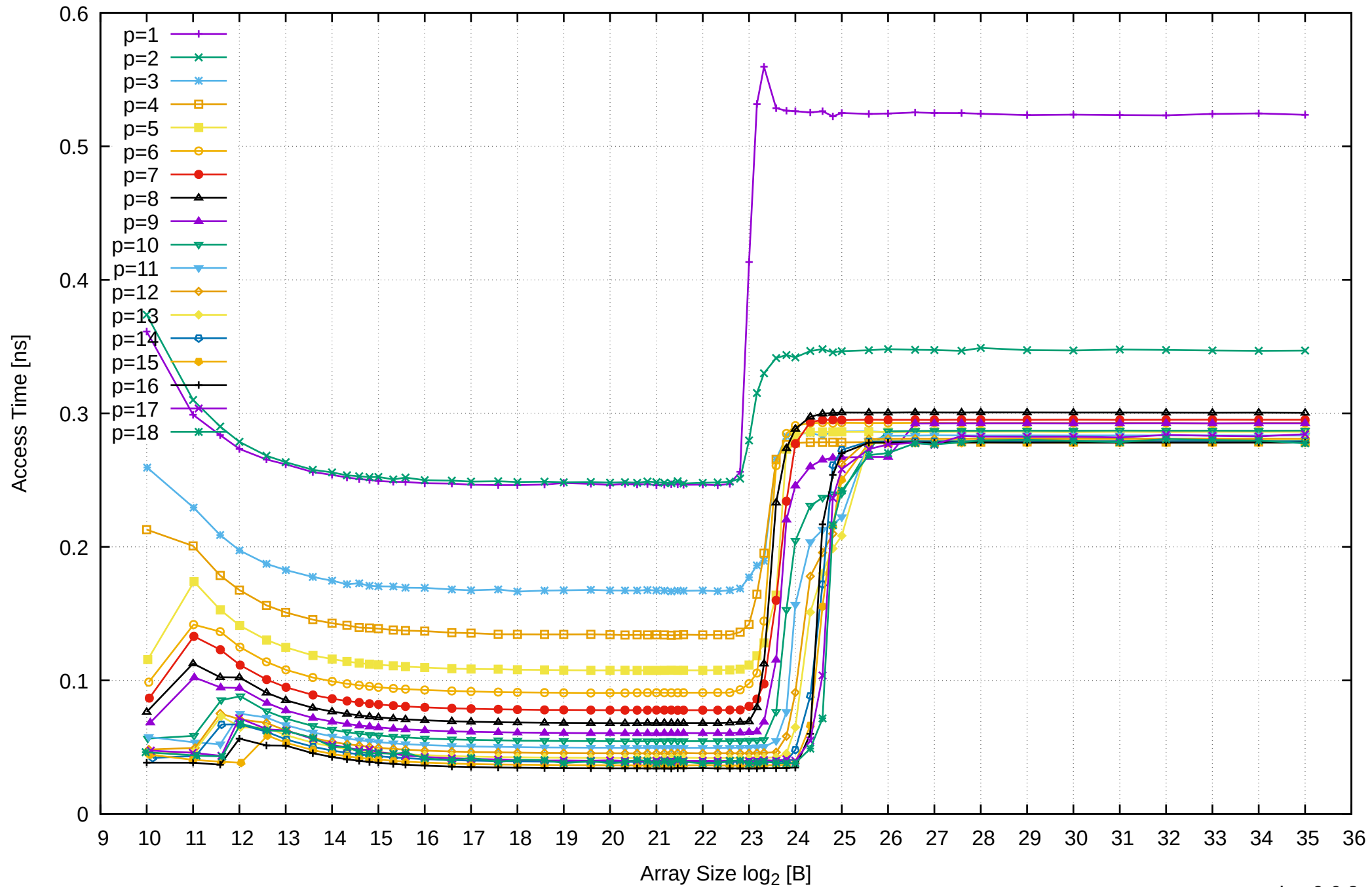
AMD Ryzen 7 1800X 64GB - Parallel Memory Access Time - ScanRead64PtrSimpleLoop
