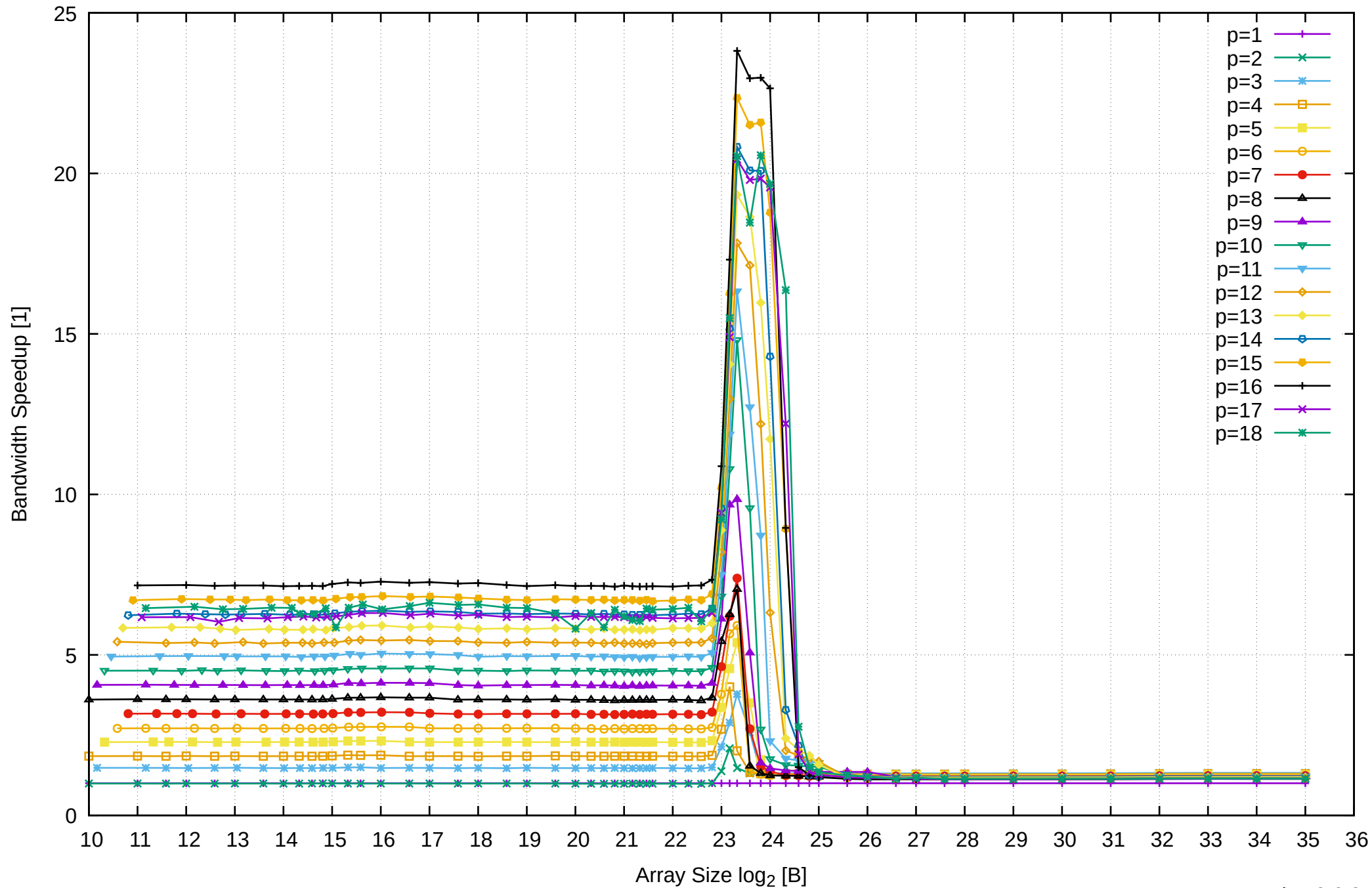
AMD Ryzen 7 1800X 64GB - Speedup of Parallel Memory Bandwidth - ScanWrite64PtrUnrollLoop
