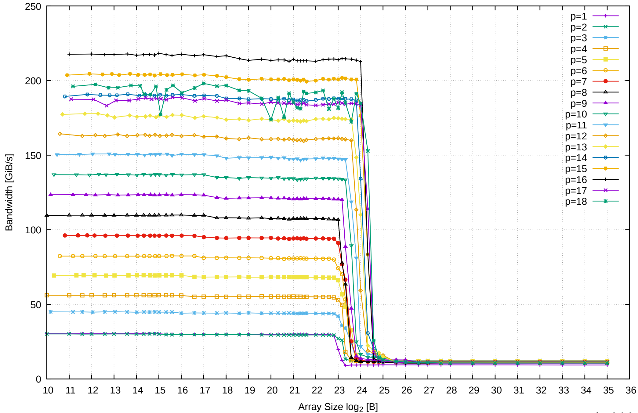
AMD Ryzen 7 1800X 64GB - Parallel Memory Bandwidth - ScanWrite64PtrUnrollLoop
