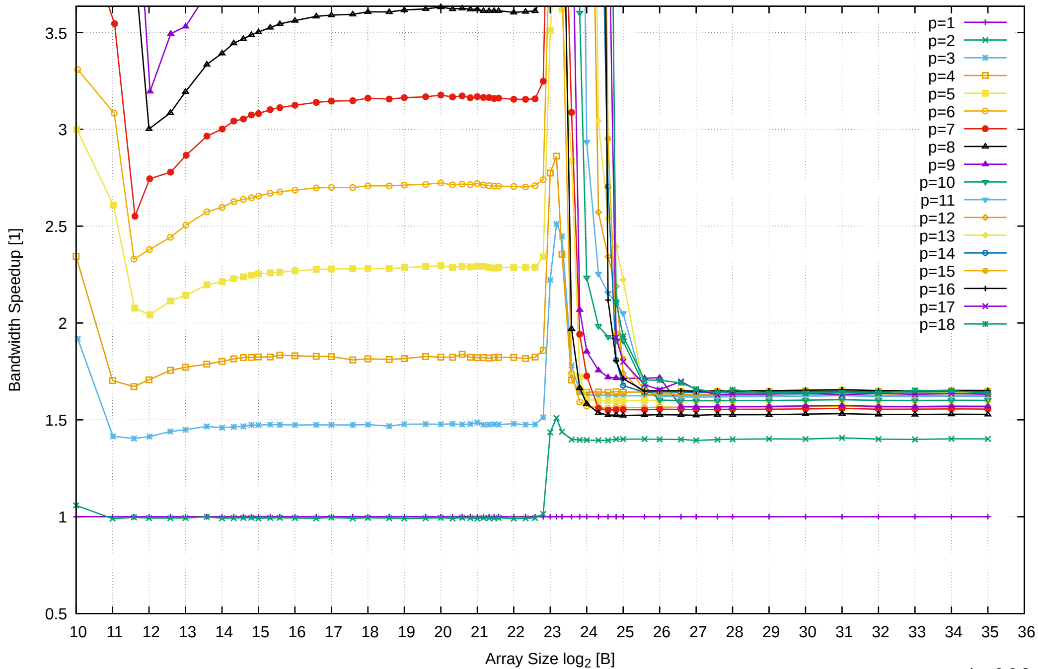
AMD Ryzen 7 1800X 64GB - Speedup of Parallel Memory Bandwidth (enlarged) - ScanRead128PtrSimpleLoop
