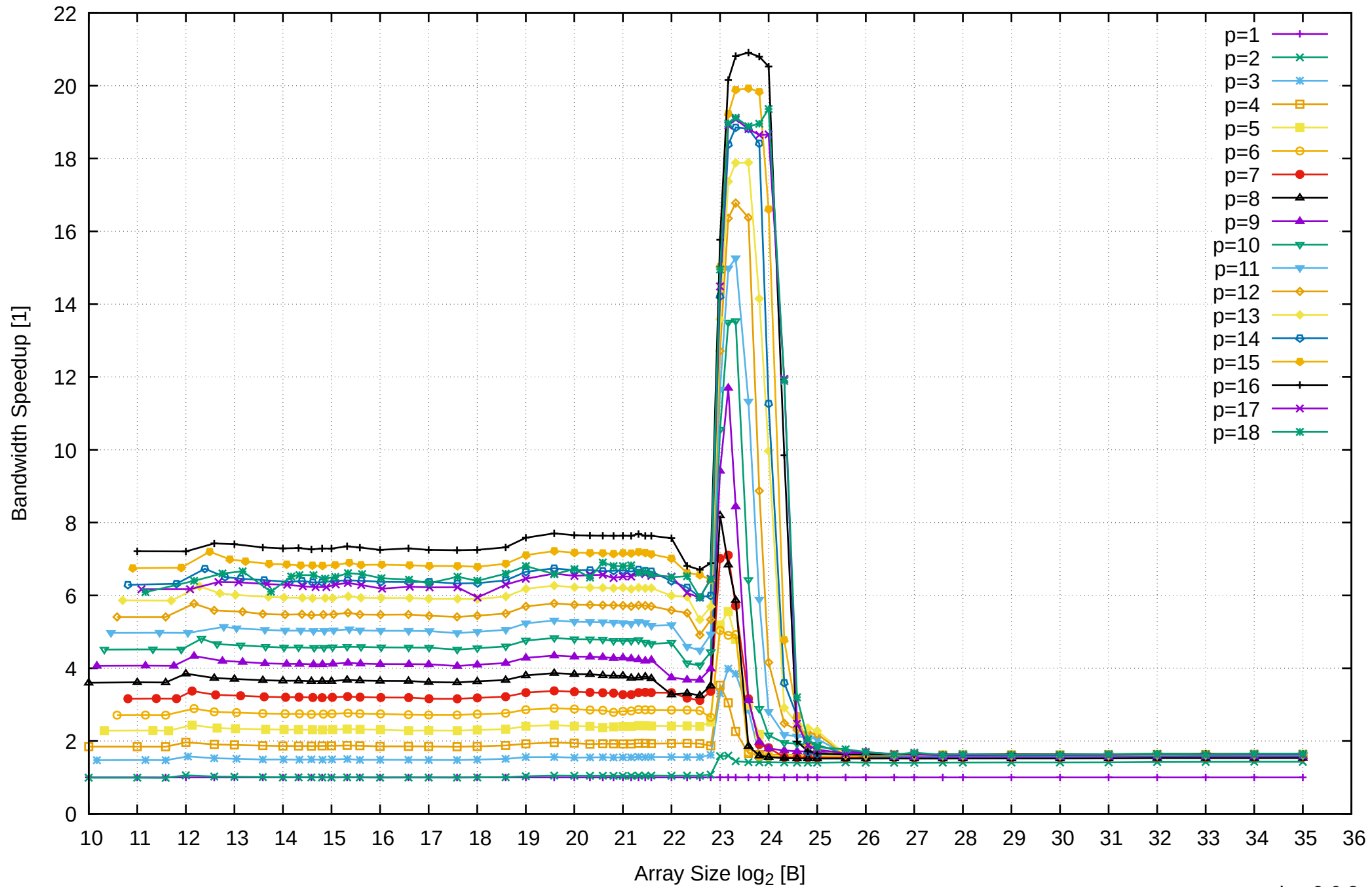
AMD Ryzen 7 1800X 64GB - Speedup of Parallel Memory Bandwidth - ScanRead64PtrUnrollLoop
