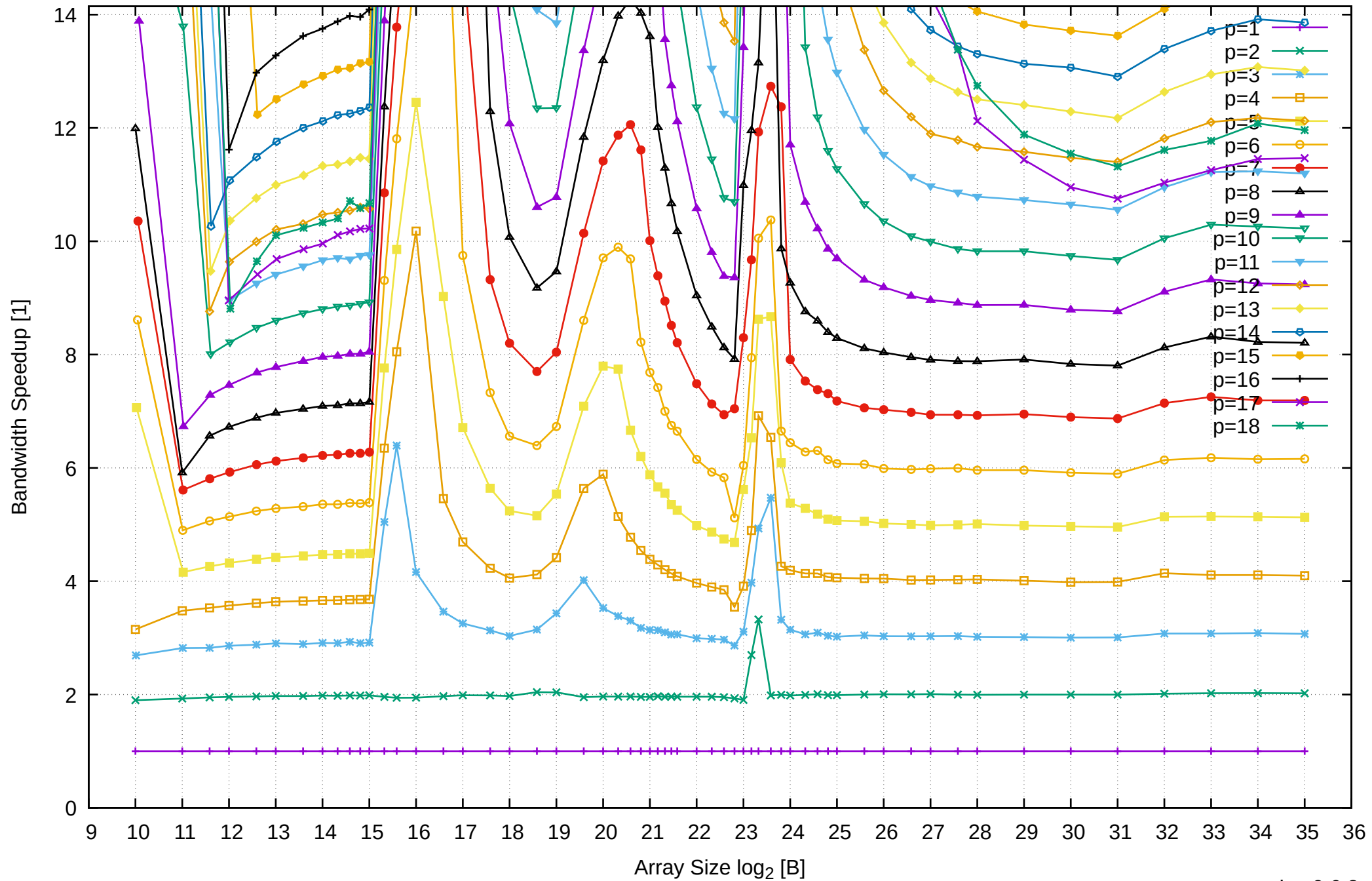
AMD Ryzen 7 1800X 64GB - Speedup of Parallel Memory Bandwidth (enlarged) - PermRead64SimpleLoop
