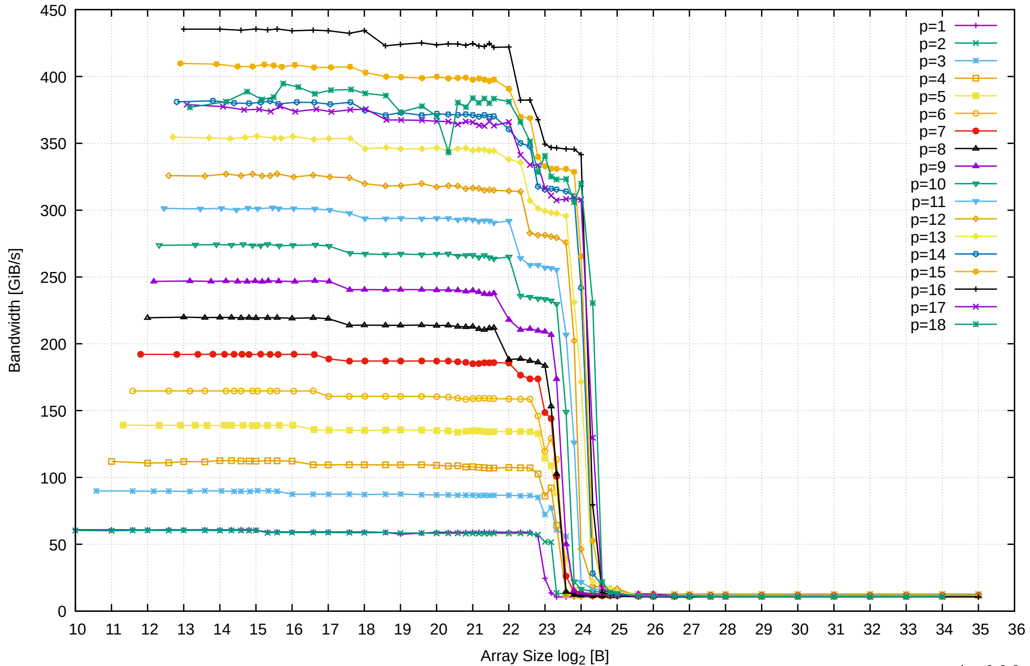
AMD Ryzen 7 1800X 64GB - Parallel Memory Bandwidth - ScanWrite256PtrUnrollLoop
