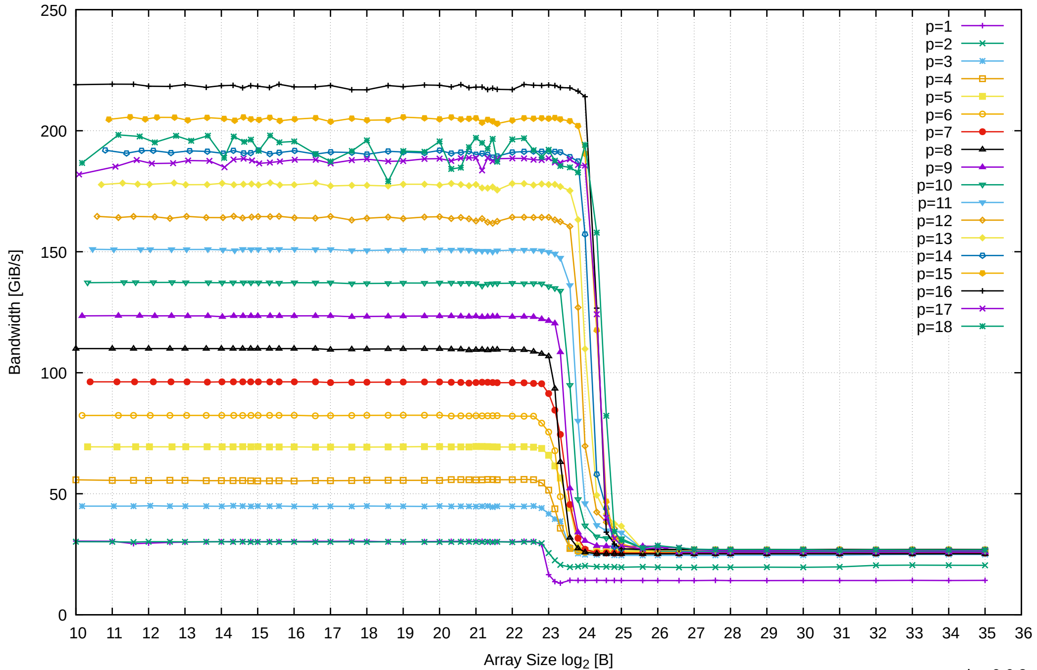
AMD Ryzen 7 1800X 64GB - Parallel Memory Bandwidth - ScanRead32PtrUnrollLoop
