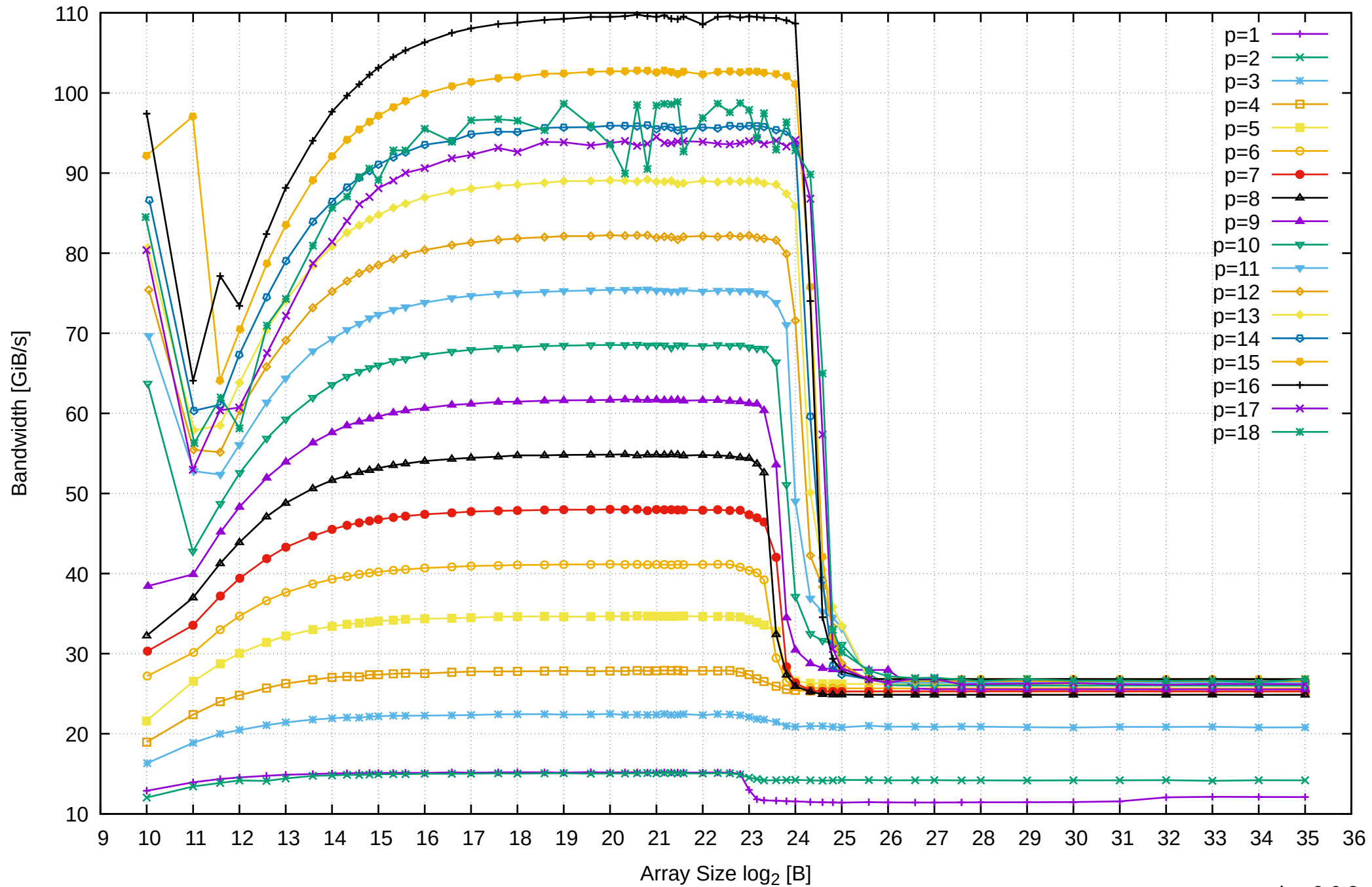
AMD Ryzen 7 1800X 64GB - Parallel Memory Bandwidth - ScanRead32PtrSimpleLoop
