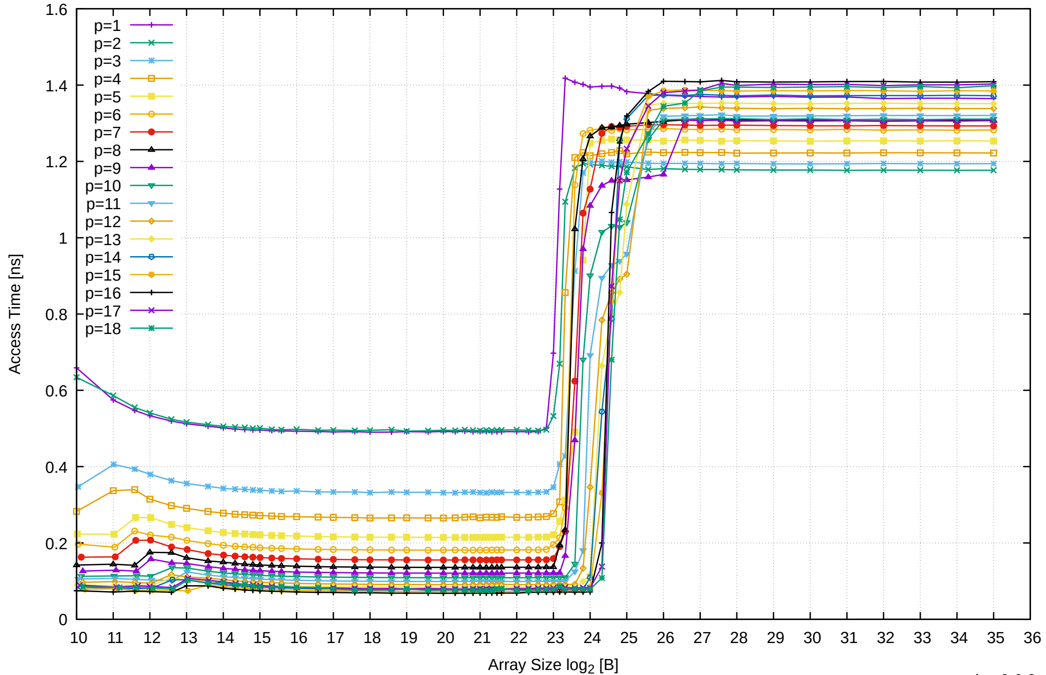
AMD Ryzen 7 1800X 64GB - Parallel Memory Access Time - ScanWrite128PtrSimpleLoop
