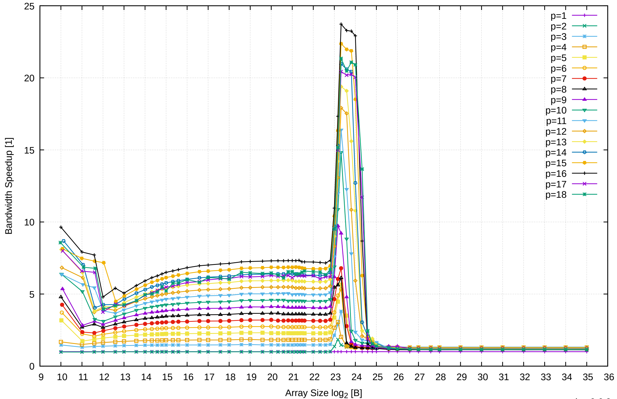
AMD Ryzen 7 1800X 64GB - Speedup of Parallel Memory Bandwidth - ScanWrite64IndexSimpleLoop
