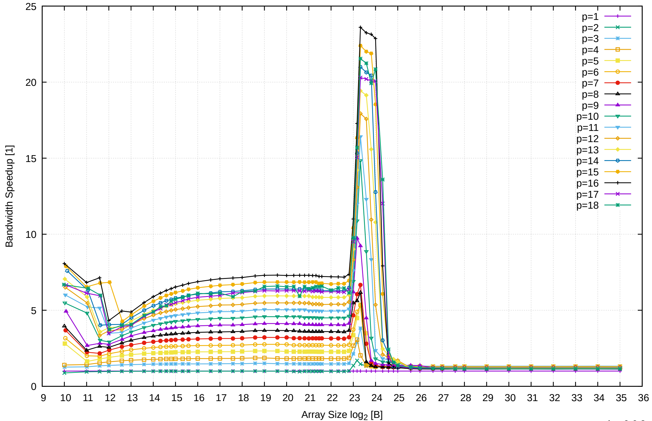
AMD Ryzen 7 1800X 64GB - Speedup of Parallel Memory Bandwidth - ScanWrite64PtrSimpleLoop
