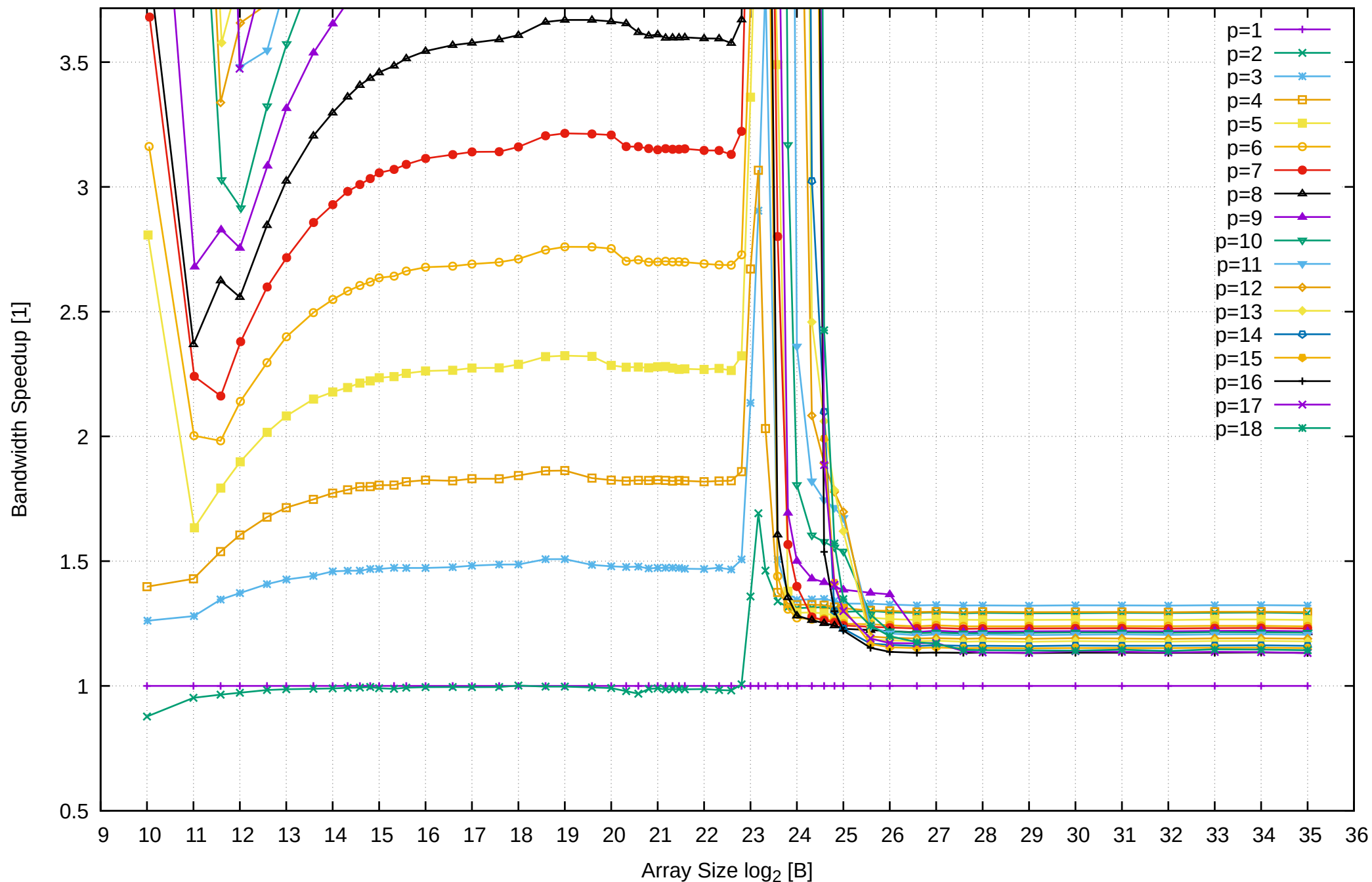
AMD Ryzen 7 1800X 64GB - Speedup of Parallel Memory Bandwidth (enlarged) - ScanWrite64PtrSimpleLoop
