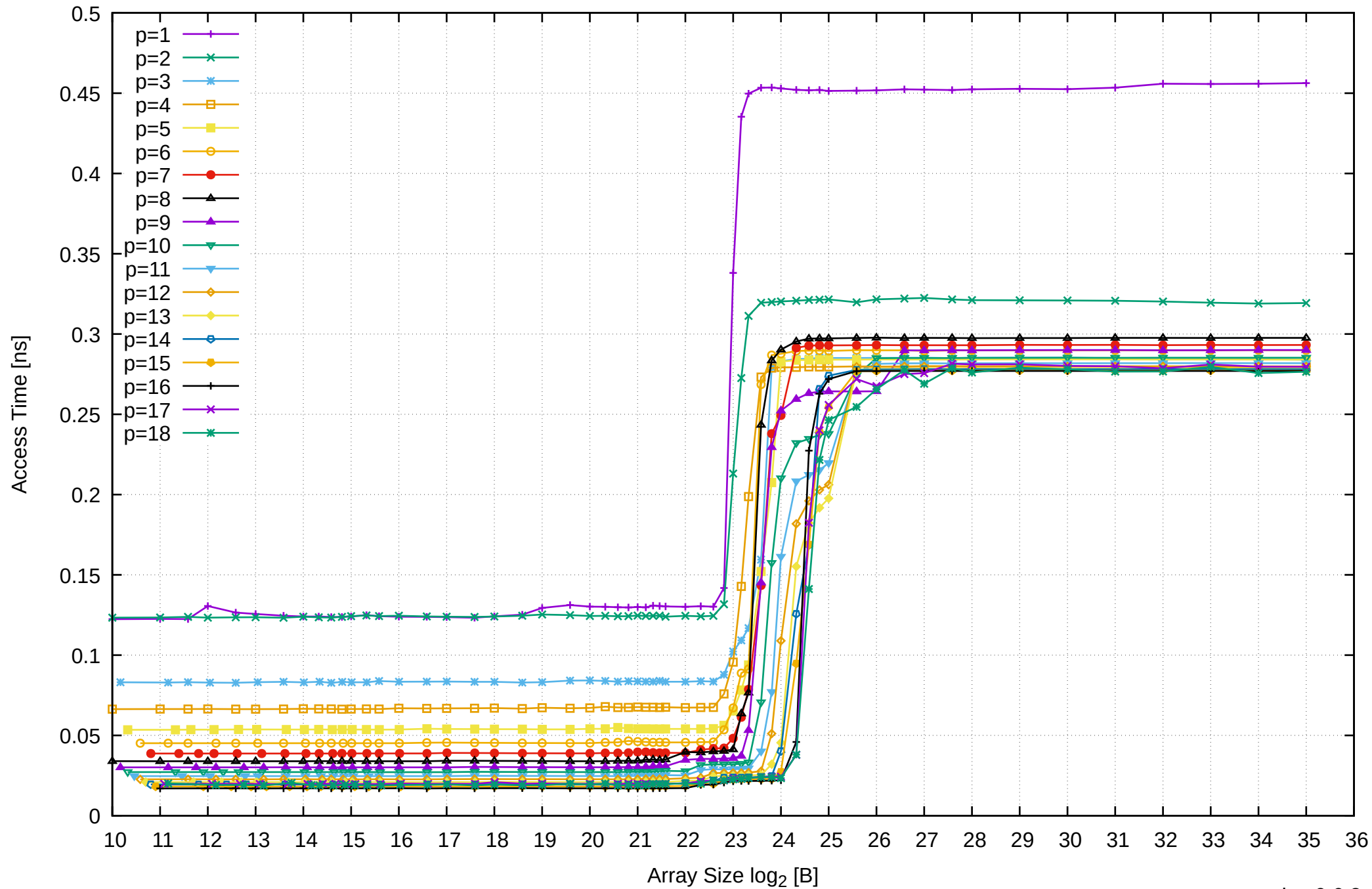
AMD Ryzen 7 1800X 64GB - Parallel Memory Access Time - ScanRead64PtrUnrollLoop
