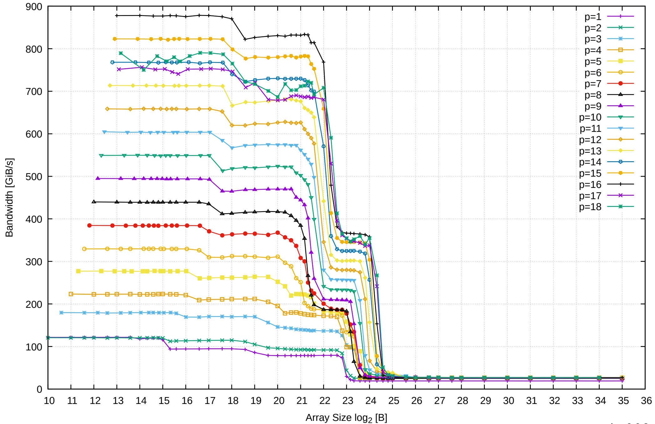
AMD Ryzen 7 1800X 64GB - Parallel Memory Bandwidth - ScanRead256PtrUnrollLoop
