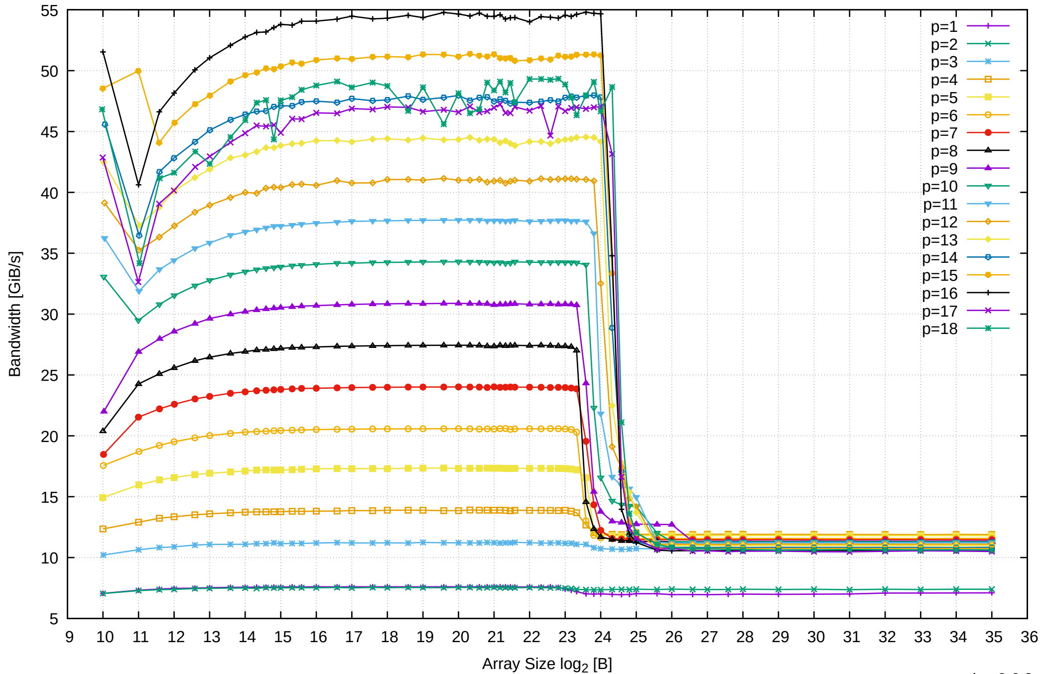
AMD Ryzen 7 1800X 64GB - Parallel Memory Bandwidth - ScanWrite32PtrSimpleLoop
