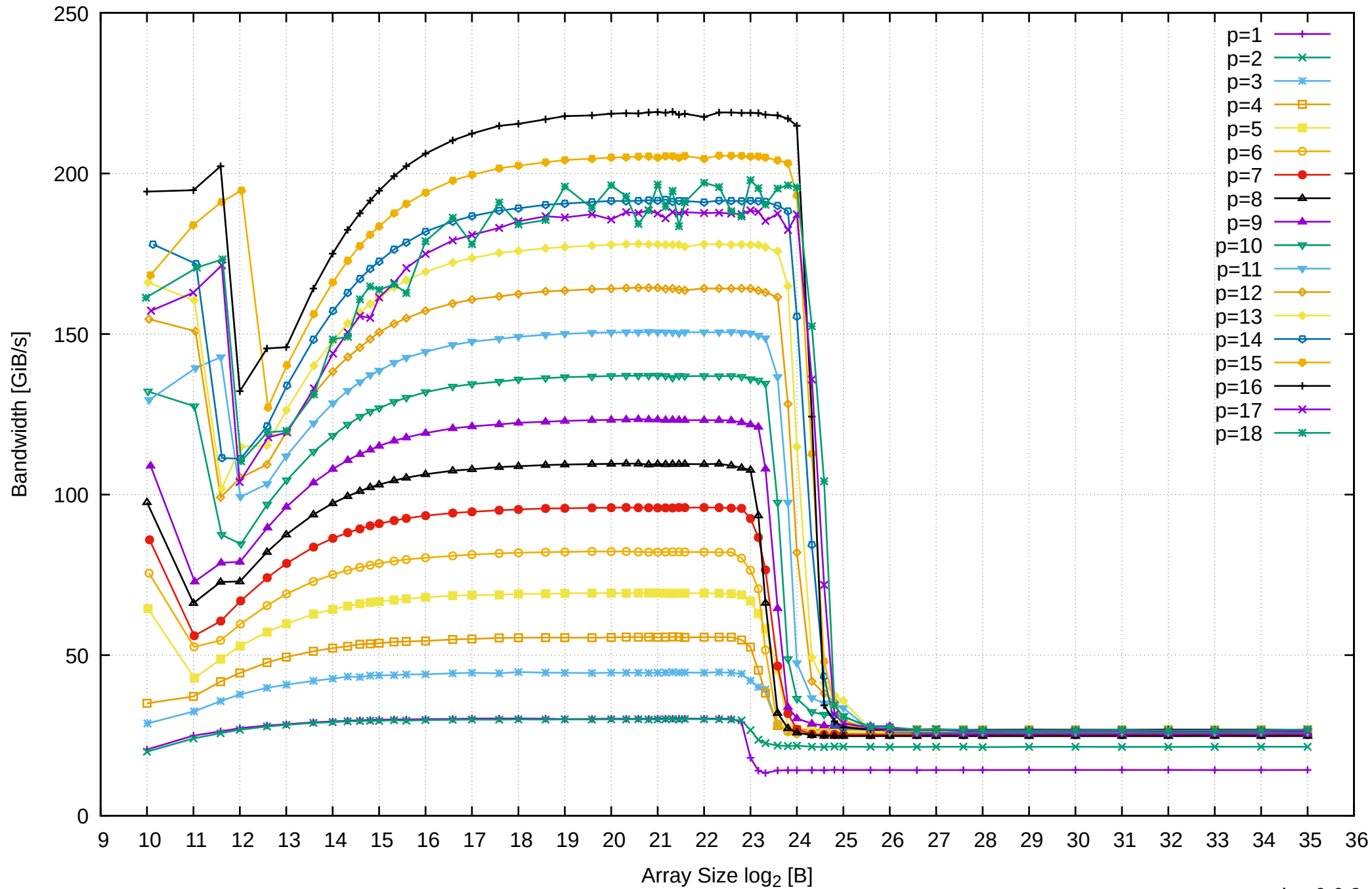
AMD Ryzen 7 1800X 64GB - Parallel Memory Bandwidth - ScanRead64PtrSimpleLoop
