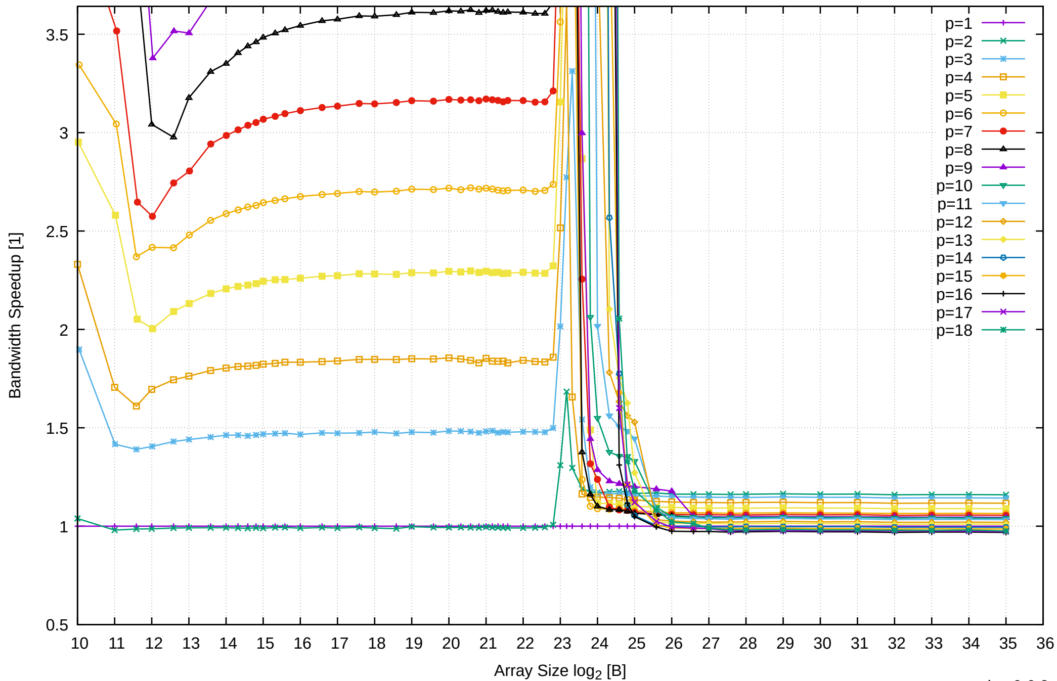
AMD Ryzen 7 1800X 64GB - Speedup of Parallel Memory Bandwidth (enlarged) - ScanWrite128PtrSimpleLoop
