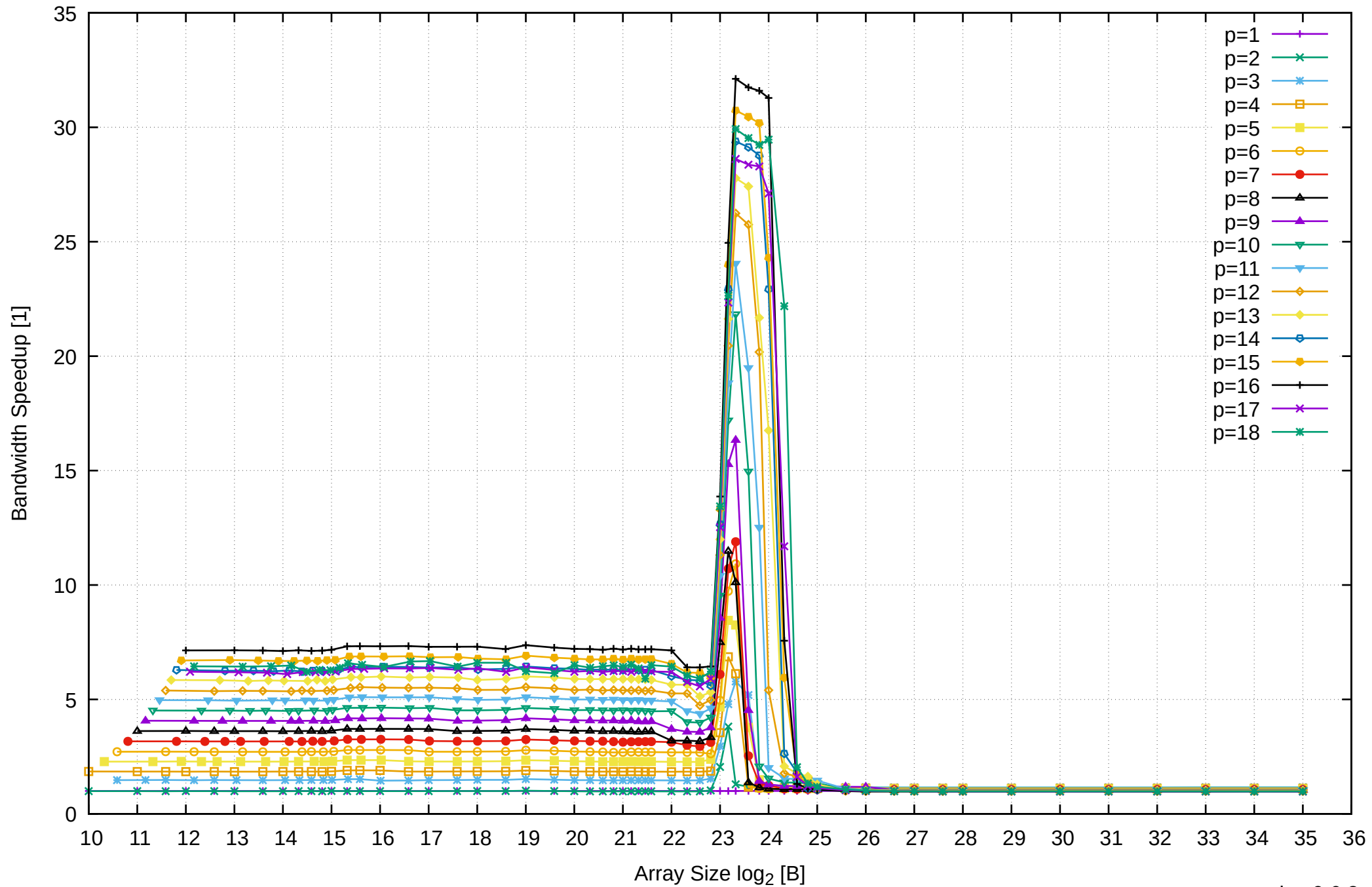
AMD Ryzen 7 1800X 64GB - Speedup of Parallel Memory Bandwidth - ScanWrite128PtrUnrollLoop
