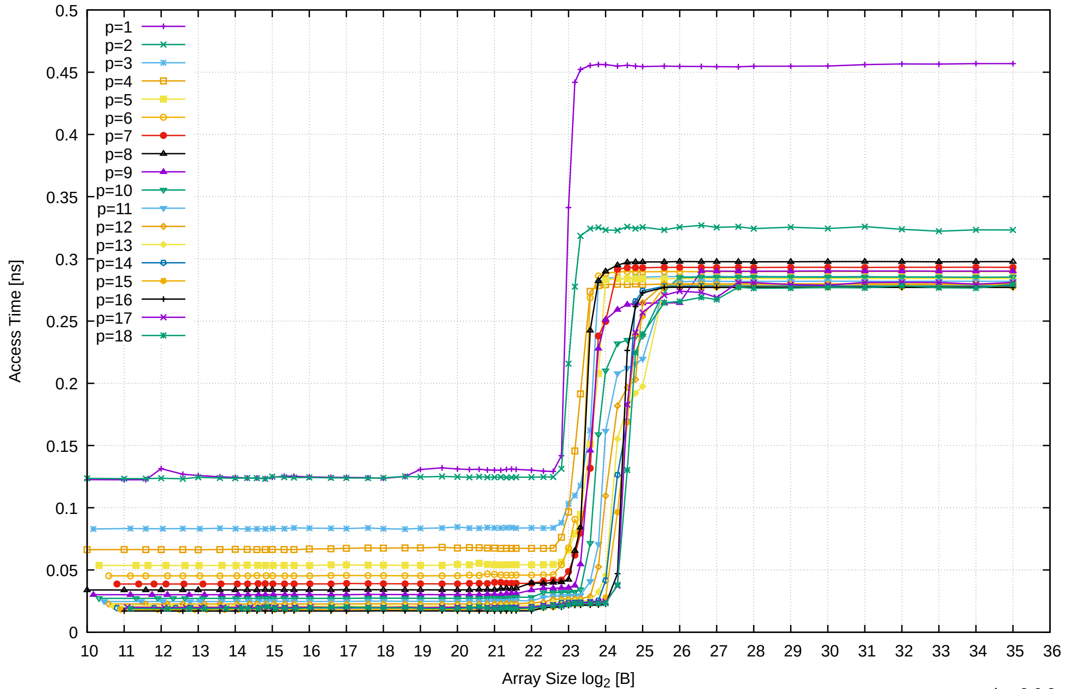
AMD Ryzen 7 1800X 64GB - Parallel Memory Access Time - ScanRead64IndexUnrollLoop
