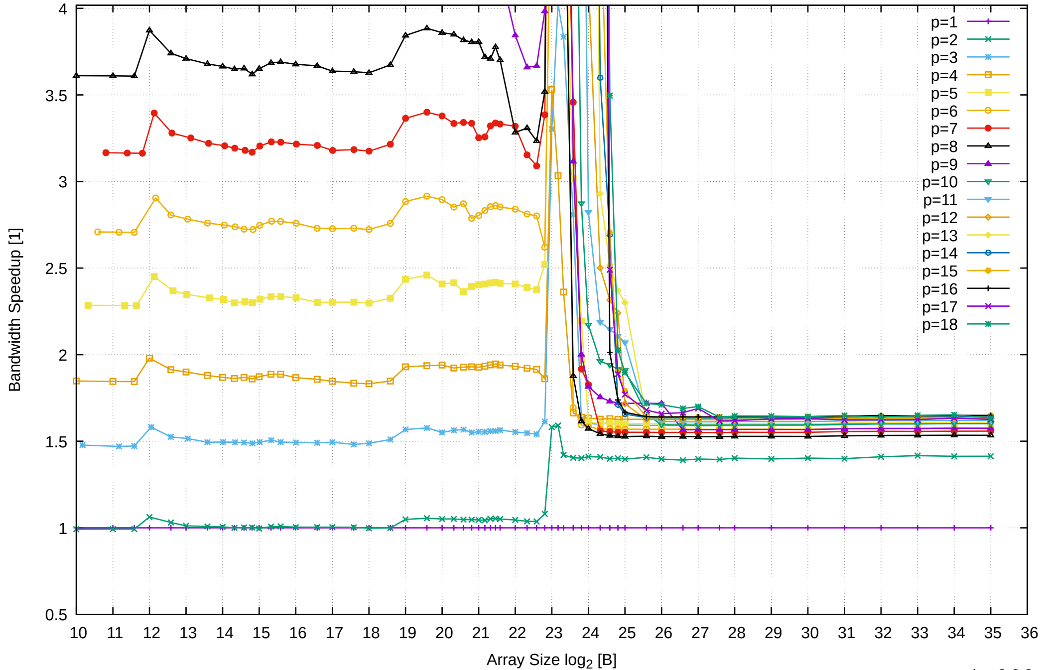
AMD Ryzen 7 1800X 64GB - Speedup of Parallel Memory Bandwidth (enlarged) - ScanRead64IndexUnrollLoop
