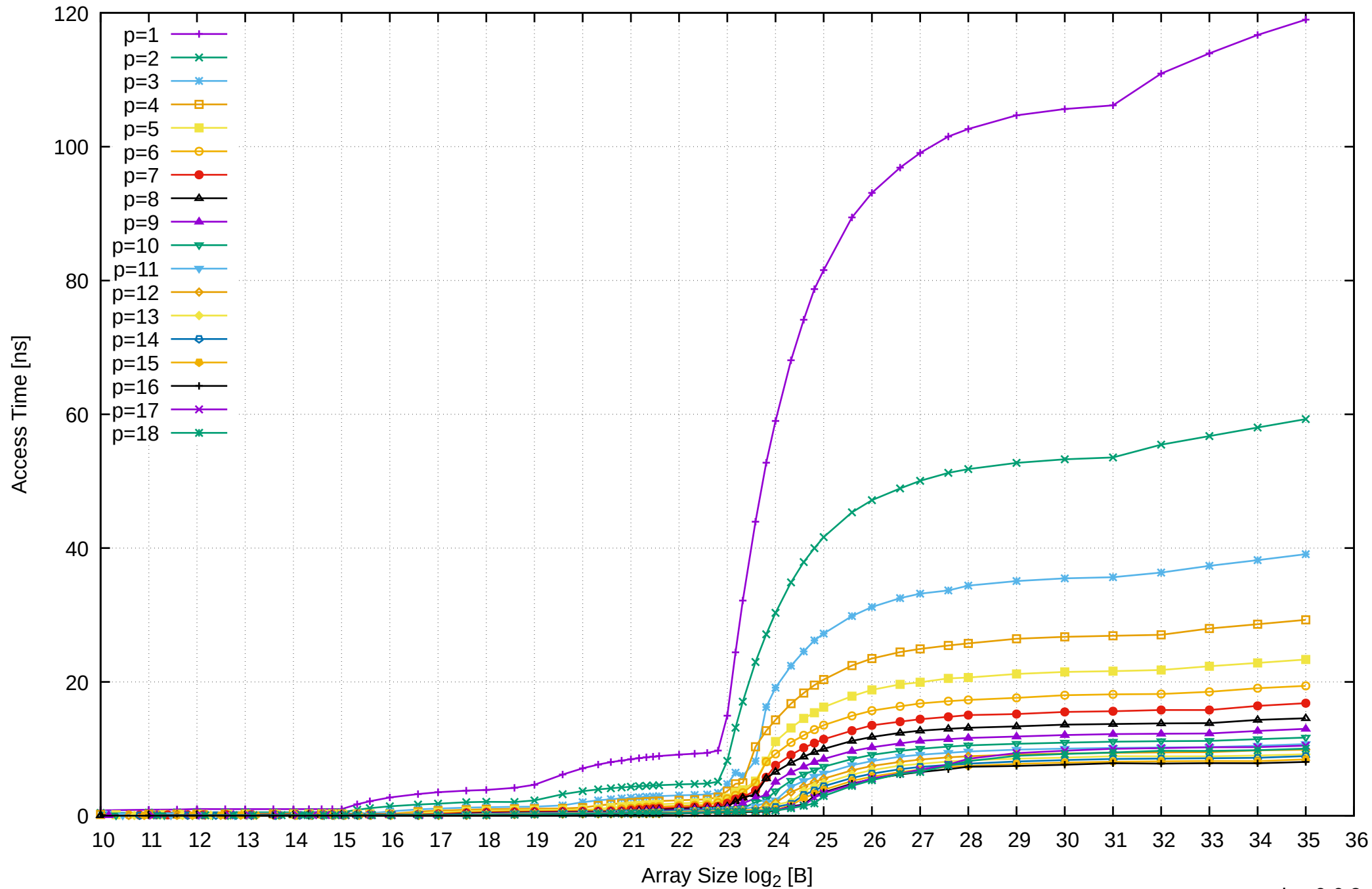
AMD Ryzen 7 1800X 64GB - Parallel Memory Access Time - PermRead64UnrollLoop
