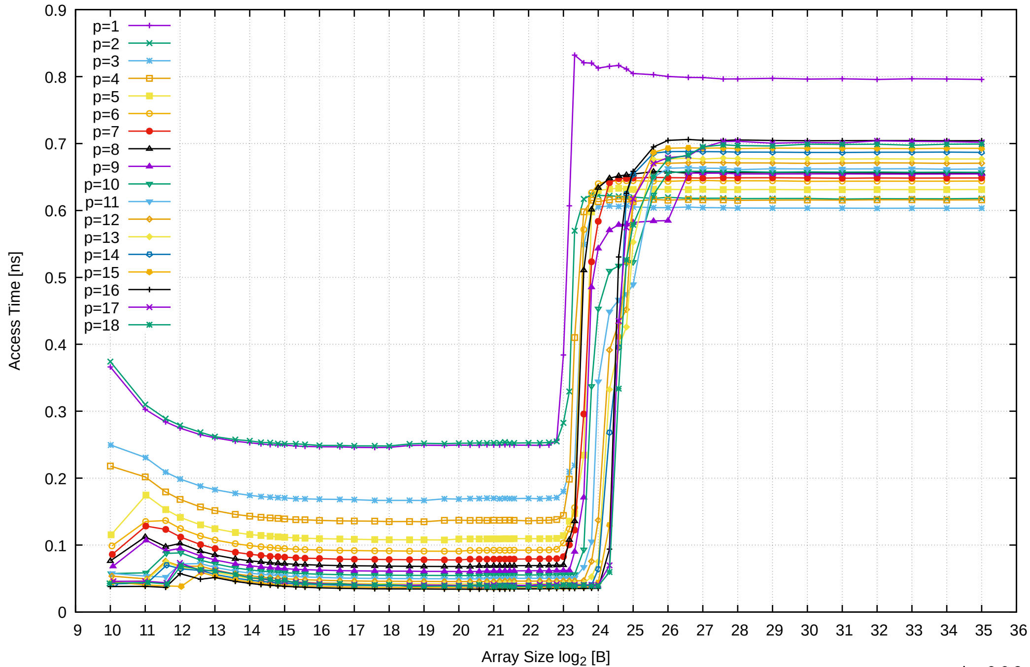
AMD Ryzen 7 1800X 64GB - Parallel Memory Access Time - ScanWrite64IndexSimpleLoop
