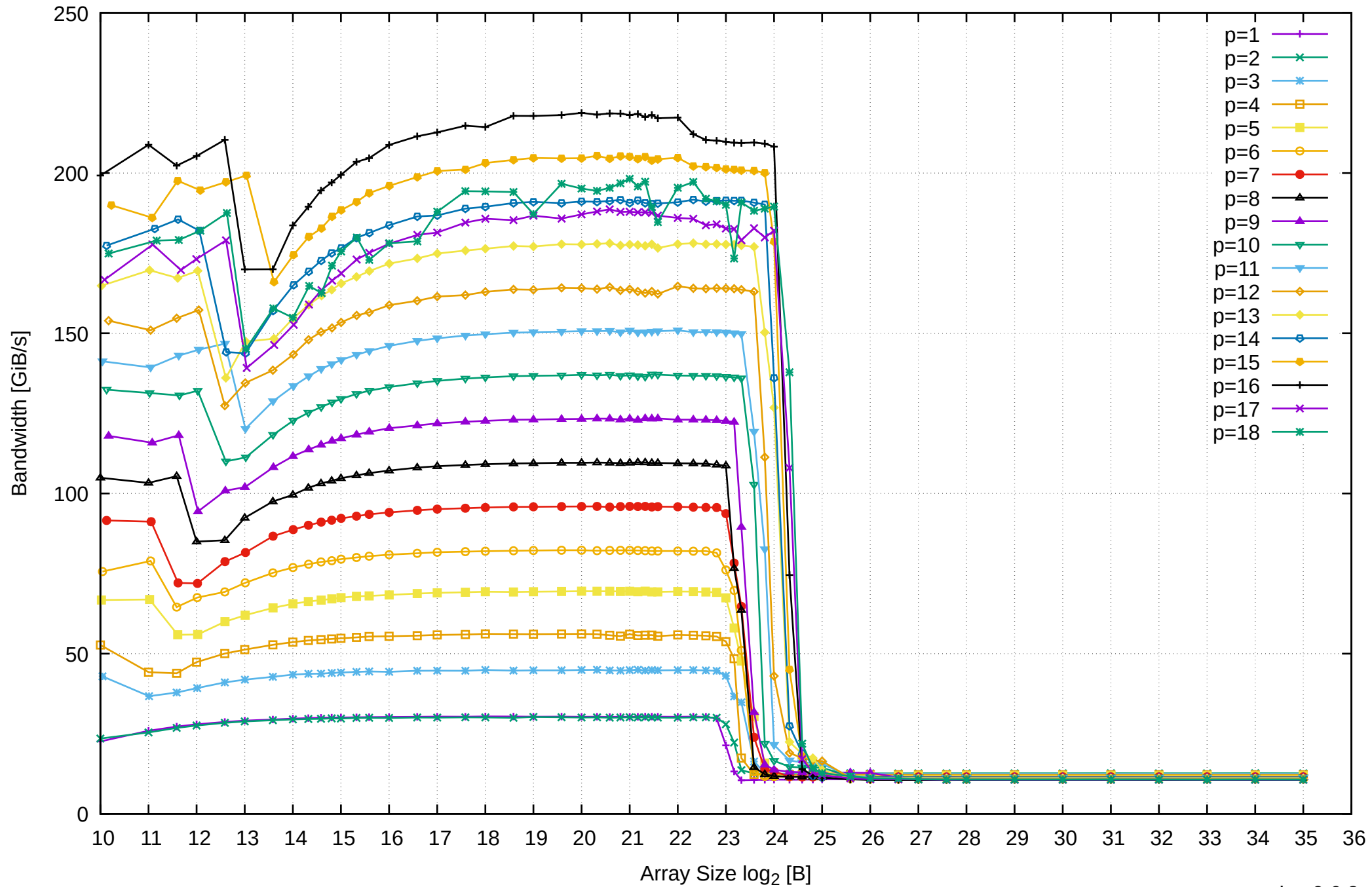
AMD Ryzen 7 1800X 64GB - Parallel Memory Bandwidth - ScanWrite128PtrSimpleLoop
