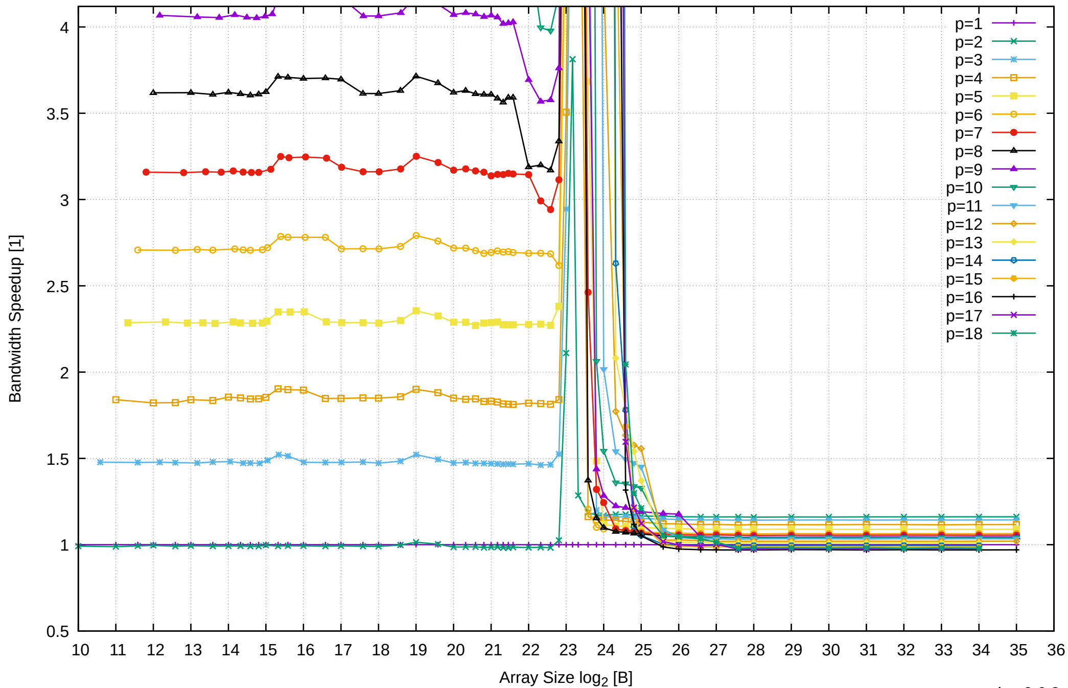
AMD Ryzen 7 1800X 64GB - Speedup of Parallel Memory Bandwidth (enlarged) - ScanWrite256PtrUnrollLoop
