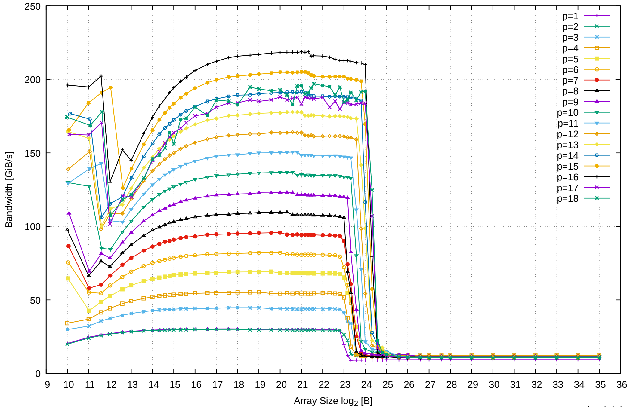
AMD Ryzen 7 1800X 64GB - Parallel Memory Bandwidth - ScanWrite64IndexSimpleLoop
