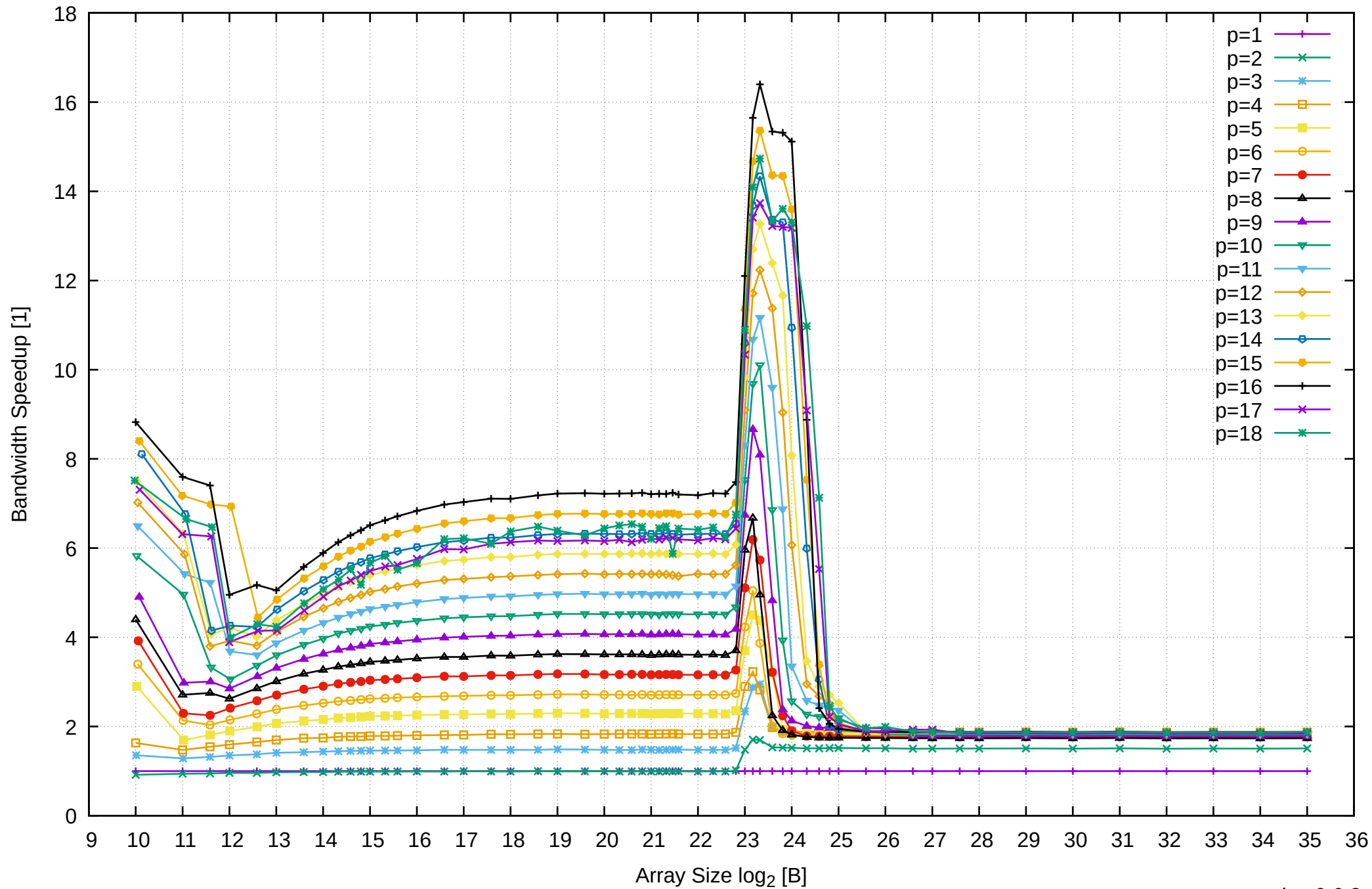
AMD Ryzen 7 1800X 64GB - Speedup of Parallel Memory Bandwidth - ScanRead64IndexSimpleLoop
