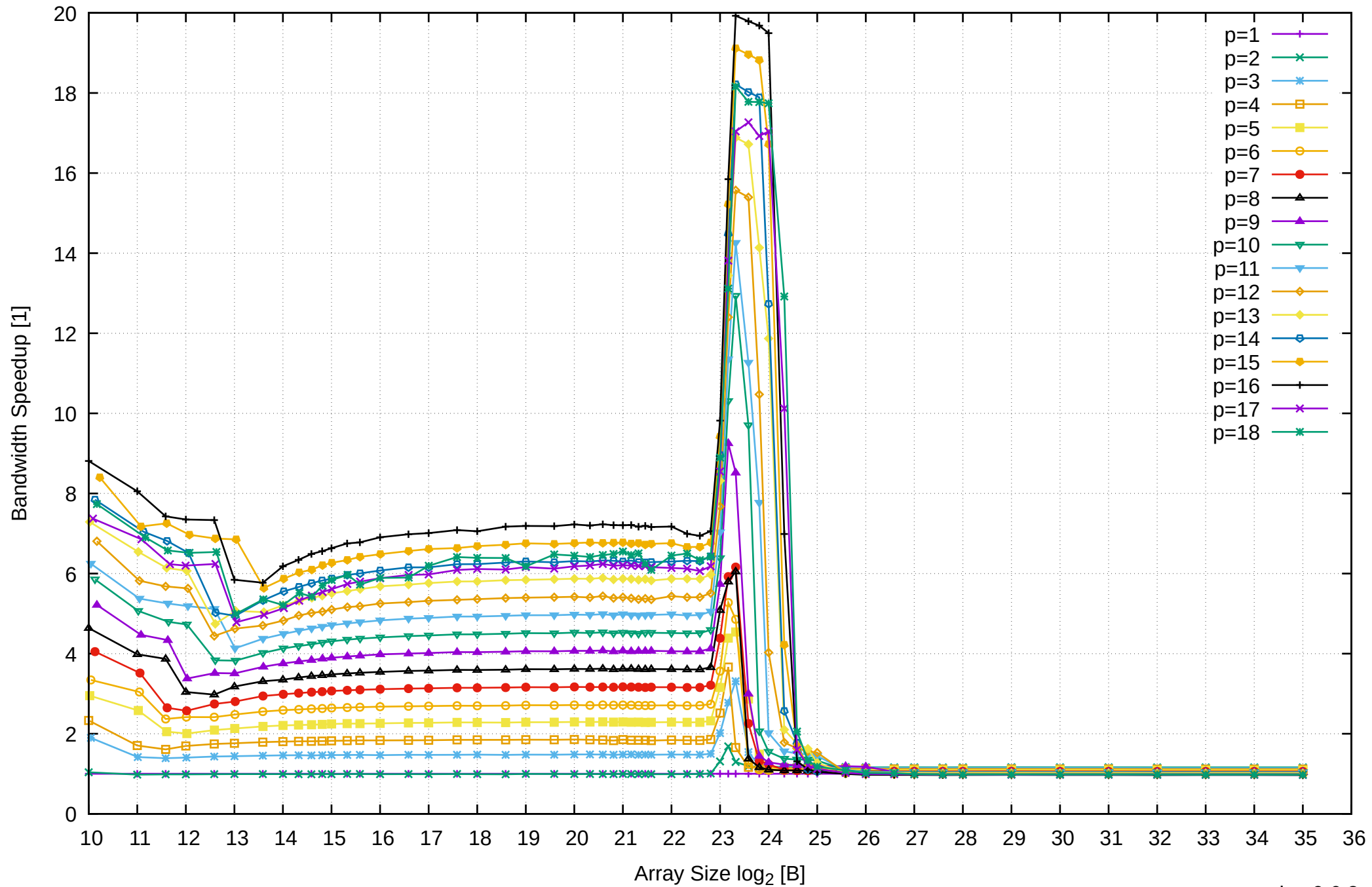
AMD Ryzen 7 1800X 64GB - Speedup of Parallel Memory Bandwidth - ScanWrite128PtrSimpleLoop
