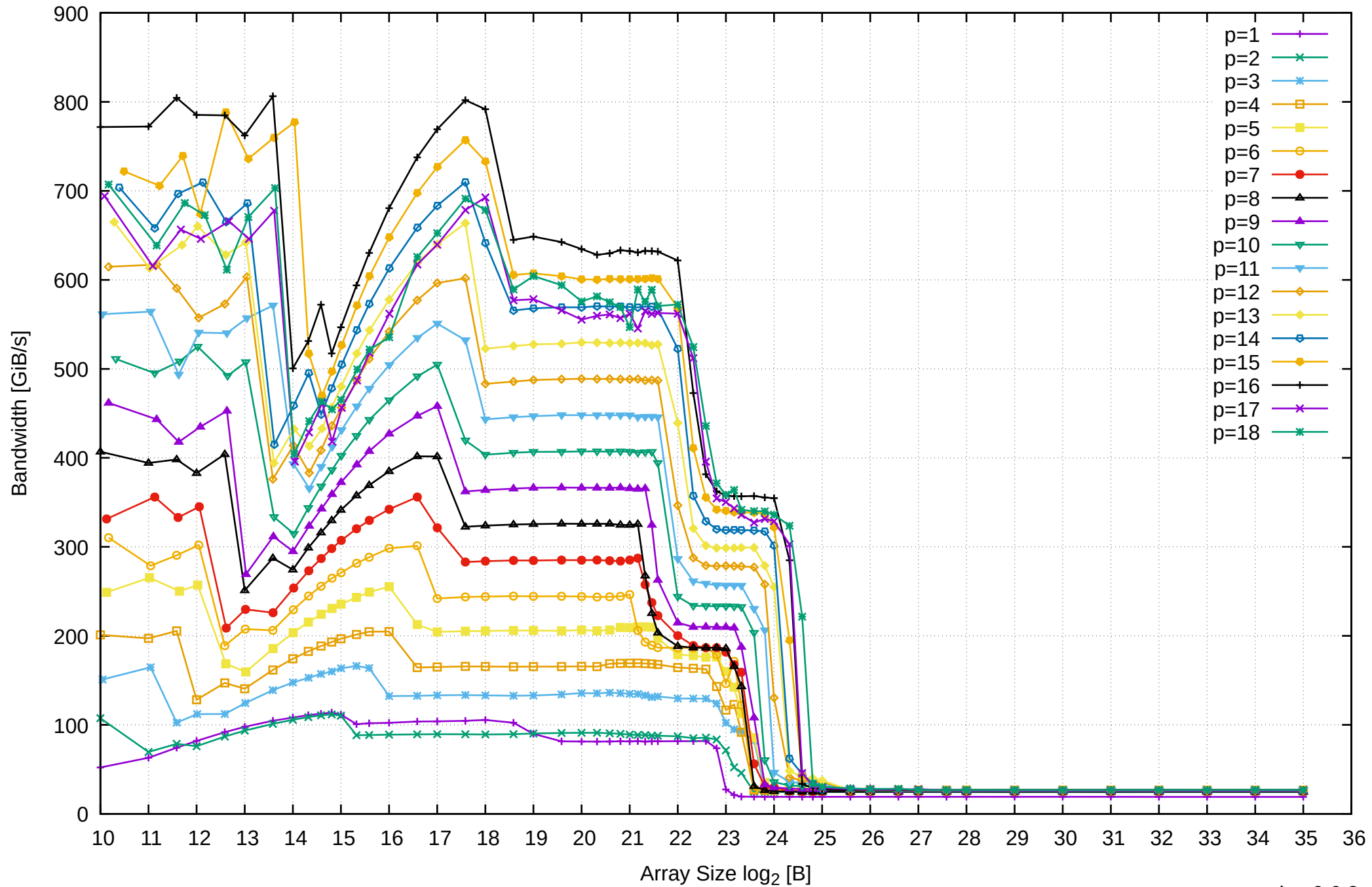
AMD Ryzen 7 1800X 64GB - Parallel Memory Bandwidth - ScanRead256PtrSimpleLoop
