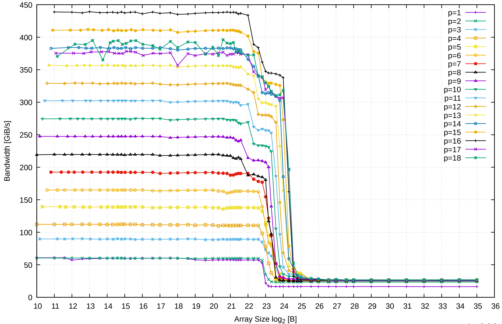
AMD Ryzen 7 1800X 64GB - Parallel Memory Bandwidth - ScanRead64PtrUnrollLoop
