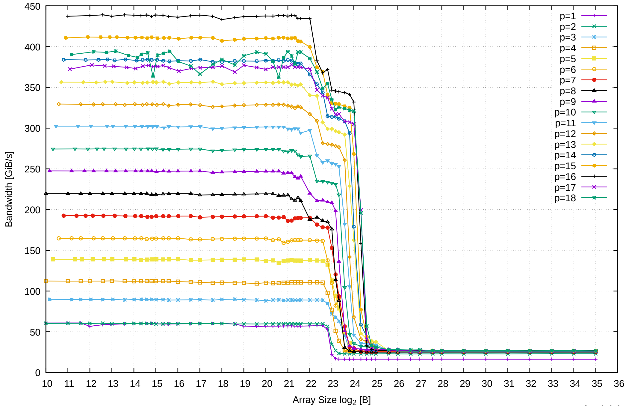
AMD Ryzen 7 1800X 64GB - Parallel Memory Bandwidth - ScanRead64IndexUnrollLoop
