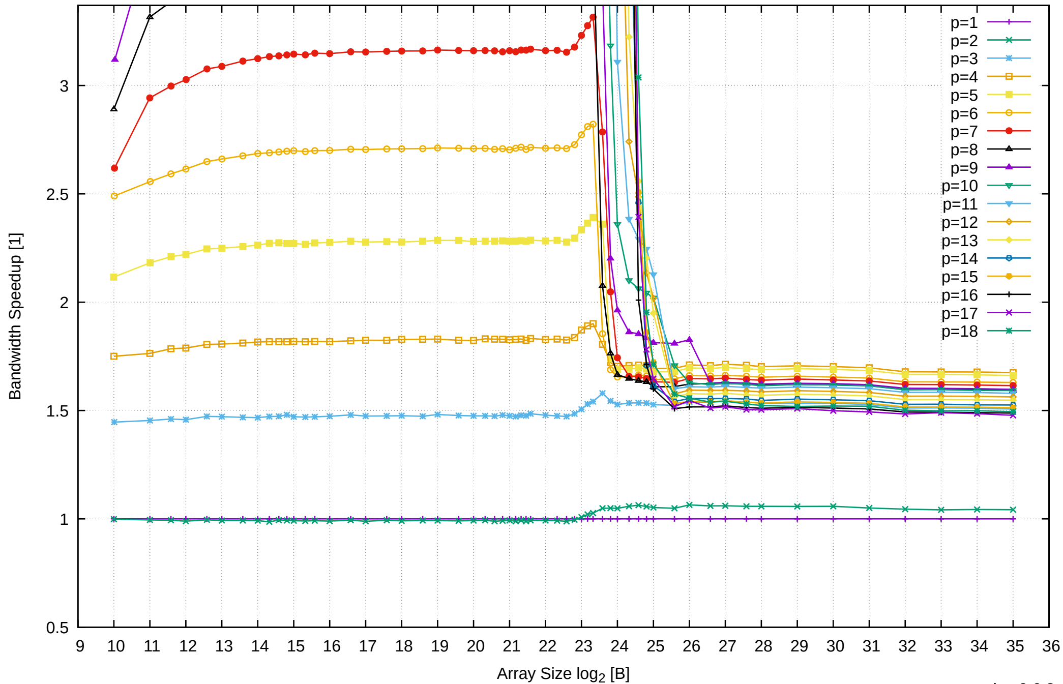
AMD Ryzen 7 1800X 64GB - Speedup of Parallel Memory Bandwidth (enlarged) - ScanWrite32PtrSimpleLoop
