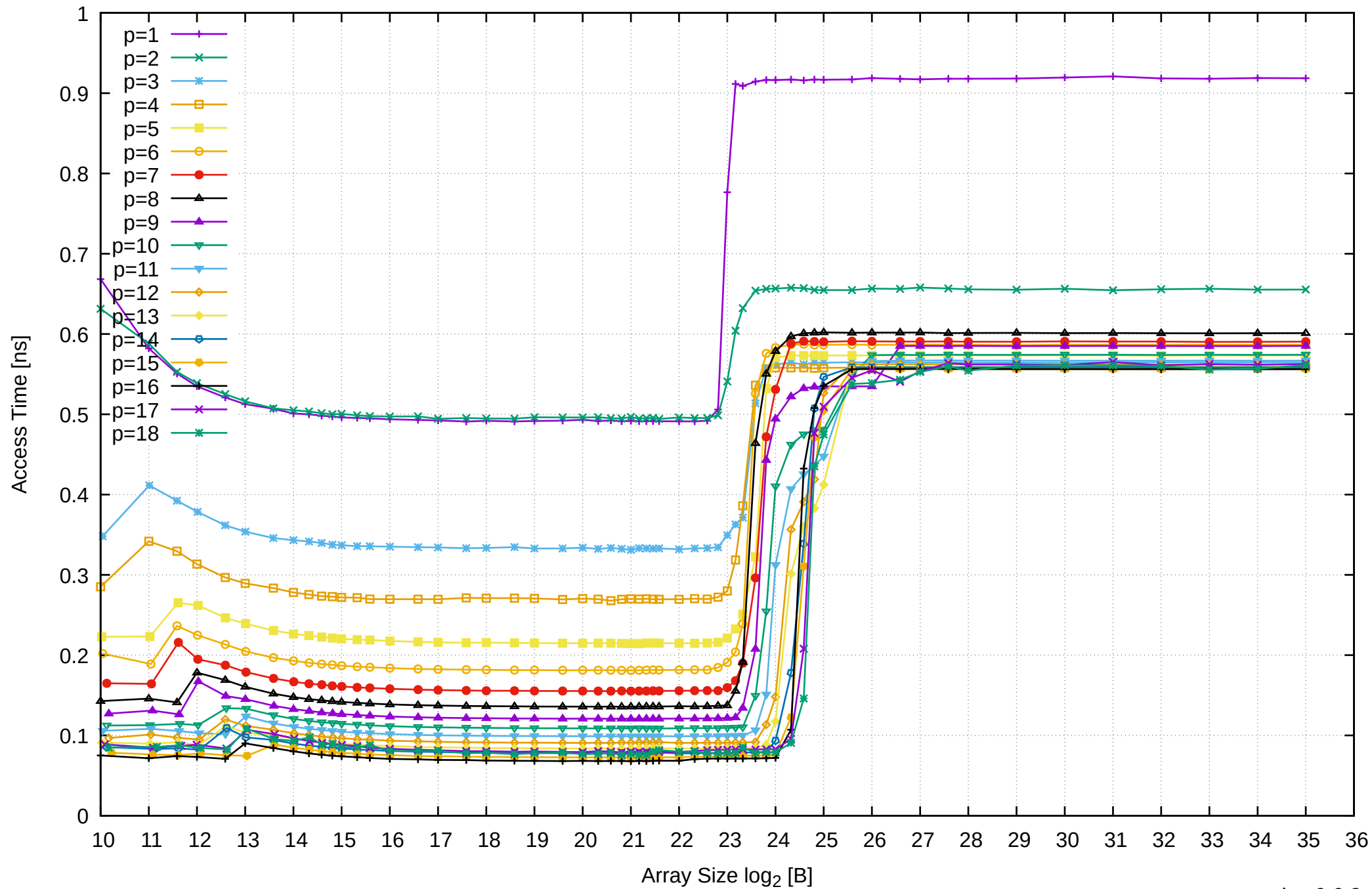
AMD Ryzen 7 1800X 64GB - Parallel Memory Access Time - ScanRead128PtrSimpleLoop
