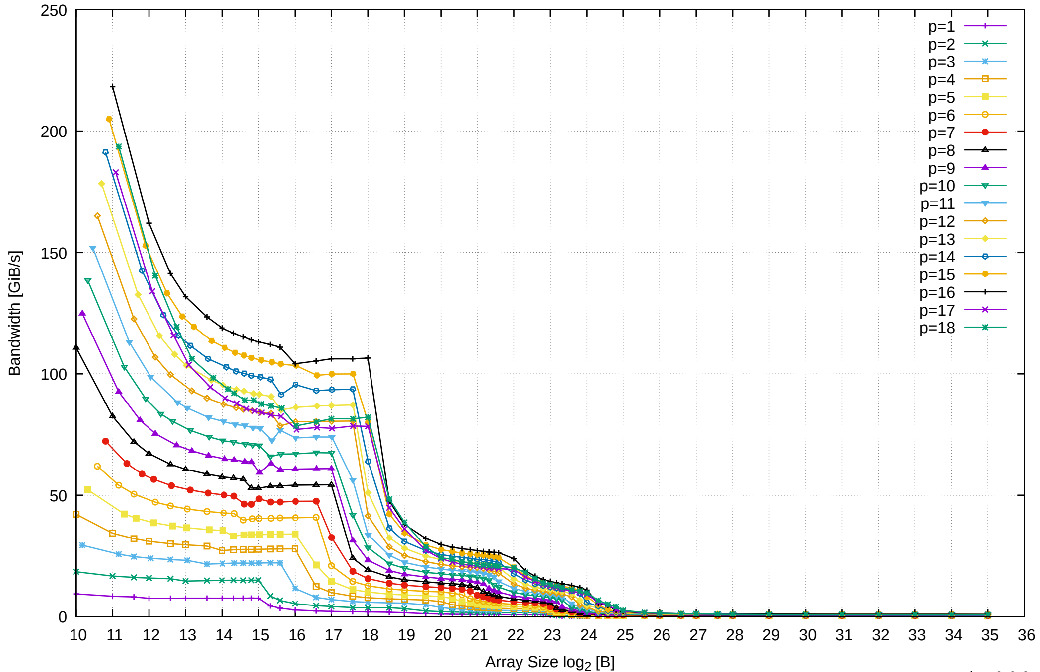
AMD Ryzen 7 1800X 64GB - Parallel Memory Bandwidth - PermRead64UnrollLoop
