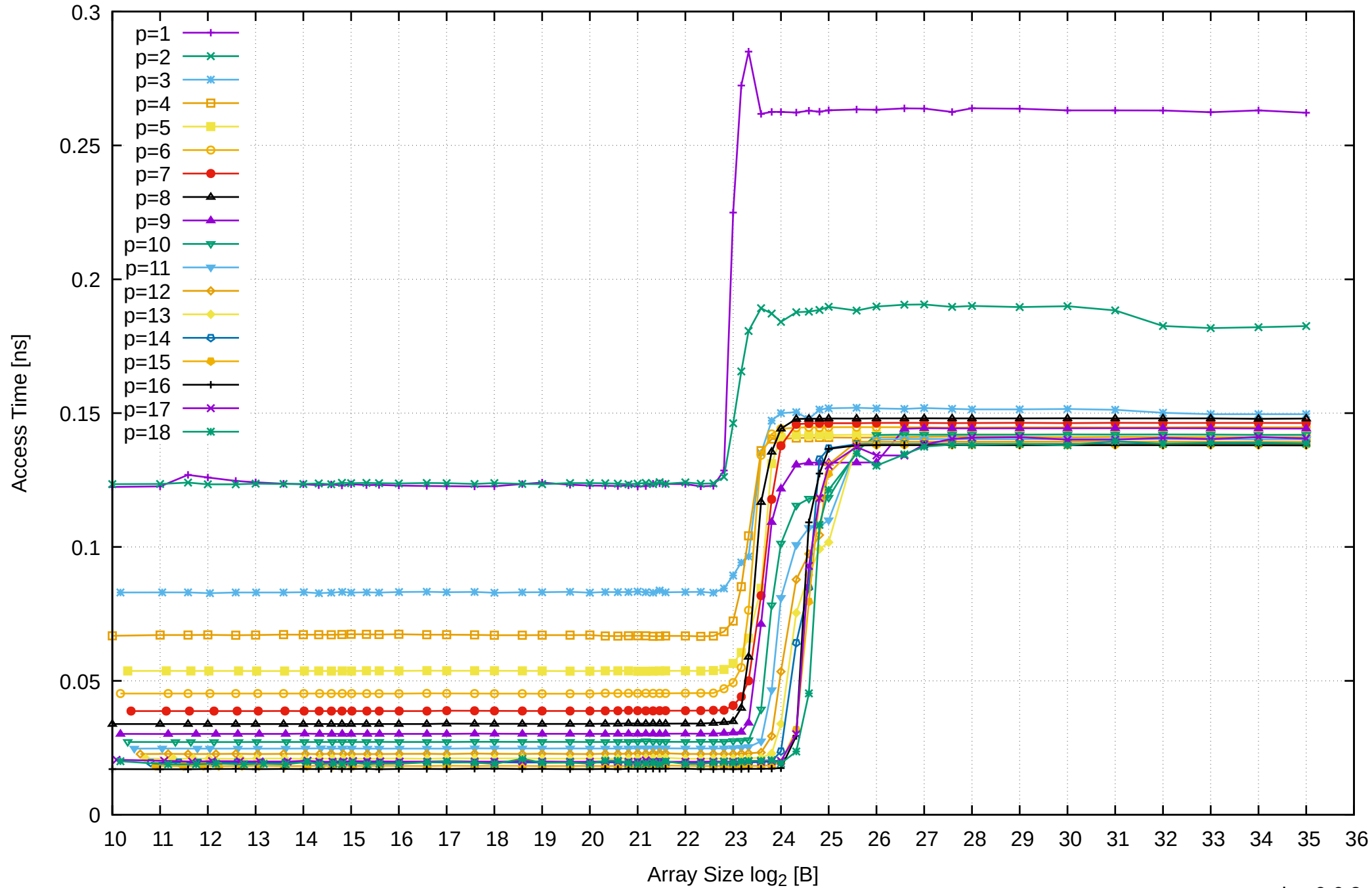
AMD Ryzen 7 1800X 64GB - Parallel Memory Access Time - ScanRead32PtrUnrollLoop
