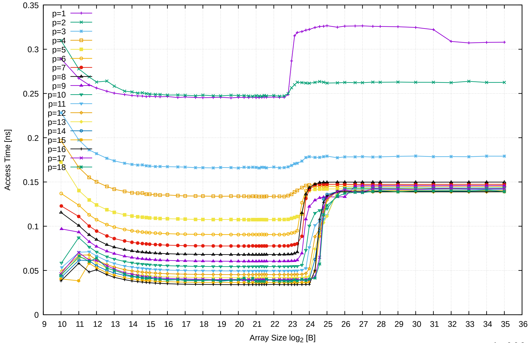
AMD Ryzen 7 1800X 64GB - Parallel Memory Access Time - ScanRead32PtrSimpleLoop
