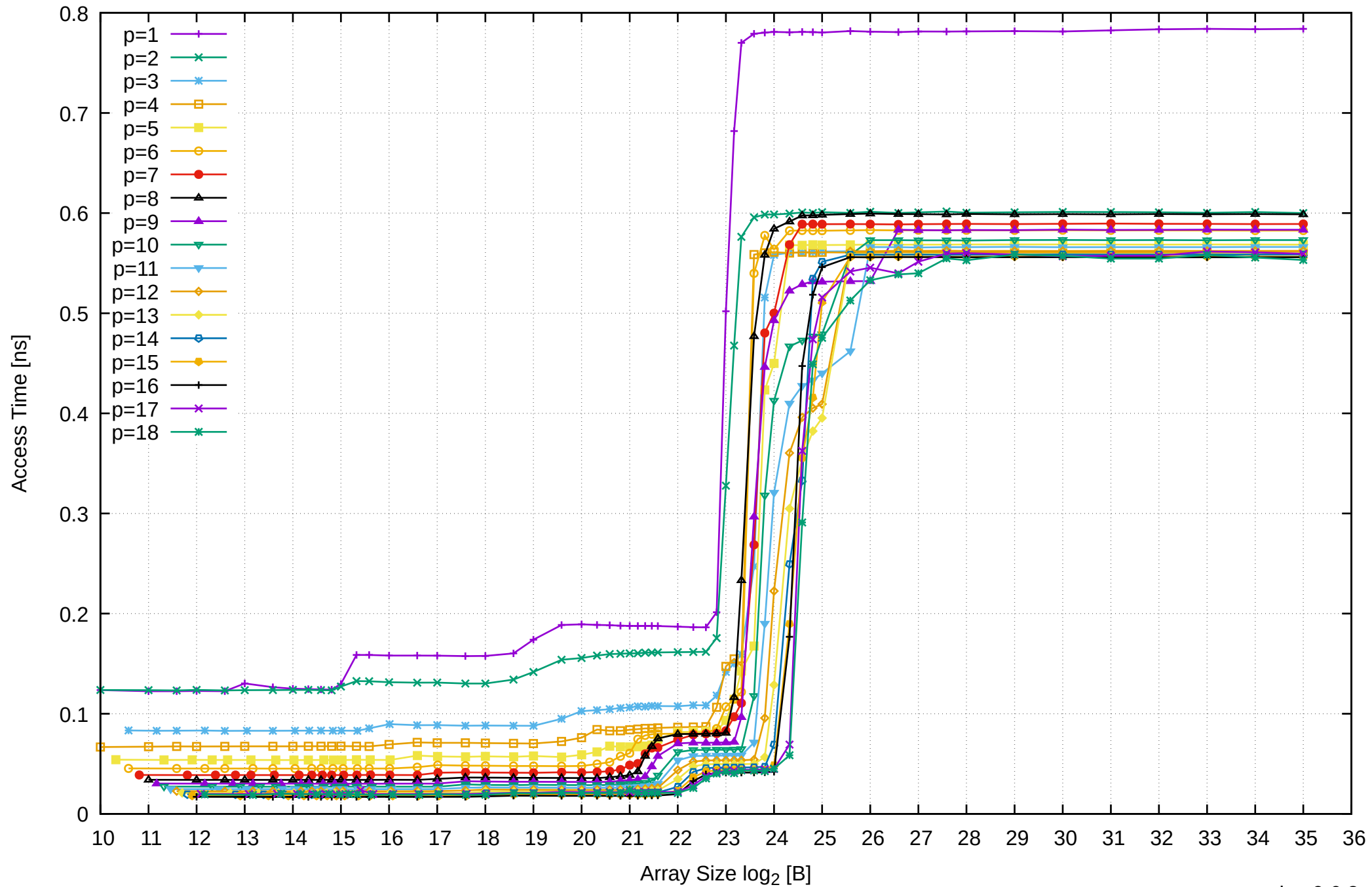
AMD Ryzen 7 1800X 64GB - Parallel Memory Access Time - ScanRead128PtrUnrollLoop
