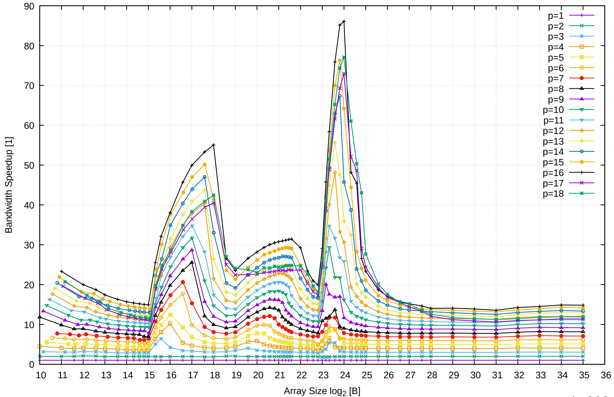
AMD Ryzen 7 1800X 64GB - Speedup of Parallel Memory Bandwidth - PermRead64UnrollLoop
