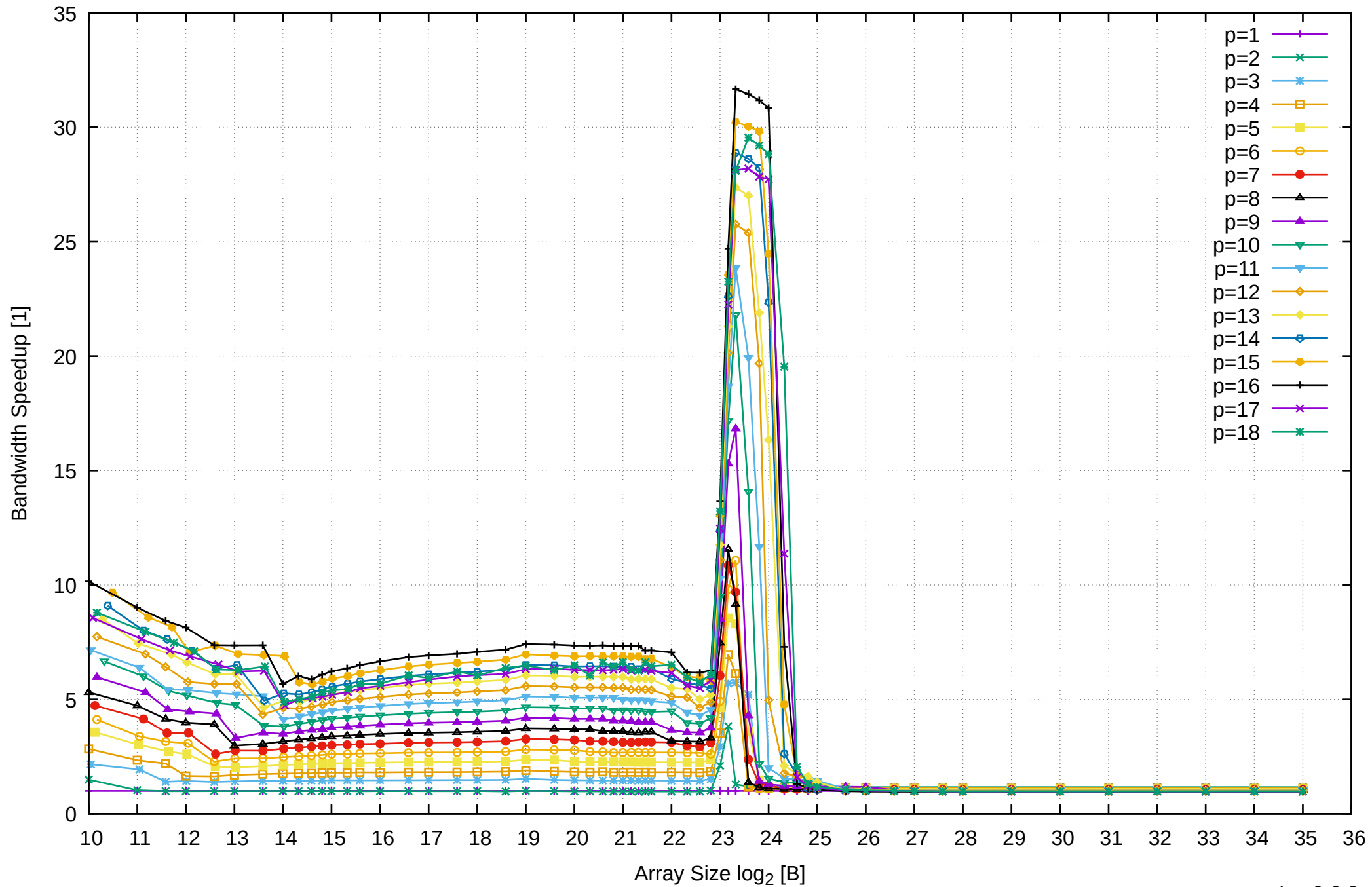
AMD Ryzen 7 1800X 64GB - Speedup of Parallel Memory Bandwidth - ScanWrite256PtrSimpleLoop
