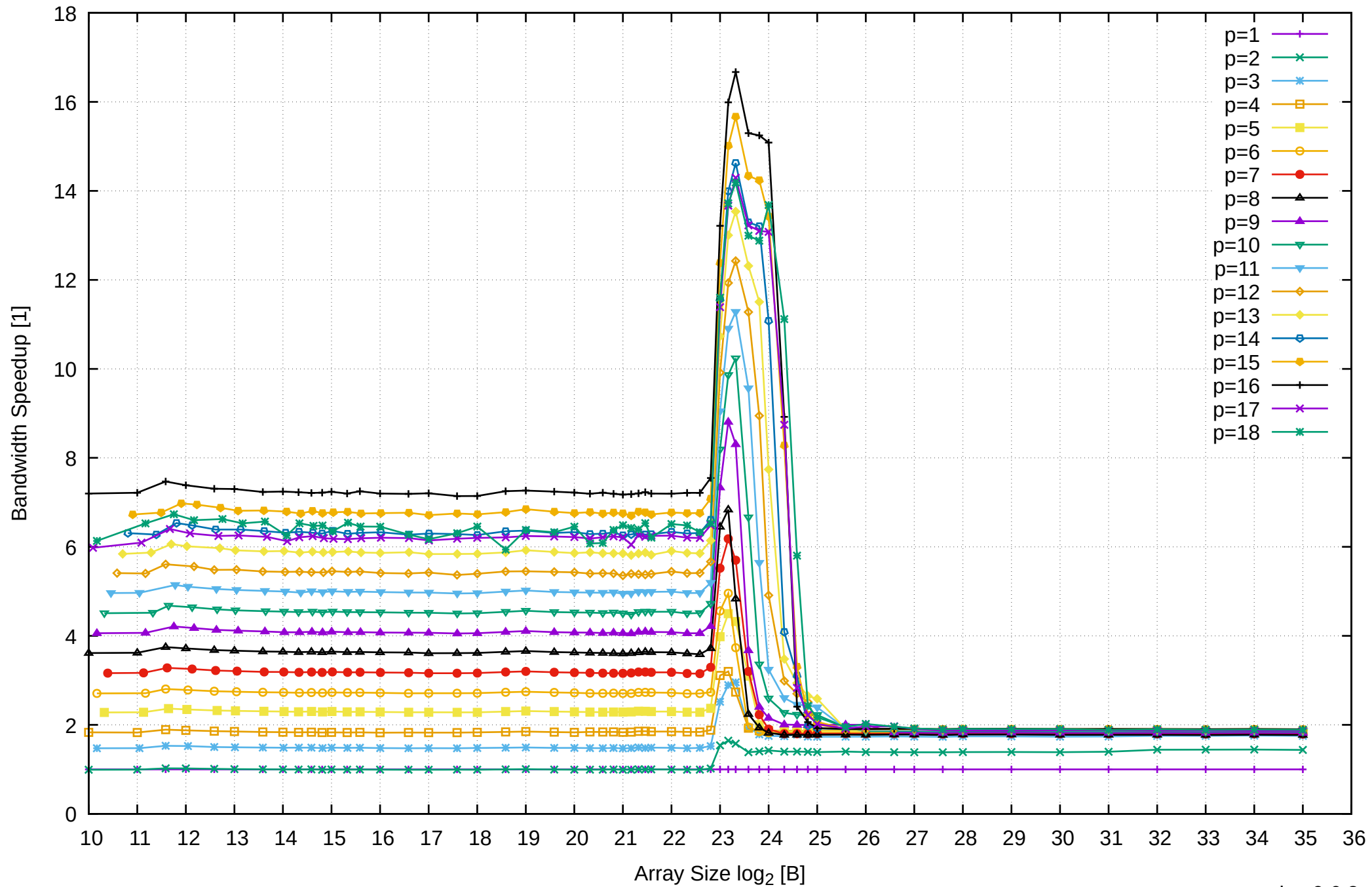
AMD Ryzen 7 1800X 64GB - Speedup of Parallel Memory Bandwidth - ScanRead32PtrUnrollLoop
