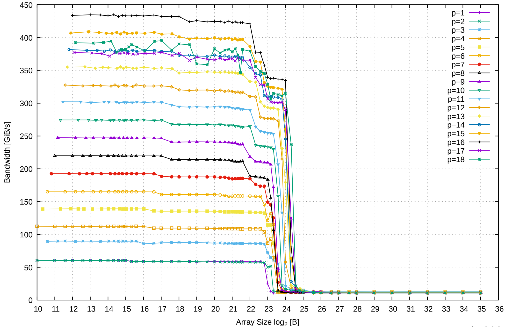
AMD Ryzen 7 1800X 64GB - Parallel Memory Bandwidth - ScanWrite128PtrUnrollLoop
