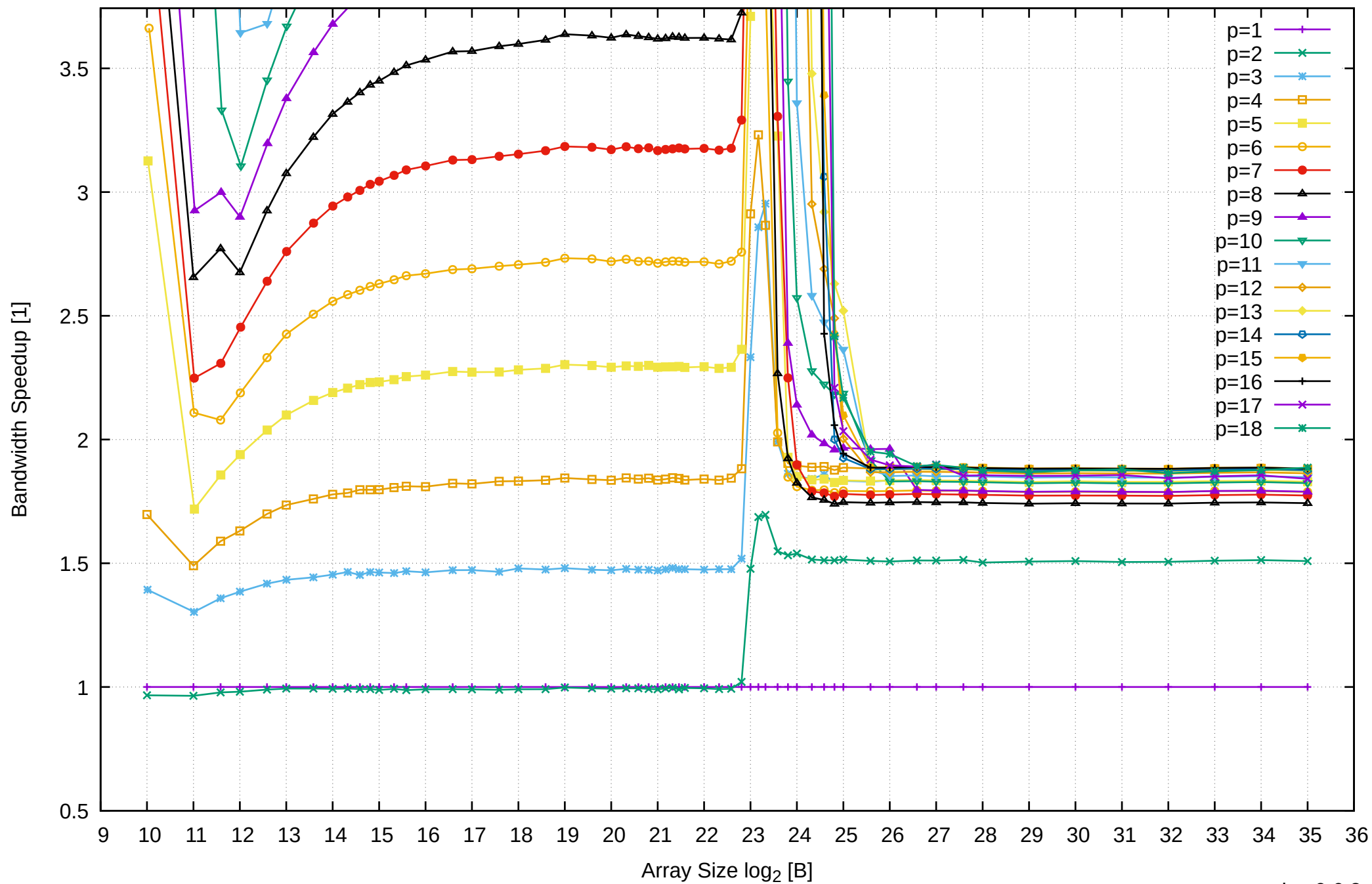
AMD Ryzen 7 1800X 64GB - Speedup of Parallel Memory Bandwidth (enlarged) - ScanRead64PtrSimpleLoop
