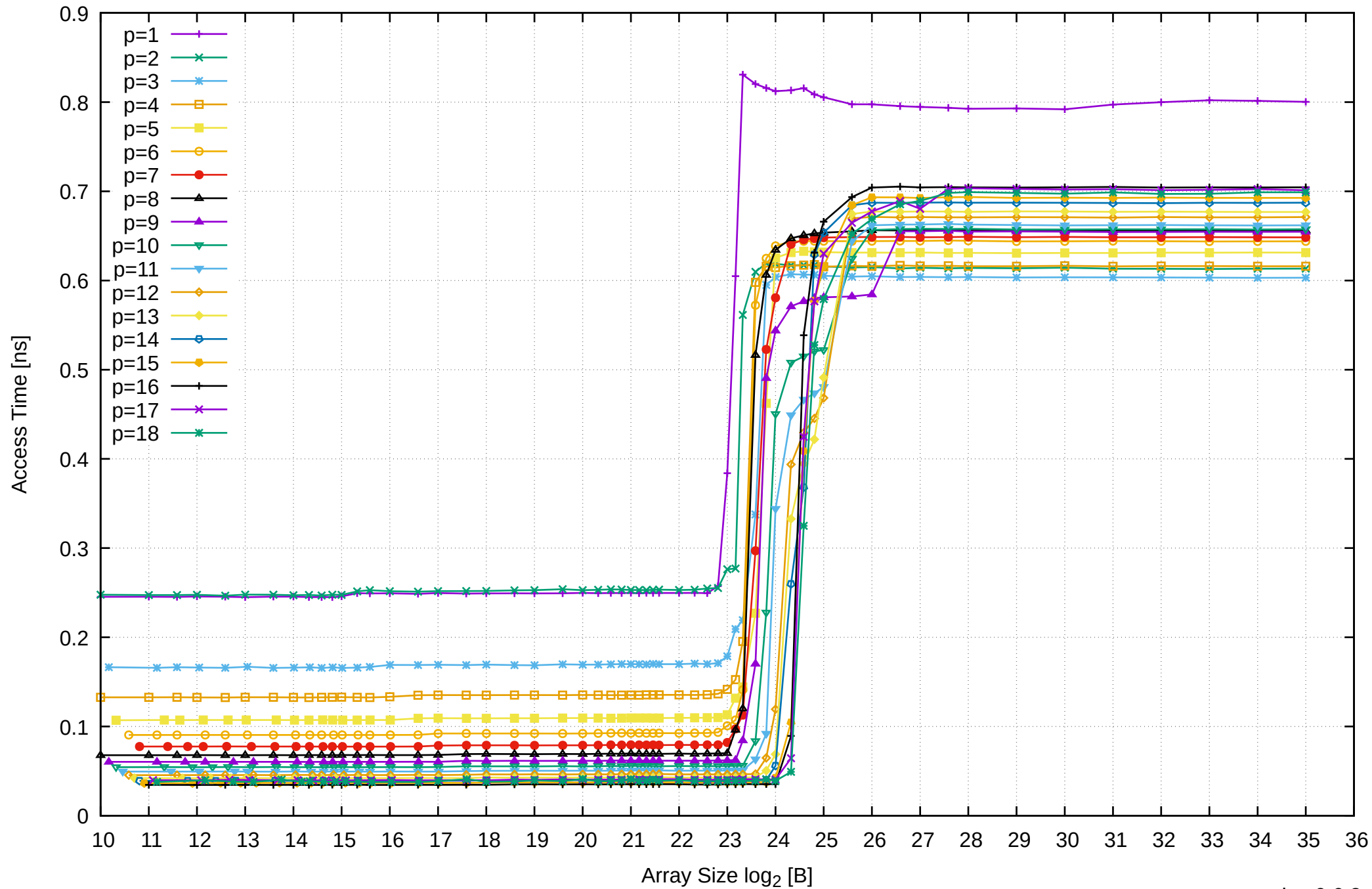
AMD Ryzen 7 1800X 64GB - Parallel Memory Access Time - ScanWrite64IndexUnrollLoop
