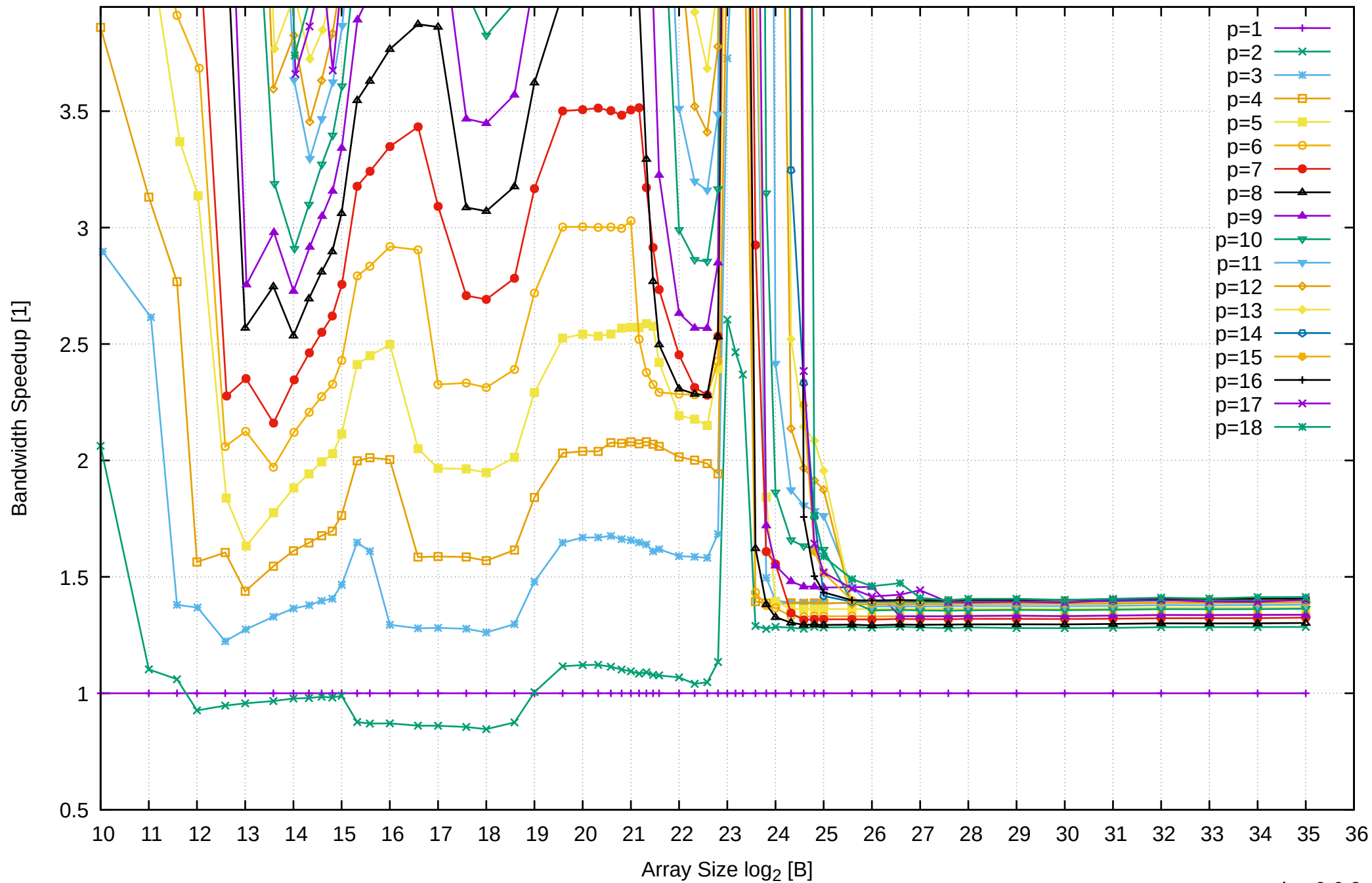
AMD Ryzen 7 1800X 64GB - Speedup of Parallel Memory Bandwidth (enlarged) - ScanRead256PtrSimpleLoop
