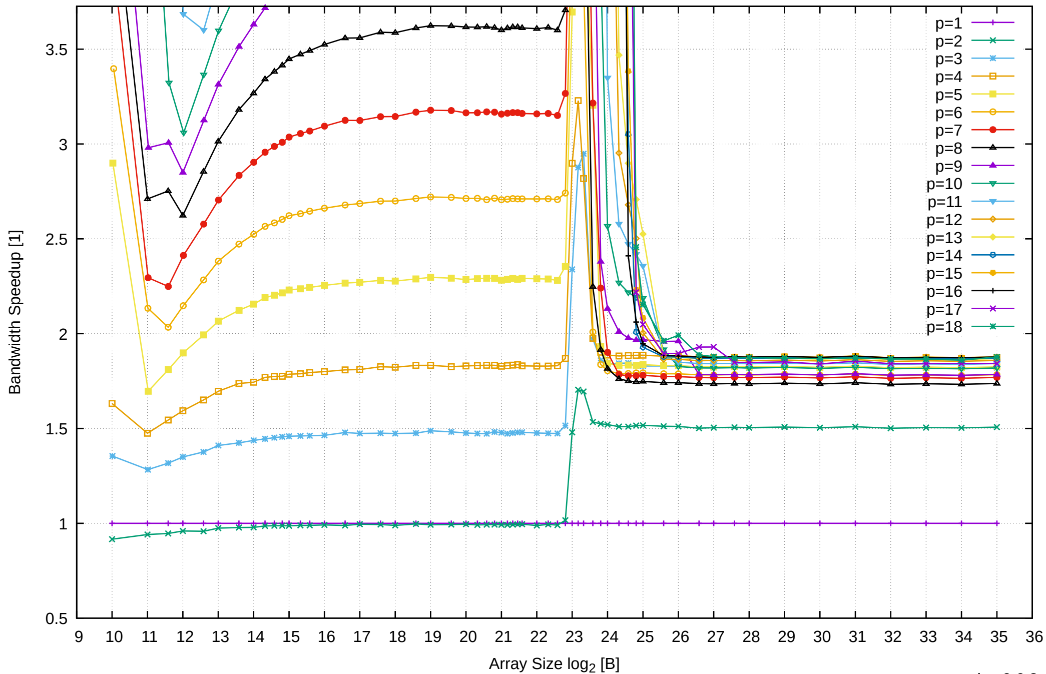
AMD Ryzen 7 1800X 64GB - Speedup of Parallel Memory Bandwidth (enlarged) - ScanRead64IndexSimpleLoop
