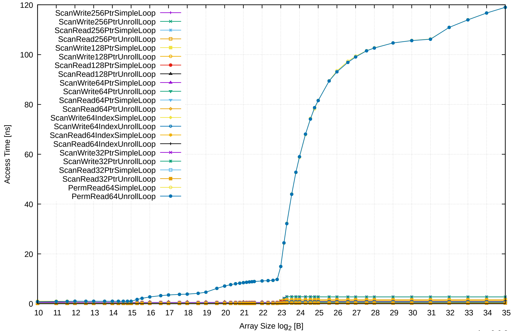
AMD Ryzen 7 1800X 64GB - One Thread Memory Latency (Access Time)
