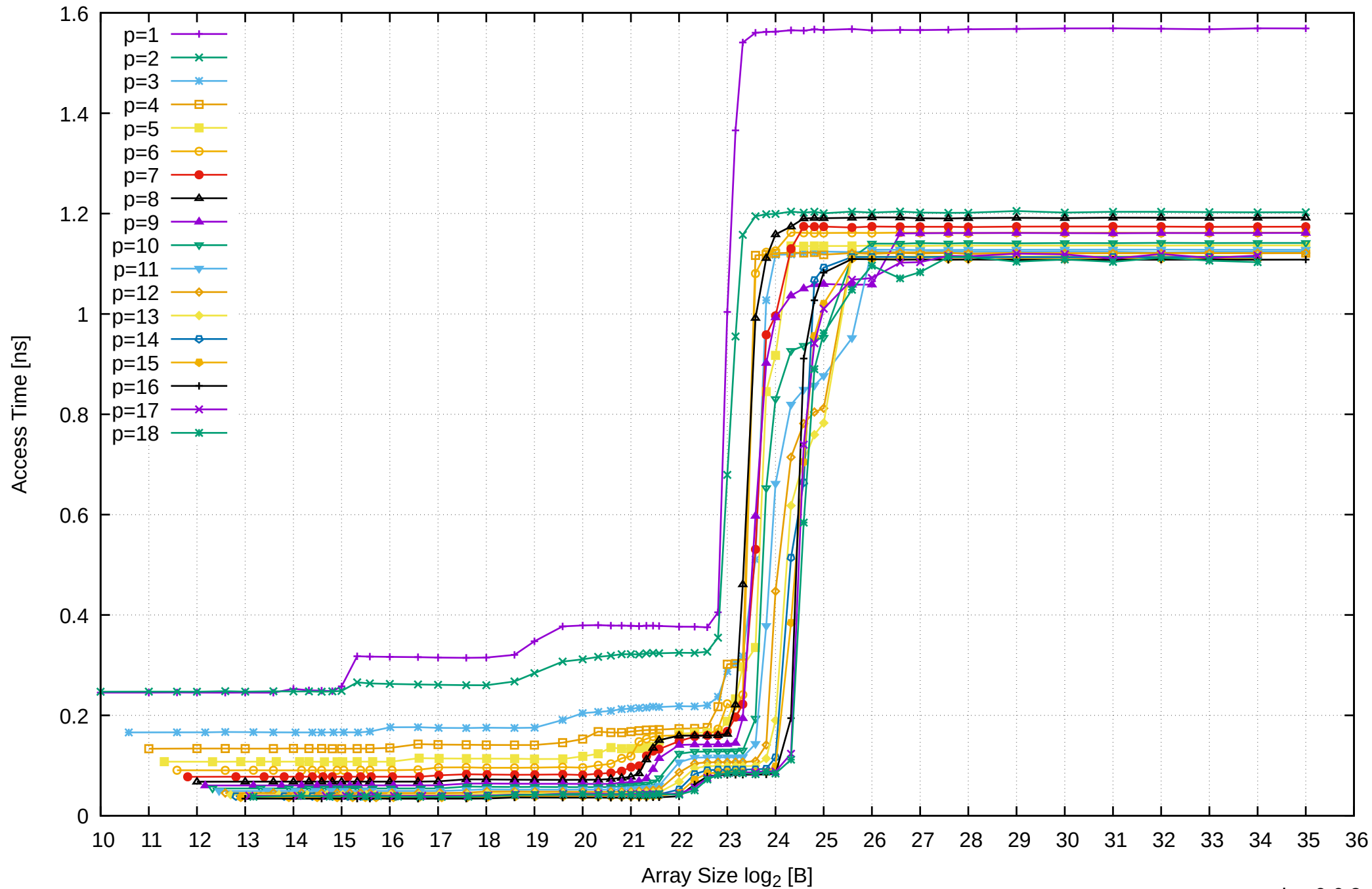
AMD Ryzen 7 1800X 64GB - Parallel Memory Access Time - ScanRead256PtrUnrollLoop
