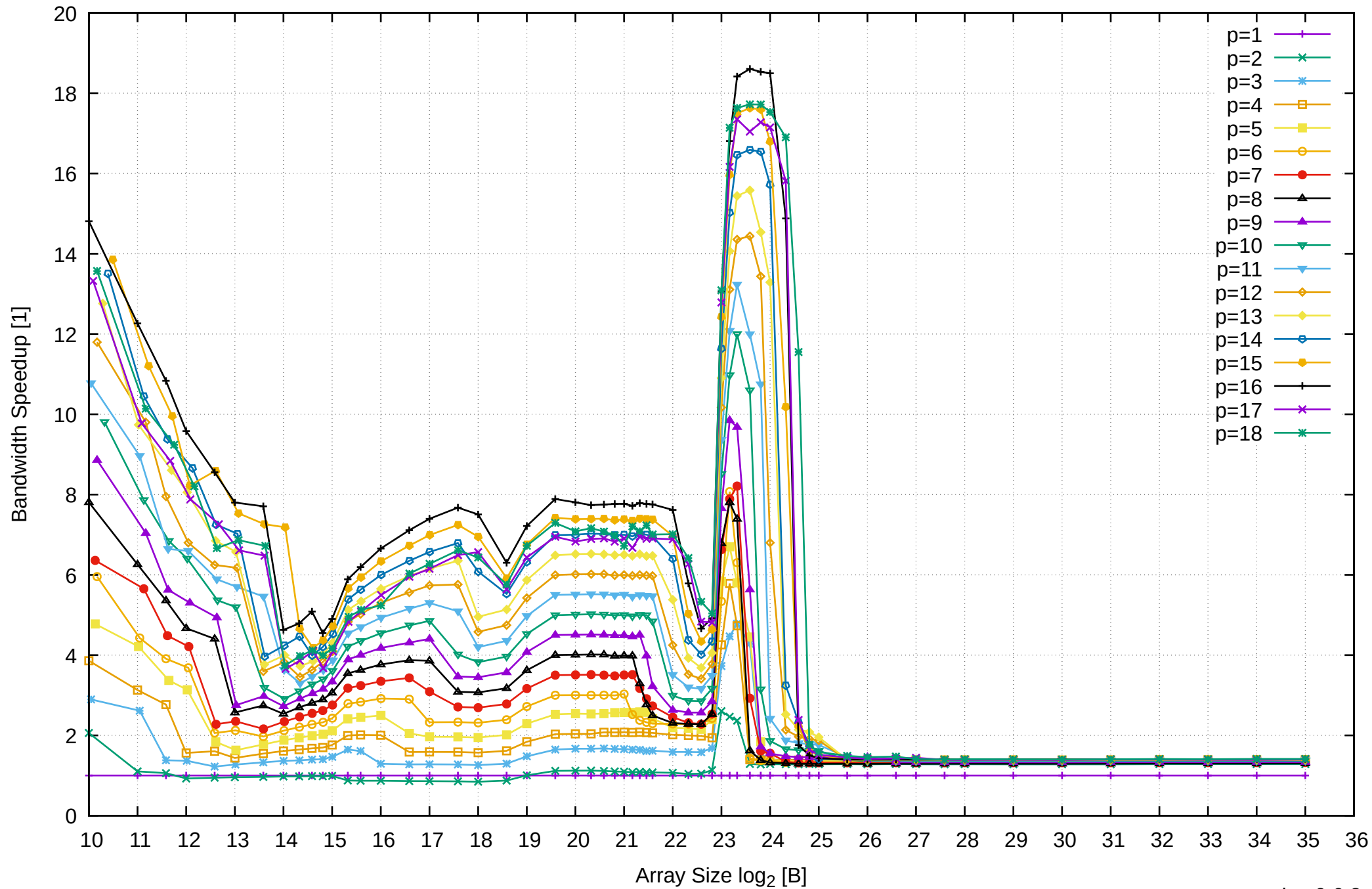
AMD Ryzen 7 1800X 64GB - Speedup of Parallel Memory Bandwidth - ScanRead256PtrSimpleLoop
