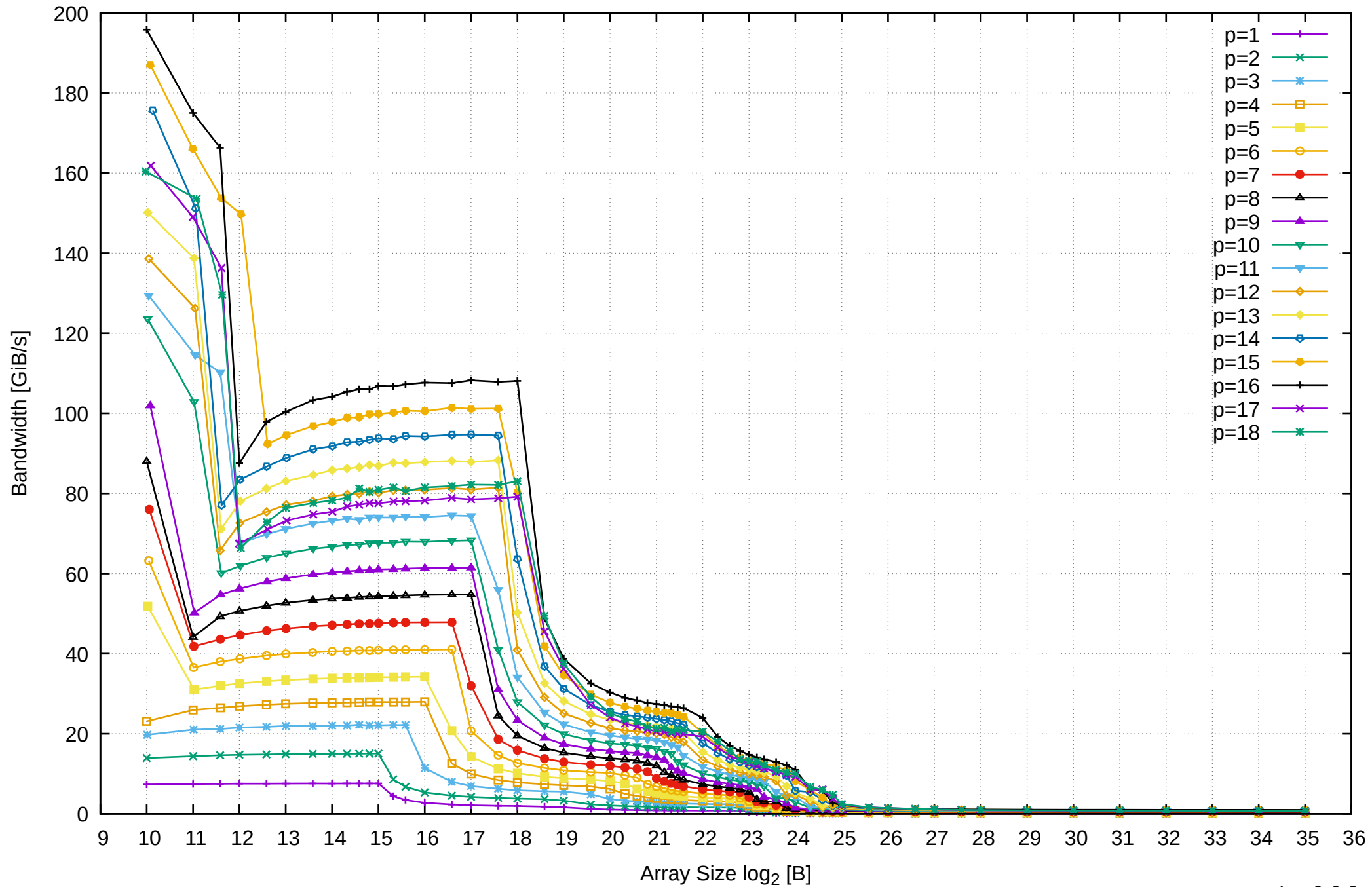
AMD Ryzen 7 1800X 64GB - Parallel Memory Bandwidth - PermRead64SimpleLoop
