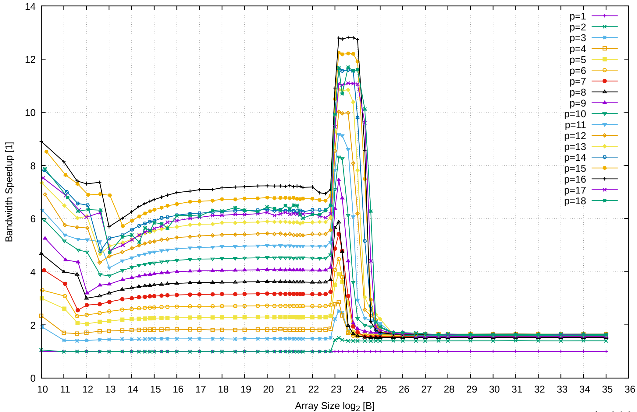
AMD Ryzen 7 1800X 64GB - Speedup of Parallel Memory Bandwidth - ScanRead128PtrSimpleLoop
