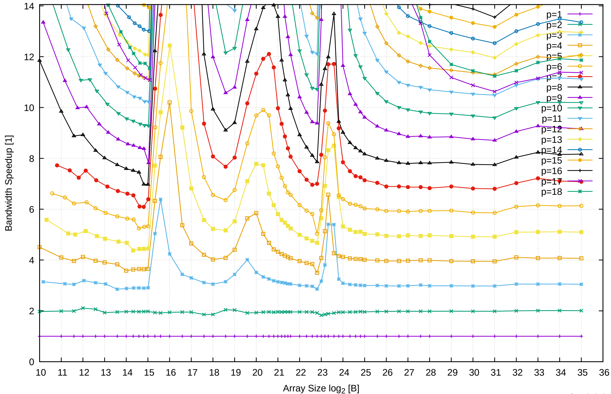
AMD Ryzen 7 1800X 64GB - Speedup of Parallel Memory Bandwidth (enlarged) - PermRead64UnrollLoop
