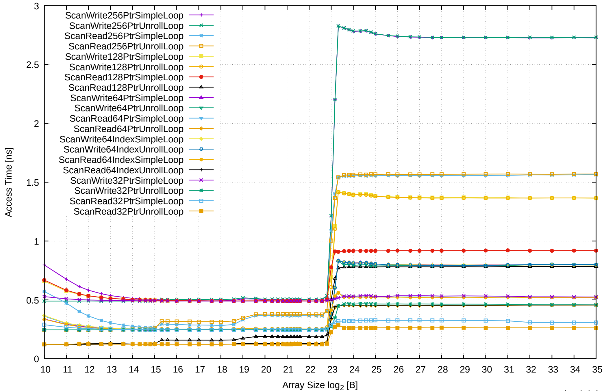
AMD Ryzen 7 1800X 64GB - One Thread Memory Latency (excluding Permutation)
