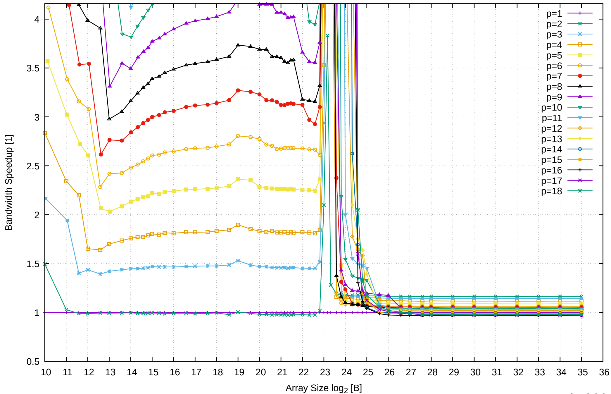
AMD Ryzen 7 1800X 64GB - Speedup of Parallel Memory Bandwidth (enlarged) - ScanWrite256PtrSimpleLoop
