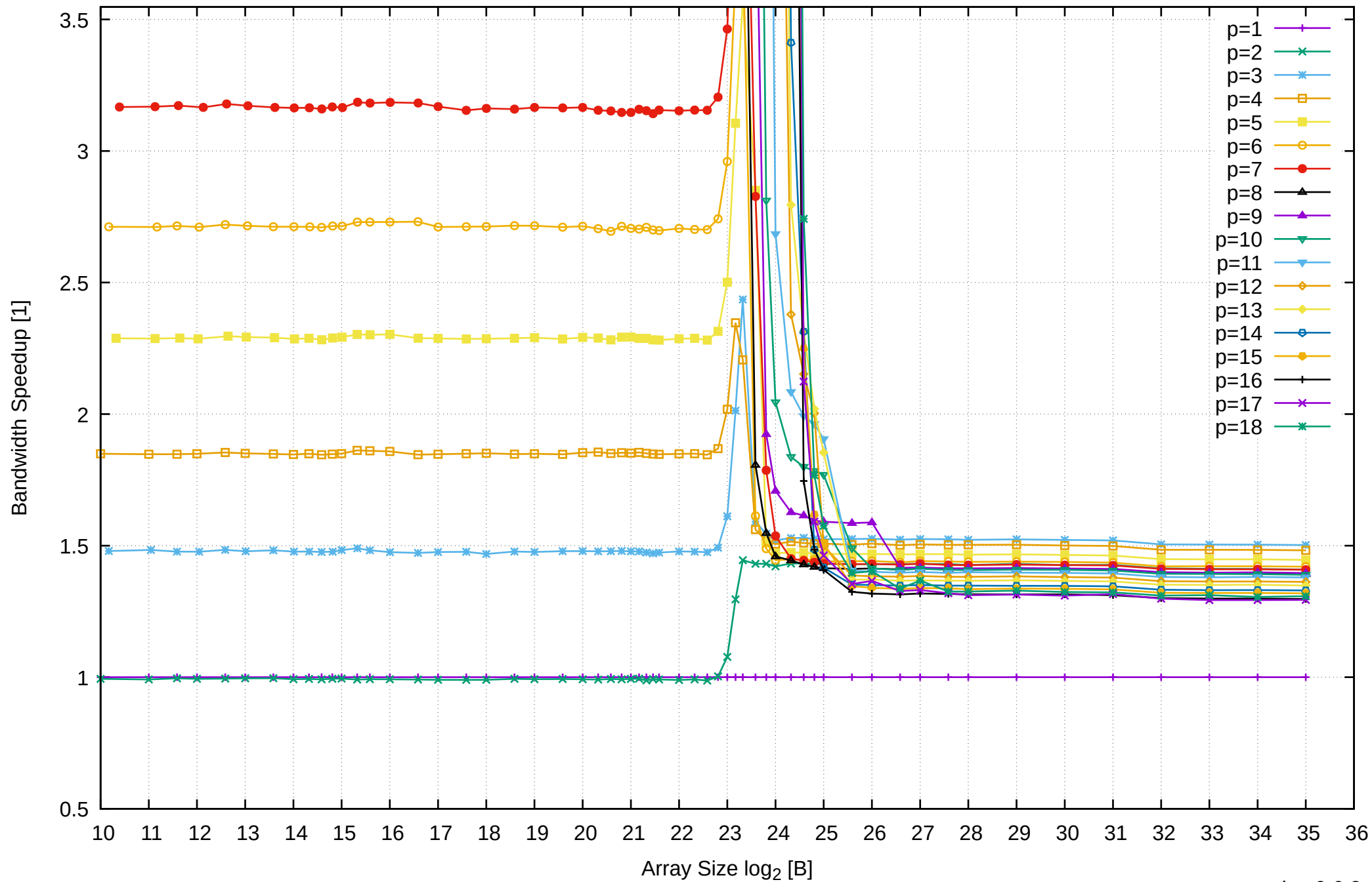
AMD Ryzen 7 1800X 64GB - Speedup of Parallel Memory Bandwidth (enlarged) - ScanWrite32PtrUnrollLoop
