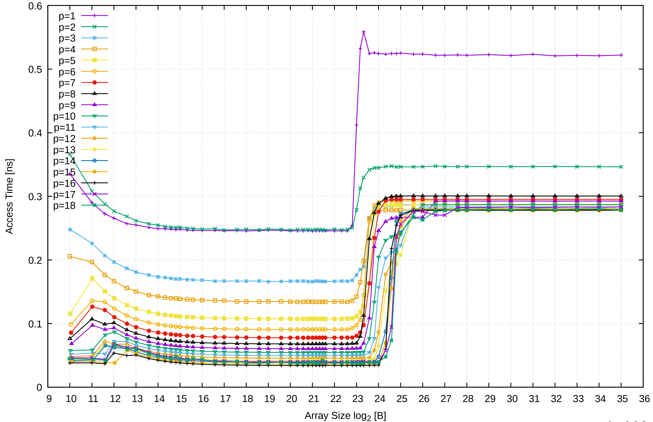
AMD Ryzen 7 1800X 64GB - Parallel Memory Access Time - ScanRead64IndexSimpleLoop
