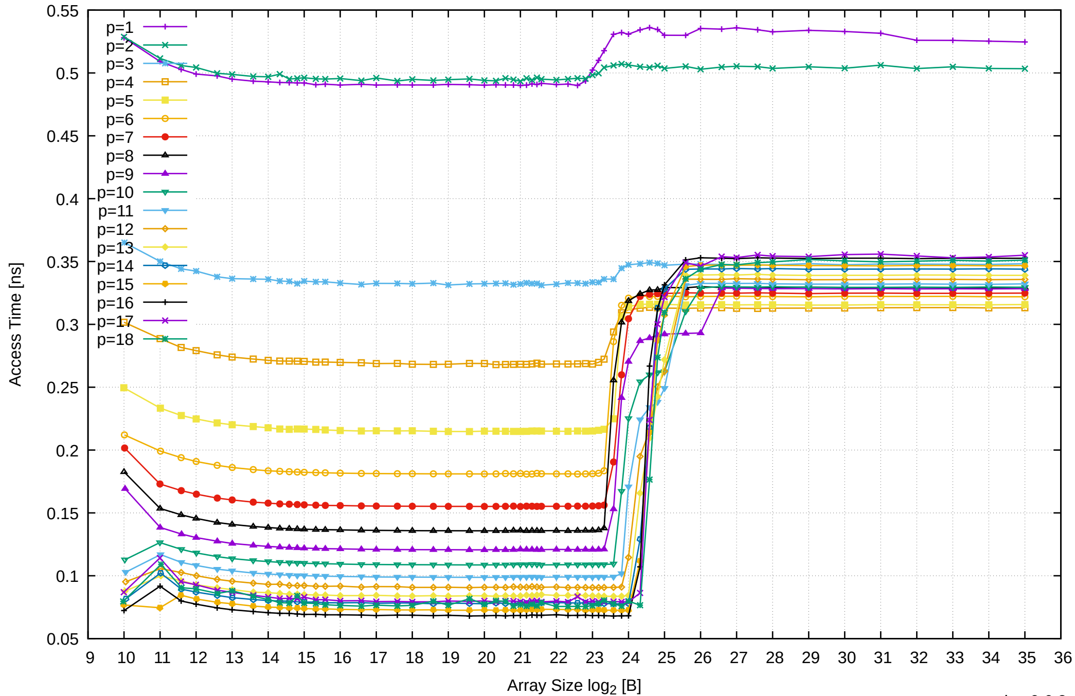
AMD Ryzen 7 1800X 64GB - Parallel Memory Access Time - ScanWrite32PtrSimpleLoop
