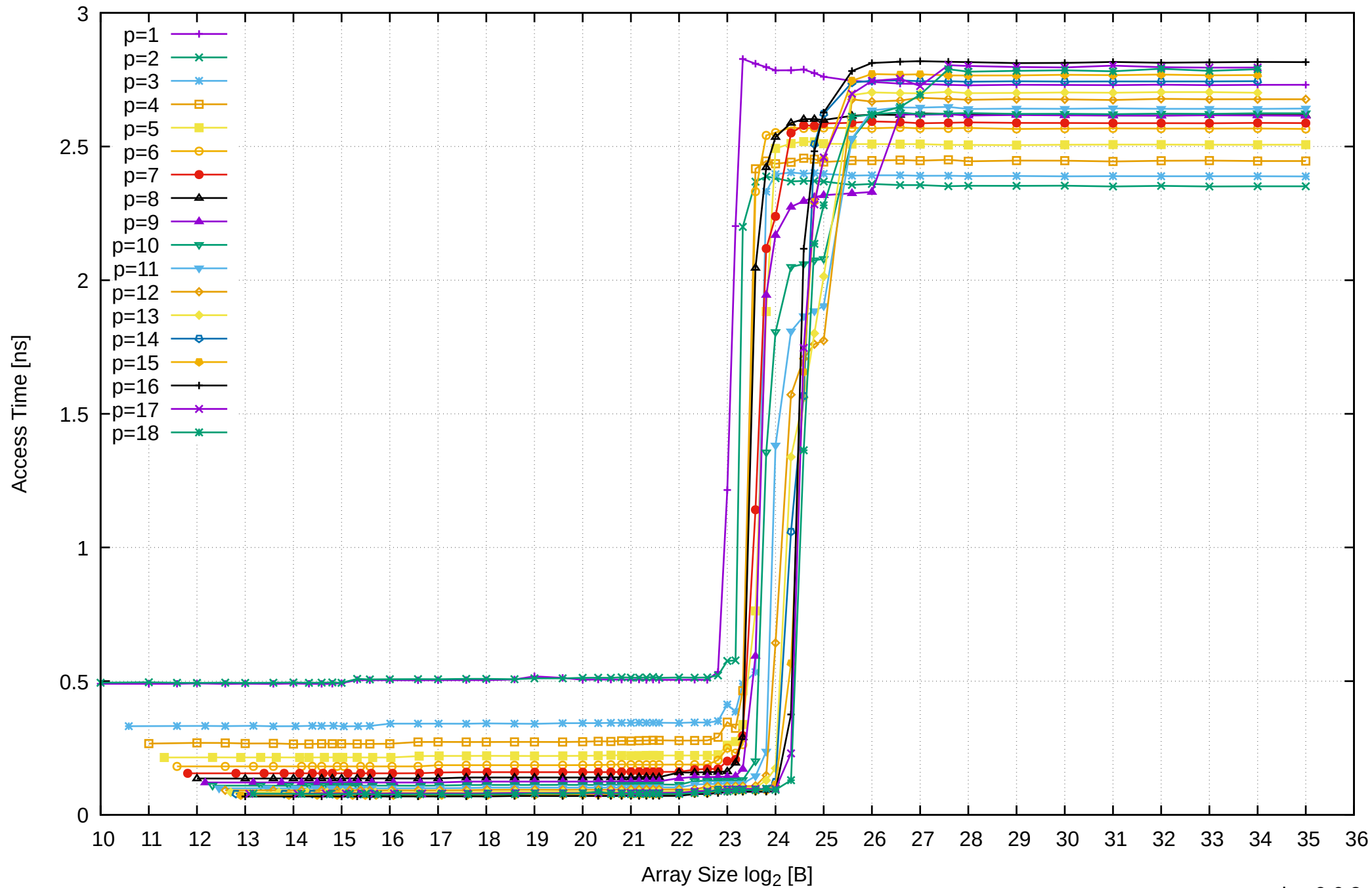
AMD Ryzen 7 1800X 64GB - Parallel Memory Access Time - ScanWrite256PtrUnrollLoop
