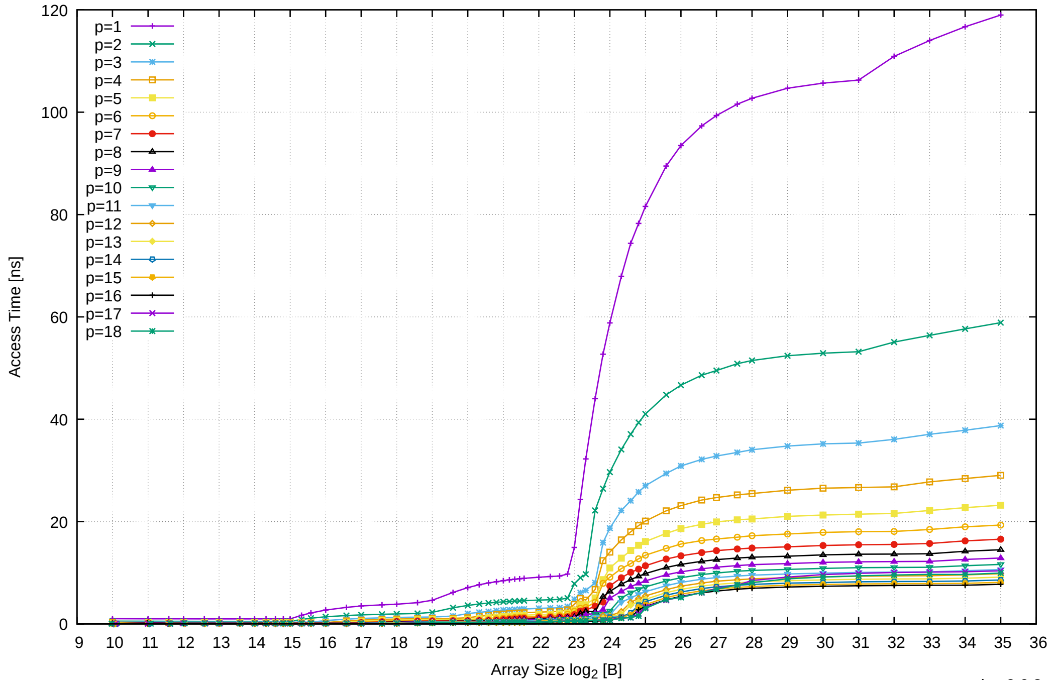
AMD Ryzen 7 1800X 64GB - Parallel Memory Access Time - PermRead64SimpleLoop
