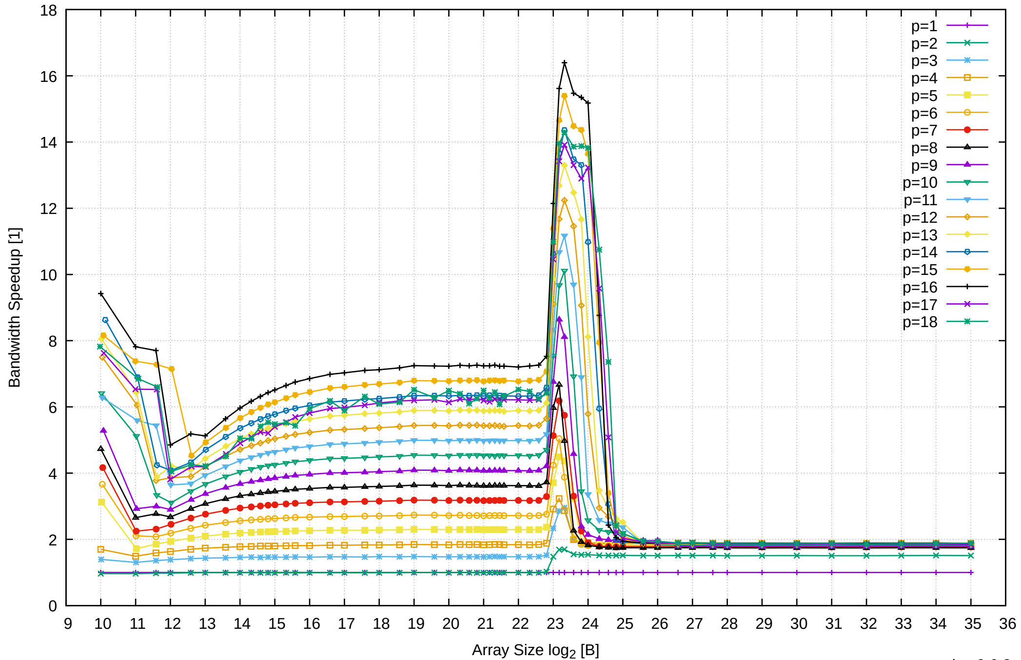
AMD Ryzen 7 1800X 64GB - Speedup of Parallel Memory Bandwidth - ScanRead64PtrSimpleLoop
