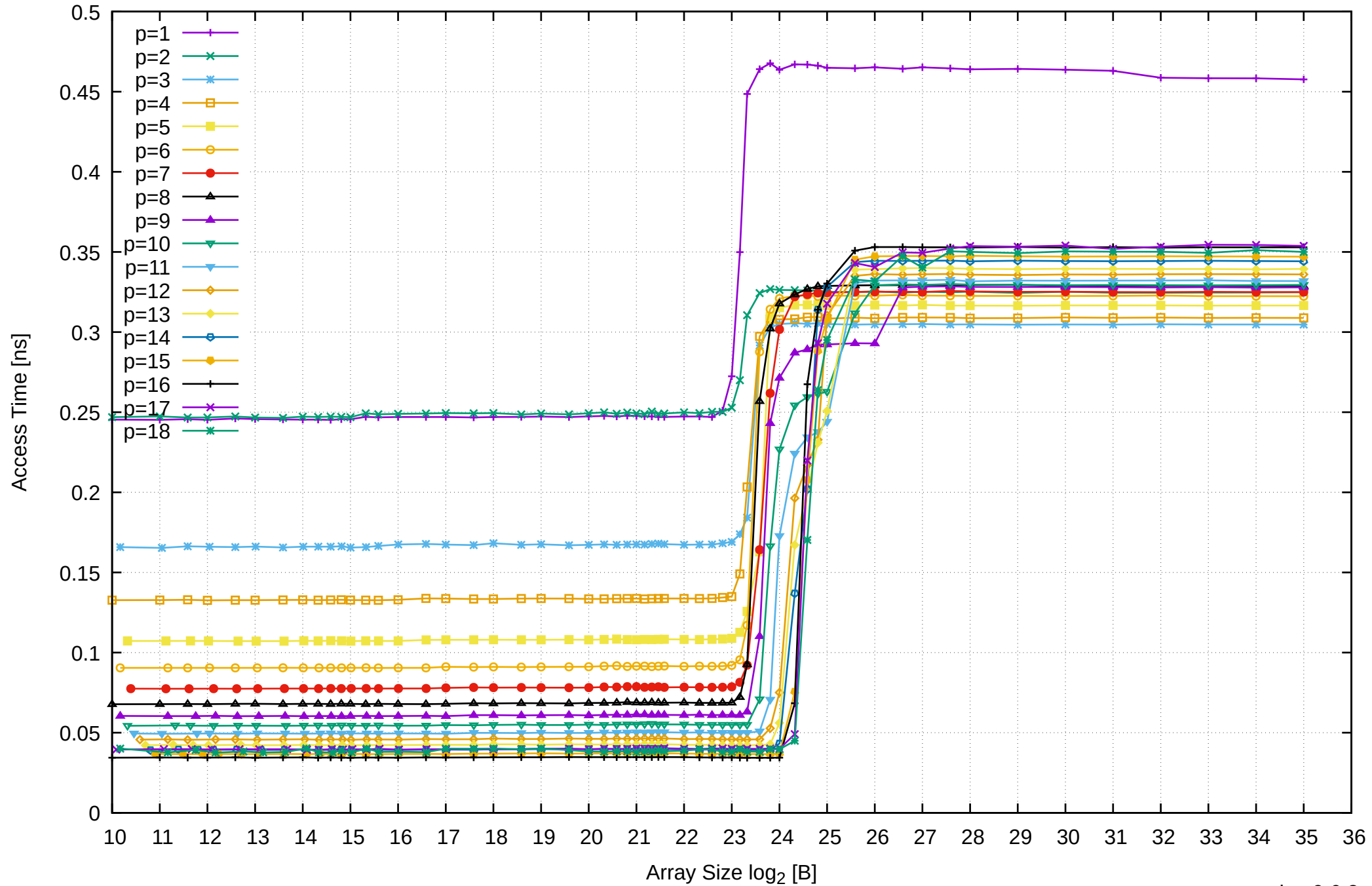
AMD Ryzen 7 1800X 64GB - Parallel Memory Access Time - ScanWrite32PtrUnrollLoop
