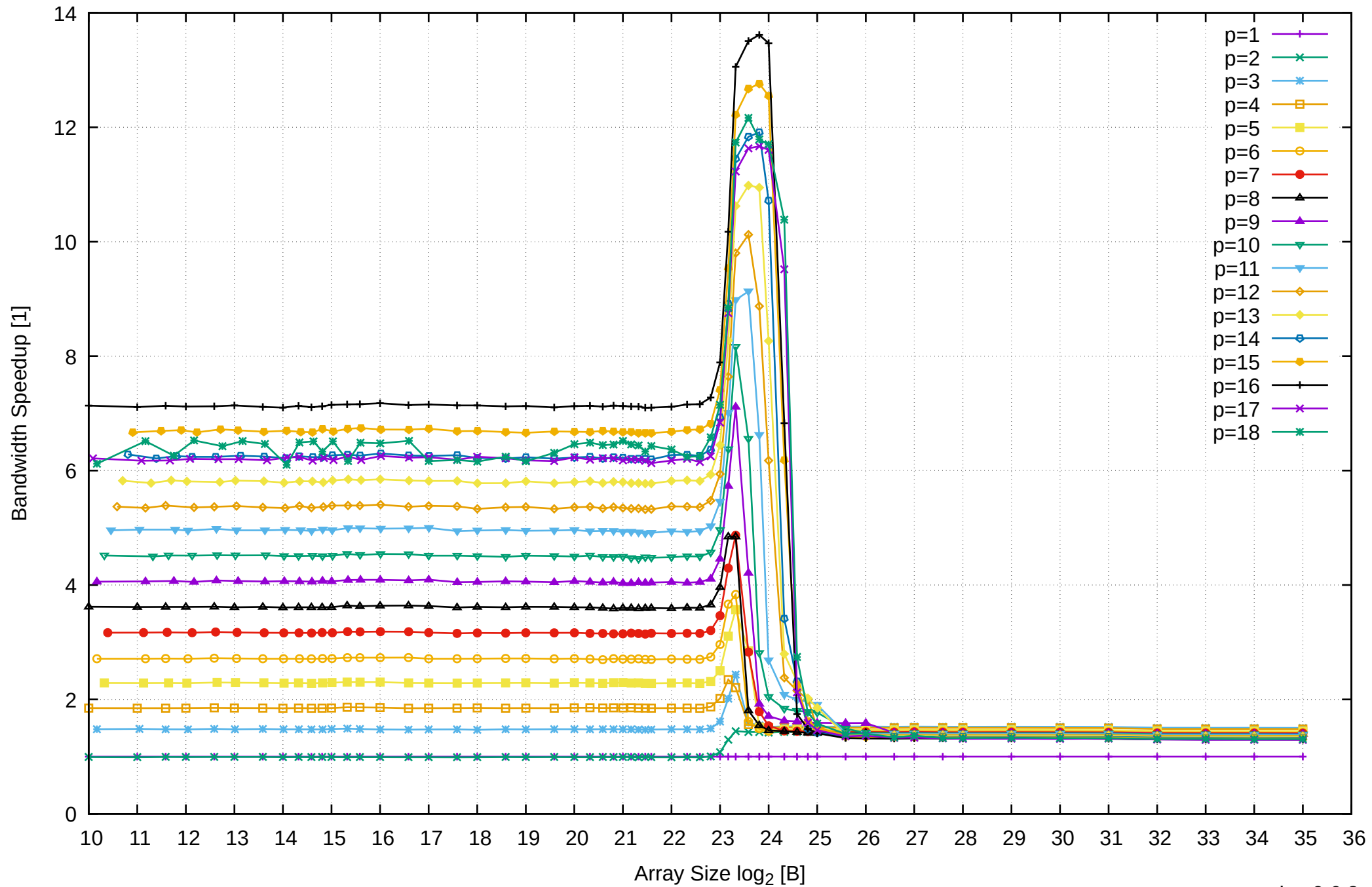
AMD Ryzen 7 1800X 64GB - Speedup of Parallel Memory Bandwidth - ScanWrite32PtrUnrollLoop
