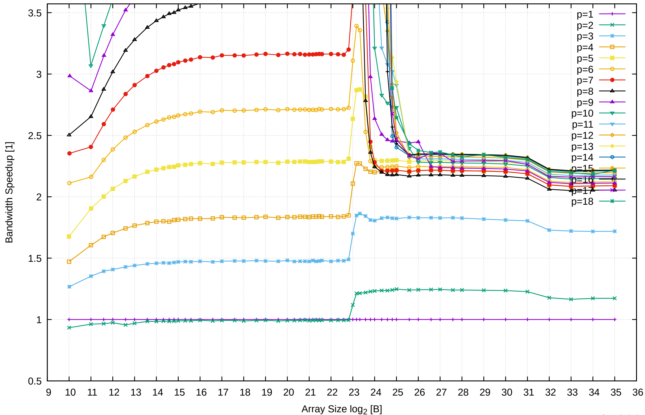
AMD Ryzen 7 1800X 64GB - Speedup of Parallel Memory Bandwidth (enlarged) - ScanRead32PtrSimpleLoop
