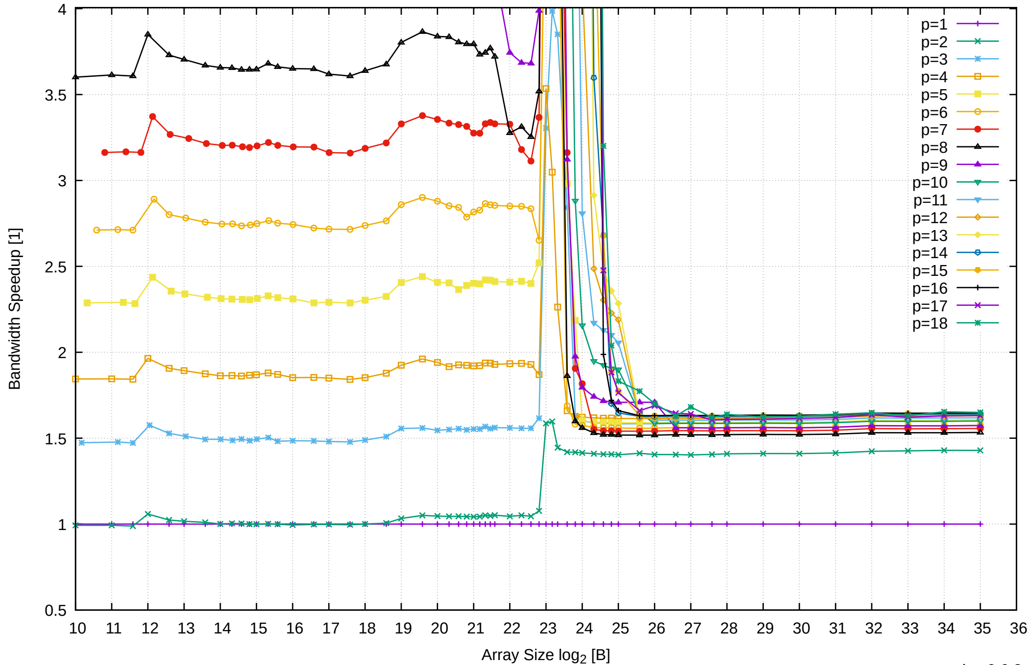
AMD Ryzen 7 1800X 64GB - Speedup of Parallel Memory Bandwidth (enlarged) - ScanRead64PtrUnrollLoop
