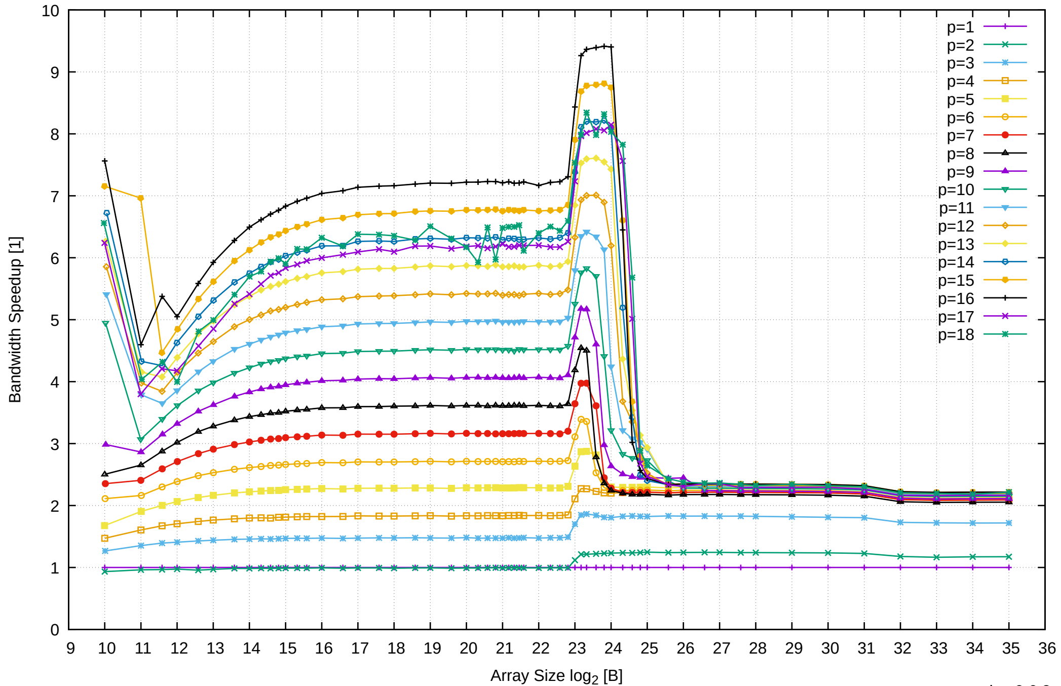
AMD Ryzen 7 1800X 64GB - Speedup of Parallel Memory Bandwidth - ScanRead32PtrSimpleLoop
