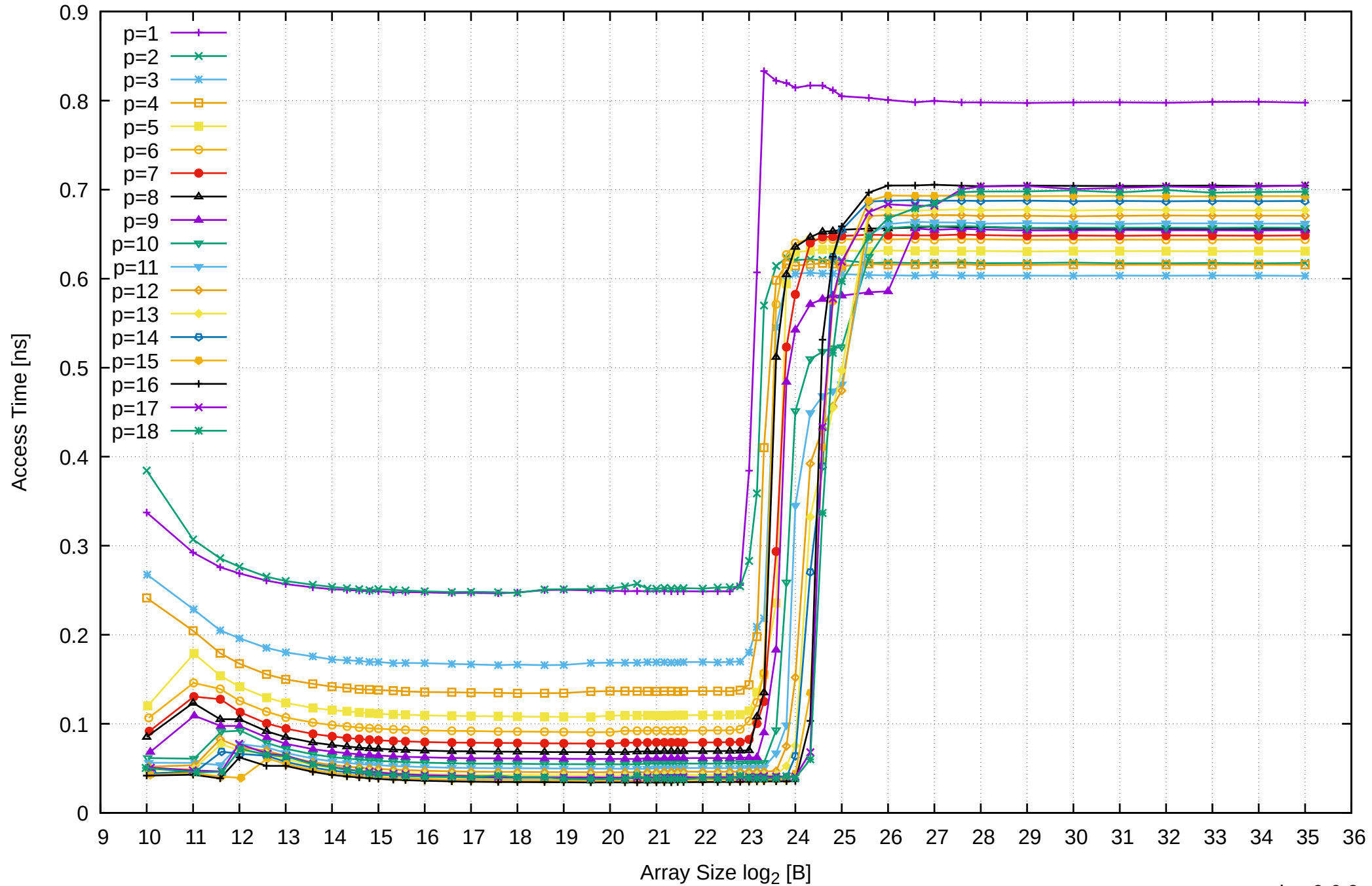
AMD Ryzen 7 1800X 64GB - Parallel Memory Access Time - ScanWrite64PtrSimpleLoop
