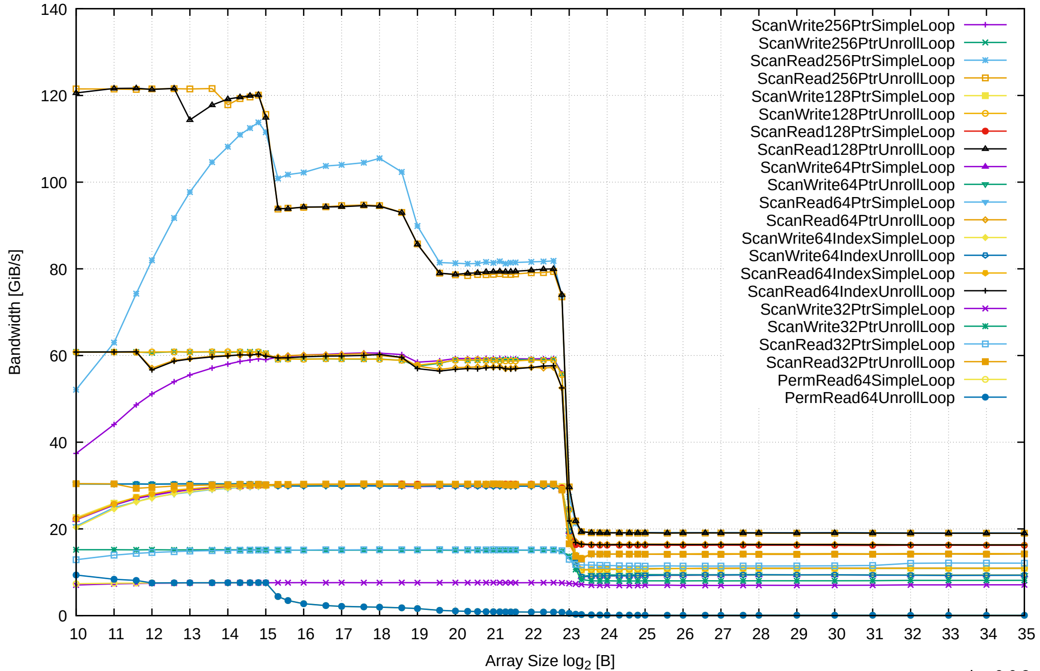
AMD Ryzen 7 1800X 64GB - One Thread Memory Bandwidth
