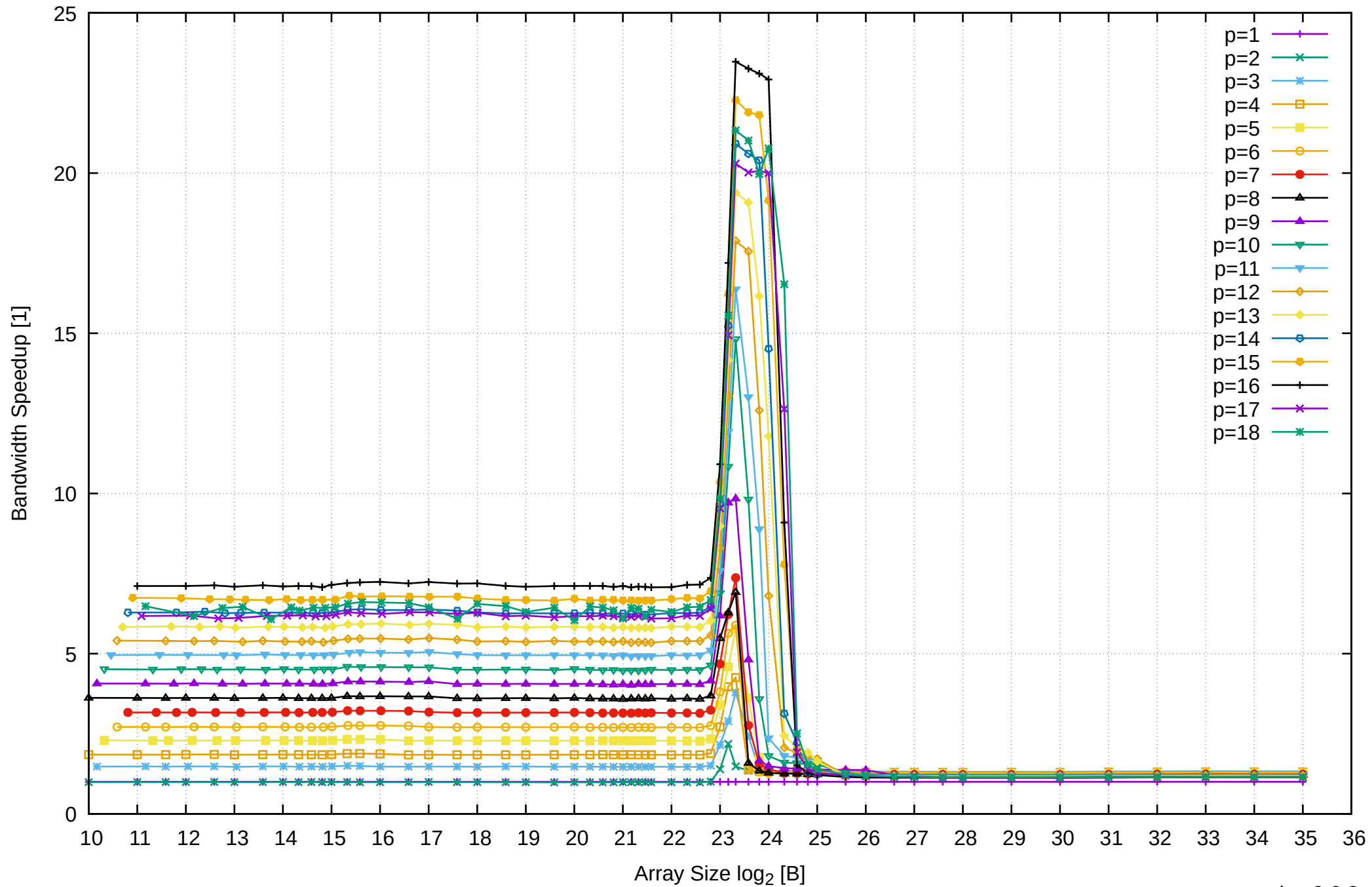
AMD Ryzen 7 1800X 64GB - Speedup of Parallel Memory Bandwidth - ScanWrite64IndexUnrollLoop
