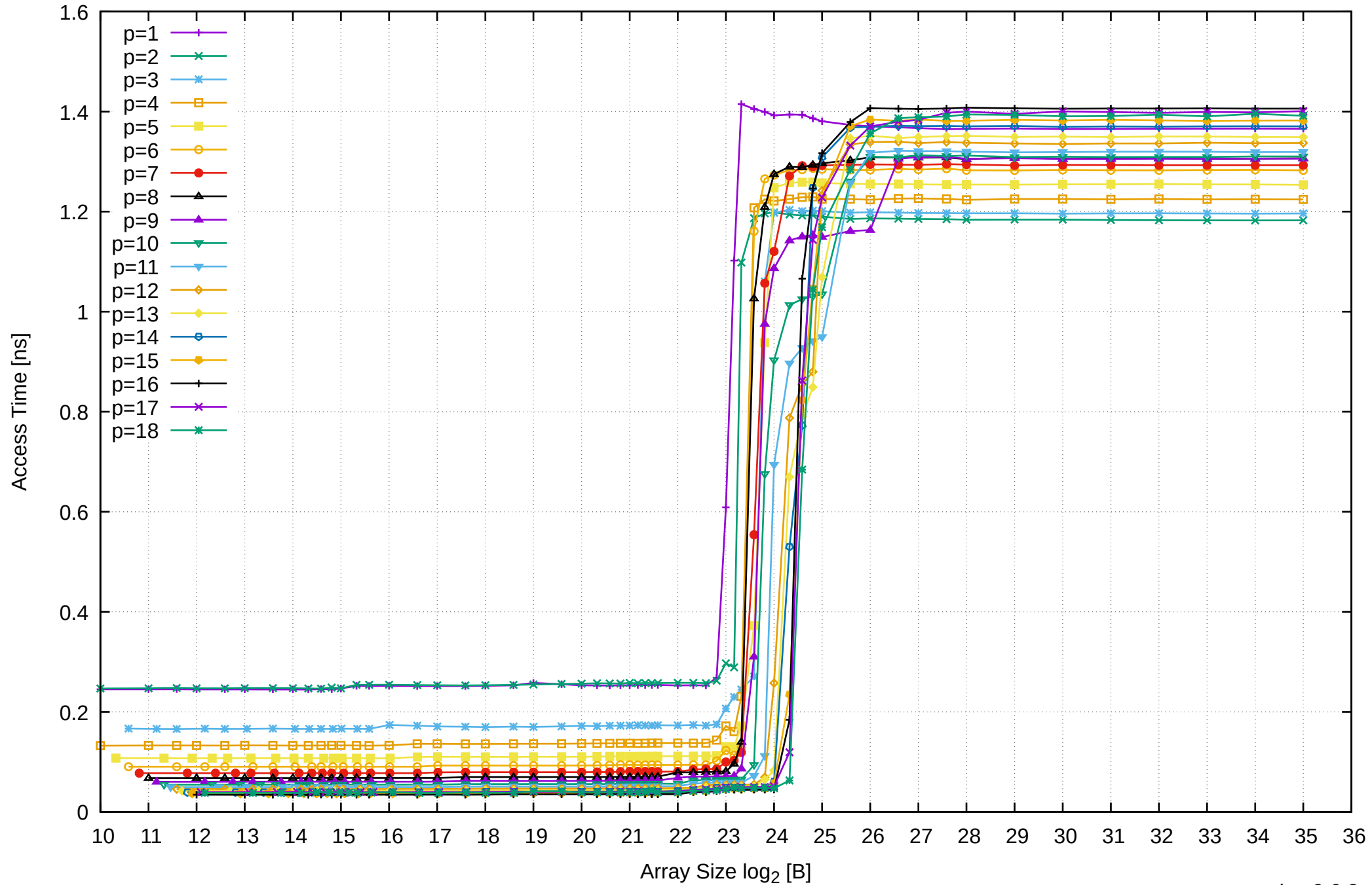
AMD Ryzen 7 1800X 64GB - Parallel Memory Access Time - ScanWrite128PtrUnrollLoop
