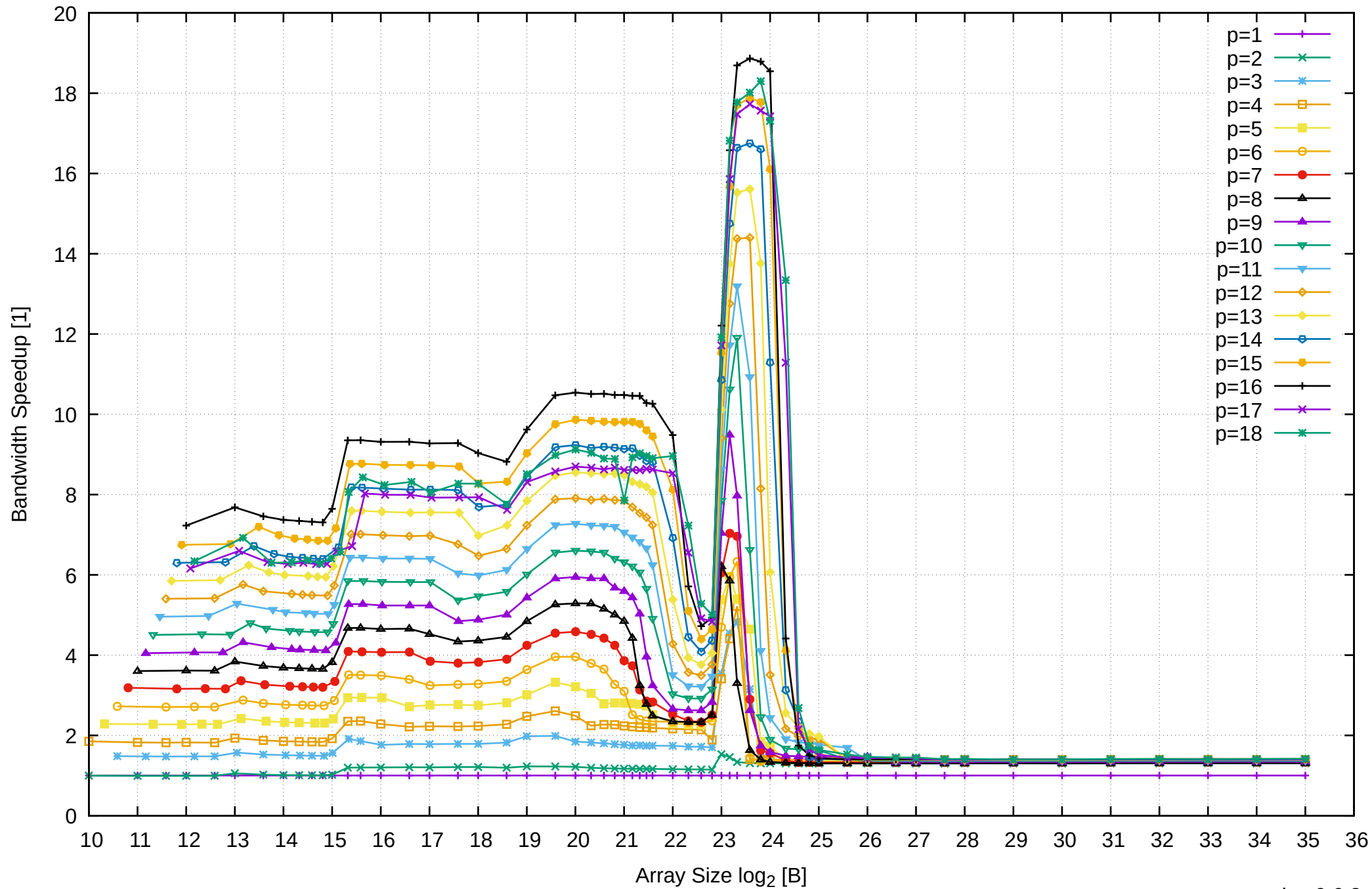
AMD Ryzen 7 1800X 64GB - Speedup of Parallel Memory Bandwidth - ScanRead128PtrUnrollLoop
