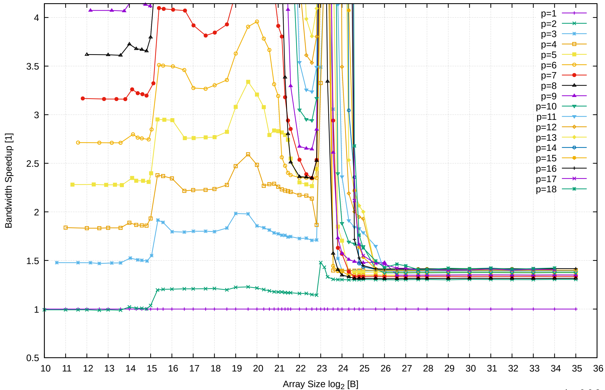
AMD Ryzen 7 1800X 64GB - Speedup of Parallel Memory Bandwidth (enlarged) - ScanRead256PtrUnrollLoop
