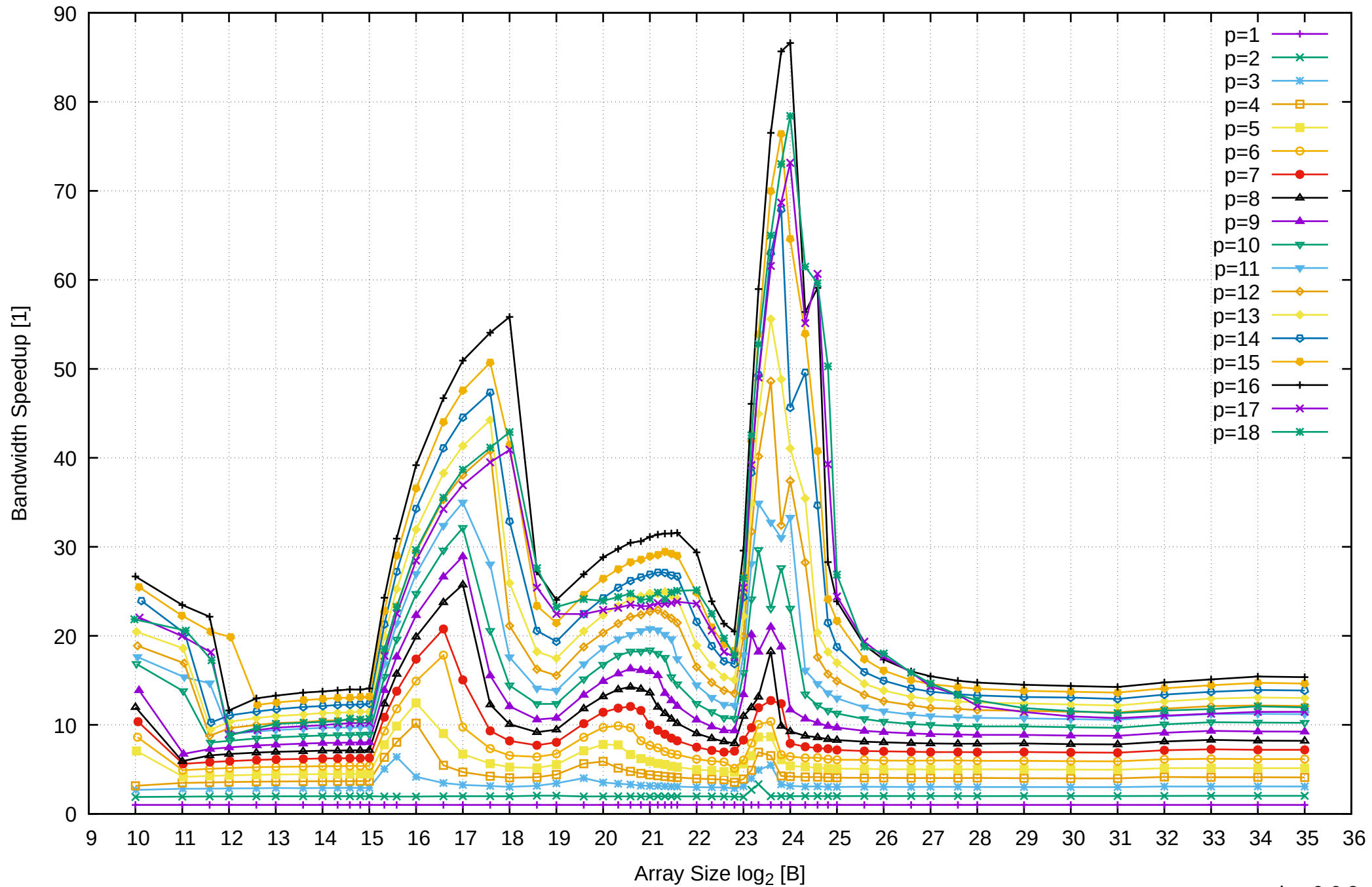
AMD Ryzen 7 1800X 64GB - Speedup of Parallel Memory Bandwidth - PermRead64SimpleLoop
