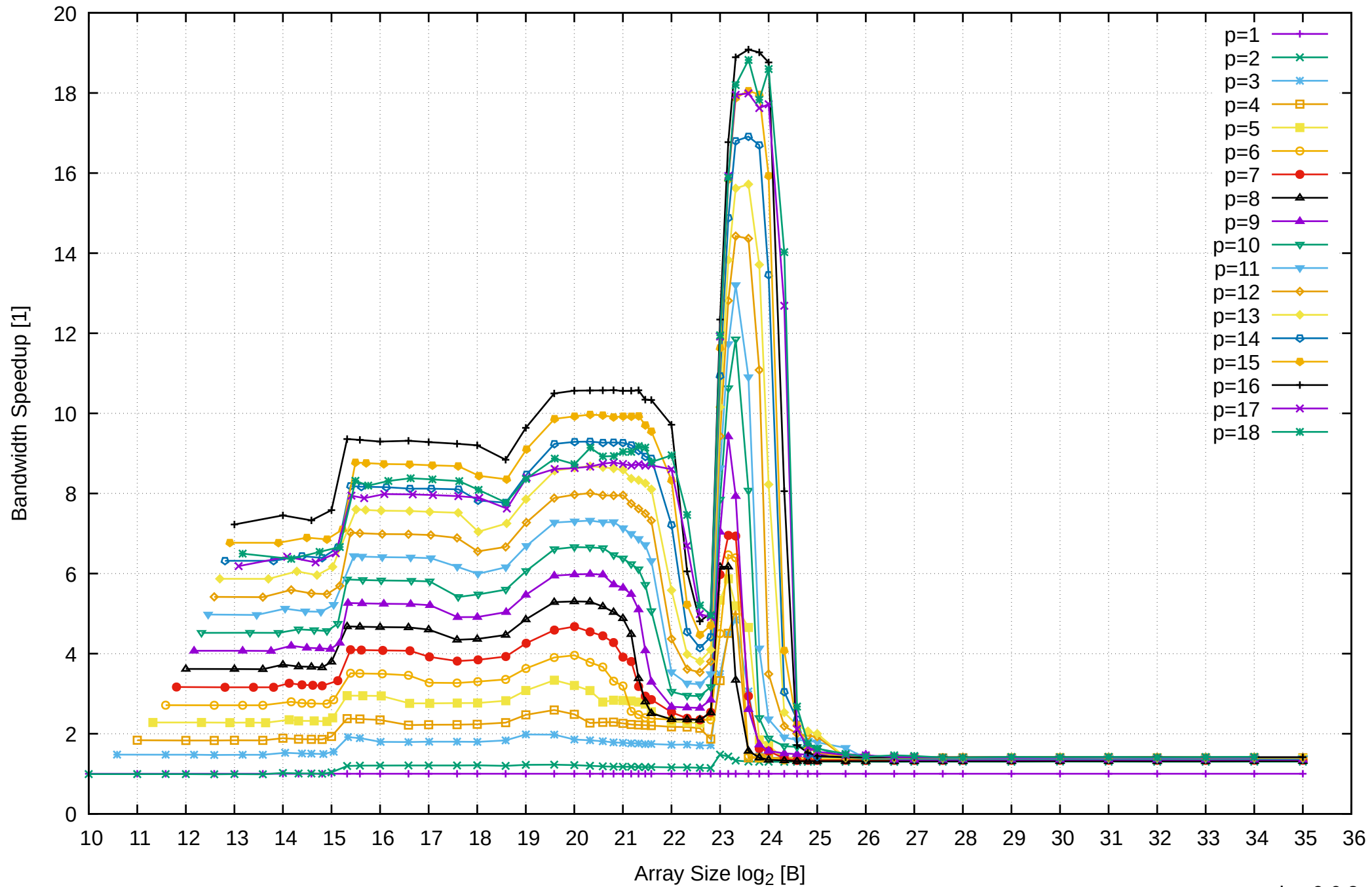
AMD Ryzen 7 1800X 64GB - Speedup of Parallel Memory Bandwidth - ScanRead256PtrUnrollLoop
