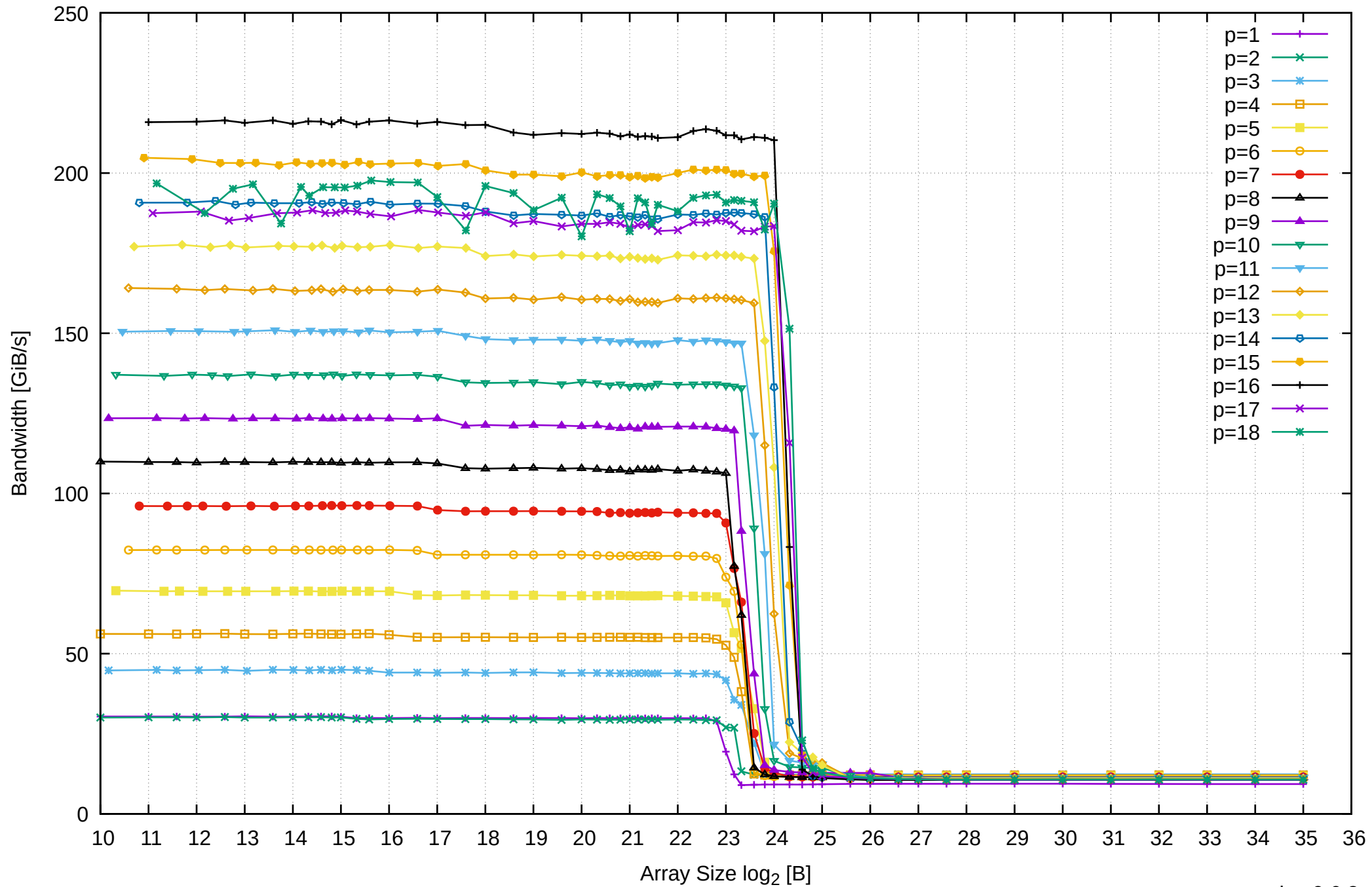
AMD Ryzen 7 1800X 64GB - Parallel Memory Bandwidth - ScanWrite64IndexUnrollLoop
