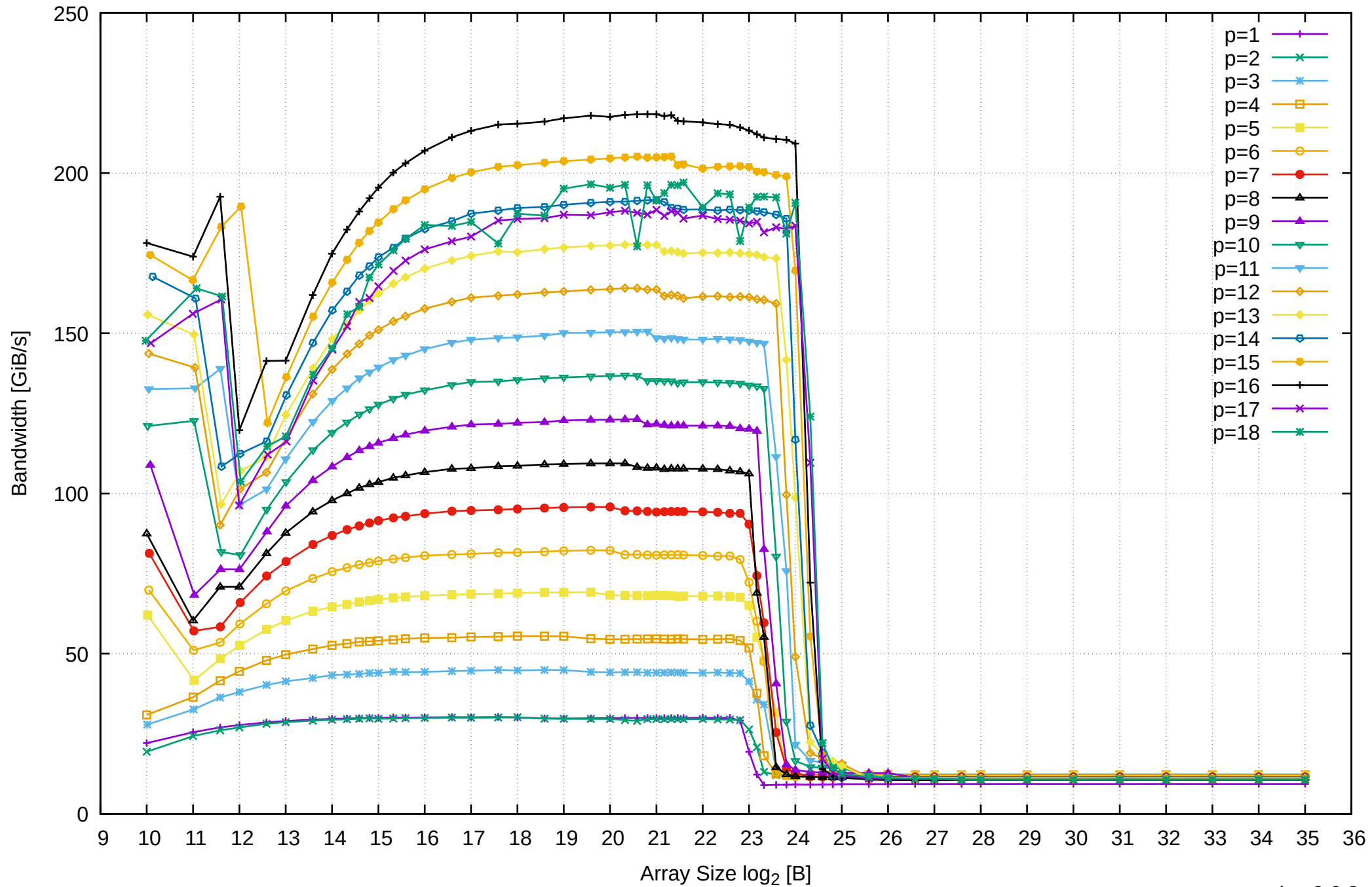
AMD Ryzen 7 1800X 64GB - Parallel Memory Bandwidth - ScanWrite64PtrSimpleLoop
