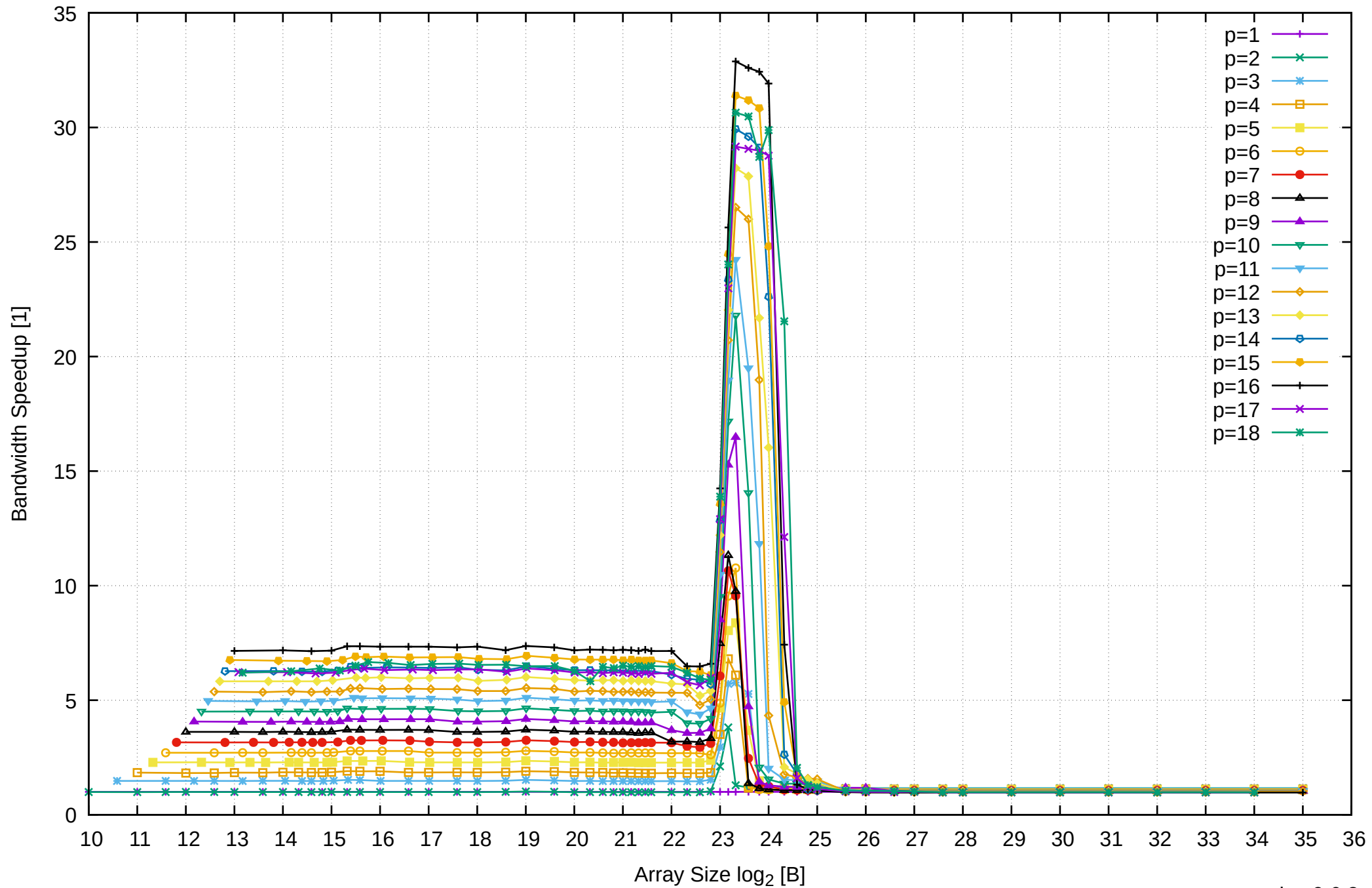
AMD Ryzen 7 1800X 64GB - Speedup of Parallel Memory Bandwidth - ScanWrite256PtrUnrollLoop
