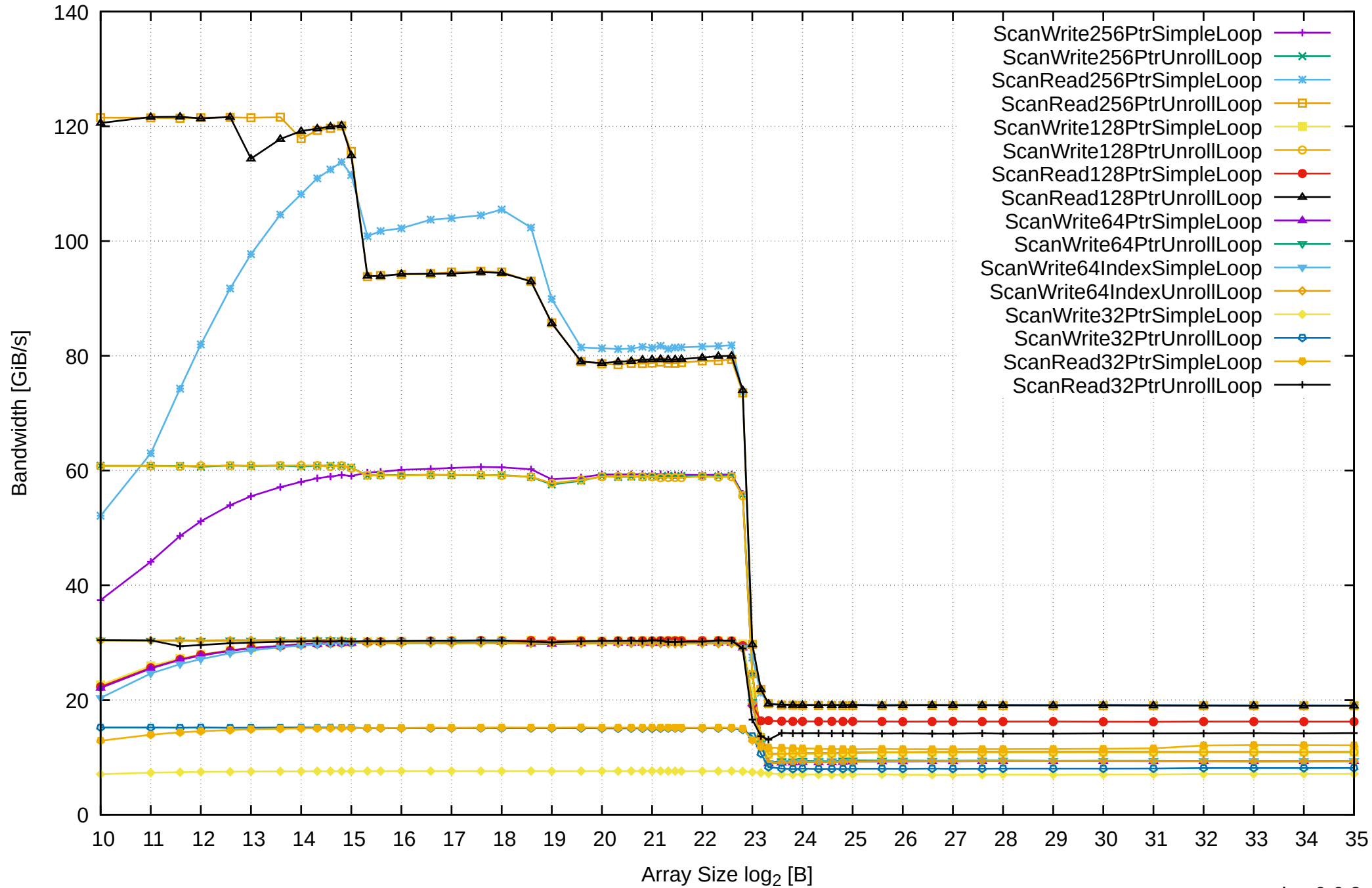
AMD Ryzen 7 1800X 64GB - One Thread Memory Bandwidth (only 64-bit Reads)
