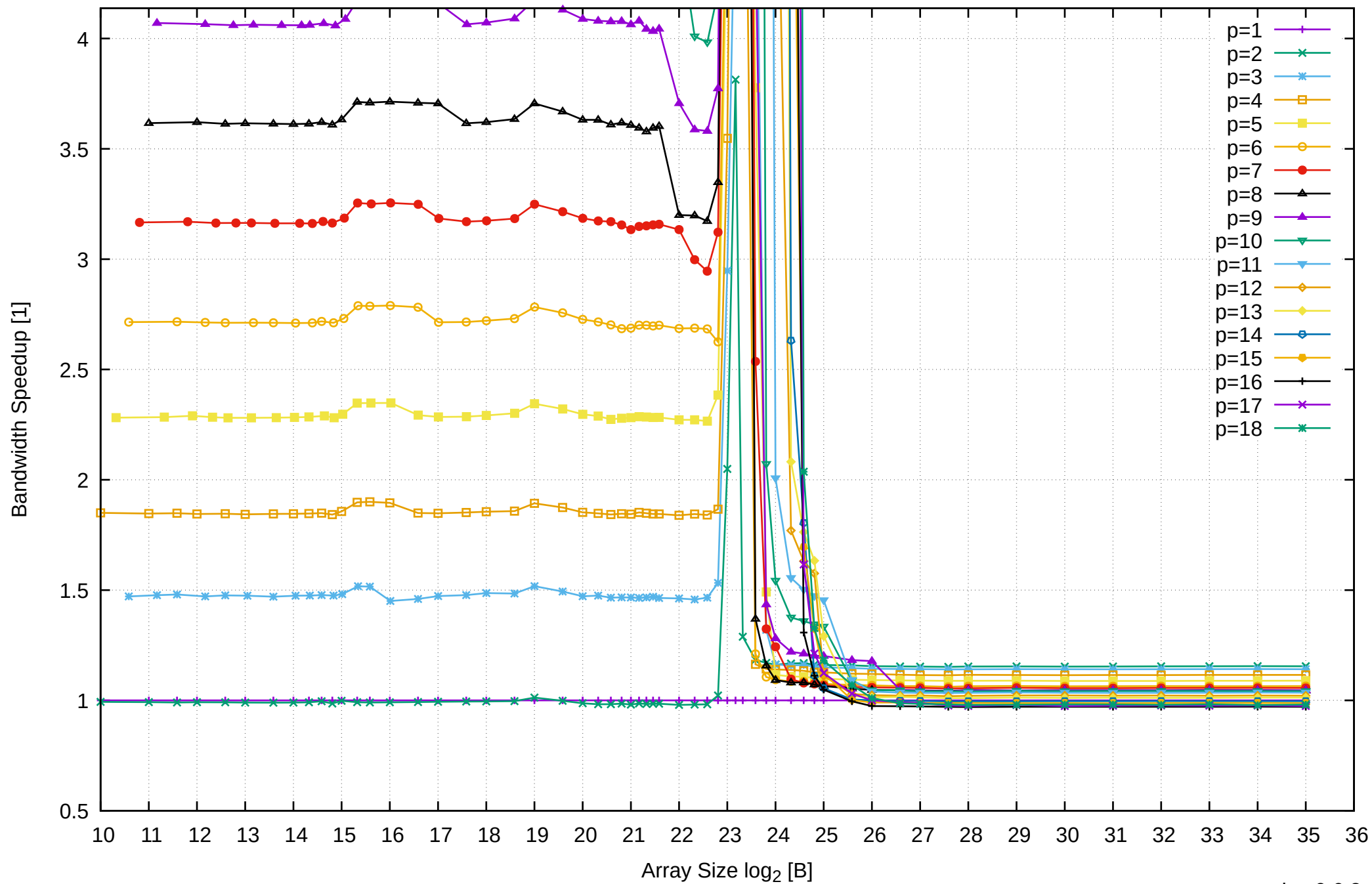
AMD Ryzen 7 1800X 64GB - Speedup of Parallel Memory Bandwidth (enlarged) - ScanWrite128PtrUnrollLoop
