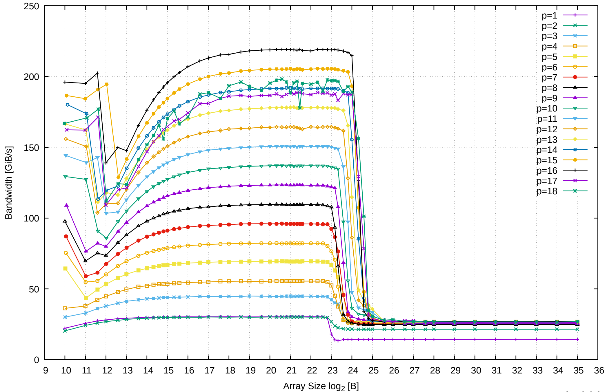
AMD Ryzen 7 1800X 64GB - Parallel Memory Bandwidth - ScanRead64IndexSimpleLoop
