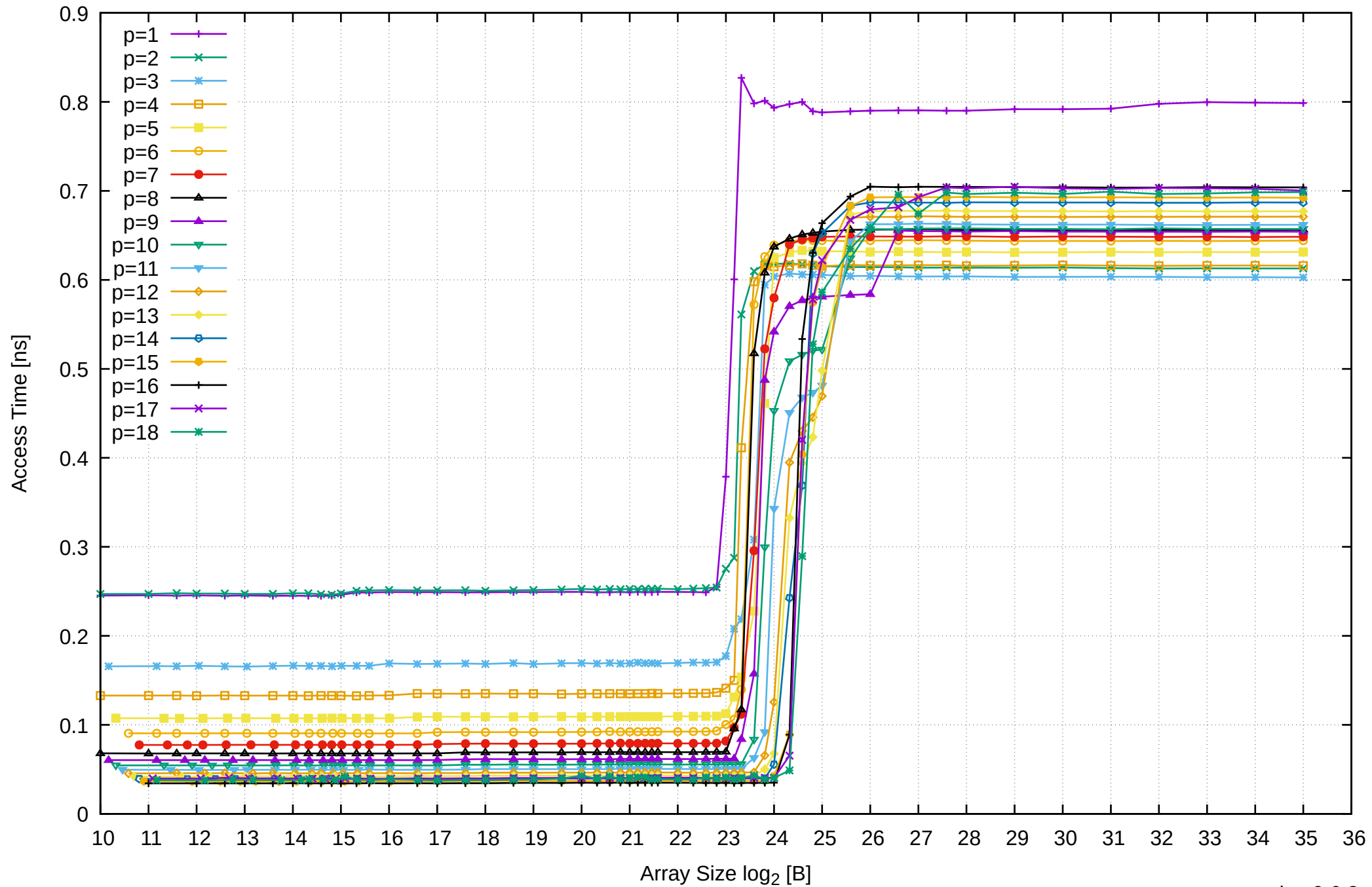
AMD Ryzen 7 1800X 64GB - Parallel Memory Access Time - ScanWrite64PtrUnrollLoop
