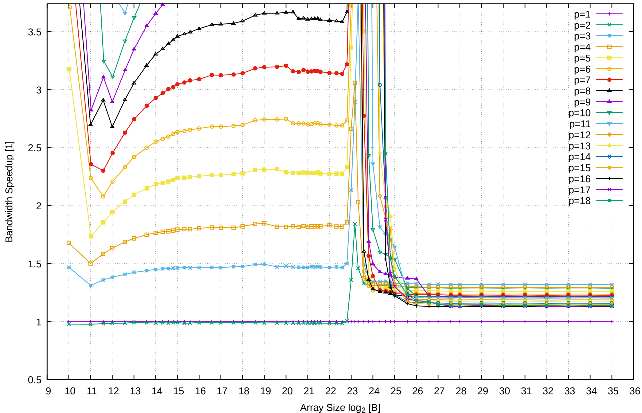
AMD Ryzen 7 1800X 64GB - Speedup of Parallel Memory Bandwidth (enlarged) - ScanWrite64IndexSimpleLoop
