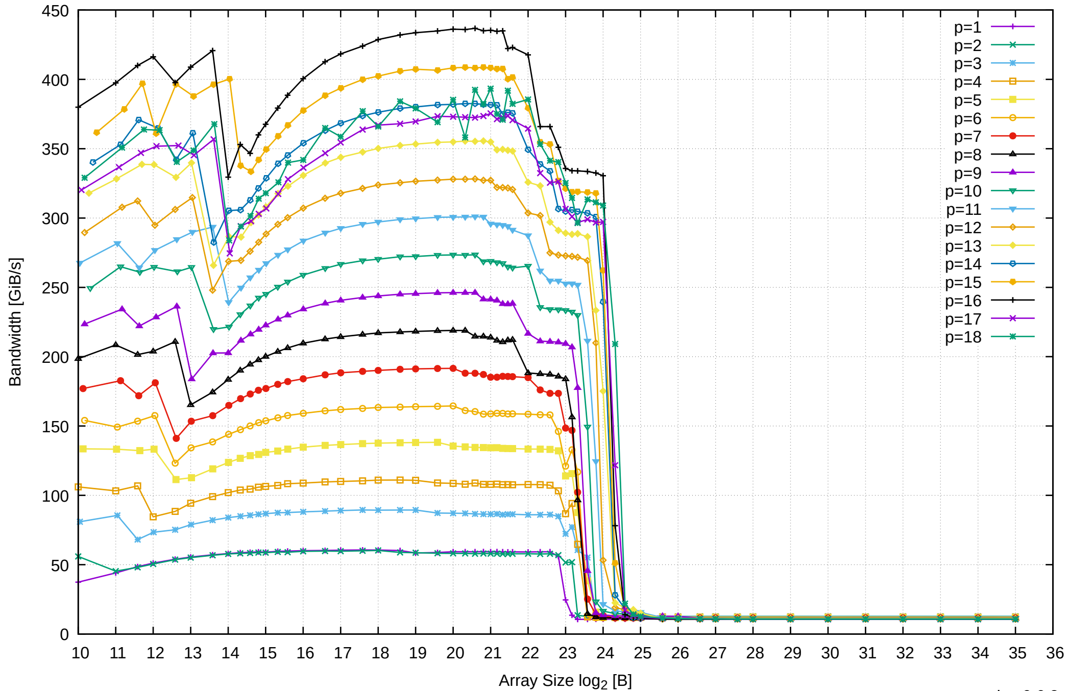
AMD Ryzen 7 1800X 64GB - Parallel Memory Bandwidth - ScanWrite256PtrSimpleLoop
