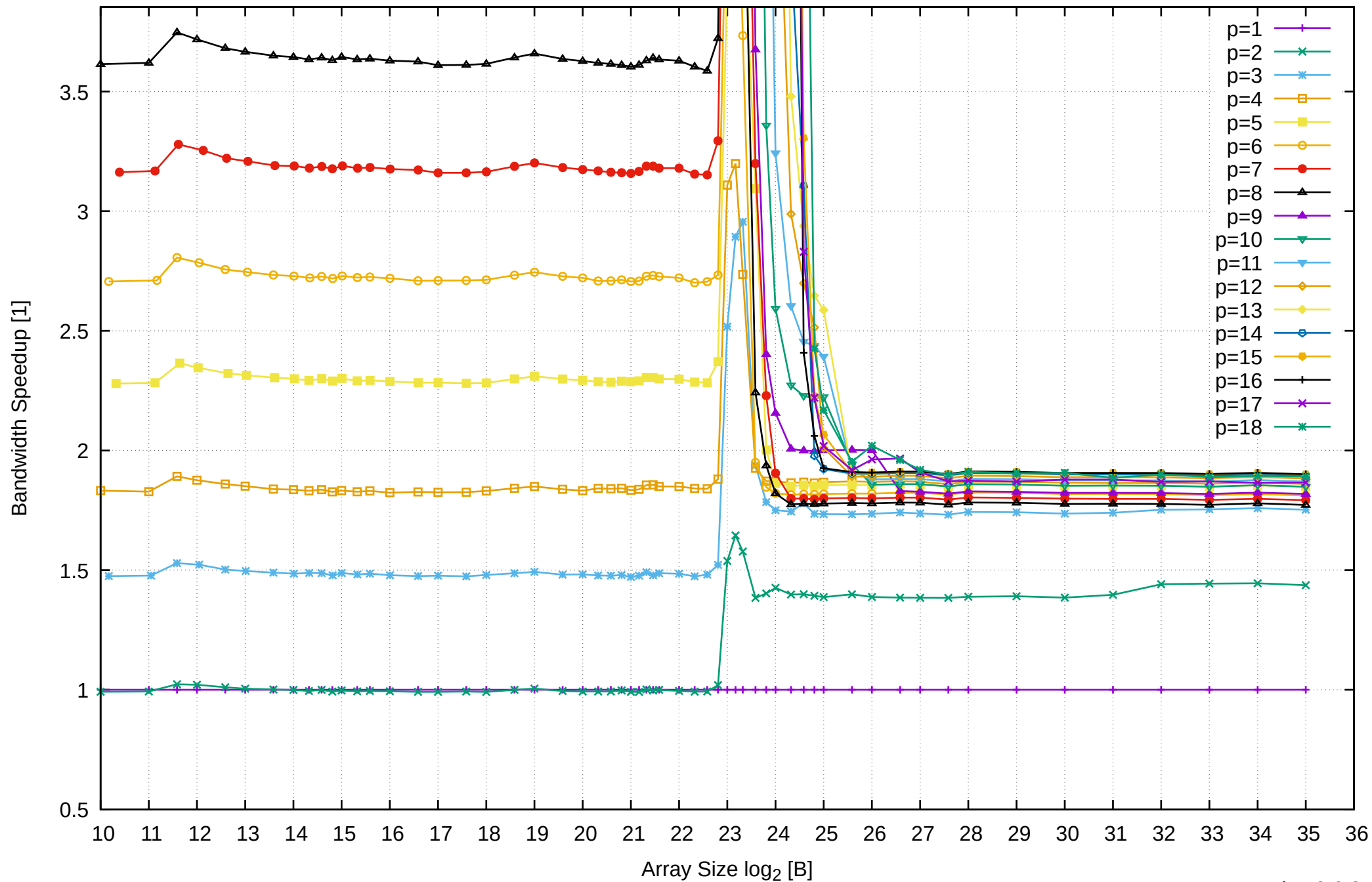
AMD Ryzen 7 1800X 64GB - Speedup of Parallel Memory Bandwidth (enlarged) - ScanRead32PtrUnrollLoop
