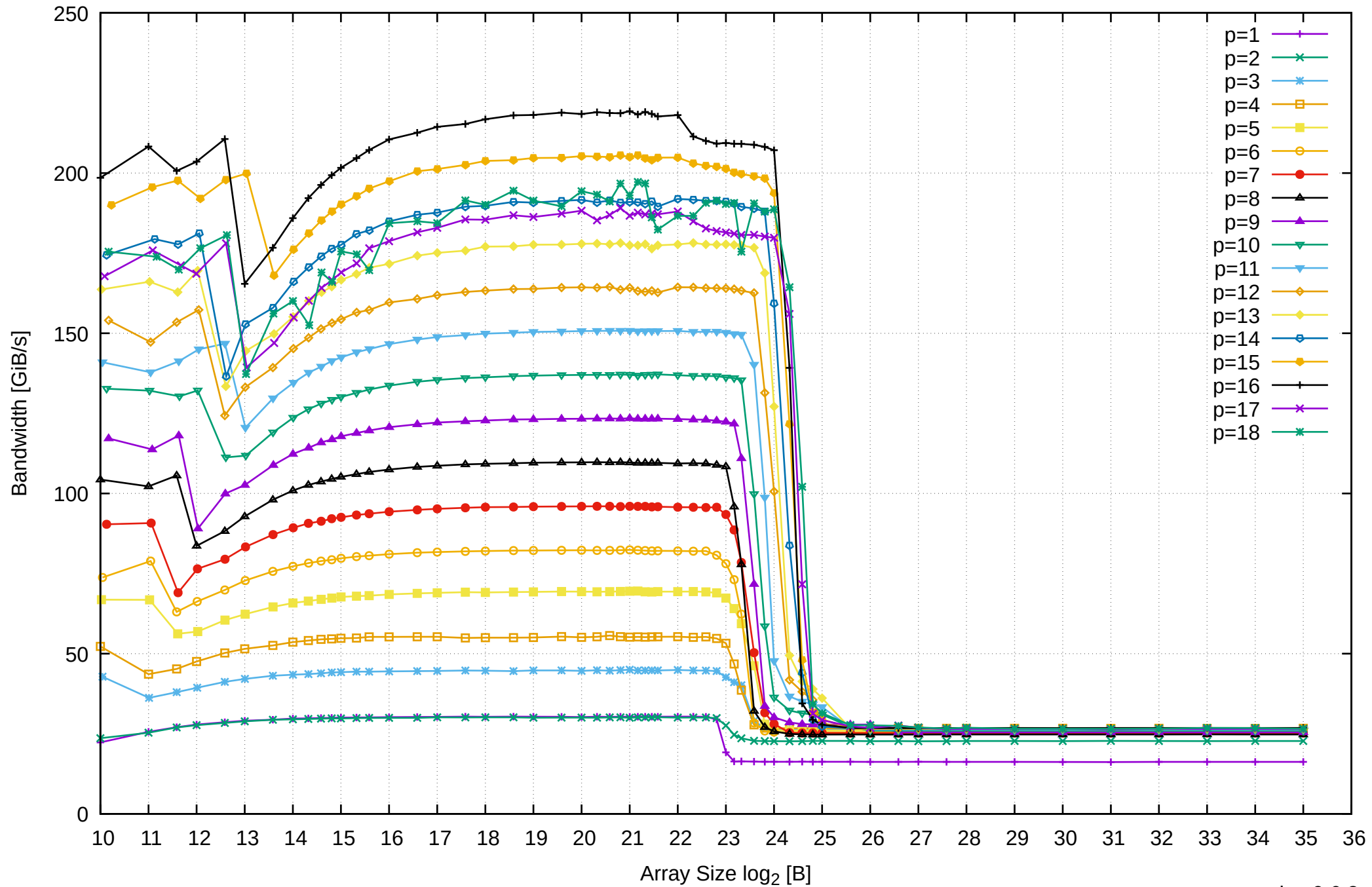
AMD Ryzen 7 1800X 64GB - Parallel Memory Bandwidth - ScanRead128PtrSimpleLoop
