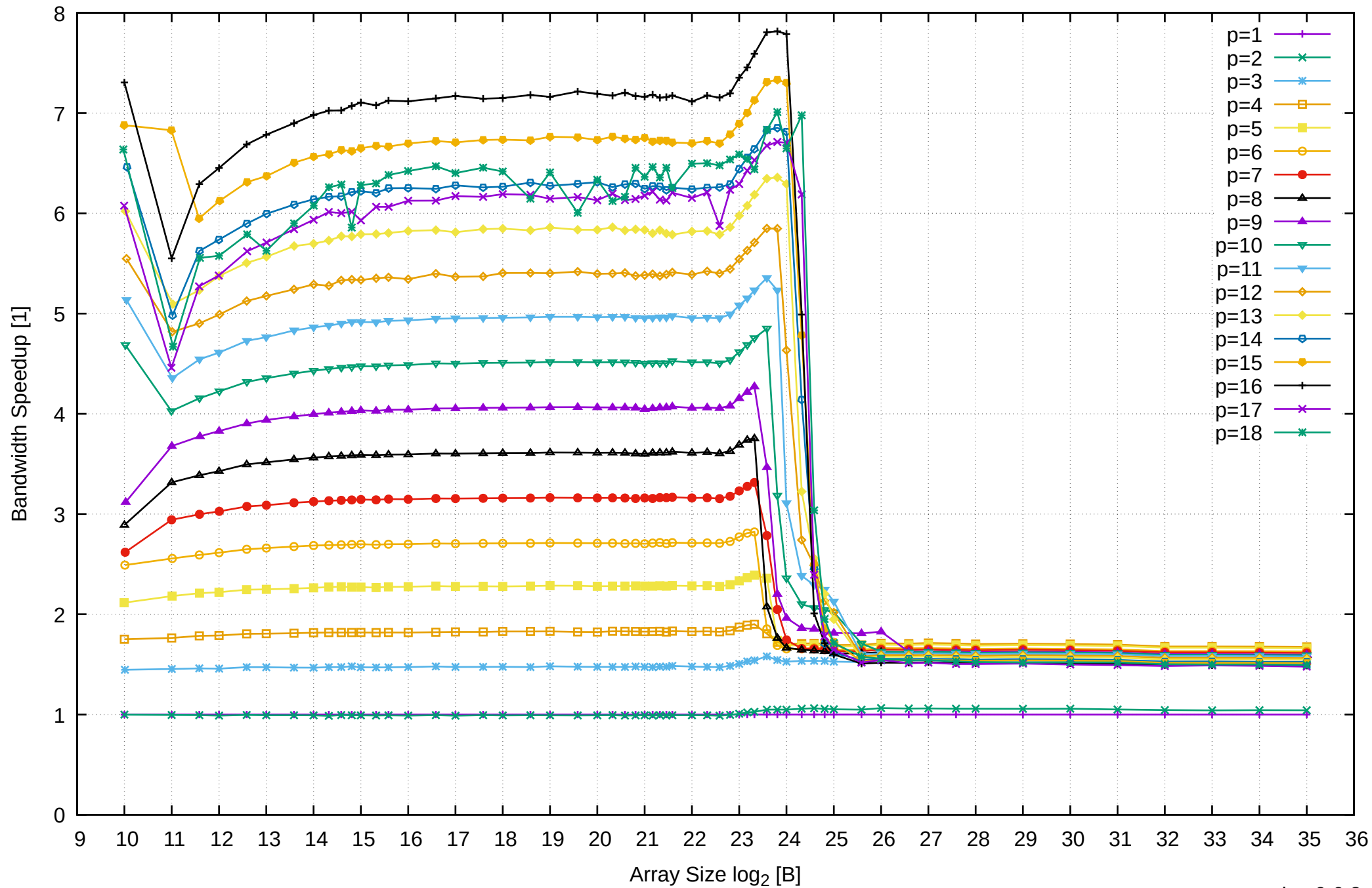
AMD Ryzen 7 1800X 64GB - Speedup of Parallel Memory Bandwidth - ScanWrite32PtrSimpleLoop
