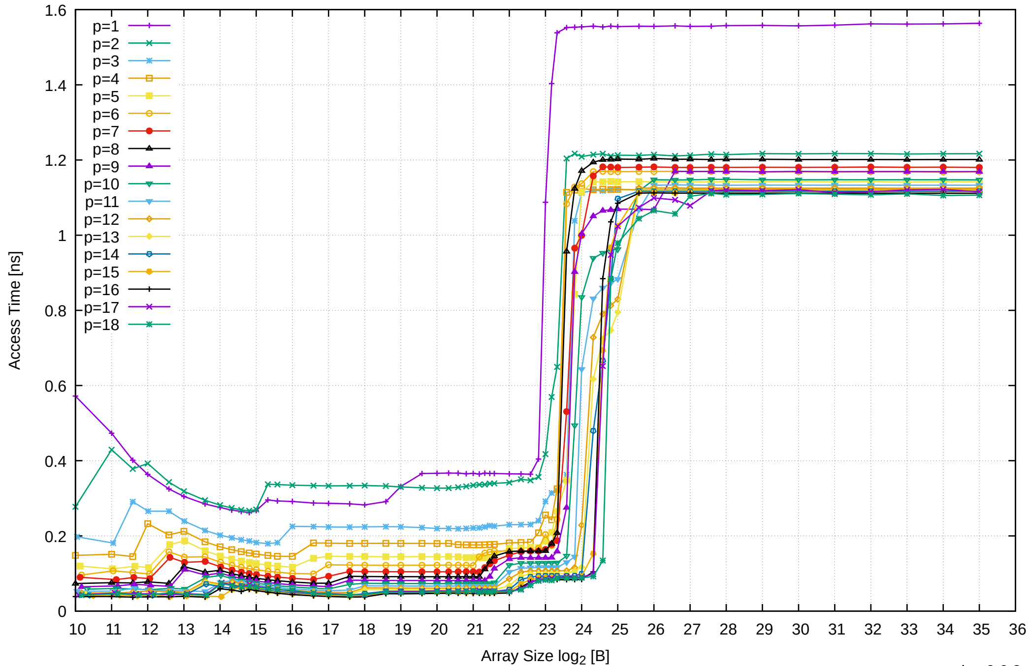
AMD Ryzen 7 1800X 64GB - Parallel Memory Access Time - ScanRead256PtrSimpleLoop
