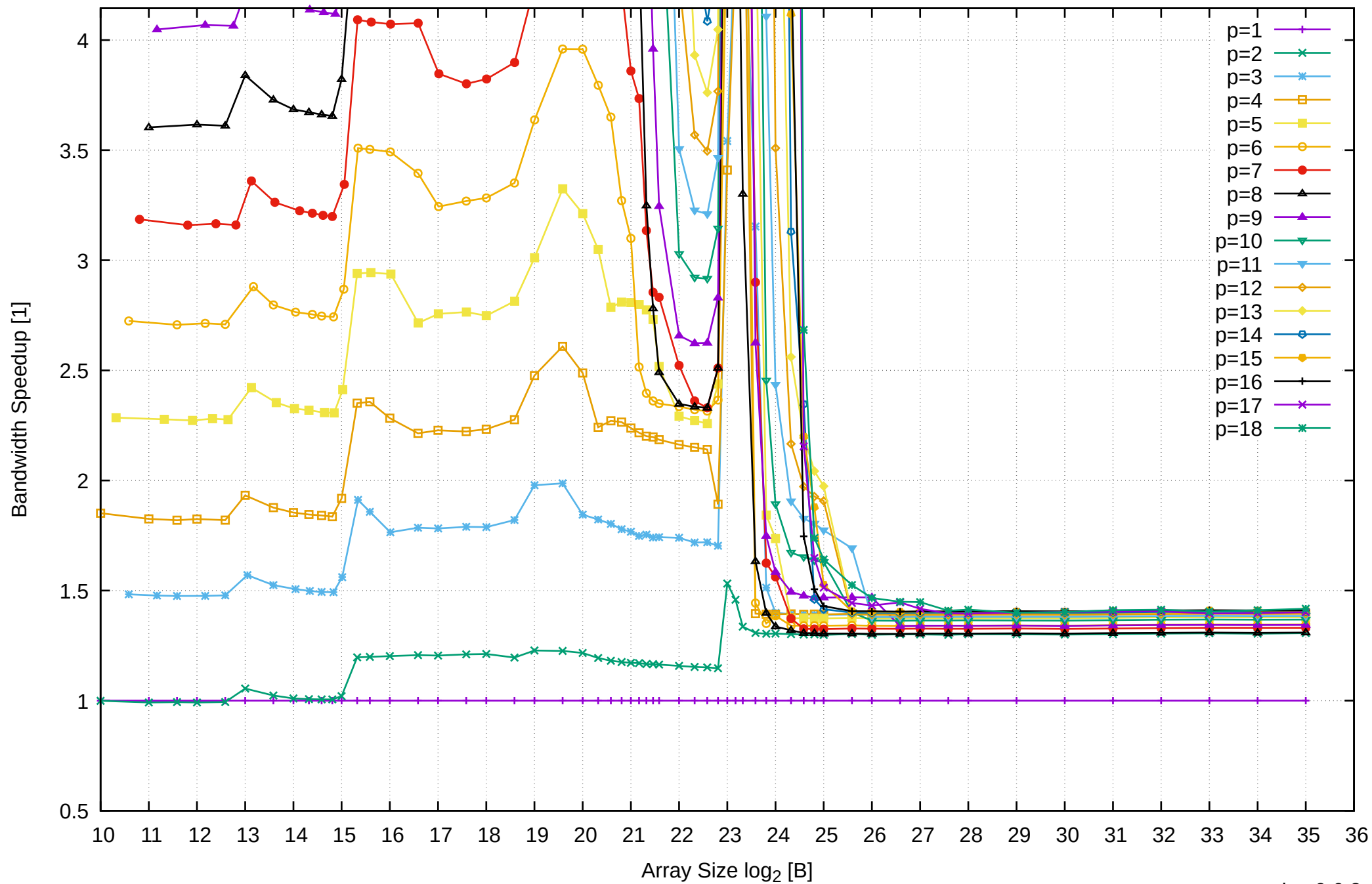
AMD Ryzen 7 1800X 64GB - Speedup of Parallel Memory Bandwidth (enlarged) - ScanRead128PtrUnrollLoop
