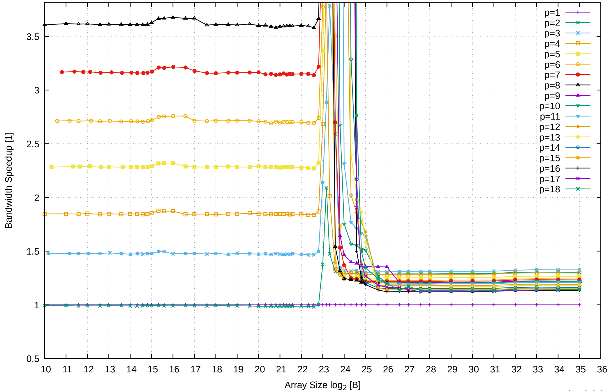
AMD Ryzen 7 1800X 64GB - Speedup of Parallel Memory Bandwidth (enlarged) - ScanWrite64PtrUnrollLoop
