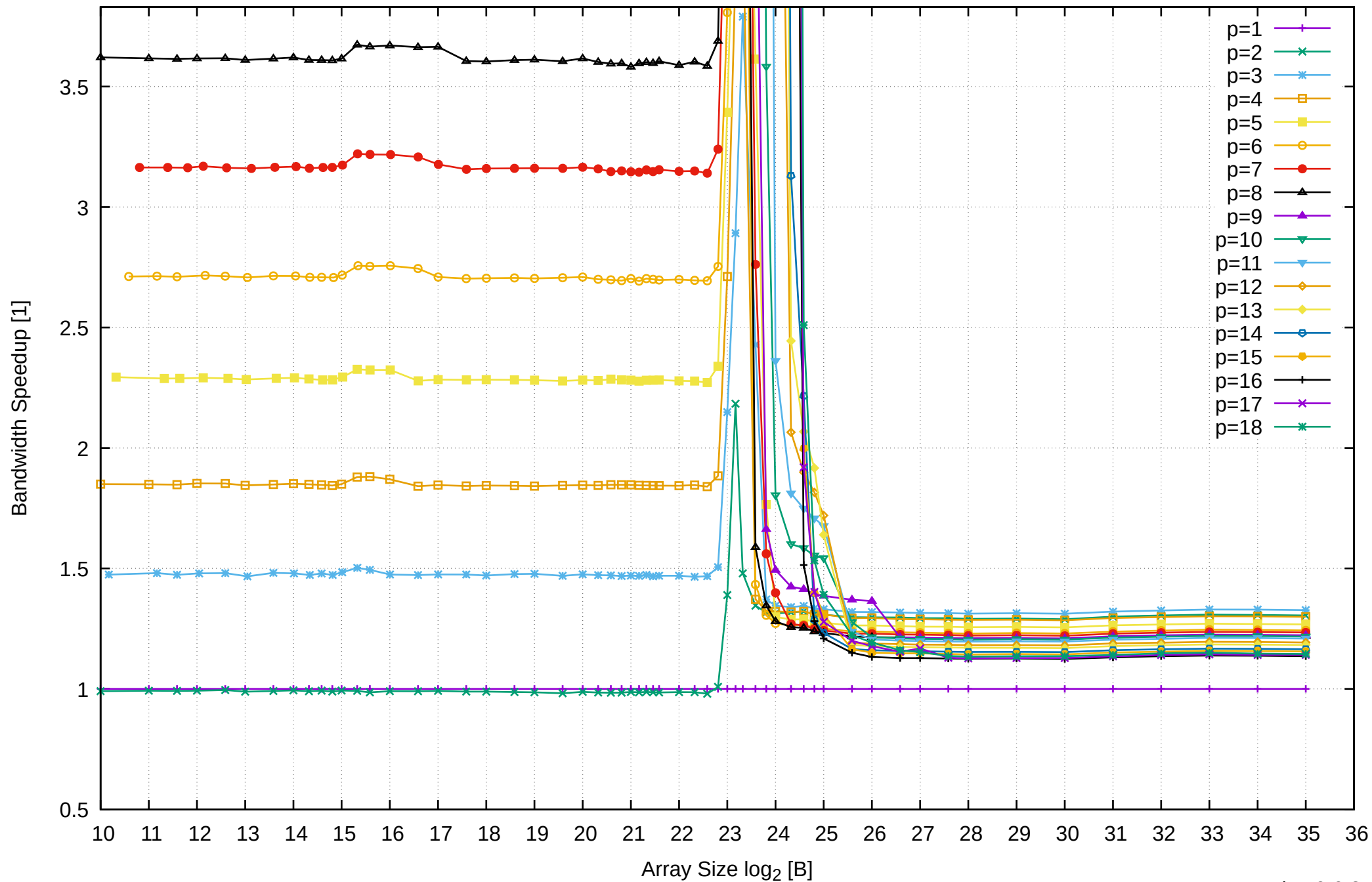
AMD Ryzen 7 1800X 64GB - Speedup of Parallel Memory Bandwidth (enlarged) - ScanWrite64IndexUnrollLoop
