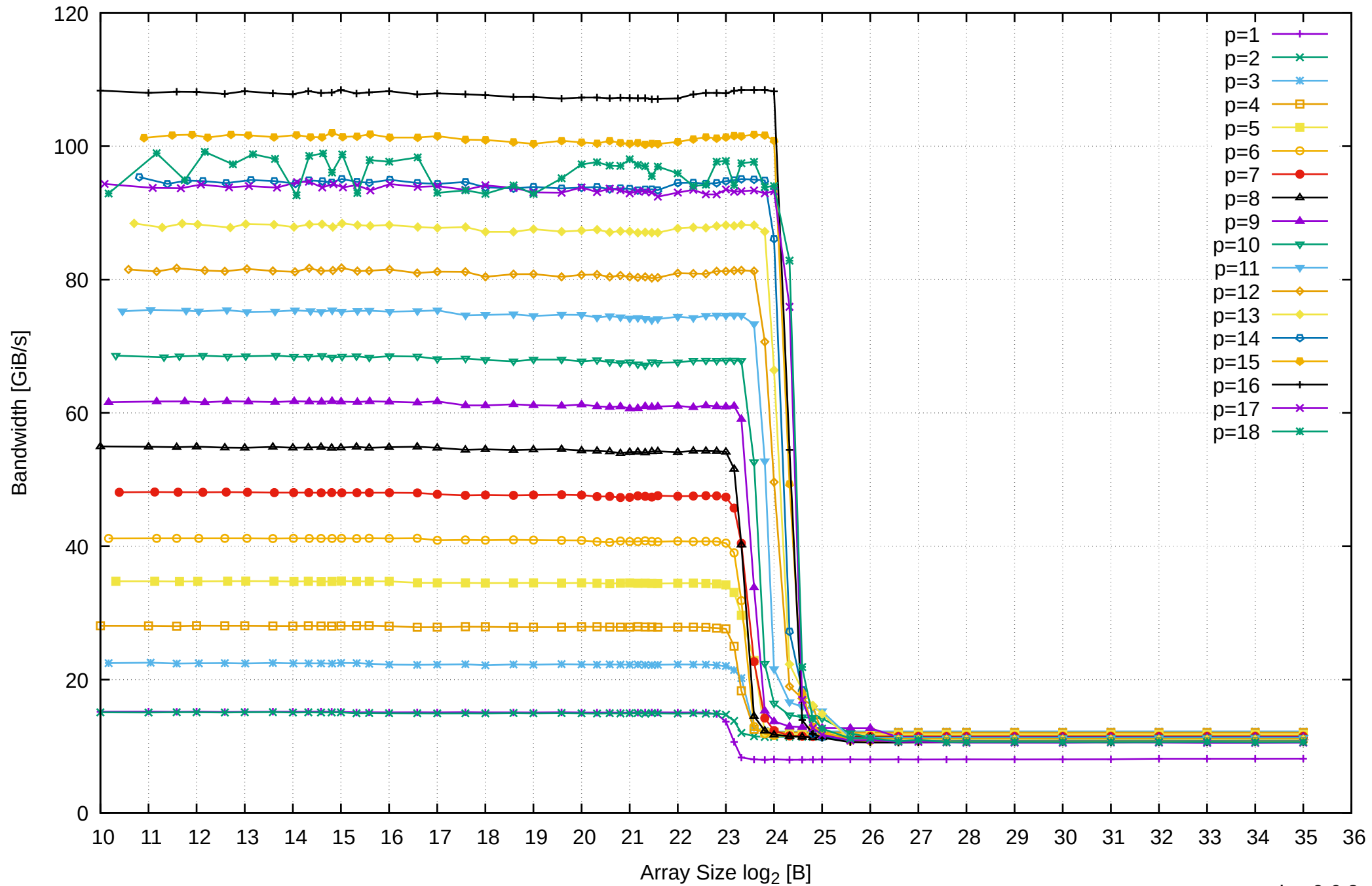
AMD Ryzen 7 1800X 64GB - Parallel Memory Bandwidth - ScanWrite32PtrUnrollLoop
