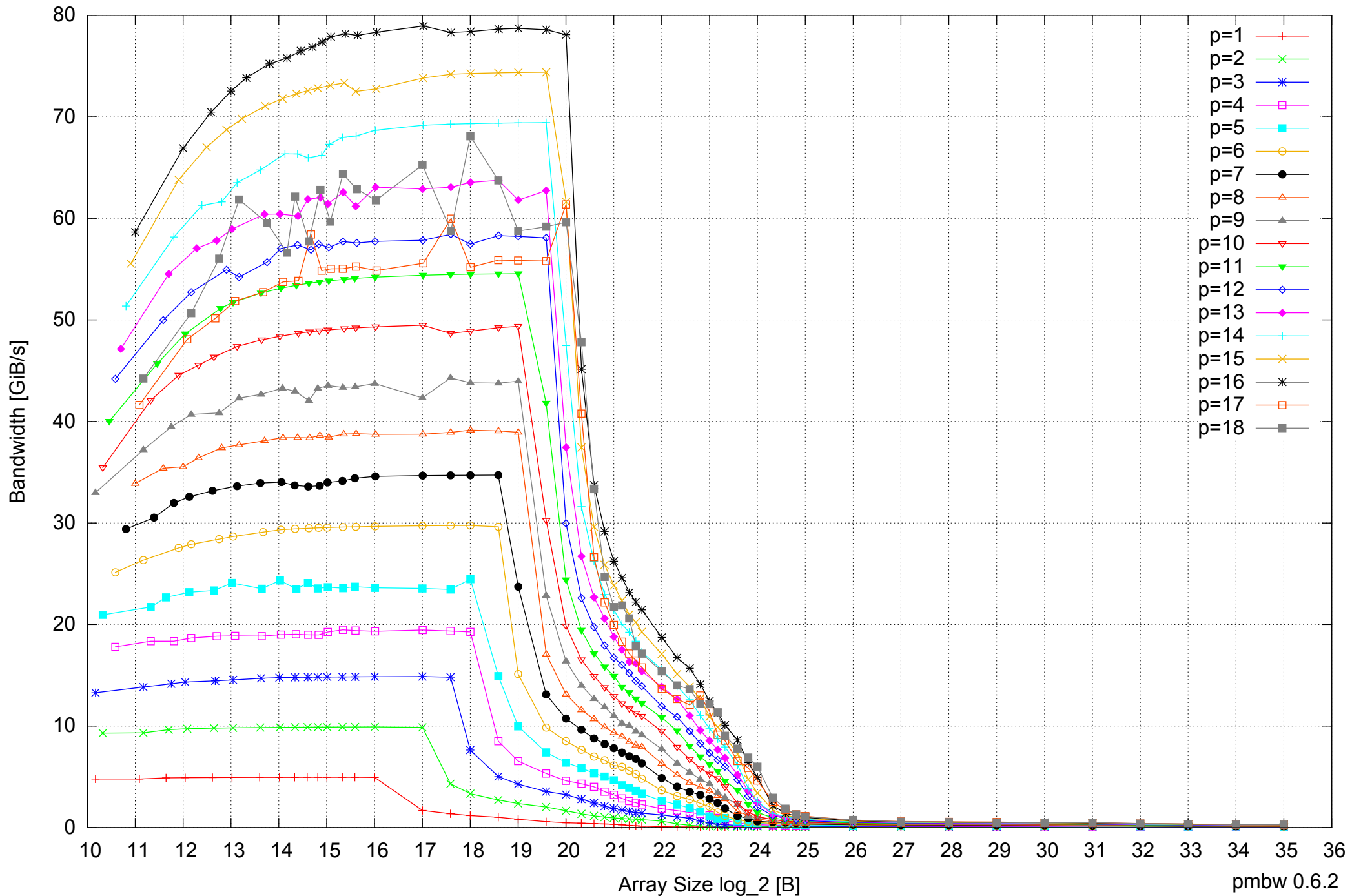
AMD Opteron 8350 64GB - Parallel Memory Bandwidth - PermRead64SimpleLoop
