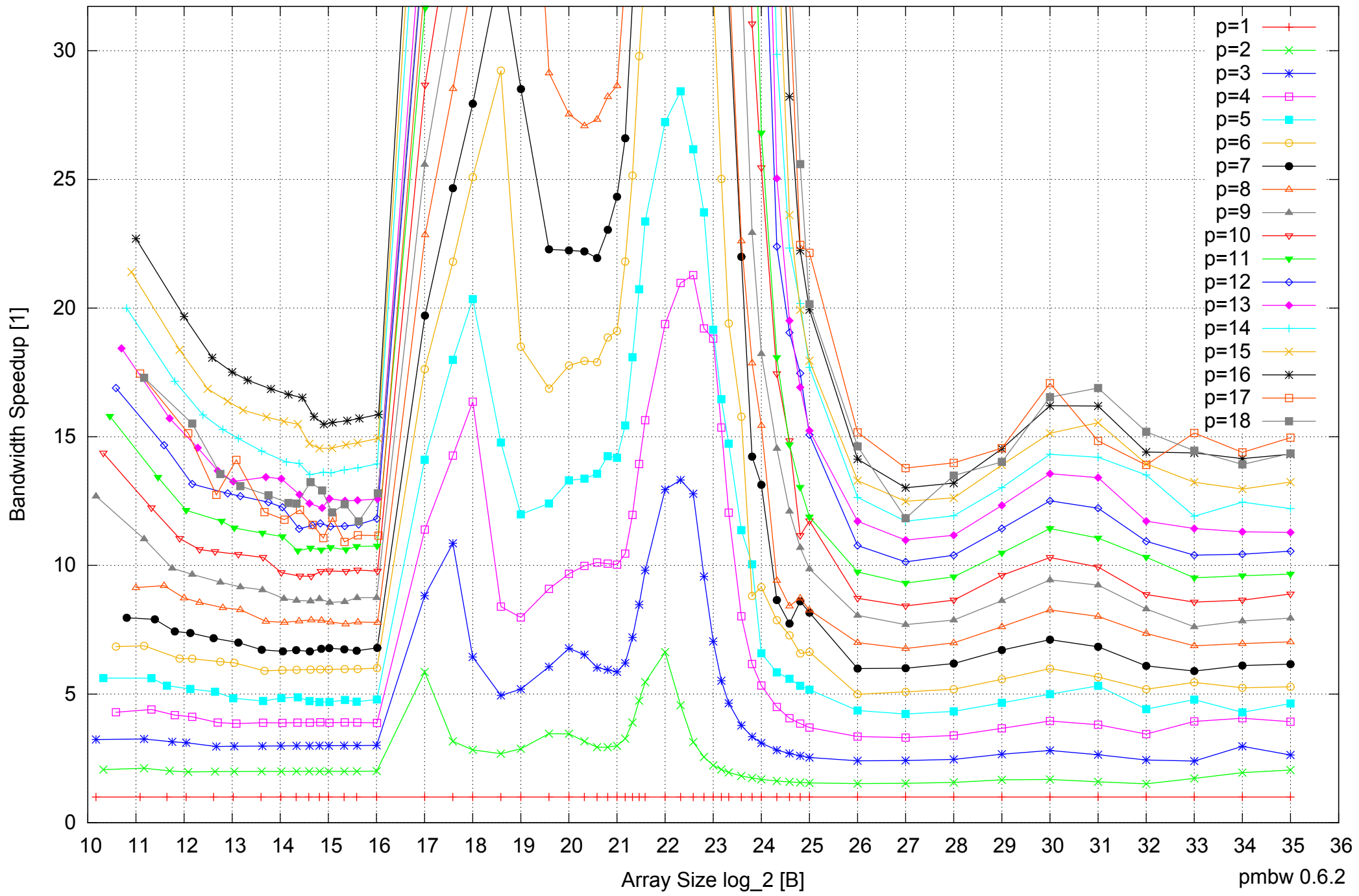
AMD Opteron 8350 64GB - Speedup of Parallel Memory Bandwidth (enlarged) - PermRead64UnrollLoop
