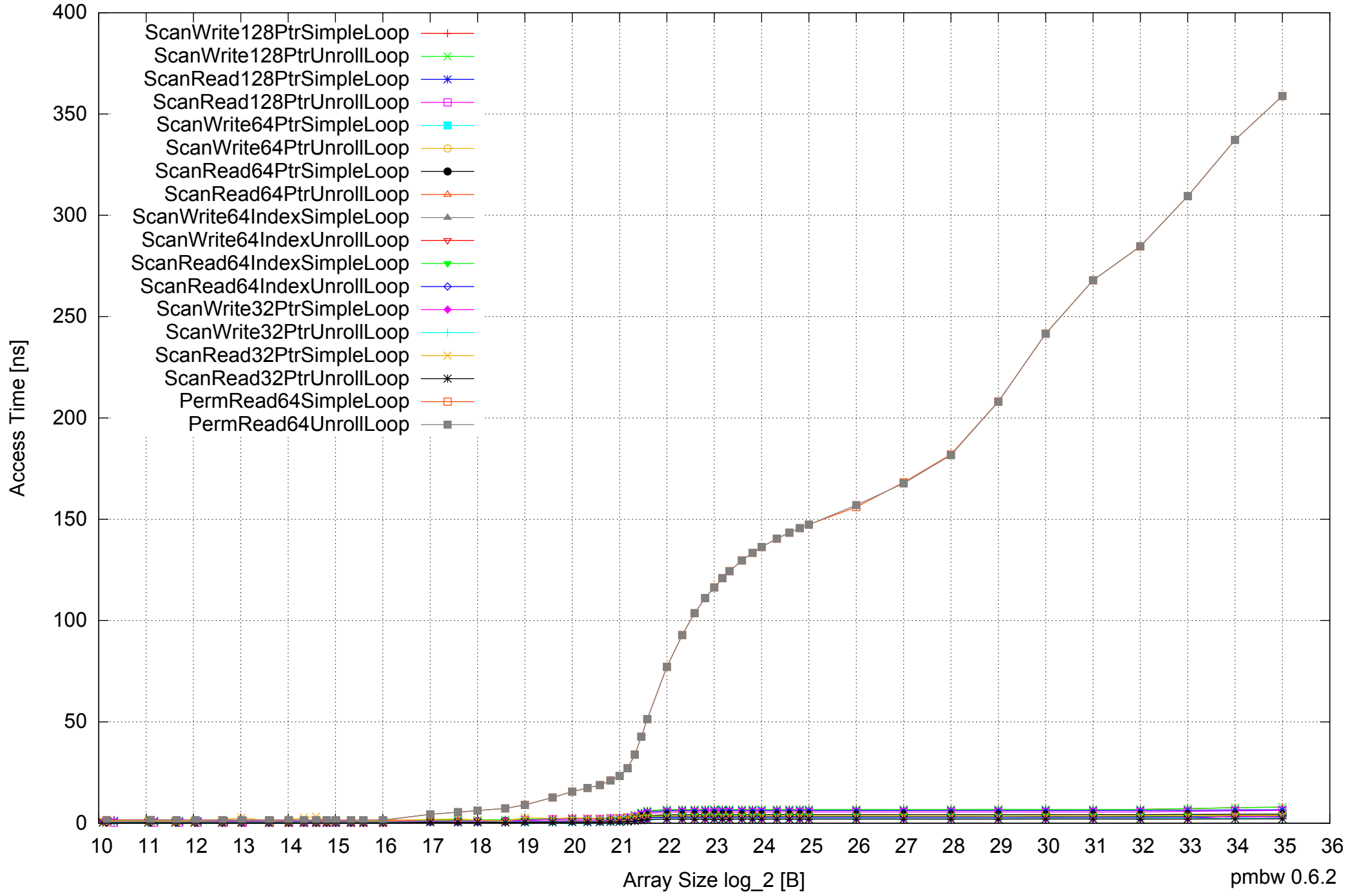
AMD Optron 8350 64GB - One Thread Memory Latency (Access Time)
