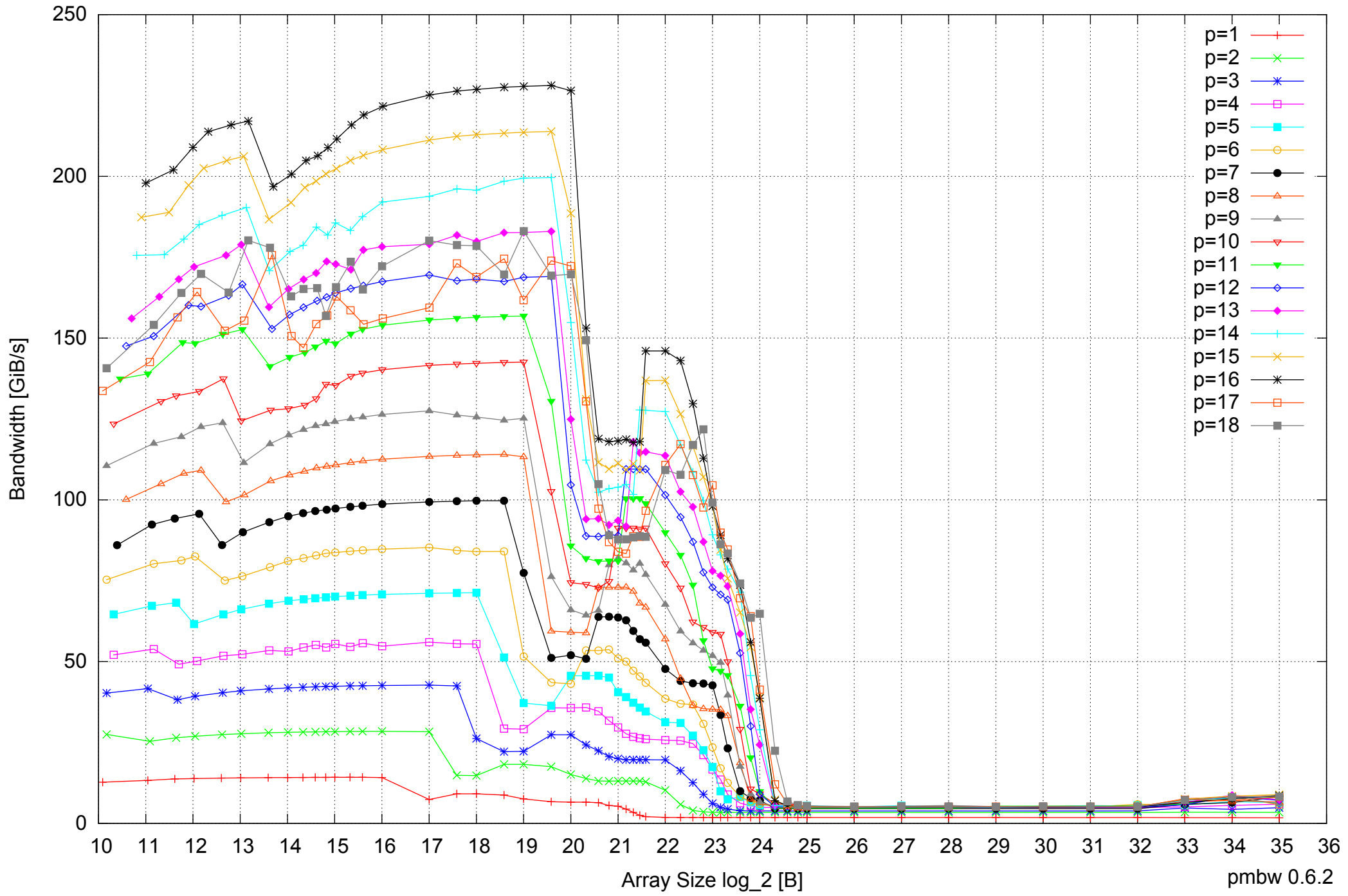
AMD Opteron 8350 64GB - Parallel Memory Bandwidth - ScanRead32PtrUnrollLoop
