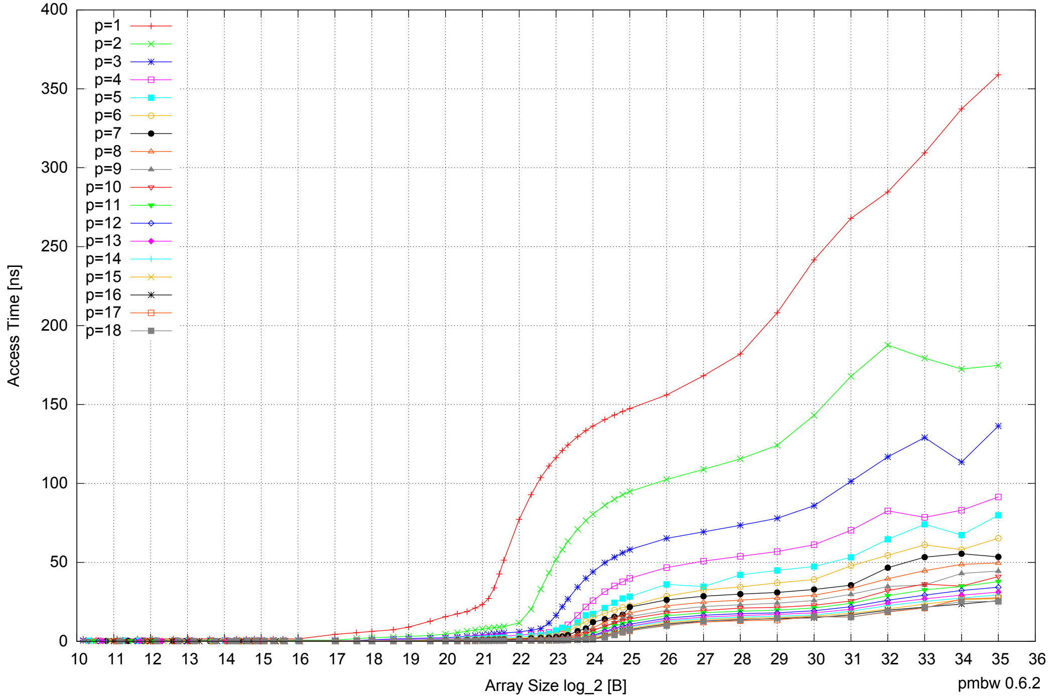
AMD Opteron 8350 64GB - Parallel Memory Access Time - PermRead64SimpleLoop
