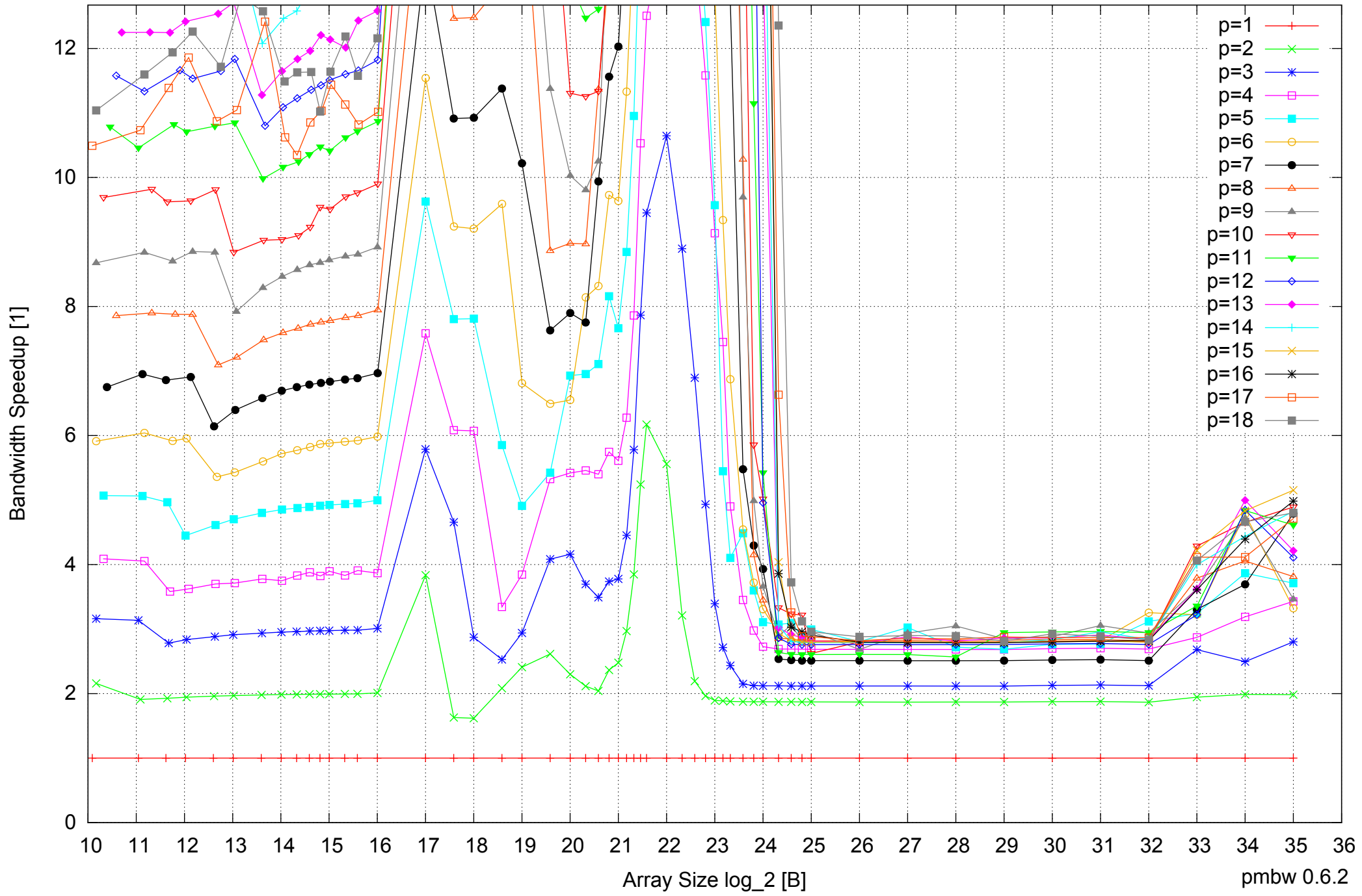
AMD Opteron 8350 64GB - Speedup of Parallel Memory Bandwidth (enlarged) - ScanRead32PtrUnrollLoop
