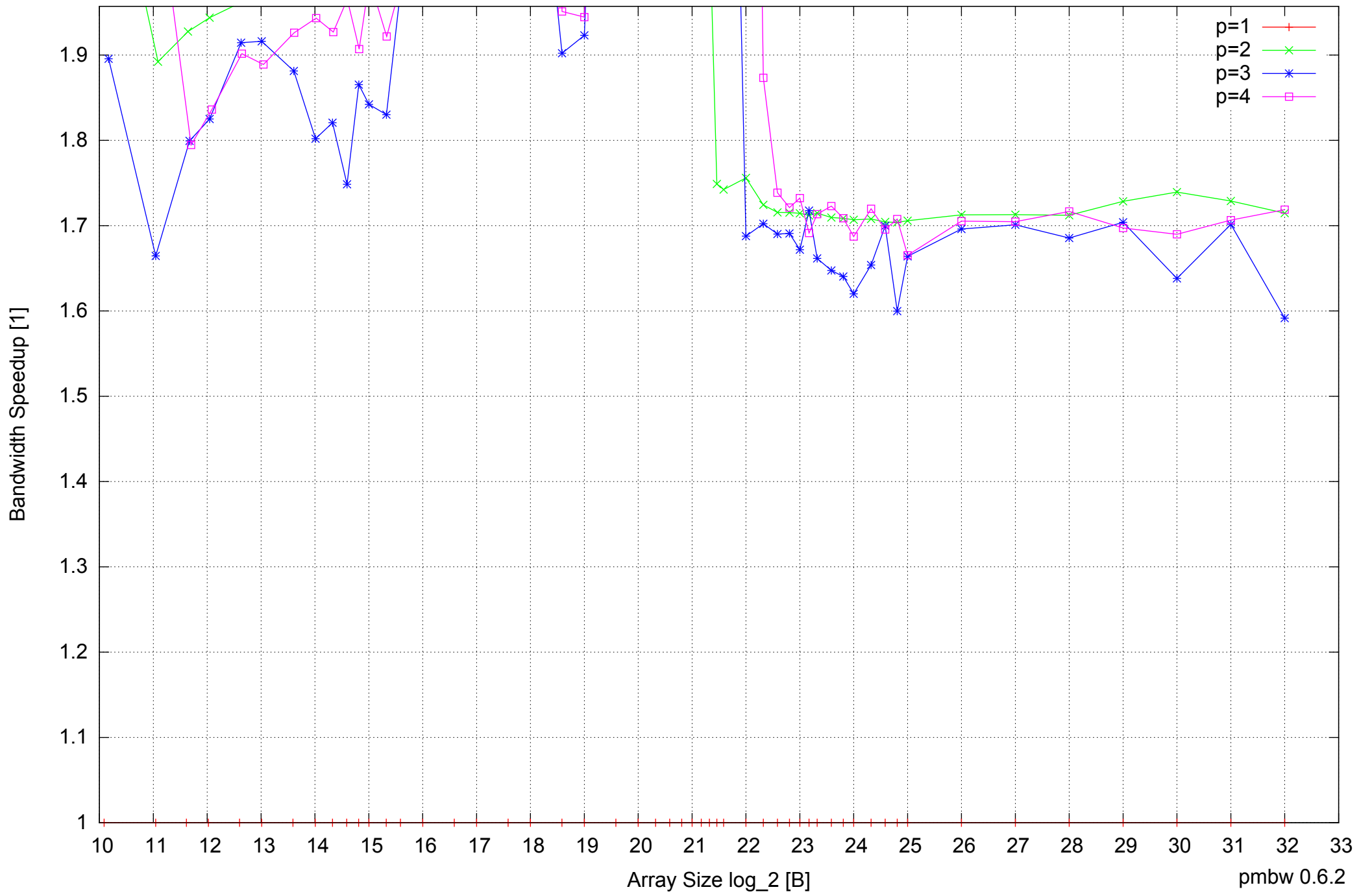
AMD Dual-Core Opteron 270 8GB - Speedup of Parallel Memory Bandwidth (enlarged) - ScanRead32PtrUnrollLoop
