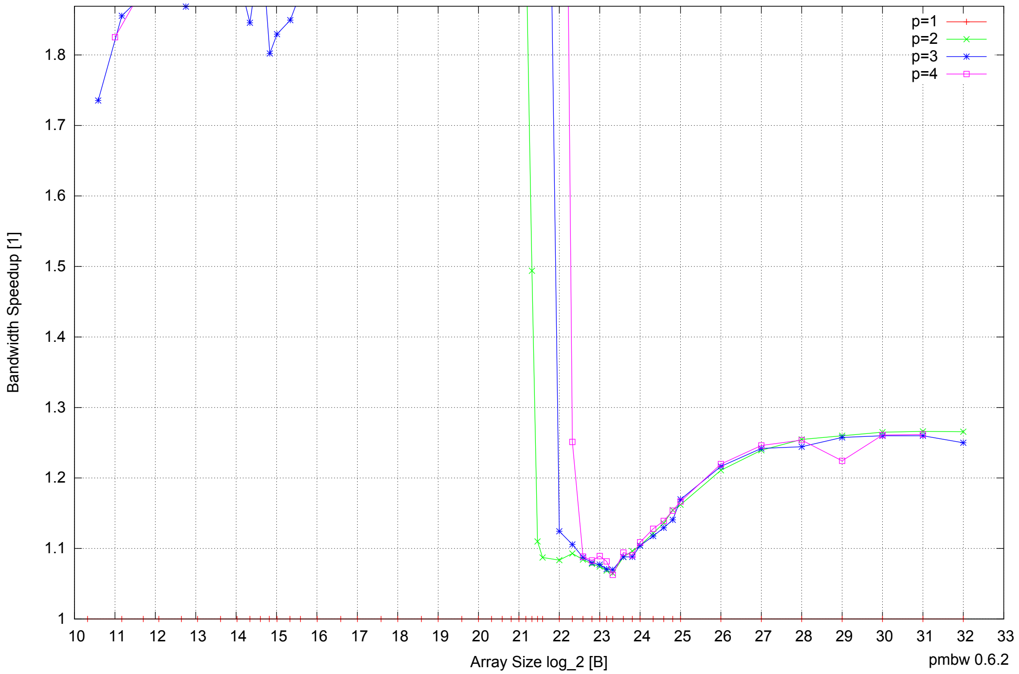
AMD Dual-Core Opteron 270 8GB - Speedup of Parallel Memory Bandwidth (enlarged) - ScanWrite128PtrSimpleLoop
