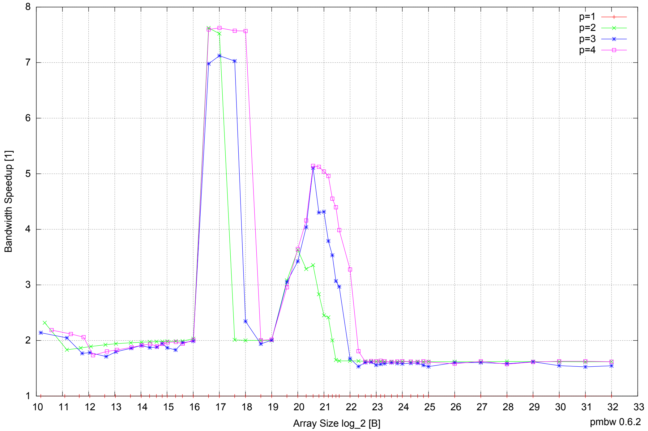
AMD Dual-Core Opteron 270 8GB - Speedup of Parallel Memory Bandwidth - ScanRead64IndexUnrollLoop
