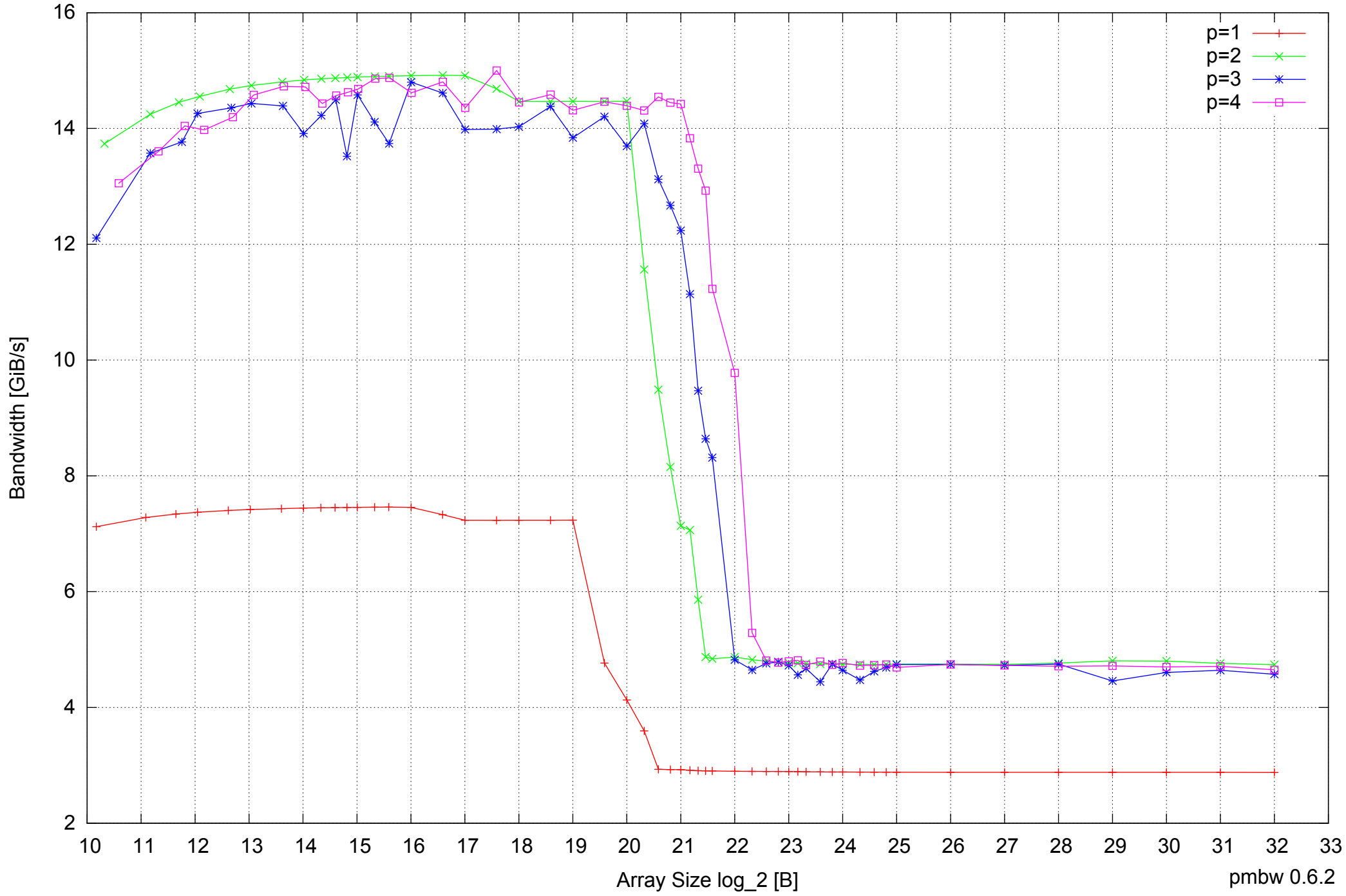
AMD Dual-Core Opteron 270 8GB - Parallel Memory Bandwidth - ScanRead64IndexSimpleLoop
