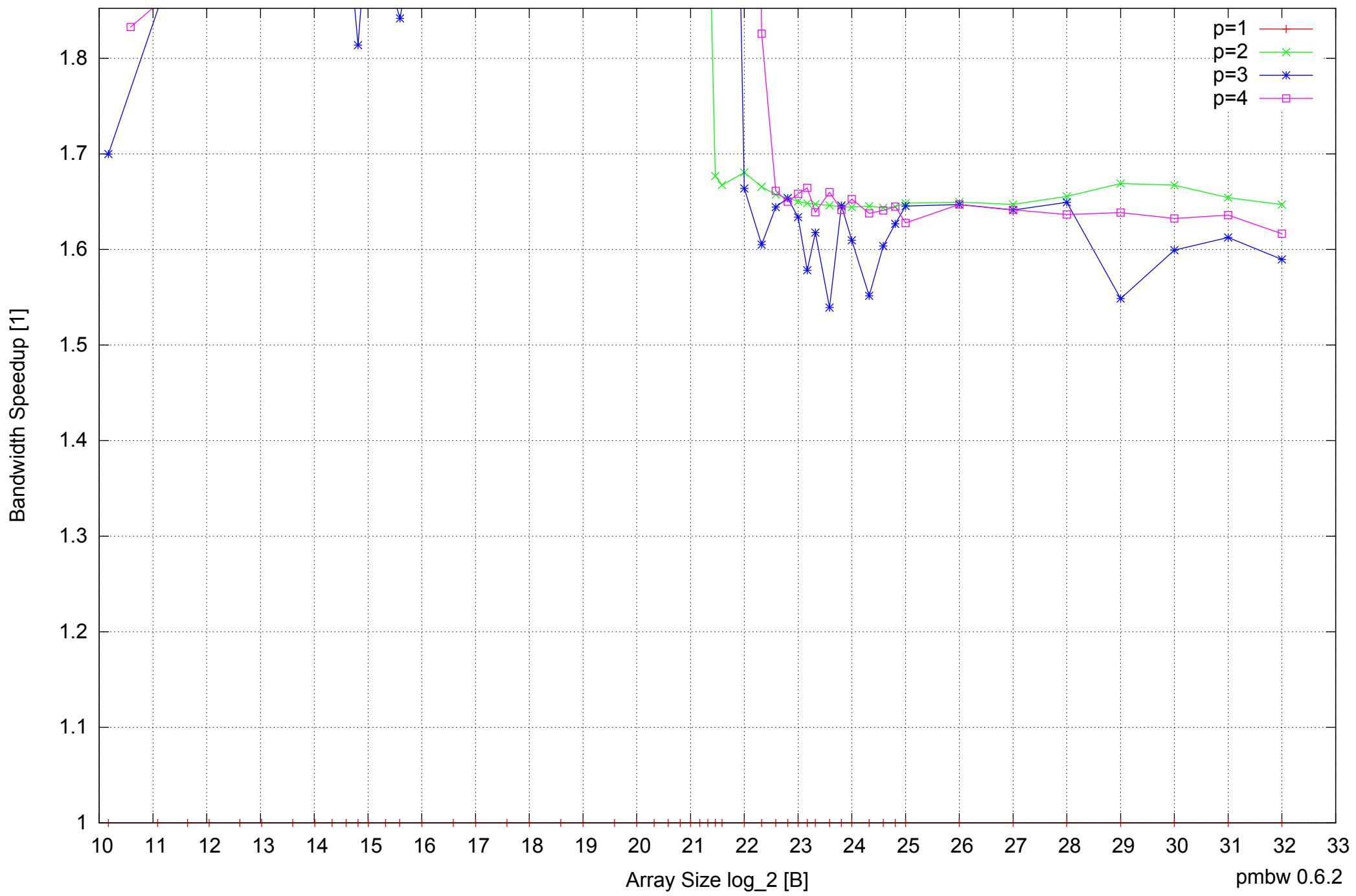
AMD Dual-Core Opteron 270 8GB - Speedup of Parallel Memory Bandwidth (enlarged) - ScanRead64IndexSimpleLoop
