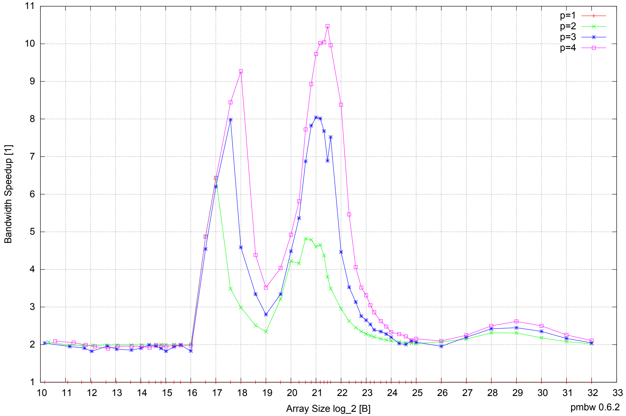
AMD Dual-Core Opteron 270 8GB - Speedup of Parallel Memory Bandwidth - PermRead64UnrollLoop
