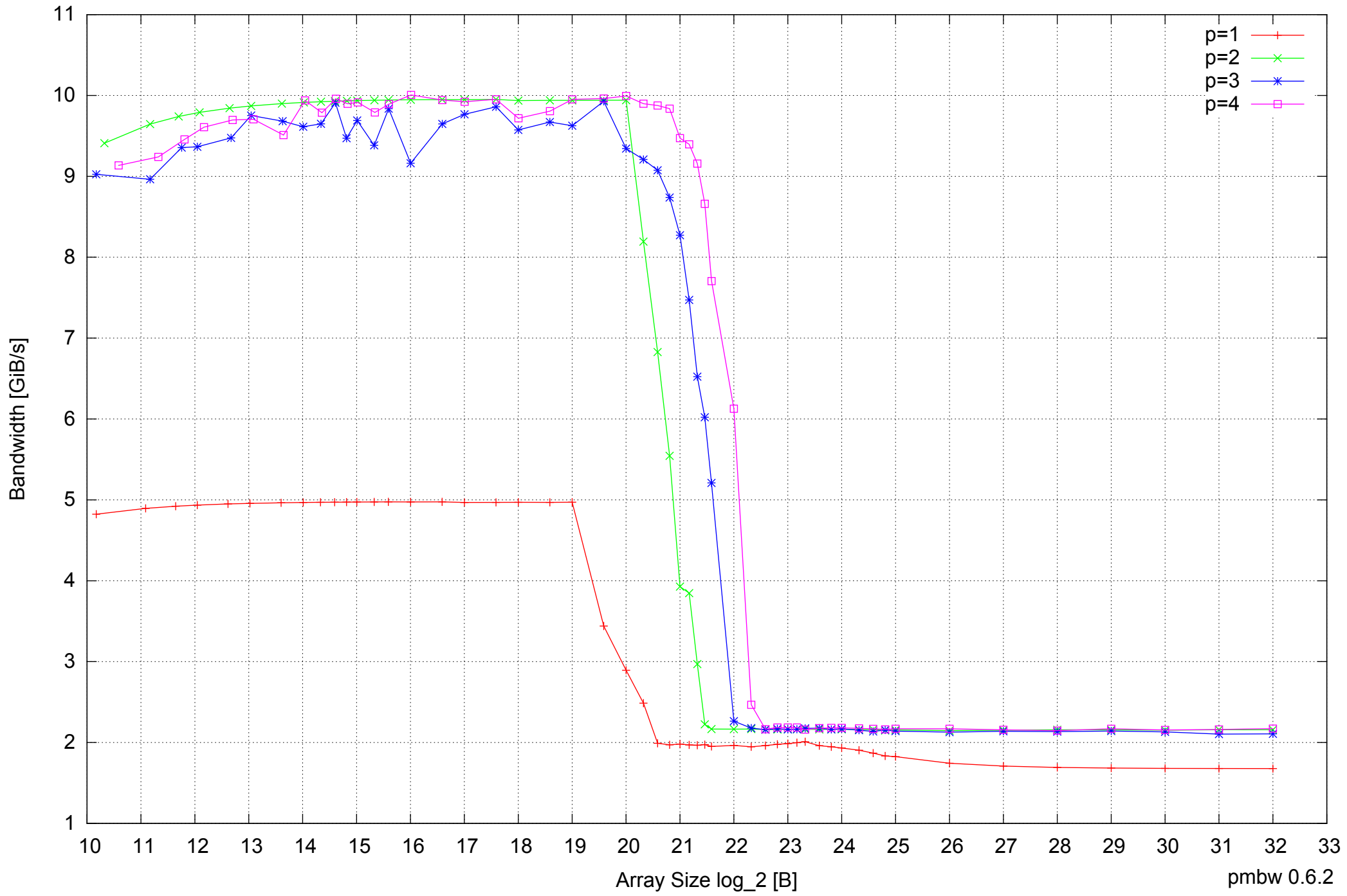
AMD Dual-Core Opteron 270 8GB - Parallel Memory Bandwidth - ScanWrite64IndexSimpleLoop
