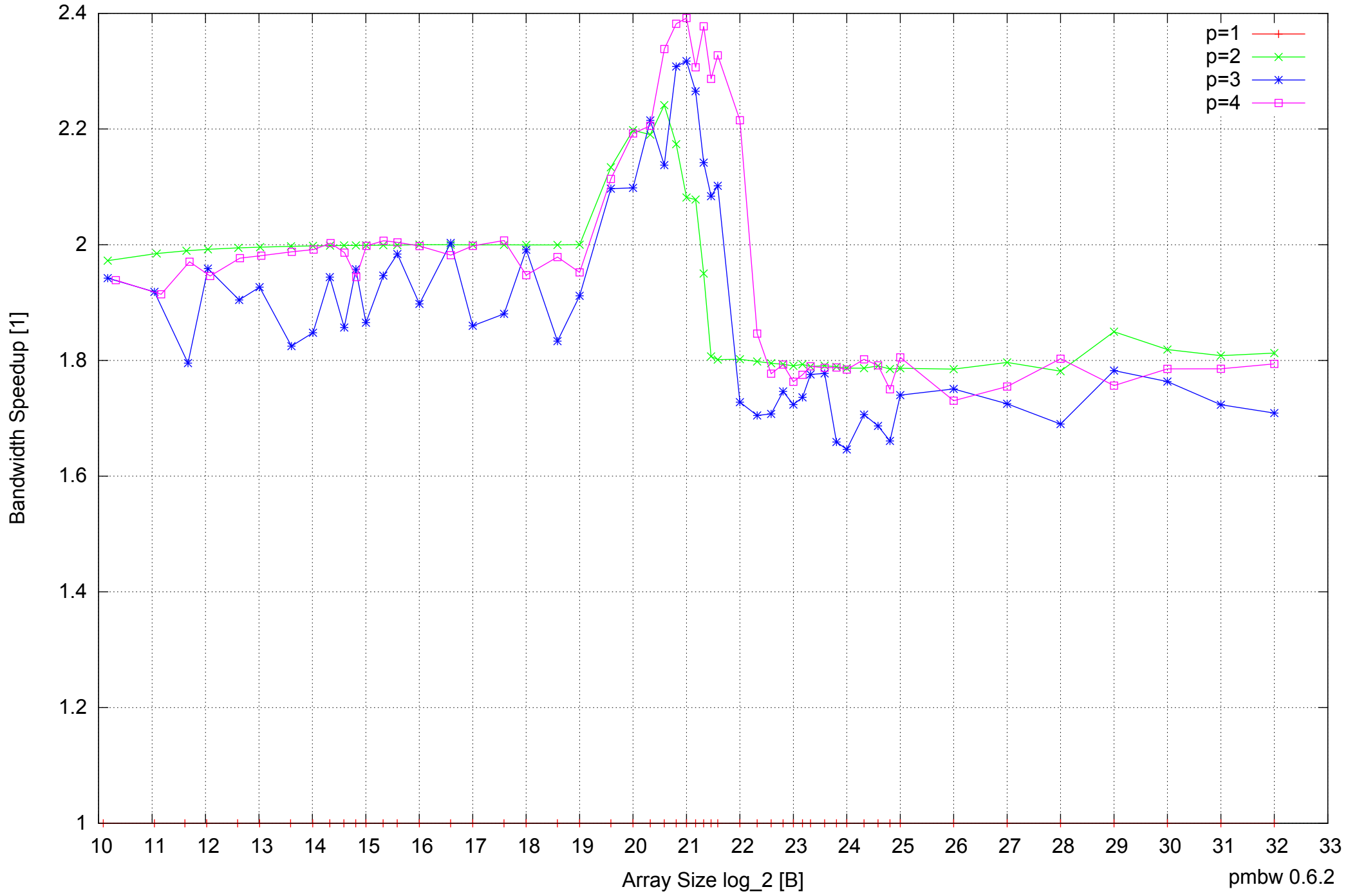
AMD Dual-Core Opteron 270 8GB - Speedup of Parallel Memory Bandwidth - ScanRead32PtrSimpleLoop
