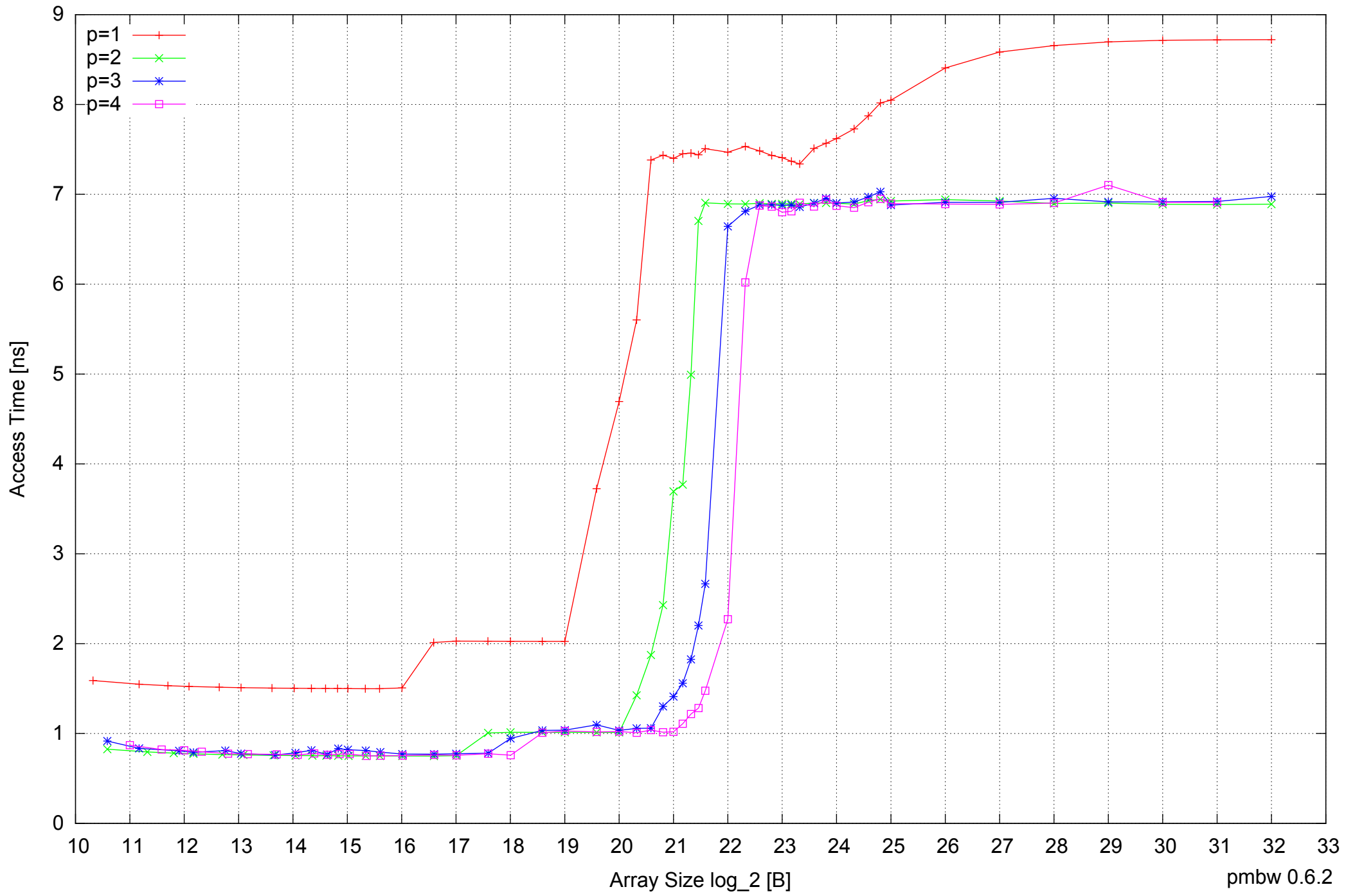
AMD Dual-Core Opteron 270 8GB - Parallel Memory Access Time - ScanWrite128PtrSimpleLoop
