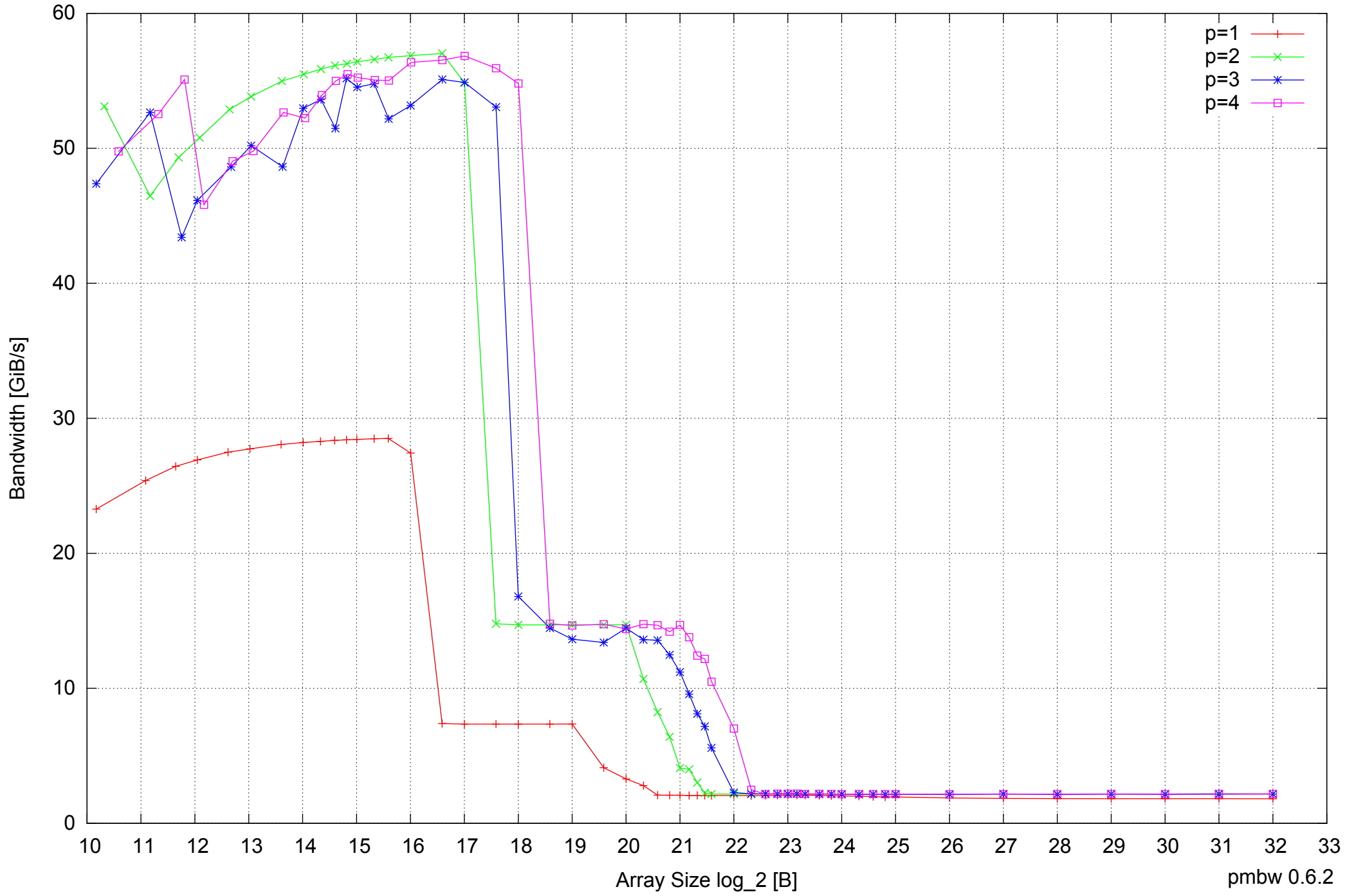
AMD Dual-Core Opteron 270 8GB - Parallel Memory Bandwidth - ScanWrite64PtrUnrollLoop
