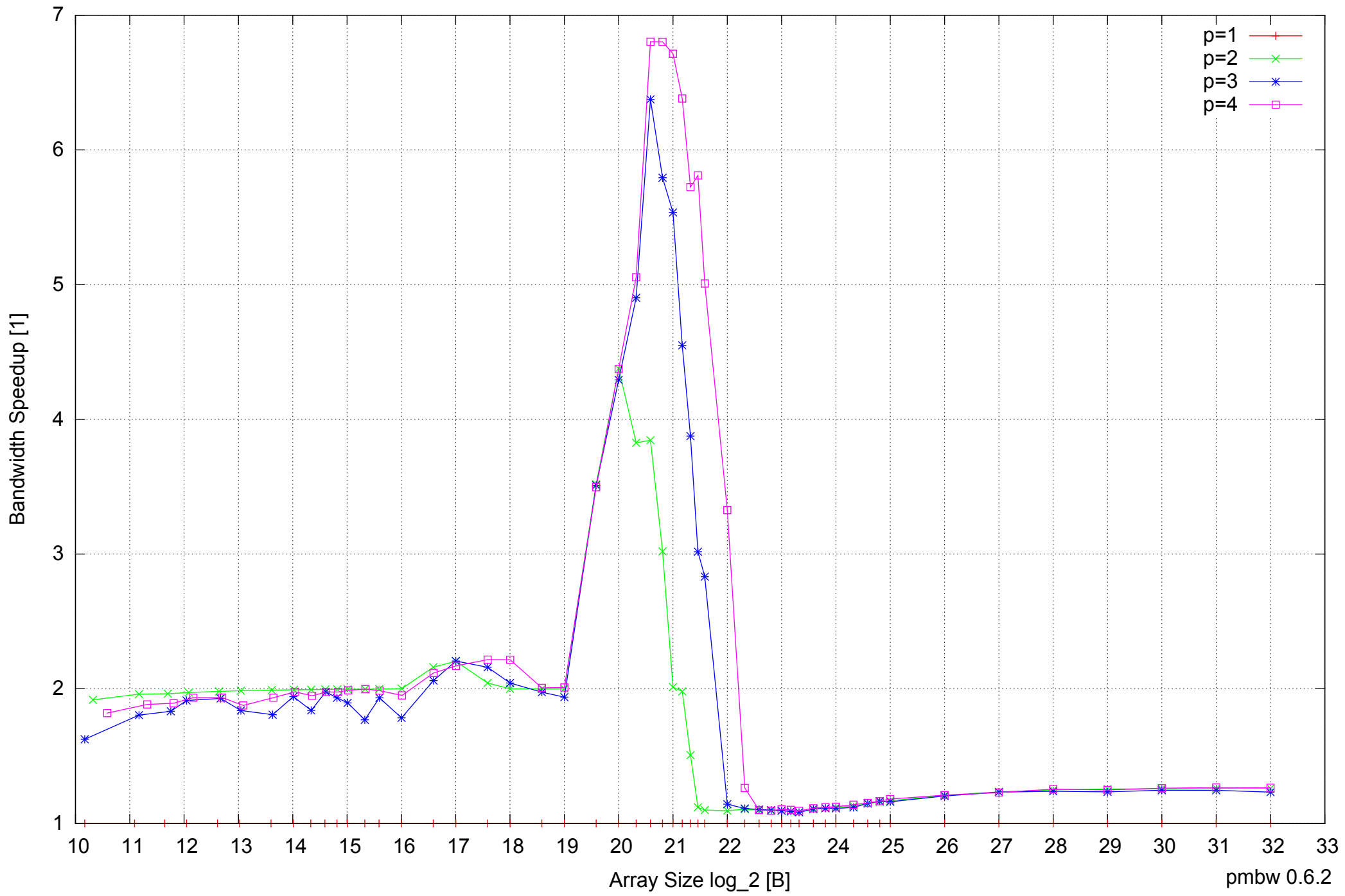
AMD Dual-Core Opteron 270 8GB - Speedup of Parallel Memory Bandwidth - ScanWrite64PtrSimpleLoop
