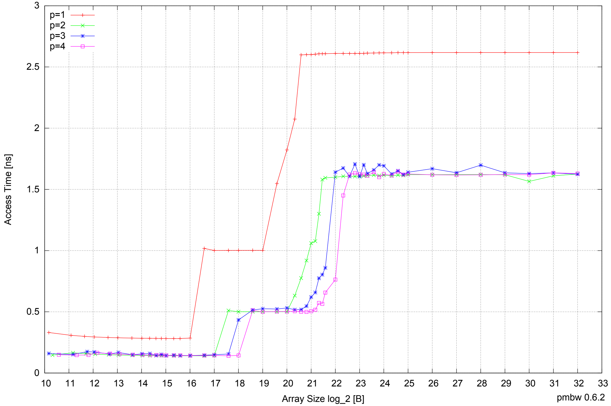
AMD Dual-Core Opteron 270 8GB - Parallel Memory Access Time - ScanRead64PtrUnrollLoop
