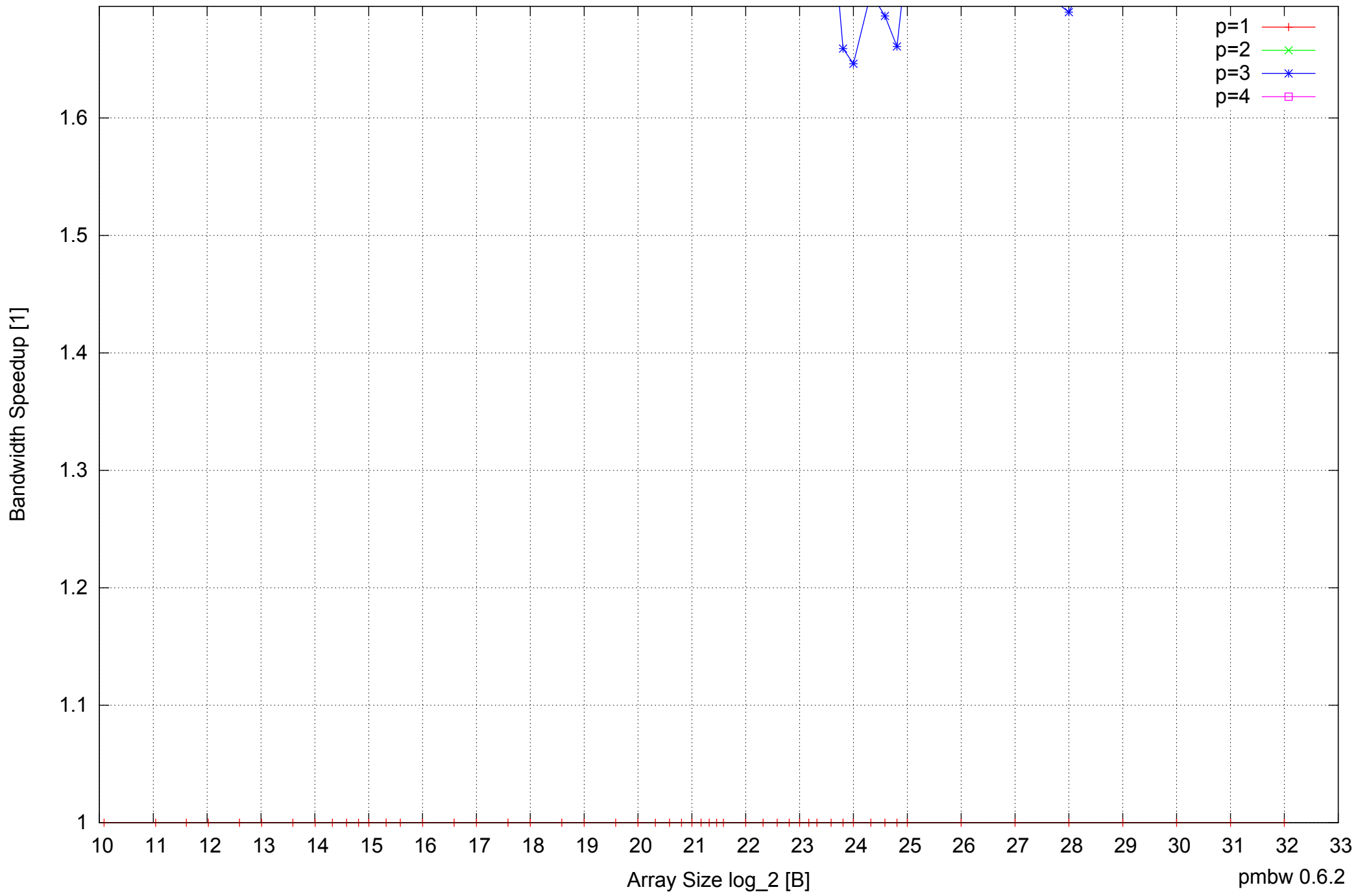
AMD Dual-Core Opteron 270 8GB - Speedup of Parallel Memory Bandwidth (enlarged) - ScanRead32PtrSimpleLoop
