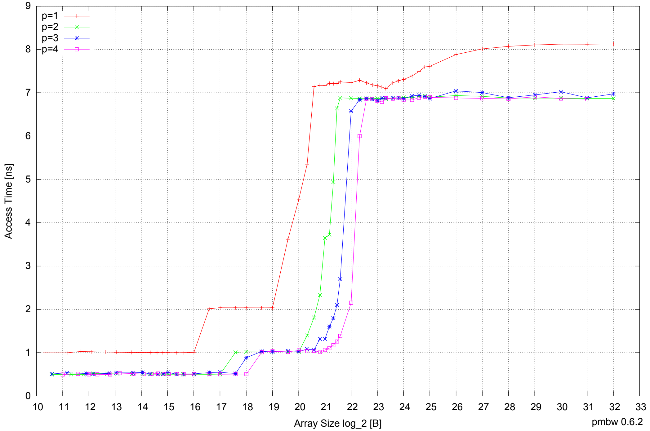
AMD Dual-Core Opteron 270 8GB - Parallel Memory Access Time - ScanWrite128PtrUnrollLoop
