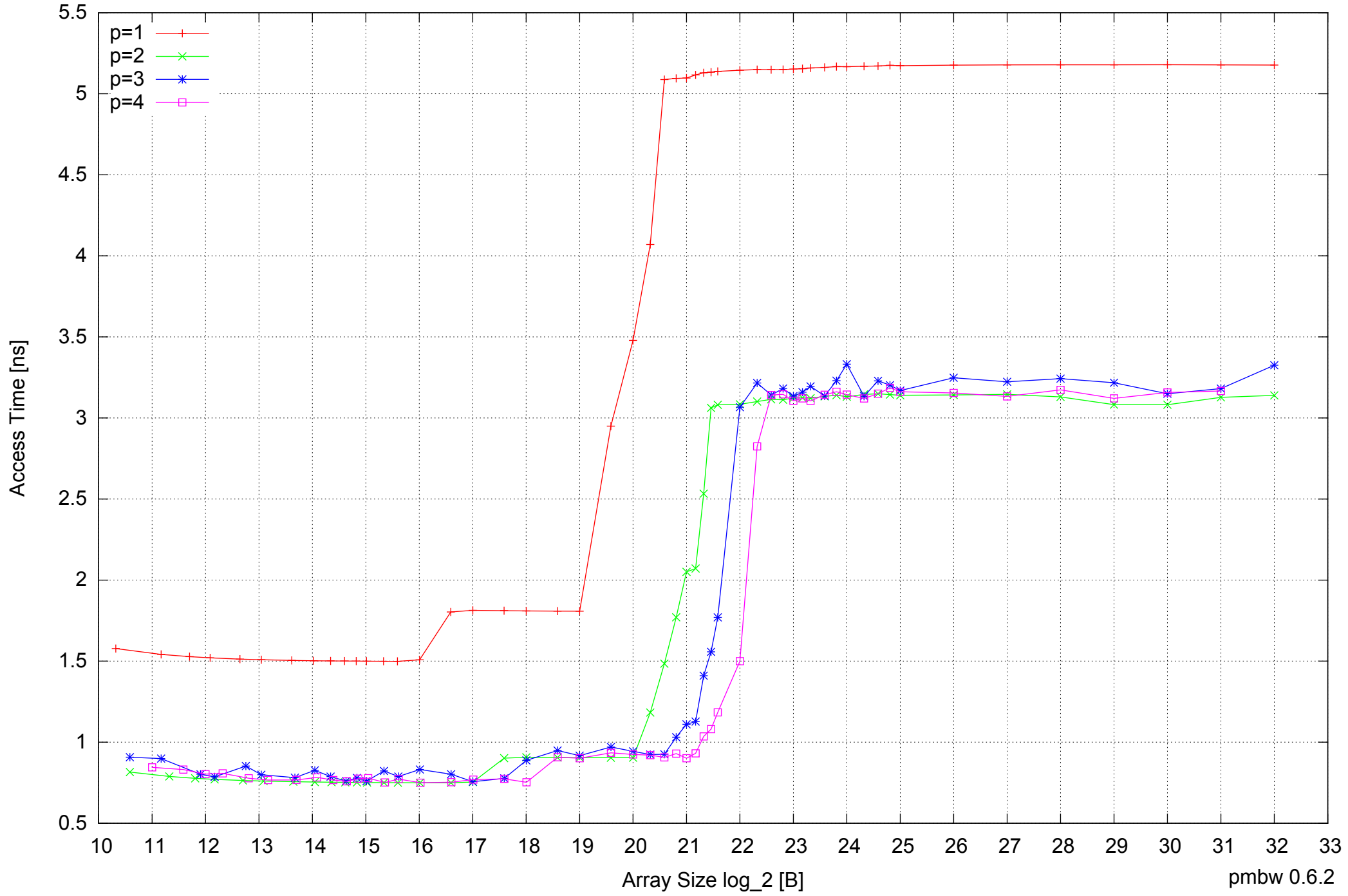
AMD Dual-Core Opteron 270 8GB - Parallel Memory Access Time - ScanRead128PtrSimpleLoop
