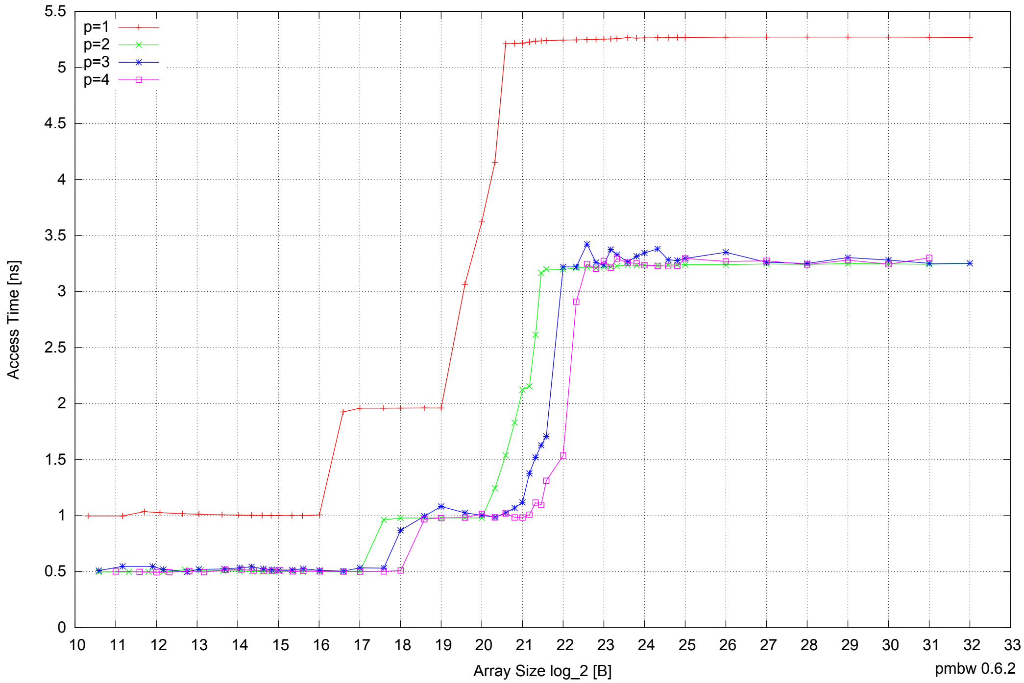
AMD Dual-Core Opteron 270 8GB - Parallel Memory Access Time - ScanRead128PtrUnrollLoop
