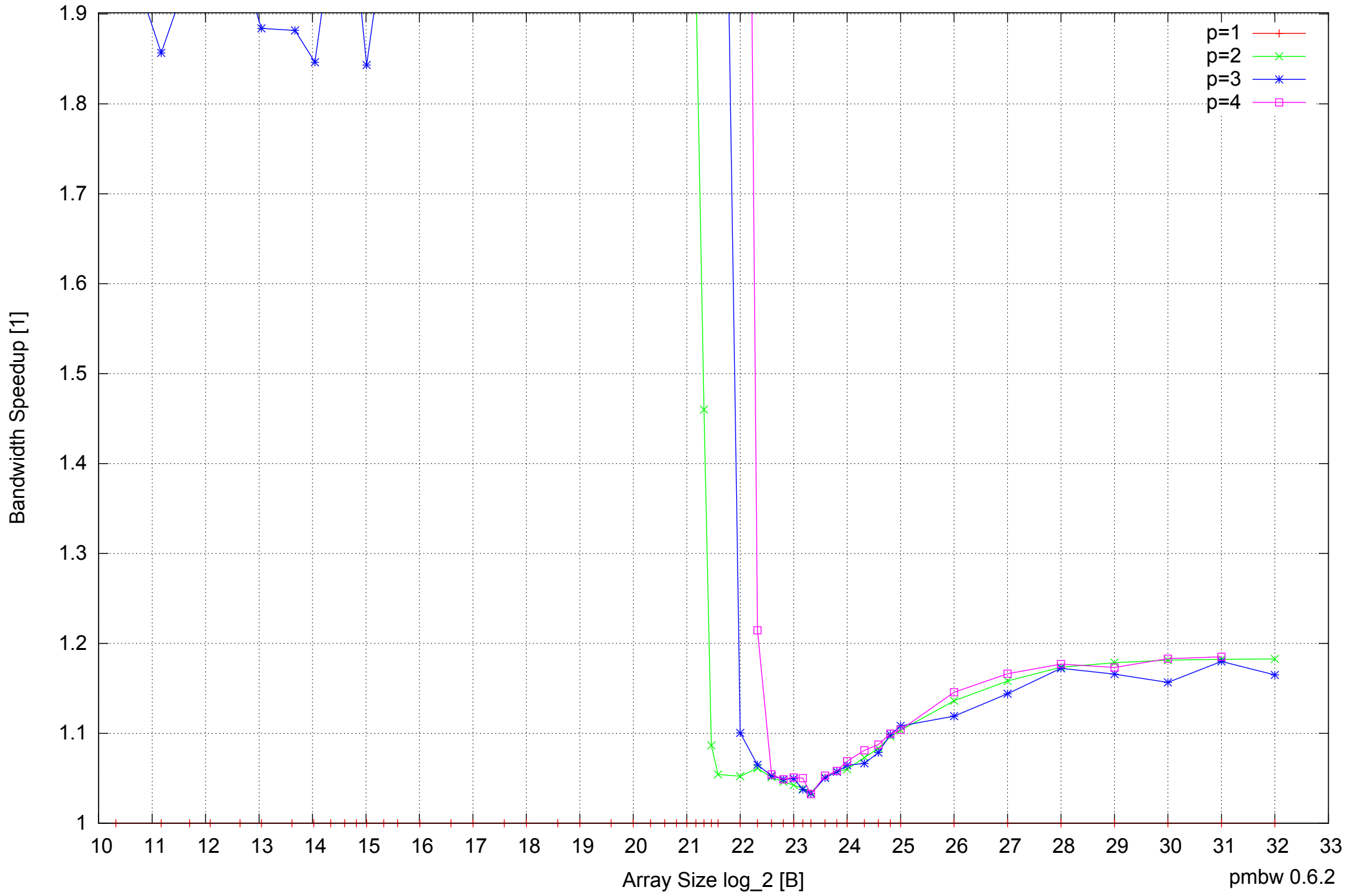
AMD Dual-Core Optron 270 8GB - Speedup of Parallel Memory Bandwidth (enlarged) - ScanWrite128PtrUnrollLoop
