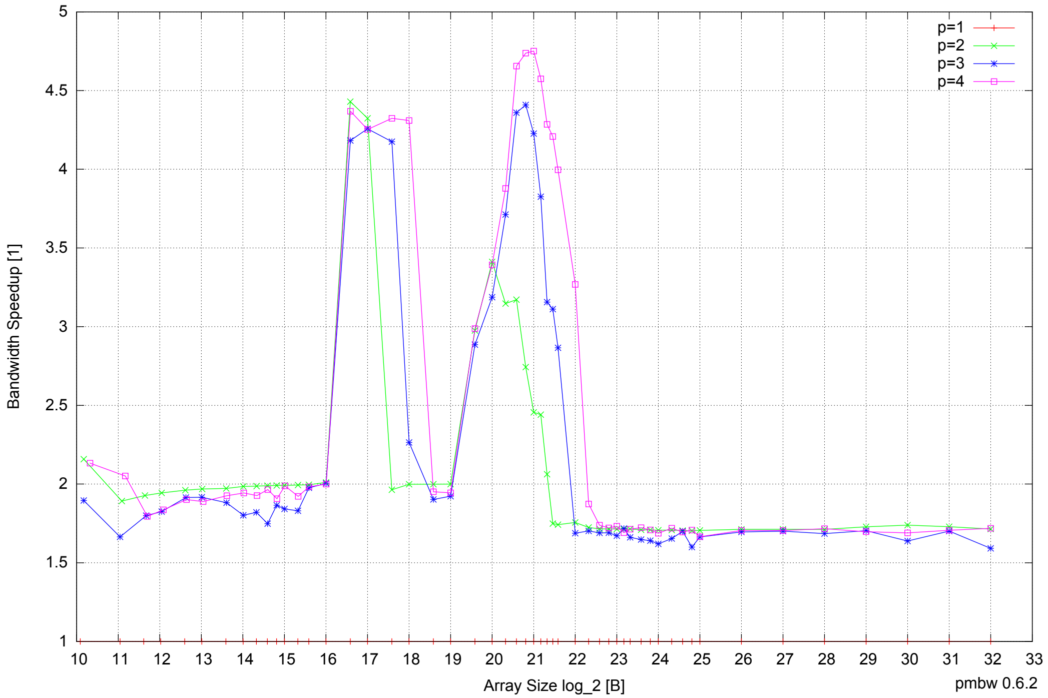
AMD Dual-Core Opteron 270 8GB - Speedup of Parallel Memory Bandwidth - ScanRead32PtrUnrollLoop
