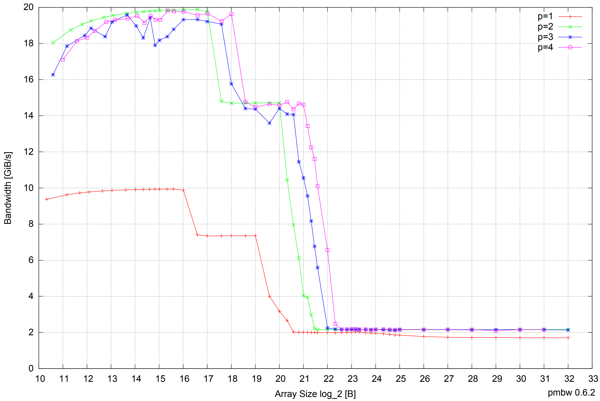
AMD Dual-Core Opteron 270 8GB - Parallel Memory Bandwidth - ScanWrite128PtrSimpleLoop
