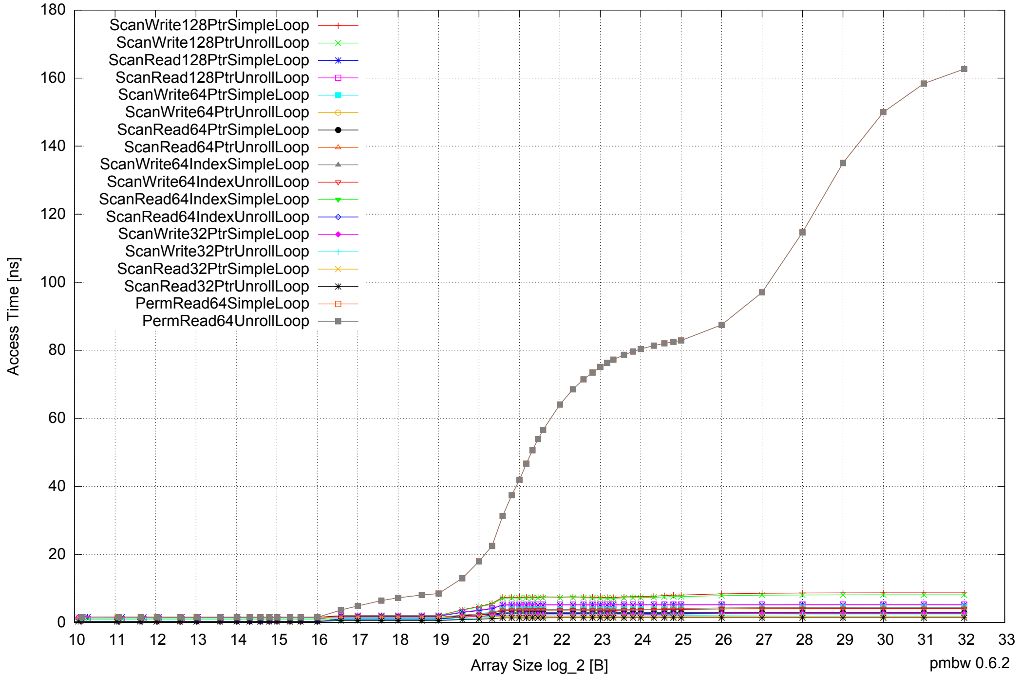
AMD Dual-Core Opteron 270 8GB - One Thread Memory Latency (Access Time)
