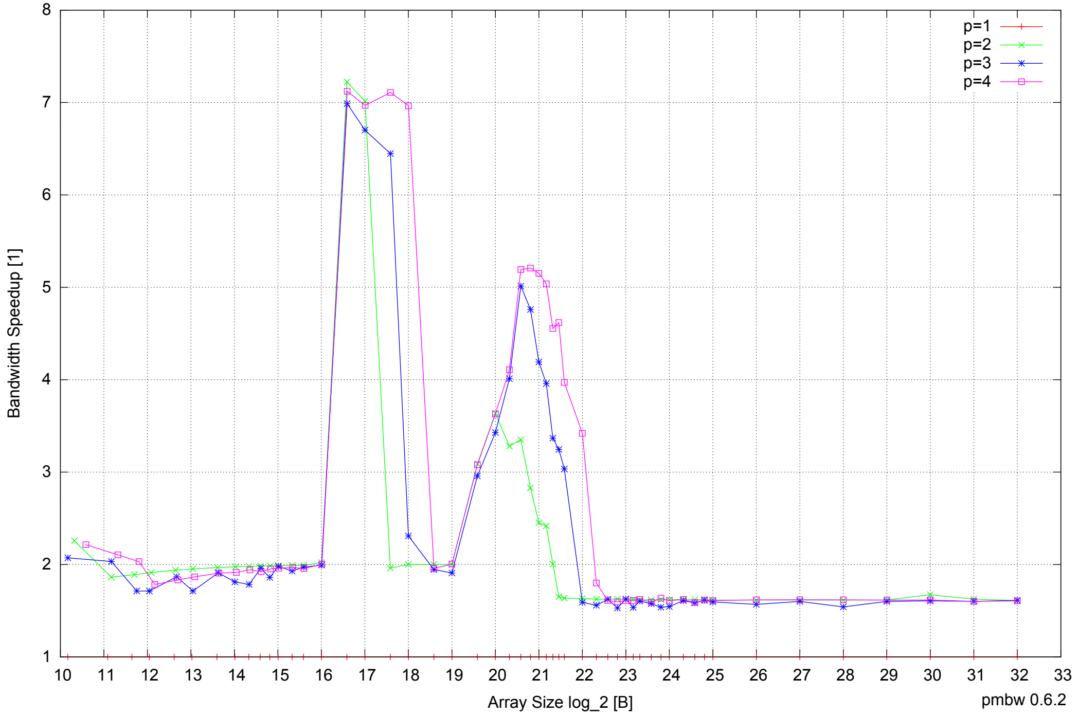
AMD Dual-Core Opteron 270 8GB - Speedup of Parallel Memory Bandwidth - ScanRead64PtrUnrollLoop
