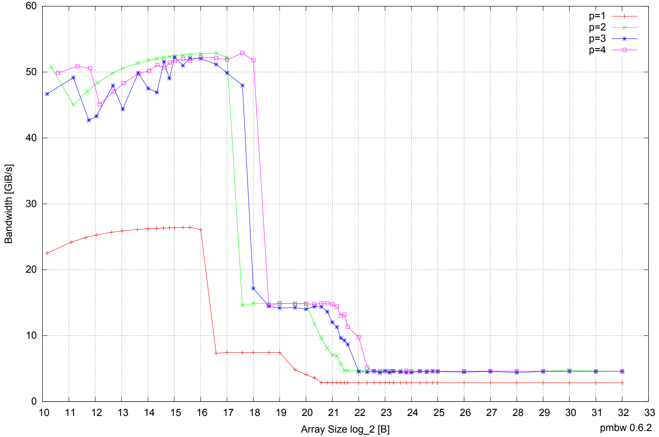
AMD Dual-Core Opteron 270 8GB - Parallel Memory Bandwidth - ScanRead64PtrUnrollLoop
