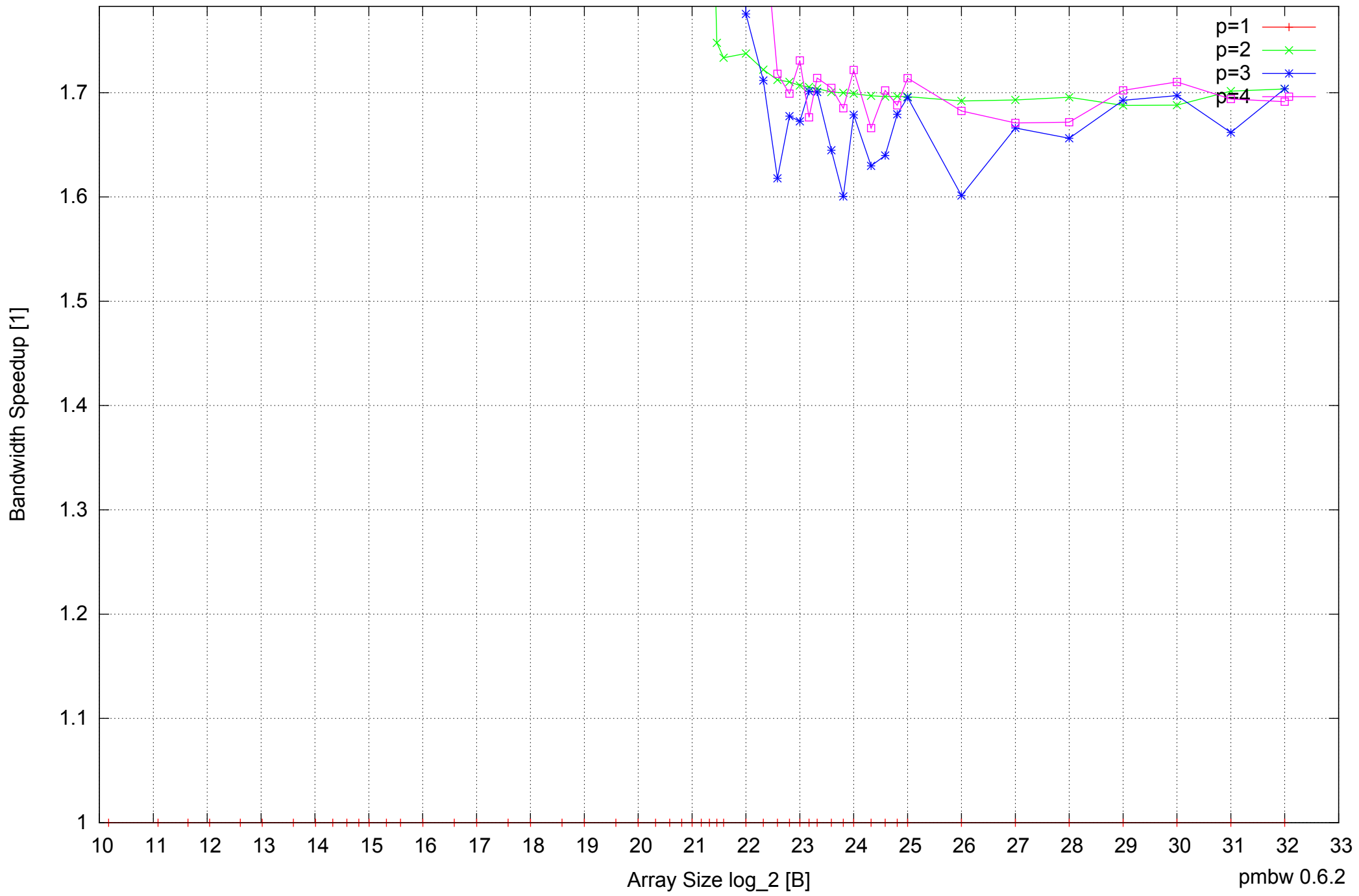
AMD Dual-Core Optron 270 8GB - Speedup of Parallel Memory Bandwidth (enlarged) - ScanRead64PtrSimpleLoop
