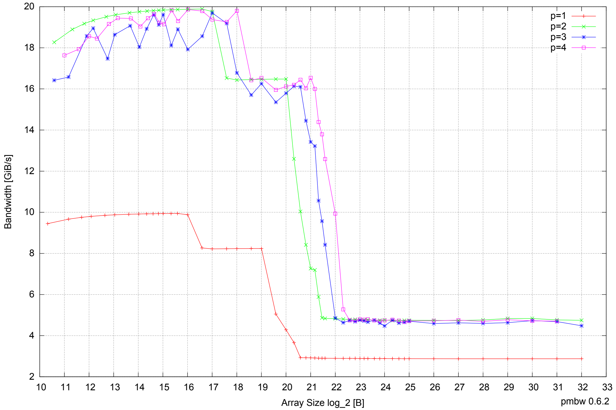
AMD Dual-Core Opteron 270 8GB - Parallel Memory Bandwidth - ScanRead128PtrSimpleLoop
