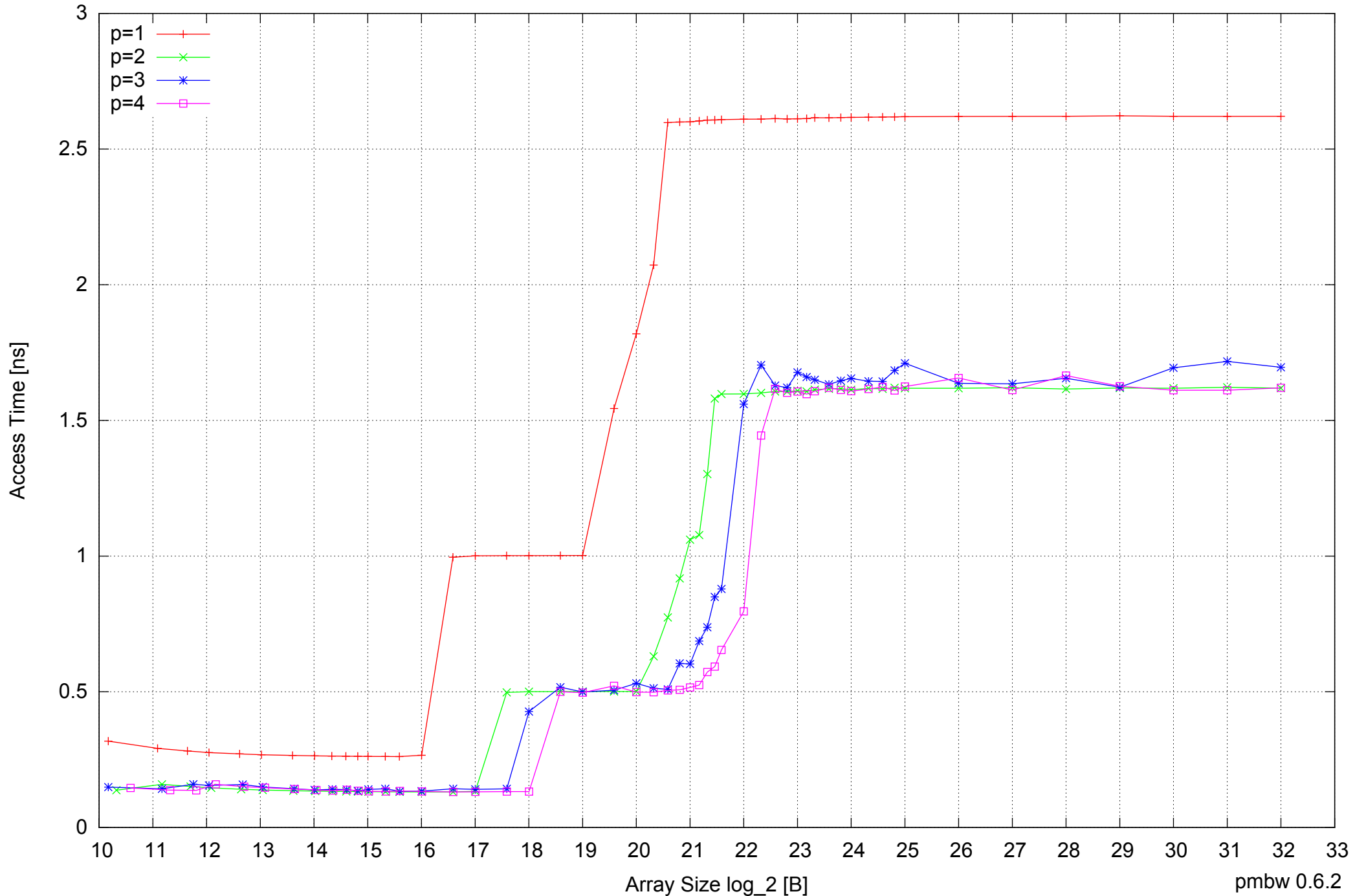
AMD Dual-Core Opteron 270 8GB - Parallel Memory Access Time - ScanRead64IndexUnrollLoop
