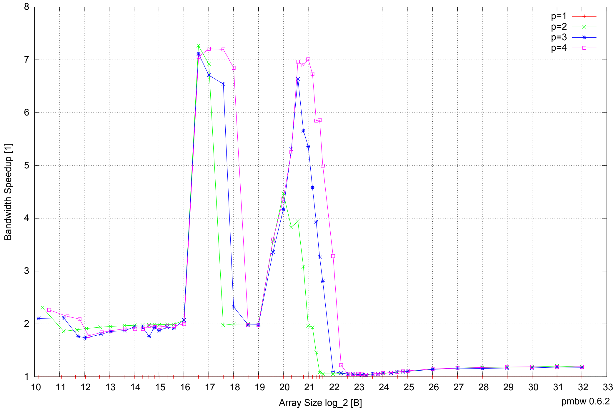
AMD Dual-Core Opteron 270 8GB - Speedup of Parallel Memory Bandwidth - ScanWrite64IndexUnrollLoop
