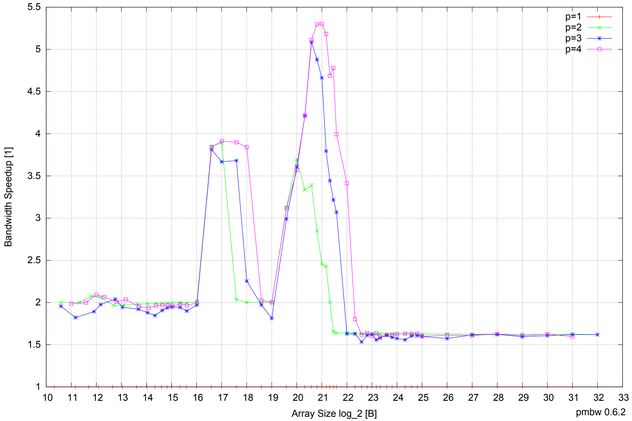
AMD Dual-Core Opteron 270 8GB - Speedup of Parallel Memory Bandwidth - ScanRead128PtrUnrollLoop
