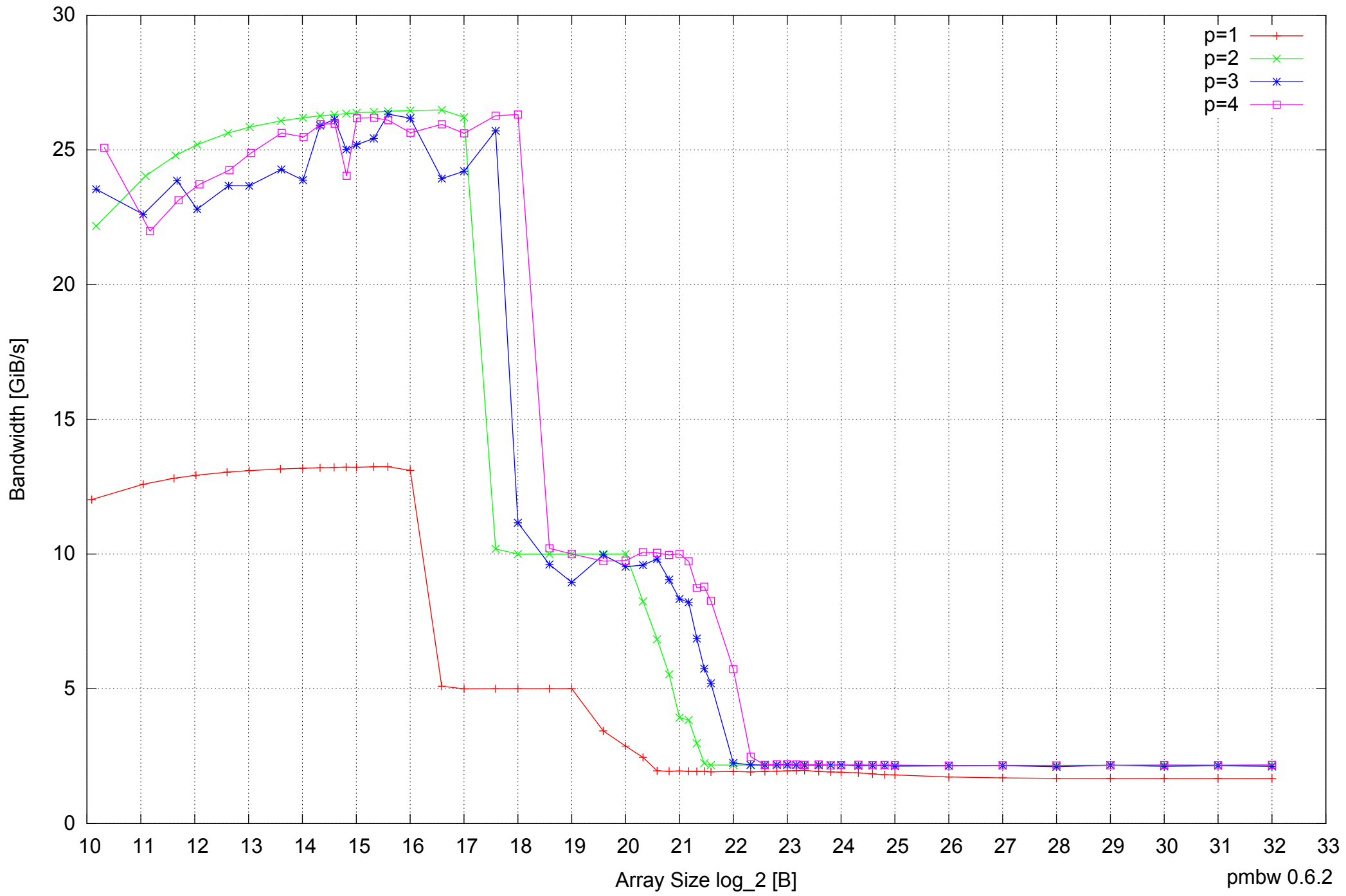
AMD Dual-Core Opteron 270 8GB - Parallel Memory Bandwidth - ScanWrite32PtrUnrollLoop
