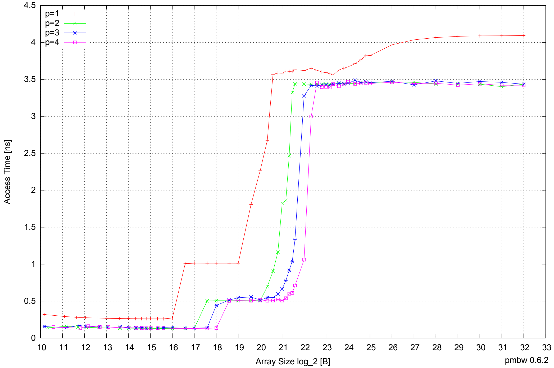
AMD Dual-Core Opteron 270 8GB - Parallel Memory Access Time - ScanWrite64PtrUnrollLoop
