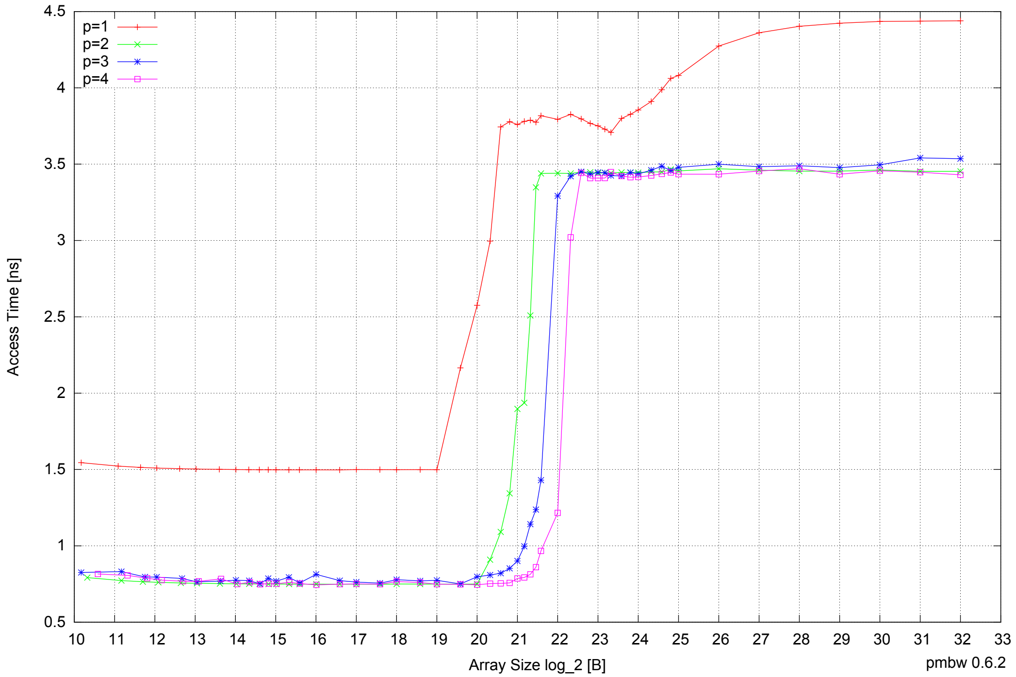
AMD Dual-Core Opteron 270 8GB - Parallel Memory Access Time - ScanWrite64IndexSimpleLoop
