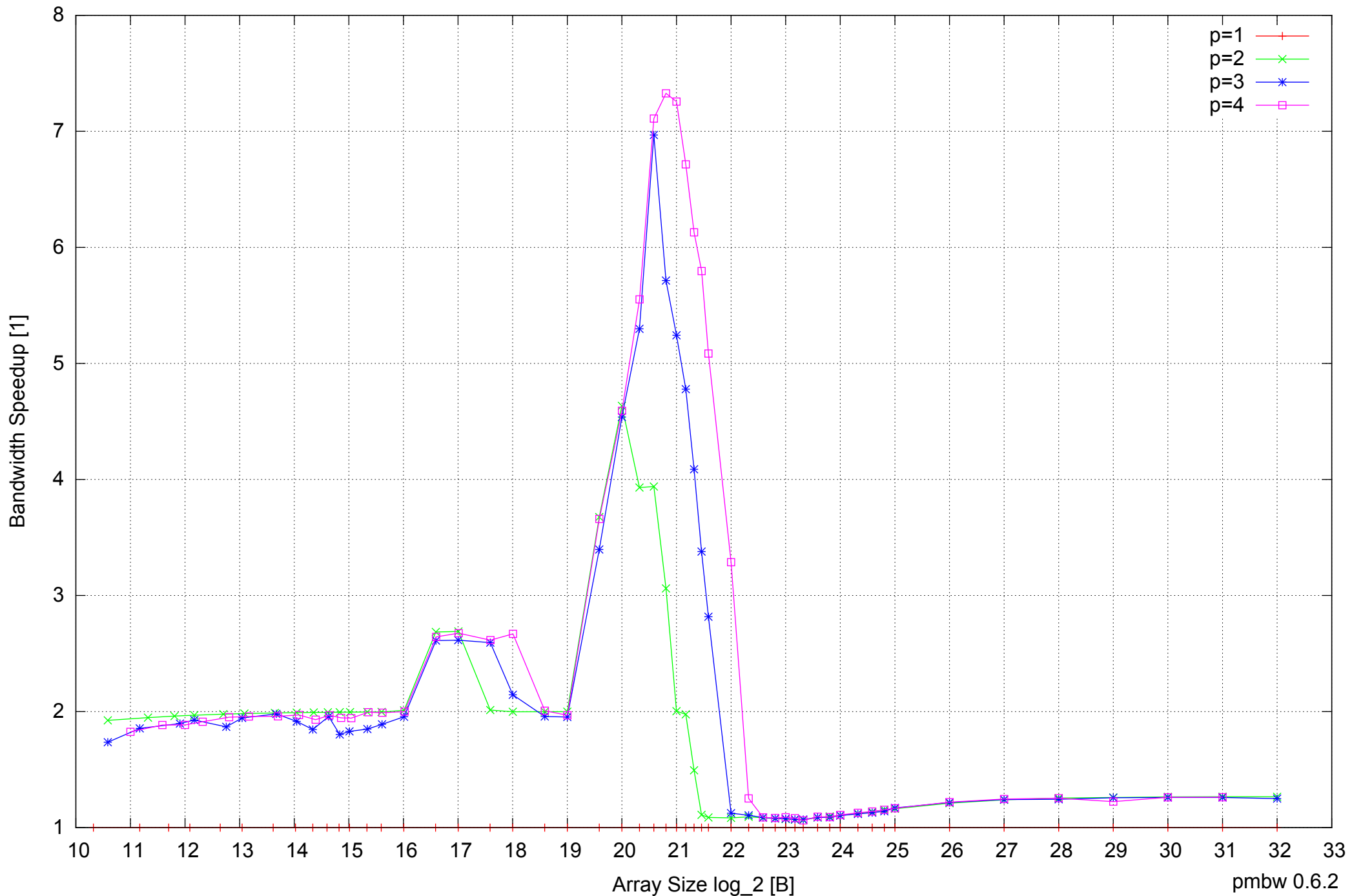
AMD Dual-Core Opteron 270 8GB - Speedup of Parallel Memory Bandwidth - ScanWrite128PtrSimpleLoop
