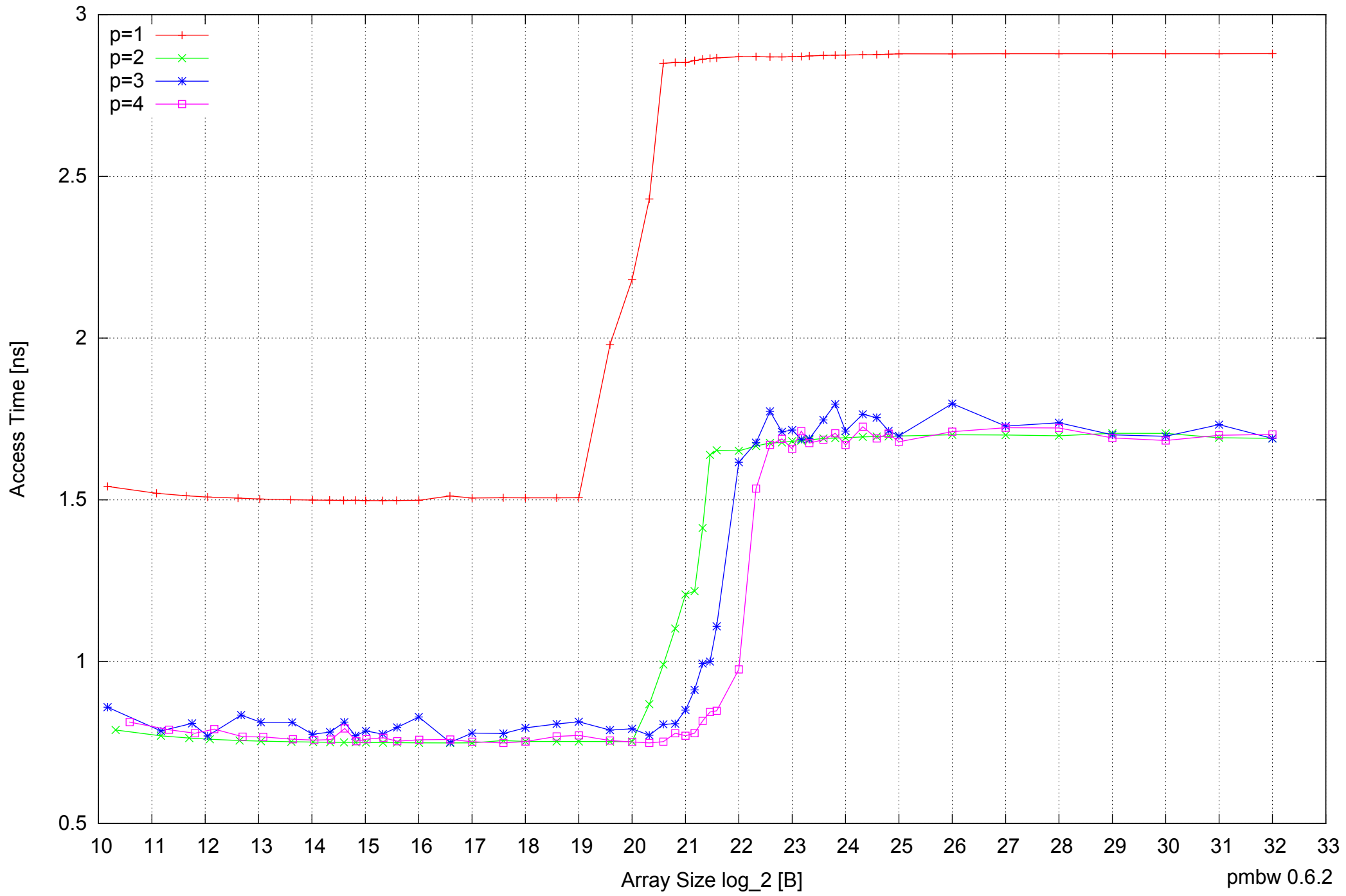
AMD Dual-Core Opteron 270 8GB - Parallel Memory Access Time - ScanRead64PtrSimpleLoop
