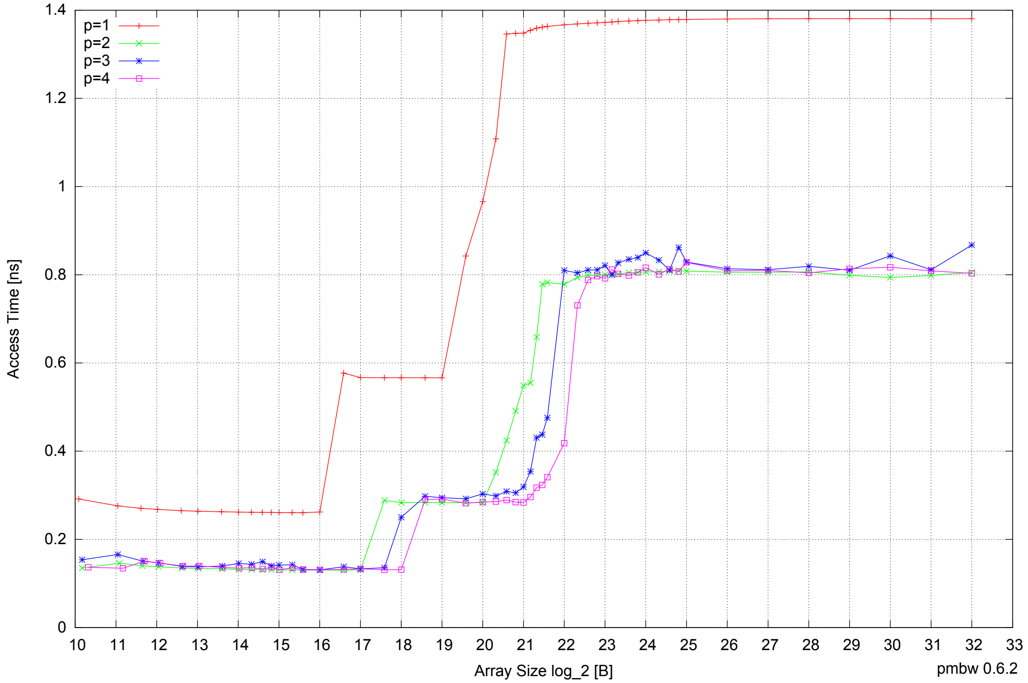
AMD Dual-Core Opteron 270 8GB - Parallel Memory Access Time - ScanRead32PtrUnrollLoop
