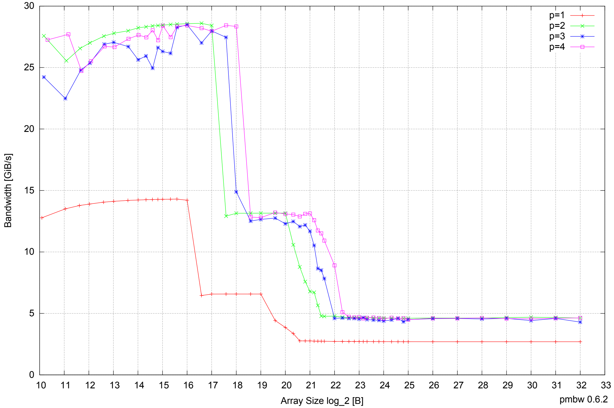
AMD Dual-Core Opteron 270 8GB - Parallel Memory Bandwidth - ScanRead32PtrUnrollLoop
