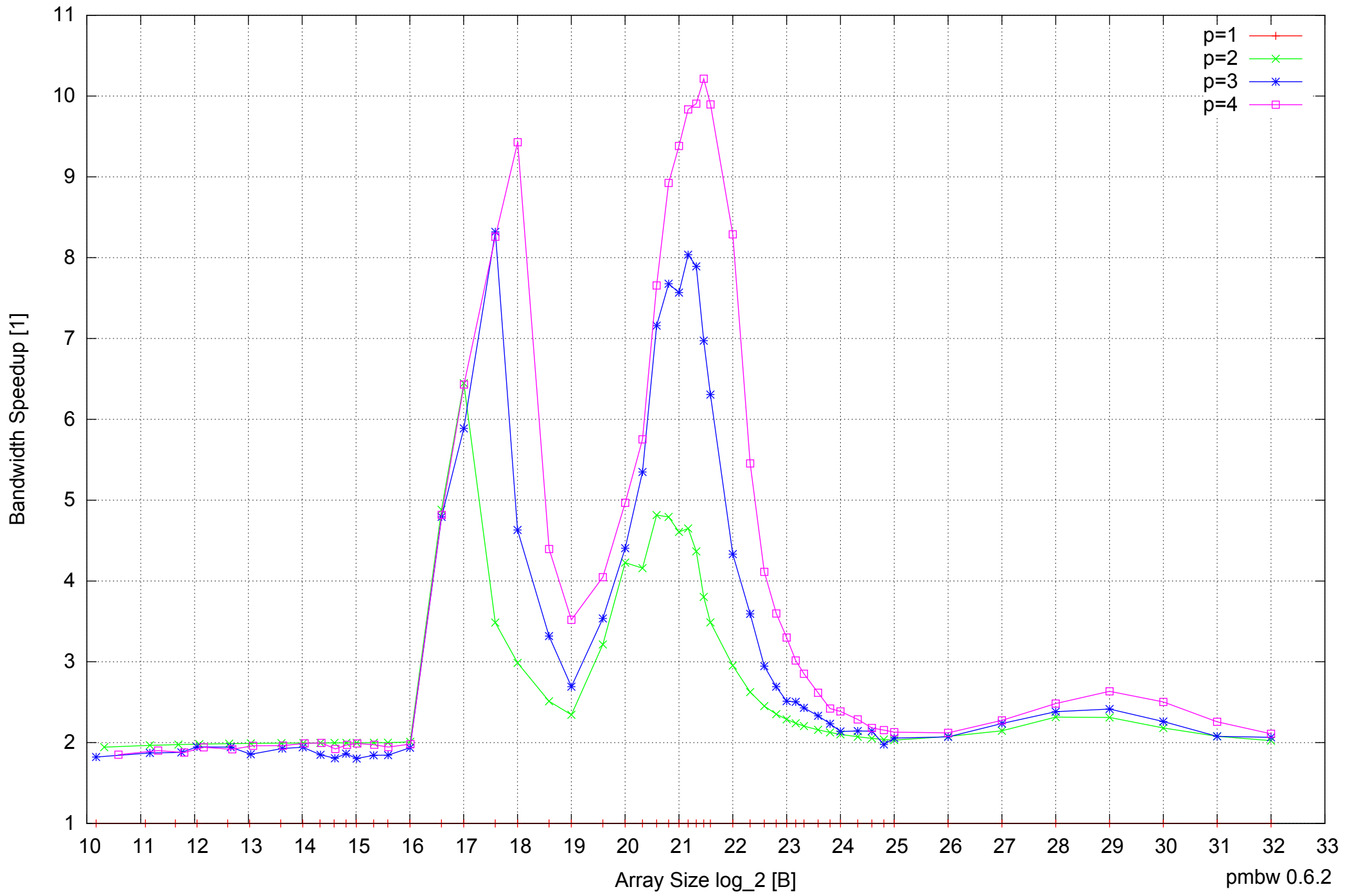
AMD Dual-Core Opteron 270 8GB - Speedup of Parallel Memory Bandwidth - PermRead64SimpleLoop
