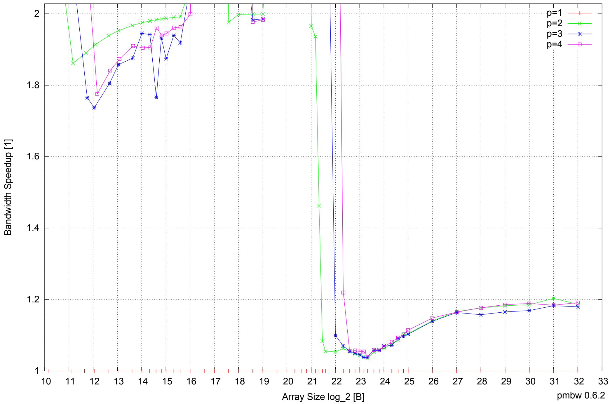
AMD Dual-Core Opteron 270 8GB - Speedup of Parallel Memory Bandwidth (enlarged) - ScanWrite64IndexUnrollLoop
