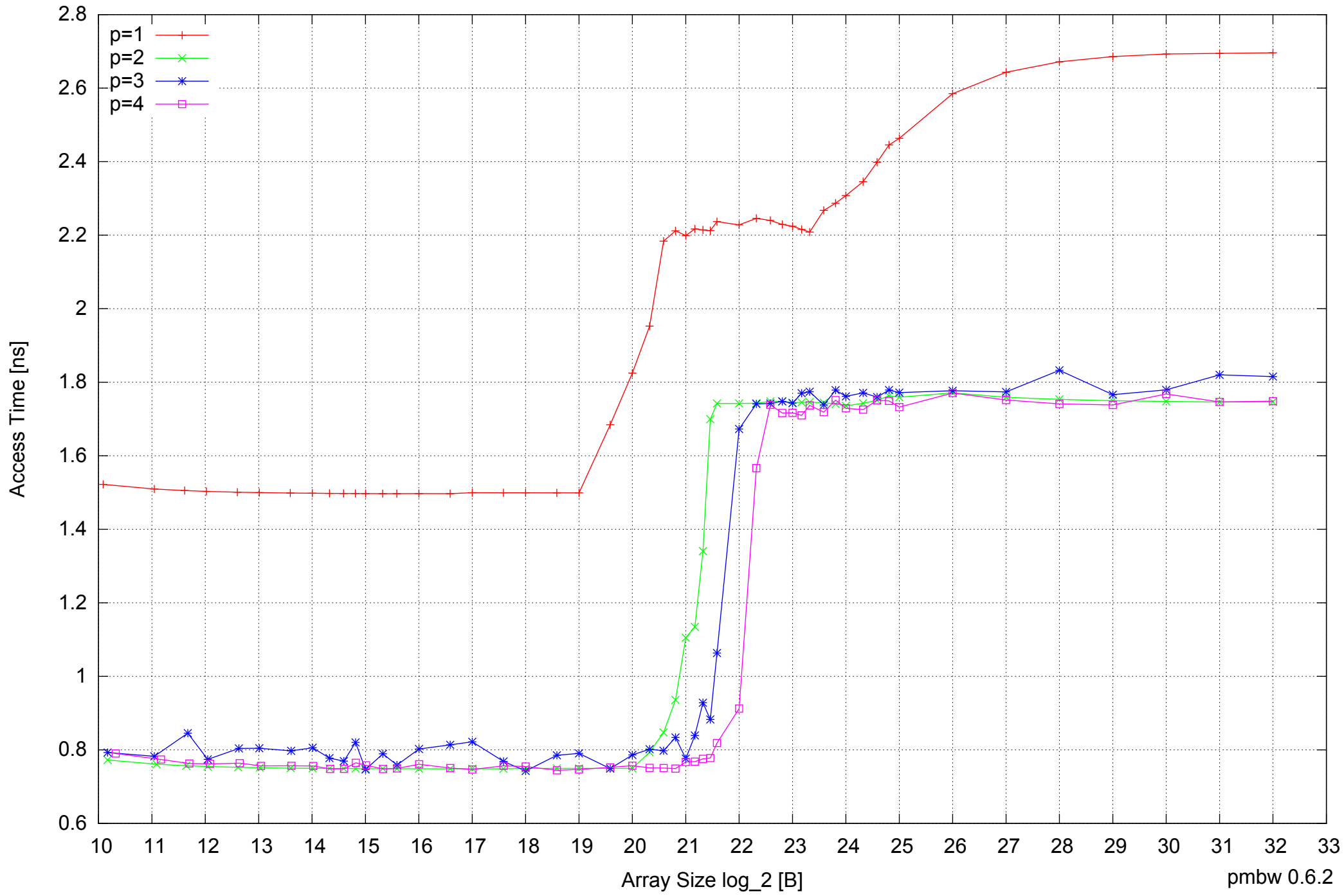
AMD Dual-Core Opteron 270 8GB - Parallel Memory Access Time - ScanWrite32PtrSimpleLoop
