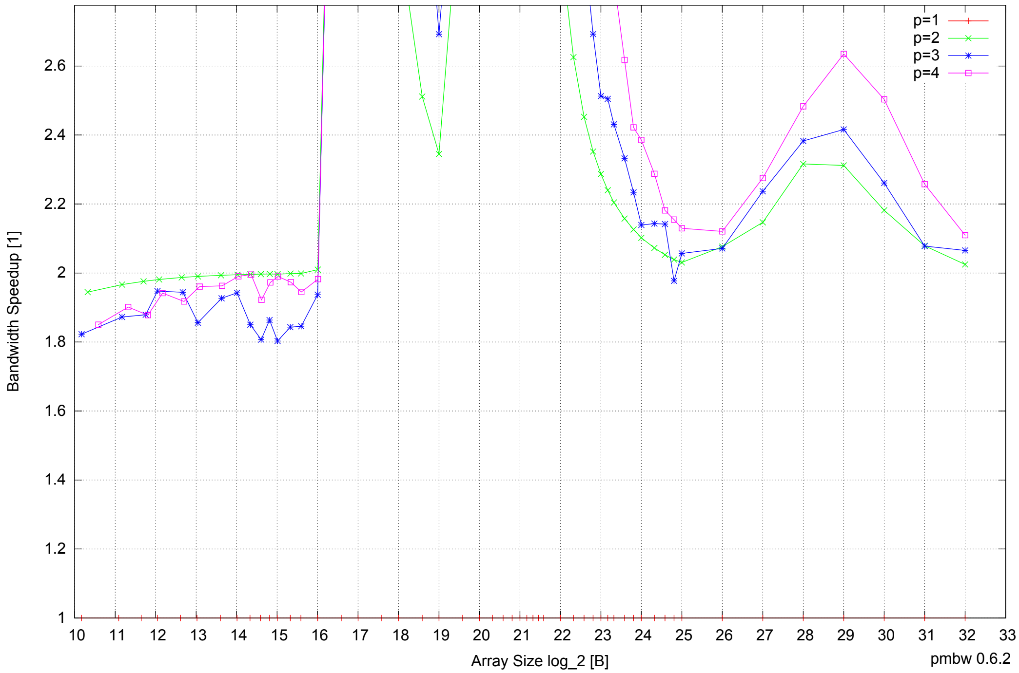
AMD Dual-Core Opteron 270 8GB - Speedup of Parallel Memory Bandwidth (enlarged) - PermRead64SimpleLoop
