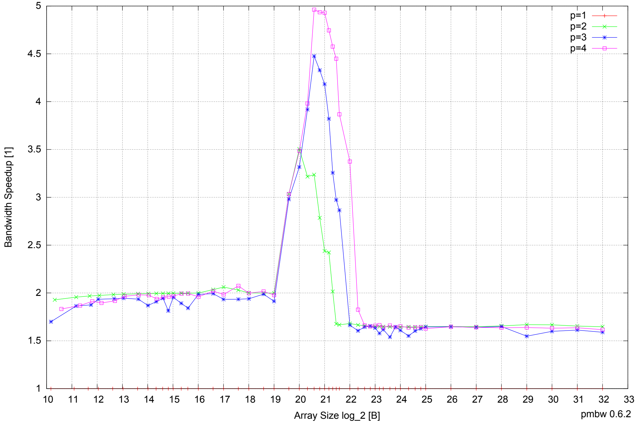
AMD Dual-Core Opteron 270 8GB - Speedup of Parallel Memory Bandwidth - ScanRead64IndexSimpleLoop
