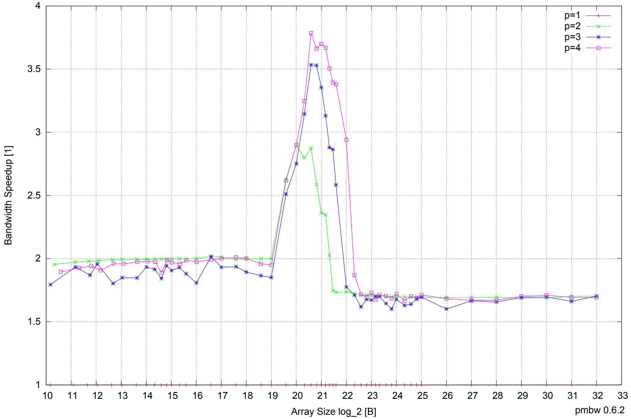
AMD Dual-Core Opteron 270 8GB - Speedup of Parallel Memory Bandwidth - ScanRead64PtrSimpleLoop
