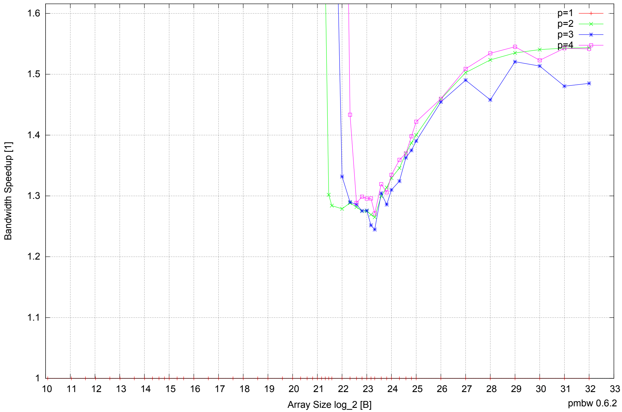
AMD Dual-Core Opteron 270 8GB - Speedup of Parallel Memory Bandwidth (enlarged) - ScanWrite32PtrSimpleLoop
