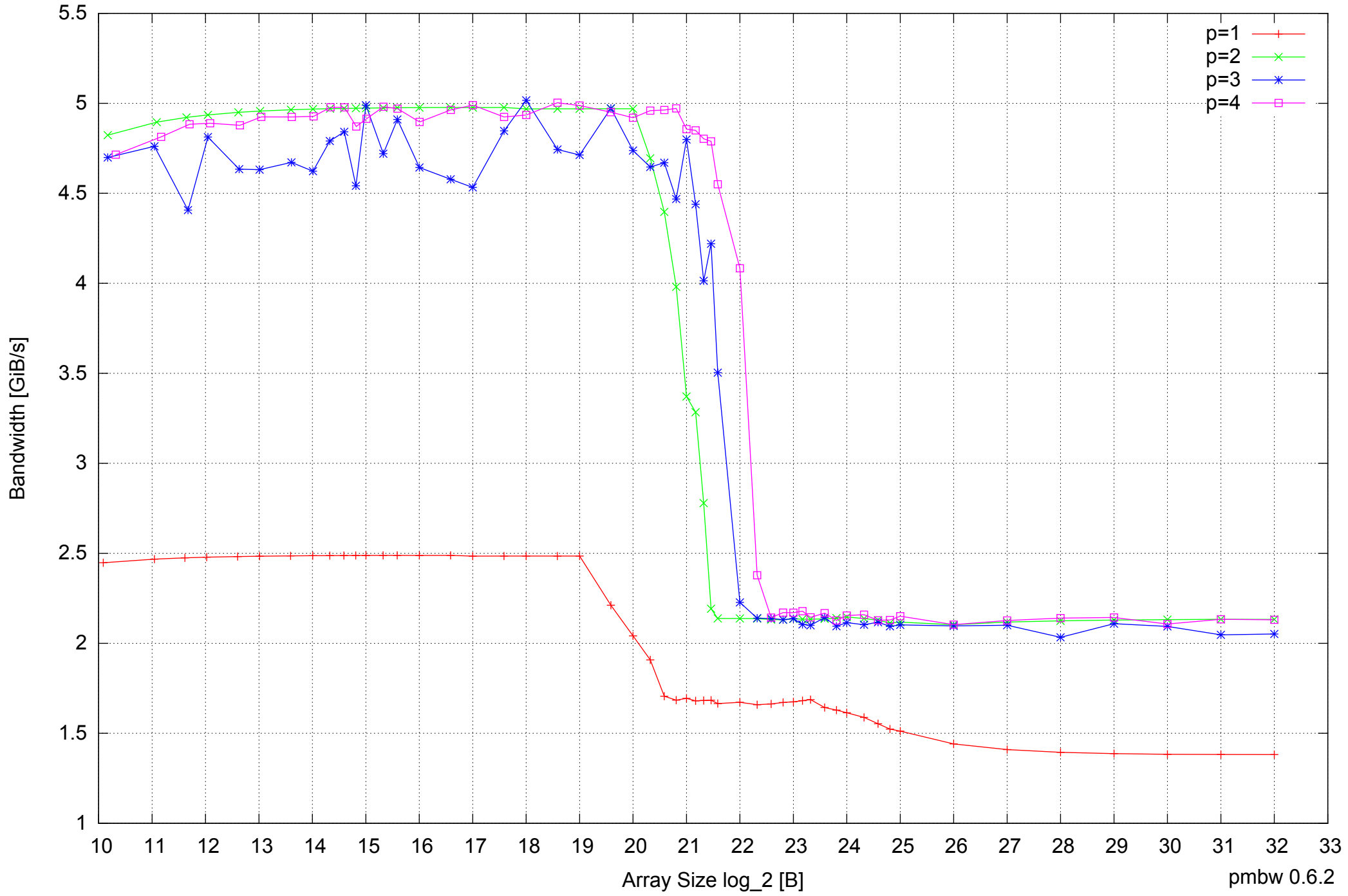
AMD Dual-Core Opteron 270 8GB - Parallel Memory Bandwidth - ScanWrite32PtrSimpleLoop
