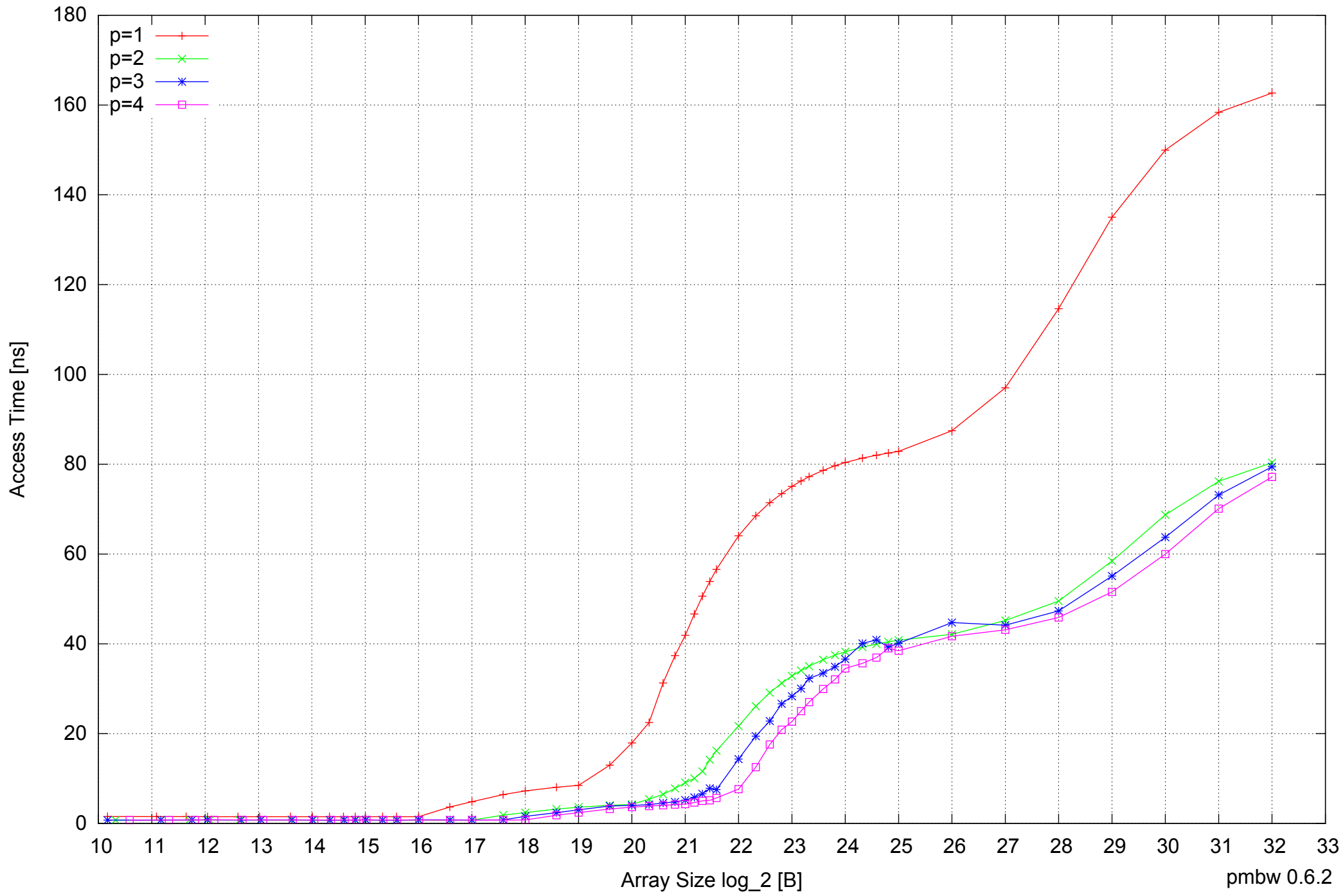
AMD Dual-Core Opteron 270 8GB - Parallel Memory Access Time - PermRead64UnrollLoop
