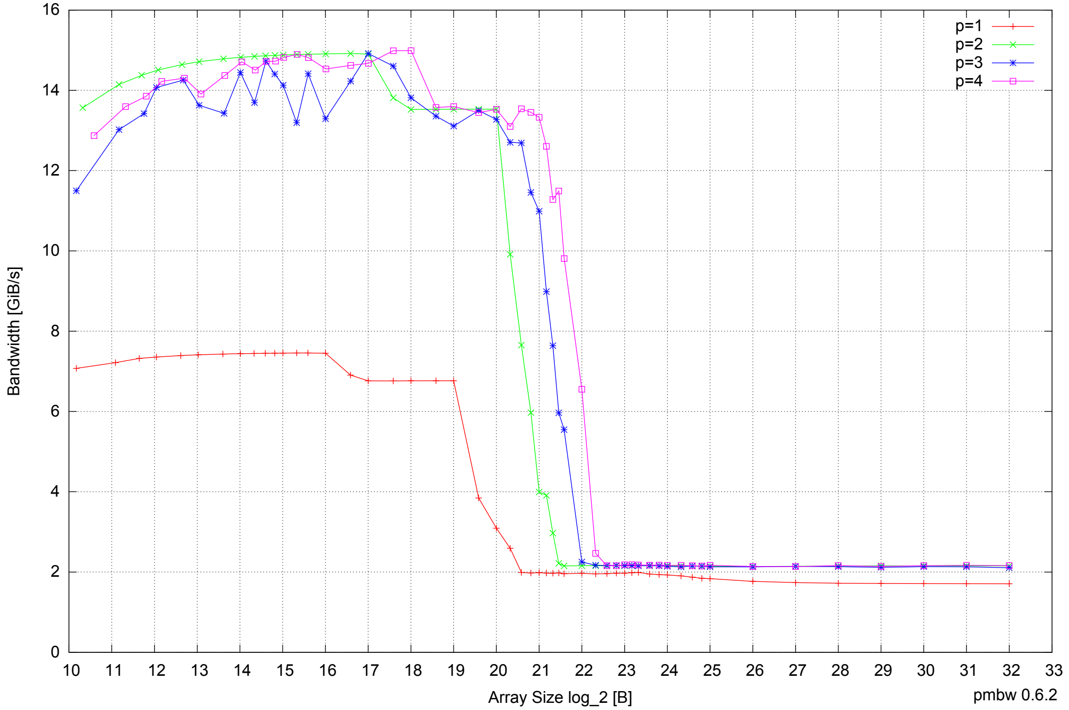
AMD Dual-Core Opteron 270 8GB - Parallel Memory Bandwidth - ScanWrite64PtrSimpleLoop
