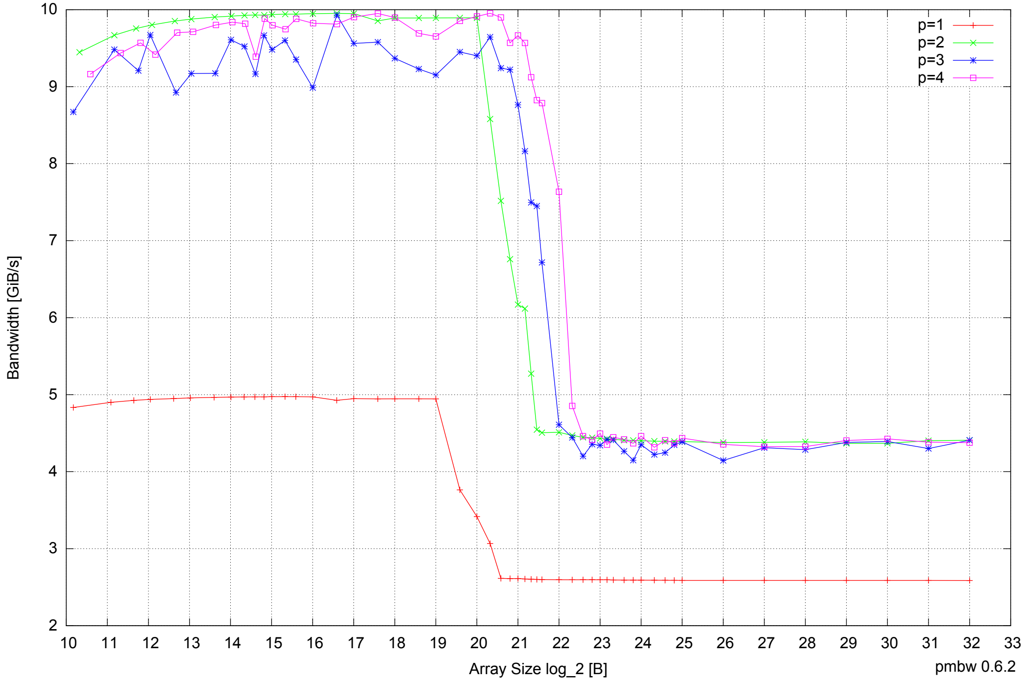
AMD Dual-Core Opteron 270 8GB - Parallel Memory Bandwidth - ScanRead64PtrSimpleLoop
