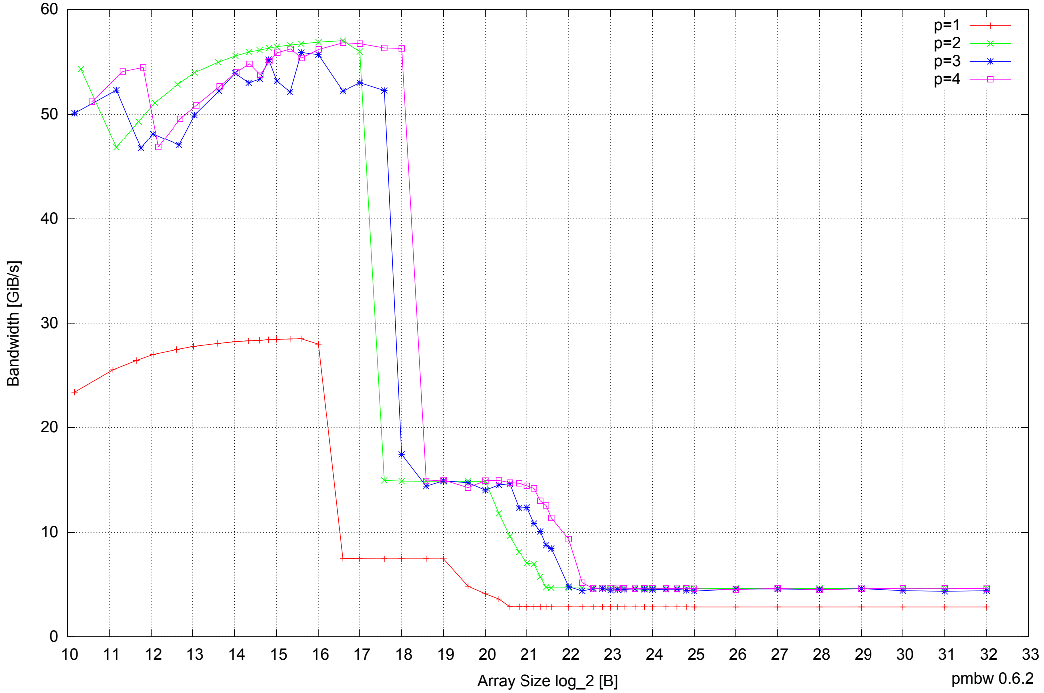
AMD Dual-Core Opteron 270 8GB - Parallel Memory Bandwidth - ScanRead64IndexUnrollLoop
