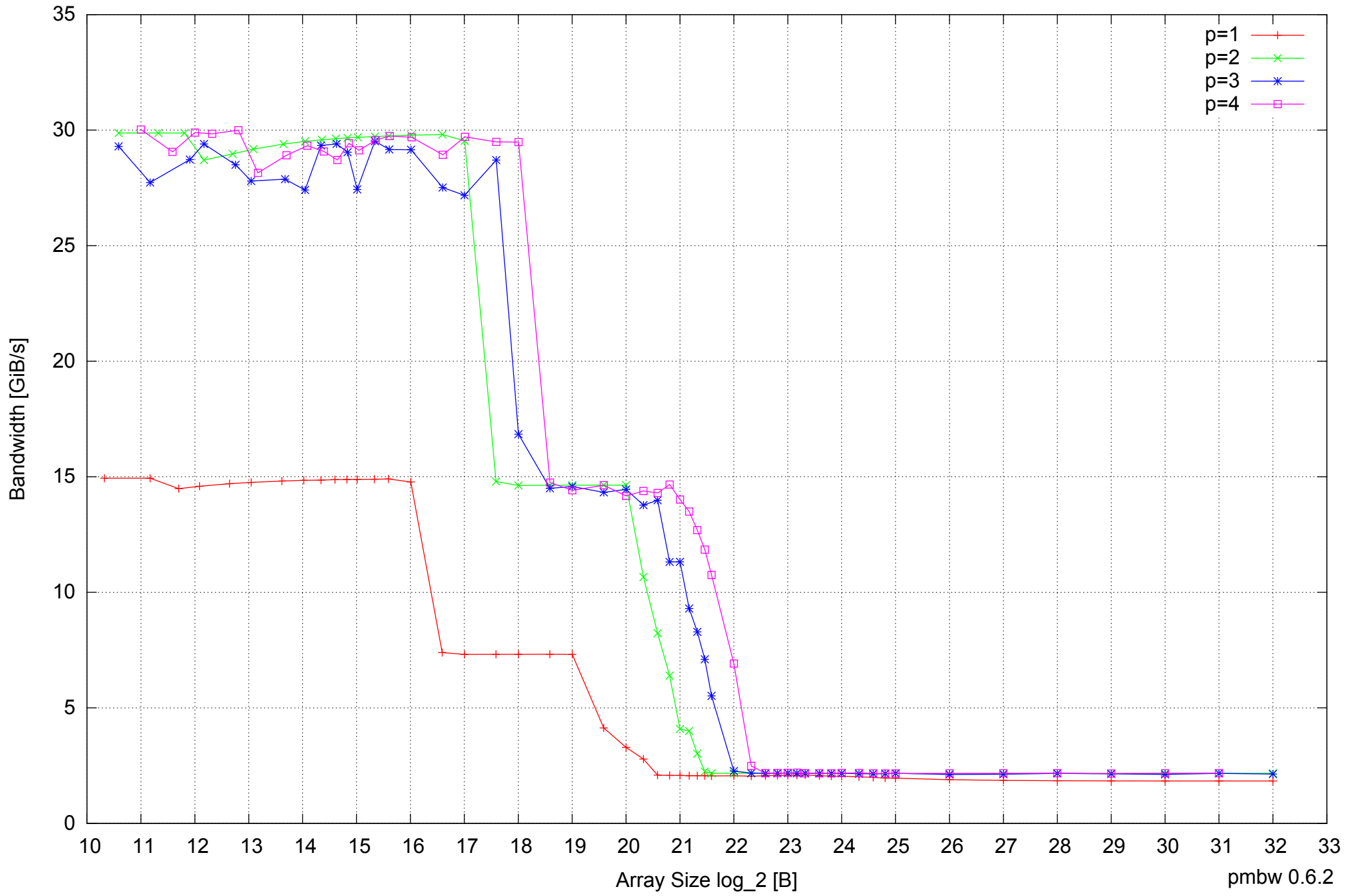
AMD Dual-Core Opteron 270 8GB - Parallel Memory Bandwidth - ScanWrite128PtrUnrollLoop
