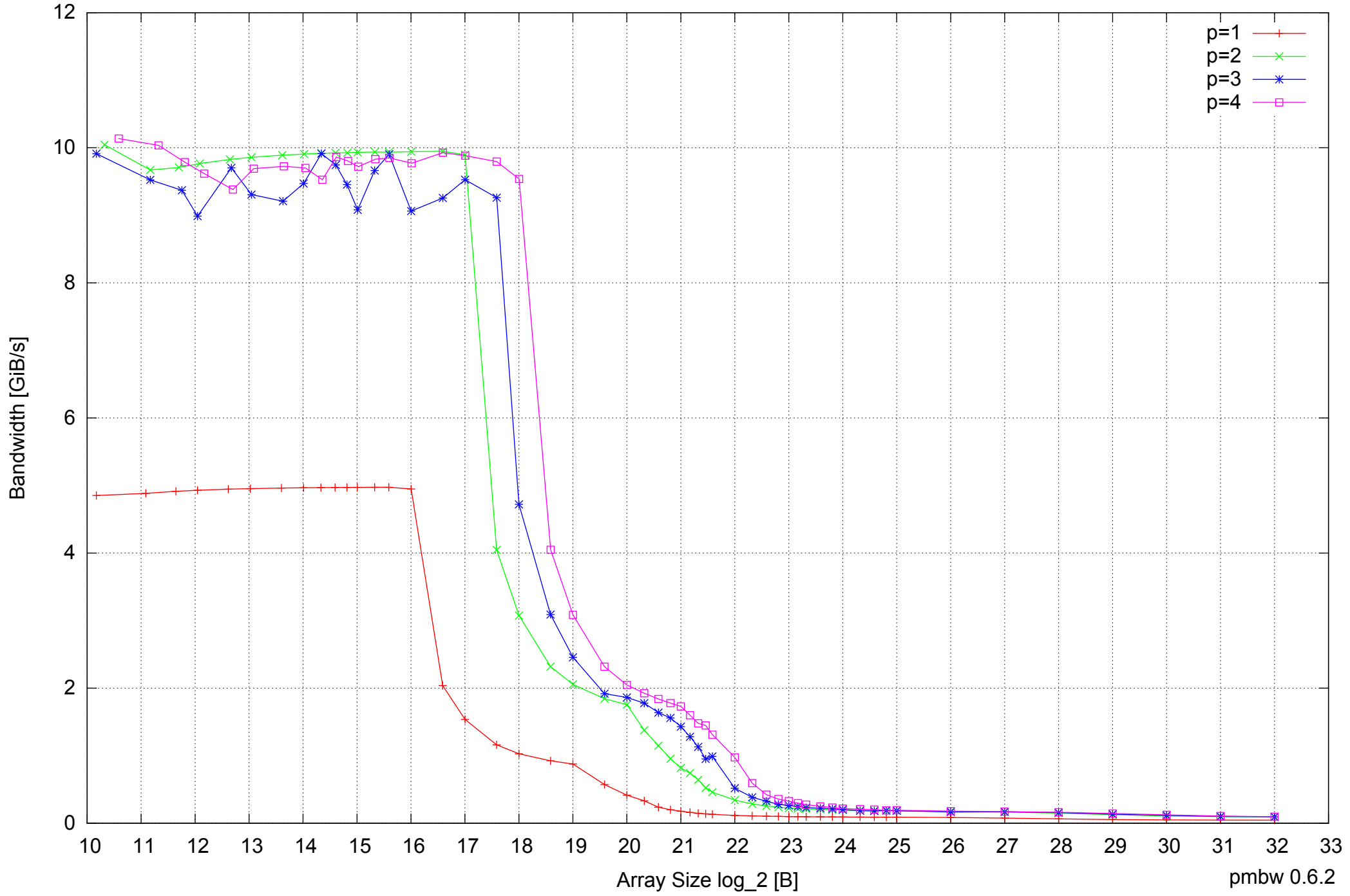
AMD Dual-Core Opteron 270 8GB - Parallel Memory Bandwidth - PermRead64UnrollLoop
