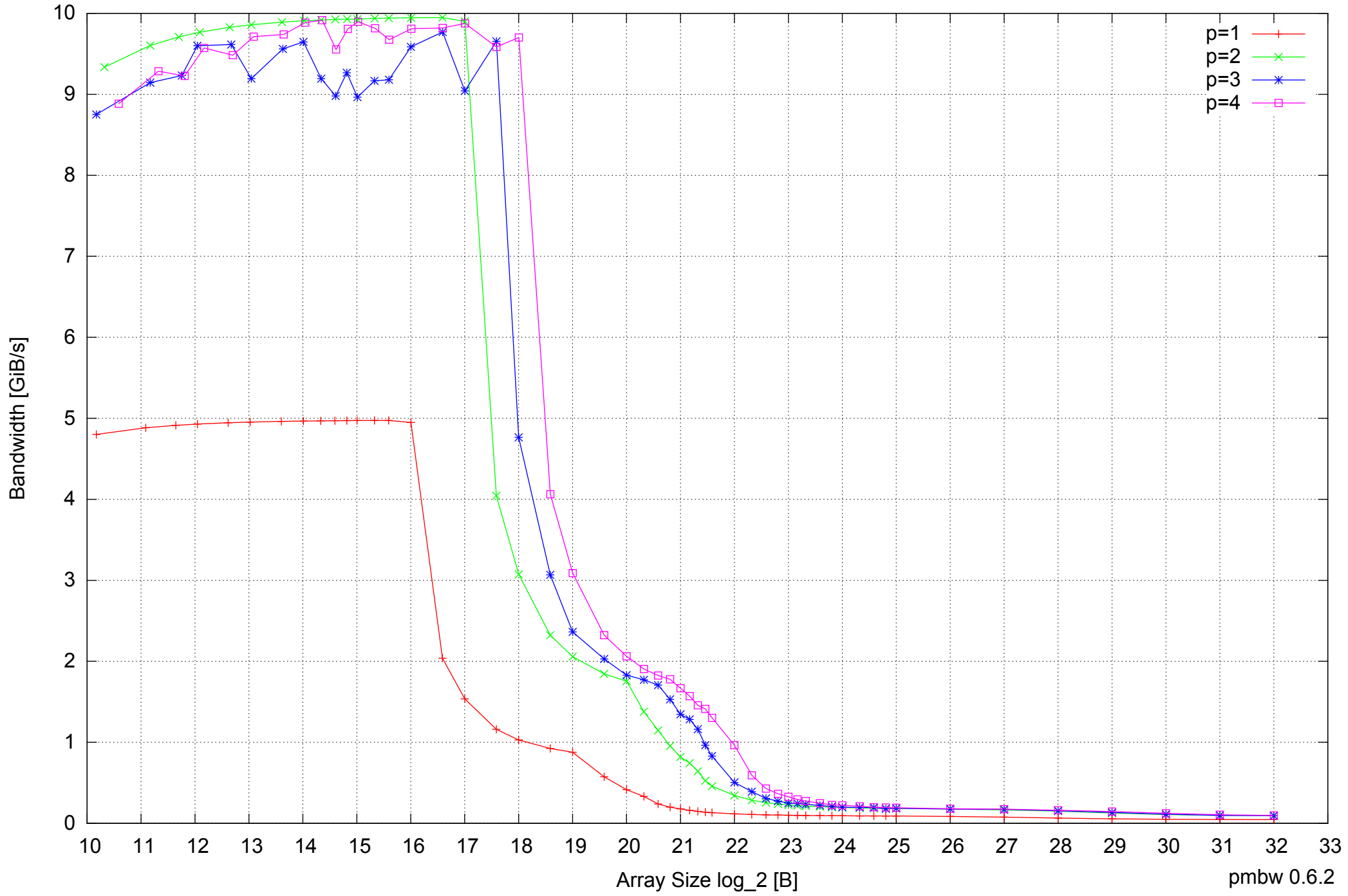
AMD Dual-Core Opteron 270 8GB - Parallel Memory Bandwidth - PermRead64SimpleLoop
