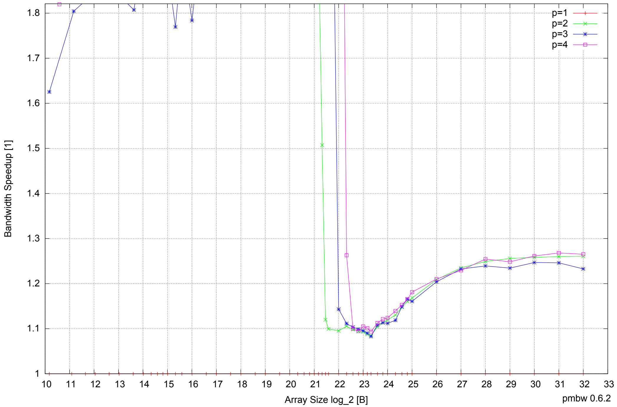
AMD Dual-Core Opteron 270 8GB - Speedup of Parallel Memory Bandwidth (enlarged) - ScanWrite64PtrSimpleLoop
