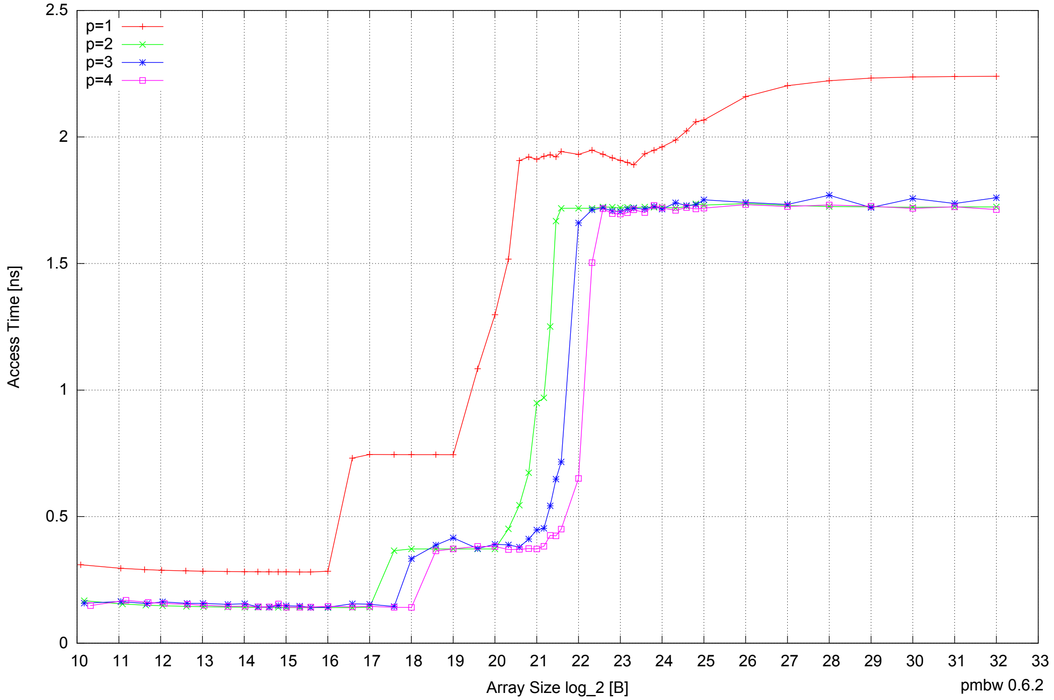
AMD Dual-Core Opteron 270 8GB - Parallel Memory Access Time - ScanWrite32PtrUnrollLoop
