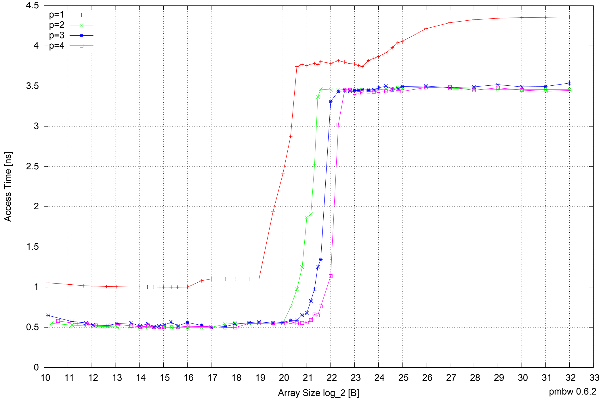
AMD Dual-Core Opteron 270 8GB - Parallel Memory Access Time - ScanWrite64PtrSimpleLoop
