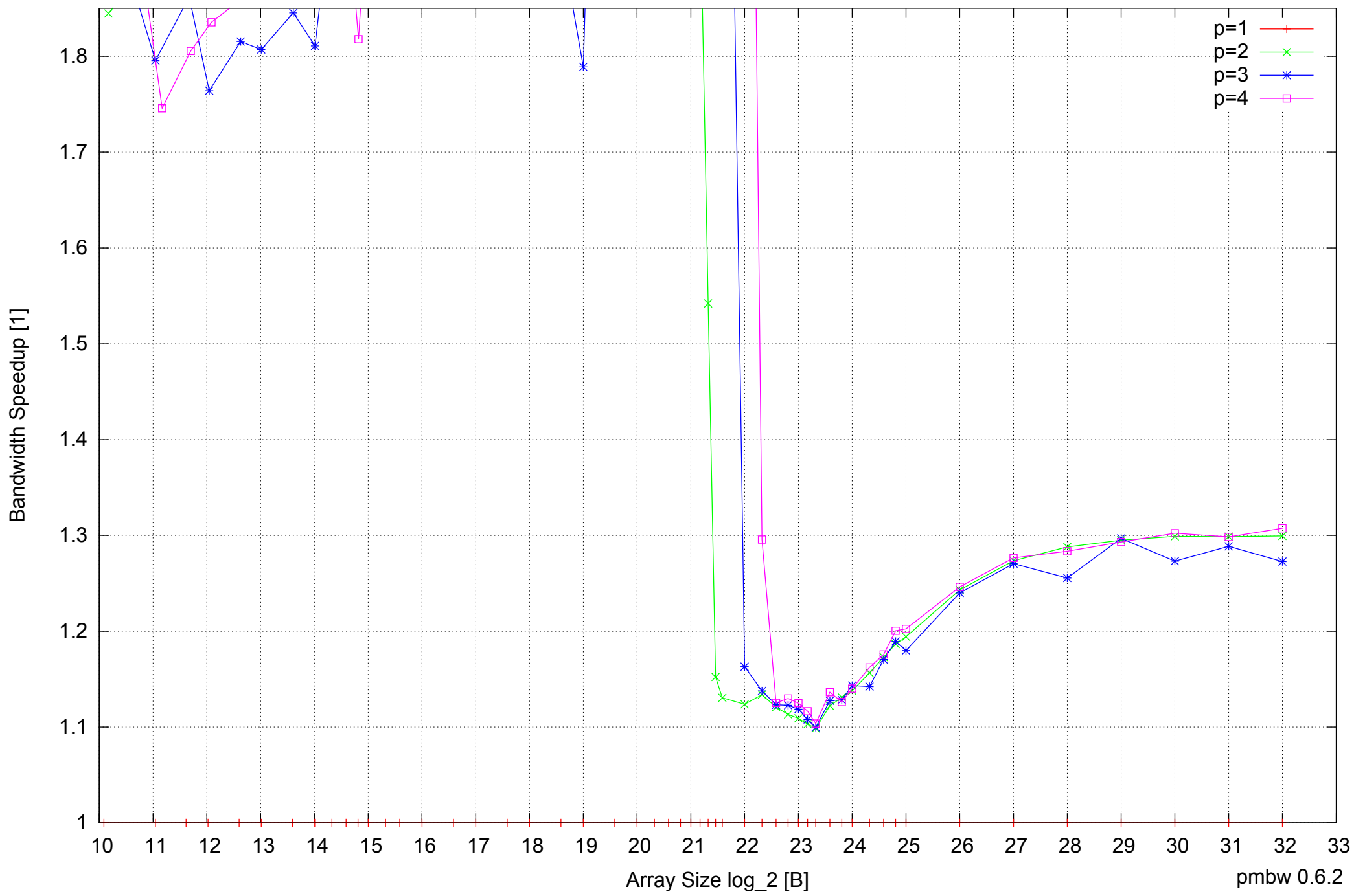
AMD Dual-Core Opteron 270 8GB - Speedup of Parallel Memory Bandwidth (enlarged) - ScanWrite32PtrUnrollLoop
