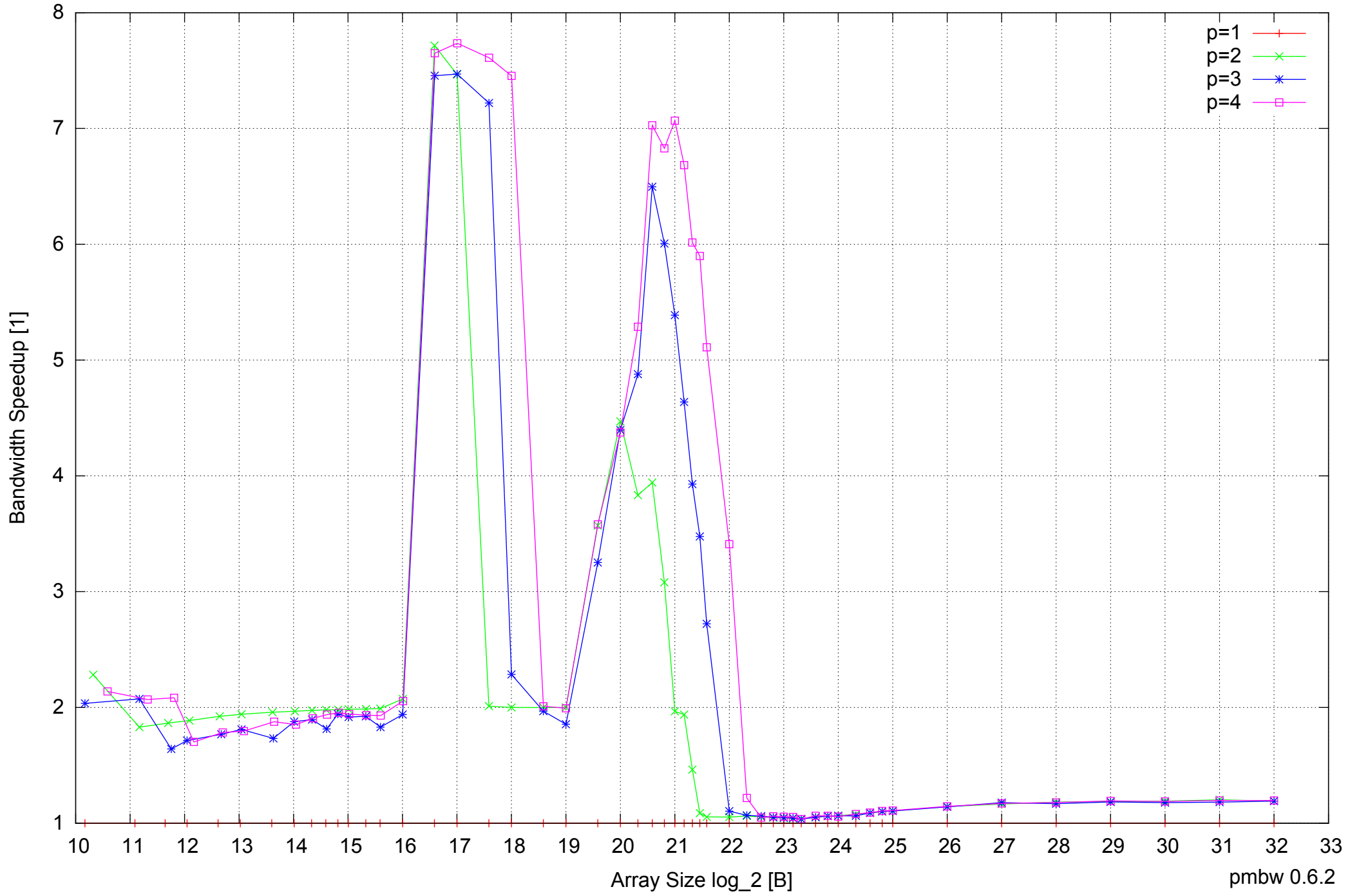
AMD Dual-Core Opteron 270 8GB - Speedup of Parallel Memory Bandwidth - ScanWrite64PtrUnrollLoop
