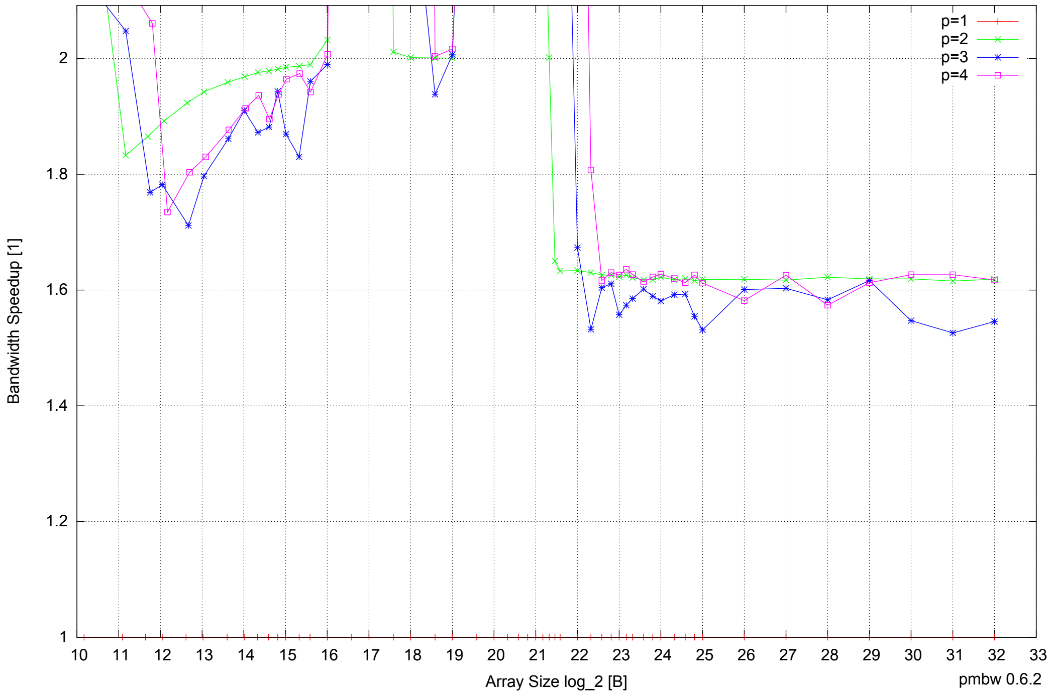
AMD Dual-Core Opteron 270 8GB - Speedup of Parallel Memory Bandwidth (enlarged) - ScanRead64IndexUnrollLoop
