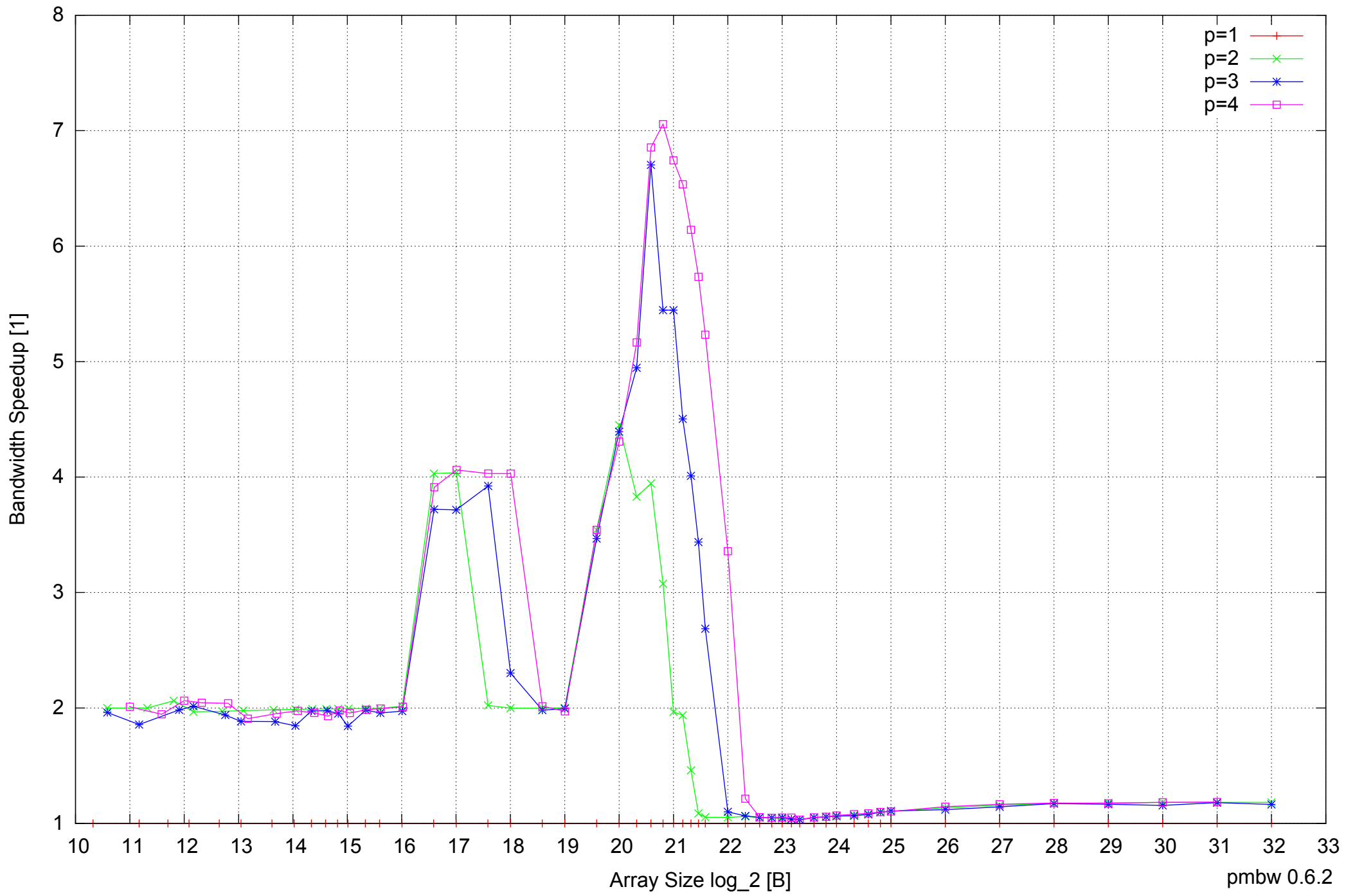
AMD Dual-Core Opteron 270 8GB - Speedup of Parallel Memory Bandwidth - ScanWrite128PtrUnrollLoop
