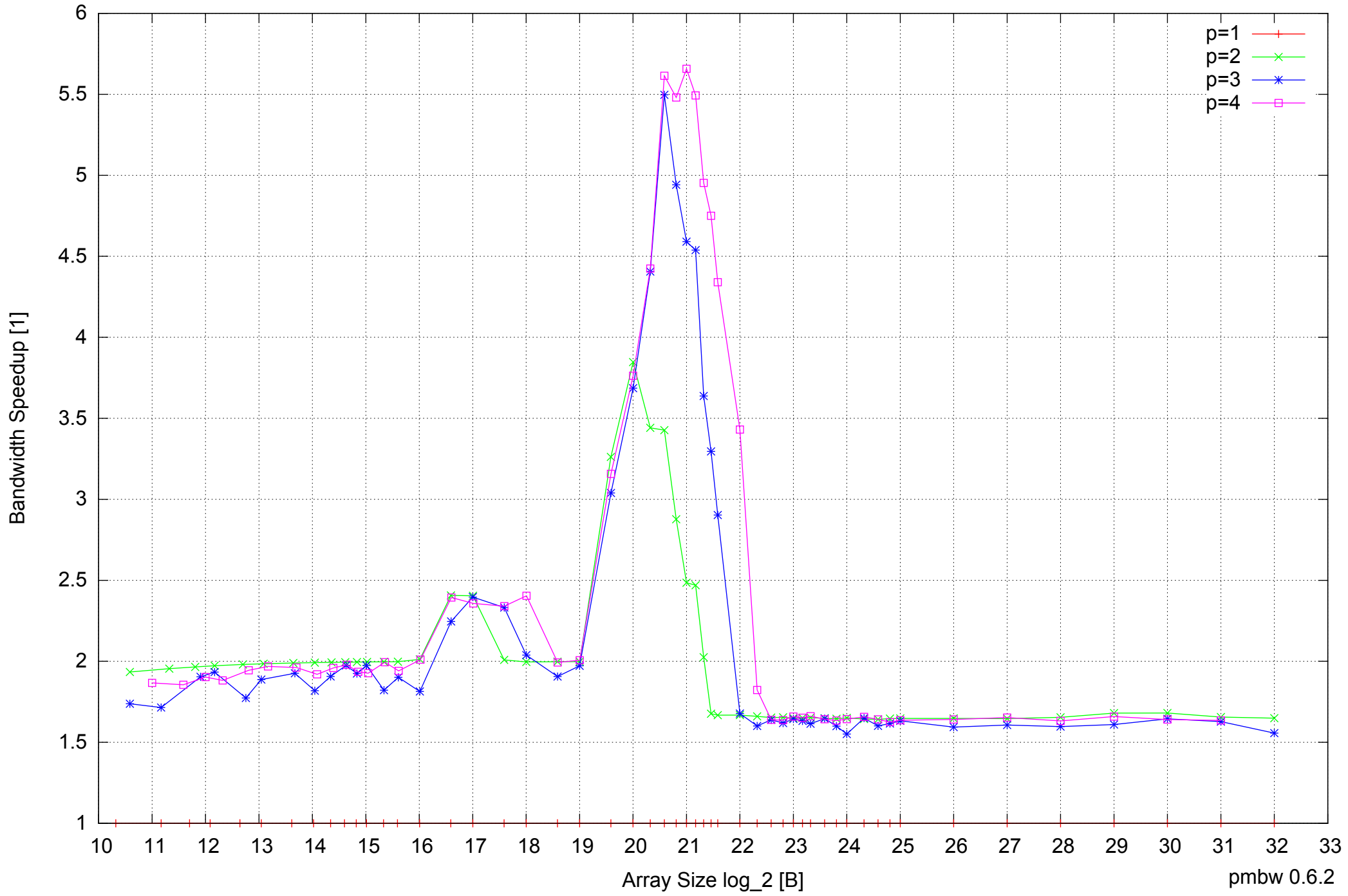
AMD Dual-Core Opteron 270 8GB - Speedup of Parallel Memory Bandwidth - ScanRead128PtrSimpleLoop
