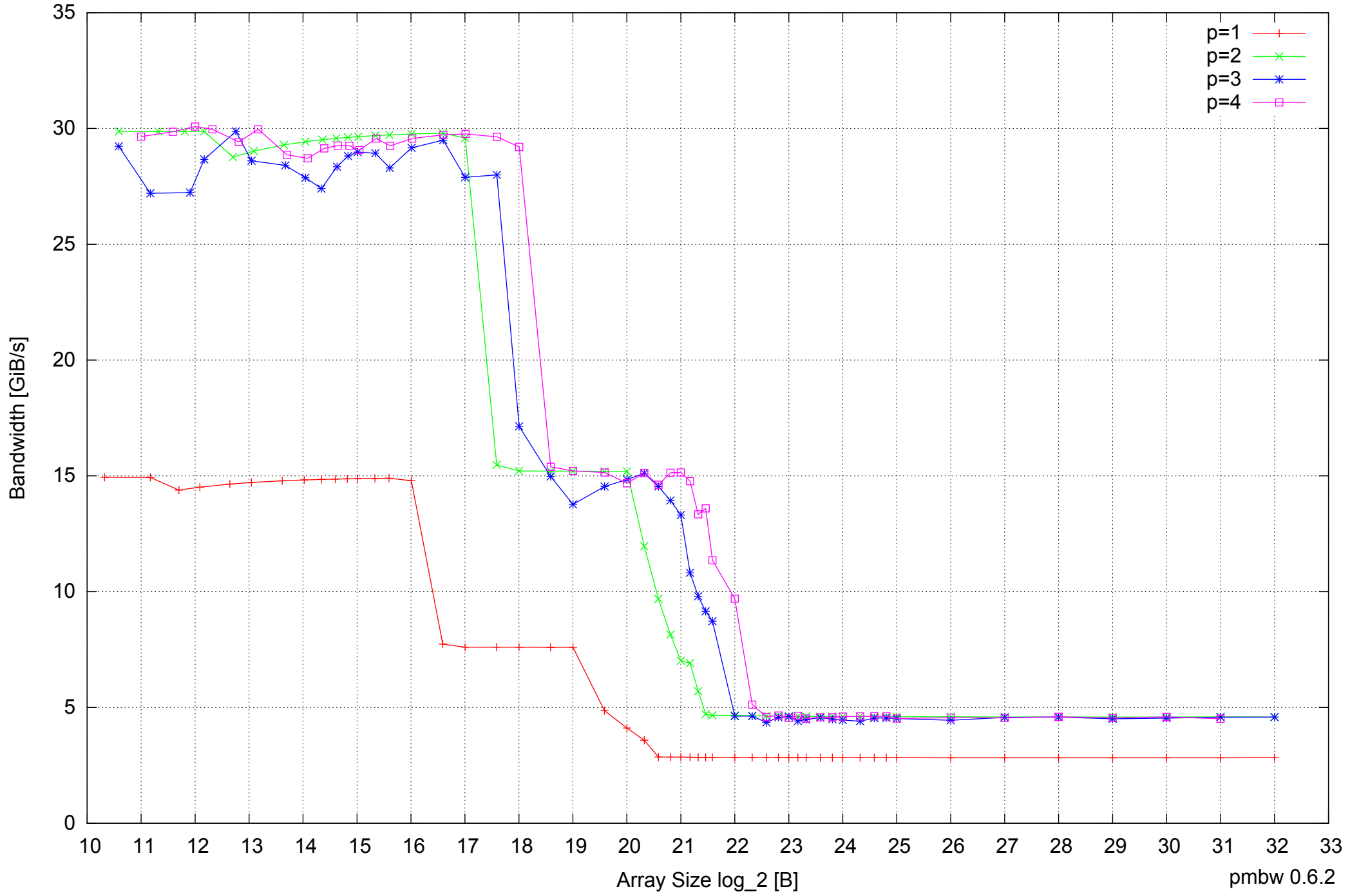
AMD Dual-Core Opteron 270 8GB - Parallel Memory Bandwidth - ScanRead128PtrUnrollLoop
