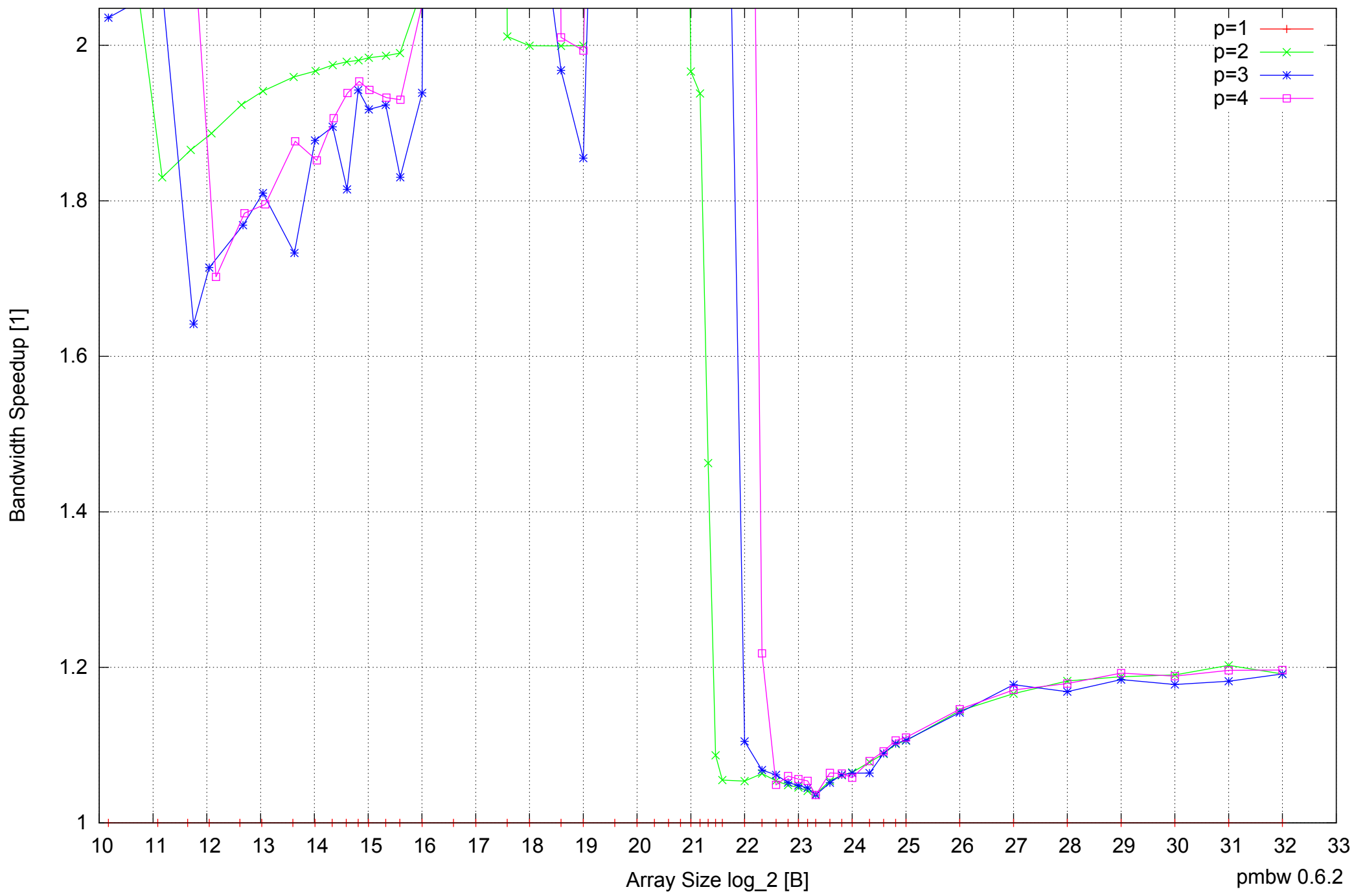
AMD Dual-Core Opteron 270 8GB - Speedup of Parallel Memory Bandwidth (enlarged) - ScanWrite64PtrUnrollLoop
