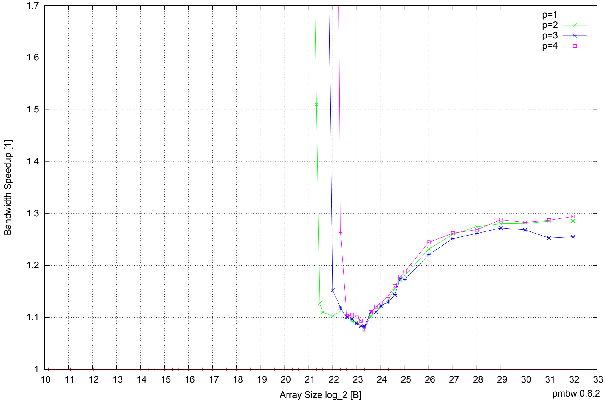
AMD Dual-Core Opteron 270 8GB - Speedup of Parallel Memory Bandwidth (enlarged) - ScanWrite64IndexSimpleLoop
