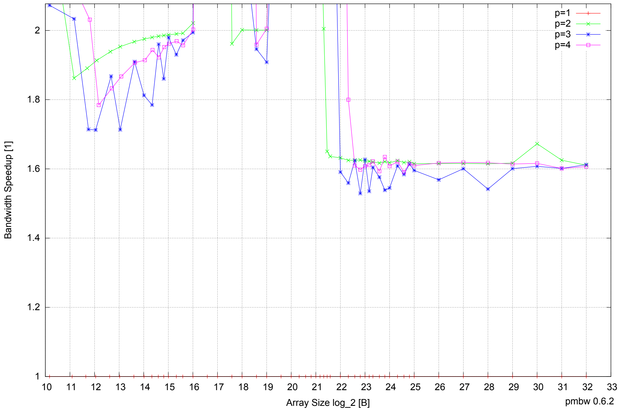
AMD Dual-Core Opteron 270 8GB - Speedup of Parallel Memory Bandwidth (enlarged) - ScanRead64PtrUnrollLoop
