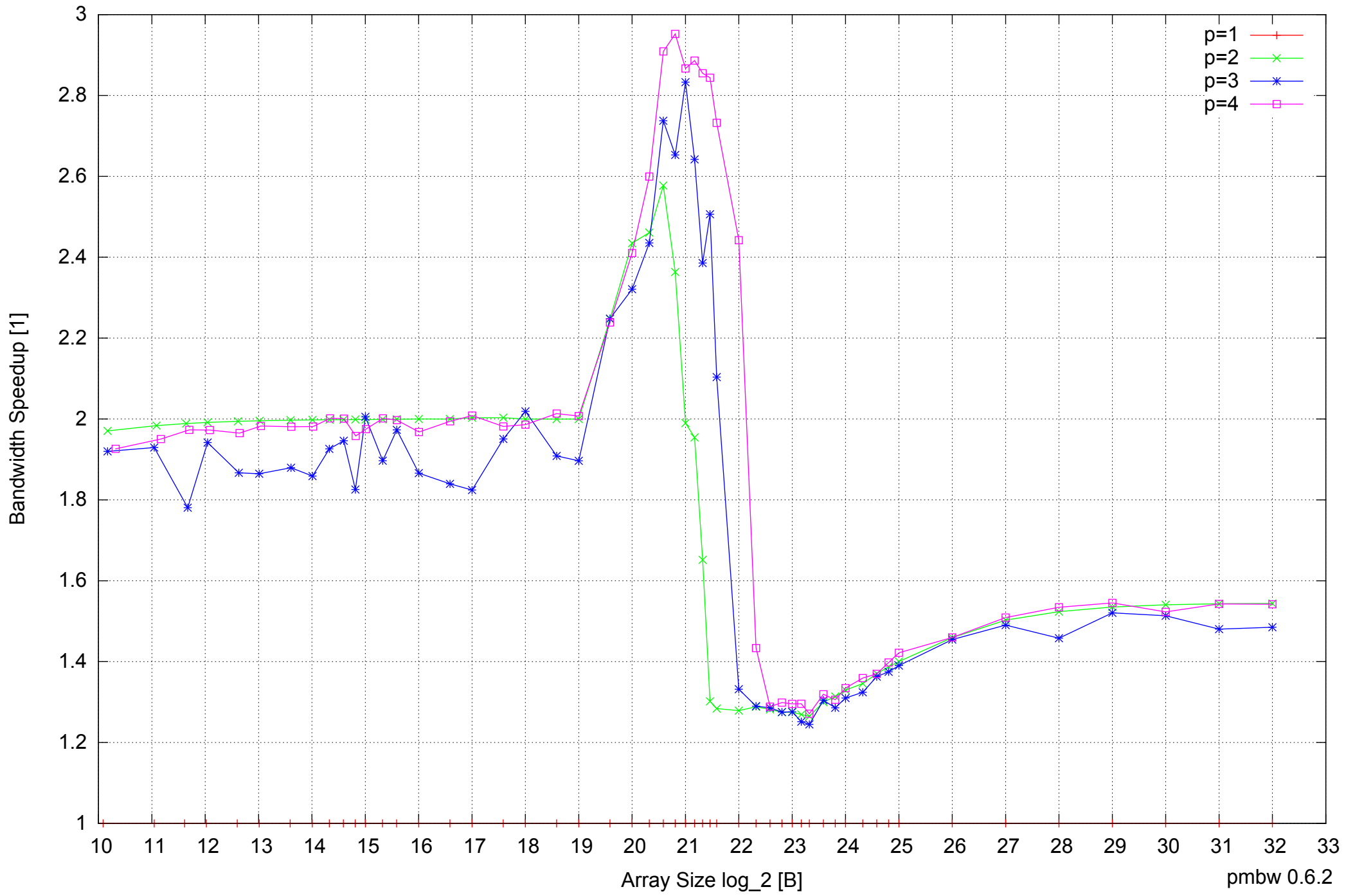
AMD Dual-Core Opteron 270 8GB - Speedup of Parallel Memory Bandwidth - ScanWrite32PtrSimpleLoop
