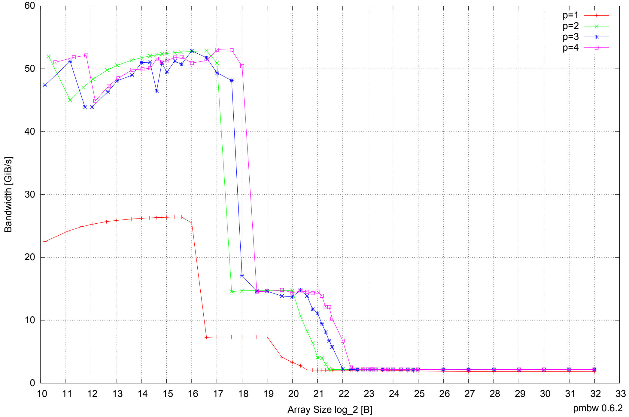
AMD Dual-Core Opteron 270 8GB - Parallel Memory Bandwidth - ScanWrite64IndexUnrollLoop
