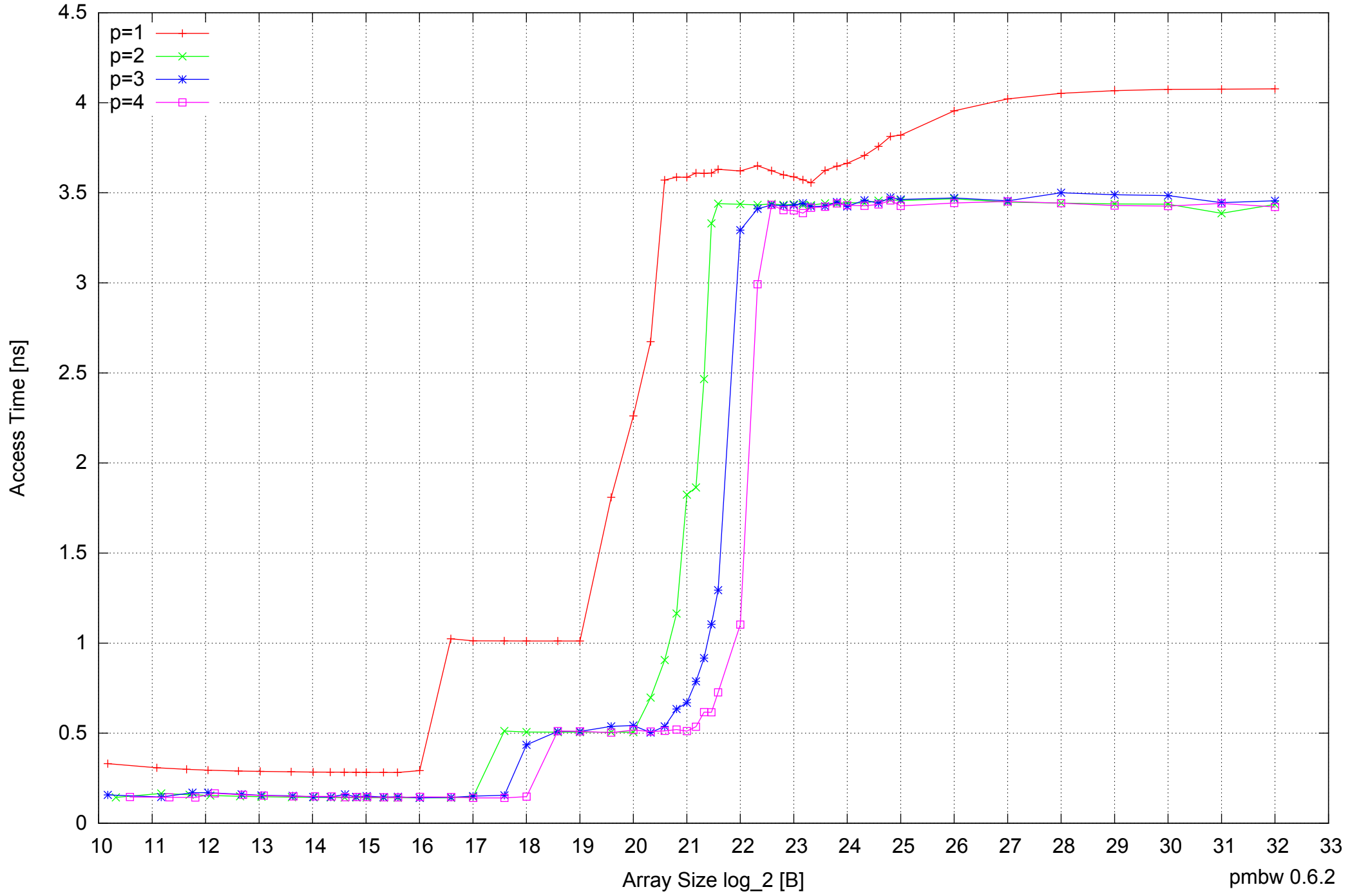
AMD Dual-Core Opteron 270 8GB - Parallel Memory Access Time - ScanWrite64IndexUnrollLoop
