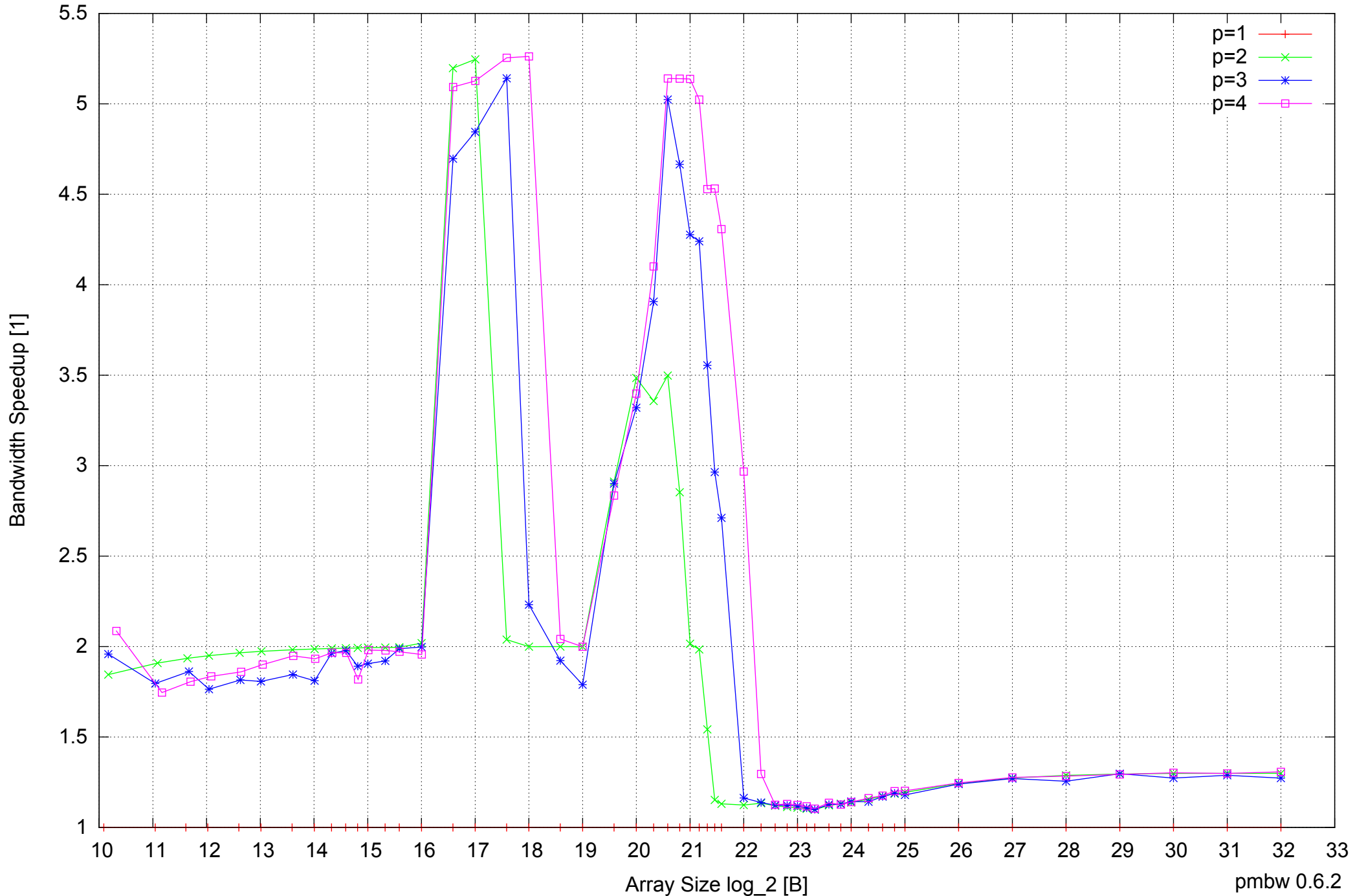
AMD Dual-Core Opteron 270 8GB - Speedup of Parallel Memory Bandwidth - ScanWrite32PtrUnrollLoop
