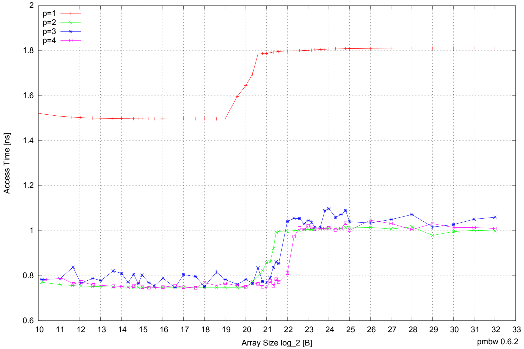
AMD Dual-Core Opteron 270 8GB - Parallel Memory Access Time - ScanRead32PtrSimpleLoop
