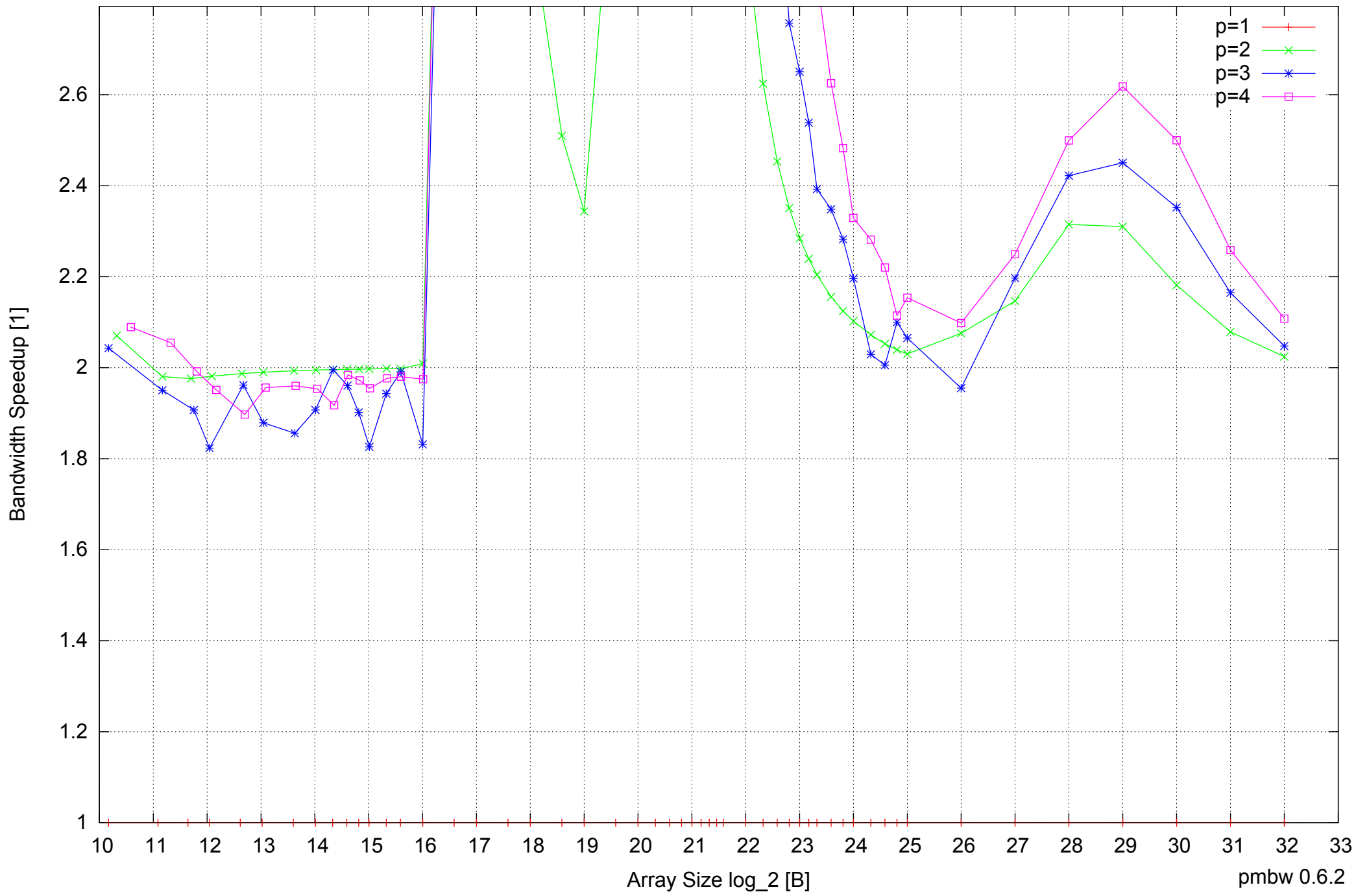
AMD Dual-Core Opteron 270 8GB - Speedup of Parallel Memory Bandwidth (enlarged) - PermRead64UnrollLoop
