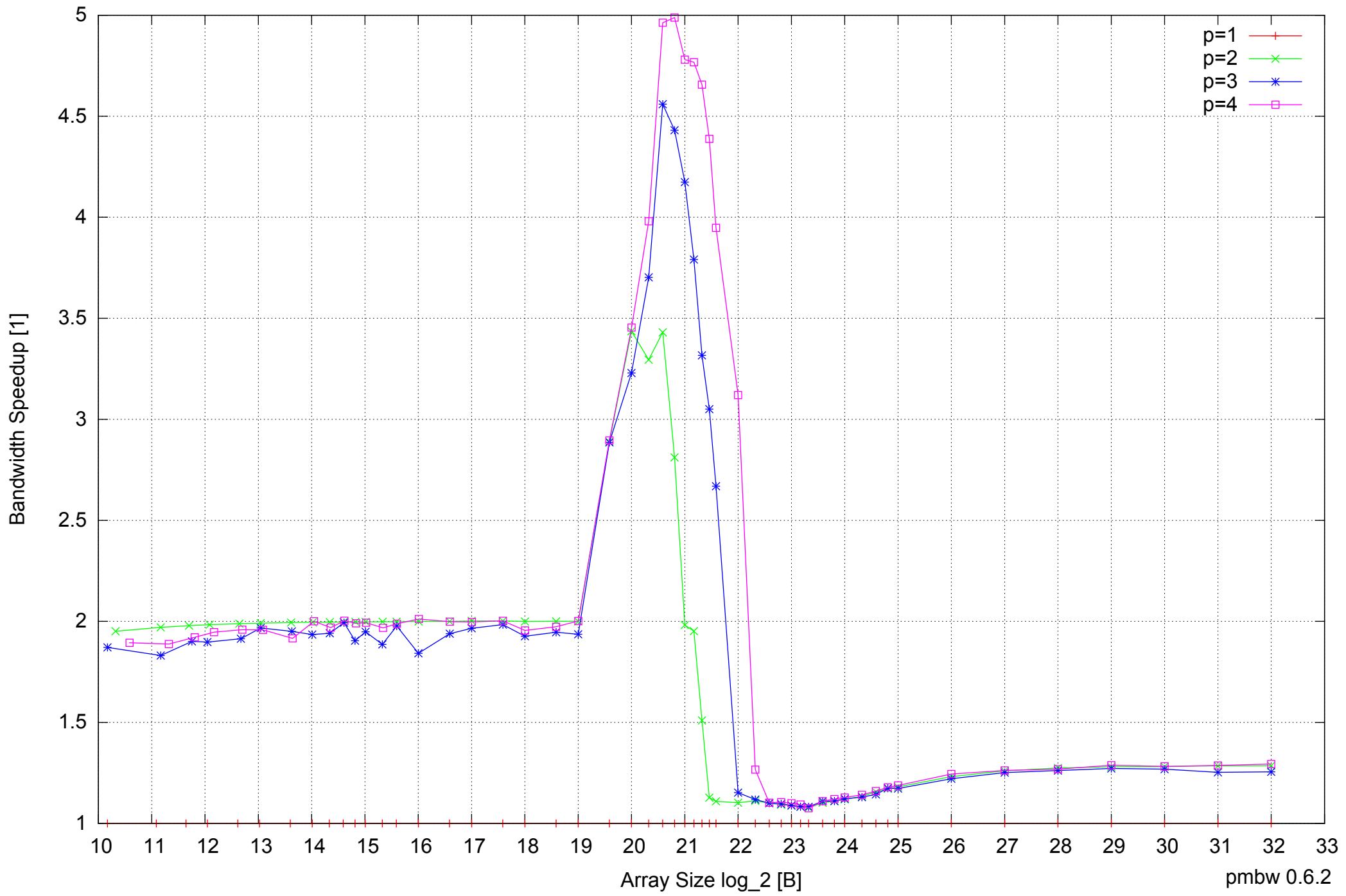
AMD Dual-Core Opteron 270 8GB - Speedup of Parallel Memory Bandwidth - ScanWrite64IndexSimpleLoop
