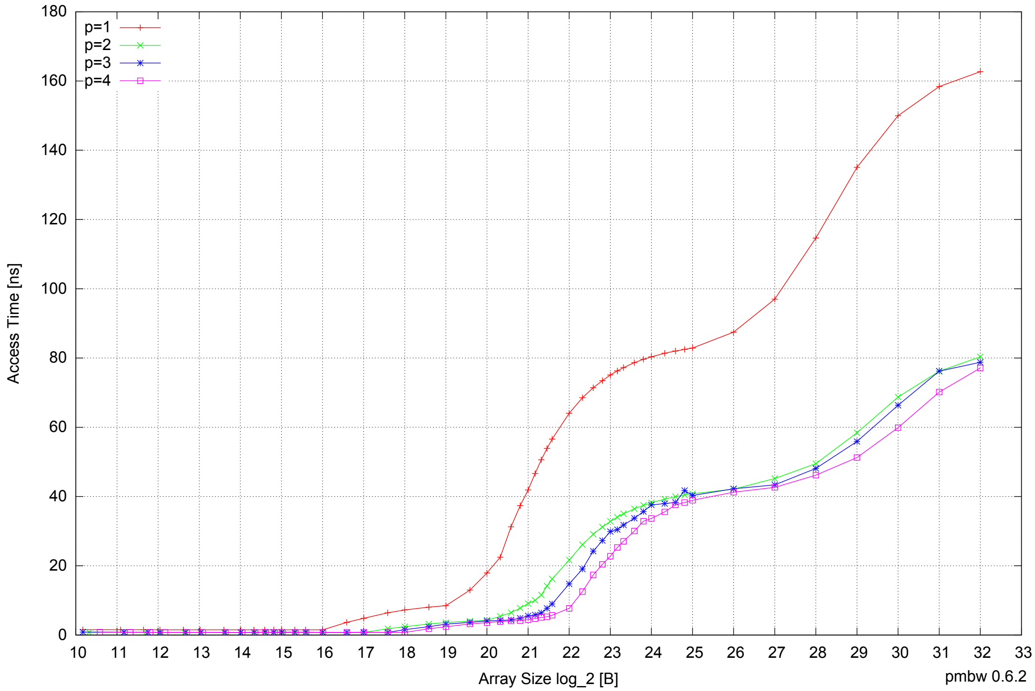
AMD Dual-Core Opteron 270 8GB - Parallel Memory Access Time - PermRead64SimpleLoop
