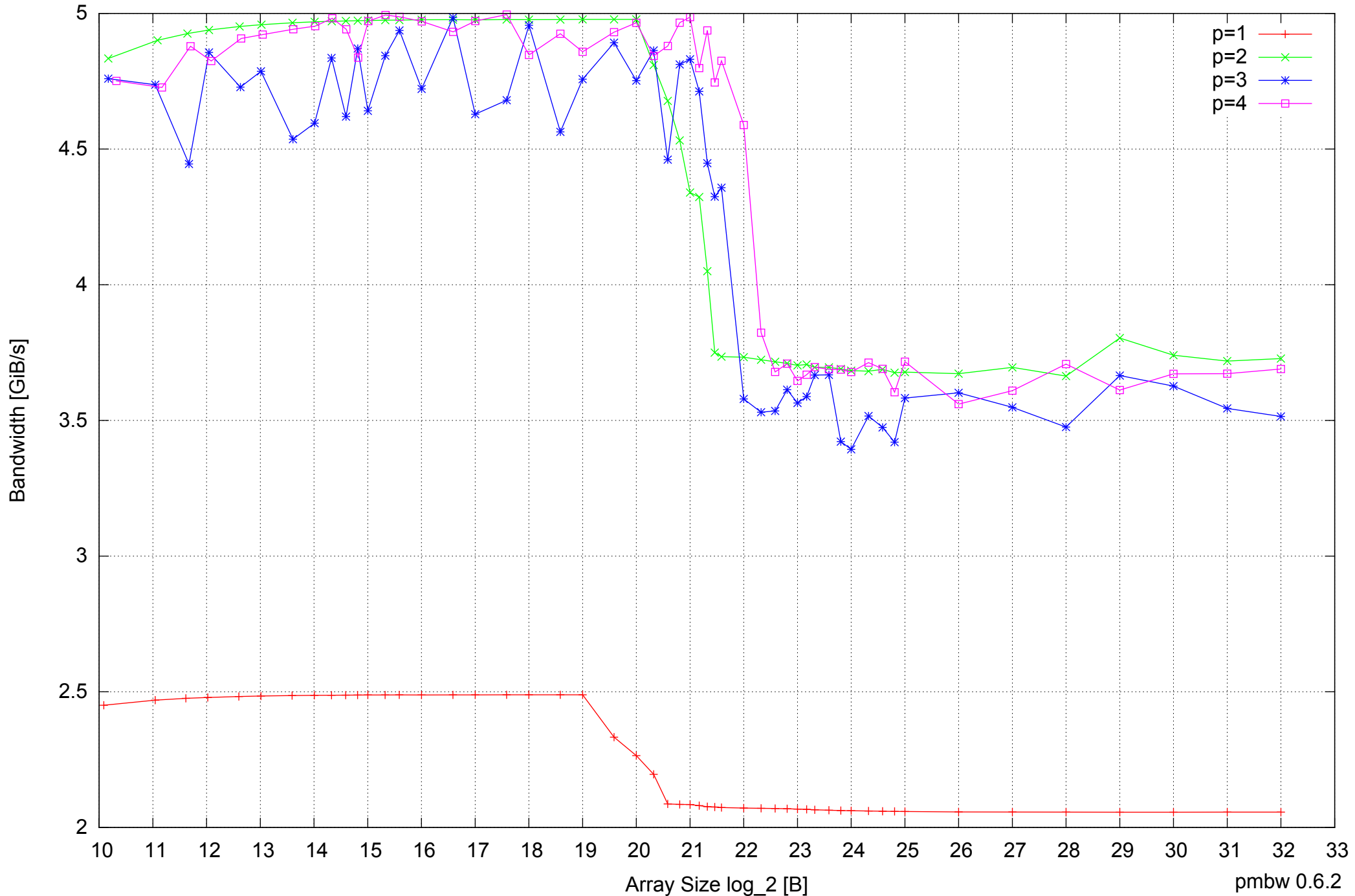
AMD Dual-Core Opteron 270 8GB - Parallel Memory Bandwidth - ScanRead32PtrSimpleLoop
