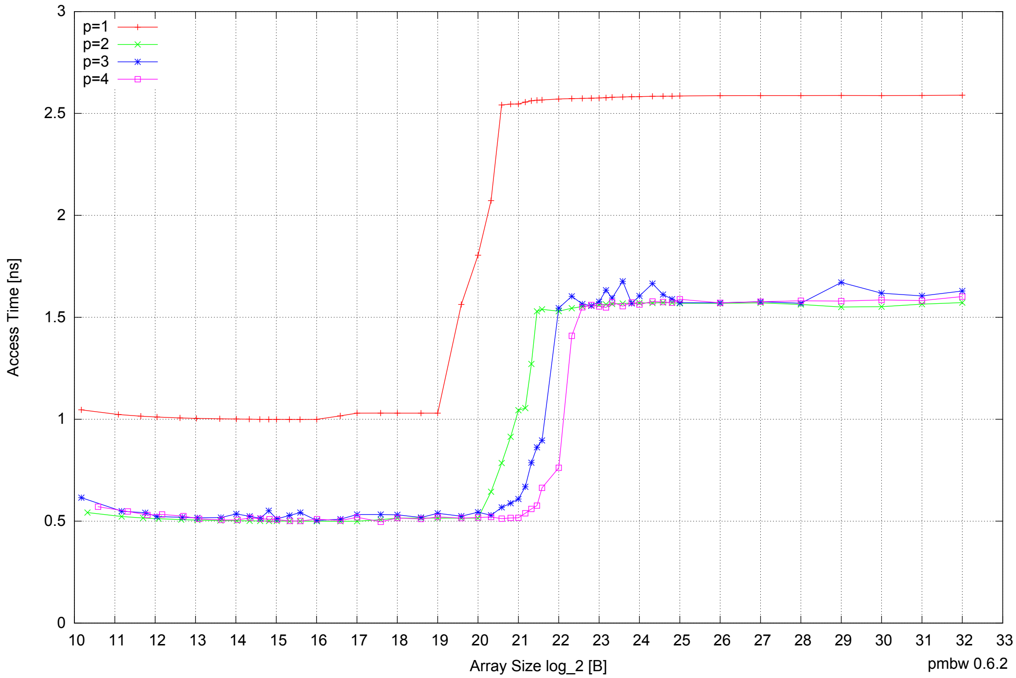
AMD Dual-Core Opteron 270 8GB - Parallel Memory Access Time - ScanRead64IndexSimpleLoop
