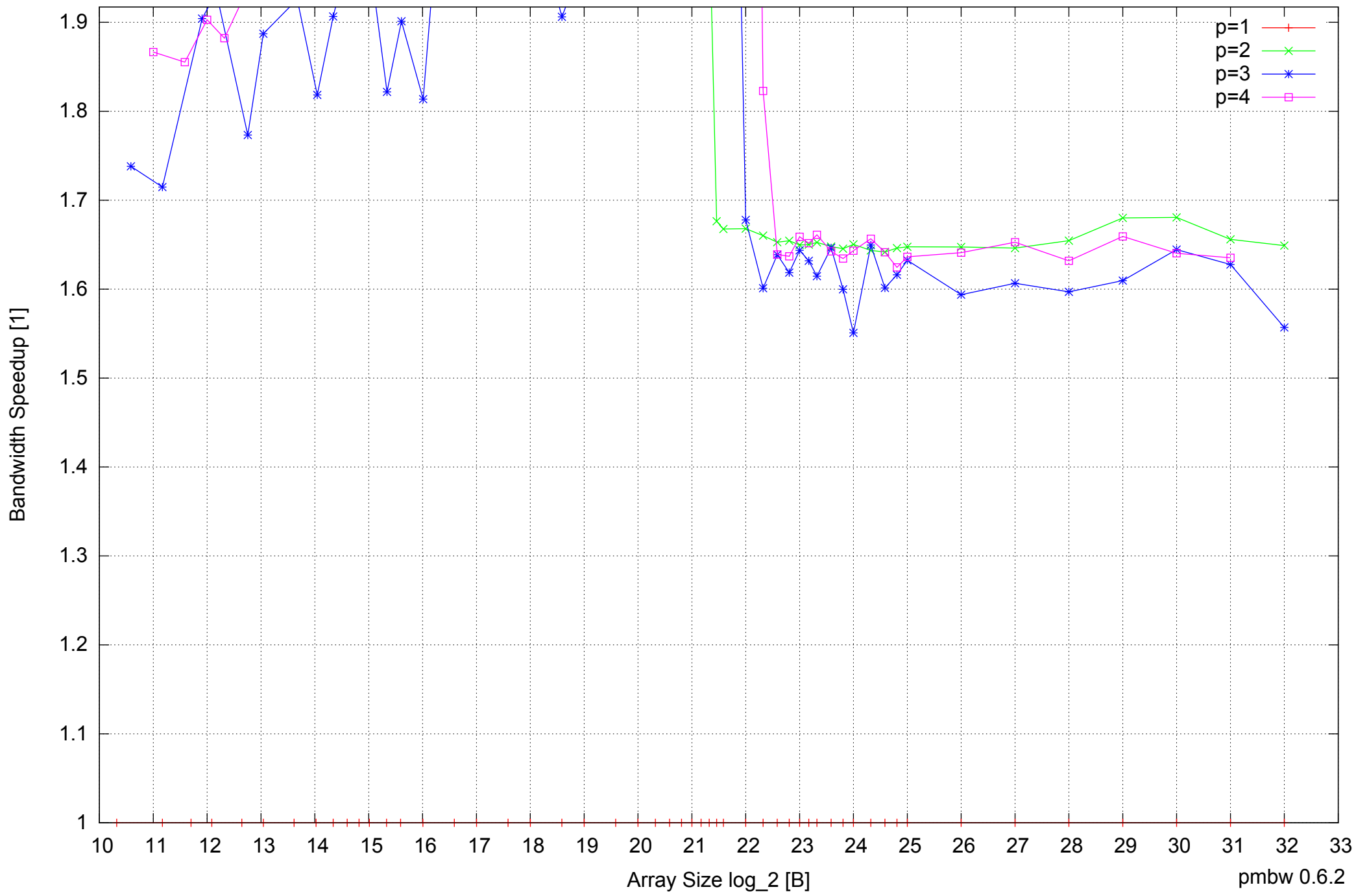
AMD Dual-Core Opteron 270 8GB - Speedup of Parallel Memory Bandwidth (enlarged) - ScanRead128PtrSimpleLoop
