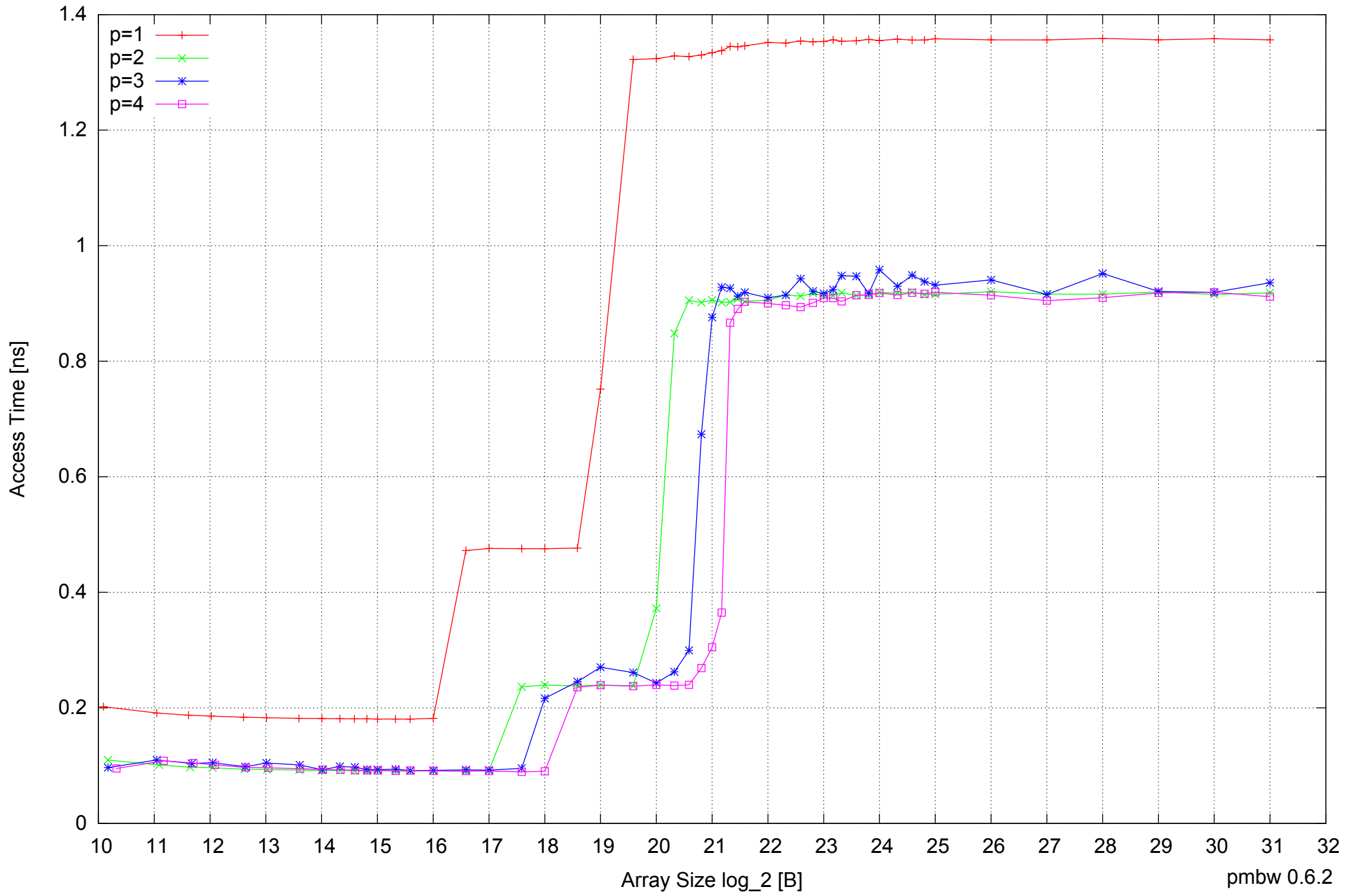
AMD Athlon 64 X2 5600+ 4GB - Parallel Memory Access Time - ScanRead32PtrUnrollLoop
