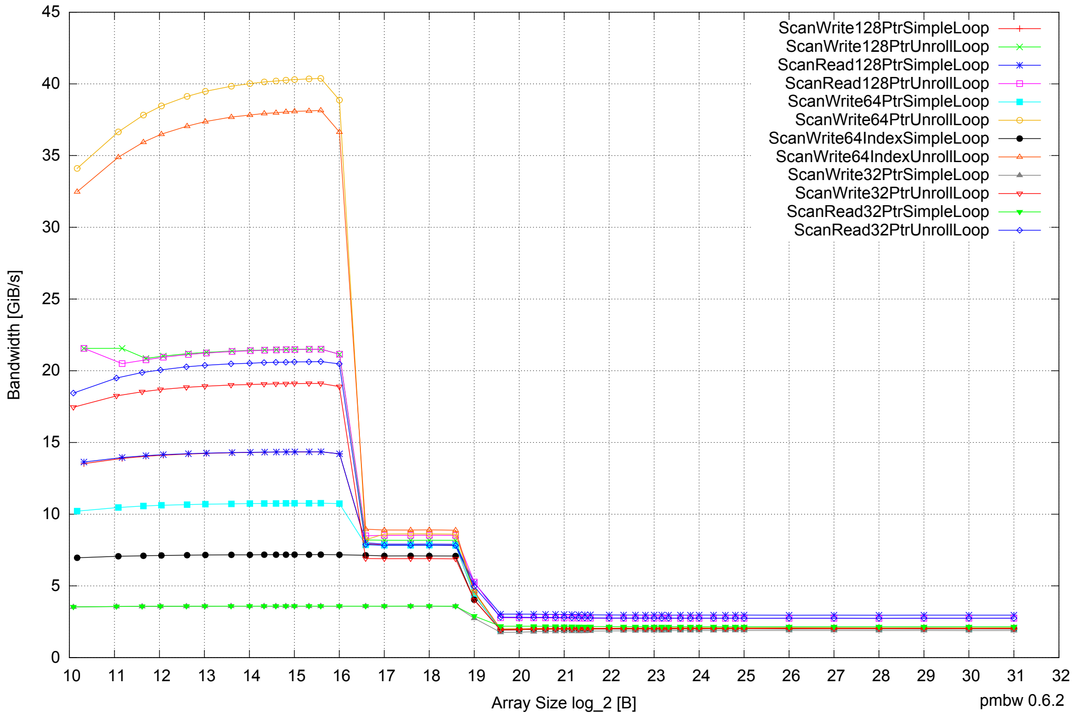
AMD Athlon 64 X2 5600+ 4GB - One Thread Memory Bandwidth (only 64-bit Reads)
