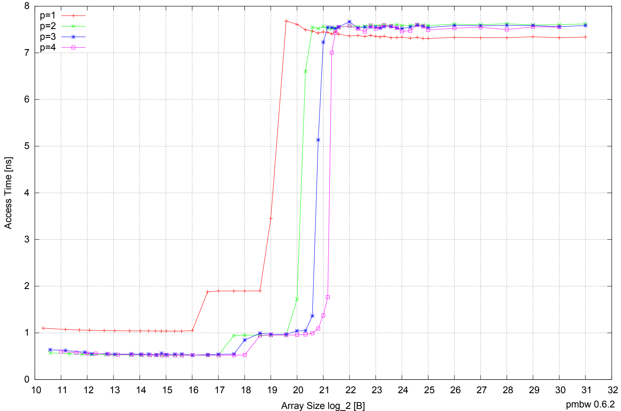
AMD Athlon 64 X2 5600+ 4GB - Parallel Memory Access Time - ScanWrite128PtrSimpleLoop
