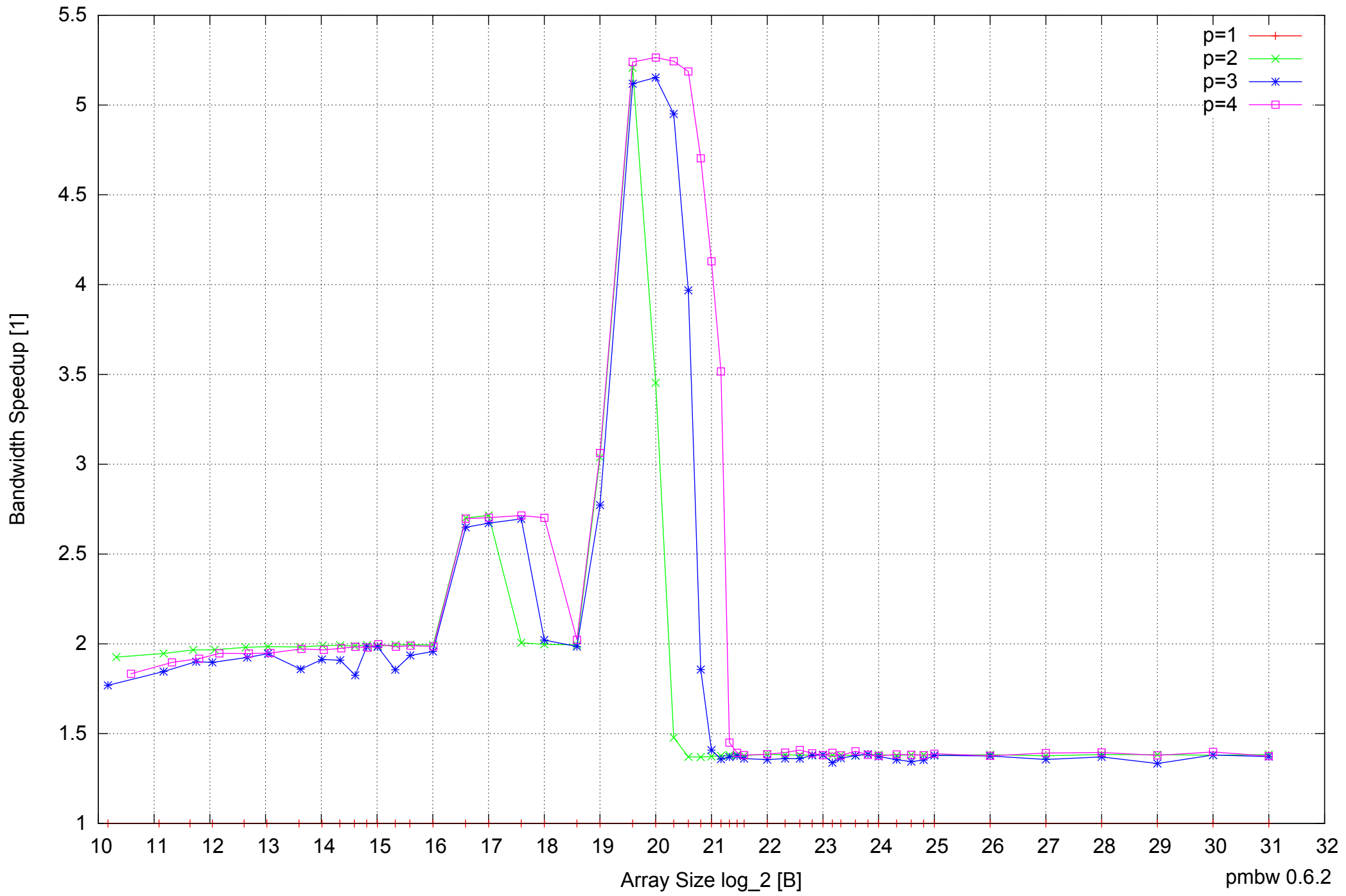
AMD Athlon 64 X2 5600+ 4GB - Speedup of Parallel Memory Bandwidth - ScanRead64IndexSimpleLoop
