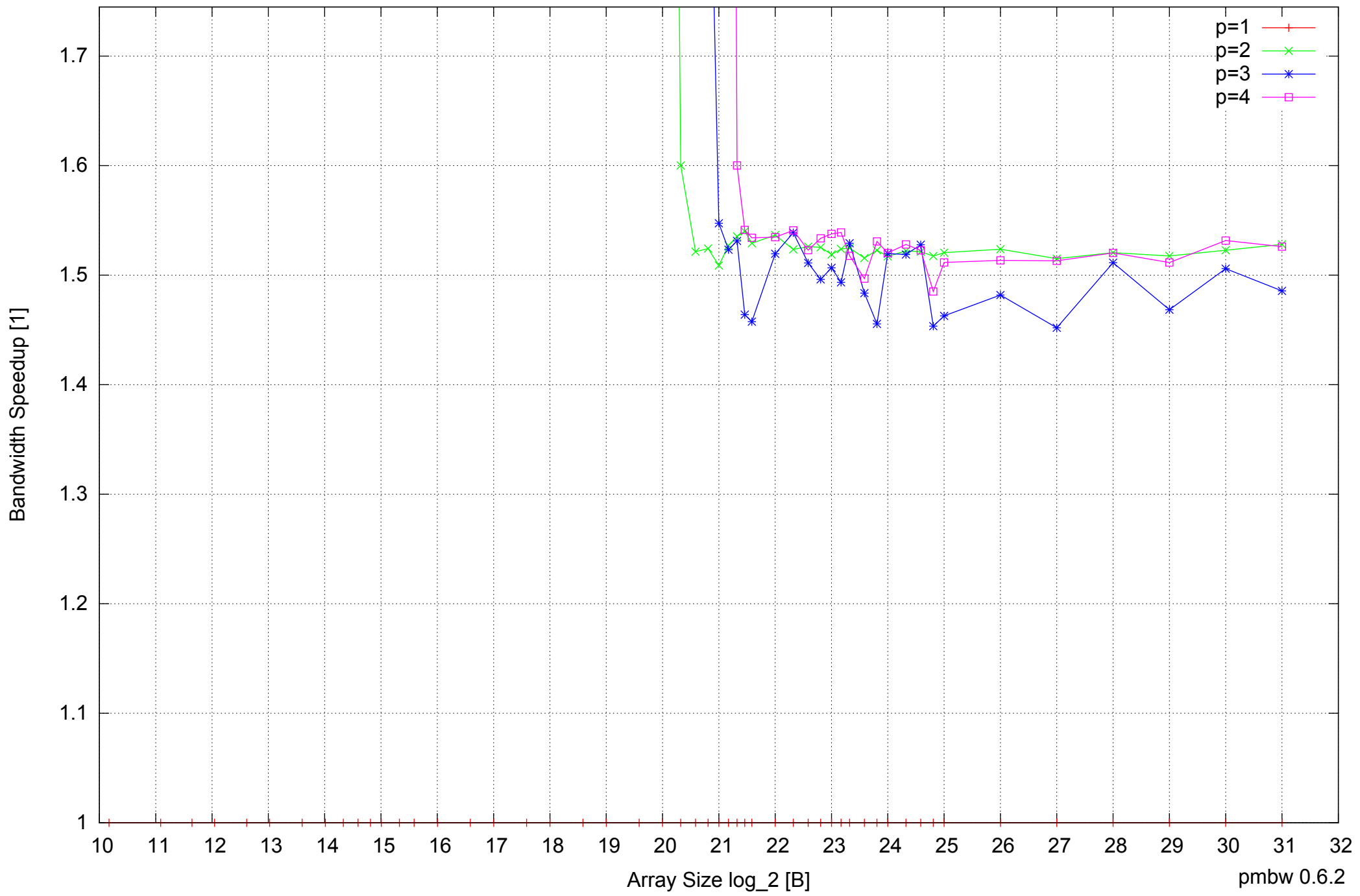
AMD Athlon 64 X2 5600+ 4GB - Speedup of Parallel Memory Bandwidth (enlarged) - ScanRead64PtrSimpleLoop
