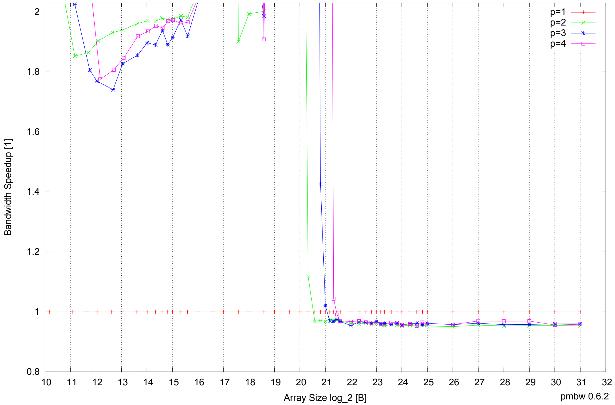
AMD Athlon 64 X2 5600+ 4GB - Speedup of Parallel Memory Bandwidth (enlarged) - ScanWrite64PtrUnrollLoop
