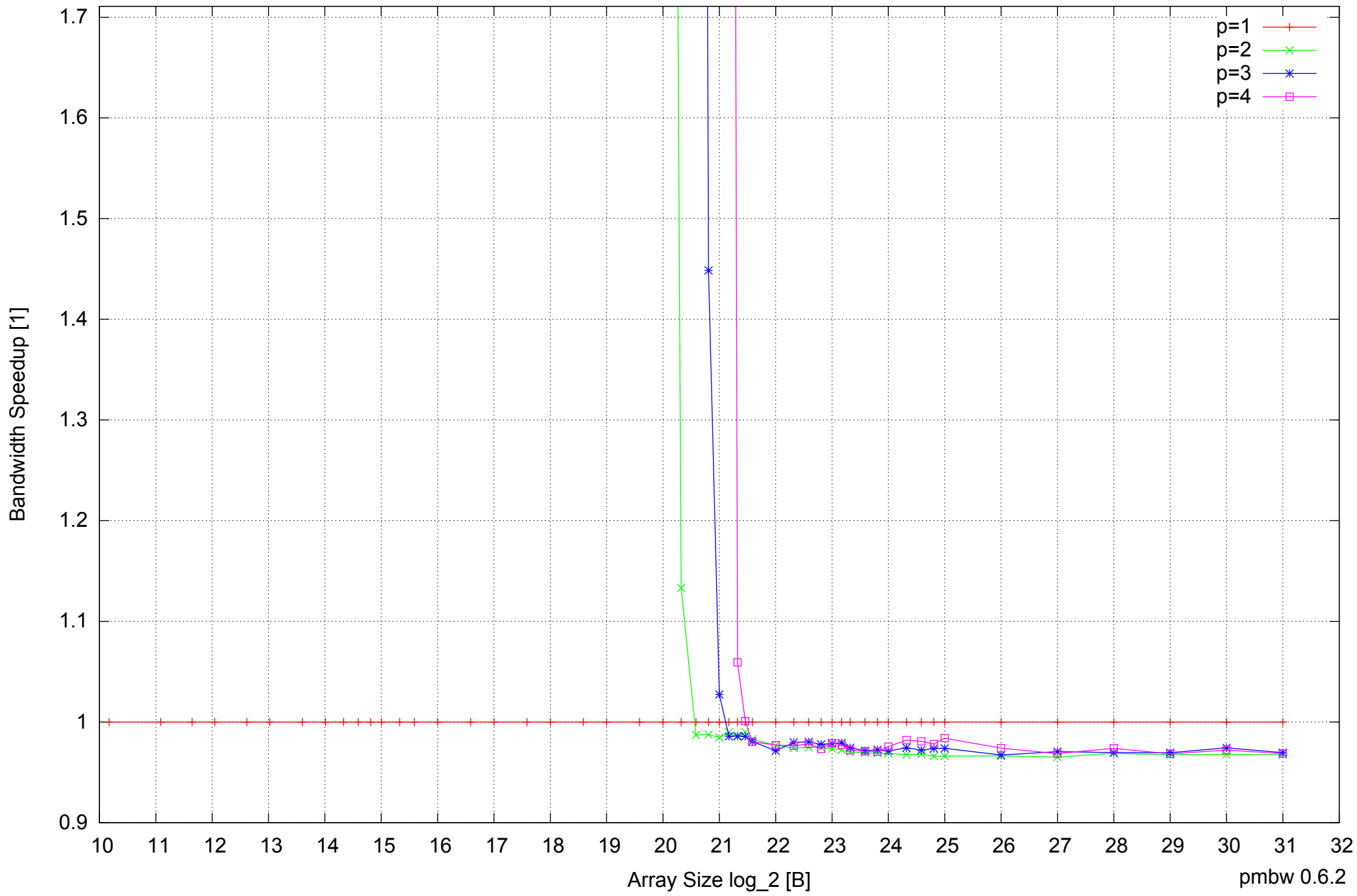
AMD Athlon 64 X2 5600+ 4GB - Speedup of Parallel Memory Bandwidth (enlarged) - ScanWrite64PtrSimpleLoop
