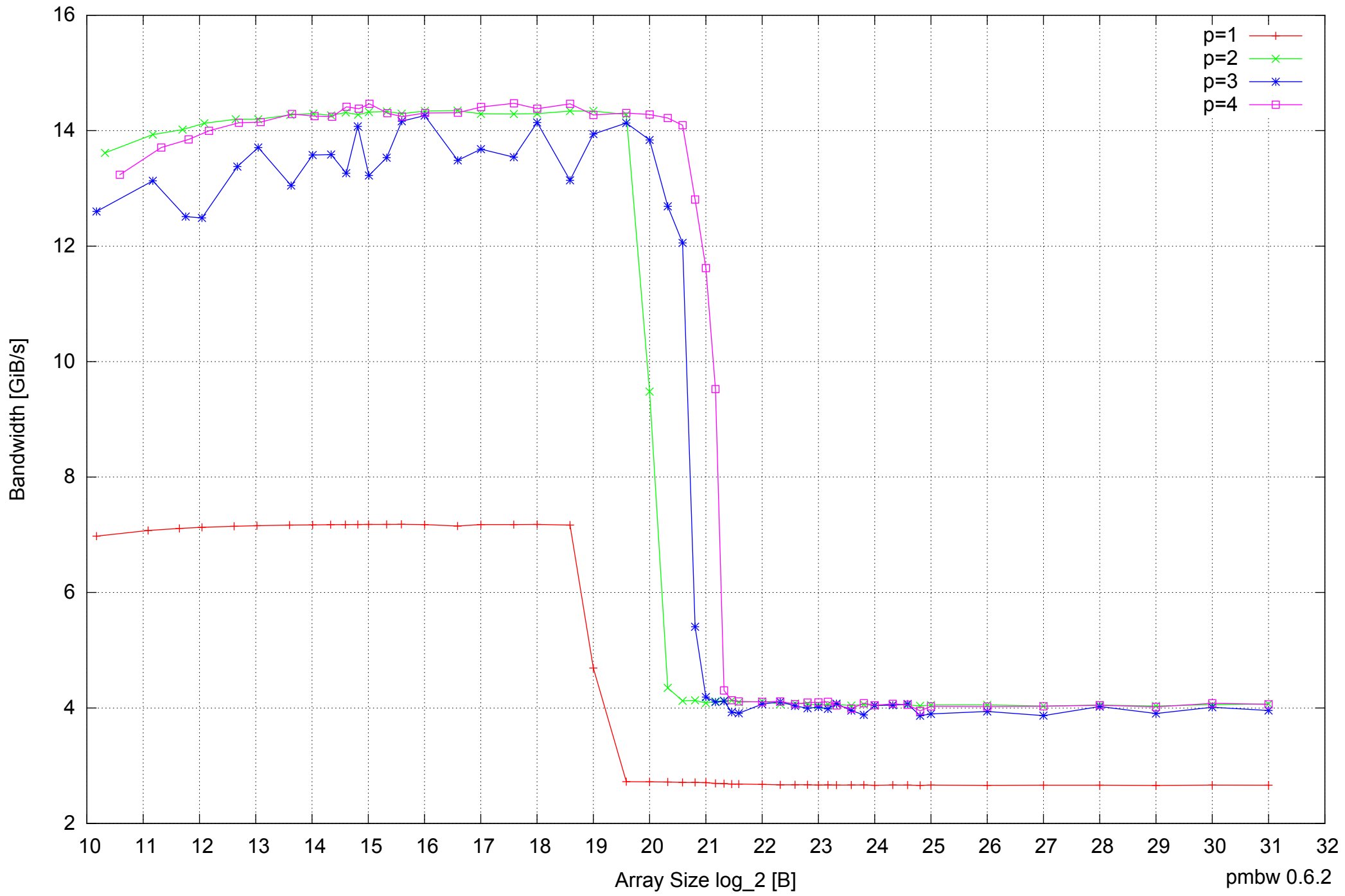
AMD Athlon 64 X2 5600+ 4GB - Parallel Memory Bandwidth - ScanRead64PtrSimpleLoop
