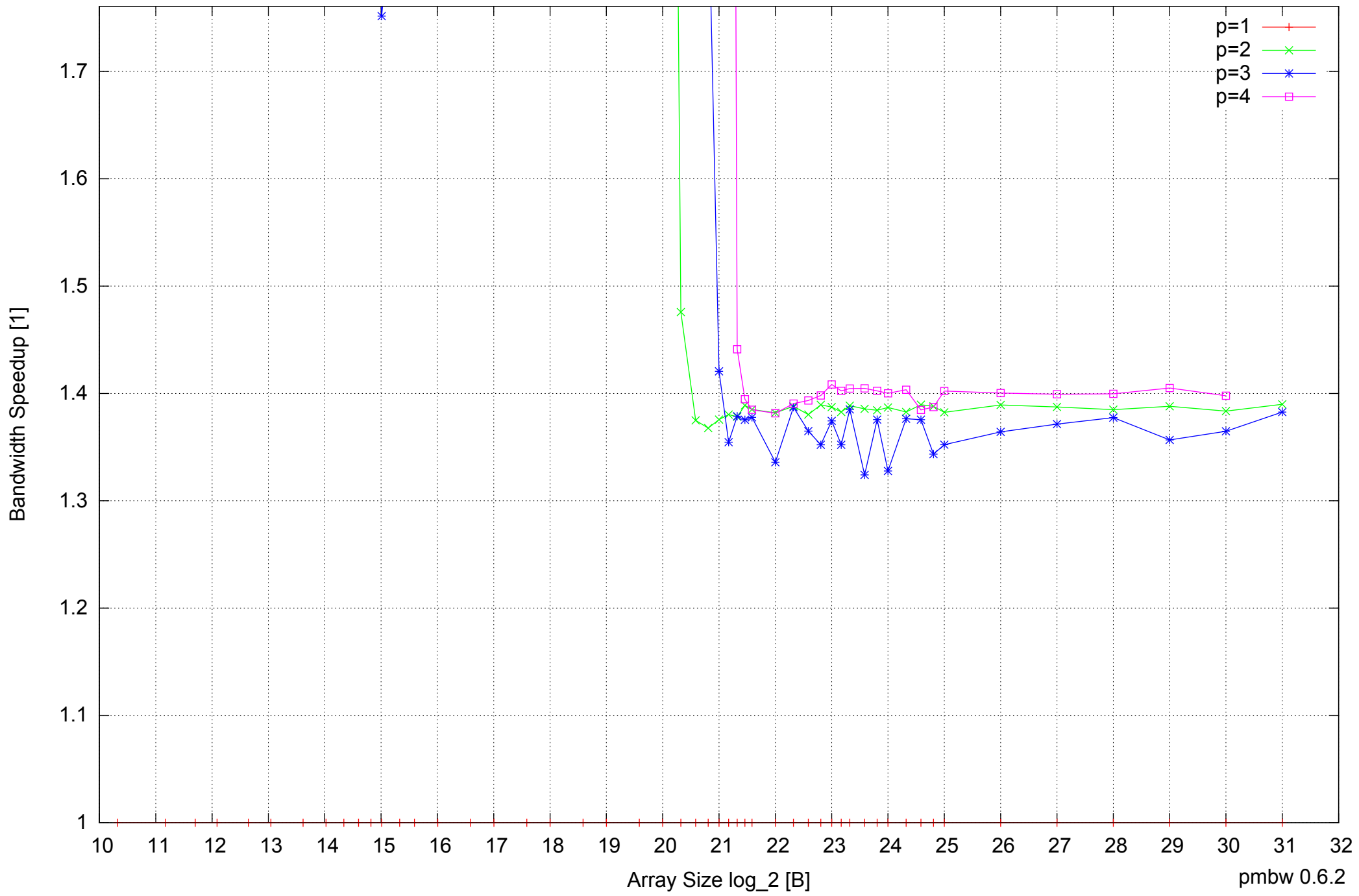
AMD Athlon 64 X2 5600+ 4GB - Speedup of Parallel Memory Bandwidth (enlarged) - ScanRead128PtrSimpleLoop
