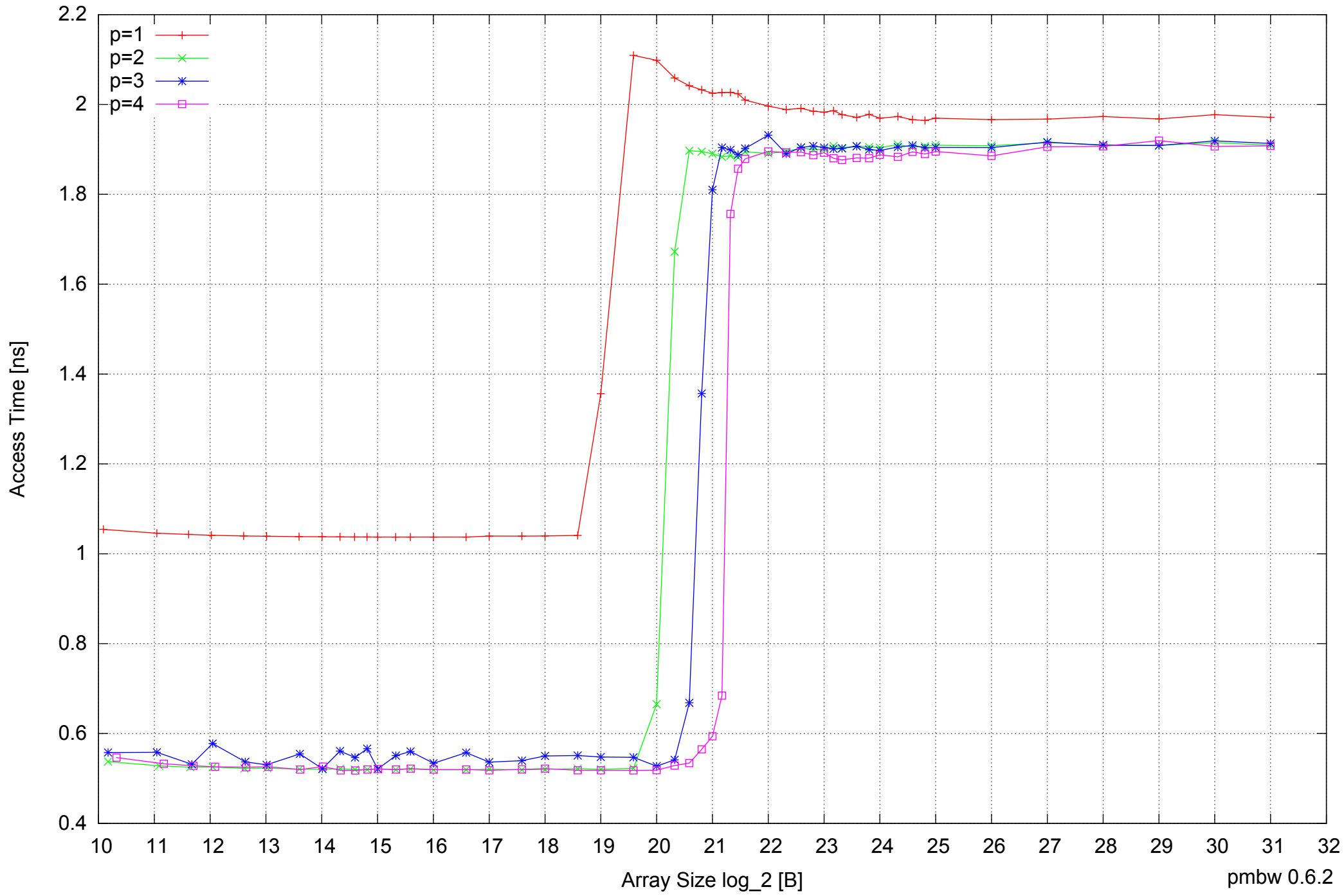
AMD Athlon 64 X2 5600+ 4GB - Parallel Memory Access Time - ScanWrite32PtrSimpleLoop
