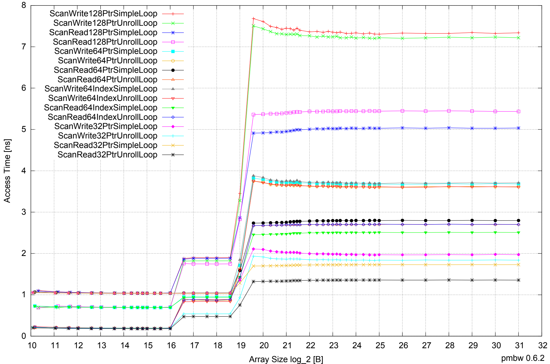
AMD Athlon 64 X2 5600+ 4GB - One Thread Memory Latency (excluding Permutation)
