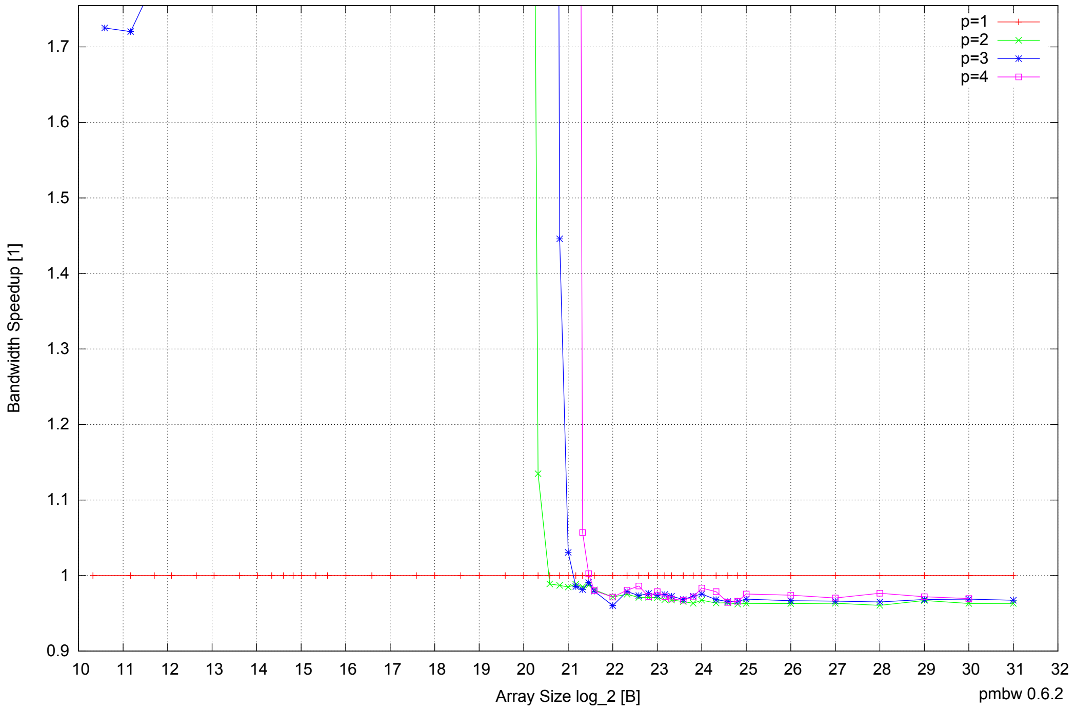
AMD Athlon 64 X2 5600+ 4GB - Speedup of Parallel Memory Bandwidth (enlarged) - ScanWrite128PtrSimpleLoop
