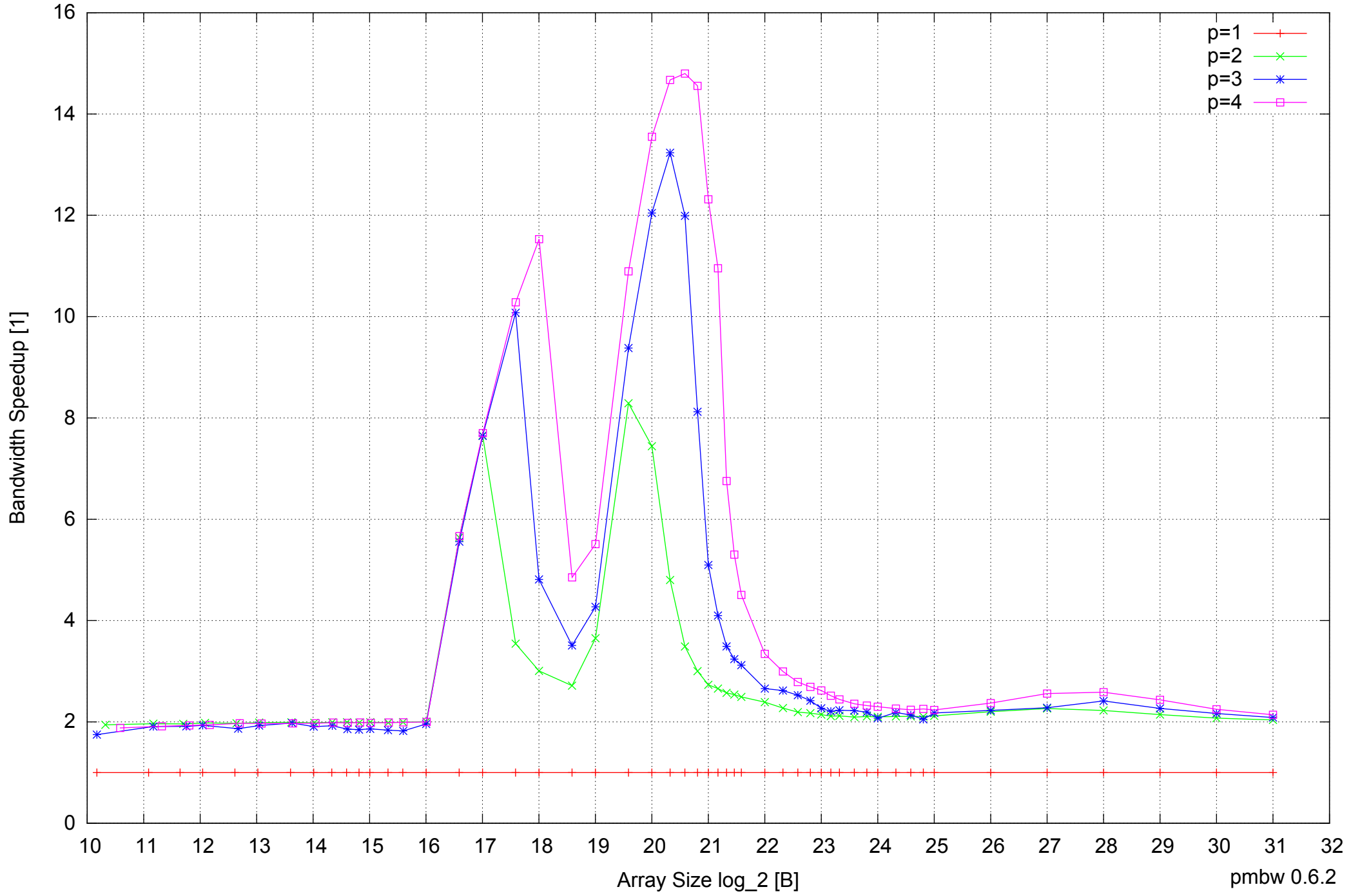
AMD Athlon 64 X2 5600+ 4GB - Speedup of Parallel Memory Bandwidth - PermRead64SimpleLoop
