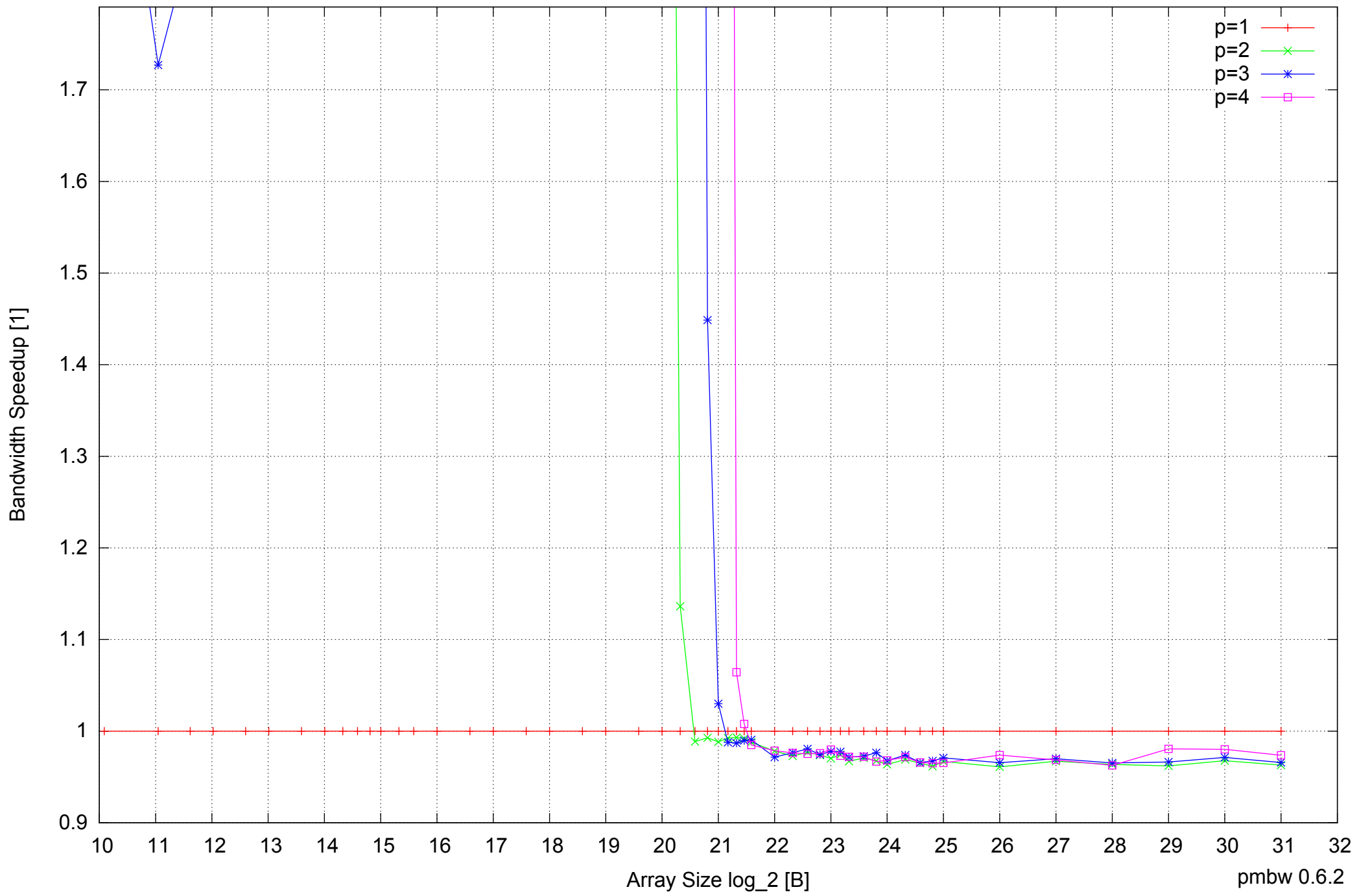
AMD Athlon 64 X2 5600+ 4GB - Speedup of Parallel Memory Bandwidth (enlarged) - ScanWrite32PtrUnrollLoop
