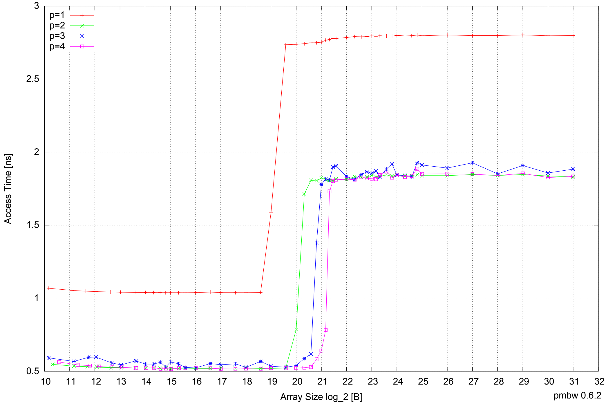
AMD Athlon 64 X2 5600+ 4GB - Parallel Memory Access Time - ScanRead64PtrSimpleLoop
