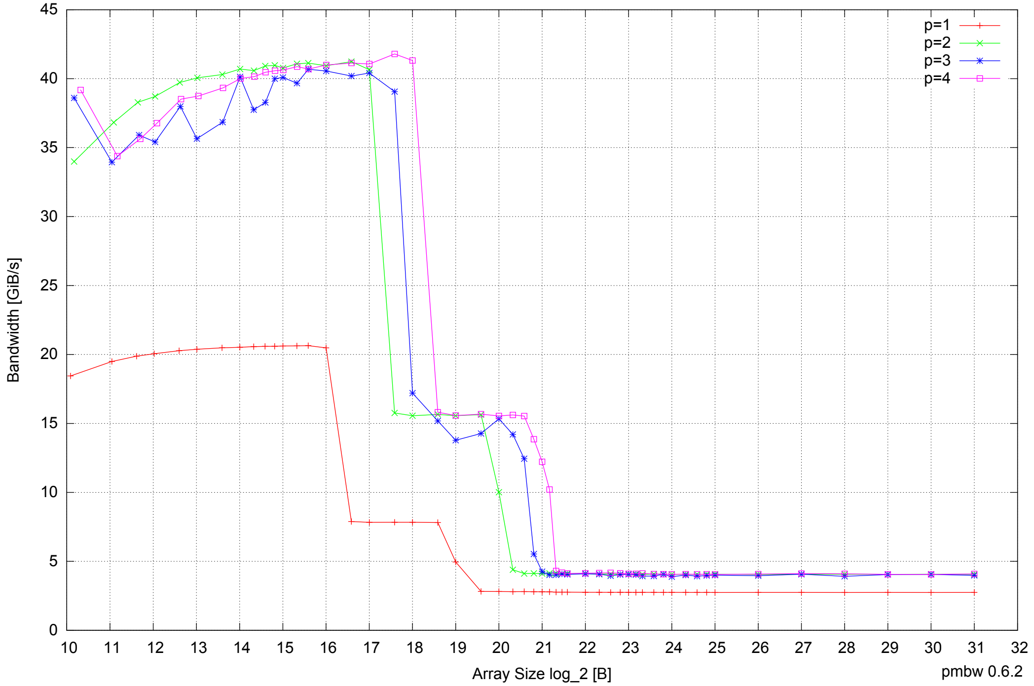
AMD Athlon 64 X2 5600+ 4GB - Parallel Memory Bandwidth - ScanRead32PtrUnrollLoop
