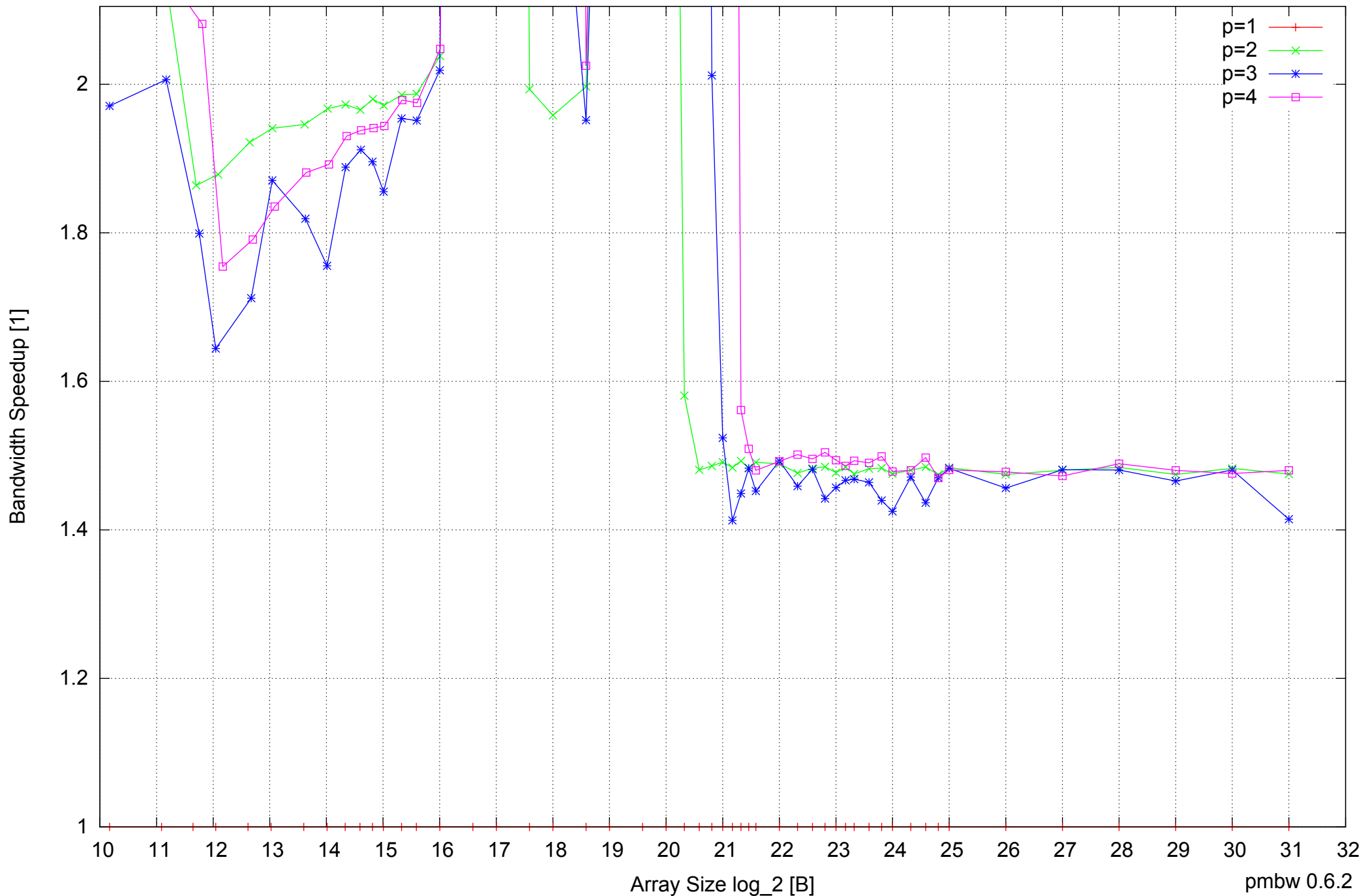
AMD Athlon 64 X2 5600+ 4GB - Speedup of Parallel Memory Bandwidth (enlarged) - ScanRead64IndexUnrollLoop
