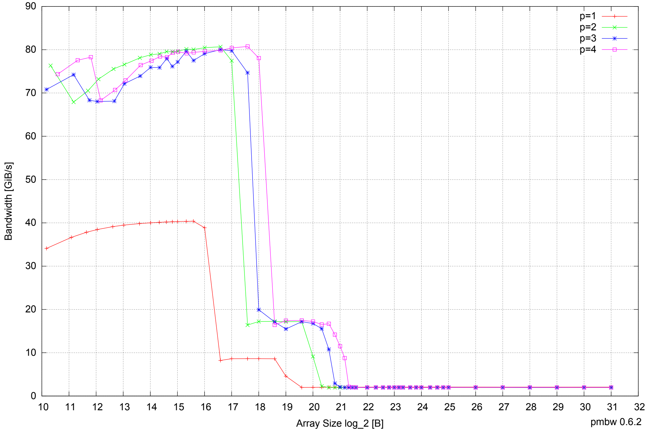
AMD Athlon 64 X2 5600+ 4GB - Parallel Memory Bandwidth - ScanWrite64PtrUnrollLoop
