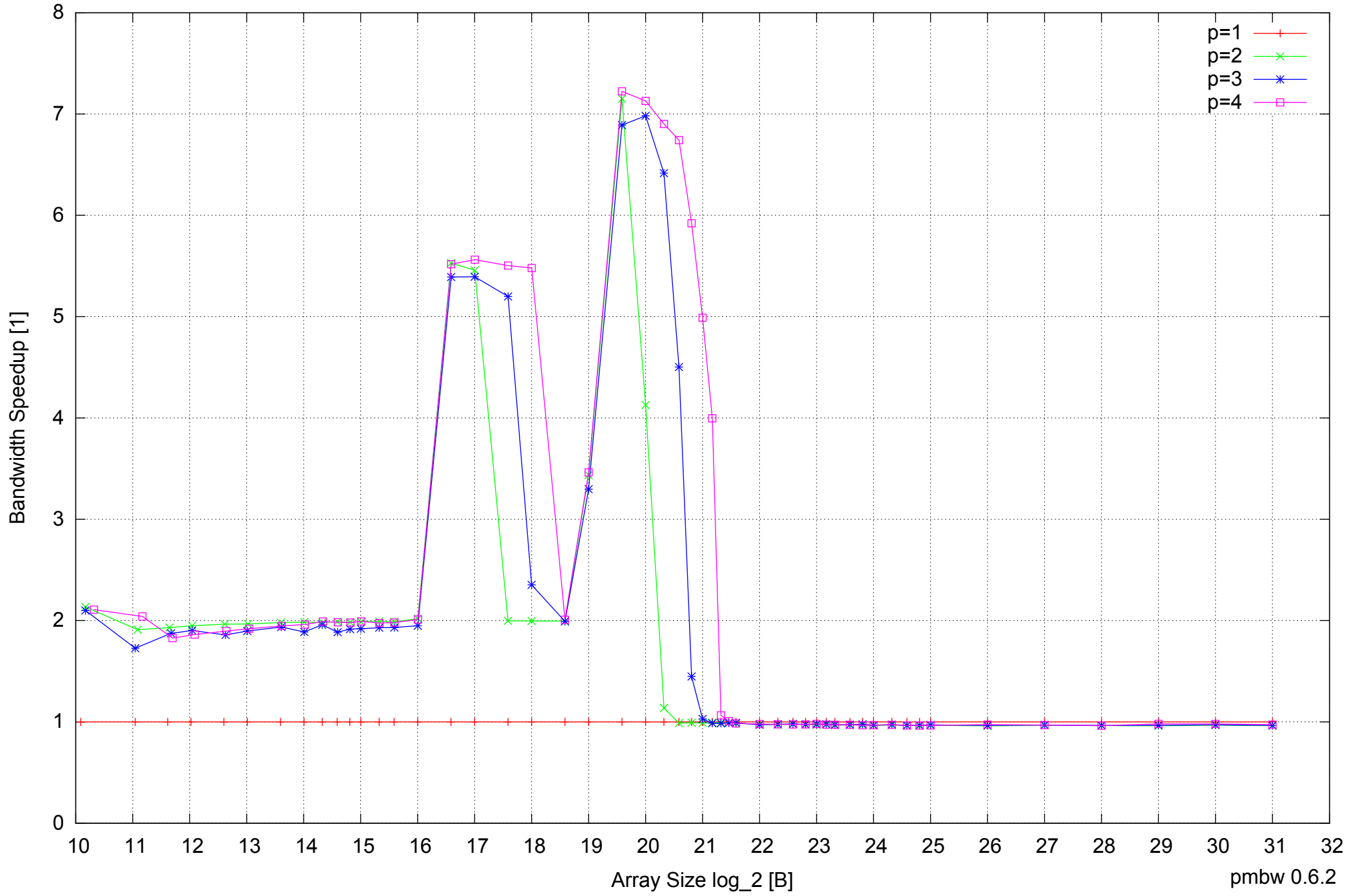
AMD Athlon 64 X2 5600+ 4GB - Speedup of Parallel Memory Bandwidth - ScanWrite32PtrUnrollLoop
