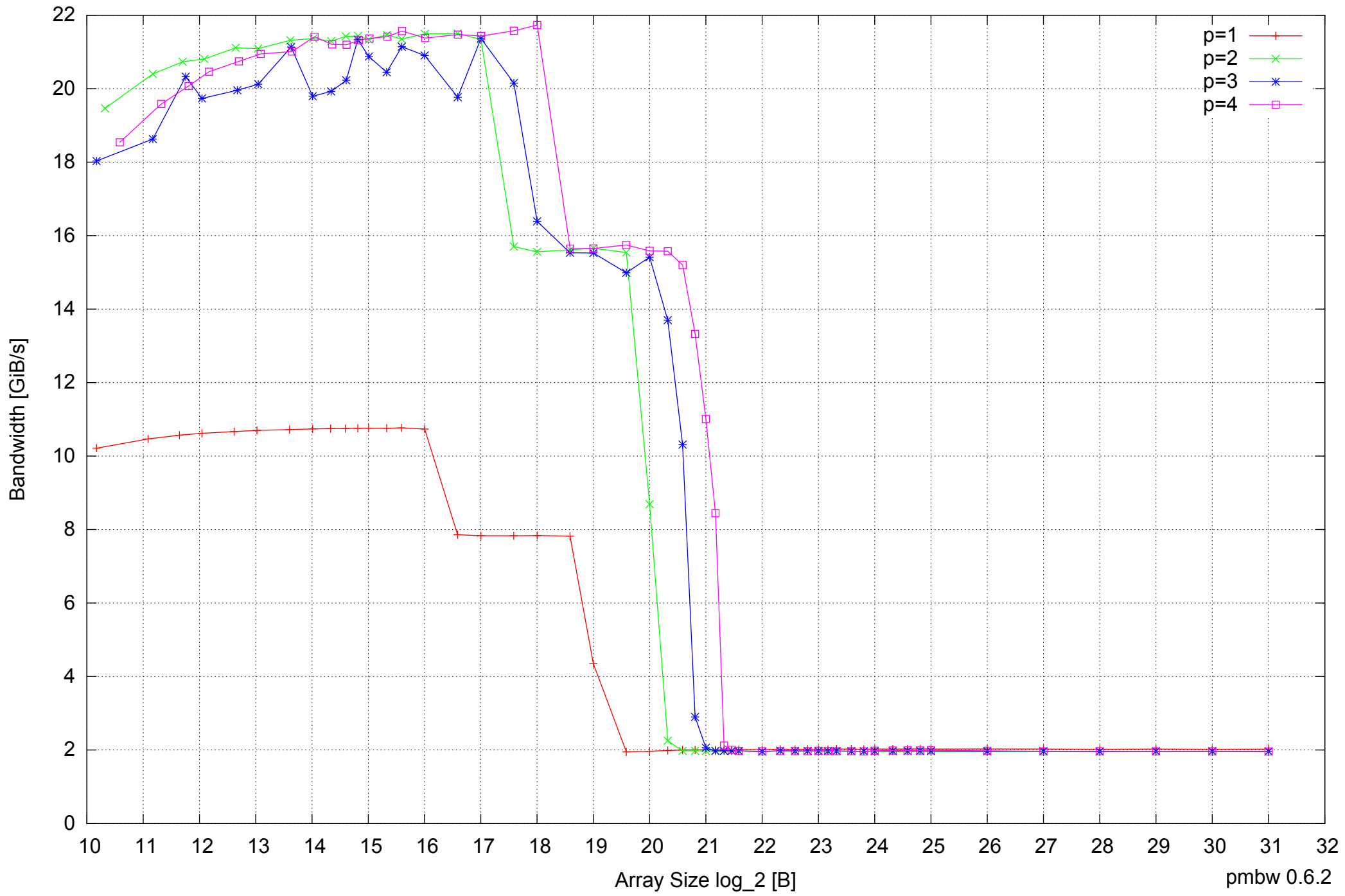
AMD Athlon 64 X2 5600+ 4GB - Parallel Memory Bandwidth - ScanWrite64PtrSimpleLoop
