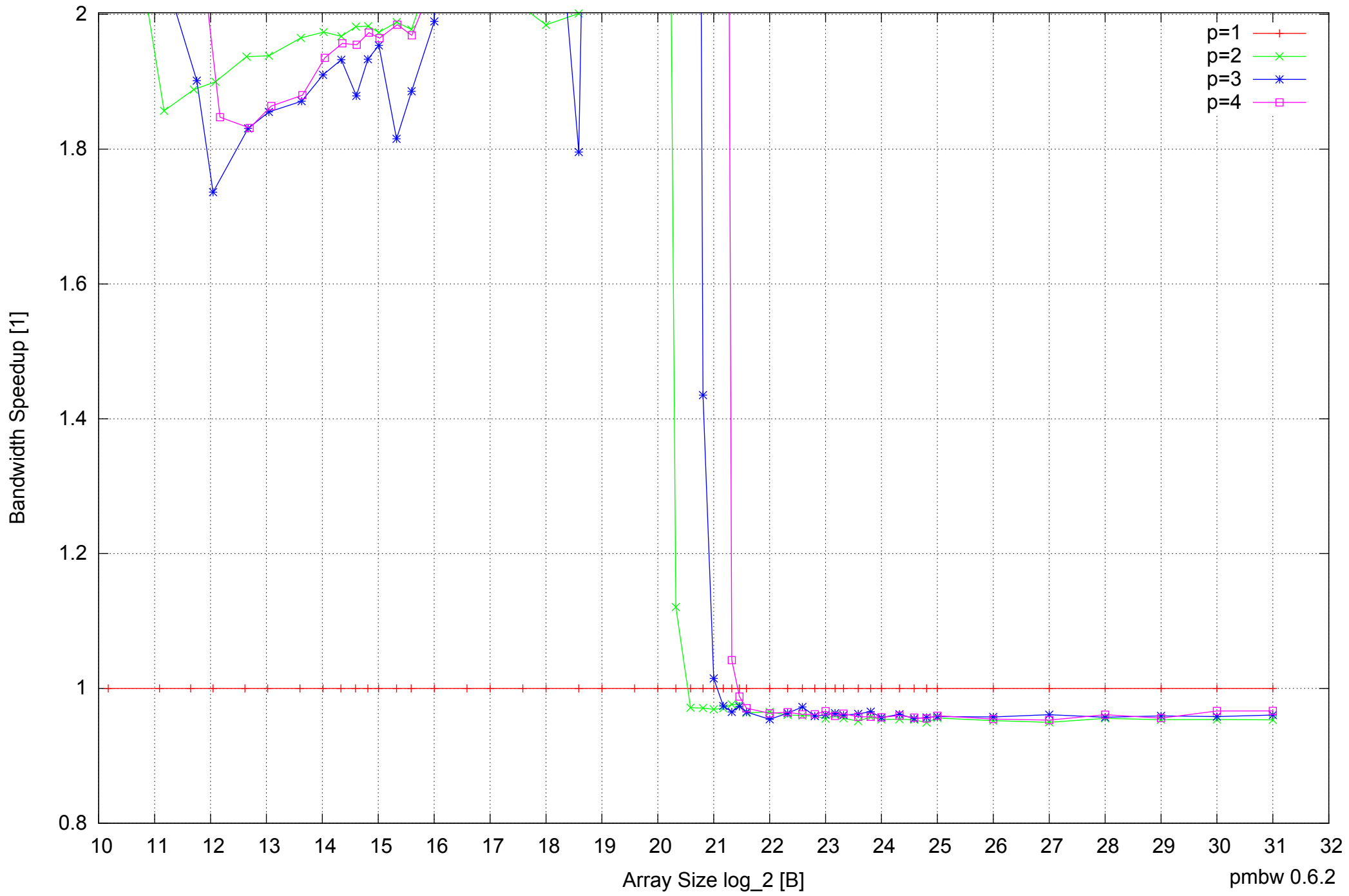
AMD Athlon 64 X2 5600+ 4GB - Speedup of Parallel Memory Bandwidth (enlarged) - ScanWrite64IndexUnrollLoop
