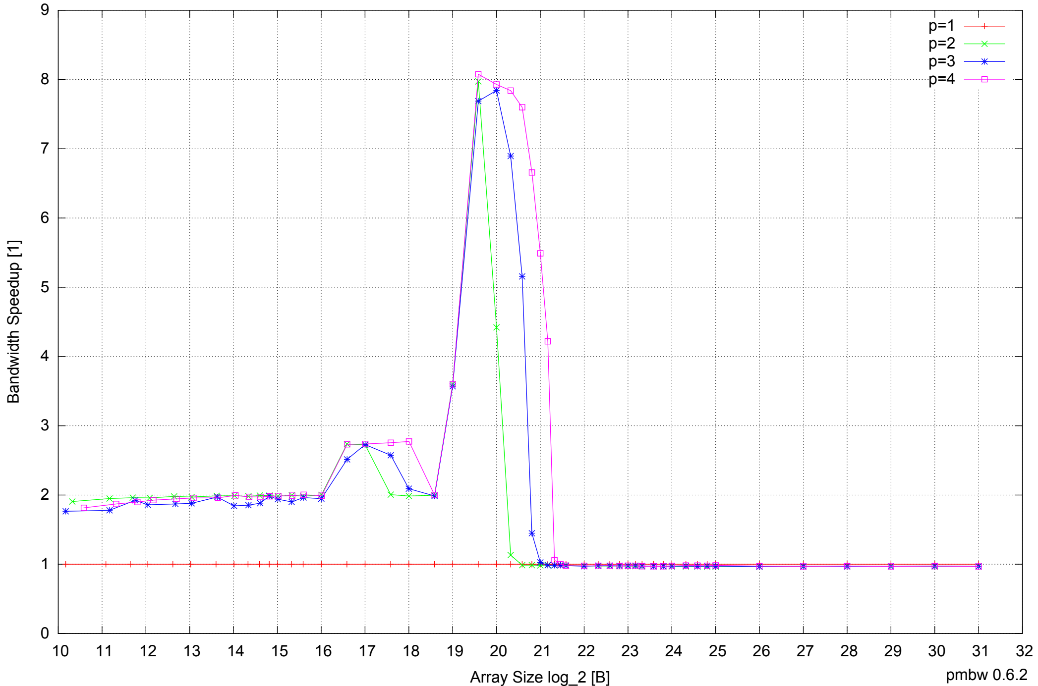
AMD Athlon 64 X2 5600+ 4GB - Speedup of Parallel Memory Bandwidth - ScanWrite64PtrSimpleLoop
