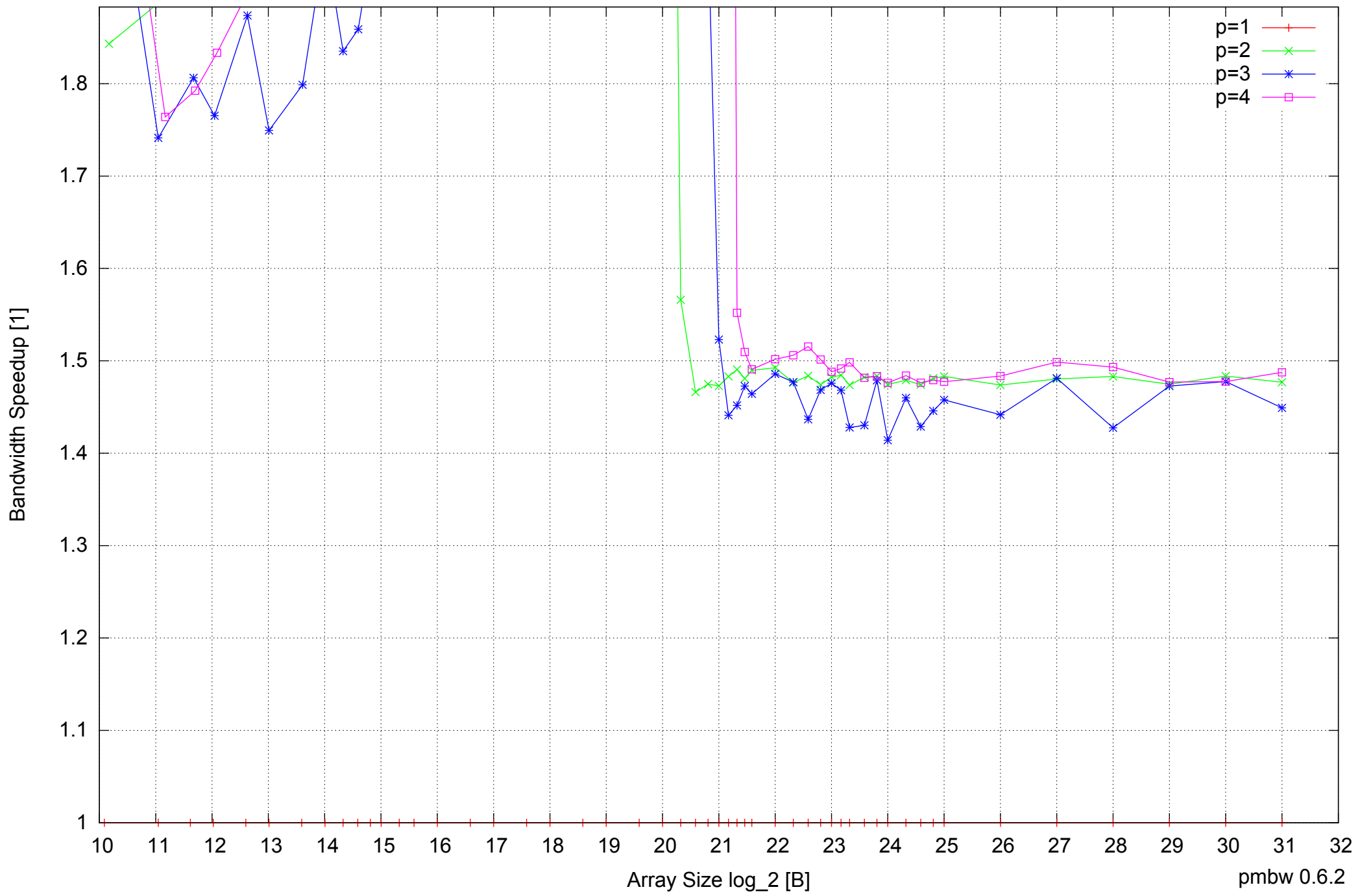
AMD Athlon 64 X2 5600+ 4GB - Speedup of Parallel Memory Bandwidth (enlarged) - ScanRead32PtrUnrollLoop
