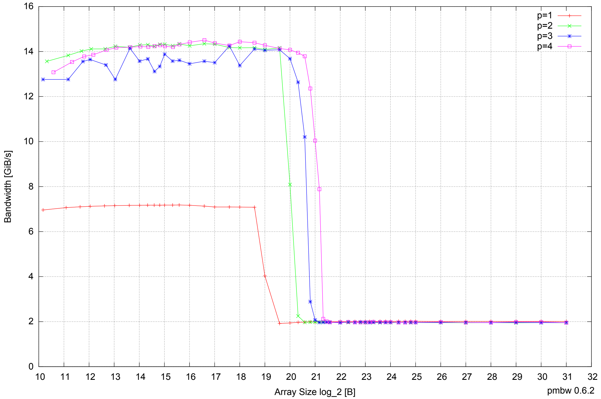
AMD Athlon 64 X2 5600+ 4GB - Parallel Memory Bandwidth - ScanWrite64IndexSimpleLoop
