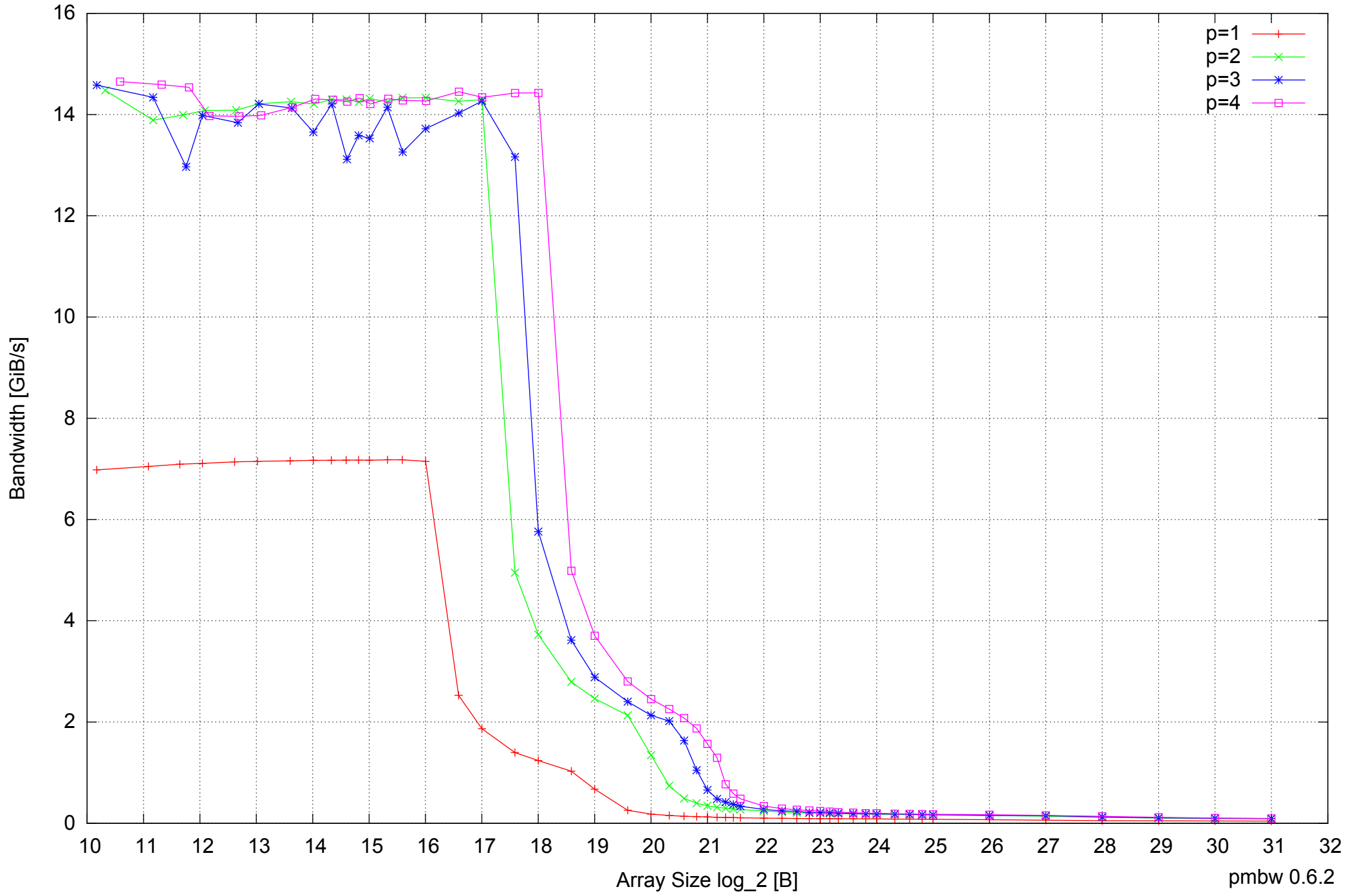
AMD Athlon 64 X2 5600+ 4GB - Parallel Memory Bandwidth - PermRead64UnrollLoop
