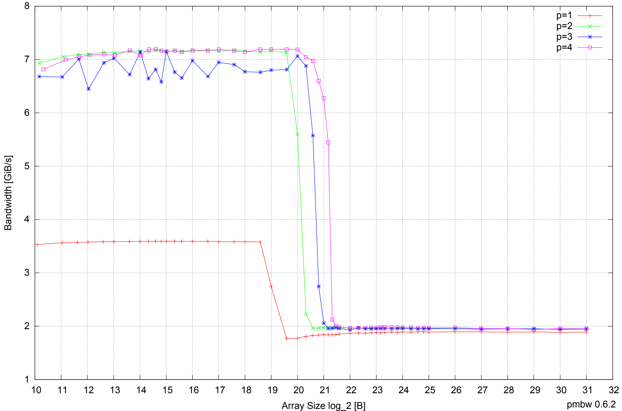
AMD Athlon 64 X2 5600+ 4GB - Parallel Memory Bandwidth - ScanWrite32PtrSimpleLoop
