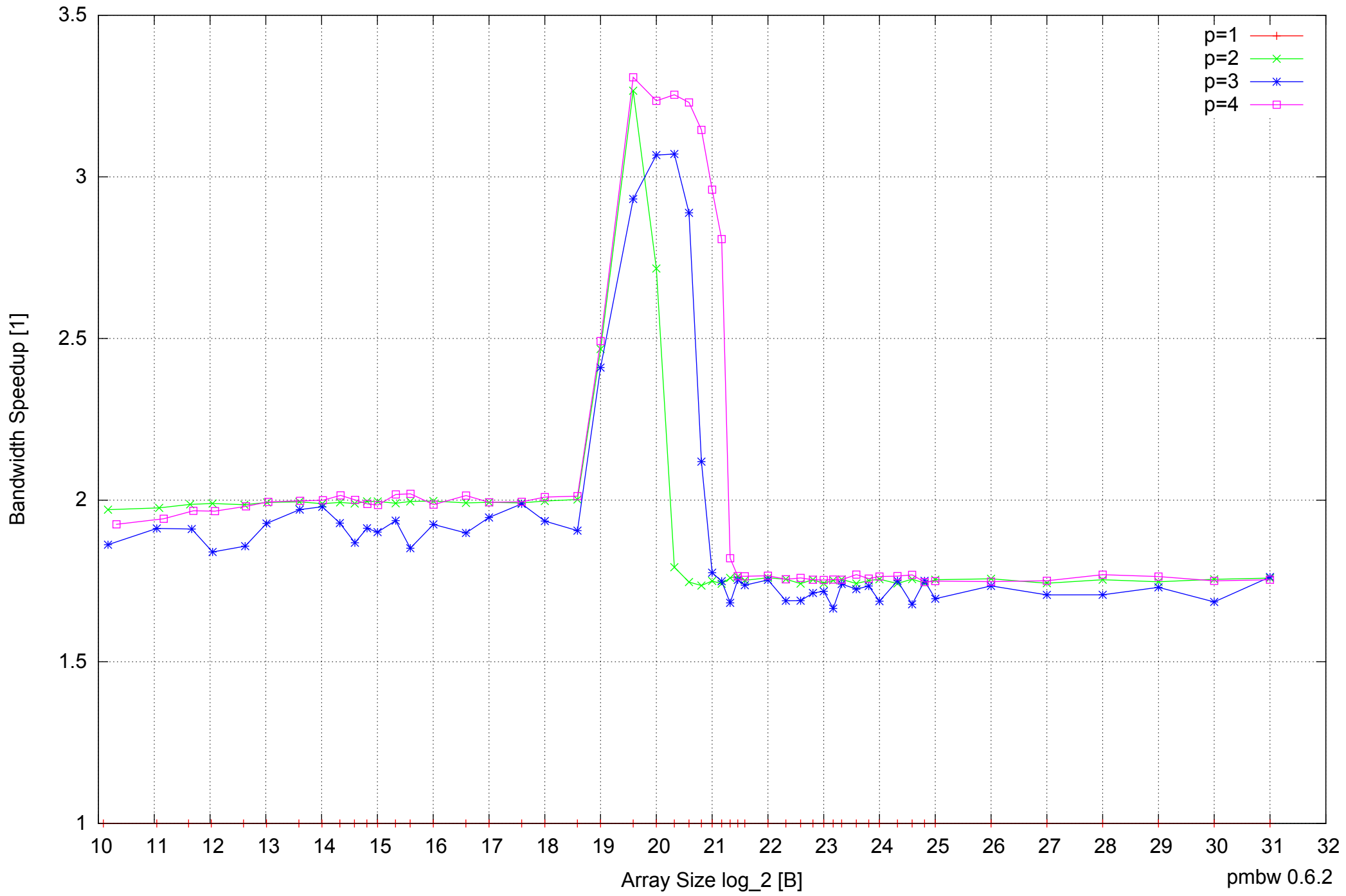
AMD Athlon 64 X2 5600+ 4GB - Speedup of Parallel Memory Bandwidth - ScanRead32PtrSimpleLoop
