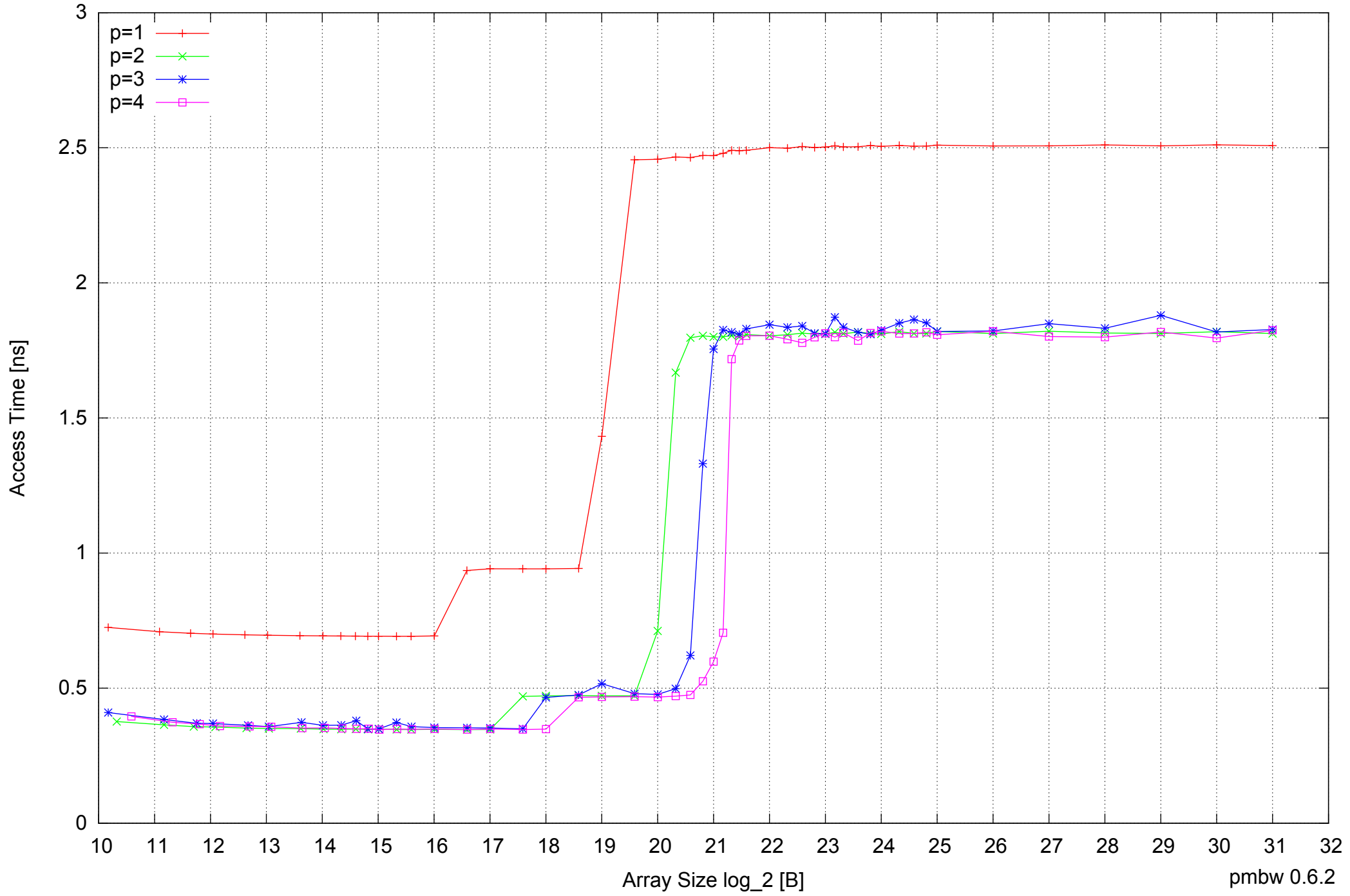
AMD Athlon 64 X2 5600+ 4GB - Parallel Memory Access Time - ScanRead64IndexSimpleLoop
