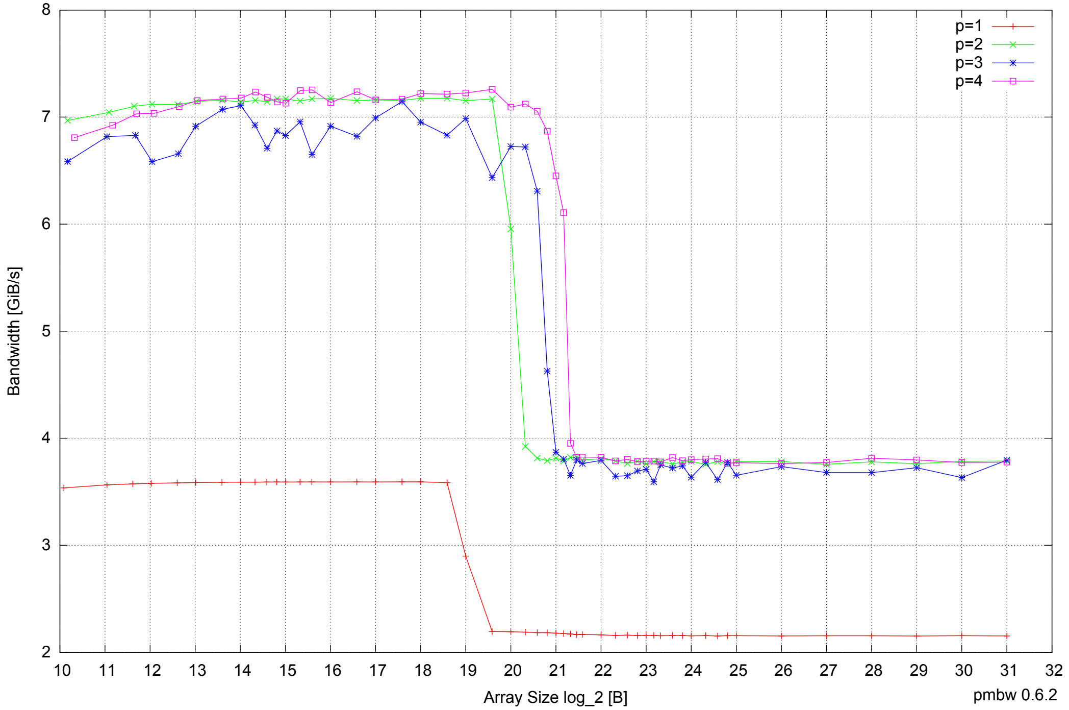
AMD Athlon 64 X2 5600+ 4GB - Parallel Memory Bandwidth - ScanRead32PtrSimpleLoop
