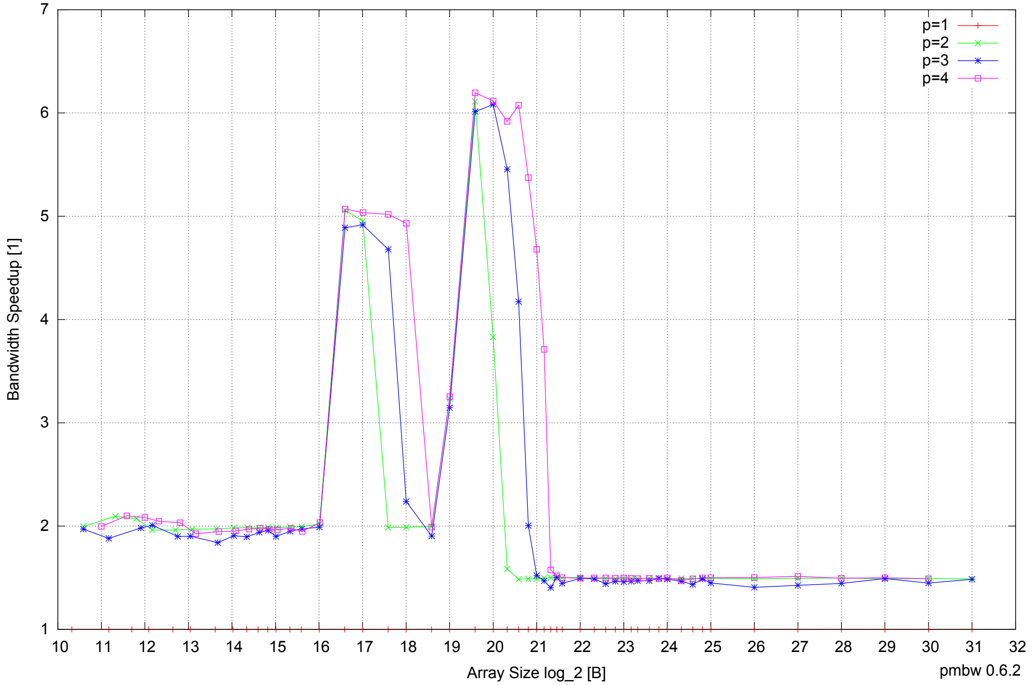
AMD Athlon 64 X2 5600+ 4GB - Speedup of Parallel Memory Bandwidth - ScanRead128PtrUnrollLoop
