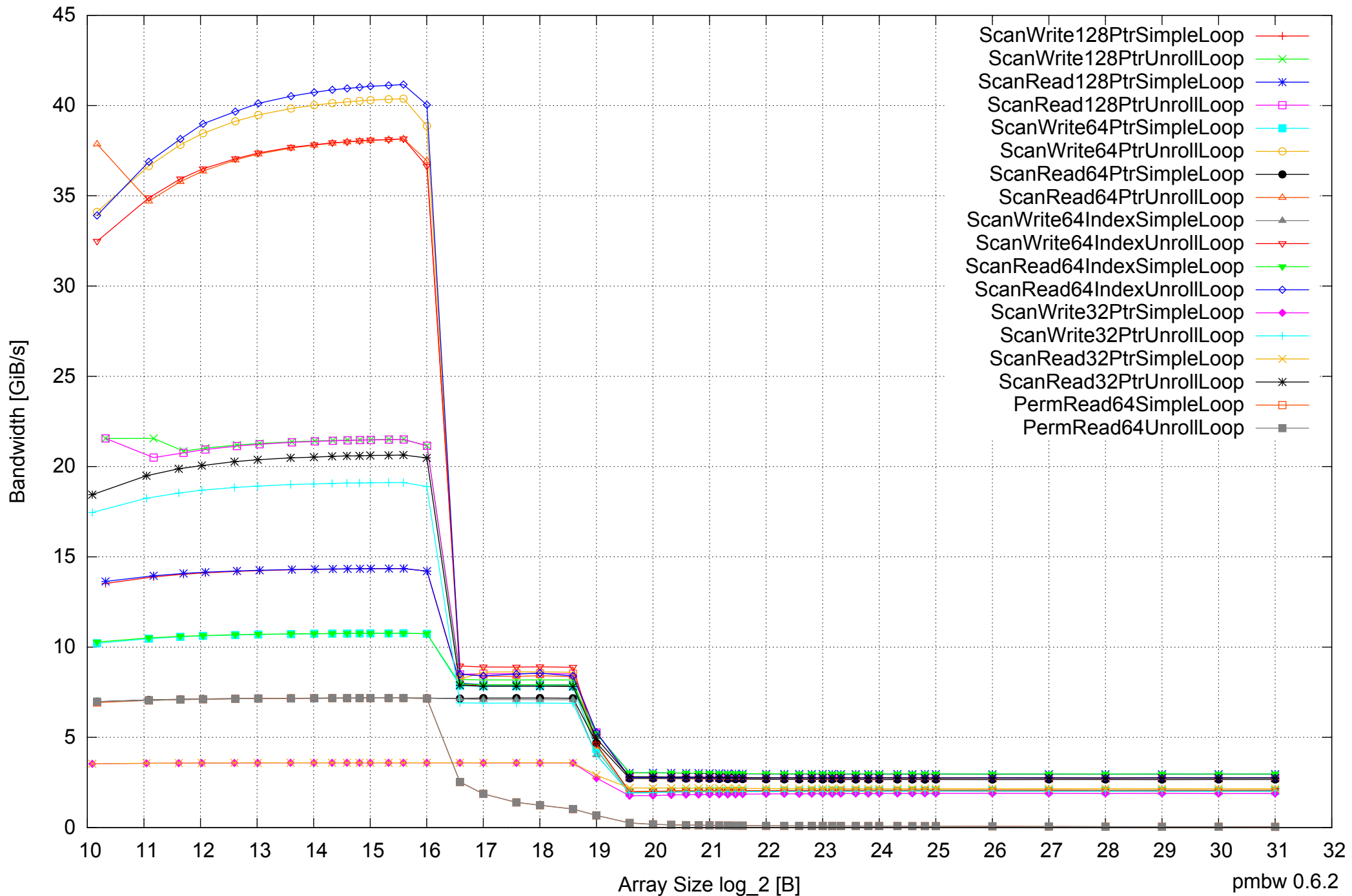
AMD Athlon 64 X2 5600+ 4GB - One Thread Memory Bandwidth
