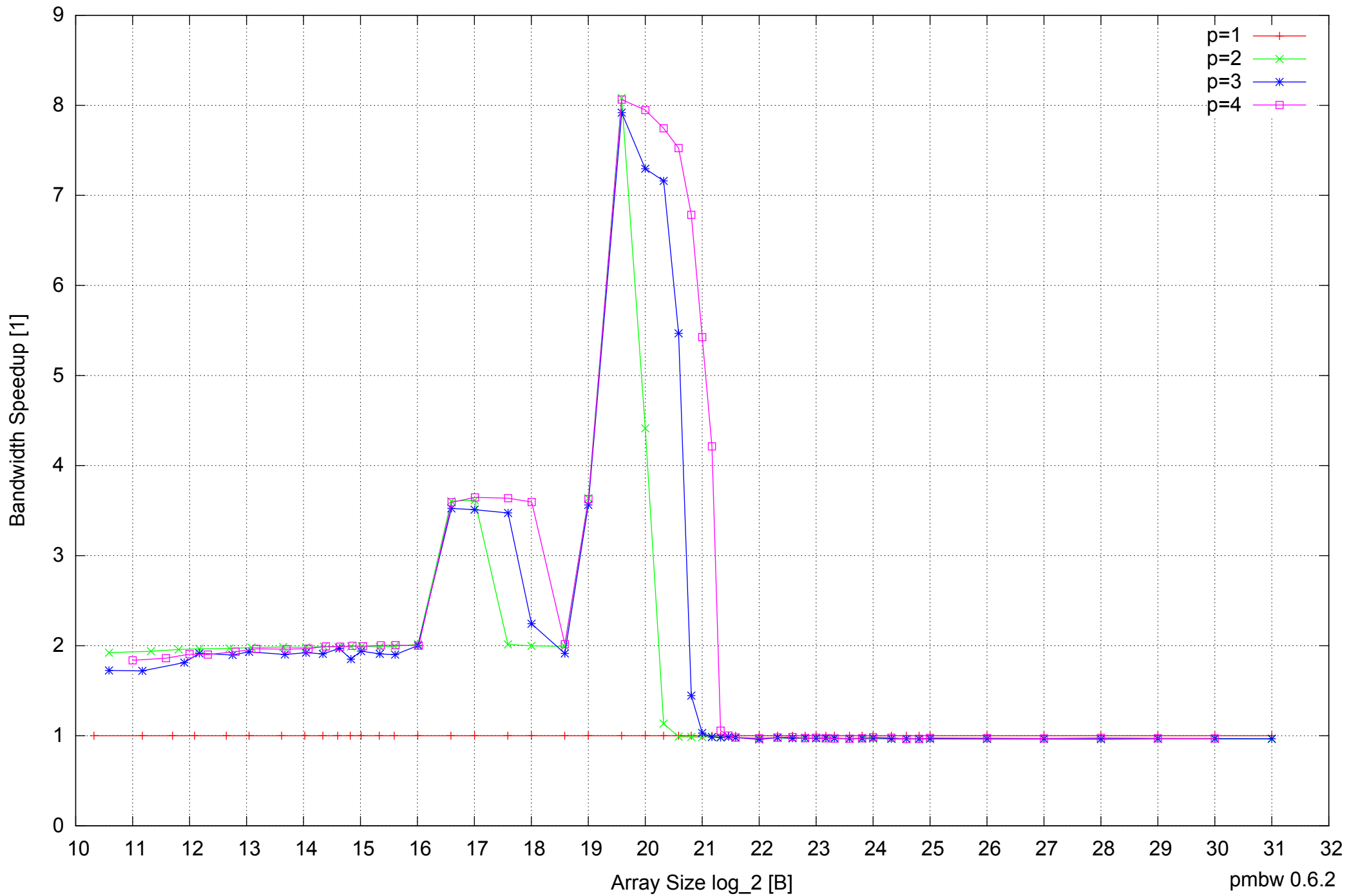
AMD Athlon 64 X2 5600+ 4GB - Speedup of Parallel Memory Bandwidth - ScanWrite128PtrSimpleLoop
