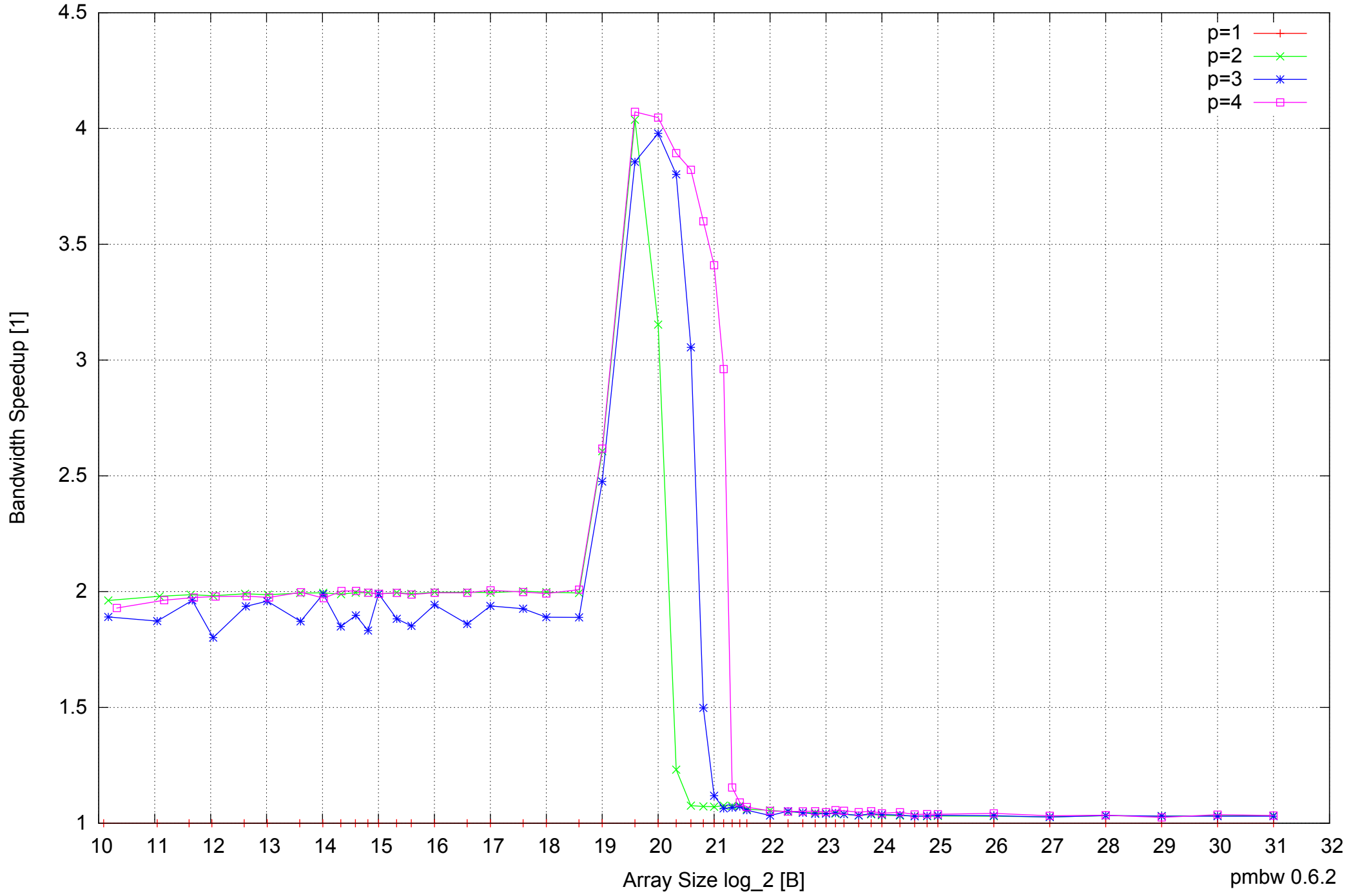
AMD Athlon 64 X2 5600+ 4GB - Speedup of Parallel Memory Bandwidth - ScanWrite32PtrSimpleLoop
