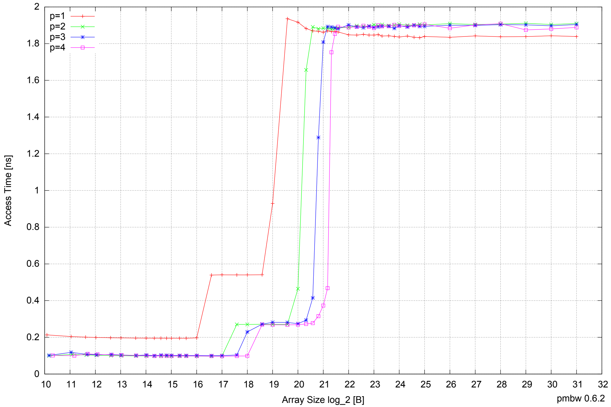
AMD Athlon 64 X2 5600+ 4GB - Parallel Memory Access Time - ScanWrite32PtrUnrollLoop
