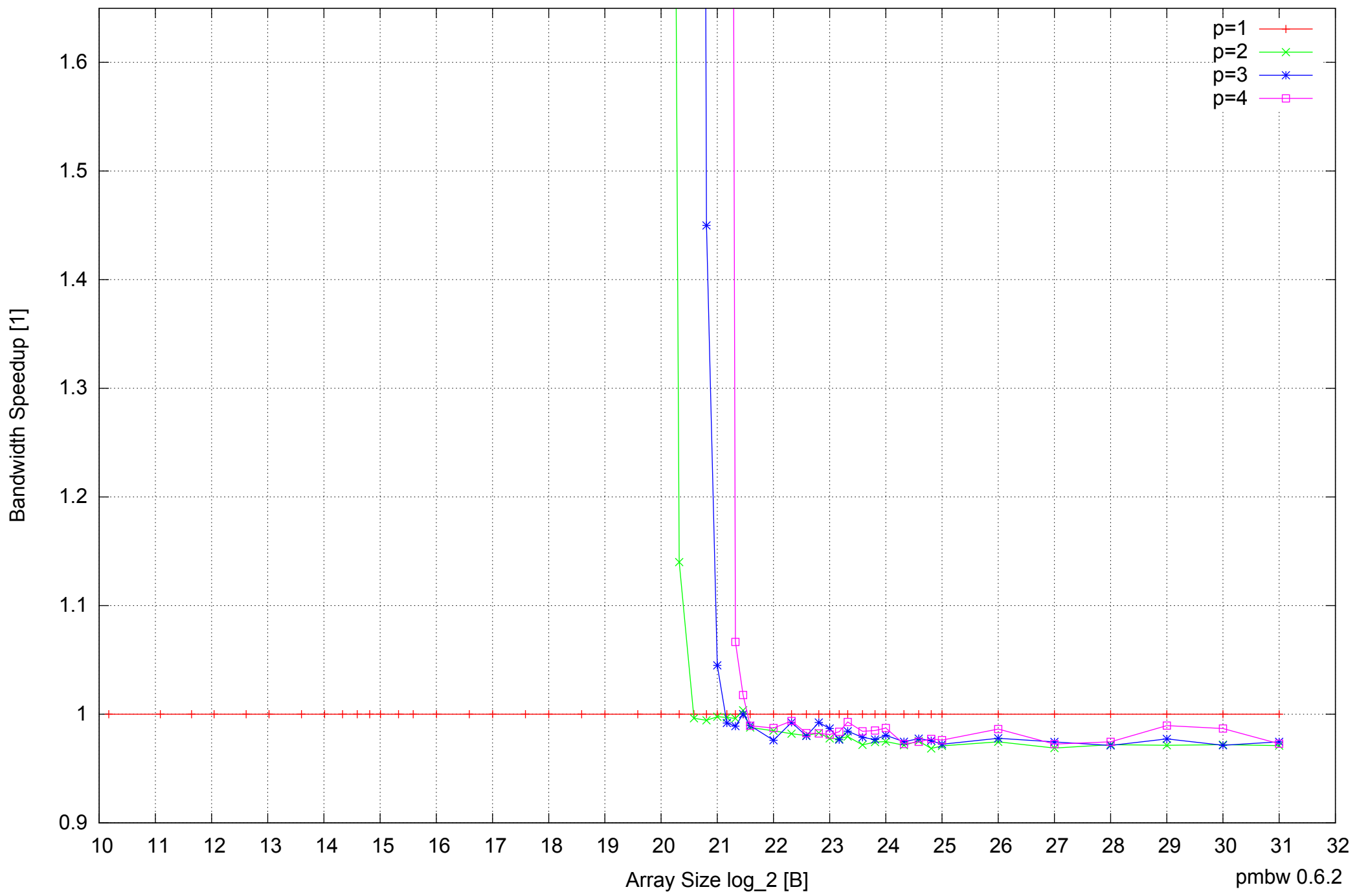
AMD Athlon 64 X2 5600+ 4GB - Speedup of Parallel Memory Bandwidth (enlarged) - ScanWrite64IndexSimpleLoop
