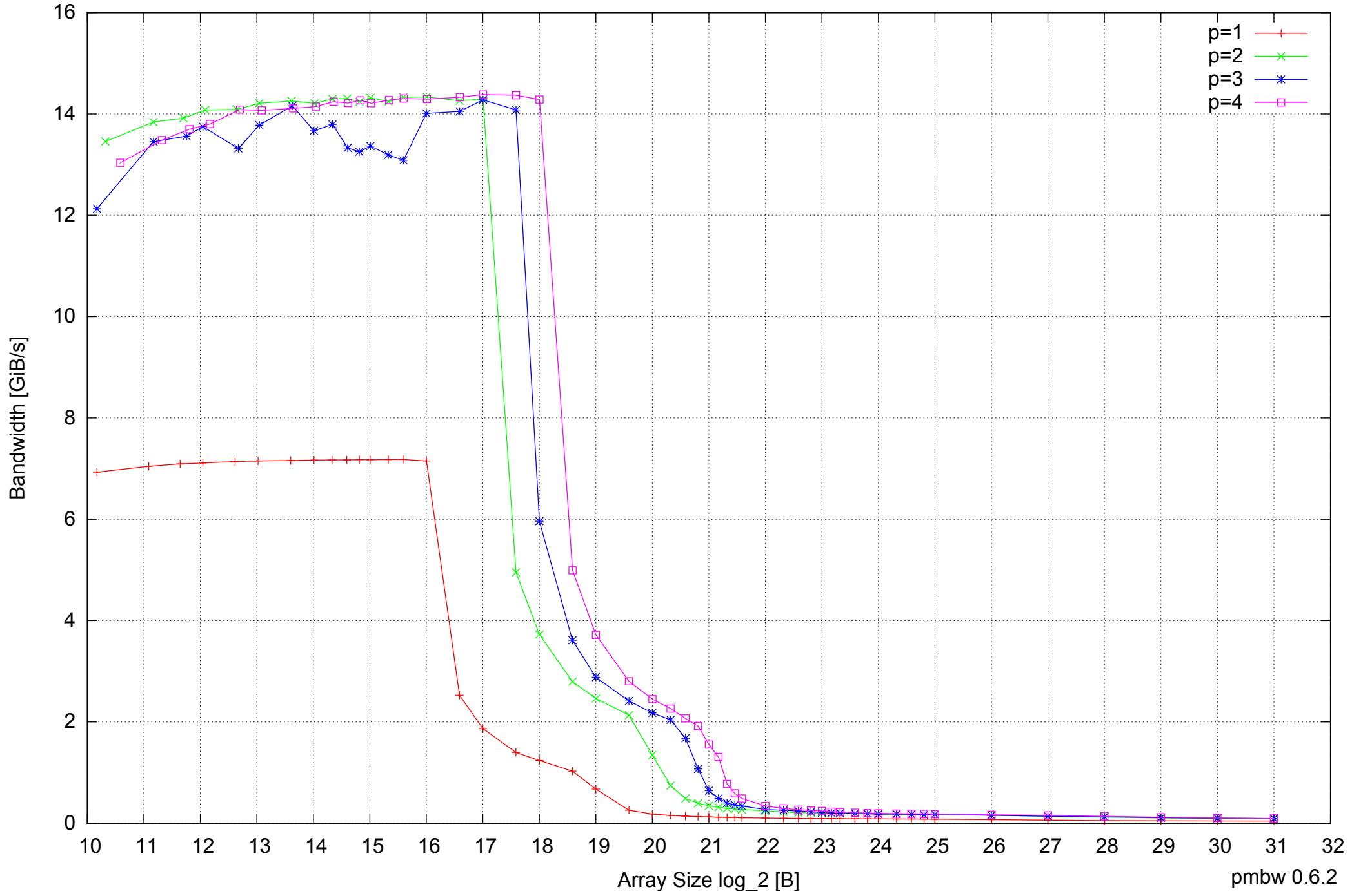
AMD Athlon 64 X2 5600+ 4GB - Parallel Memory Bandwidth - PermRead64SimpleLoop
