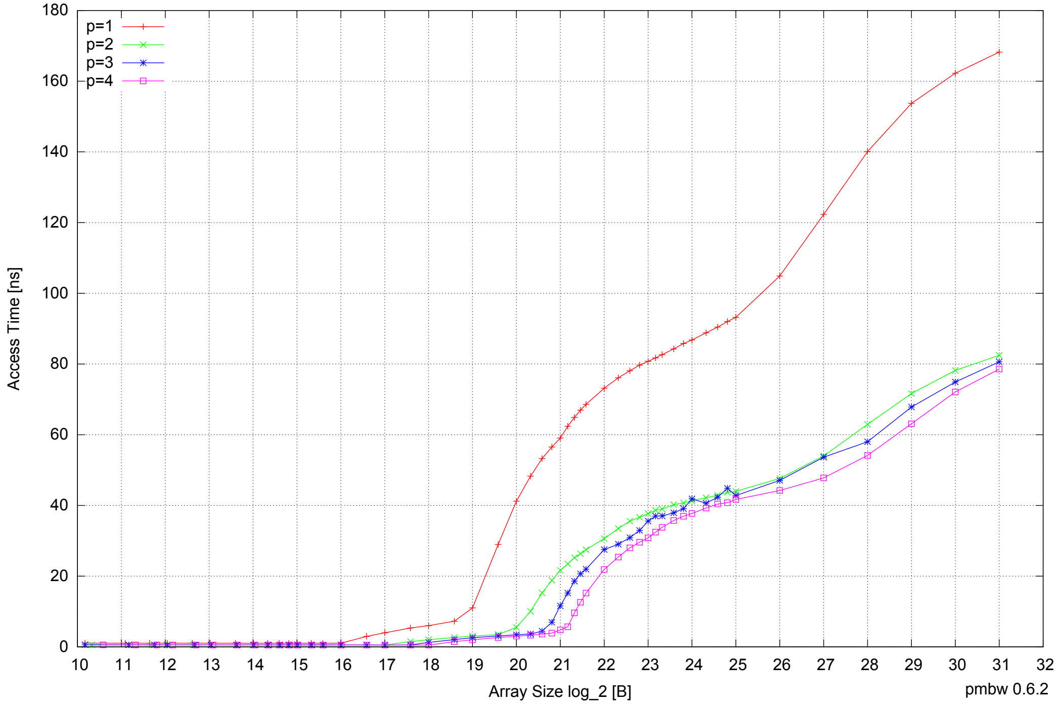
AMD Athlon 64 X2 5600+ 4GB - Parallel Memory Access Time - PermRead64SimpleLoop
