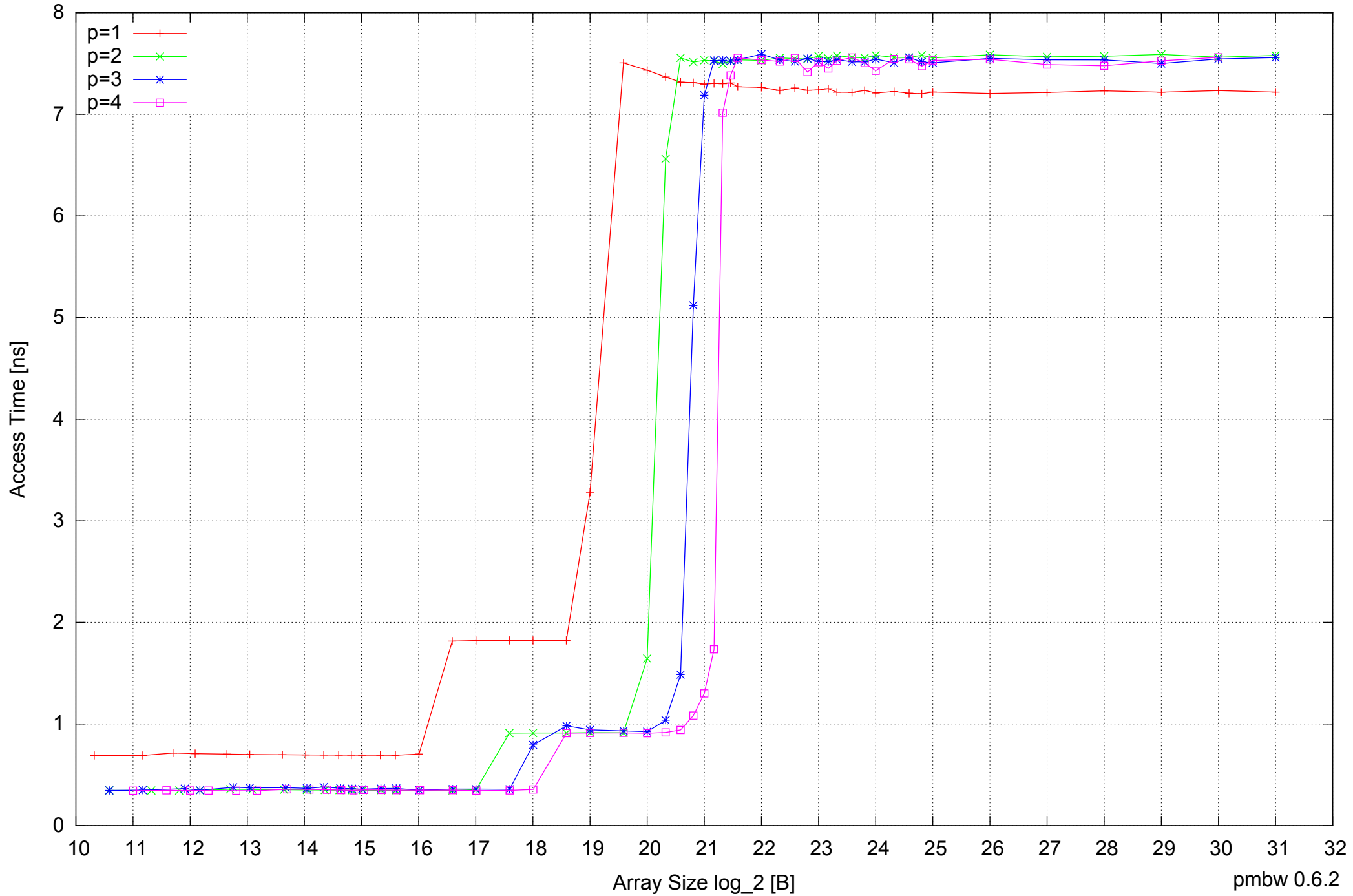
AMD Athlon 64 X2 5600+ 4GB - Parallel Memory Access Time - ScanWrite128PtrUnrollLoop
