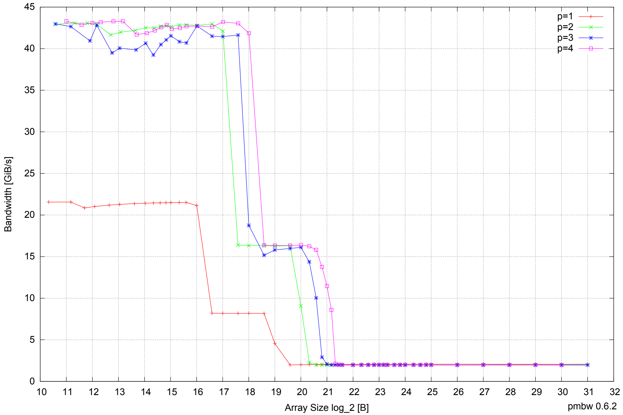
AMD Athlon 64 X2 5600+ 4GB - Parallel Memory Bandwidth - ScanWrite128PtrUnrollLoop
