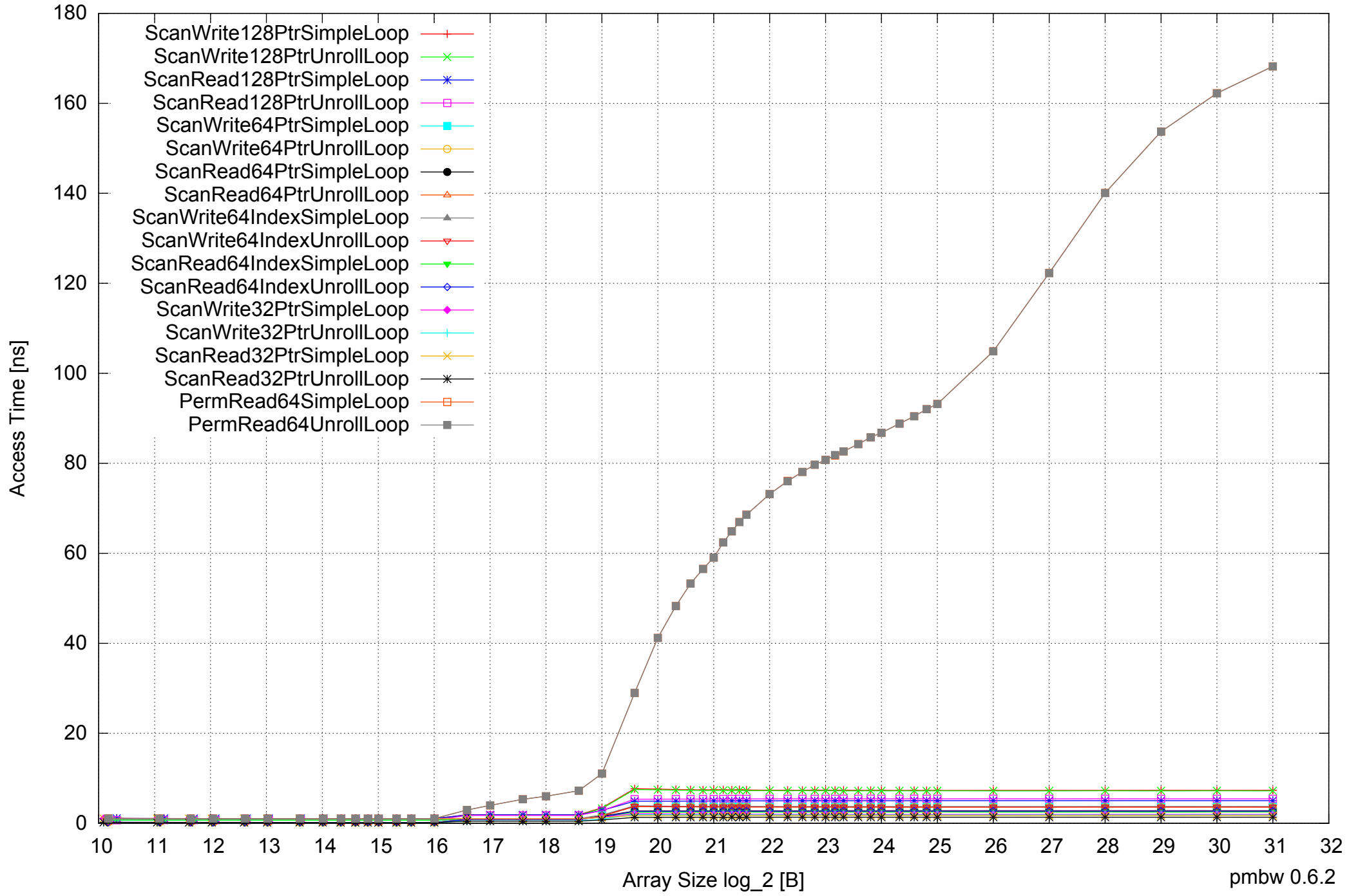
AMD Athlon 64 X2 5600+ 4GB - One Thread Memory Latency (Access Time)
