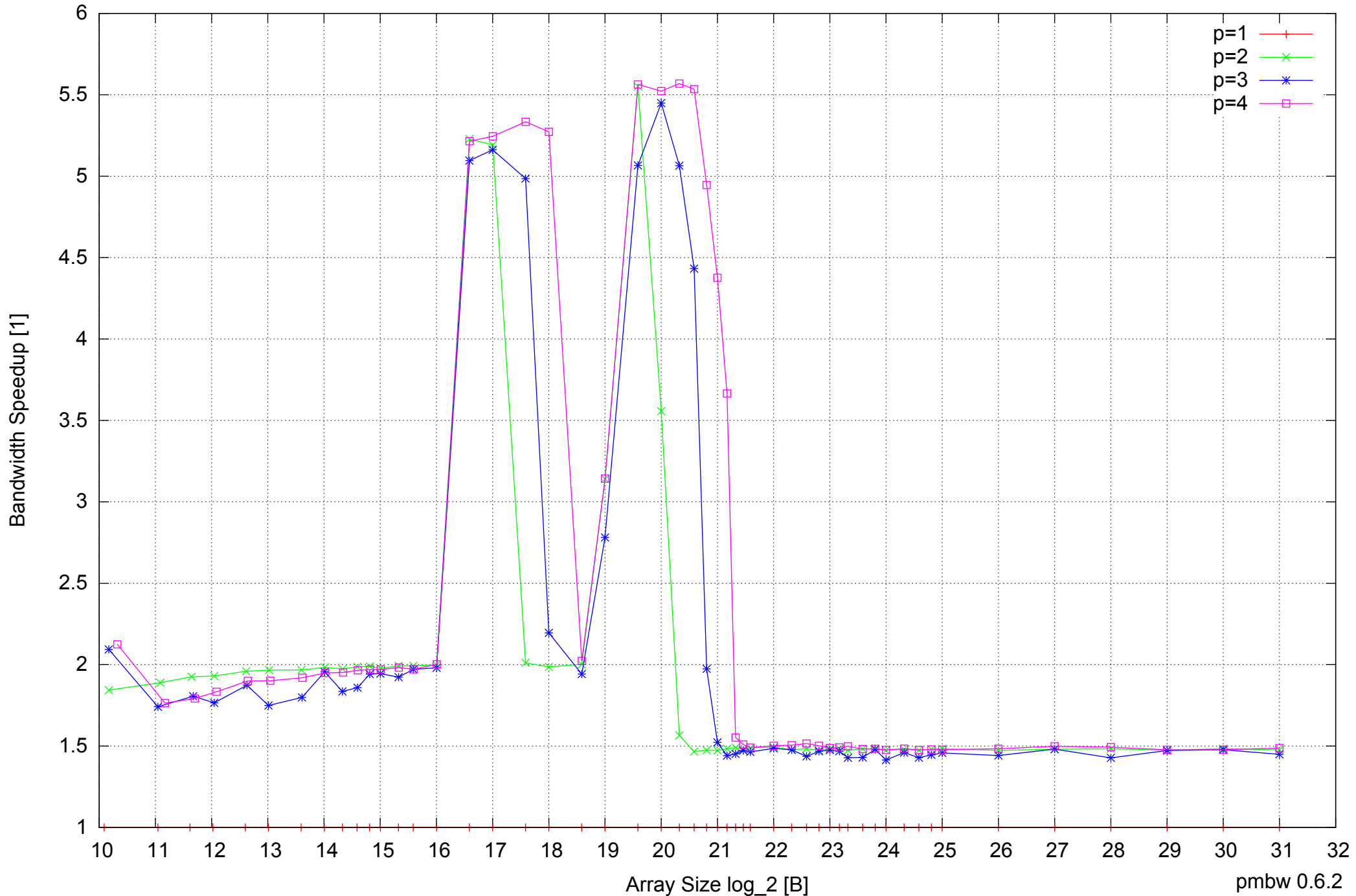
AMD Athlon 64 X2 5600+ 4GB - Speedup of Parallel Memory Bandwidth - ScanRead32PtrUnrollLoop
