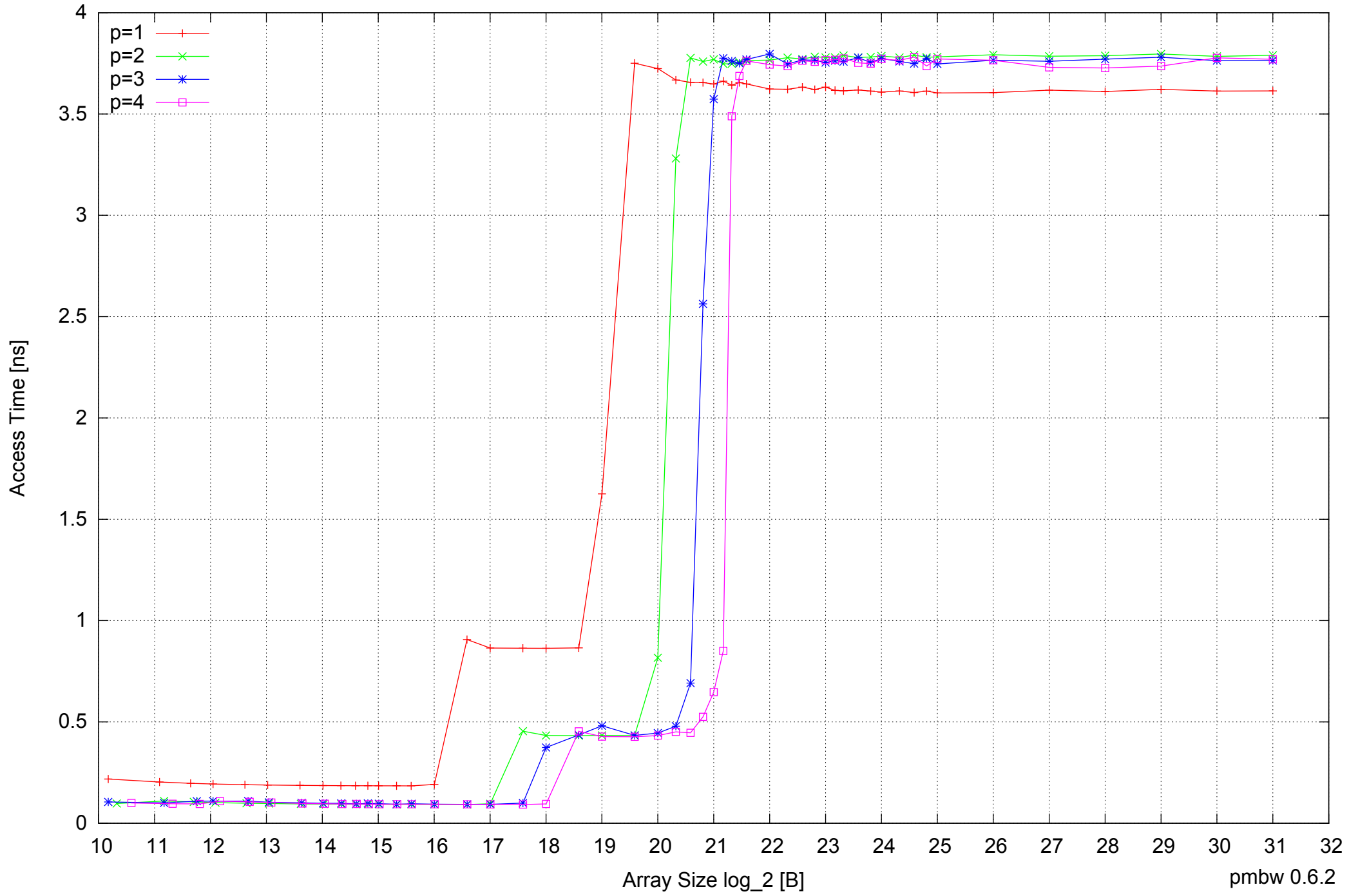
AMD Athlon 64 X2 5600+ 4GB - Parallel Memory Access Time - ScanWrite64PtrUnrollLoop
