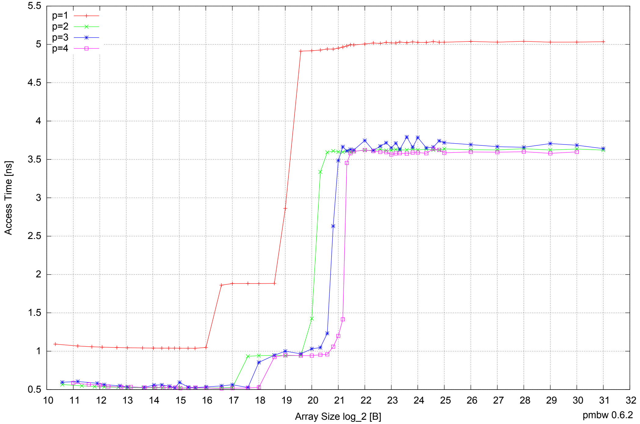
AMD Athlon 64 X2 5600+ 4GB - Parallel Memory Access Time - ScanRead128PtrSimpleLoop
