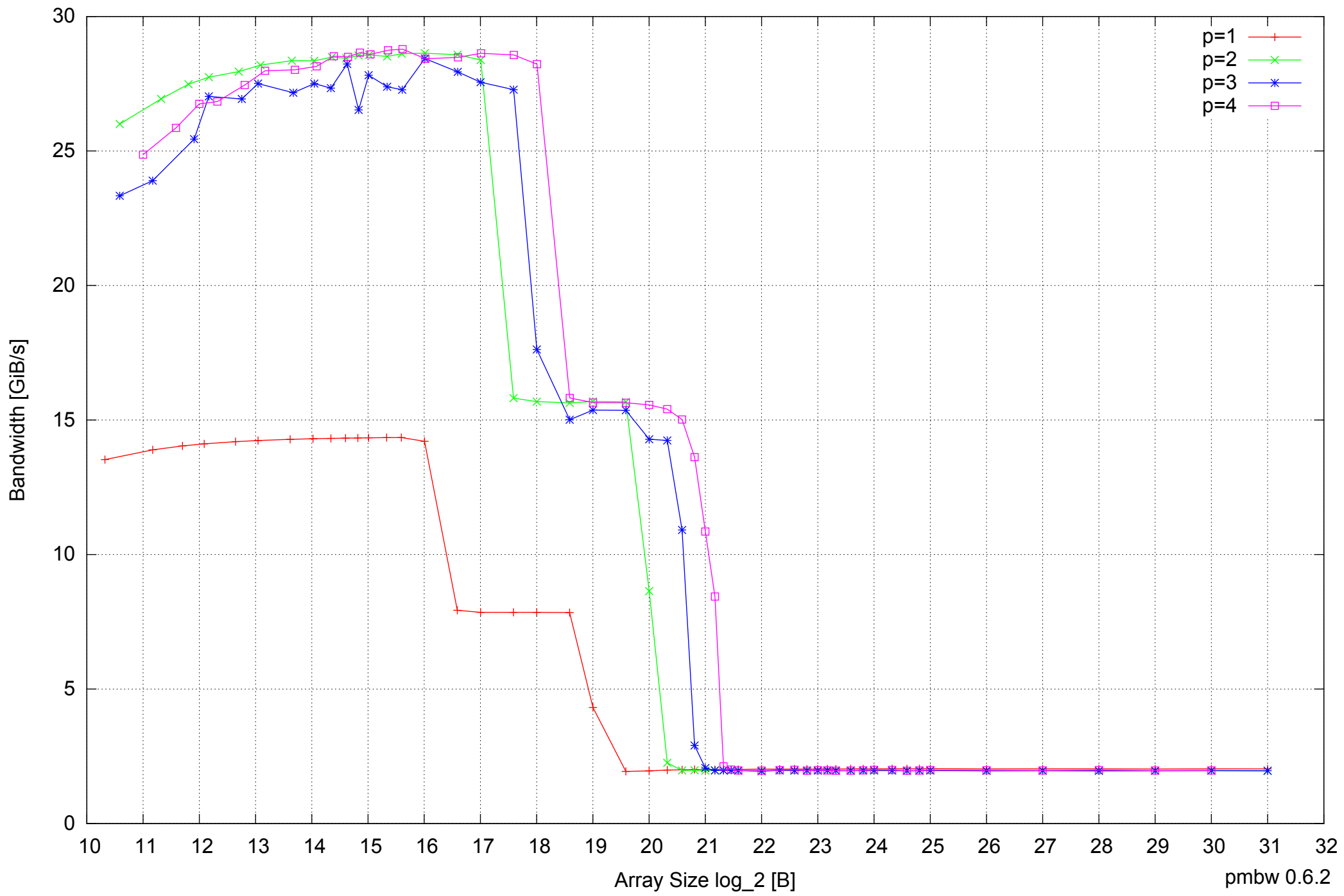
AMD Athlon 64 X2 5600+ 4GB - Parallel Memory Bandwidth - ScanWrite128PtrSimpleLoop
