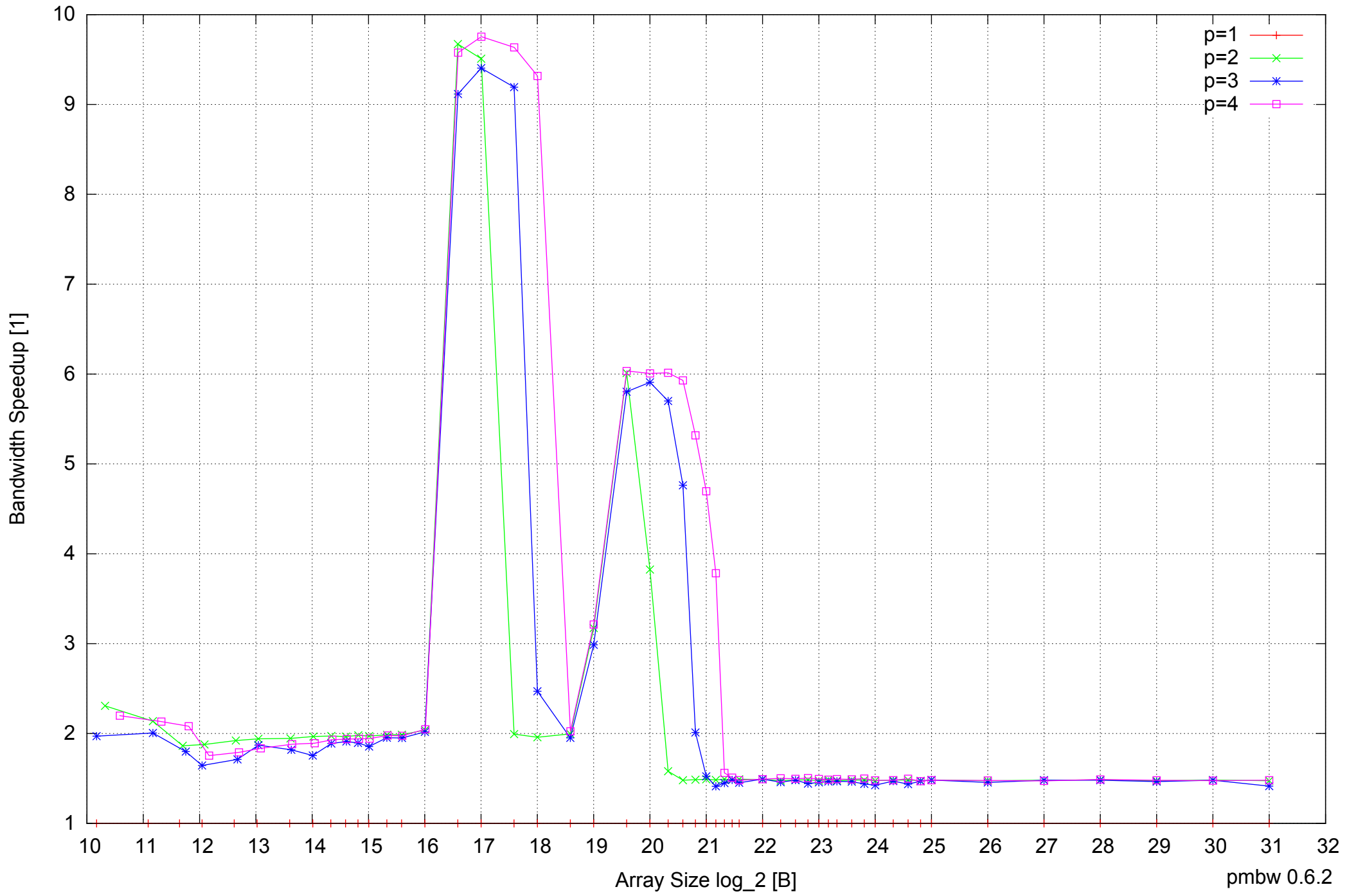
AMD Athlon 64 X2 5600+ 4GB - Speedup of Parallel Memory Bandwidth - ScanRead64IndexUnrollLoop
