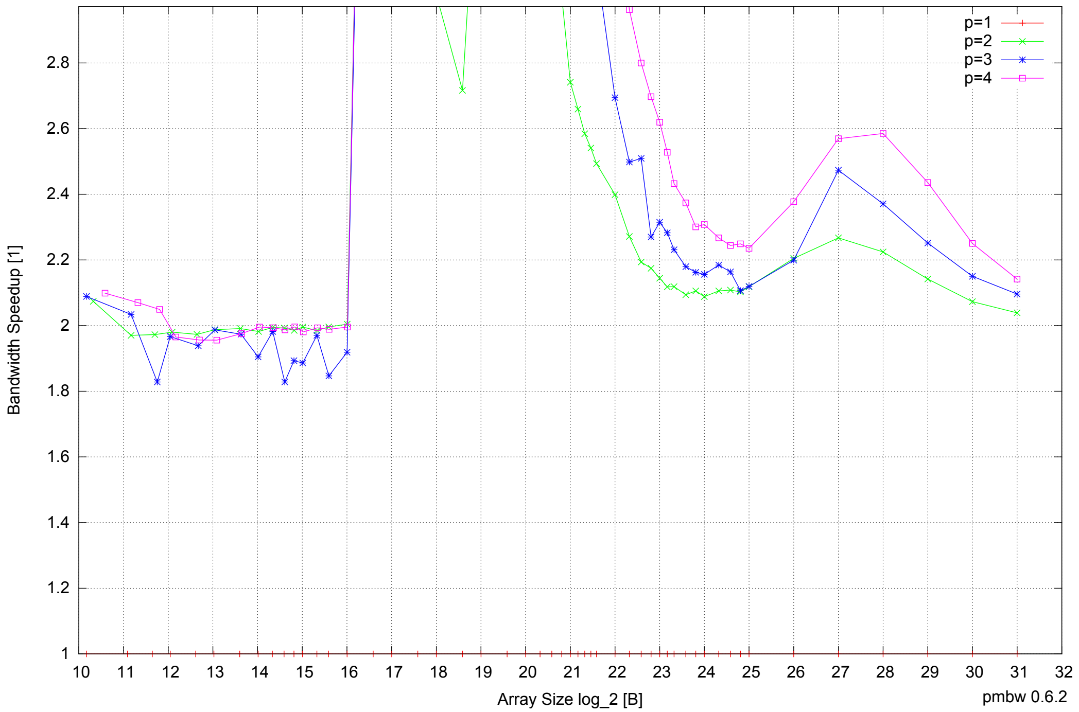
AMD Athlon 64 X2 5600+ 4GB - Speedup of Parallel Memory Bandwidth (enlarged) - PermRead64UnrollLoop
