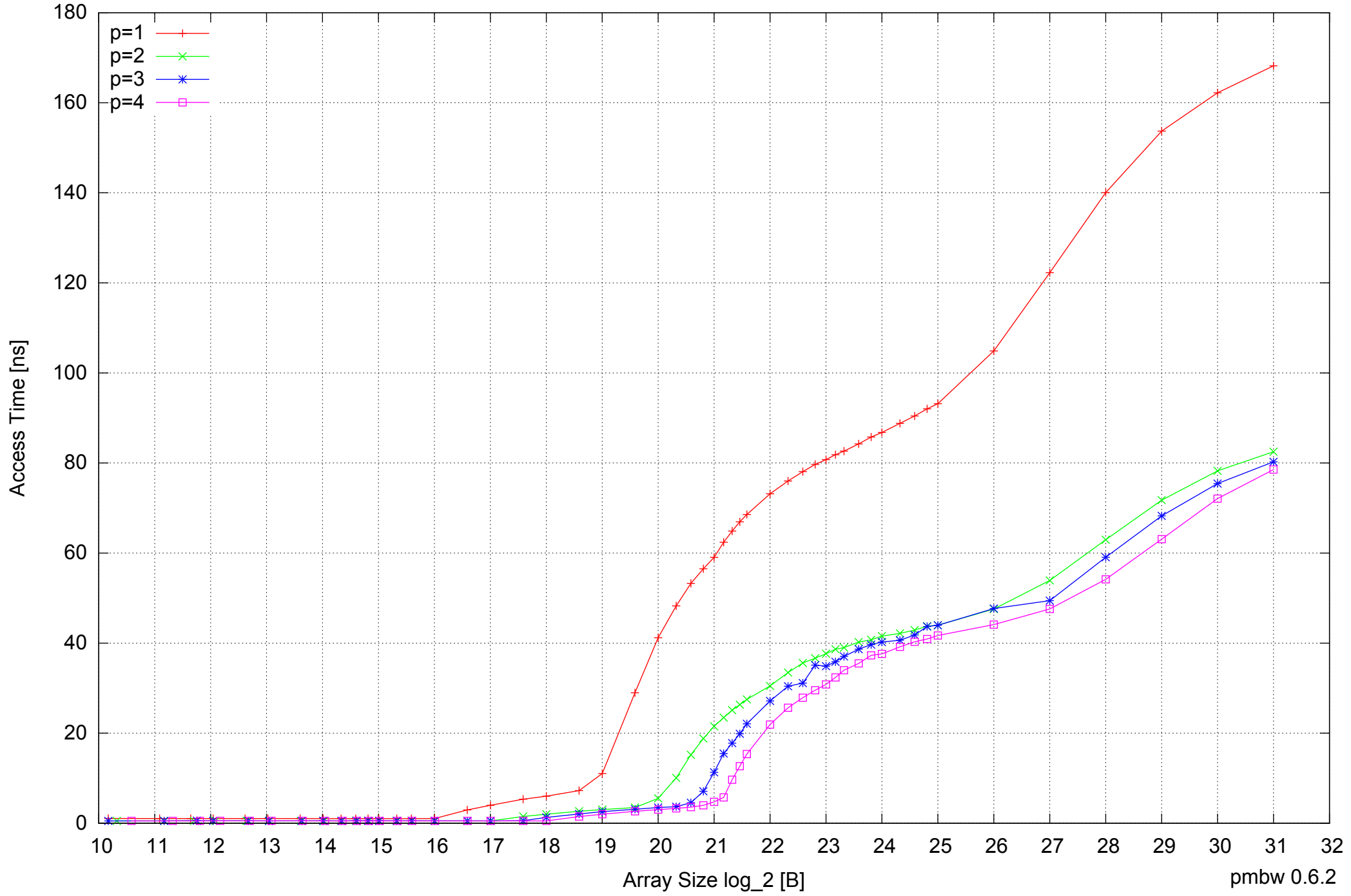
AMD Athlon 64 X2 5600+ 4GB - Parallel Memory Access Time - PermRead64UnrollLoop
