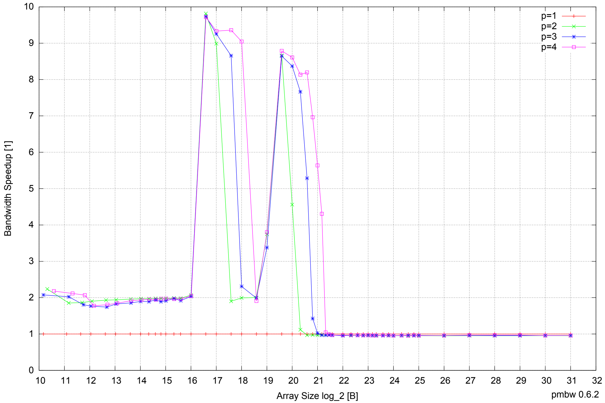
AMD Athlon 64 X2 5600+ 4GB - Speedup of Parallel Memory Bandwidth - ScanWrite64PtrUnrollLoop
