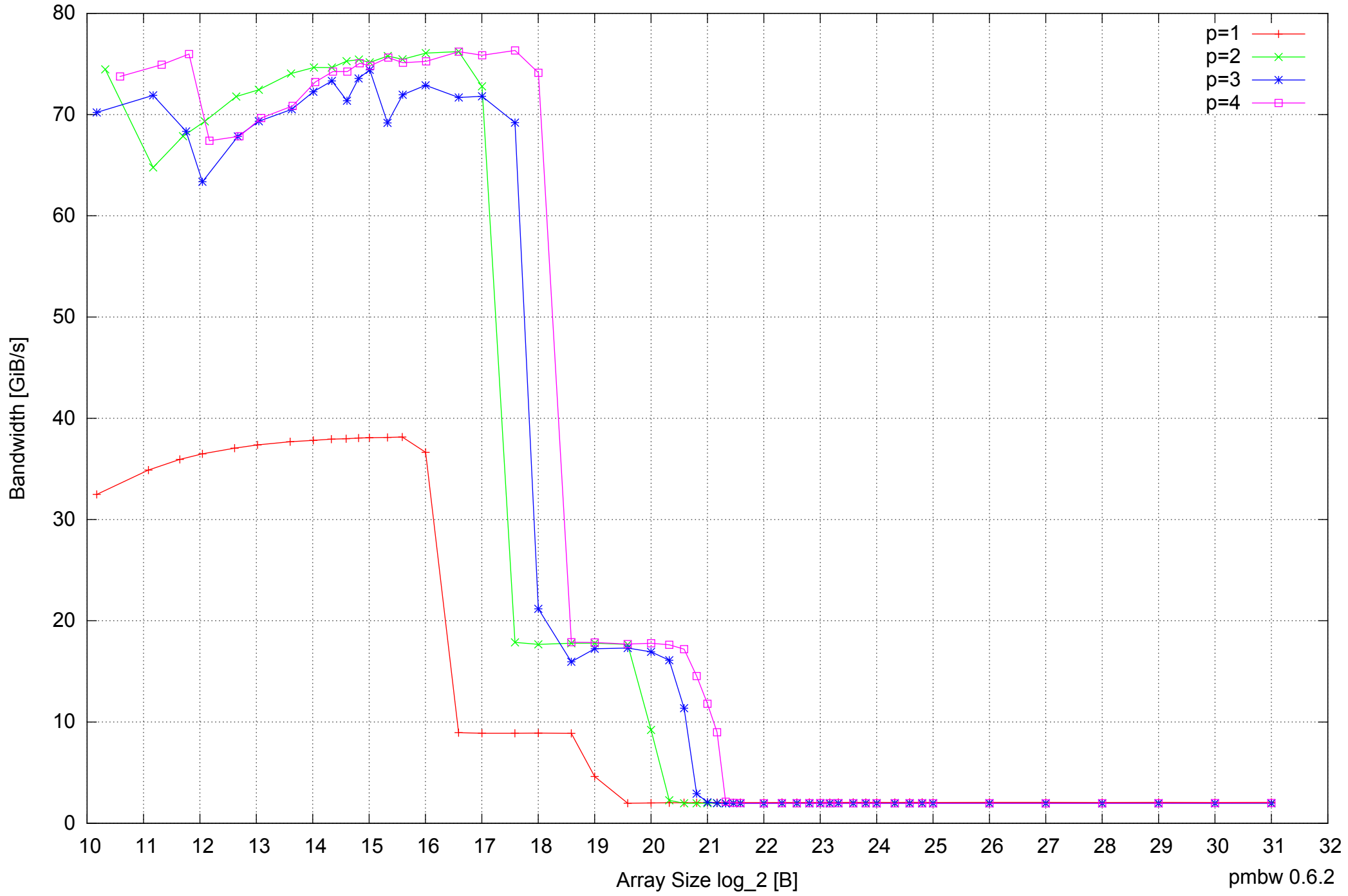
AMD Athlon 64 X2 5600+ 4GB - Parallel Memory Bandwidth - ScanWrite64IndexUnrollLoop
