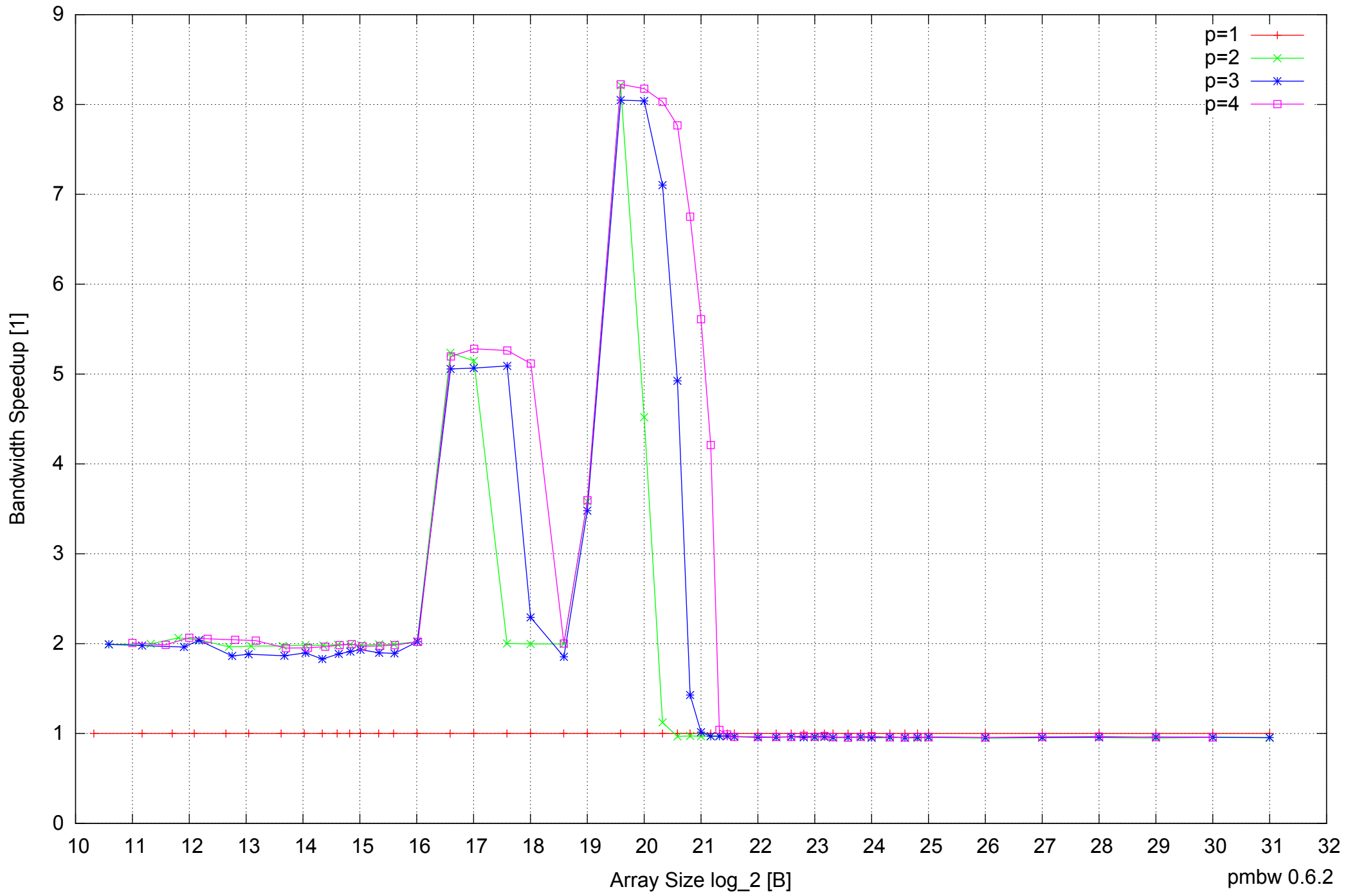
AMD Athlon 64 X2 5600+ 4GB - Speedup of Parallel Memory Bandwidth - ScanWrite128PtrUnrollLoop
