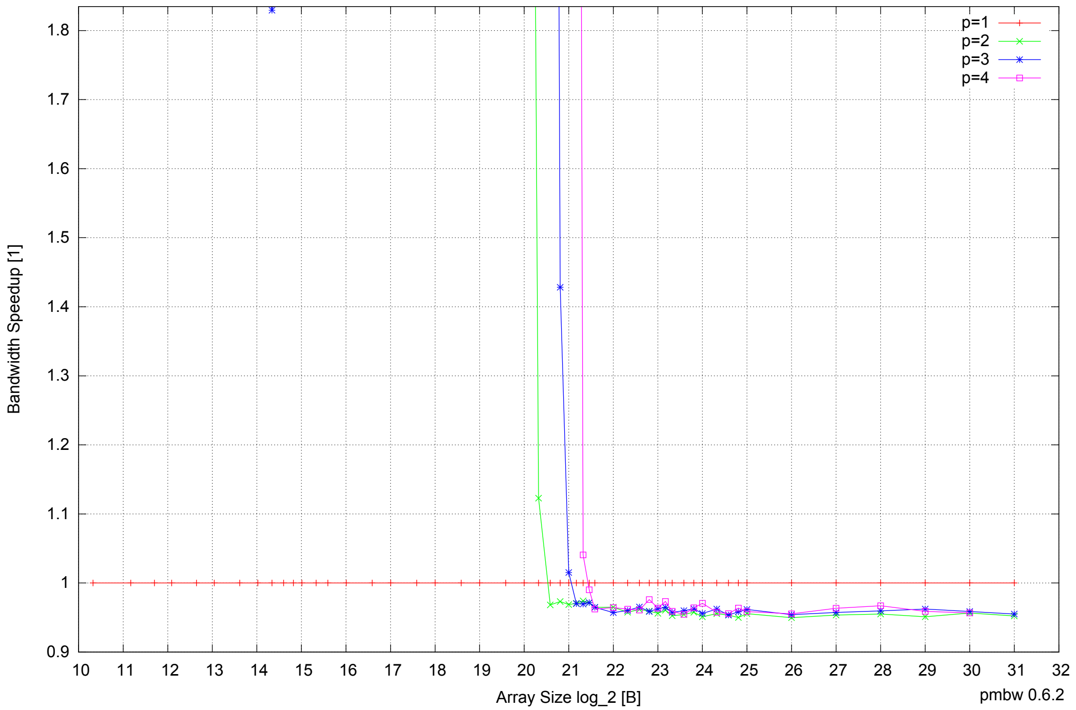
AMD Athlon 64 X2 5600+ 4GB - Speedup of Parallel Memory Bandwidth (enlarged) - ScanWrite128PtrUnrollLoop
