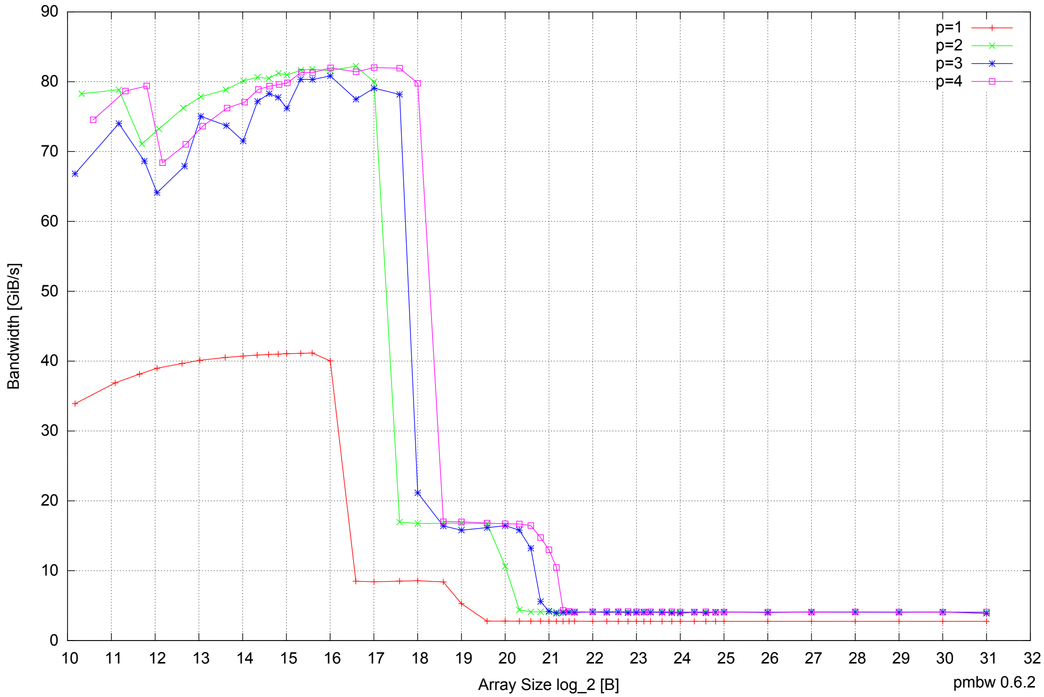
AMD Athlon 64 X2 5600+ 4GB - Parallel Memory Bandwidth - ScanRead64IndexUnrollLoop
