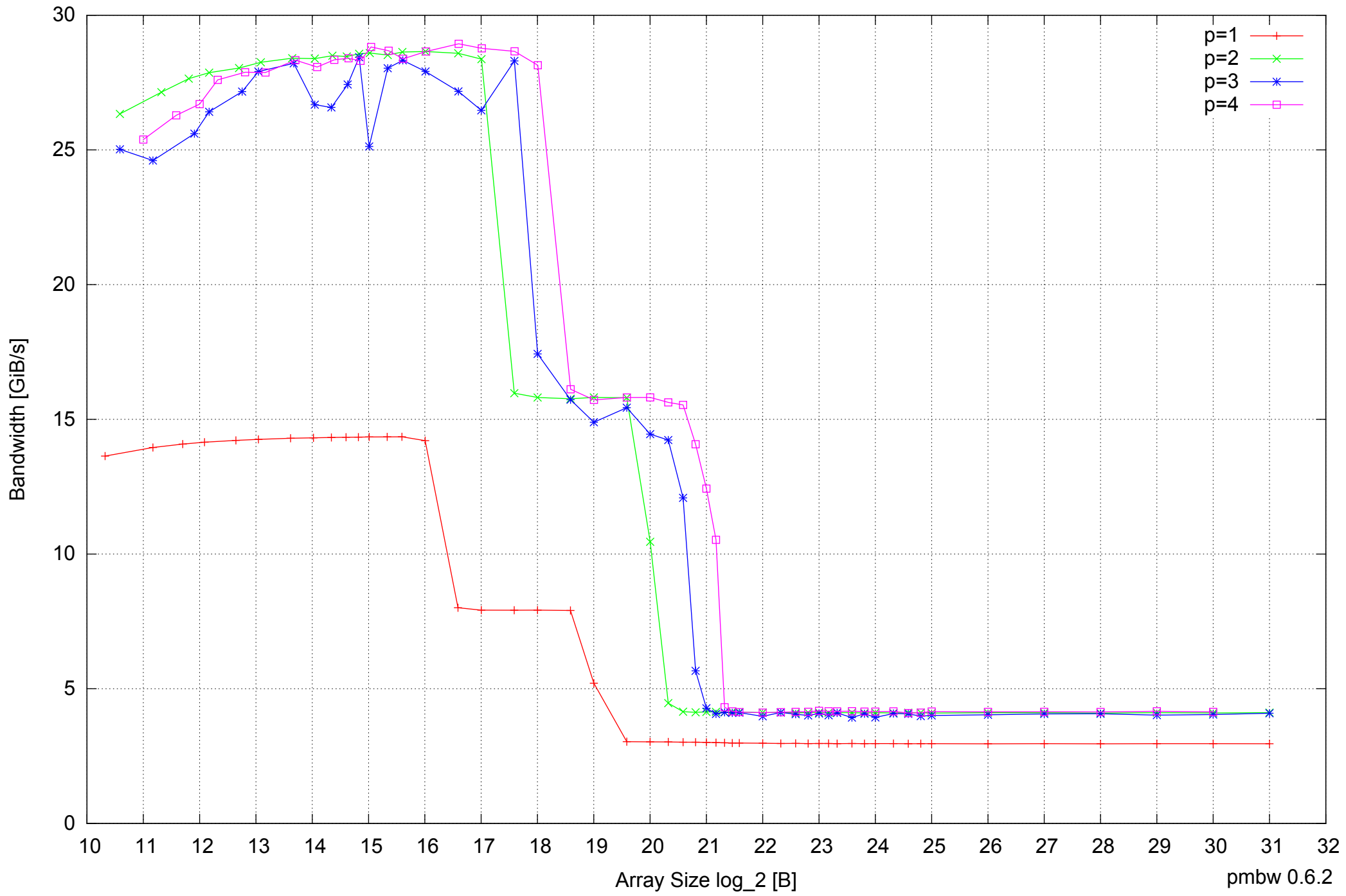
AMD Athlon 64 X2 5600+ 4GB - Parallel Memory Bandwidth - ScanRead128PtrSimpleLoop
