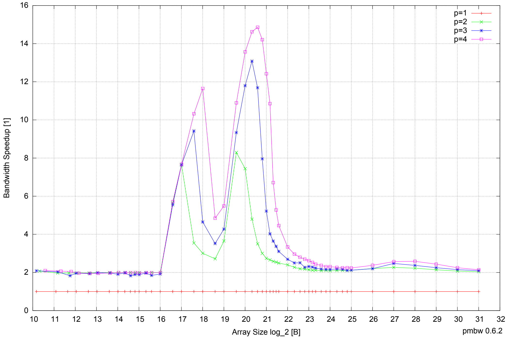
AMD Athlon 64 X2 5600+ 4GB - Speedup of Parallel Memory Bandwidth - PermRead64UnrollLoop
