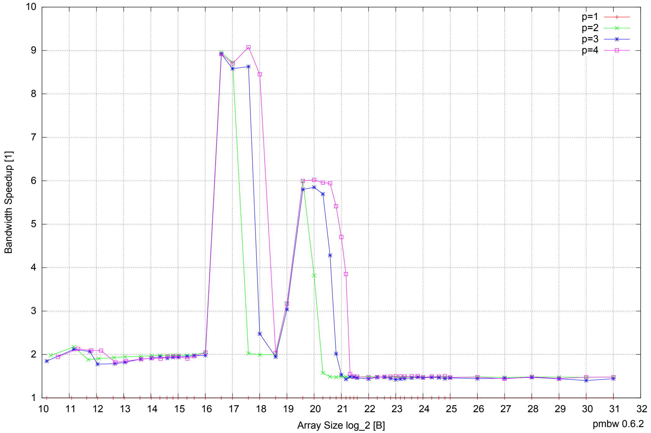
AMD Athlon 64 X2 5600+ 4GB - Speedup of Parallel Memory Bandwidth - ScanRead64PtrUnrollLoop
