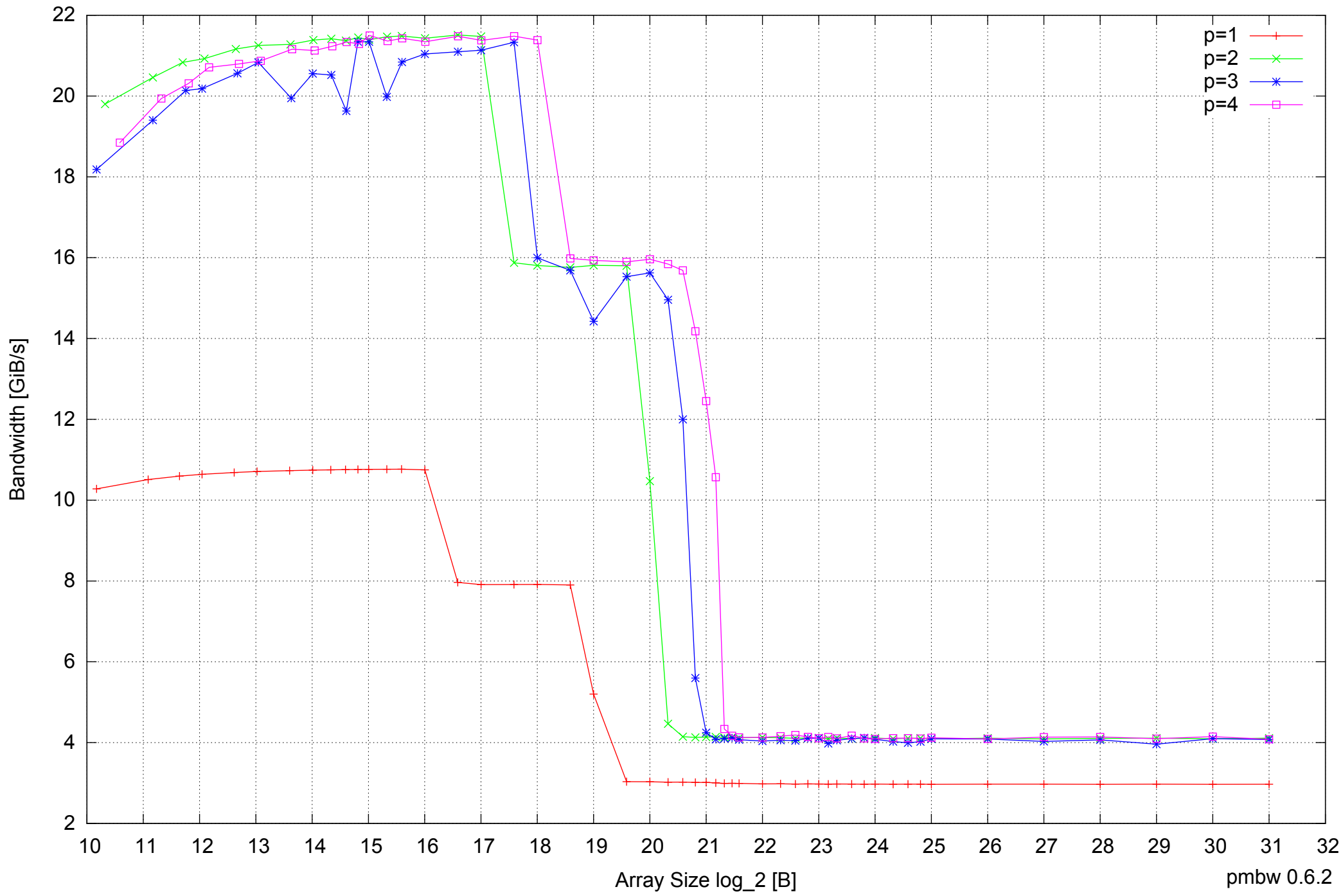
AMD Athlon 64 X2 5600+ 4GB - Parallel Memory Bandwidth - ScanRead64IndexSimpleLoop
