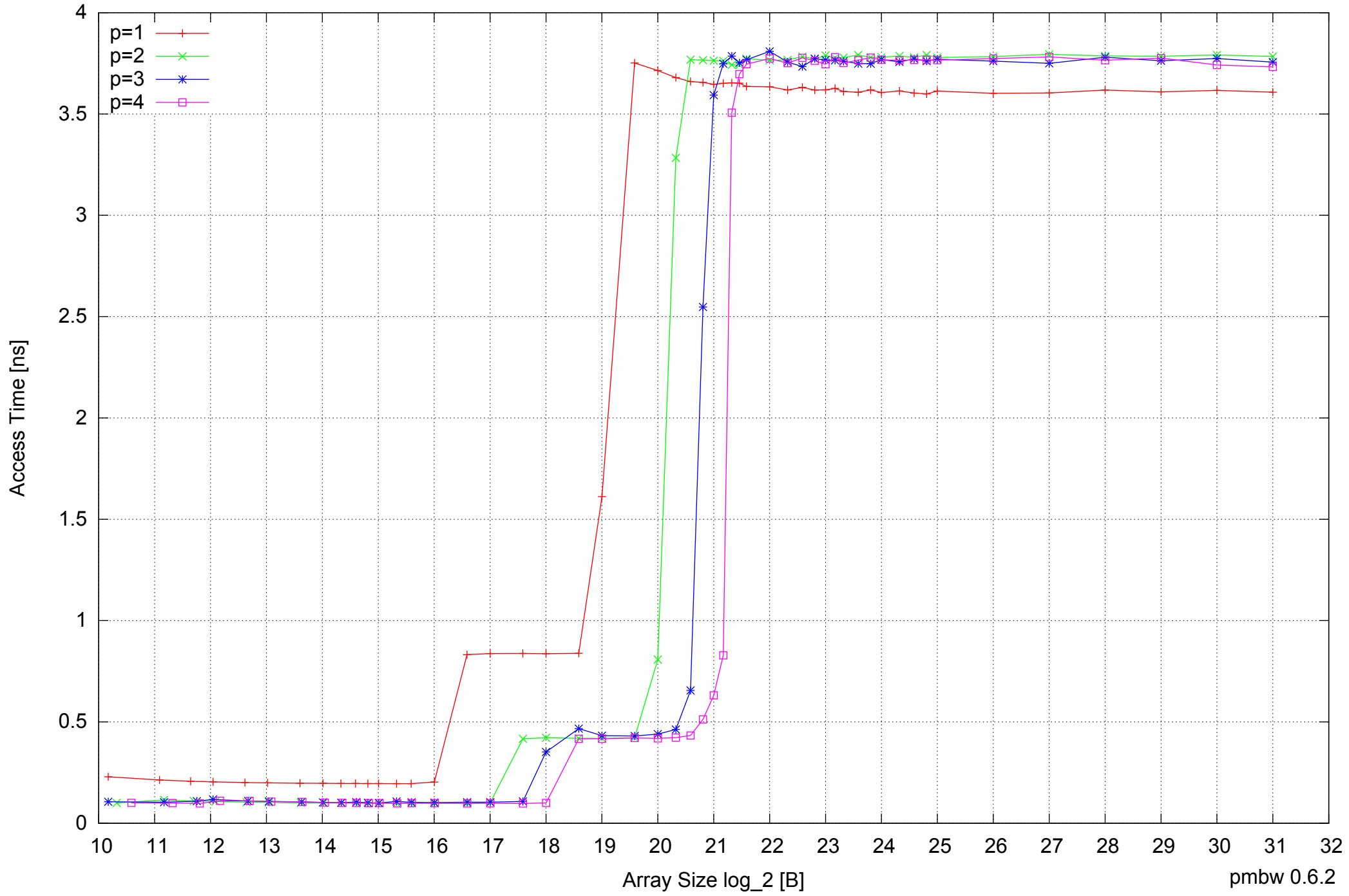
AMD Athlon 64 X2 5600+ 4GB - Parallel Memory Access Time - ScanWrite64IndexUnrollLoop
