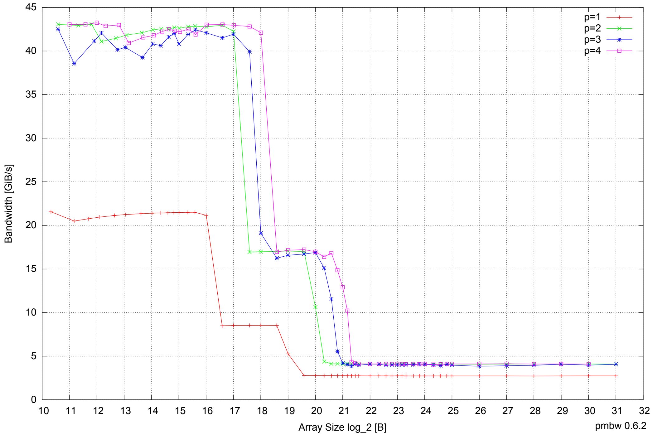
AMD Athlon 64 X2 5600+ 4GB - Parallel Memory Bandwidth - ScanRead128PtrUnrollLoop
