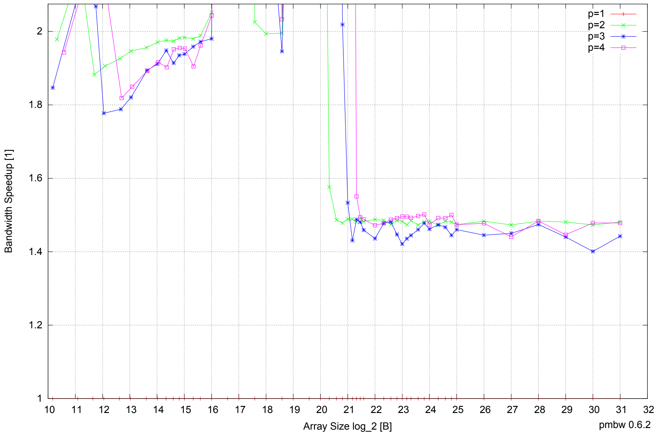
AMD Athlon 64 X2 5600+ 4GB - Speedup of Parallel Memory Bandwidth (enlarged) - ScanRead64PtrUnrollLoop
