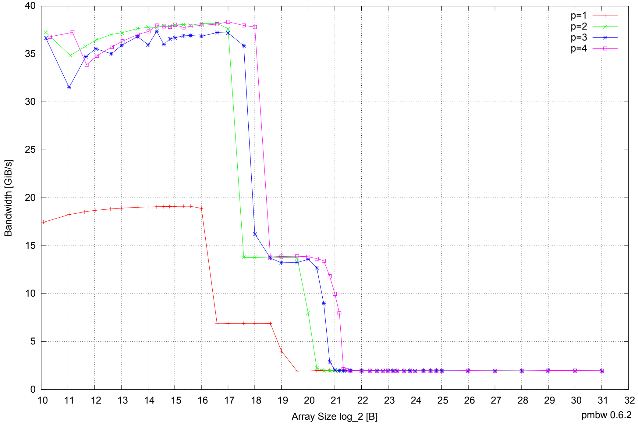
AMD Athlon 64 X2 5600+ 4GB - Parallel Memory Bandwidth - ScanWrite32PtrUnrollLoop
