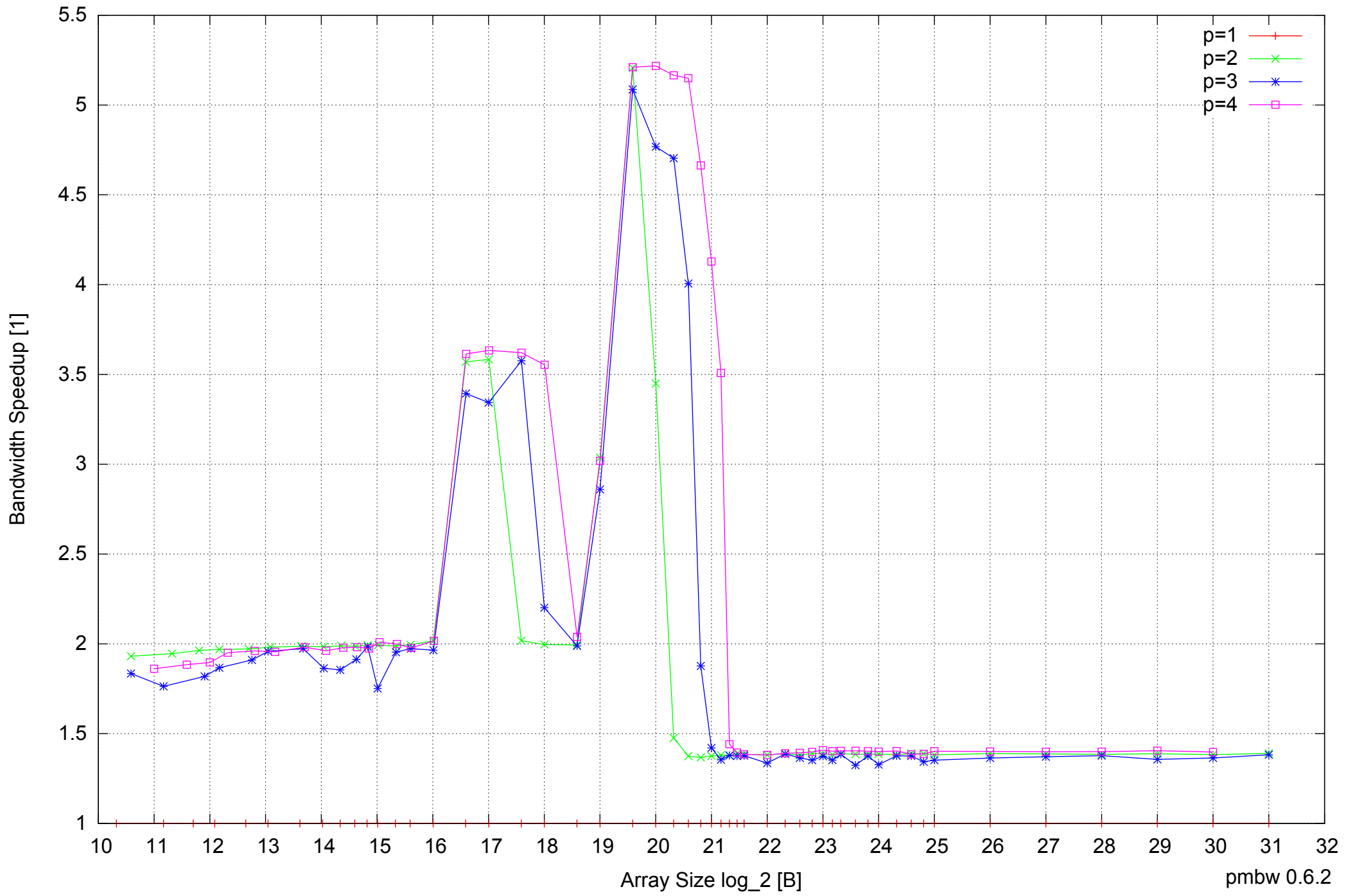
AMD Athlon 64 X2 5600+ 4GB - Speedup of Parallel Memory Bandwidth - ScanRead128PtrSimpleLoop
