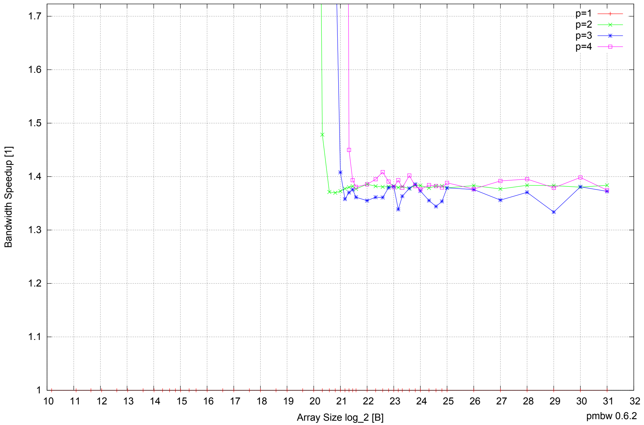
AMD Athlon 64 X2 5600+ 4GB - Speedup of Parallel Memory Bandwidth (enlarged) - ScanRead64IndexSimpleLoop
