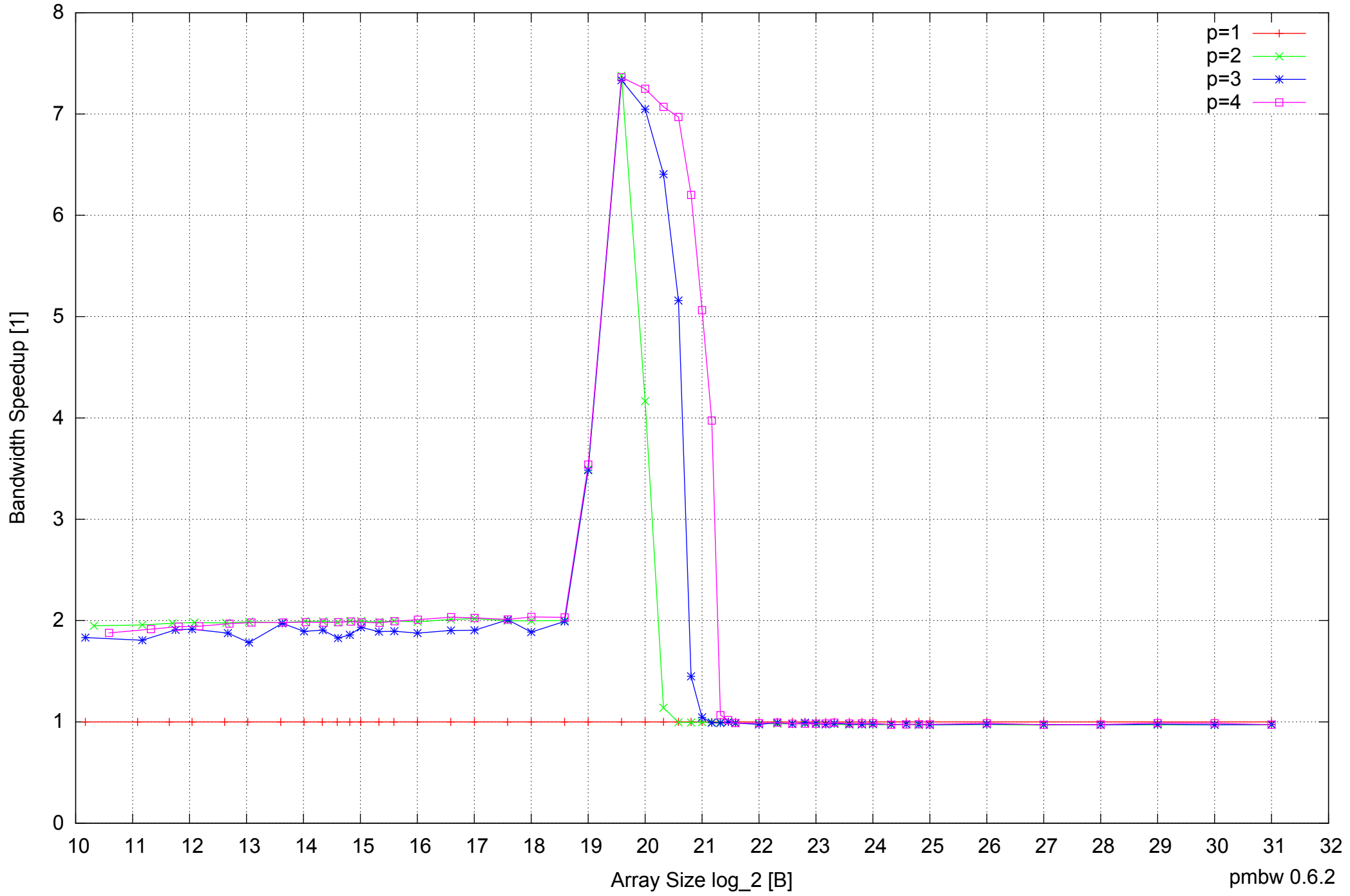
AMD Athlon 64 X2 5600+ 4GB - Speedup of Parallel Memory Bandwidth - ScanWrite64IndexSimpleLoop
