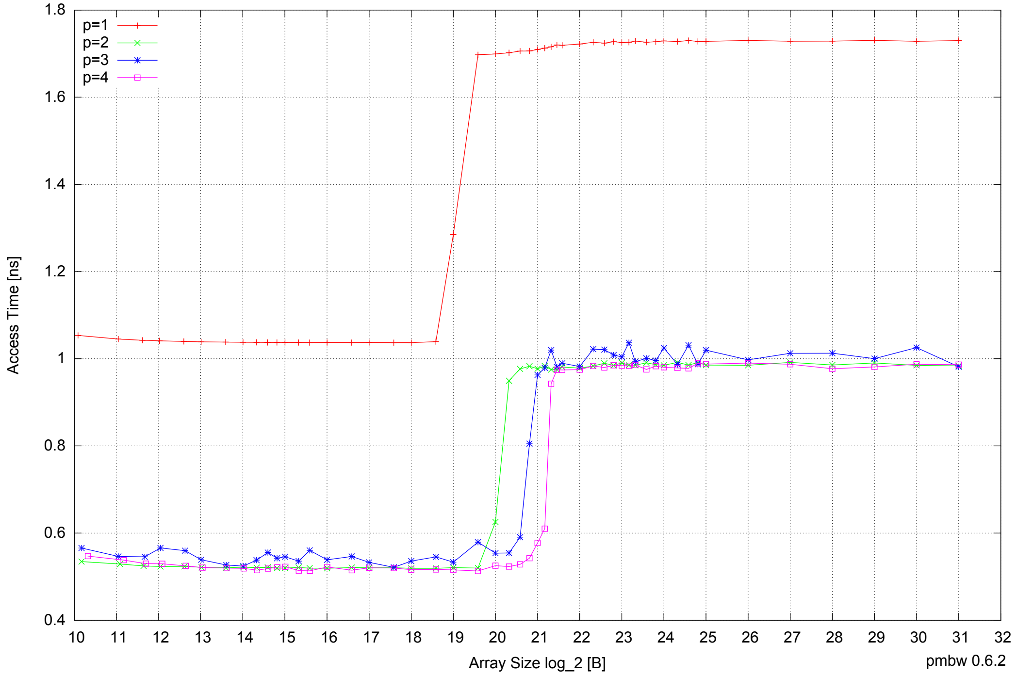
AMD Athlon 64 X2 5600+ 4GB - Parallel Memory Access Time - ScanRead32PtrSimpleLoop
