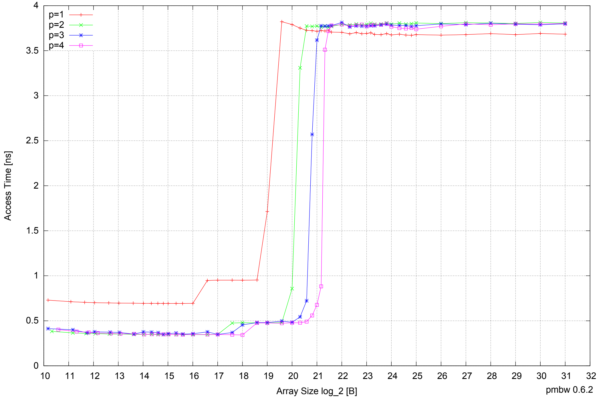
AMD Athlon 64 X2 5600+ 4GB - Parallel Memory Access Time - ScanWrite64PtrSimpleLoop
