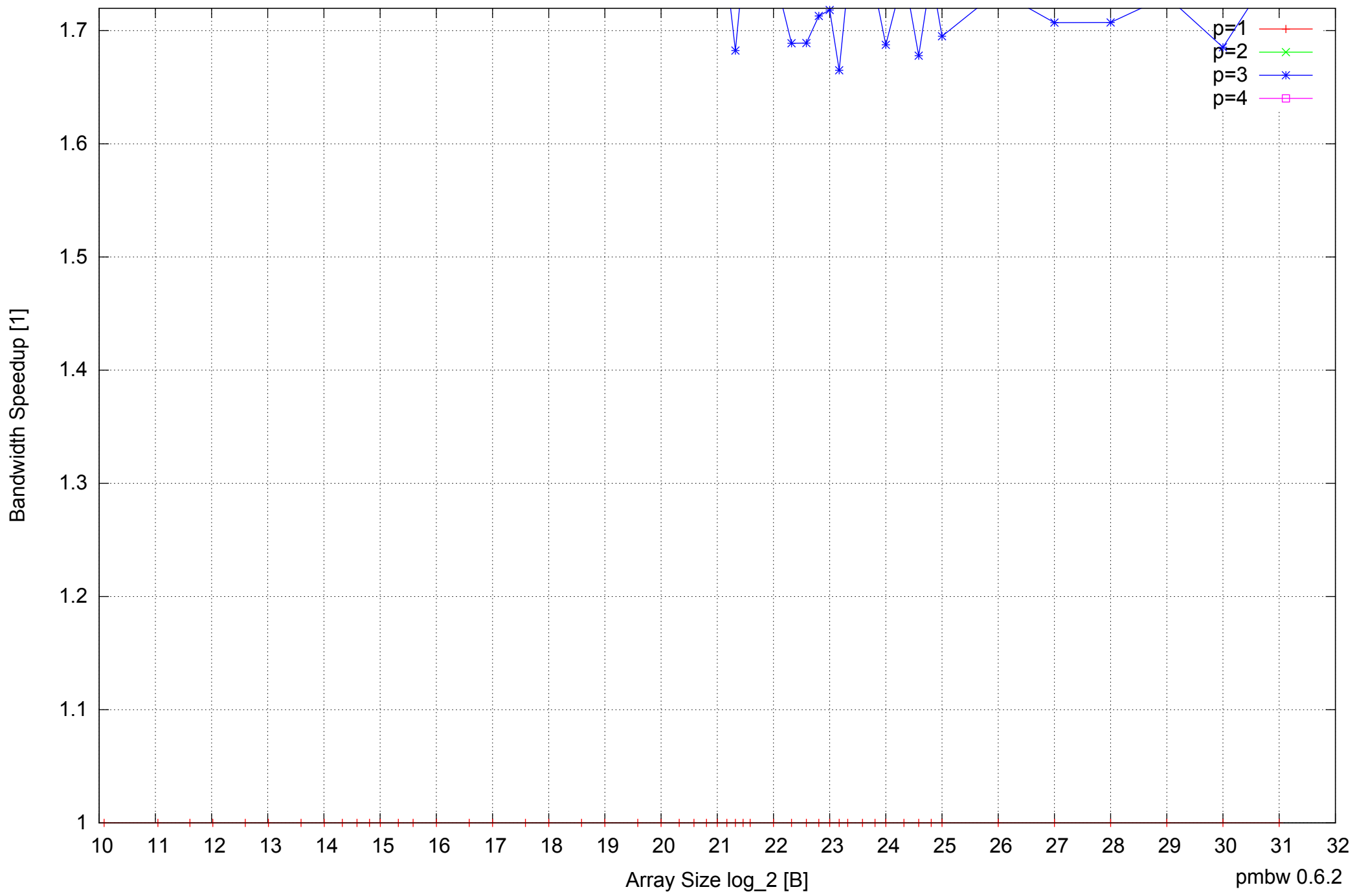
AMD Athlon 64 X2 5600+ 4GB - Speedup of Parallel Memory Bandwidth (enlarged) - ScanRead32PtrSimpleLoop
