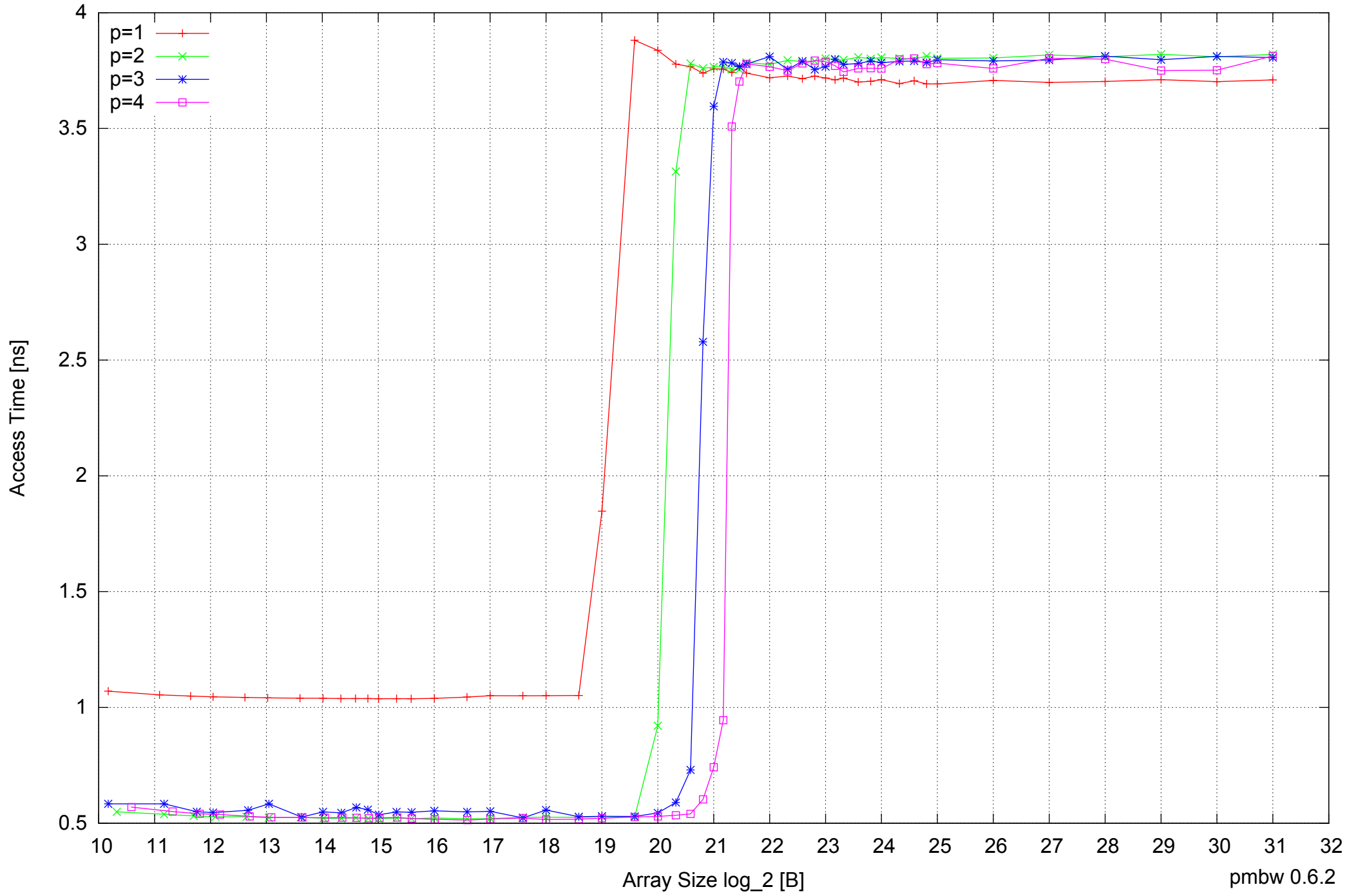
AMD Athlon 64 X2 5600+ 4GB - Parallel Memory Access Time - ScanWrite64IndexSimpleLoop
