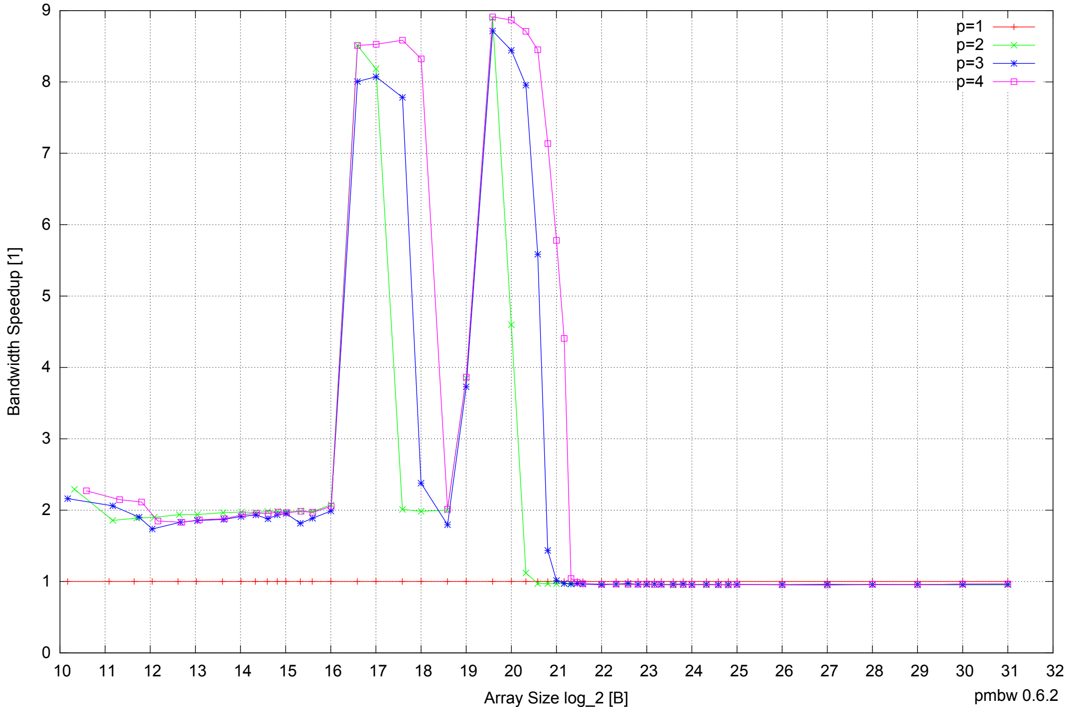
AMD Athlon 64 X2 5600+ 4GB - Speedup of Parallel Memory Bandwidth - ScanWrite64IndexUnrollLoop
