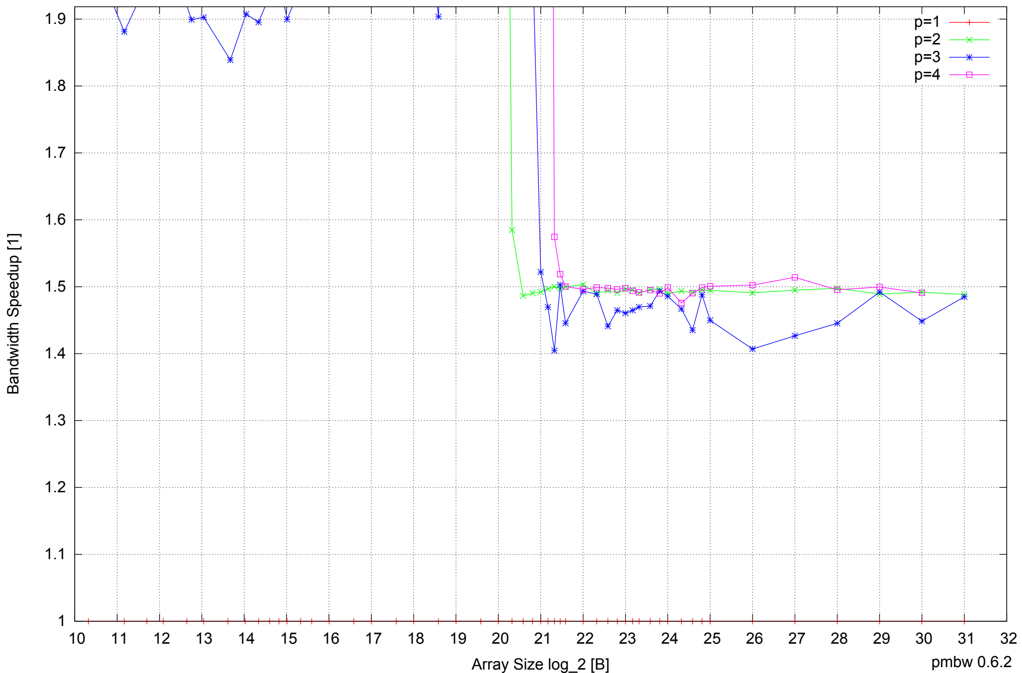
AMD Athlon 64 X2 5600+ 4GB - Speedup of Parallel Memory Bandwidth (enlarged) - ScanRead128PtrUnrollLoop
