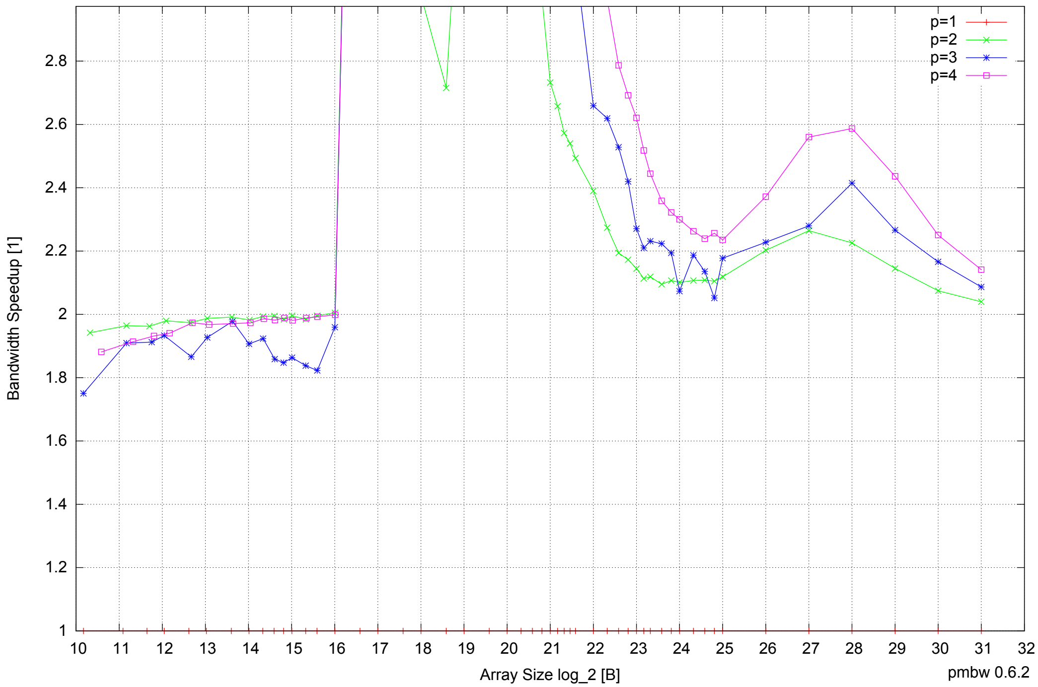
AMD Athlon 64 X2 5600+ 4GB - Speedup of Parallel Memory Bandwidth (enlarged) - PermRead64SimpleLoop
