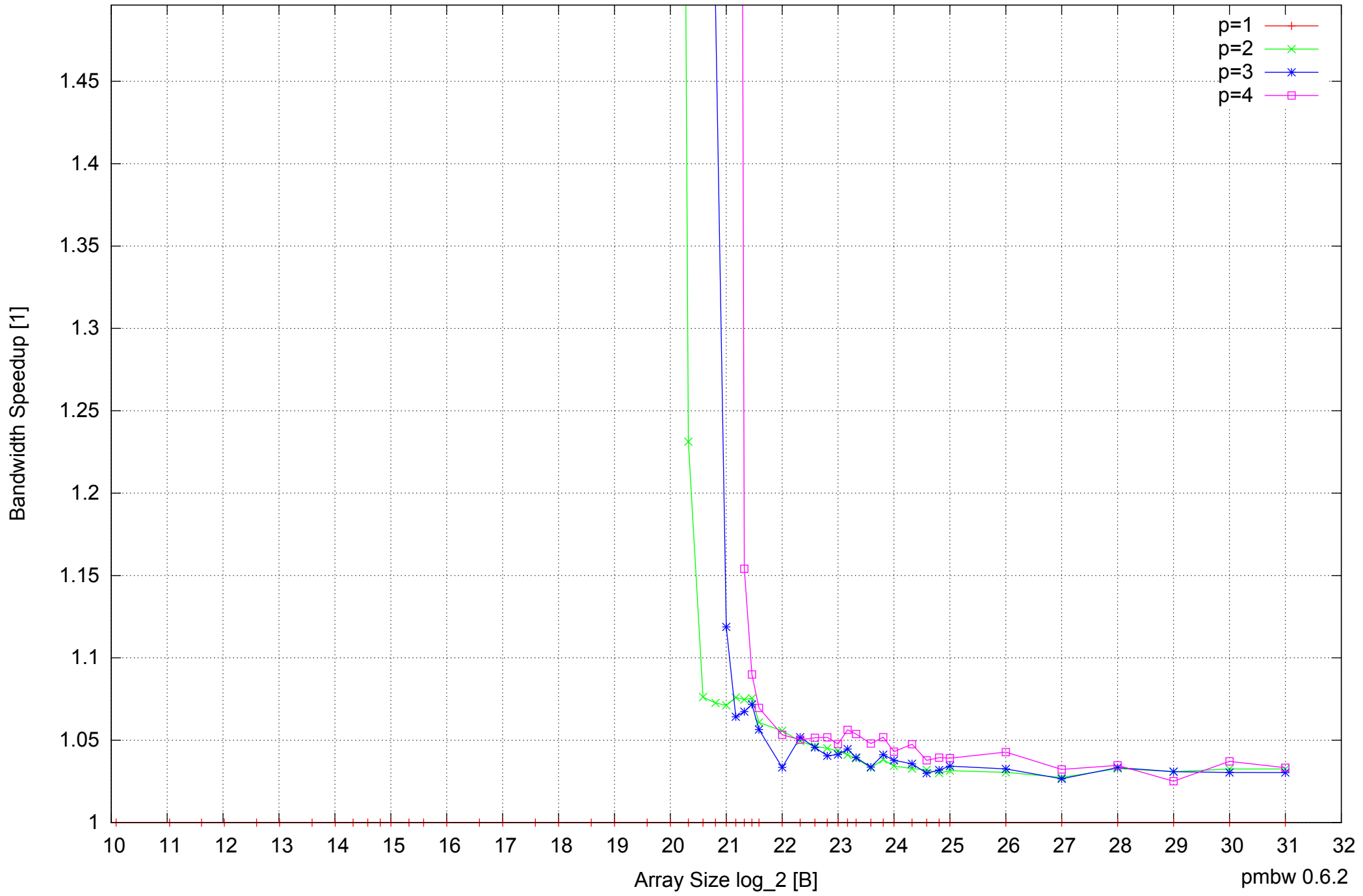
AMD Athlon 64 X2 5600+ 4GB - Speedup of Parallel Memory Bandwidth (enlarged) - ScanWrite32PtrSimpleLoop
