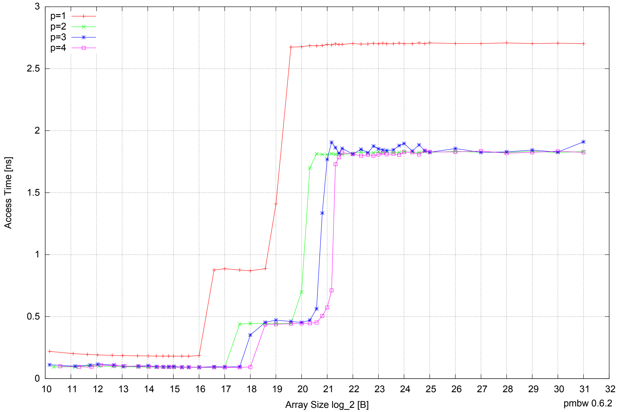
AMD Athlon 64 X2 5600+ 4GB - Parallel Memory Access Time - ScanRead64IndexUnrollLoop
