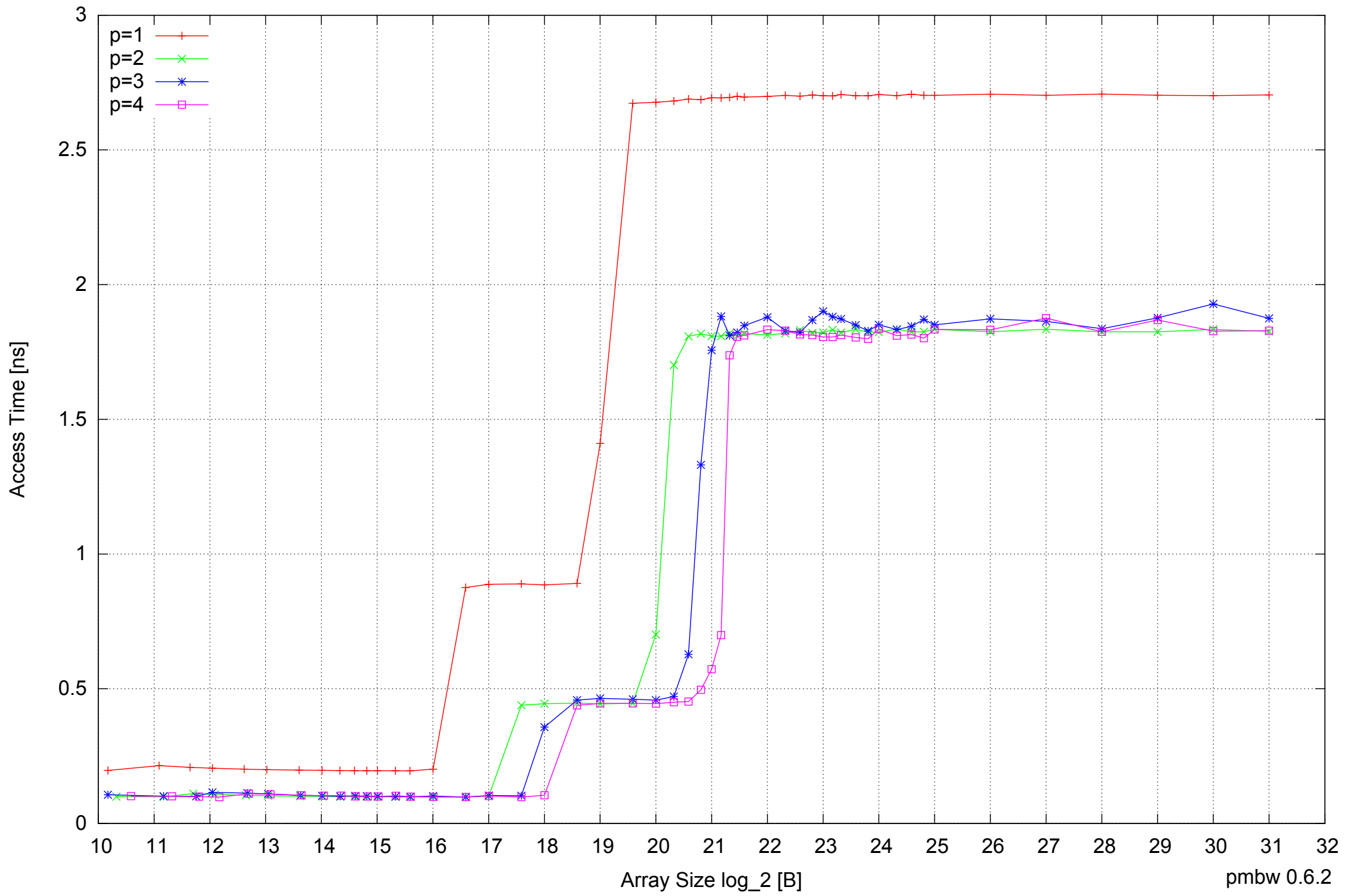
AMD Athlon 64 X2 5600+ 4GB - Parallel Memory Access Time - ScanRead64PtrUnrollLoop
