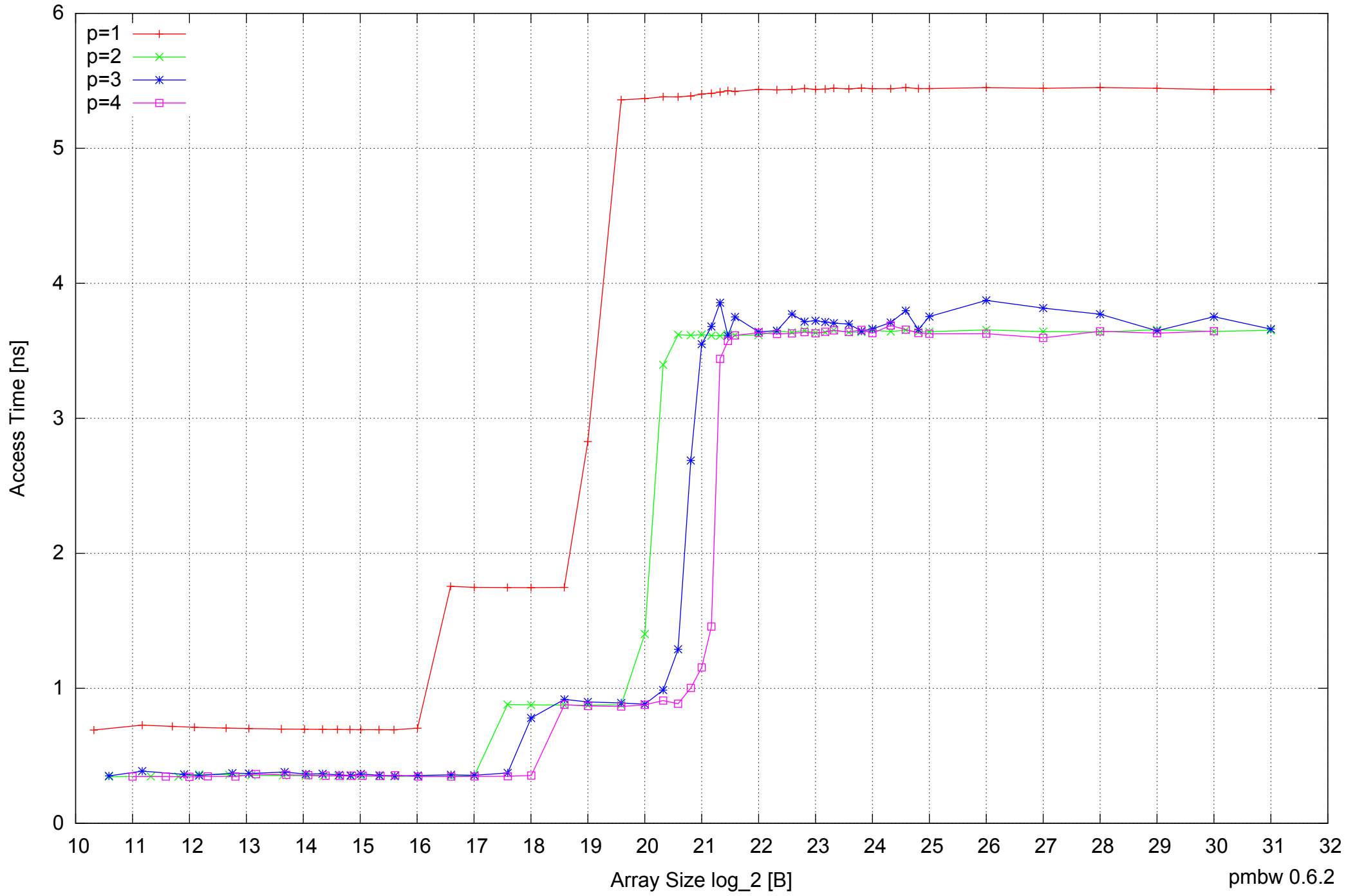
AMD Athlon 64 X2 5600+ 4GB - Parallel Memory Access Time - ScanRead128PtrUnrollLoop
