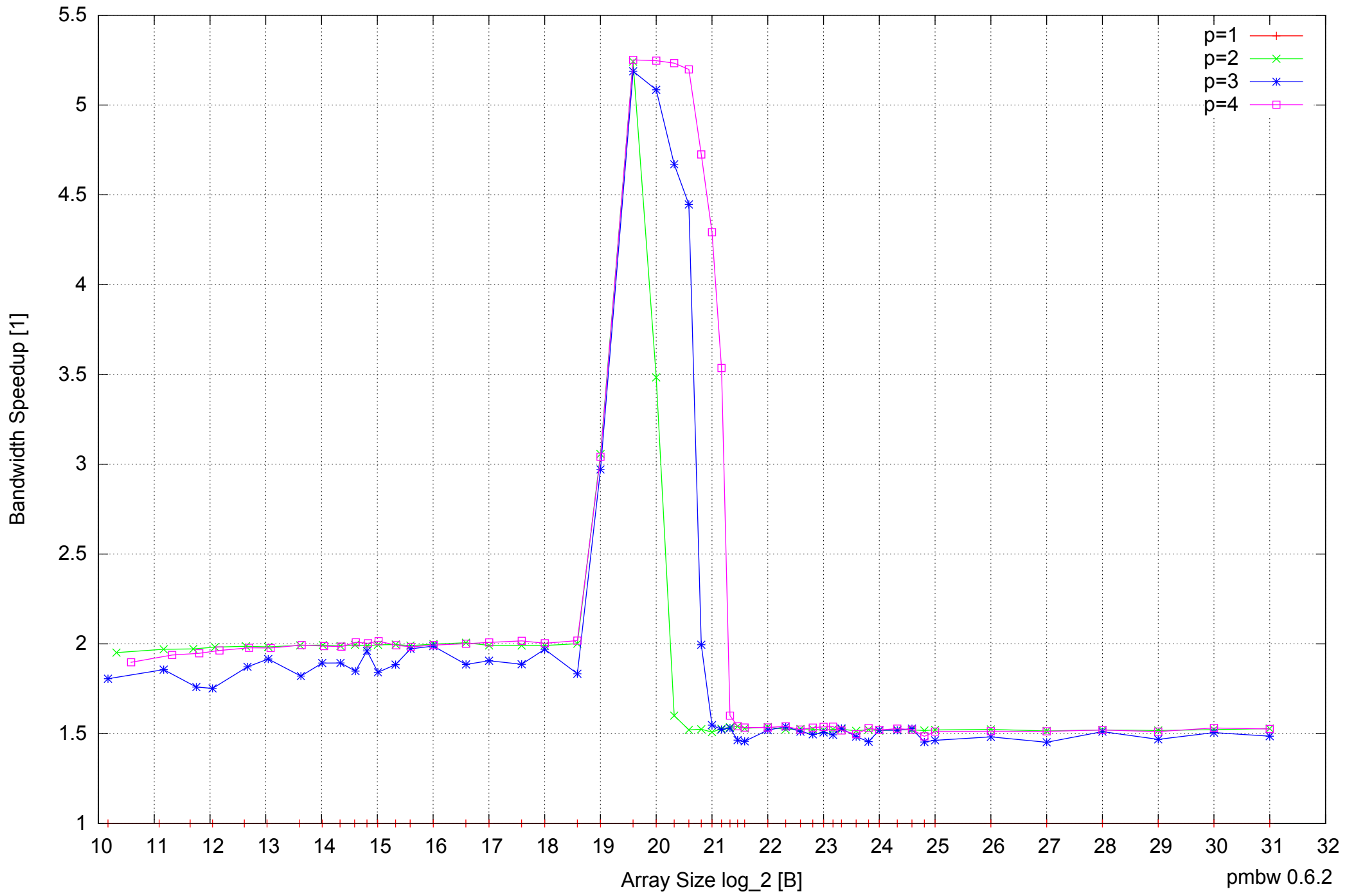
AMD Athlon 64 X2 5600+ 4GB - Speedup of Parallel Memory Bandwidth - ScanRead64PtrSimpleLoop
