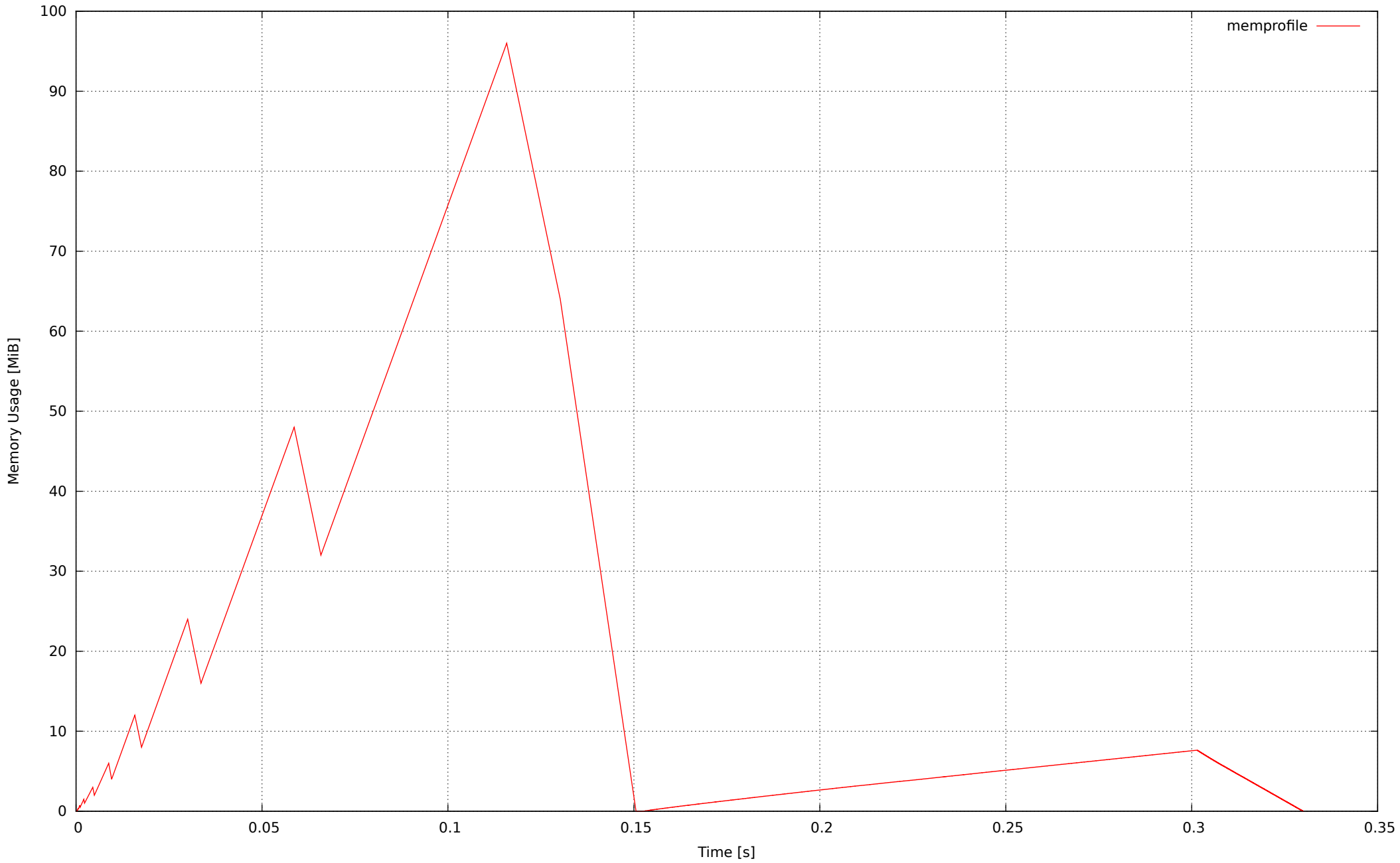
Memory Profile of Test Program
