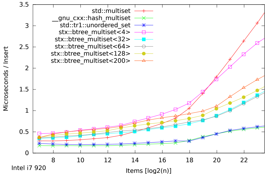
Speed Test Multimap - Normalized Time - Insert/Find/Erace (125-65536000 Items)
