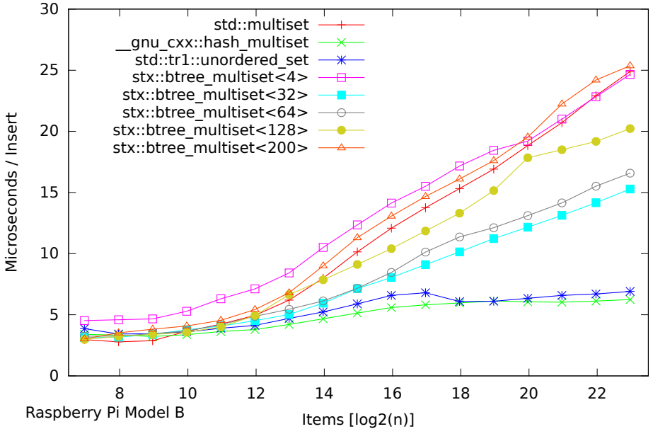
Speed Test Multimap - Normalized Time - Insert/Find/Eraser (125-8192000 Items)
