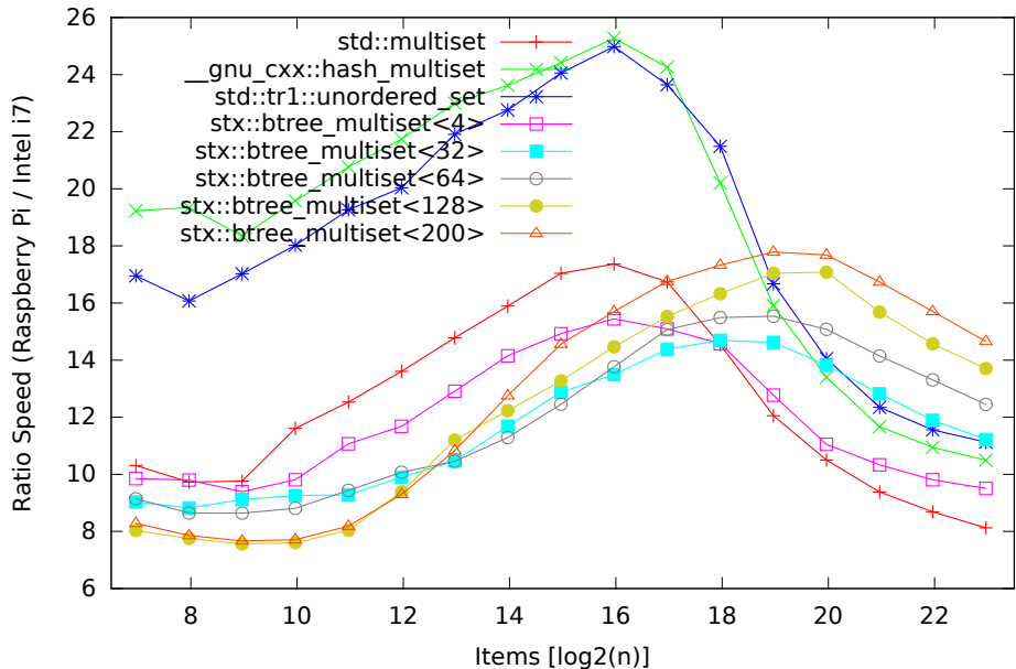
Speed Test Multimap - Ratio - Insert/Find/Erase (125-8192000 Items)
