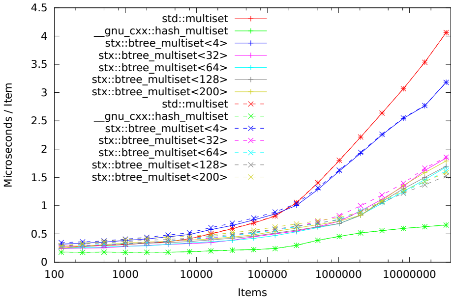
Speed Test Multiset - Normalized Time - Insert/Find/Erased (125-32768000 Items)
