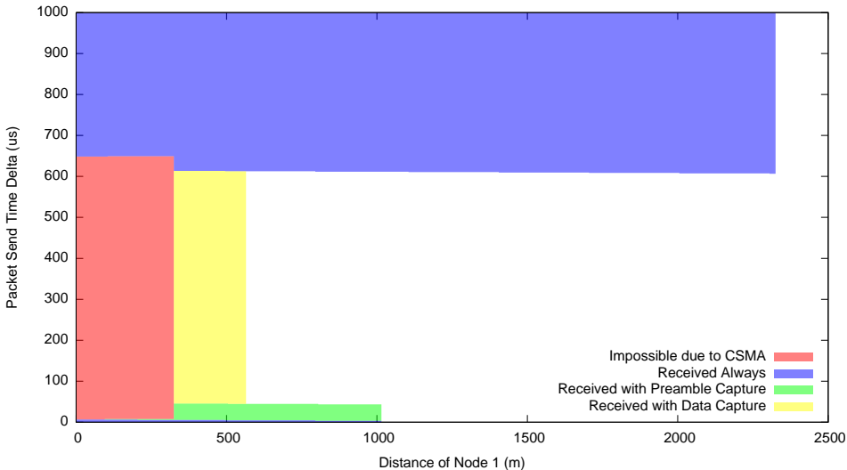
Three Wireless Nodes - Reception on Node 0 of Packets from Node 1 (Moving Nearer Sender)
