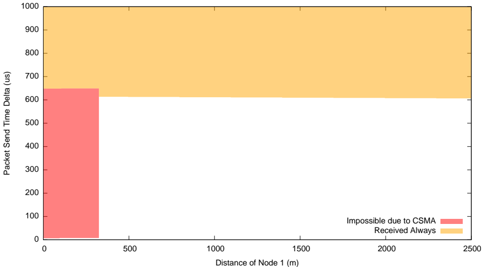
Three Wireless Nodes - Reception on Node 0 of Packets from Node 2 (Non-moving Interferer)
