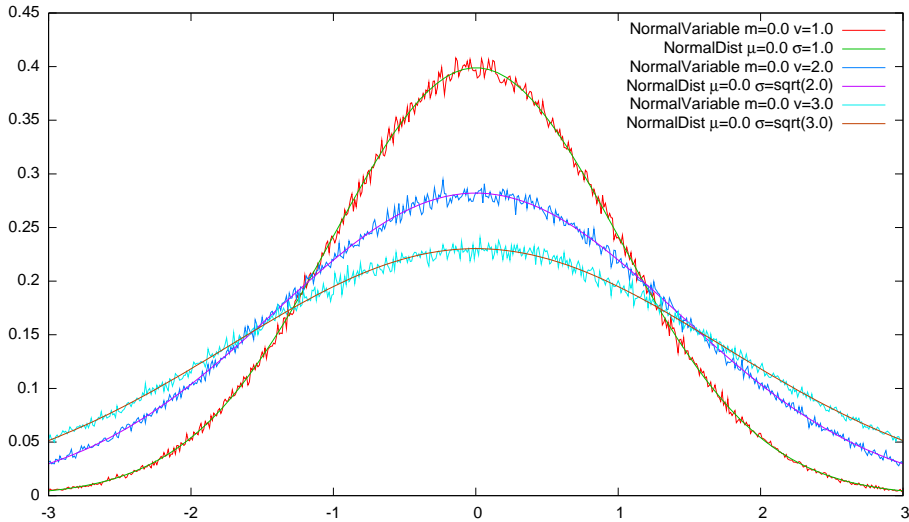
NormalVariable
