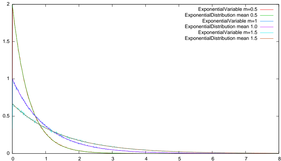
ExponentialVariable
