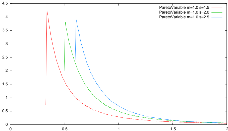
ParetoVariable
