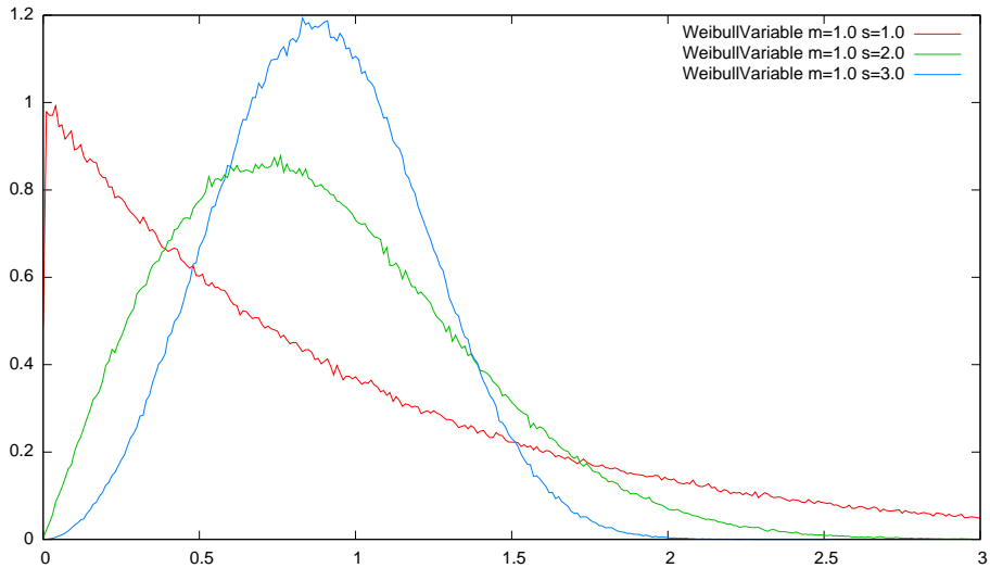
WeibullVariable
