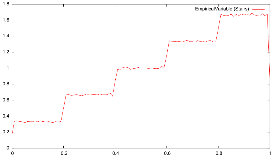
EmpiricalVariable
