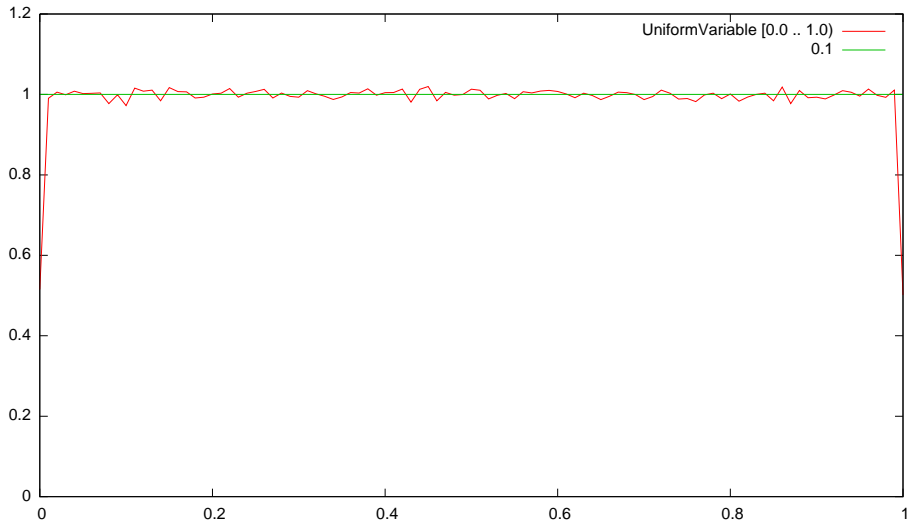
UniformVariable
