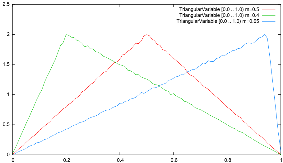
TriangularVariable
