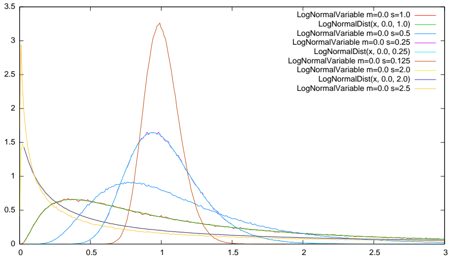
LogNormalVariable
