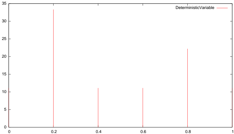
DeterministicVariable
