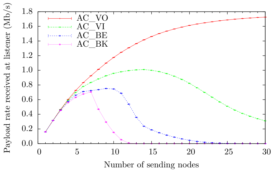
(b) UnACKed broadcast with EDCA parameters in 802.11p/D4.02
