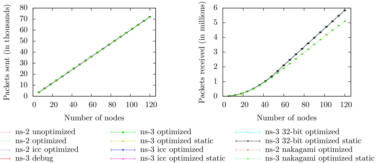
Figure 8.2: Total packets sent and received during simulation
