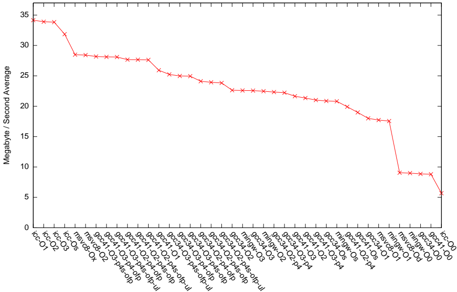
Compiler Flags Comparison
