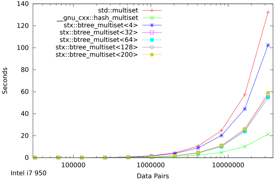
Speed Test Multiset - Insert/Find/Erace (32000-32768000 Items)
