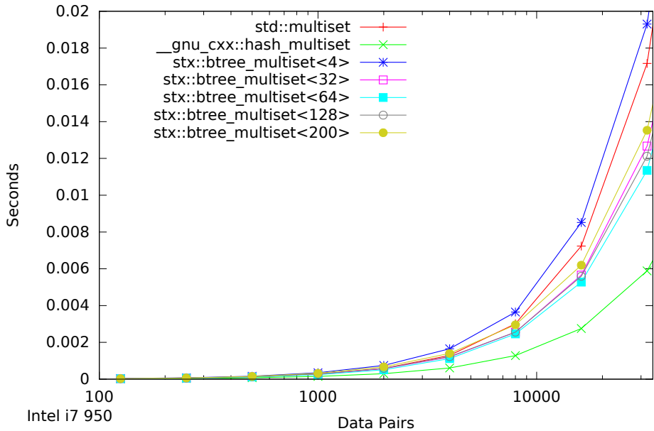
Speed Test Multiset - Insert/Find/Erace (125-32000 Items)
