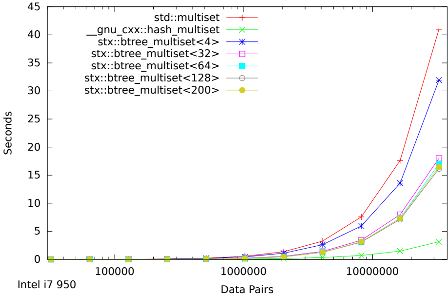
Speed Test Multiset - Find Only (32000-32768000 Items)
