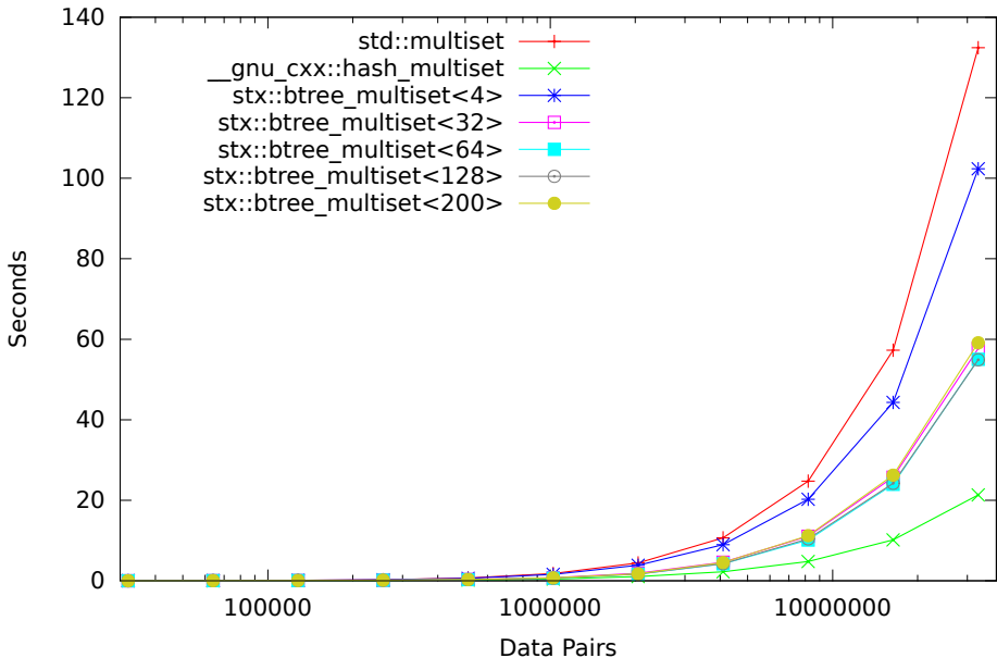
Speed Test Multiset - Insert/Find/Erace (32000-32768000 Items)
