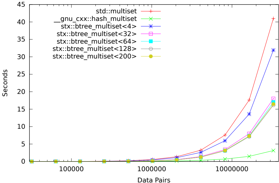
Speed Test Multiset - Find Only (32000-32768000 Items)
