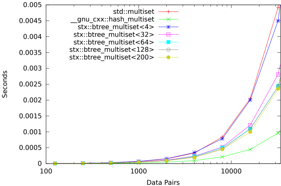
Speed Test Multiset - Find Only (125-32000 Items)
