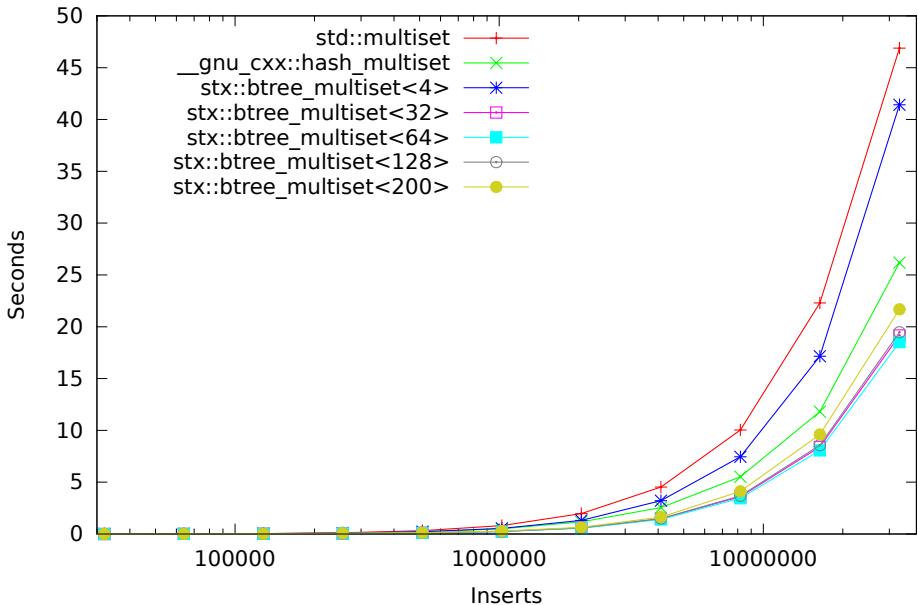
Speed Test Multiset - Absolute Time - Insertion Only (32000-32768000 Items)
