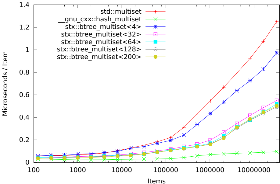
Speed Test Multiset - Normalized Time - Find Only (125-32768000 Items)
