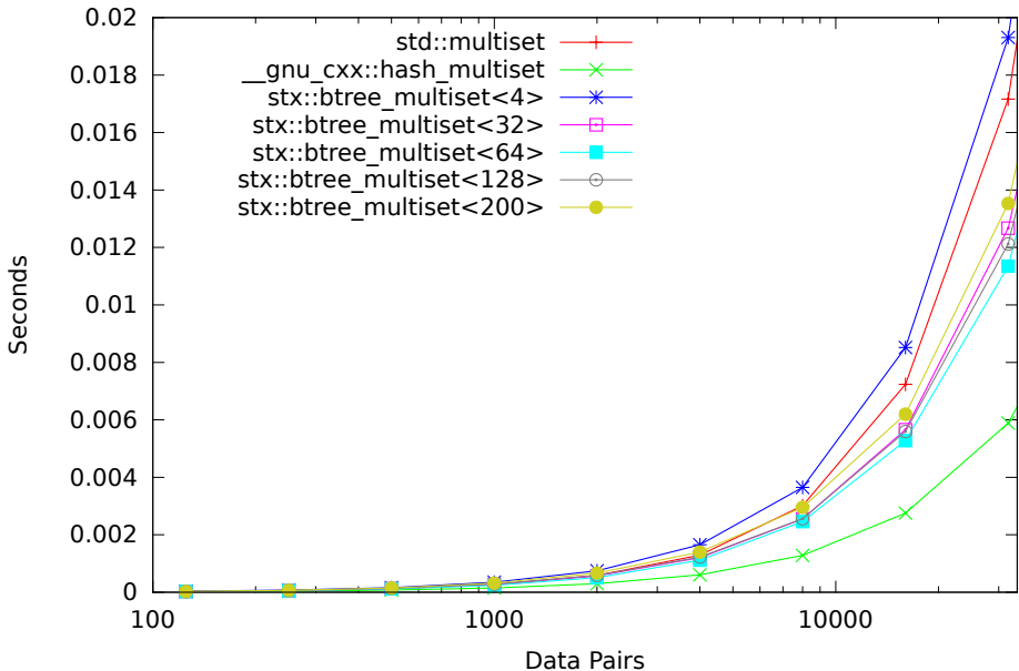
Speed Test Multiset - Insert/Find/Eraser (125-32000 Items)
