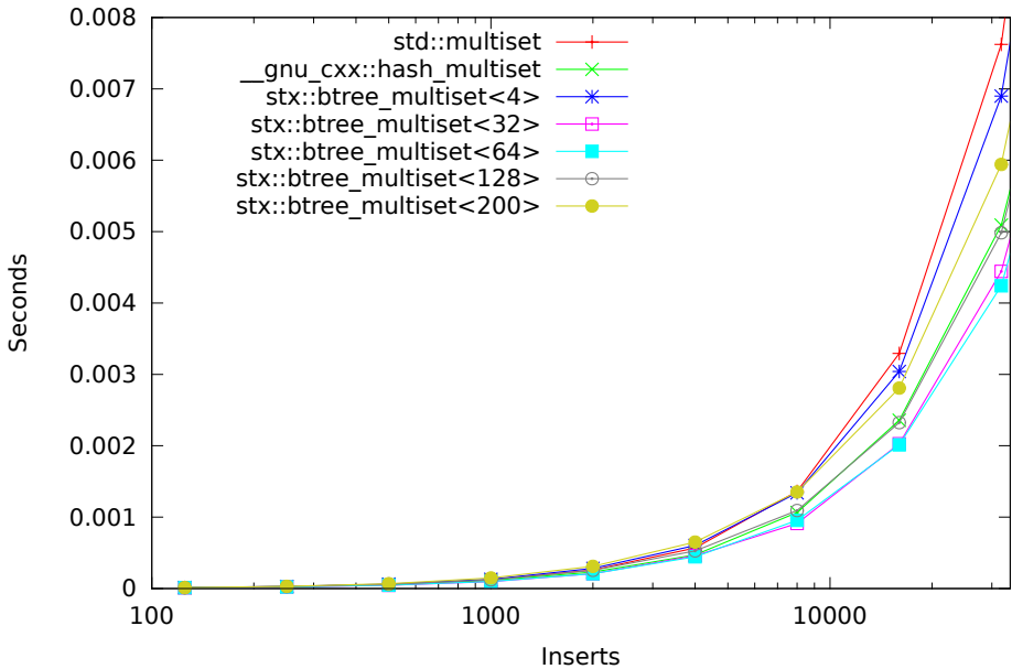
Speed Test Multiset - Absolute Time - Insertion Only (125-32000 Items)
