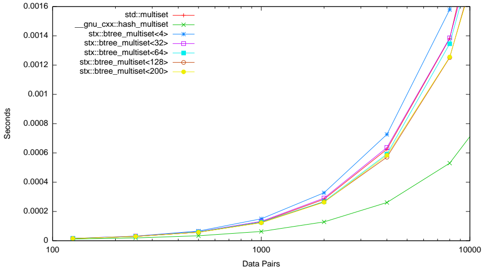
Speed Test Multiset - Find Only (125-8000 Items)
