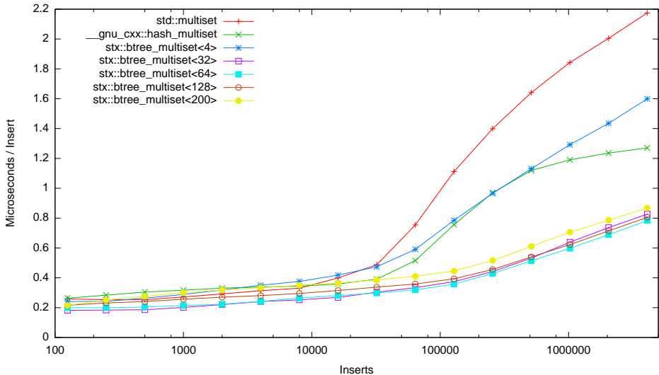
Speed Test Multipart - Normalized Time - Insertion Only (125-4096000 Items)
