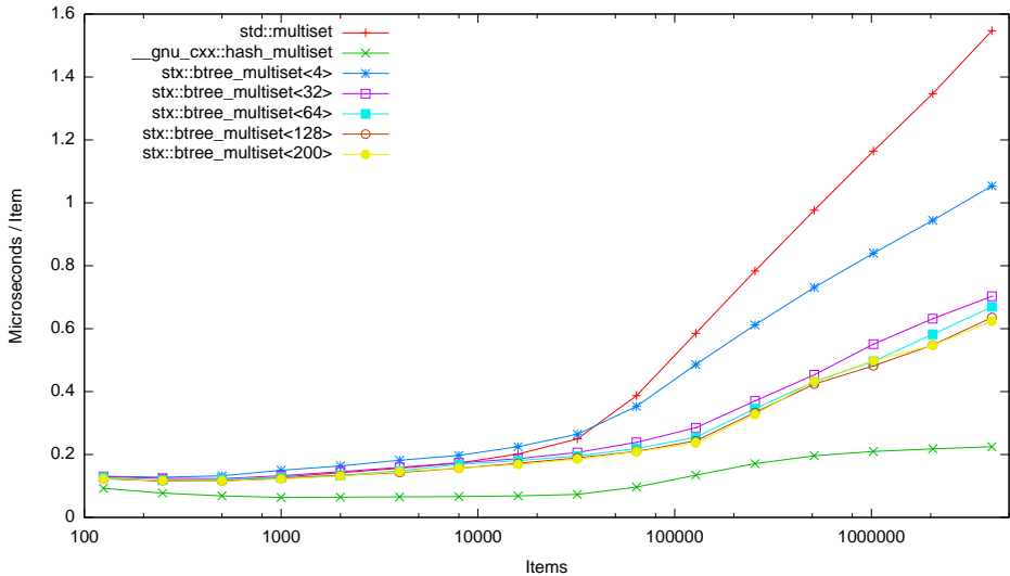
Speed Test Multiset - Normalized Time - Find Only (125-4096000 Items)
