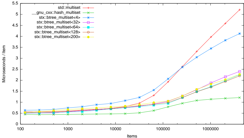
Speed Test Multiset - Normalized Time - Insert/Find/Erased (125-4096000 Items)
