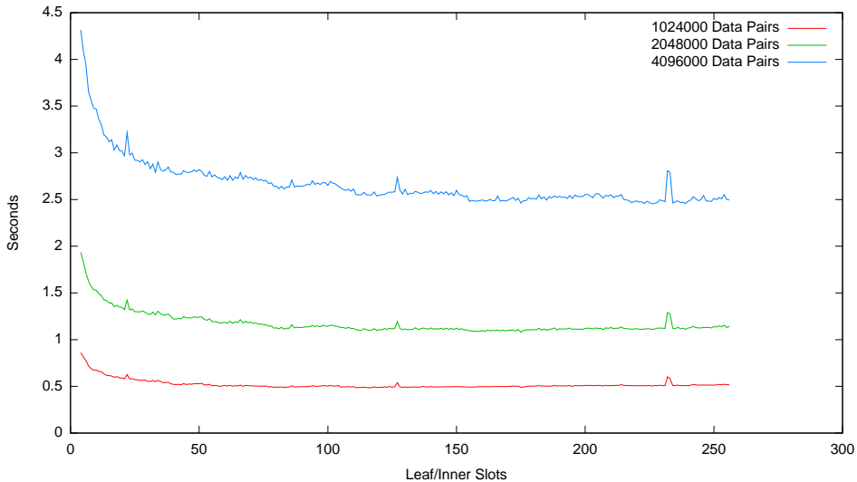
Speed Test - Finding the Best Slot Size - Find Only - Plotted by Leaf/Inner Slots in B+ Tree
