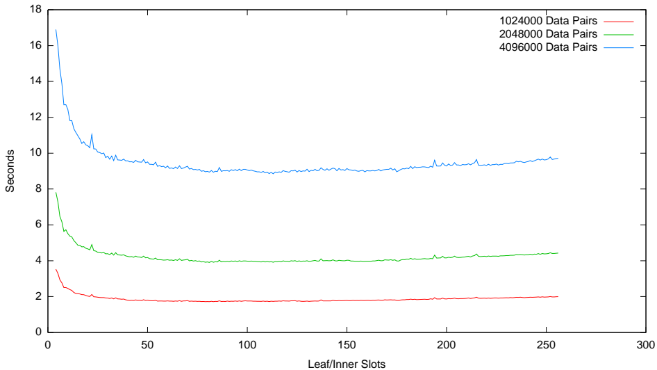
Speed Test - Finding the Best Slot Size - Insert/Find/Erace - Plotted by Leaf/Inner Slots in B+ Tree
