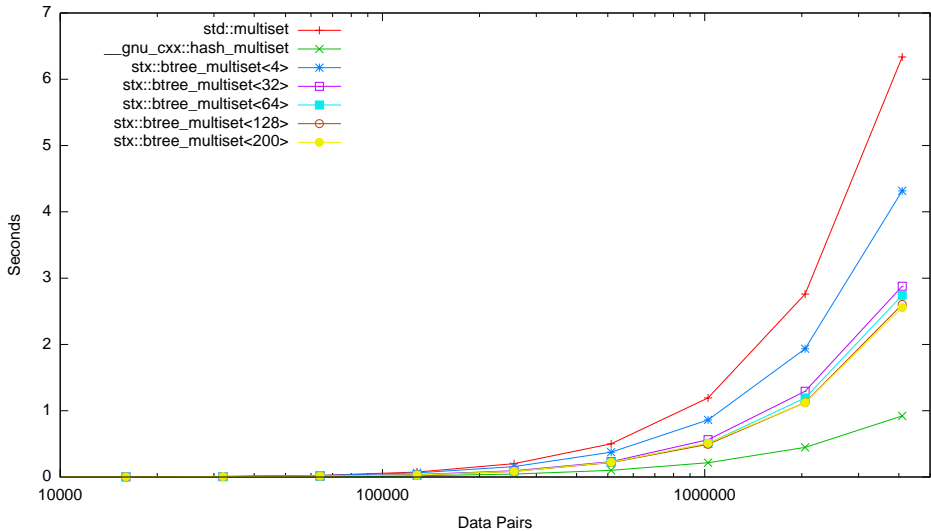
Speed Test Multiset - Find Only (16000-4096000 Items)
