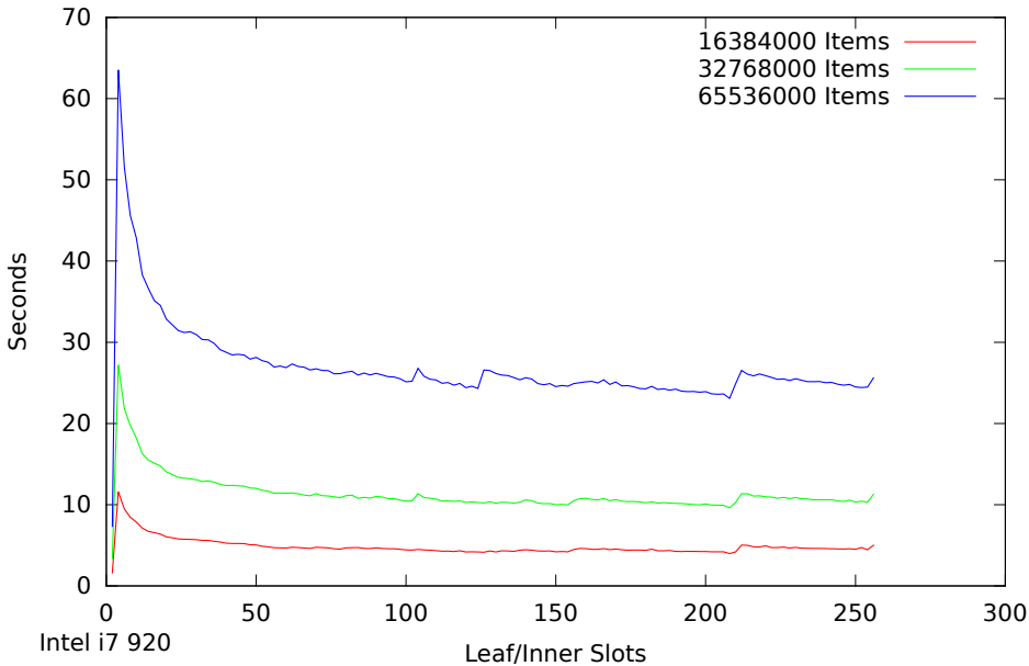
Speed Test - Finding the Best Slot Size - Find Only - Plotted by Slots in B+ Tree
