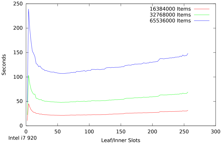
Speed Test - Finding the Best Slot Size - Insert/Find/Eraser - Plotted by Slots in B+ Tree
