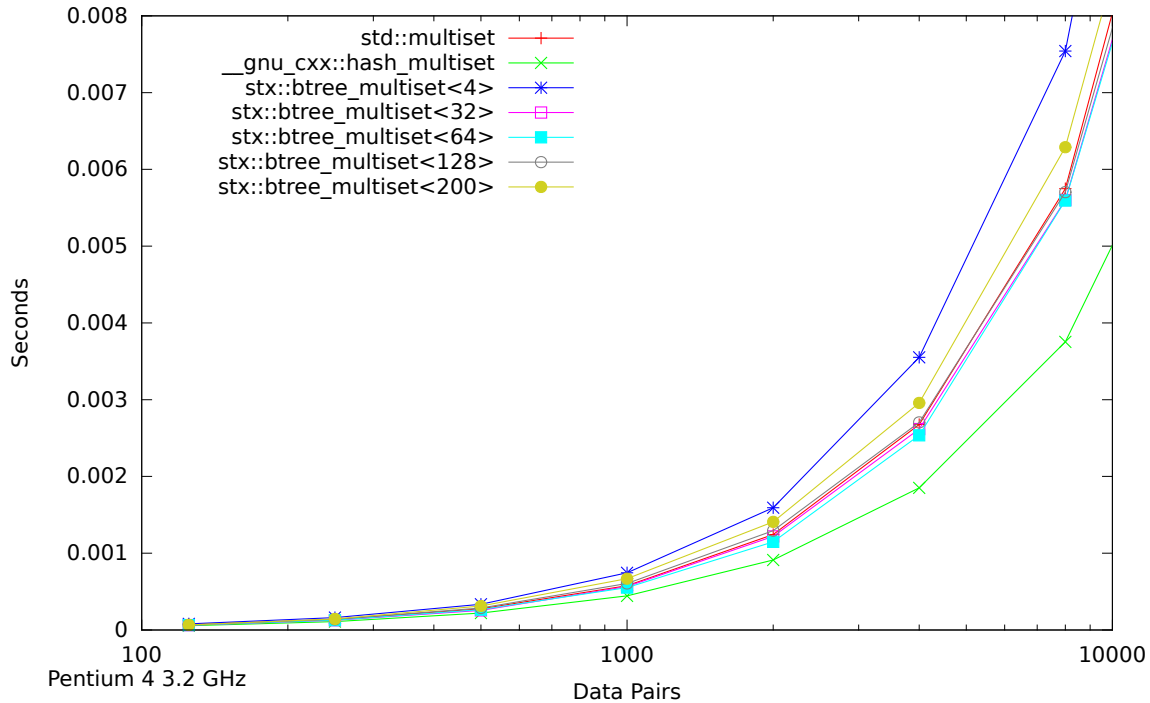
Speed Test Multiset - Insert/Find/Erace (125-8000 Items)
