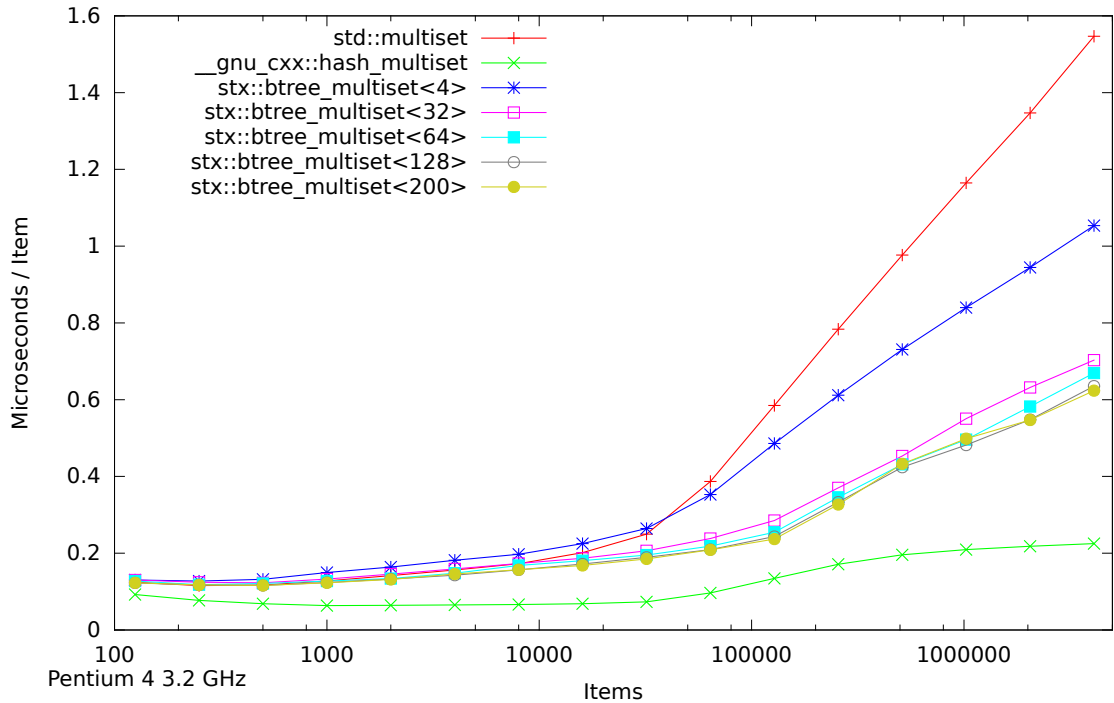
Speed Test Multiset - Normalized Time - Find Only (125-4096000 Items)
