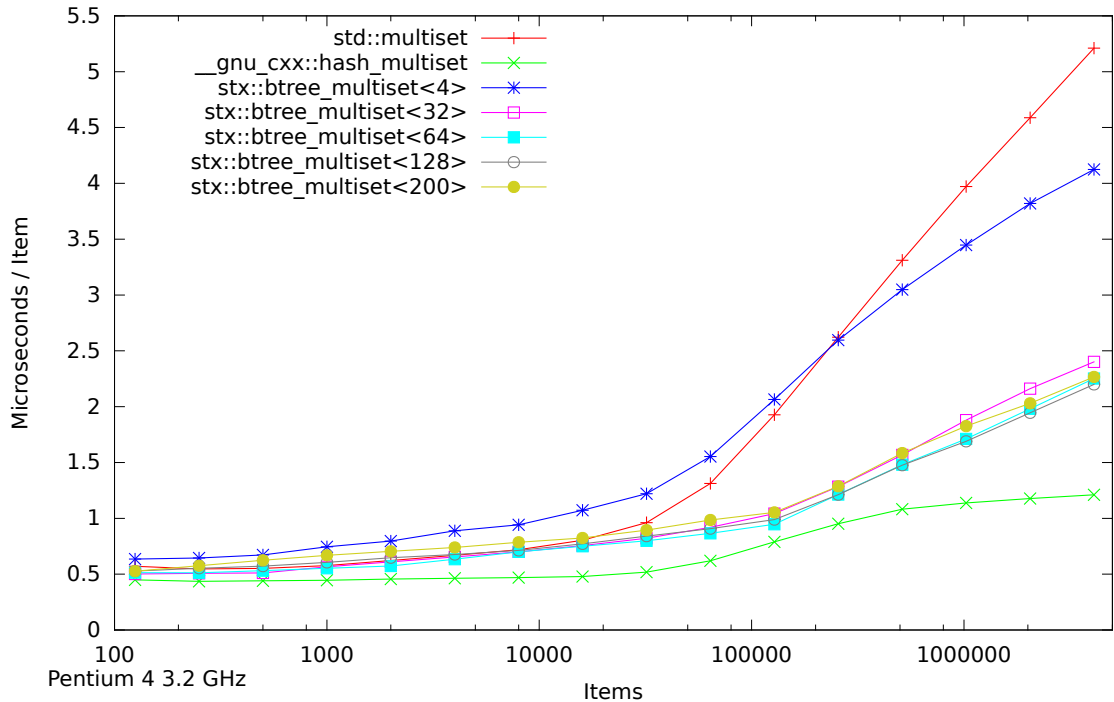
Speed Test Multiset - Normalized Time - Insert/Find/Erse (125-4096000 Items)
