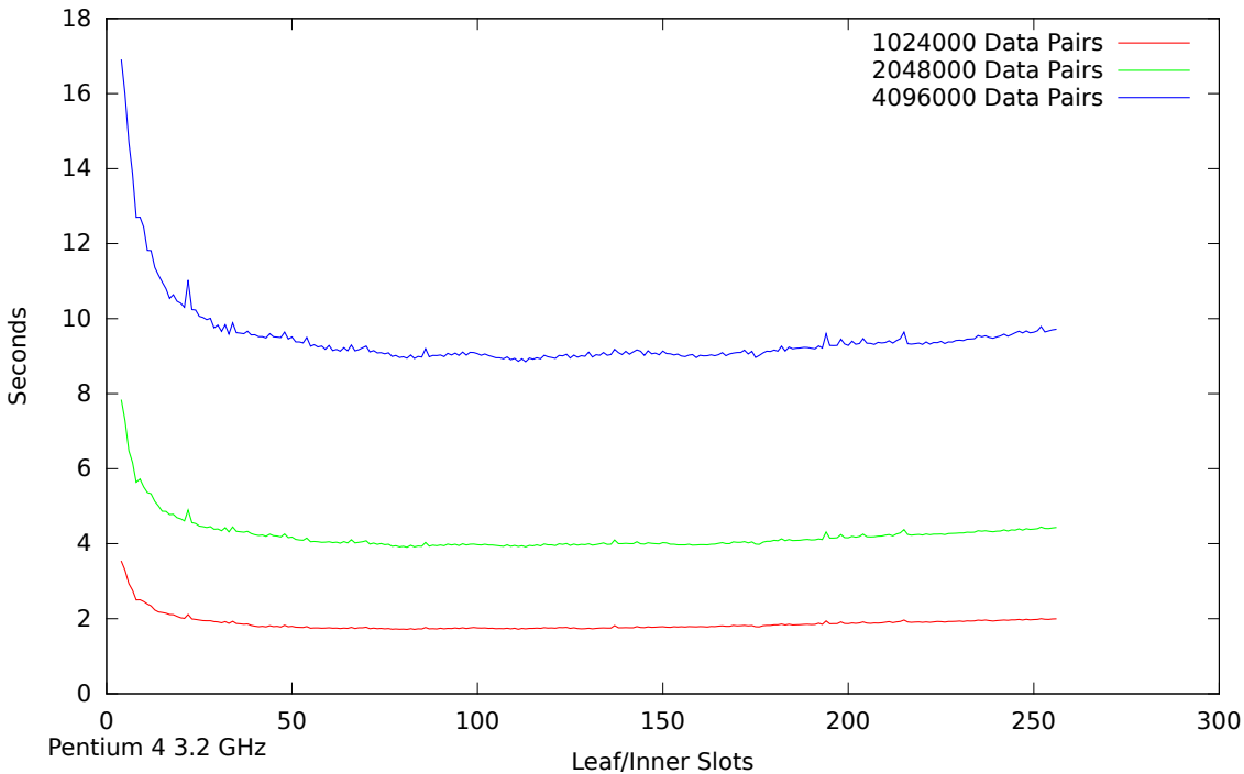
Speed Test - Finding the Best Slot Size - Insert/Find/Erased - Plotted by Leaf/Inner Slots in B+ Tree
