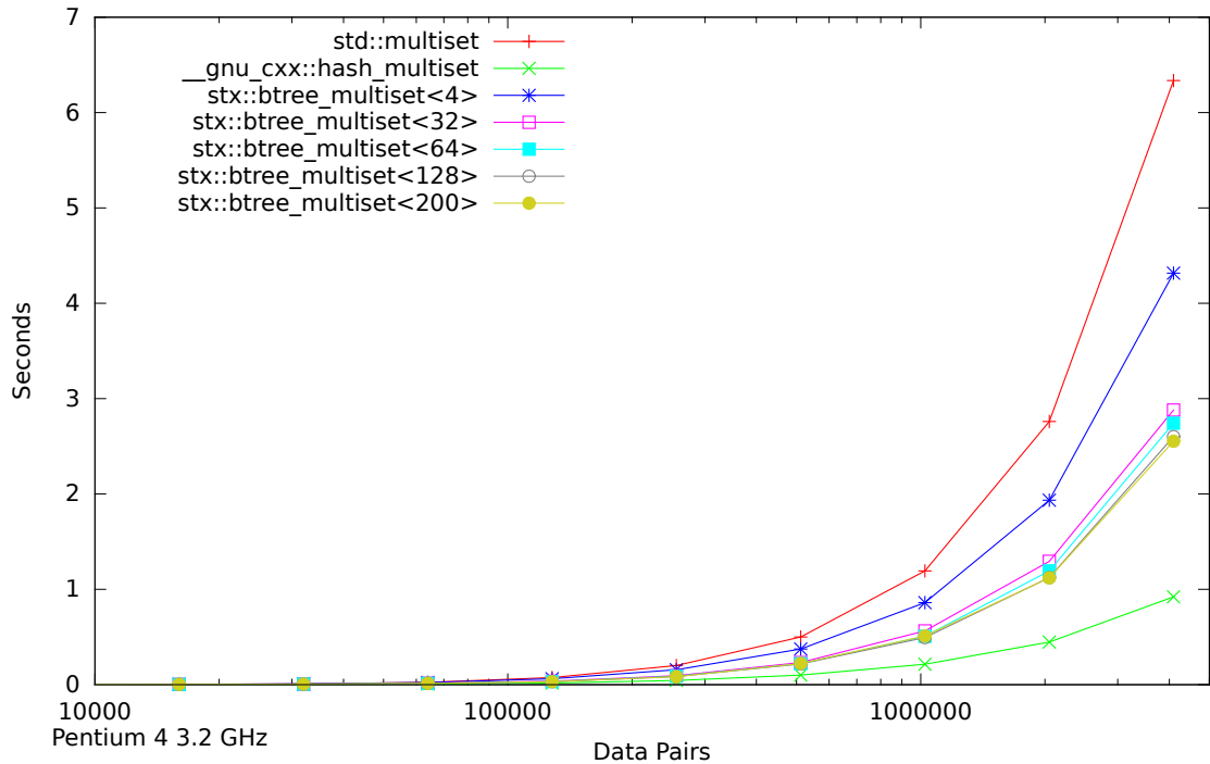
Speed Test Multiset - Find Only (16000-4096000 Items)
