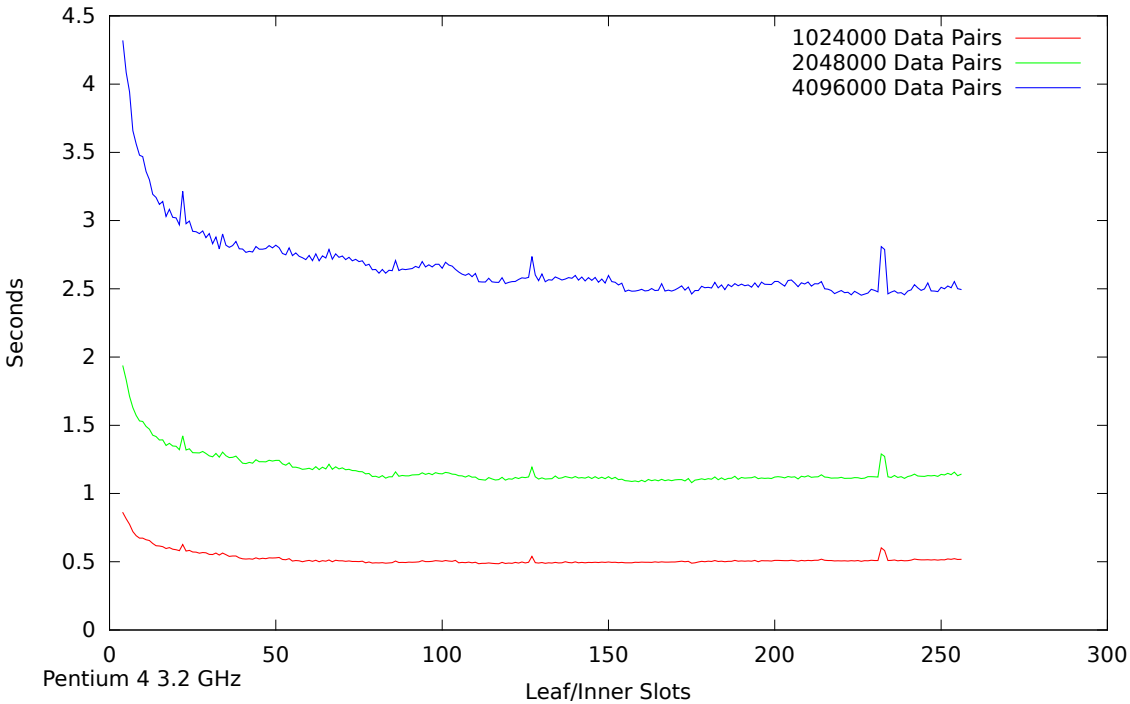
Speed Test - Finding the Best Slot Size - Find Only - Plotted by Leaf/Inner Slots in B+ Tree
