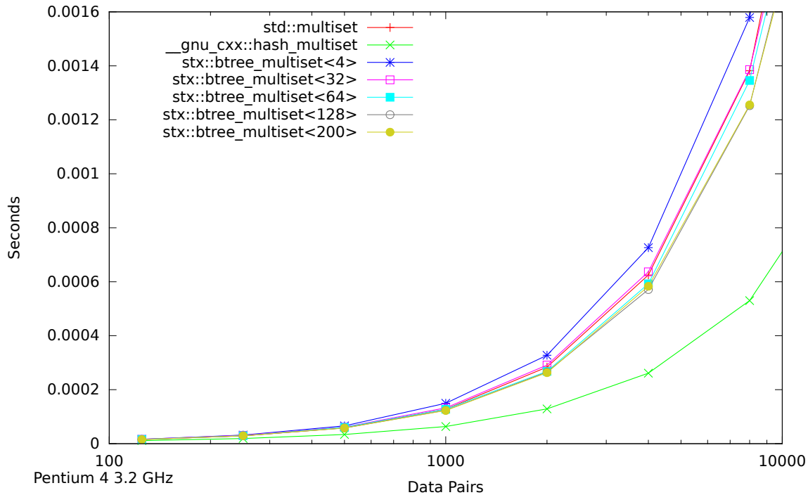
Speed Test Multiset - Find Only (125-8000 Items)
